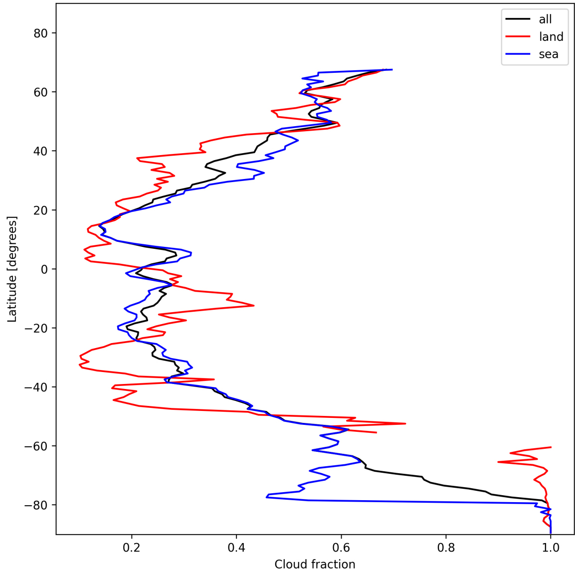
Figure 15: Zonal average of “Cloud fraction” for 2025-01-15 to 2025-01-17.
