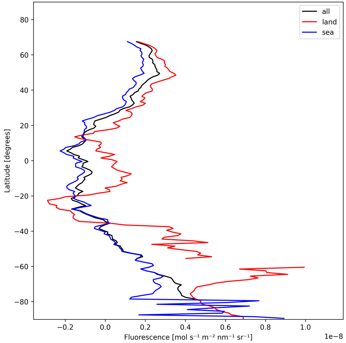
Figure 23: Zonal average of “Fluorescence” for 2025-01-15 to 2025-01-17.
