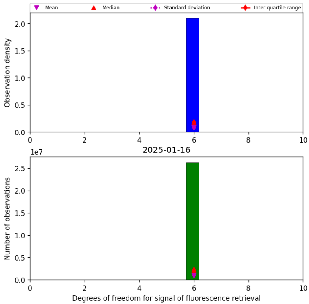
Figure 43: Histogram of "Degrees of freedom for signal of fluorescence retrieval" for 2025-01-15 to 2025-01-17
