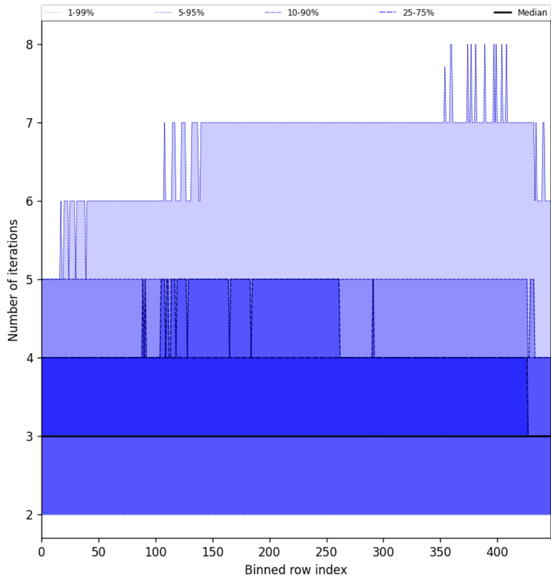
Figure 56: Along track statistics of “Number of iterations” for 2025-01-15 to 2025-01-17
