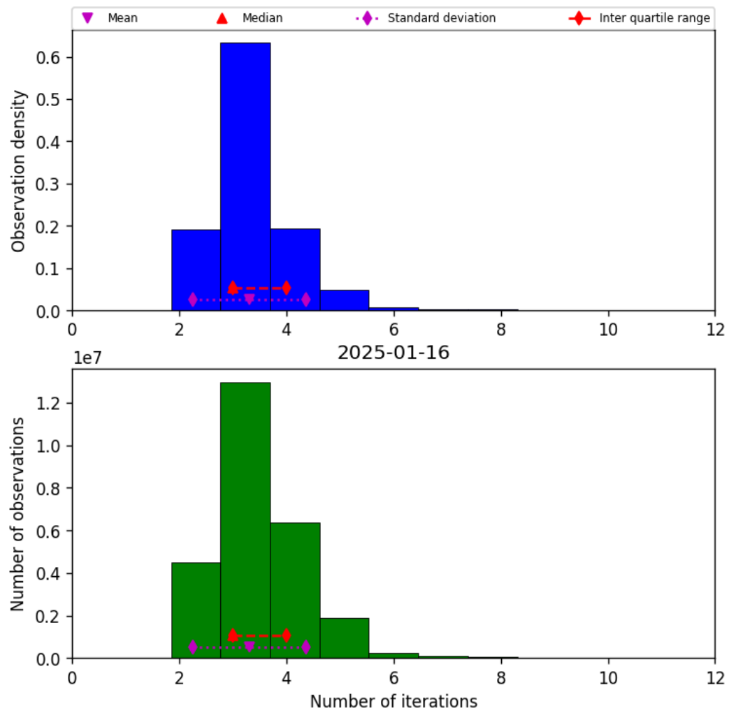
Figure 39: Histogram of “Number of iterations” for 2025-01-15 to 2025-01-17
