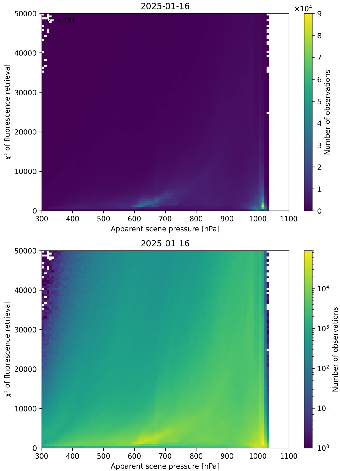
Figure 63: Scatter density plot of “Apparent scene pressure” against “ \chi^2 of fluorescence retrieval” for 2025-01-15 to 2025-01-17.
