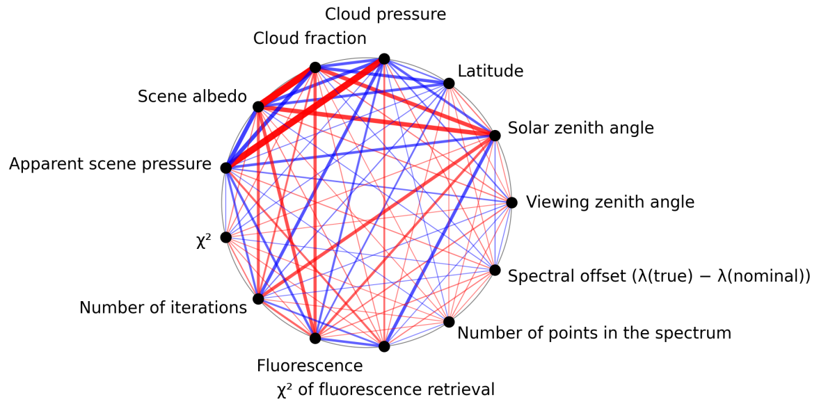
Figure 1: Map of correlation graph for 2025-01-15 to 2025-01-17.
