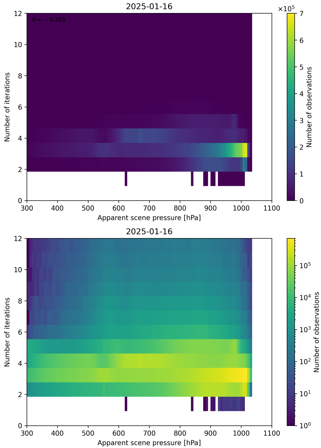
Figure 65: Scatter density plot of “Apparent scene pressure” against “Number of iterations” for 2025-01-15 to 2025-01-17.
