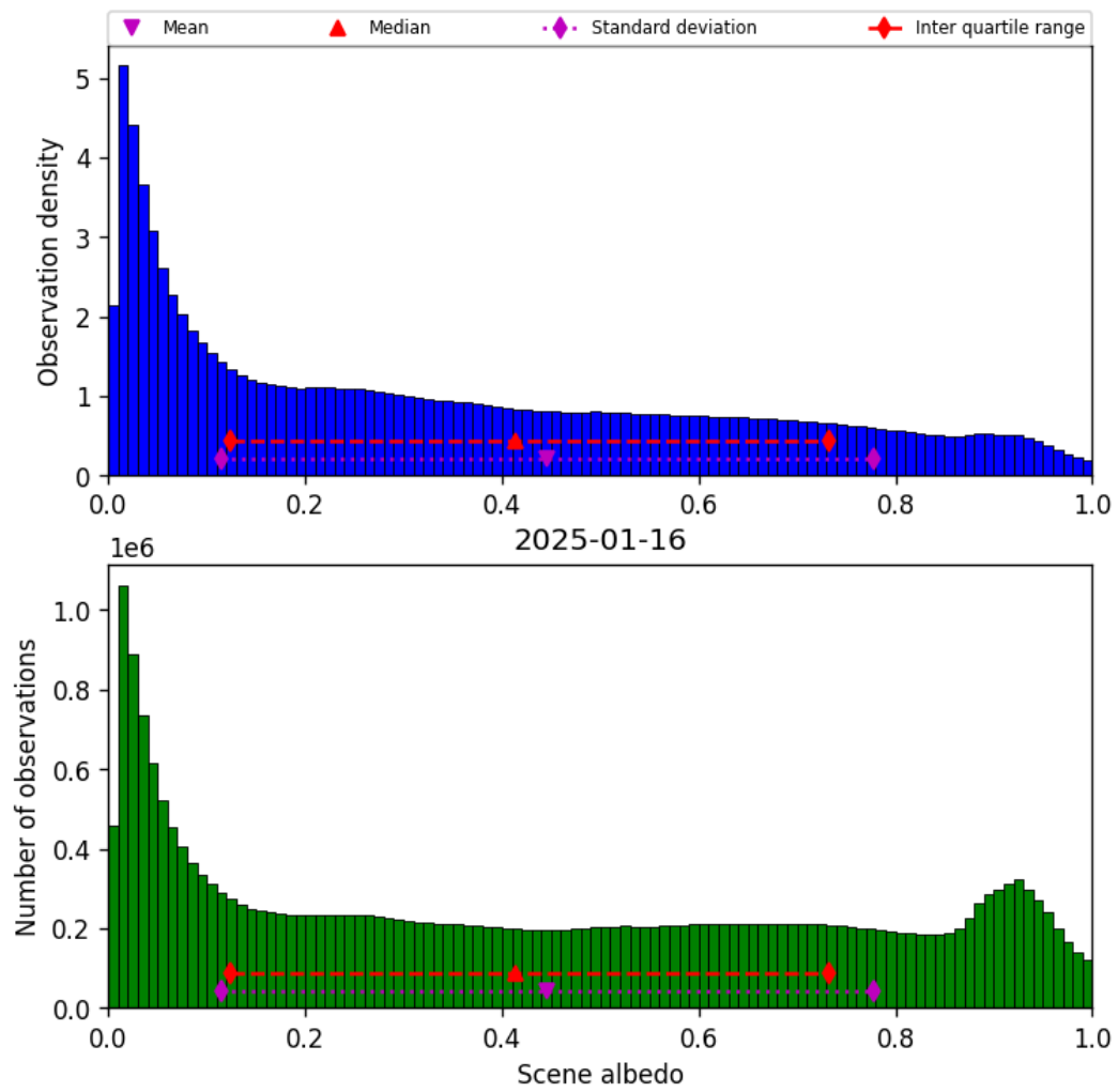
Figure 34: Histogram of “Scene albedo” for 2025-01-15 to 2025-01-17
