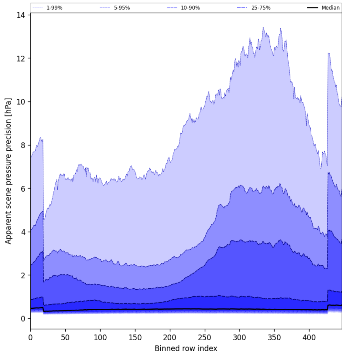
Figure 54: Along track statistics of “Apparent scene pressure precision” for 2025-01-15 to 2025-01-17
