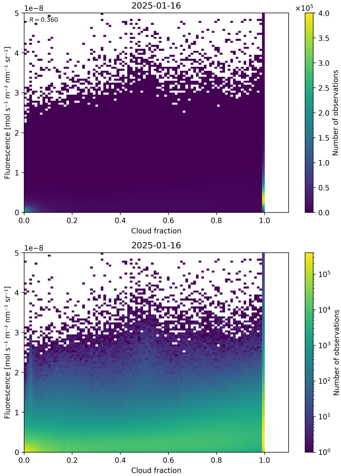
Figure 72: Scatter density plot of “Cloud fraction” against “Fluorescence” for 2025-01-15 to 2025-01-17.
