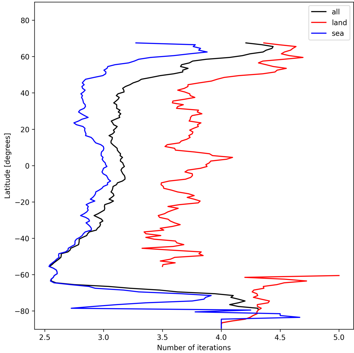
Figure 22: Zonal average of “Number of iterations” for 2025-01-15 to 2025-01-17.
