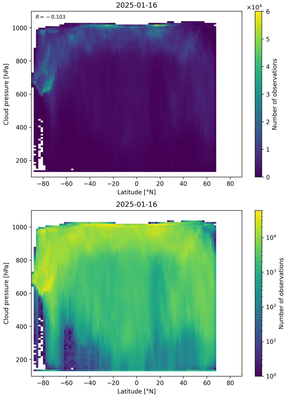
Figure 91: Scatter density plot of “Latitude” against “Cloud pressure” for 2025-01-15 to 2025-01-17.
