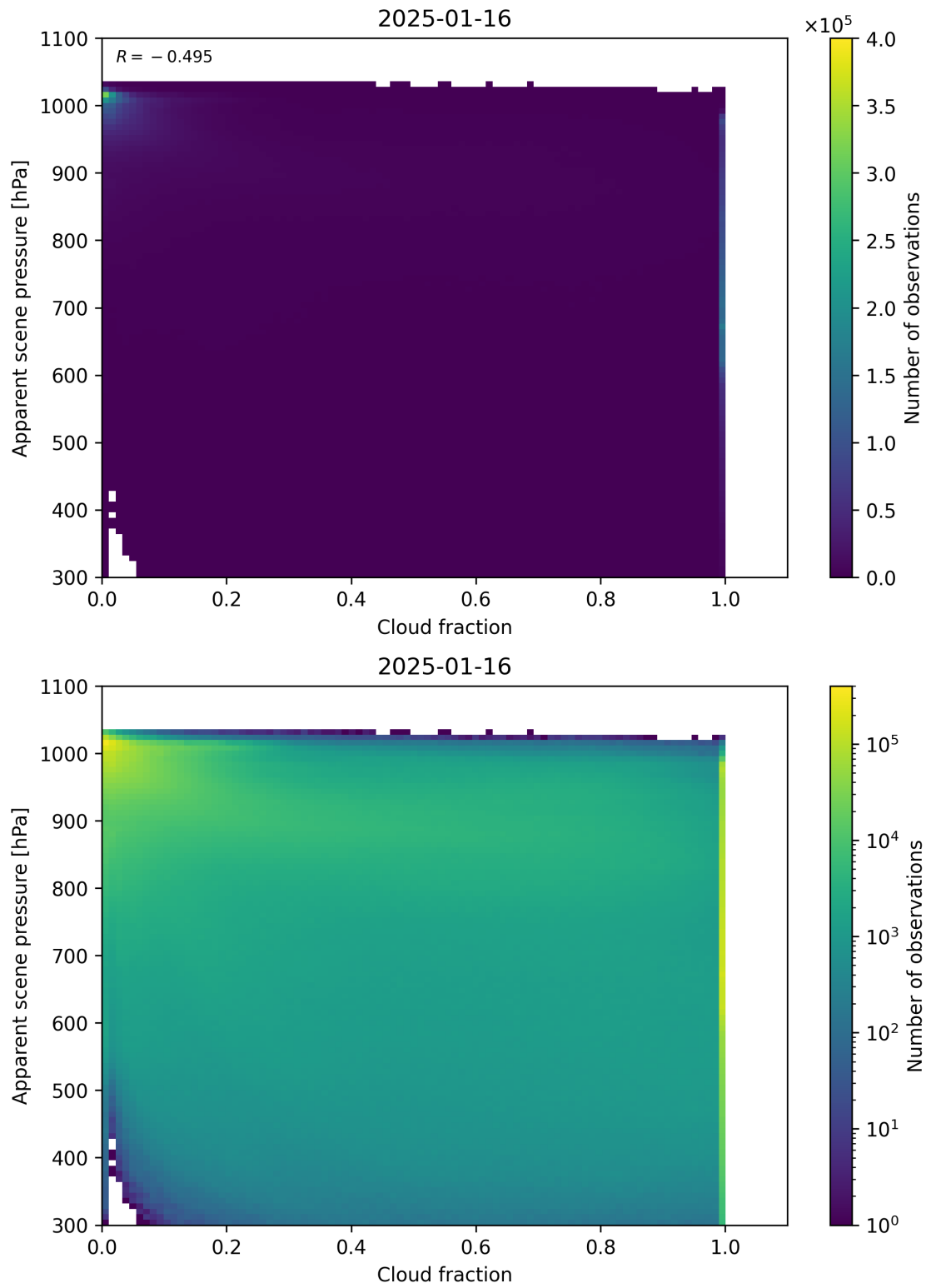
Figure 70: Scatter density plot of “Cloud fraction” against “Apparent scene pressure” for 2025-01-15 to 2025-01-17.
