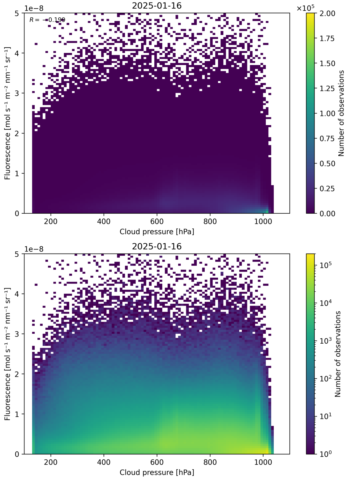
Figure 80: Scatter density plot of “Cloud pressure” against “Fluorescence” for 2025-01-15 to 2025-01-17.
