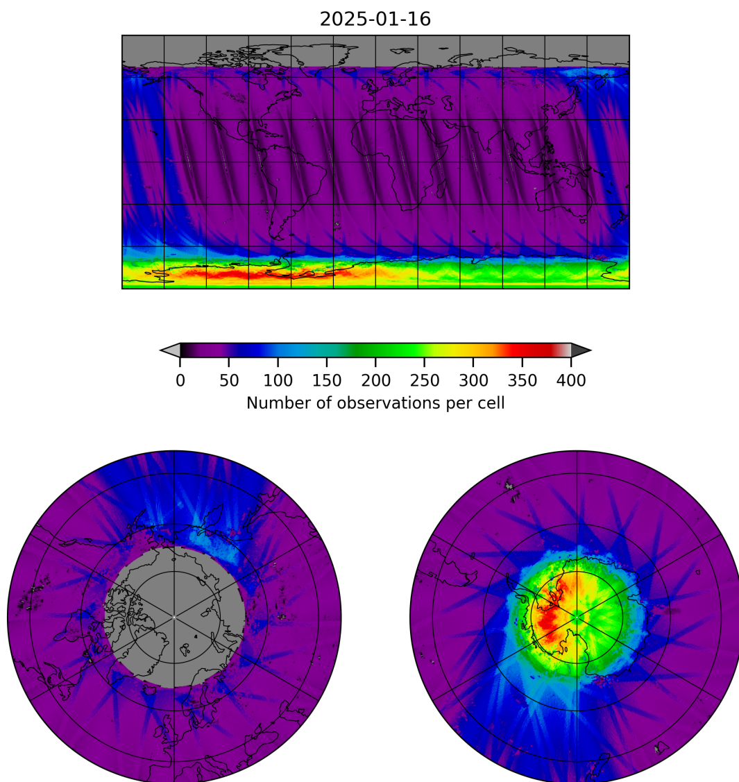
Figure 11: Map of the number of observations for 2025-01-15 to 2025-01-17
