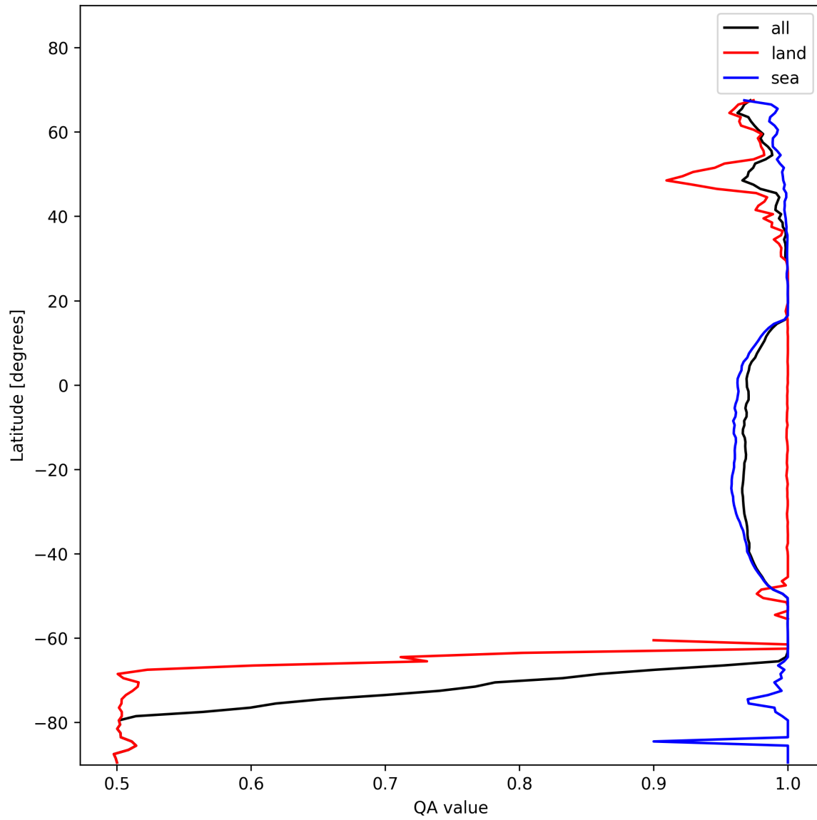
Figure 12: Zonal average of “QA value” for 2025-01-15 to 2025-01-17.
