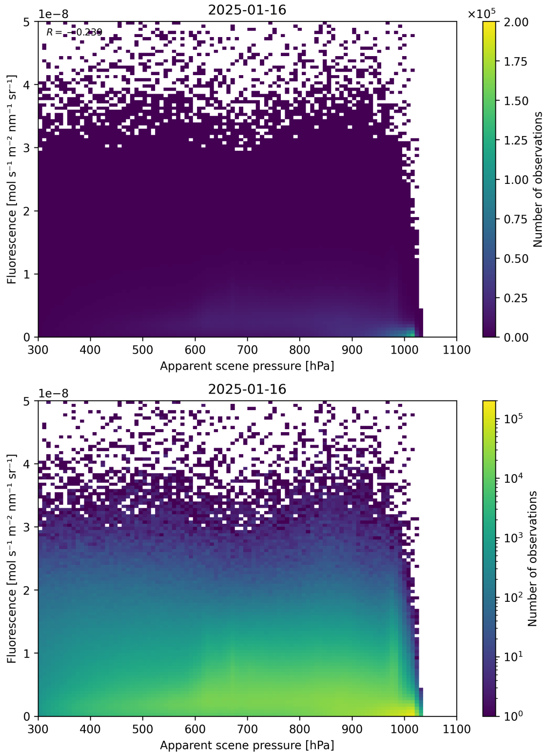
Figure 64: Scatter density plot of “Apparent scene pressure” against “Fluorescence” for 2025-01-15 to 2025-01-17.
