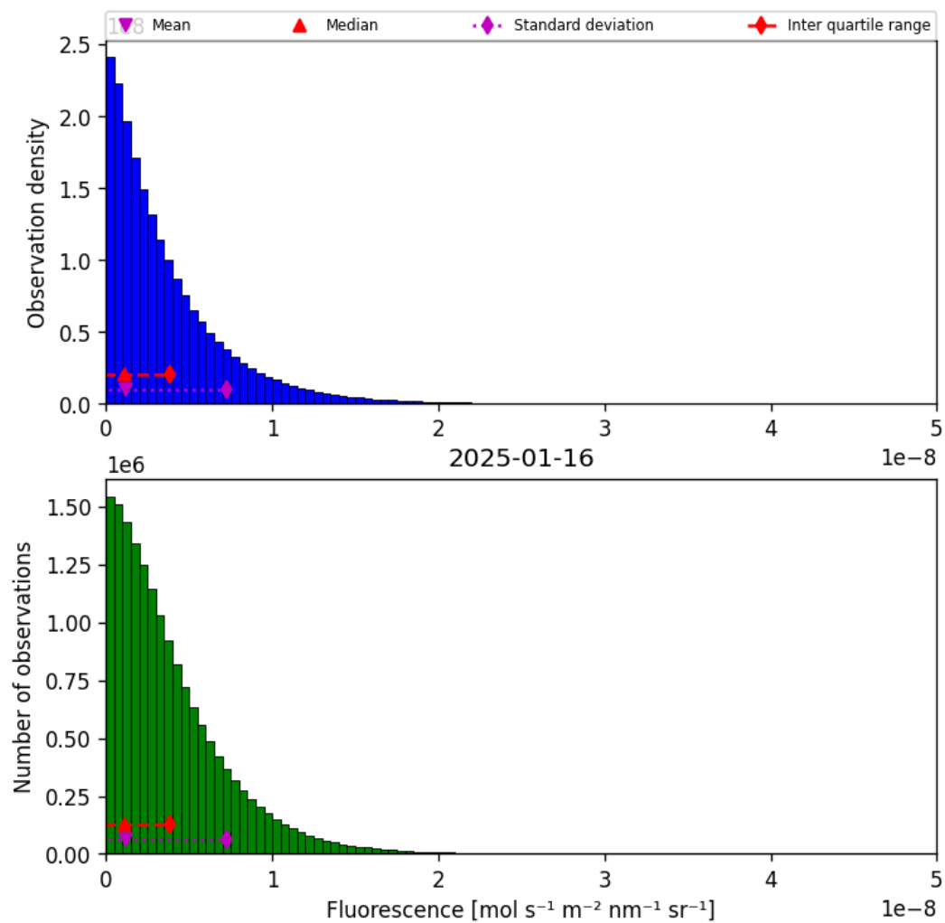
Figure 40: Histogram of “Fluorescence” for 2025-01-15 to 2025-01-17
