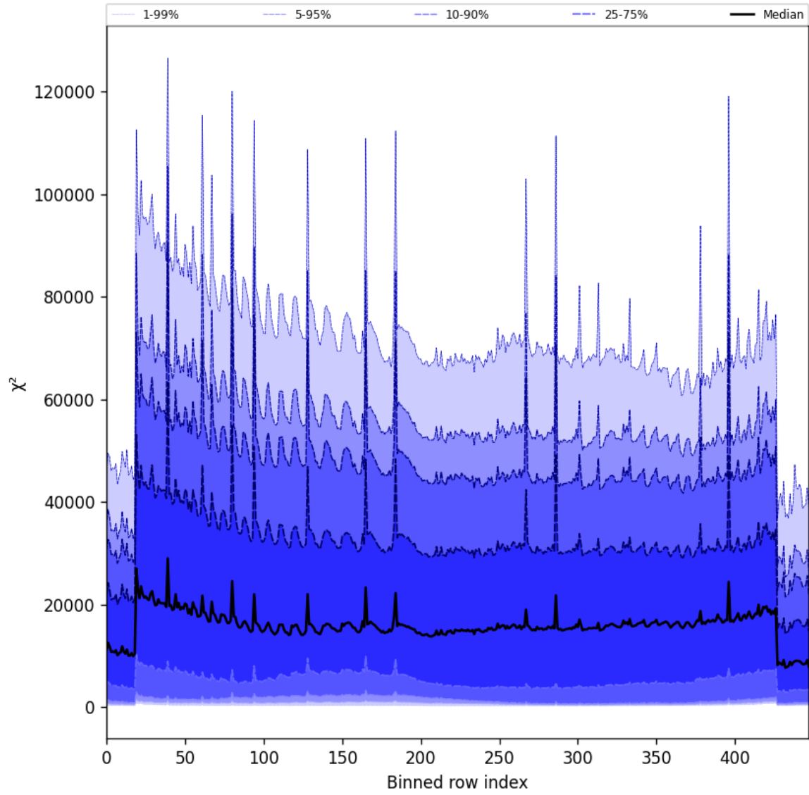
Figure 55: Along track statistics of “ \chi^2 ” for 2025-01-15 to 2025-01-17
