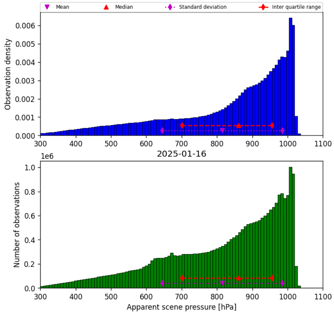
Figure 36: Histogram of “Apparent scene pressure” for 2025-01-15 to 2025-01-17
