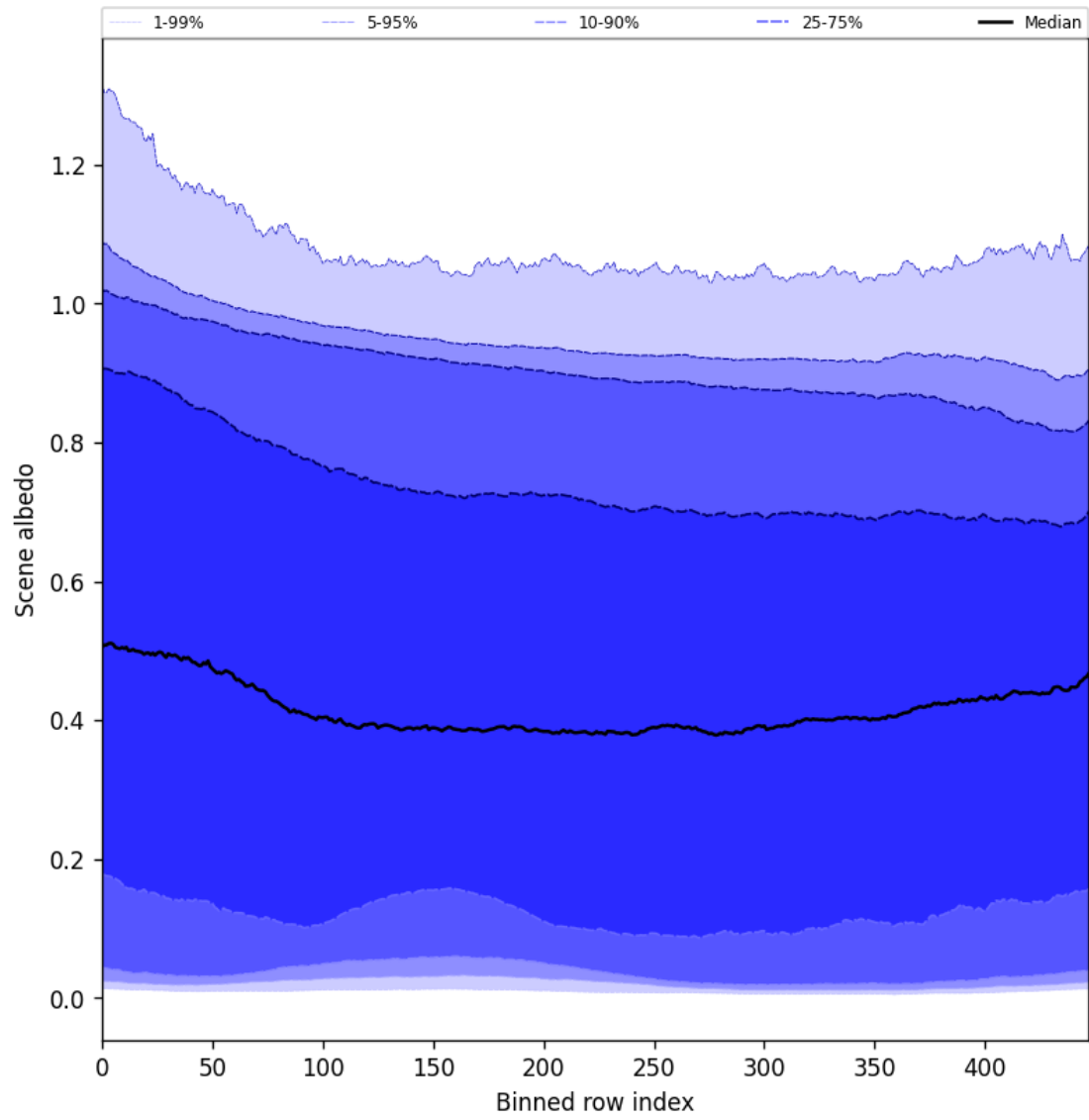
Figure 51: Along track statistics of “Scene albedo” for 2025-01-15 to 2025-01-17
