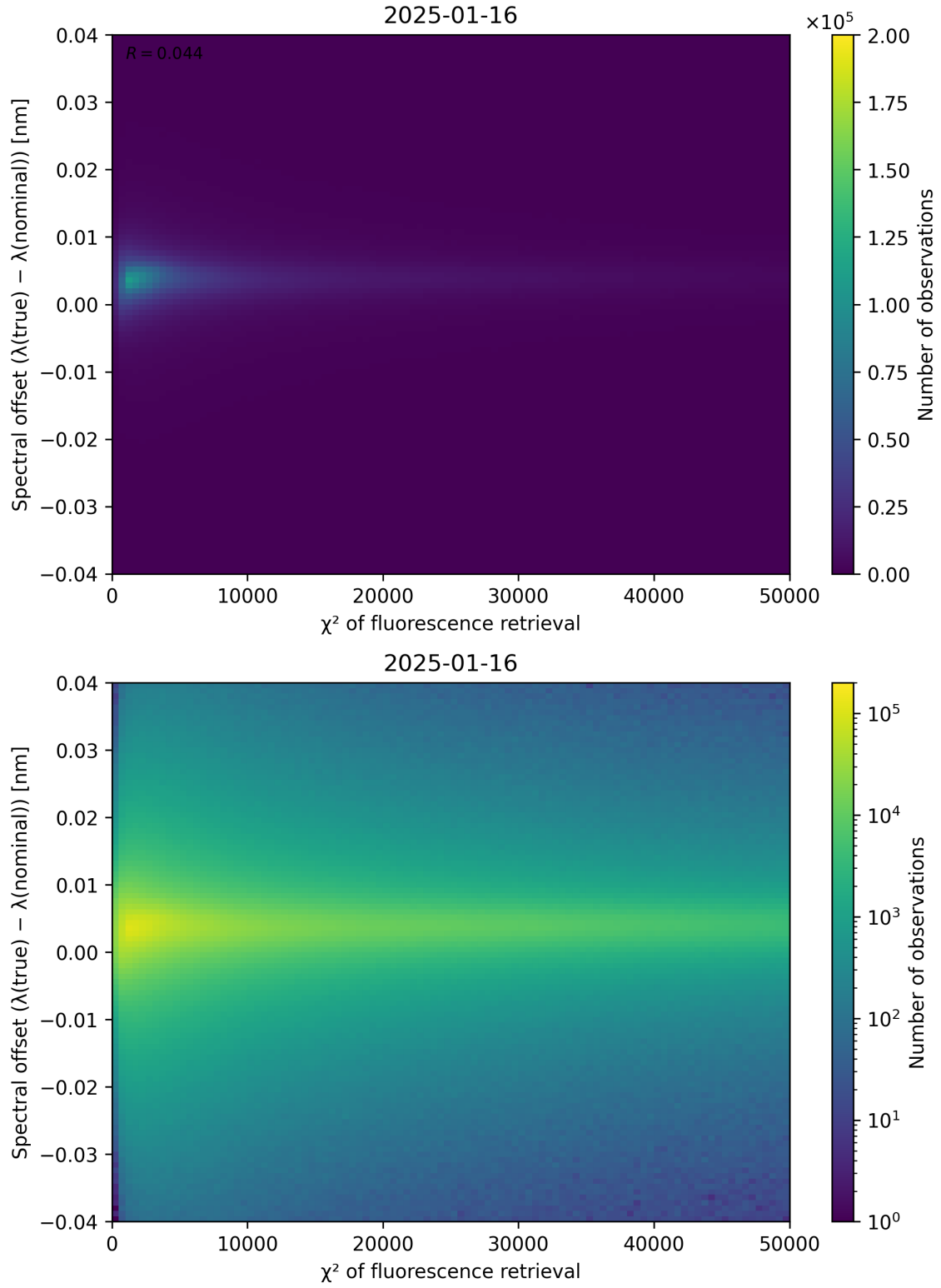
Figure 69: Scatter density plot of “ \chi^2 of fluorescence retrieval” against “Spectral offset ( \lambda_{\text{true}} - \lambda_{\text{nominal}} )” for 2025-01-15 to 2025-01-17.
