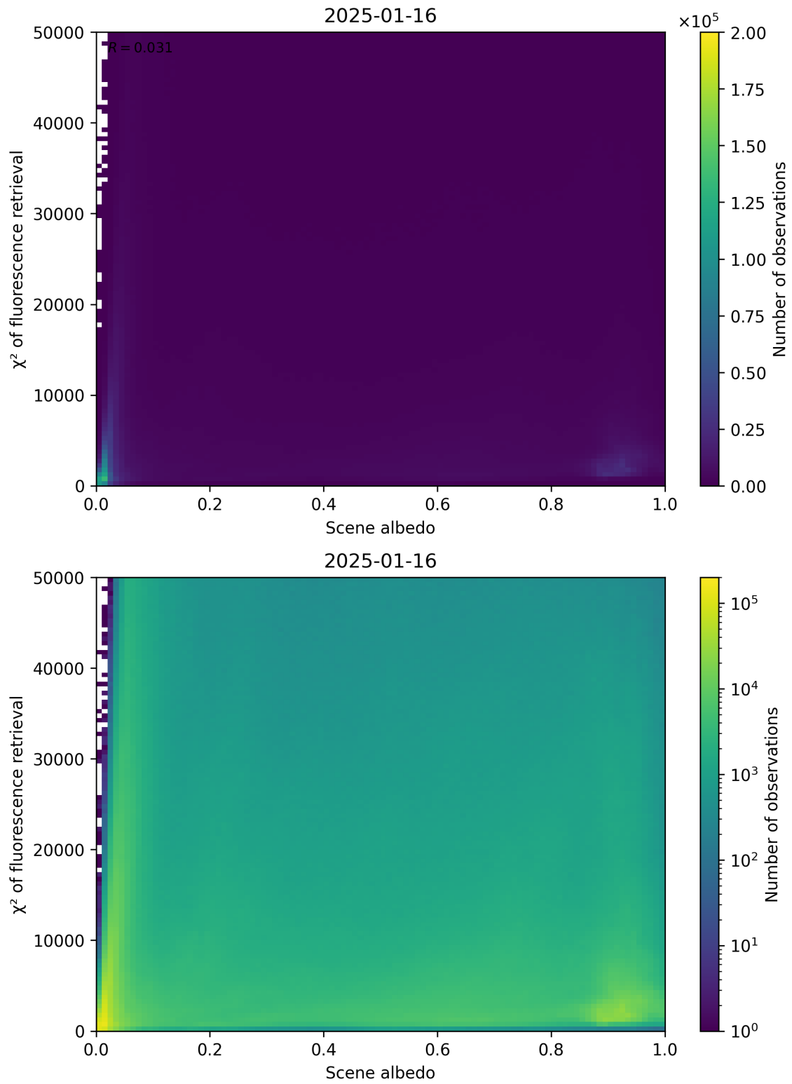
Figure 103: Scatter density plot of “Scene albedo” against “ \chi^2 of fluorescence retrieval” for 2025-01-15 to 2025-01-17.
