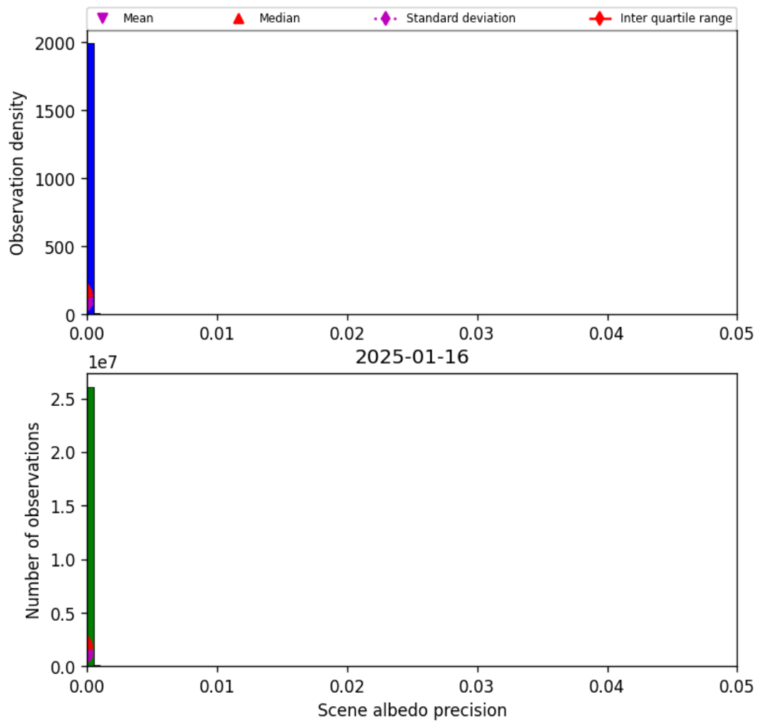
Figure 35: Histogram of “Scene albedo precision” for 2025-01-15 to 2025-01-17
