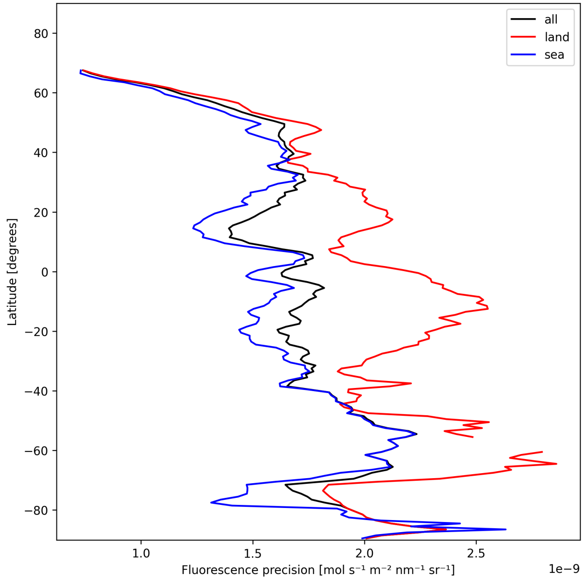
Figure 24: Zonal average of “Fluorescence precision” for 2025-01-15 to 2025-01-17.
