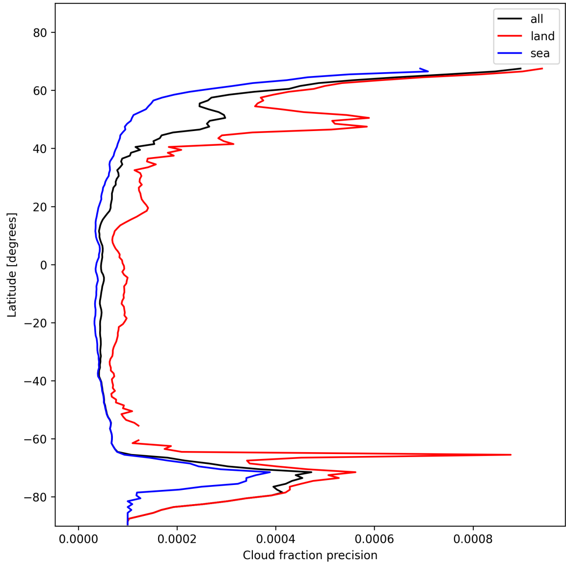
Figure 16: Zonal average of “Cloud fraction precision” for 2025-01-15 to 2025-01-17.
