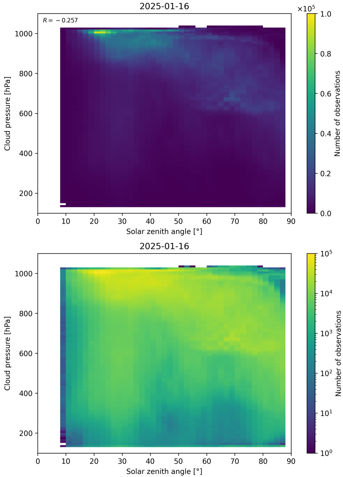
Figure 111: Scatter density plot of “Solar zenith angle” against “Cloud pressure” for 2025-01-15 to 2025-01-17.
