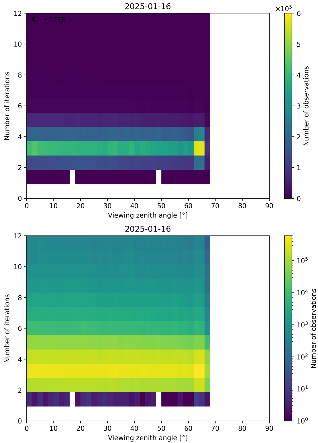
Figure 124: Scatter density plot of “Viewing zenith angle” against “Number of iterations” for 2025-01-15 to 2025-01-17.
