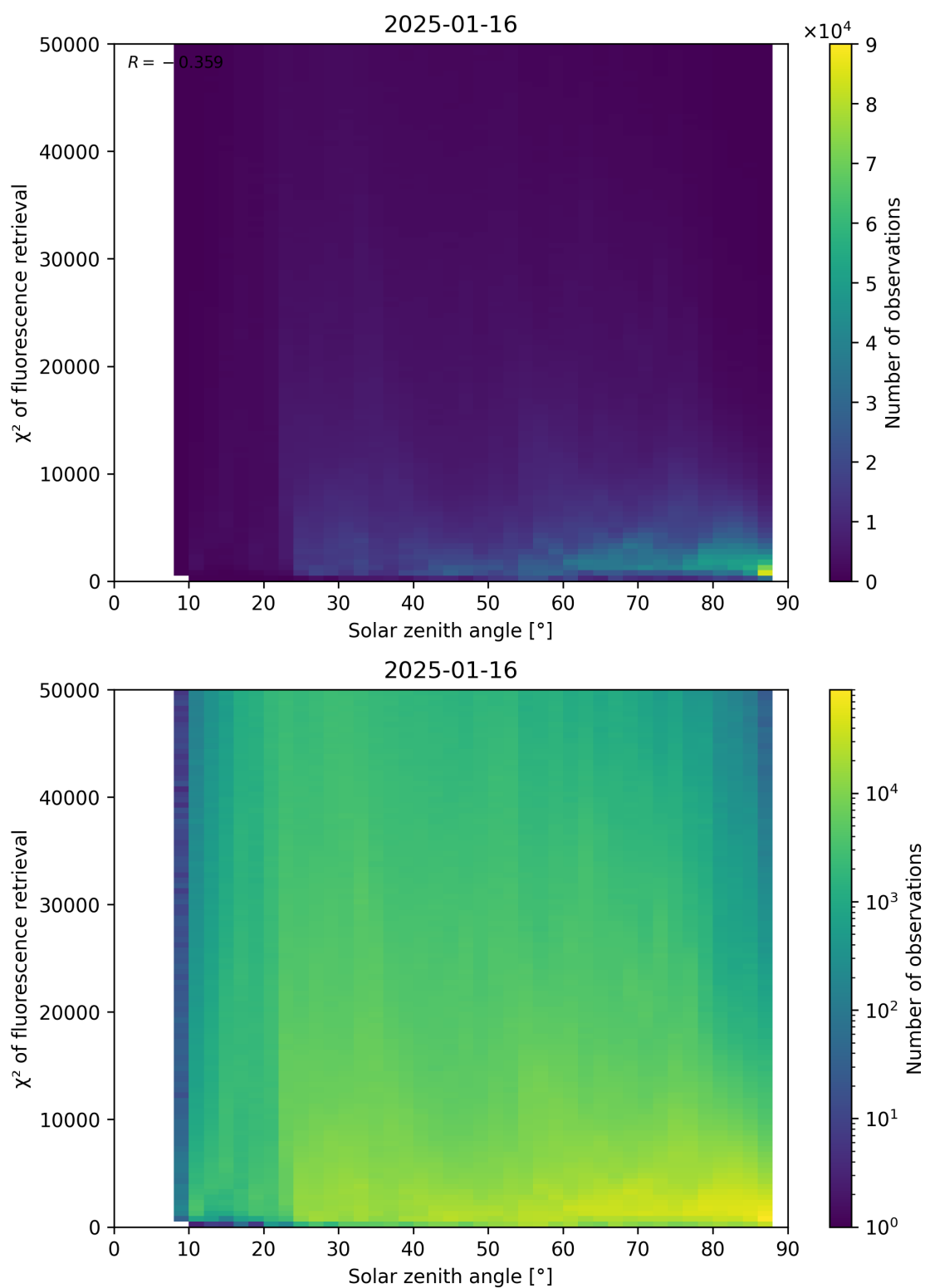
Figure 109: Scatter density plot of “Solar zenith angle” against “ \chi^2 of fluorescence retrieval” for 2025-01-15 to 2025-01-17.
