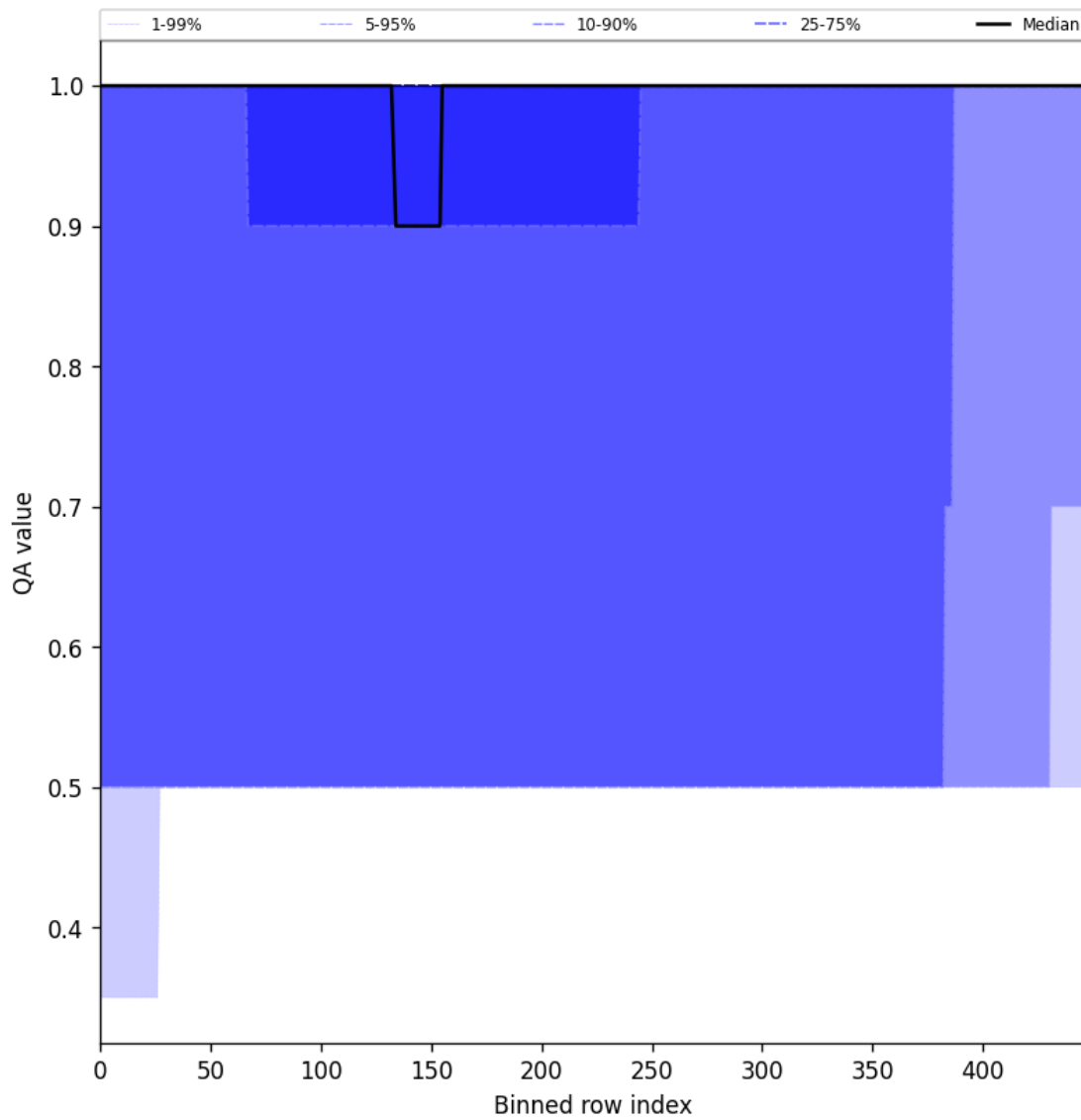
Figure 46: Along track statistics of “QA value” for 2025-01-15 to 2025-01-17
