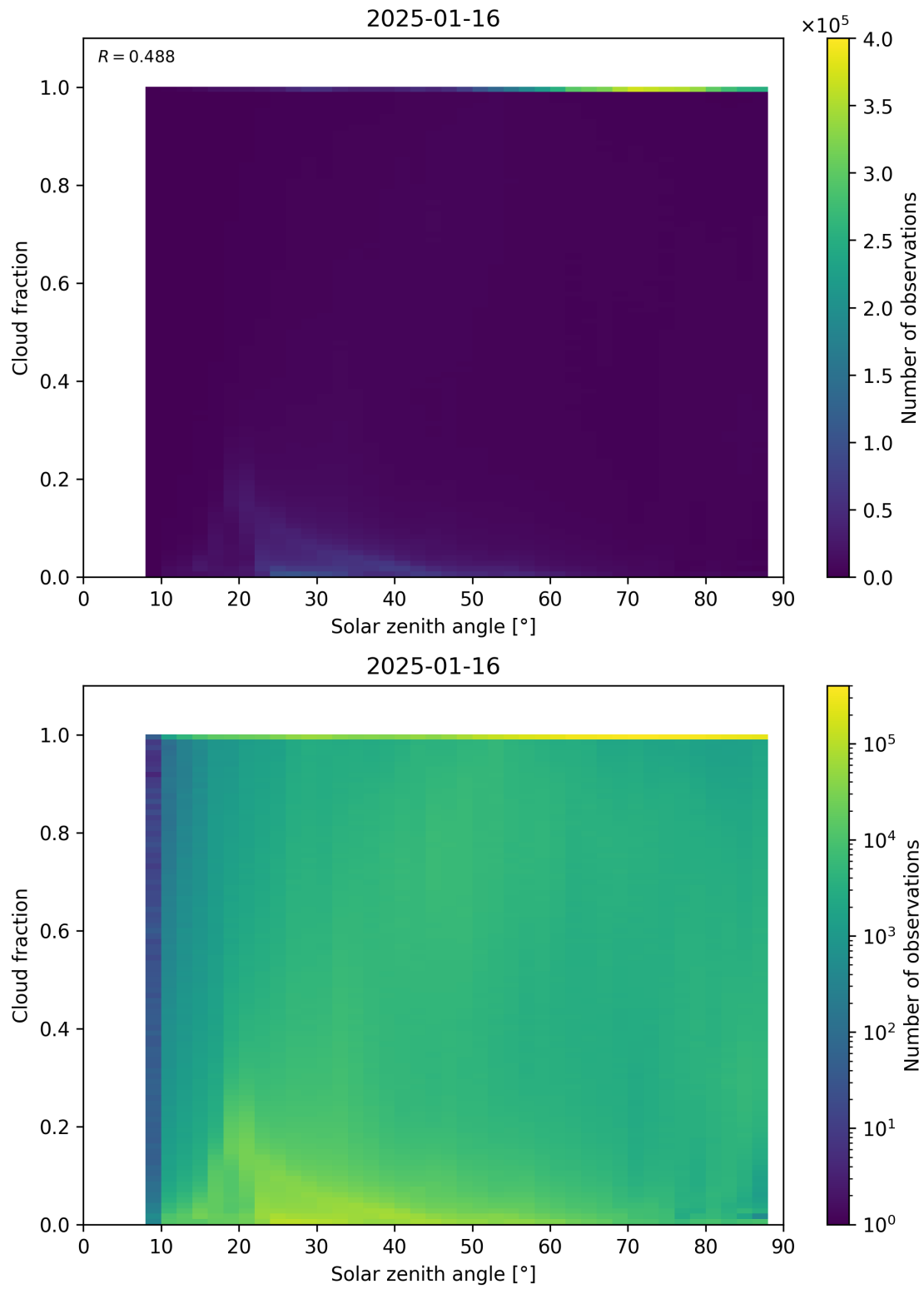
Figure 110: Scatter density plot of “Solar zenith angle” against “Cloud fraction” for 2025-01-15 to 2025-01-17.
