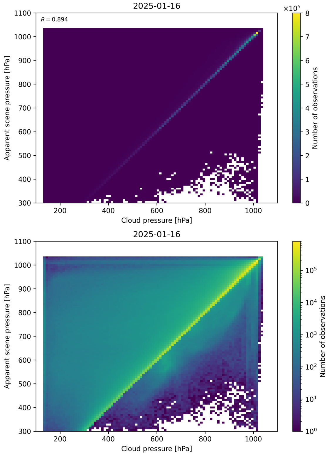
Figure 77: Scatter density plot of “Cloud pressure” against “Apparent scene pressure” for 2025-01-15 to 2025-01-17.
