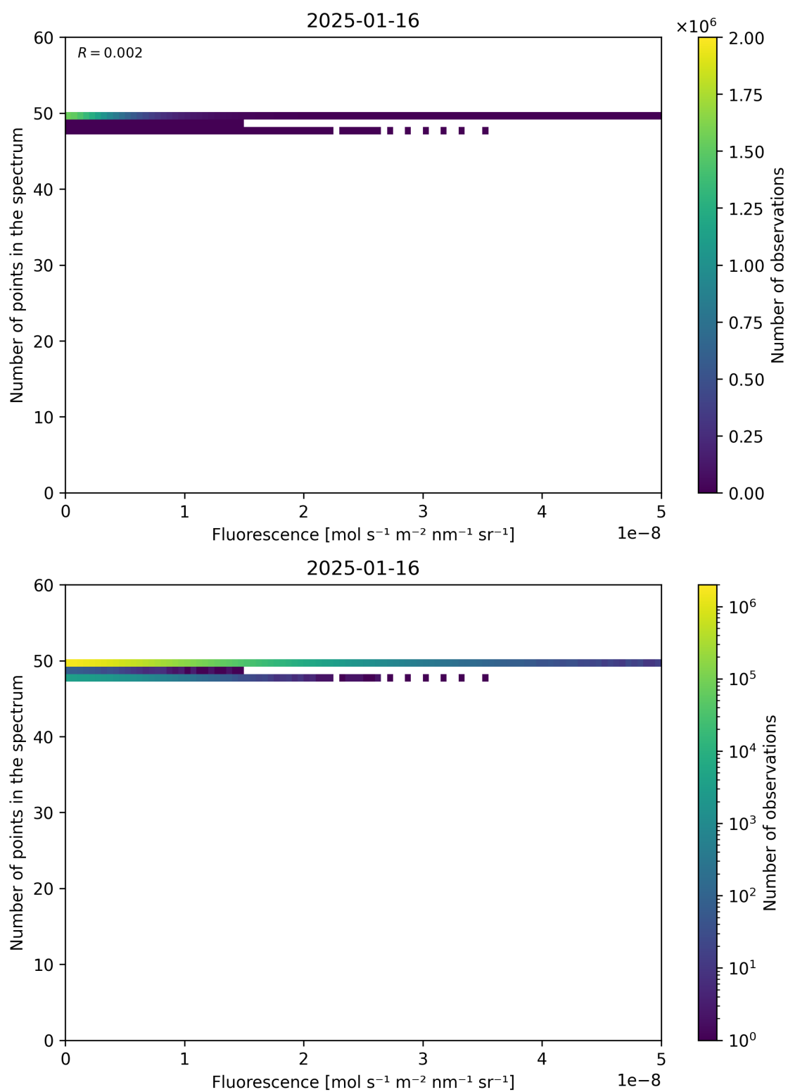
Figure 86: Scatter density plot of “Fluorescence” against “Number of points in the spectrum” for 2025-01-15 to 2025-01-17.
