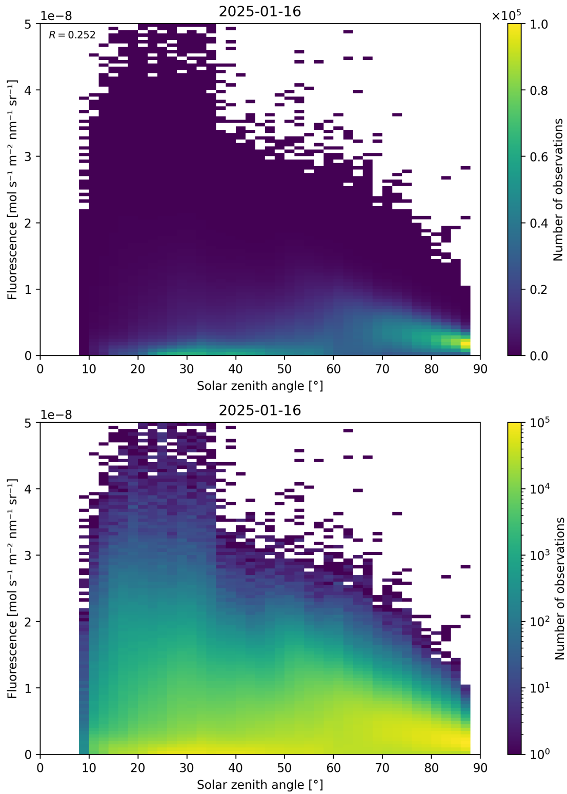
Figure 112: Scatter density plot of “Solar zenith angle” against “Fluorescence” for 2025-01-15 to 2025-01-17.
