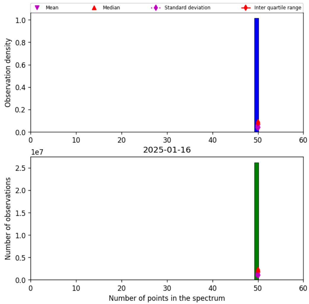
Figure 44: Histogram of “Number of points in the spectrum” for 2025-01-15 to 2025-01-17
