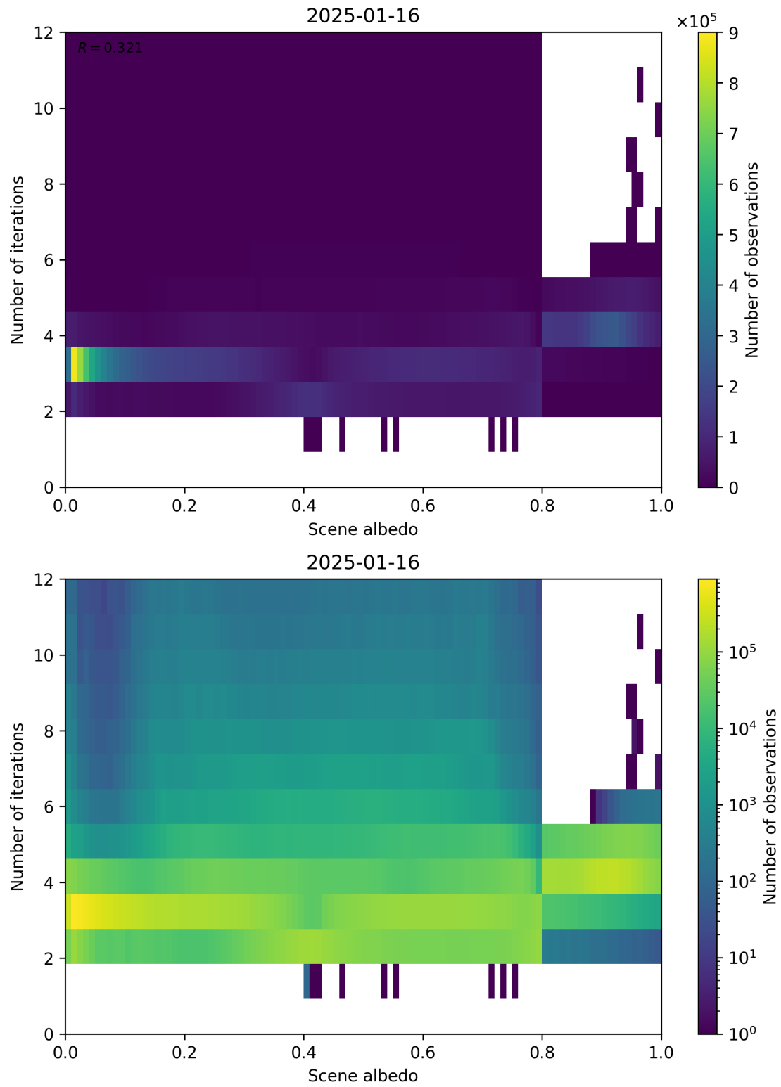
Figure 105: Scatter density plot of “Scene albedo” against “Number of iterations” for 2025-01-15 to 2025-01-17.
