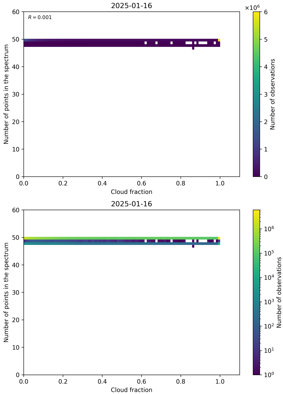
Figure 74: Scatter density plot of “Cloud fraction” against “Number of points in the spectrum” for 2025-01-15 to 2025-01-17.
