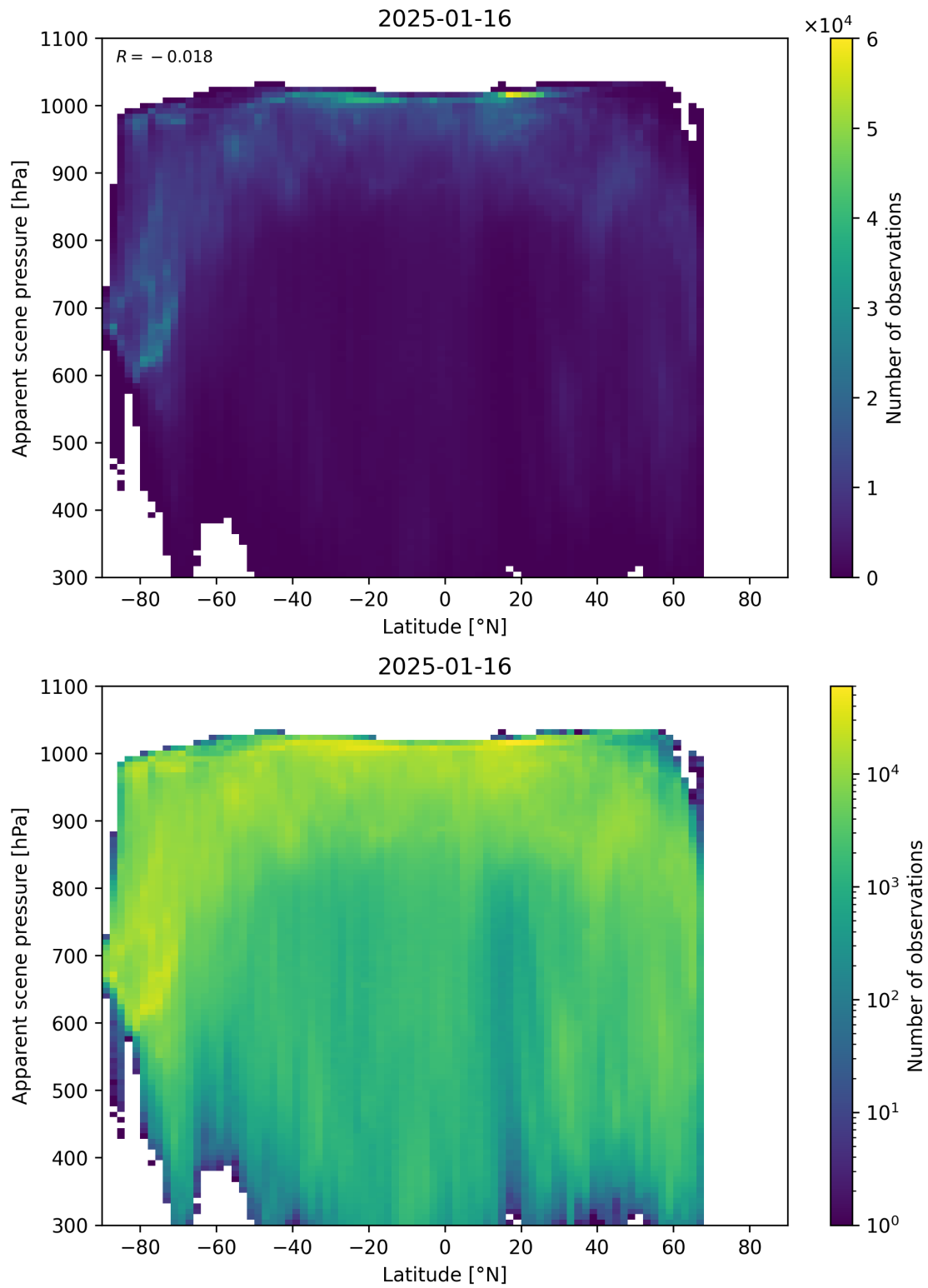
Figure 88: Scatter density plot of “Latitude” against “Apparent scene pressure” for 2025-01-15 to 2025-01-17.
