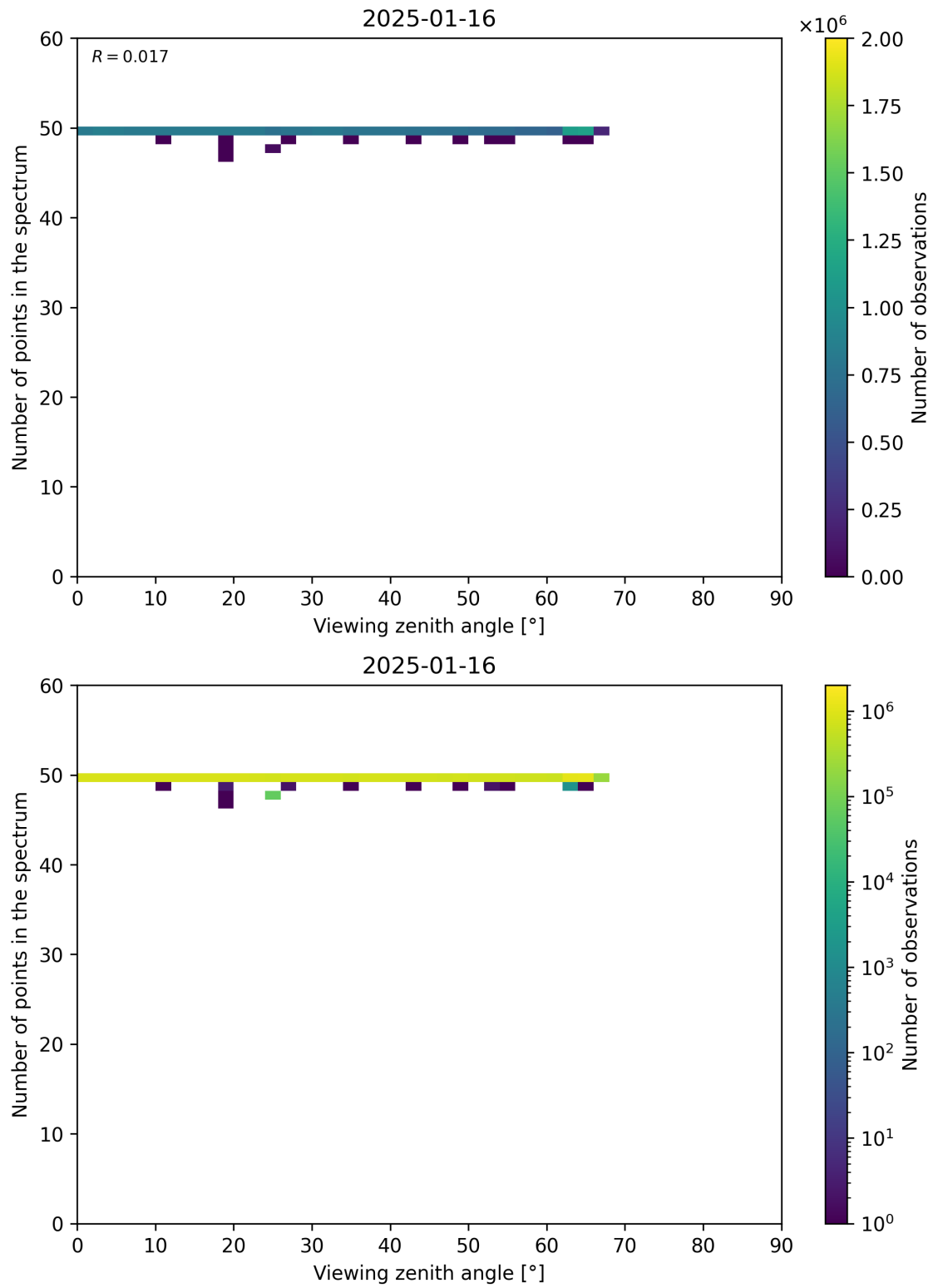
Figure 125: Scatter density plot of “Viewing zenith angle” against “Number of points in the spectrum” for 2025-01-15 to 2025-01-17.
