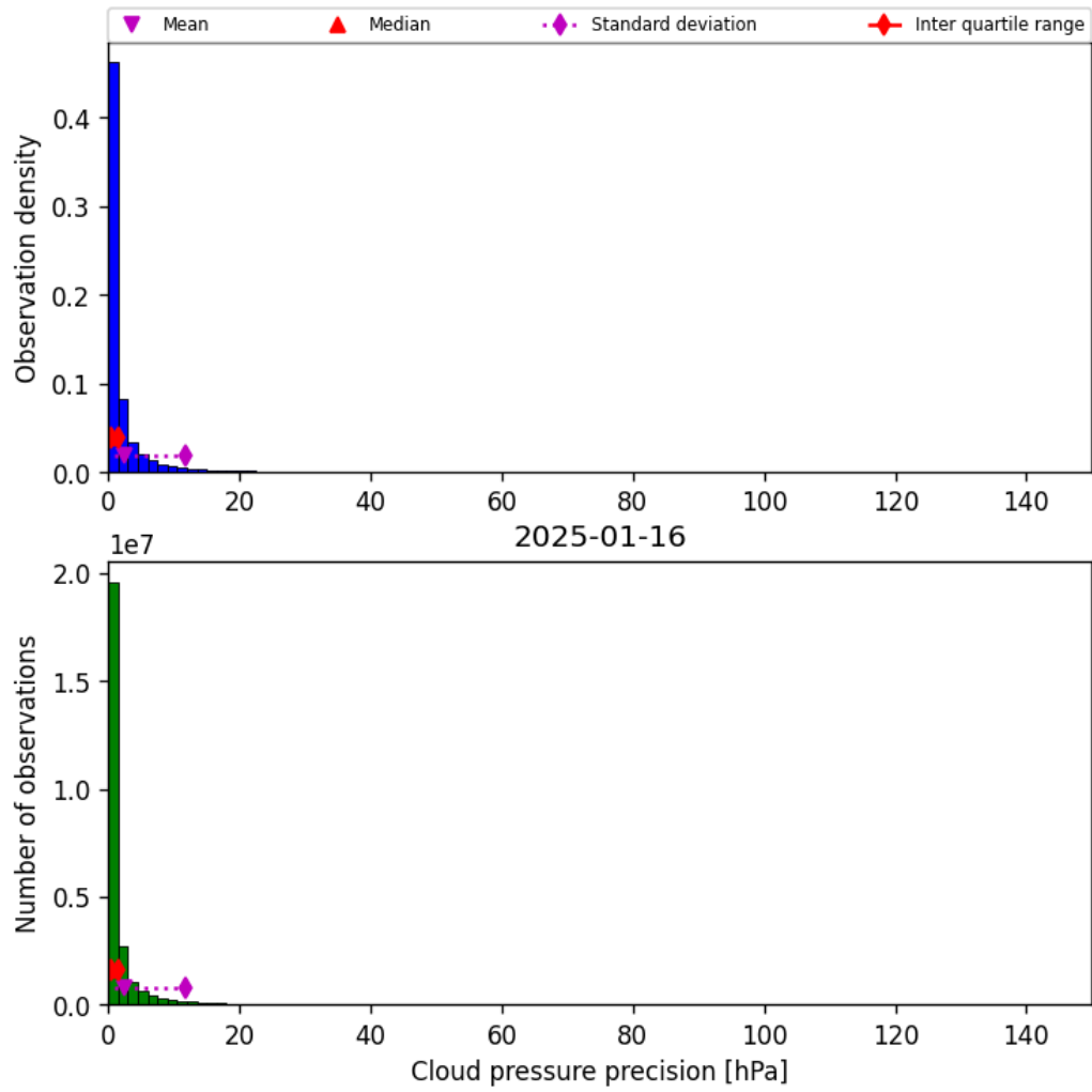
Figure 31: Histogram of “Cloud pressure precision” for 2025-01-15 to 2025-01-17
