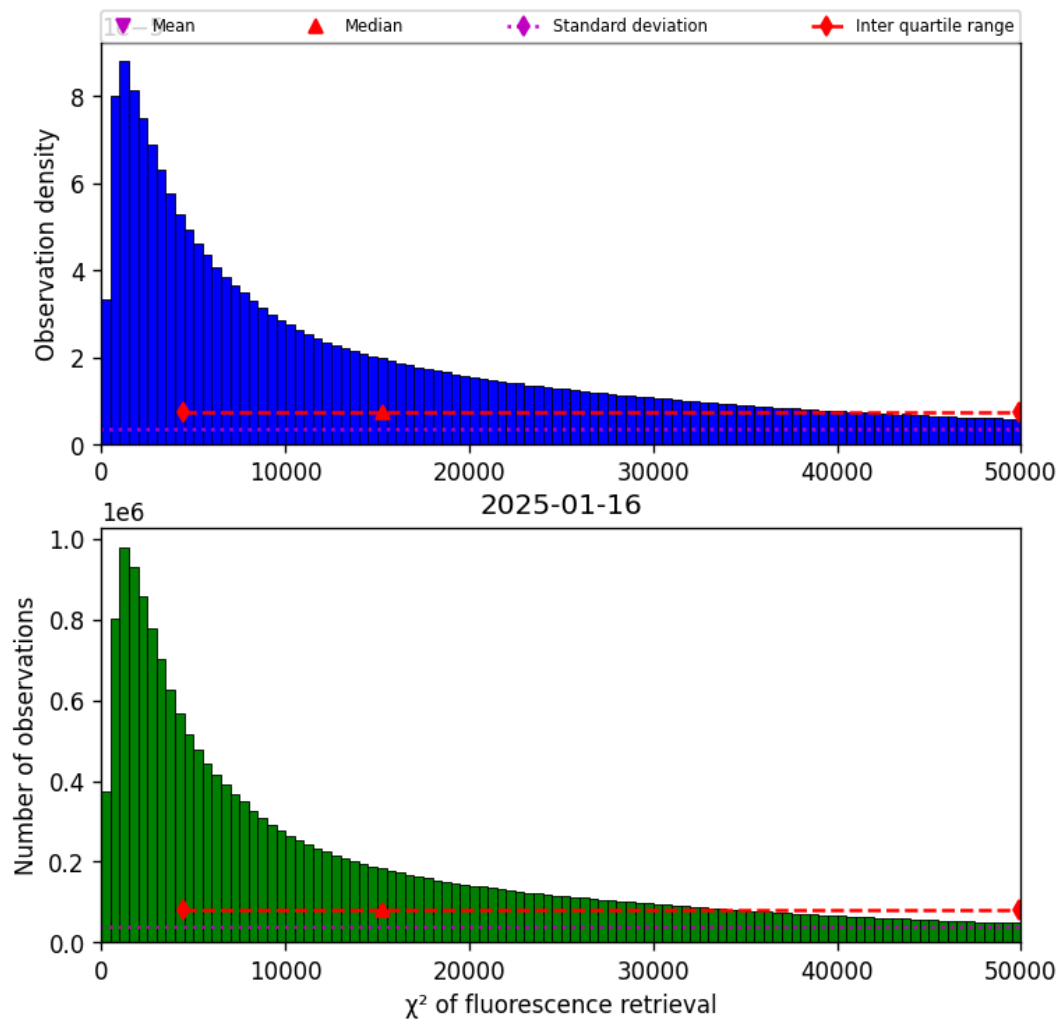
Figure 42: Histogram of “ \chi^2 of fluorescence retrieval” for 2025-01-15 to 2025-01-17
