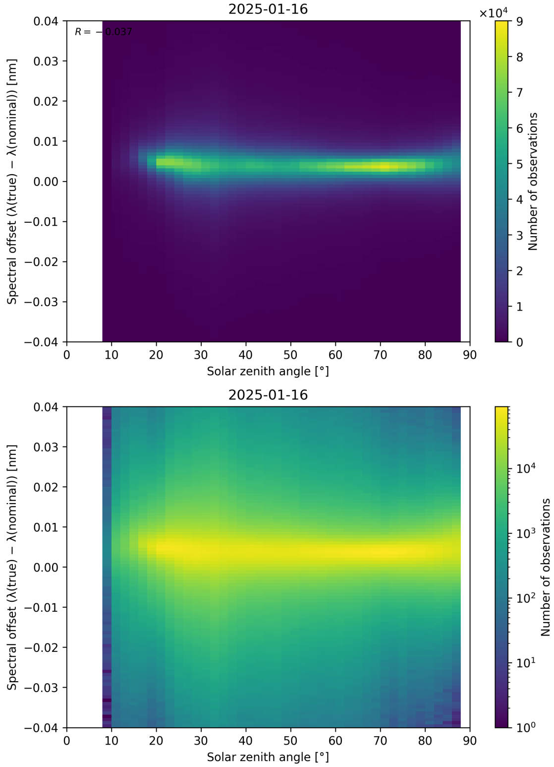
Figure 117: Scatter density plot of “Solar zenith angle” against “Spectral offset ( \lambda_{\text{true}} - \lambda_{\text{nominal}} )” for 2025-01-15 to 2025-01-17.
