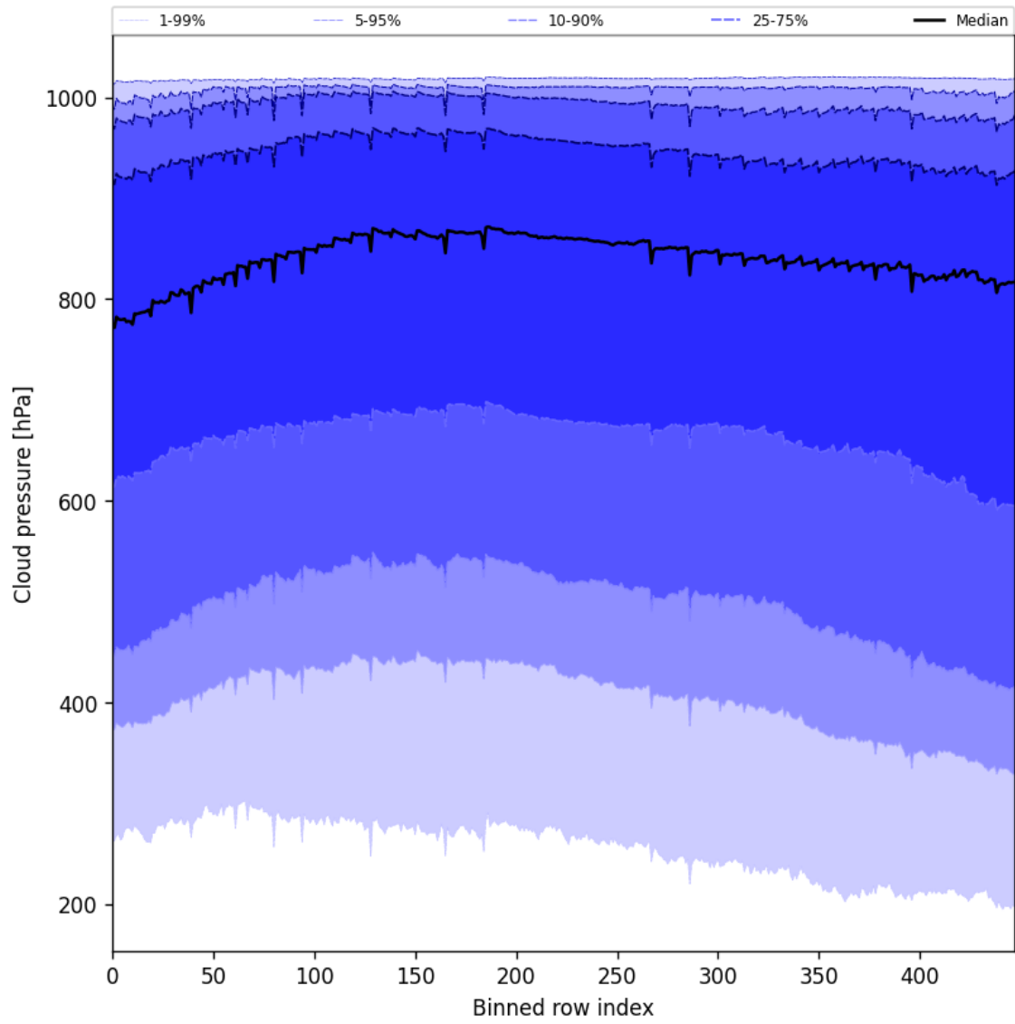
Figure 47: Along track statistics of “Cloud pressure” for 2025-01-15 to 2025-01-17
