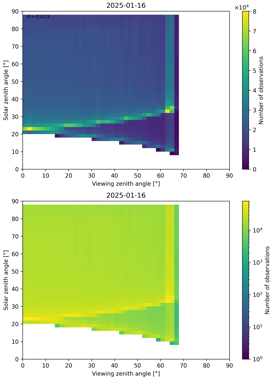
Figure 127: Scatter density plot of “Viewing zenith angle” against “Solar zenith angle” for 2025-01-15 to 2025-01-17.
