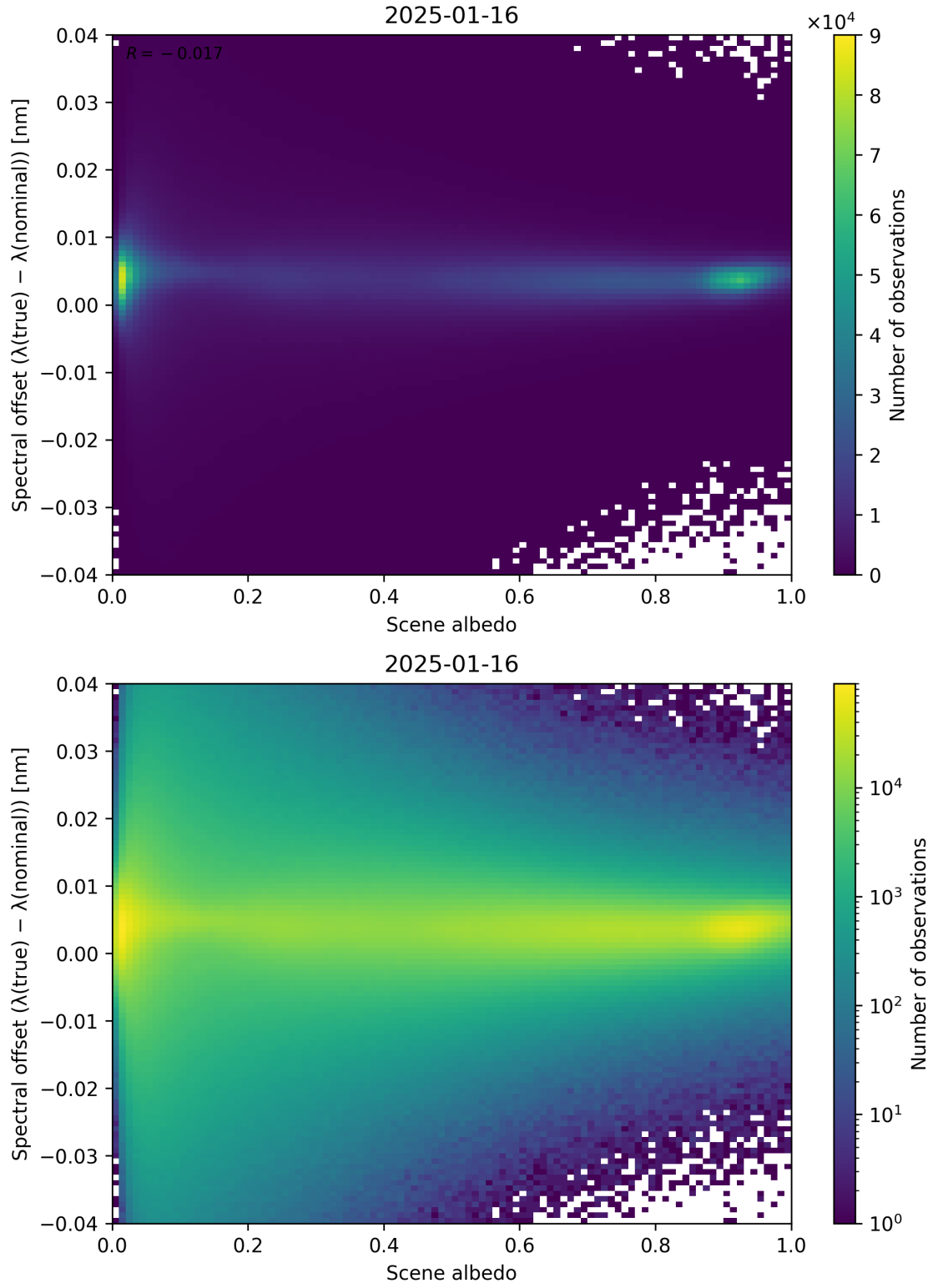
Figure 107: Scatter density plot of “Scene albedo” against “Spectral offset ( \lambda_{\text{true}} - \lambda_{\text{nominal}} )” for 2025-01-15 to 2025-01-17.
