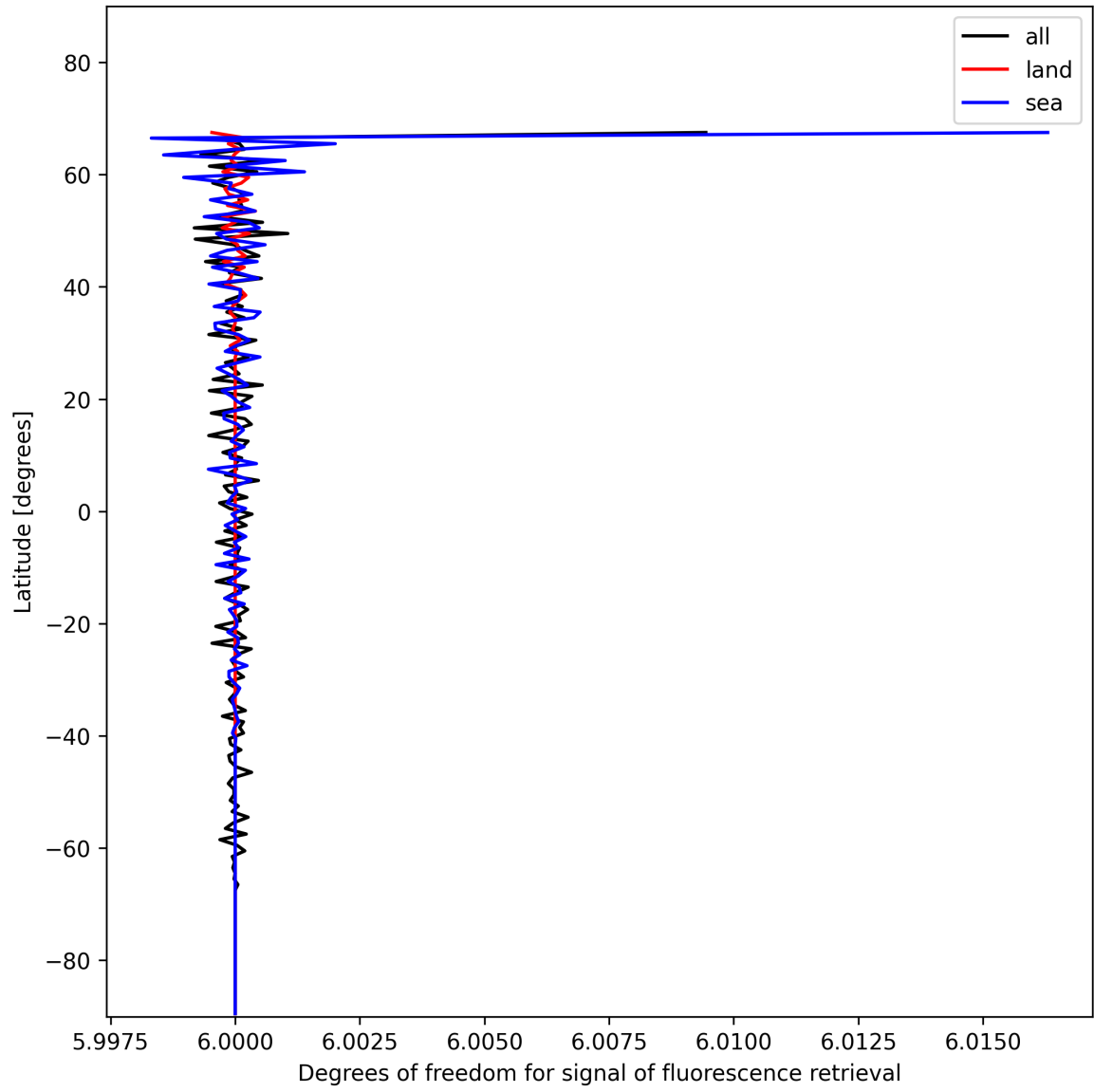
Figure 26: Zonal average of “Degrees of freedom for signal of fluorescence retrieval” for 2025-01-15 to 2025-01-17.
