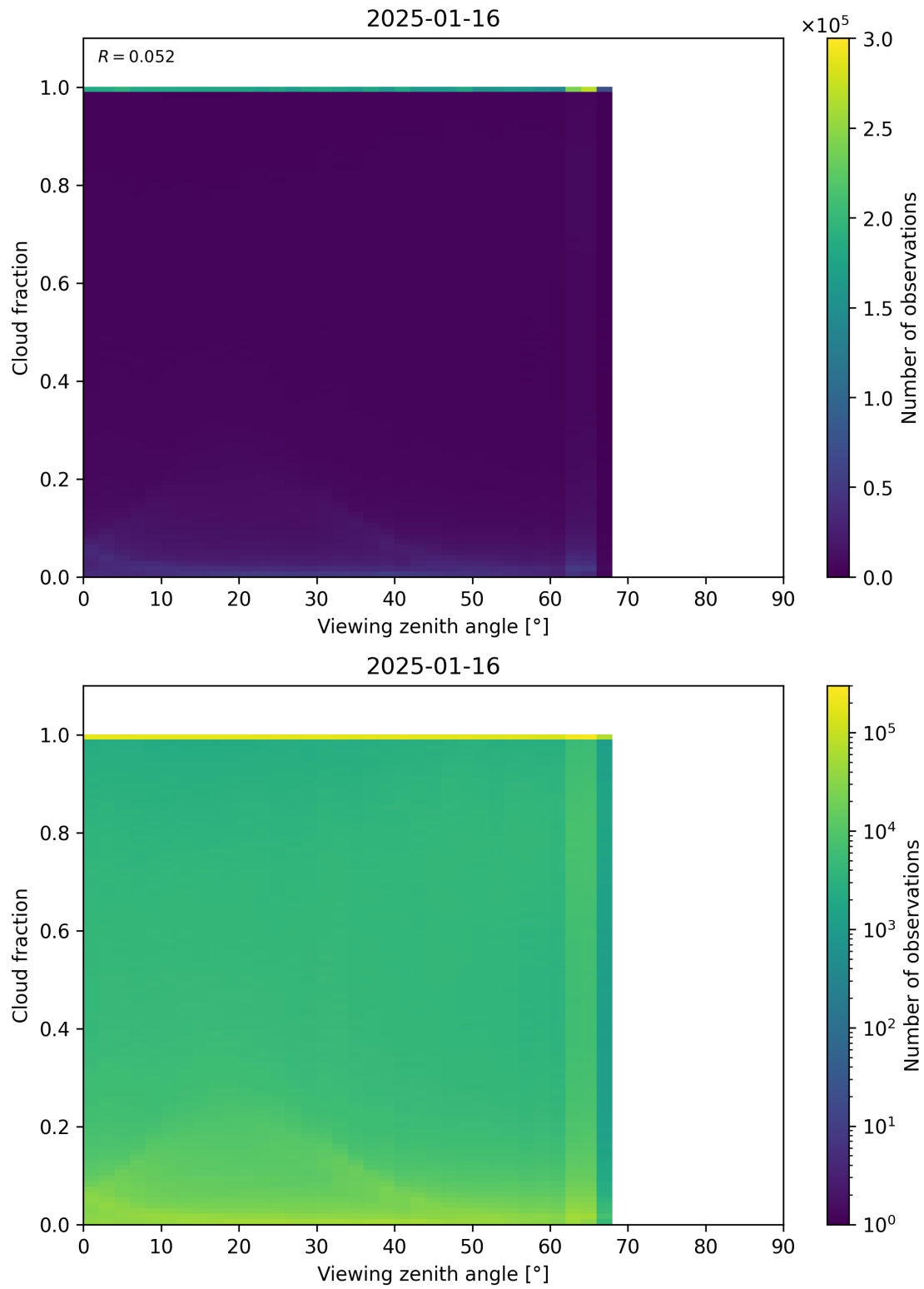
Figure 120: Scatter density plot of “Viewing zenith angle” against “Cloud fraction” for 2025-01-15 to 2025-01-17.
