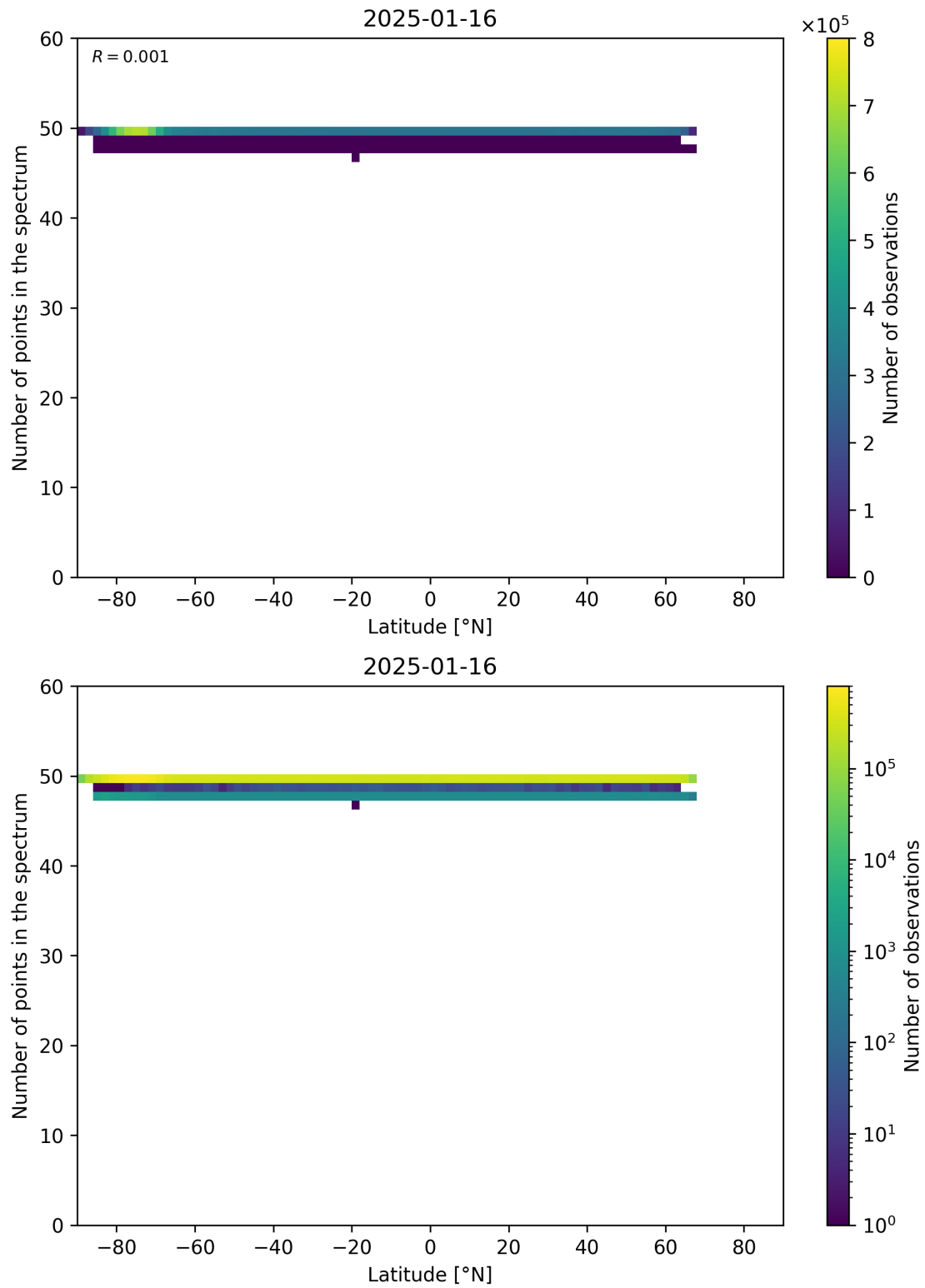
Figure 94: Scatter density plot of “Latitude” against “Number of points in the spectrum” for 2025-01-15 to 2025-01-17.
