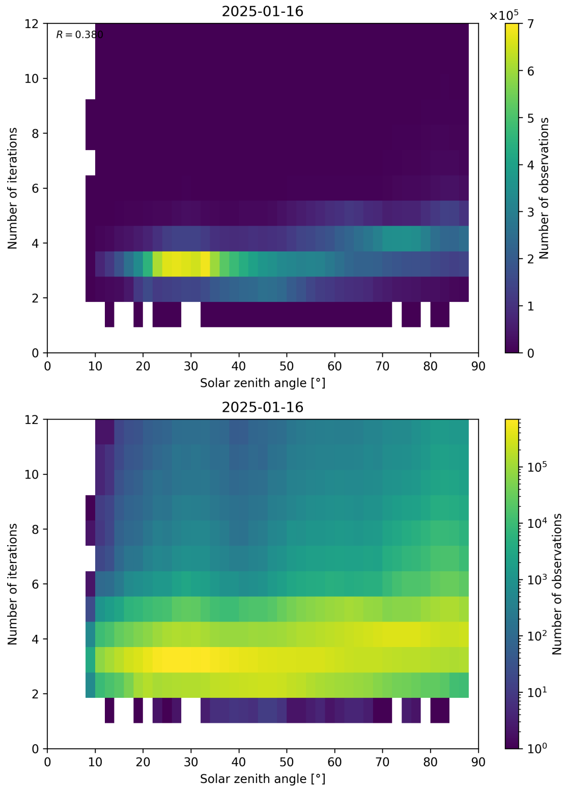
Figure 114: Scatter density plot of “Solar zenith angle” against “Number of iterations” for 2025-01-15 to 2025-01-17.
