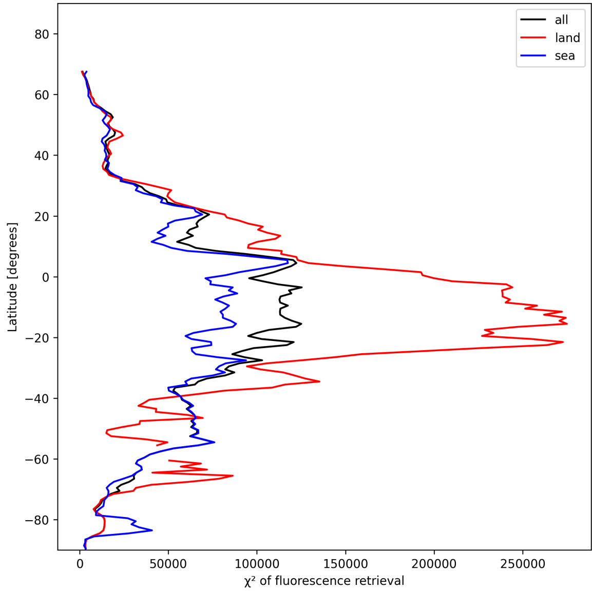
Figure 25: Zonal average of “ \chi^2 of fluorescence retrieval” for 2025-01-15 to 2025-01-17.
