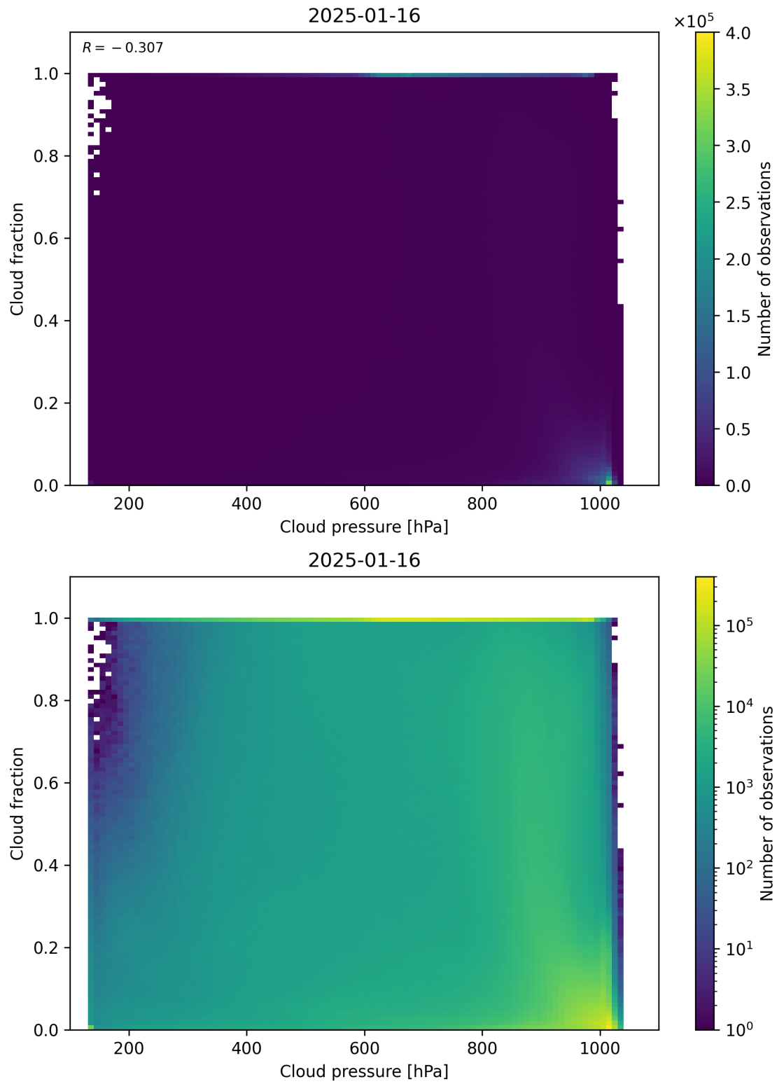
Figure 79: Scatter density plot of “Cloud pressure” against “Cloud fraction” for 2025-01-15 to 2025-01-17.
