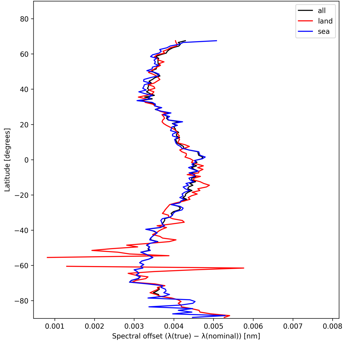
Figure 28: Zonal average of “Spectral offset ( \lambda_{\text{true}} - \lambda_{\text{nominal}} )” for 2025-01-15 to 2025-01-17.
