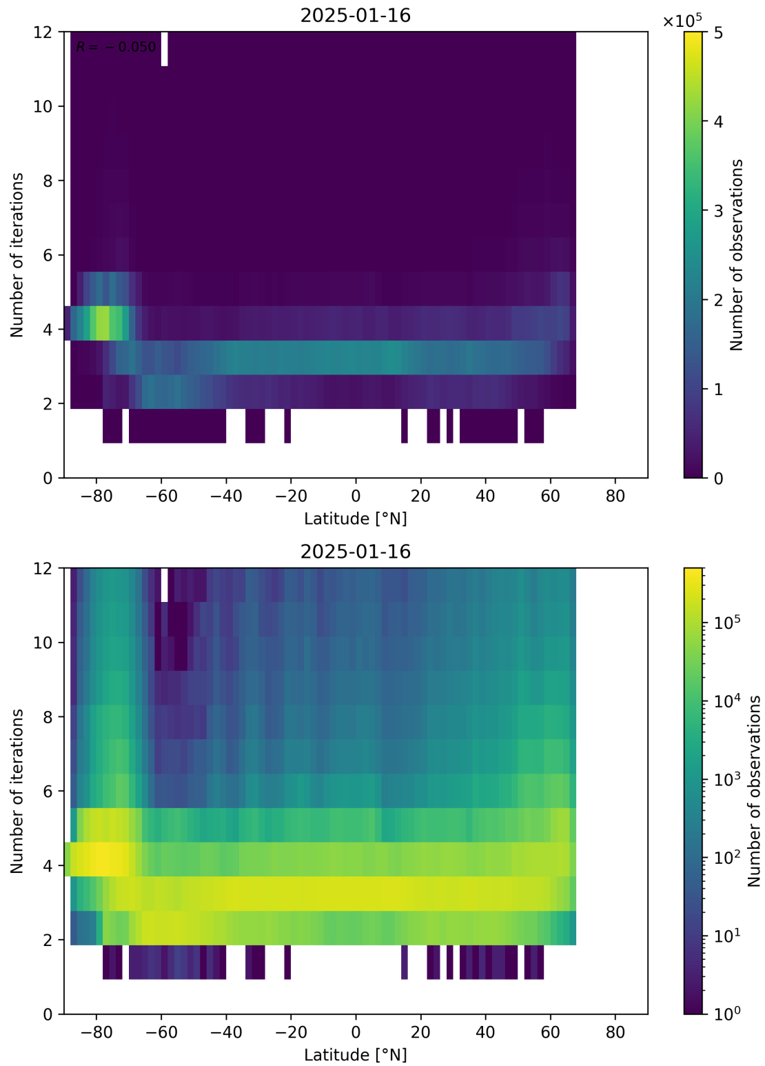
Figure 93: Scatter density plot of “Latitude” against “Number of iterations” for 2025-01-15 to 2025-01-17.
