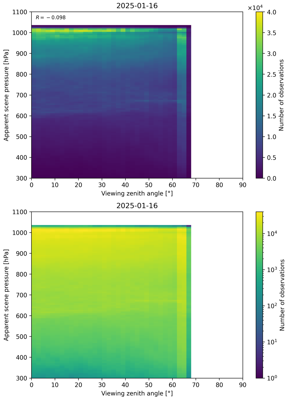
Figure 118: Scatter density plot of “Viewing zenith angle” against “Apparent scene pressure” for 2025-01-15 to 2025-01-17.
