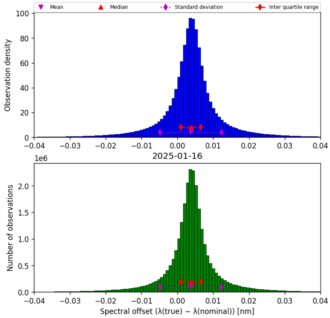
Figure 45: Histogram of “Spectral offset ( \lambda_{\text{true}} - \lambda_{\text{nominal}} )” for 2025-01-15 to 2025-01-17
