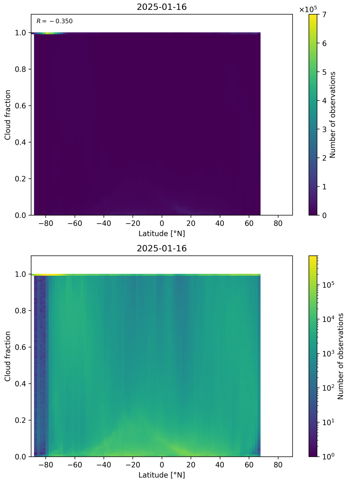
Figure 90: Scatter density plot of “Latitude” against “Cloud fraction” for 2025-01-15 to 2025-01-17.
