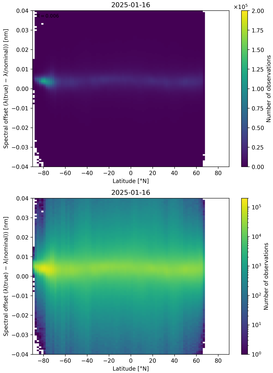
Figure 96: Scatter density plot of “Latitude” against “Spectral offset ( \lambda_{\text{true}} - \lambda_{\text{nominal}} )” for 2025-01-15 to 2025-01-17.
