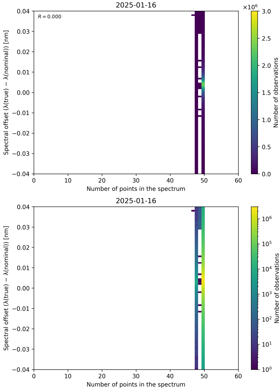
Figure 101: Scatter density plot of “Number of points in the spectrum” against “Spectral offset ( \lambda_{\text{true}} - \lambda_{\text{nominal}} )” for 2025-01-15 to 2025-01-17.
