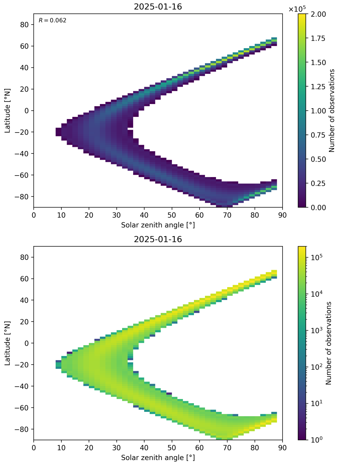
Figure 113: Scatter density plot of “Solar zenith angle” against “Latitude” for 2025-01-15 to 2025-01-17.
