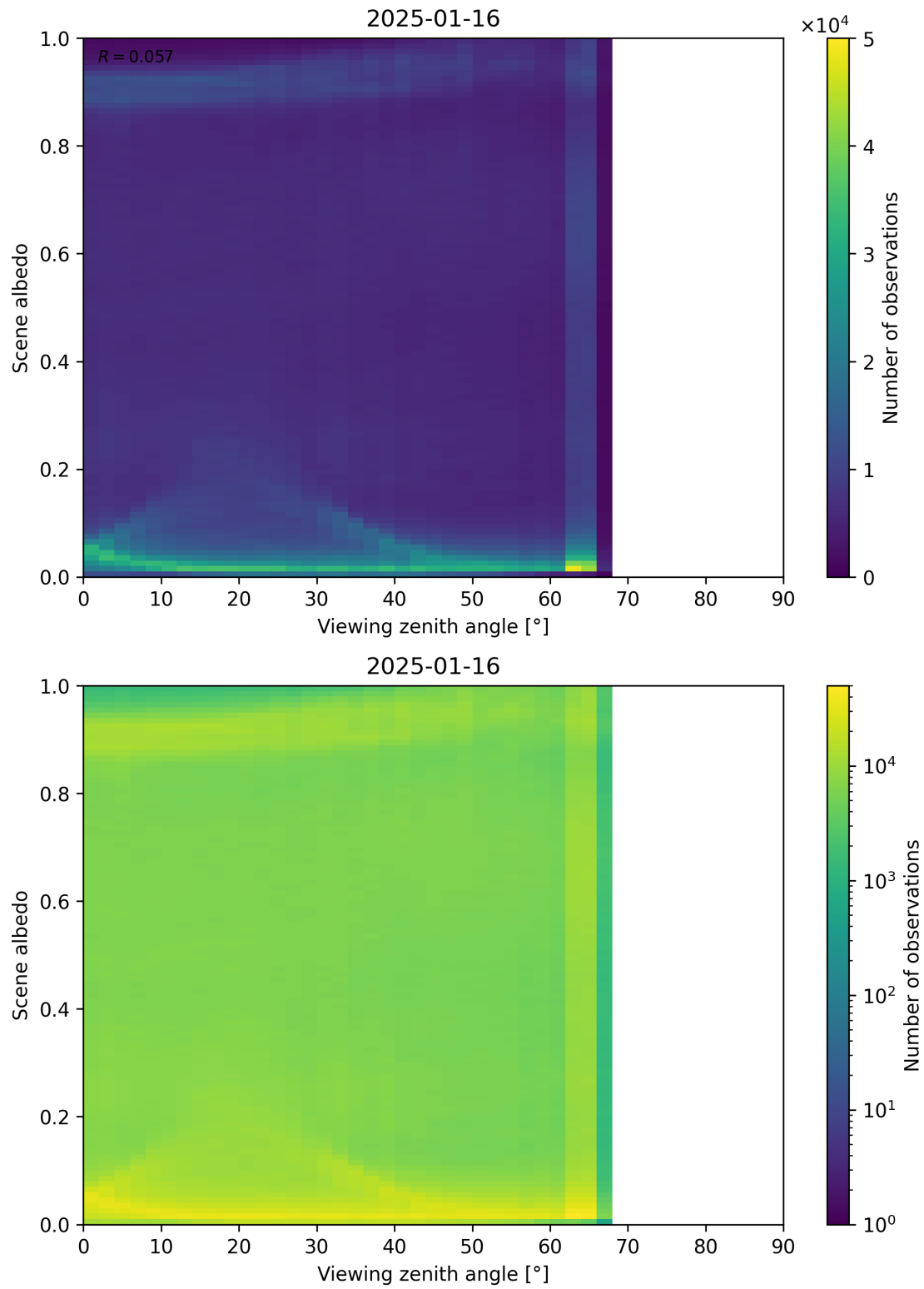
Figure 126: Scatter density plot of “Viewing zenith angle” against “Scene albedo” for 2025-01-15 to 2025-01-17.
