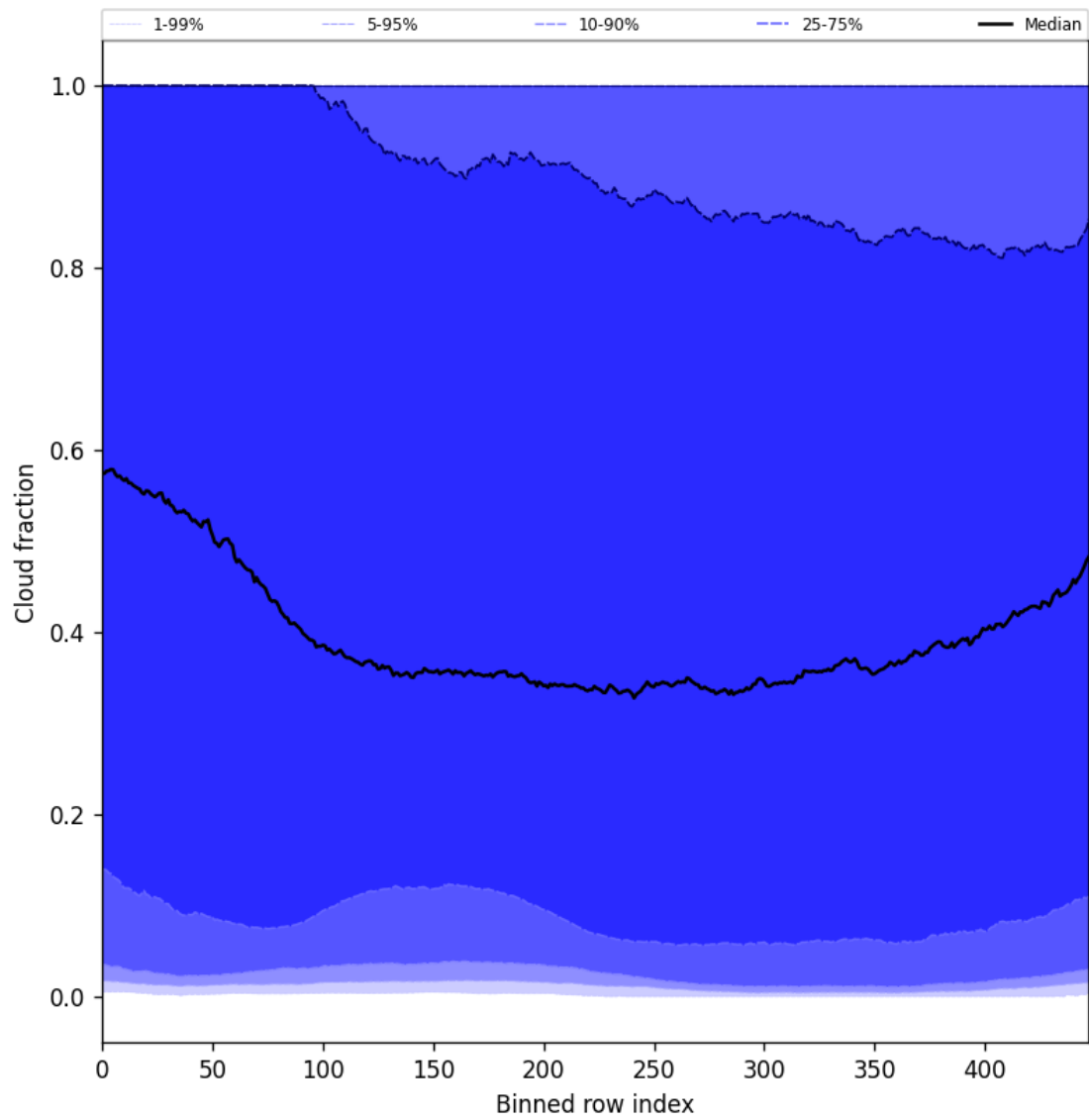
Figure 49: Along track statistics of “Cloud fraction” for 2025-01-15 to 2025-01-17
