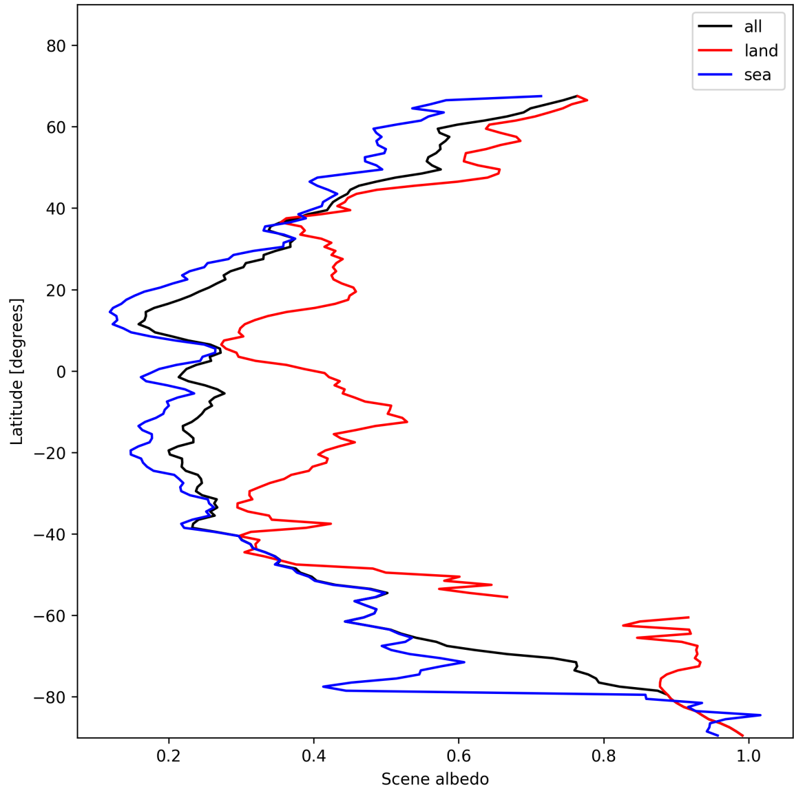
Figure 17: Zonal average of “Scene albedo” for 2025-01-15 to 2025-01-17.
