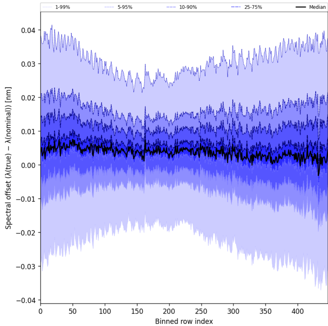
Figure 62: Along track statistics of “Spectral offset ( \lambda_{\text{true}} - \lambda_{\text{nominal}} )” for 2025-01-15 to 2025-01-17
