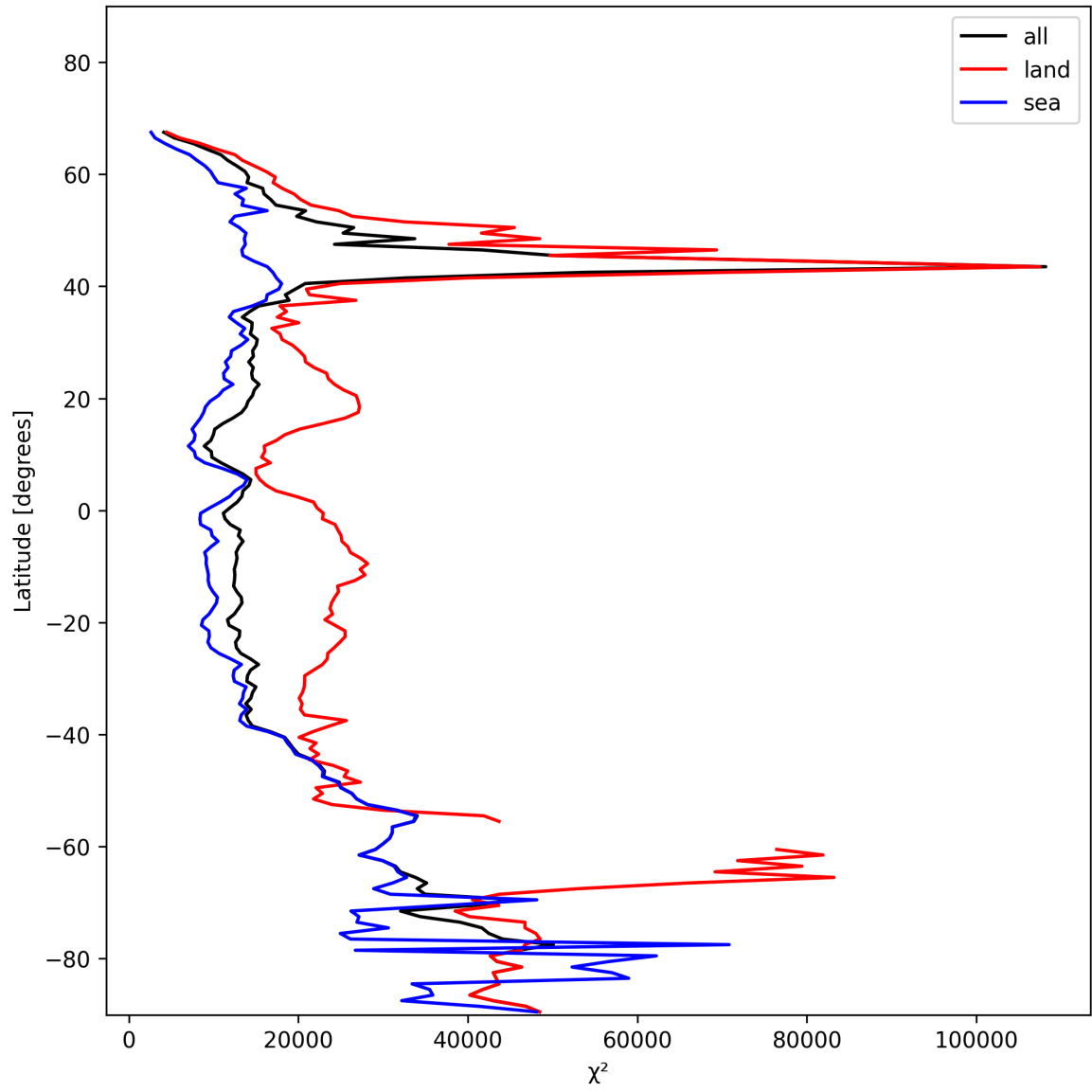
Figure 21: Zonal average of “ \chi^2 ” for 2025-01-15 to 2025-01-17.
