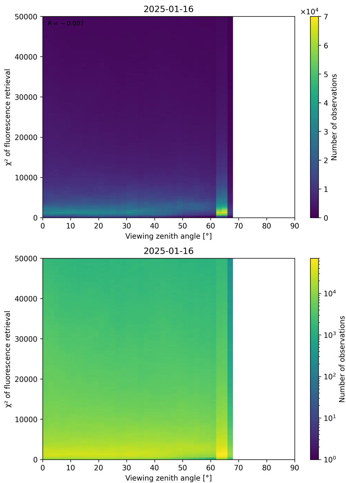
Figure 119: Scatter density plot of “Viewing zenith angle” against “ \chi^2 of fluorescence retrieval” for 2025-01-15 to 2025-01-17.
