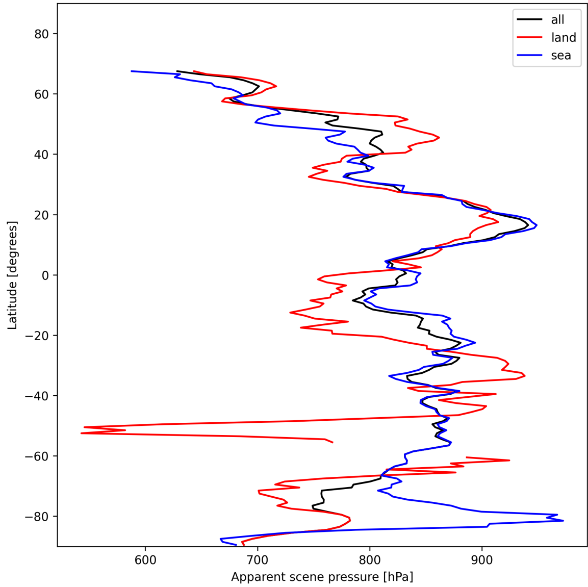
Figure 19: Zonal average of “Apparent scene pressure” for 2025-01-15 to 2025-01-17.
