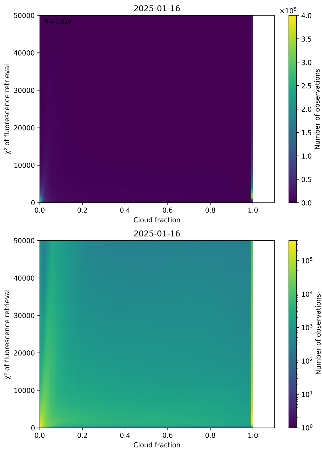
Figure 71: Scatter density plot of “Cloud fraction” against “ \chi^2 of fluorescence retrieval” for 2025-01-15 to 2025-01-17.
