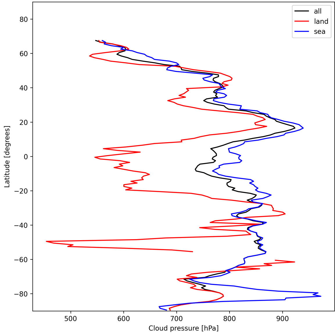
Figure 13: Zonal average of “Cloud pressure” for 2025-01-15 to 2025-01-17.
