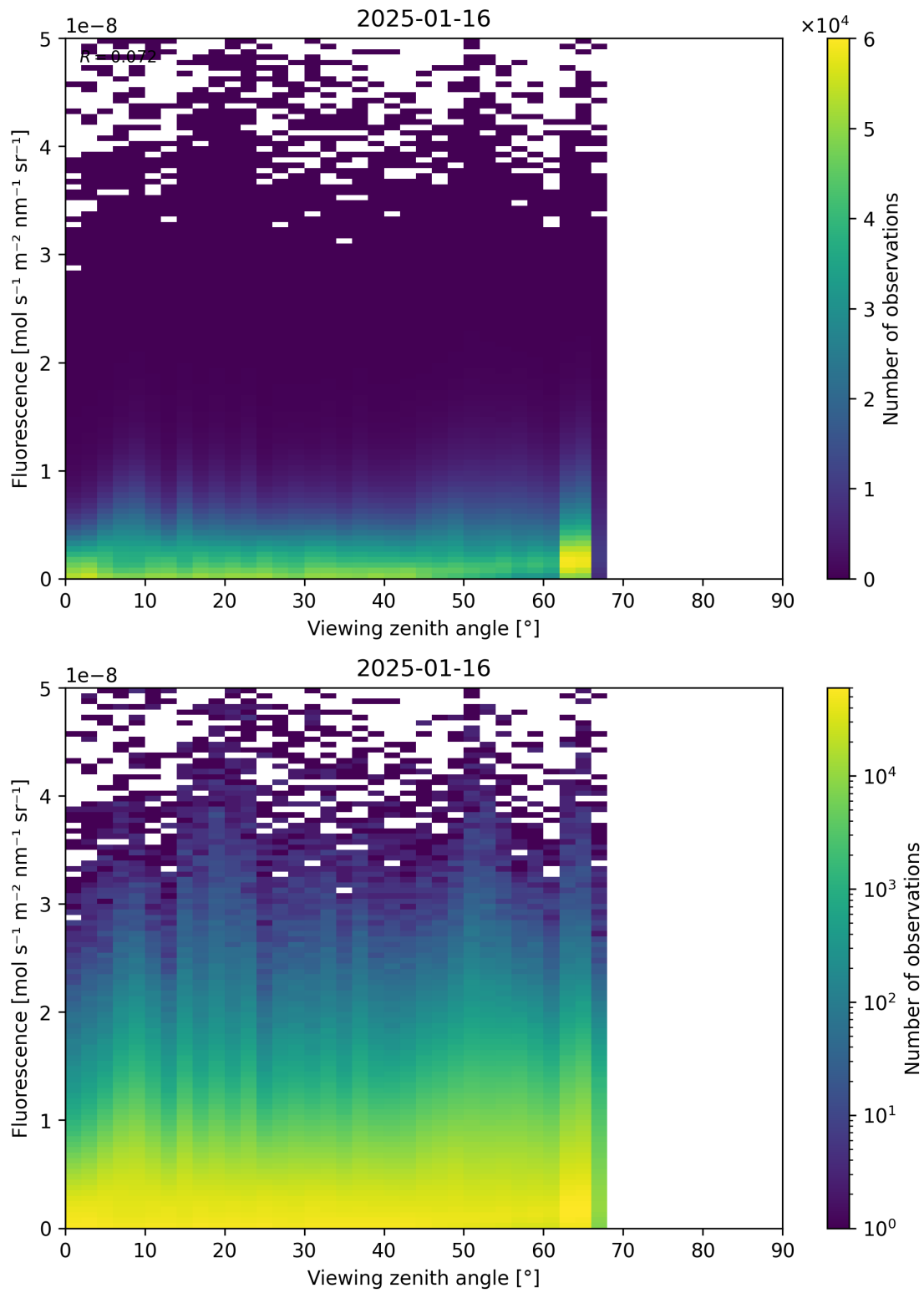
Figure 122: Scatter density plot of “Viewing zenith angle” against “Fluorescence” for 2025-01-15 to 2025-01-17.
