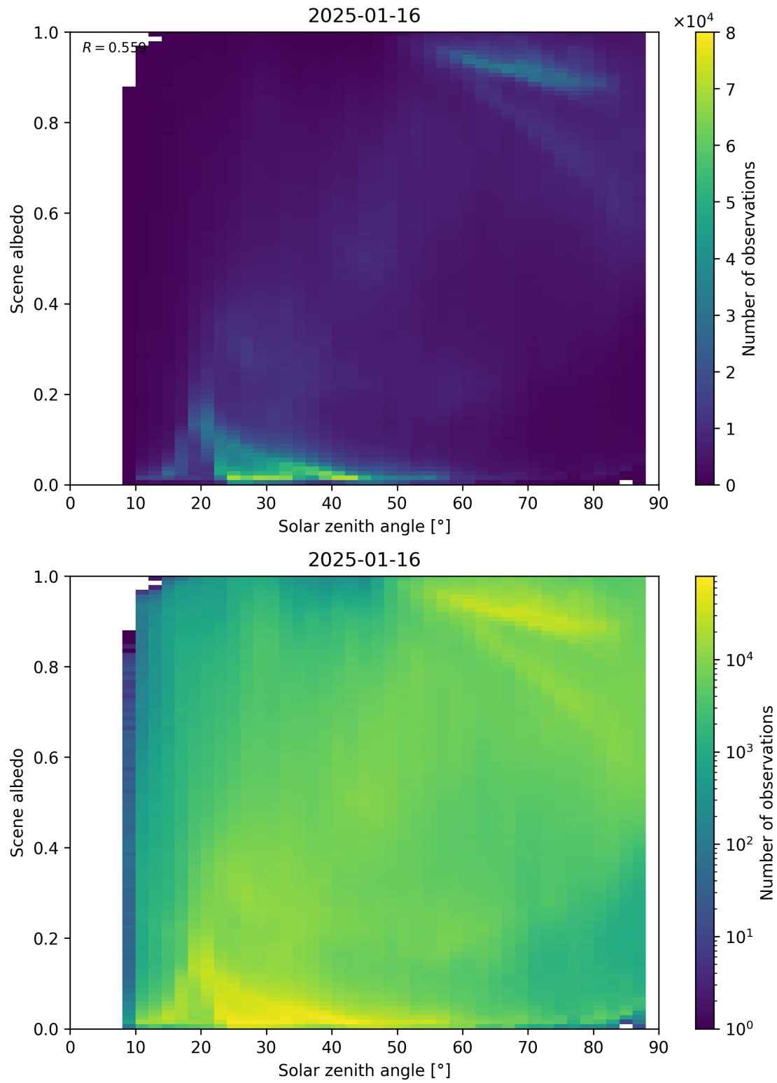
Figure 116: Scatter density plot of “Solar zenith angle” against “Scene albedo” for 2025-01-15 to 2025-01-17.
