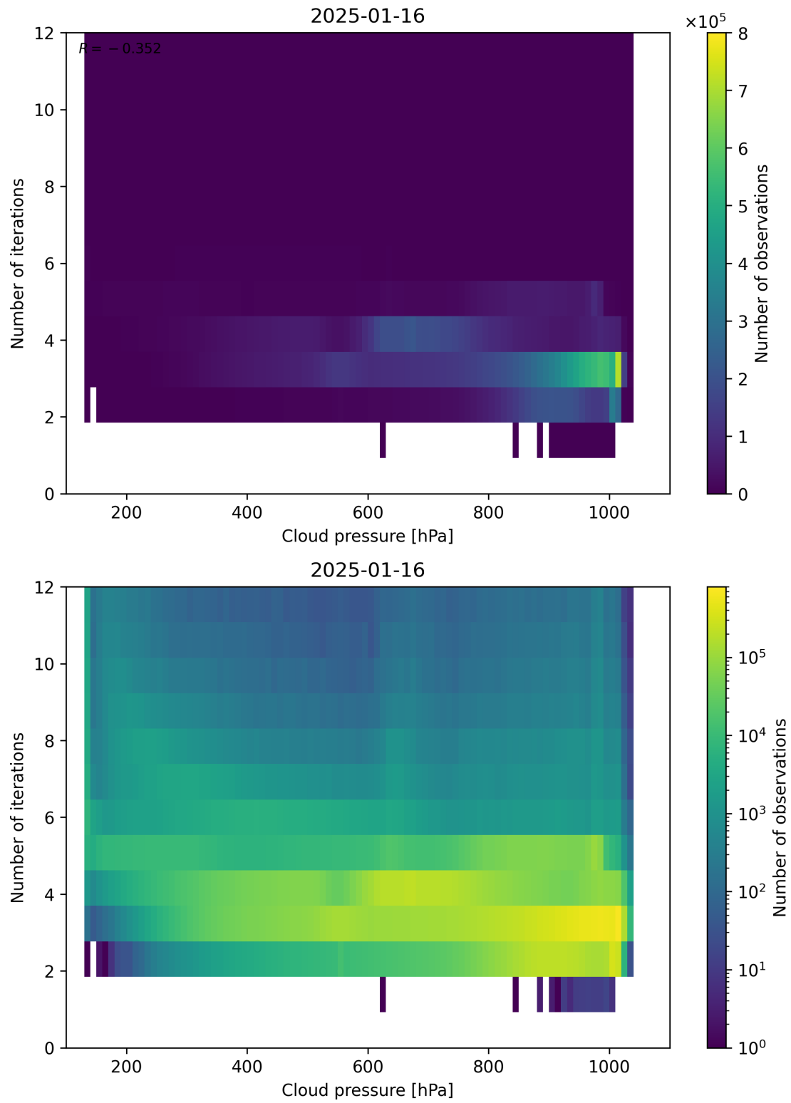
Figure 81: Scatter density plot of “Cloud pressure” against “Number of iterations” for 2025-01-15 to 2025-01-17.
