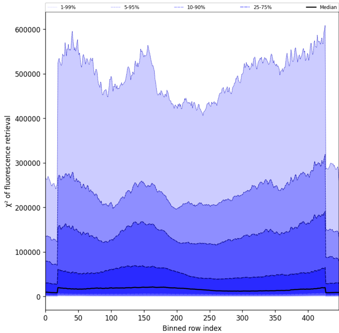
Figure 59: Along track statistics of “ \chi^2 of fluorescence retrieval” for 2025-01-15 to 2025-01-17
