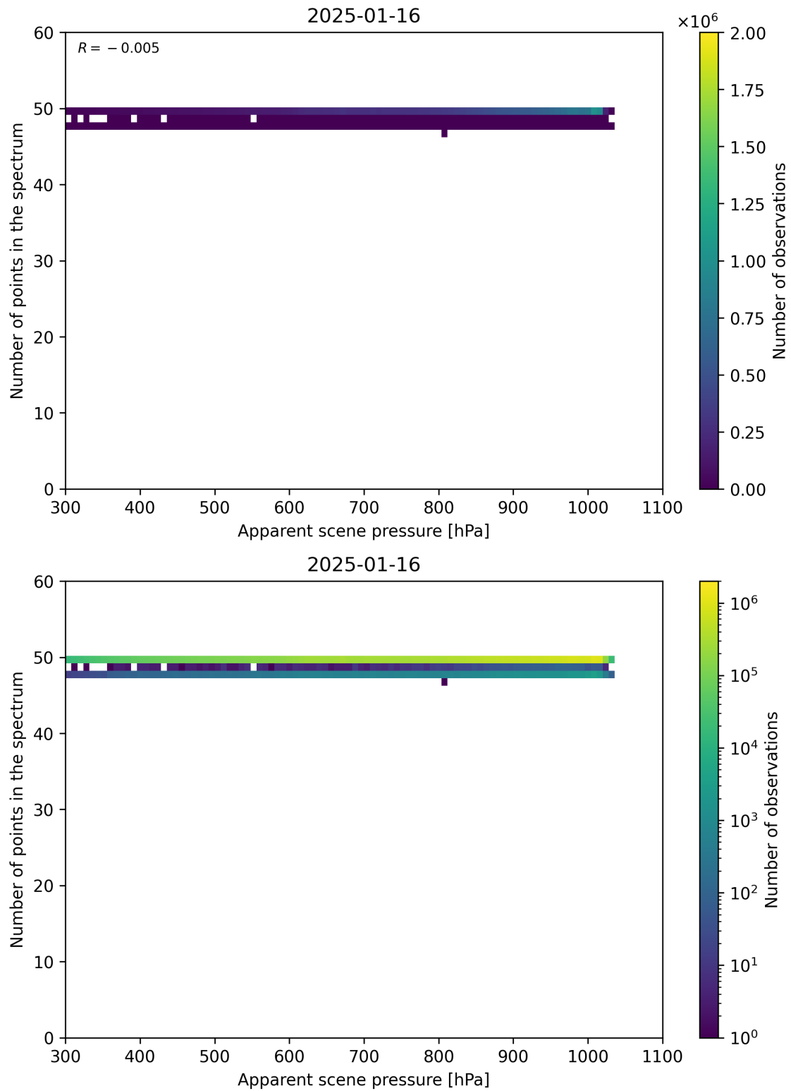
Figure 66: Scatter density plot of “Apparent scene pressure” against “Number of points in the spectrum” for 2025-01-15 to 2025-01-17.
