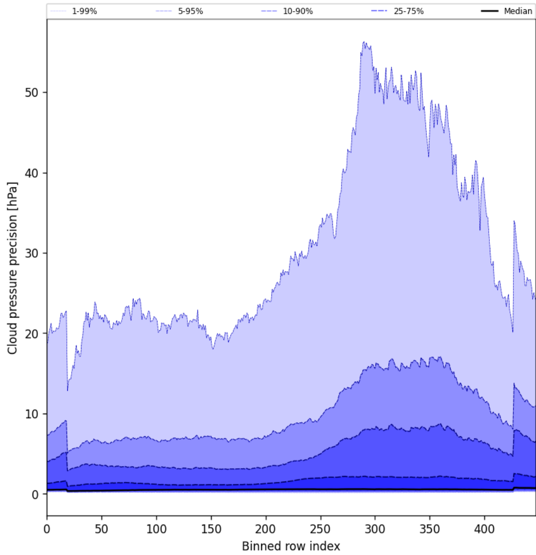
Figure 48: Along track statistics of “Cloud pressure precision” for 2025-01-15 to 2025-01-17
