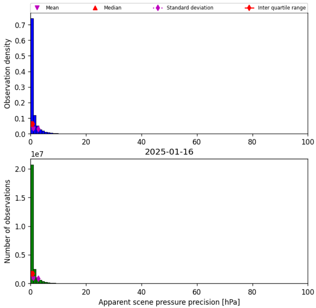
Figure 37: Histogram of “Apparent scene pressure precision” for 2025-01-15 to 2025-01-17
