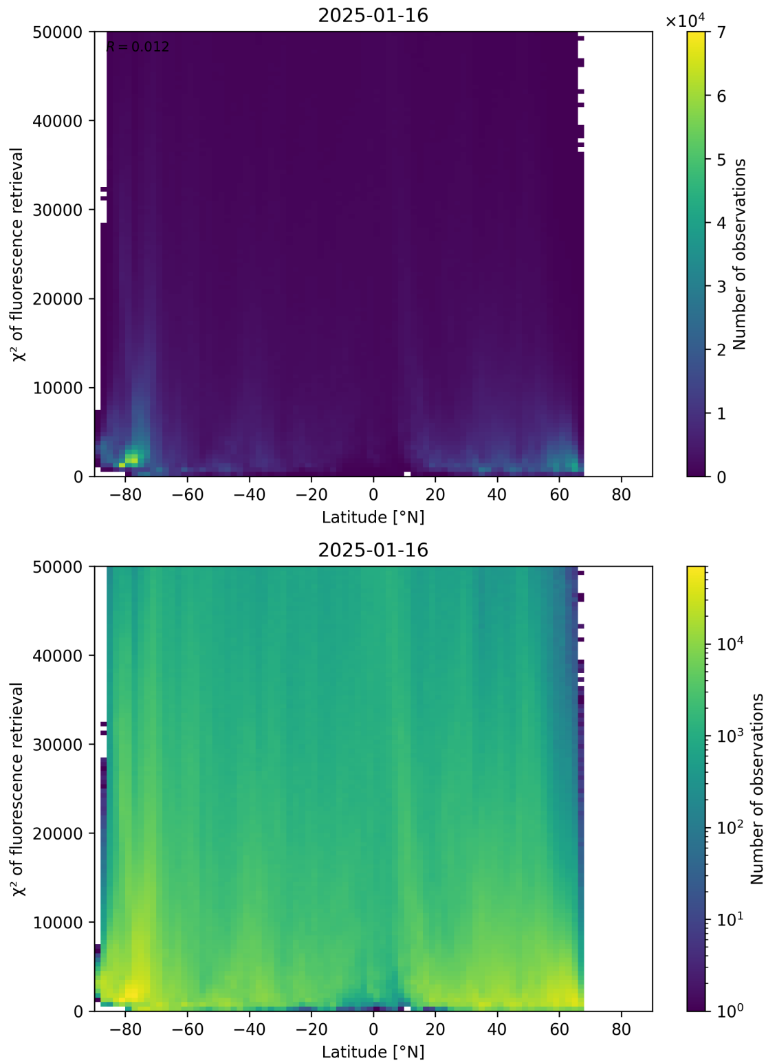
Figure 89: Scatter density plot of “Latitude” against “ \chi^2 of fluorescence retrieval” for 2025-01-15 to 2025-01-17.
