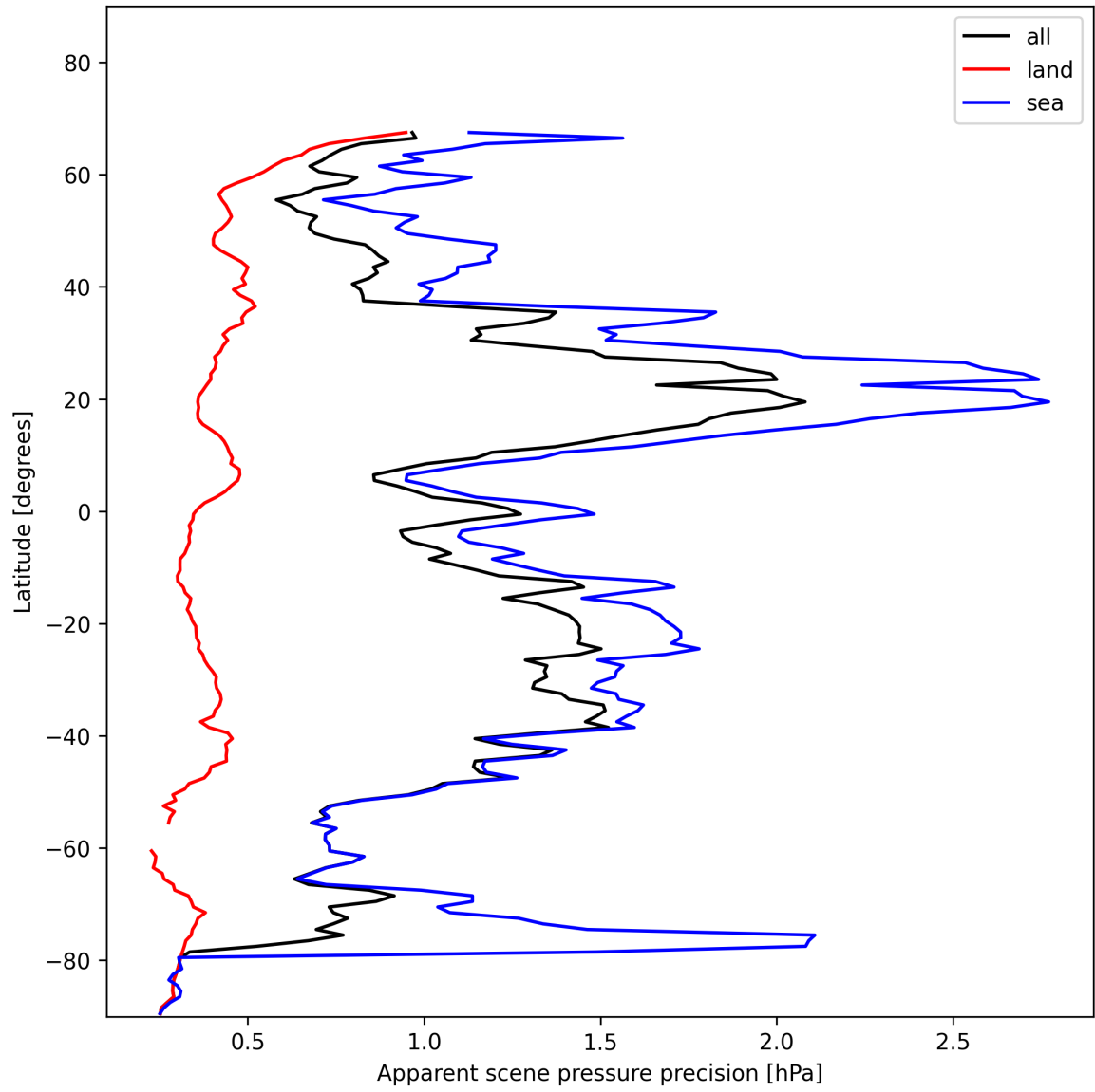
Figure 20: Zonal average of “Apparent scene pressure precision” for 2025-01-15 to 2025-01-17.
