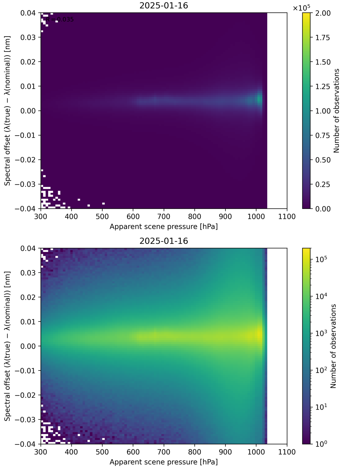
Figure 67: Scatter density plot of “Apparent scene pressure” against “Spectral offset ( \lambda_{\text{true}} - \lambda_{\text{nominal}} )” for 2025-01-15 to 2025-01-17.
