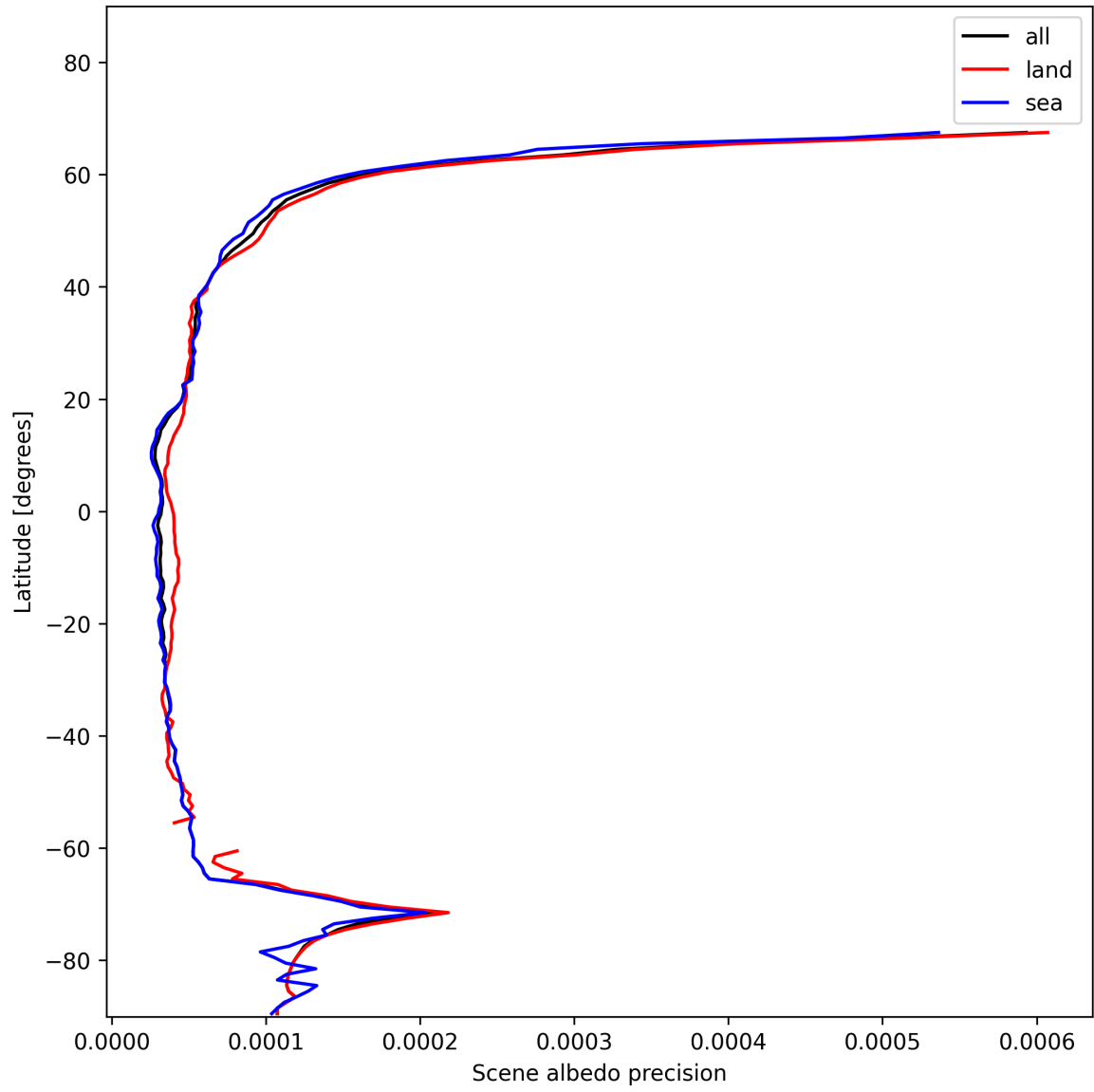
Figure 18: Zonal average of “Scene albedo precision” for 2025-01-15 to 2025-01-17.
