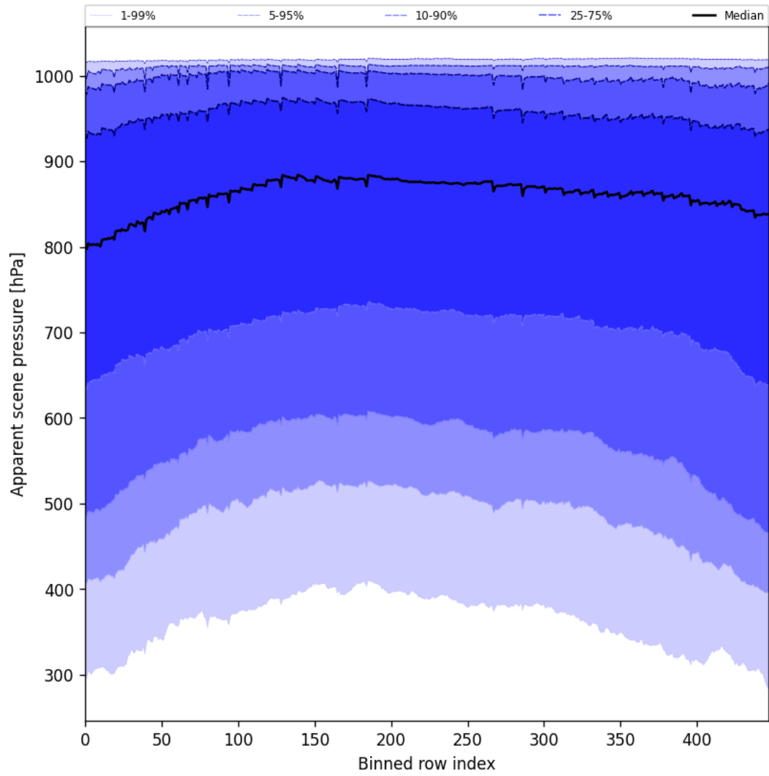
Figure 53: Along track statistics of “Apparent scene pressure” for 2025-01-15 to 2025-01-17
