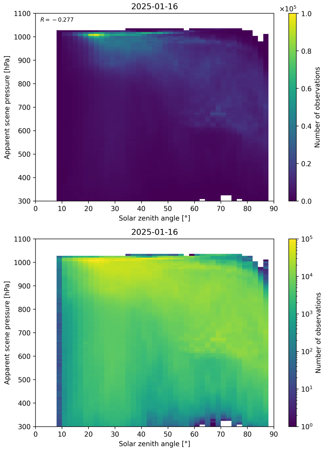
Figure 108: Scatter density plot of “Solar zenith angle” against “Apparent scene pressure” for 2025-01-15 to 2025-01-17.
