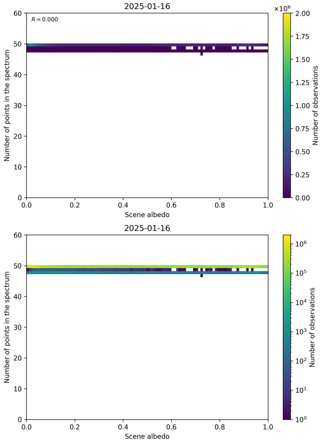
Figure 106: Scatter density plot of “Scene albedo” against “Number of points in the spectrum” for 2025-01-15 to 2025-01-17.
