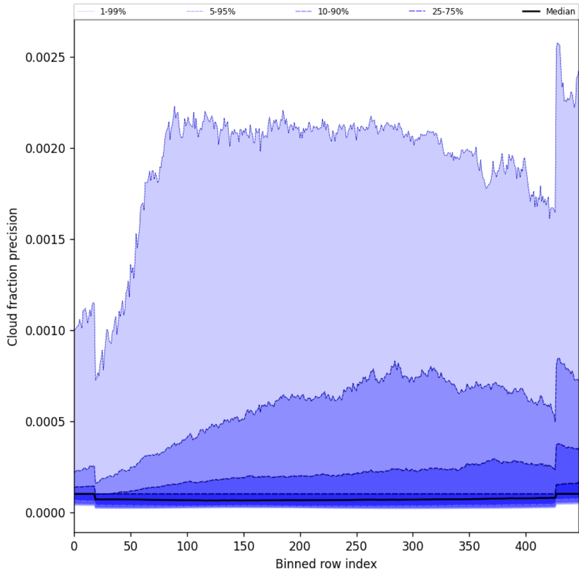
Figure 50: Along track statistics of “Cloud fraction precision” for 2025-01-15 to 2025-01-17
