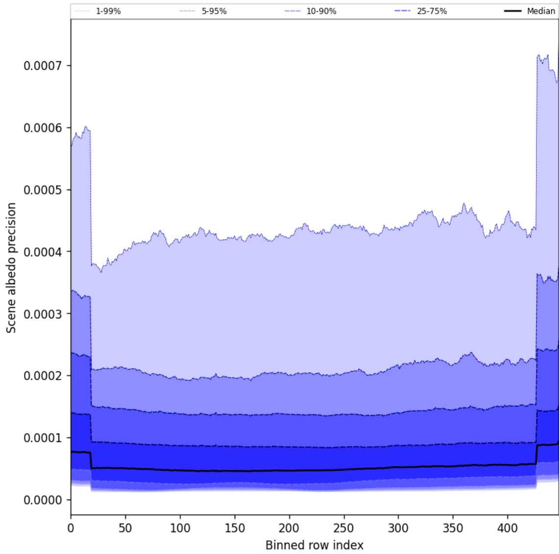
Figure 52: Along track statistics of “Scene albedo precision” for 2025-01-15 to 2025-01-17
