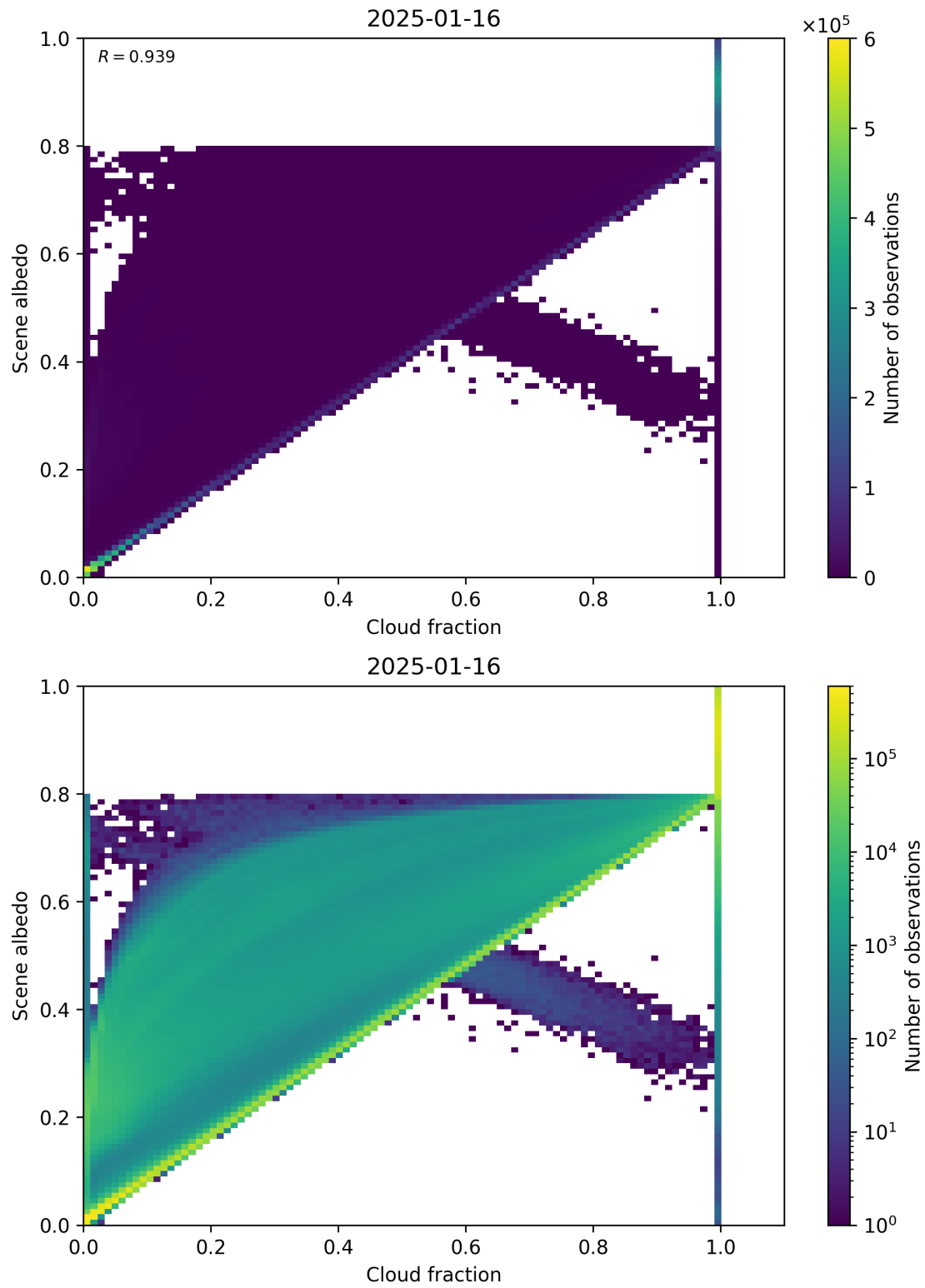
Figure 75: Scatter density plot of “Cloud fraction” against “Scene albedo” for 2025-01-15 to 2025-01-17.
