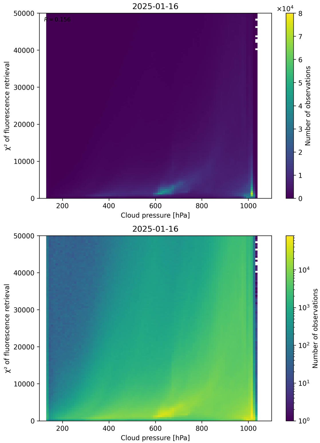
Figure 78: Scatter density plot of “Cloud pressure” against “ \chi^2 of fluorescence retrieval” for 2025-01-15 to 2025-01-17.
