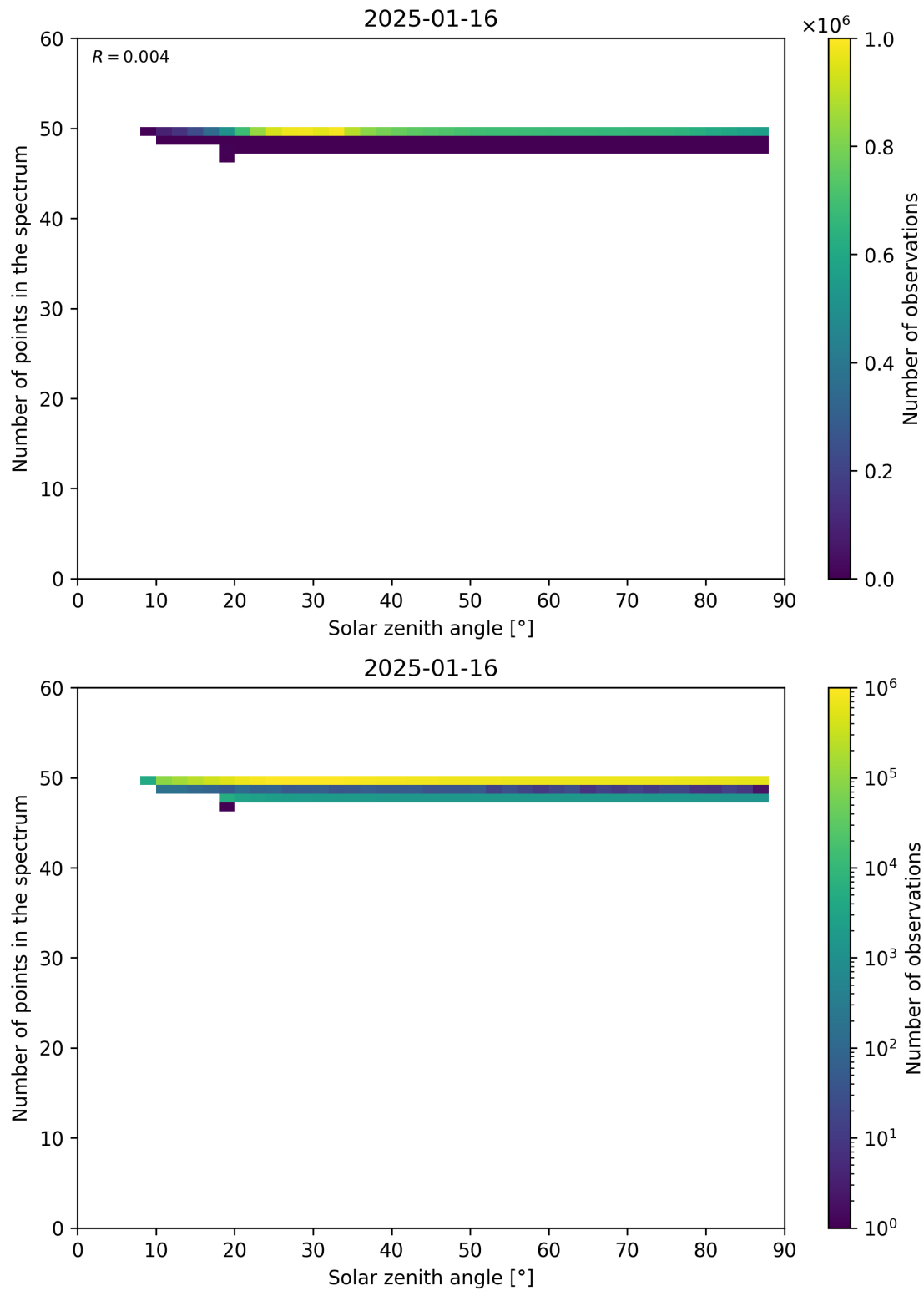
Figure 115: Scatter density plot of “Solar zenith angle” against “Number of points in the spectrum” for 2025-01-15 to 2025-01-17.
