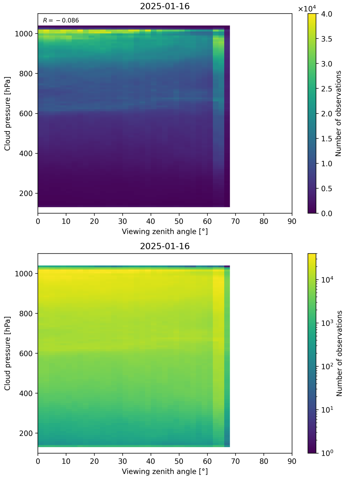
Figure 121: Scatter density plot of “Viewing zenith angle” against “Cloud pressure” for 2025-01-15 to 2025-01-17.
