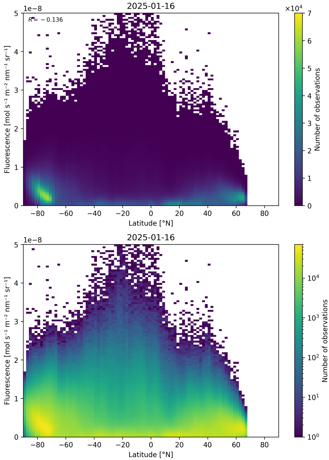
Figure 92: Scatter density plot of “Latitude” against “Fluorescence” for 2025-01-15 to 2025-01-17.
