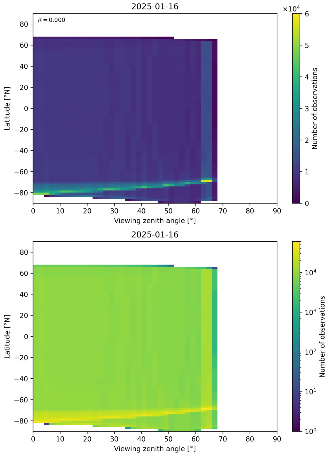
Figure 123: Scatter density plot of “Viewing zenith angle” against “Latitude” for 2025-01-15 to 2025-01-17.
