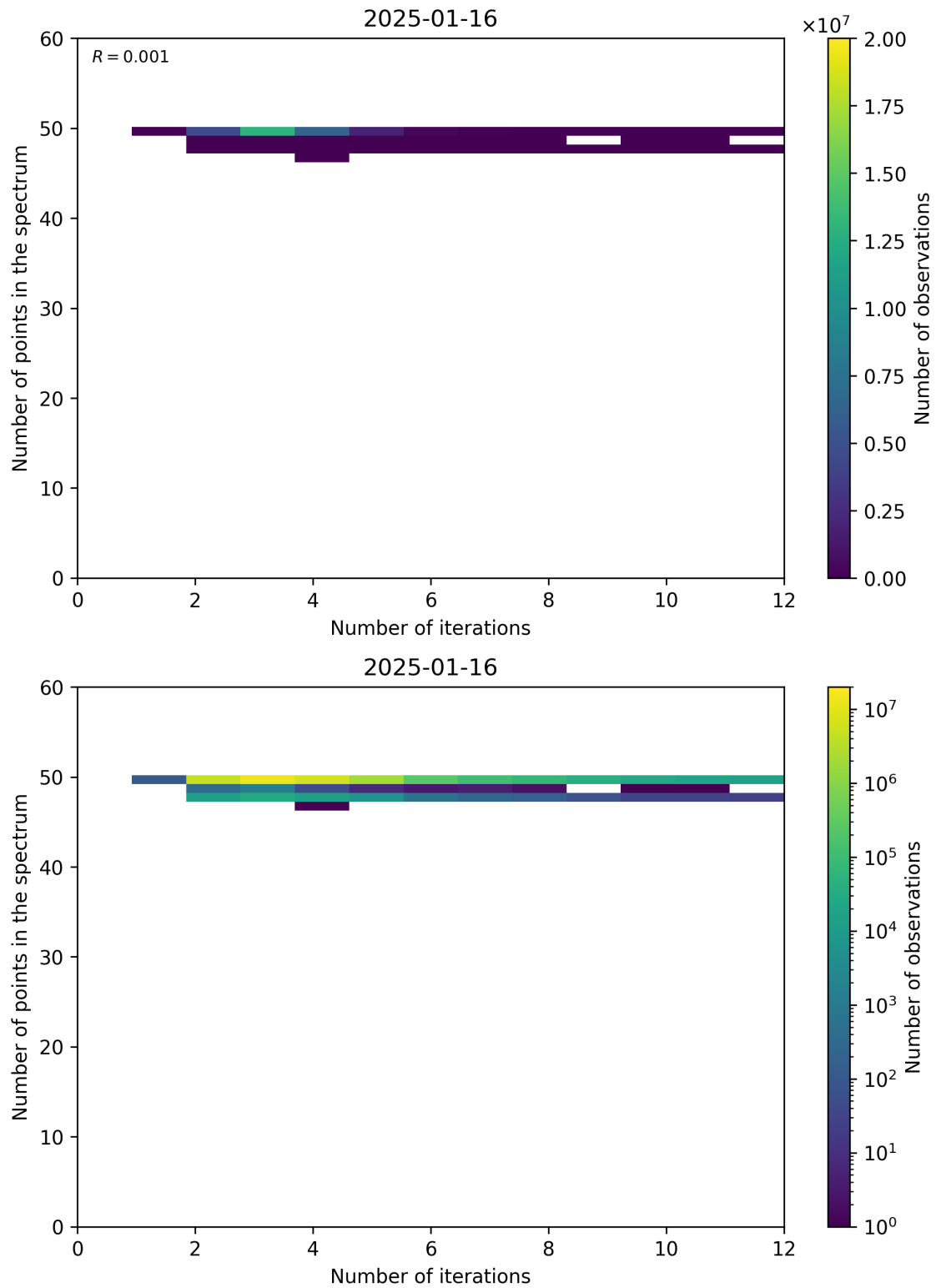
Figure 99: Scatter density plot of “Number of iterations” against “Number of points in the spectrum” for 2025-01-15 to 2025-01-17.
