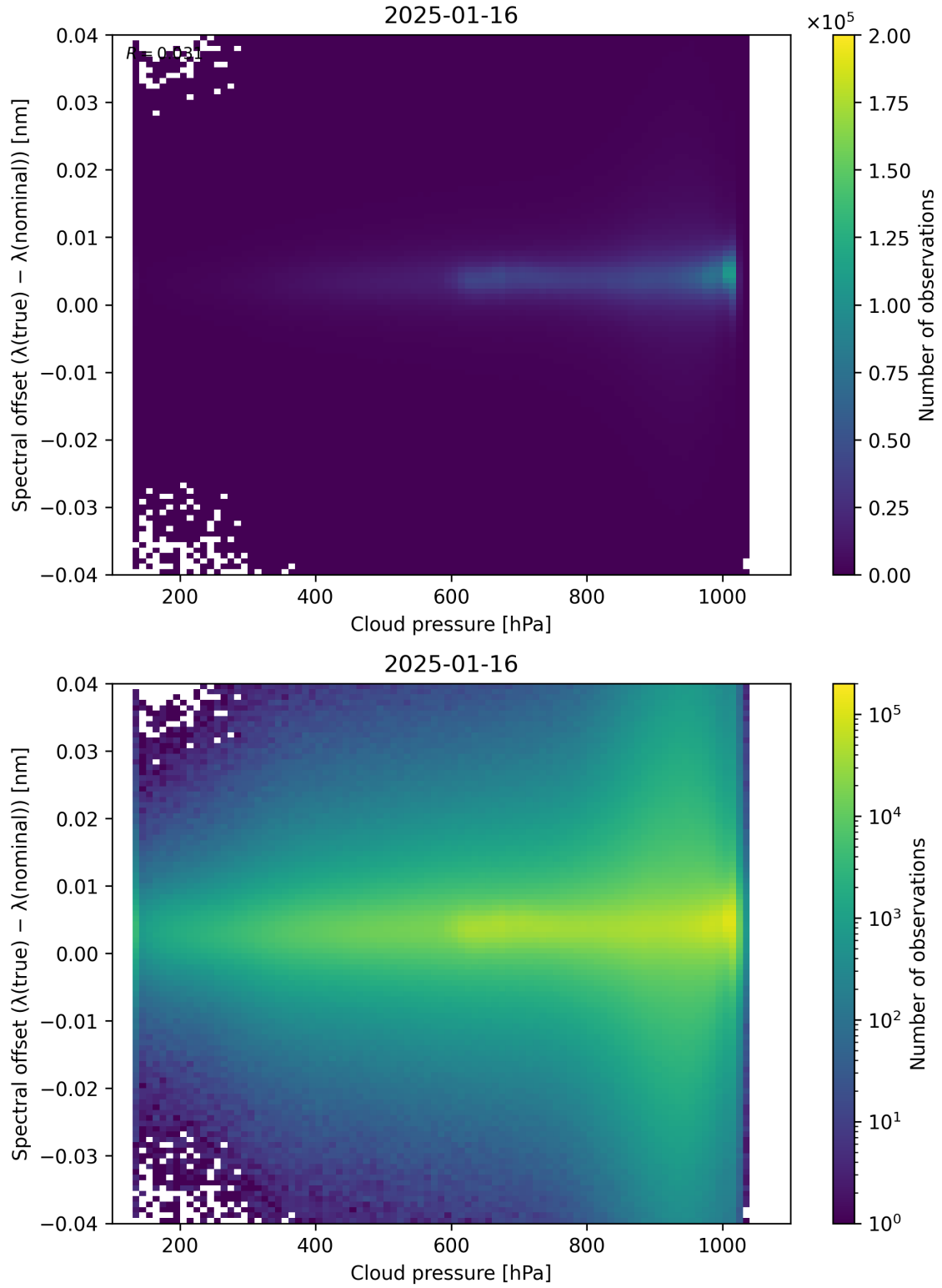
Figure 84: Scatter density plot of “Cloud pressure” against “Spectral offset ( \lambda_{\text{true}} - \lambda_{\text{nominal}} )” for 2025-01-15 to 2025-01-17.
