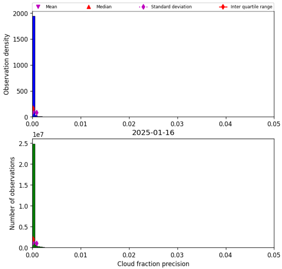
Figure 33: Histogram of “Cloud fraction precision” for 2025-01-15 to 2025-01-17
