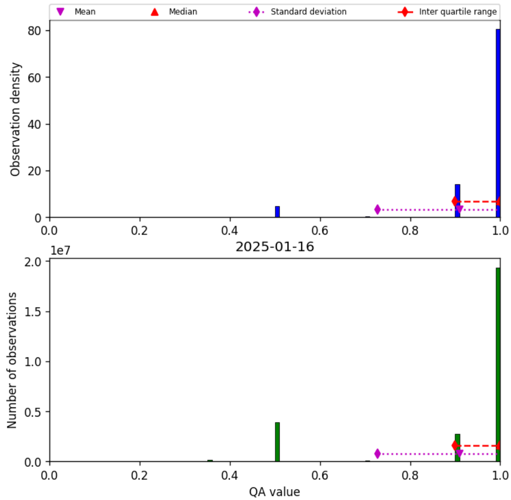
Figure 29: Histogram of “QA value” for 2025-01-15 to 2025-01-17
