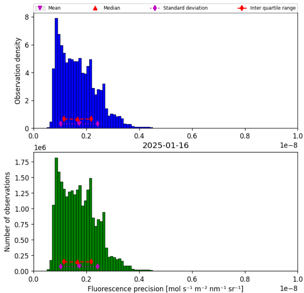
Figure 41: Histogram of “Fluorescence precision” for 2025-01-15 to 2025-01-17
