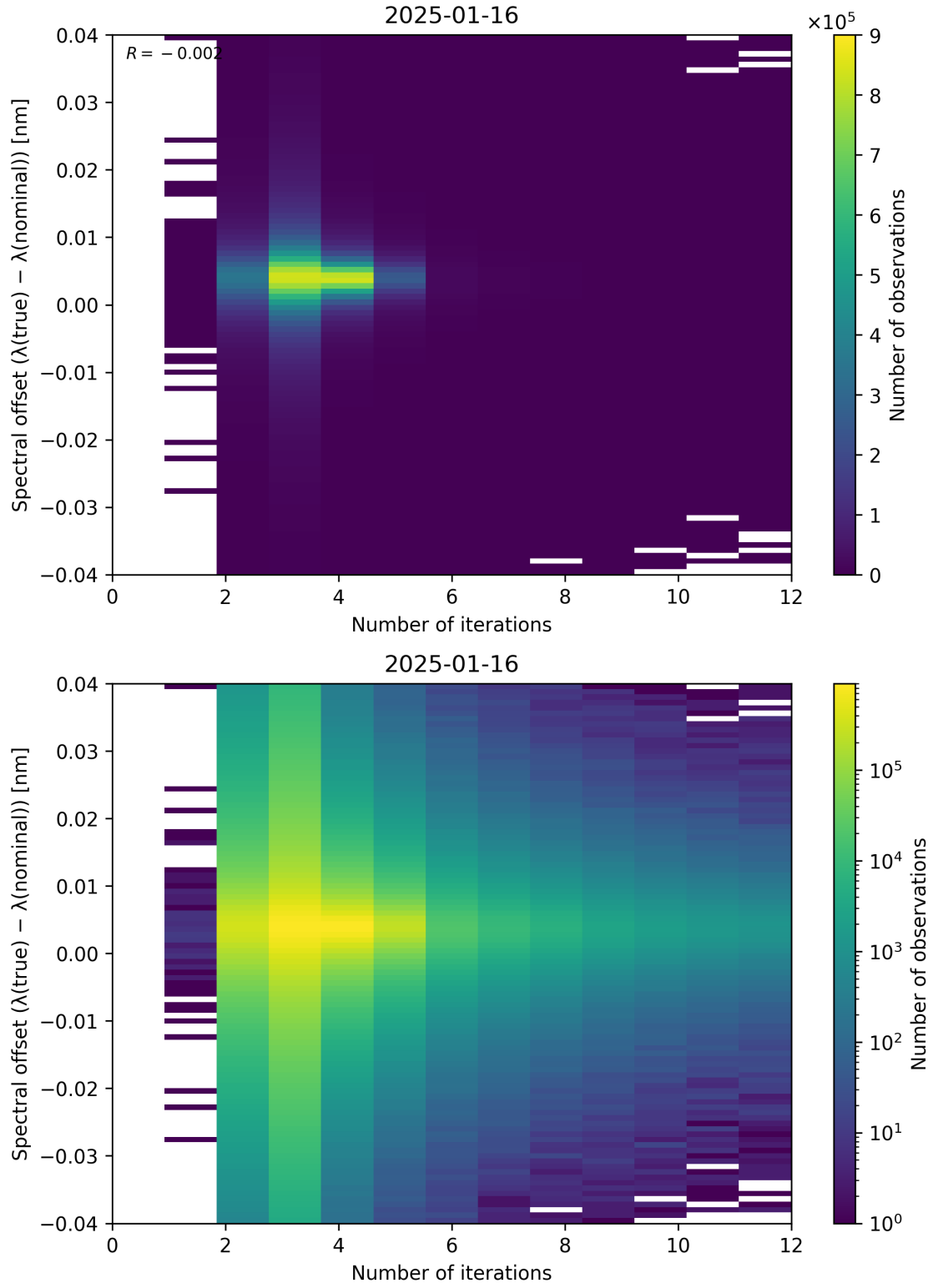
Figure 100: Scatter density plot of “Number of iterations” against “Spectral offset ( \lambda_{\text{true}} - \lambda_{\text{nominal}} )” for 2025-01-15 to 2025-01-17.
