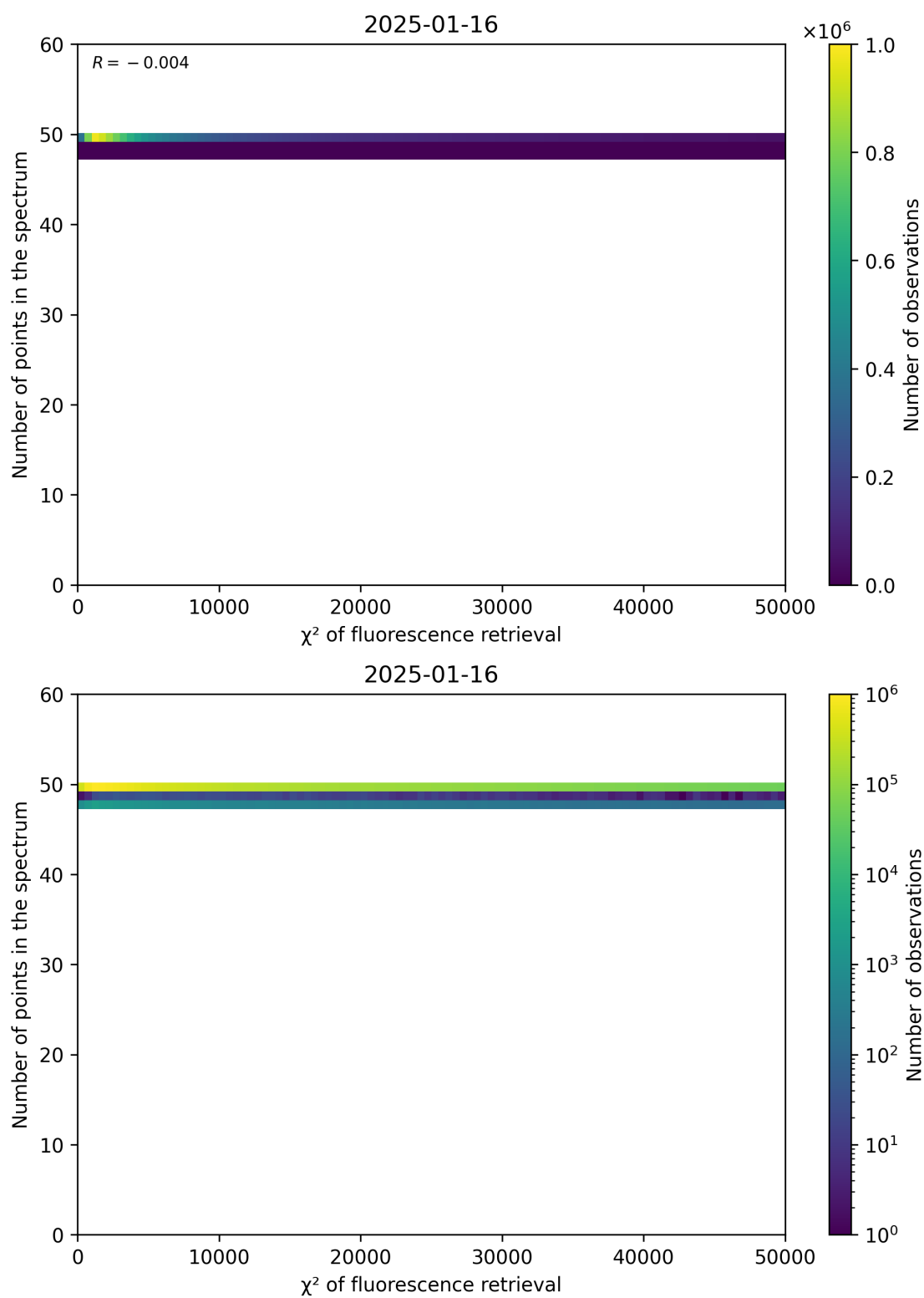
Figure 68: Scatter density plot of “ \chi^2 of fluorescence retrieval” against “Number of points in the spectrum” for 2025-01-15 to 2025-01-17.
