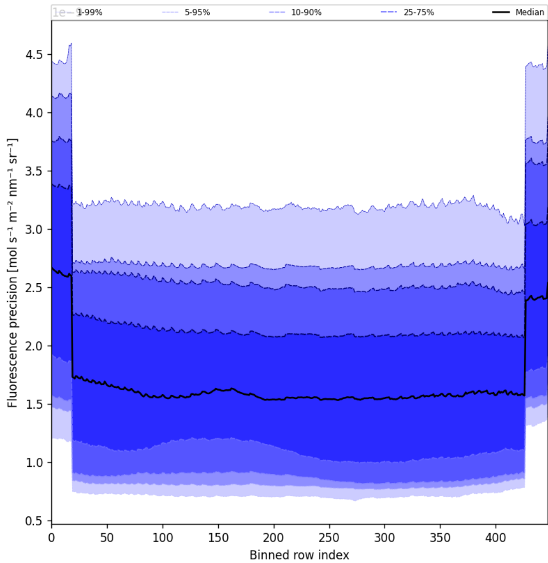
Figure 58: Along track statistics of “Fluorescence precision” for 2025-01-15 to 2025-01-17
