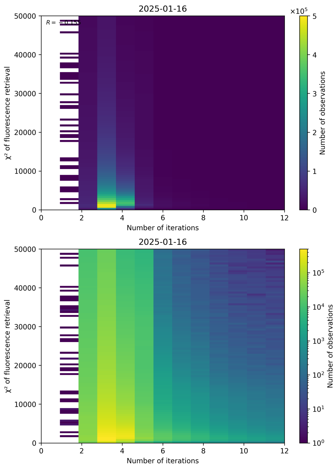
Figure 97: Scatter density plot of “Number of iterations” against “ \chi^2 of fluorescence retrieval” for 2025-01-15 to 2025-01-17.
