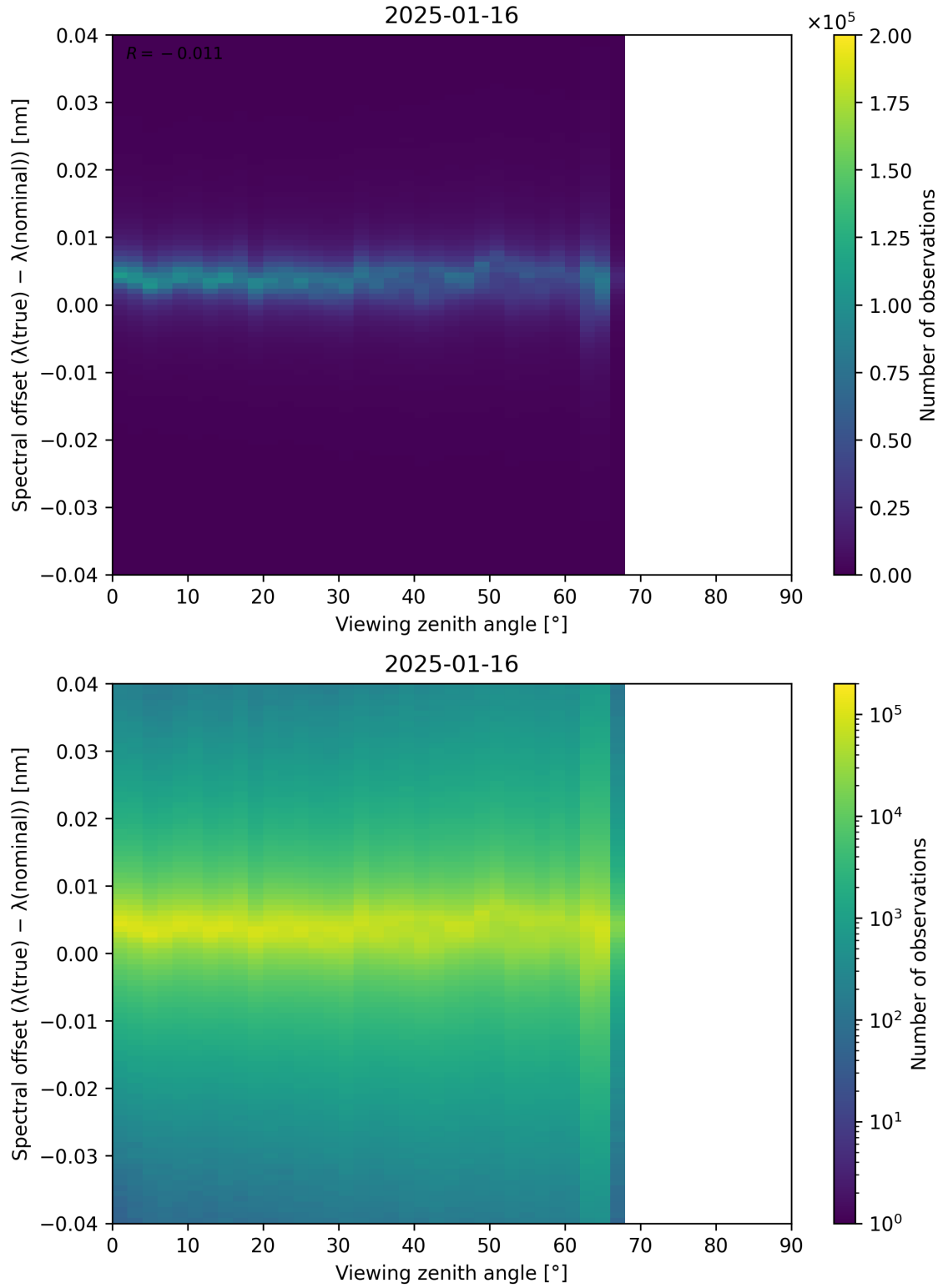
Figure 128: Scatter density plot of “Viewing zenith angle” against “Spectral offset ( \lambda_{\text{true}} - \lambda_{\text{nominal}} )” for 2025-01-15 to 2025-01-17.
