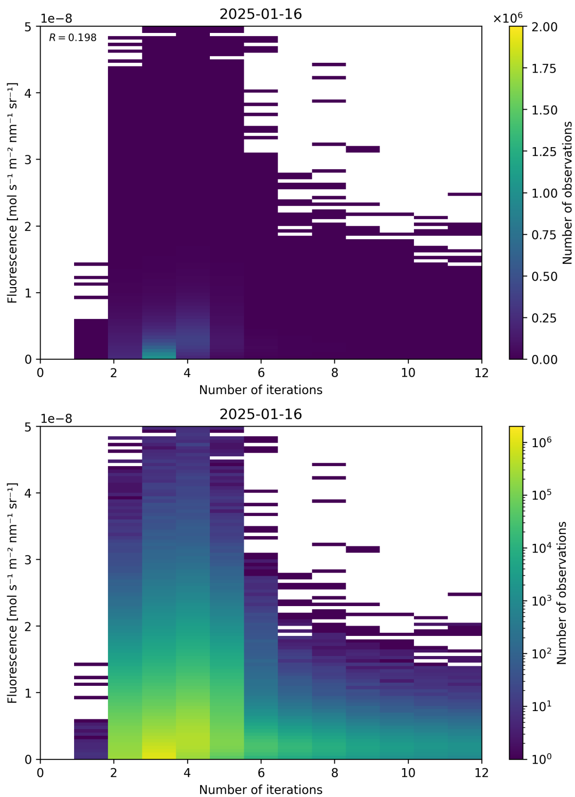
Figure 98: Scatter density plot of “Number of iterations” against “Fluorescence” for 2025-01-15 to 2025-01-17.
