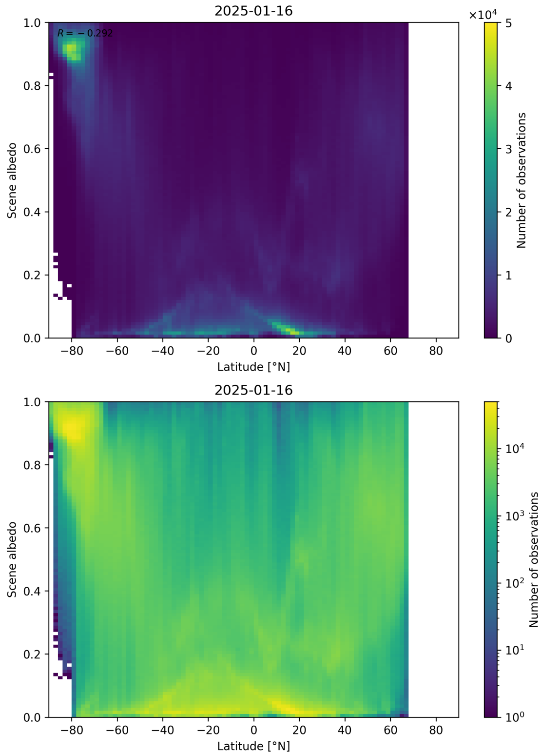
Figure 95: Scatter density plot of “Latitude” against “Scene albedo” for 2025-01-15 to 2025-01-17.
