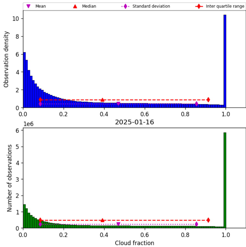
Figure 32: Histogram of “Cloud fraction” for 2025-01-15 to 2025-01-17
