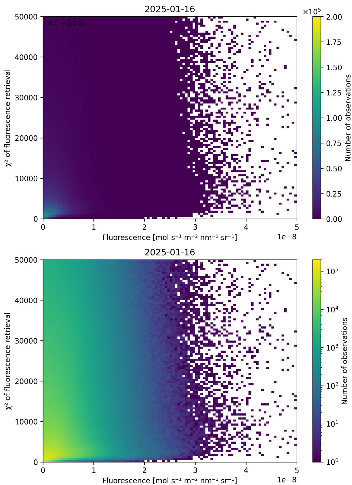
Figure 85: Scatter density plot of “Fluorescence” against “ \chi^2 of fluorescence retrieval” for 2025-01-15 to 2025-01-17.
