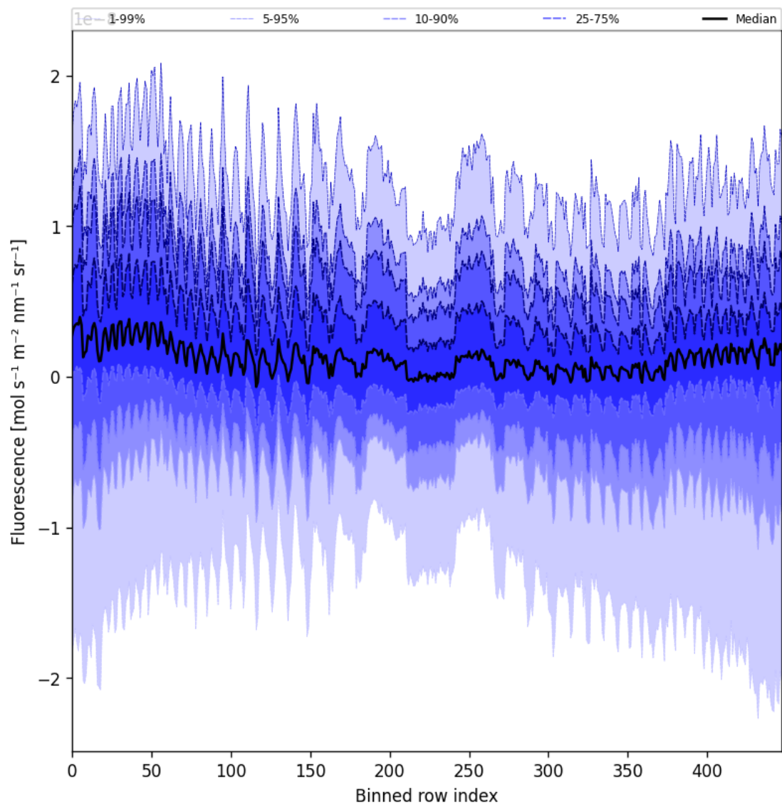
Figure 57: Along track statistics of “Fluorescence” for 2025-01-15 to 2025-01-17
