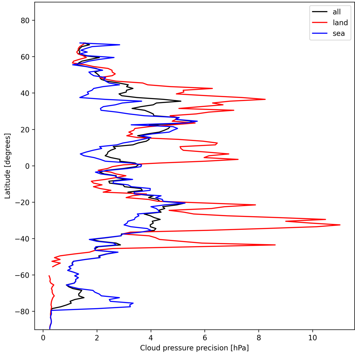
Figure 14: Zonal average of “Cloud pressure precision” for 2025-01-15 to 2025-01-17.
