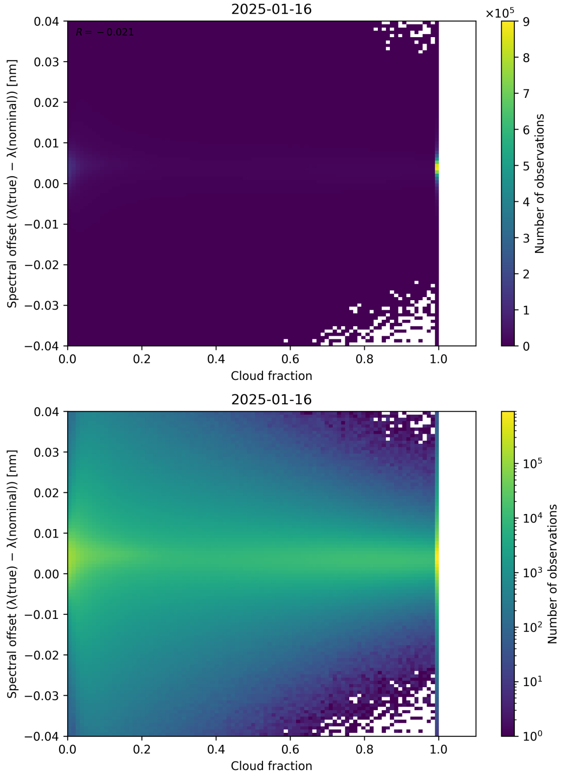
Figure 76: Scatter density plot of “Cloud fraction” against “Spectral offset ( \lambda_{\text{true}} - \lambda_{\text{nominal}} )” for 2025-01-15 to 2025-01-17.
