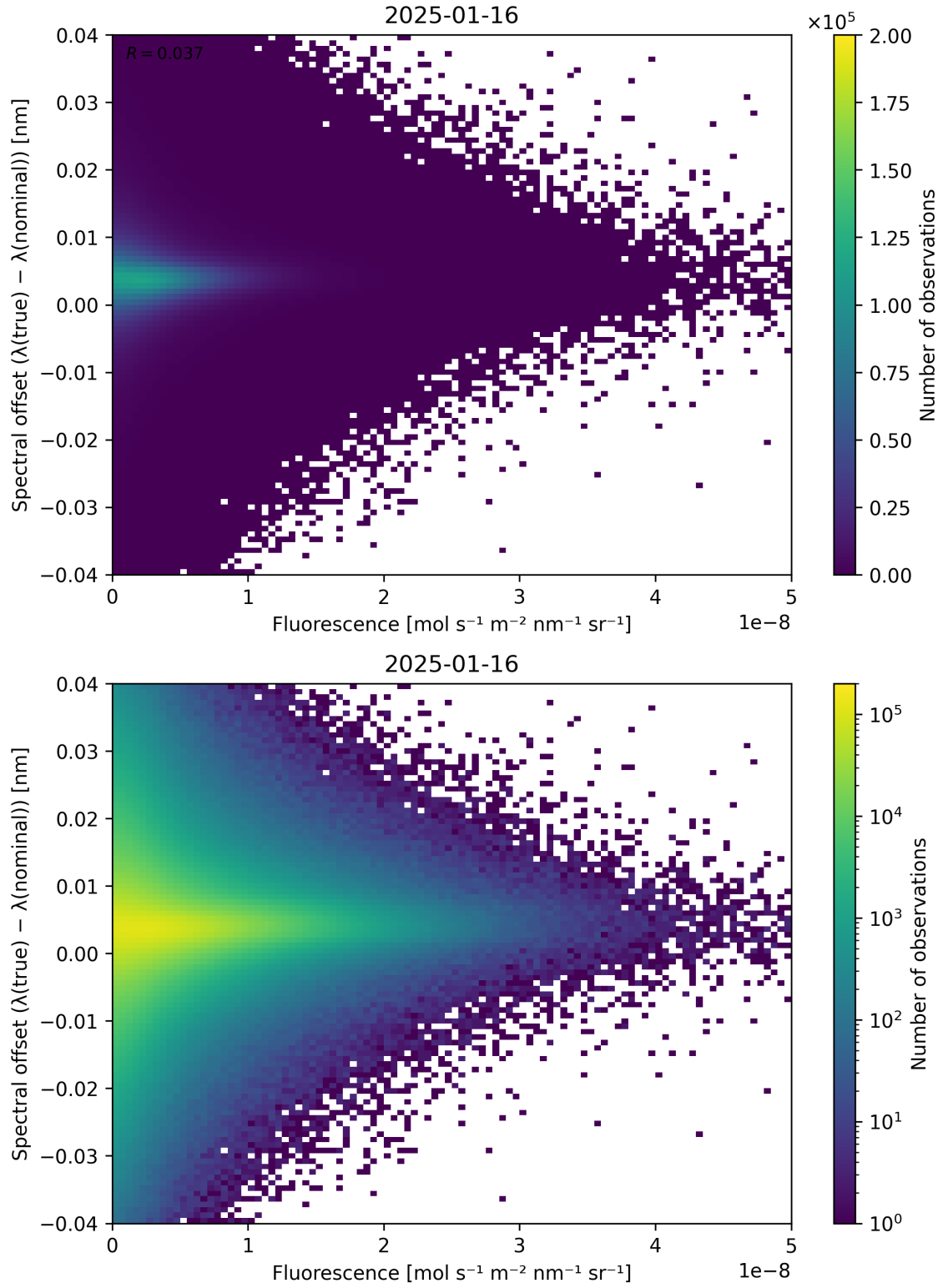
Figure 87: Scatter density plot of “Fluorescence” against “Spectral offset ( \lambda_{\text{true}} - \lambda_{\text{nominal}} )” for 2025-01-15 to 2025-01-17.
