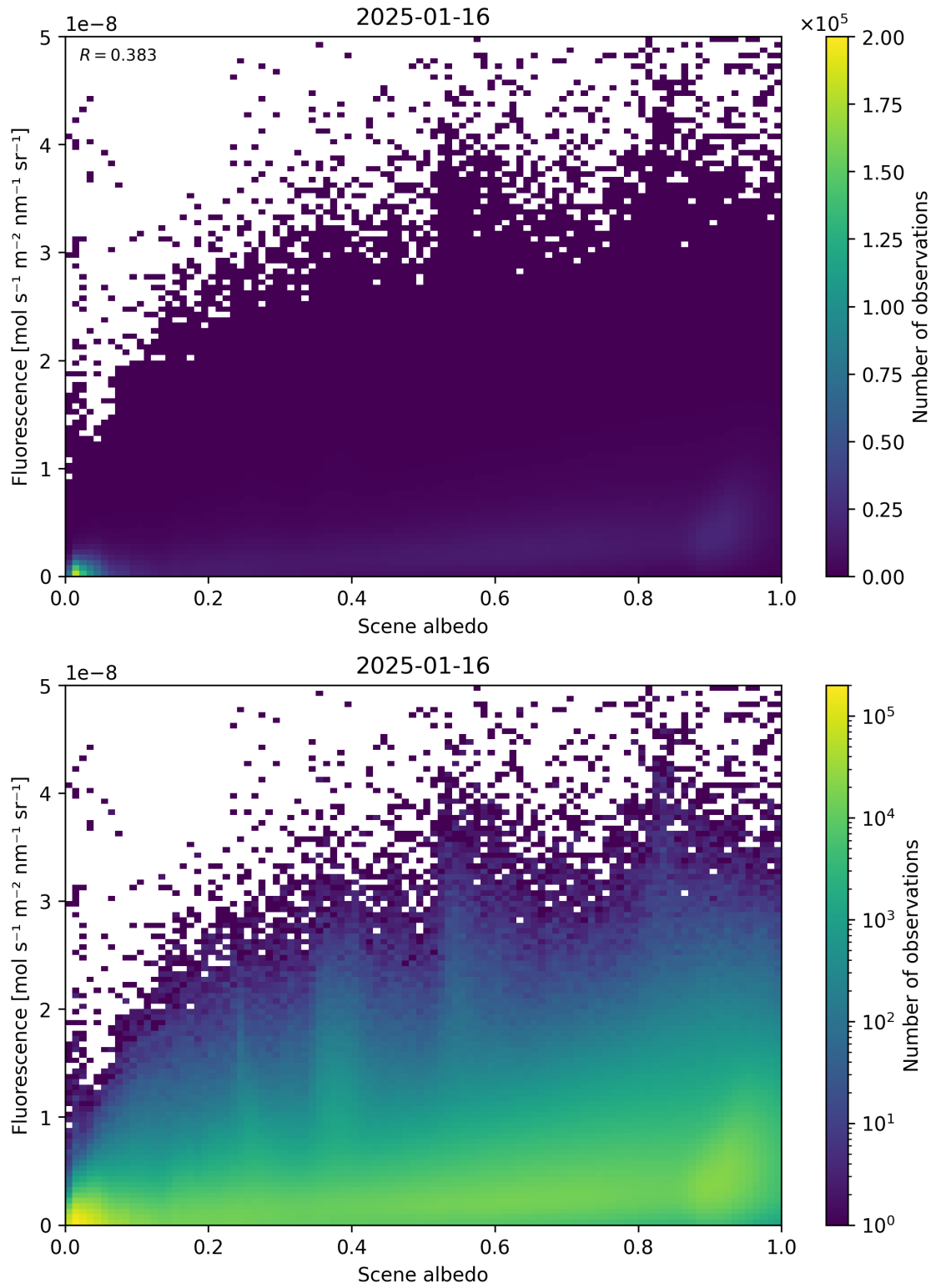
Figure 104: Scatter density plot of “Scene albedo” against “Fluorescence” for 2025-01-15 to 2025-01-17.
