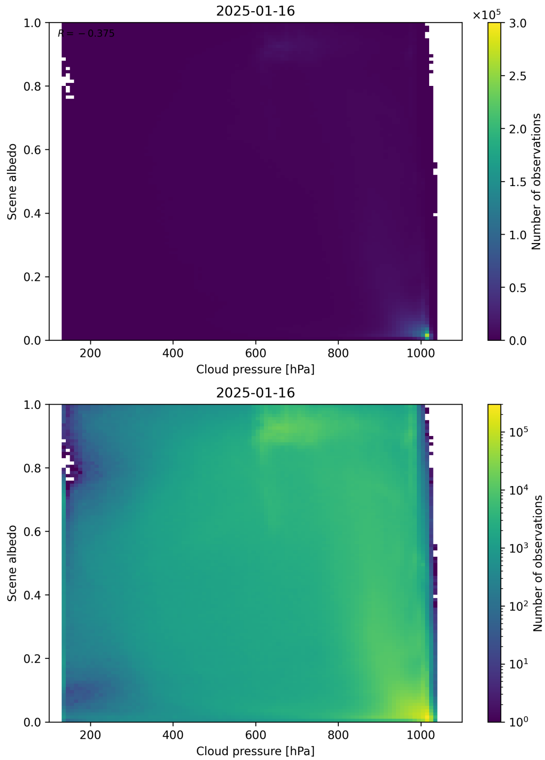
Figure 83: Scatter density plot of “Cloud pressure” against “Scene albedo” for 2025-01-15 to 2025-01-17.
