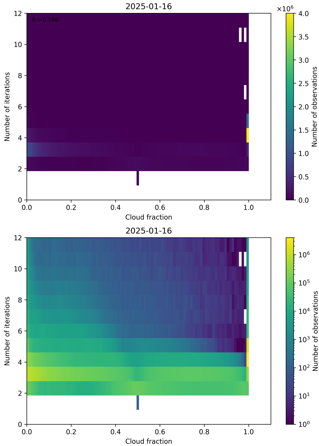
Figure 73: Scatter density plot of “Cloud fraction” against “Number of iterations” for 2025-01-15 to 2025-01-17.
