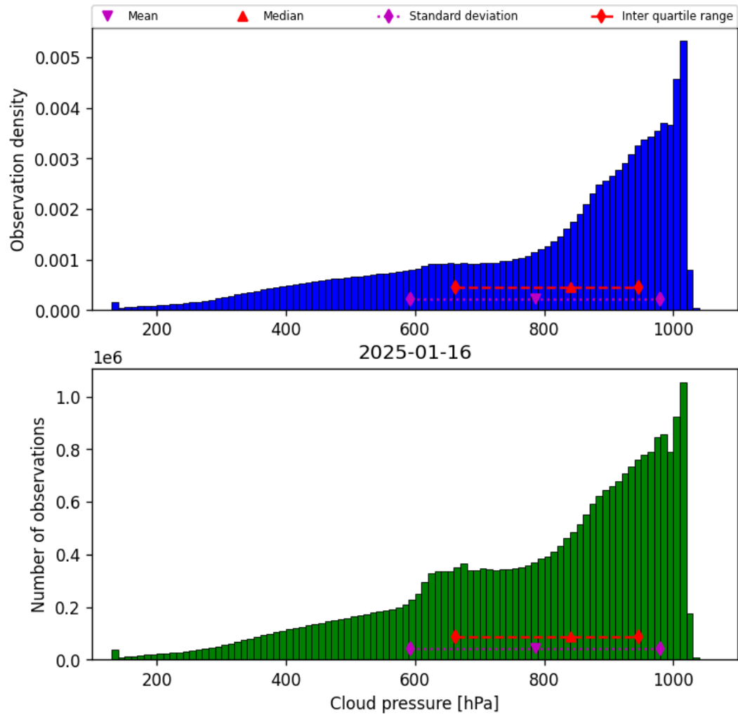
Figure 30: Histogram of “Cloud pressure” for 2025-01-15 to 2025-01-17
