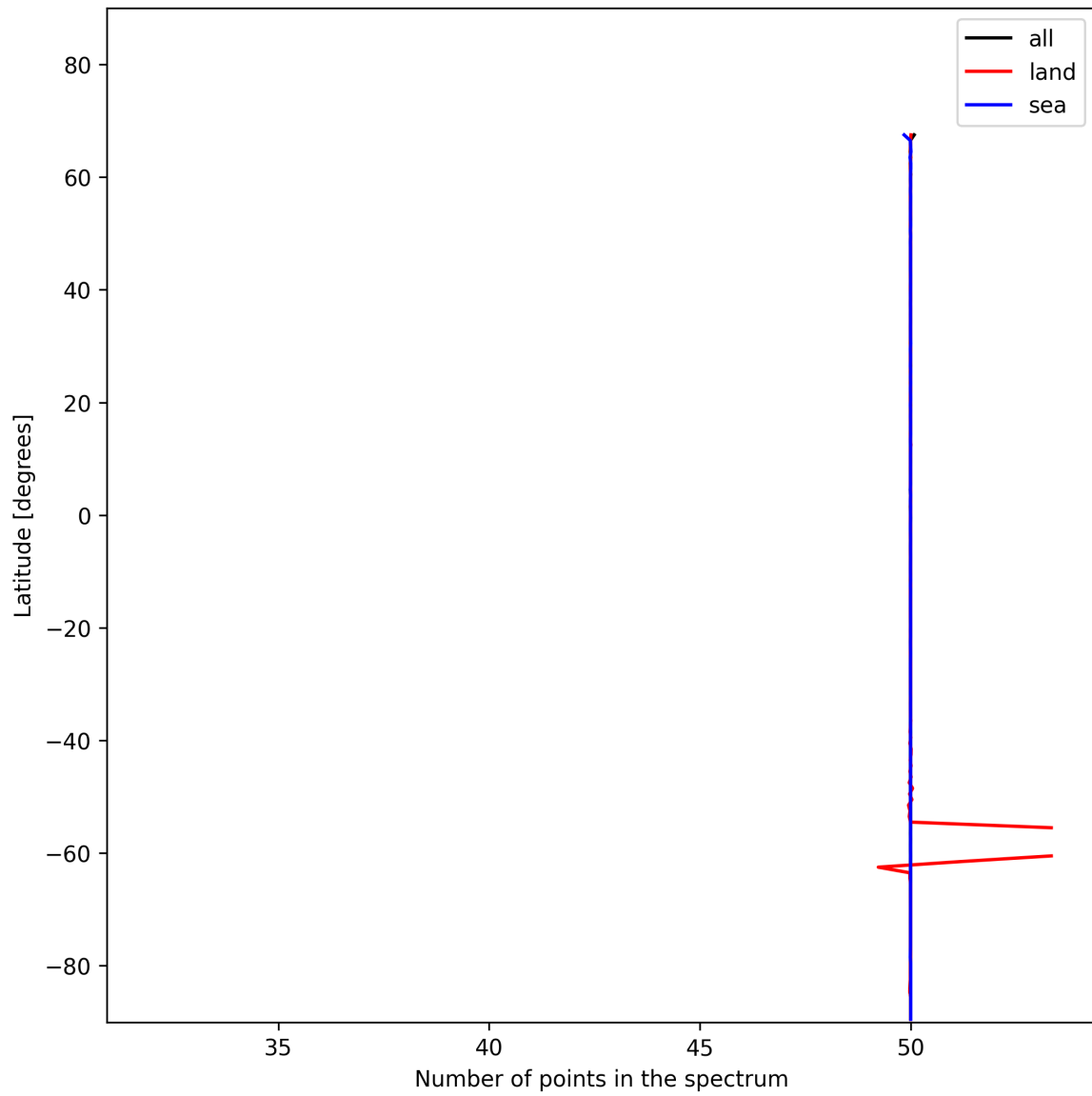
Figure 27: Zonal average of “Number of points in the spectrum” for 2025-01-15 to 2025-01-17.
