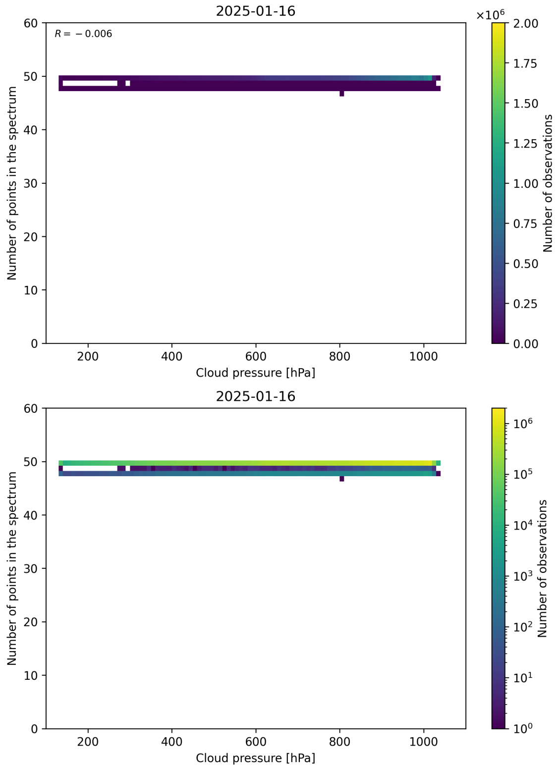
Figure 82: Scatter density plot of “Cloud pressure” against “Number of points in the spectrum” for 2025-01-15 to 2025-01-17.
