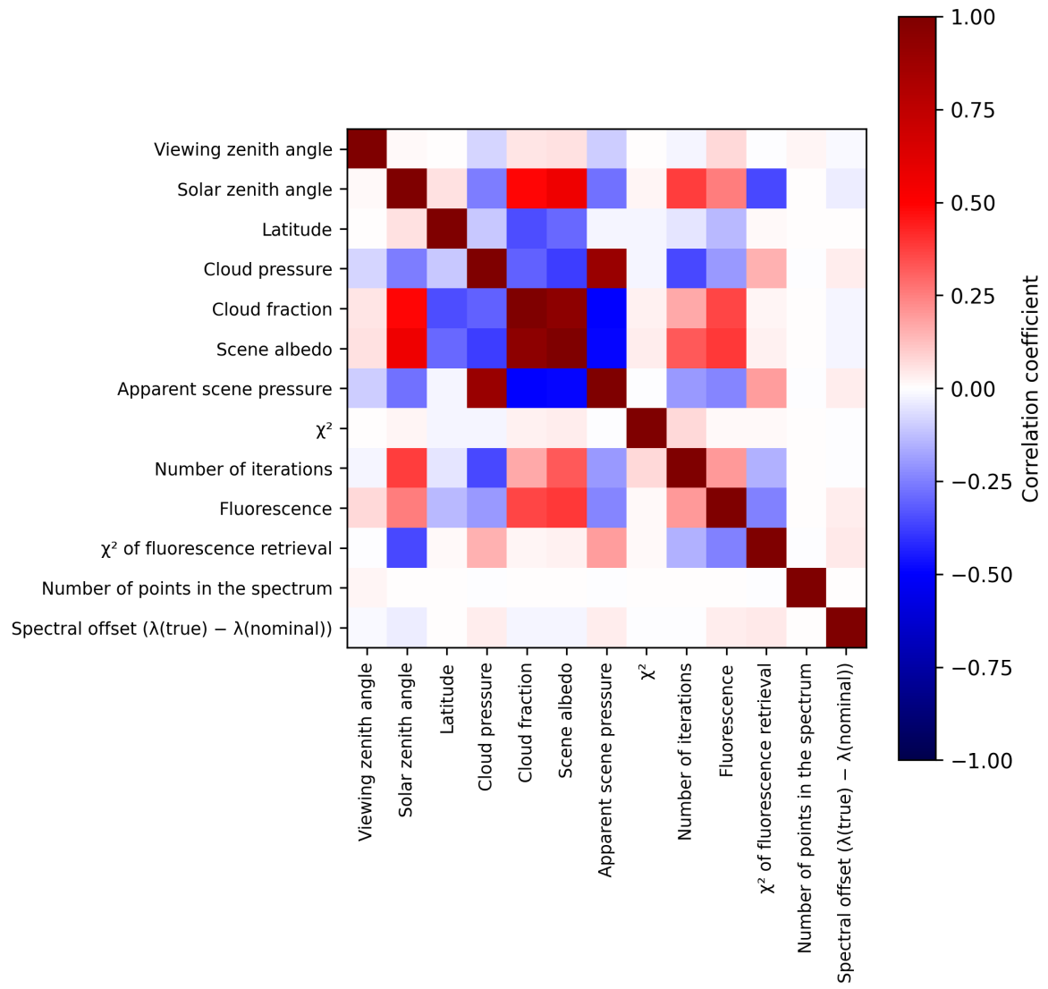
Figure 2: Map of correlation matrix for 2025-01-15 to 2025-01-17.
