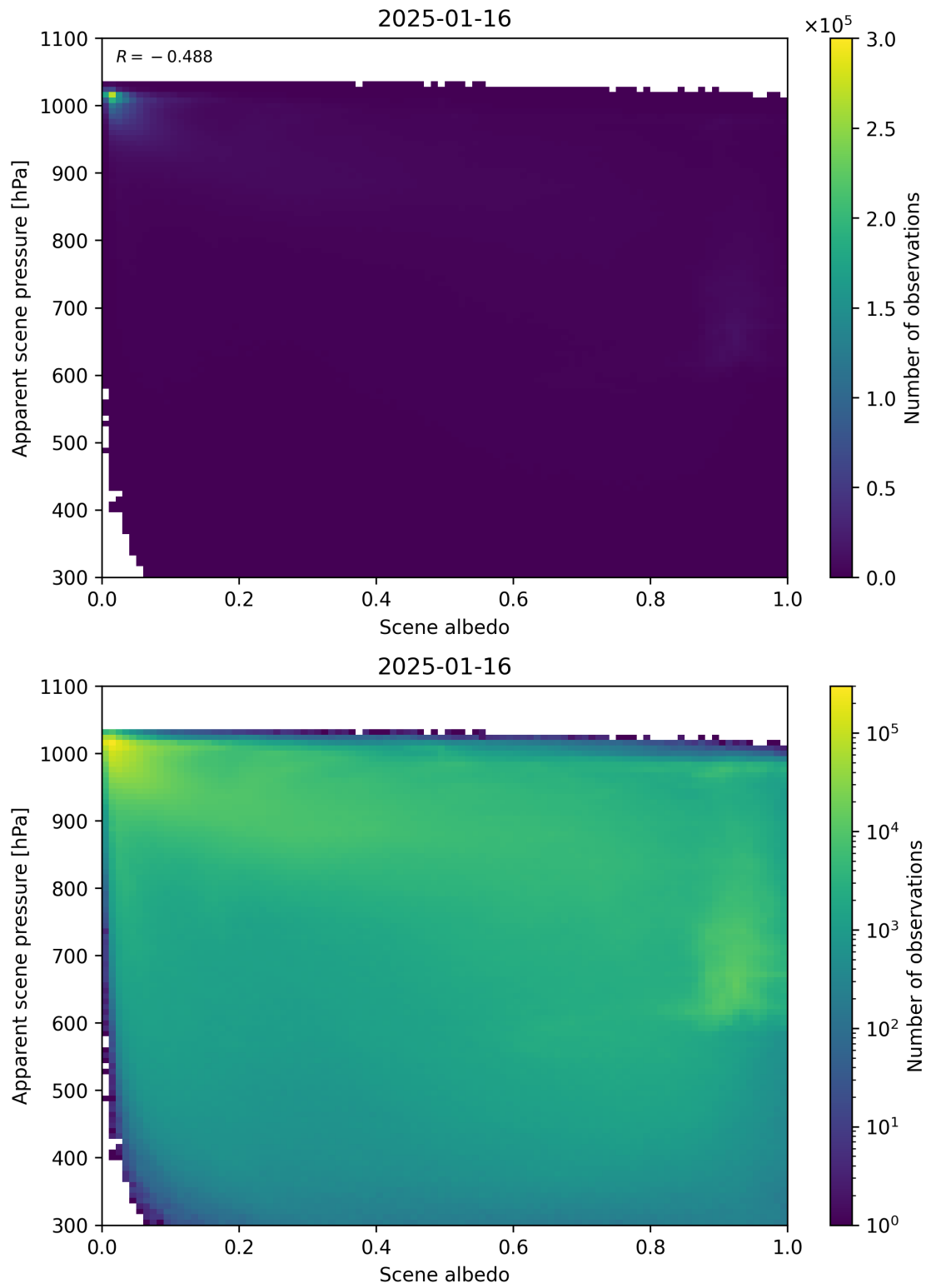
Figure 102: Scatter density plot of “Scene albedo” against “Apparent scene pressure” for 2025-01-15 to 2025-01-17.
