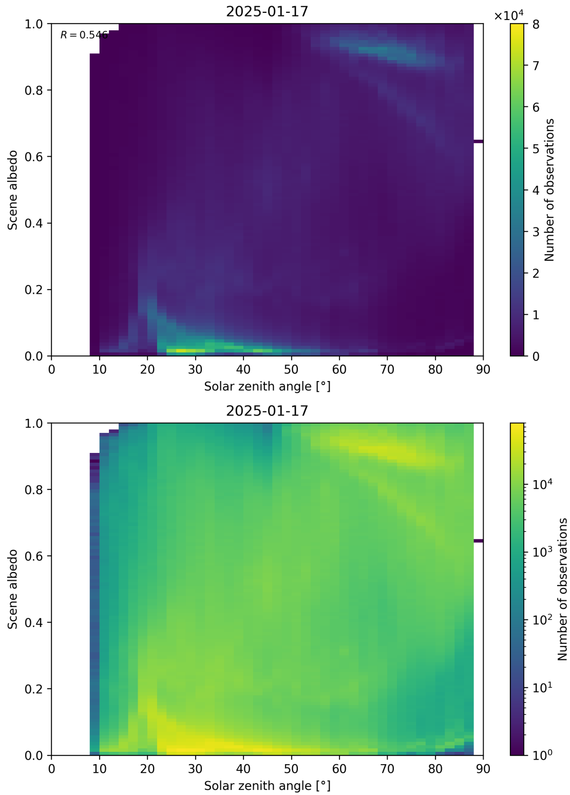
Figure 116: Scatter density plot of “Solar zenith angle” against “Scene albedo” for 2025-01-17 to 2025-01-18.
