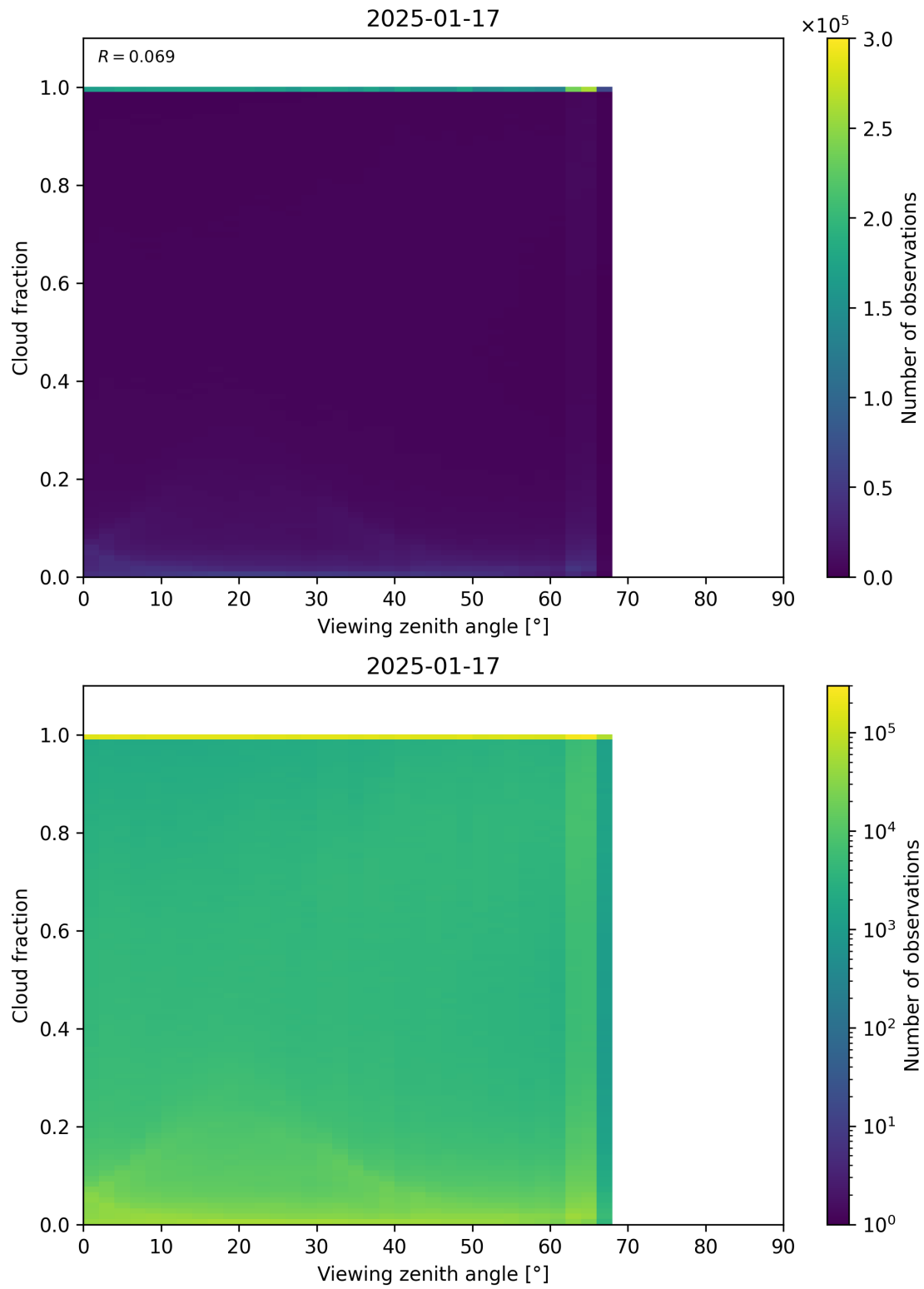
Figure 120: Scatter density plot of “Viewing zenith angle” against “Cloud fraction” for 2025-01-17 to 2025-01-18.
