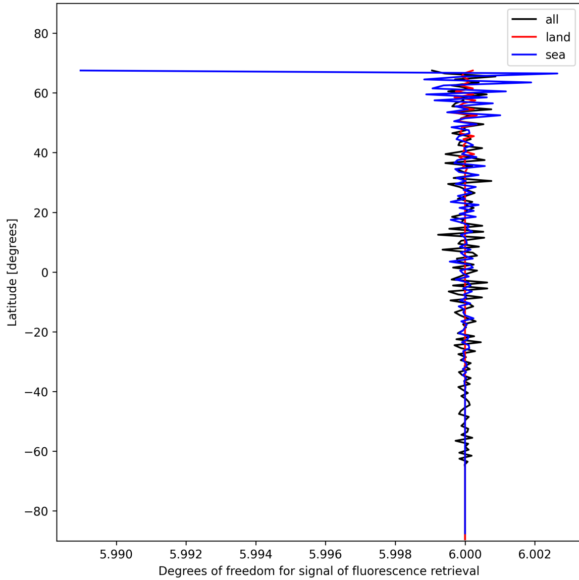
Figure 26: Zonal average of “Degrees of freedom for signal of fluorescence retrieval” for 2025-01-17 to 2025-01-18.
