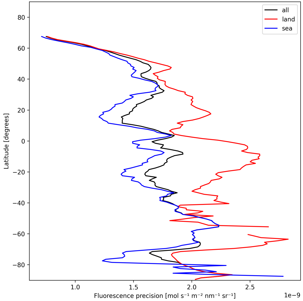
Figure 24: Zonal average of “Fluorescence precision” for 2025-01-17 to 2025-01-18.
