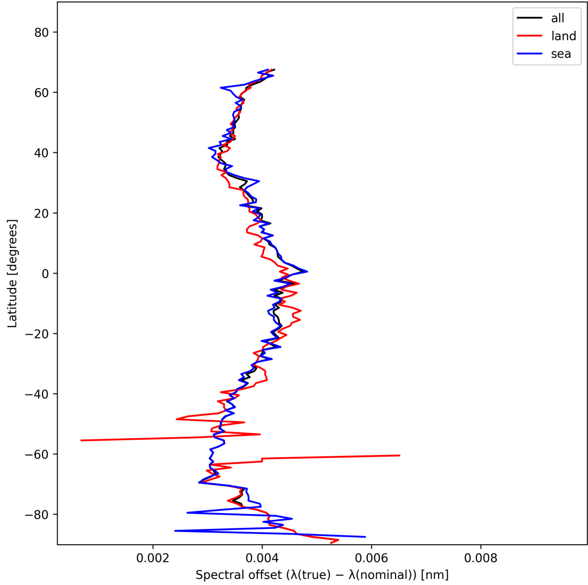
Figure 28: Zonal average of “Spectral offset ( \lambda_{\text{true}} - \lambda_{\text{nominal}} )” for 2025-01-17 to 2025-01-18.
