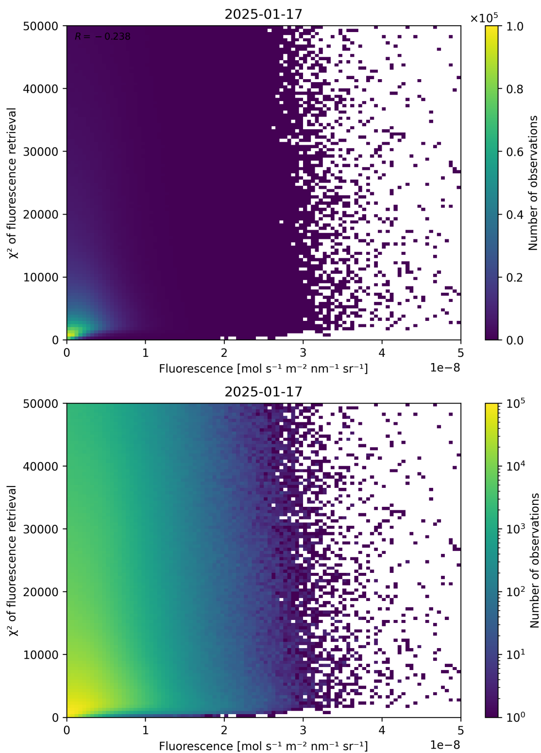
Figure 85: Scatter density plot of “Fluorescence” against “ \chi^2 of fluorescence retrieval” for 2025-01-17 to 2025-01-18.
