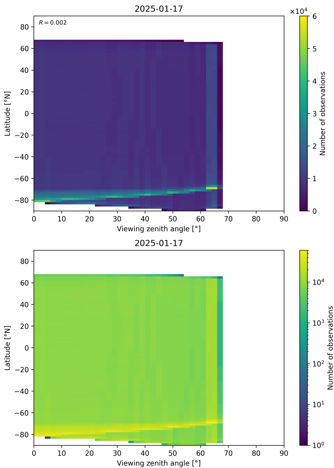
Figure 123: Scatter density plot of “Viewing zenith angle” against “Latitude” for 2025-01-17 to 2025-01-18.
