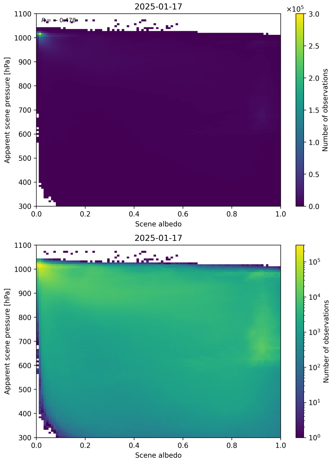
Figure 102: Scatter density plot of “Scene albedo” against “Apparent scene pressure” for 2025-01-17 to 2025-01-18.
