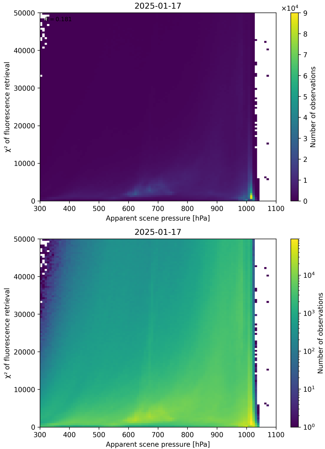
Figure 63: Scatter density plot of “Apparent scene pressure” against “ \chi^2 of fluorescence retrieval” for 2025-01-17 to 2025-01-18.
