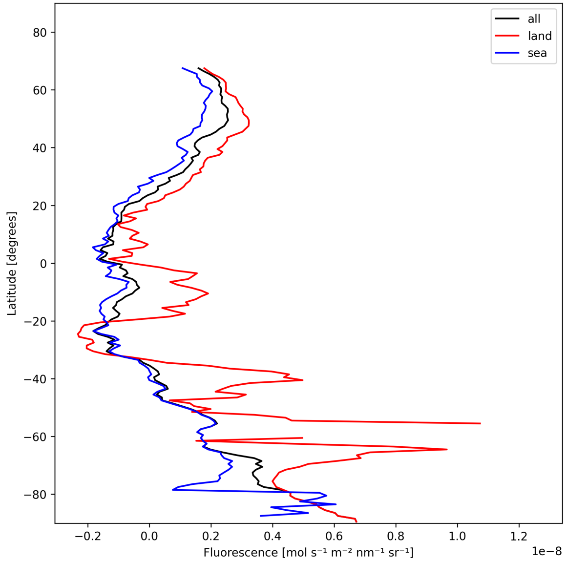
Figure 23: Zonal average of “Fluorescence” for 2025-01-17 to 2025-01-18.
