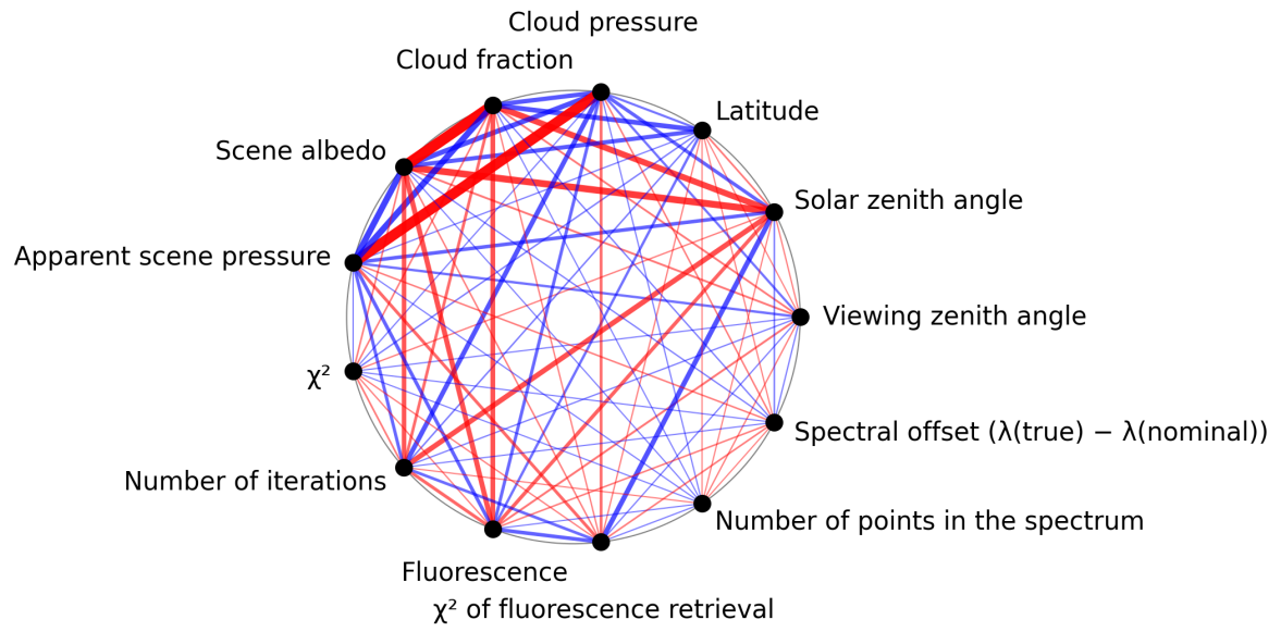
Figure 1: Map of correlation graph for 2025-01-17 to 2025-01-18.
