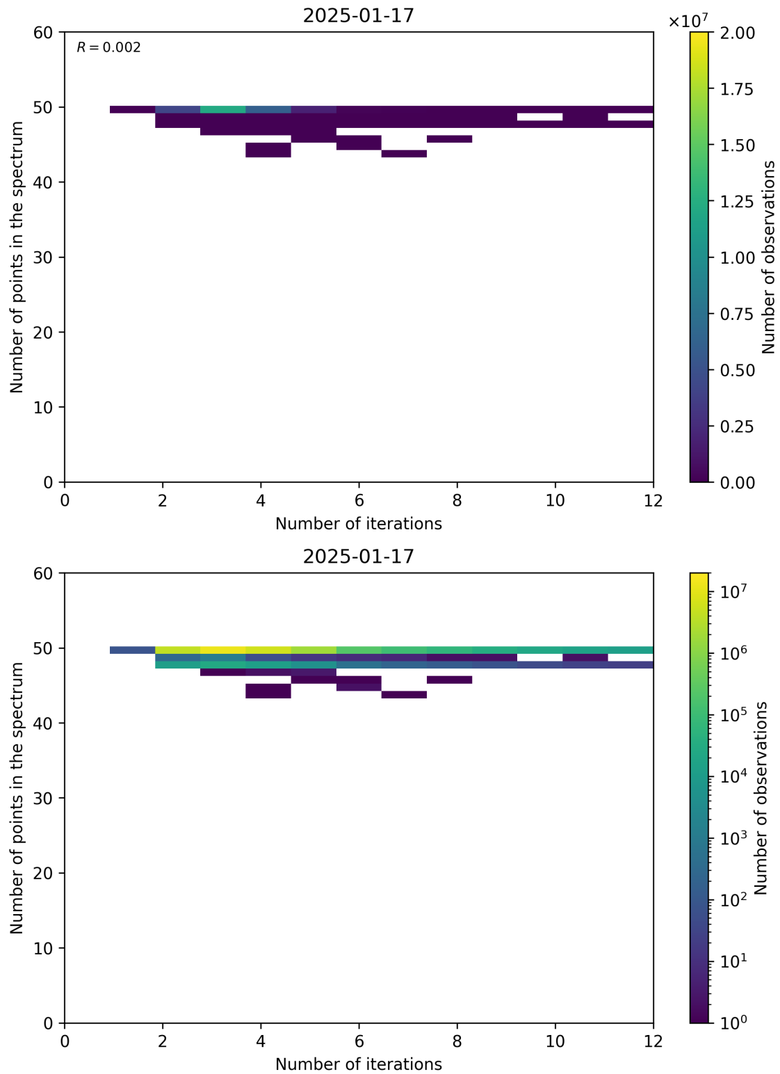
Figure 99: Scatter density plot of “Number of iterations” against “Number of points in the spectrum” for 2025-01-17 to 2025-01-18.
