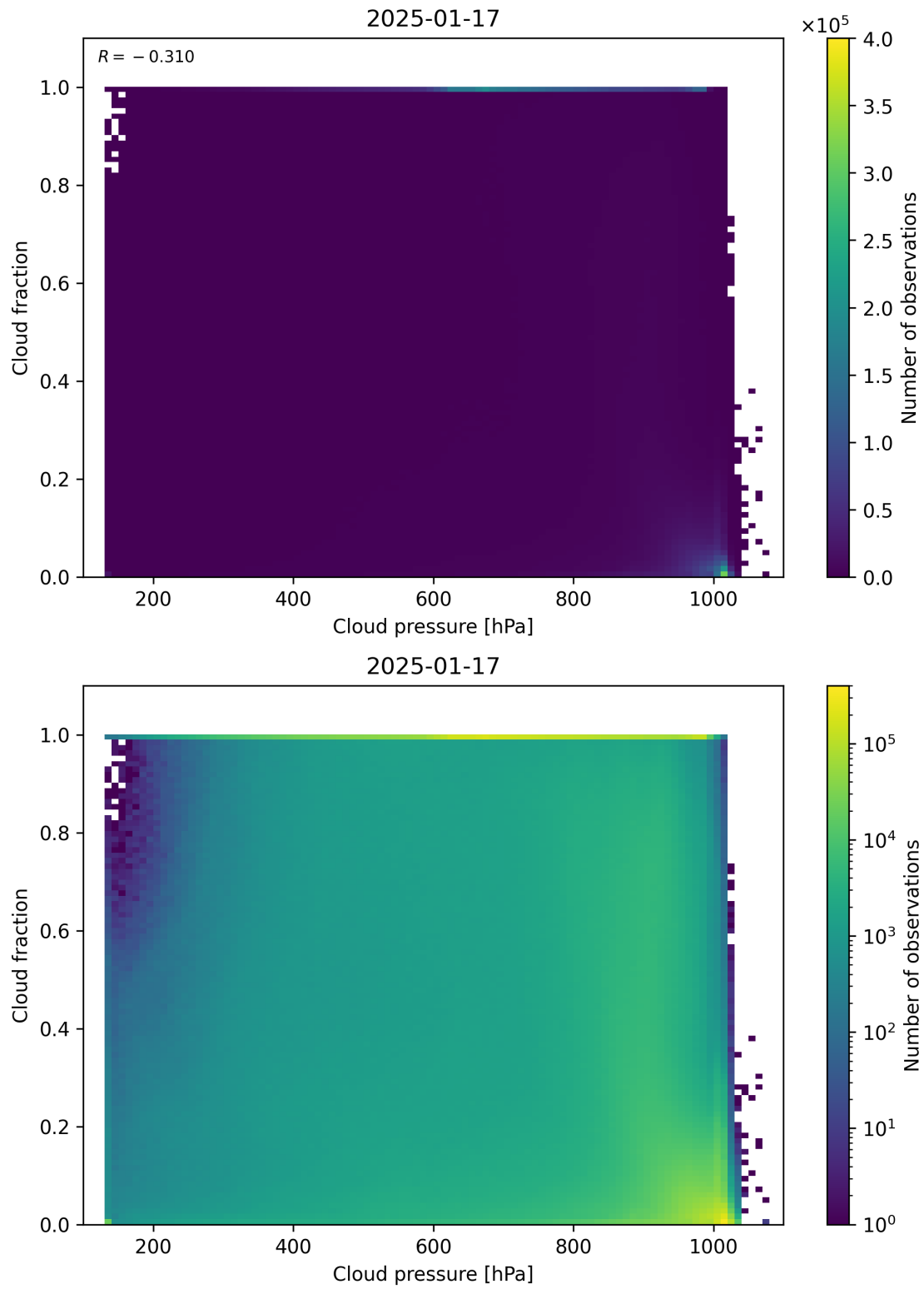
Figure 79: Scatter density plot of “Cloud pressure” against “Cloud fraction” for 2025-01-17 to 2025-01-18.
