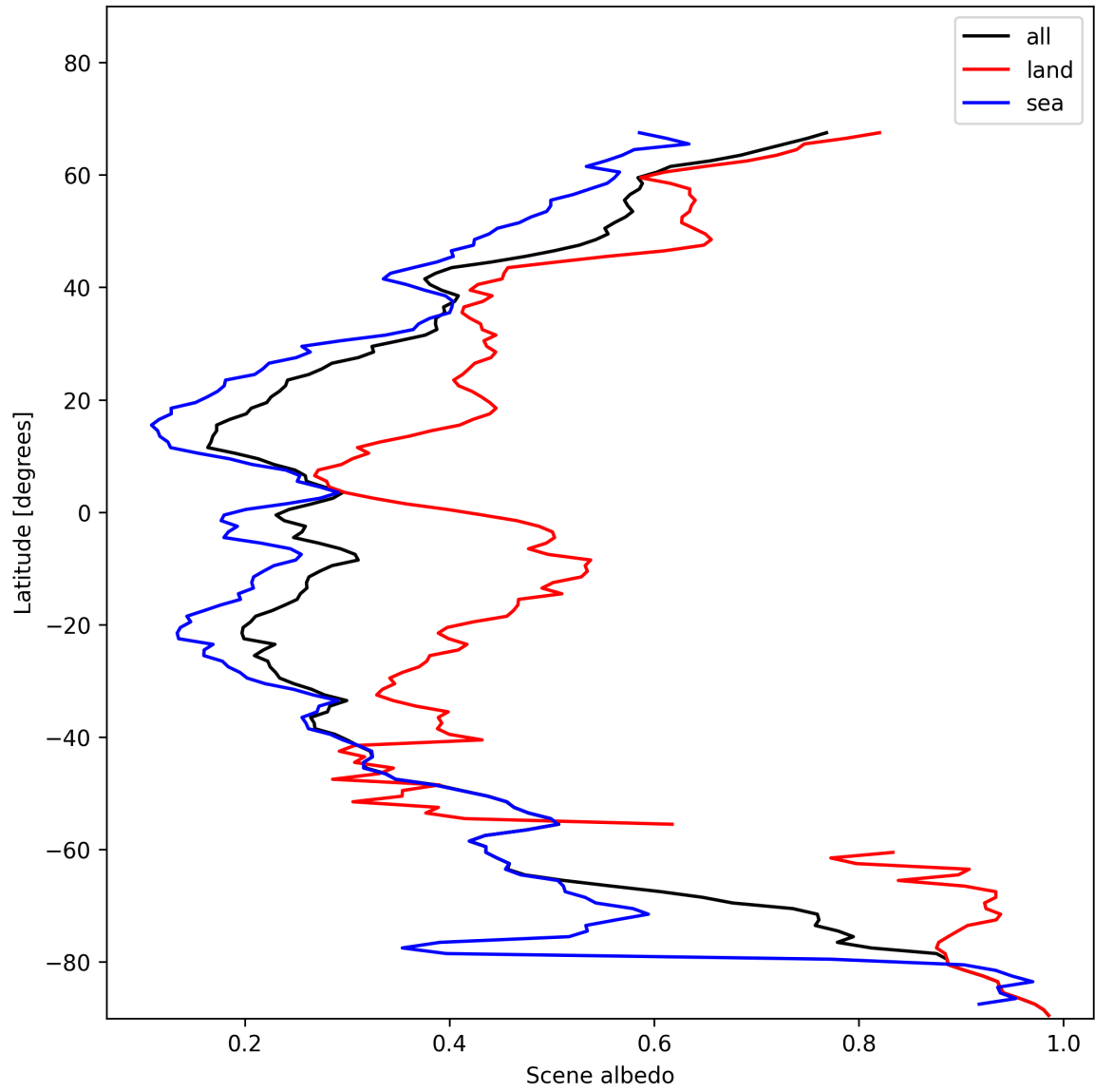
Figure 17: Zonal average of “Scene albedo” for 2025-01-17 to 2025-01-18.
