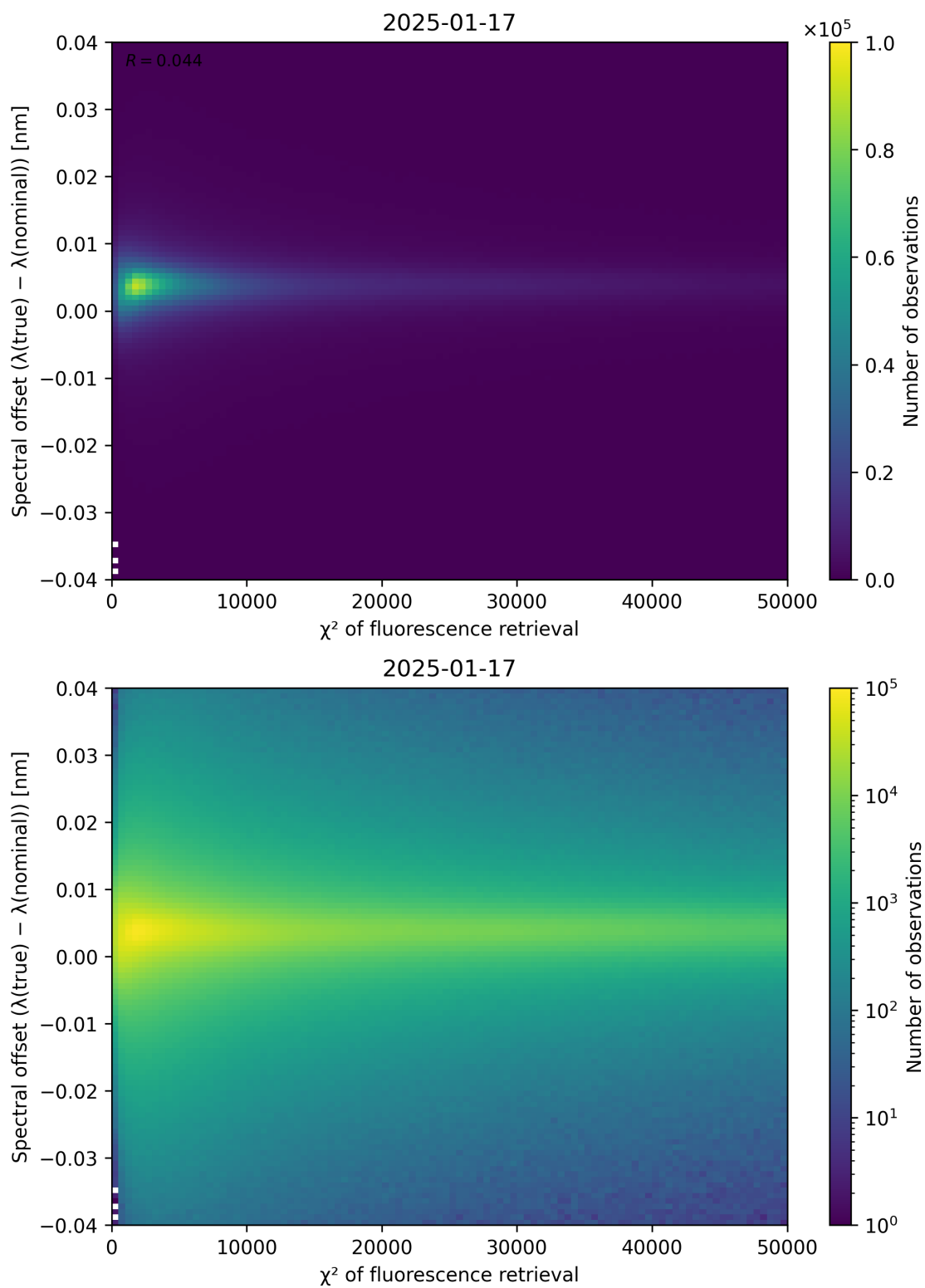
Figure 69: Scatter density plot of “ \chi^2 of fluorescence retrieval” against “Spectral offset ( \lambda_{\text{true}} - \lambda_{\text{nominal}} )” for 2025-01-17 to 2025-01-18.
