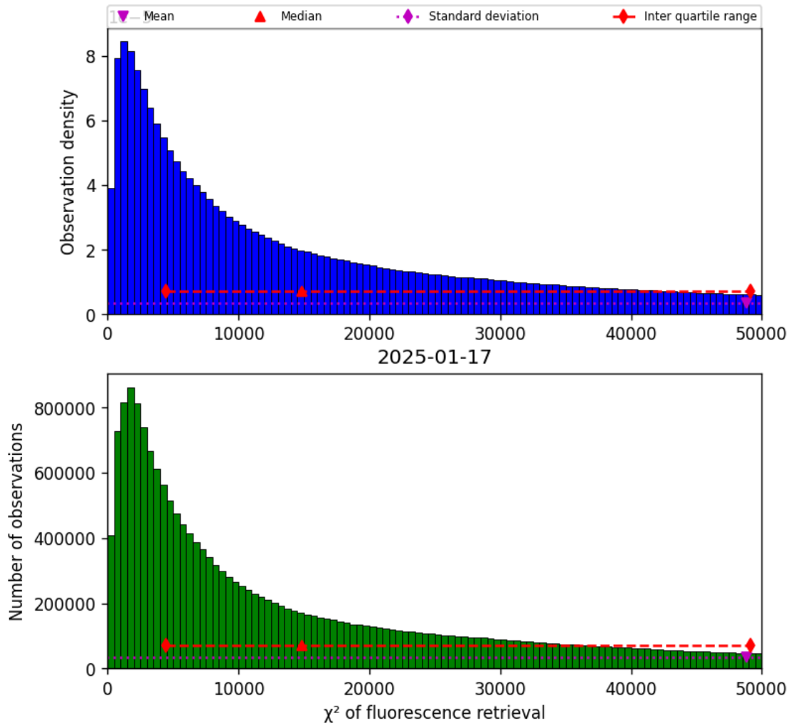
Figure 42: Histogram of “ \chi^2 of fluorescence retrieval” for 2025-01-17 to 2025-01-18
