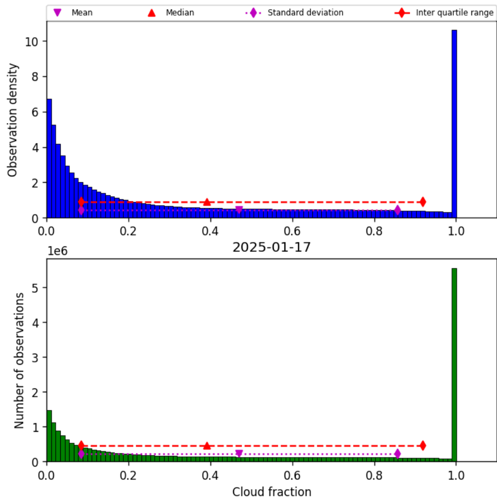
Figure 32: Histogram of “Cloud fraction” for 2025-01-17 to 2025-01-18
