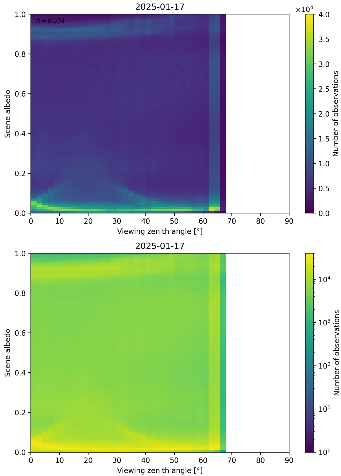
Figure 126: Scatter density plot of “Viewing zenith angle” against “Scene albedo” for 2025-01-17 to 2025-01-18.
