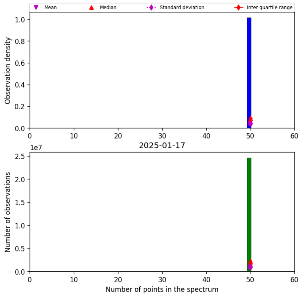
Figure 44: Histogram of “Number of points in the spectrum” for 2025-01-17 to 2025-01-18
