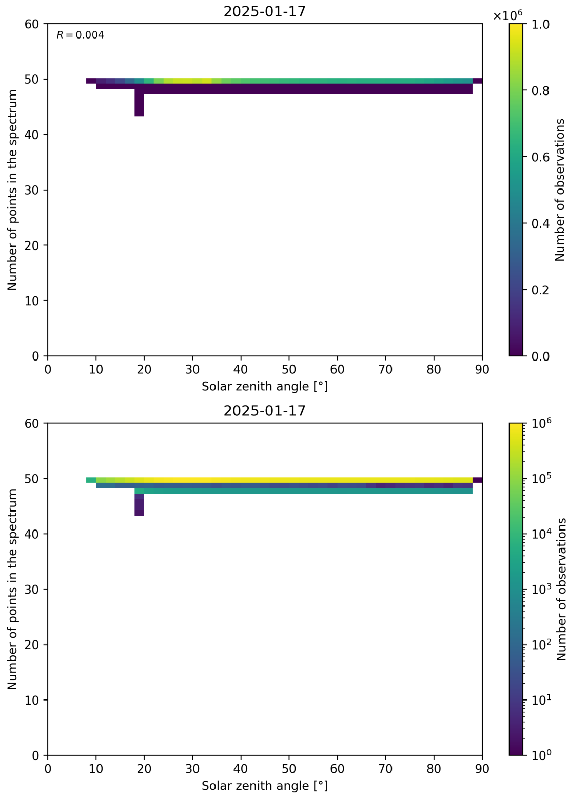
Figure 115: Scatter density plot of “Solar zenith angle” against “Number of points in the spectrum” for 2025-01-17 to 2025-01-18.
