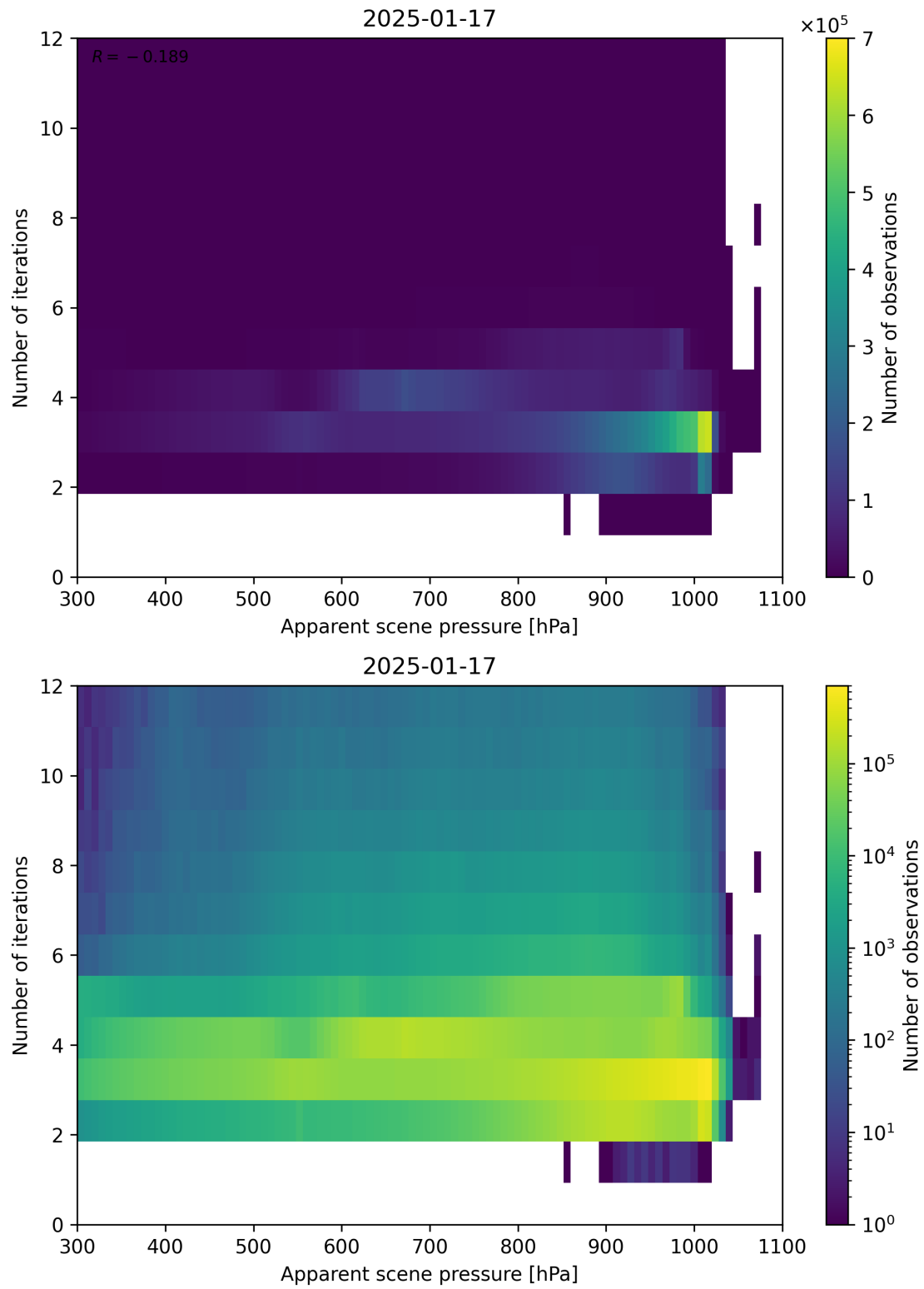
Figure 65: Scatter density plot of “Apparent scene pressure” against “Number of iterations” for 2025-01-17 to 2025-01-18.
