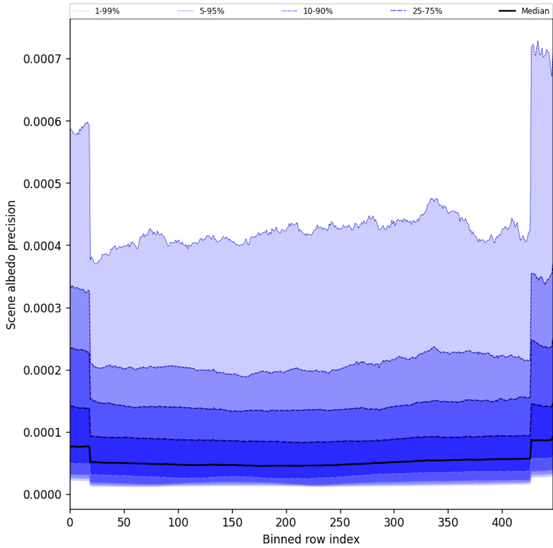
Figure 52: Along track statistics of “Scene albedo precision” for 2025-01-17 to 2025-01-18
