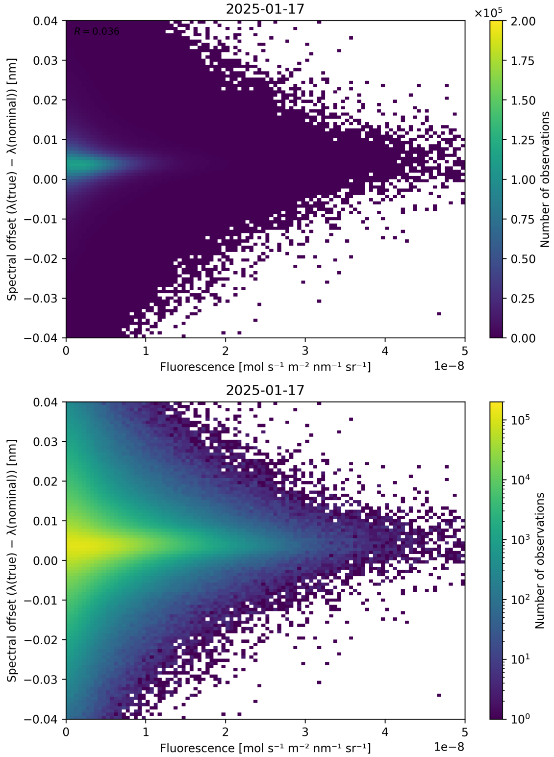
Figure 87: Scatter density plot of “Fluorescence” against “Spectral offset ( \lambda_{\text{true}} - \lambda_{\text{nominal}} )” for 2025-01-17 to 2025-01-18.
