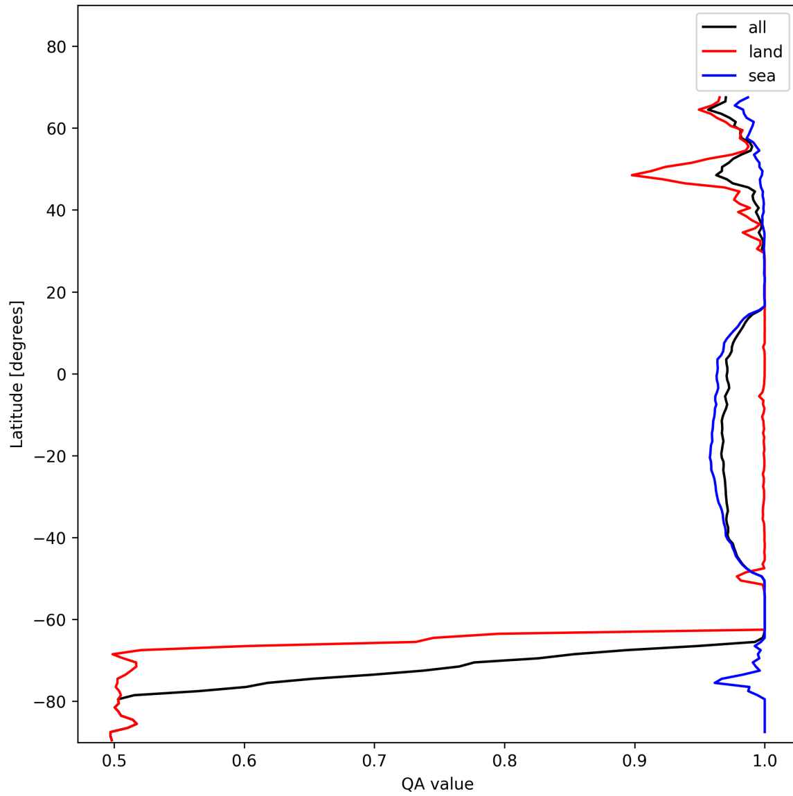
Figure 12: Zonal average of “QA value” for 2025-01-17 to 2025-01-18.
