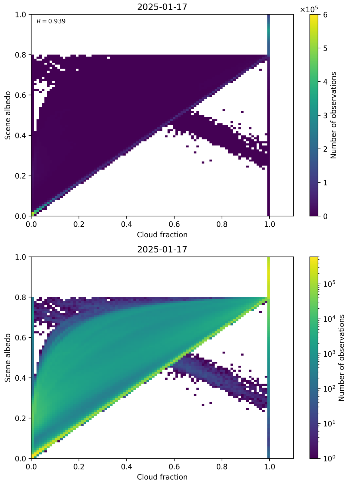
Figure 75: Scatter density plot of “Cloud fraction” against “Scene albedo” for 2025-01-17 to 2025-01-18.
