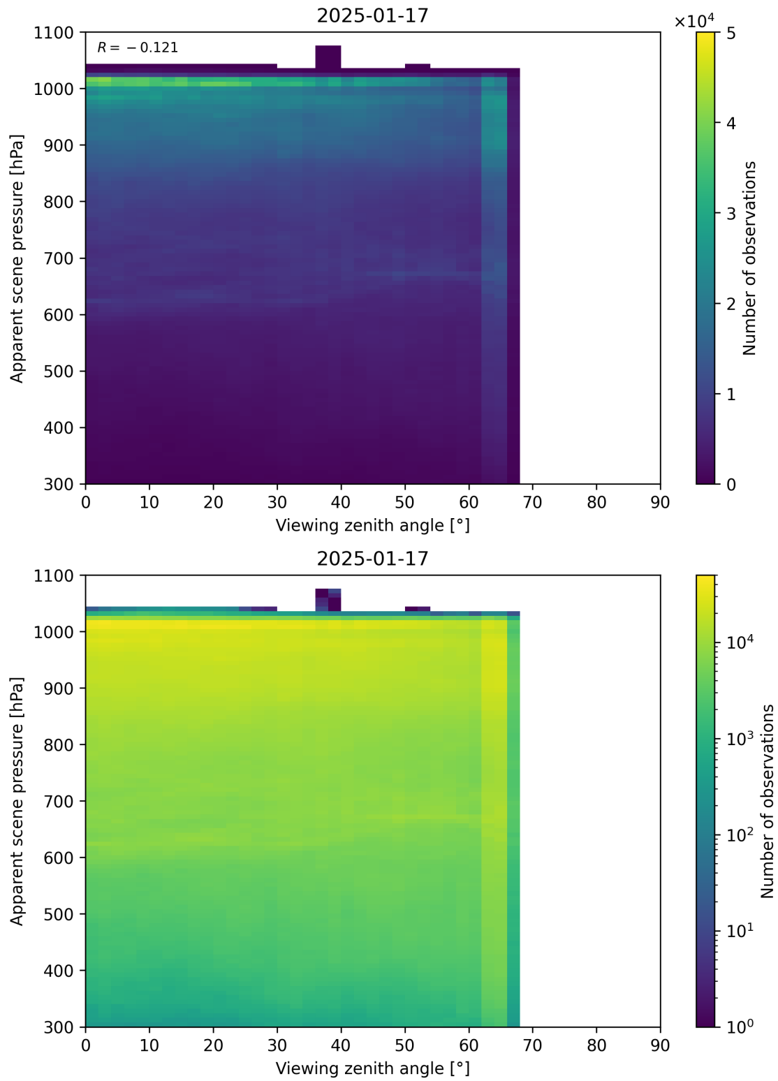
Figure 118: Scatter density plot of “Viewing zenith angle” against “Apparent scene pressure” for 2025-01-17 to 2025-01-18.
