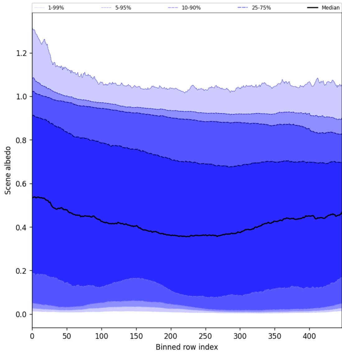
Figure 51: Along track statistics of “Scene albedo” for 2025-01-17 to 2025-01-18
