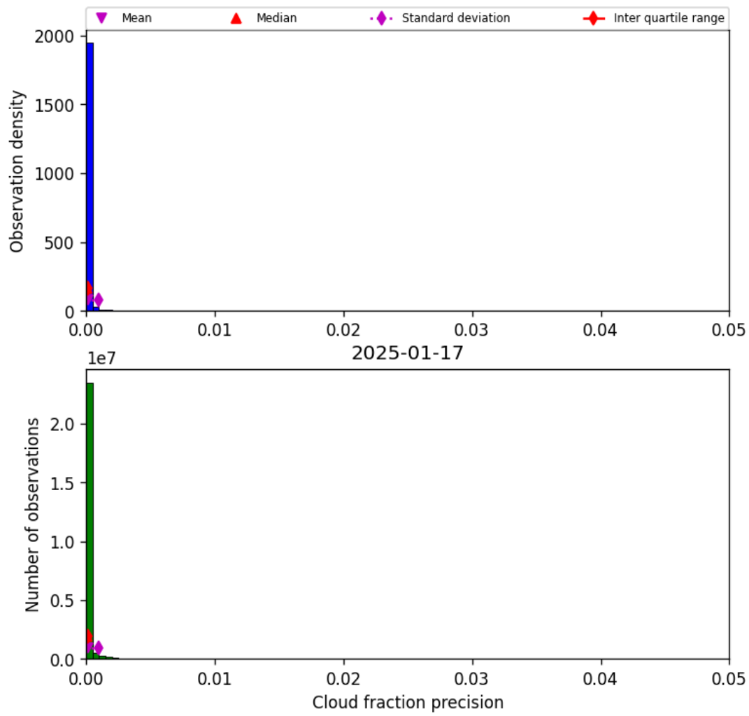
Figure 33: Histogram of “Cloud fraction precision” for 2025-01-17 to 2025-01-18
