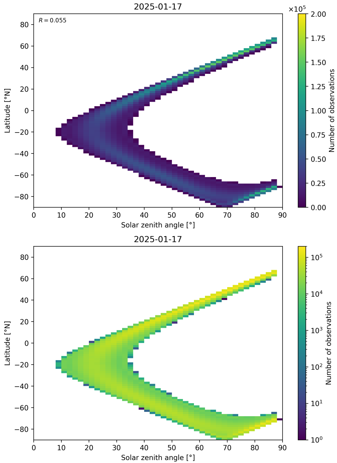
Figure 113: Scatter density plot of “Solar zenith angle” against “Latitude” for 2025-01-17 to 2025-01-18.
