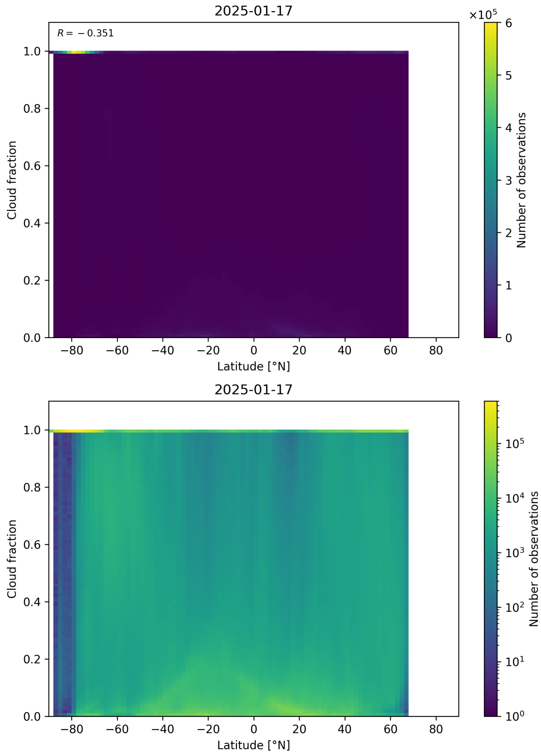
Figure 90: Scatter density plot of “Latitude” against “Cloud fraction” for 2025-01-17 to 2025-01-18.
