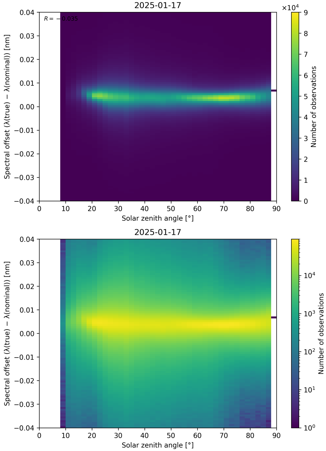
Figure 117: Scatter density plot of “Solar zenith angle” against “Spectral offset ( \lambda_{\text{true}} - \lambda_{\text{nominal}} )” for 2025-01-17 to 2025-01-18.
