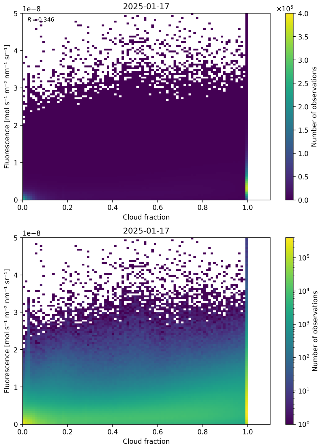
Figure 72: Scatter density plot of “Cloud fraction” against “Fluorescence” for 2025-01-17 to 2025-01-18.
