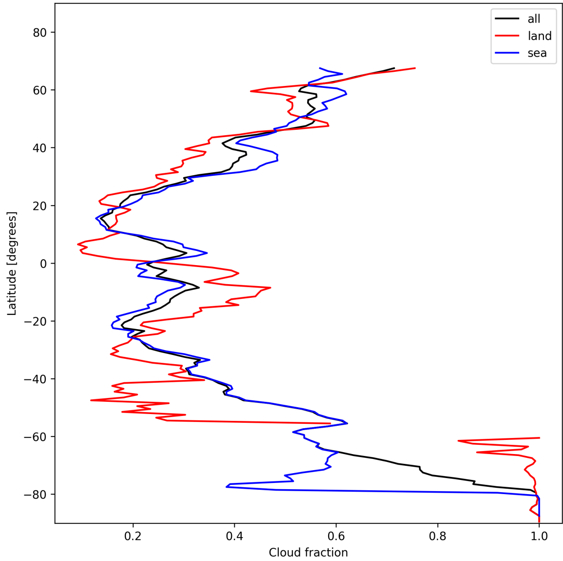
Figure 15: Zonal average of “Cloud fraction” for 2025-01-17 to 2025-01-18.
