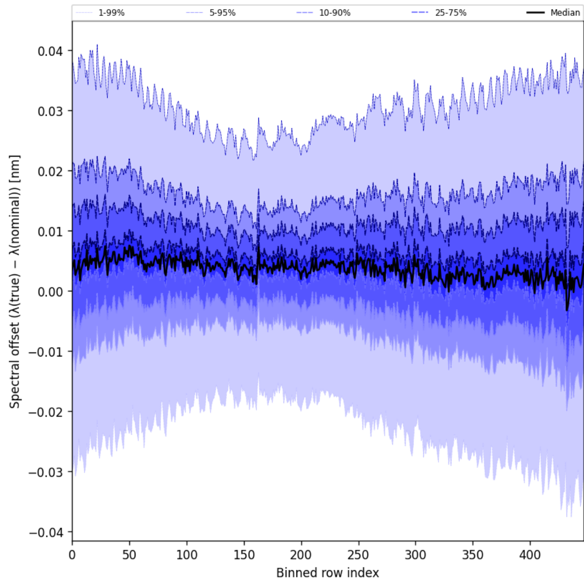
Figure 62: Along track statistics of “Spectral offset ( \lambda_{\text{true}} - \lambda_{\text{nominal}} )” for 2025-01-17 to 2025-01-18
