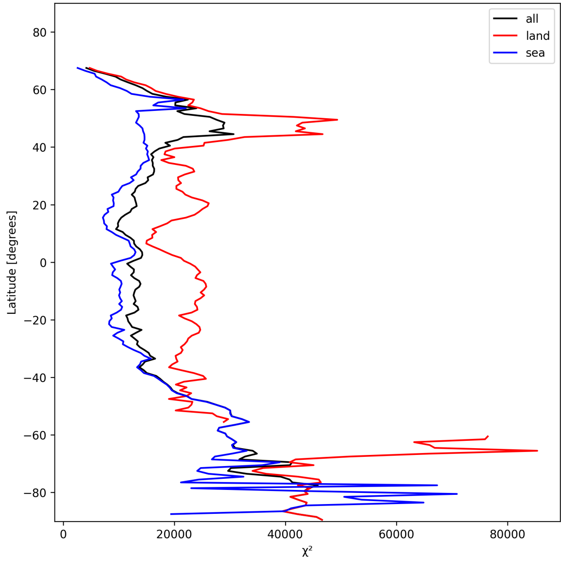
Figure 21: Zonal average of “ \chi^2 ” for 2025-01-17 to 2025-01-18.
