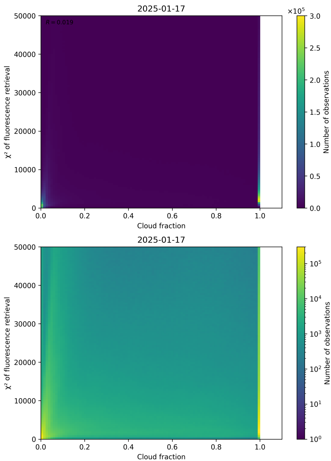
Figure 71: Scatter density plot of “Cloud fraction” against “ \chi^2 of fluorescence retrieval” for 2025-01-17 to 2025-01-18.
