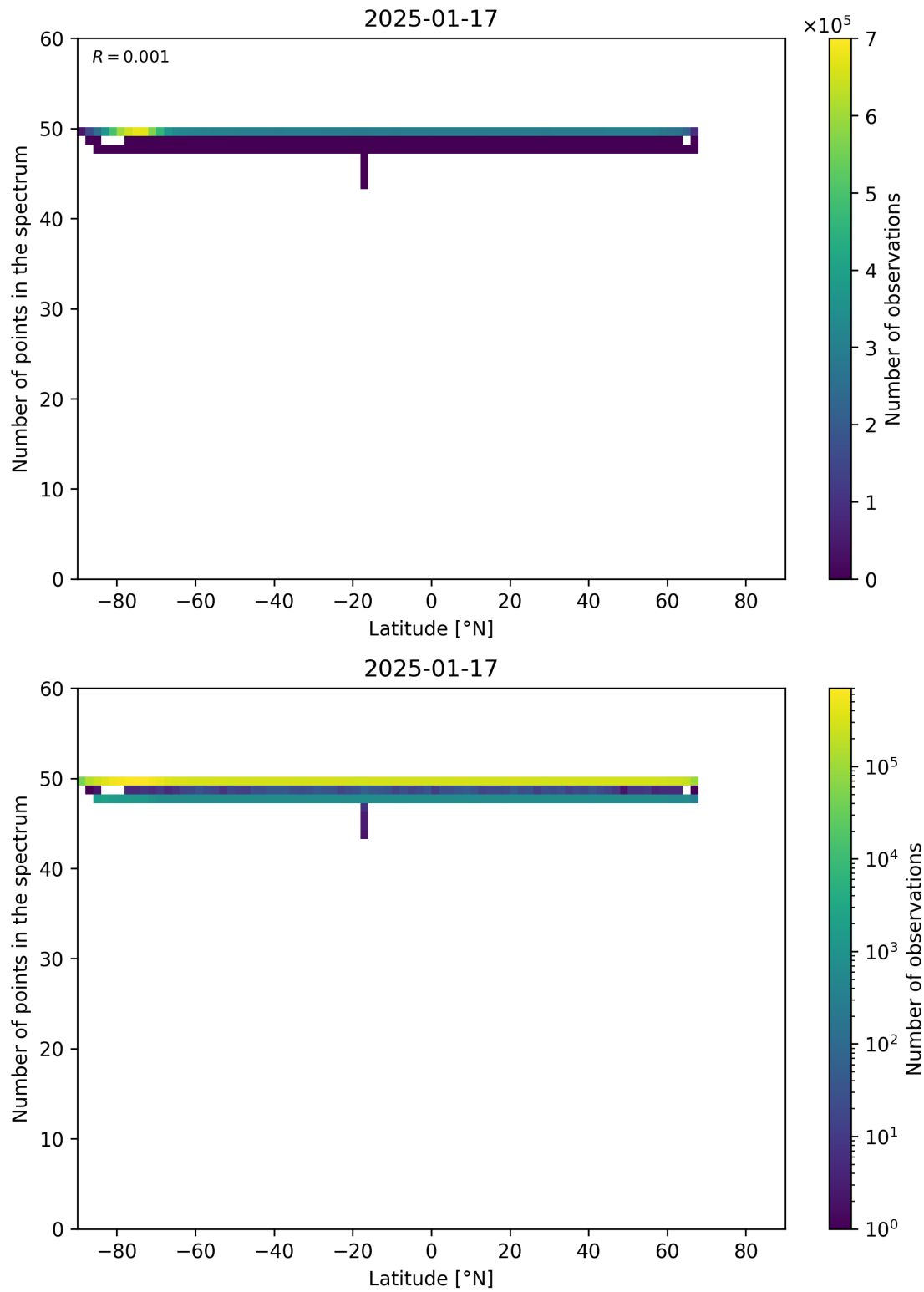
Figure 94: Scatter density plot of “Latitude” against “Number of points in the spectrum” for 2025-01-17 to 2025-01-18.
