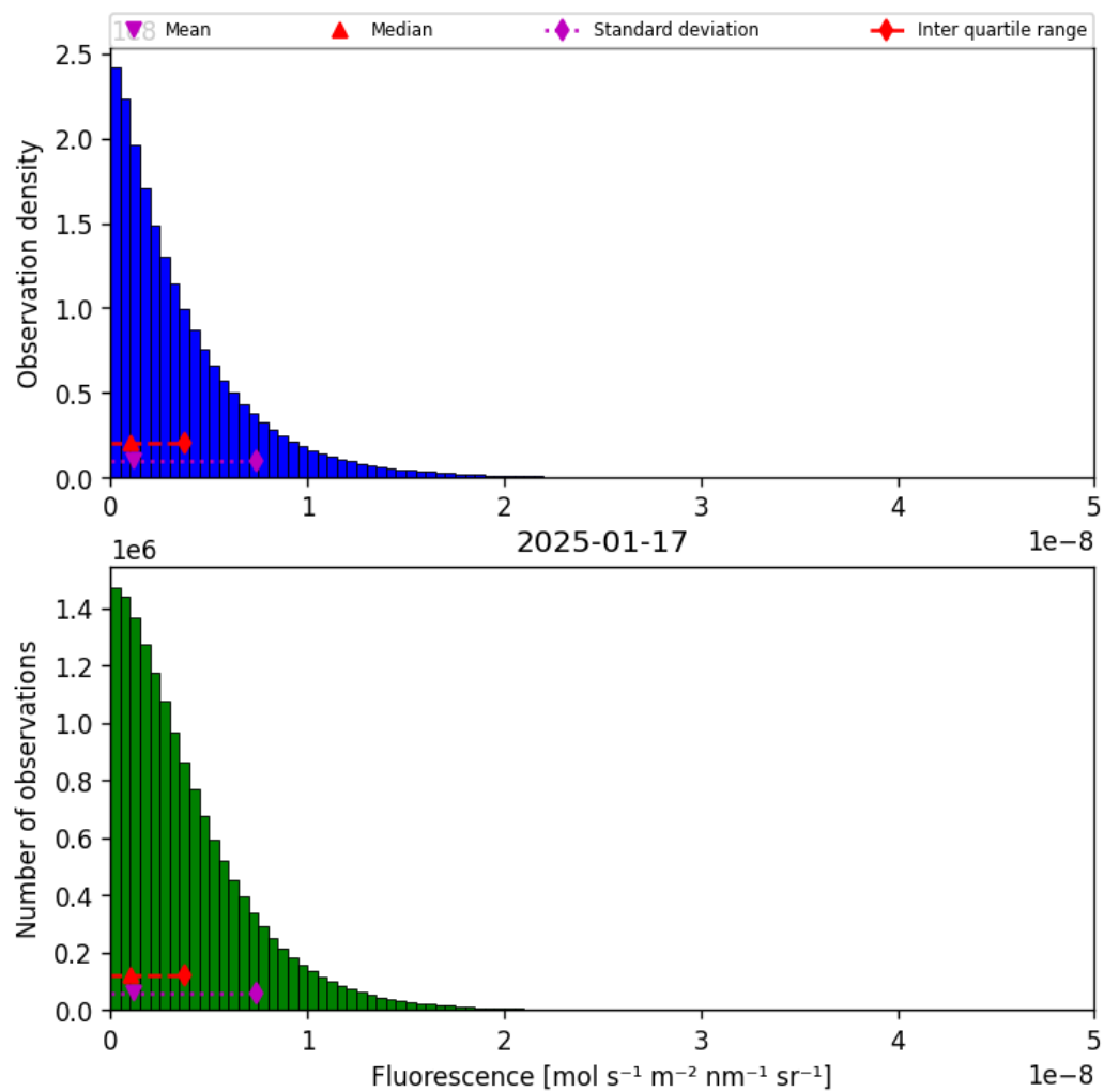
Figure 40: Histogram of “Fluorescence” for 2025-01-17 to 2025-01-18
