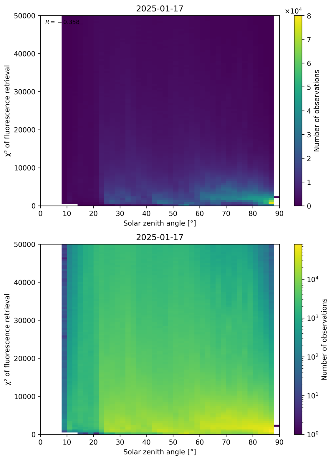
Figure 109: Scatter density plot of “Solar zenith angle” against “ \chi^2 of fluorescence retrieval” for 2025-01-17 to 2025-01-18.
