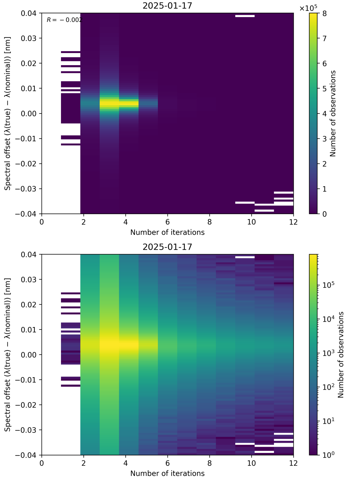
Figure 100: Scatter density plot of “Number of iterations” against “Spectral offset ( \lambda_{\text{true}} - \lambda_{\text{nominal}} )” for 2025-01-17 to 2025-01-18.
