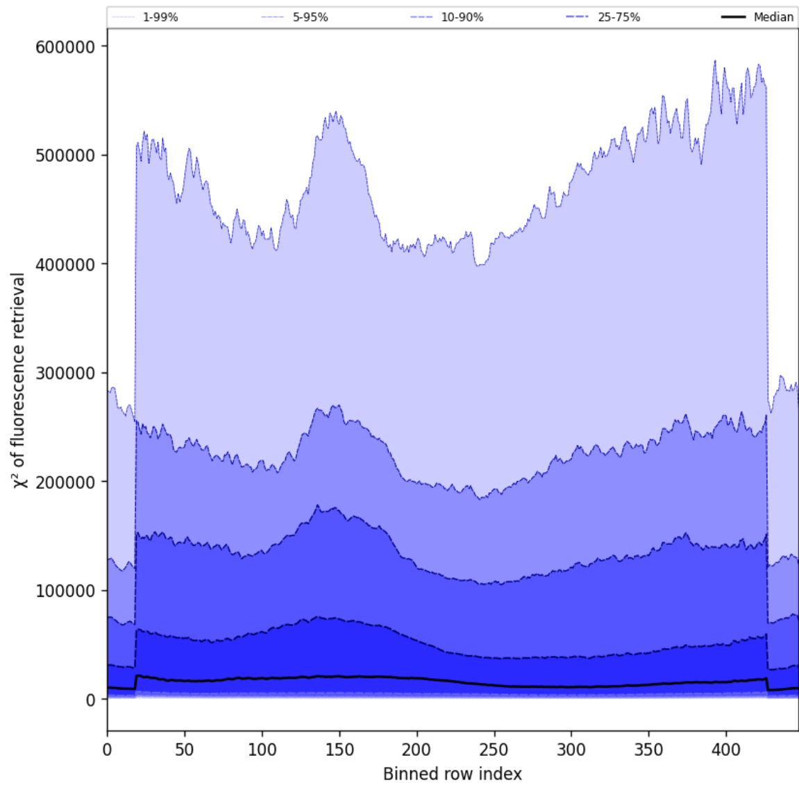
Figure 59: Along track statistics of “ \chi^2 of fluorescence retrieval” for 2025-01-17 to 2025-01-18
