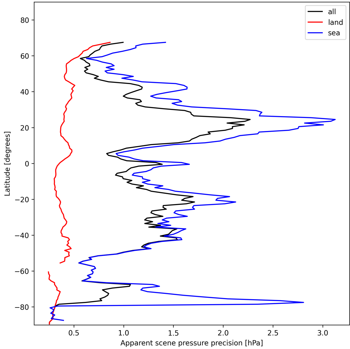
Figure 20: Zonal average of “Apparent scene pressure precision” for 2025-01-17 to 2025-01-18.
