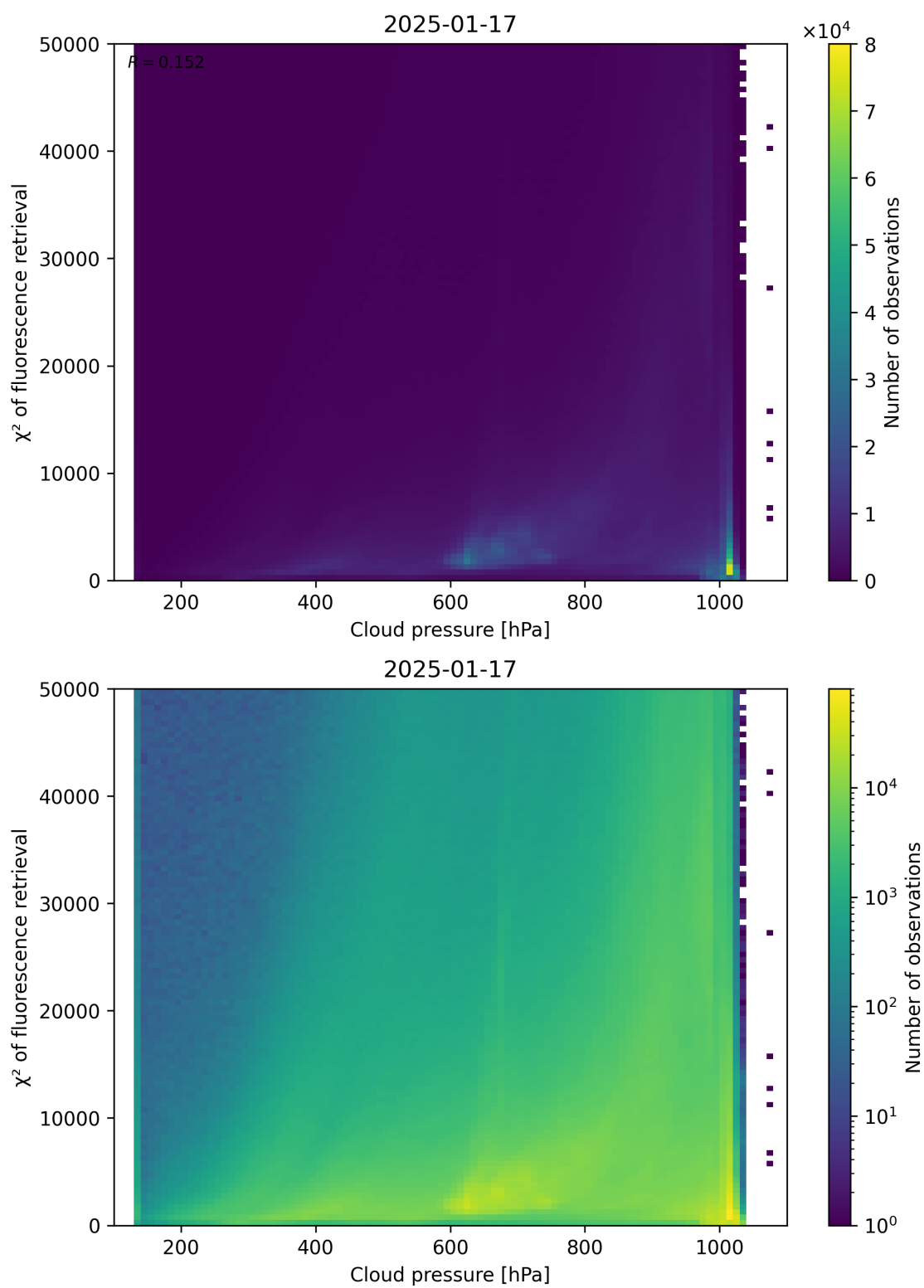
Figure 78: Scatter density plot of “Cloud pressure” against “ \chi^2 of fluorescence retrieval” for 2025-01-17 to 2025-01-18.
