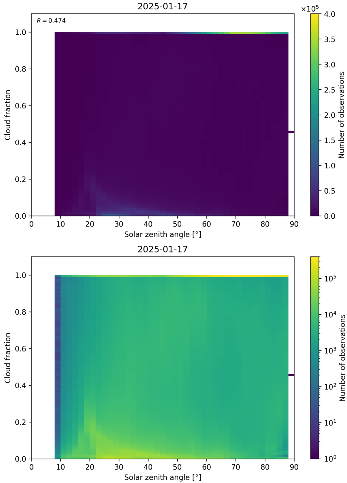
Figure 110: Scatter density plot of “Solar zenith angle” against “Cloud fraction” for 2025-01-17 to 2025-01-18.
