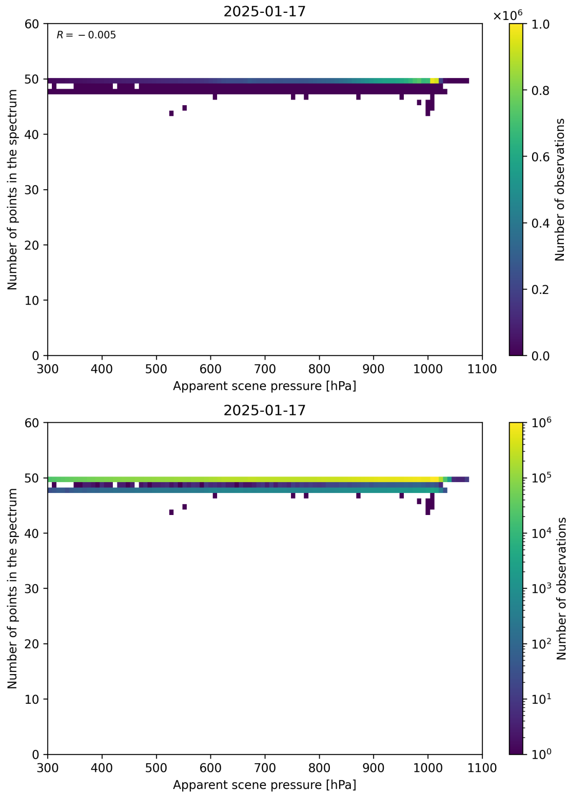
Figure 66: Scatter density plot of “Apparent scene pressure” against “Number of points in the spectrum” for 2025-01-17 to 2025-01-18.
