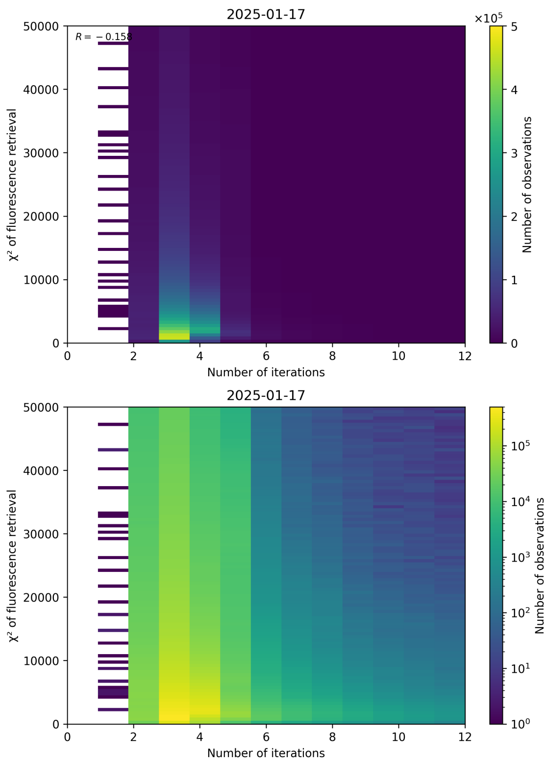
Figure 97: Scatter density plot of “Number of iterations” against “ \chi^2 of fluorescence retrieval” for 2025-01-17 to 2025-01-18.
