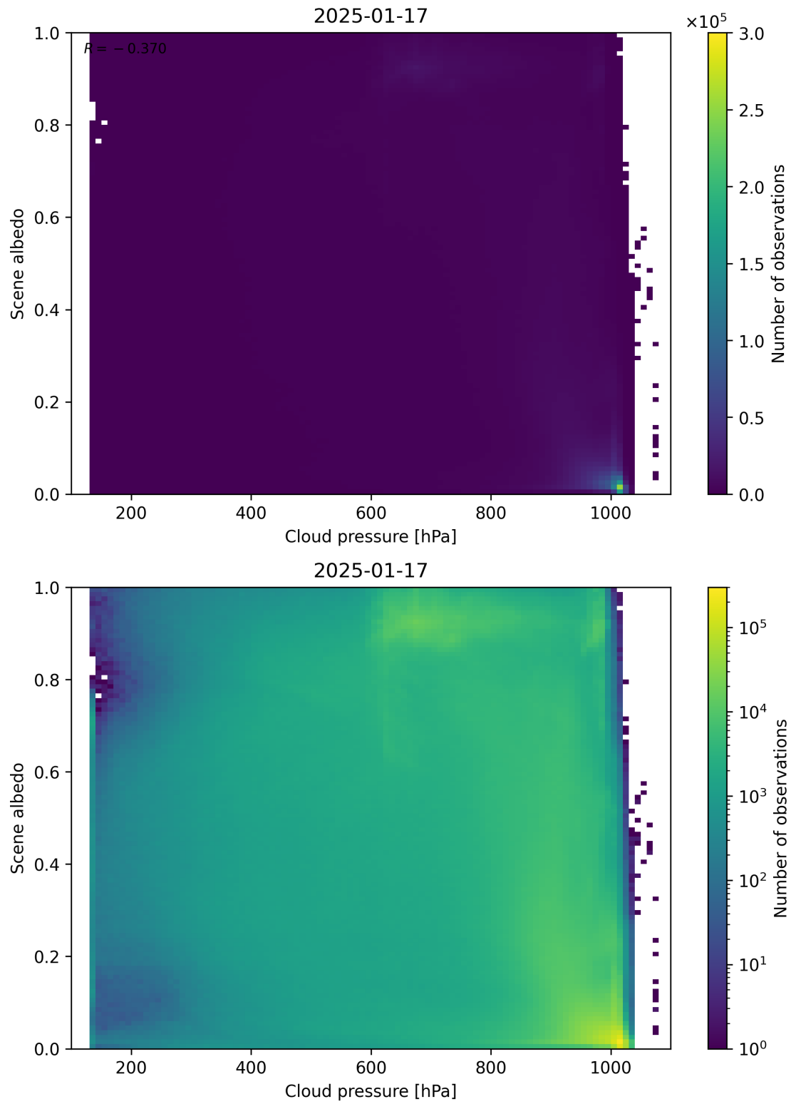
Figure 83: Scatter density plot of “Cloud pressure” against “Scene albedo” for 2025-01-17 to 2025-01-18.
