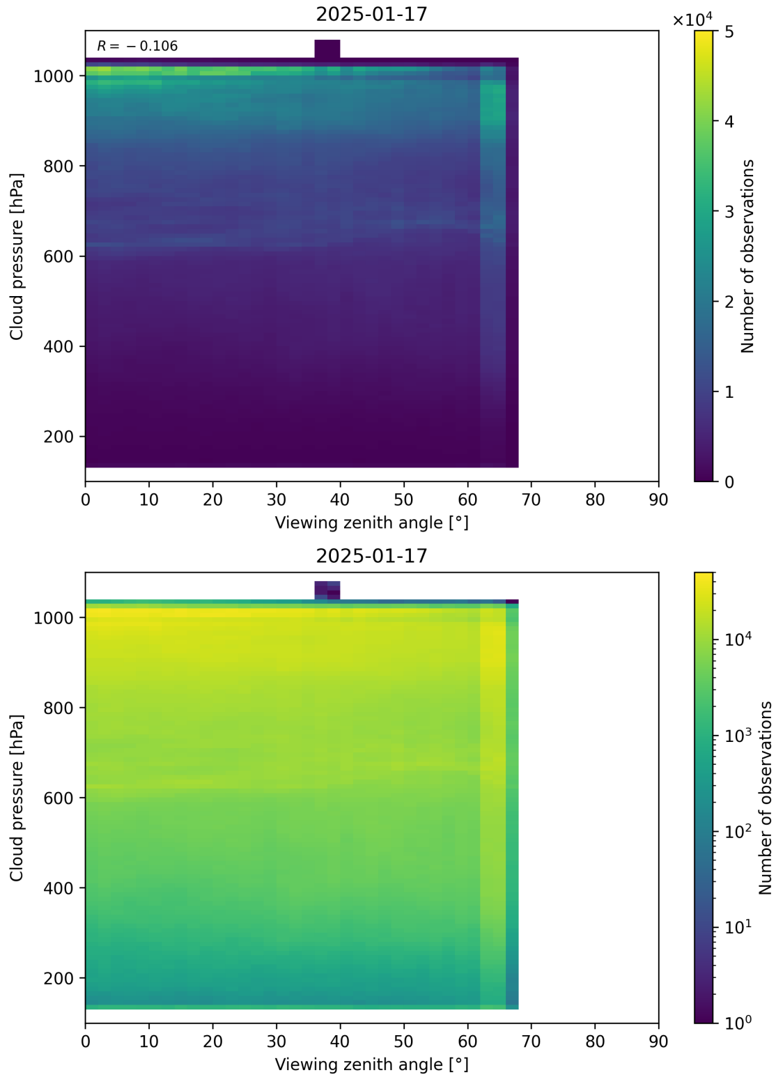
Figure 121: Scatter density plot of “Viewing zenith angle” against “Cloud pressure” for 2025-01-17 to 2025-01-18.
