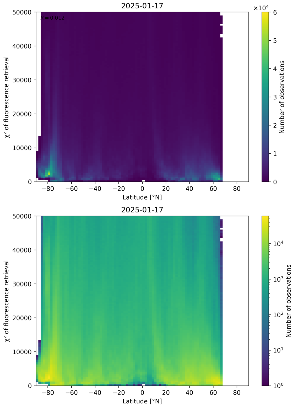
Figure 89: Scatter density plot of “Latitude” against “ \chi^2 of fluorescence retrieval” for 2025-01-17 to 2025-01-18.
