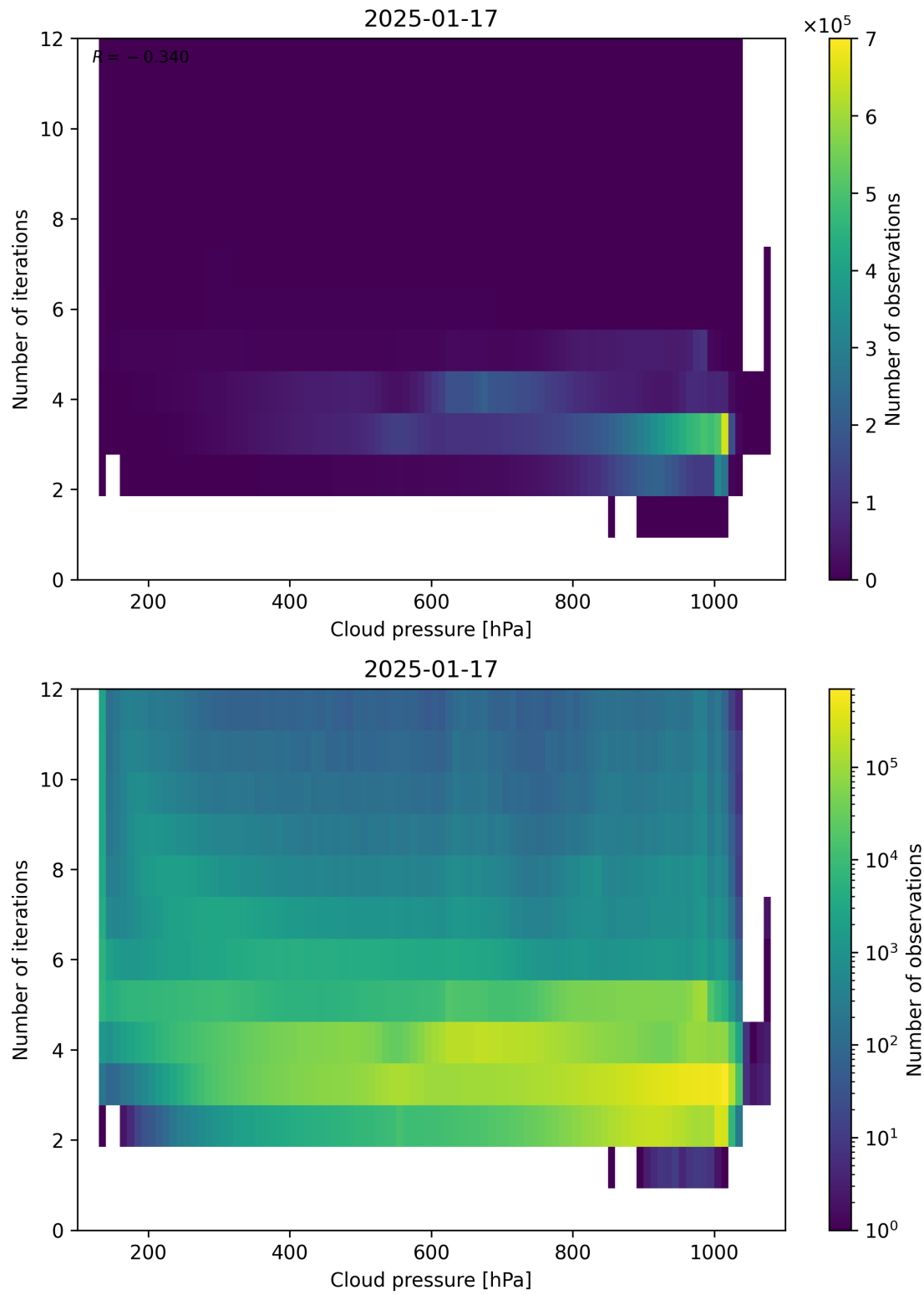
Figure 81: Scatter density plot of “Cloud pressure” against “Number of iterations” for 2025-01-17 to 2025-01-18.
