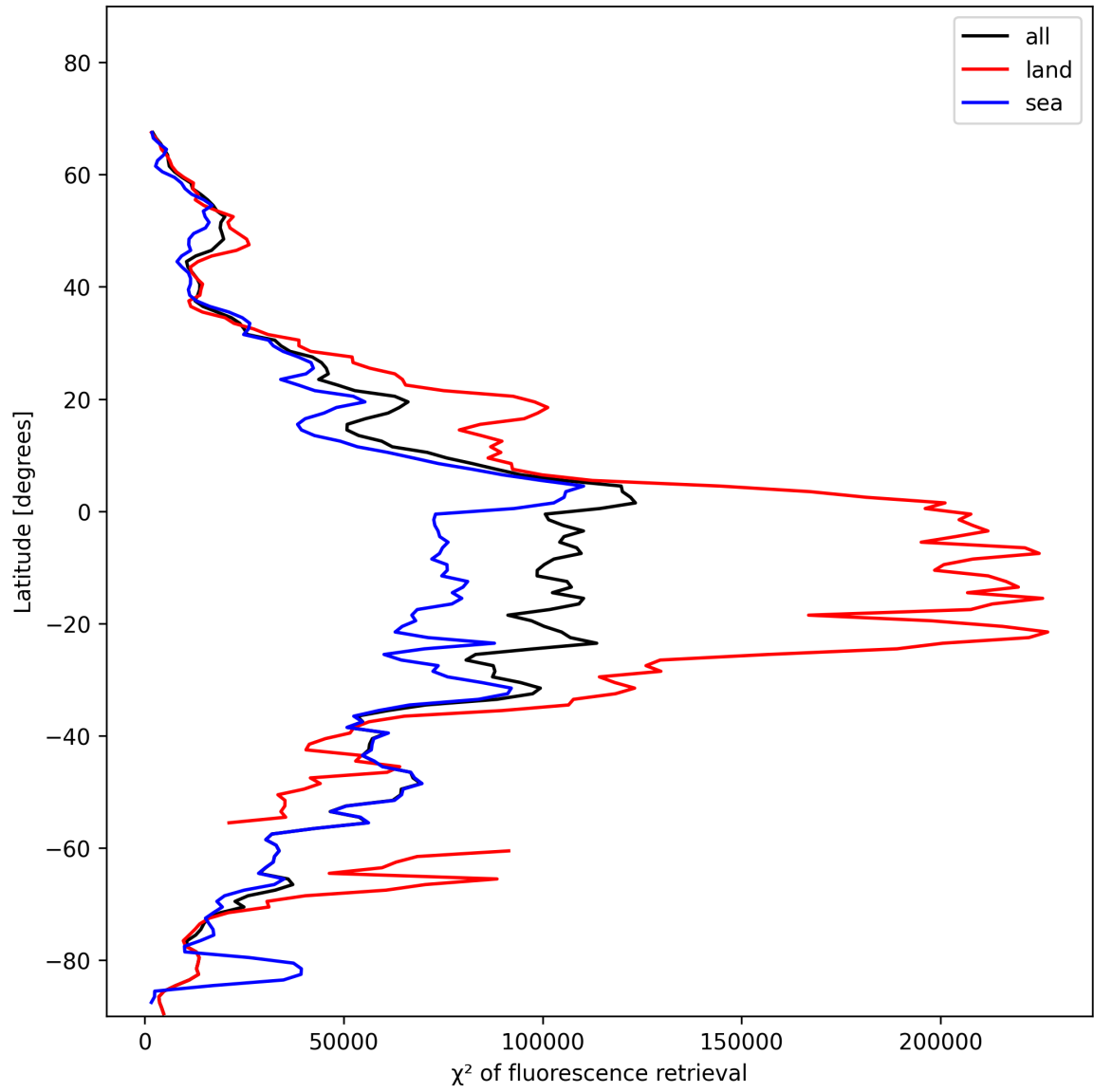
Figure 25: Zonal average of “ \chi^2 of fluorescence retrieval” for 2025-01-17 to 2025-01-18.
