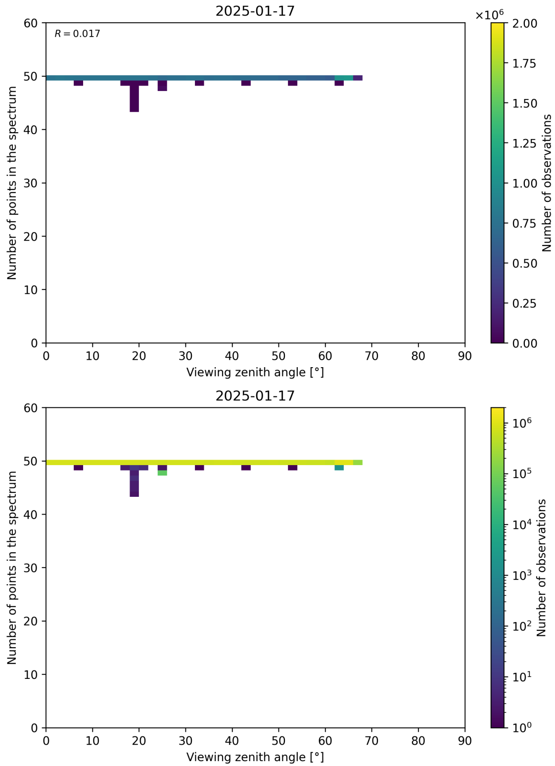
Figure 125: Scatter density plot of “Viewing zenith angle” against “Number of points in the spectrum” for 2025-01-17 to 2025-01-18.
