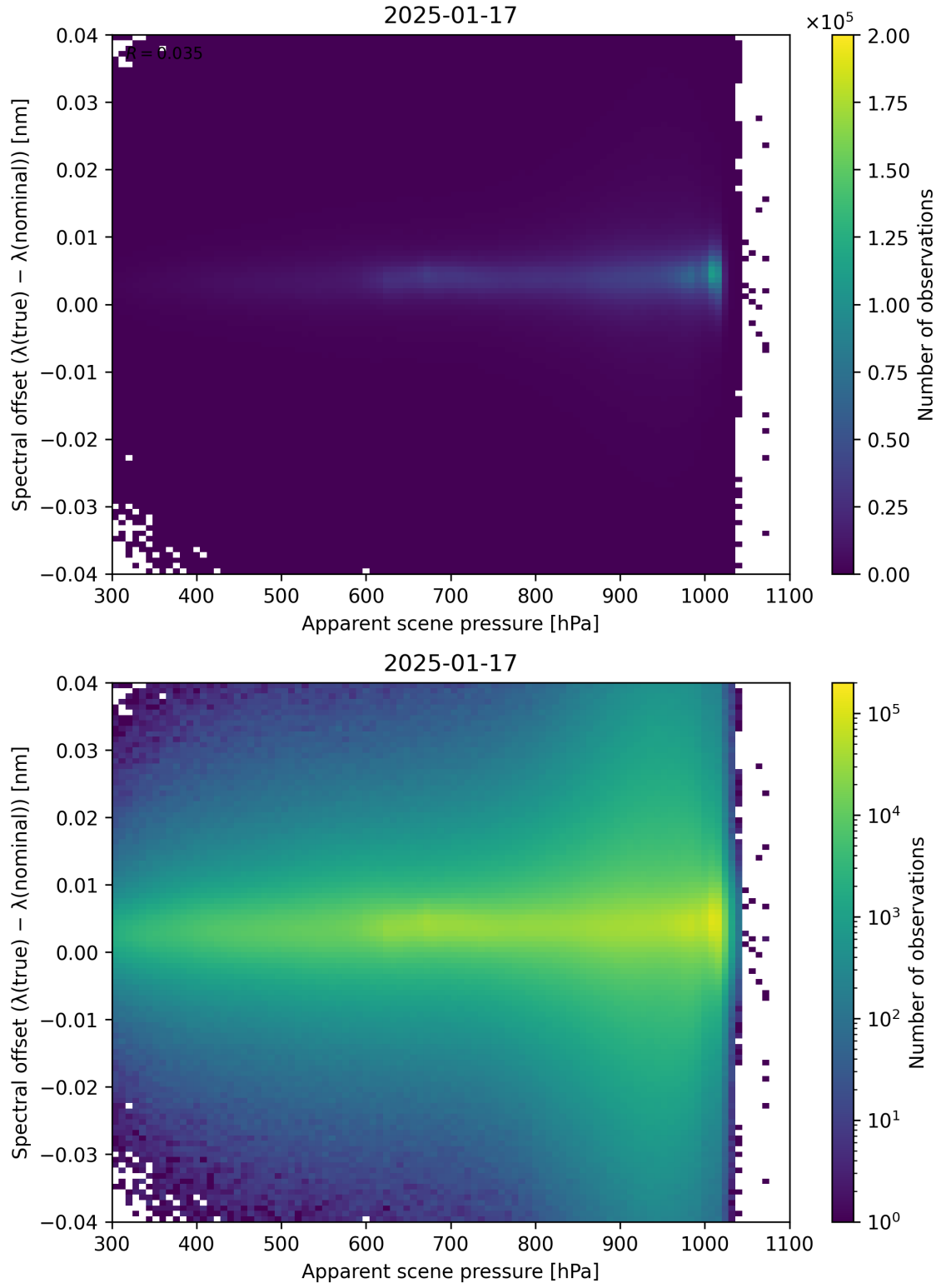
Figure 67: Scatter density plot of “Apparent scene pressure” against “Spectral offset ( \lambda_{\text{true}} - \lambda_{\text{nominal}} )” for 2025-01-17 to 2025-01-18.
