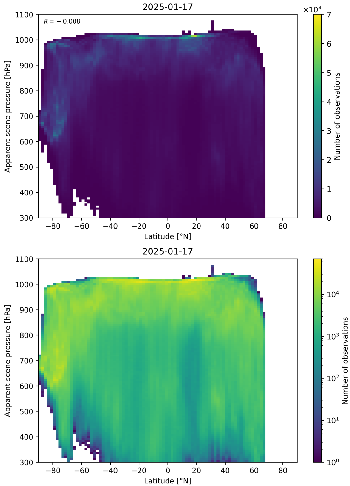
Figure 88: Scatter density plot of “Latitude” against “Apparent scene pressure” for 2025-01-17 to 2025-01-18.
