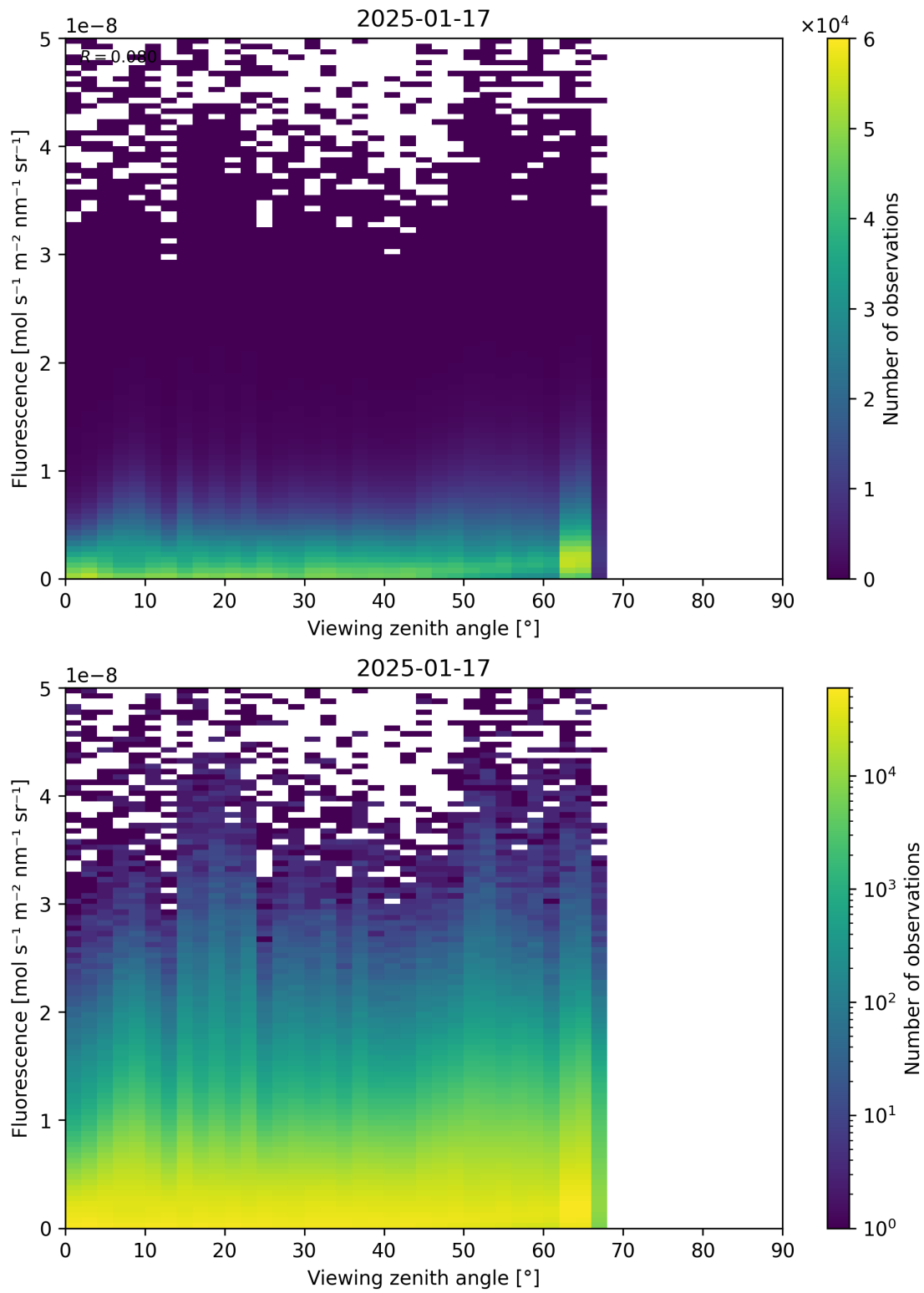
Figure 122: Scatter density plot of “Viewing zenith angle” against “Fluorescence” for 2025-01-17 to 2025-01-18.
