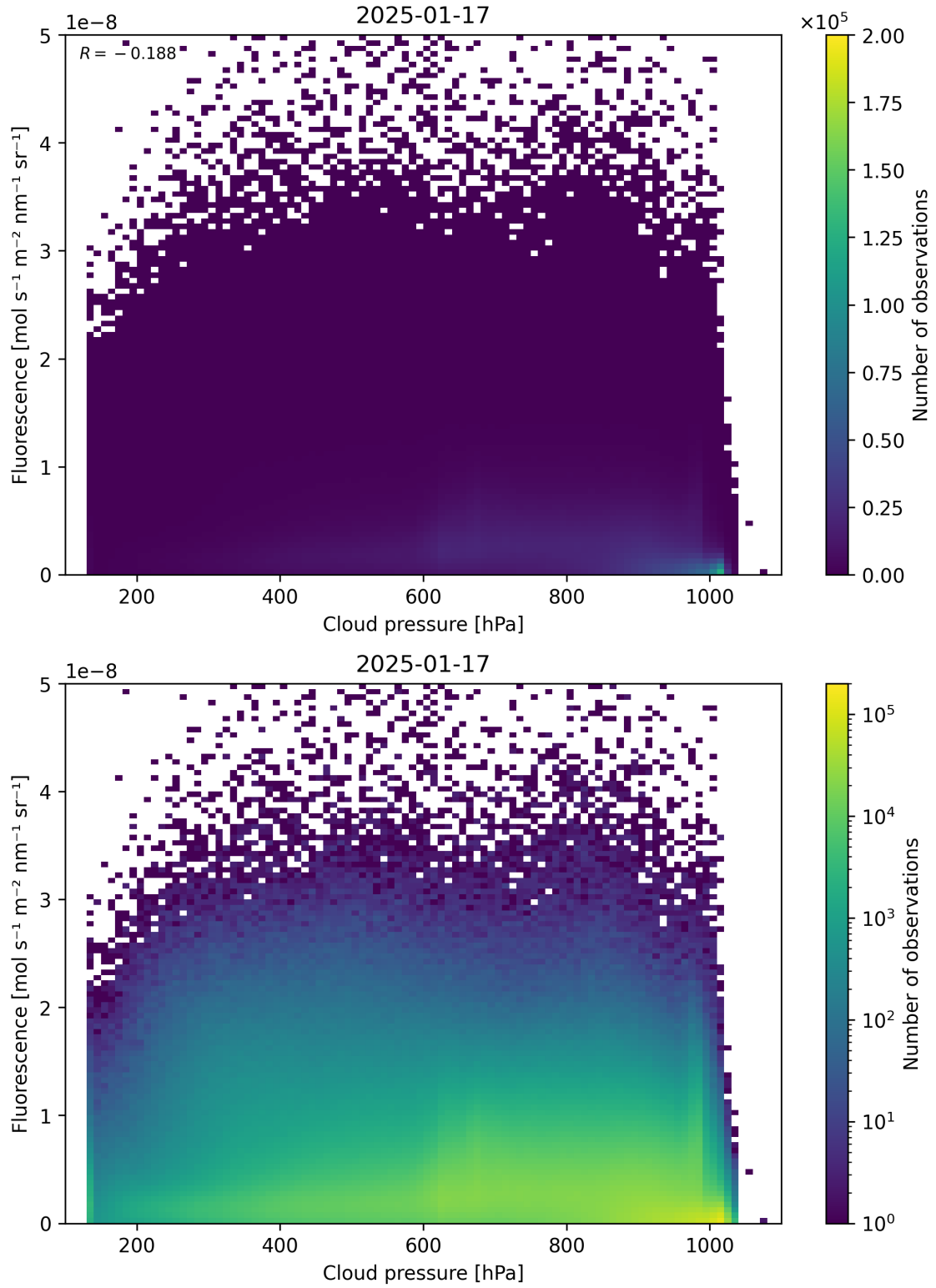
Figure 80: Scatter density plot of “Cloud pressure” against “Fluorescence” for 2025-01-17 to 2025-01-18.
