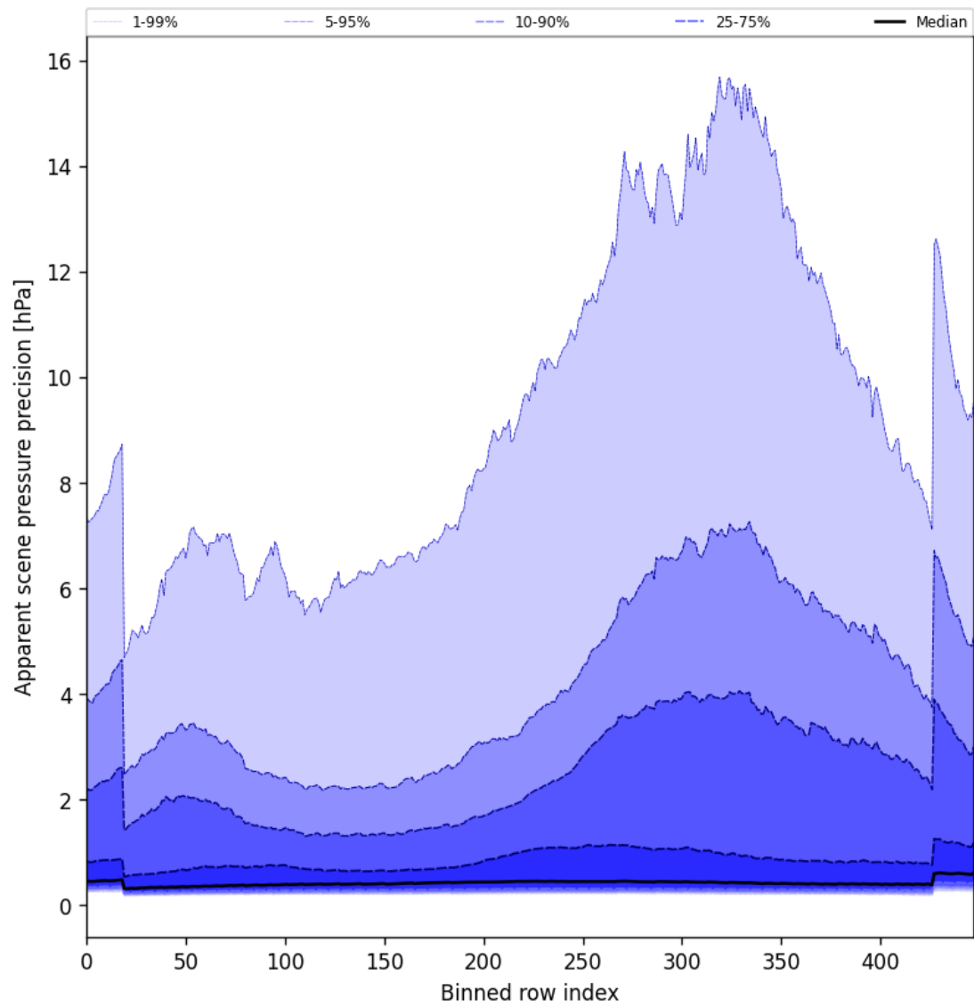
Figure 54: Along track statistics of “Apparent scene pressure precision” for 2025-01-17 to 2025-01-18
