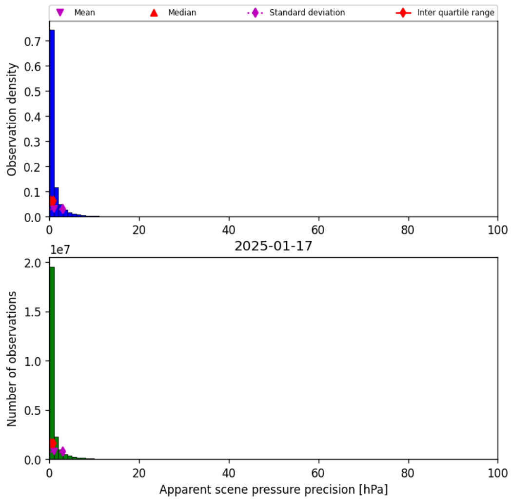
Figure 37: Histogram of “Apparent scene pressure precision” for 2025-01-17 to 2025-01-18
