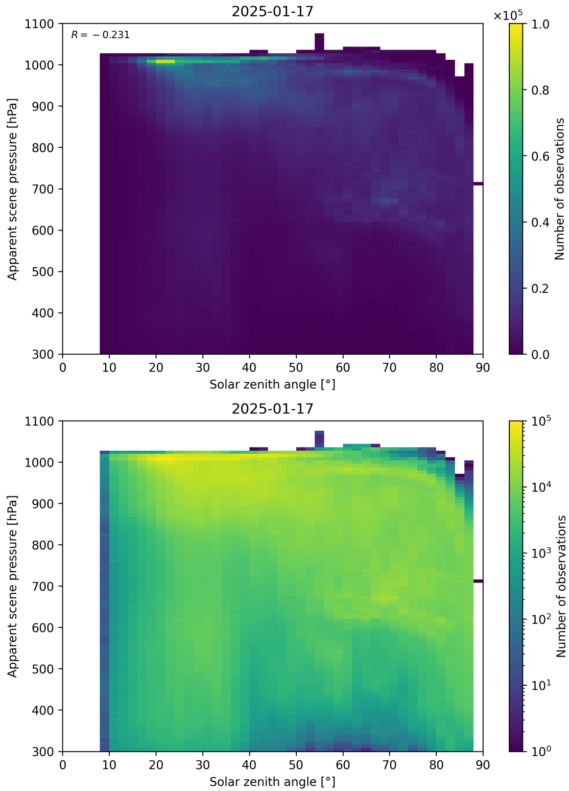
Figure 108: Scatter density plot of “Solar zenith angle” against “Apparent scene pressure” for 2025-01-17 to 2025-01-18.
