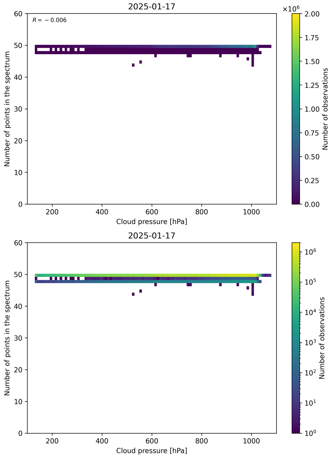
Figure 82: Scatter density plot of “Cloud pressure” against “Number of points in the spectrum” for 2025-01-17 to 2025-01-18.
