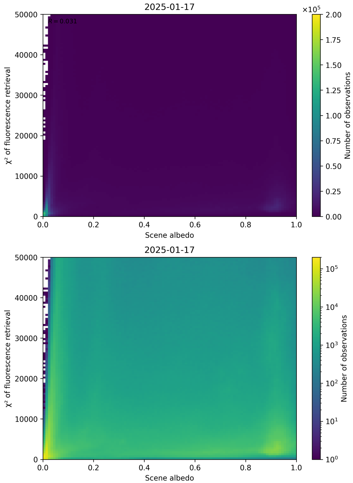
Figure 103: Scatter density plot of “Scene albedo” against “ \chi^2 of fluorescence retrieval” for 2025-01-17 to 2025-01-18.
