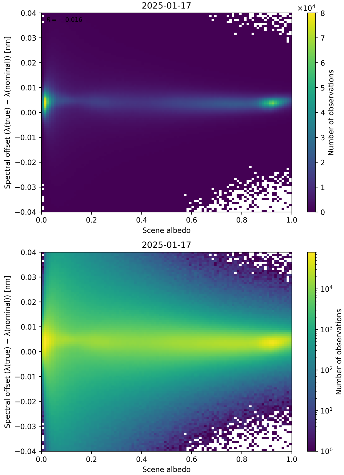
Figure 107: Scatter density plot of “Scene albedo” against “Spectral offset ( \lambda_{\text{true}} - \lambda_{\text{nominal}} )” for 2025-01-17 to 2025-01-18.
