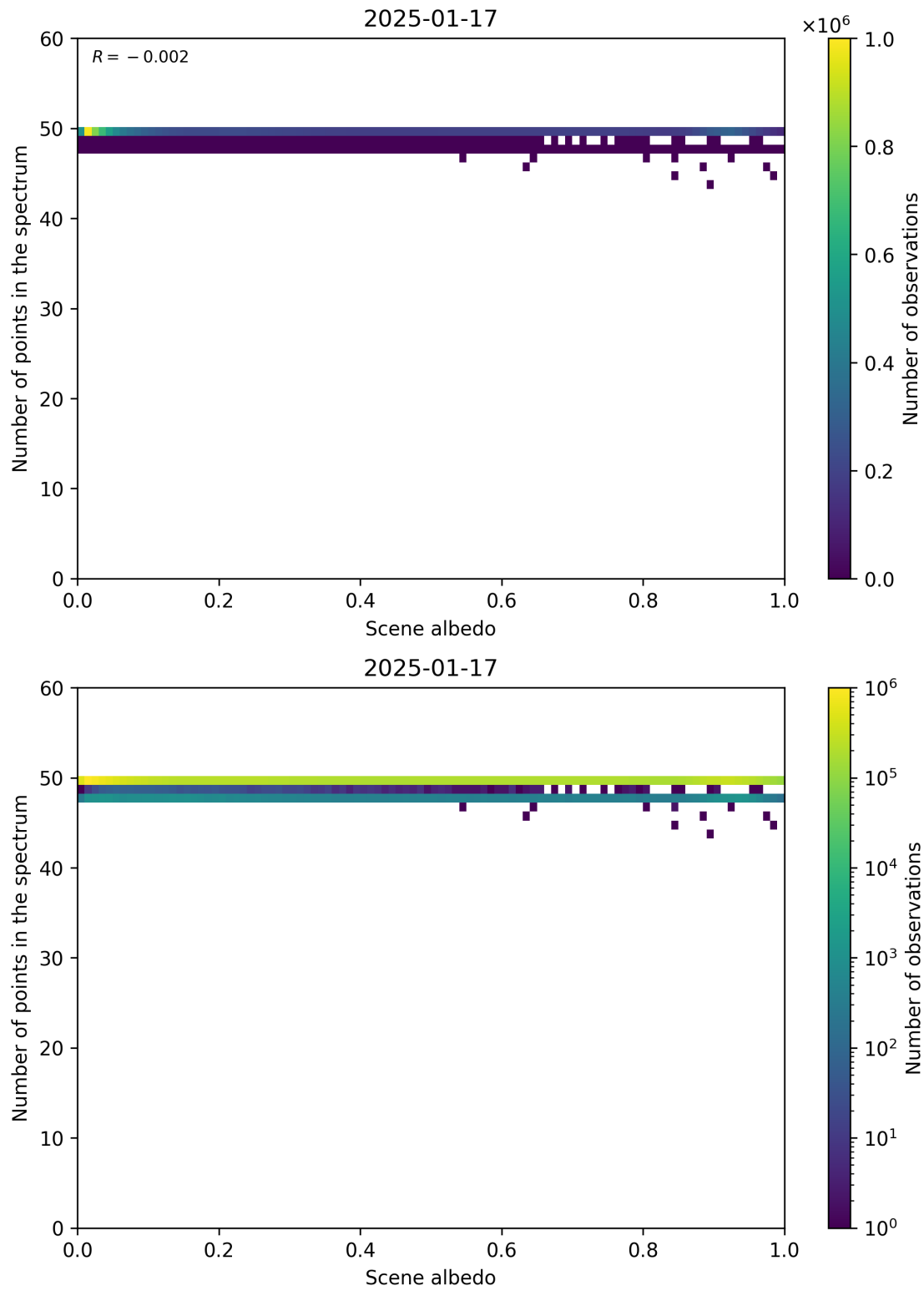
Figure 106: Scatter density plot of “Scene albedo” against “Number of points in the spectrum” for 2025-01-17 to 2025-01-18.
