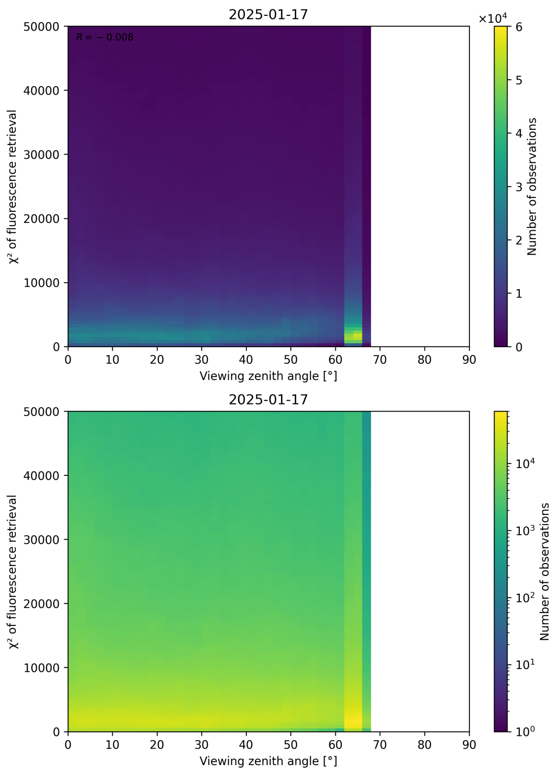
Figure 119: Scatter density plot of “Viewing zenith angle” against “ \chi^2 of fluorescence retrieval” for 2025-01-17 to 2025-01-18.
