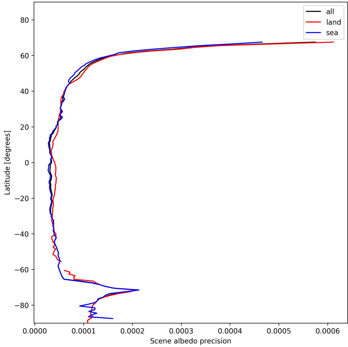
Figure 18: Zonal average of “Scene albedo precision” for 2025-01-17 to 2025-01-18.
