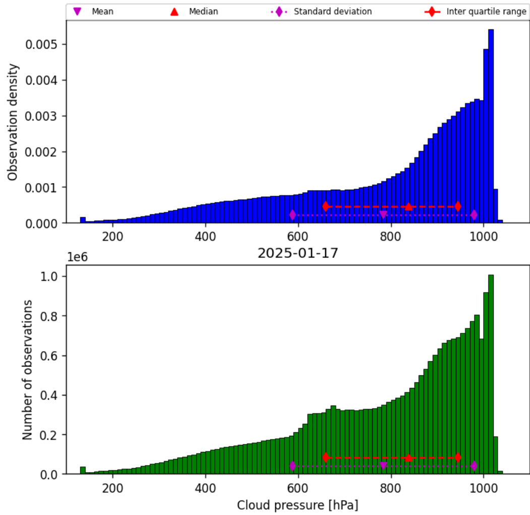
Figure 30: Histogram of “Cloud pressure” for 2025-01-17 to 2025-01-18
