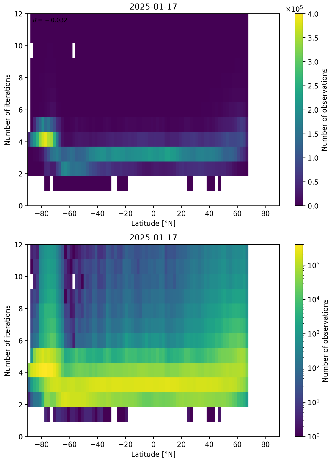
Figure 93: Scatter density plot of “Latitude” against “Number of iterations” for 2025-01-17 to 2025-01-18.
