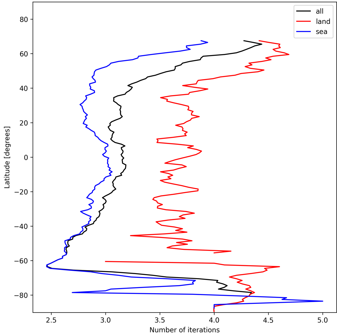
Figure 22: Zonal average of “Number of iterations” for 2025-01-17 to 2025-01-18.
