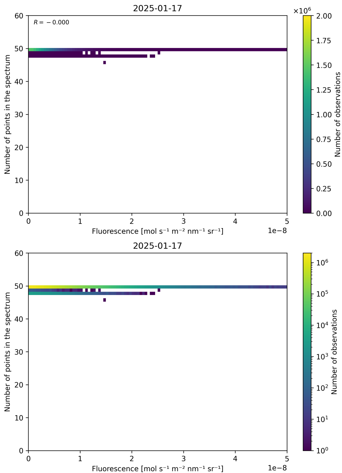
Figure 86: Scatter density plot of “Fluorescence” against “Number of points in the spectrum” for 2025-01-17 to 2025-01-18.
