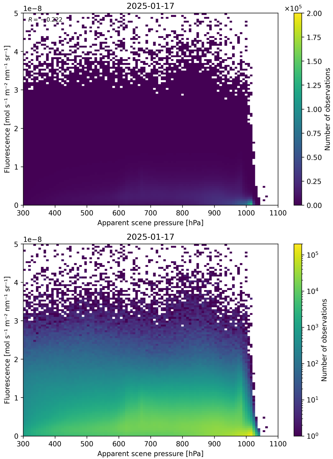
Figure 64: Scatter density plot of “Apparent scene pressure” against “Fluorescence” for 2025-01-17 to 2025-01-18.
