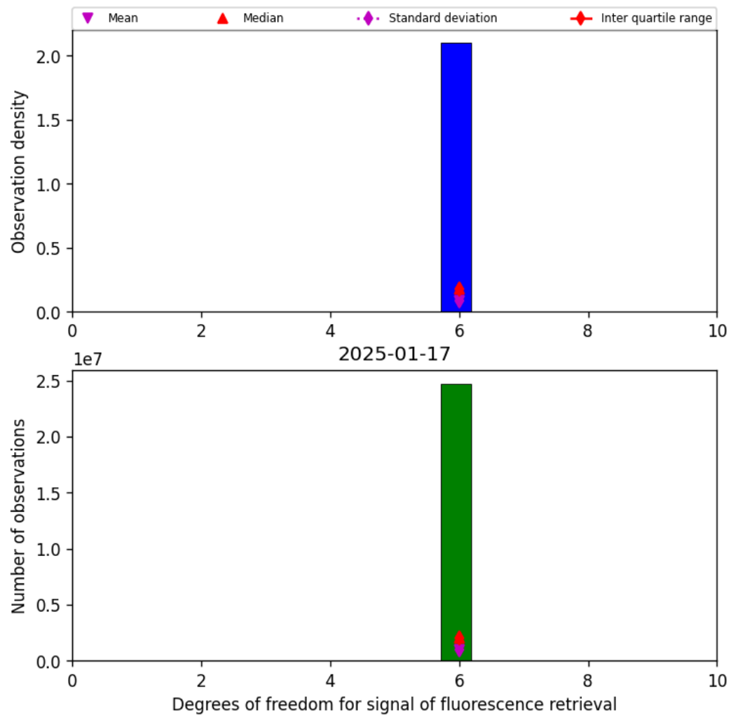
Figure 43: Histogram of “Degrees of freedom for signal of fluorescence retrieval” for 2025-01-17 to 2025-01-18
