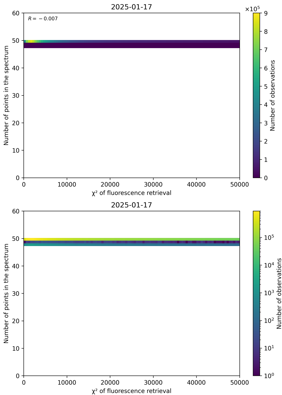
Figure 68: Scatter density plot of “ \chi^2 of fluorescence retrieval” against “Number of points in the spectrum” for 2025-01-17 to 2025-01-18.
