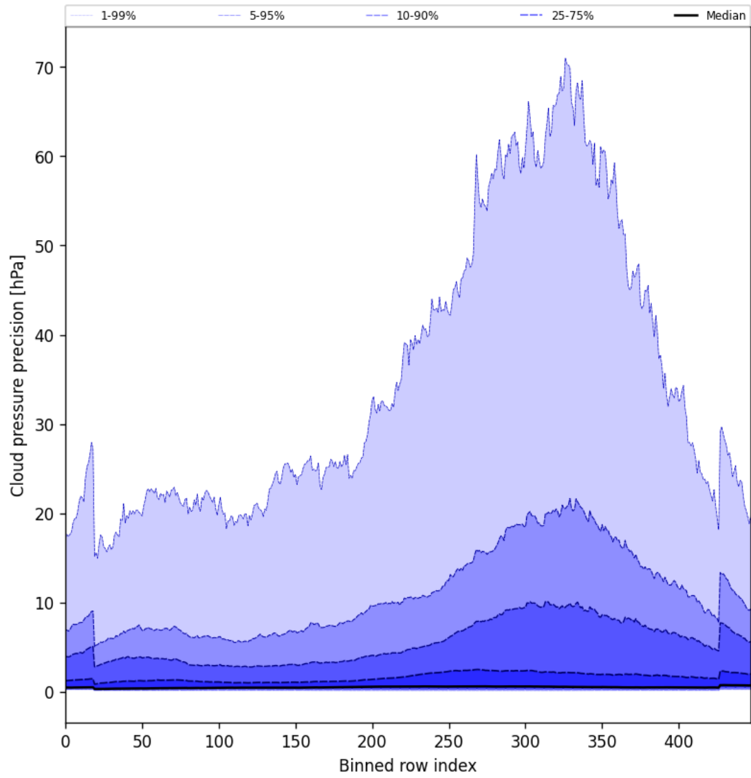
Figure 48: Along track statistics of “Cloud pressure precision” for 2025-01-17 to 2025-01-18
