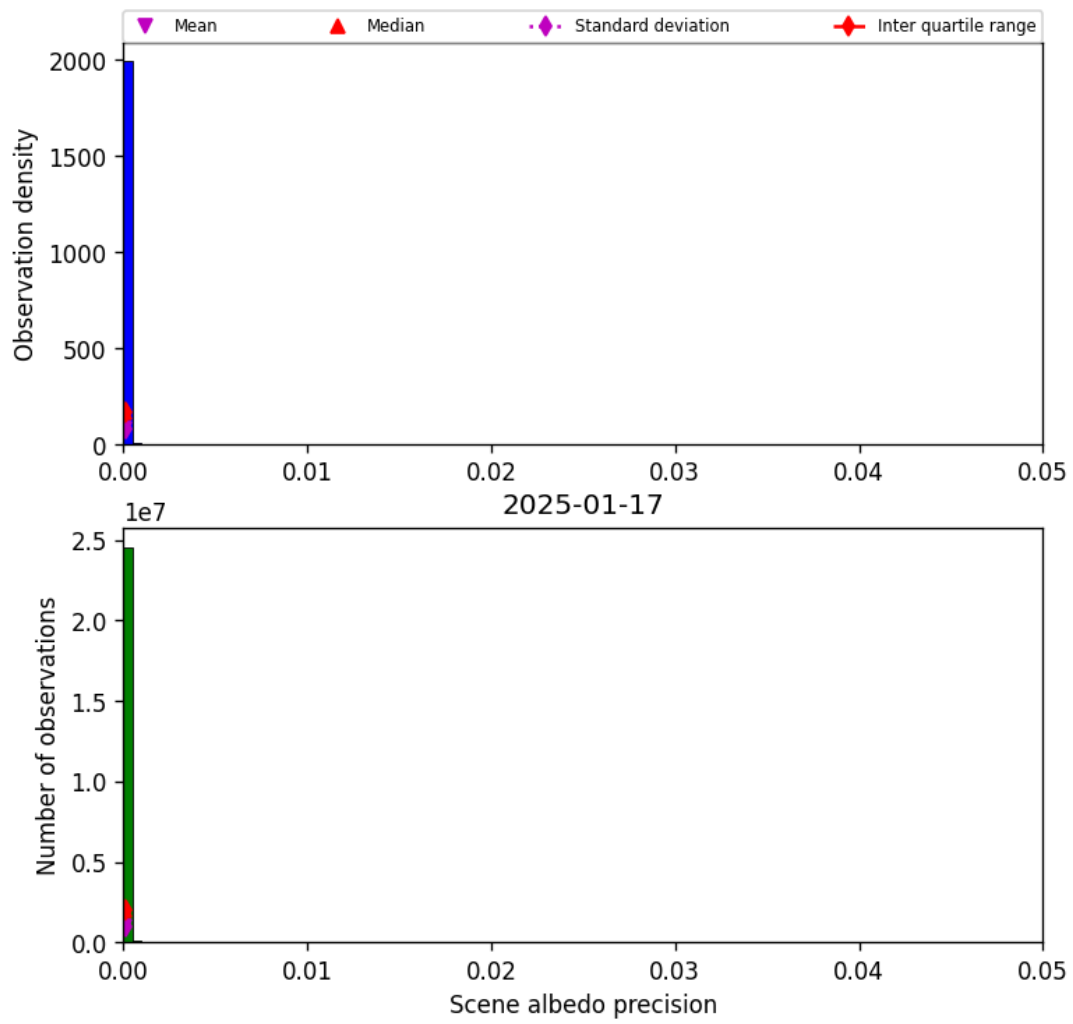
Figure 35: Histogram of “Scene albedo precision” for 2025-01-17 to 2025-01-18
