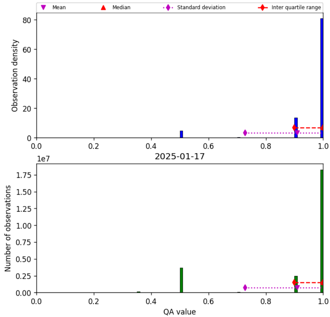
Figure 29: Histogram of “QA value” for 2025-01-17 to 2025-01-18
