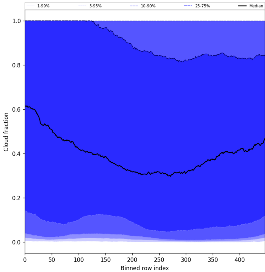
Figure 49: Along track statistics of “Cloud fraction” for 2025-01-17 to 2025-01-18
