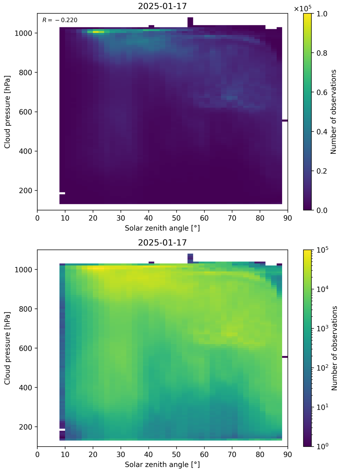
Figure 111: Scatter density plot of “Solar zenith angle” against “Cloud pressure” for 2025-01-17 to 2025-01-18.
