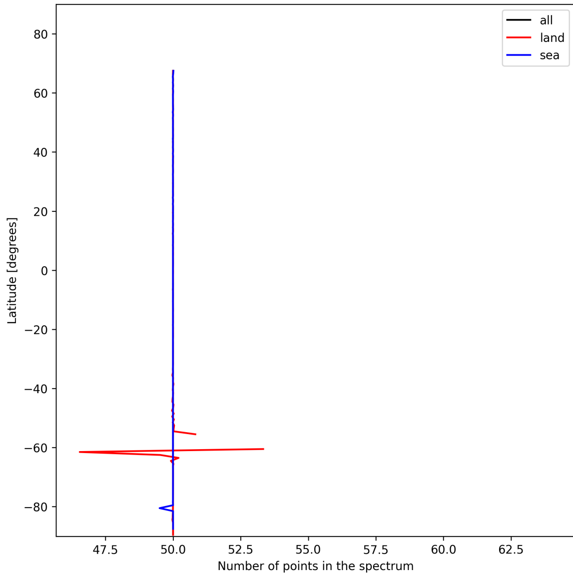
Figure 27: Zonal average of “Number of points in the spectrum” for 2025-01-17 to 2025-01-18.
