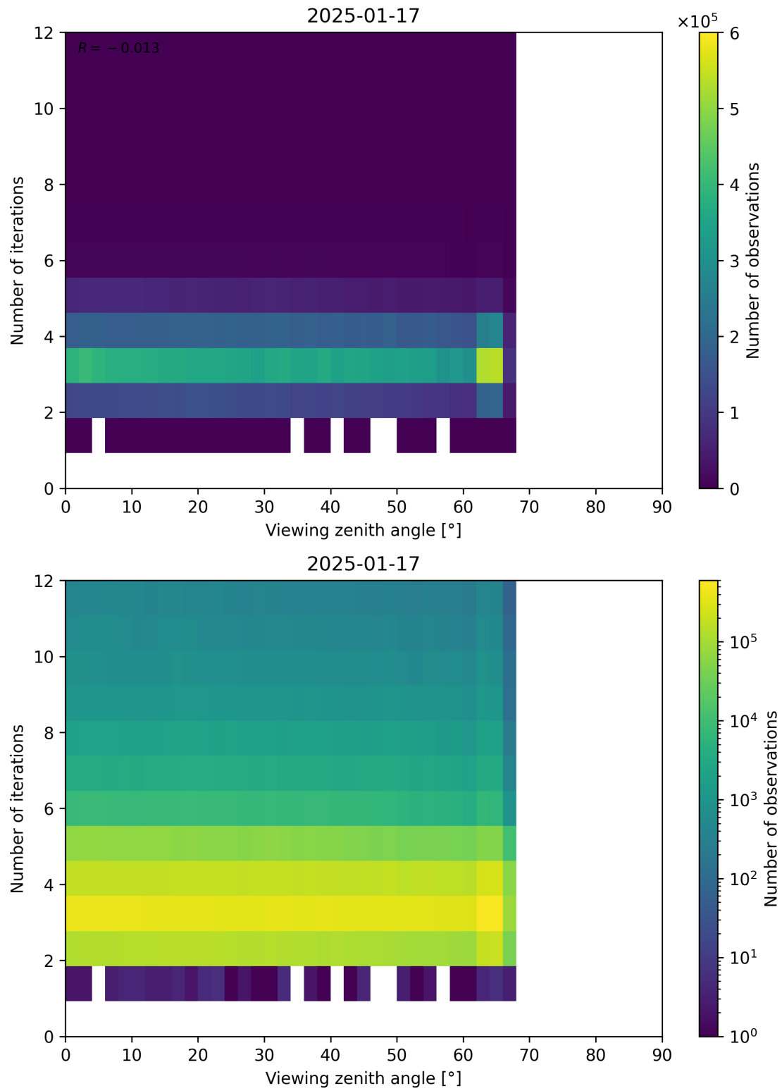
Figure 124: Scatter density plot of “Viewing zenith angle” against “Number of iterations” for 2025-01-17 to 2025-01-18.
