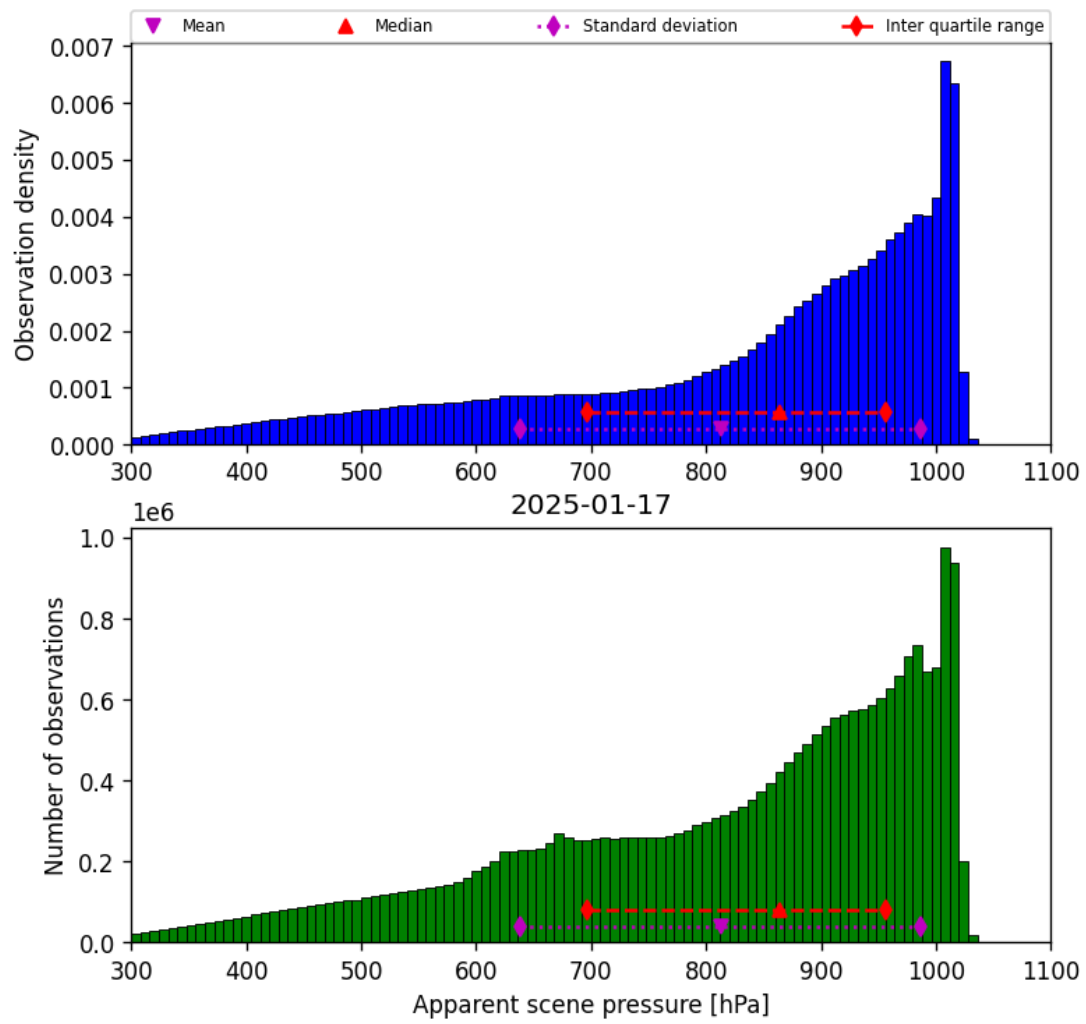
Figure 36: Histogram of “Apparent scene pressure” for 2025-01-17 to 2025-01-18
