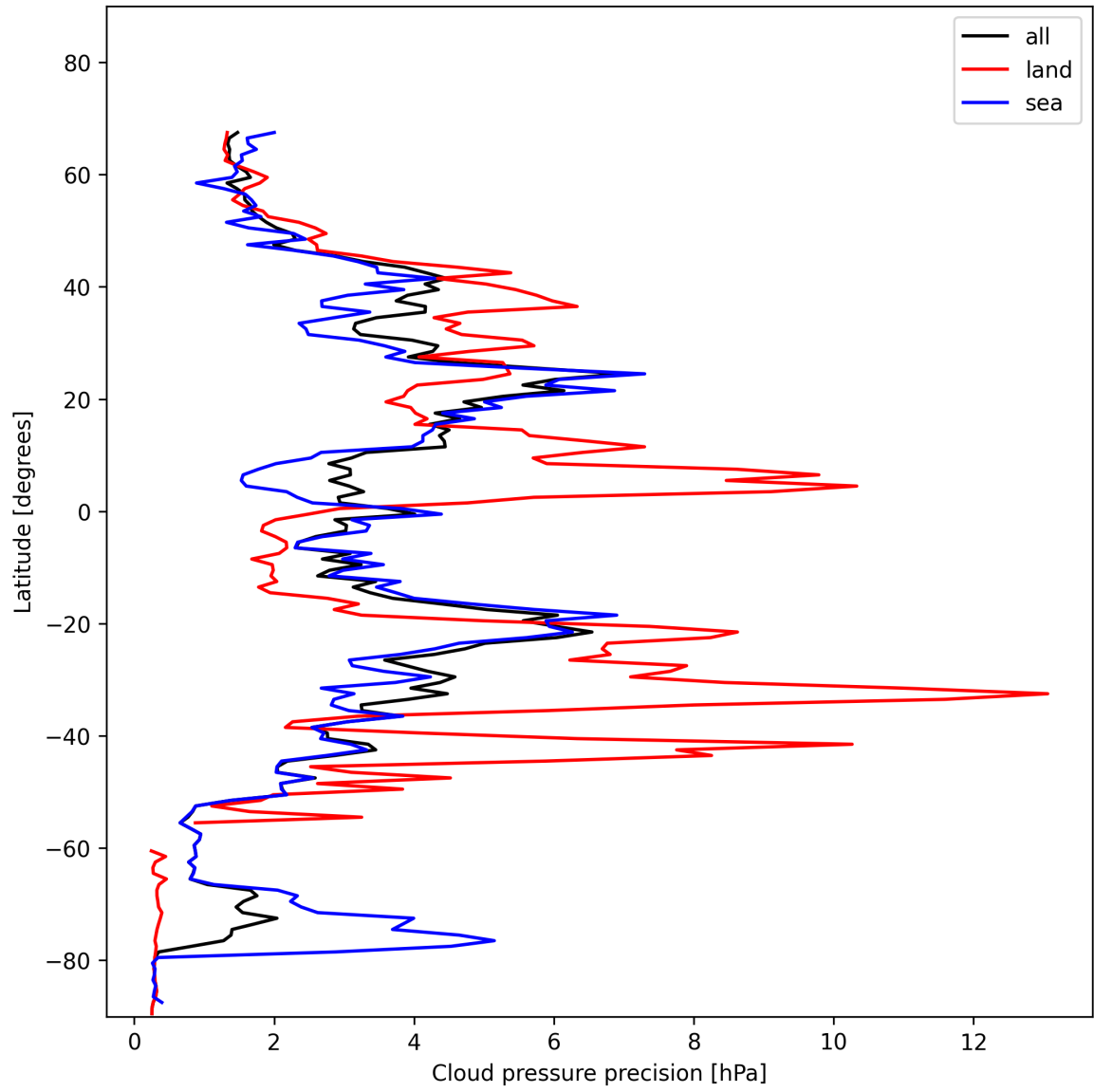
Figure 14: Zonal average of "Cloud pressure precision" for 2025-01-17 to 2025-01-18.
