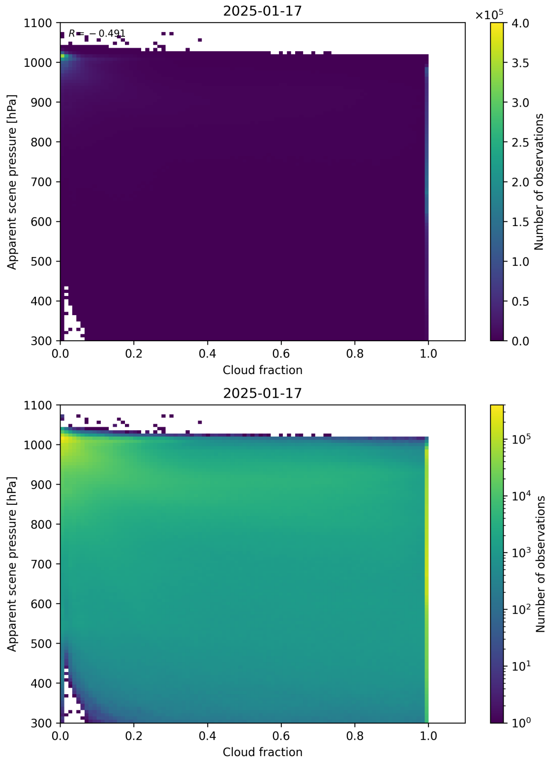
Figure 70: Scatter density plot of “Cloud fraction” against “Apparent scene pressure” for 2025-01-17 to 2025-01-18.
