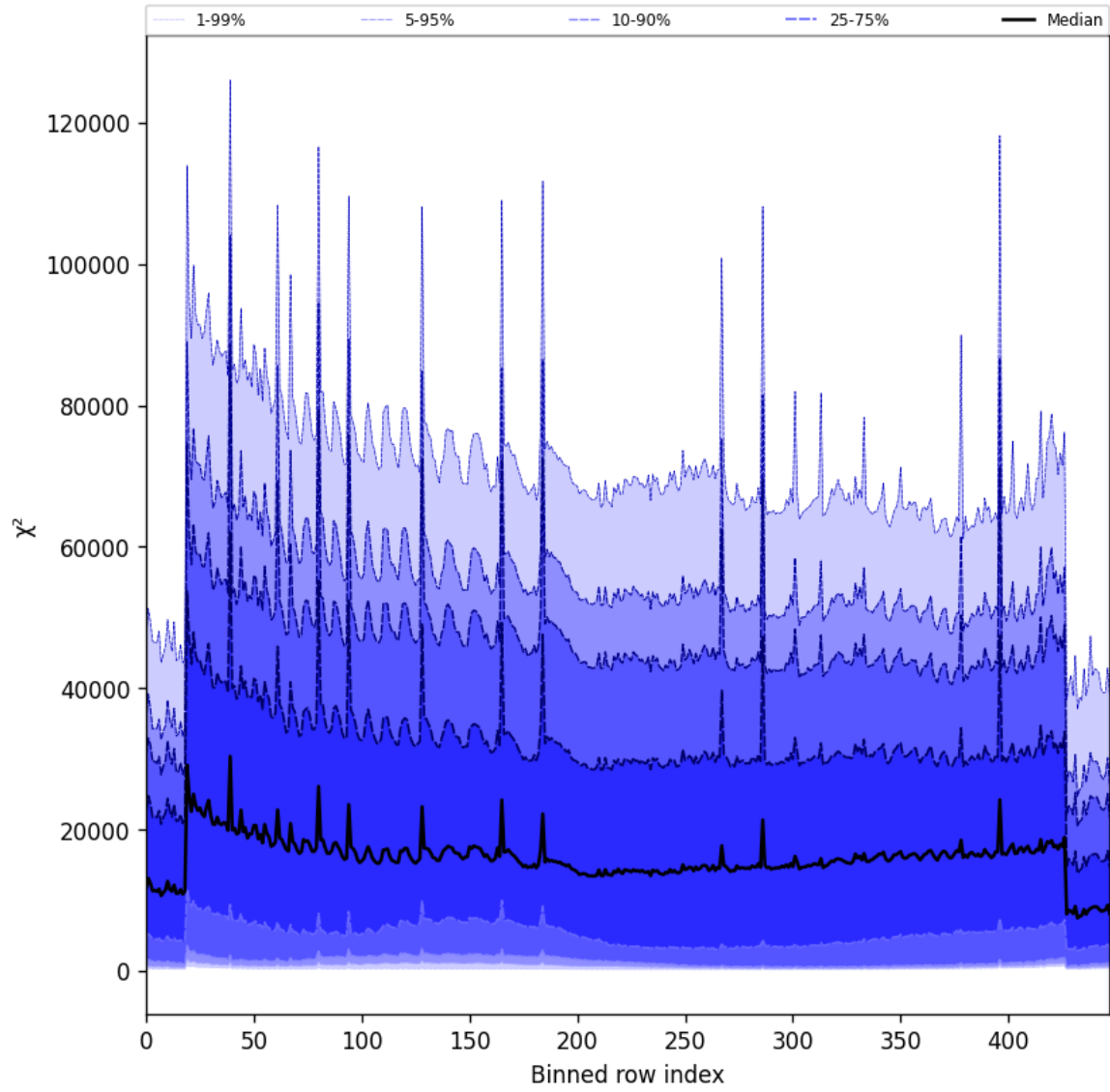
Figure 55: Along track statistics of “ \chi^2 ” for 2025-01-17 to 2025-01-18
