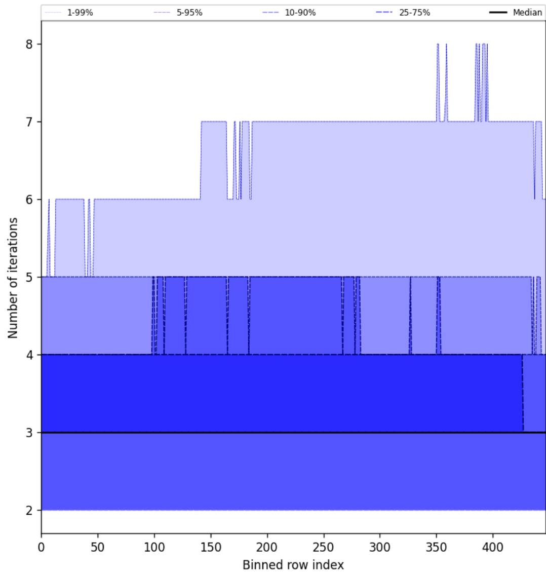
Figure 56: Along track statistics of “Number of iterations” for 2025-01-17 to 2025-01-18
