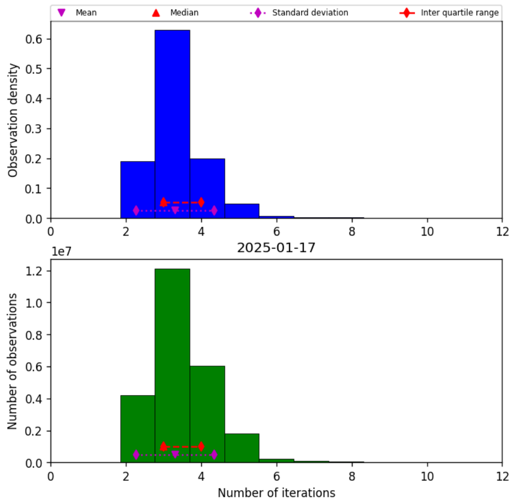
Figure 39: Histogram of “Number of iterations” for 2025-01-17 to 2025-01-18
