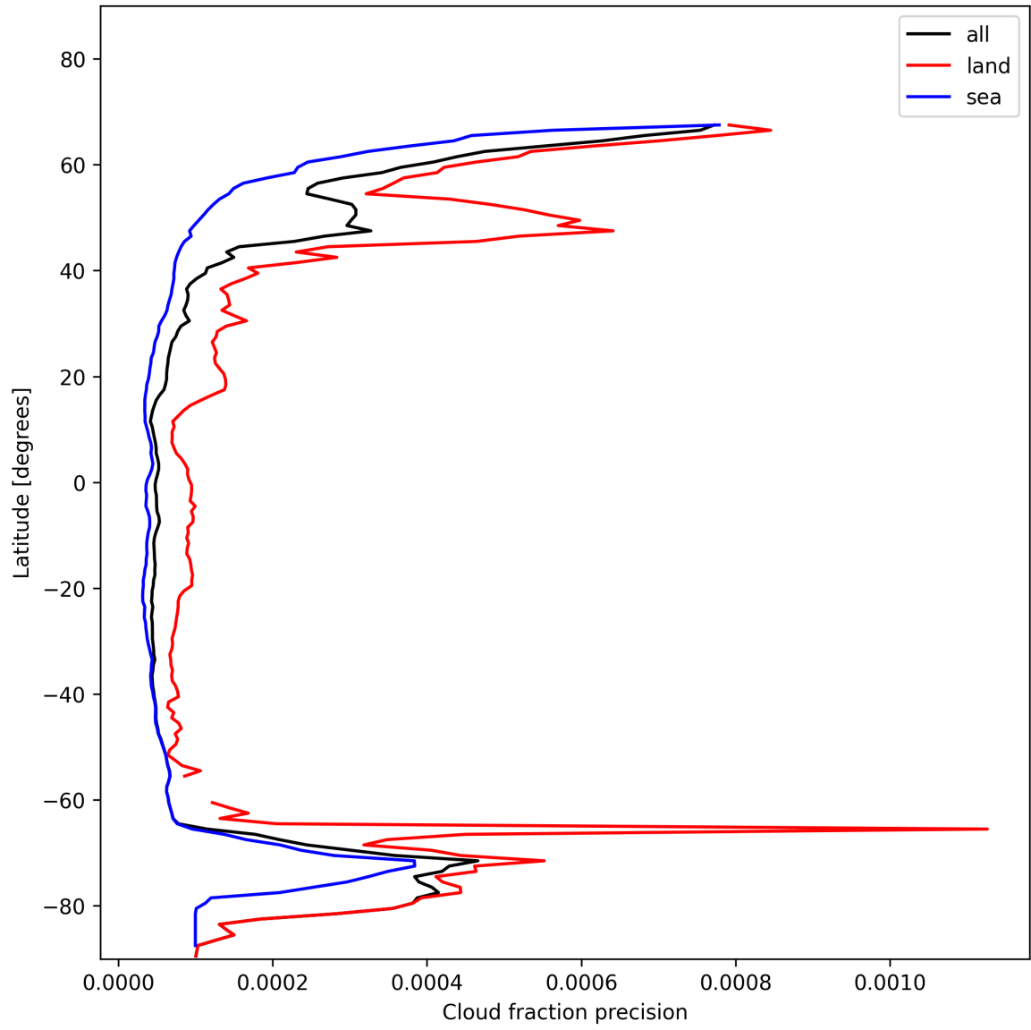
Figure 16: Zonal average of “Cloud fraction precision” for 2025-01-17 to 2025-01-18.
