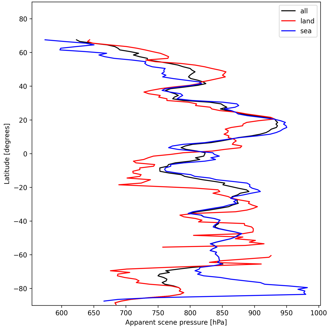
Figure 19: Zonal average of “Apparent scene pressure” for 2025-01-17 to 2025-01-18.
