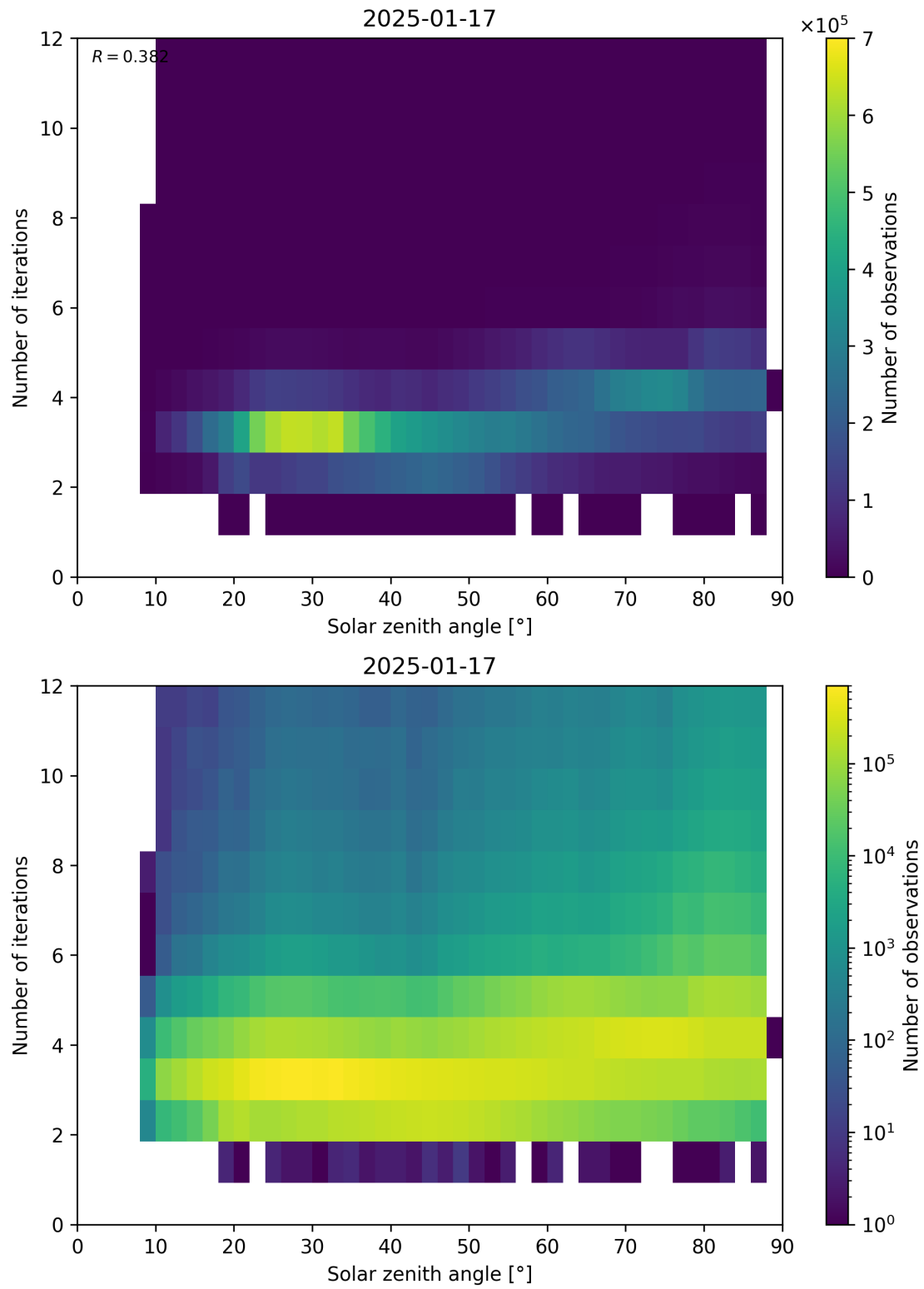
Figure 114: Scatter density plot of “Solar zenith angle” against “Number of iterations” for 2025-01-17 to 2025-01-18.
