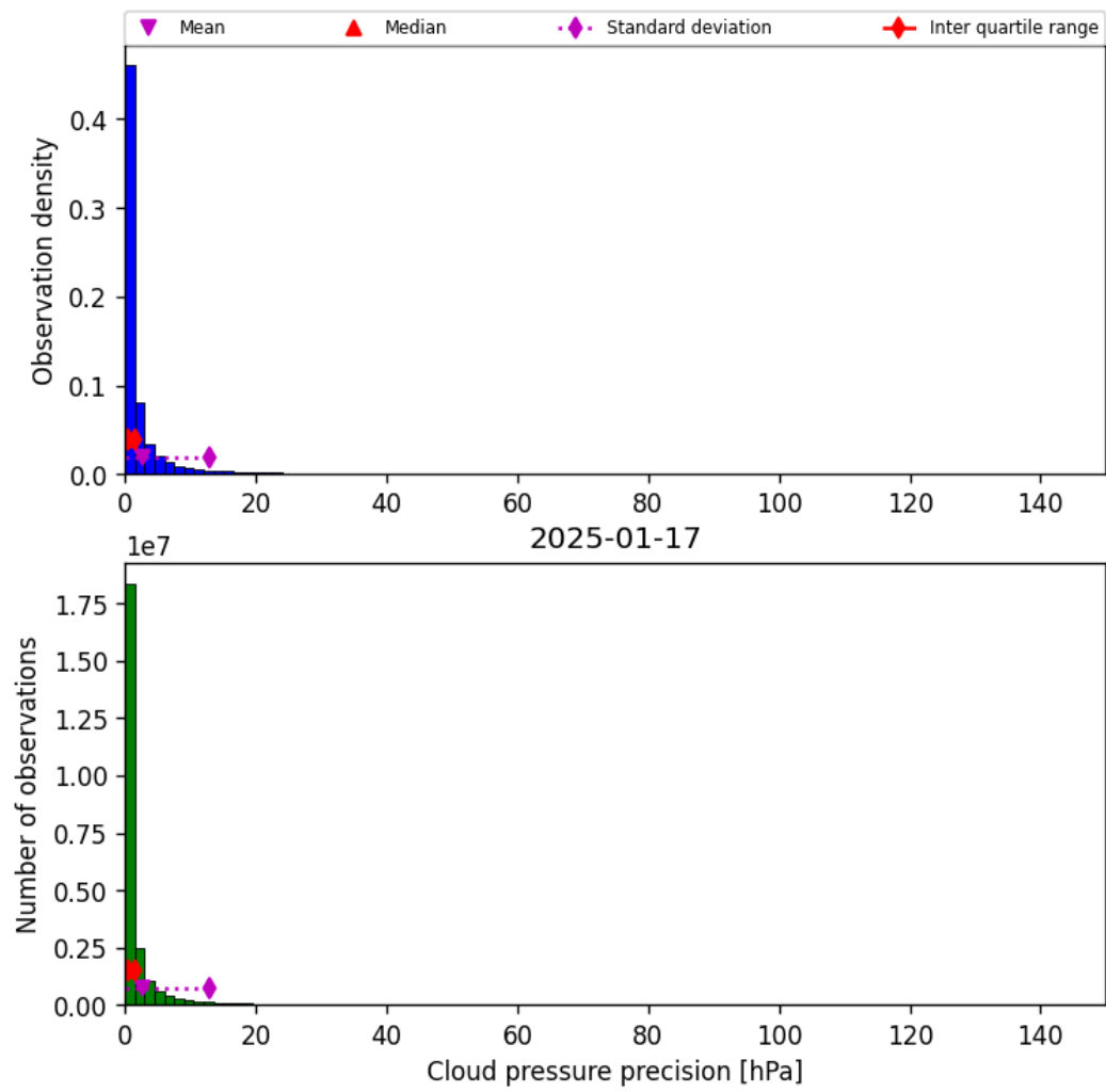
Figure 31: Histogram of “Cloud pressure precision” for 2025-01-17 to 2025-01-18
