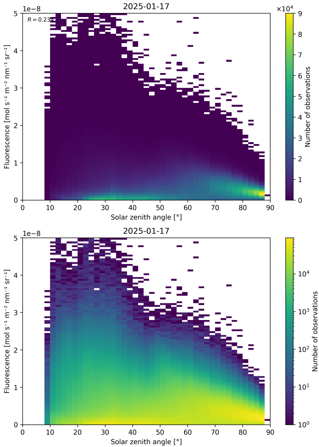
Figure 112: Scatter density plot of “Solar zenith angle” against “Fluorescence” for 2025-01-17 to 2025-01-18.
