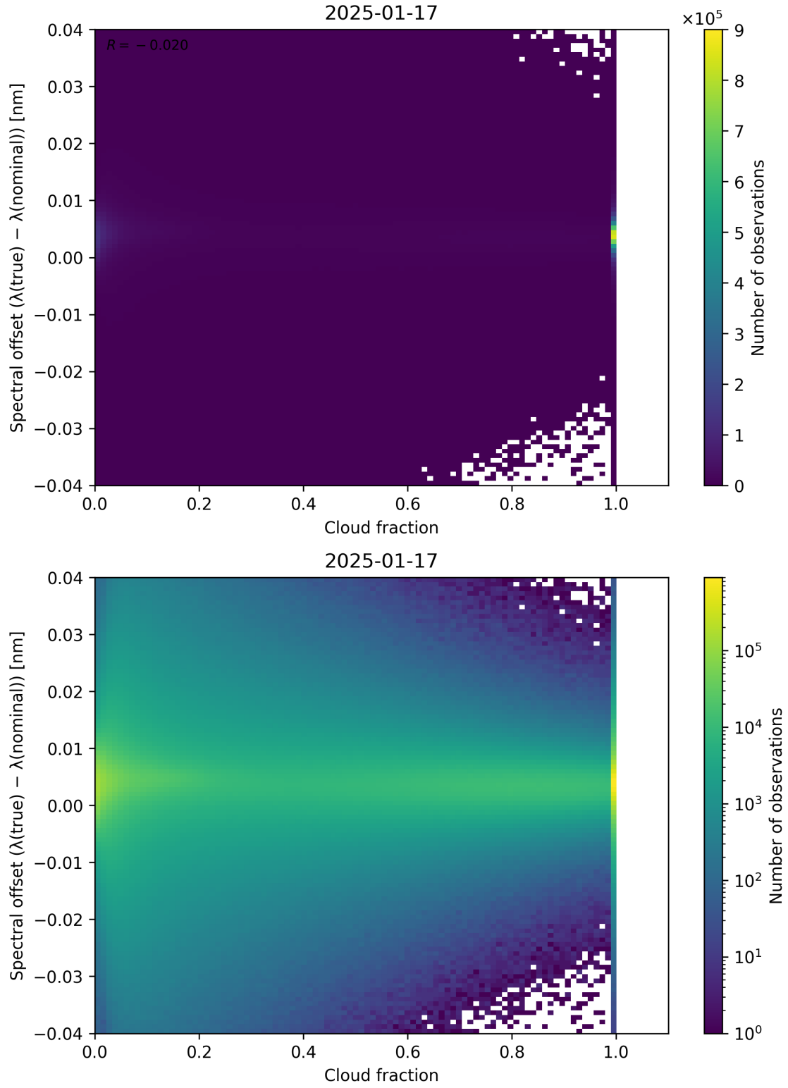
Figure 76: Scatter density plot of “Cloud fraction” against “Spectral offset ( \lambda_{\text{true}} - \lambda_{\text{nominal}} )” for 2025-01-17 to 2025-01-18.
