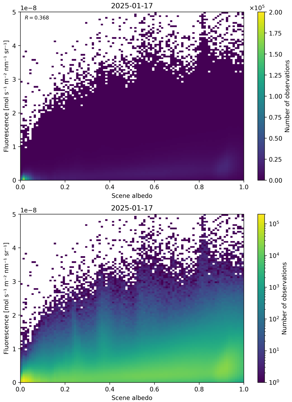
Figure 104: Scatter density plot of “Scene albedo” against “Fluorescence” for 2025-01-17 to 2025-01-18.
