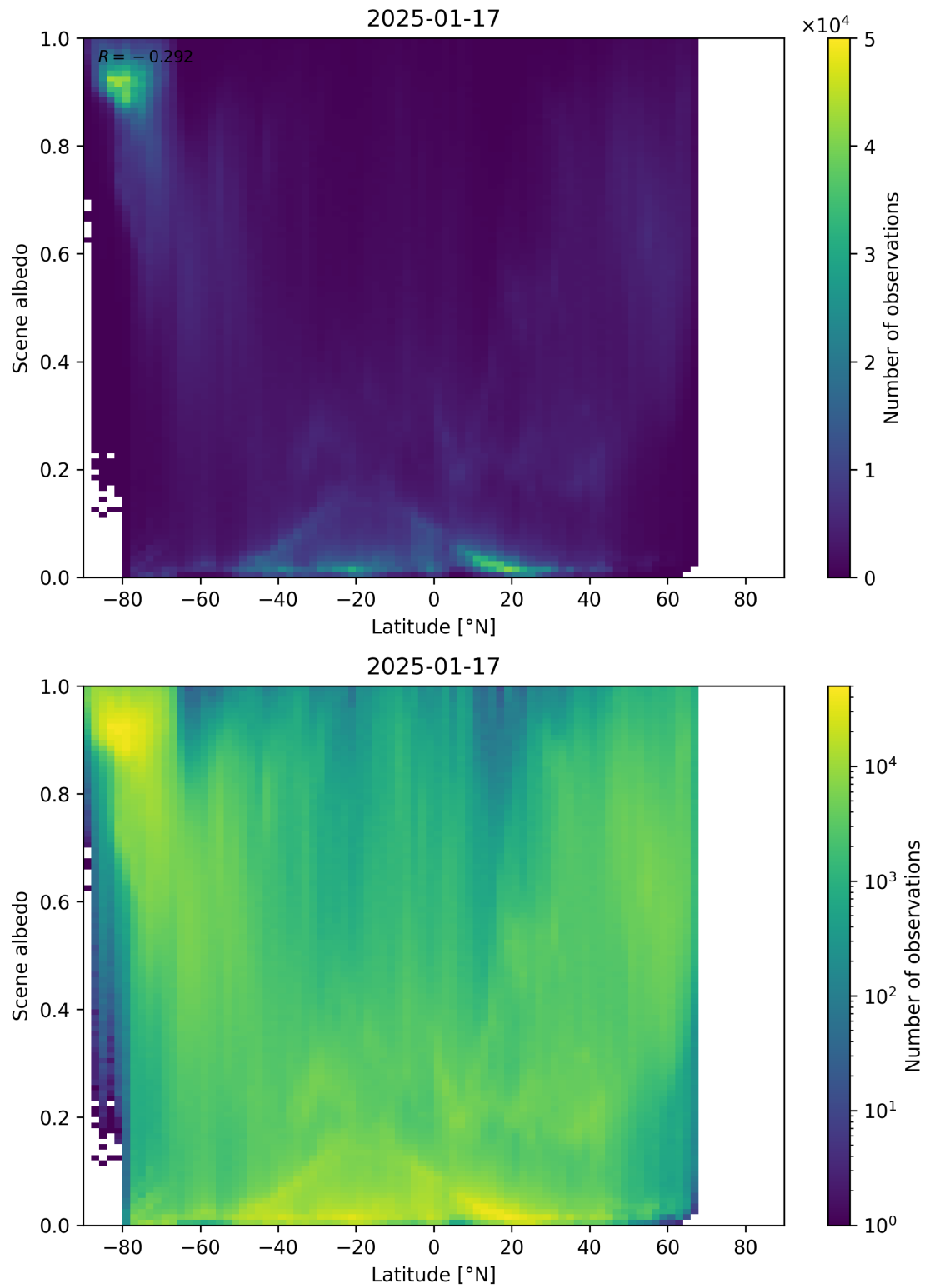
Figure 95: Scatter density plot of “Latitude” against “Scene albedo” for 2025-01-17 to 2025-01-18.
