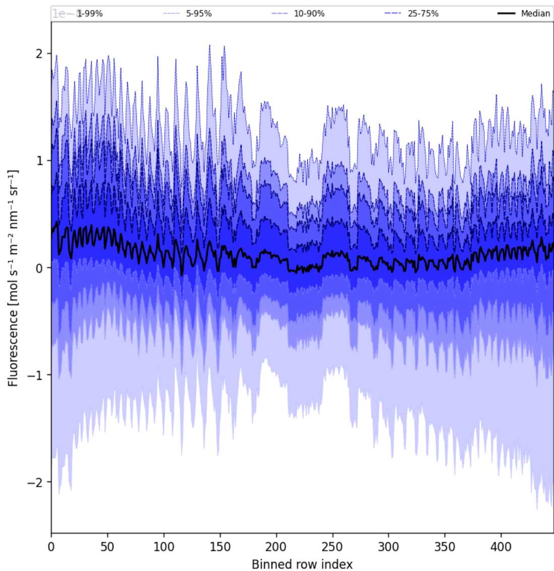
Figure 57: Along track statistics of “Fluorescence” for 2025-01-17 to 2025-01-18
