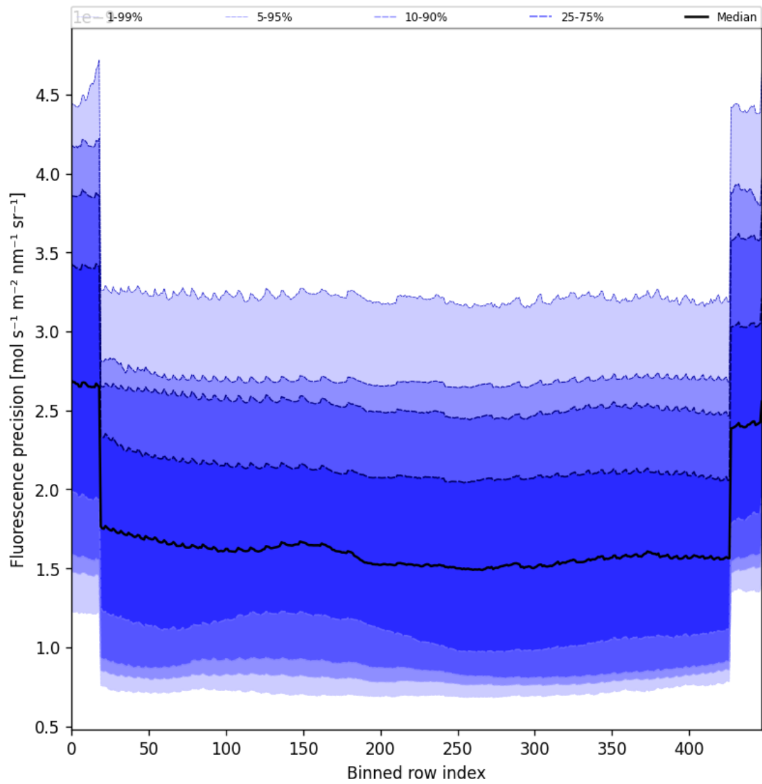
Figure 58: Along track statistics of “Fluorescence precision” for 2025-01-17 to 2025-01-18
