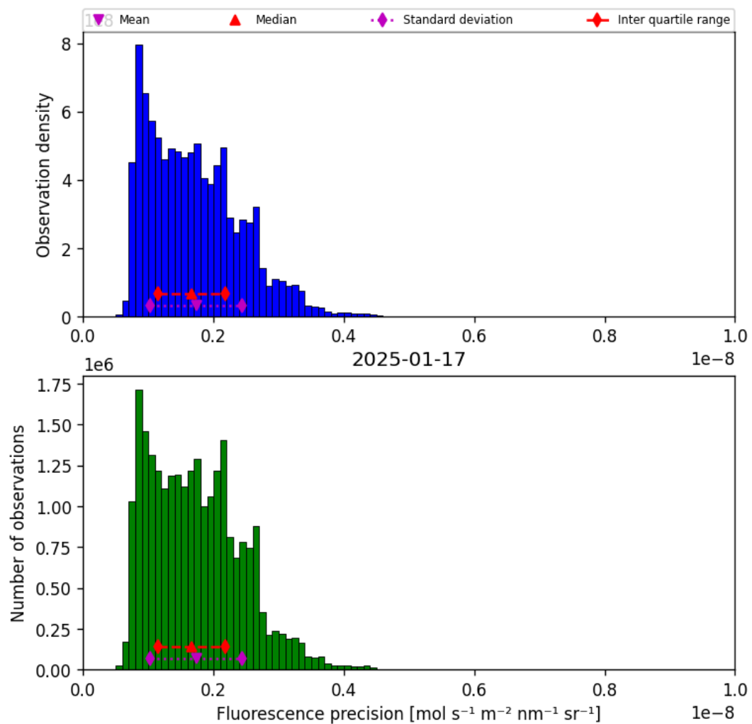
Figure 41: Histogram of “Fluorescence precision” for 2025-01-17 to 2025-01-18
