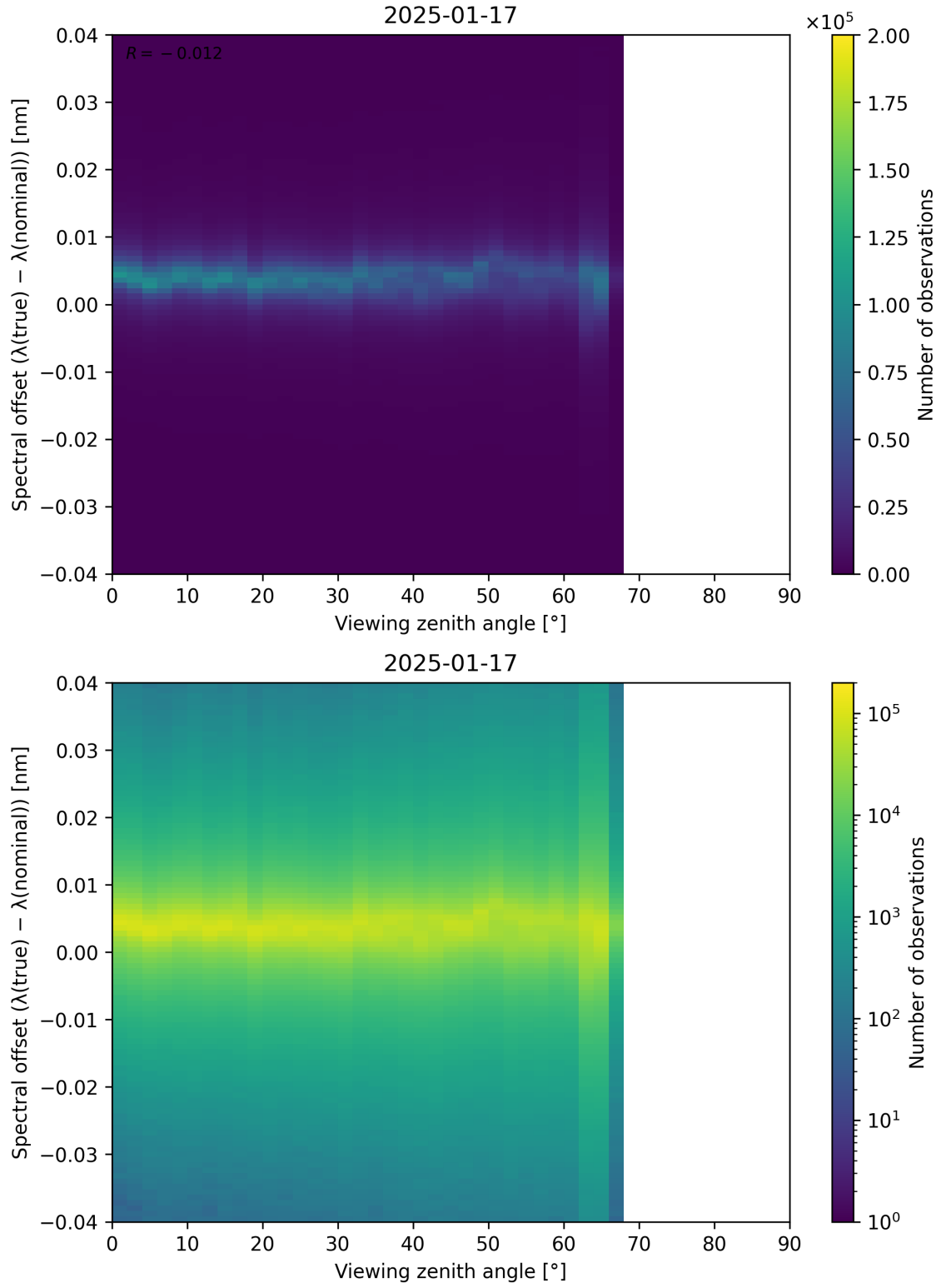
Figure 128: Scatter density plot of “Viewing zenith angle” against “Spectral offset ( \lambda_{\text{true}} - \lambda_{\text{nominal}} )” for 2025-01-17 to 2025-01-18.
