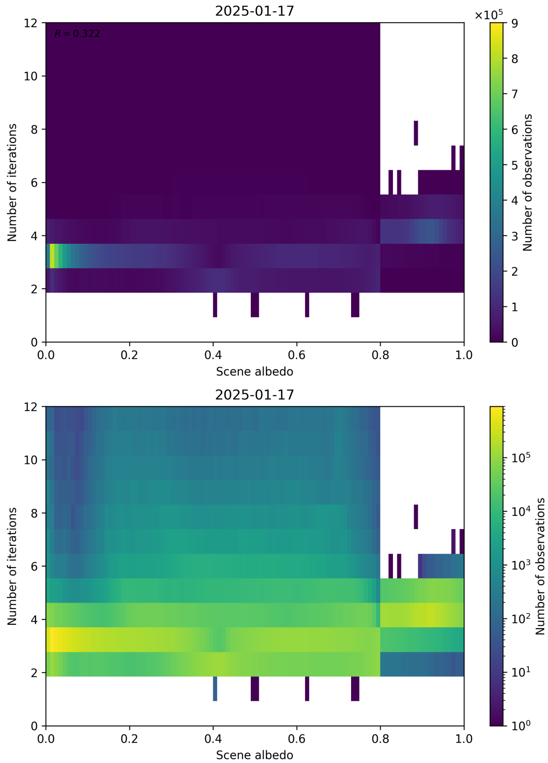
Figure 105: Scatter density plot of “Scene albedo” against “Number of iterations” for 2025-01-17 to 2025-01-18.
