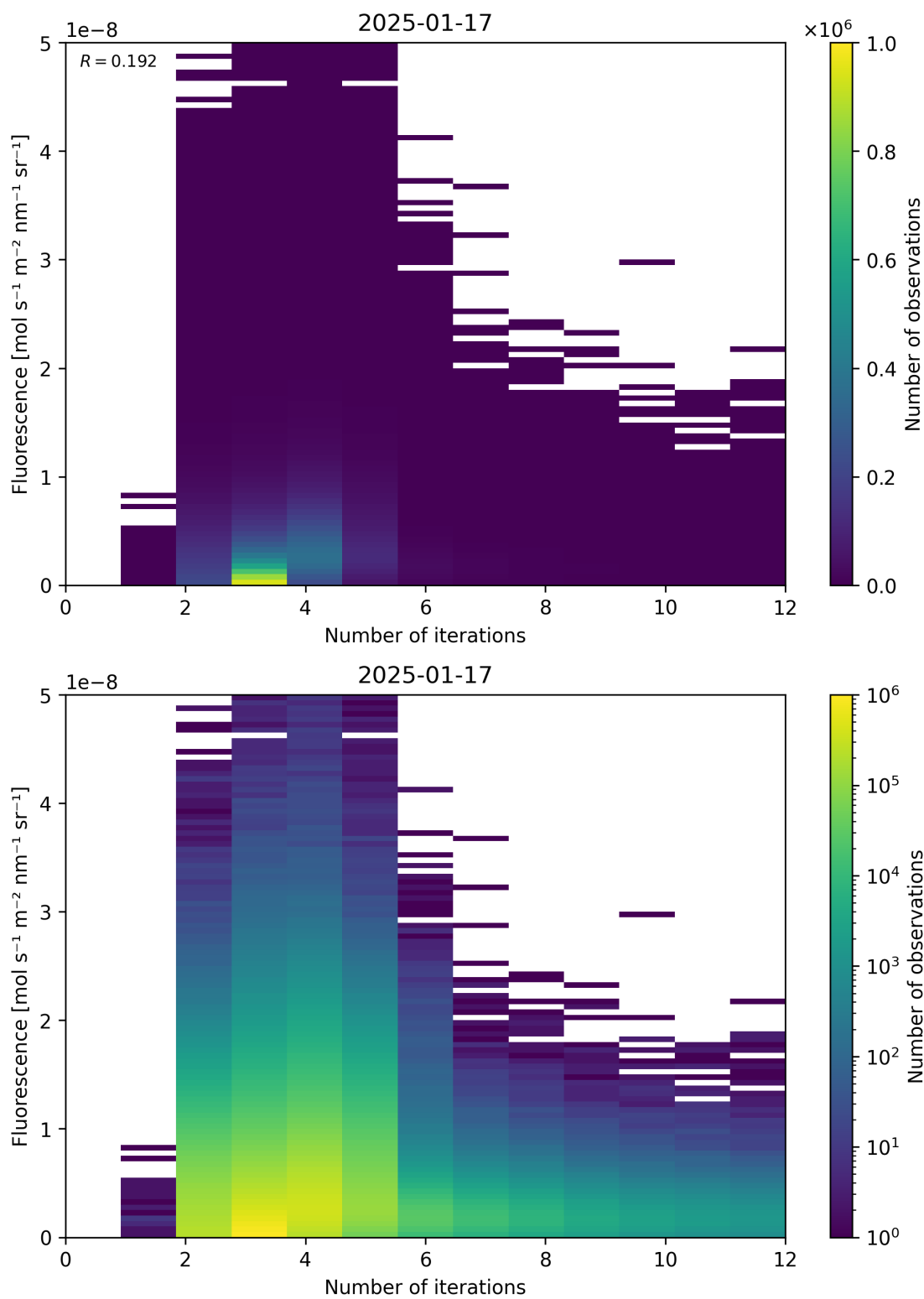
Figure 98: Scatter density plot of “Number of iterations” against “Fluorescence” for 2025-01-17 to 2025-01-18.
