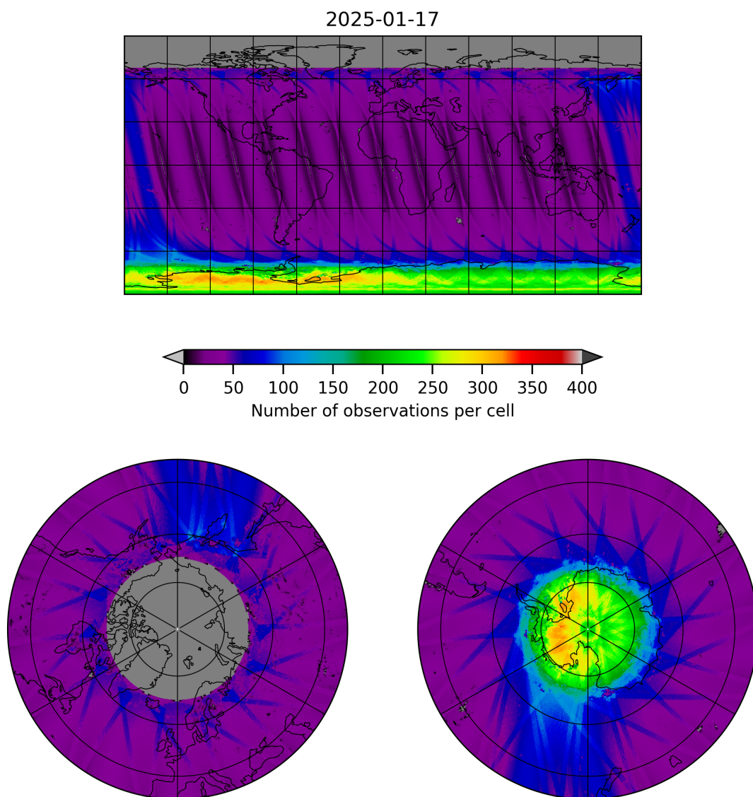
Figure 11: Map of the number of observations for 2025-01-17 to 2025-01-18
