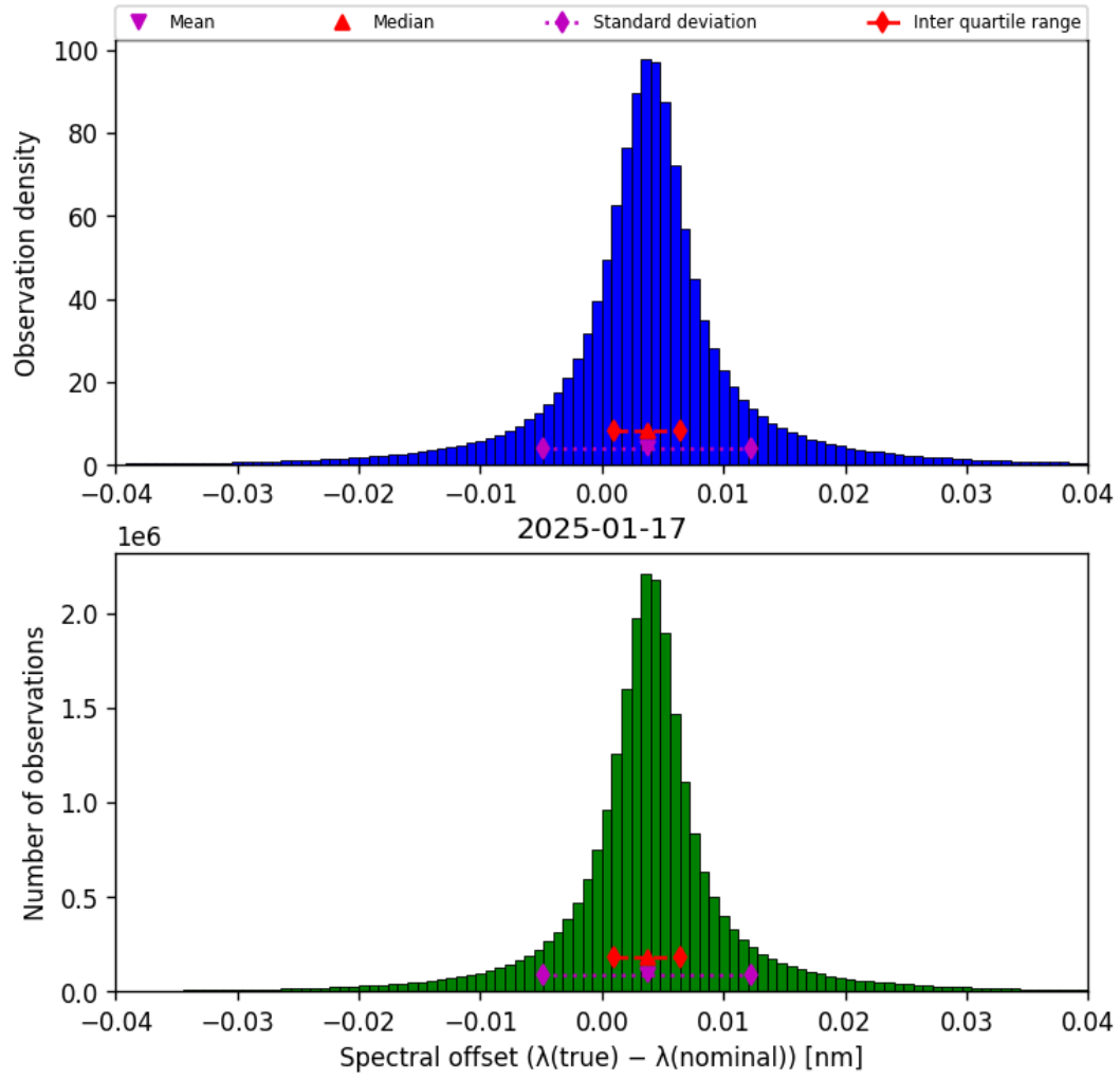
Figure 45: Histogram of “Spectral offset ( \lambda_{\text{true}} - \lambda_{\text{nominal}} )” for 2025-01-17 to 2025-01-18
