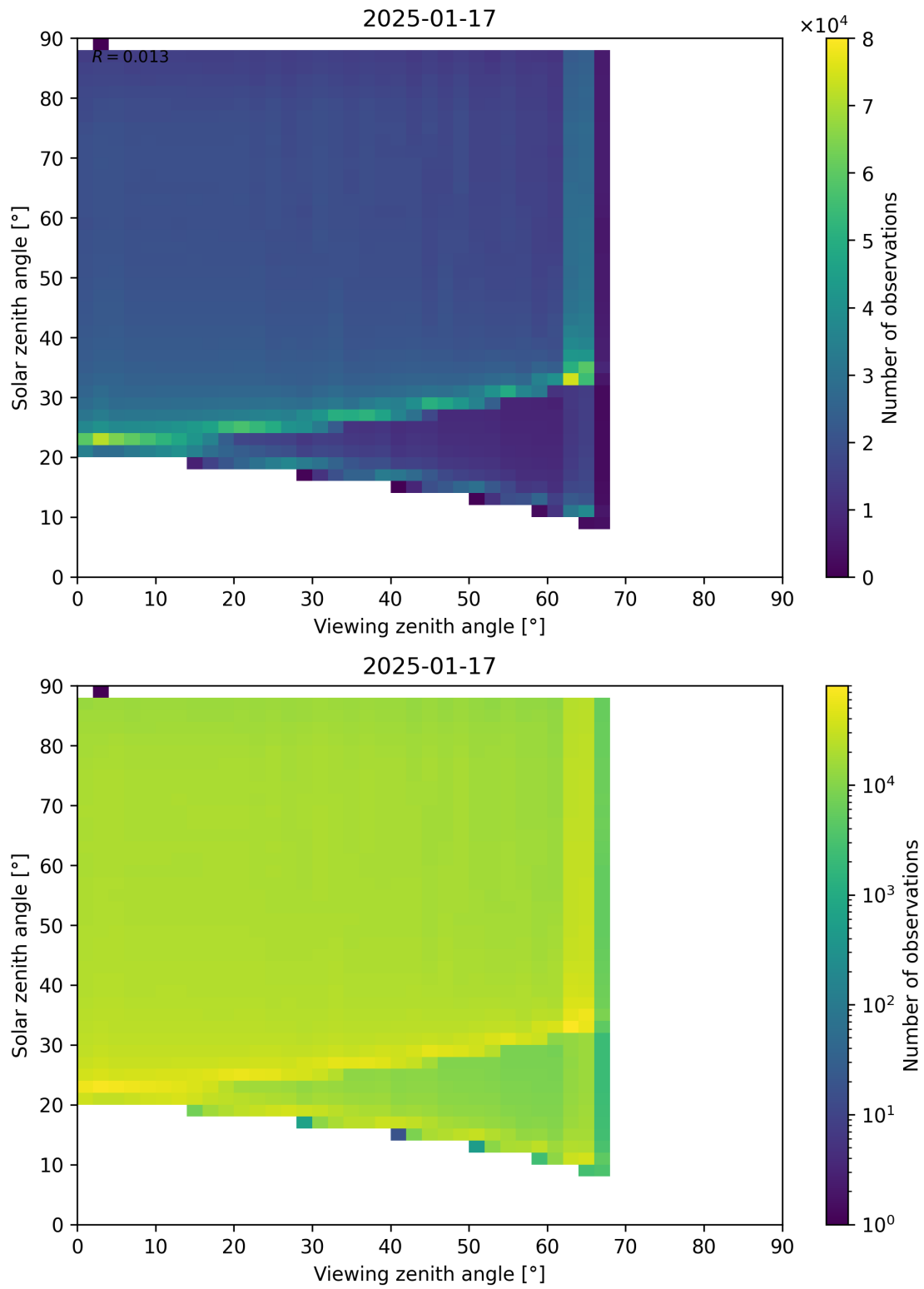
Figure 127: Scatter density plot of “Viewing zenith angle” against “Solar zenith angle” for 2025-01-17 to 2025-01-18.
