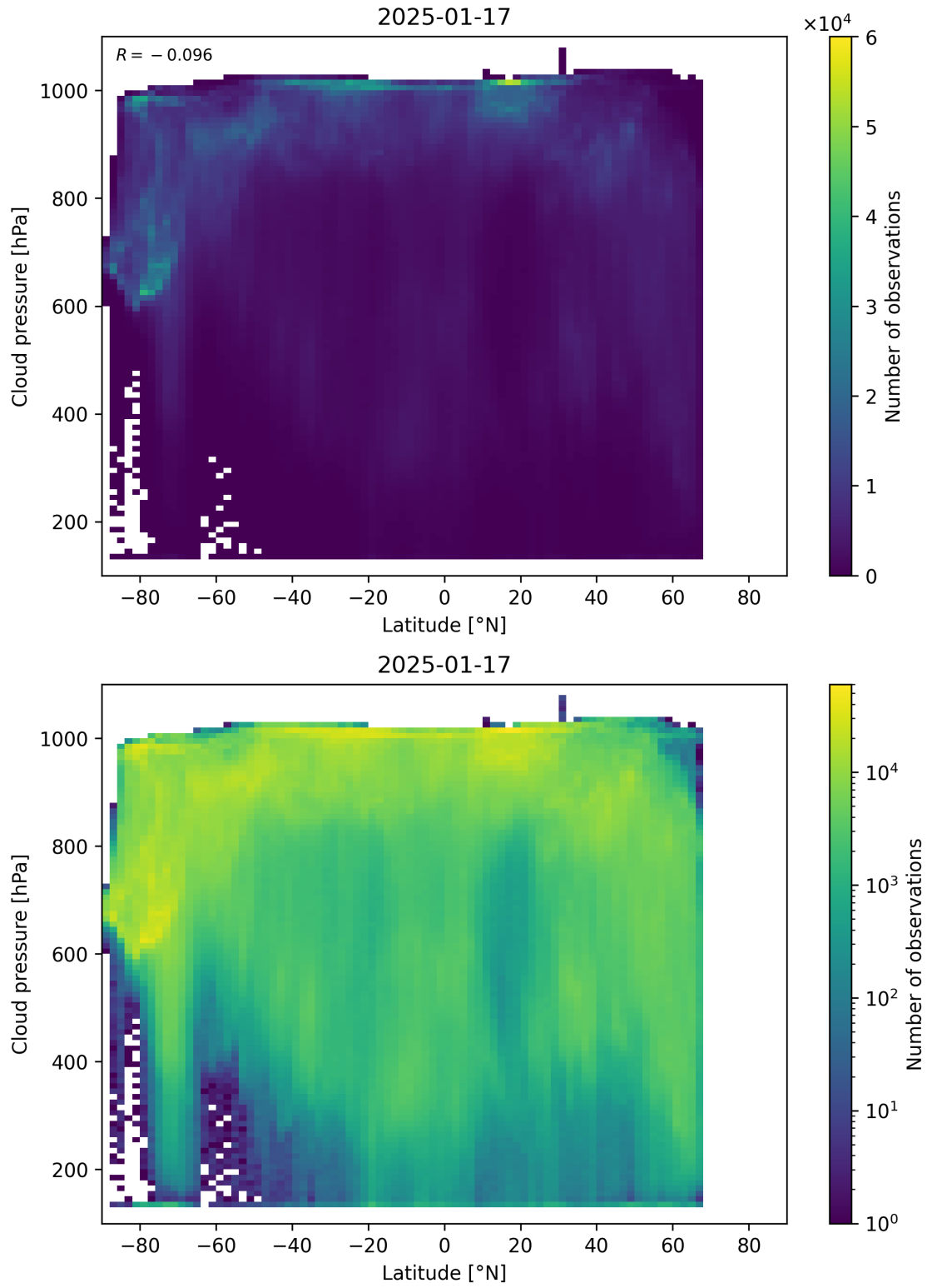
Figure 91: Scatter density plot of “Latitude” against “Cloud pressure” for 2025-01-17 to 2025-01-18.
