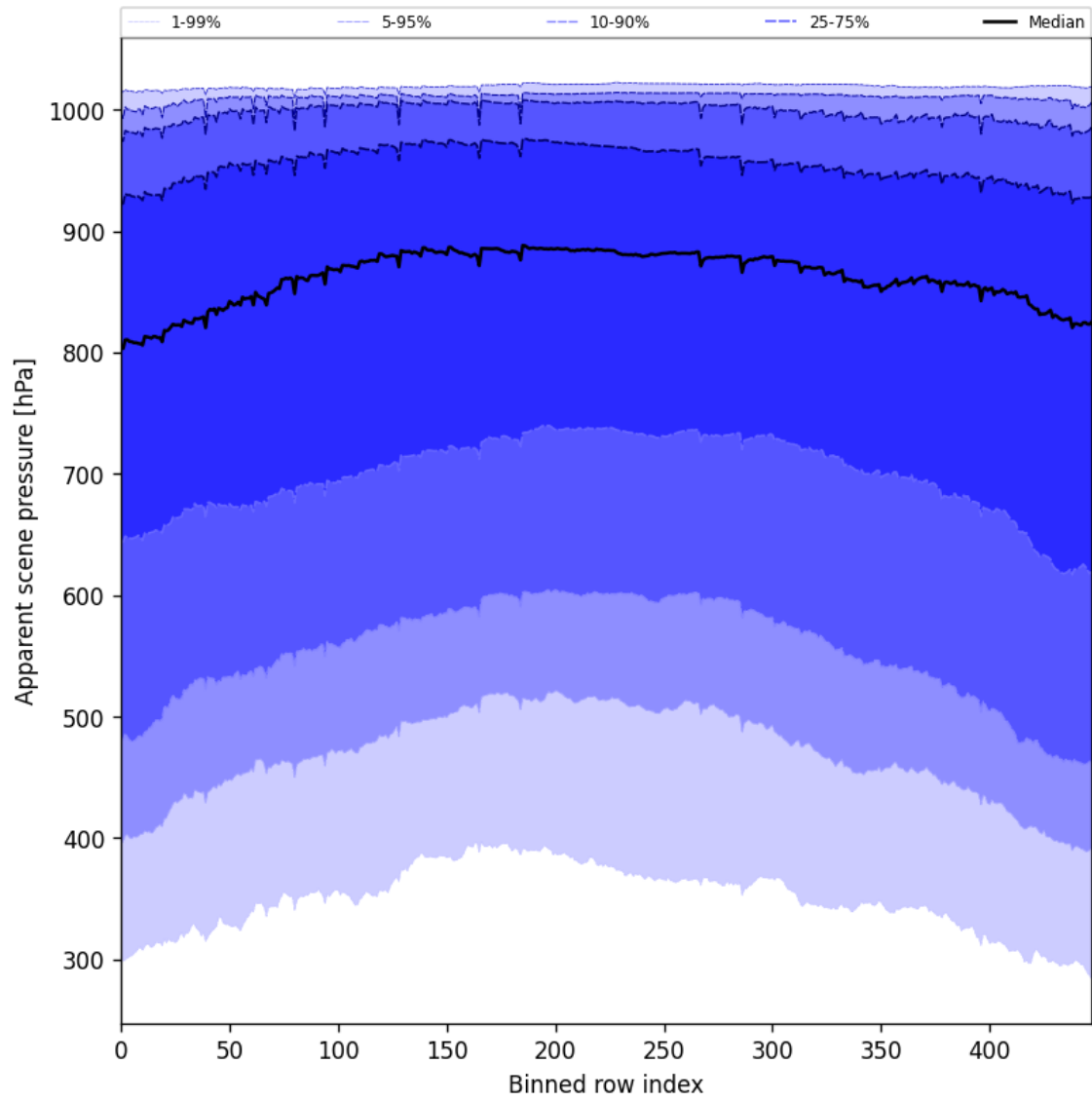
Figure 53: Along track statistics of “Apparent scene pressure” for 2025-01-17 to 2025-01-18
