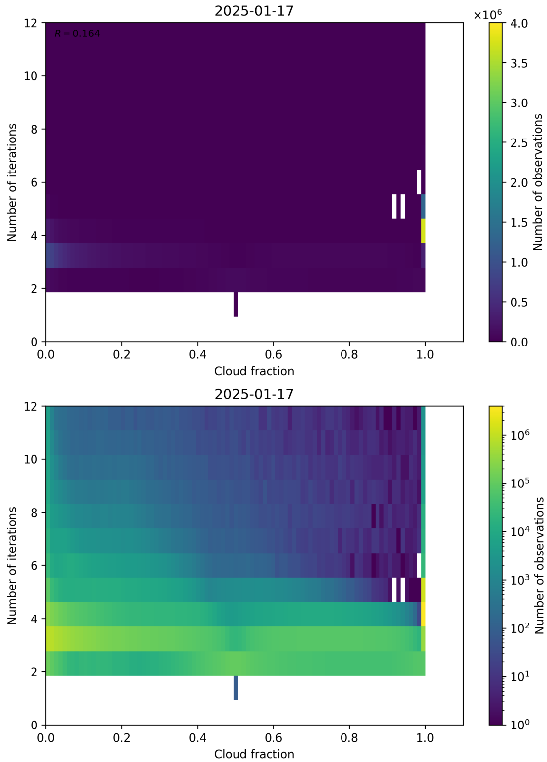
Figure 73: Scatter density plot of “Cloud fraction” against “Number of iterations” for 2025-01-17 to 2025-01-18.
