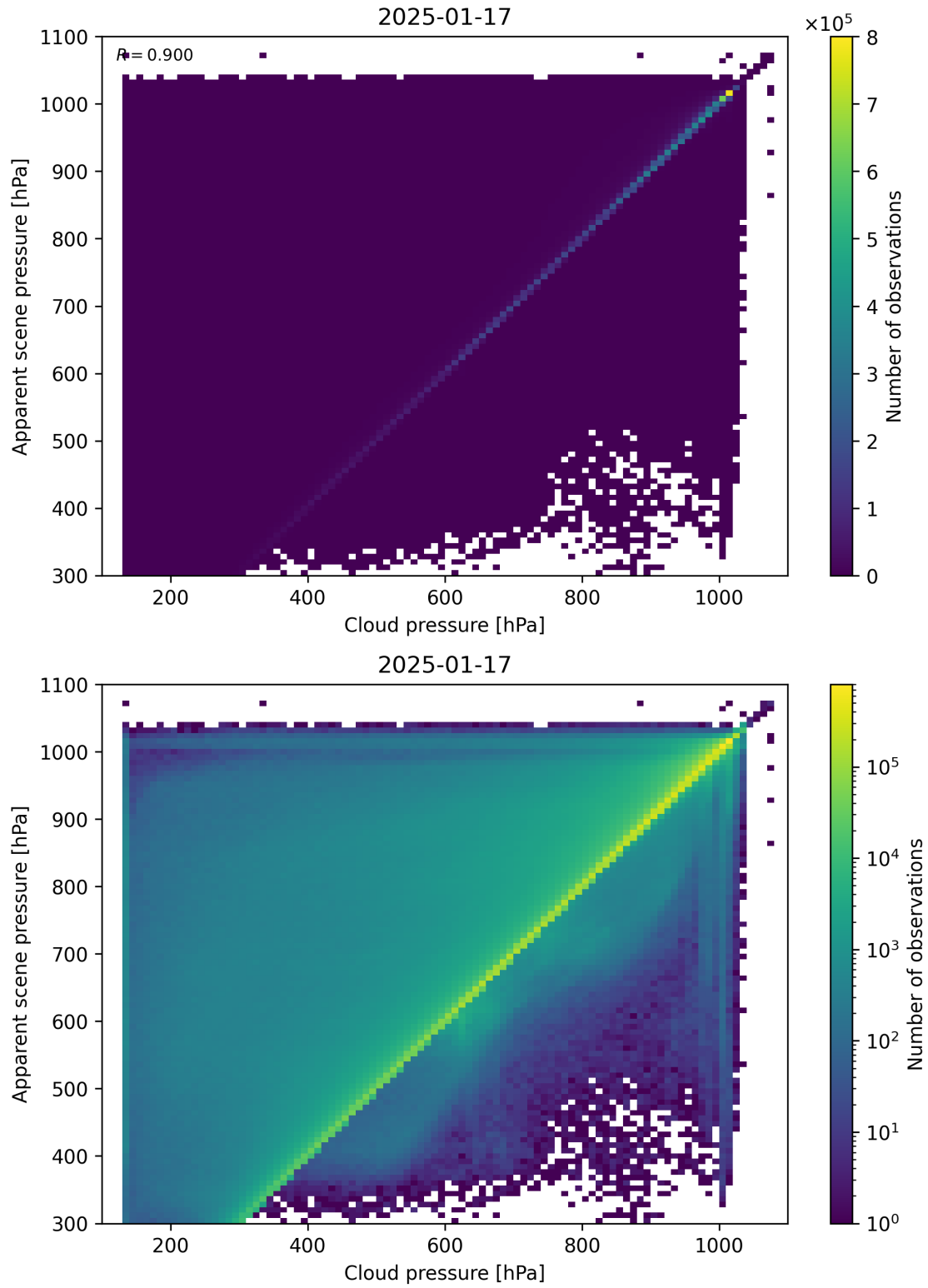
Figure 77: Scatter density plot of “Cloud pressure” against “Apparent scene pressure” for 2025-01-17 to 2025-01-18.
