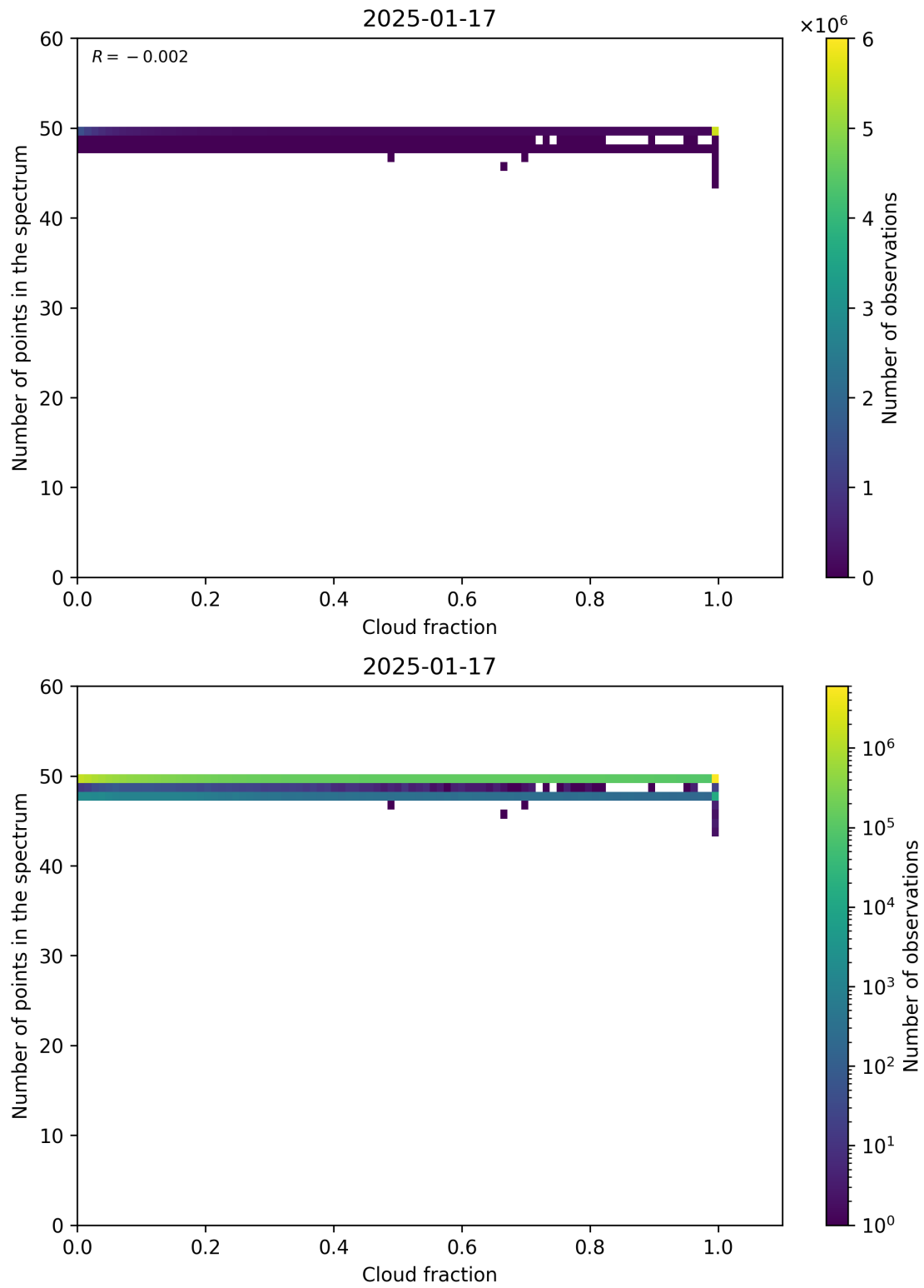
Figure 74: Scatter density plot of “Cloud fraction” against “Number of points in the spectrum” for 2025-01-17 to 2025-01-18.
