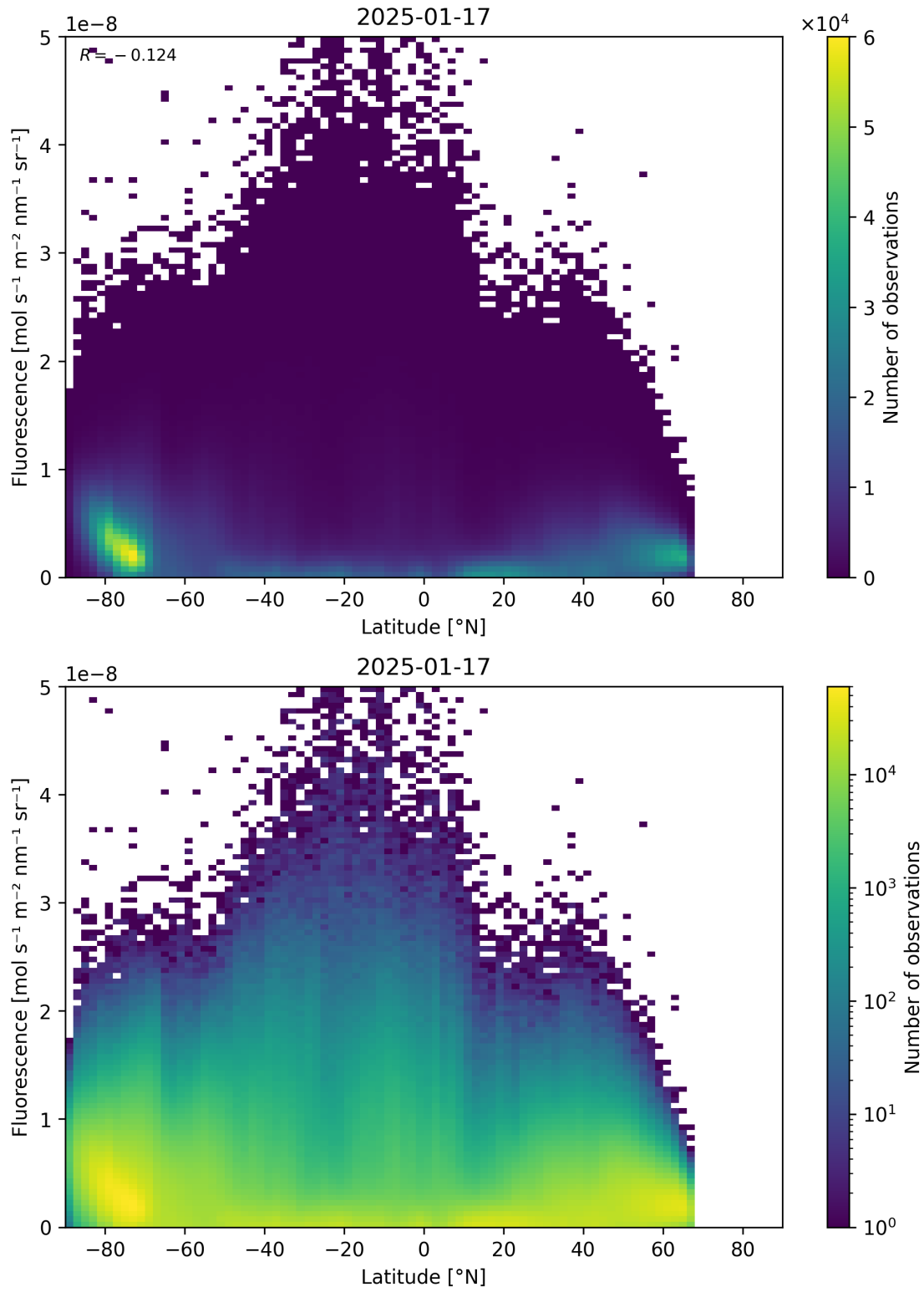
Figure 92: Scatter density plot of “Latitude” against “Fluorescence” for 2025-01-17 to 2025-01-18.
