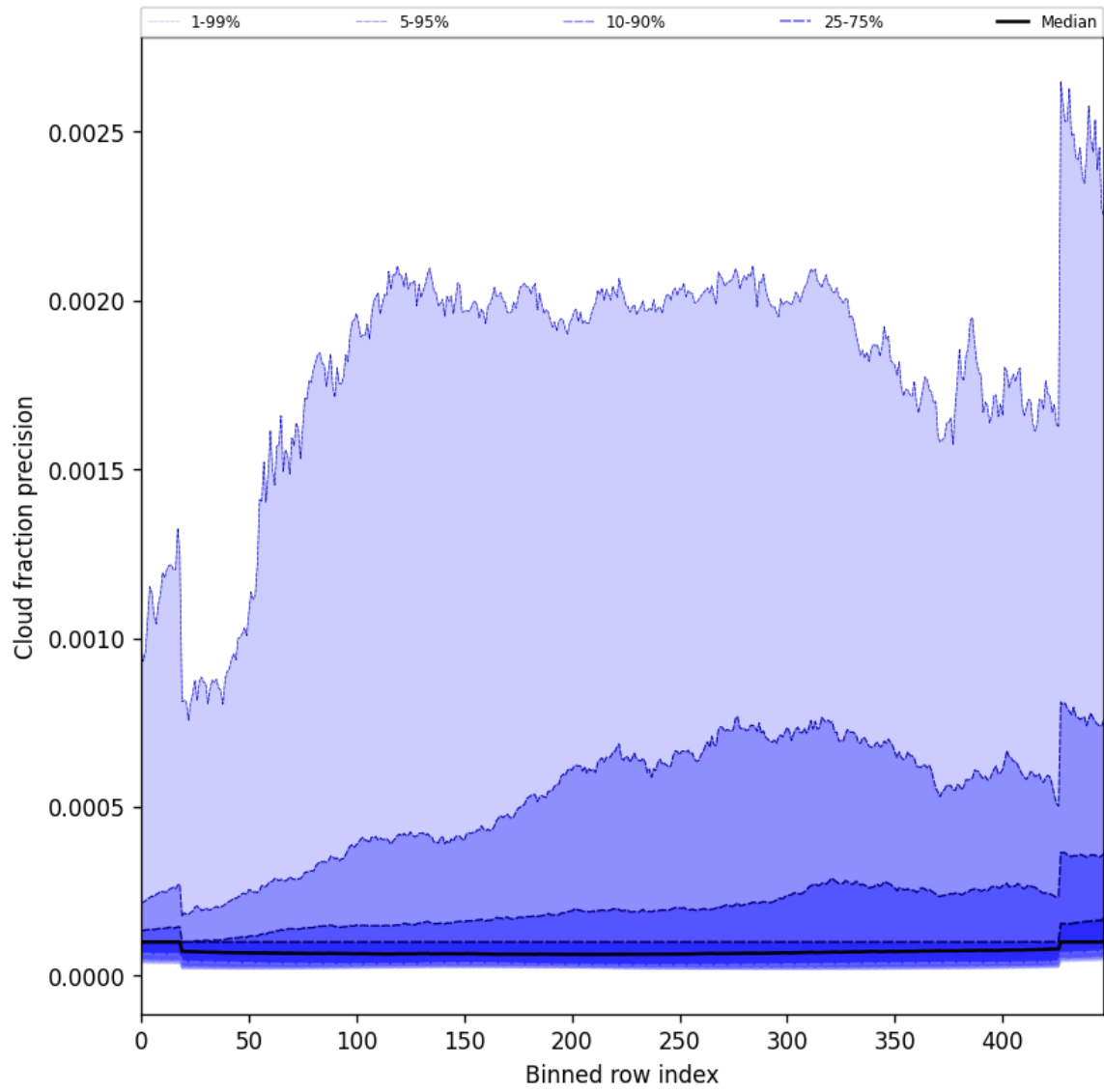
Figure 50: Along track statistics of “Cloud fraction precision” for 2025-01-17 to 2025-01-18
