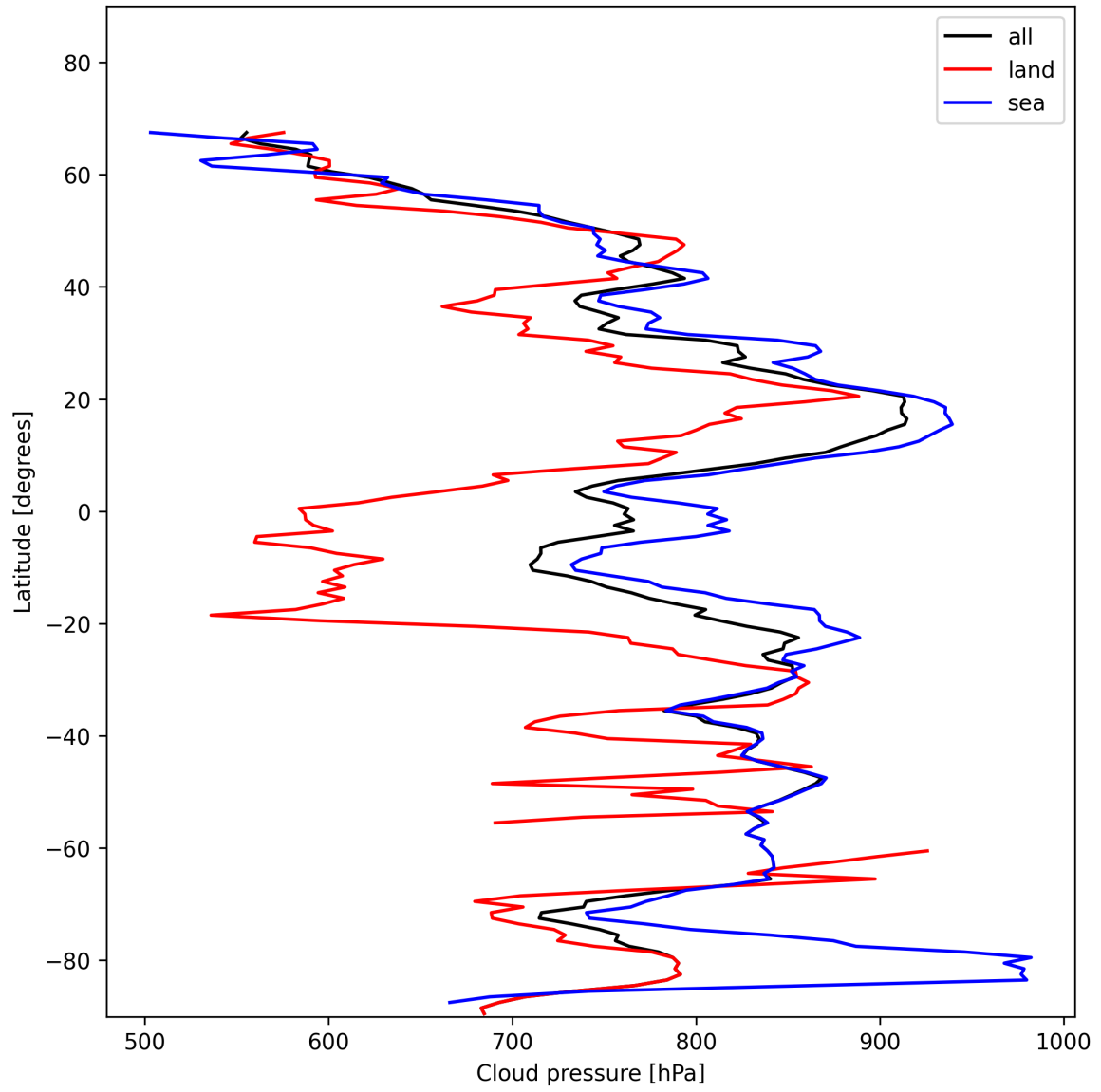
Figure 13: Zonal average of “Cloud pressure” for 2025-01-17 to 2025-01-18.
