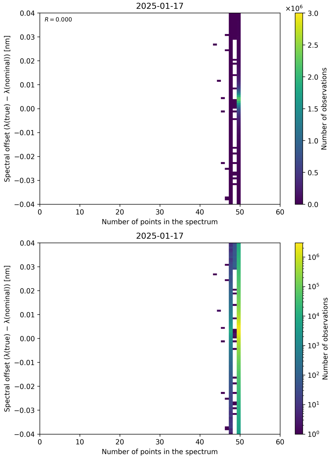
Figure 101: Scatter density plot of “Number of points in the spectrum” against “Spectral offset ( \lambda_{\text{true}} - \lambda_{\text{nominal}} )” for 2025-01-17 to 2025-01-18.
