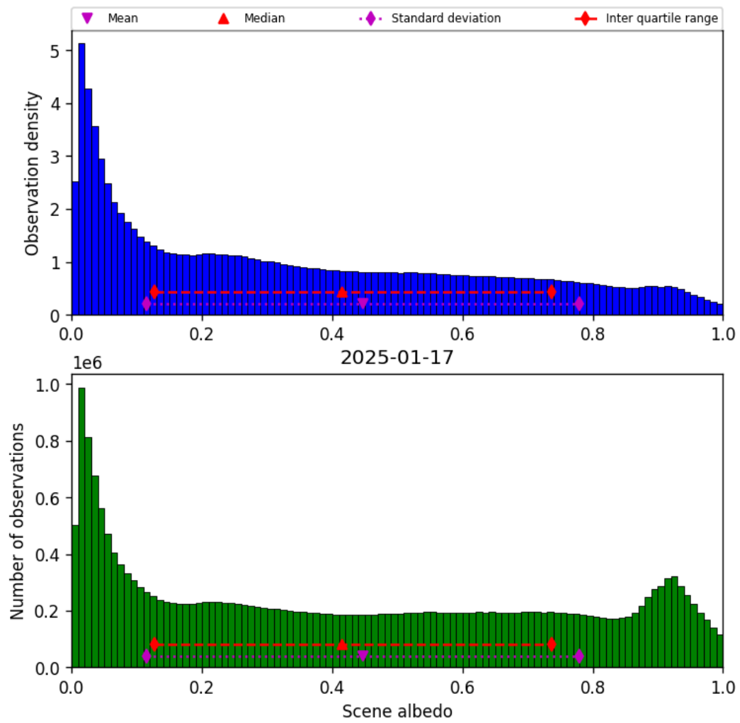
Figure 34: Histogram of “Scene albedo” for 2025-01-17 to 2025-01-18
