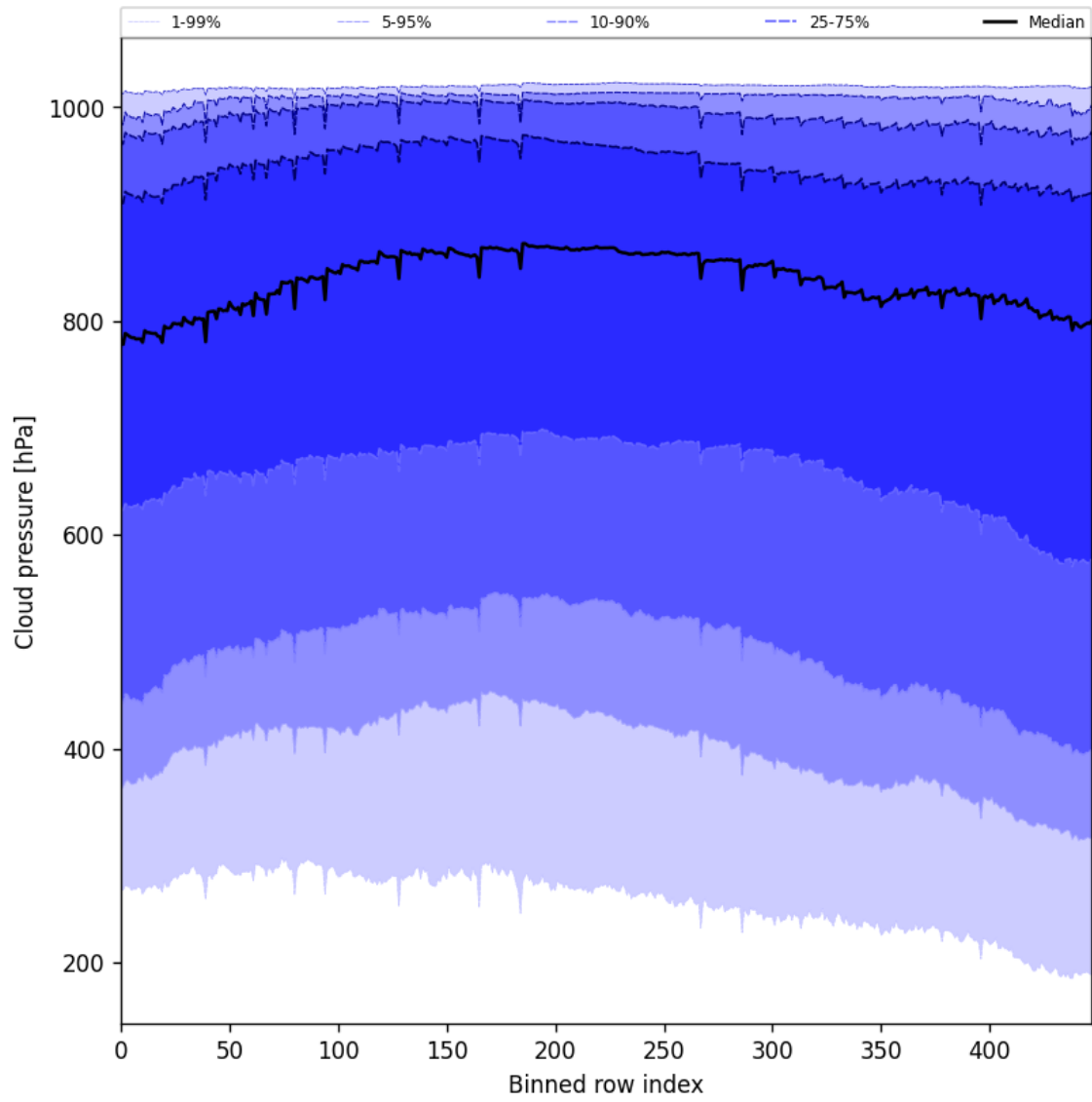
Figure 47: Along track statistics of “Cloud pressure” for 2025-01-17 to 2025-01-18
