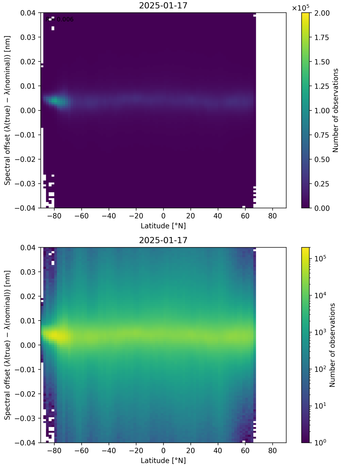
Figure 96: Scatter density plot of “Latitude” against “Spectral offset ( \lambda_{\text{true}} - \lambda_{\text{nominal}} )” for 2025-01-17 to 2025-01-18.
