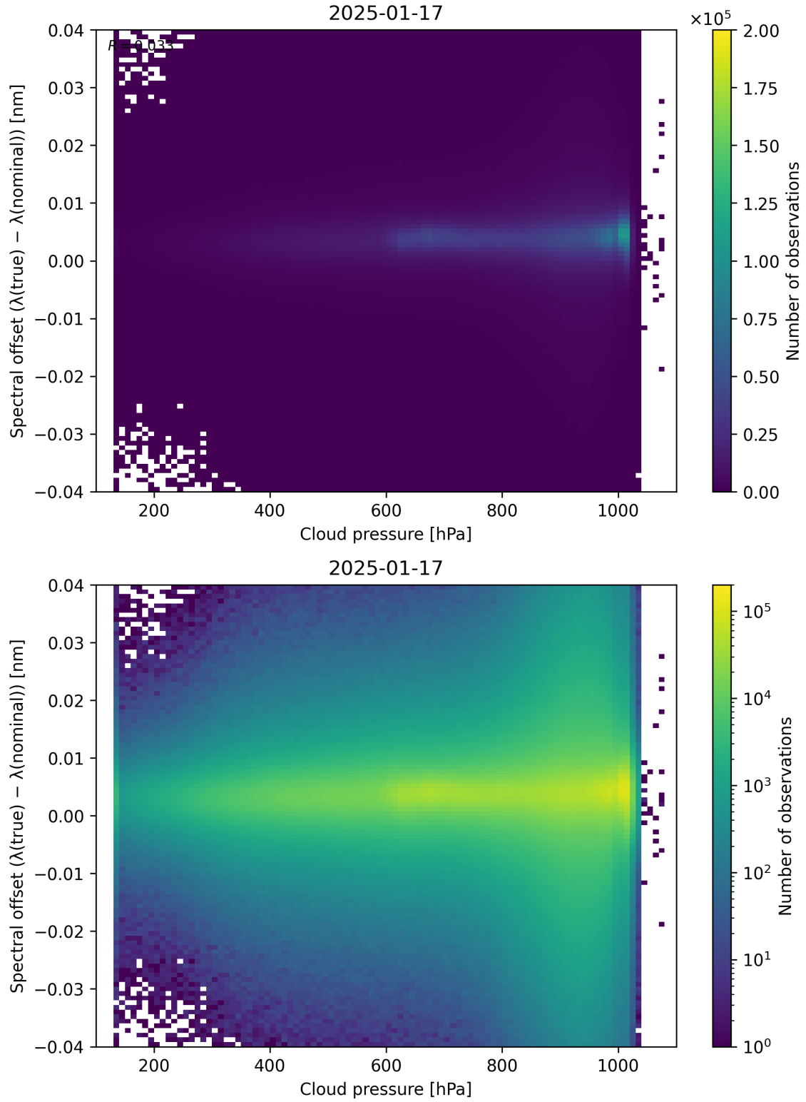
Figure 84: Scatter density plot of “Cloud pressure” against “Spectral offset ( \lambda_{\text{true}} - \lambda_{\text{nominal}} )” for 2025-01-17 to 2025-01-18.
