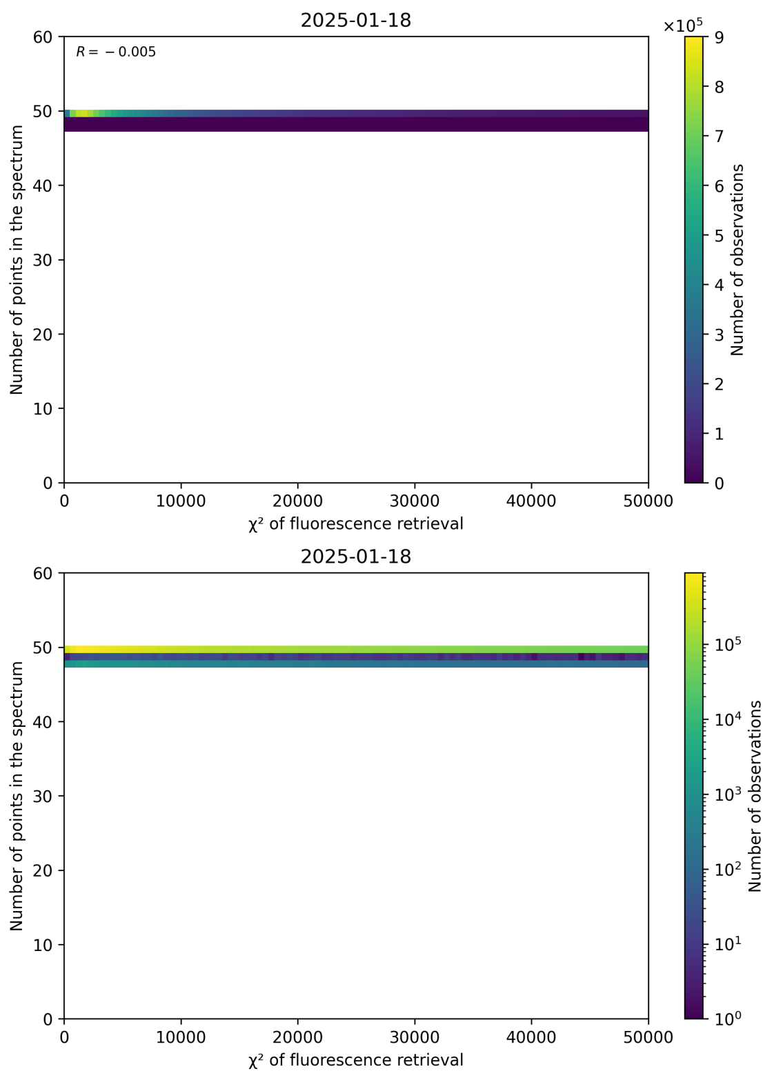
Figure 68: Scatter density plot of " \chi^2 of fluorescence retrieval" against "Number of points in the spectrum" for 2025-01-17 to 2025-01-19.
