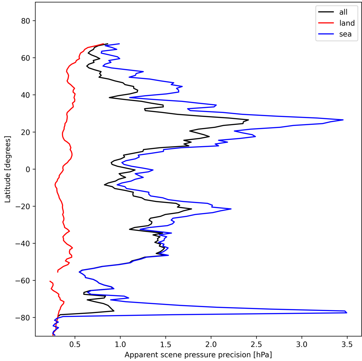
Figure 20: Zonal average of “Apparent scene pressure precision” for 2025-01-17 to 2025-01-19.
