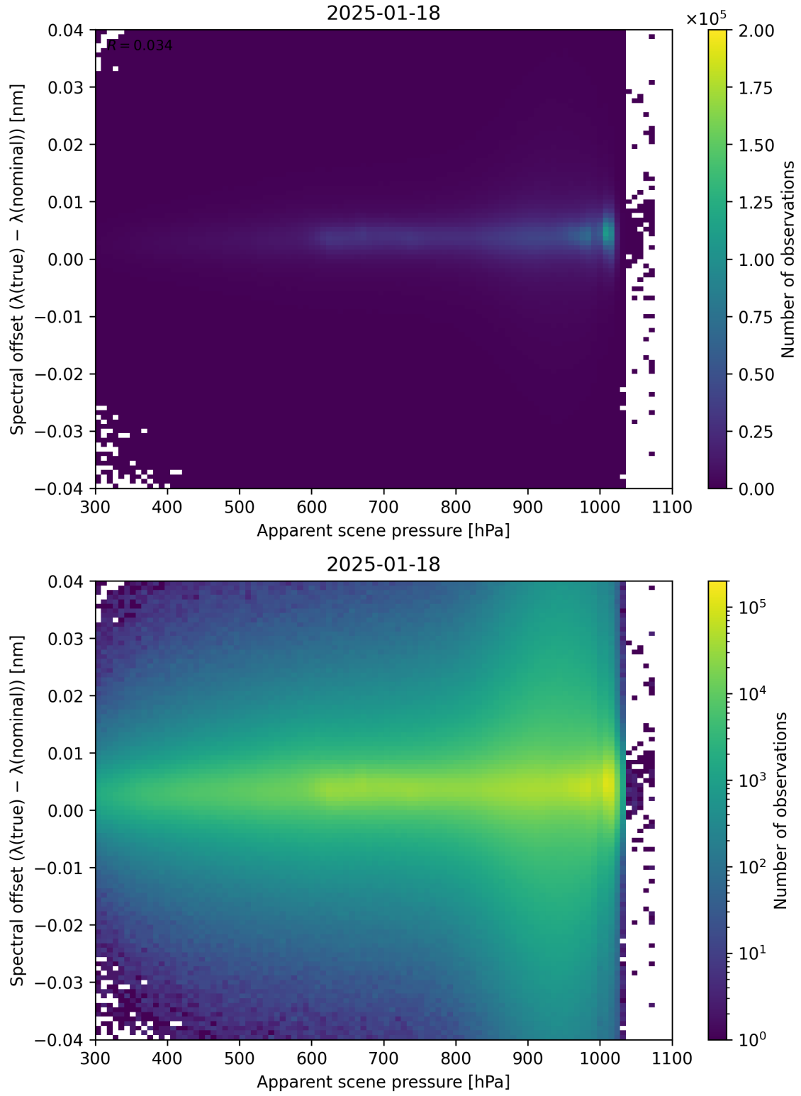
Figure 67: Scatter density plot of “Apparent scene pressure” against “Spectral offset ( \lambda_{\text{true}} - \lambda_{\text{nominal}} )” for 2025-01-17 to 2025-01-19.
