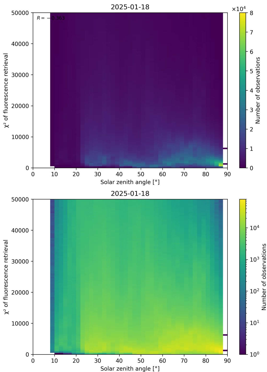
Figure 109: Scatter density plot of “Solar zenith angle” against “ \chi^2 of fluorescence retrieval” for 2025-01-17 to 2025-01-19.
