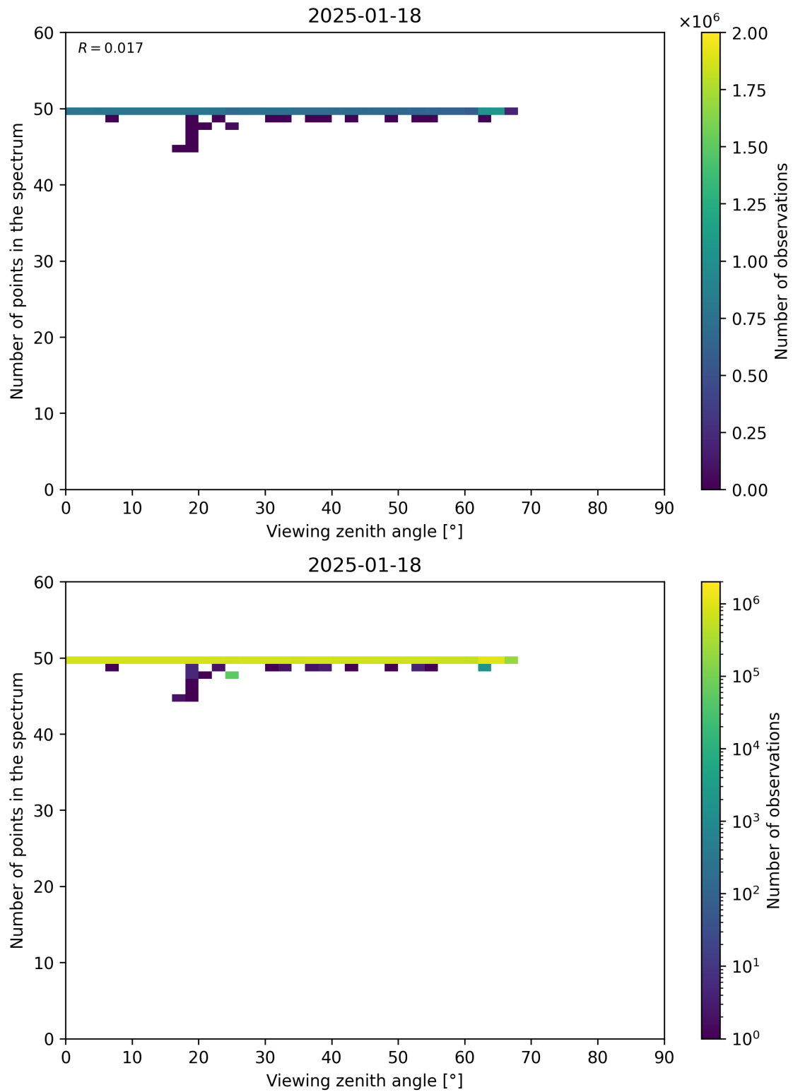
Figure 125: Scatter density plot of “Viewing zenith angle” against “Number of points in the spectrum” for 2025-01-17 to 2025-01-19.
