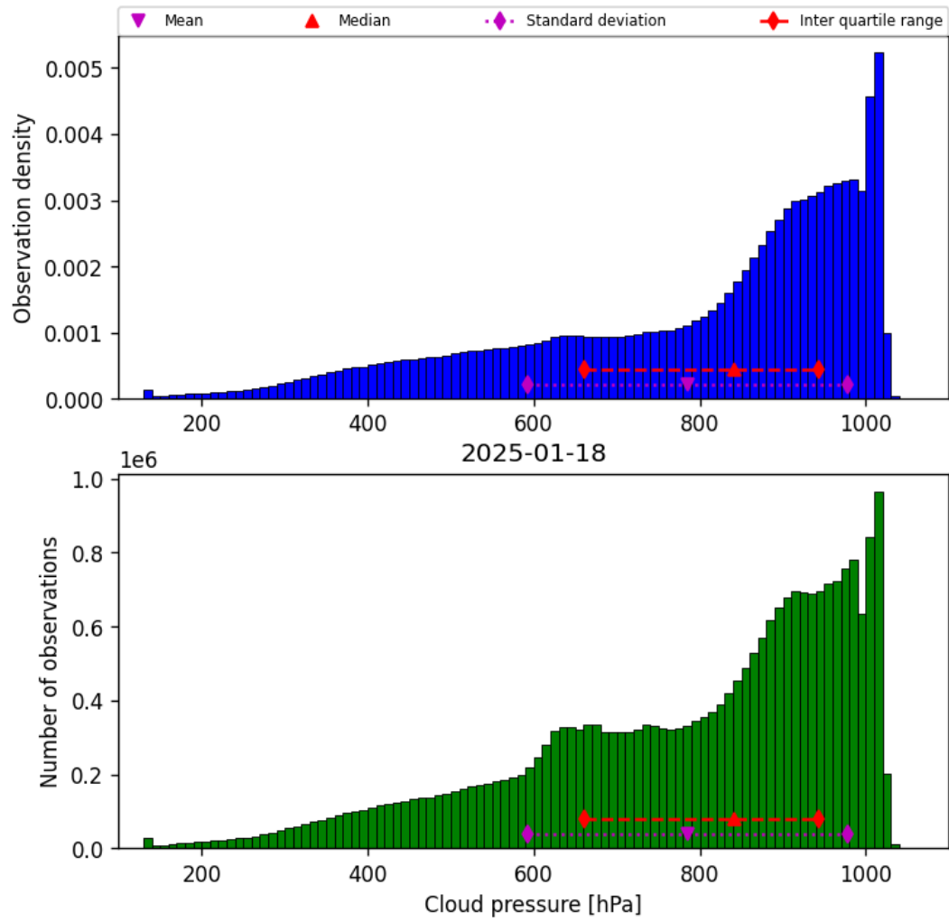
Figure 30: Histogram of “Cloud pressure” for 2025-01-17 to 2025-01-19
