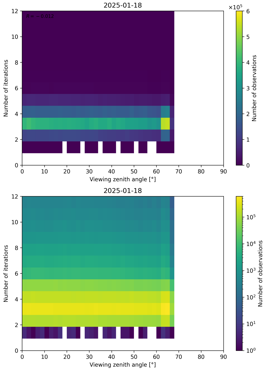
Figure 124: Scatter density plot of “Viewing zenith angle” against “Number of iterations” for 2025-01-17 to 2025-01-19.
