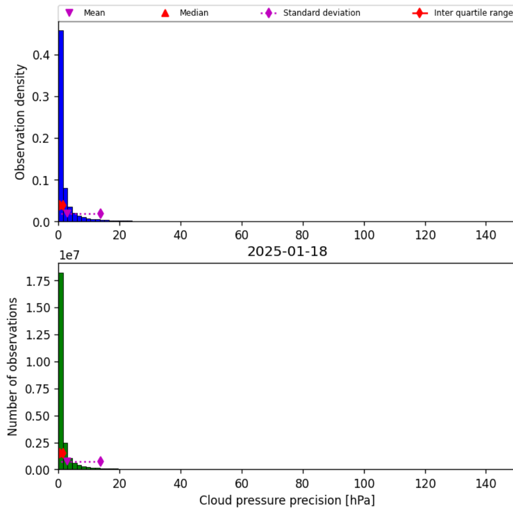
Figure 31: Histogram of “Cloud pressure precision” for 2025-01-17 to 2025-01-19
