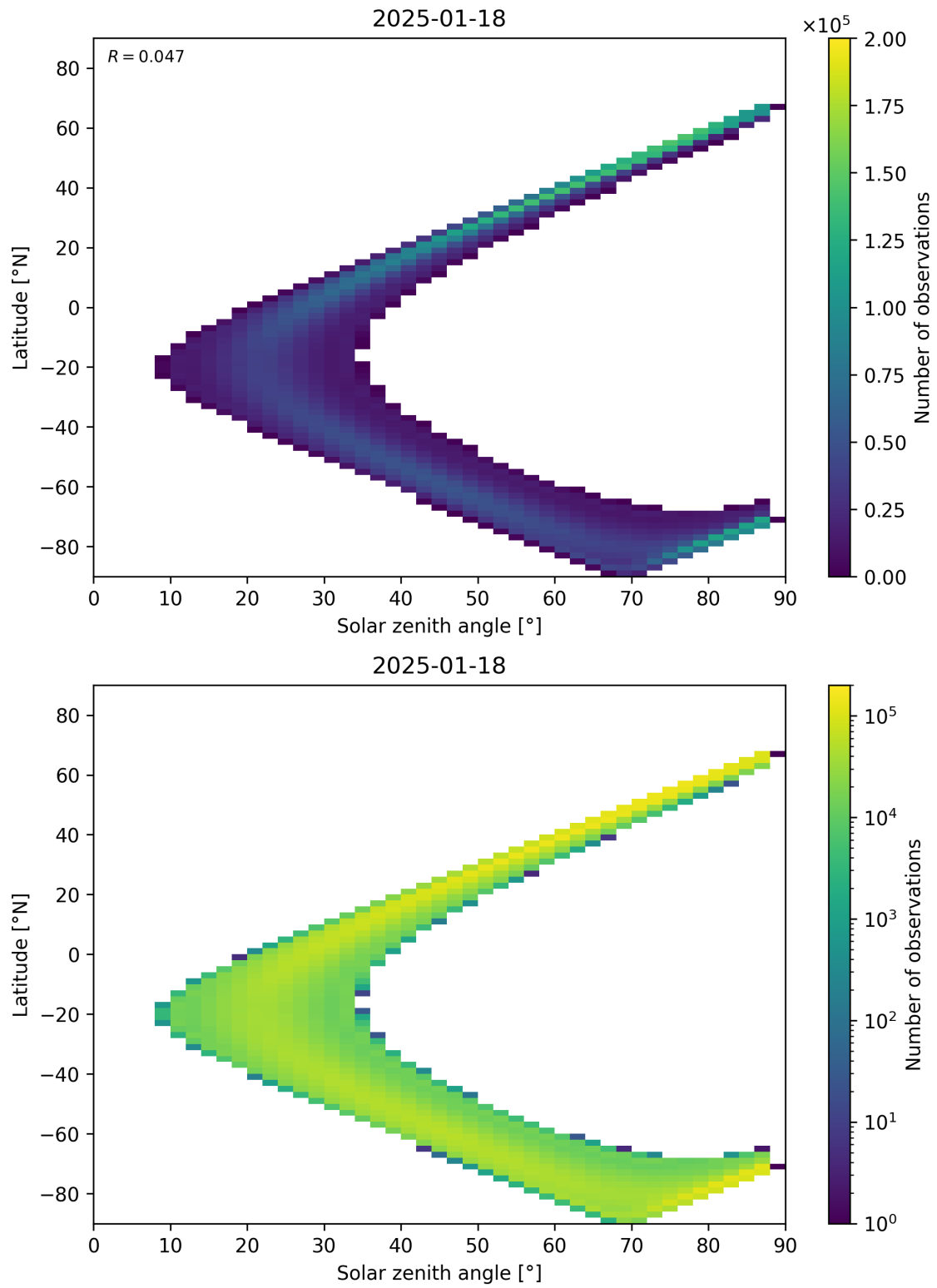
Figure 113: Scatter density plot of “Solar zenith angle” against “Latitude” for 2025-01-17 to 2025-01-19.
