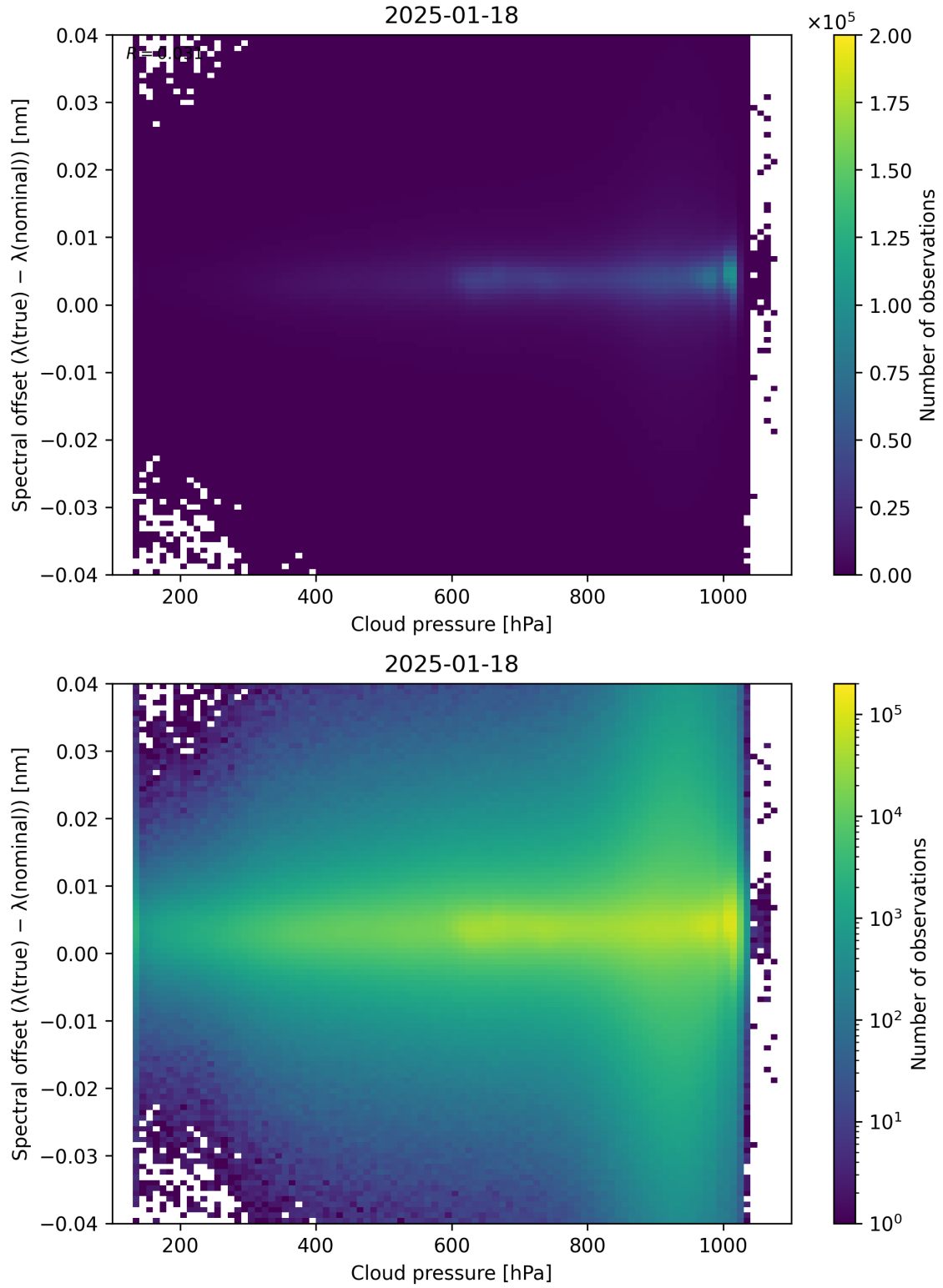
Figure 84: Scatter density plot of “Cloud pressure” against “Spectral offset ( \lambda_{\text{true}} - \lambda_{\text{nominal}} )” for 2025-01-17 to 2025-01-19.
