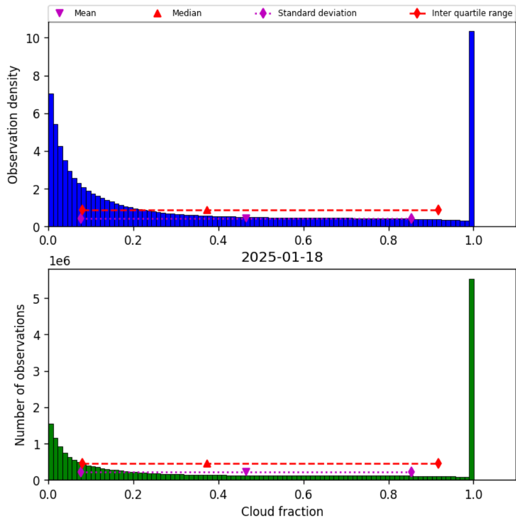
Figure 32: Histogram of “Cloud fraction” for 2025-01-17 to 2025-01-19
