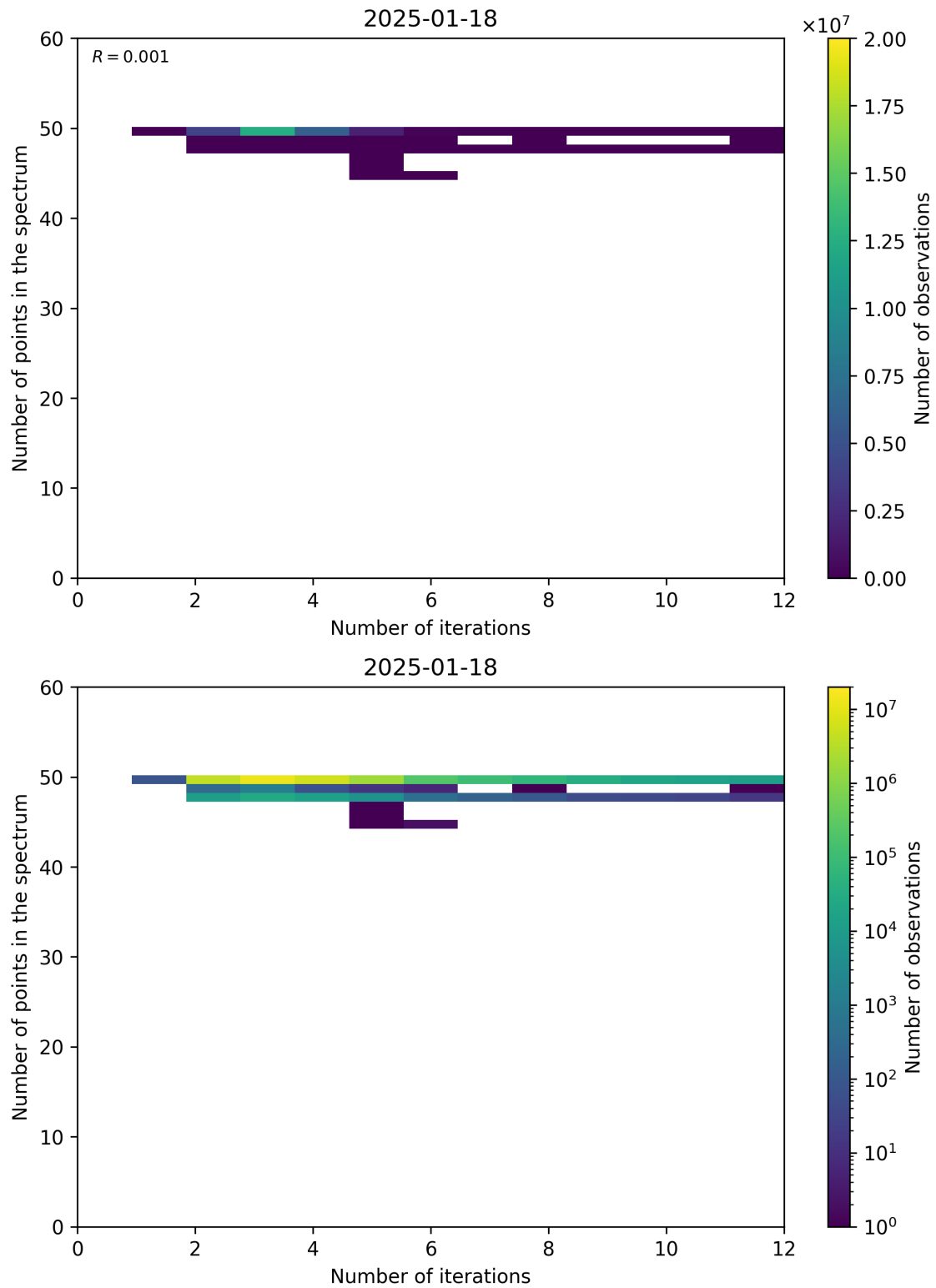
Figure 99: Scatter density plot of “Number of iterations” against “Number of points in the spectrum” for 2025-01-17 to 2025-01-19.
