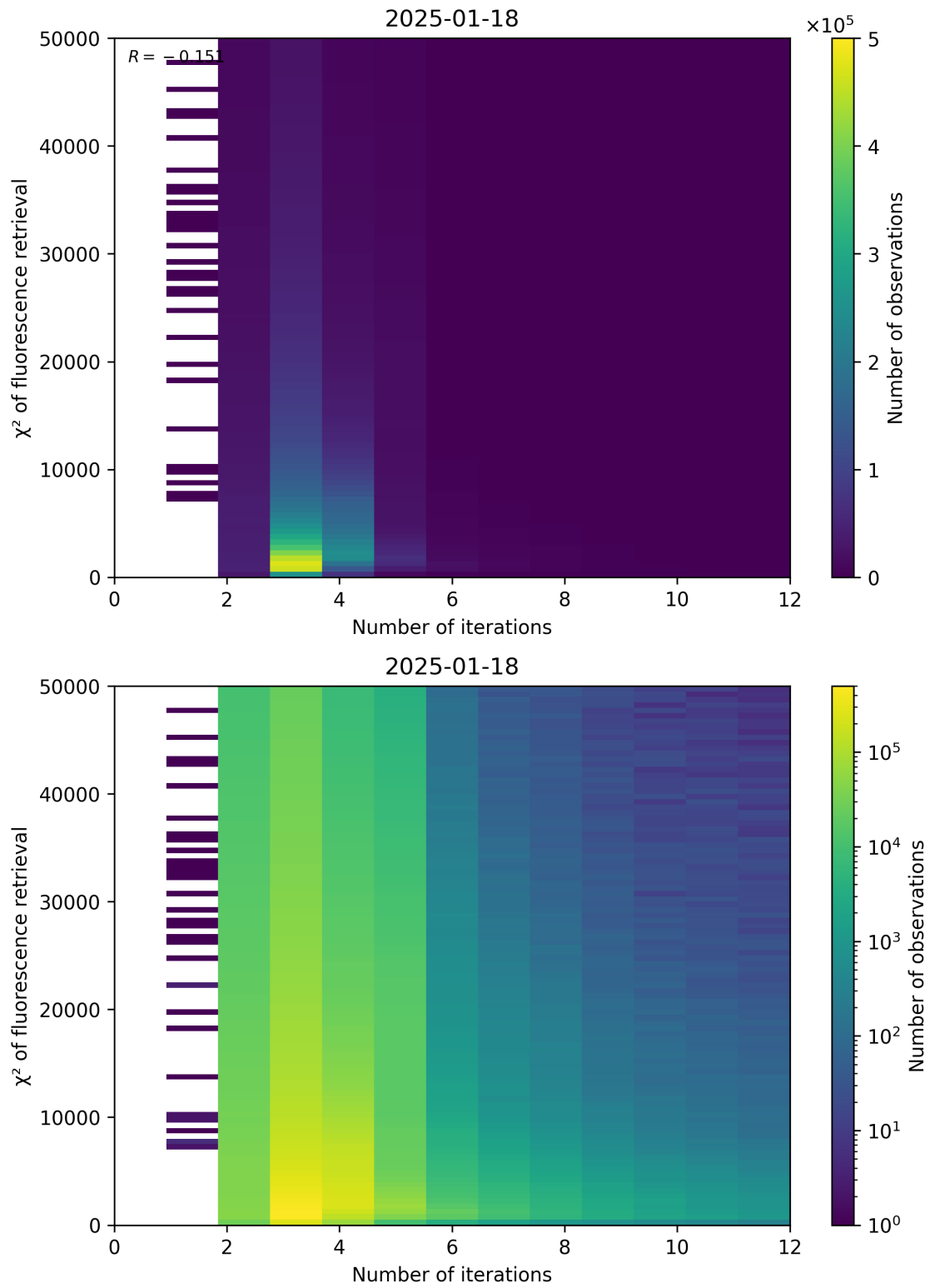
Figure 97: Scatter density plot of “Number of iterations” against “ \chi^2 of fluorescence retrieval” for 2025-01-17 to 2025-01-19.
