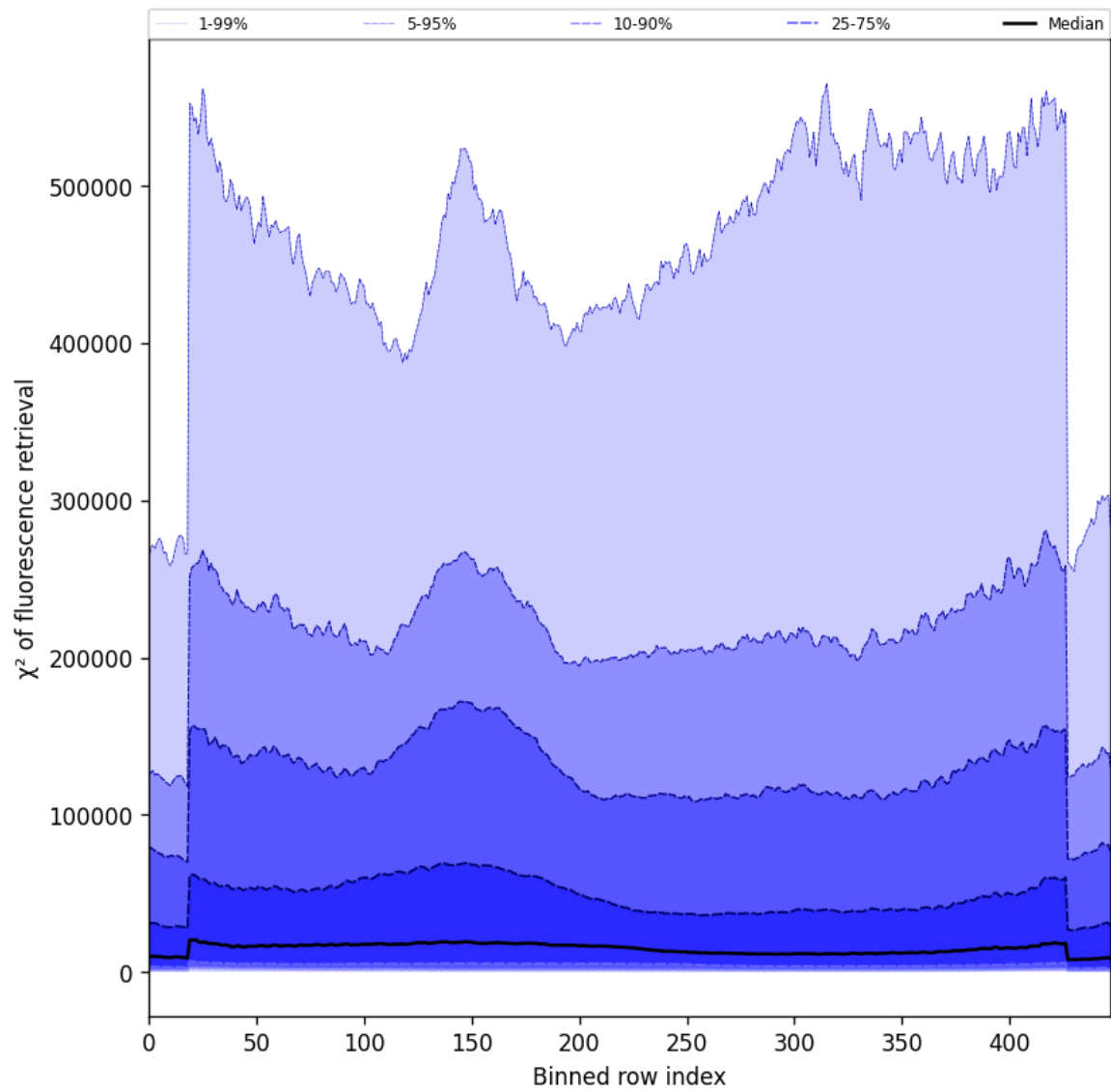
Figure 59: Along track statistics of “ \chi^2 of fluorescence retrieval” for 2025-01-17 to 2025-01-19
