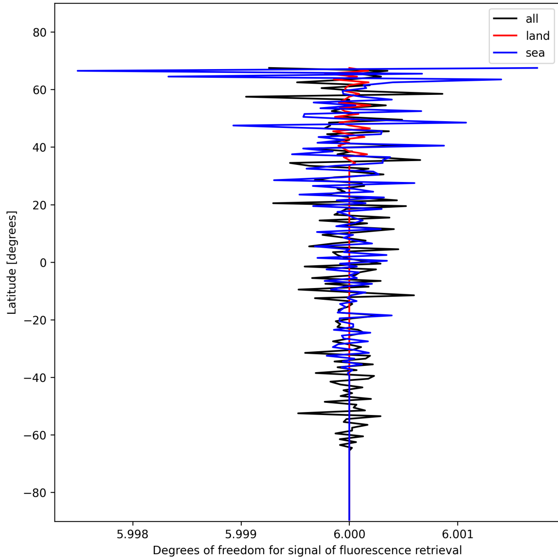
Figure 26: Zonal average of “Degrees of freedom for signal of fluorescence retrieval” for 2025-01-17 to 2025-01-19.
