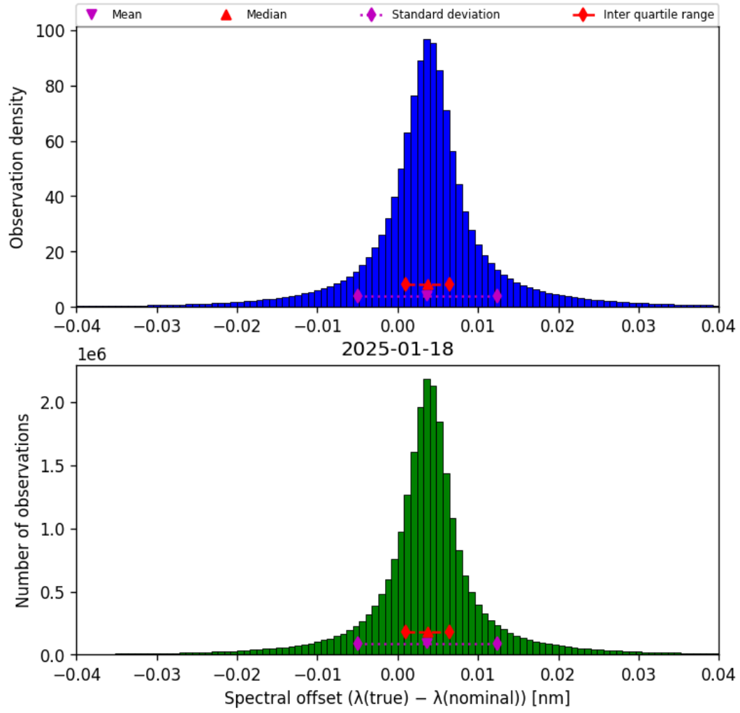
Figure 45: Histogram of “Spectral offset ( \lambda_{\text{true}} - \lambda_{\text{nominal}} )” for 2025-01-17 to 2025-01-19
