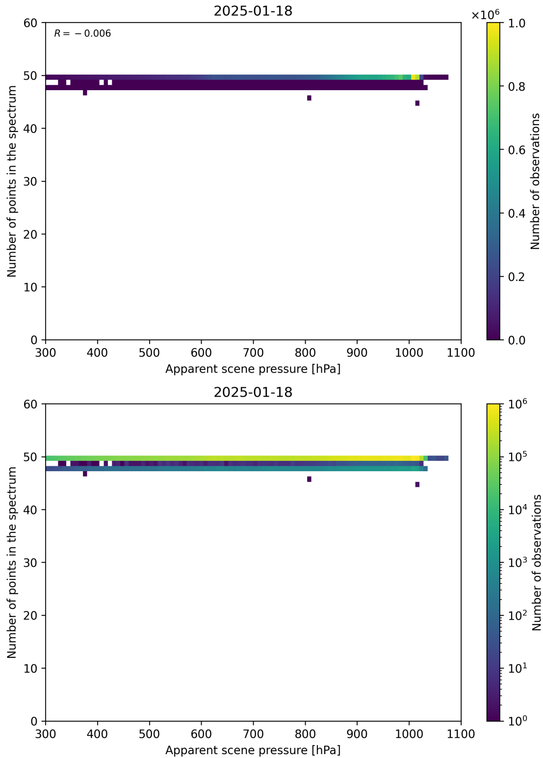
Figure 66: Scatter density plot of “Apparent scene pressure” against “Number of points in the spectrum” for 2025-01-17 to 2025-01-19.
