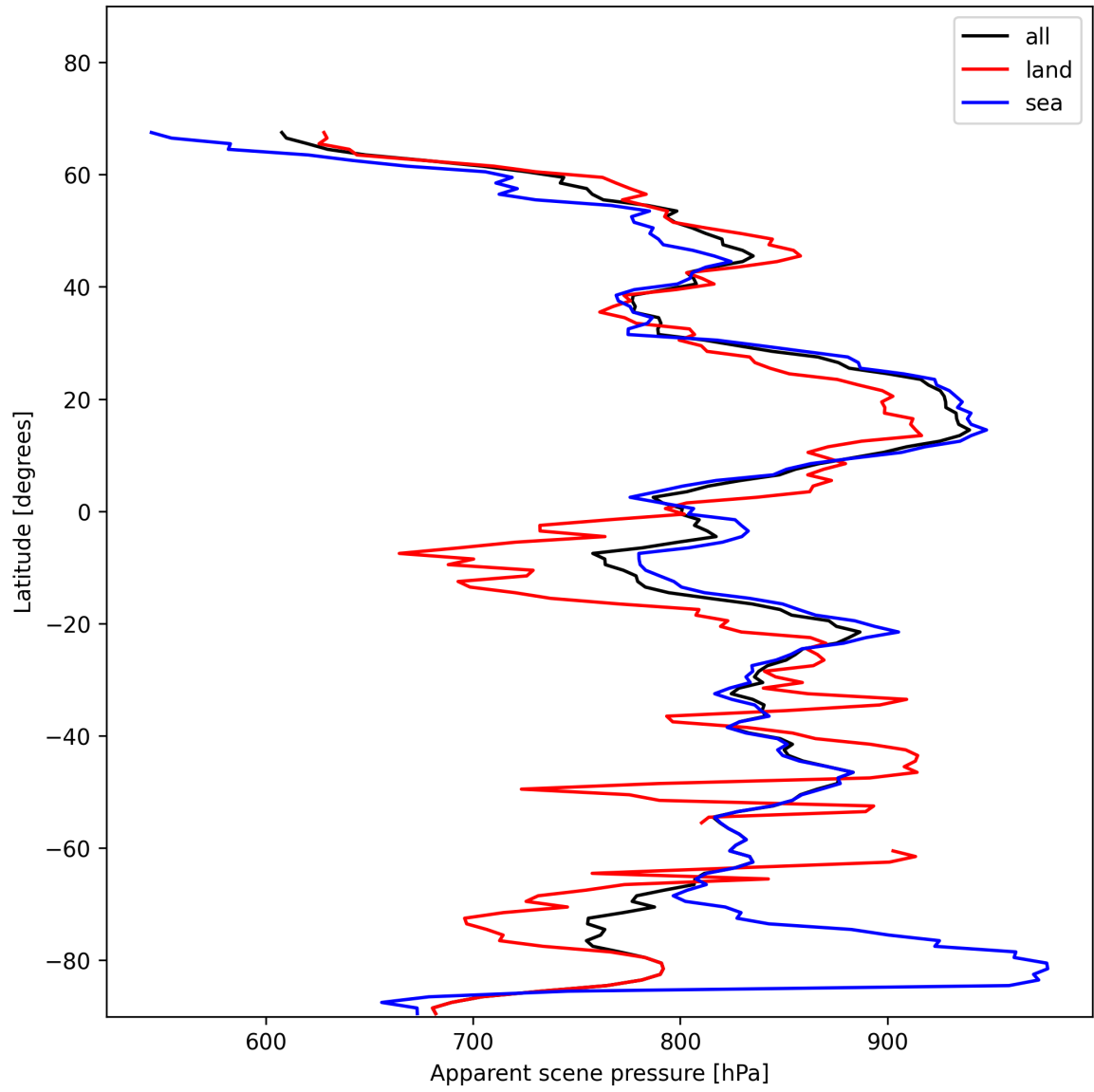
Figure 19: Zonal average of “Apparent scene pressure” for 2025-01-17 to 2025-01-19.
