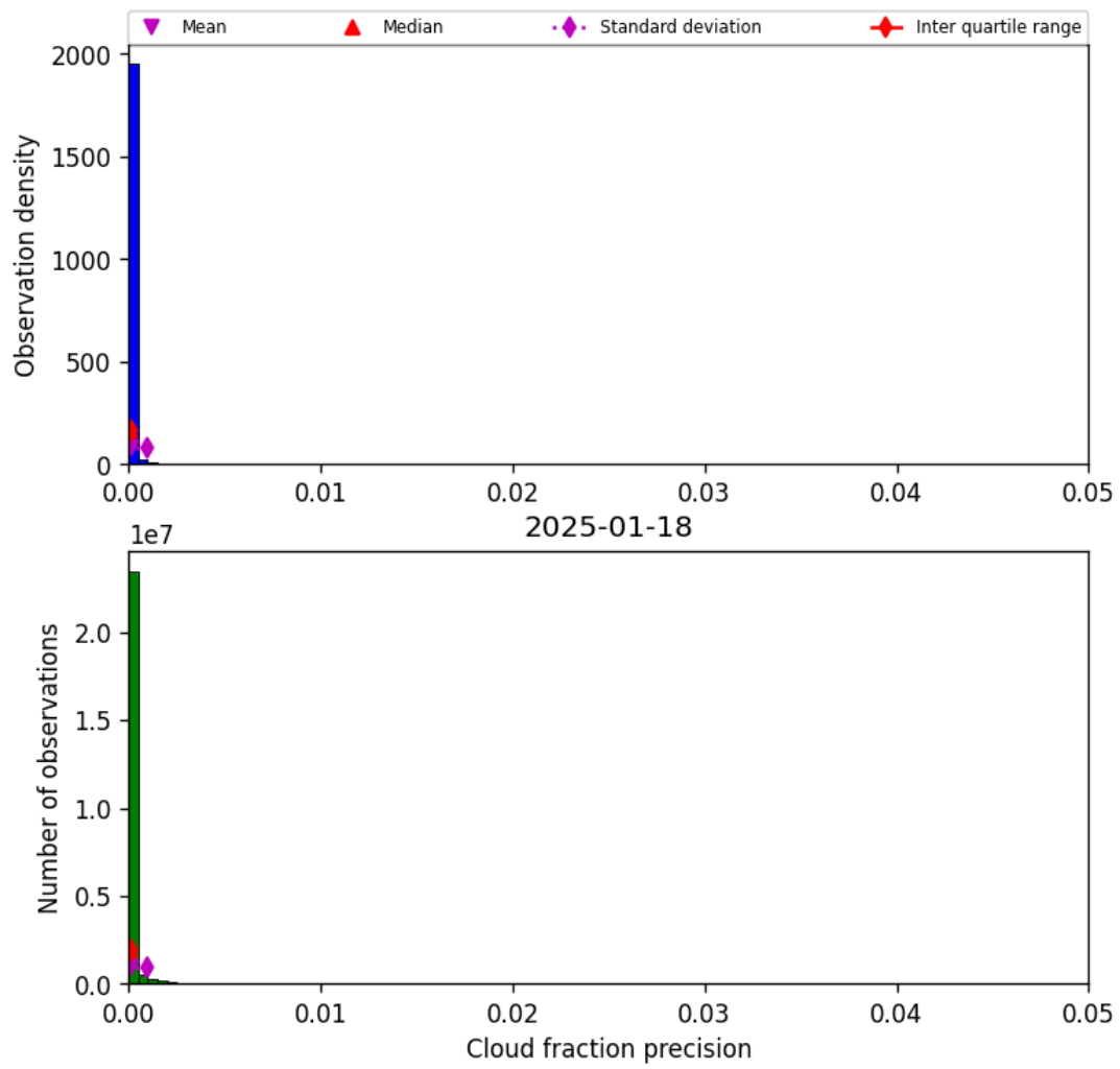
Figure 33: Histogram of “Cloud fraction precision” for 2025-01-17 to 2025-01-19
