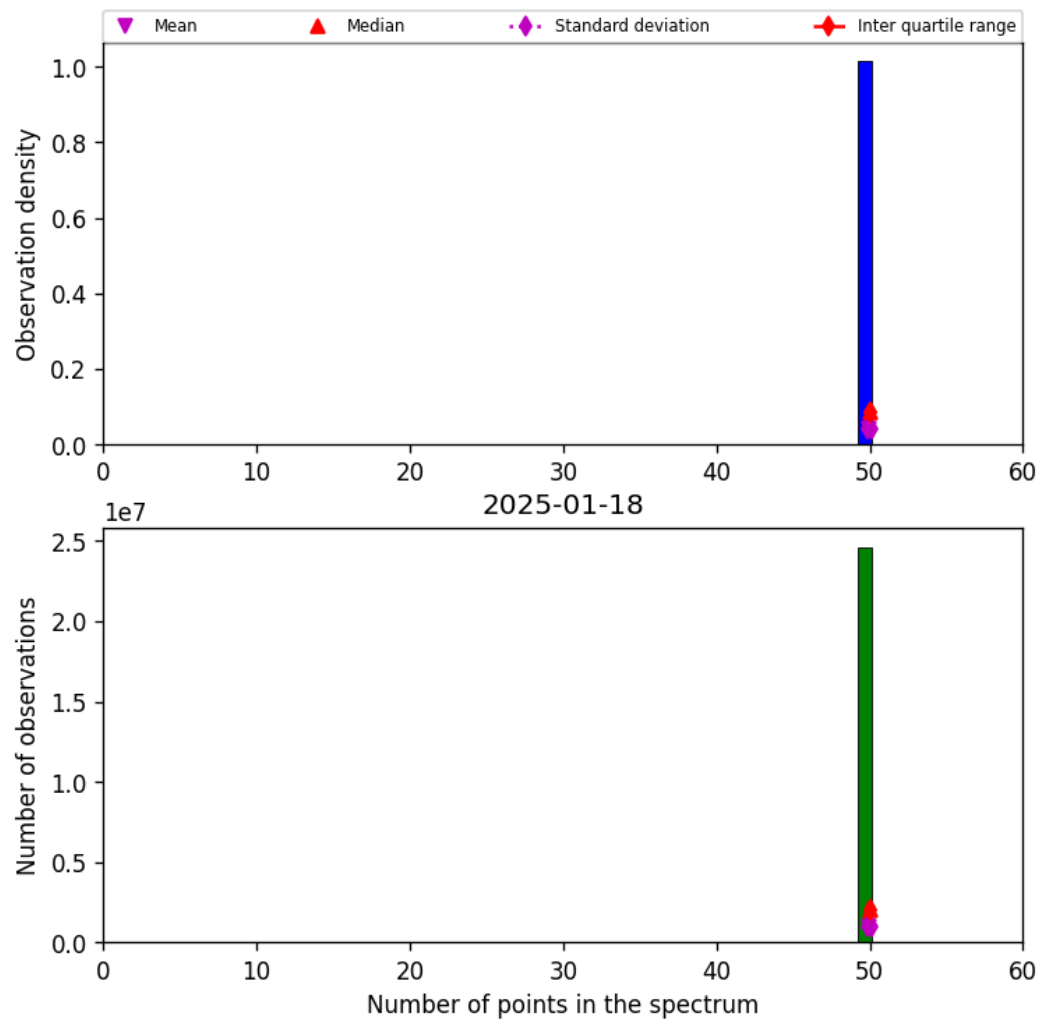
Figure 44: Histogram of “Number of points in the spectrum” for 2025-01-17 to 2025-01-19
