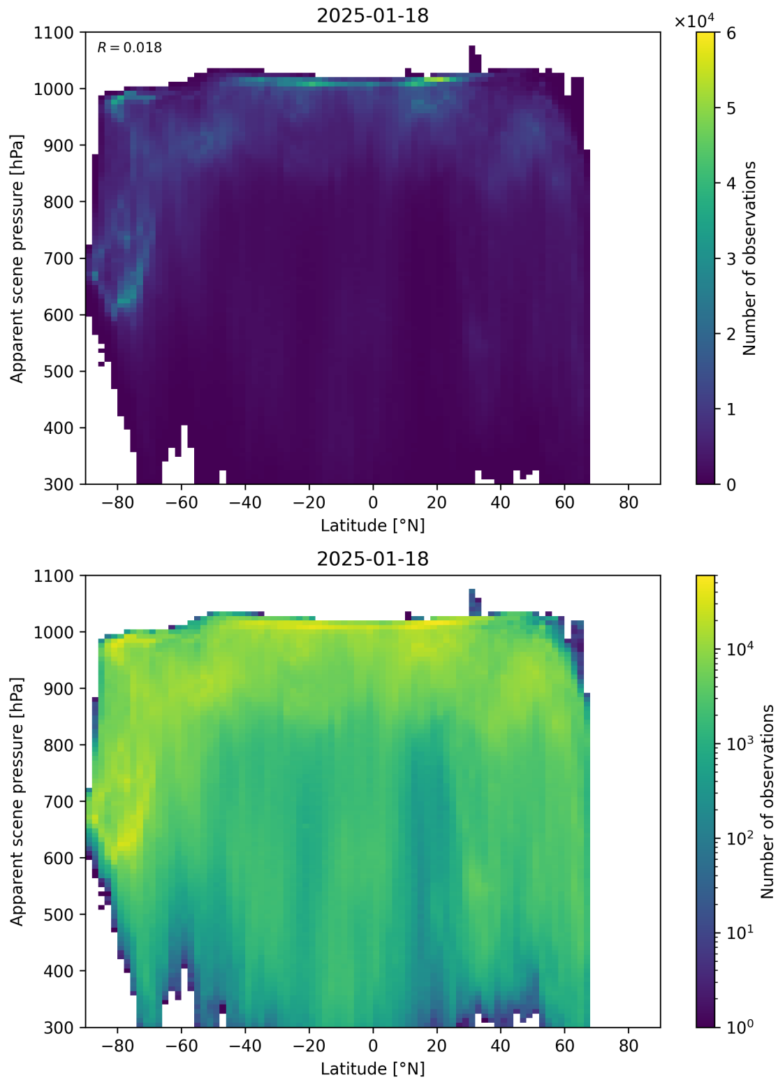
Figure 88: Scatter density plot of “Latitude” against “Apparent scene pressure” for 2025-01-17 to 2025-01-19.
