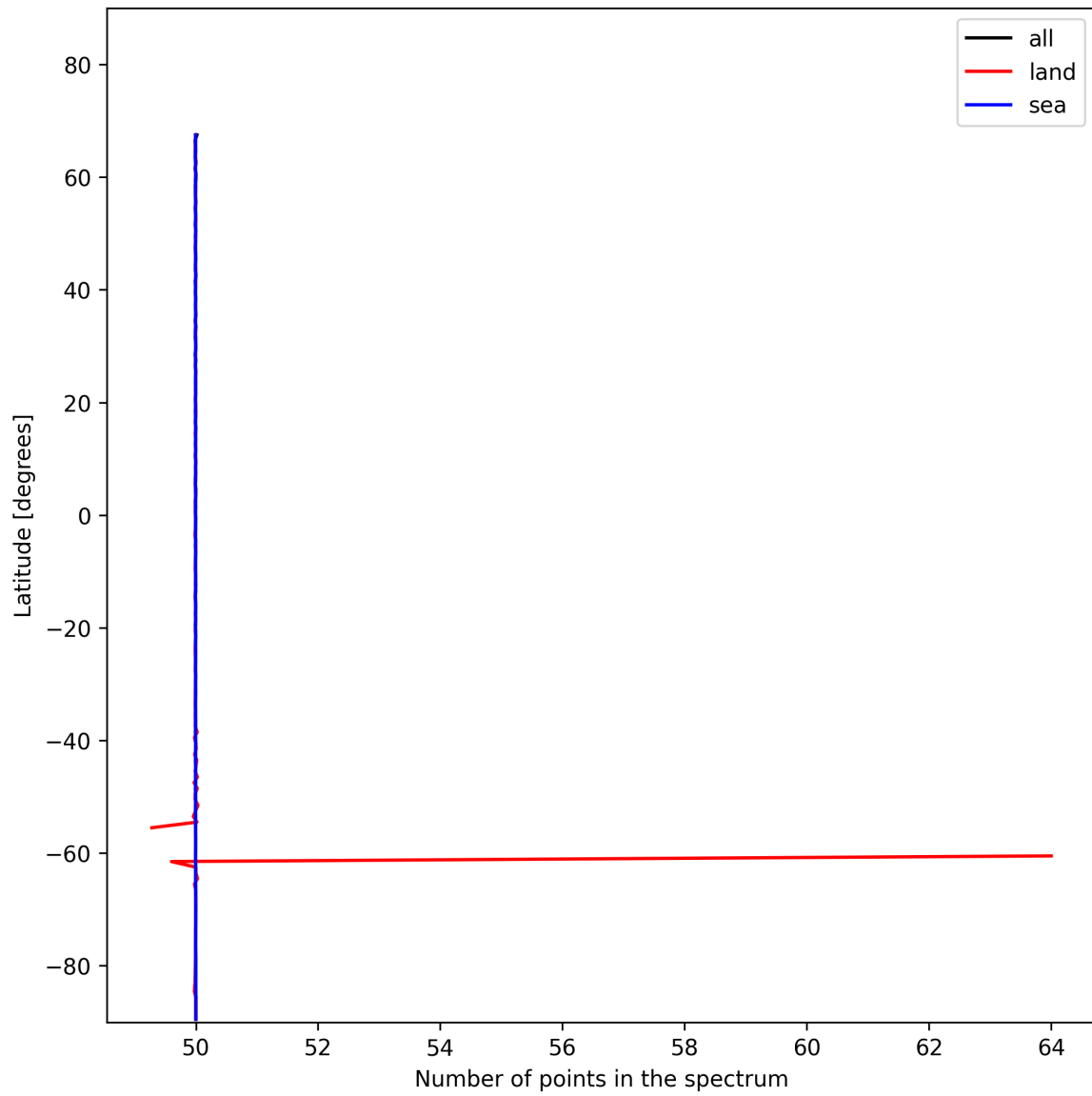
Figure 27: Zonal average of “Number of points in the spectrum” for 2025-01-17 to 2025-01-19.
