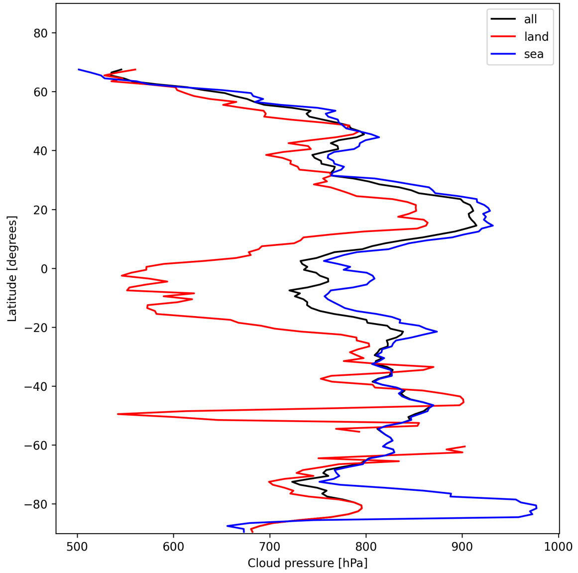
Figure 13: Zonal average of “Cloud pressure” for 2025-01-17 to 2025-01-19.
