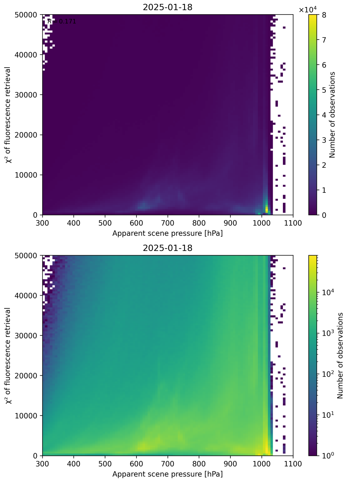
Figure 63: Scatter density plot of “Apparent scene pressure” against “ \chi^2 of fluorescence retrieval” for 2025-01-17 to 2025-01-19.
