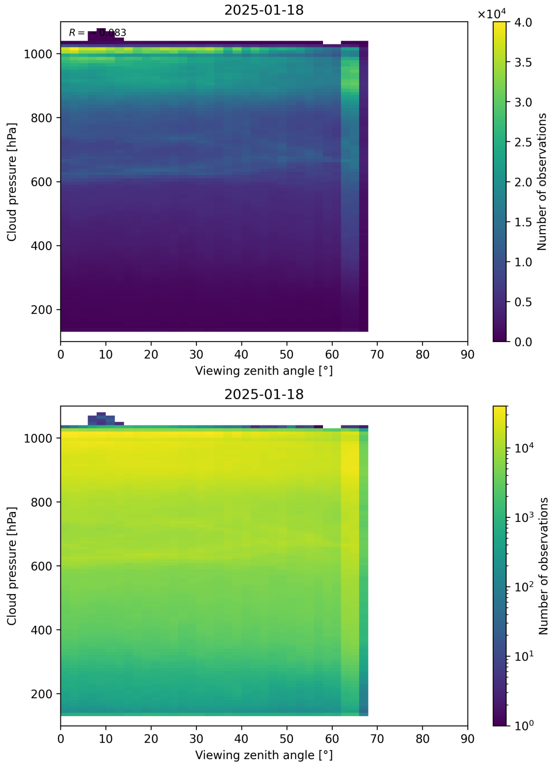
Figure 121: Scatter density plot of “Viewing zenith angle” against “Cloud pressure” for 2025-01-17 to 2025-01-19.
