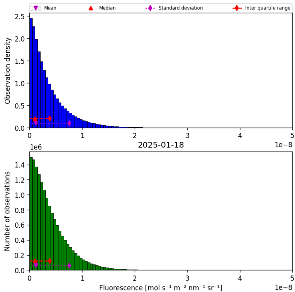
Figure 40: Histogram of “Fluorescence” for 2025-01-17 to 2025-01-19
