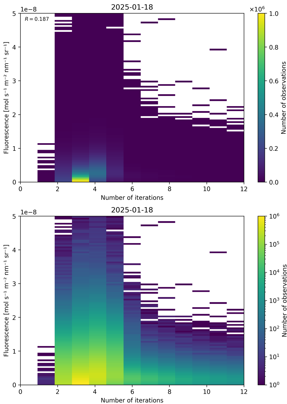
Figure 98: Scatter density plot of “Number of iterations” against “Fluorescence” for 2025-01-17 to 2025-01-19.
