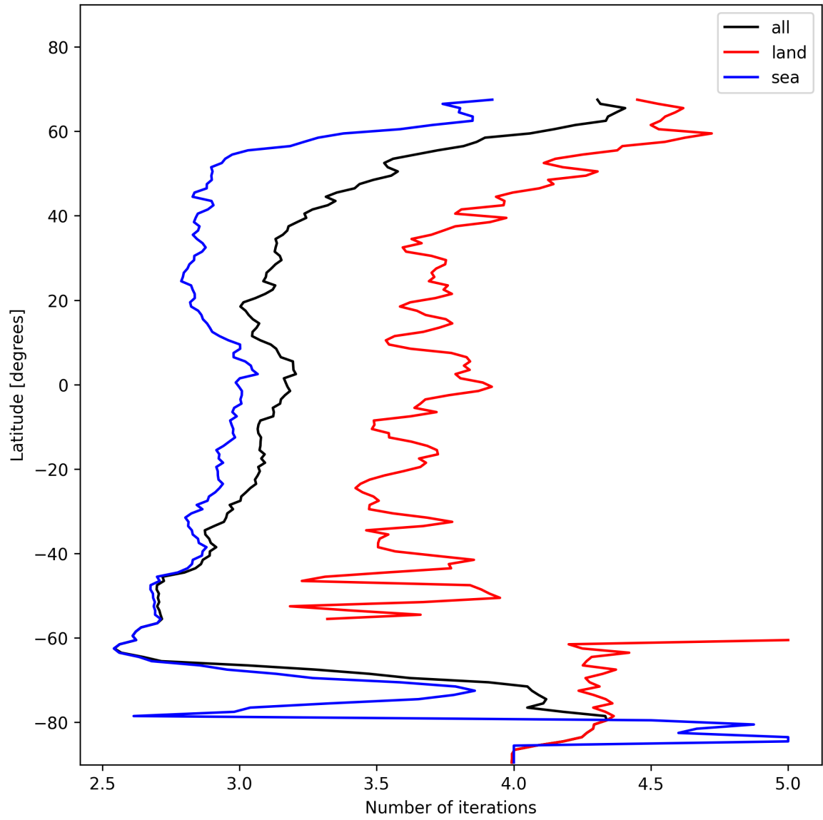
Figure 22: Zonal average of “Number of iterations” for 2025-01-17 to 2025-01-19.
