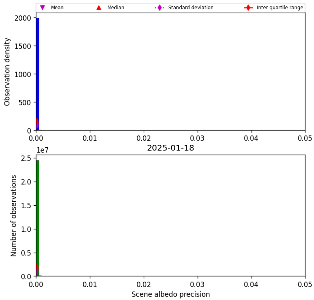
Figure 35: Histogram of “Scene albedo precision” for 2025-01-17 to 2025-01-19
