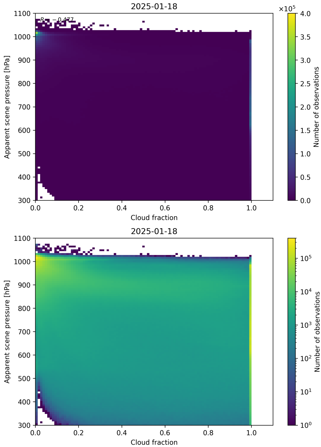
Figure 70: Scatter density plot of “Cloud fraction” against “Apparent scene pressure” for 2025-01-17 to 2025-01-19.
