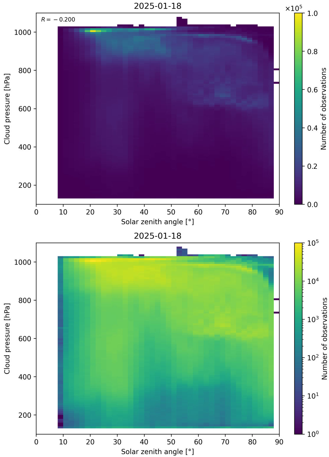
Figure 111: Scatter density plot of “Solar zenith angle” against “Cloud pressure” for 2025-01-17 to 2025-01-19.
