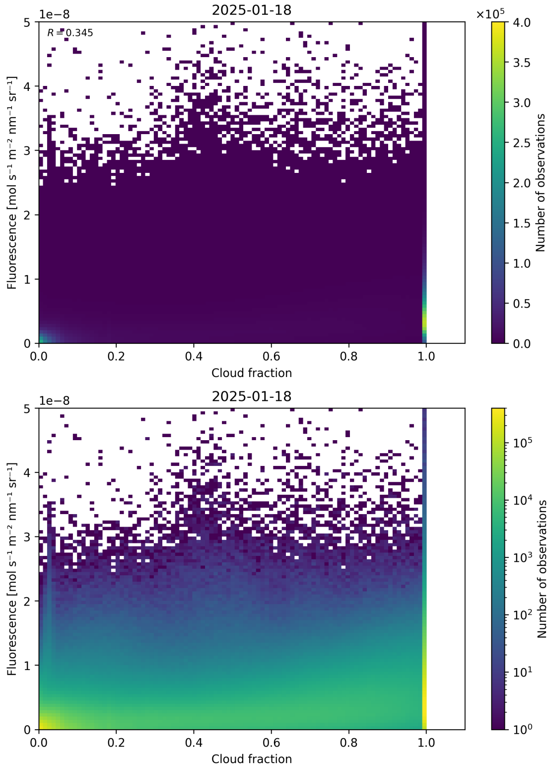
Figure 72: Scatter density plot of “Cloud fraction” against “Fluorescence” for 2025-01-17 to 2025-01-19.
