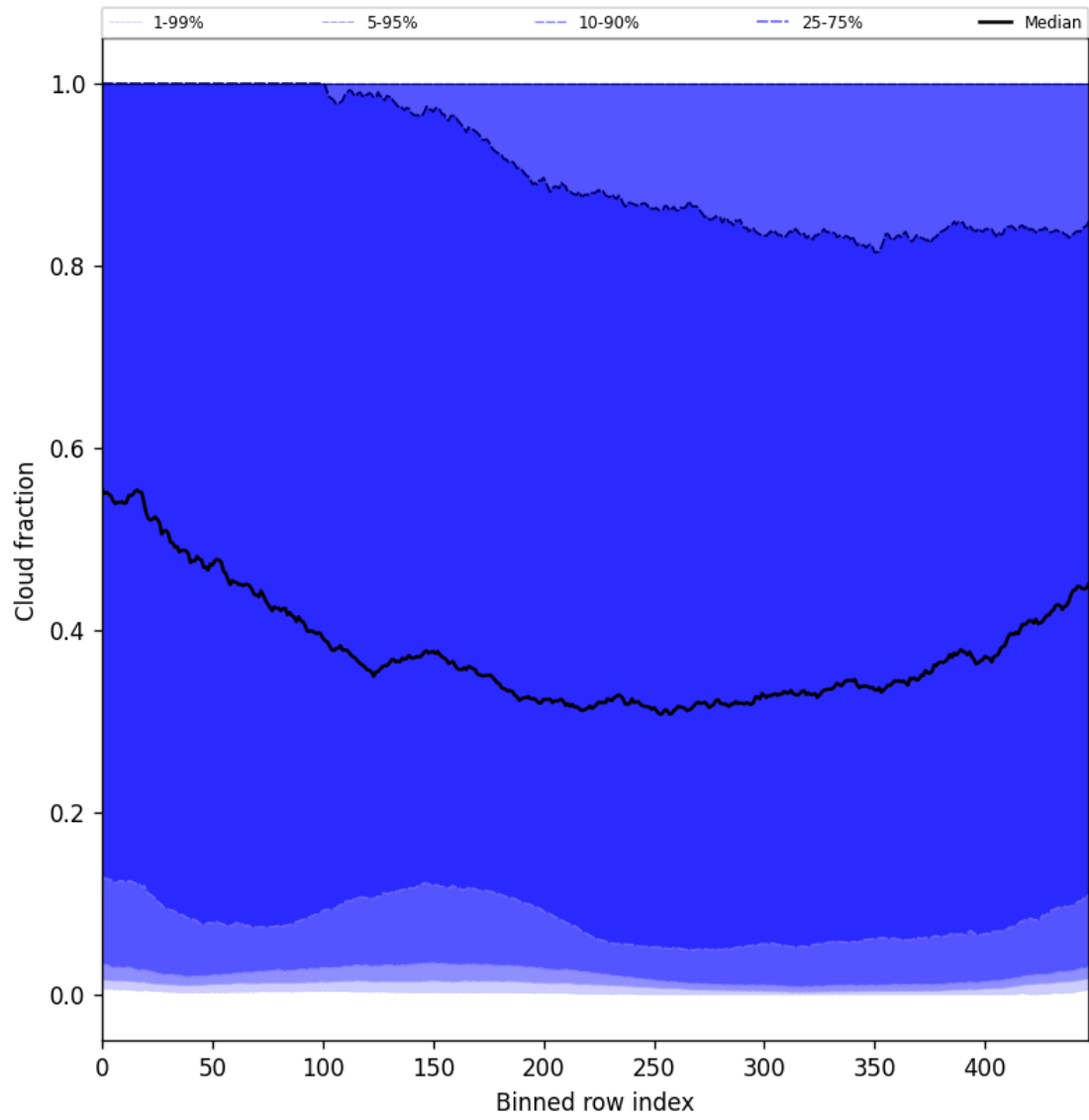
Figure 49: Along track statistics of “Cloud fraction” for 2025-01-17 to 2025-01-19
