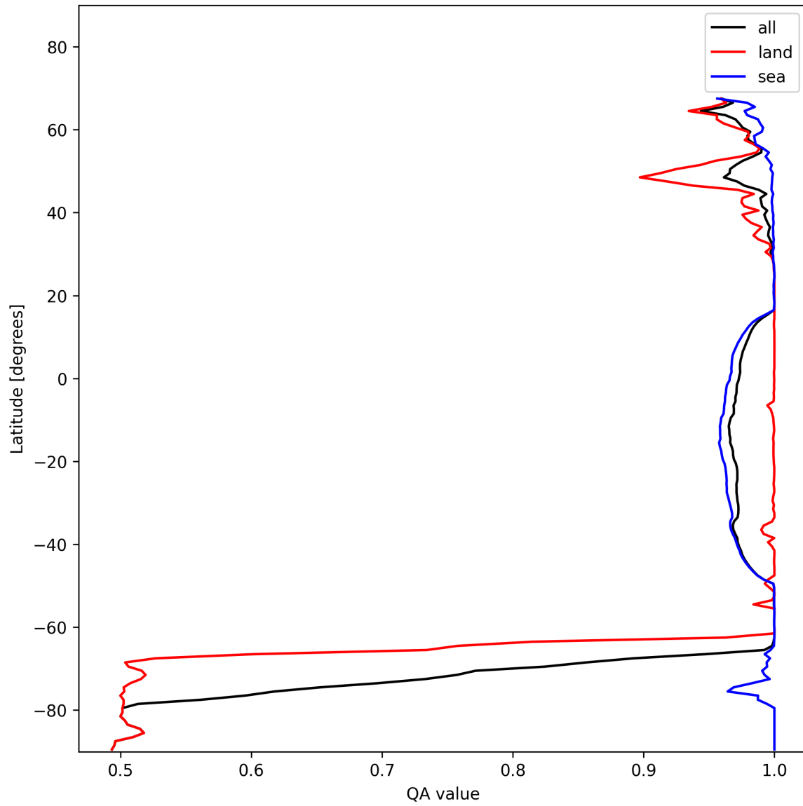
Figure 12: Zonal average of “QA value” for 2025-01-17 to 2025-01-19.
