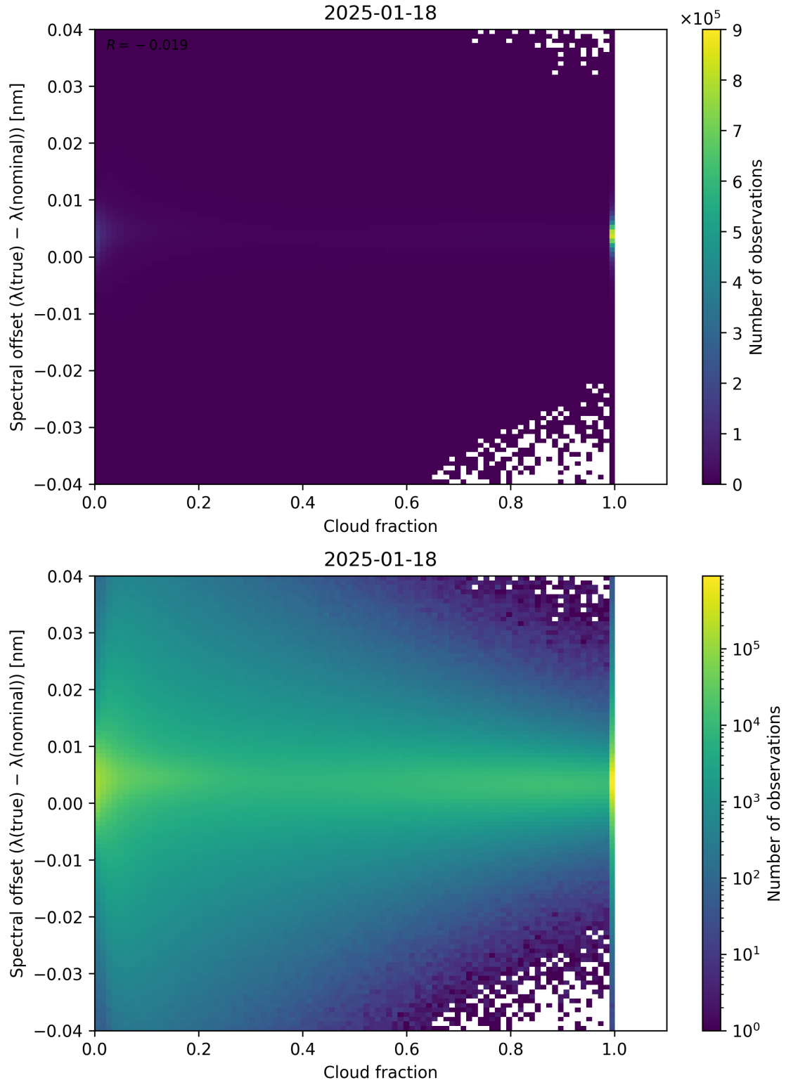
Figure 76: Scatter density plot of “Cloud fraction” against “Spectral offset ( \lambda_{\text{true}} - \lambda_{\text{nominal}} )” for 2025-01-17 to 2025-01-19.
