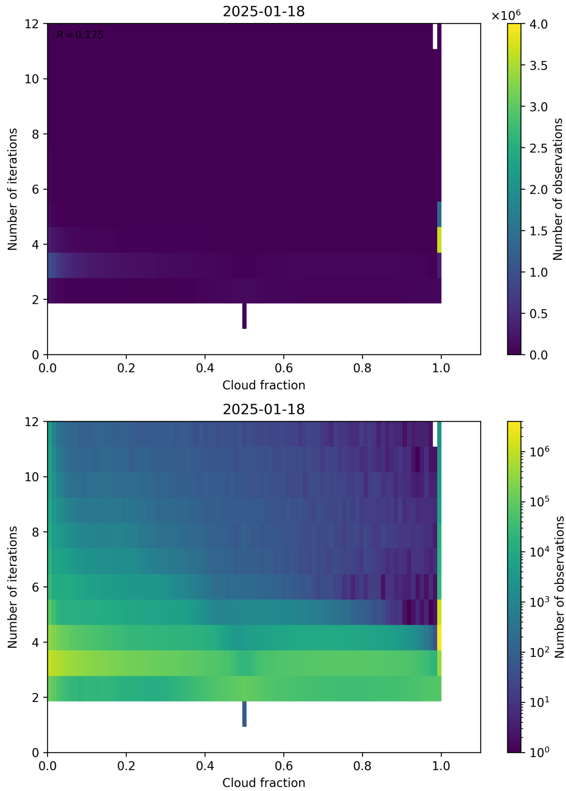
Figure 73: Scatter density plot of “Cloud fraction” against “Number of iterations” for 2025-01-17 to 2025-01-19.
