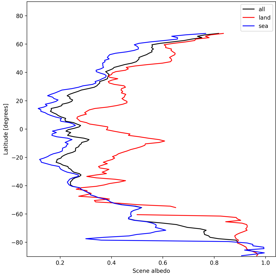
Figure 17: Zonal average of “Scene albedo” for 2025-01-17 to 2025-01-19.
