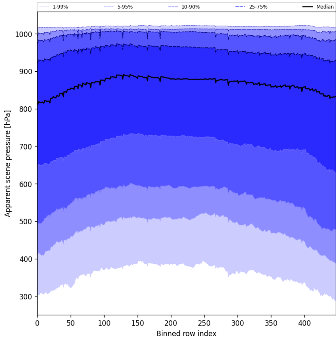
Figure 53: Along track statistics of “Apparent scene pressure” for 2025-01-17 to 2025-01-19
