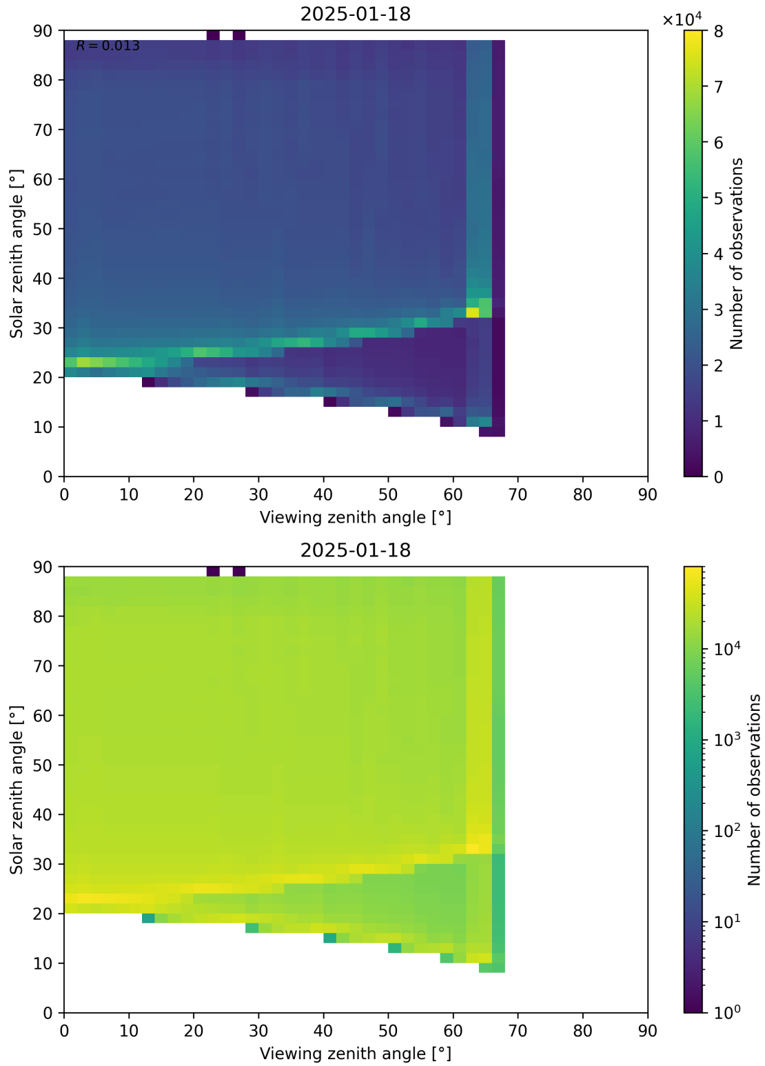
Figure 127: Scatter density plot of “Viewing zenith angle” against “Solar zenith angle” for 2025-01-17 to 2025-01-19.
