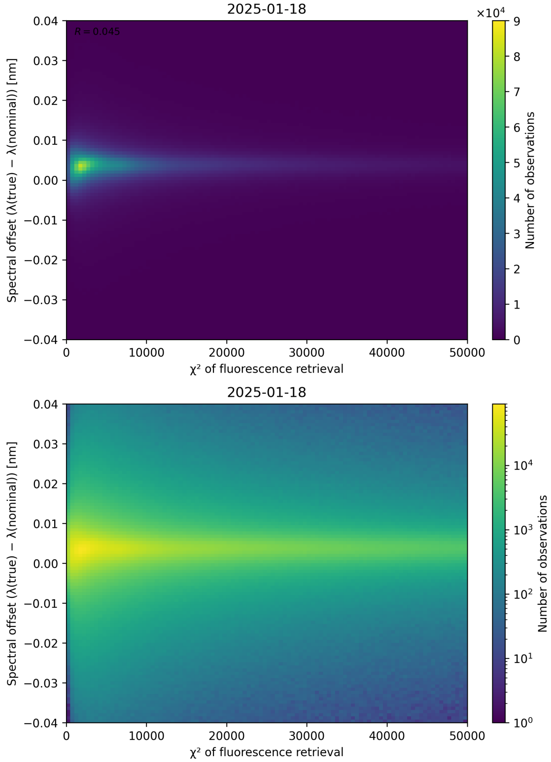
Figure 69: Scatter density plot of “ \chi^2 of fluorescence retrieval” against “Spectral offset ( \lambda_{\text{true}} - \lambda_{\text{nominal}} )” for 2025-01-17 to 2025-01-19.
