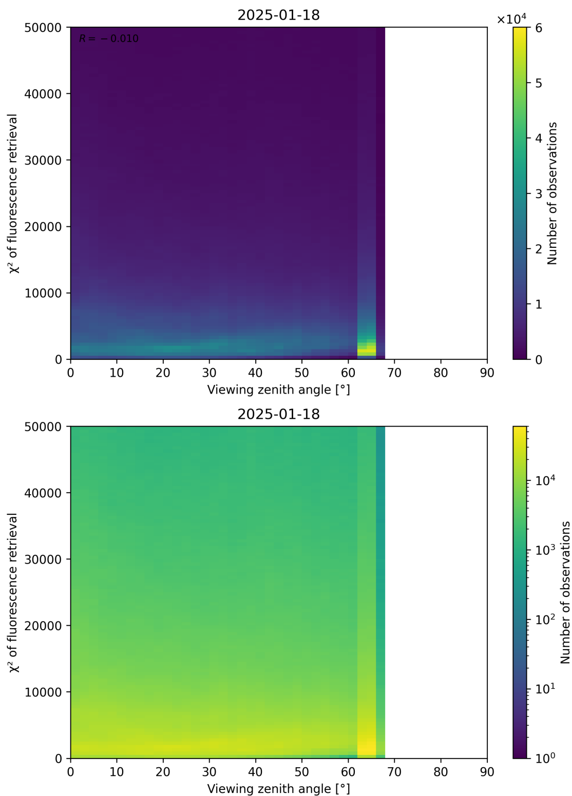
Figure 119: Scatter density plot of “Viewing zenith angle” against “ \chi^2 of fluorescence retrieval” for 2025-01-17 to 2025-01-19.
