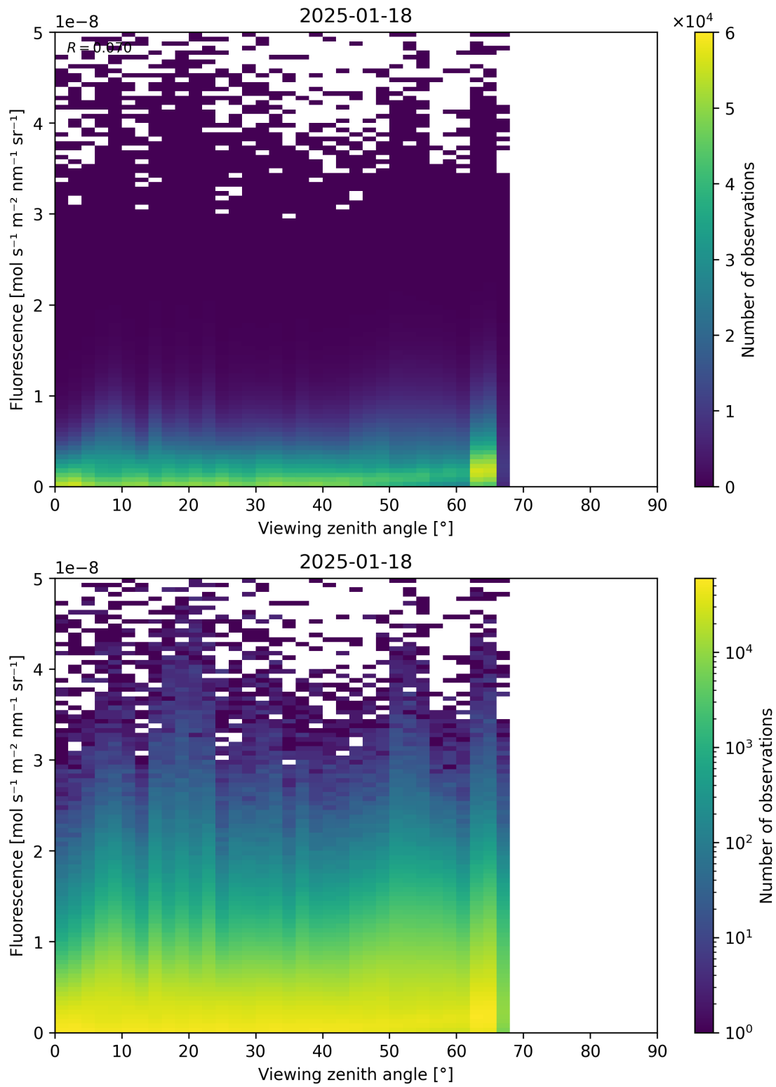
Figure 122: Scatter density plot of “Viewing zenith angle” against “Fluorescence” for 2025-01-17 to 2025-01-19.
