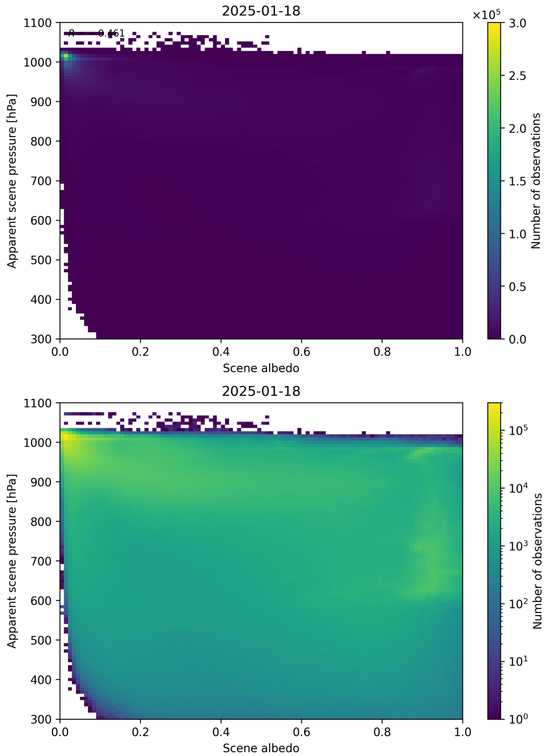
Figure 102: Scatter density plot of “Scene albedo” against “Apparent scene pressure” for 2025-01-17 to 2025-01-19.
