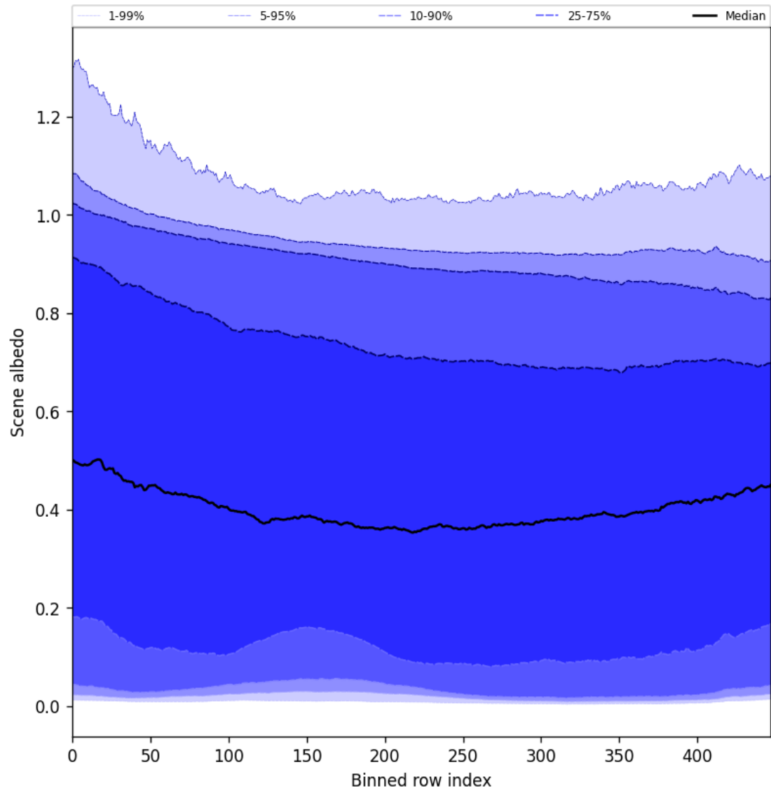
Figure 51: Along track statistics of “Scene albedo” for 2025-01-17 to 2025-01-19
