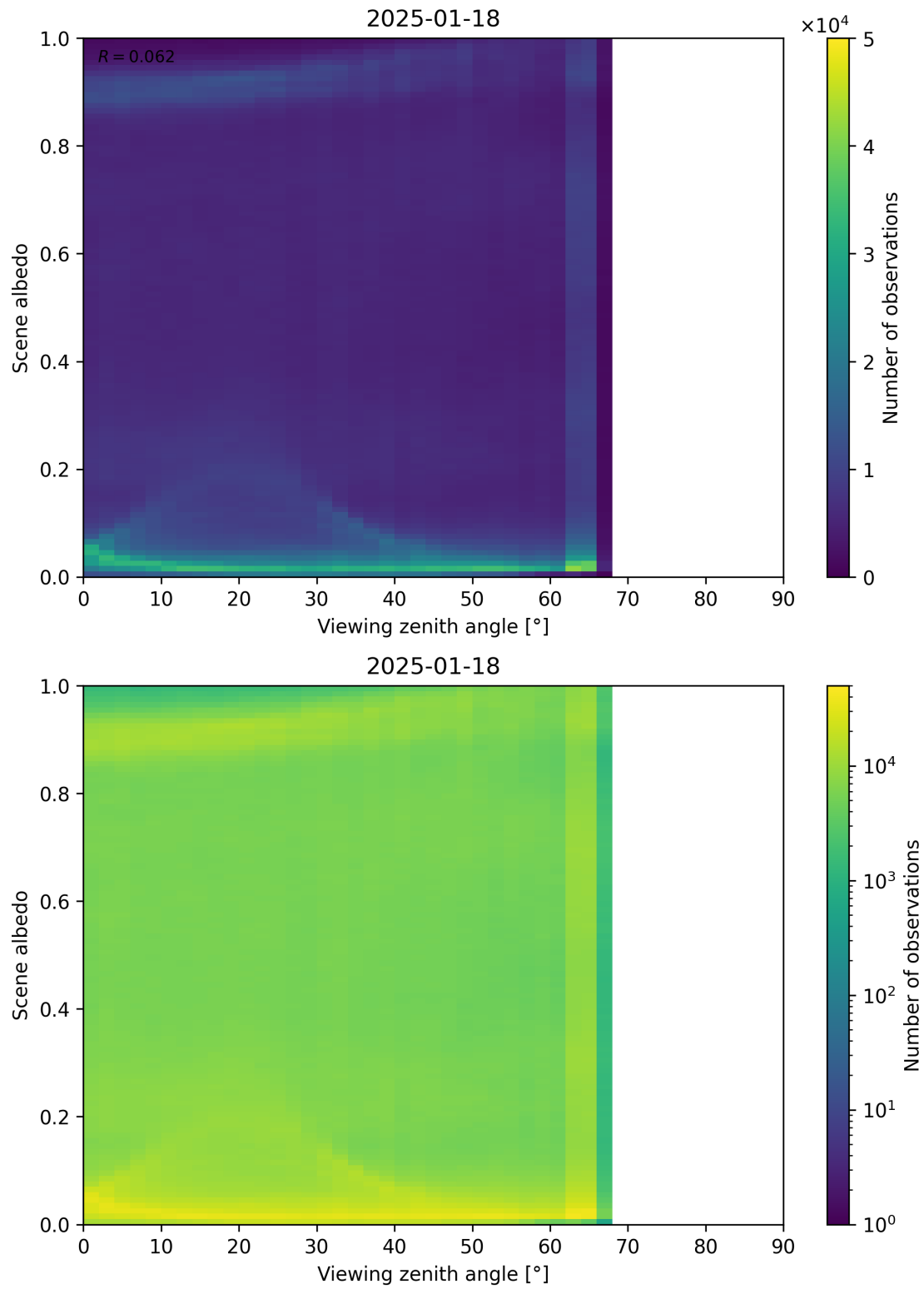
Figure 126: Scatter density plot of “Viewing zenith angle” against “Scene albedo” for 2025-01-17 to 2025-01-19.
