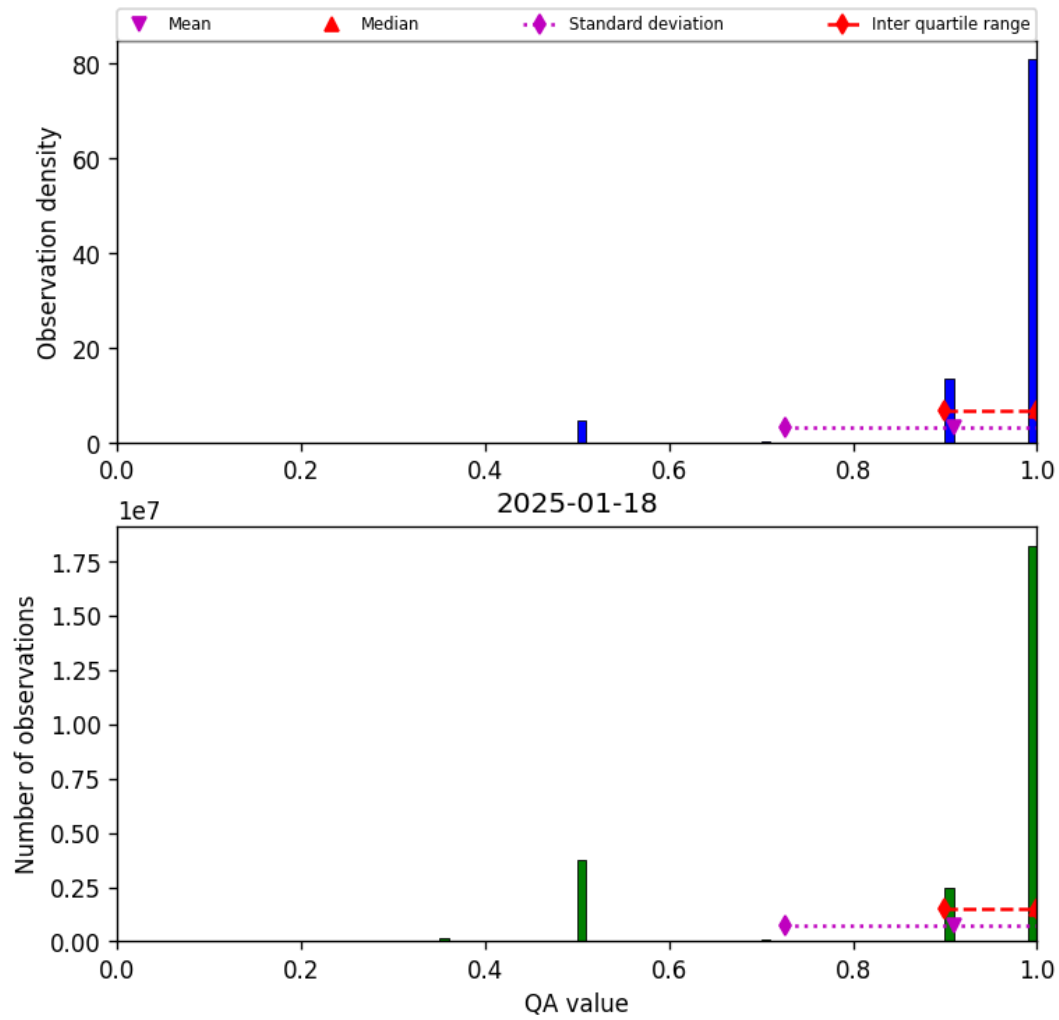
Figure 29: Histogram of “QA value” for 2025-01-17 to 2025-01-19
