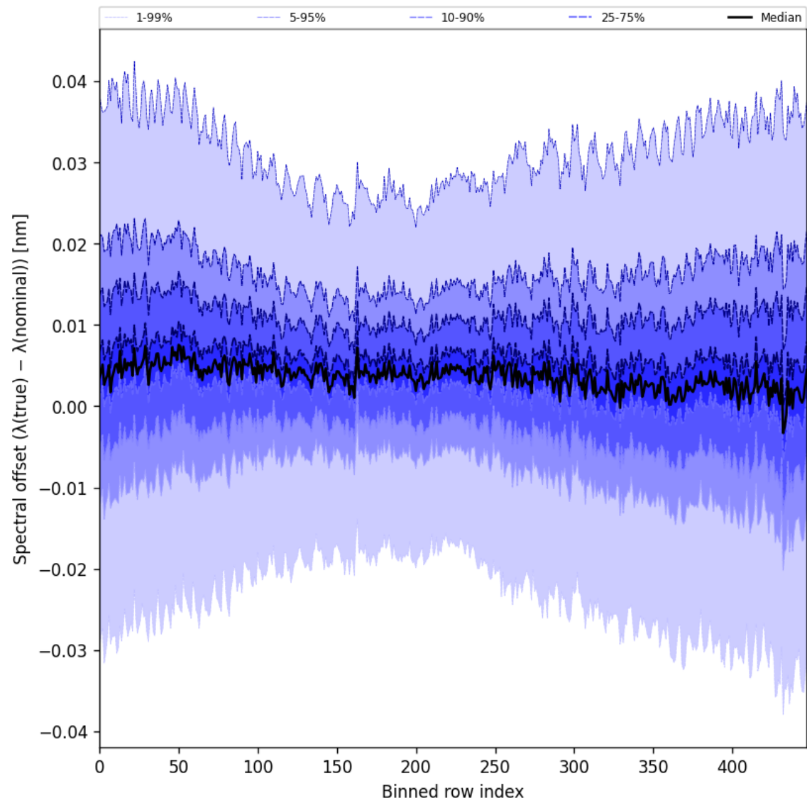
Figure 62: Along track statistics of “Spectral offset ( \lambda_{\text{true}} - \lambda_{\text{nominal}} )” for 2025-01-17 to 2025-01-19
