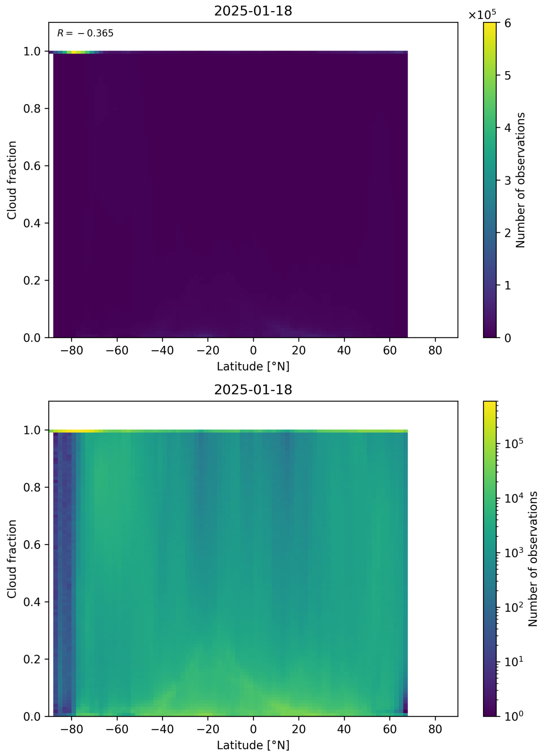
Figure 90: Scatter density plot of “Latitude” against “Cloud fraction” for 2025-01-17 to 2025-01-19.
