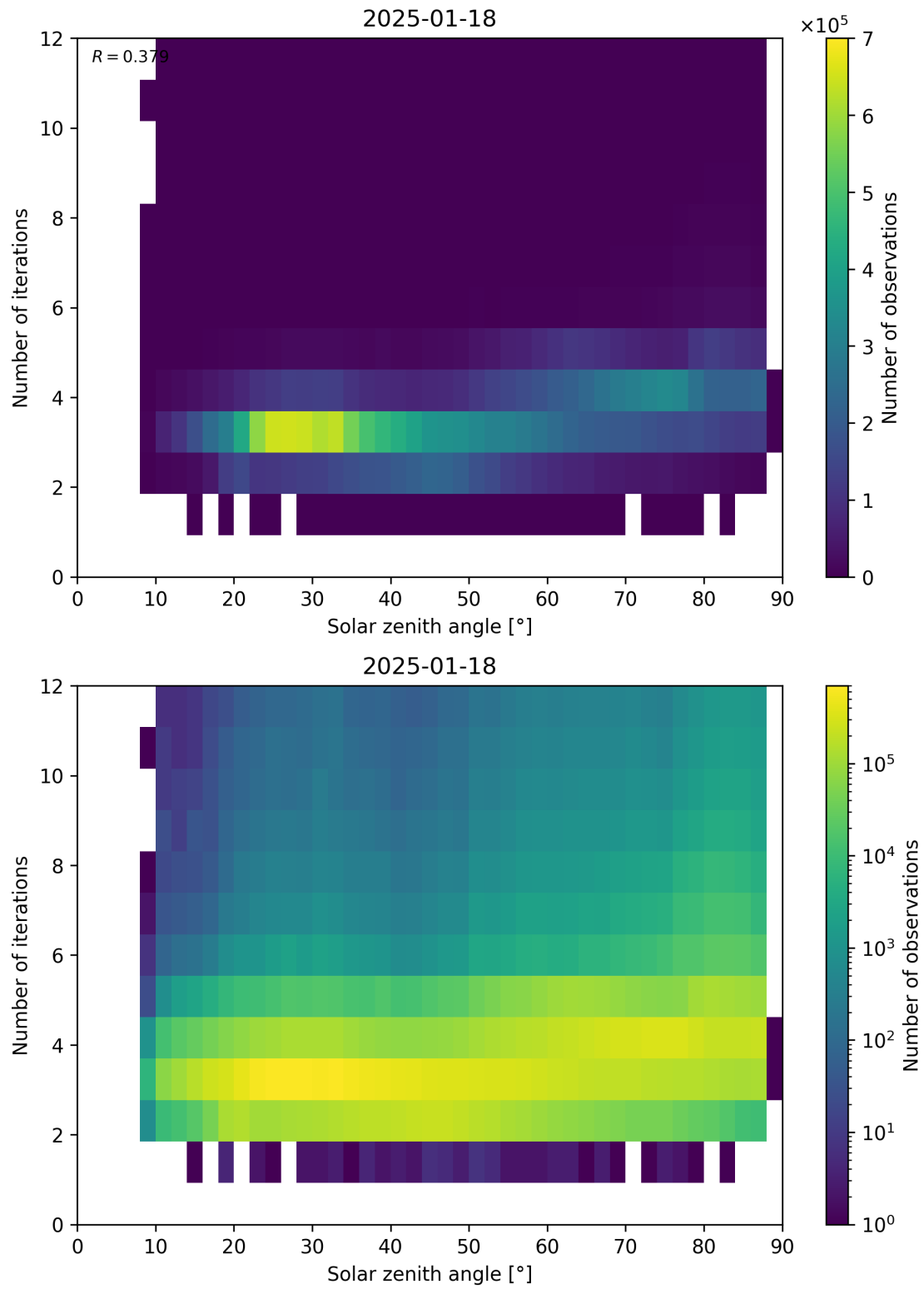
Figure 114: Scatter density plot of “Solar zenith angle” against “Number of iterations” for 2025-01-17 to 2025-01-19.
