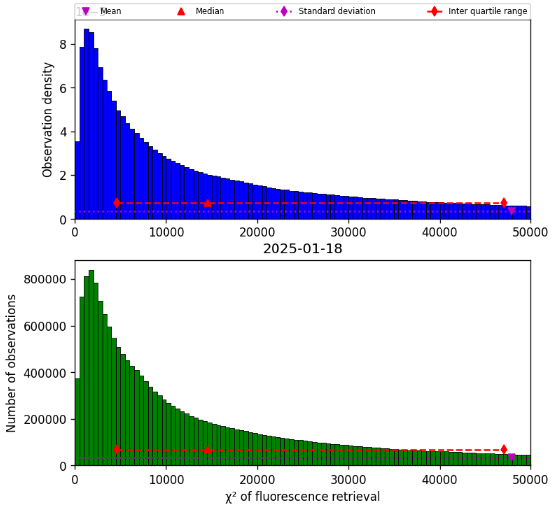
Figure 42: Histogram of “ \chi^2 of fluorescence retrieval” for 2025-01-17 to 2025-01-19
