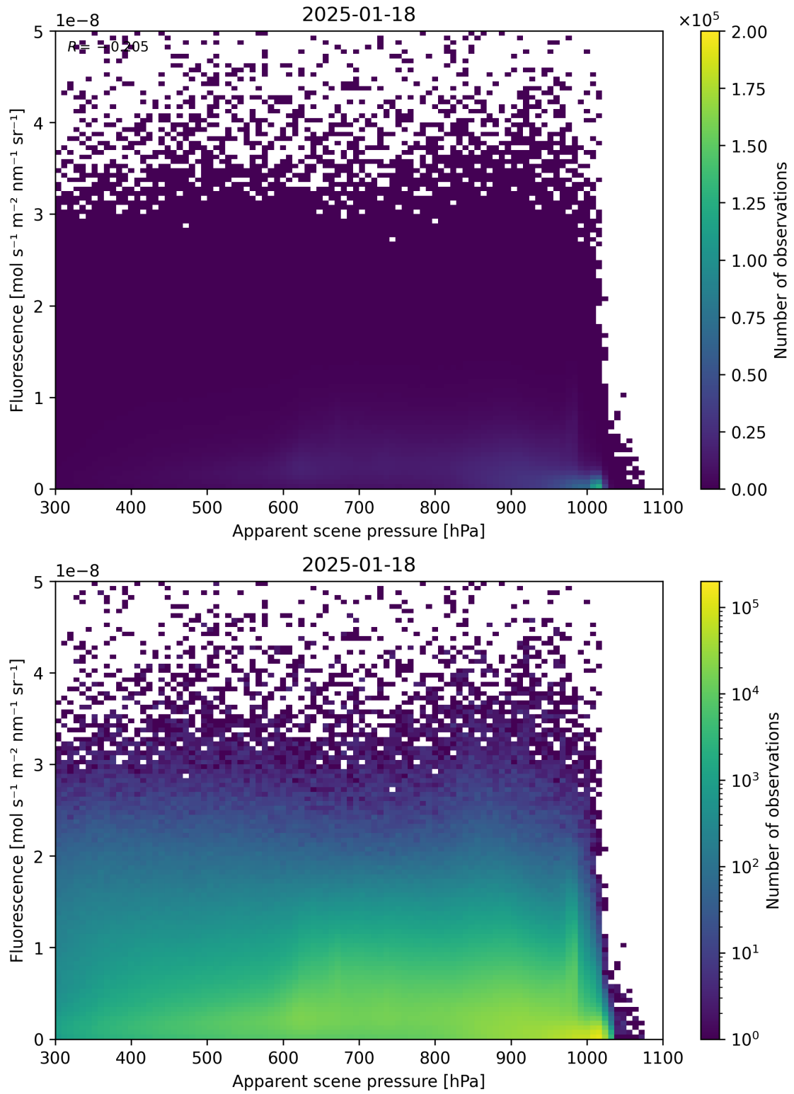
Figure 64: Scatter density plot of “Apparent scene pressure” against “Fluorescence” for 2025-01-17 to 2025-01-19.
