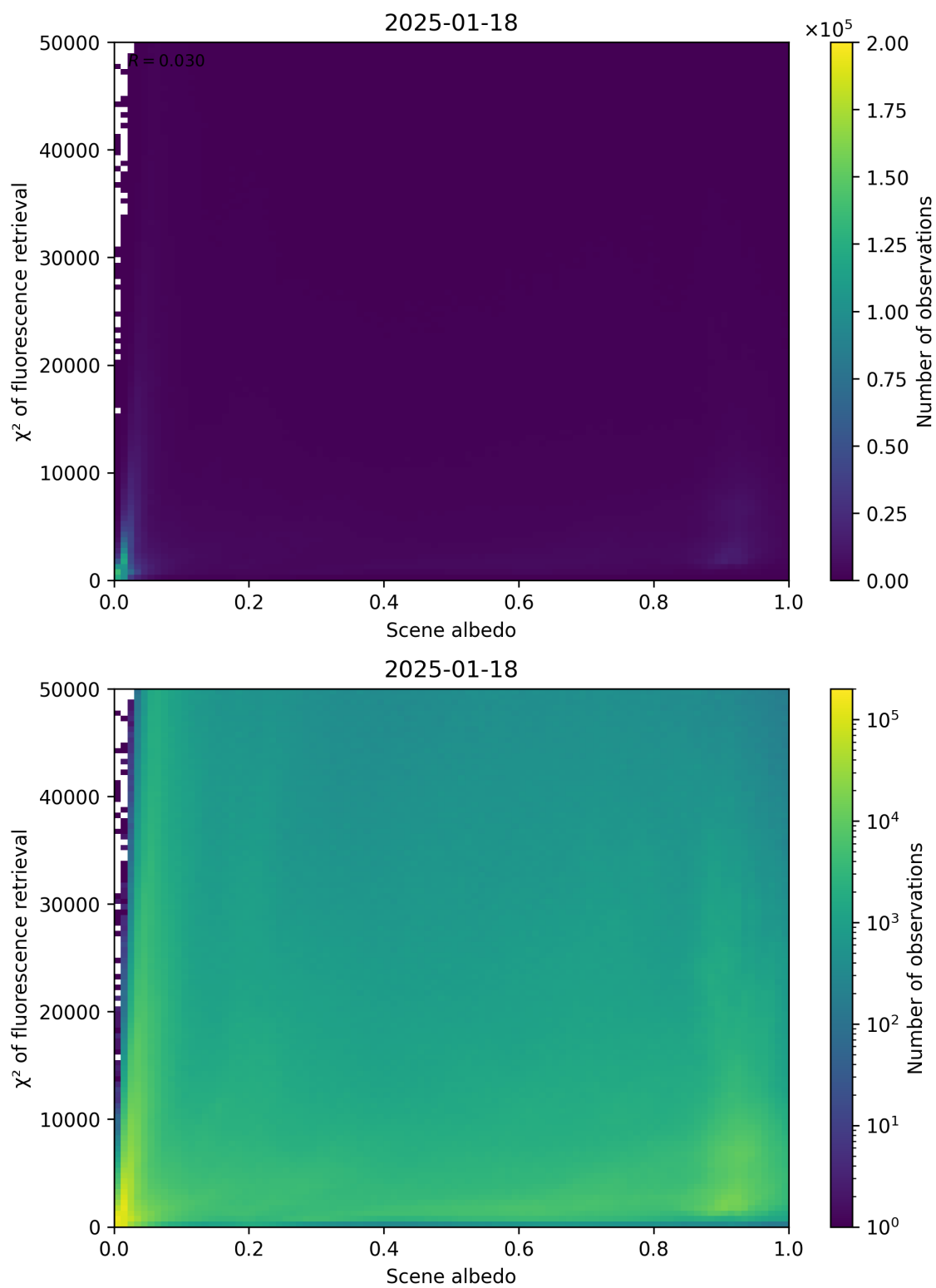
Figure 103: Scatter density plot of “Scene albedo” against “ \chi^2 of fluorescence retrieval” for 2025-01-17 to 2025-01-19.
