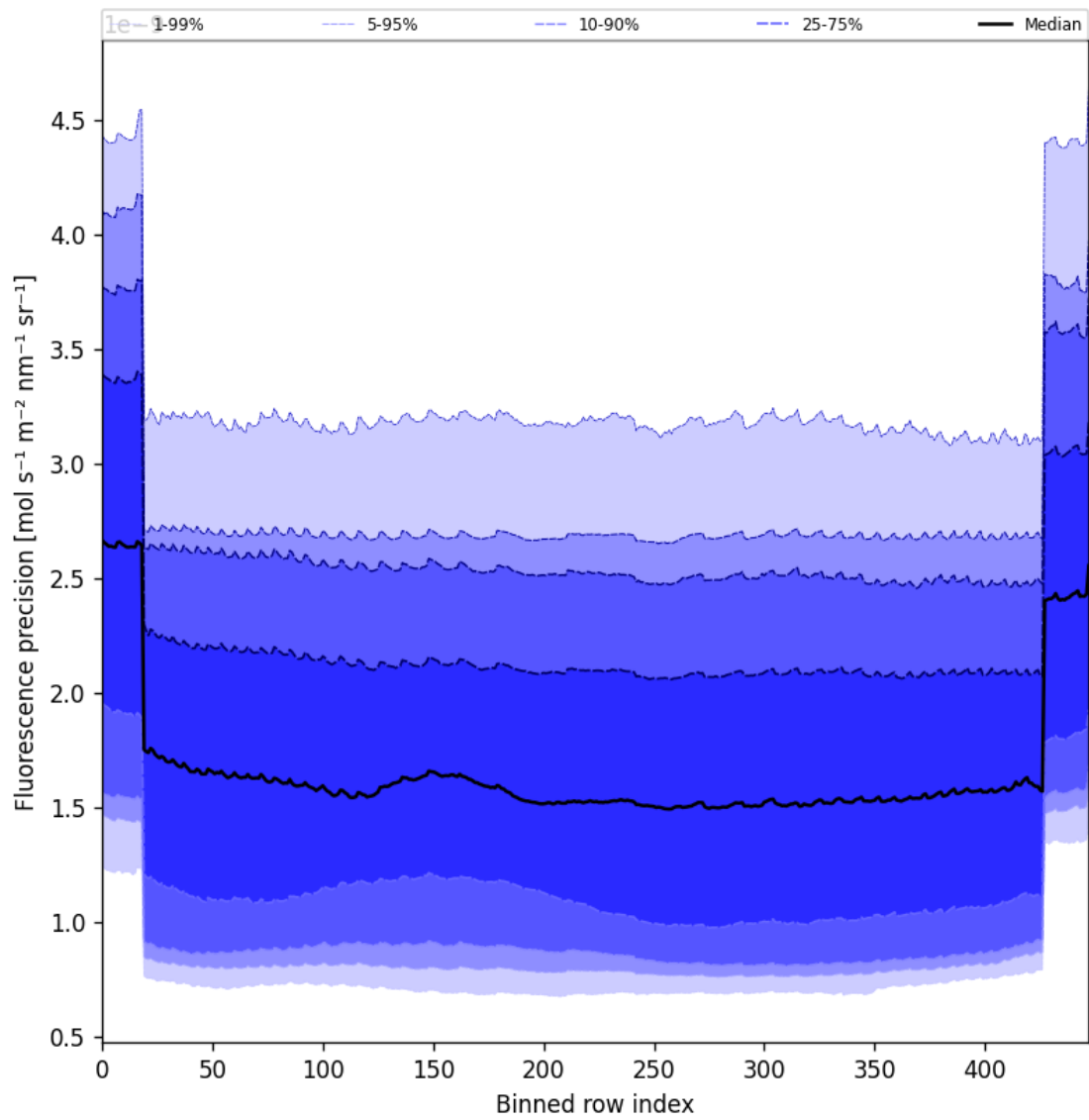
Figure 58: Along track statistics of “Fluorescence precision” for 2025-01-17 to 2025-01-19
