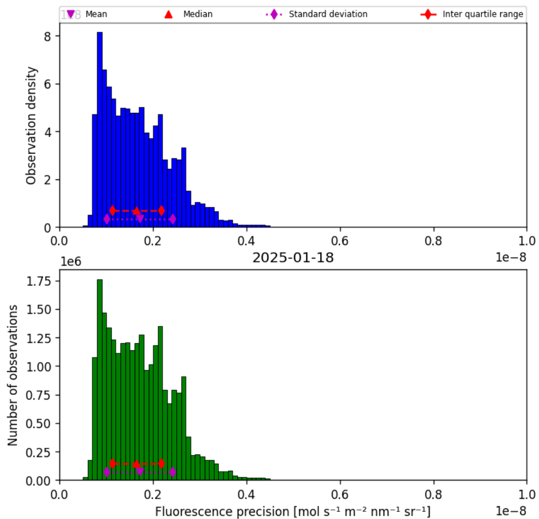
Figure 41: Histogram of “Fluorescence precision” for 2025-01-17 to 2025-01-19
