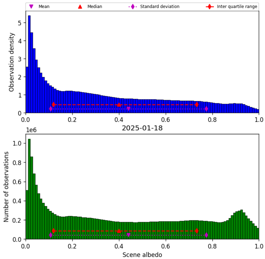
Figure 34: Histogram of “Scene albedo” for 2025-01-17 to 2025-01-19
