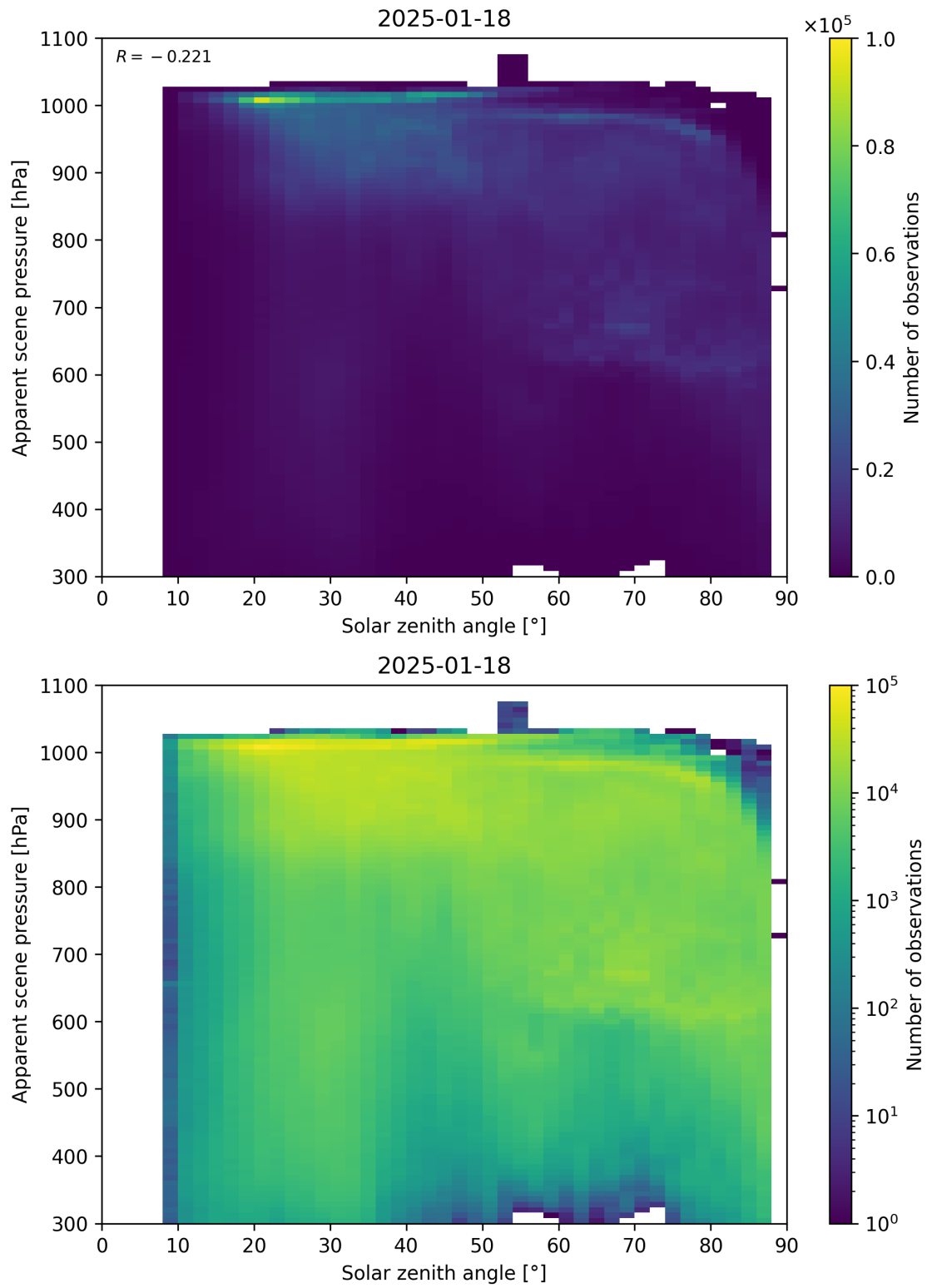
Figure 108: Scatter density plot of “Solar zenith angle” against “Apparent scene pressure” for 2025-01-17 to 2025-01-19.
