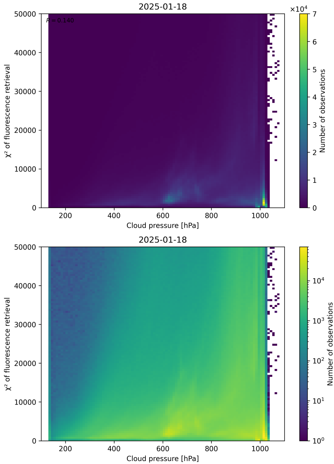
Figure 78: Scatter density plot of “Cloud pressure” against “ \chi^2 of fluorescence retrieval” for 2025-01-17 to 2025-01-19.
