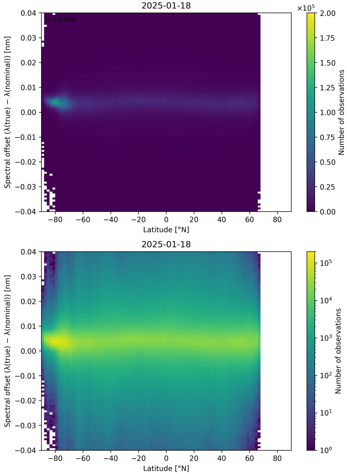
Figure 96: Scatter density plot of “Latitude” against “Spectral offset ( \lambda_{\text{true}} - \lambda_{\text{nominal}} )” for 2025-01-17 to 2025-01-19.
