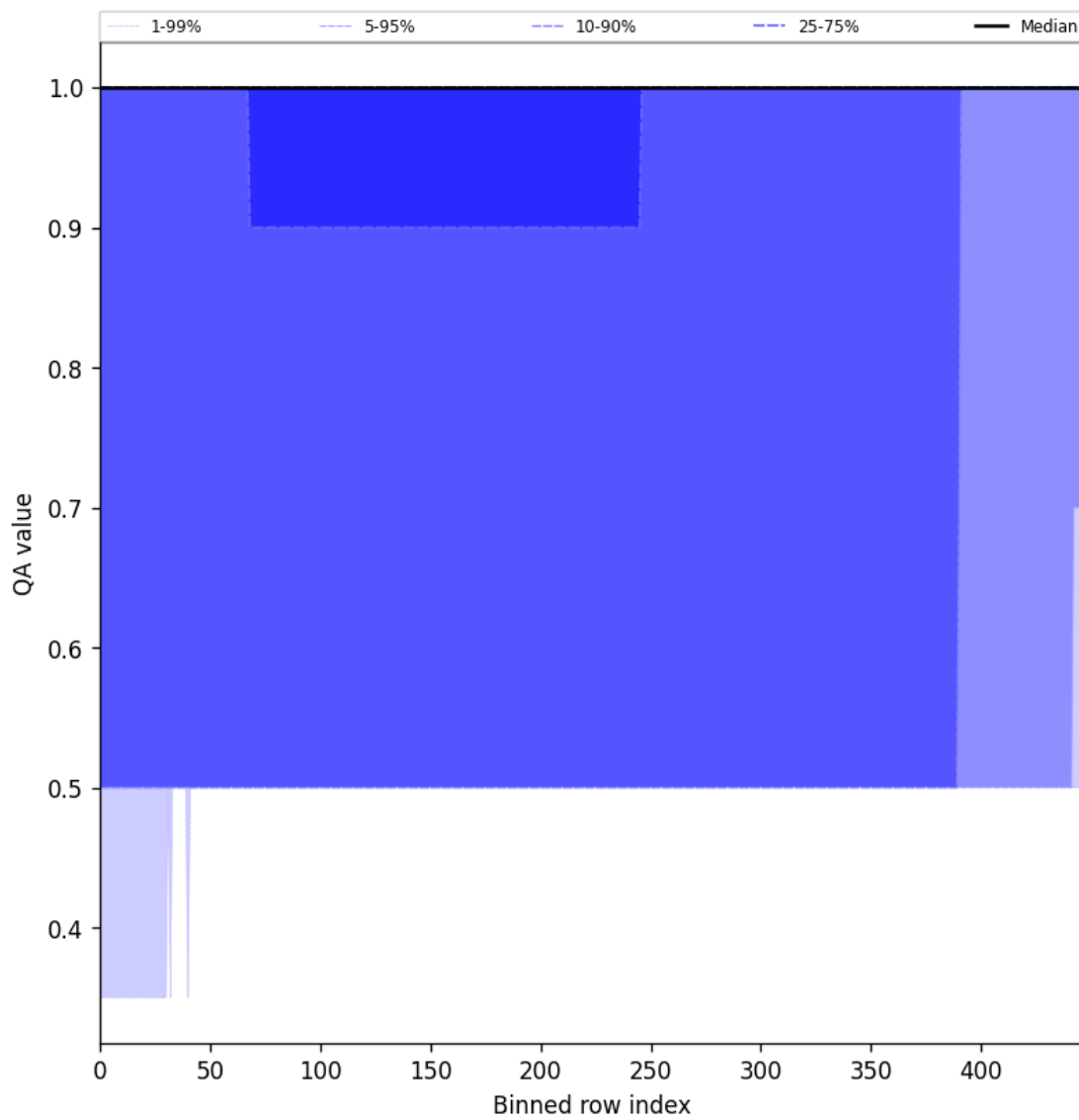
Figure 46: Along track statistics of “QA value” for 2025-01-17 to 2025-01-19
