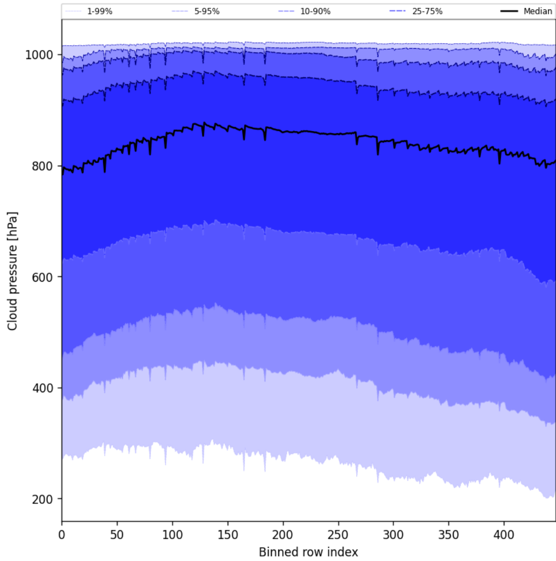
Figure 47: Along track statistics of “Cloud pressure” for 2025-01-17 to 2025-01-19
