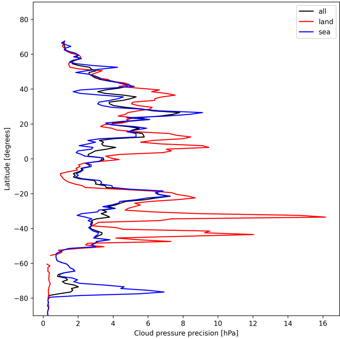
Figure 14: Zonal average of “Cloud pressure precision” for 2025-01-17 to 2025-01-19.
