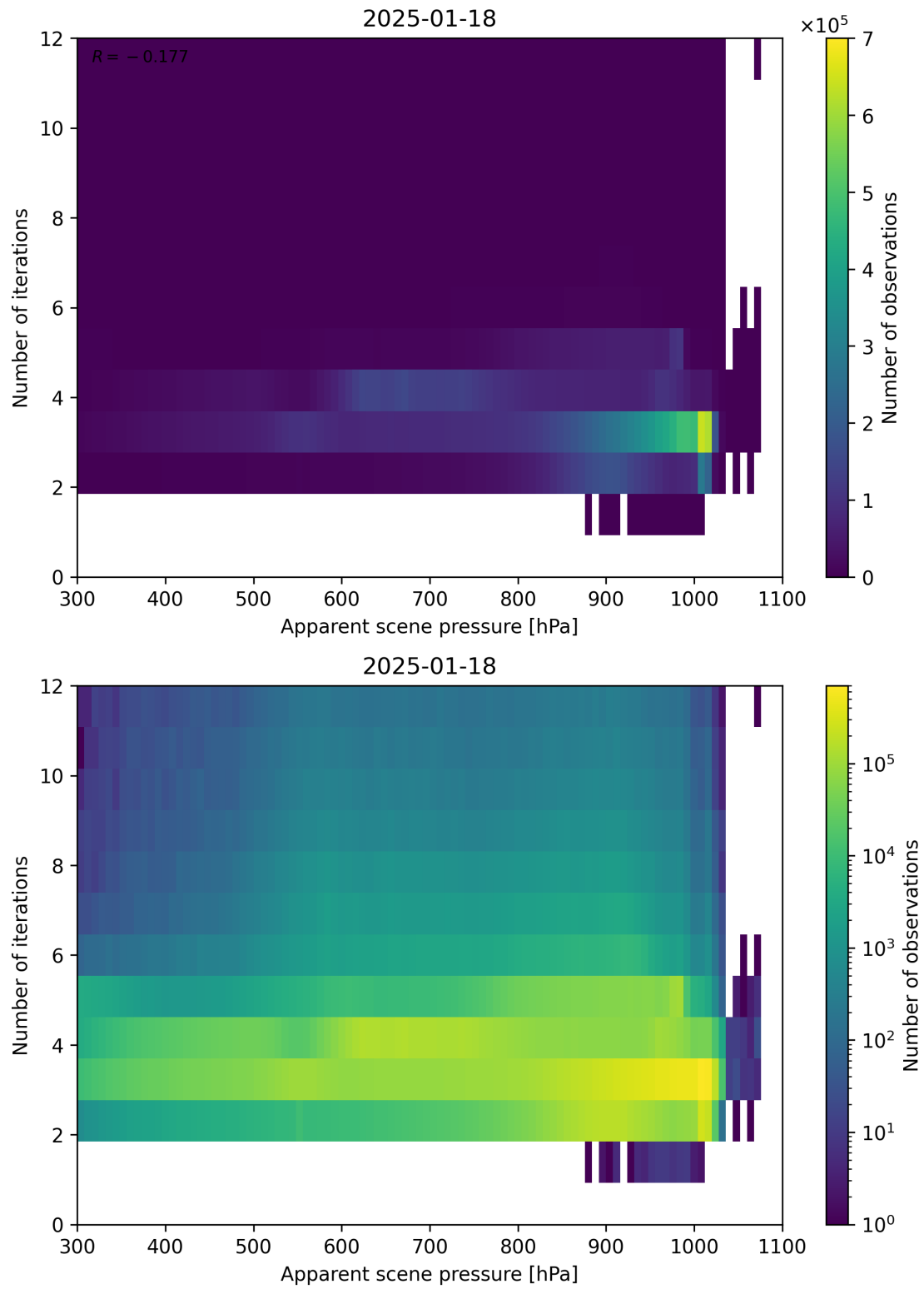
Figure 65: Scatter density plot of “Apparent scene pressure” against “Number of iterations” for 2025-01-17 to 2025-01-19.
