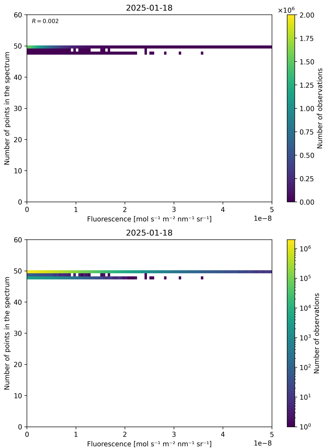
Figure 86: Scatter density plot of “Fluorescence” against “Number of points in the spectrum” for 2025-01-17 to 2025-01-19.
