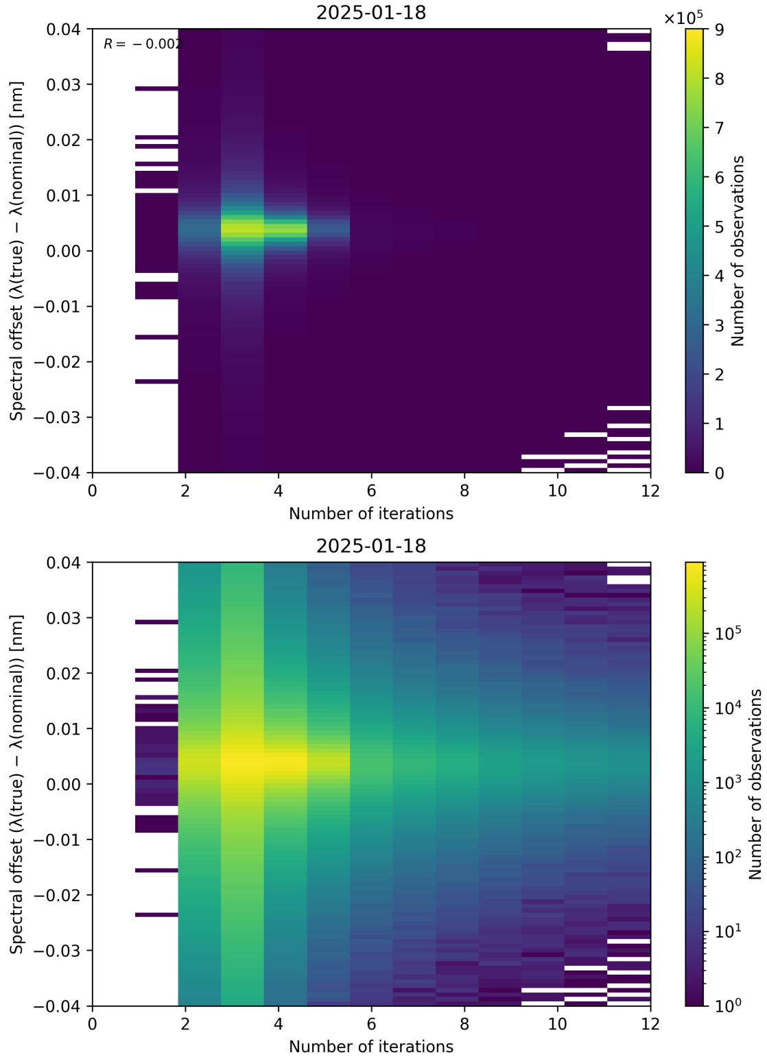
Figure 100: Scatter density plot of “Number of iterations” against “Spectral offset ( \lambda_{\text{true}} - \lambda_{\text{nominal}} )” for 2025-01-17 to 2025-01-19.
