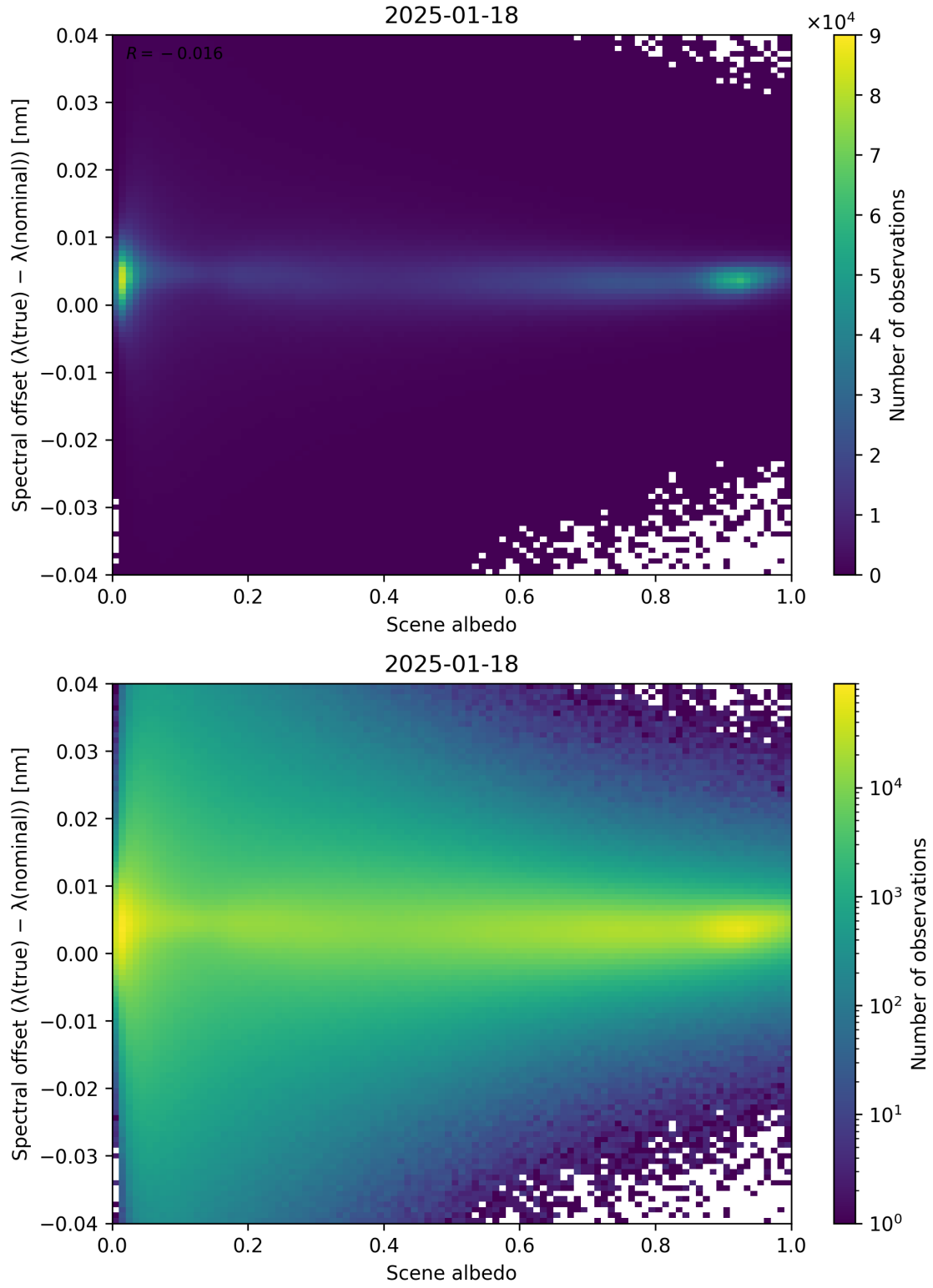
Figure 107: Scatter density plot of “Scene albedo” against “Spectral offset ( \lambda_{\text{true}} - \lambda_{\text{nominal}} )” for 2025-01-17 to 2025-01-19.
