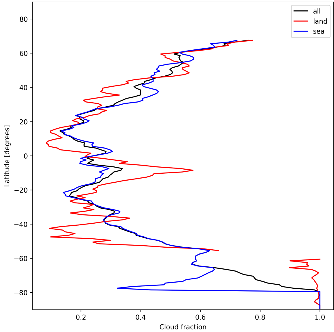
Figure 15: Zonal average of “Cloud fraction” for 2025-01-17 to 2025-01-19.
