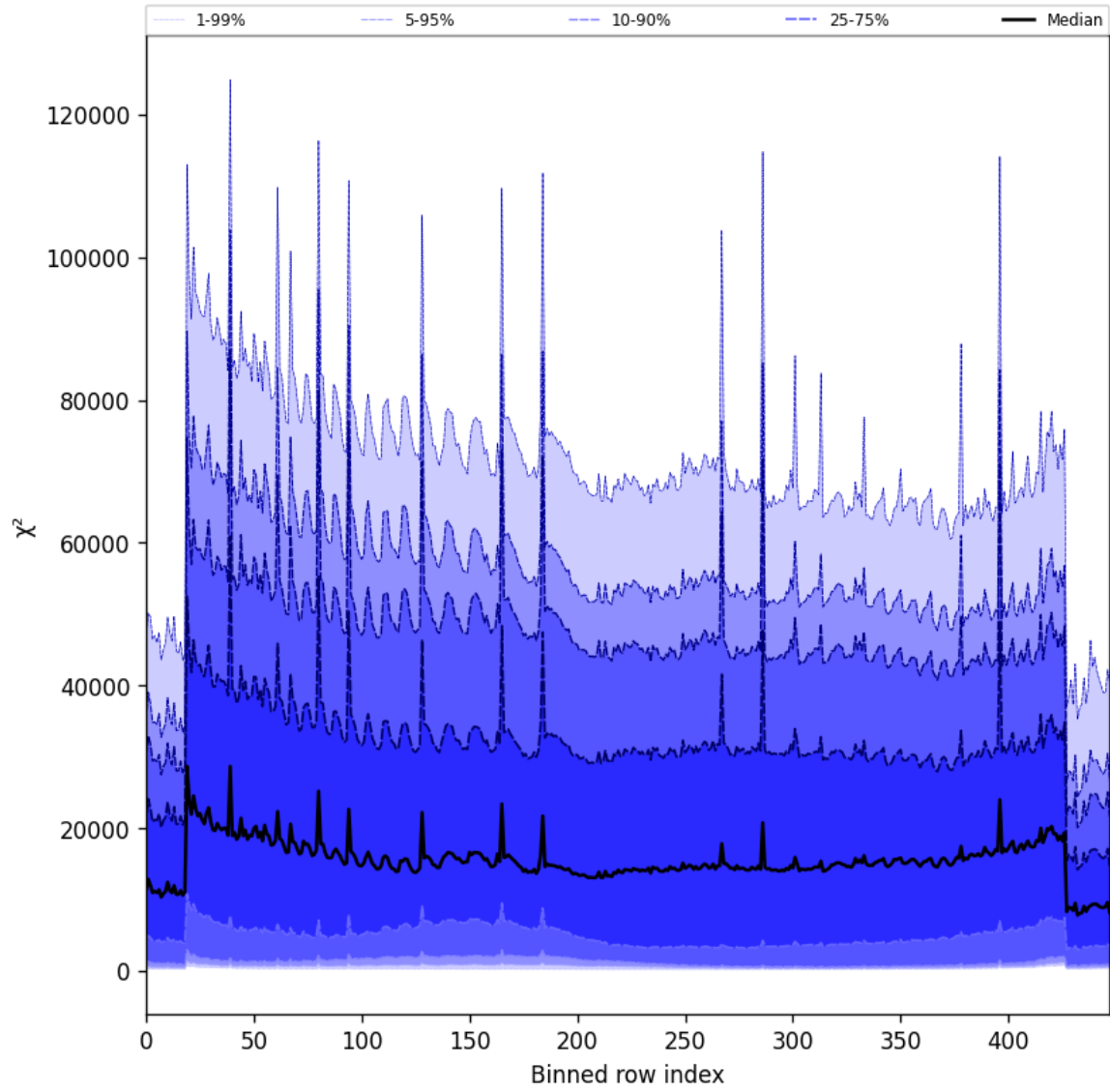
Figure 55: Along track statistics of “ \chi^2 ” for 2025-01-17 to 2025-01-19
