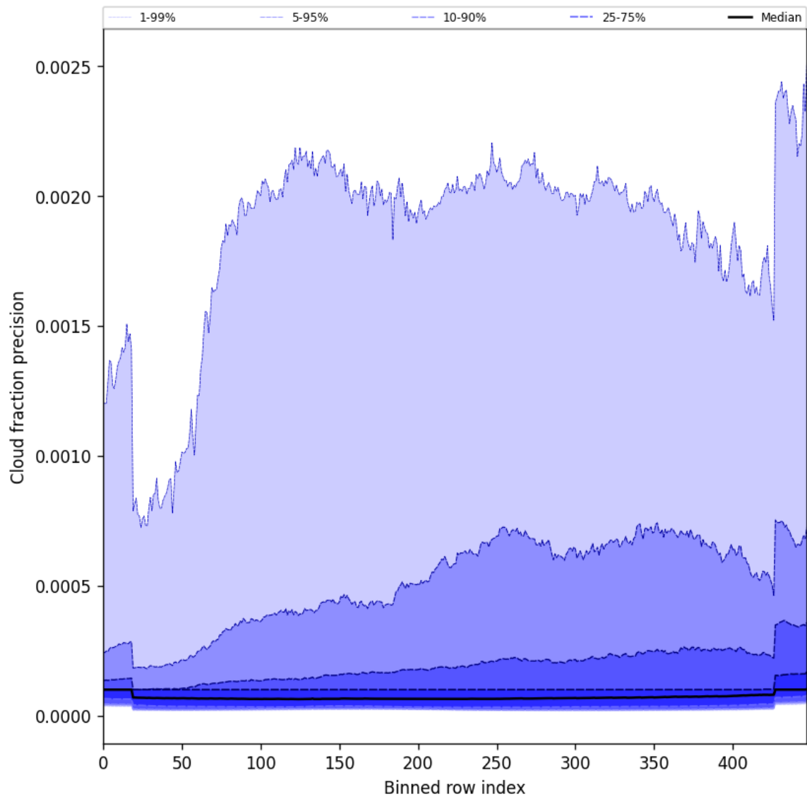
Figure 50: Along track statistics of “Cloud fraction precision” for 2025-01-17 to 2025-01-19
