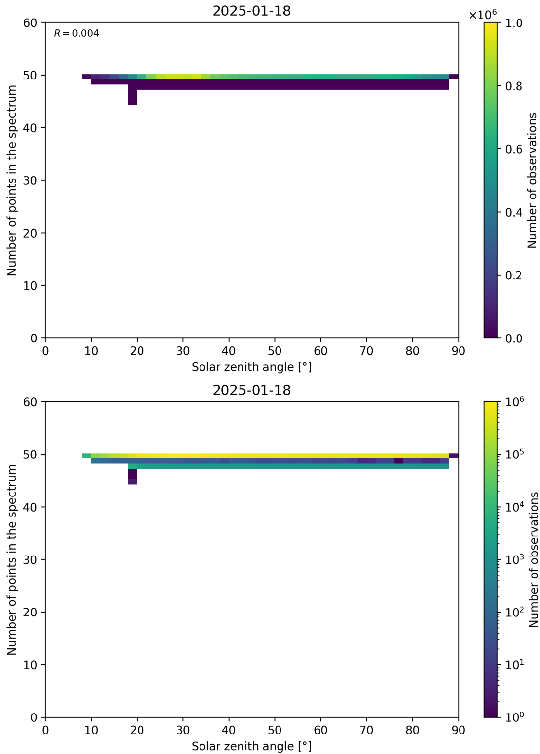
Figure 115: Scatter density plot of “Solar zenith angle” against “Number of points in the spectrum” for 2025-01-17 to 2025-01-19.
