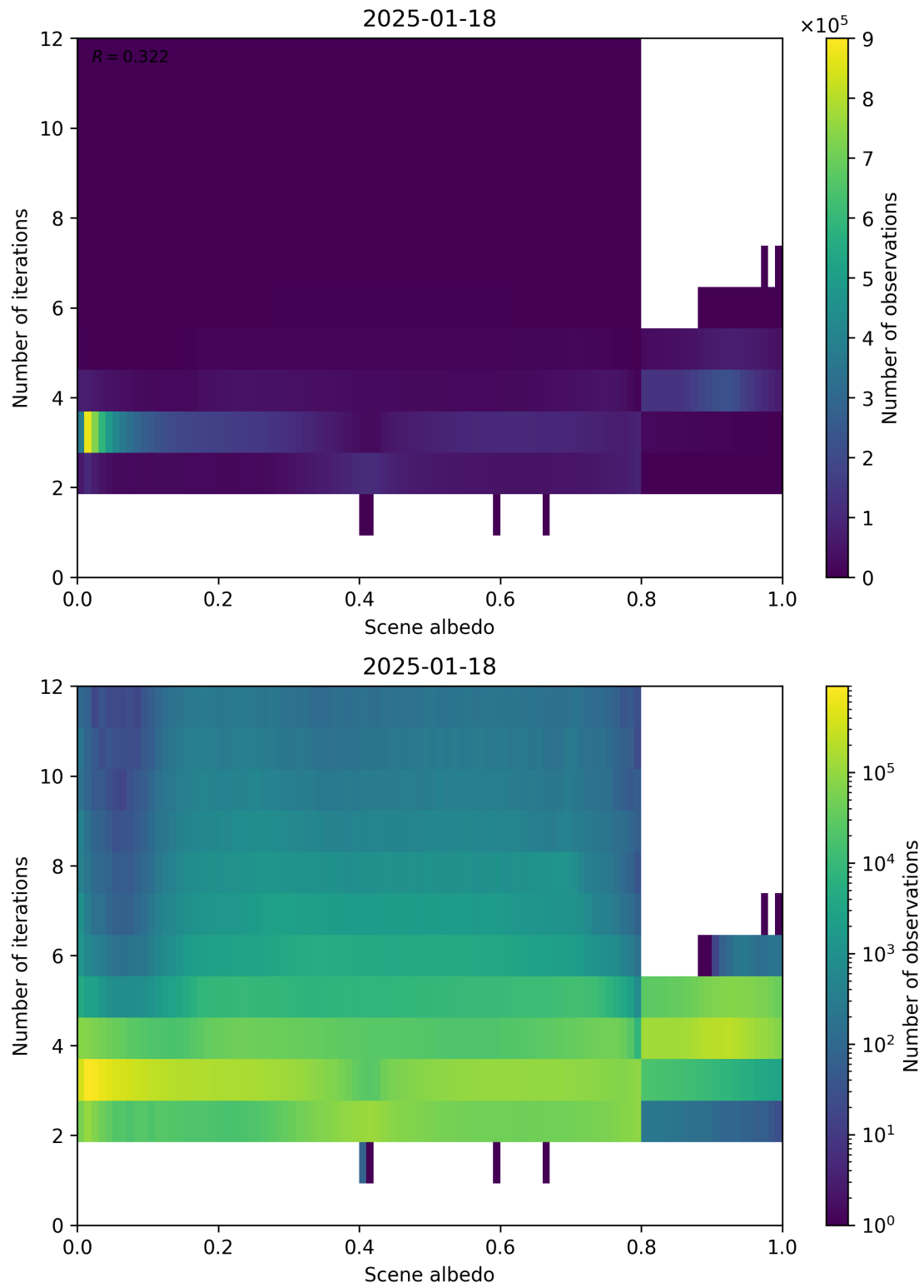
Figure 105: Scatter density plot of “Scene albedo” against “Number of iterations” for 2025-01-17 to 2025-01-19.
