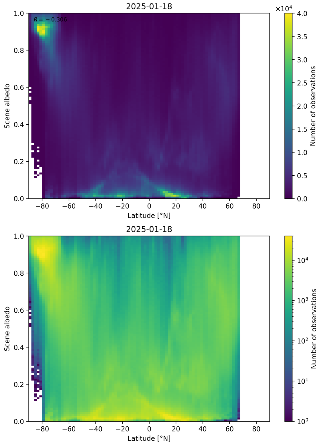
Figure 95: Scatter density plot of “Latitude” against “Scene albedo” for 2025-01-17 to 2025-01-19.
