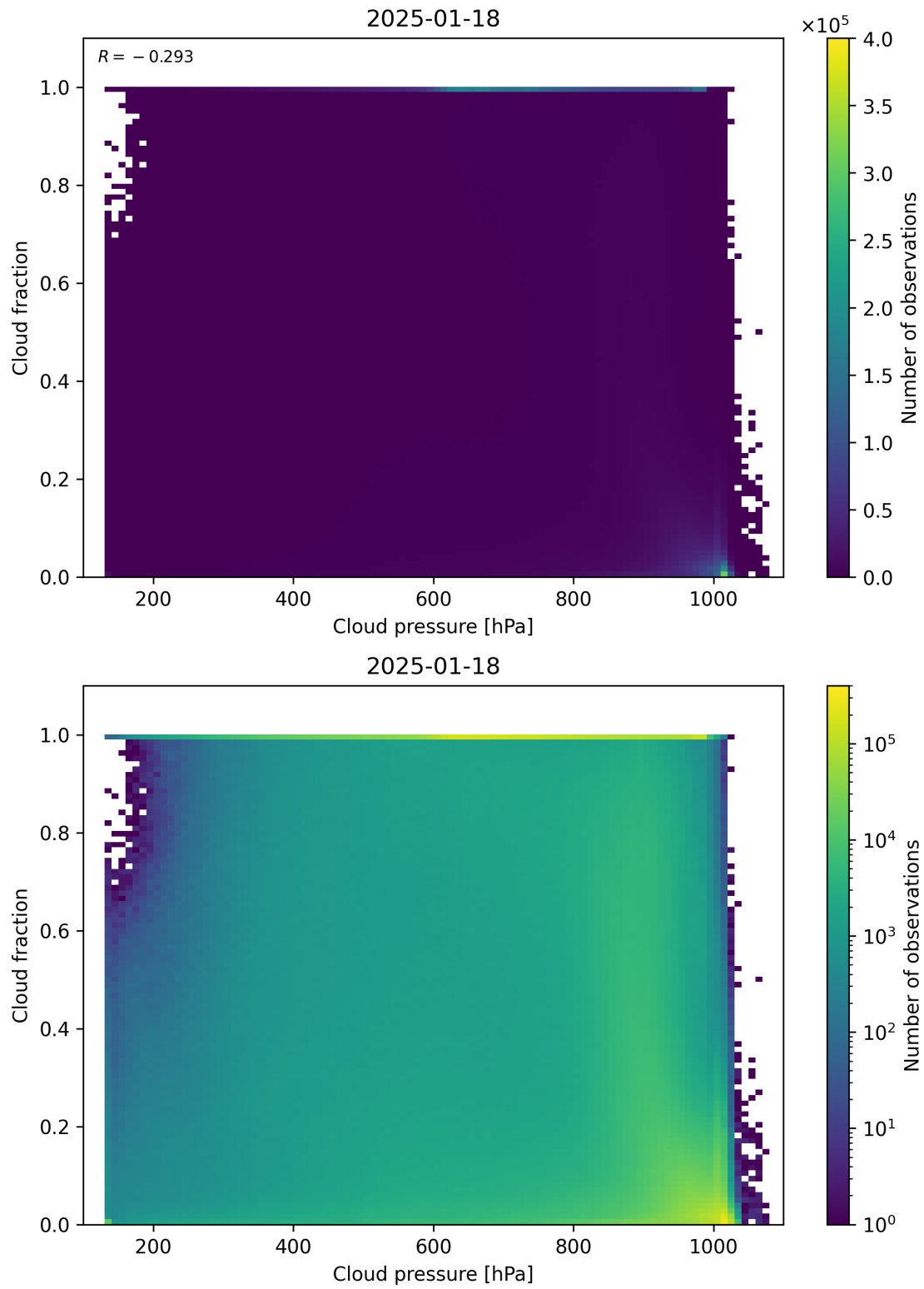
Figure 79: Scatter density plot of “Cloud pressure” against “Cloud fraction” for 2025-01-17 to 2025-01-19.
