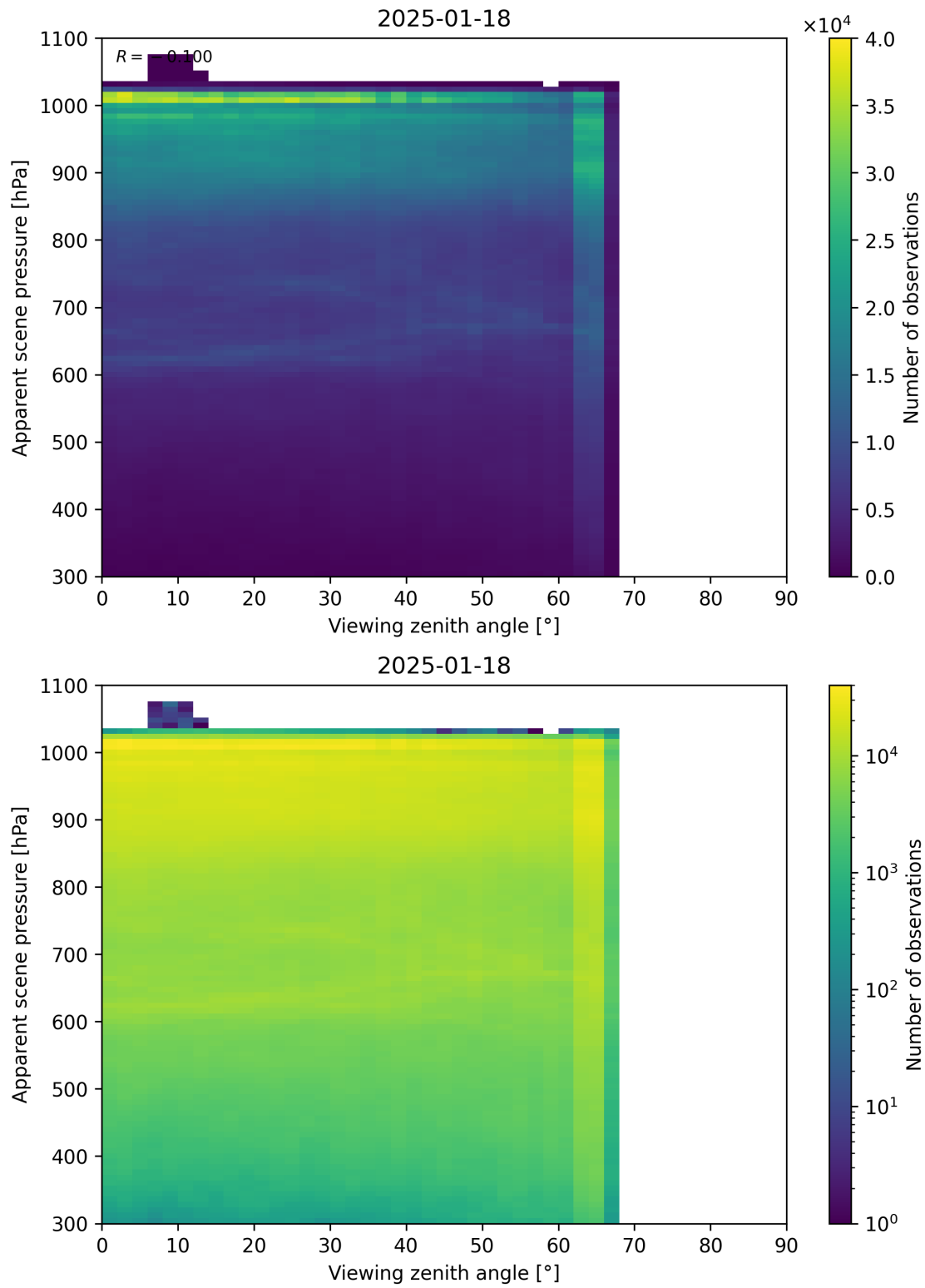
Figure 118: Scatter density plot of “Viewing zenith angle” against “Apparent scene pressure” for 2025-01-17 to 2025-01-19.
