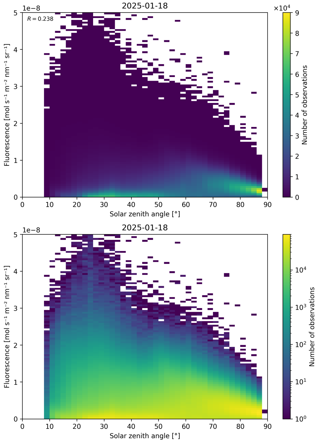
Figure 112: Scatter density plot of “Solar zenith angle” against “Fluorescence” for 2025-01-17 to 2025-01-19.
