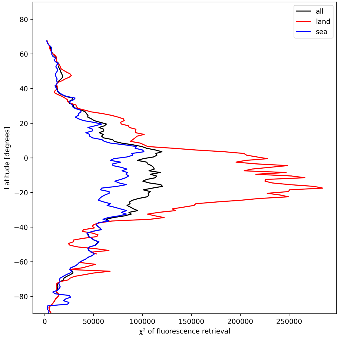
Figure 25: Zonal average of “ \chi^2 of fluorescence retrieval” for 2025-01-17 to 2025-01-19.
