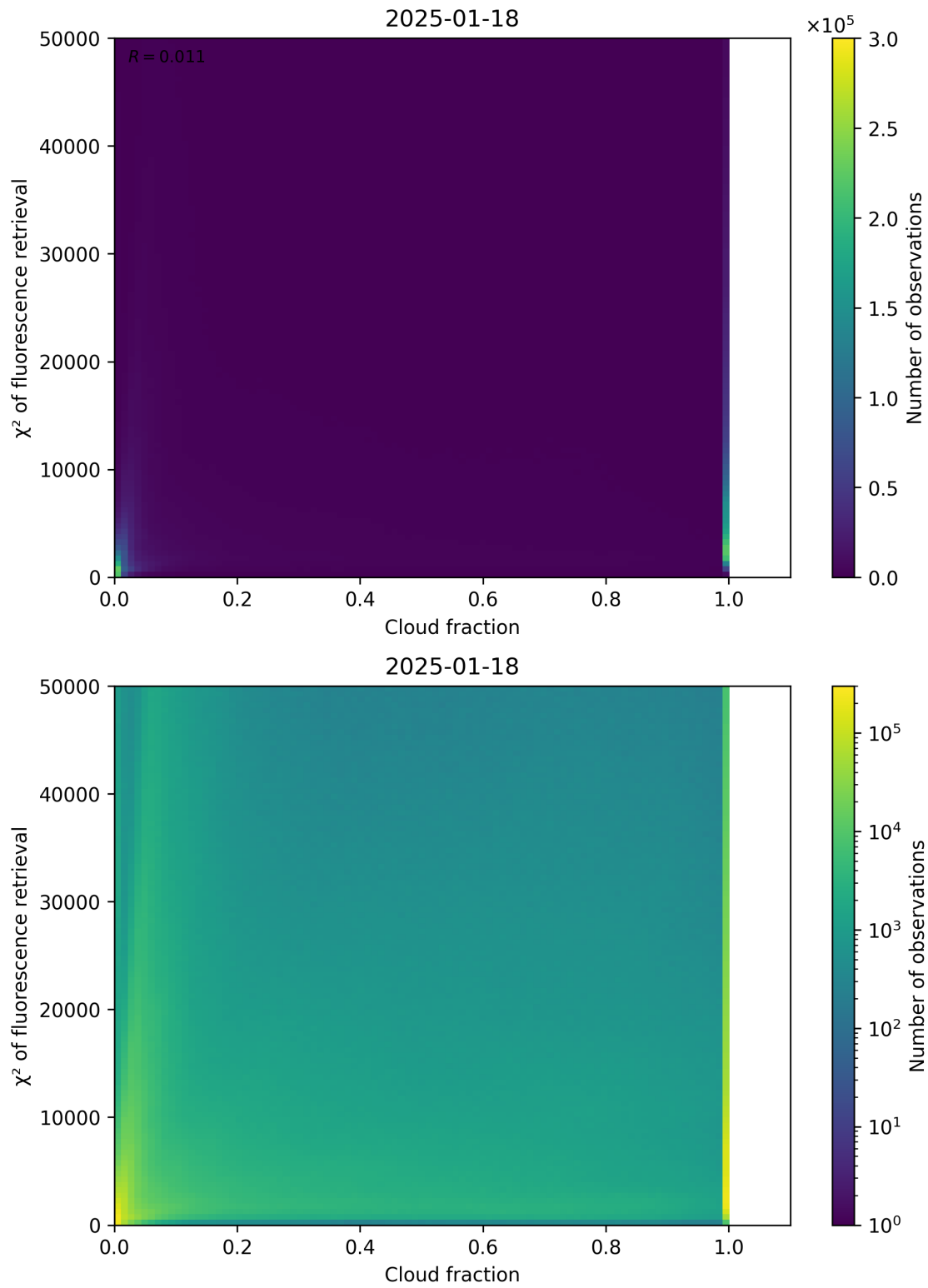
Figure 71: Scatter density plot of “Cloud fraction” against “ \chi^2 of fluorescence retrieval” for 2025-01-17 to 2025-01-19.
