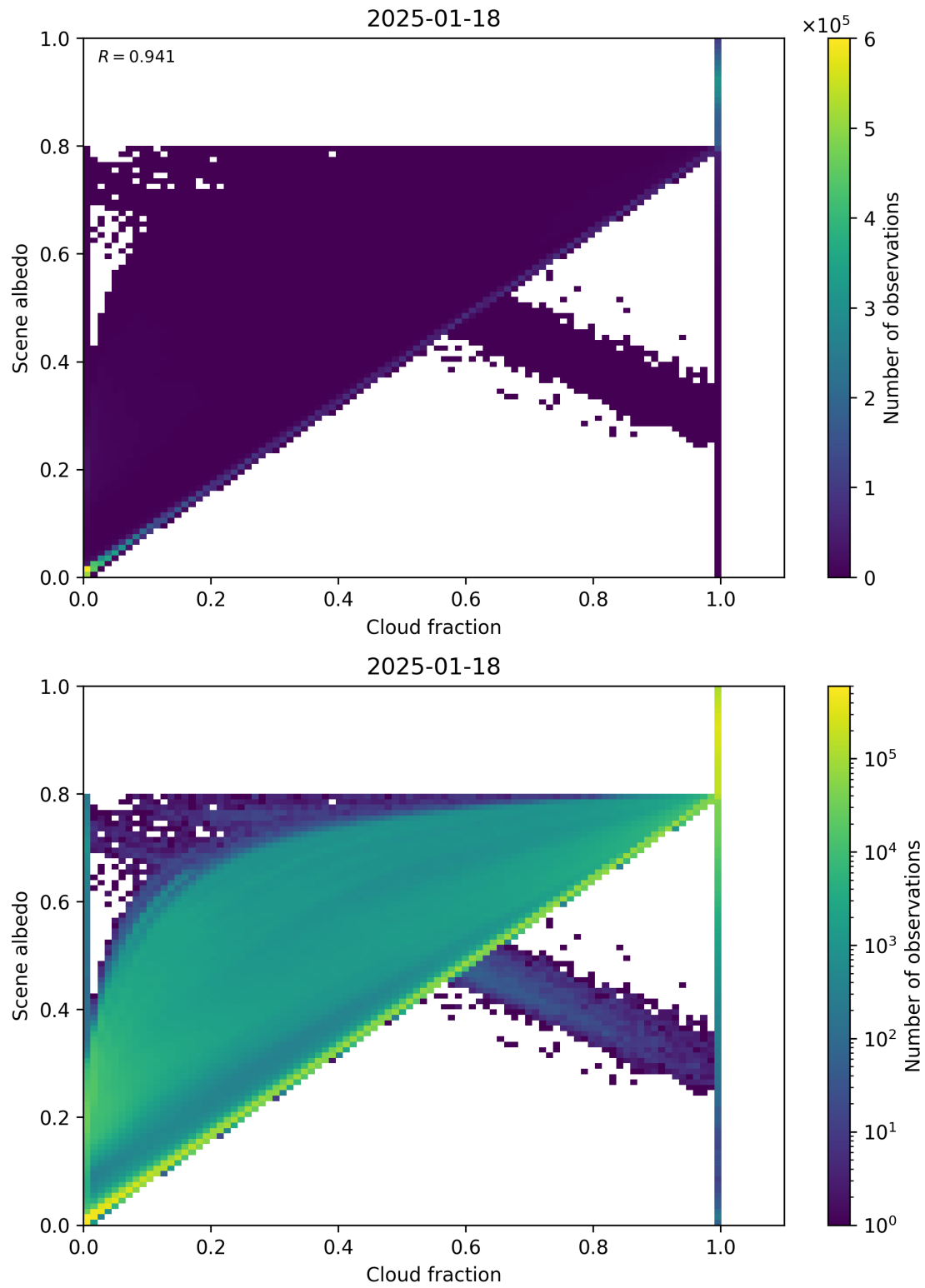
Figure 75: Scatter density plot of “Cloud fraction” against “Scene albedo” for 2025-01-17 to 2025-01-19.
