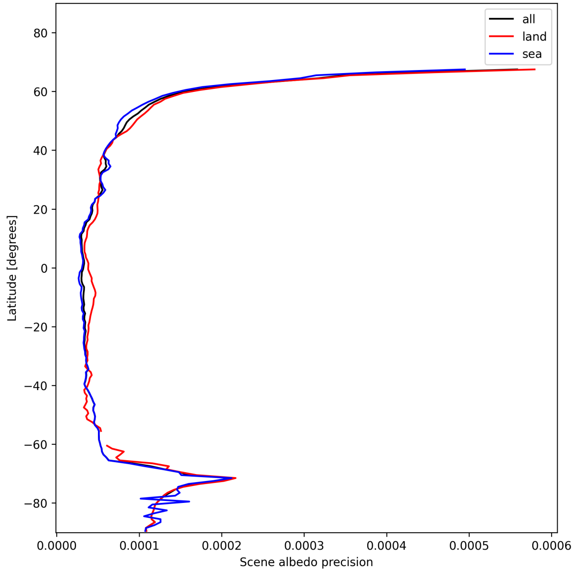
Figure 18: Zonal average of “Scene albedo precision” for 2025-01-17 to 2025-01-19.
