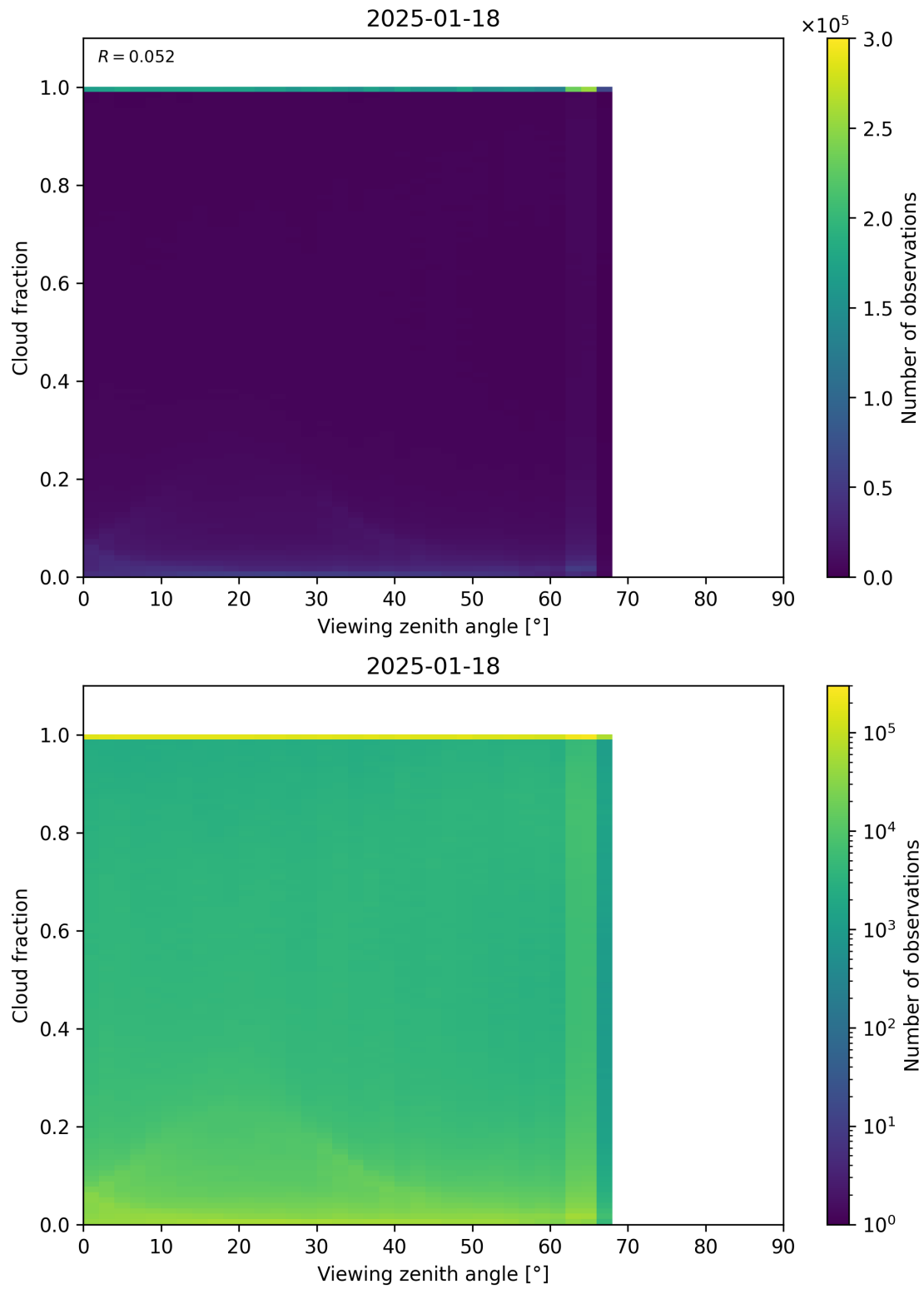
Figure 120: Scatter density plot of “Viewing zenith angle” against “Cloud fraction” for 2025-01-17 to 2025-01-19.
