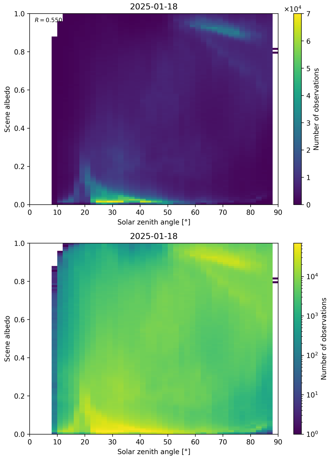
Figure 116: Scatter density plot of “Solar zenith angle” against “Scene albedo” for 2025-01-17 to 2025-01-19.
