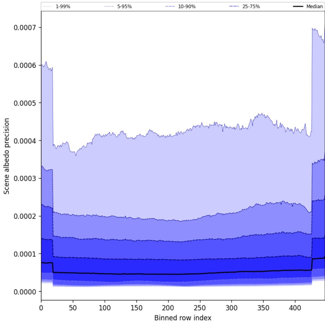
Figure 52: Along track statistics of “Scene albedo precision” for 2025-01-17 to 2025-01-19
