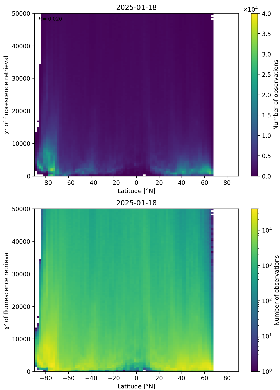
Figure 89: Scatter density plot of “Latitude” against “ \chi^2 of fluorescence retrieval” for 2025-01-17 to 2025-01-19.
