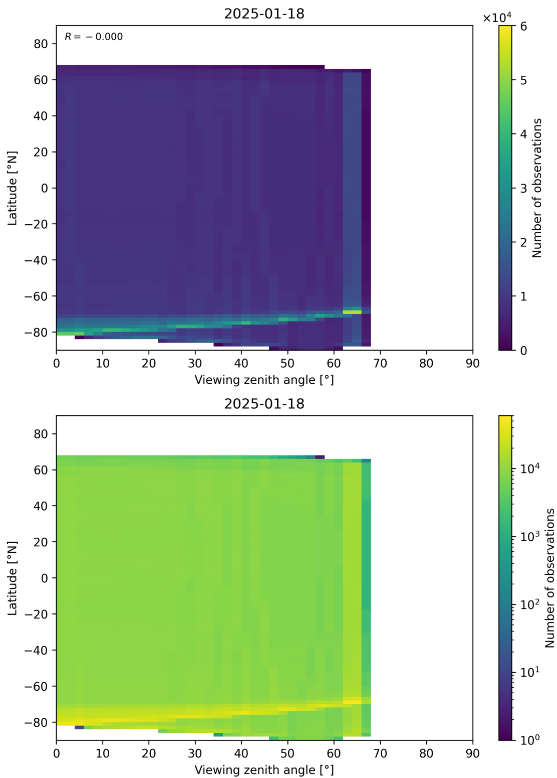
Figure 123: Scatter density plot of “Viewing zenith angle” against “Latitude” for 2025-01-17 to 2025-01-19.
