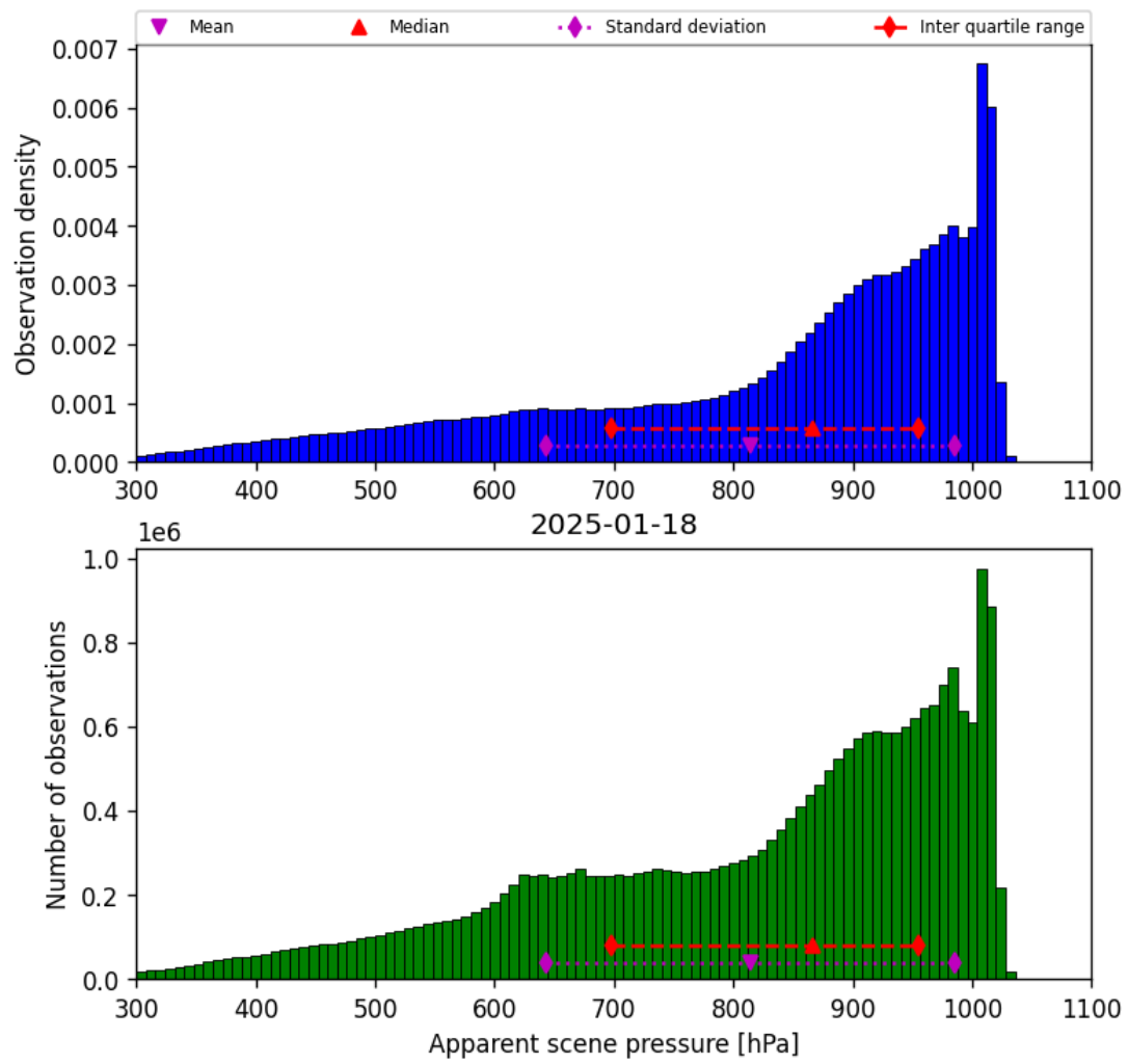
Figure 36: Histogram of “Apparent scene pressure” for 2025-01-17 to 2025-01-19
