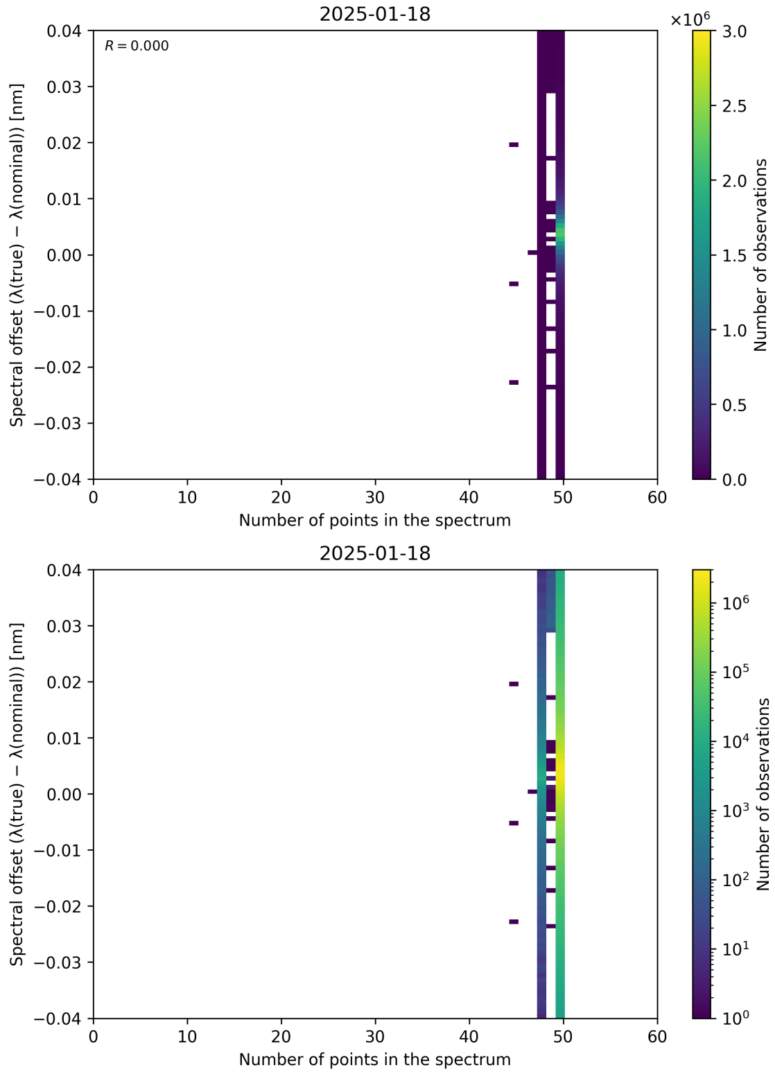
Figure 101: Scatter density plot of “Number of points in the spectrum” against “Spectral offset ( \lambda_{\text{true}} - \lambda_{\text{nominal}} )” for 2025-01-17 to 2025-01-19.
