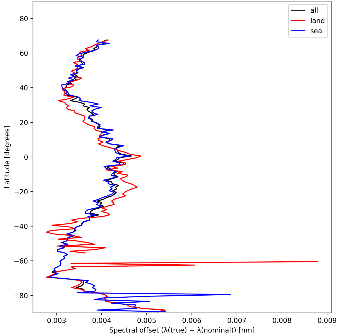
Figure 28: Zonal average of “Spectral offset ( \lambda_{\text{true}} - \lambda_{\text{nominal}} )” for 2025-01-17 to 2025-01-19.
