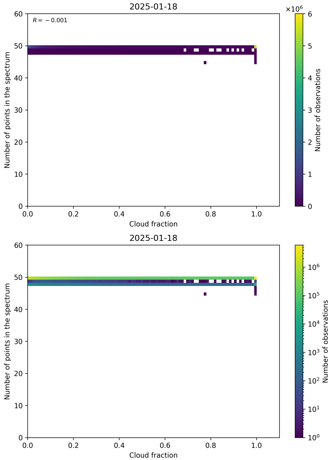
Figure 74: Scatter density plot of “Cloud fraction” against “Number of points in the spectrum” for 2025-01-17 to 2025-01-19.
