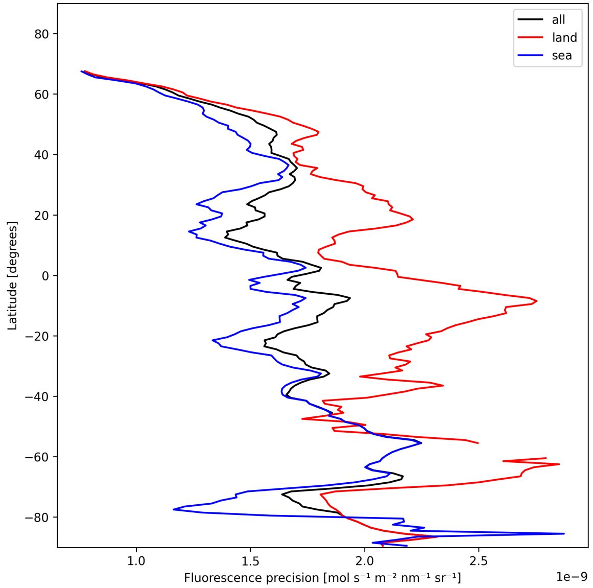
Figure 24: Zonal average of “Fluorescence precision” for 2025-01-17 to 2025-01-19.
