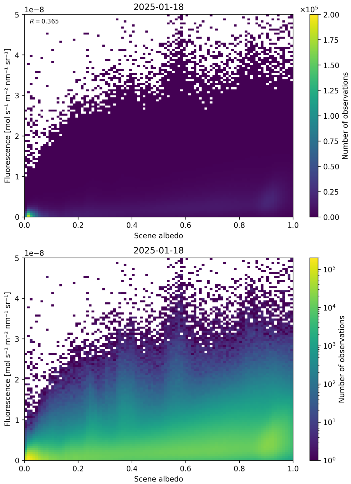
Figure 104: Scatter density plot of “Scene albedo” against “Fluorescence” for 2025-01-17 to 2025-01-19.
