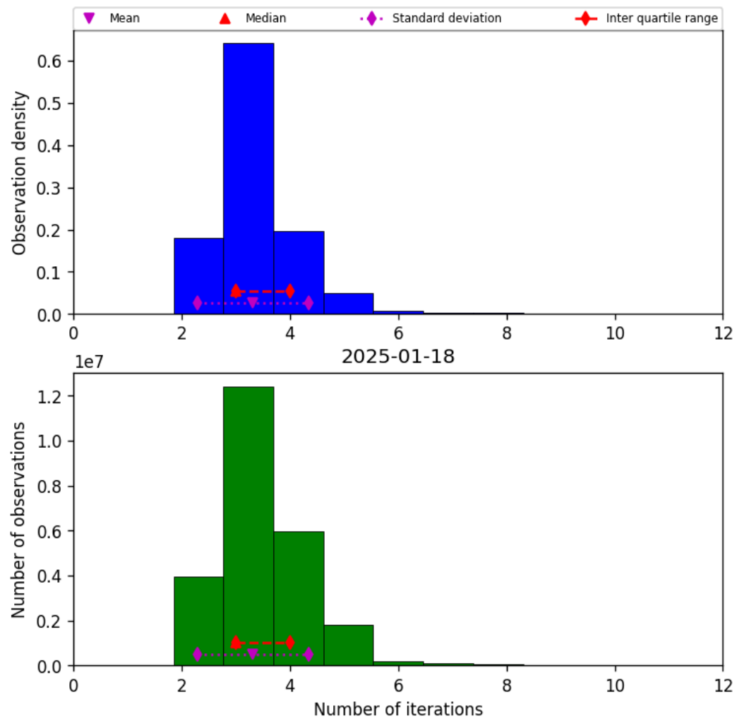
Figure 39: Histogram of “Number of iterations” for 2025-01-17 to 2025-01-19
