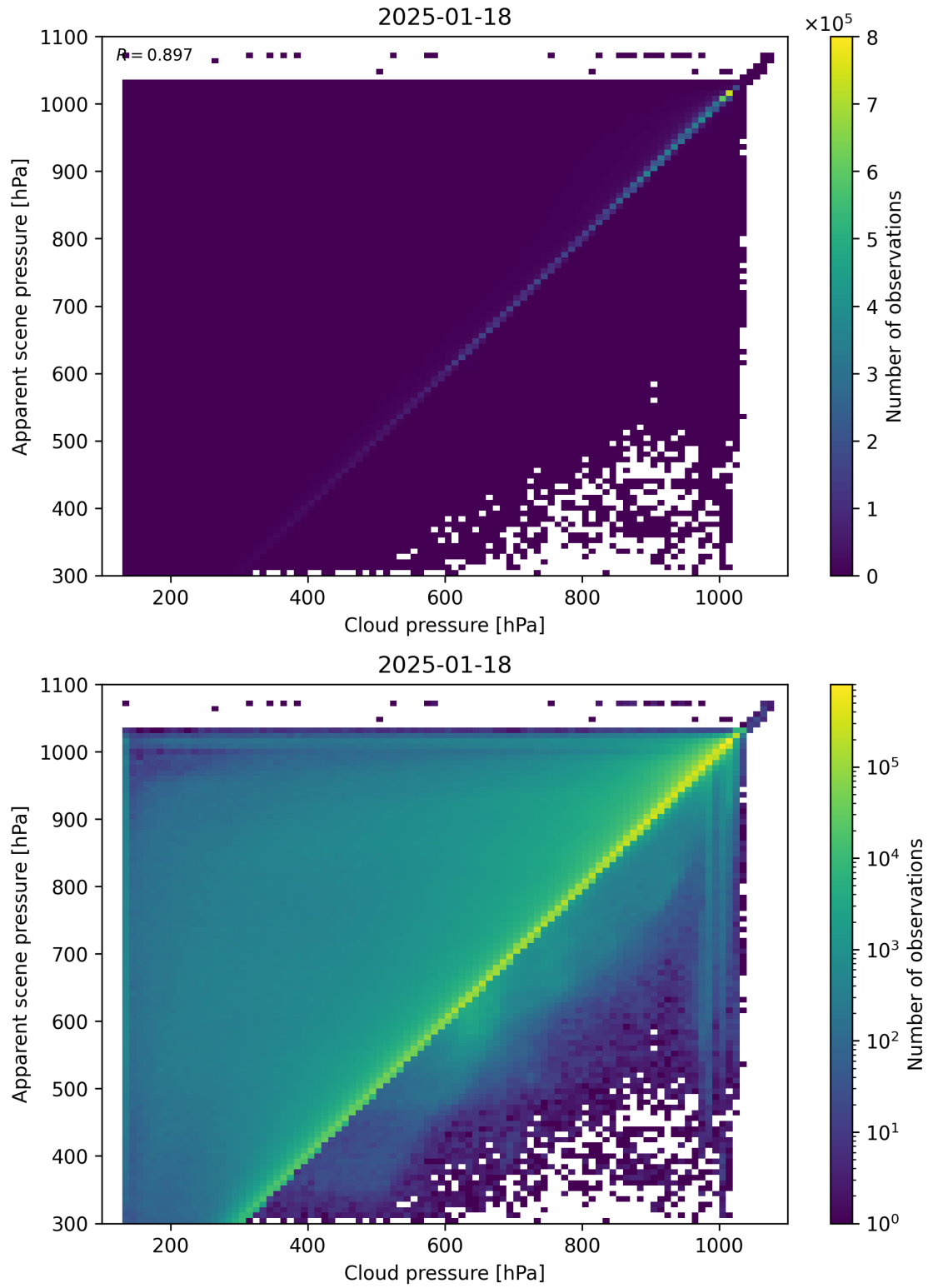
Figure 77: Scatter density plot of “Cloud pressure” against “Apparent scene pressure” for 2025-01-17 to 2025-01-19.
