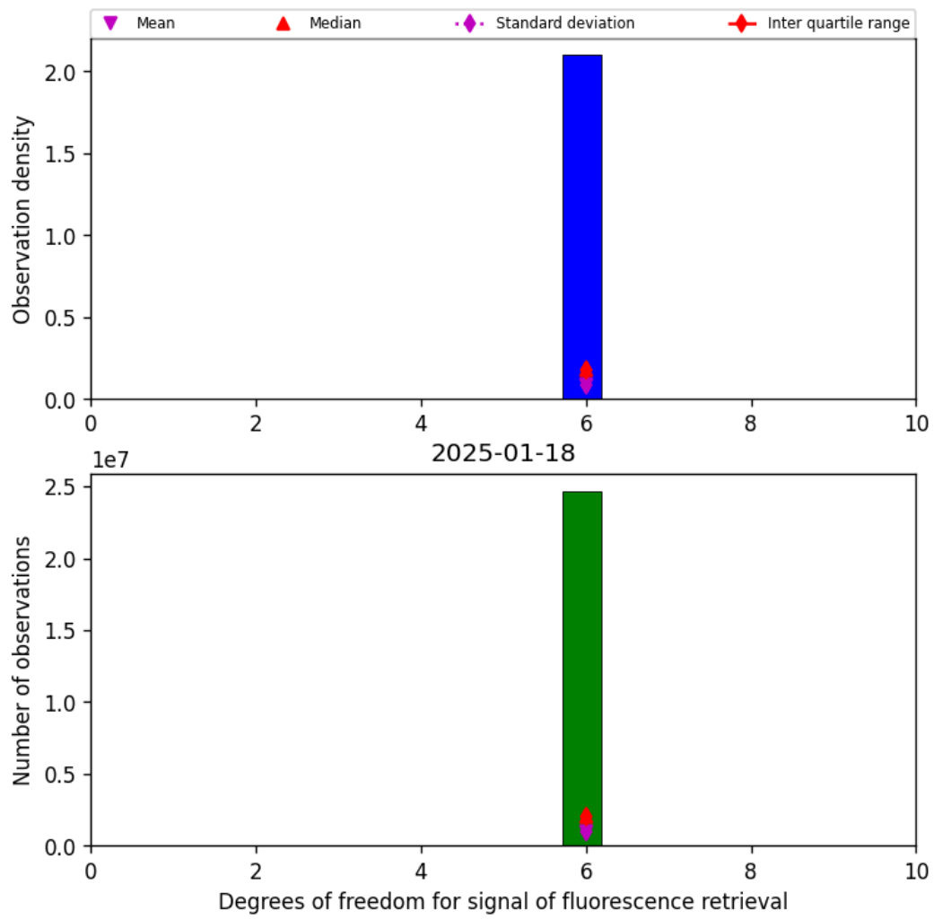
Figure 43: Histogram of “Degrees of freedom for signal of fluorescence retrieval” for 2025-01-17 to 2025-01-19
