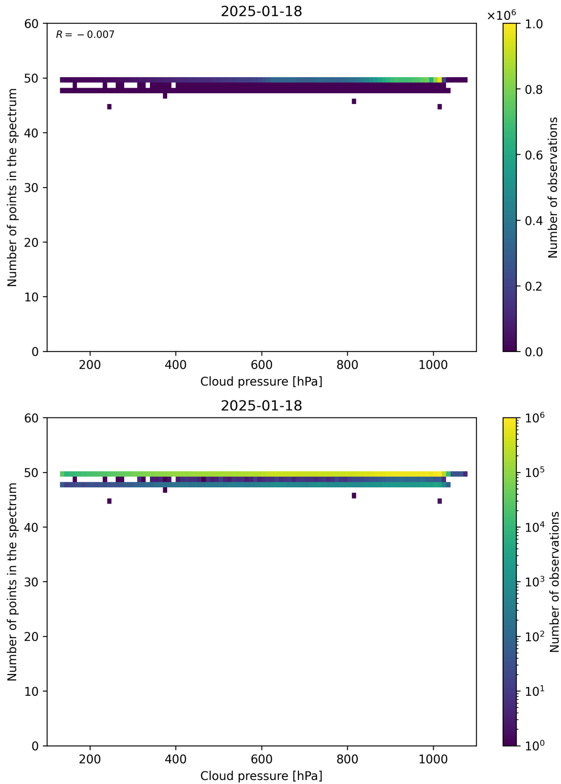
Figure 82: Scatter density plot of “Cloud pressure” against “Number of points in the spectrum” for 2025-01-17 to 2025-01-19.
