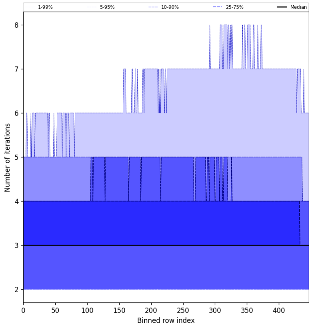
Figure 56: Along track statistics of “Number of iterations” for 2025-01-17 to 2025-01-19
