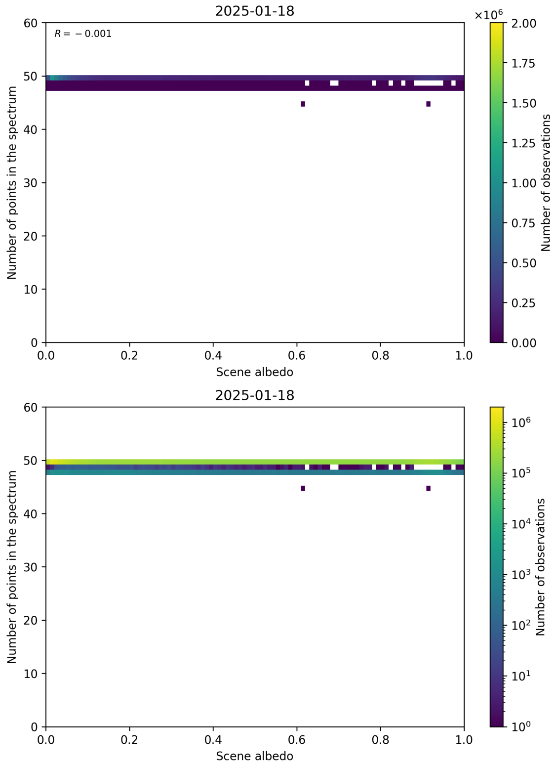
Figure 106: Scatter density plot of “Scene albedo” against “Number of points in the spectrum” for 2025-01-17 to 2025-01-19.
