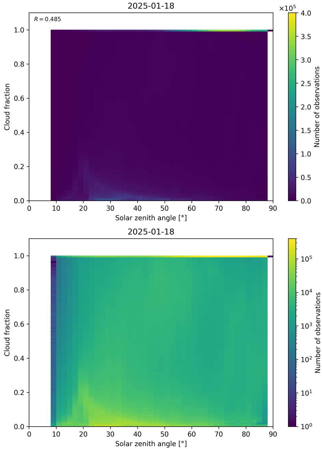
Figure 110: Scatter density plot of “Solar zenith angle” against “Cloud fraction” for 2025-01-17 to 2025-01-19.
