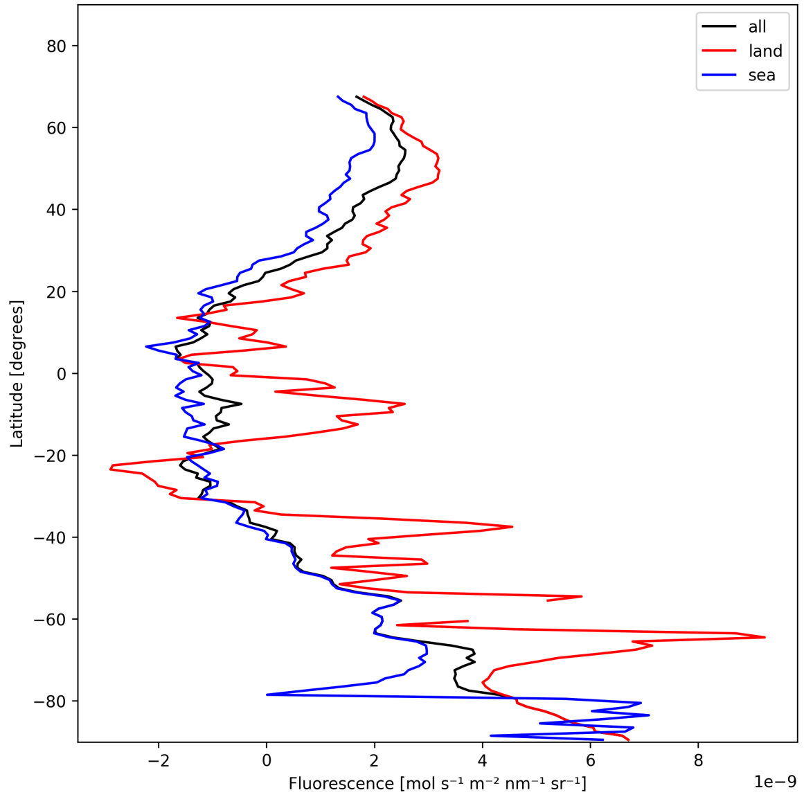
Figure 23: Zonal average of “Fluorescence” for 2025-01-17 to 2025-01-19.
