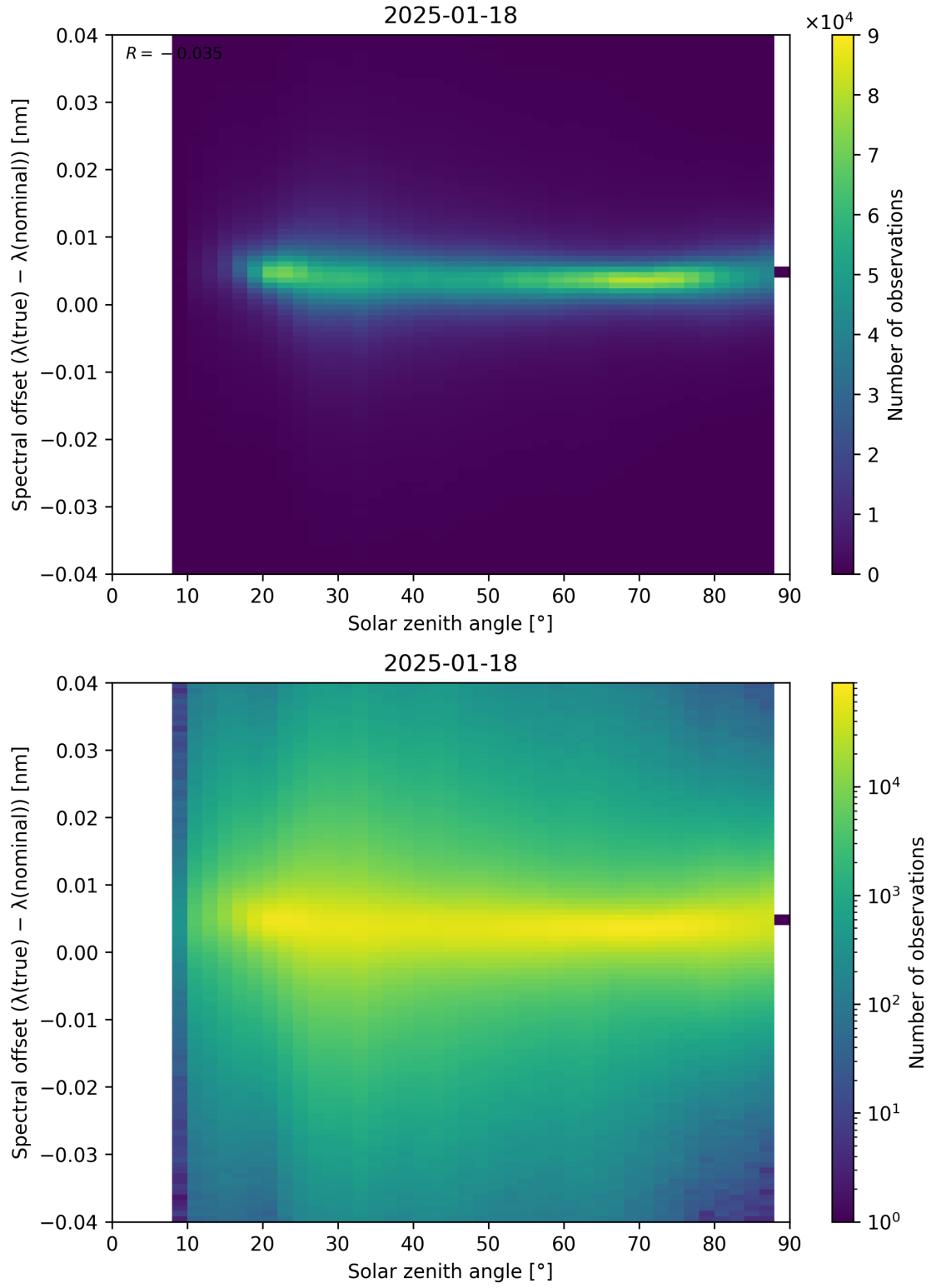
Figure 117: Scatter density plot of “Solar zenith angle” against “Spectral offset ( \lambda_{\text{true}} - \lambda_{\text{nominal}} )” for 2025-01-17 to 2025-01-19.
