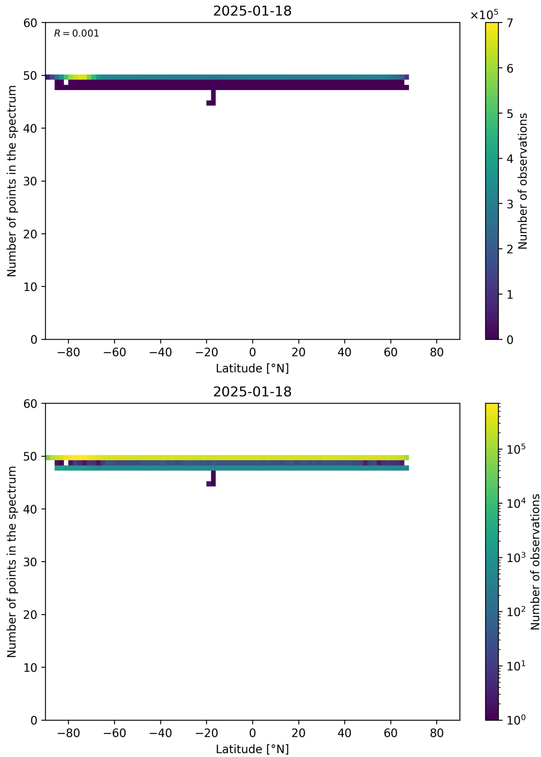
Figure 94: Scatter density plot of “Latitude” against “Number of points in the spectrum” for 2025-01-17 to 2025-01-19.
