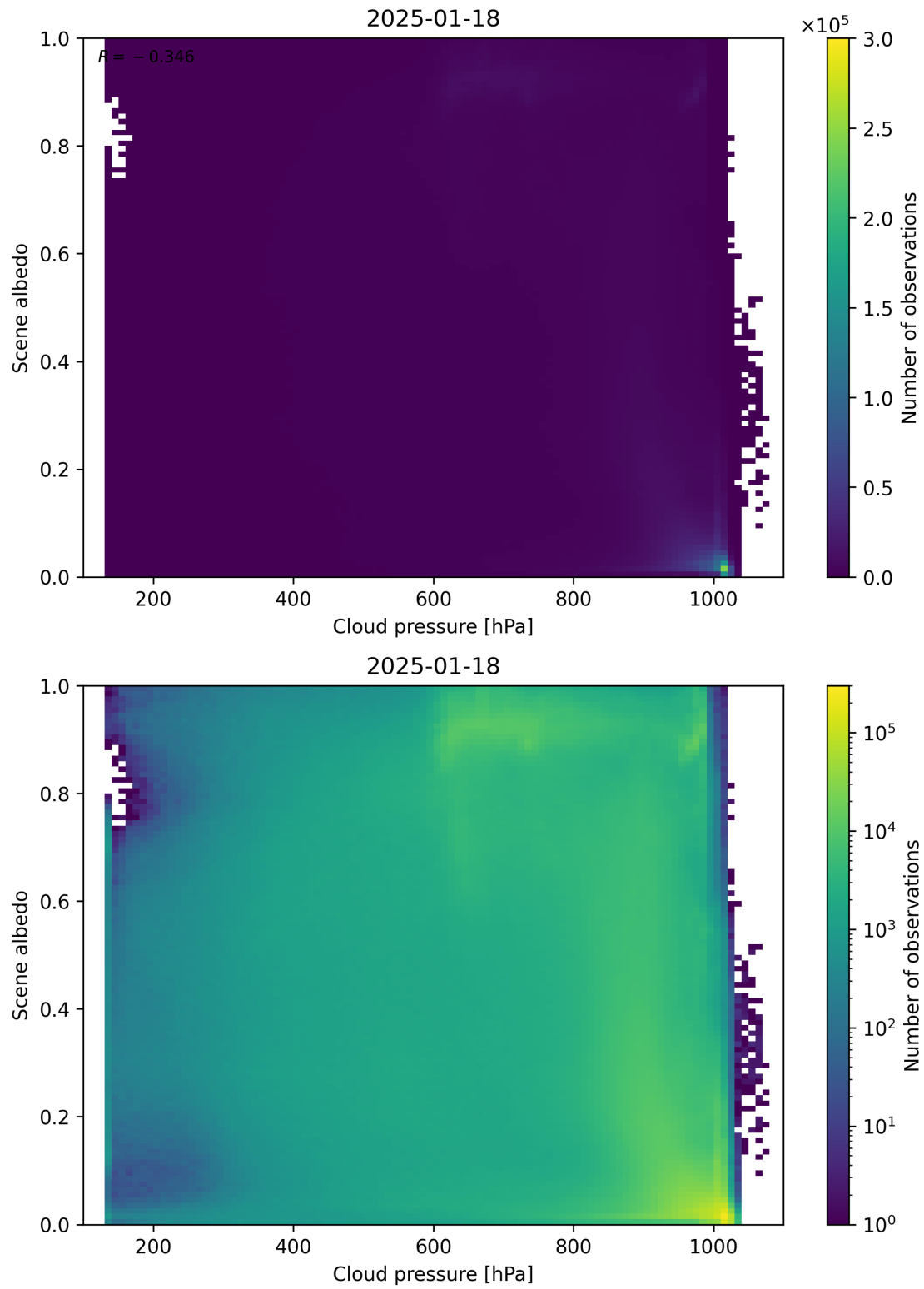
Figure 83: Scatter density plot of “Cloud pressure” against “Scene albedo” for 2025-01-17 to 2025-01-19.
