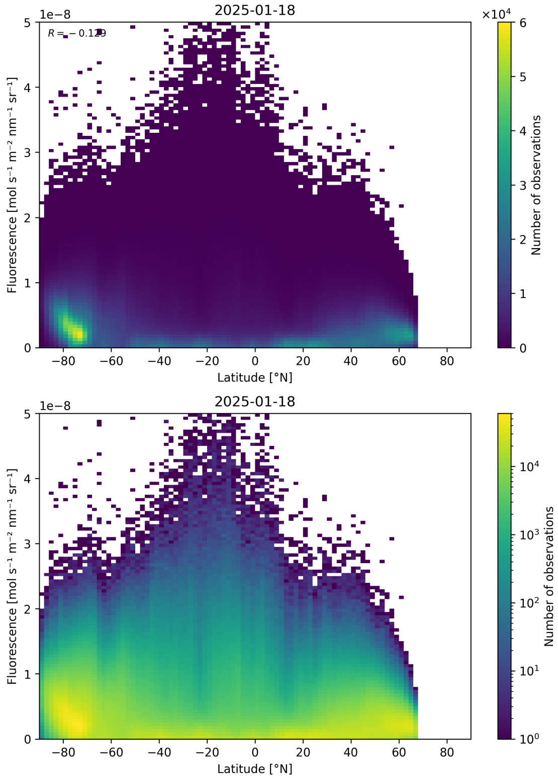
Figure 92: Scatter density plot of “Latitude” against “Fluorescence” for 2025-01-17 to 2025-01-19.
