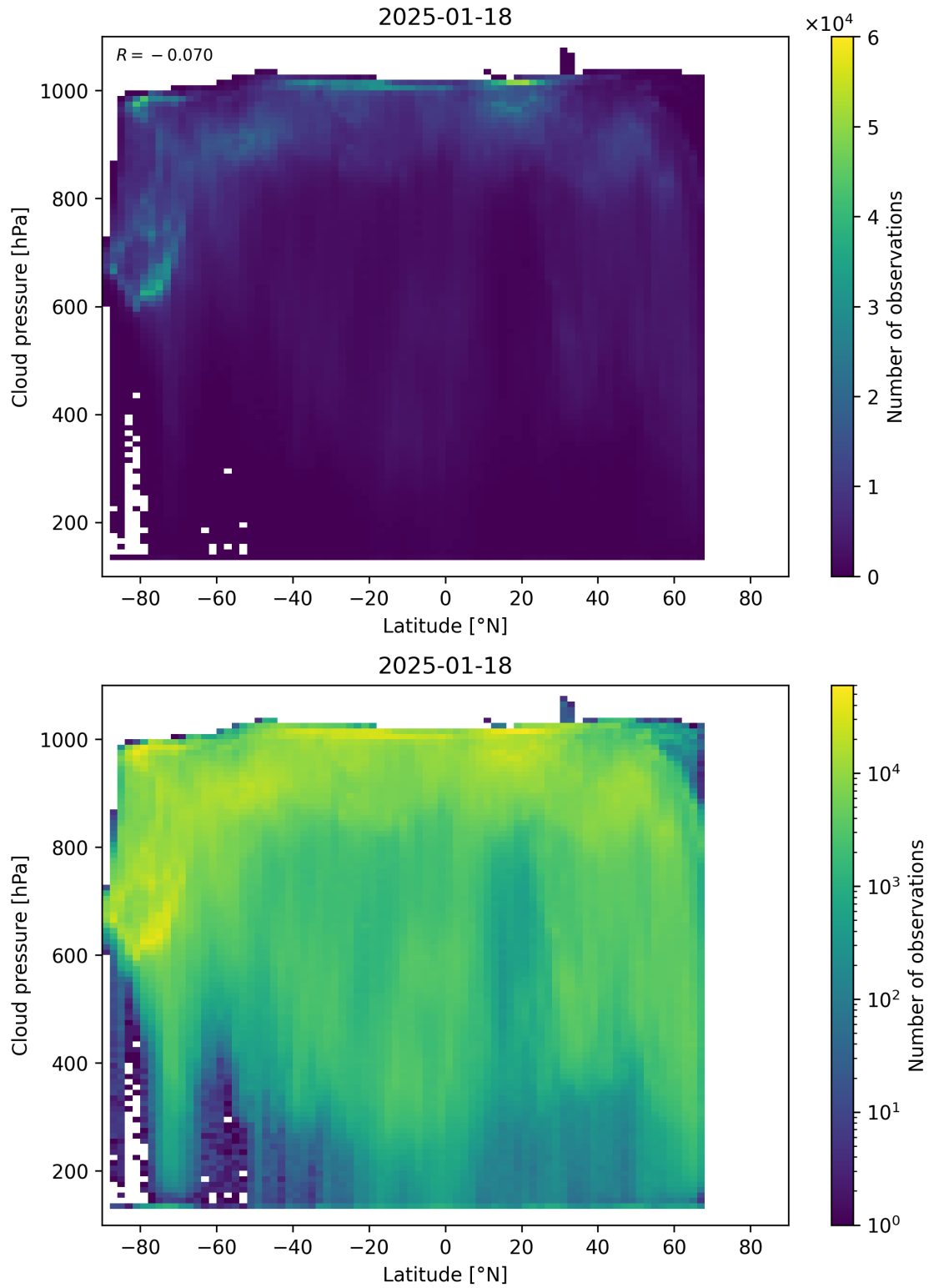
Figure 91: Scatter density plot of “Latitude” against “Cloud pressure” for 2025-01-17 to 2025-01-19.
