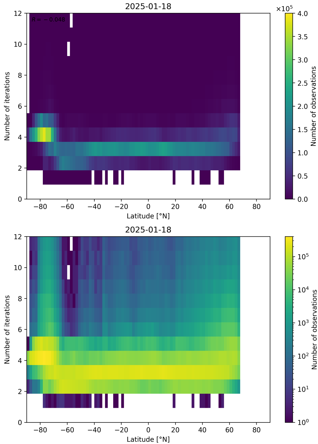
Figure 93: Scatter density plot of “Latitude” against “Number of iterations” for 2025-01-17 to 2025-01-19.
