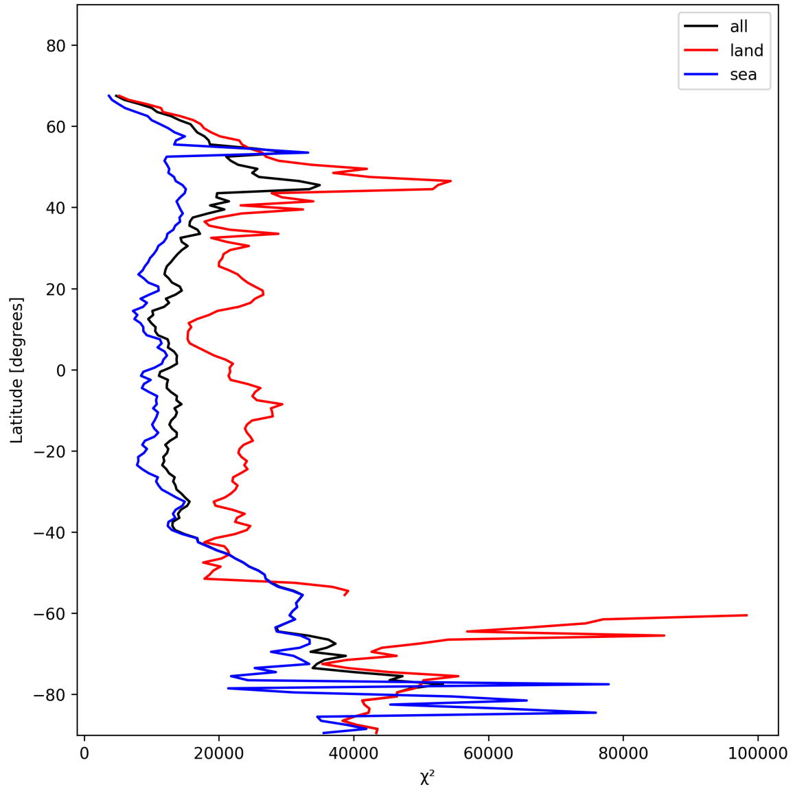
Figure 21: Zonal average of “ \chi^2 ” for 2025-01-17 to 2025-01-19.
