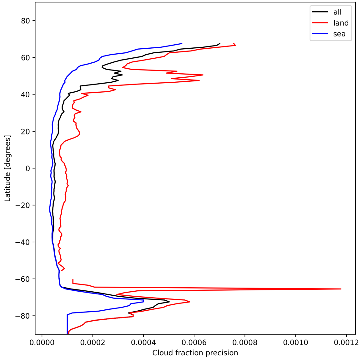
Figure 16: Zonal average of “Cloud fraction precision” for 2025-01-17 to 2025-01-19.
