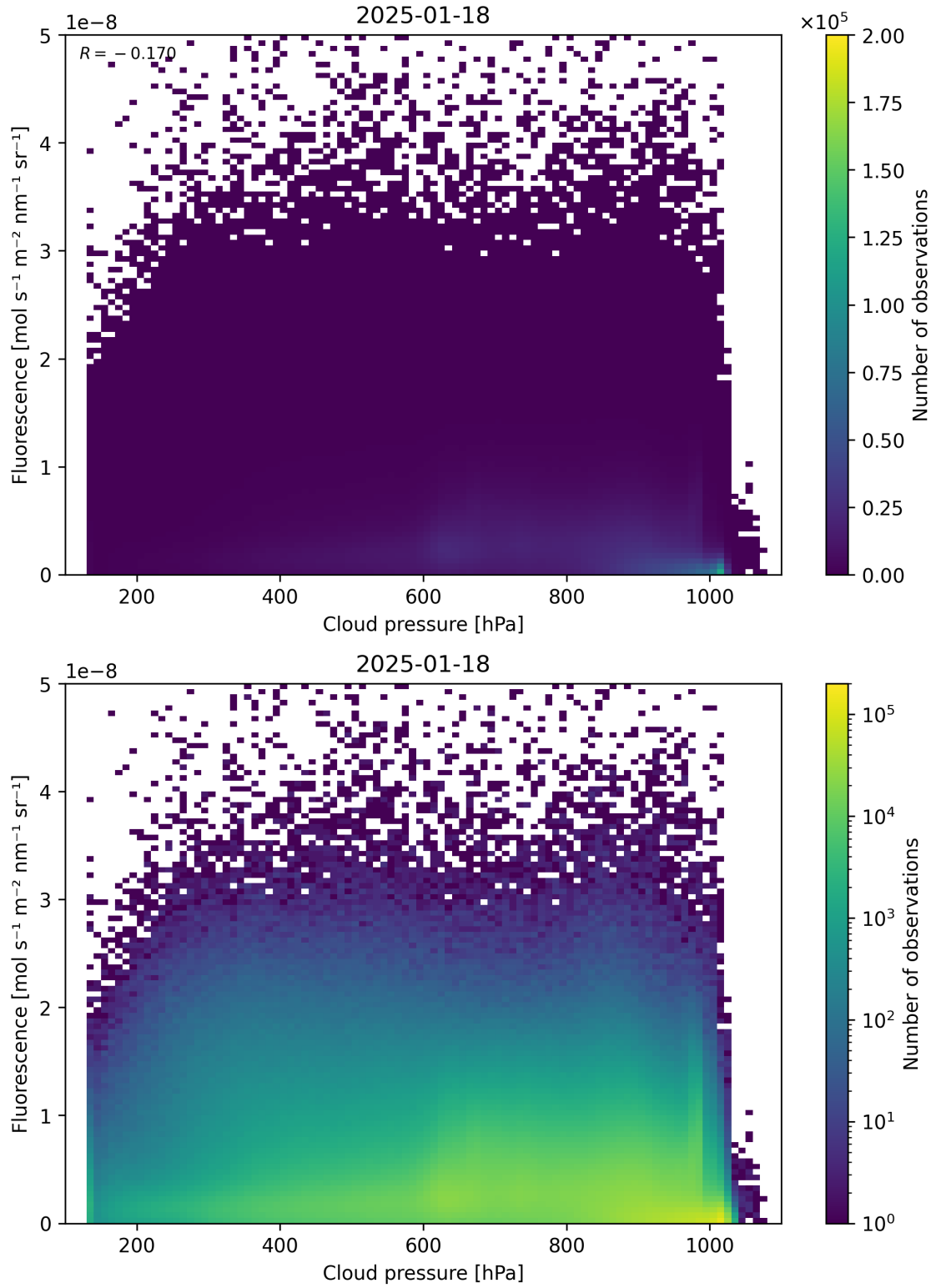
Figure 80: Scatter density plot of “Cloud pressure” against “Fluorescence” for 2025-01-17 to 2025-01-19.
