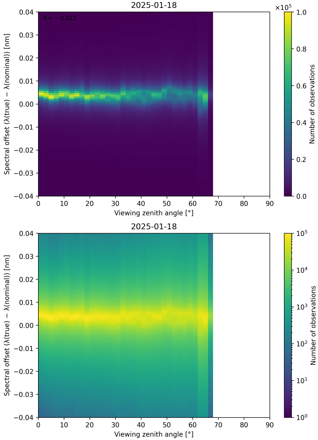
Figure 128: Scatter density plot of “Viewing zenith angle” against “Spectral offset ( \lambda_{\text{true}} - \lambda_{\text{nominal}} )” for 2025-01-17 to 2025-01-19.
