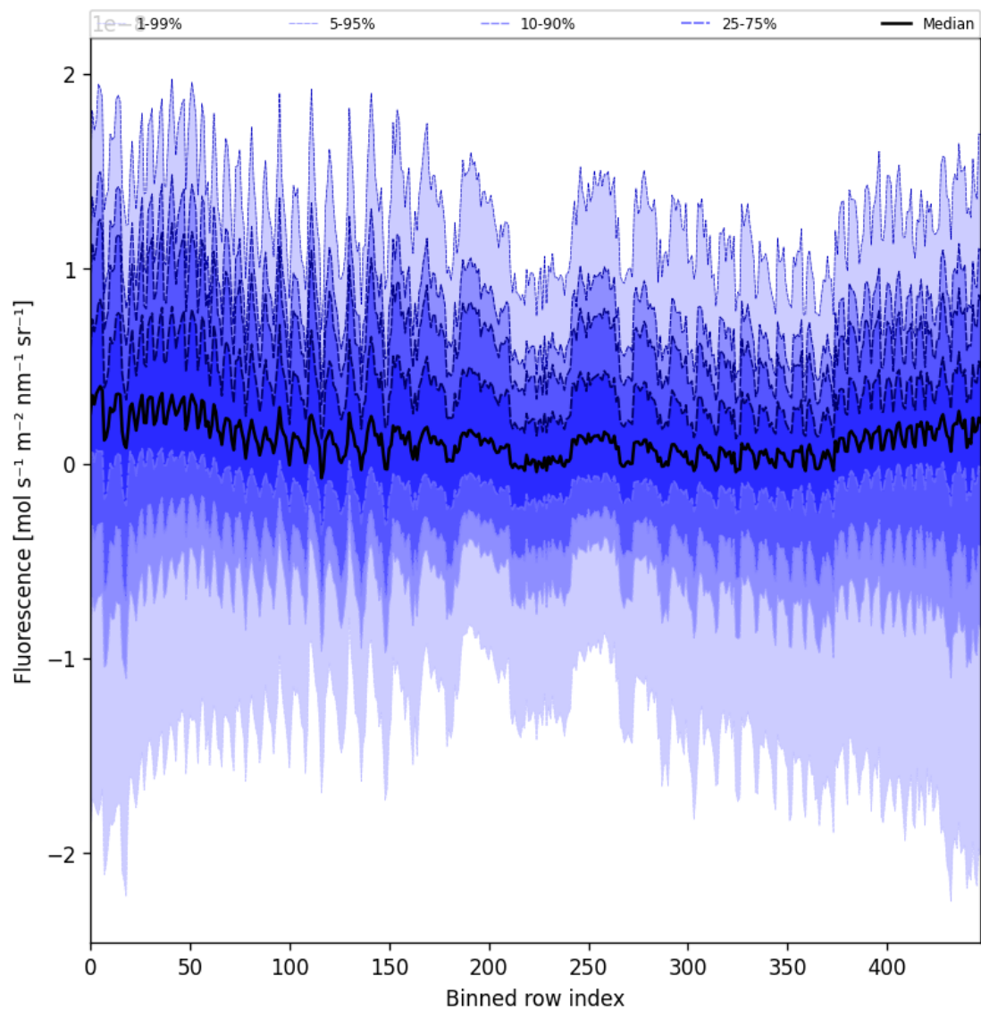
Figure 57: Along track statistics of “Fluorescence” for 2025-01-17 to 2025-01-19
