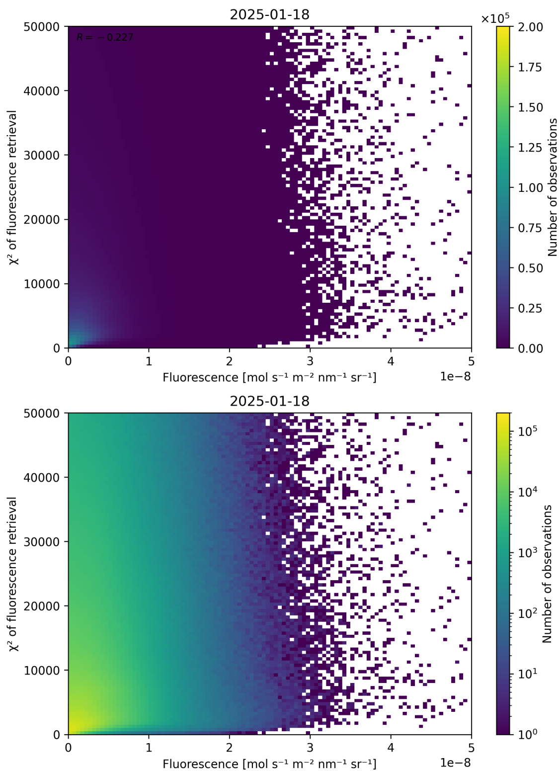
Figure 85: Scatter density plot of “Fluorescence” against “ \chi^2 of fluorescence retrieval” for 2025-01-17 to 2025-01-19.
