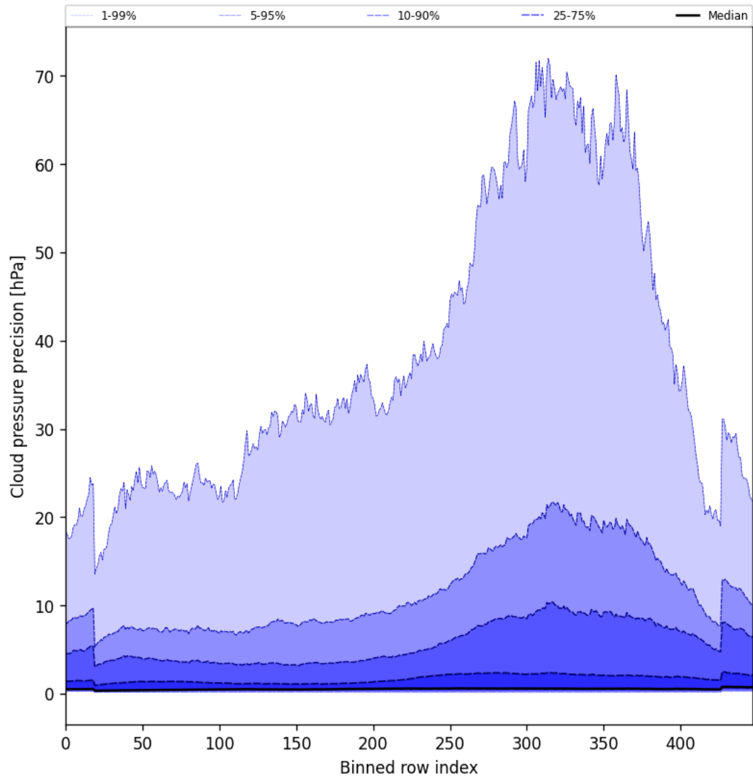
Figure 48: Along track statistics of “Cloud pressure precision” for 2025-01-17 to 2025-01-19
