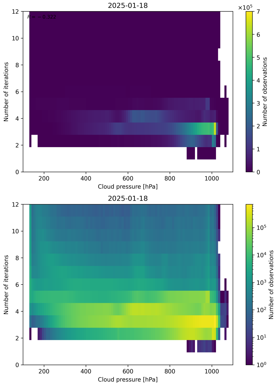
Figure 81: Scatter density plot of “Cloud pressure” against “Number of iterations” for 2025-01-17 to 2025-01-19.
