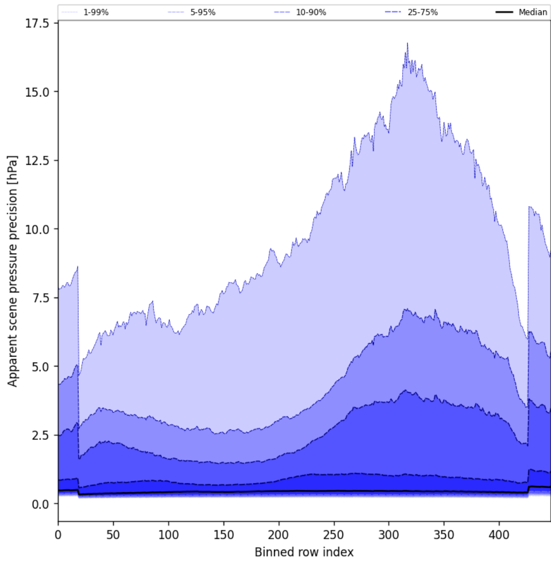
Figure 54: Along track statistics of “Apparent scene pressure precision” for 2025-01-17 to 2025-01-19
