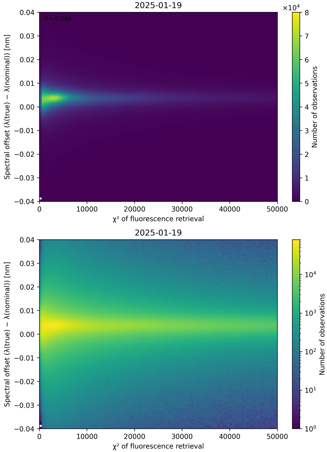
Figure 69: Scatter density plot of “ \chi^2 of fluorescence retrieval” against “Spectral offset ( \lambda_{\text{true}} - \lambda_{\text{nominal}} )” for 2025-01-18 to 2025-01-20.
