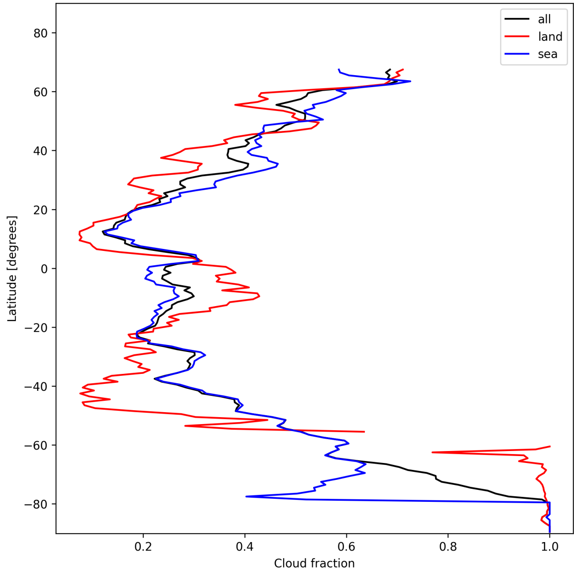
Figure 15: Zonal average of “Cloud fraction” for 2025-01-18 to 2025-01-20.
