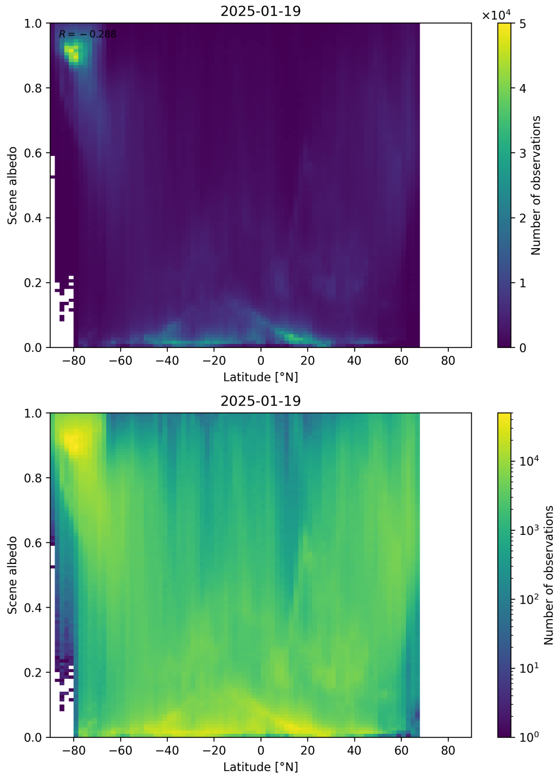
Figure 95: Scatter density plot of “Latitude” against “Scene albedo” for 2025-01-18 to 2025-01-20.
