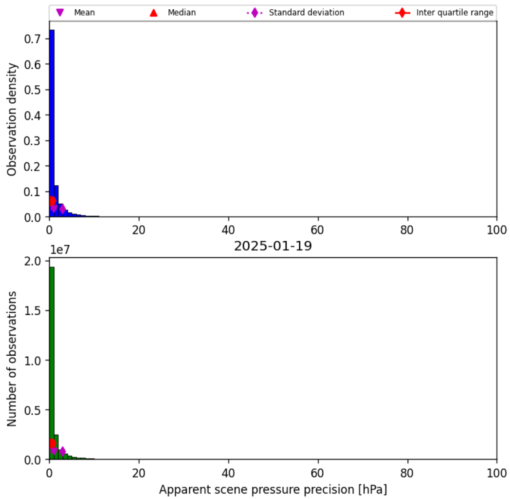
Figure 37: Histogram of “Apparent scene pressure precision” for 2025-01-18 to 2025-01-20
