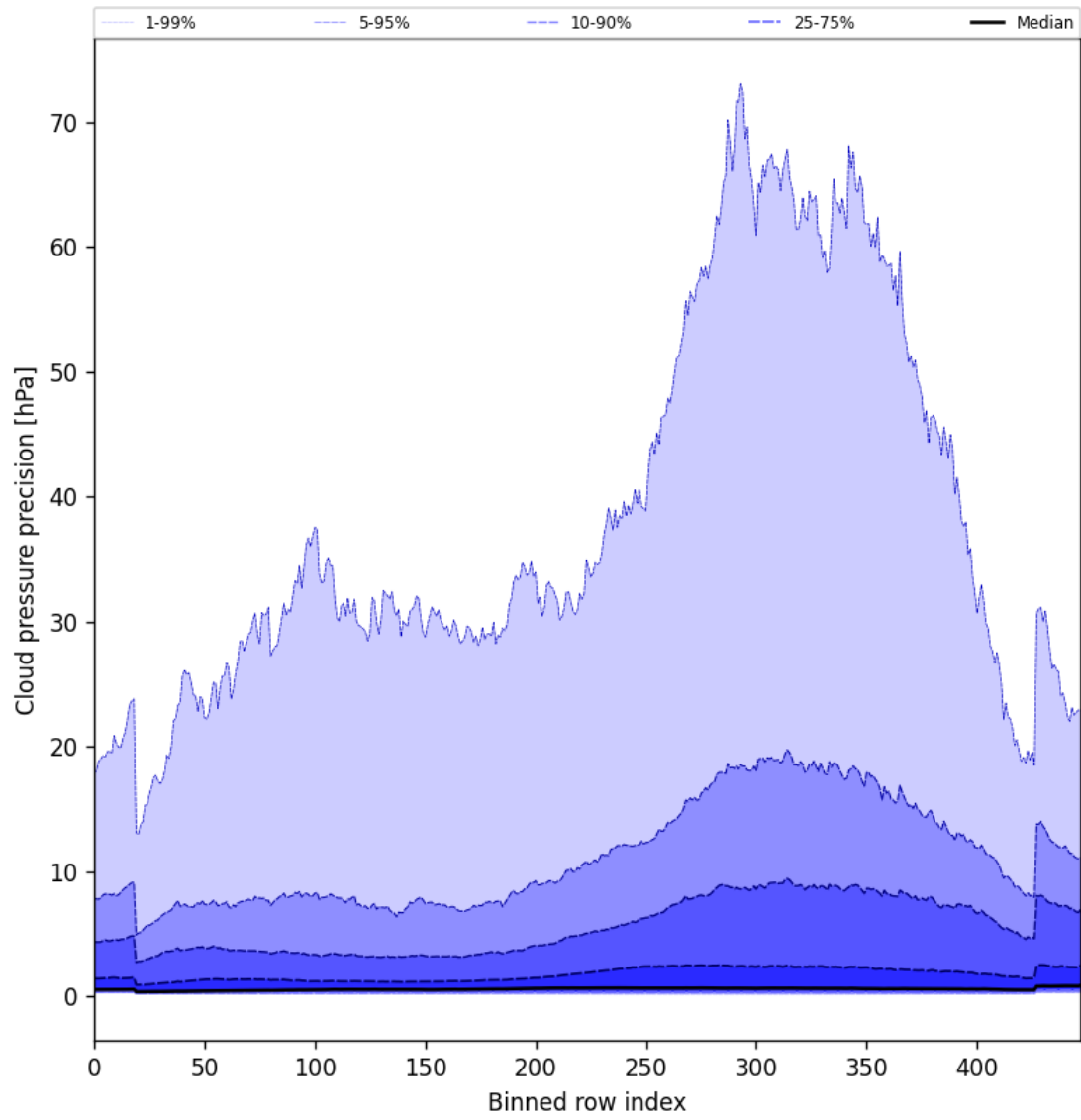
Figure 48: Along track statistics of “Cloud pressure precision” for 2025-01-18 to 2025-01-20
