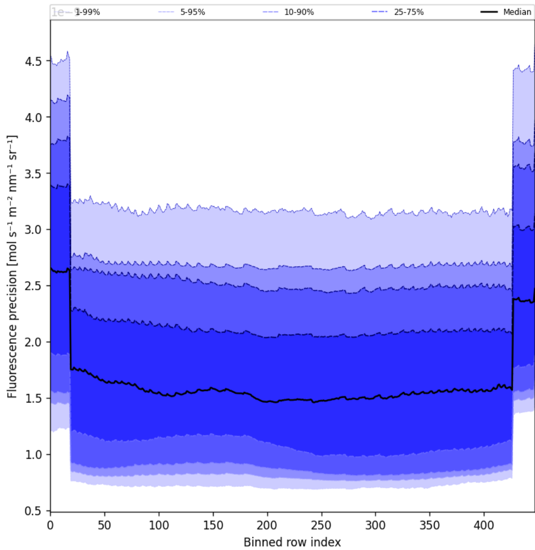
Figure 58: Along track statistics of “Fluorescence precision” for 2025-01-18 to 2025-01-20
