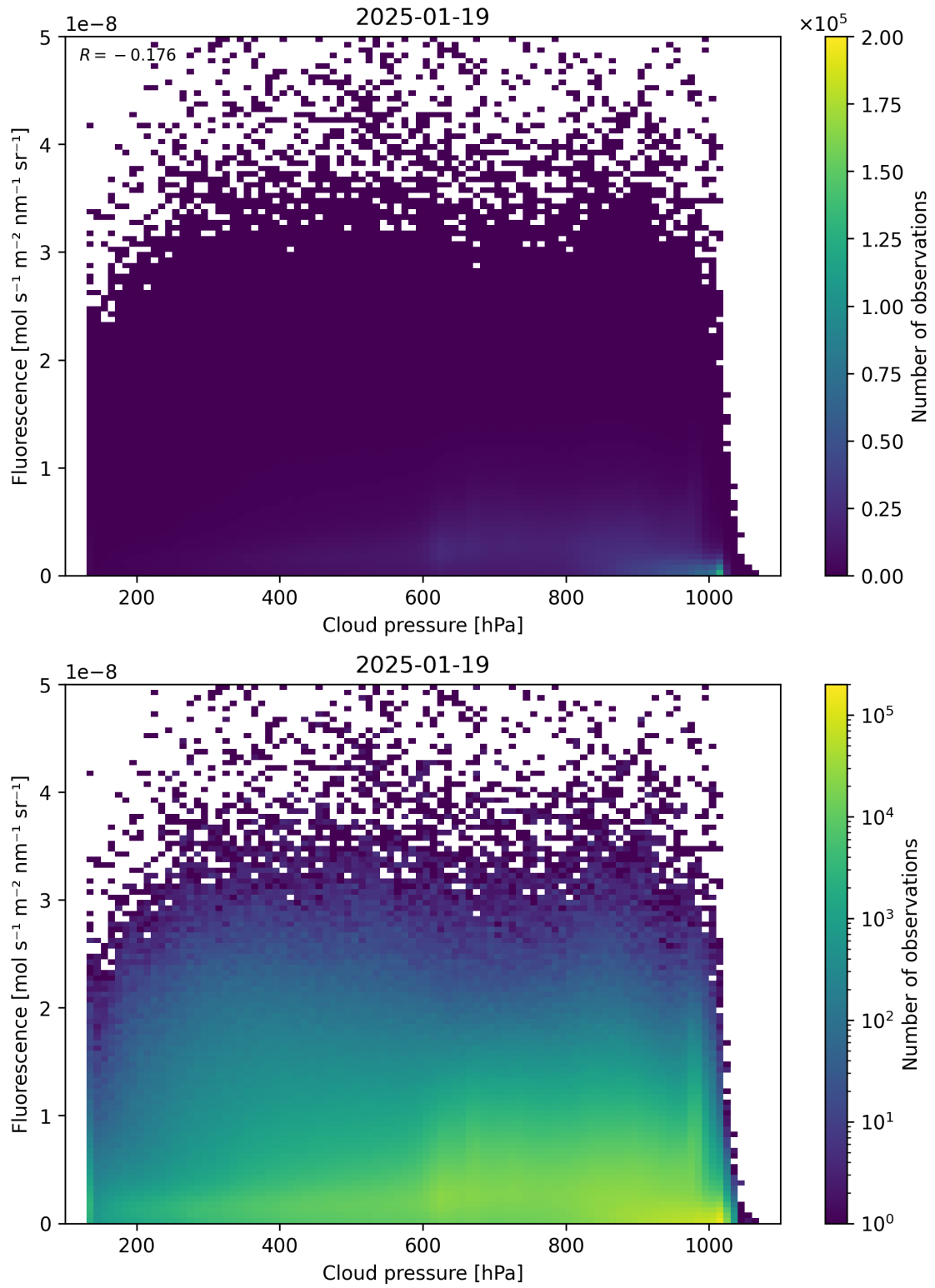
Figure 80: Scatter density plot of “Cloud pressure” against “Fluorescence” for 2025-01-18 to 2025-01-20.
