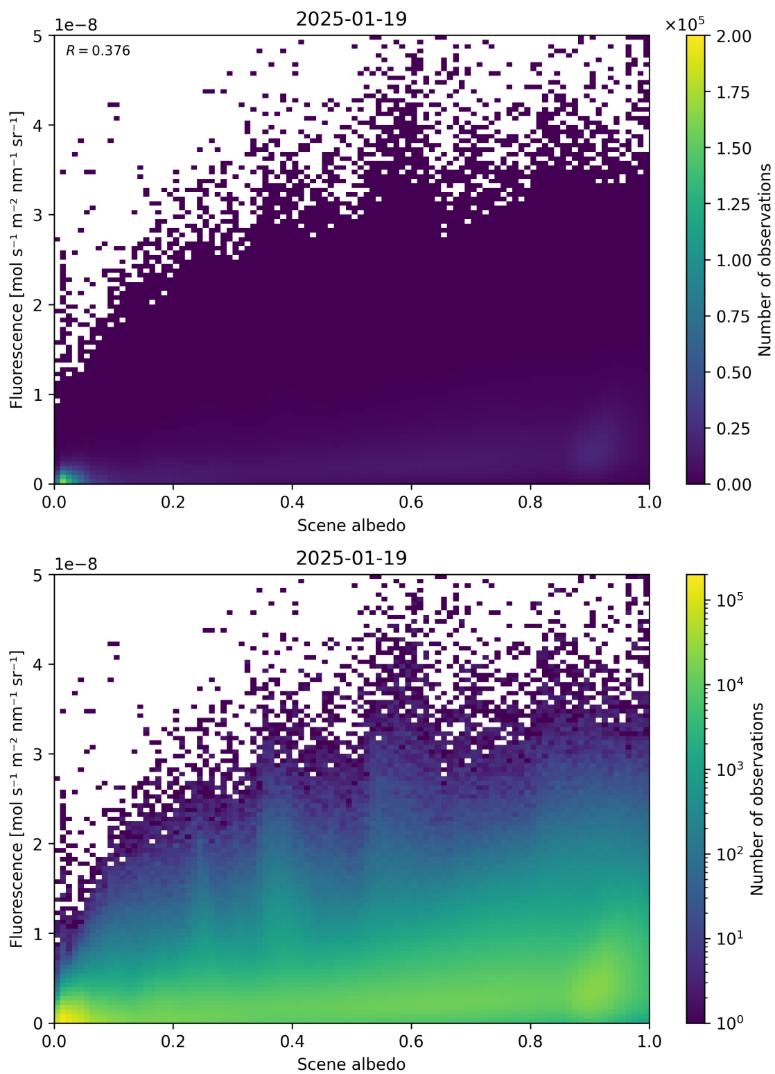
Figure 104: Scatter density plot of “Scene albedo” against “Fluorescence” for 2025-01-18 to 2025-01-20.
