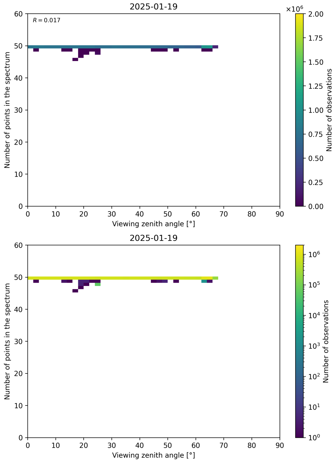
Figure 125: Scatter density plot of “Viewing zenith angle” against “Number of points in the spectrum” for 2025-01-18 to 2025-01-20.
