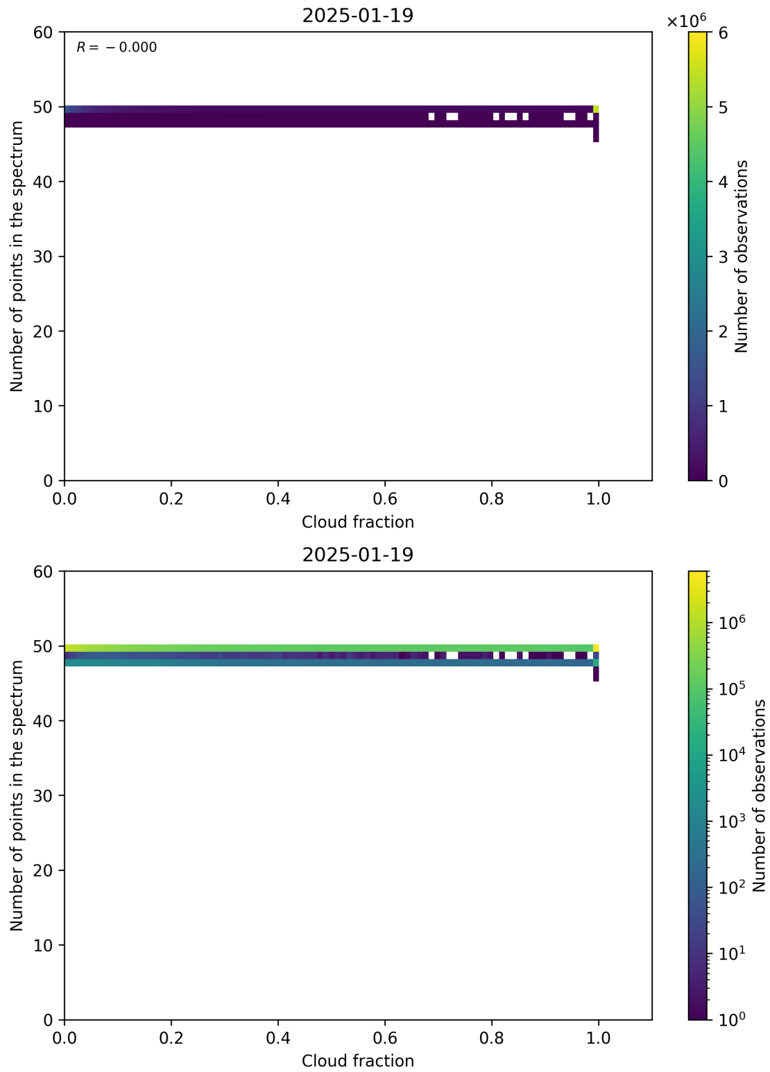
Figure 74: Scatter density plot of “Cloud fraction” against “Number of points in the spectrum” for 2025-01-18 to 2025-01-20.
