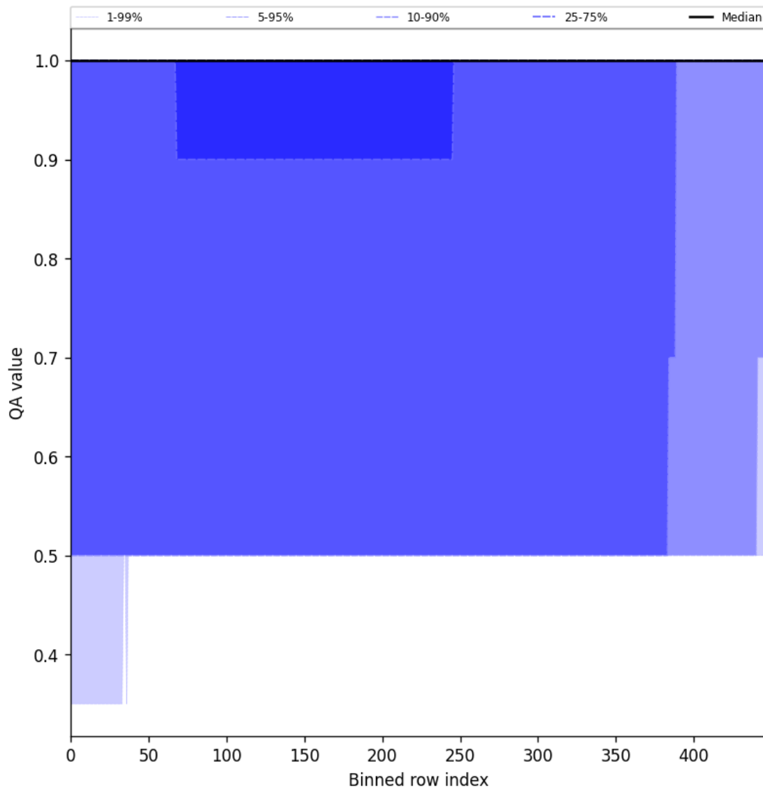
Figure 46: Along track statistics of “QA value” for 2025-01-18 to 2025-01-20
