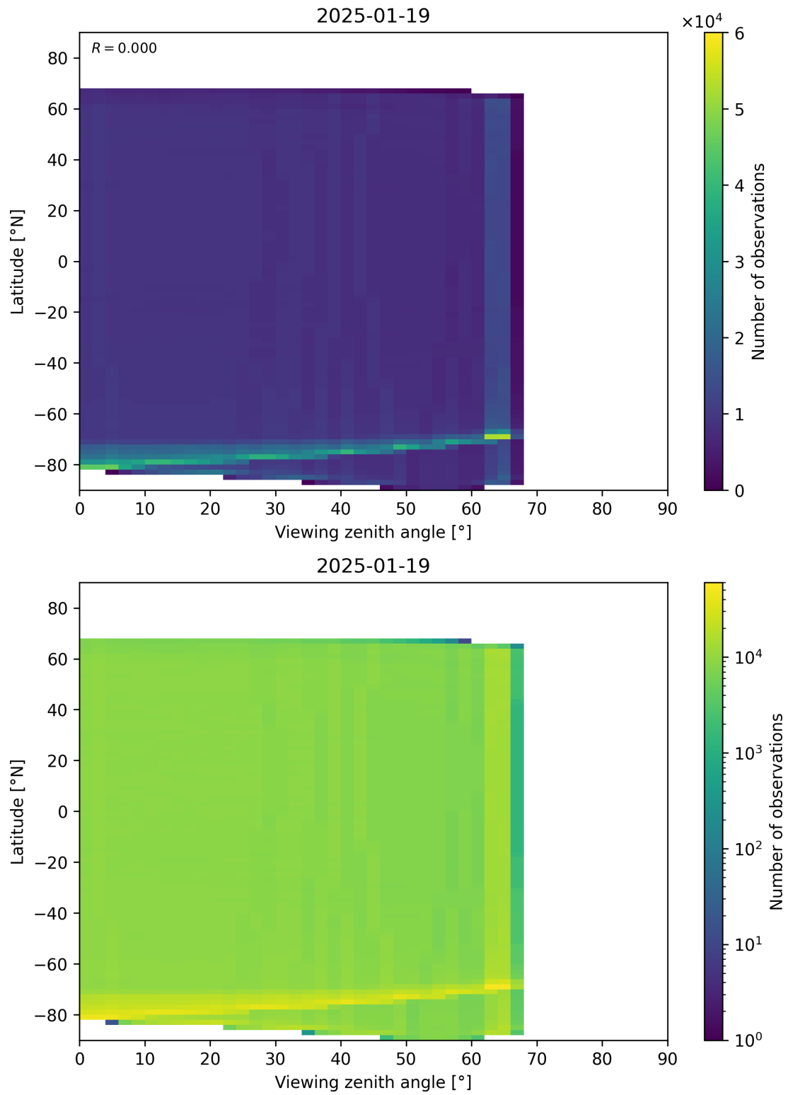
Figure 123: Scatter density plot of “Viewing zenith angle” against “Latitude” for 2025-01-18 to 2025-01-20.
