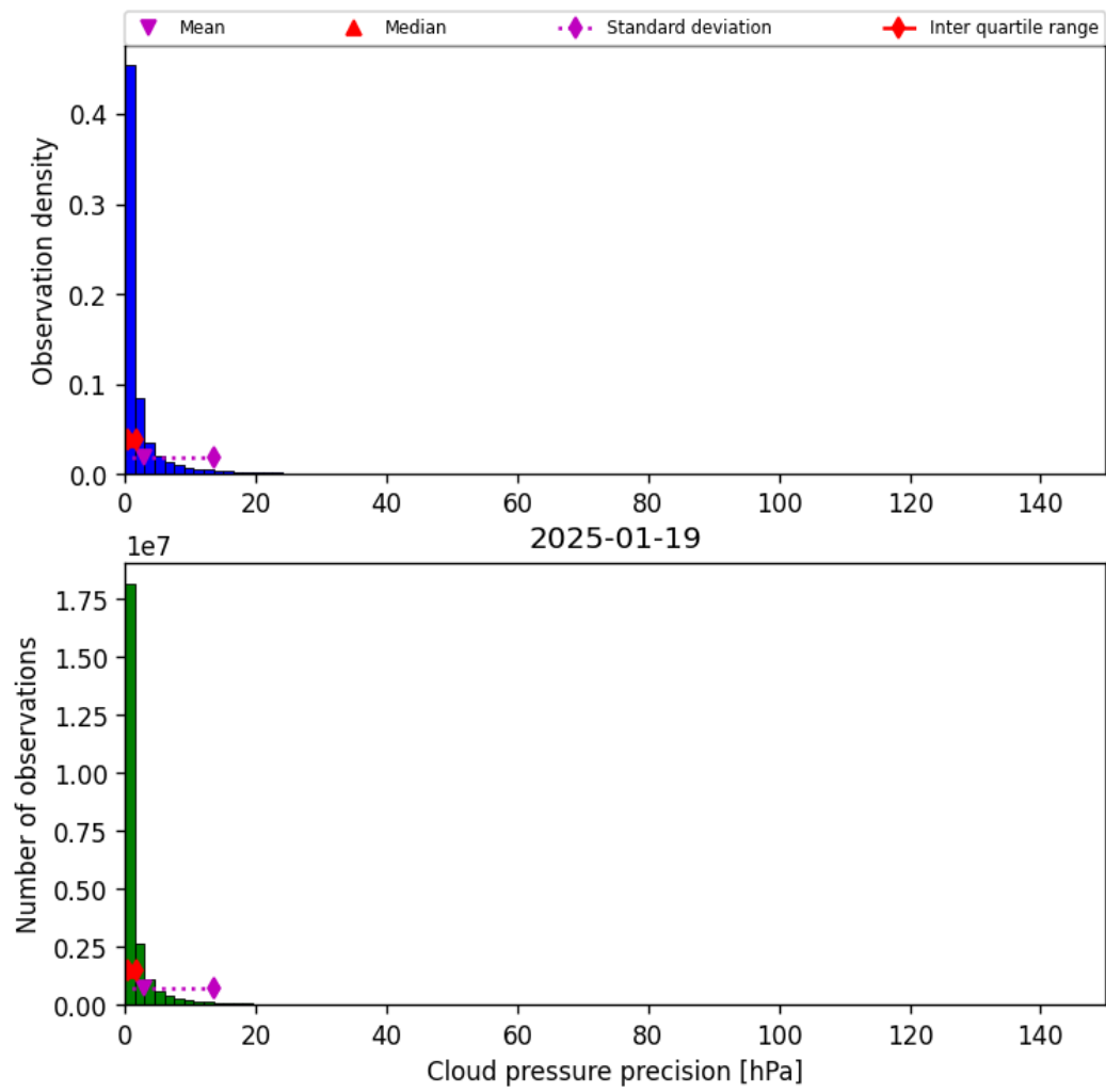
Figure 31: Histogram of “Cloud pressure precision” for 2025-01-18 to 2025-01-20
