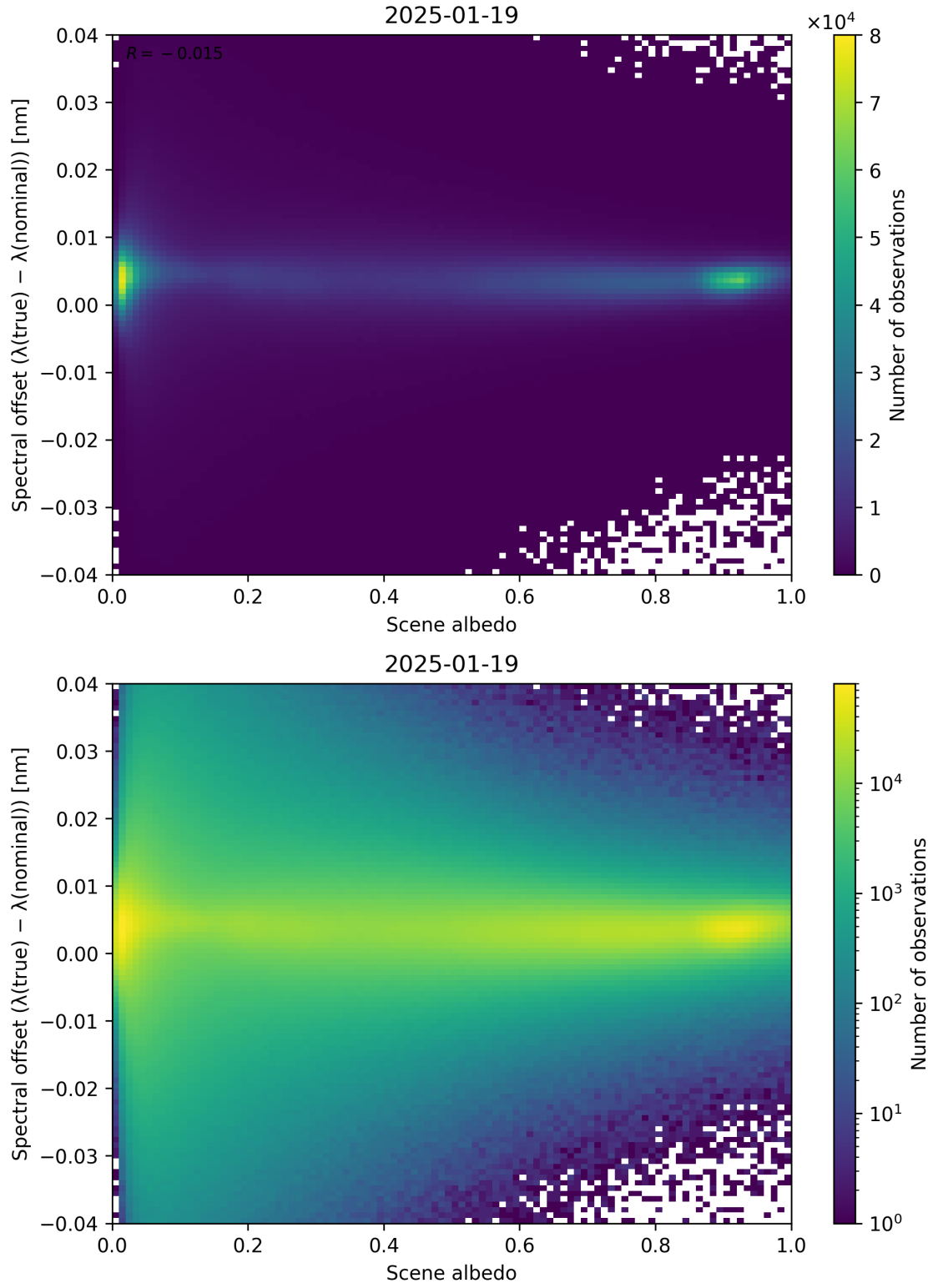
Figure 107: Scatter density plot of “Scene albedo” against “Spectral offset ( \lambda_{\text{true}} - \lambda_{\text{nominal}} )” for 2025-01-18 to 2025-01-20.
