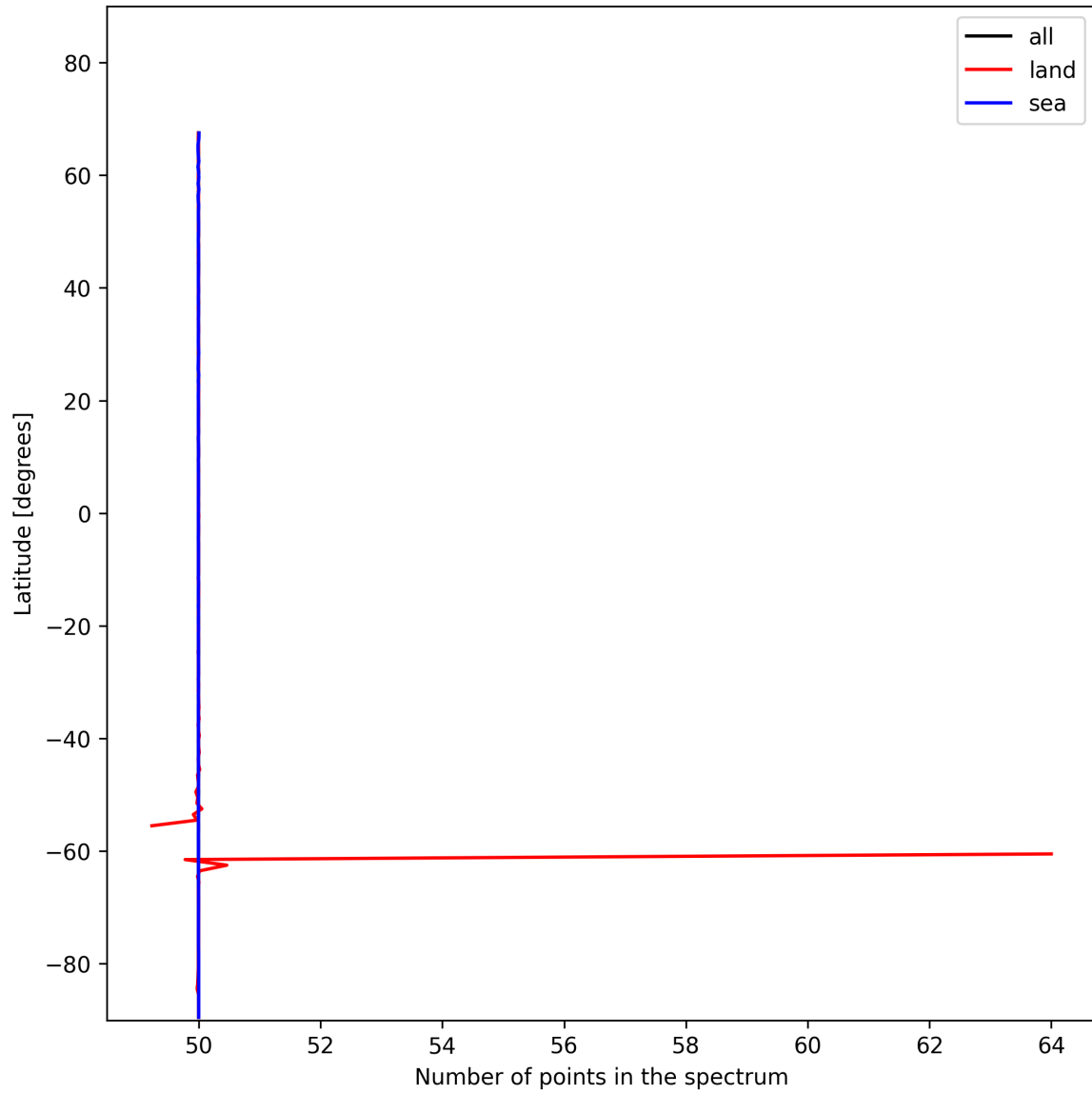
Figure 27: Zonal average of “Number of points in the spectrum” for 2025-01-18 to 2025-01-20.
