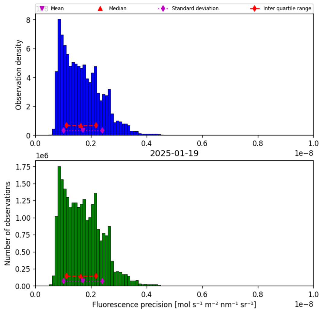
Figure 41: Histogram of “Fluorescence precision” for 2025-01-18 to 2025-01-20
