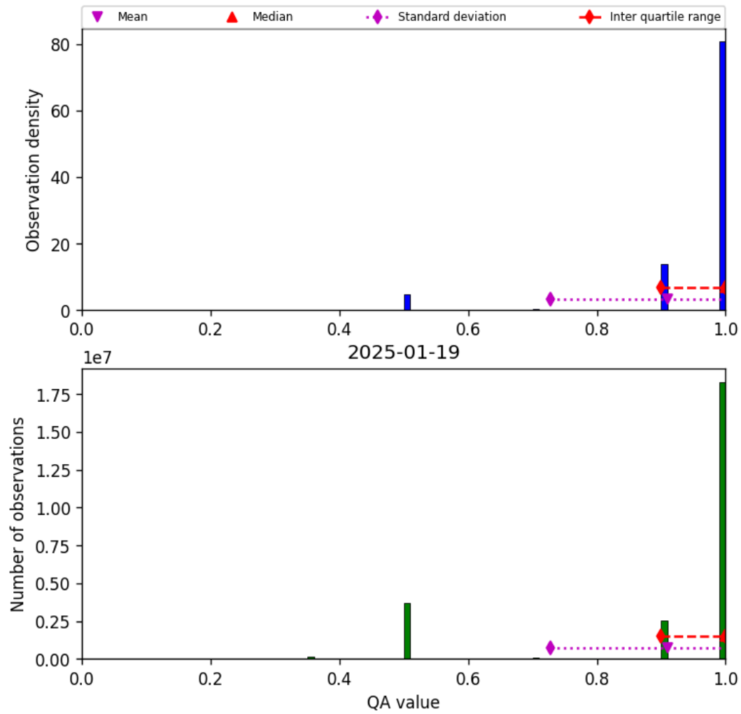
Figure 29: Histogram of “QA value” for 2025-01-18 to 2025-01-20
