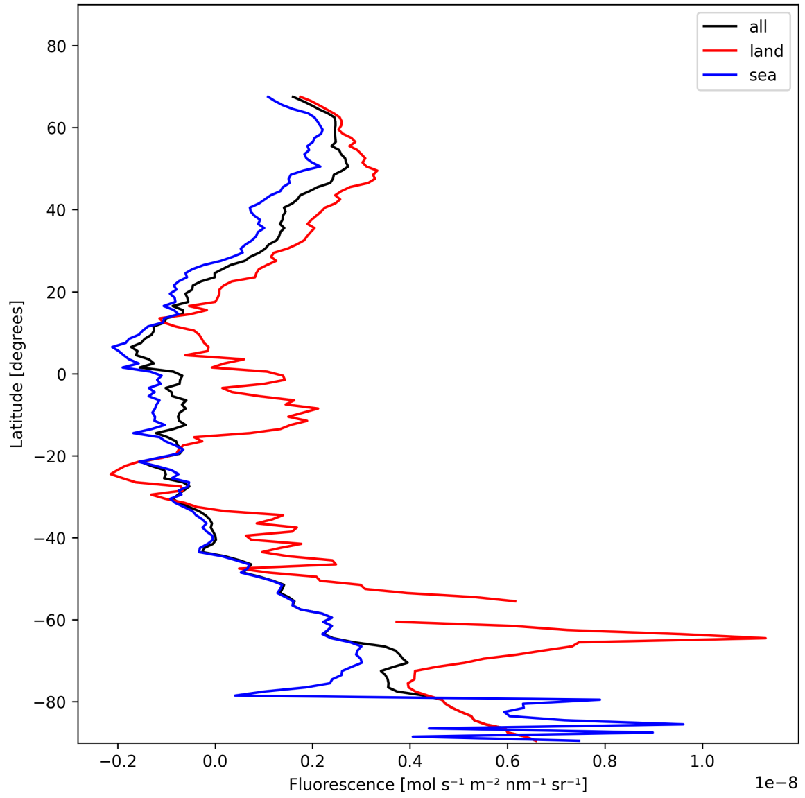
Figure 23: Zonal average of “Fluorescence” for 2025-01-18 to 2025-01-20.
