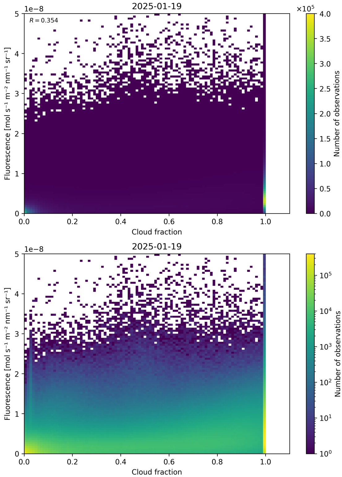
Figure 72: Scatter density plot of “Cloud fraction” against “Fluorescence” for 2025-01-18 to 2025-01-20.
