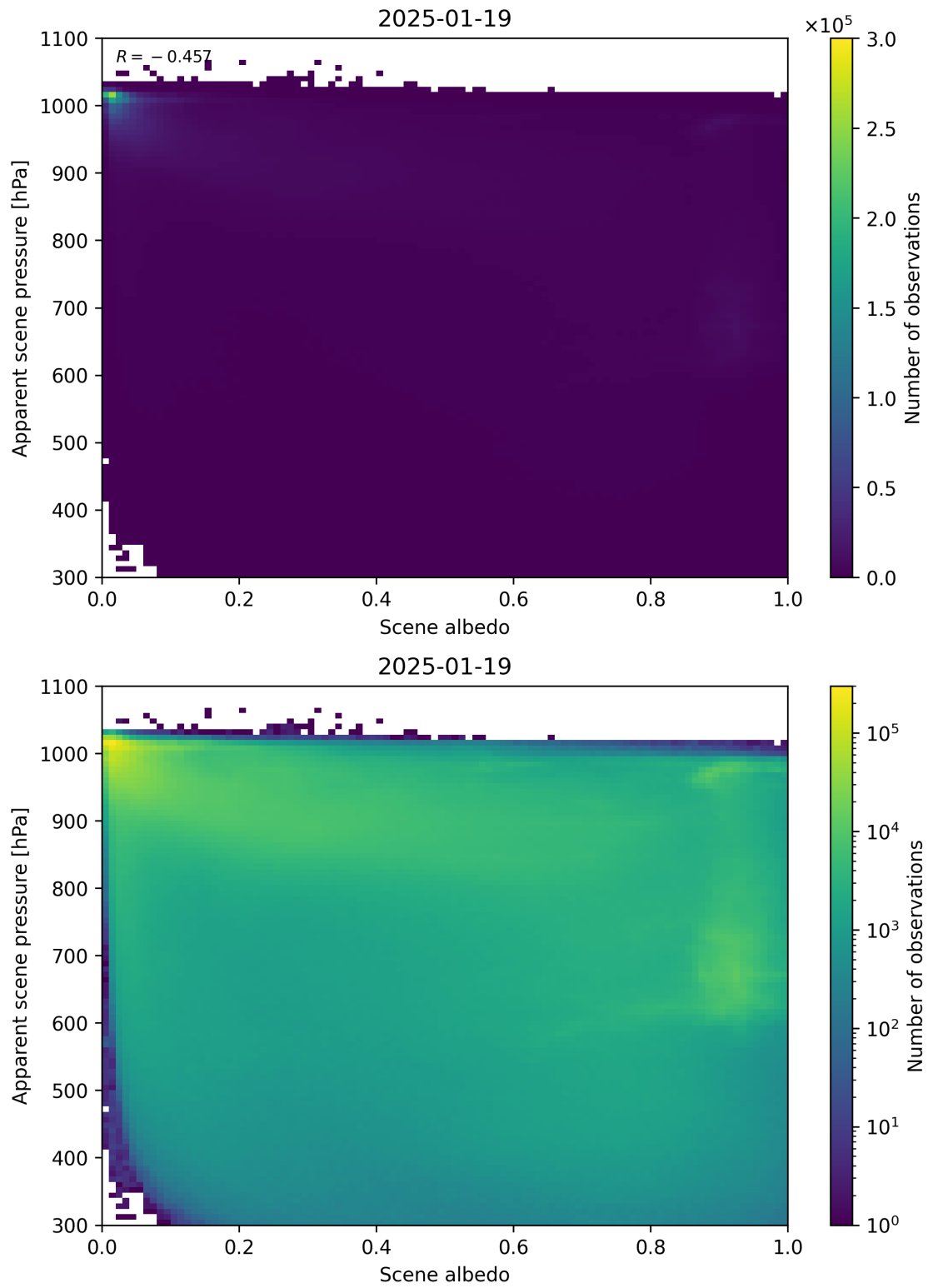
Figure 102: Scatter density plot of “Scene albedo” against “Apparent scene pressure” for 2025-01-18 to 2025-01-20.
