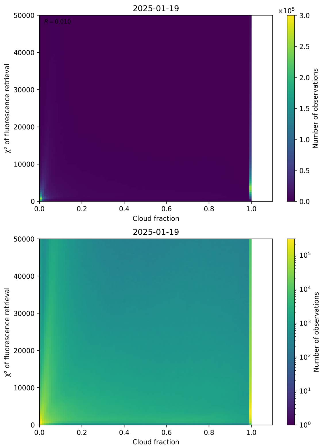
Figure 71: Scatter density plot of “Cloud fraction” against “ \chi^2 of fluorescence retrieval” for 2025-01-18 to 2025-01-20.
