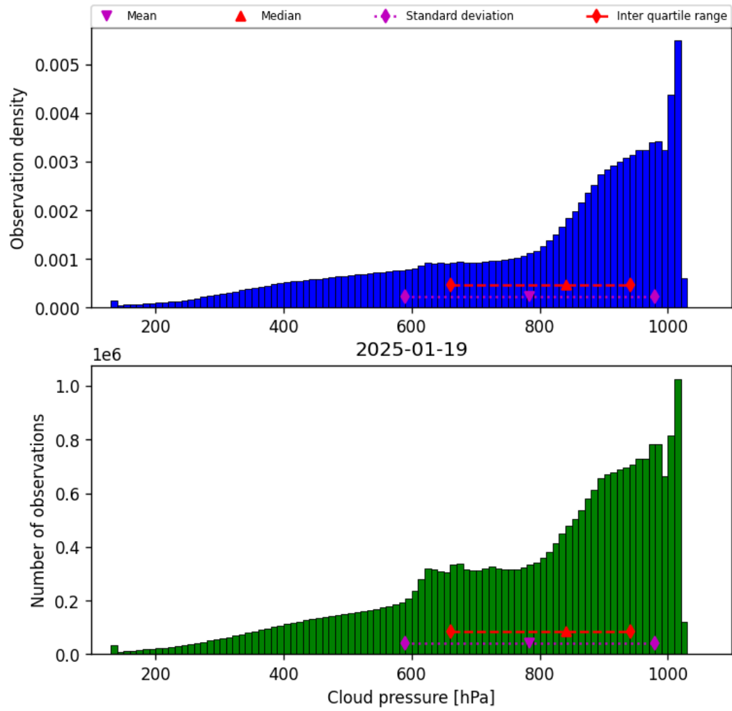
Figure 30: Histogram of “Cloud pressure” for 2025-01-18 to 2025-01-20
