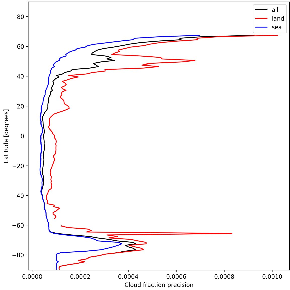
Figure 16: Zonal average of “Cloud fraction precision” for 2025-01-18 to 2025-01-20.
