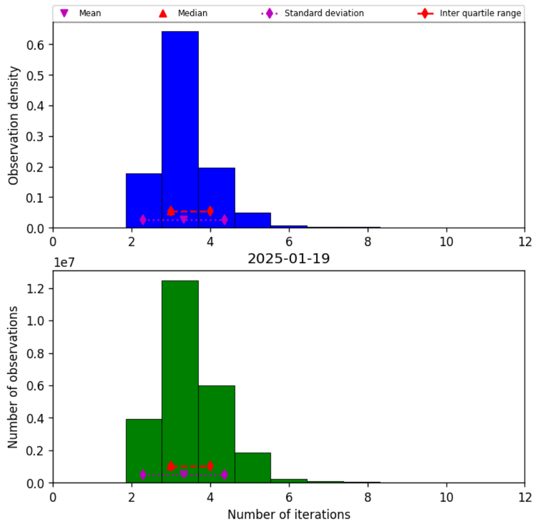
Figure 39: Histogram of “Number of iterations” for 2025-01-18 to 2025-01-20
