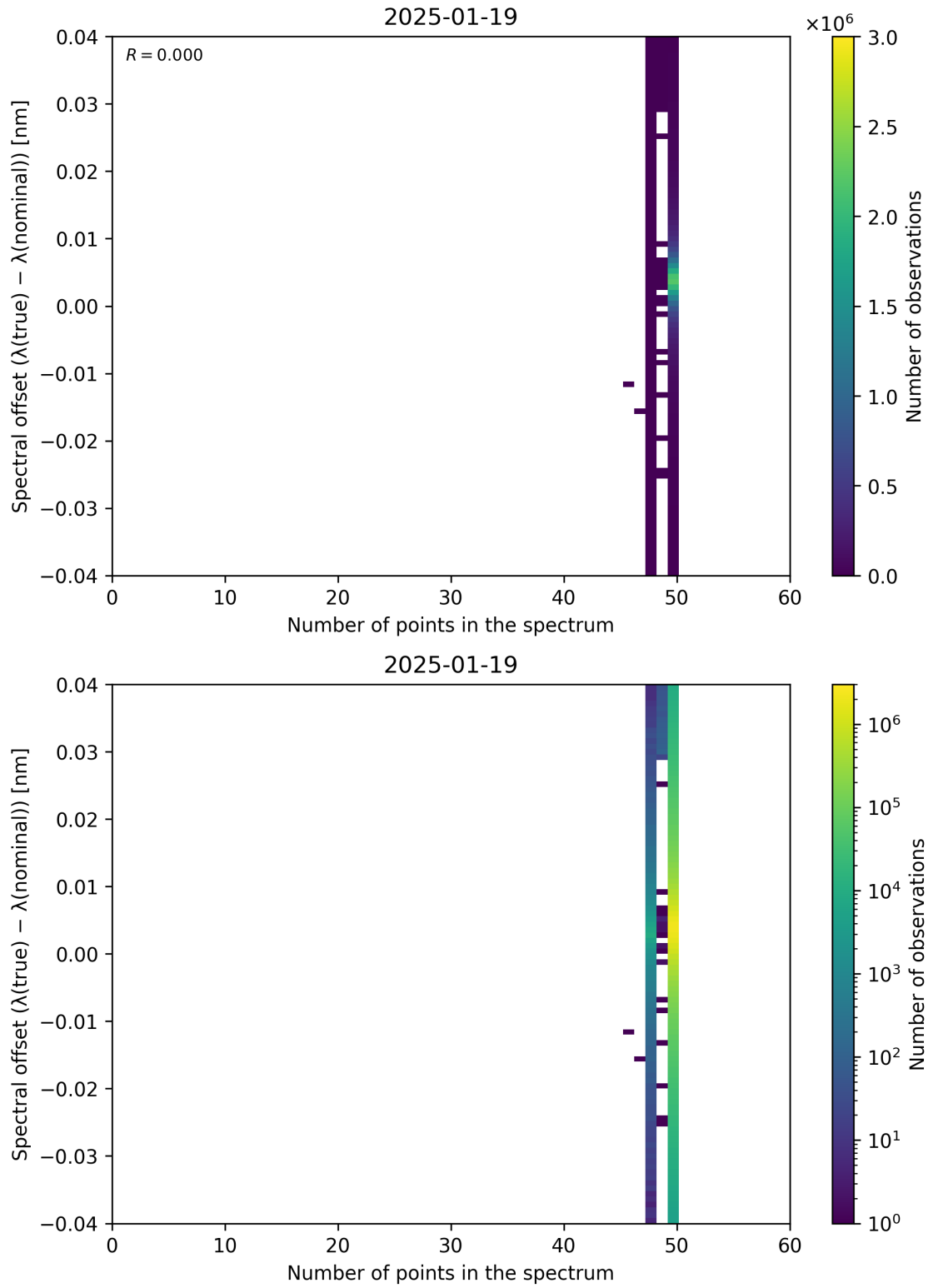
Figure 101: Scatter density plot of “Number of points in the spectrum” against “Spectral offset ( \lambda_{\text{true}} - \lambda_{\text{nominal}} )” for 2025-01-18 to 2025-01-20.
