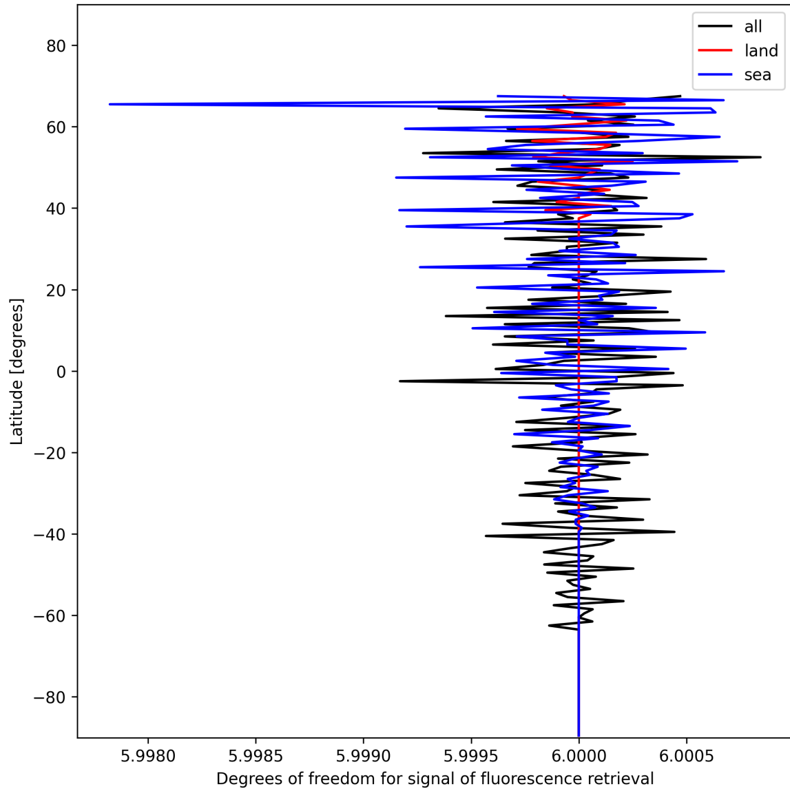
Figure 26: Zonal average of “Degrees of freedom for signal of fluorescence retrieval” for 2025-01-18 to 2025-01-20.
