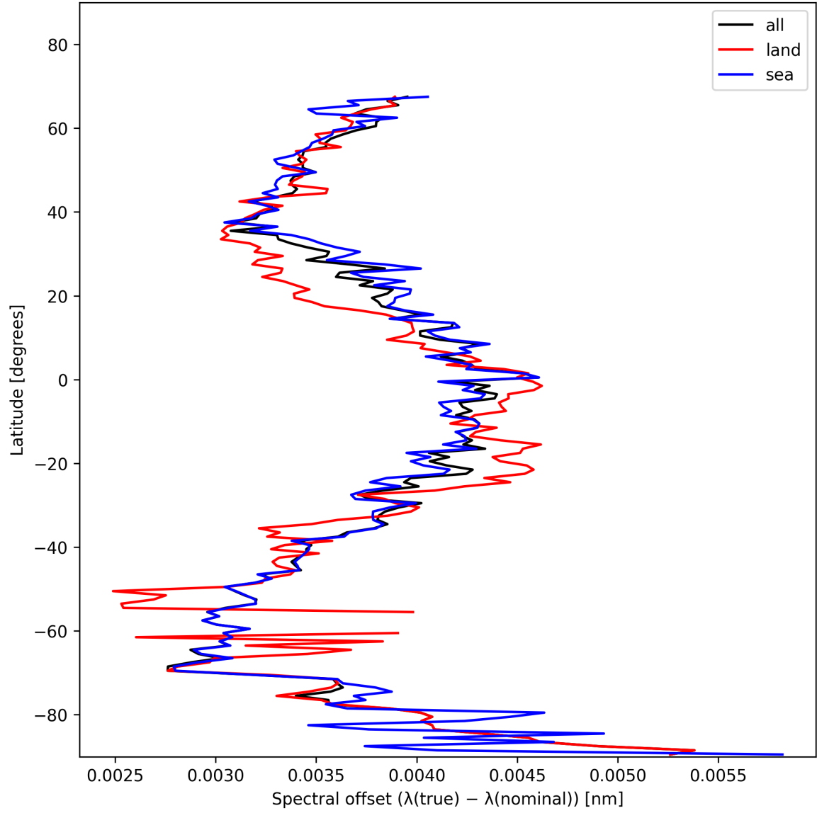
Figure 28: Zonal average of “Spectral offset ( \lambda_{\text{true}} - \lambda_{\text{nominal}} )” for 2025-01-18 to 2025-01-20.
