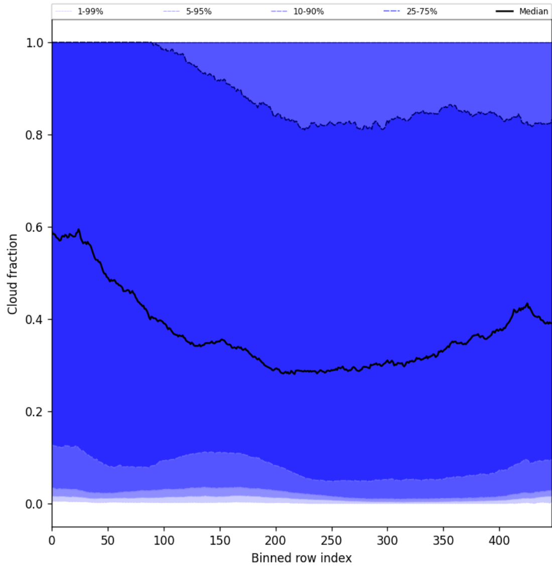
Figure 49: Along track statistics of “Cloud fraction” for 2025-01-18 to 2025-01-20
