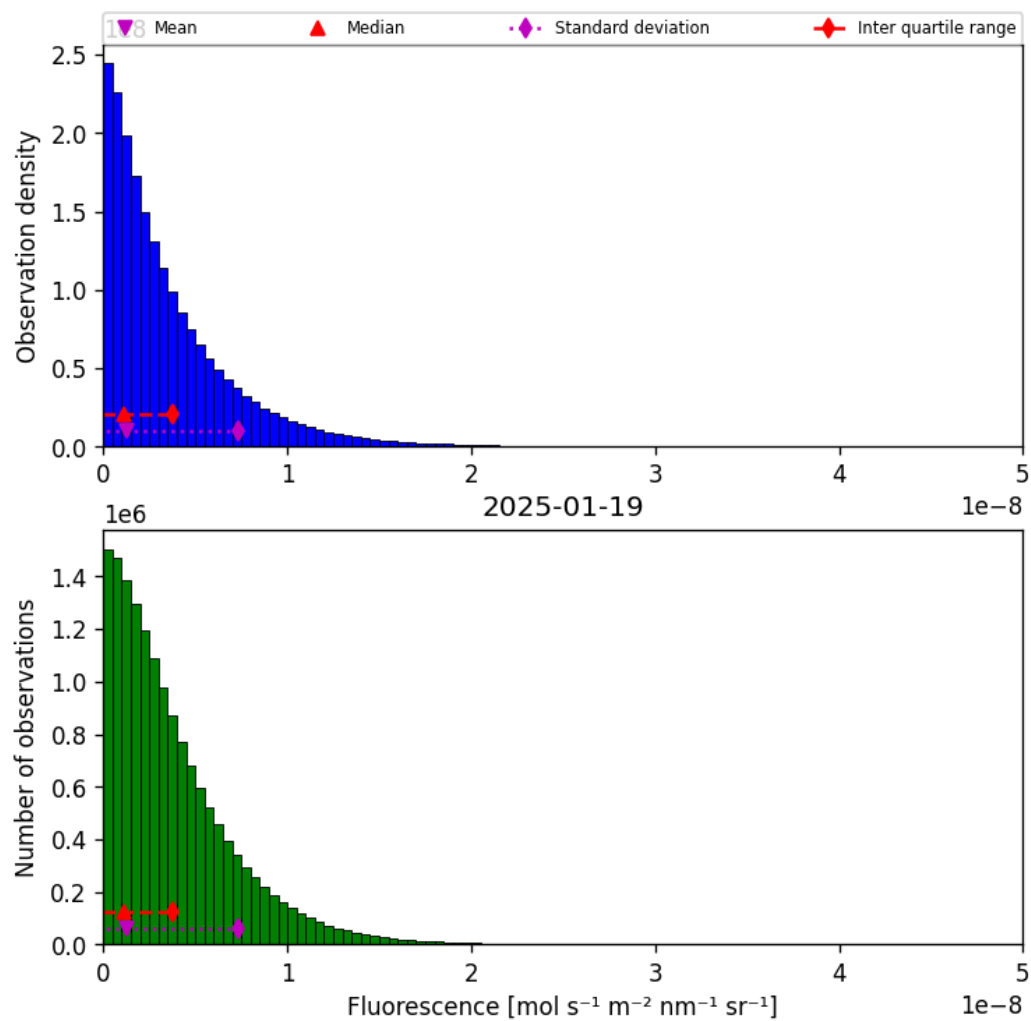
Figure 40: Histogram of “Fluorescence” for 2025-01-18 to 2025-01-20
