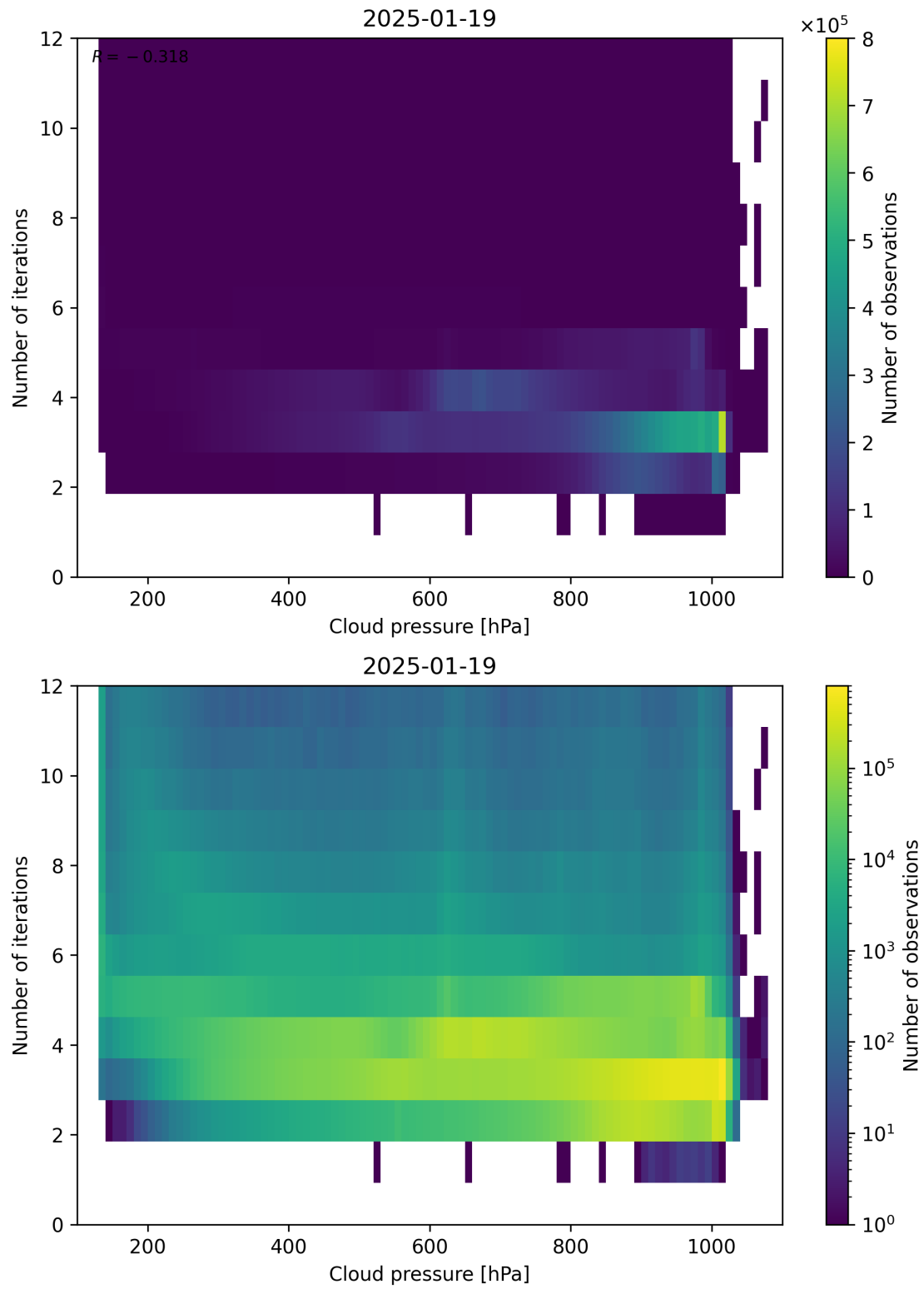
Figure 81: Scatter density plot of “Cloud pressure” against “Number of iterations” for 2025-01-18 to 2025-01-20.
