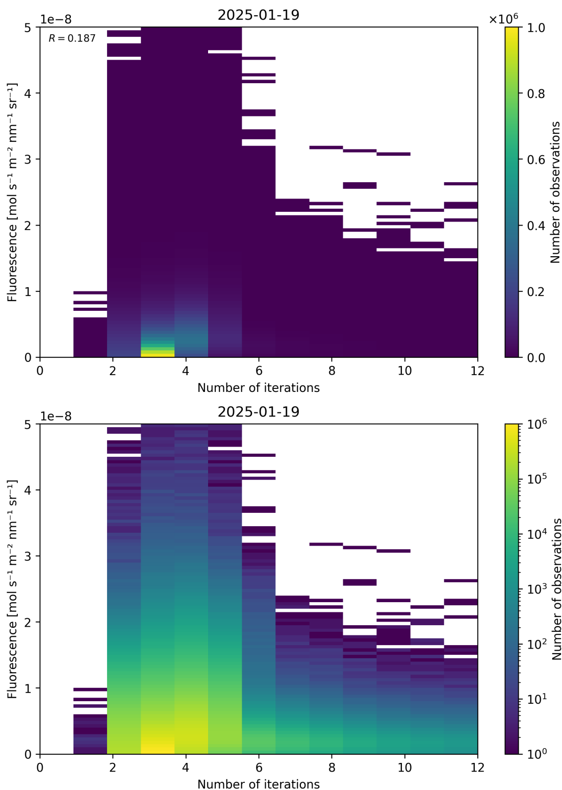
Figure 98: Scatter density plot of “Number of iterations” against “Fluorescence” for 2025-01-18 to 2025-01-20.
