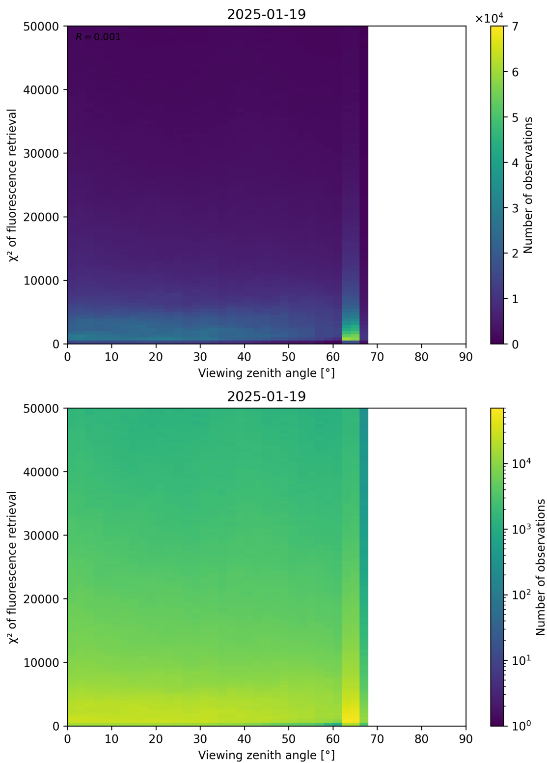
Figure 119: Scatter density plot of “Viewing zenith angle” against “ \chi^2 of fluorescence retrieval” for 2025-01-18 to 2025-01-20.
