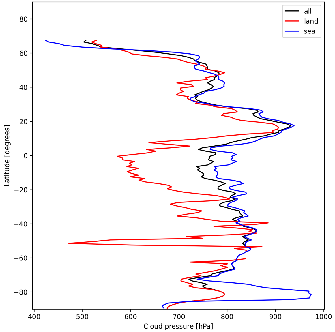
Figure 13: Zonal average of “Cloud pressure” for 2025-01-18 to 2025-01-20.
