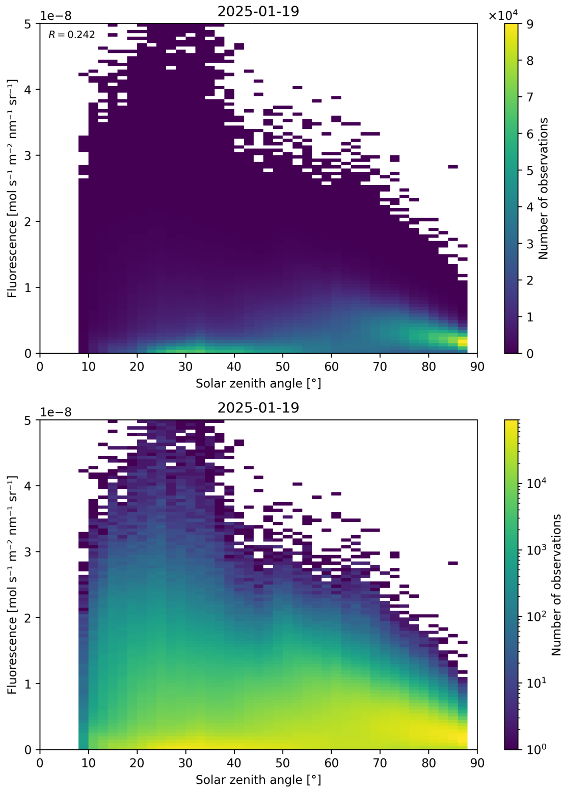
Figure 112: Scatter density plot of “Solar zenith angle” against “Fluorescence” for 2025-01-18 to 2025-01-20.
