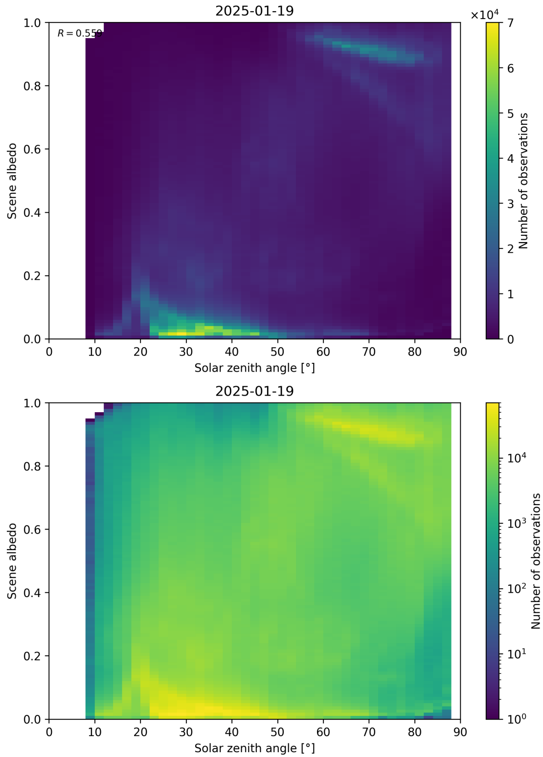
Figure 116: Scatter density plot of “Solar zenith angle” against “Scene albedo” for 2025-01-18 to 2025-01-20.
