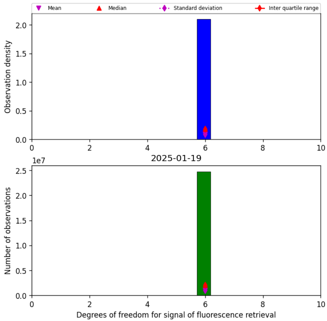
Figure 43: Histogram of “Degrees of freedom for signal of fluorescence retrieval” for 2025-01-18 to 2025-01-20
