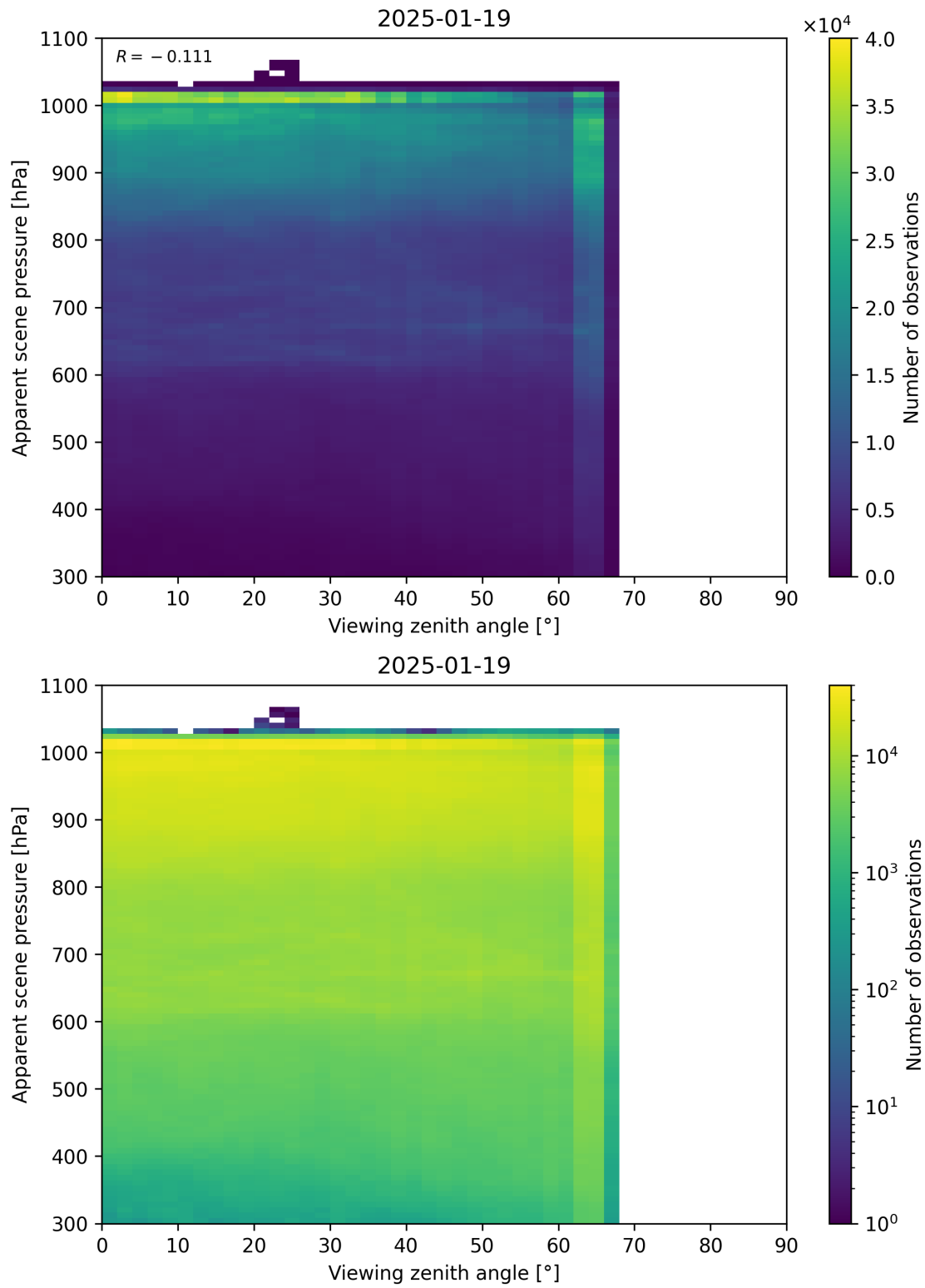
Figure 118: Scatter density plot of “Viewing zenith angle” against “Apparent scene pressure” for 2025-01-18 to 2025-01-20.
