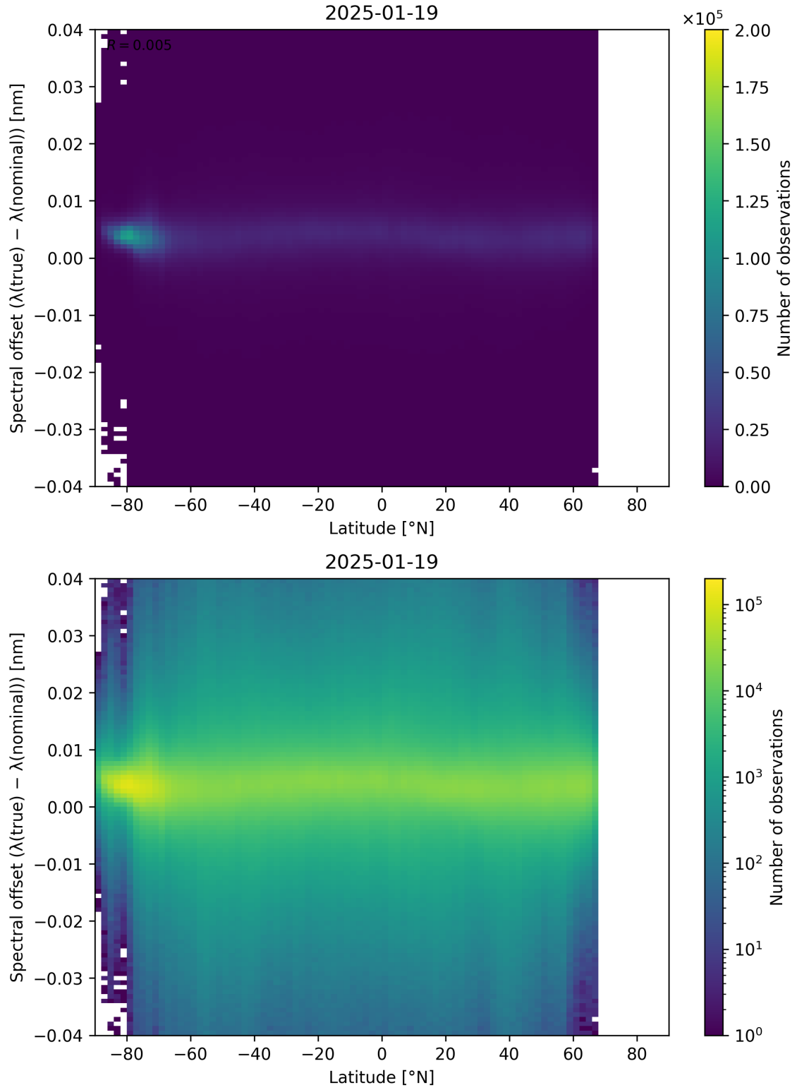
Figure 96: Scatter density plot of “Latitude” against “Spectral offset ( \lambda_{\text{true}} - \lambda_{\text{nominal}} )” for 2025-01-18 to 2025-01-20.
