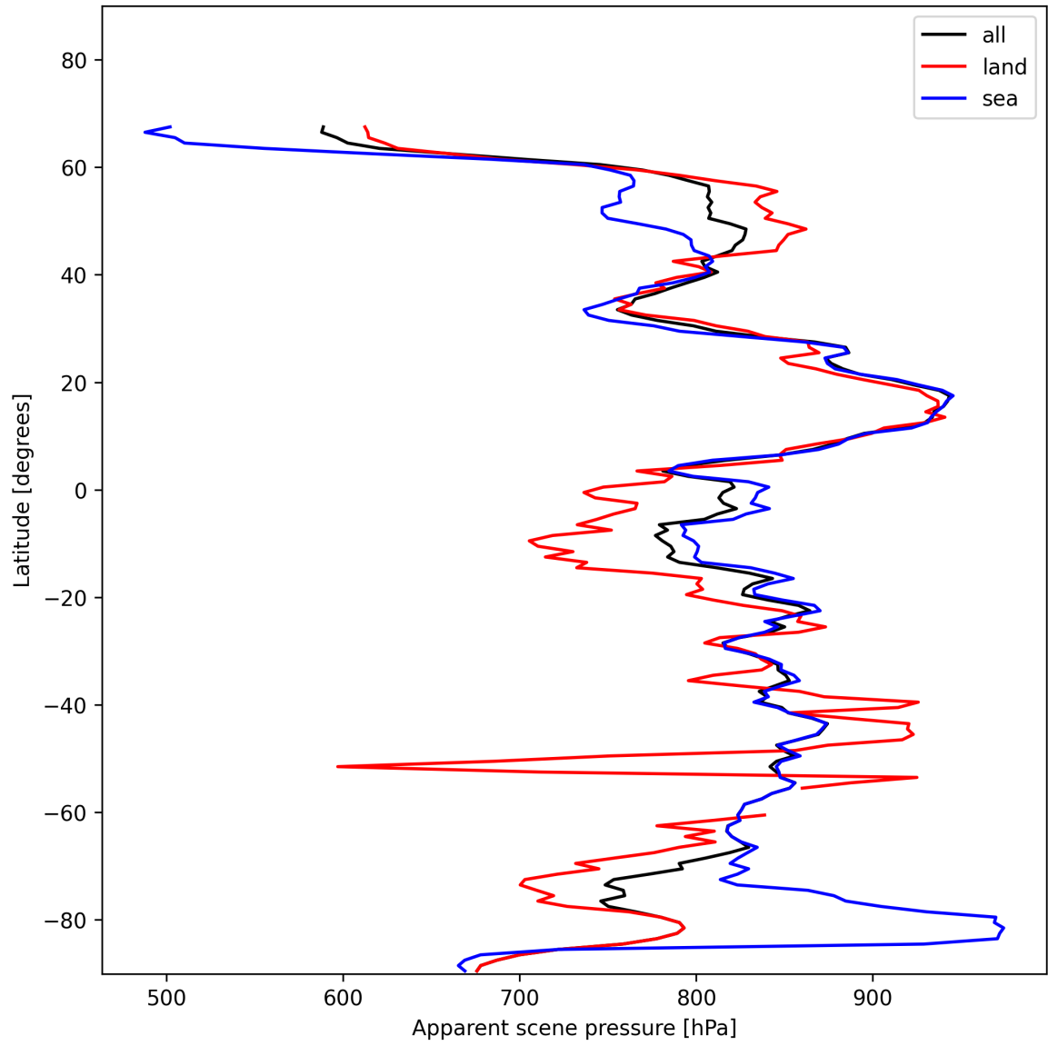
Figure 19: Zonal average of “Apparent scene pressure” for 2025-01-18 to 2025-01-20.
