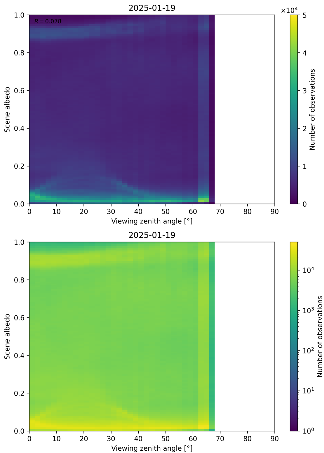
Figure 126: Scatter density plot of “Viewing zenith angle” against “Scene albedo” for 2025-01-18 to 2025-01-20.
