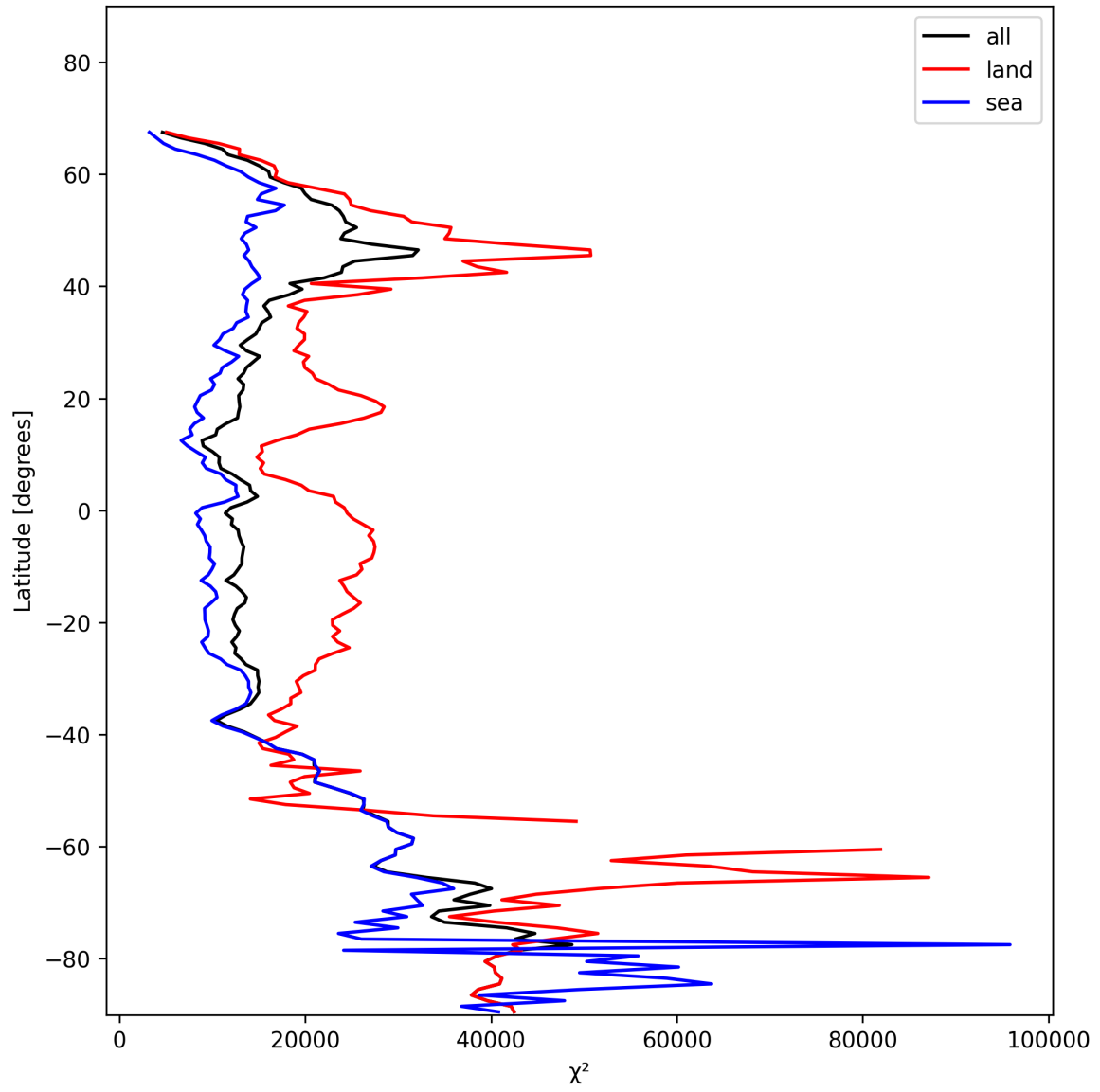
Figure 21: Zonal average of “ \chi^2 ” for 2025-01-18 to 2025-01-20.
