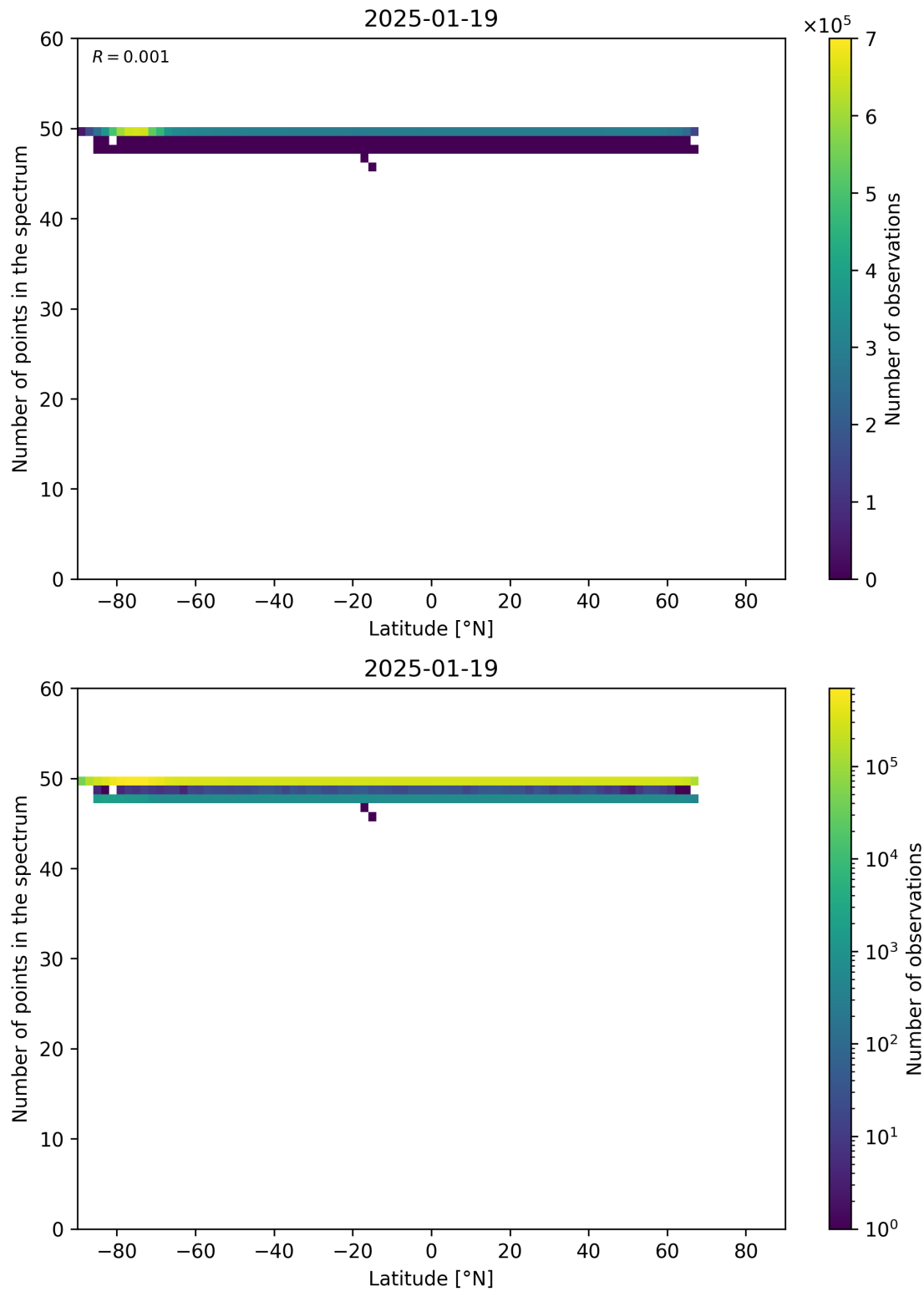
Figure 94: Scatter density plot of “Latitude” against “Number of points in the spectrum” for 2025-01-18 to 2025-01-20.
