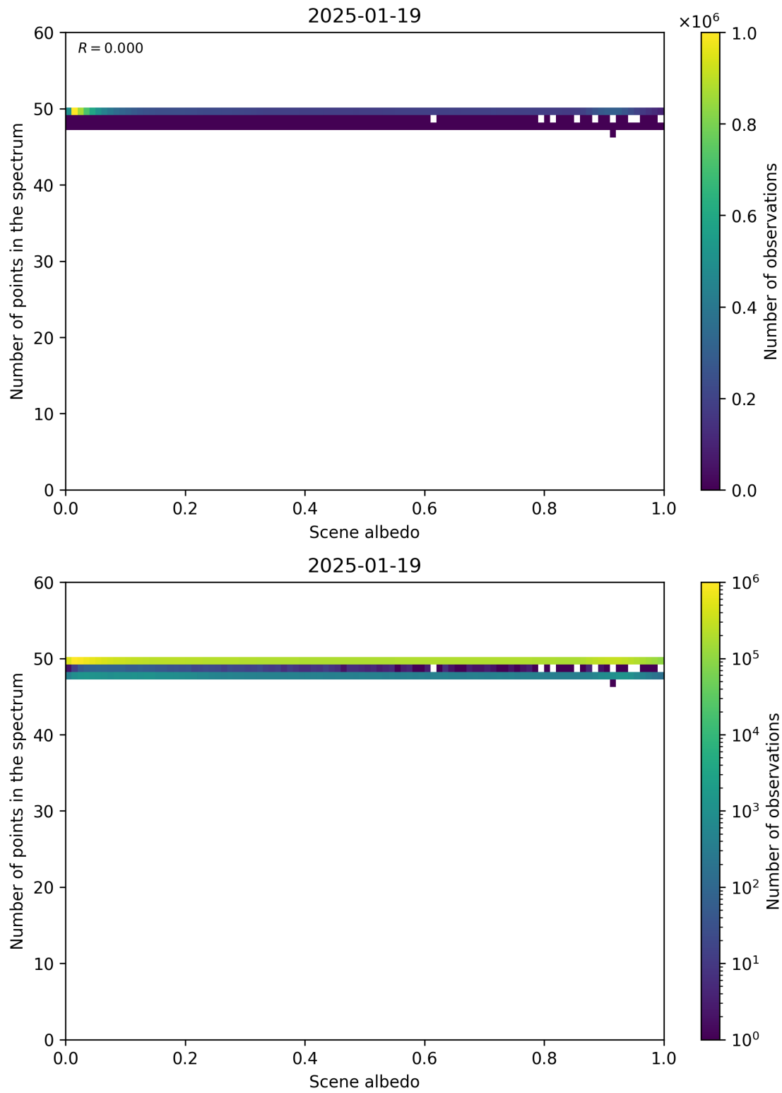
Figure 106: Scatter density plot of “Scene albedo” against “Number of points in the spectrum” for 2025-01-18 to 2025-01-20.
