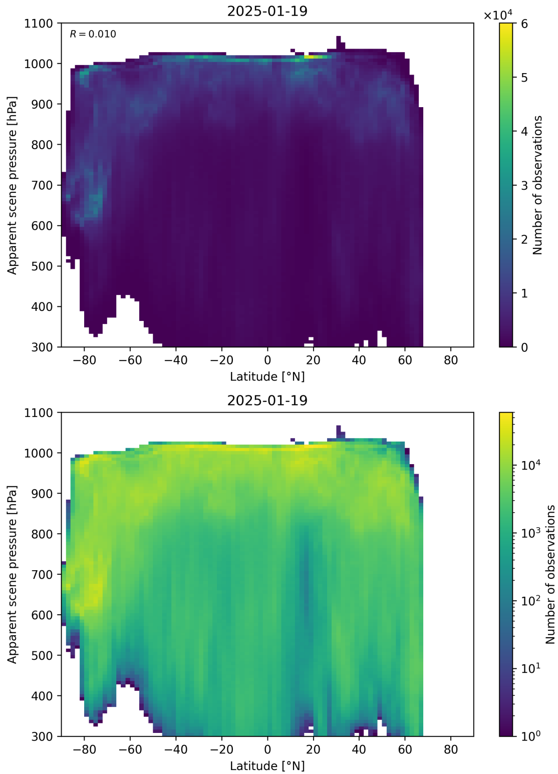
Figure 88: Scatter density plot of “Latitude” against “Apparent scene pressure” for 2025-01-18 to 2025-01-20.
