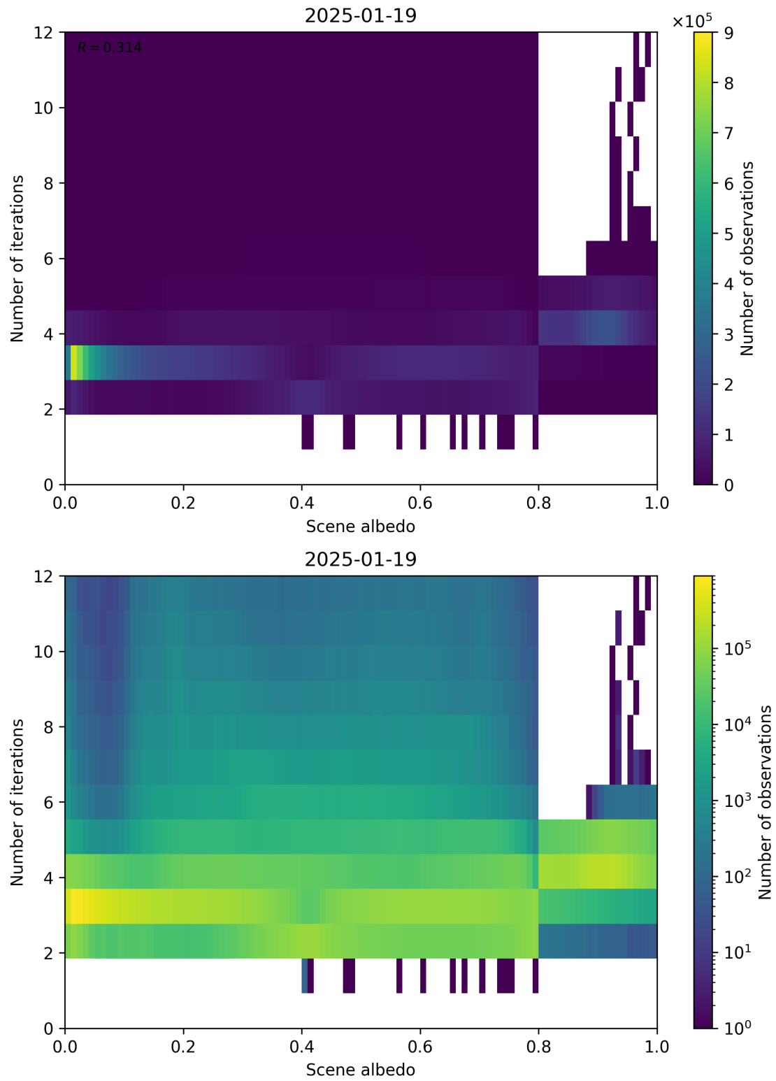
Figure 105: Scatter density plot of “Scene albedo” against “Number of iterations” for 2025-01-18 to 2025-01-20.
