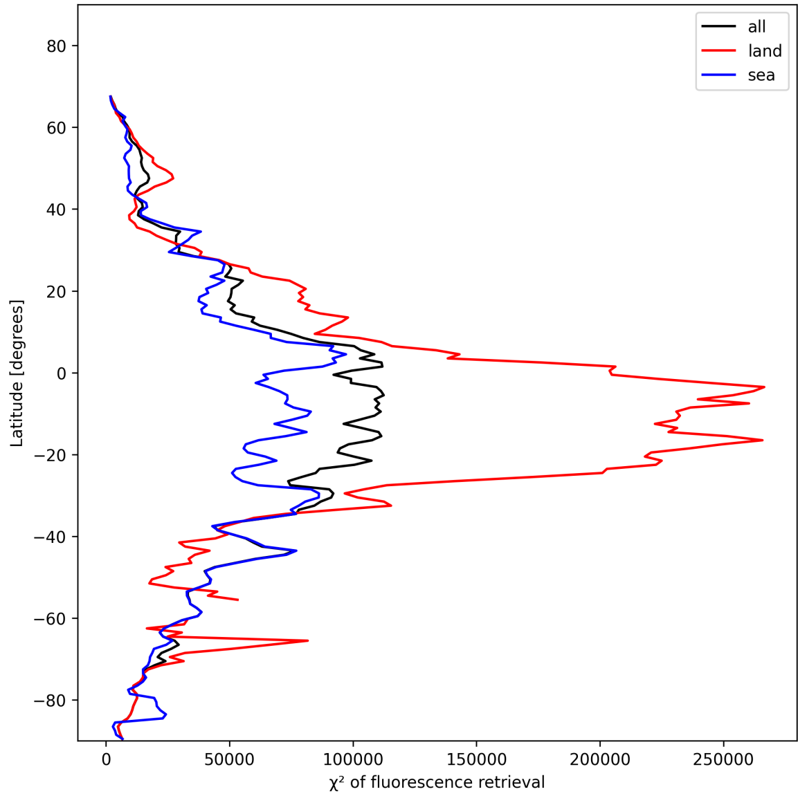
Figure 25: Zonal average of “ \chi^2 of fluorescence retrieval” for 2025-01-18 to 2025-01-20.
