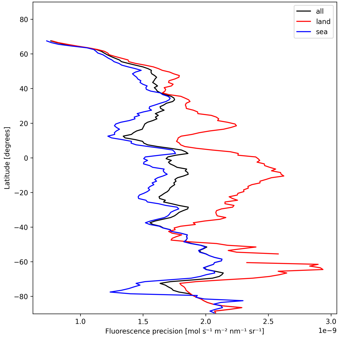
Figure 24: Zonal average of “Fluorescence precision” for 2025-01-18 to 2025-01-20.
