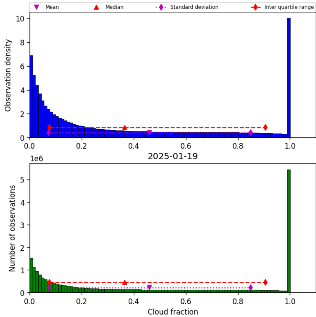
Figure 32: Histogram of “Cloud fraction” for 2025-01-18 to 2025-01-20
