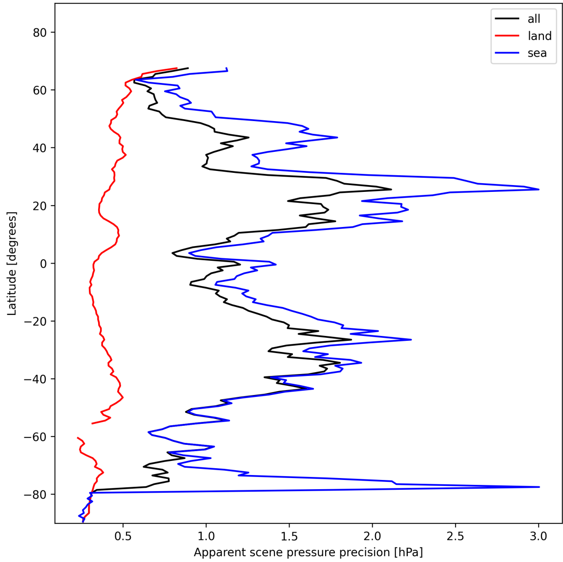
Figure 20: Zonal average of “Apparent scene pressure precision” for 2025-01-18 to 2025-01-20.
