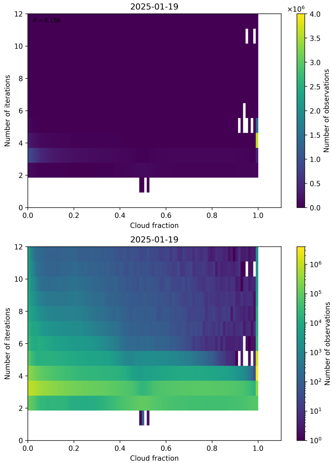
Figure 73: Scatter density plot of “Cloud fraction” against “Number of iterations” for 2025-01-18 to 2025-01-20.
