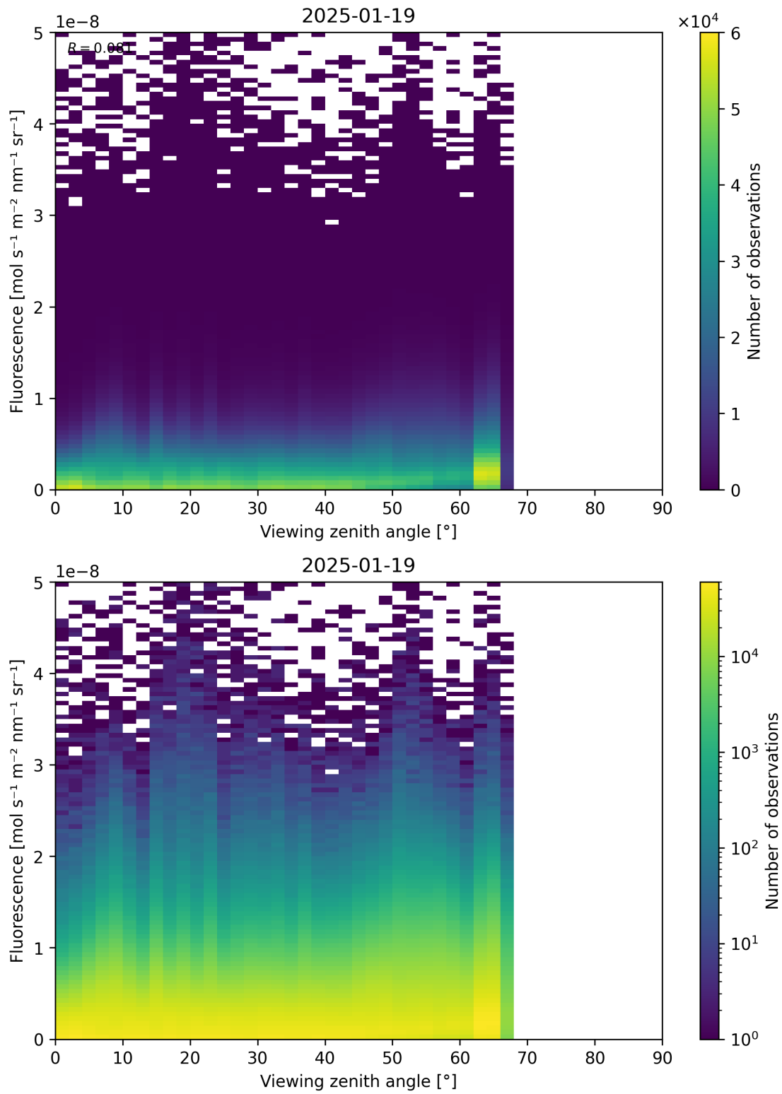
Figure 122: Scatter density plot of “Viewing zenith angle” against “Fluorescence” for 2025-01-18 to 2025-01-20.
