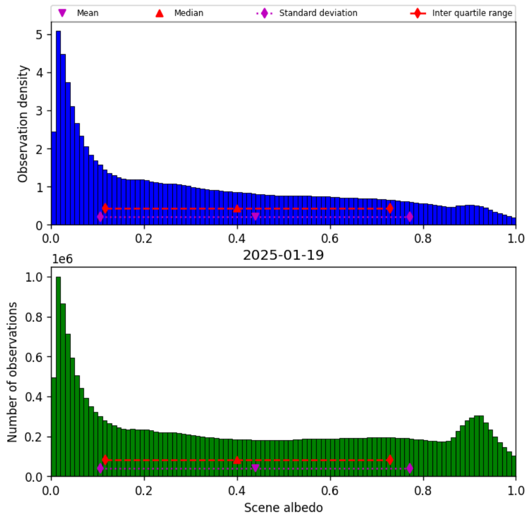
Figure 34: Histogram of “Scene albedo” for 2025-01-18 to 2025-01-20
