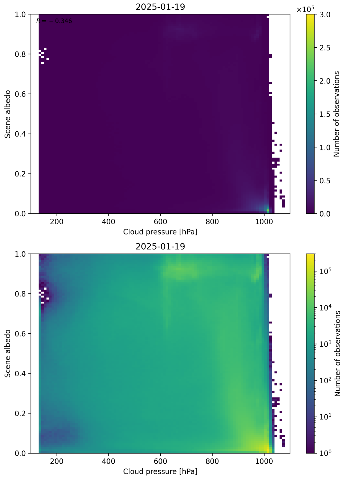
Figure 83: Scatter density plot of “Cloud pressure” against “Scene albedo” for 2025-01-18 to 2025-01-20.
