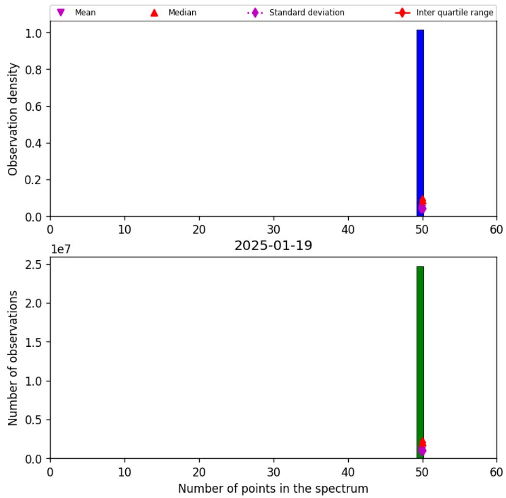
Figure 44: Histogram of “Number of points in the spectrum” for 2025-01-18 to 2025-01-20
