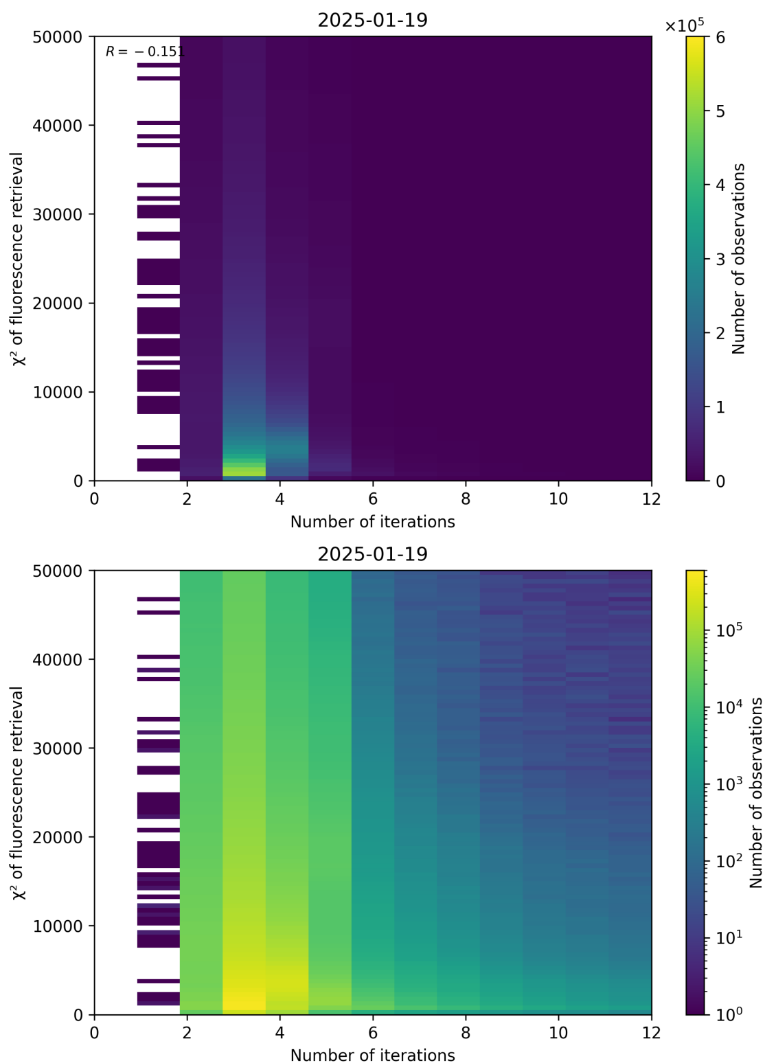
Figure 97: Scatter density plot of “Number of iterations” against “ \chi^2 of fluorescence retrieval” for 2025-01-18 to 2025-01-20.
