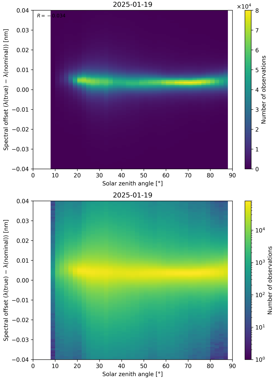
Figure 117: Scatter density plot of “Solar zenith angle” against “Spectral offset ( \lambda_{\text{true}} - \lambda_{\text{nominal}} )” for 2025-01-18 to 2025-01-20.
