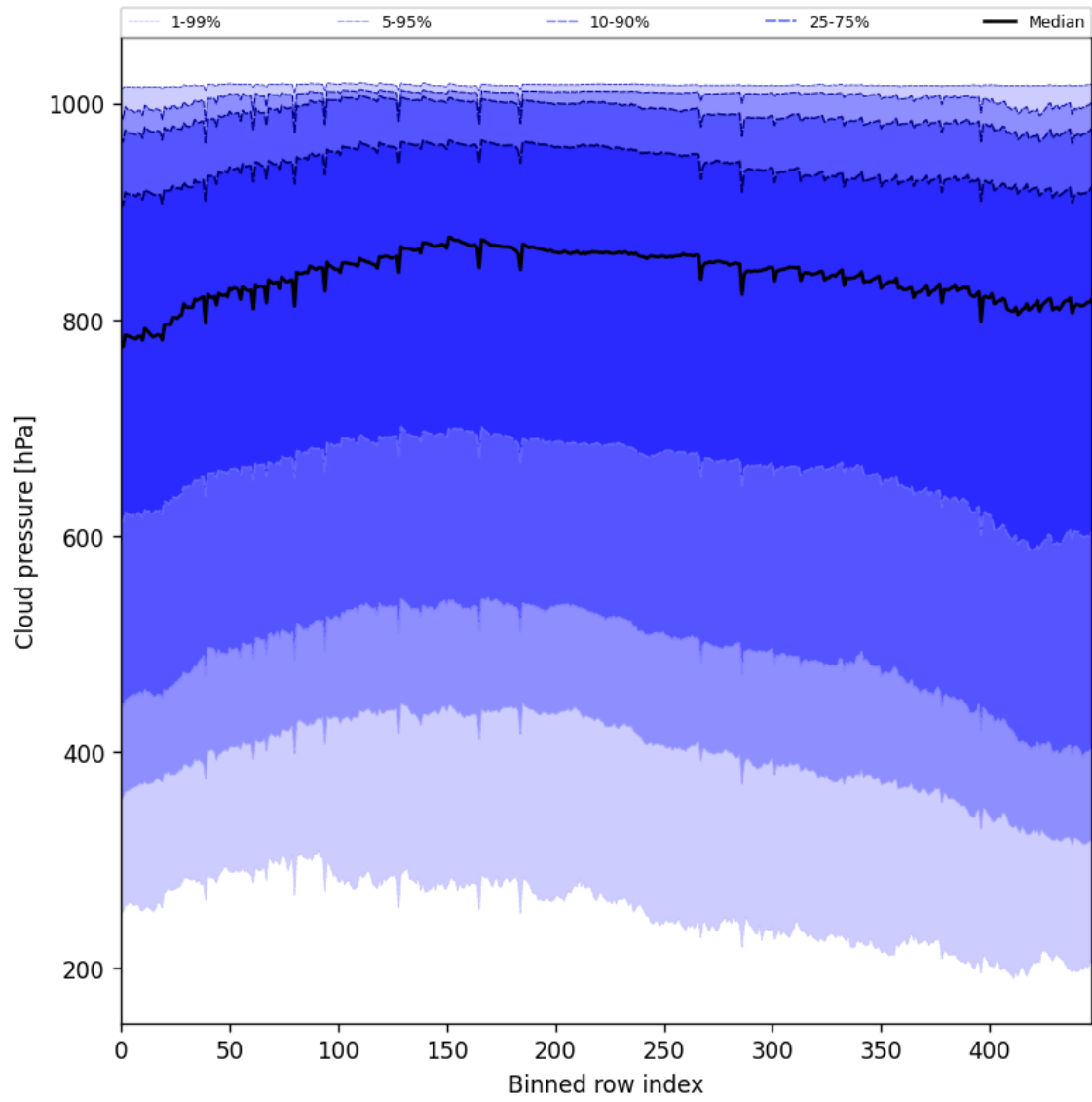
Figure 47: Along track statistics of “Cloud pressure” for 2025-01-18 to 2025-01-20
