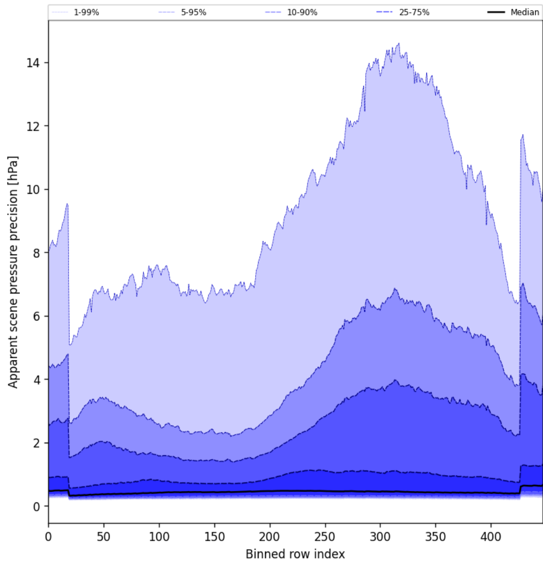
Figure 54: Along track statistics of “Apparent scene pressure precision” for 2025-01-18 to 2025-01-20
