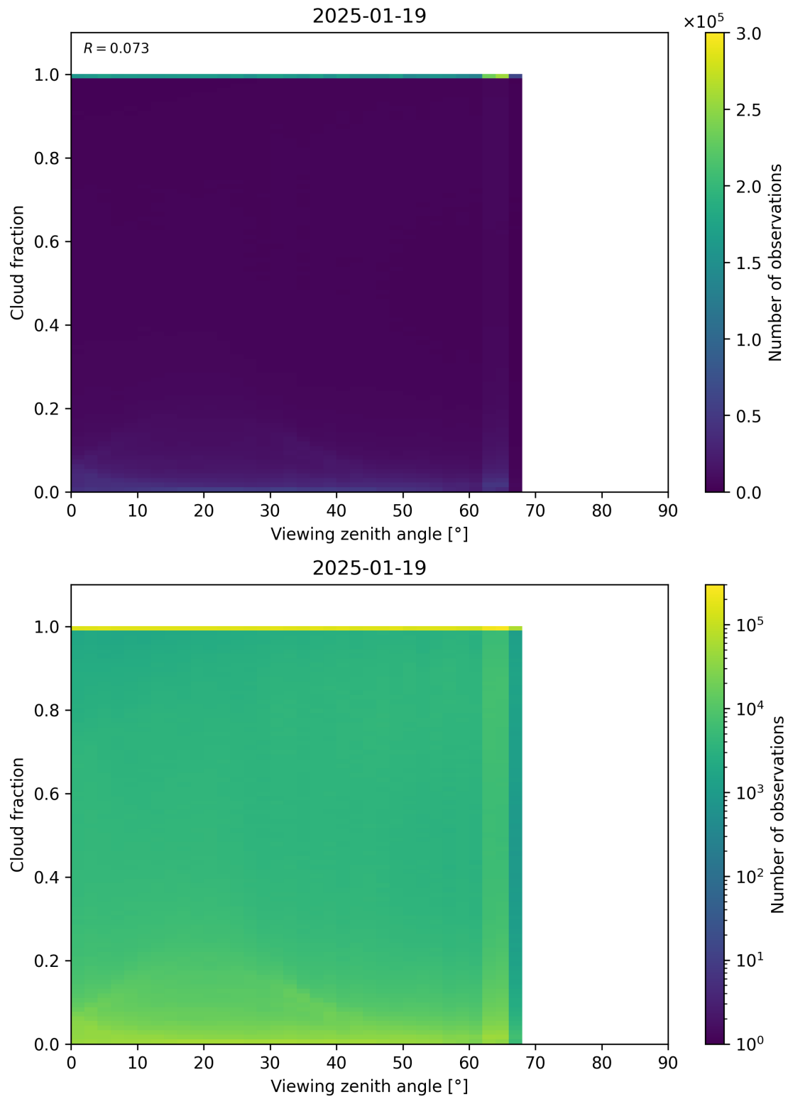
Figure 120: Scatter density plot of “Viewing zenith angle” against “Cloud fraction” for 2025-01-18 to 2025-01-20.
