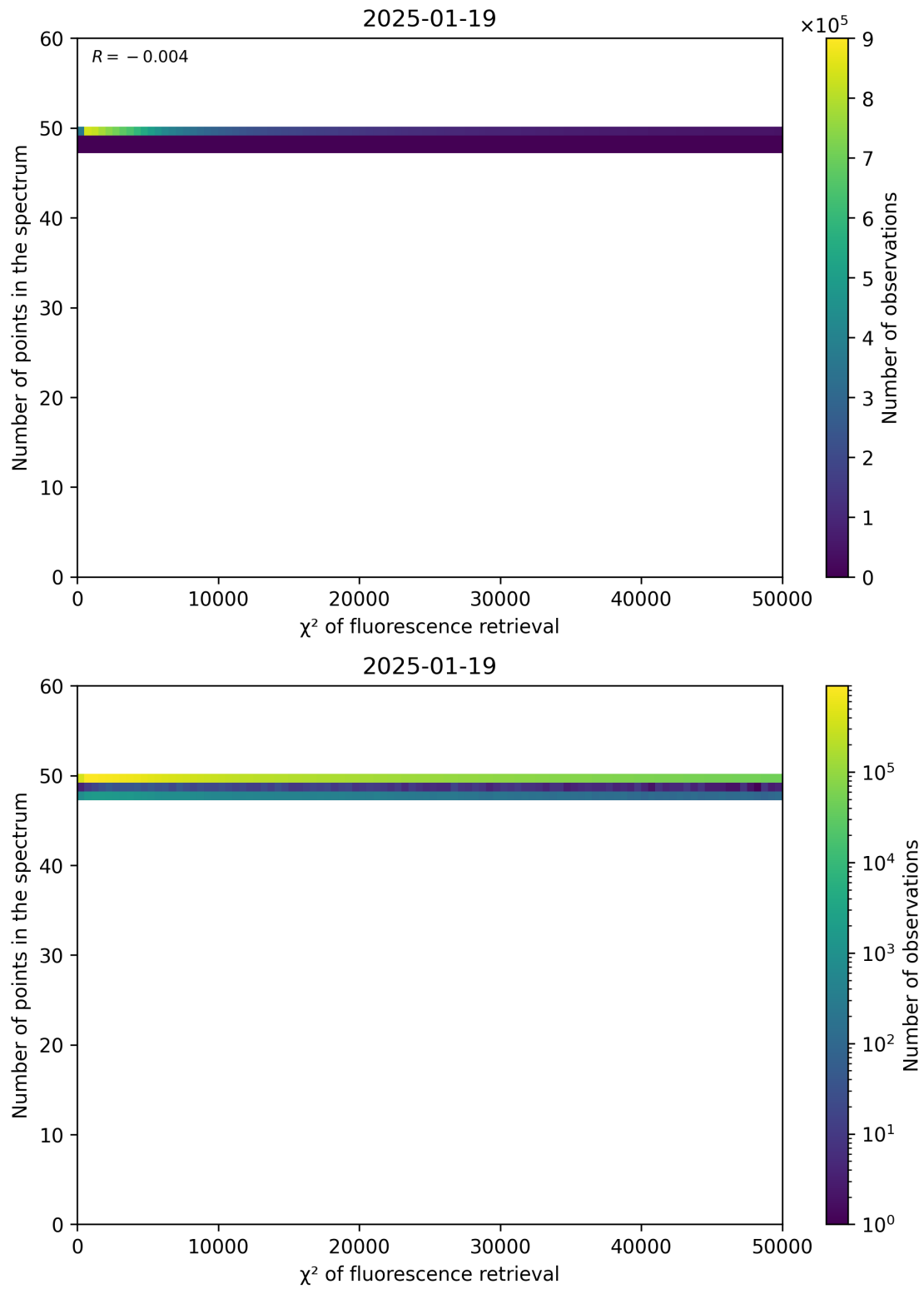
Figure 68: Scatter density plot of " \chi^2 of fluorescence retrieval" against "Number of points in the spectrum" for 2025-01-18 to 2025-01-20.
