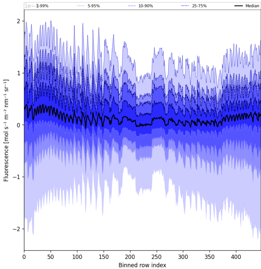
Figure 57: Along track statistics of “Fluorescence” for 2025-01-18 to 2025-01-20
