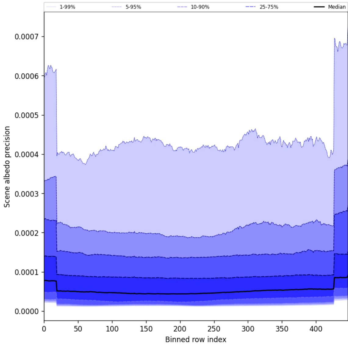
Figure 52: Along track statistics of “Scene albedo precision” for 2025-01-18 to 2025-01-20
