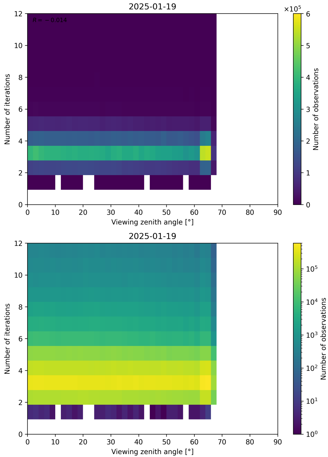
Figure 124: Scatter density plot of “Viewing zenith angle” against “Number of iterations” for 2025-01-18 to 2025-01-20.
