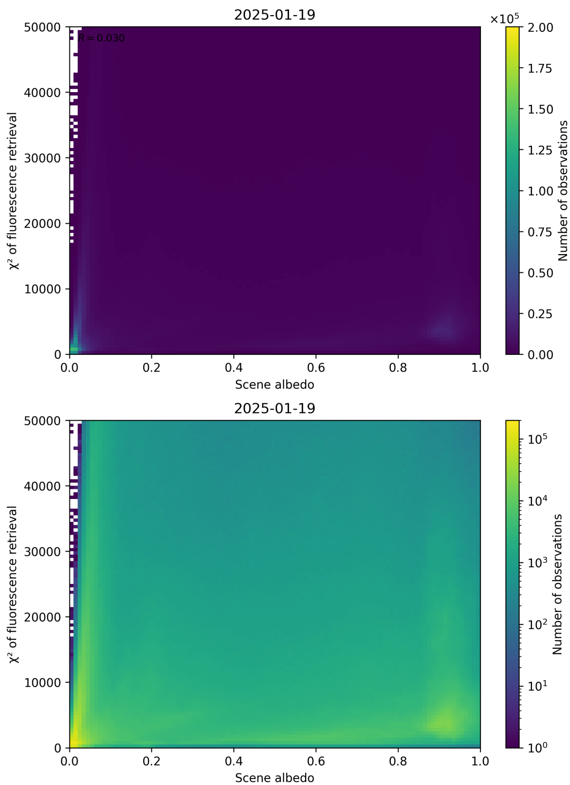
Figure 103: Scatter density plot of “Scene albedo” against “ \chi^2 of fluorescence retrieval” for 2025-01-18 to 2025-01-20.
