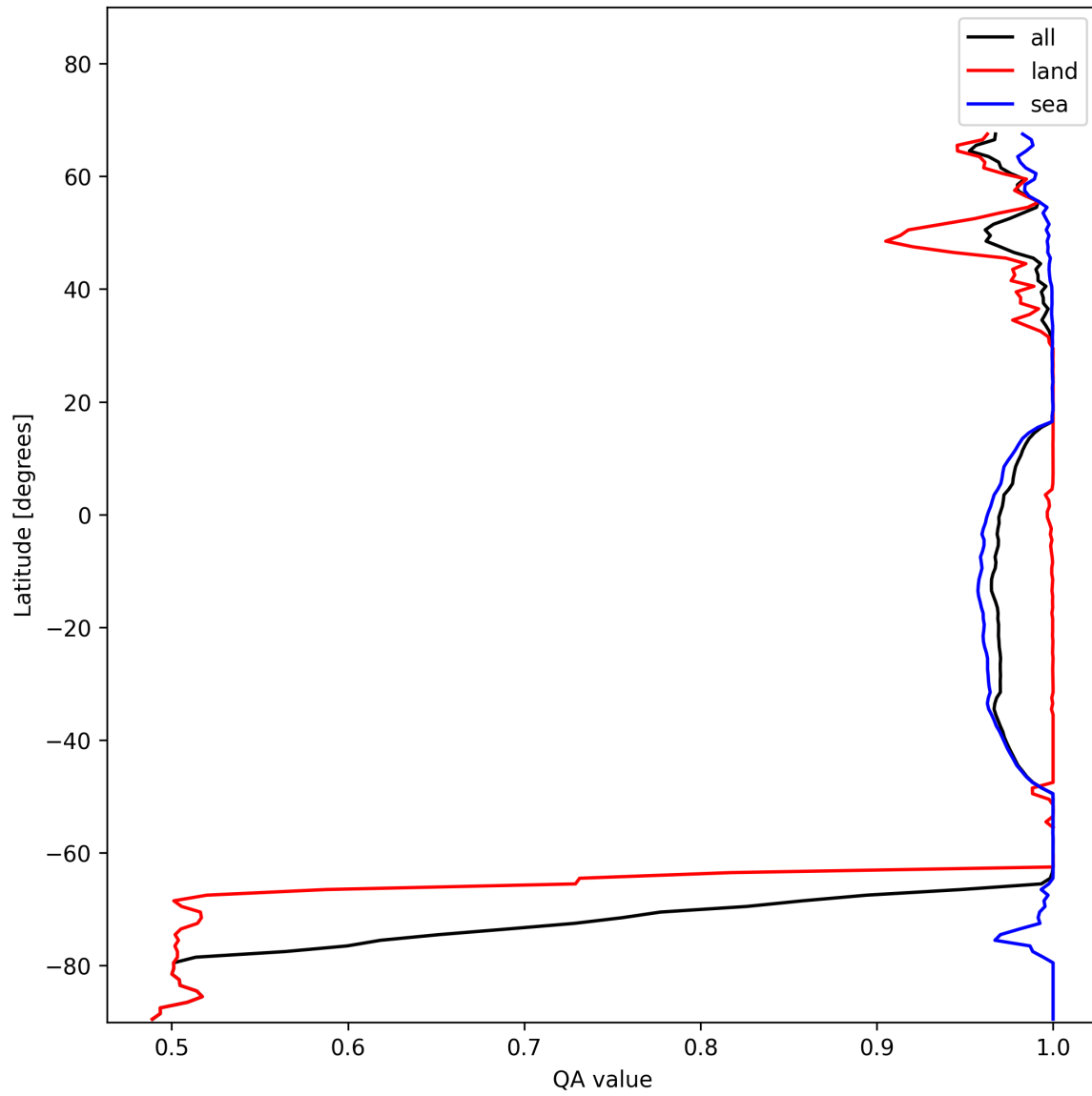
Figure 12: Zonal average of “QA value” for 2025-01-18 to 2025-01-20.
