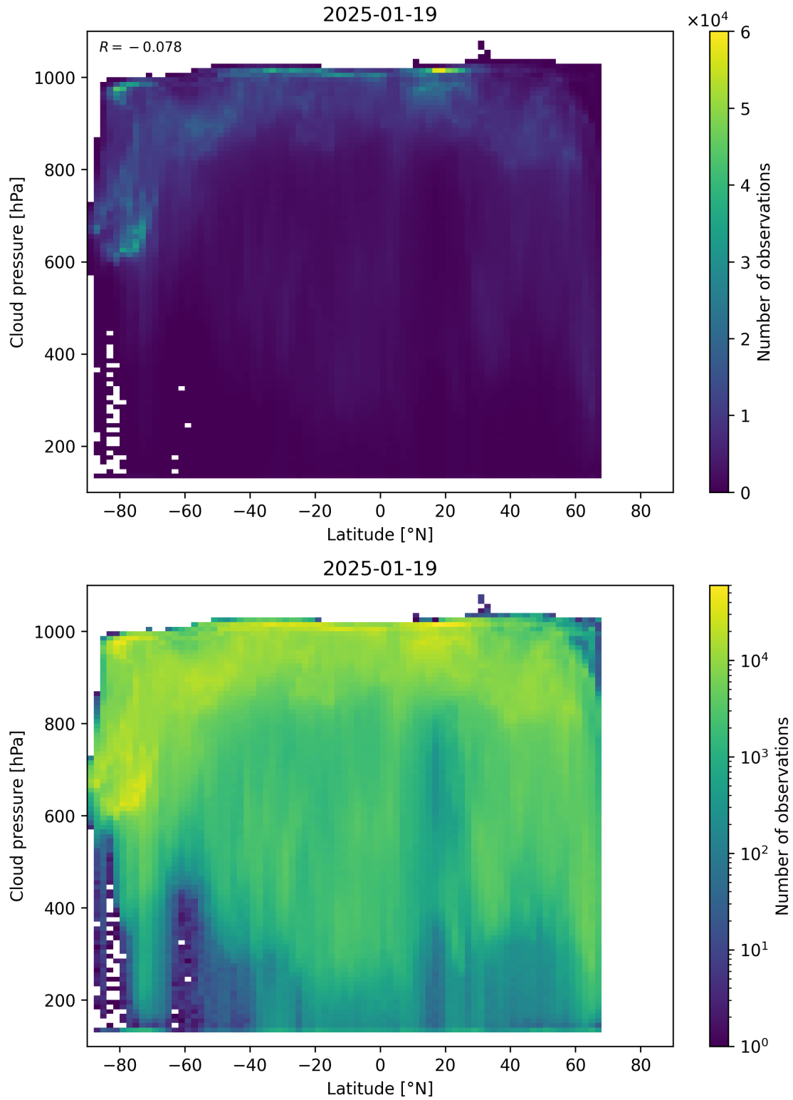
Figure 91: Scatter density plot of “Latitude” against “Cloud pressure” for 2025-01-18 to 2025-01-20.
