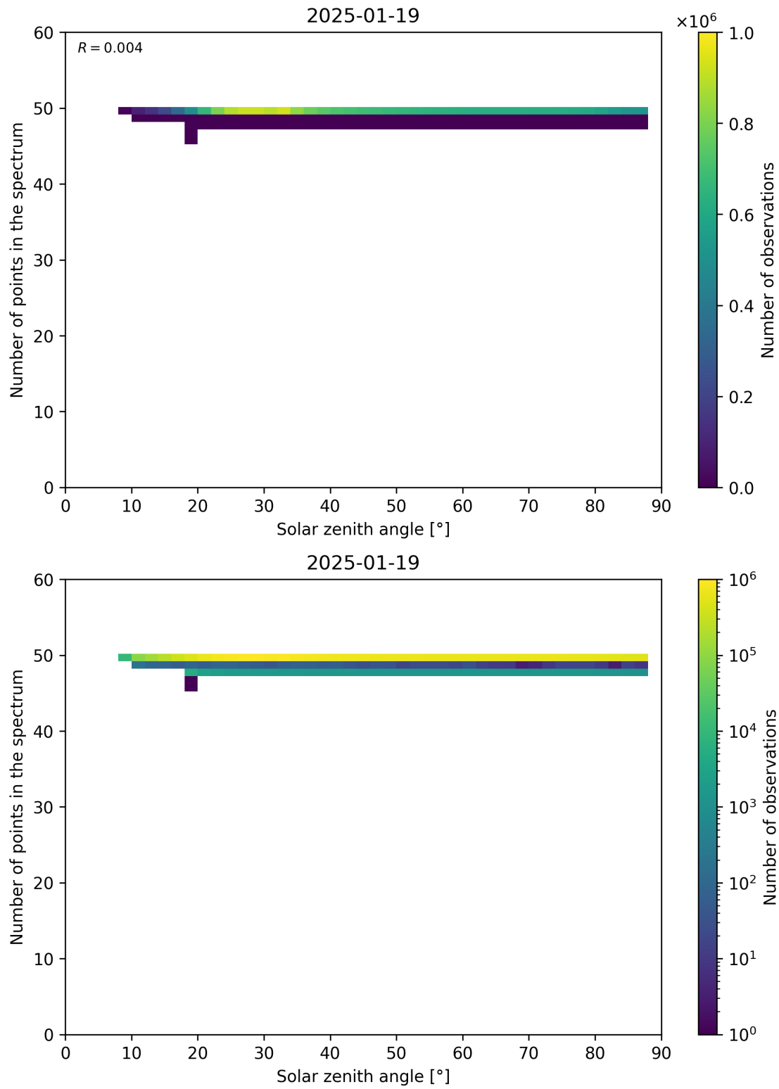
Figure 115: Scatter density plot of “Solar zenith angle” against “Number of points in the spectrum” for 2025-01-18 to 2025-01-20.
