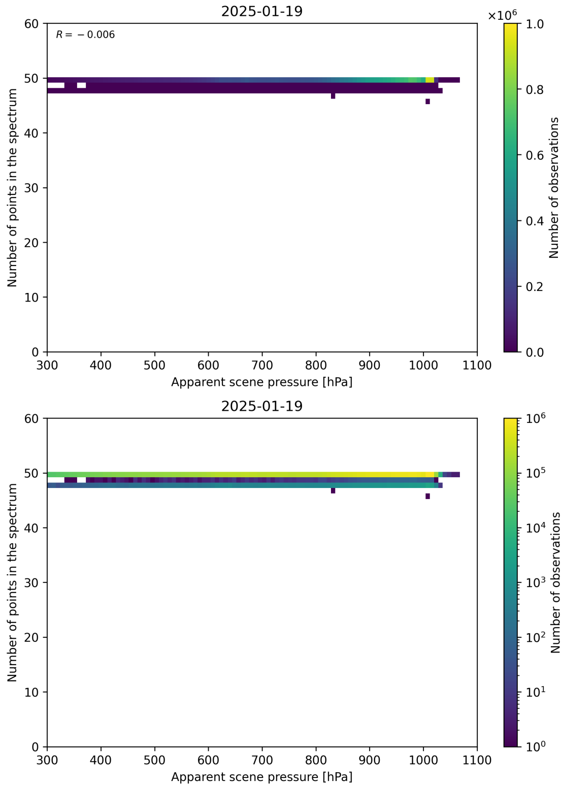
Figure 66: Scatter density plot of “Apparent scene pressure” against “Number of points in the spectrum” for 2025-01-18 to 2025-01-20.
