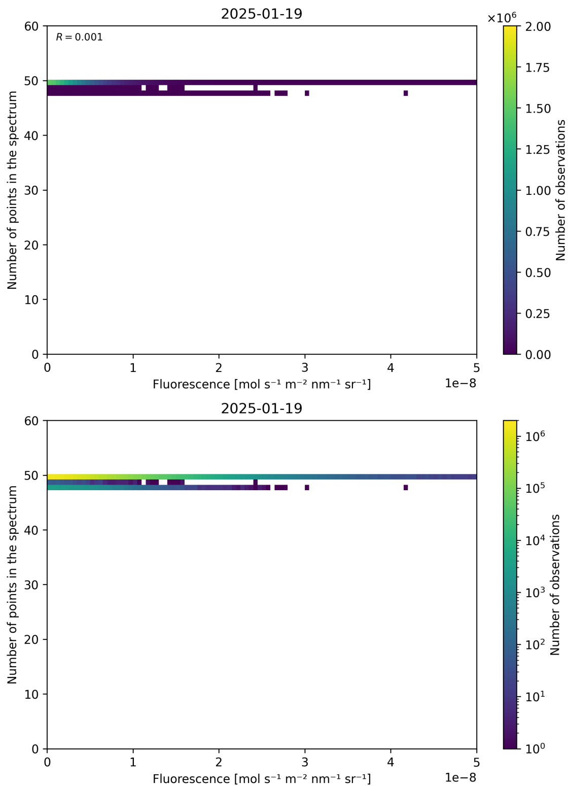
Figure 86: Scatter density plot of “Fluorescence” against “Number of points in the spectrum” for 2025-01-18 to 2025-01-20.
