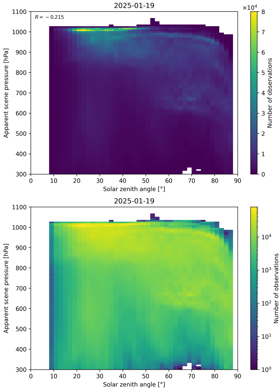
Figure 108: Scatter density plot of “Solar zenith angle” against “Apparent scene pressure” for 2025-01-18 to 2025-01-20.
