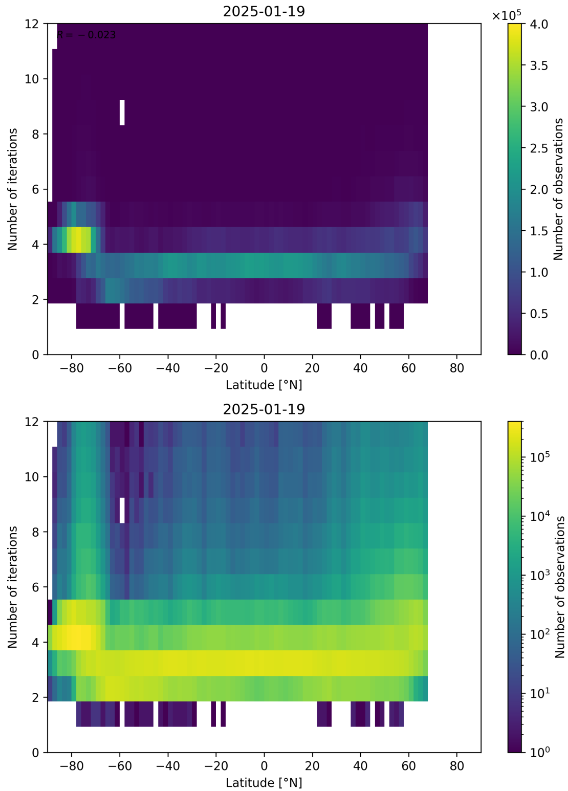
Figure 93: Scatter density plot of “Latitude” against “Number of iterations” for 2025-01-18 to 2025-01-20.
