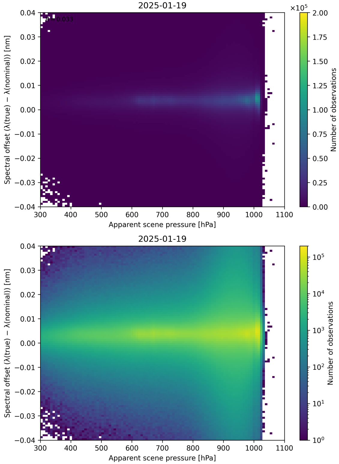
Figure 67: Scatter density plot of “Apparent scene pressure” against “Spectral offset ( \lambda_{\text{true}} - \lambda_{\text{nominal}} )” for 2025-01-18 to 2025-01-20.
