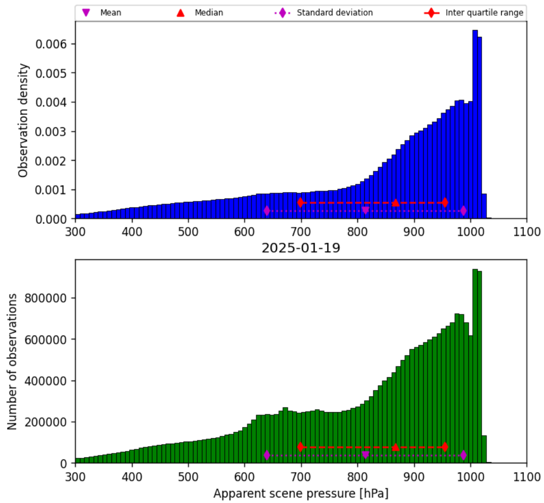
Figure 36: Histogram of “Apparent scene pressure” for 2025-01-18 to 2025-01-20
