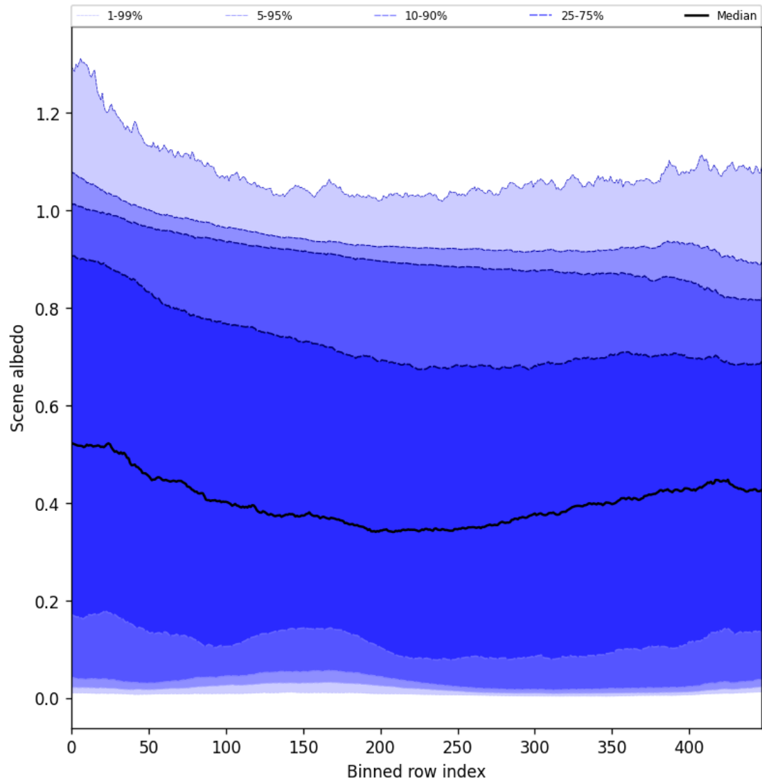
Figure 51: Along track statistics of “Scene albedo” for 2025-01-18 to 2025-01-20
