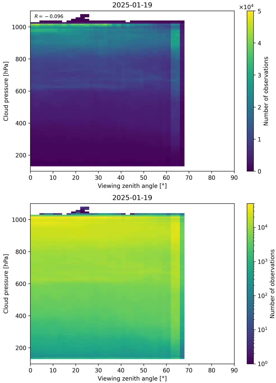
Figure 121: Scatter density plot of “Viewing zenith angle” against “Cloud pressure” for 2025-01-18 to 2025-01-20.
