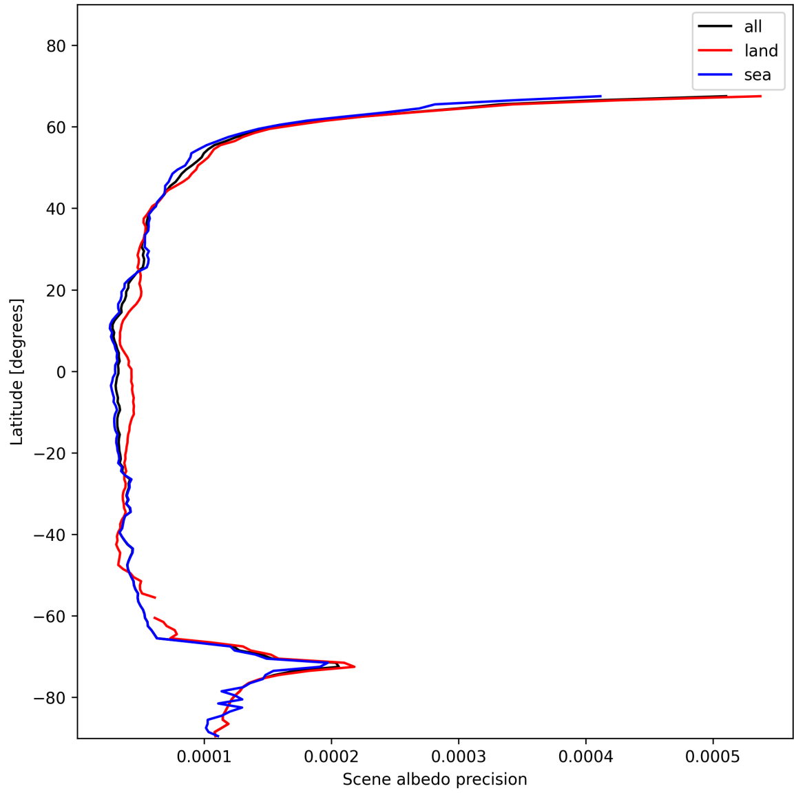
Figure 18: Zonal average of “Scene albedo precision” for 2025-01-18 to 2025-01-20.
