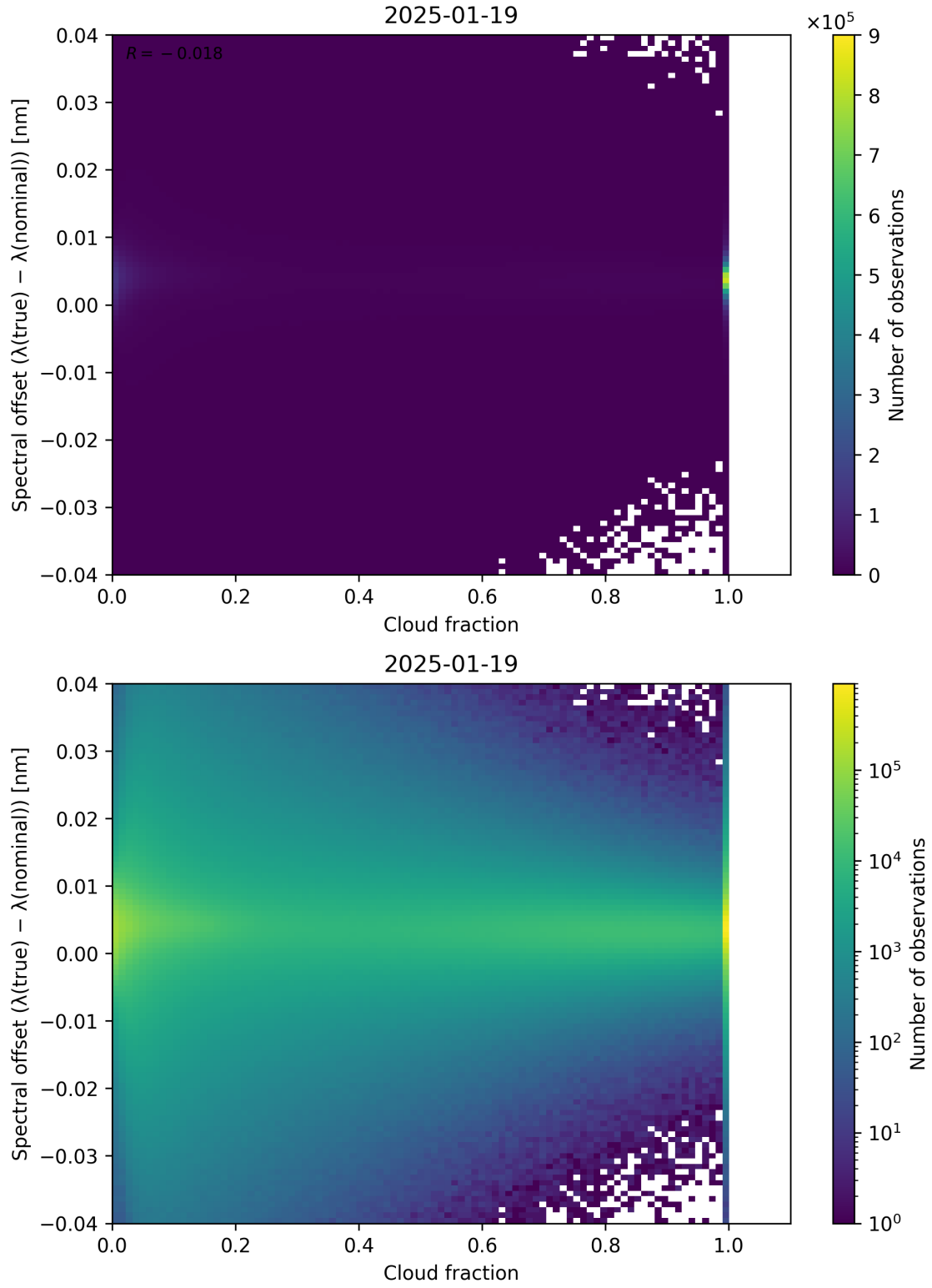
Figure 76: Scatter density plot of “Cloud fraction” against “Spectral offset ( \lambda_{\text{true}} - \lambda_{\text{nominal}} )” for 2025-01-18 to 2025-01-20.
