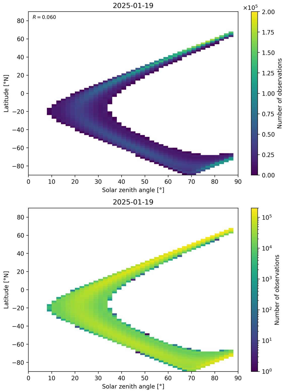
Figure 113: Scatter density plot of “Solar zenith angle” against “Latitude” for 2025-01-18 to 2025-01-20.
