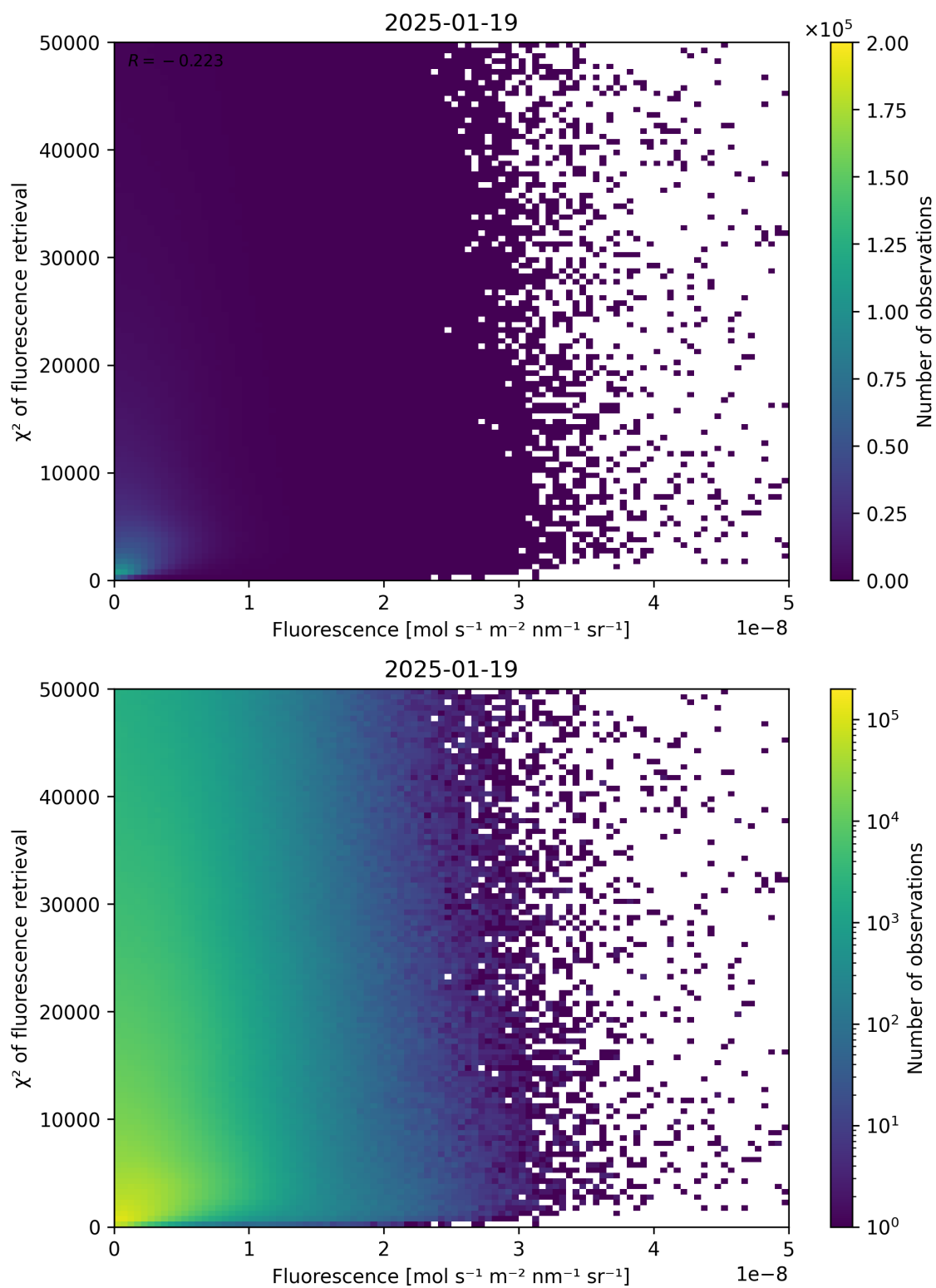
Figure 85: Scatter density plot of “Fluorescence” against “ \chi^2 of fluorescence retrieval” for 2025-01-18 to 2025-01-20.
