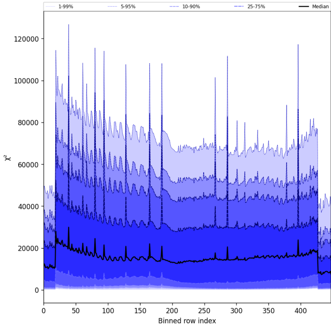
Figure 55: Along track statistics of “ \chi^2 ” for 2025-01-18 to 2025-01-20
