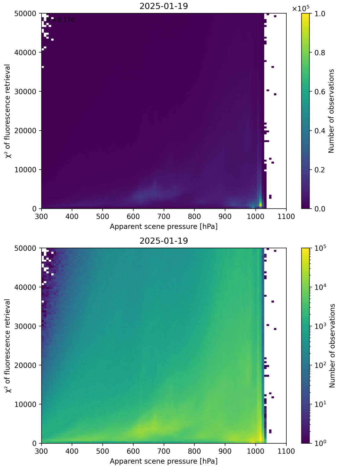
Figure 63: Scatter density plot of “Apparent scene pressure” against “ \chi^2 of fluorescence retrieval” for 2025-01-18 to 2025-01-20.
