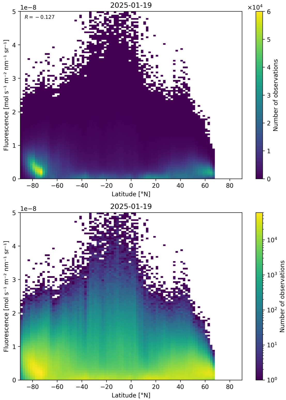
Figure 92: Scatter density plot of “Latitude” against “Fluorescence” for 2025-01-18 to 2025-01-20.
