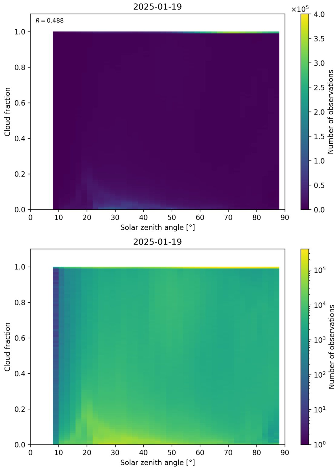
Figure 110: Scatter density plot of “Solar zenith angle” against “Cloud fraction” for 2025-01-18 to 2025-01-20.
