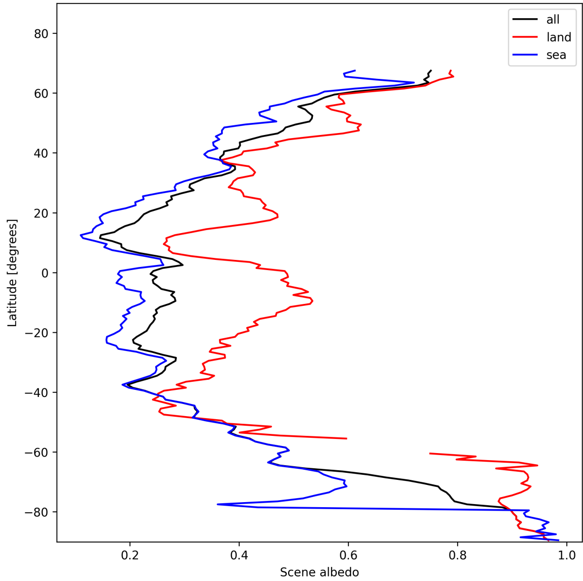
Figure 17: Zonal average of “Scene albedo” for 2025-01-18 to 2025-01-20.
