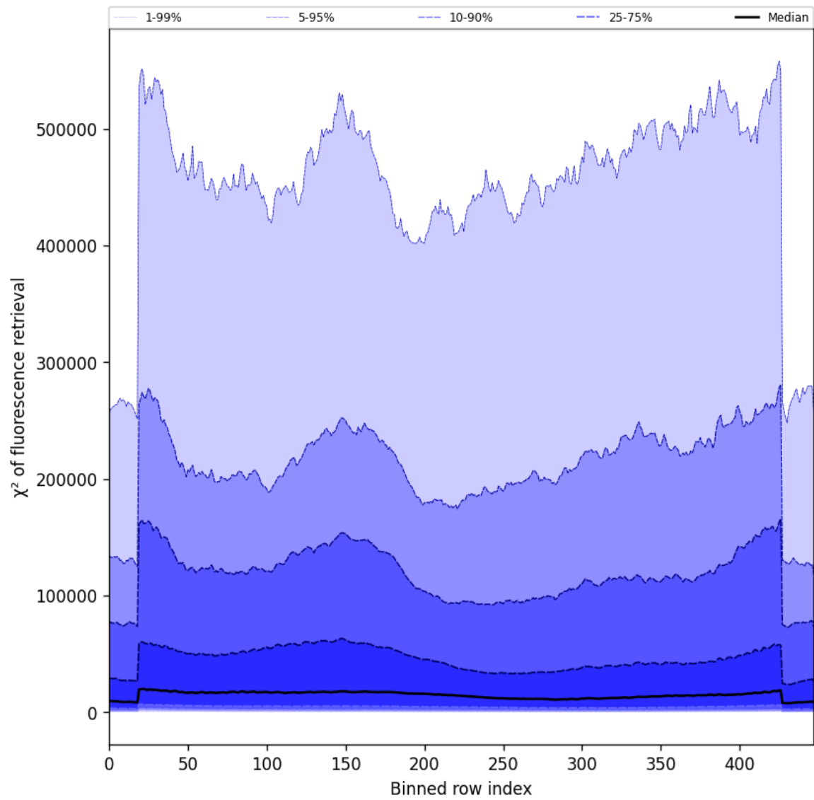
Figure 59: Along track statistics of “ \chi^2 of fluorescence retrieval” for 2025-01-18 to 2025-01-20
