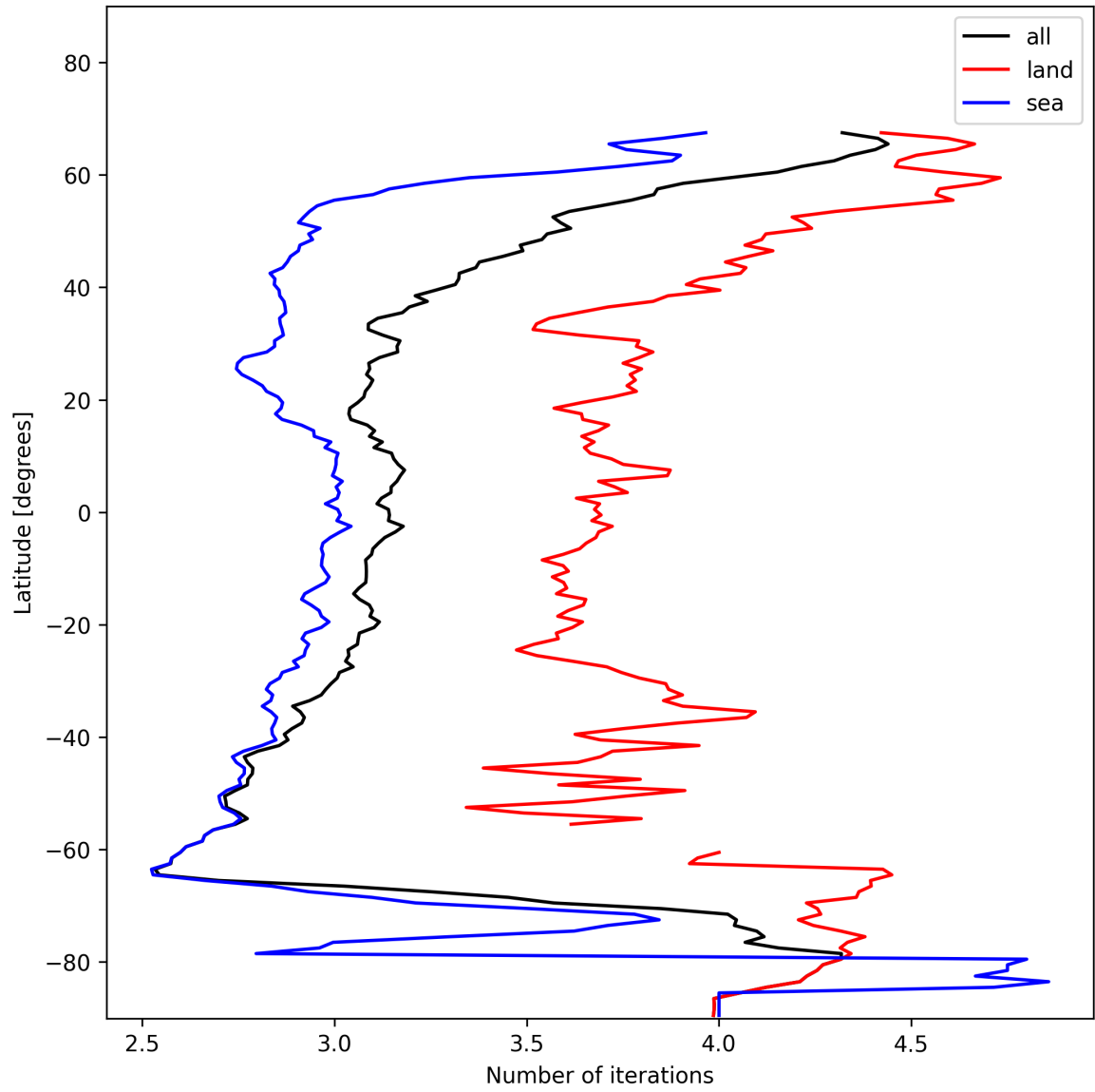
Figure 22: Zonal average of “Number of iterations” for 2025-01-18 to 2025-01-20.
