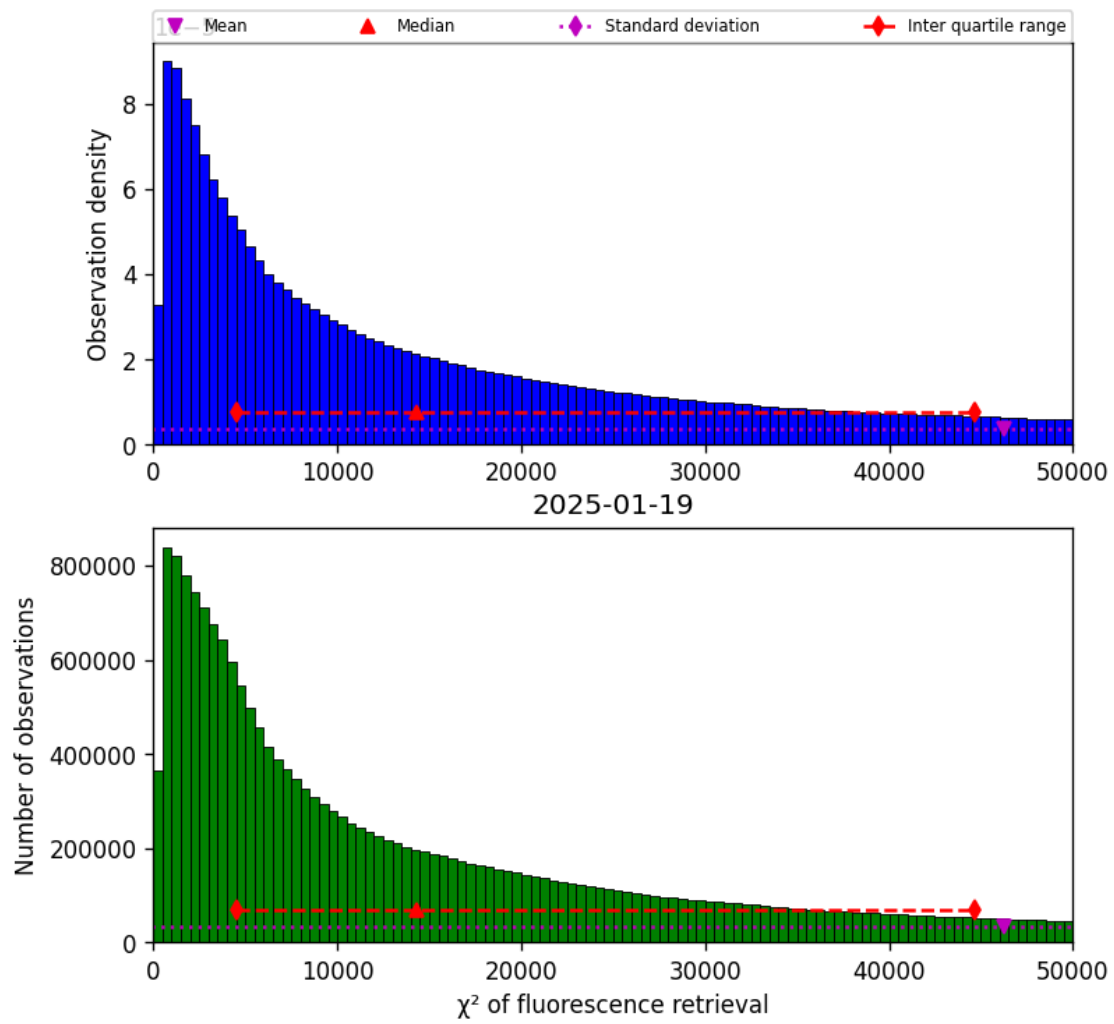
Figure 42: Histogram of “ \chi^2 of fluorescence retrieval” for 2025-01-18 to 2025-01-20
