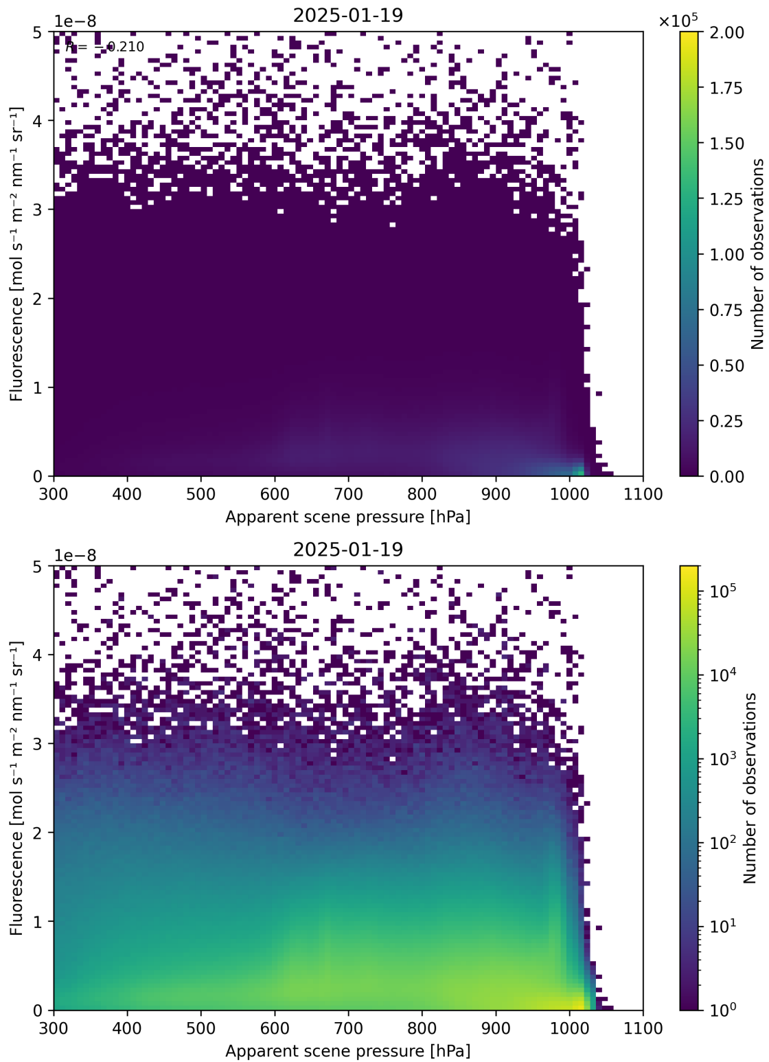
Figure 64: Scatter density plot of “Apparent scene pressure” against “Fluorescence” for 2025-01-18 to 2025-01-20.
