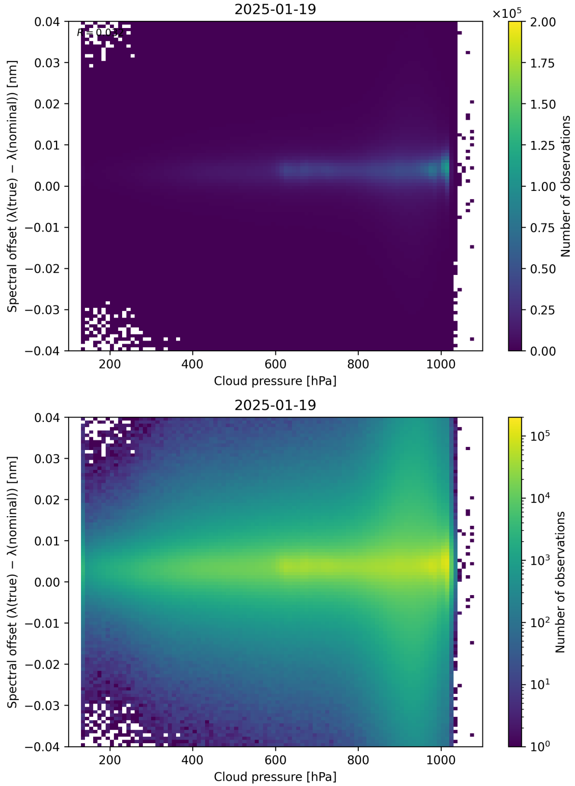
Figure 84: Scatter density plot of “Cloud pressure” against “Spectral offset ( \lambda_{\text{true}} - \lambda_{\text{nominal}} )” for 2025-01-18 to 2025-01-20.
