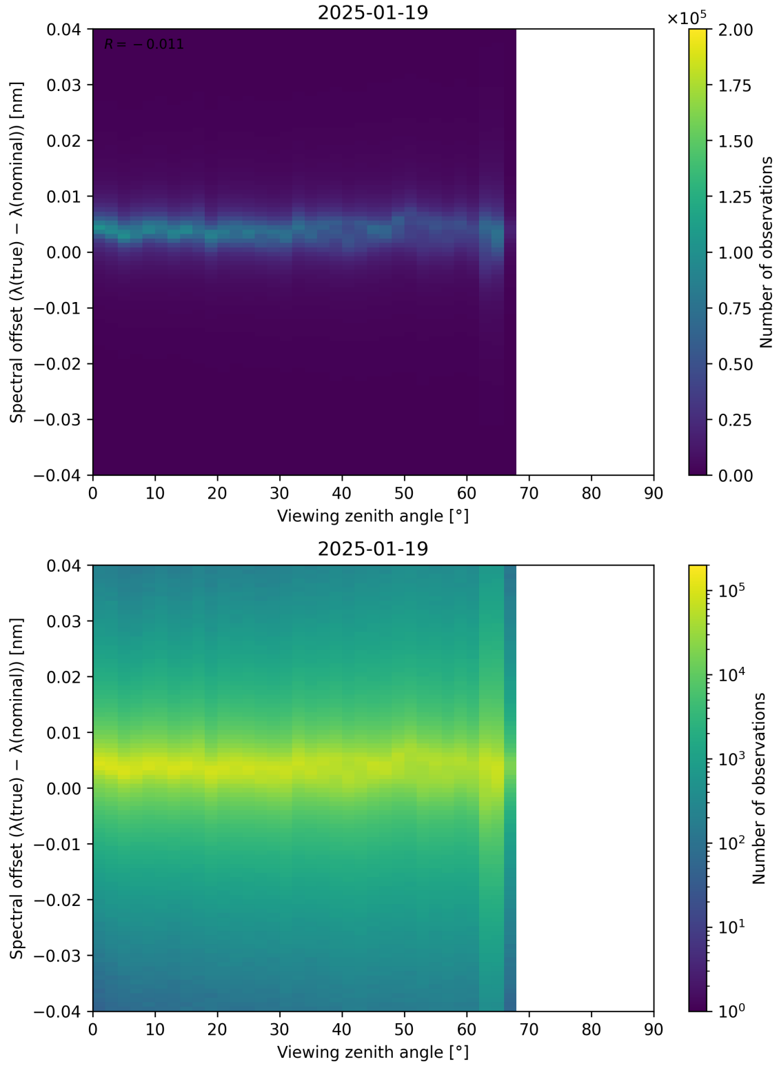
Figure 128: Scatter density plot of “Viewing zenith angle” against “Spectral offset ( \lambda_{\text{true}} - \lambda_{\text{nominal}} )” for 2025-01-18 to 2025-01-20.
