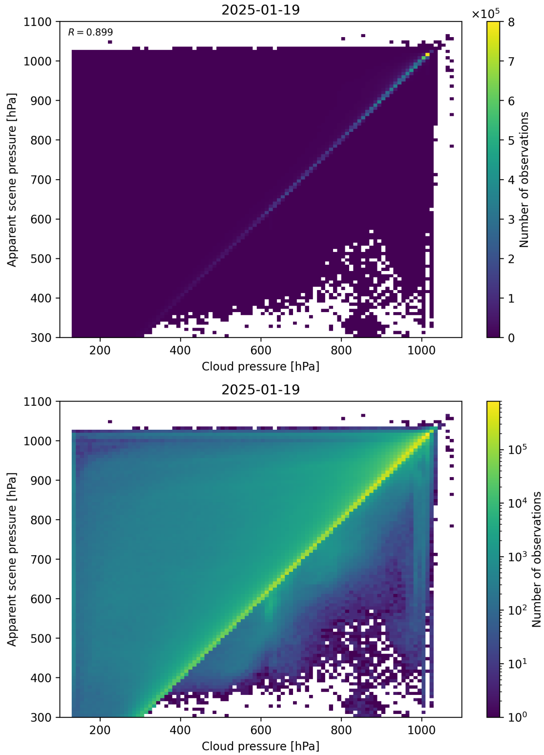
Figure 77: Scatter density plot of “Cloud pressure” against “Apparent scene pressure” for 2025-01-18 to 2025-01-20.
