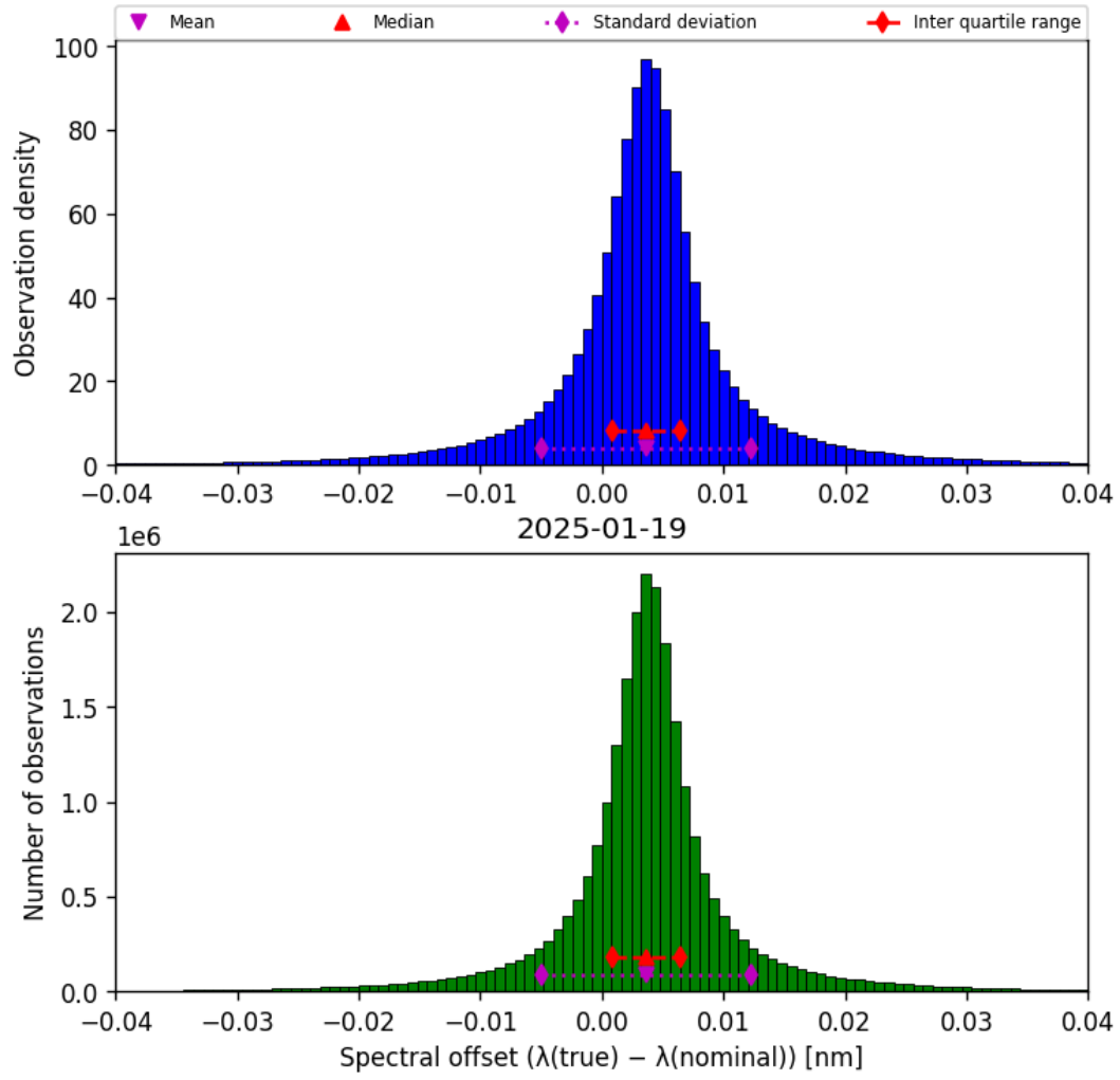
Figure 45: Histogram of “Spectral offset ( \lambda_{\text{true}} - \lambda_{\text{nominal}} )” for 2025-01-18 to 2025-01-20
