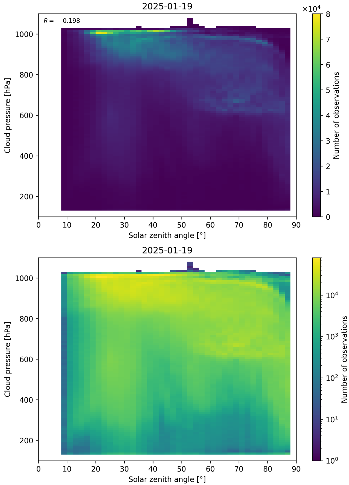
Figure 111: Scatter density plot of “Solar zenith angle” against “Cloud pressure” for 2025-01-18 to 2025-01-20.
