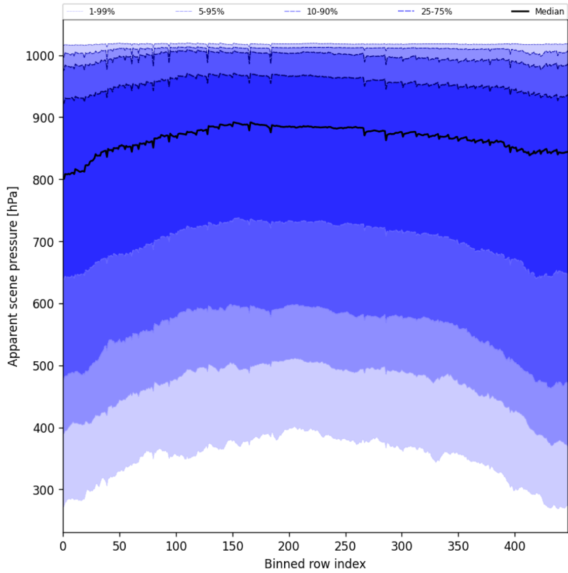
Figure 53: Along track statistics of “Apparent scene pressure” for 2025-01-18 to 2025-01-20
