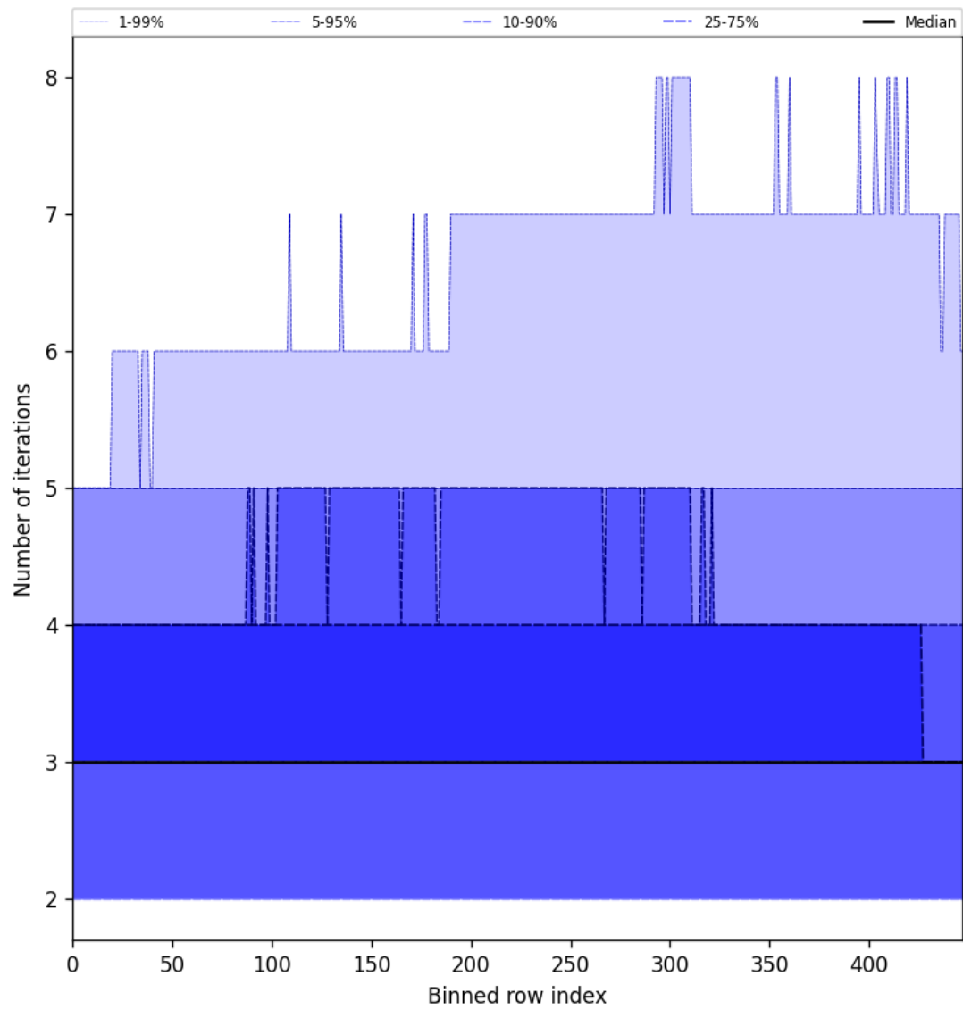
Figure 56: Along track statistics of “Number of iterations” for 2025-01-18 to 2025-01-20
