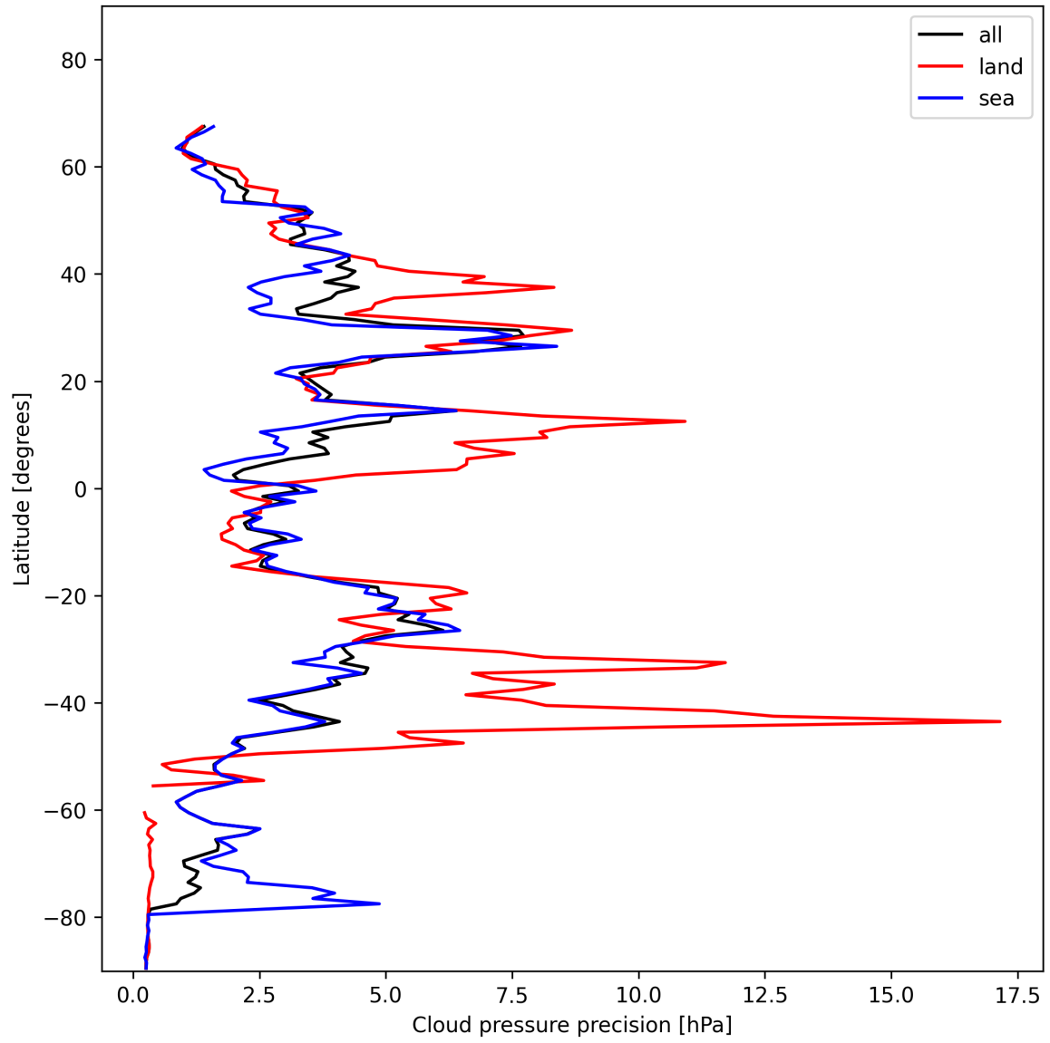
Figure 14: Zonal average of “Cloud pressure precision” for 2025-01-18 to 2025-01-20.
