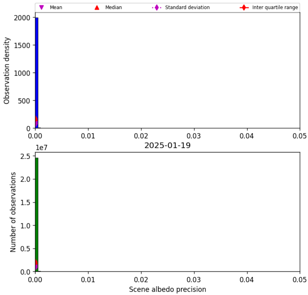
Figure 35: Histogram of “Scene albedo precision” for 2025-01-18 to 2025-01-20
