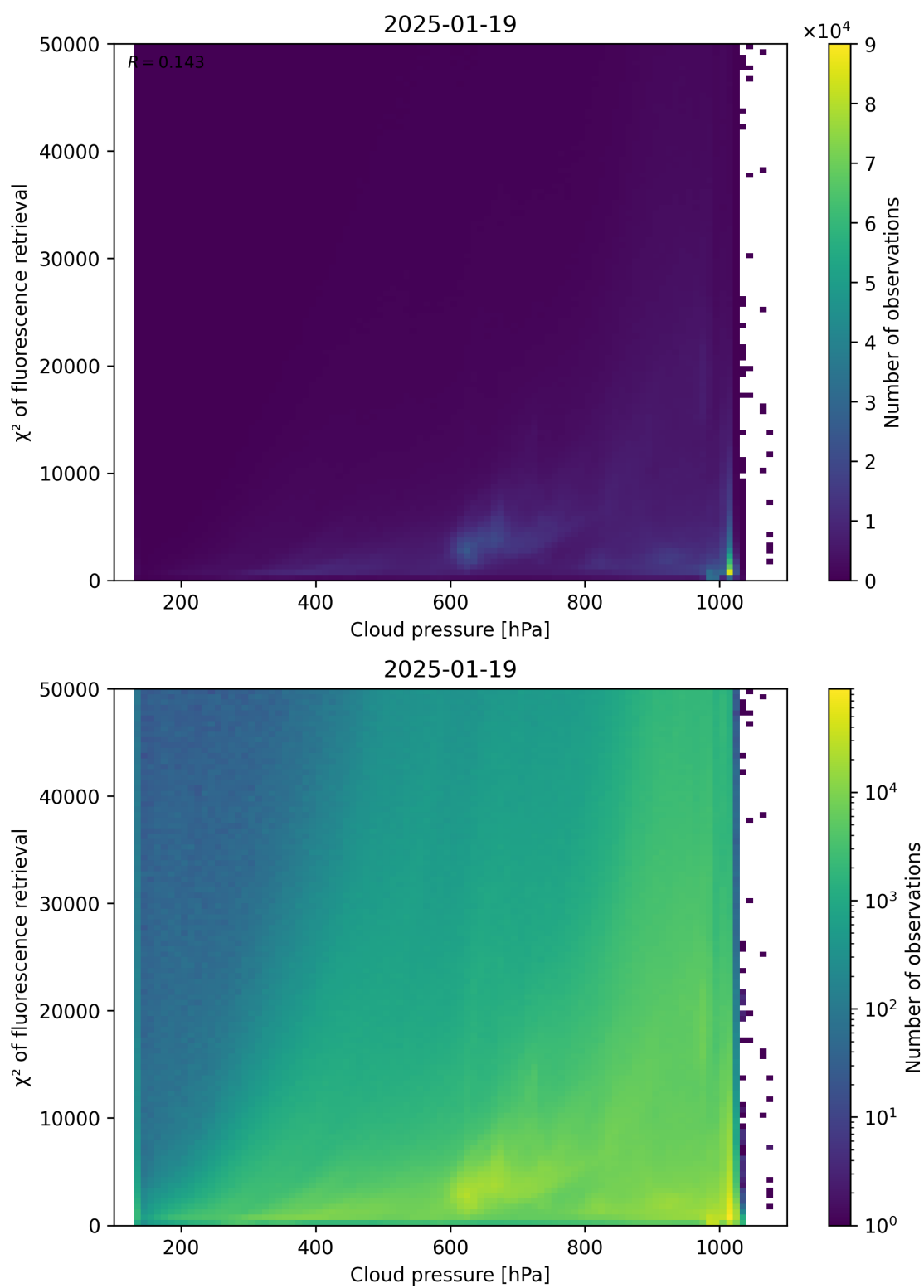
Figure 78: Scatter density plot of “Cloud pressure” against “ \chi^2 of fluorescence retrieval” for 2025-01-18 to 2025-01-20.
