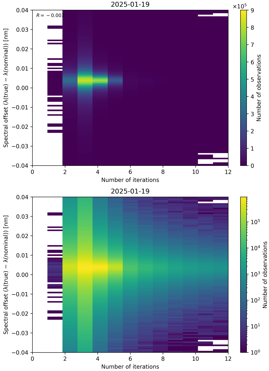
Figure 100: Scatter density plot of “Number of iterations” against “Spectral offset ( \lambda_{\text{true}} - \lambda_{\text{nominal}} )” for 2025-01-18 to 2025-01-20.
