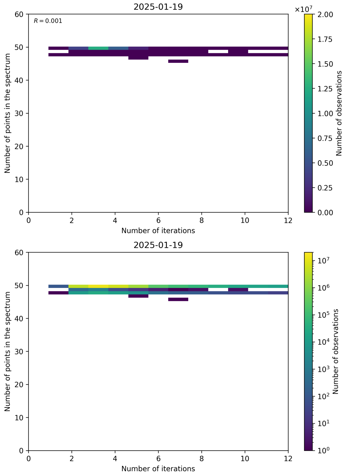
Figure 99: Scatter density plot of “Number of iterations” against “Number of points in the spectrum” for 2025-01-18 to 2025-01-20.
