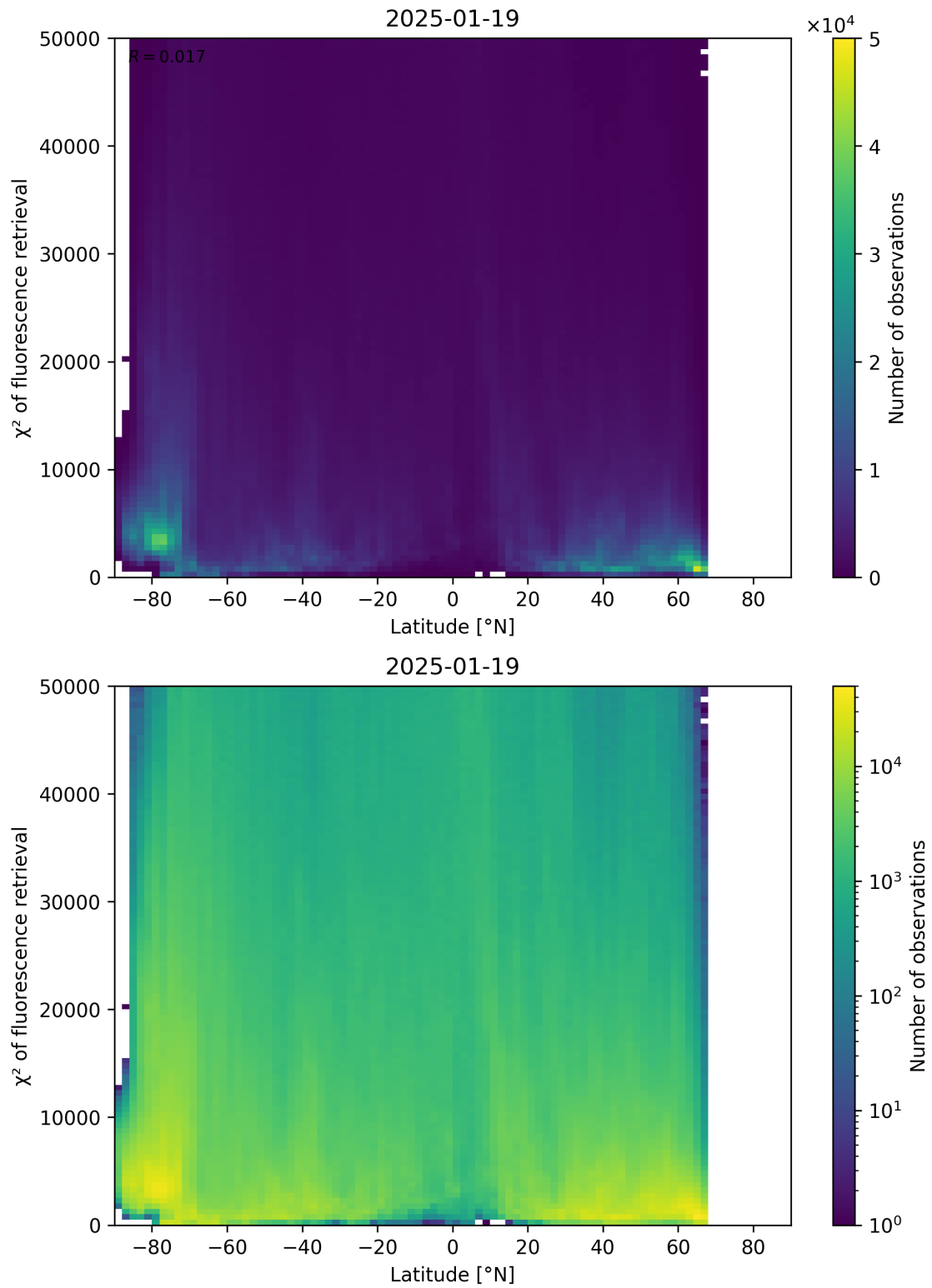
Figure 89: Scatter density plot of “Latitude” against “ \chi^2 of fluorescence retrieval” for 2025-01-18 to 2025-01-20.
