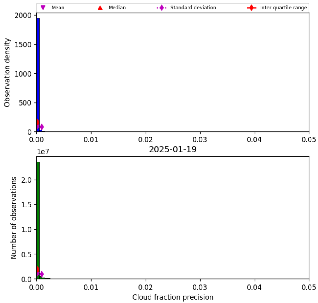
Figure 33: Histogram of “Cloud fraction precision” for 2025-01-18 to 2025-01-20
