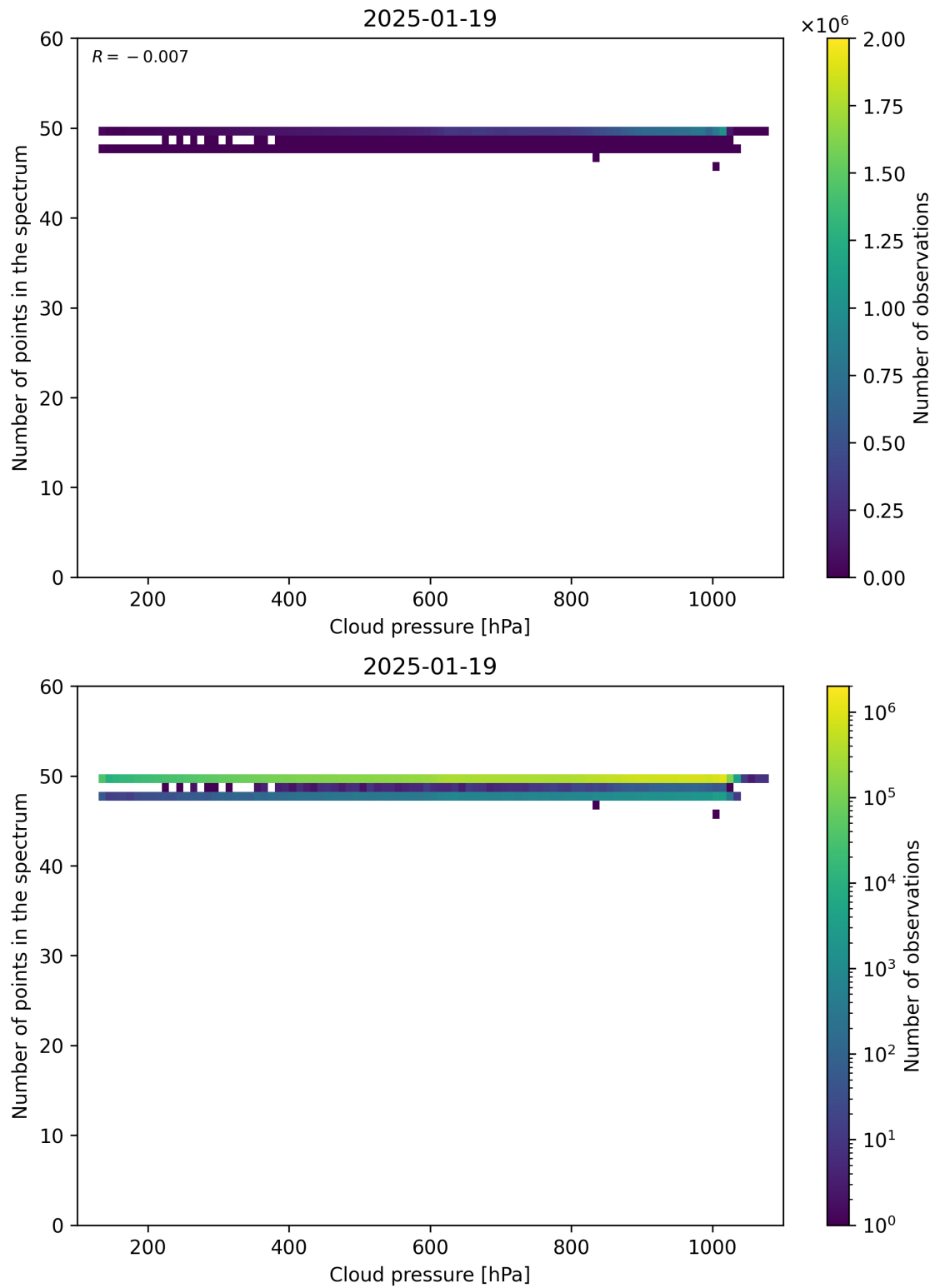
Figure 82: Scatter density plot of “Cloud pressure” against “Number of points in the spectrum” for 2025-01-18 to 2025-01-20.
