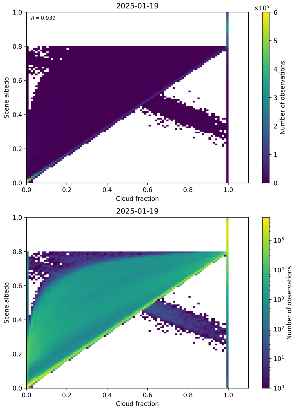
Figure 75: Scatter density plot of “Cloud fraction” against “Scene albedo” for 2025-01-18 to 2025-01-20.
