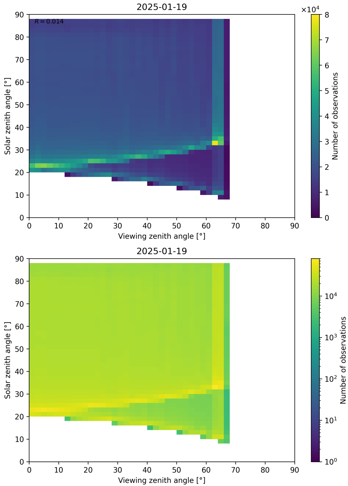
Figure 127: Scatter density plot of “Viewing zenith angle” against “Solar zenith angle” for 2025-01-18 to 2025-01-20.
