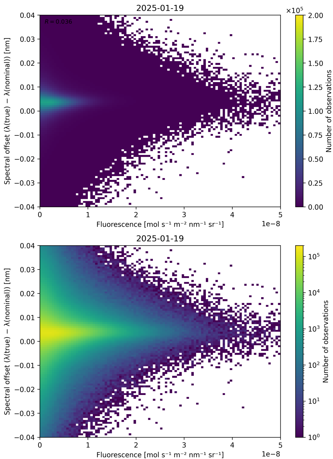
Figure 87: Scatter density plot of “Fluorescence” against “Spectral offset ( \lambda_{\text{true}} - \lambda_{\text{nominal}} )” for 2025-01-18 to 2025-01-20.
