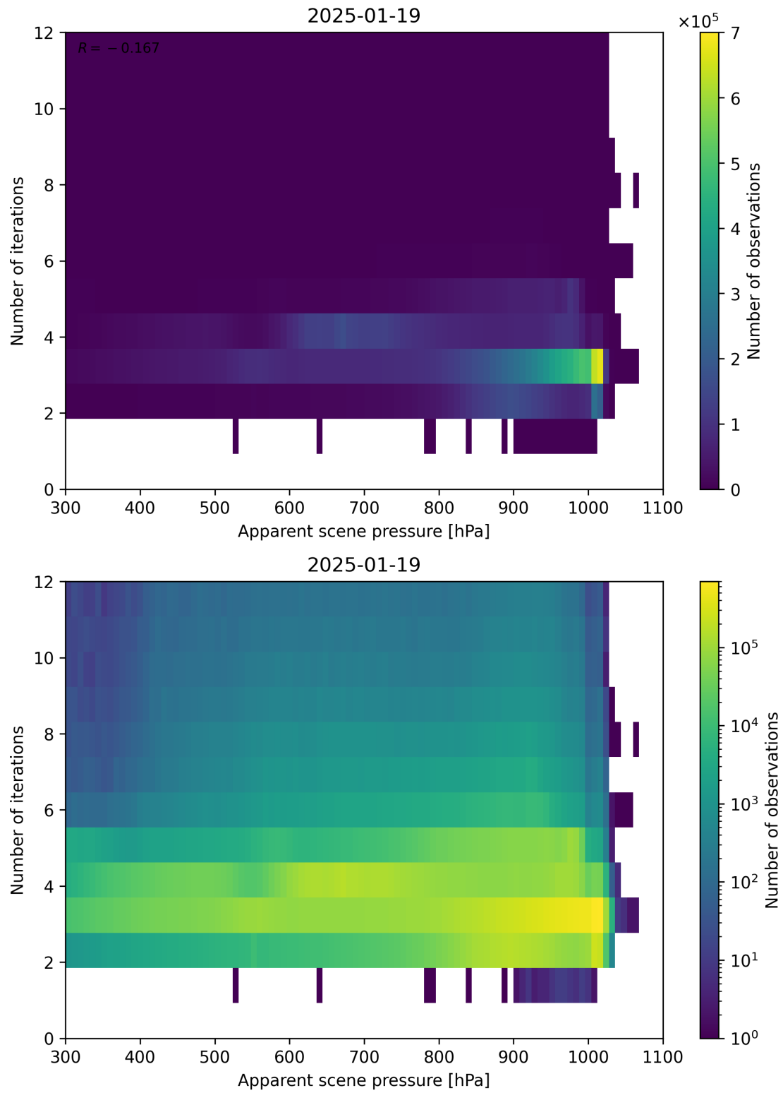
Figure 65: Scatter density plot of “Apparent scene pressure” against “Number of iterations” for 2025-01-18 to 2025-01-20.
