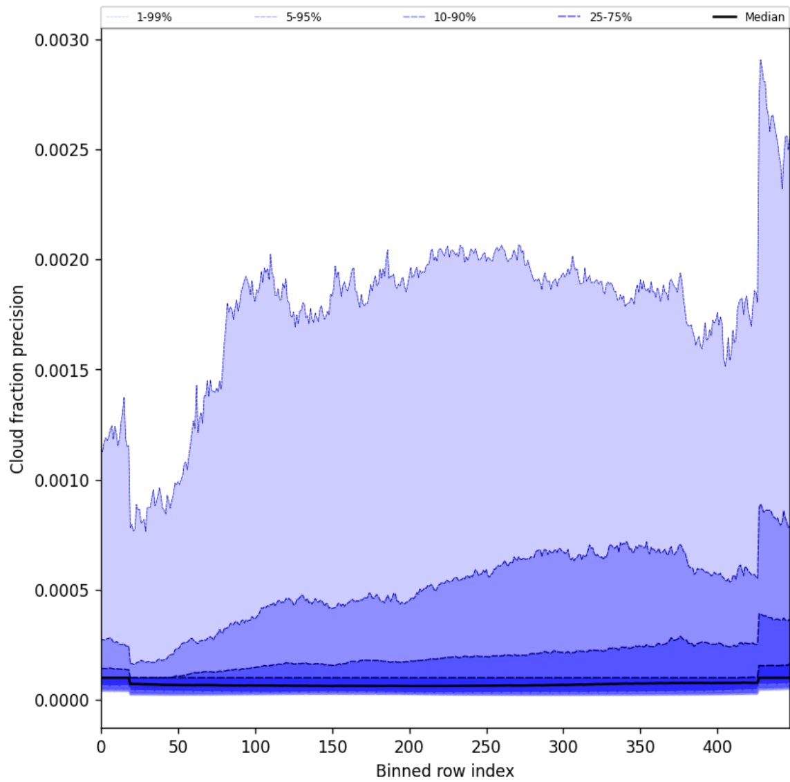
Figure 50: Along track statistics of “Cloud fraction precision” for 2025-01-18 to 2025-01-20
