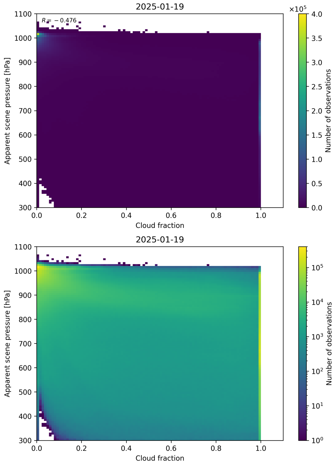
Figure 70: Scatter density plot of “Cloud fraction” against “Apparent scene pressure” for 2025-01-18 to 2025-01-20.
