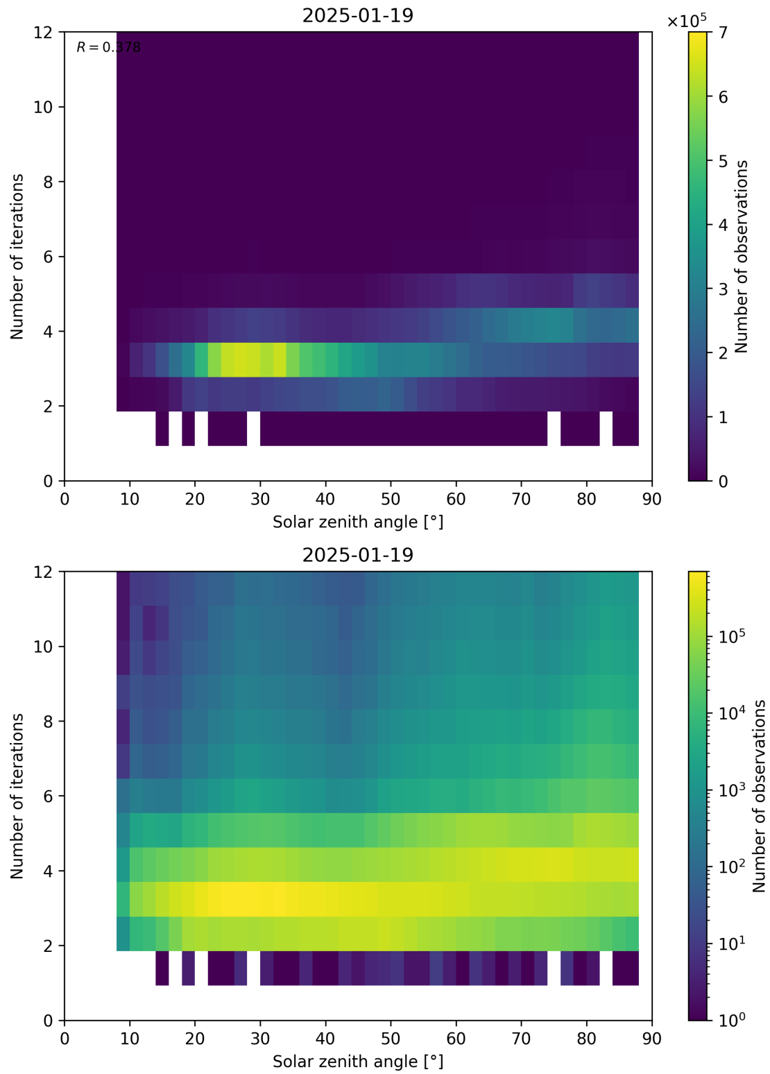
Figure 114: Scatter density plot of “Solar zenith angle” against “Number of iterations” for 2025-01-18 to 2025-01-20.
