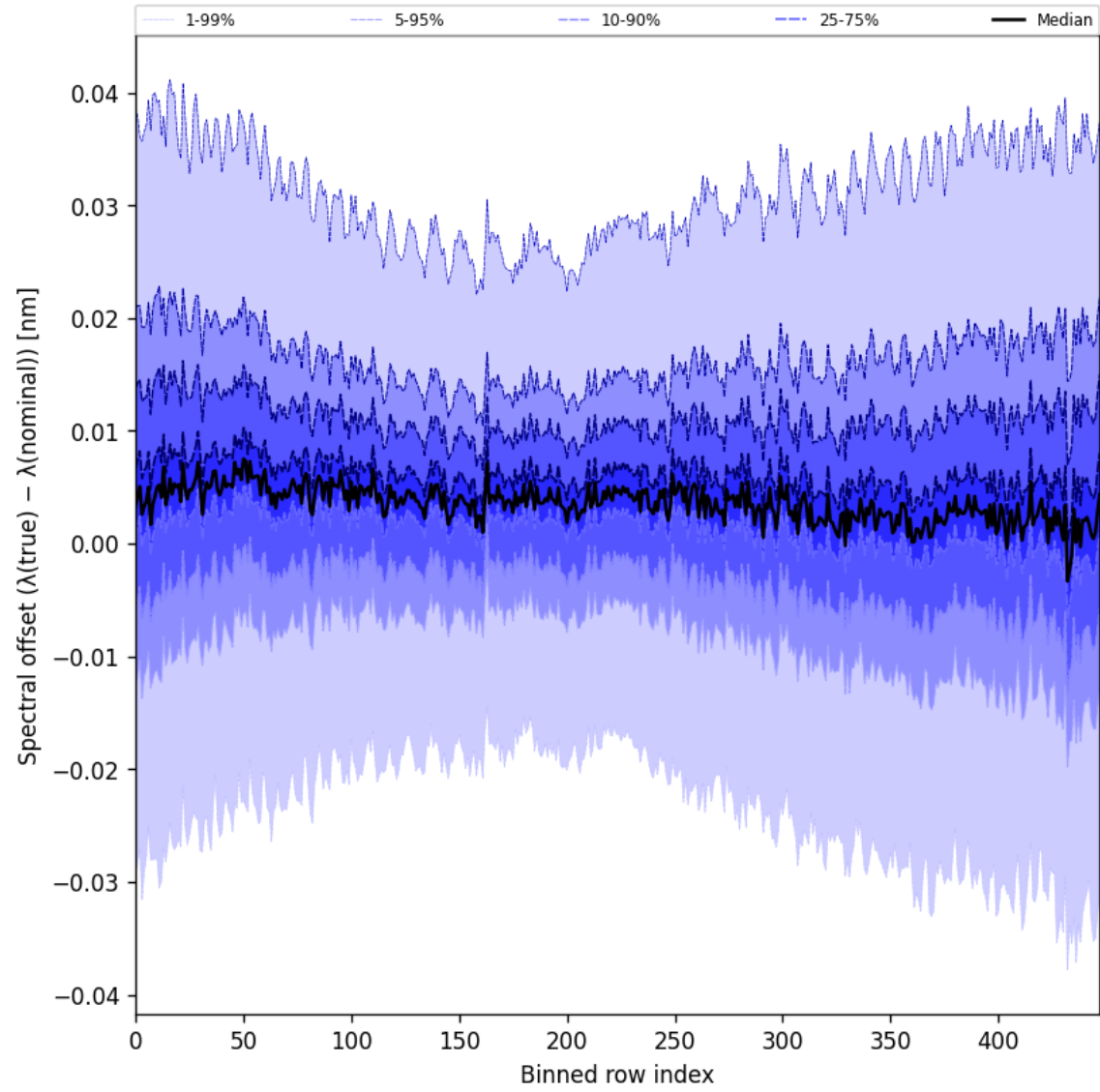
Figure 62: Along track statistics of “Spectral offset ( \lambda_{\text{true}} - \lambda_{\text{nominal}} )” for 2025-01-18 to 2025-01-20
