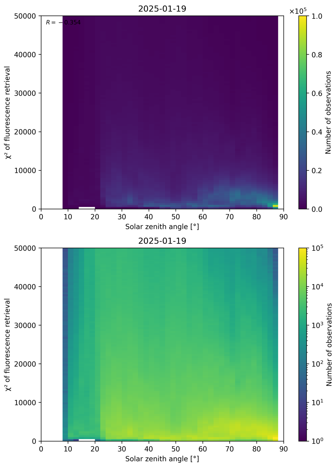
Figure 109: Scatter density plot of “Solar zenith angle” against “ \chi^2 of fluorescence retrieval” for 2025-01-18 to 2025-01-20.
