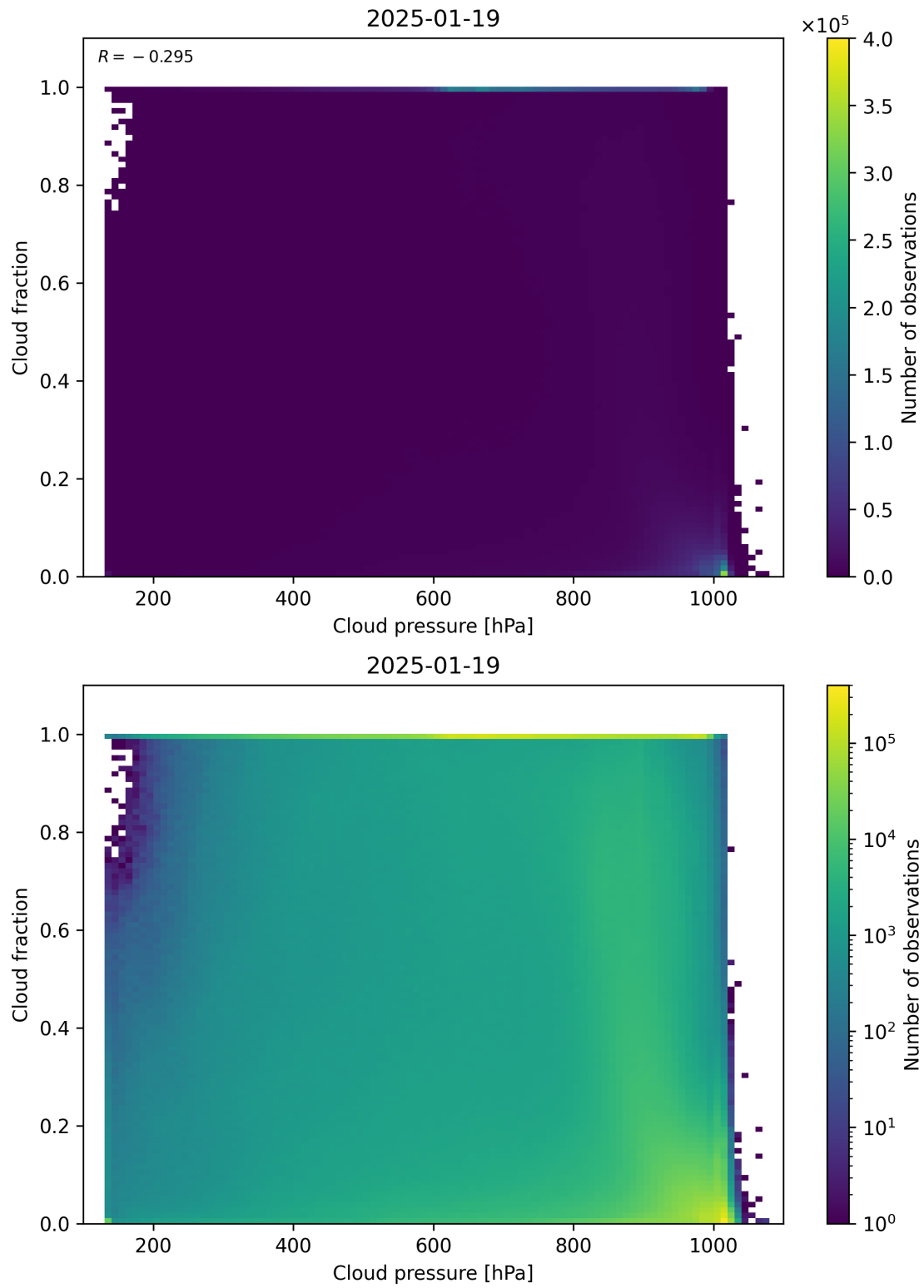
Figure 79: Scatter density plot of “Cloud pressure” against “Cloud fraction” for 2025-01-18 to 2025-01-20.
