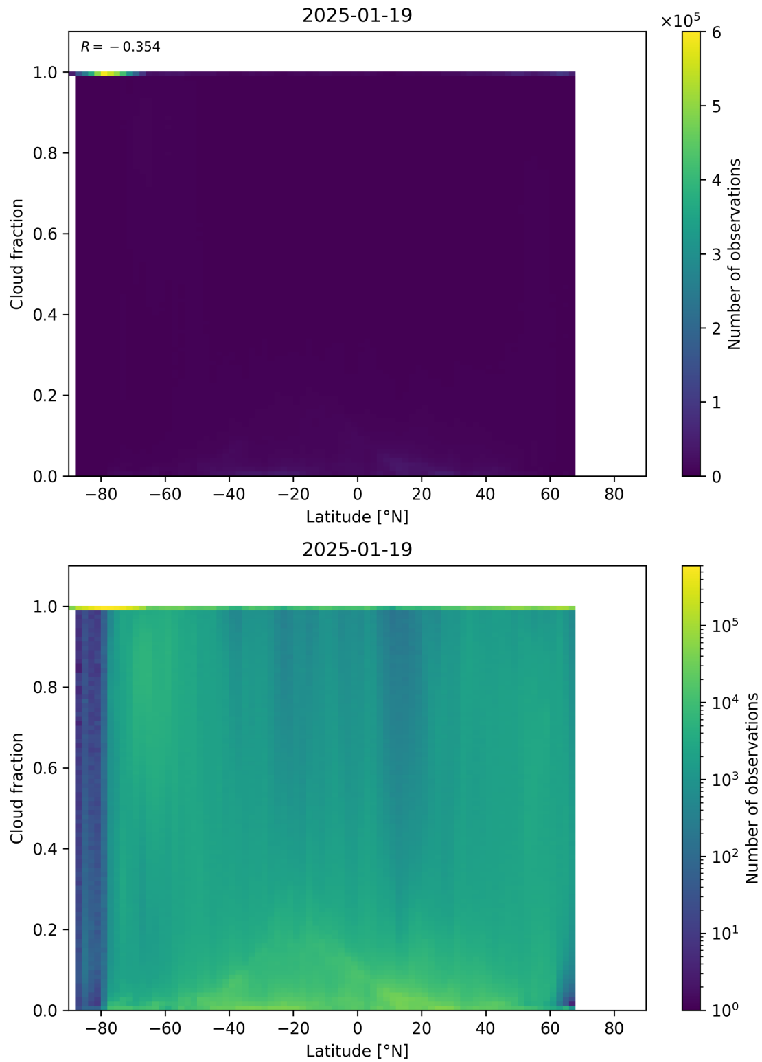
Figure 90: Scatter density plot of “Latitude” against “Cloud fraction” for 2025-01-18 to 2025-01-20.
