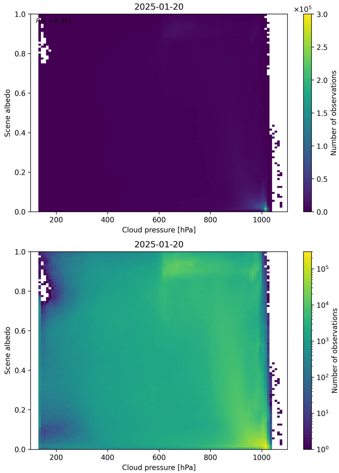
Figure 83: Scatter density plot of “Cloud pressure” against “Scene albedo” for 2025-01-19 to 2025-01-21.
