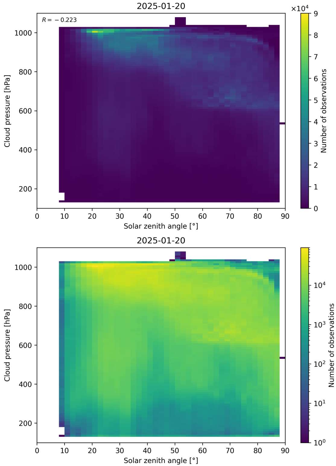
Figure 111: Scatter density plot of “Solar zenith angle” against “Cloud pressure” for 2025-01-19 to 2025-01-21.
