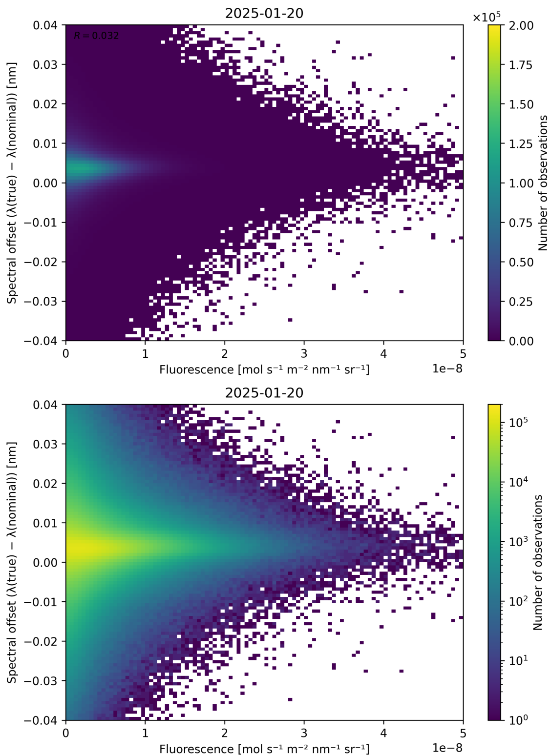
Figure 87: Scatter density plot of “Fluorescence” against “Spectral offset ( \lambda_{\text{true}} - \lambda_{\text{nominal}} )” for 2025-01-19 to 2025-01-21.
