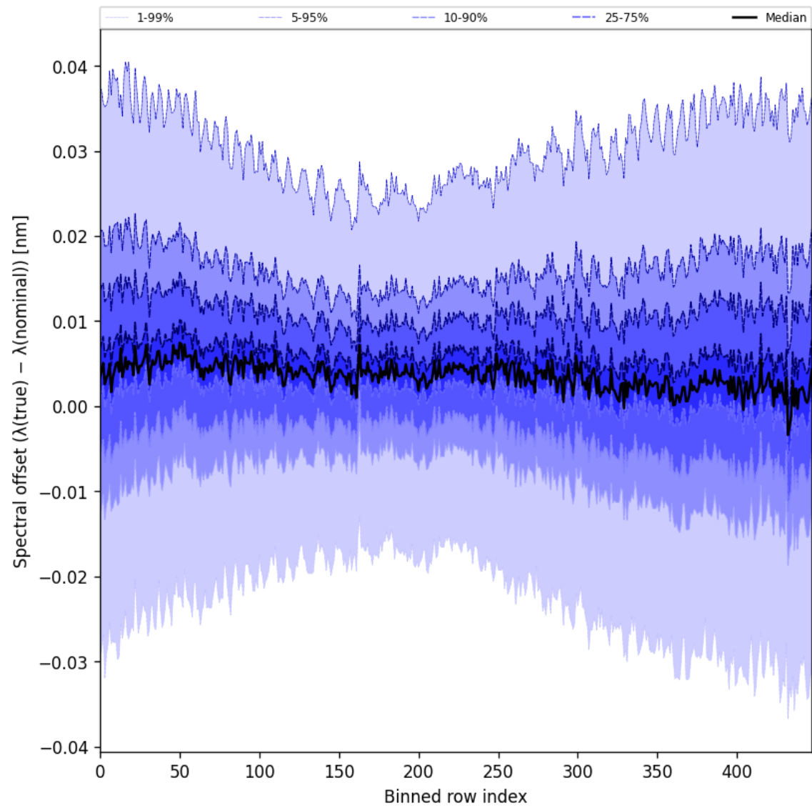
Figure 62: Along track statistics of “Spectral offset ( \lambda_{\text{true}} - \lambda_{\text{nominal}} )” for 2025-01-19 to 2025-01-21
