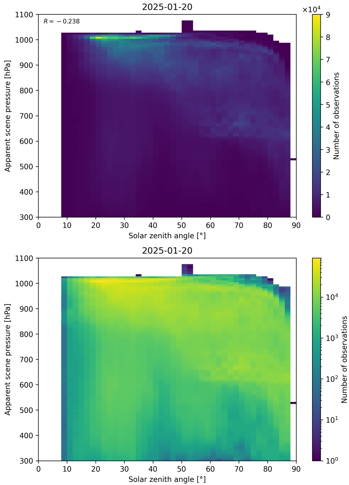
Figure 108: Scatter density plot of “Solar zenith angle” against “Apparent scene pressure” for 2025-01-19 to 2025-01-21.
