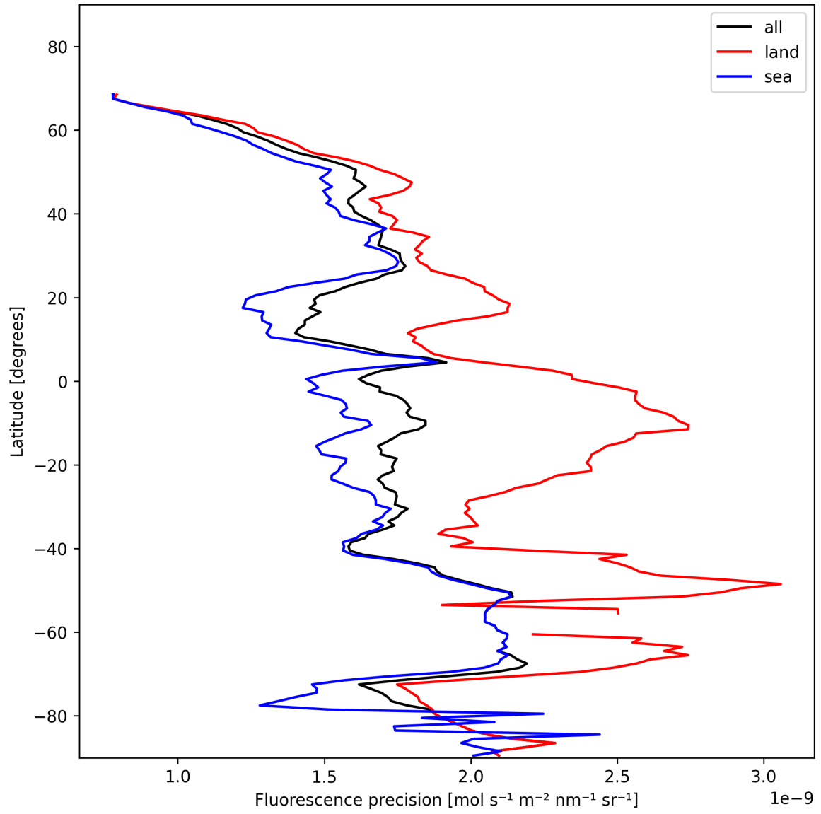
Figure 24: Zonal average of “Fluorescence precision” for 2025-01-19 to 2025-01-21.
