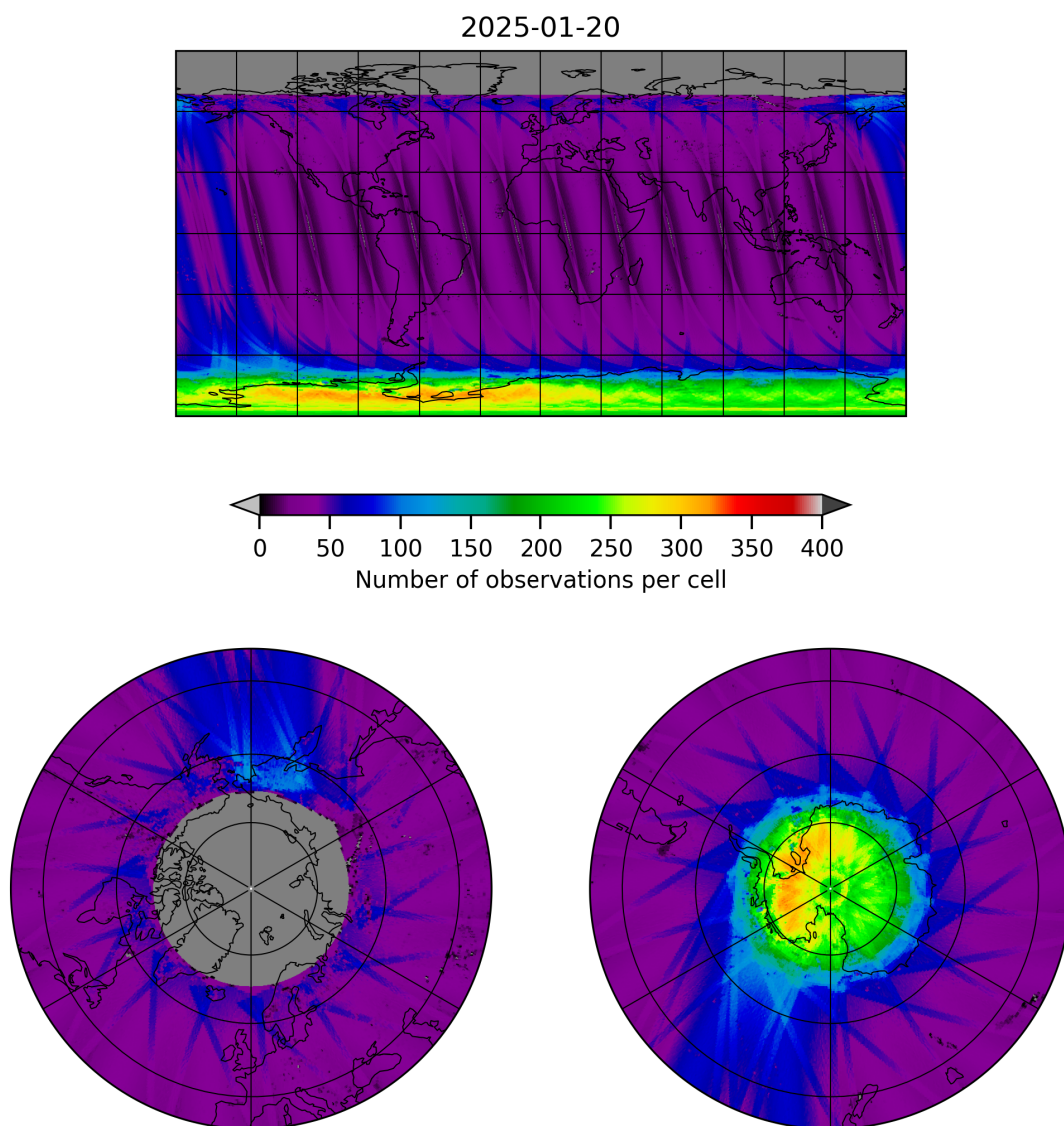
Figure 11: Map of the number of observations for 2025-01-19 to 2025-01-21
