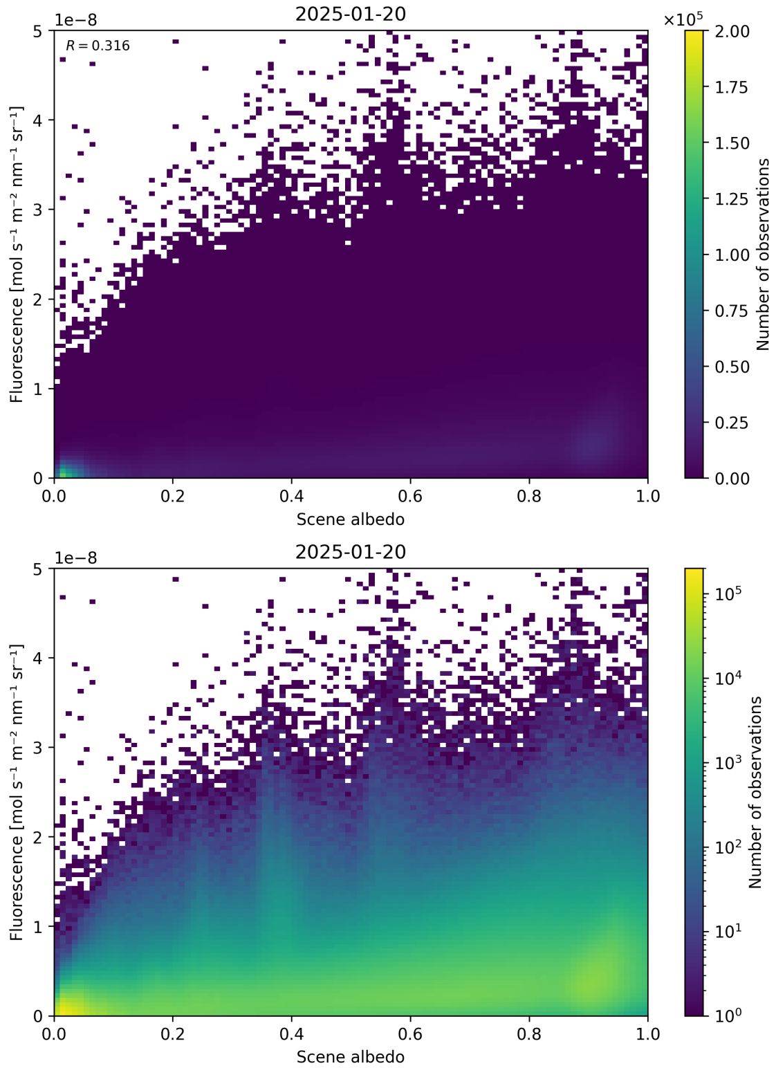
Figure 104: Scatter density plot of “Scene albedo” against “Fluorescence” for 2025-01-19 to 2025-01-21.
