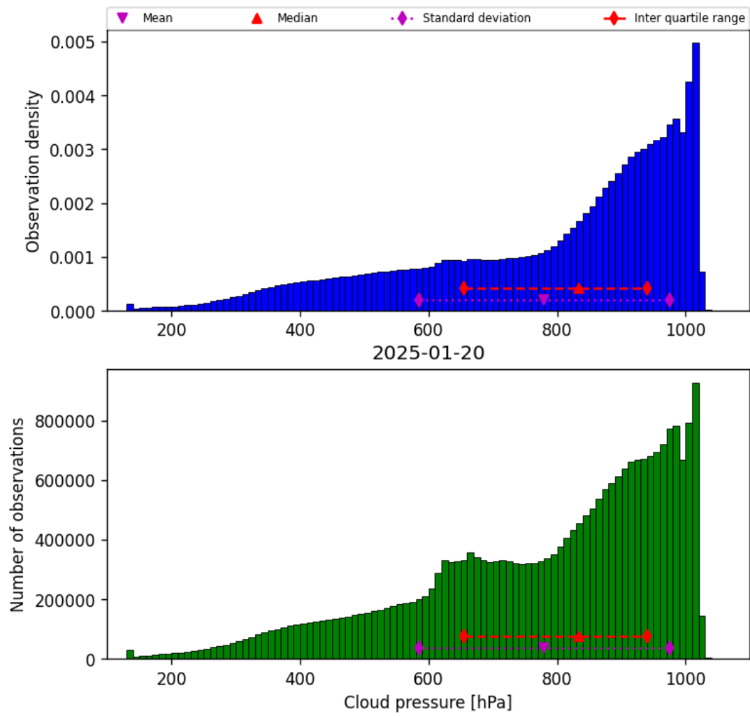
Figure 30: Histogram of “Cloud pressure” for 2025-01-19 to 2025-01-21
