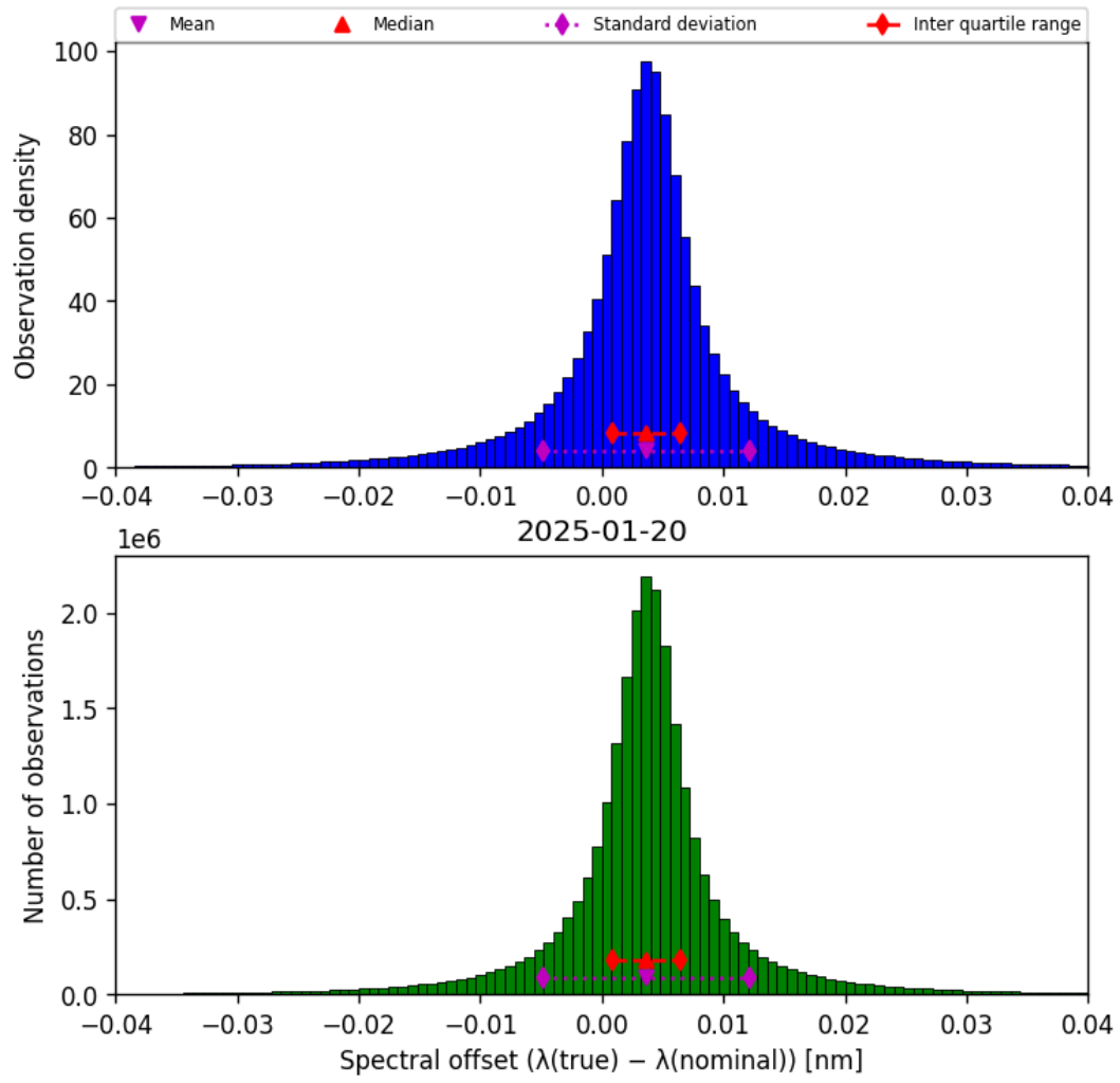
Figure 45: Histogram of “Spectral offset ( \lambda_{\text{true}} - \lambda_{\text{nominal}} )” for 2025-01-19 to 2025-01-21
