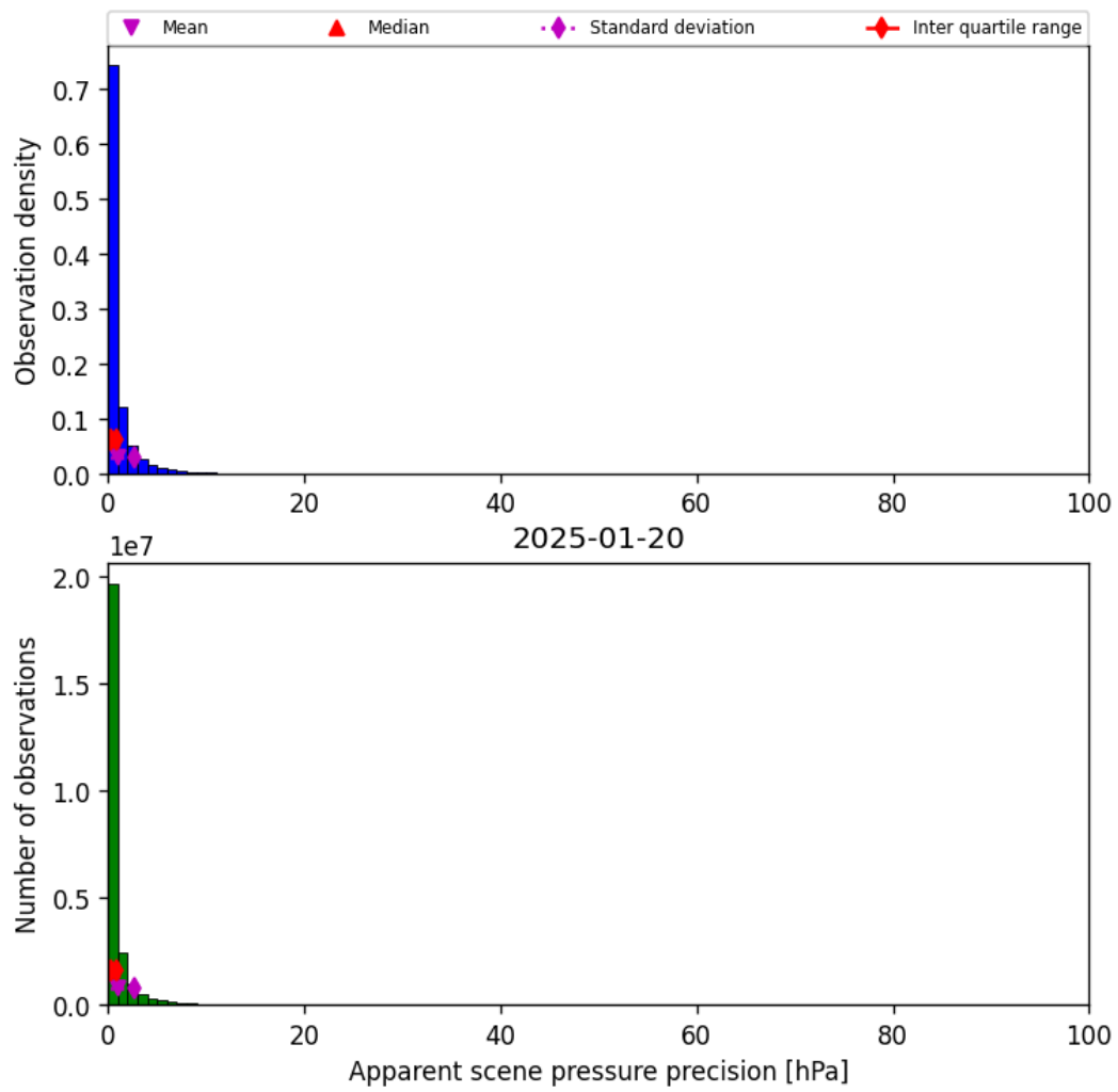
Figure 37: Histogram of “Apparent scene pressure precision” for 2025-01-19 to 2025-01-21
