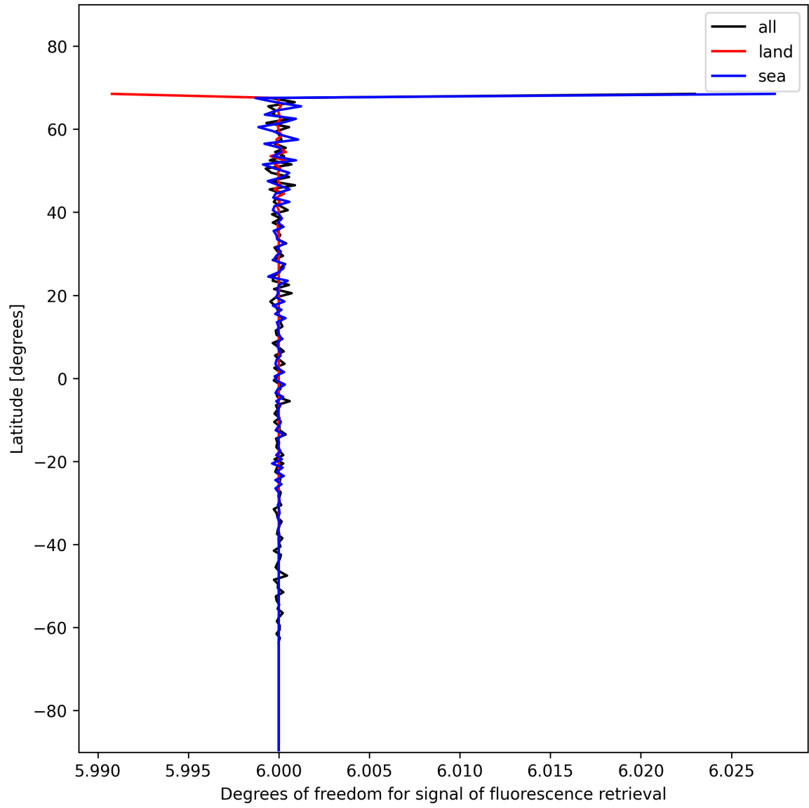
Figure 26: Zonal average of “Degrees of freedom for signal of fluorescence retrieval” for 2025-01-19 to 2025-01-21.
