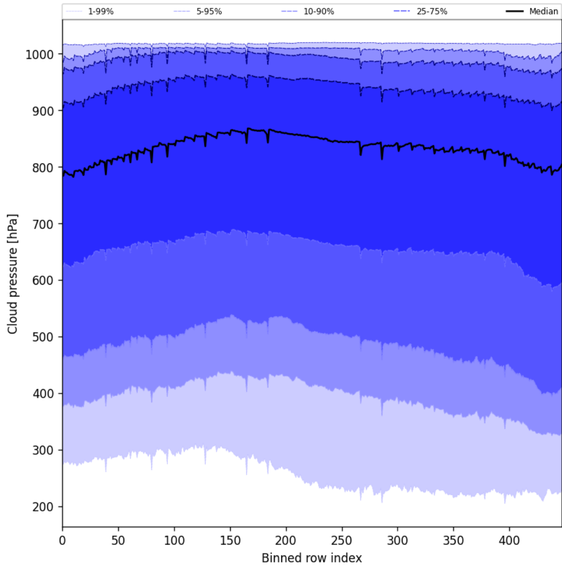
Figure 47: Along track statistics of “Cloud pressure” for 2025-01-19 to 2025-01-21
