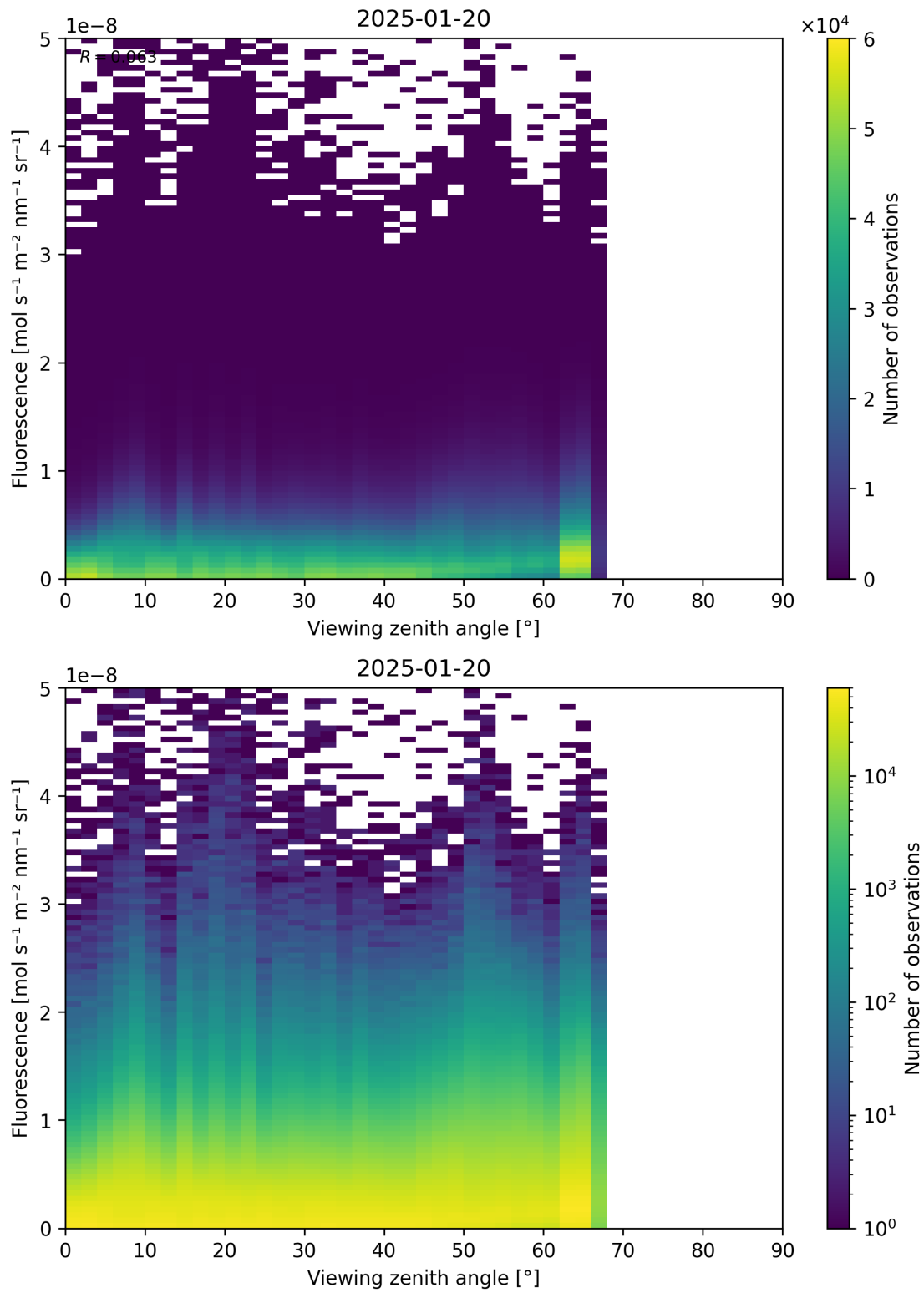
Figure 122: Scatter density plot of “Viewing zenith angle” against “Fluorescence” for 2025-01-19 to 2025-01-21.
