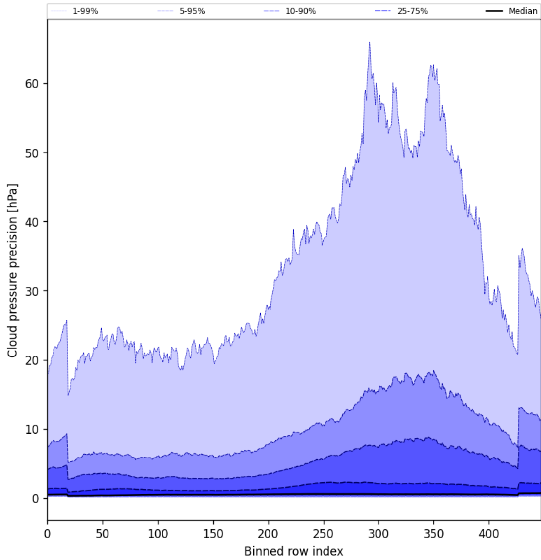
Figure 48: Along track statistics of “Cloud pressure precision” for 2025-01-19 to 2025-01-21
