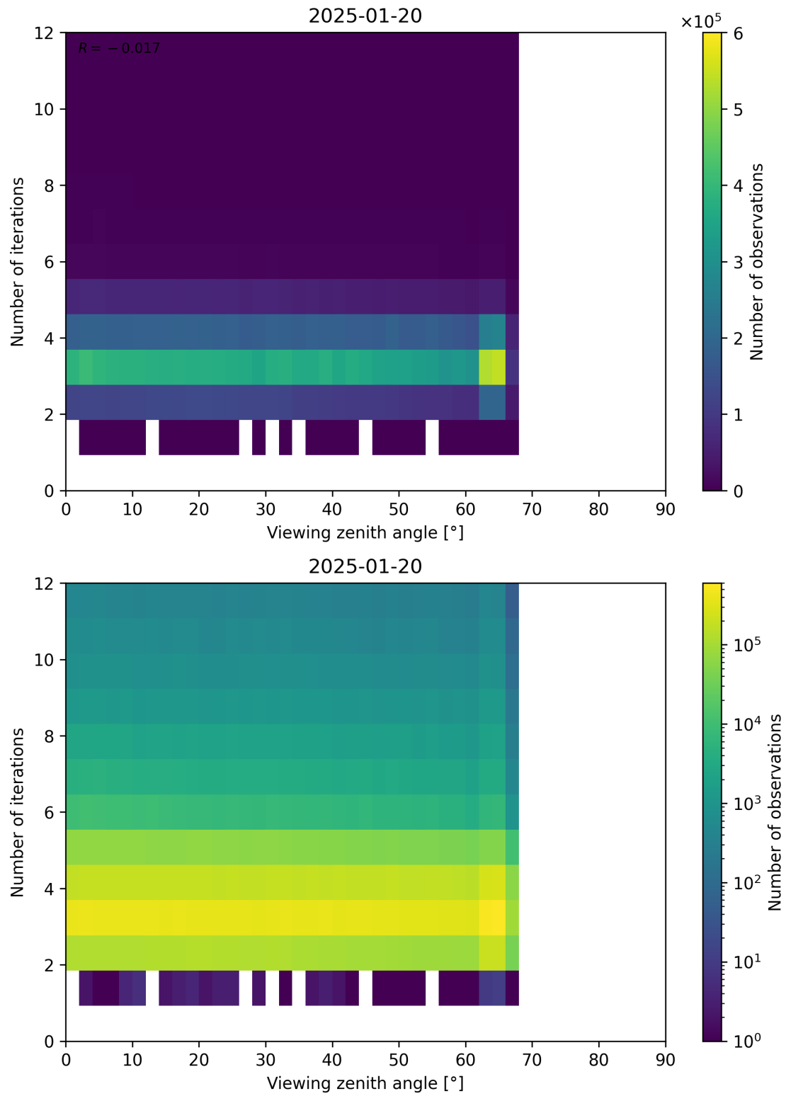
Figure 124: Scatter density plot of “Viewing zenith angle” against “Number of iterations” for 2025-01-19 to 2025-01-21.
