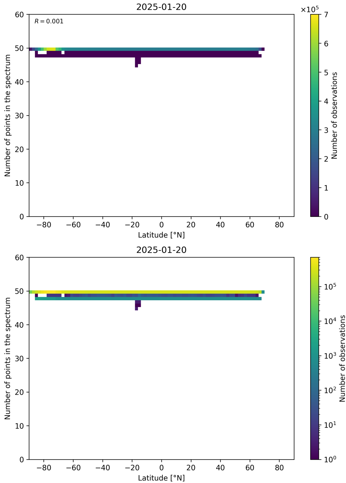
Figure 94: Scatter density plot of “Latitude” against “Number of points in the spectrum” for 2025-01-19 to 2025-01-21.
