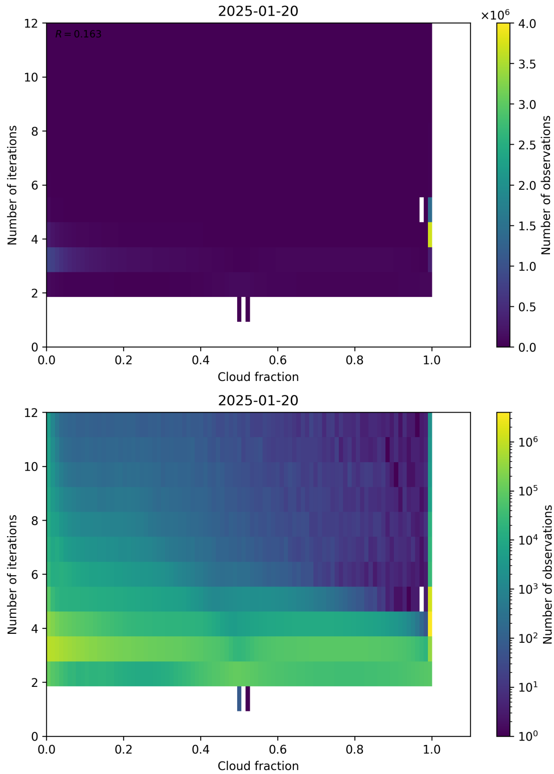
Figure 73: Scatter density plot of “Cloud fraction” against “Number of iterations” for 2025-01-19 to 2025-01-21.
