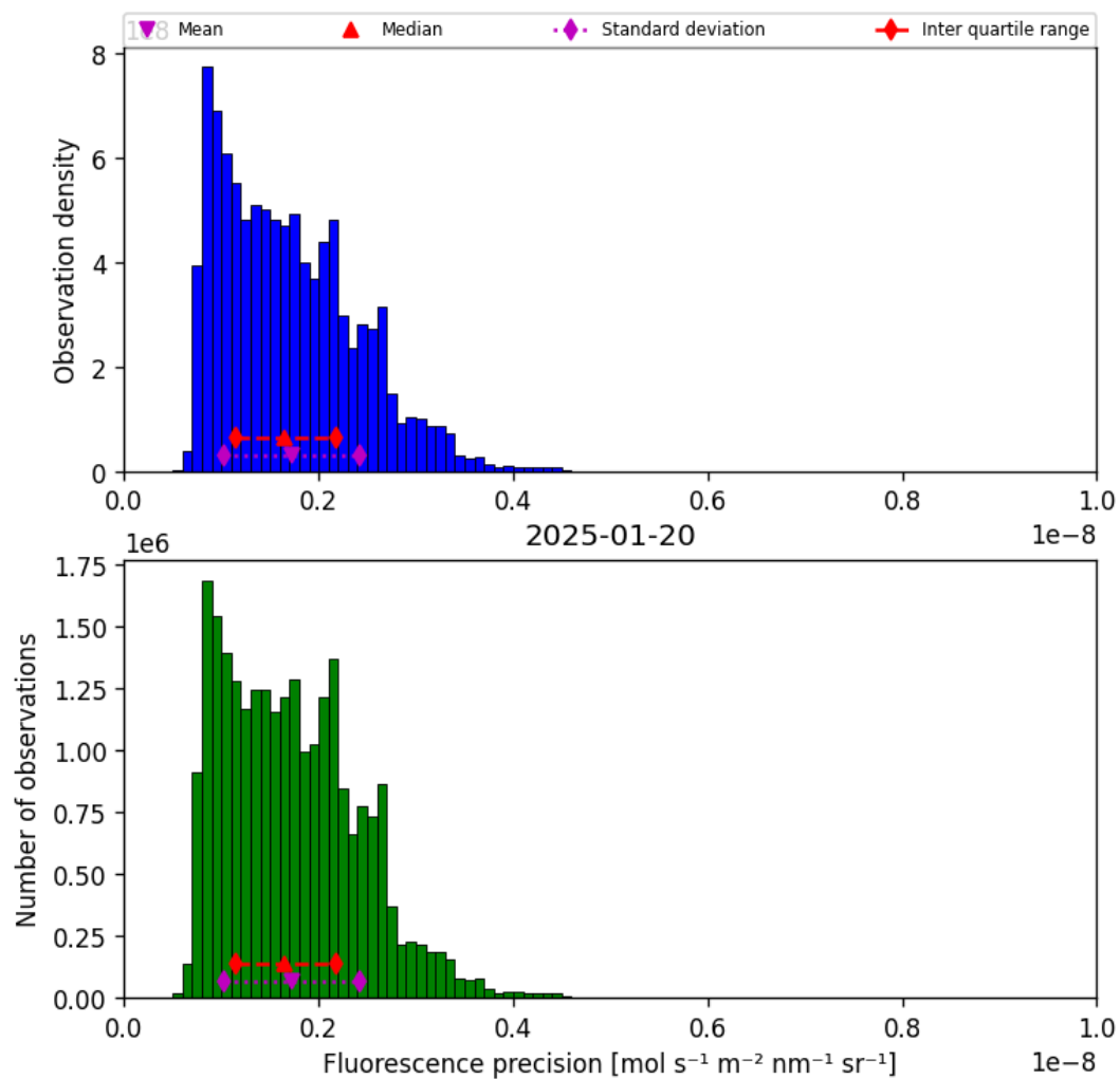
Figure 41: Histogram of “Fluorescence precision” for 2025-01-19 to 2025-01-21
