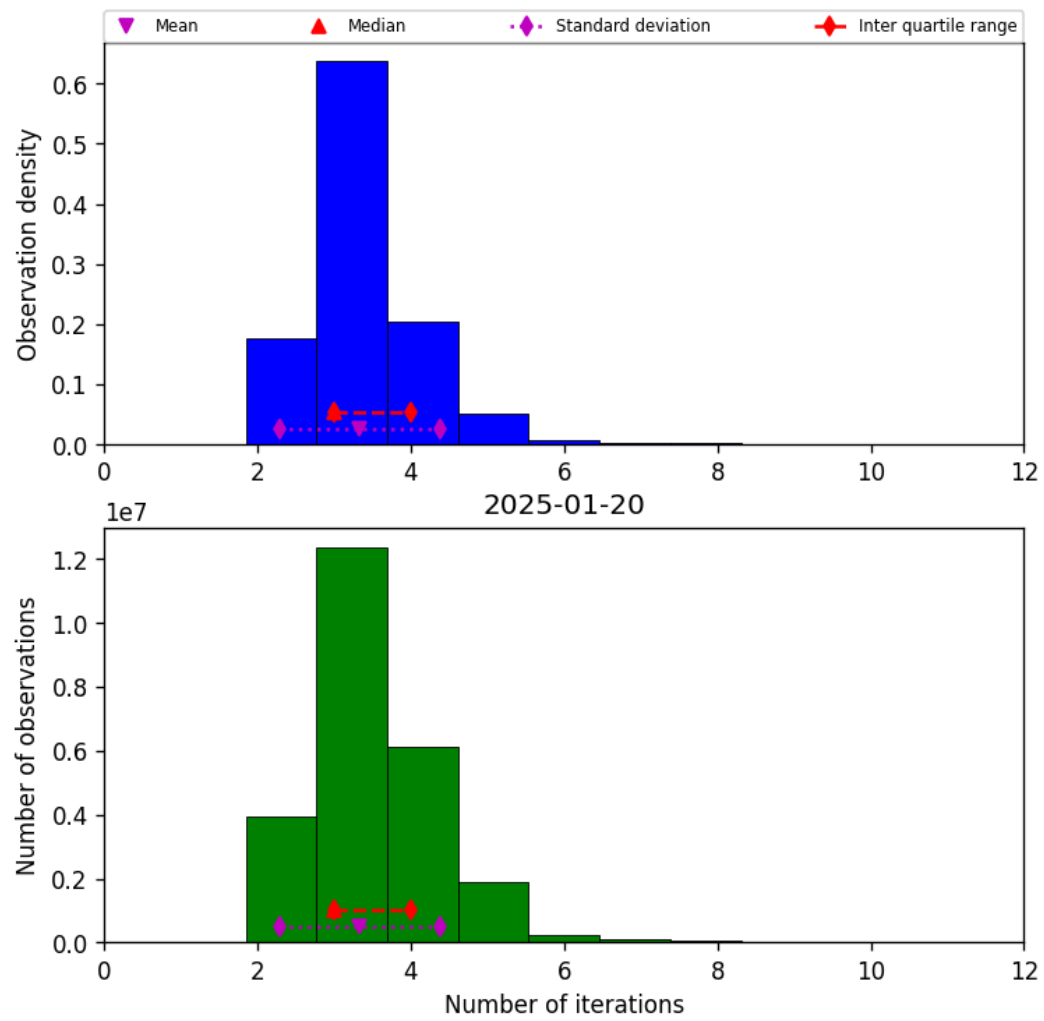
Figure 39: Histogram of “Number of iterations” for 2025-01-19 to 2025-01-21
