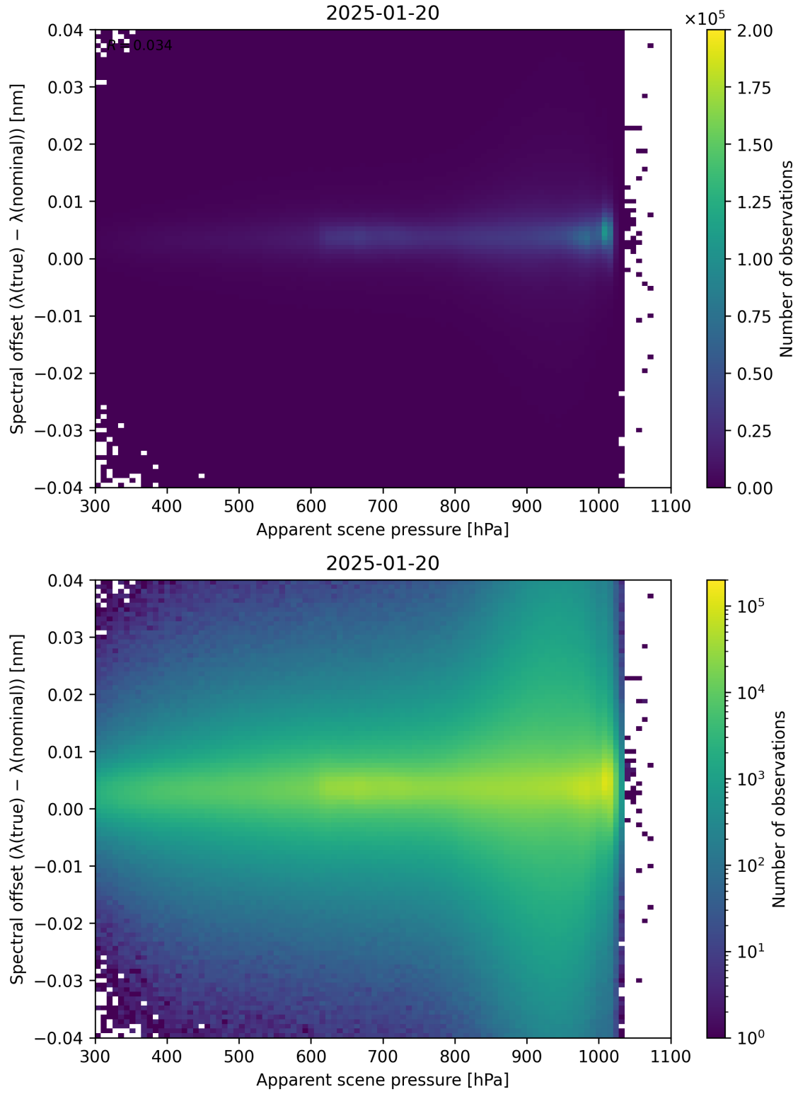
Figure 67: Scatter density plot of “Apparent scene pressure” against “Spectral offset ( \lambda_{\text{true}} - \lambda_{\text{nominal}} )” for 2025-01-19 to 2025-01-21.
