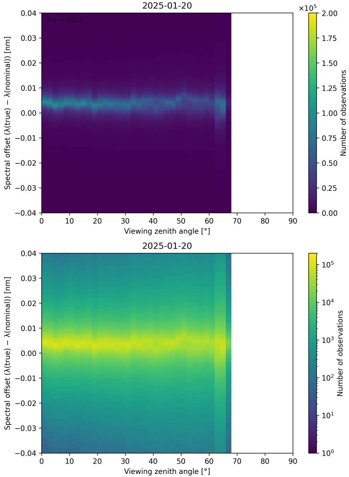
Figure 128: Scatter density plot of “Viewing zenith angle” against “Spectral offset ( \lambda_{\text{true}} - \lambda_{\text{nominal}} )” for 2025-01-19 to 2025-01-21.
