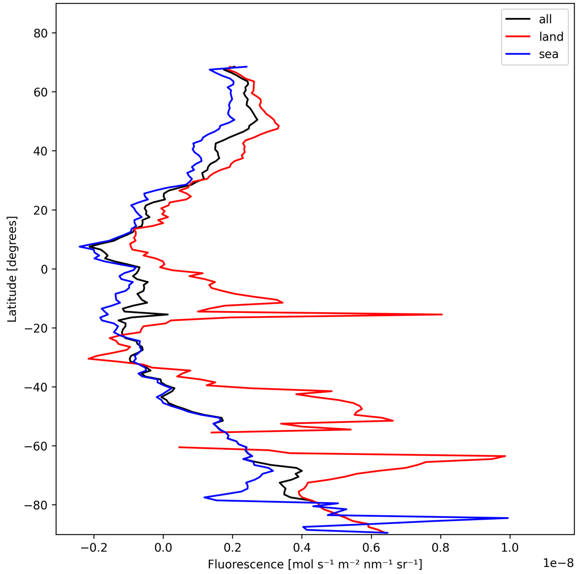
Figure 23: Zonal average of “Fluorescence” for 2025-01-19 to 2025-01-21.
