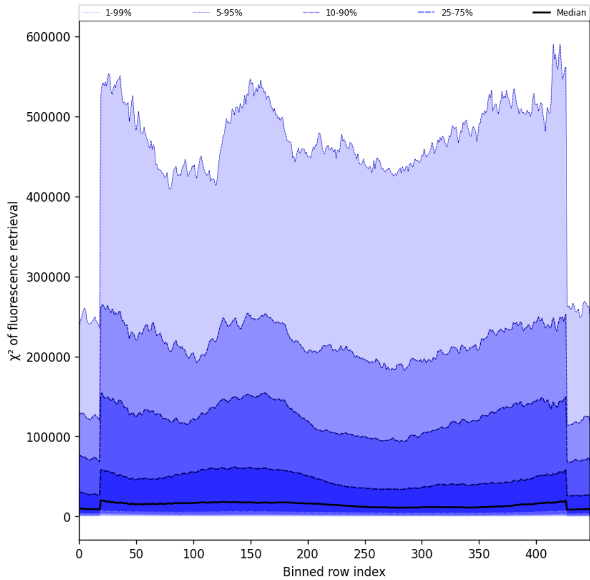
Figure 59: Along track statistics of “ \chi^2 of fluorescence retrieval” for 2025-01-19 to 2025-01-21
