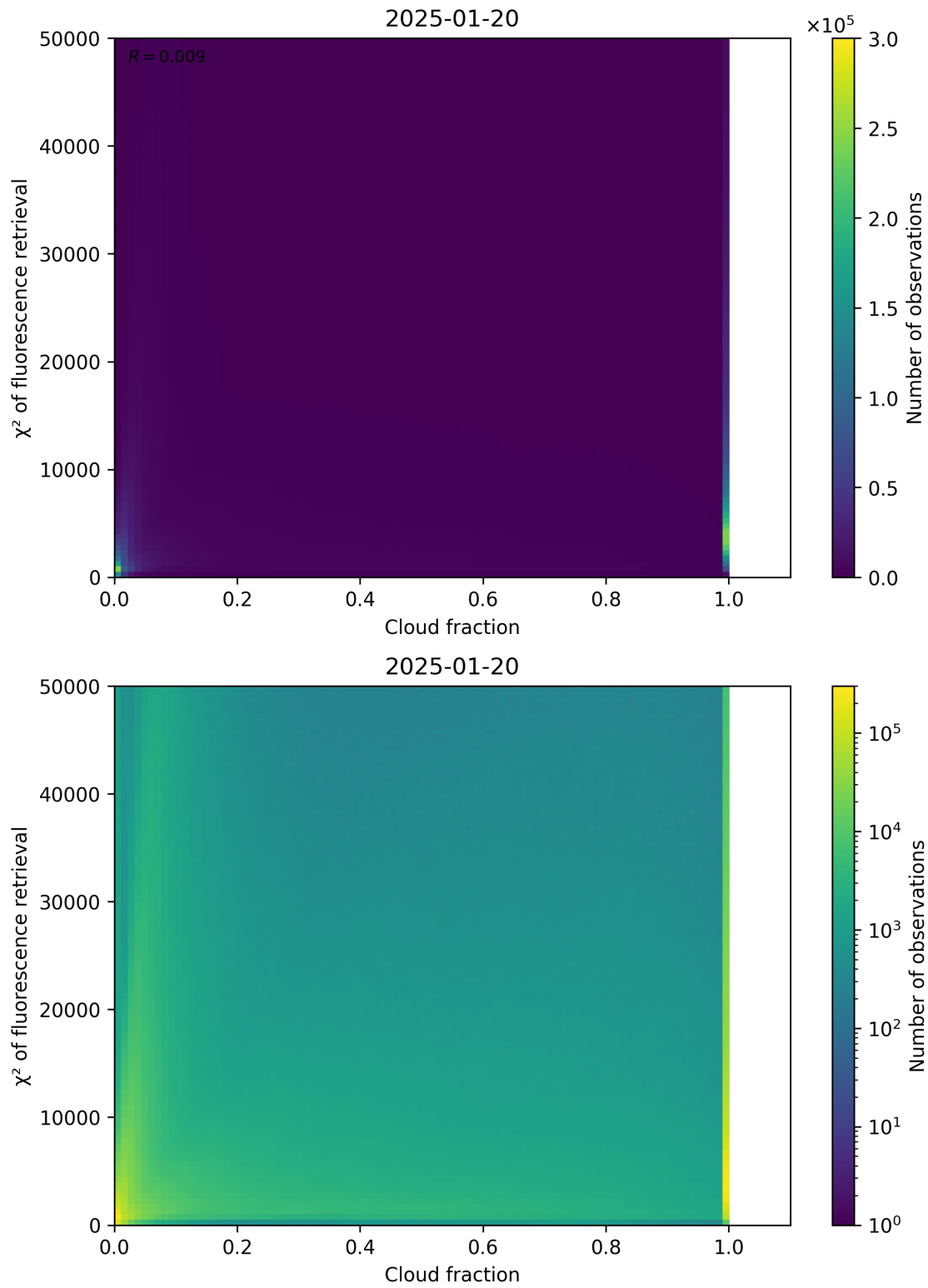
Figure 71: Scatter density plot of “Cloud fraction” against “ \chi^2 of fluorescence retrieval” for 2025-01-19 to 2025-01-21.
