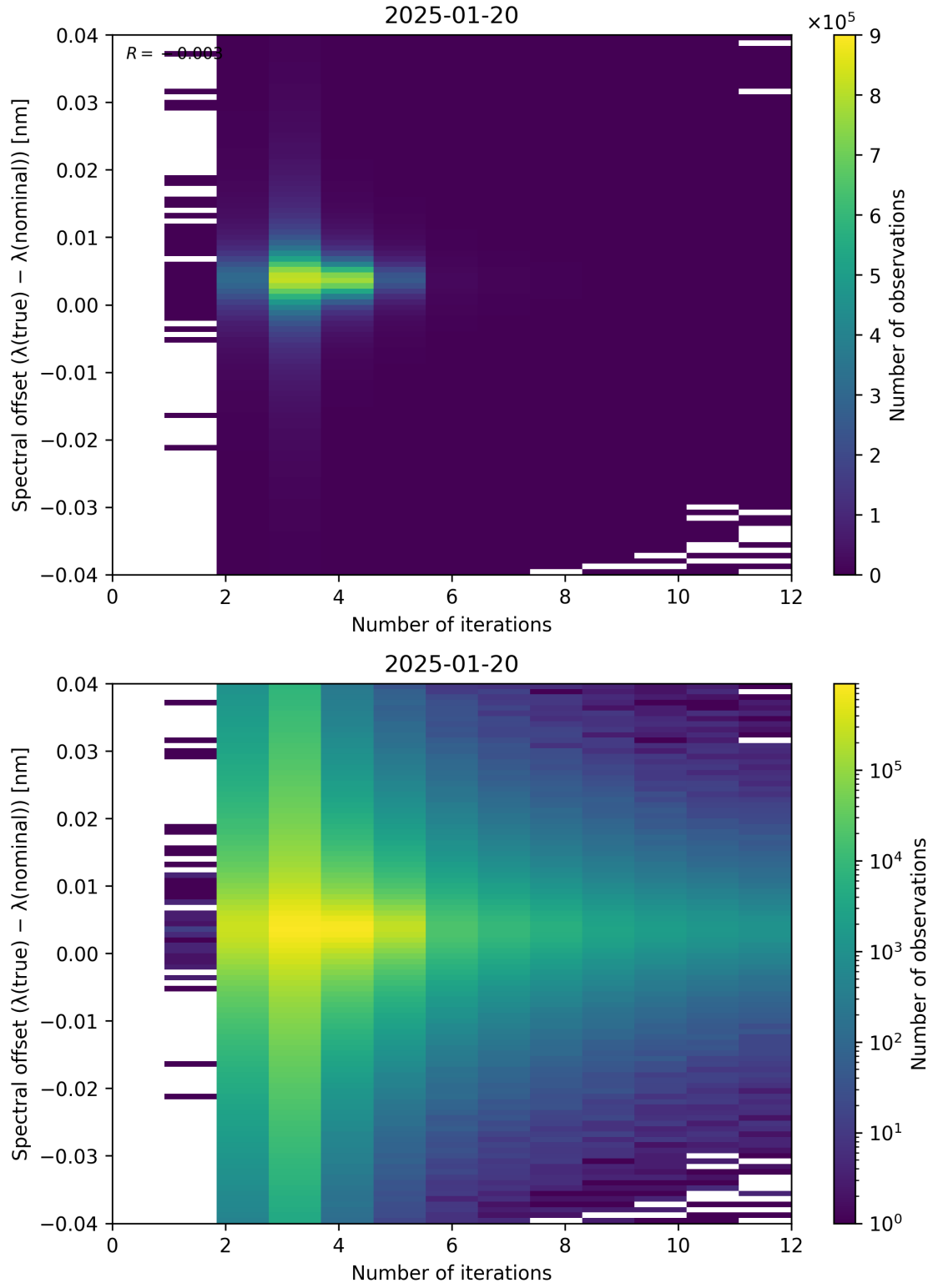
Figure 100: Scatter density plot of “Number of iterations” against “Spectral offset ( \lambda_{\text{true}} - \lambda_{\text{nominal}} )” for 2025-01-19 to 2025-01-21.
