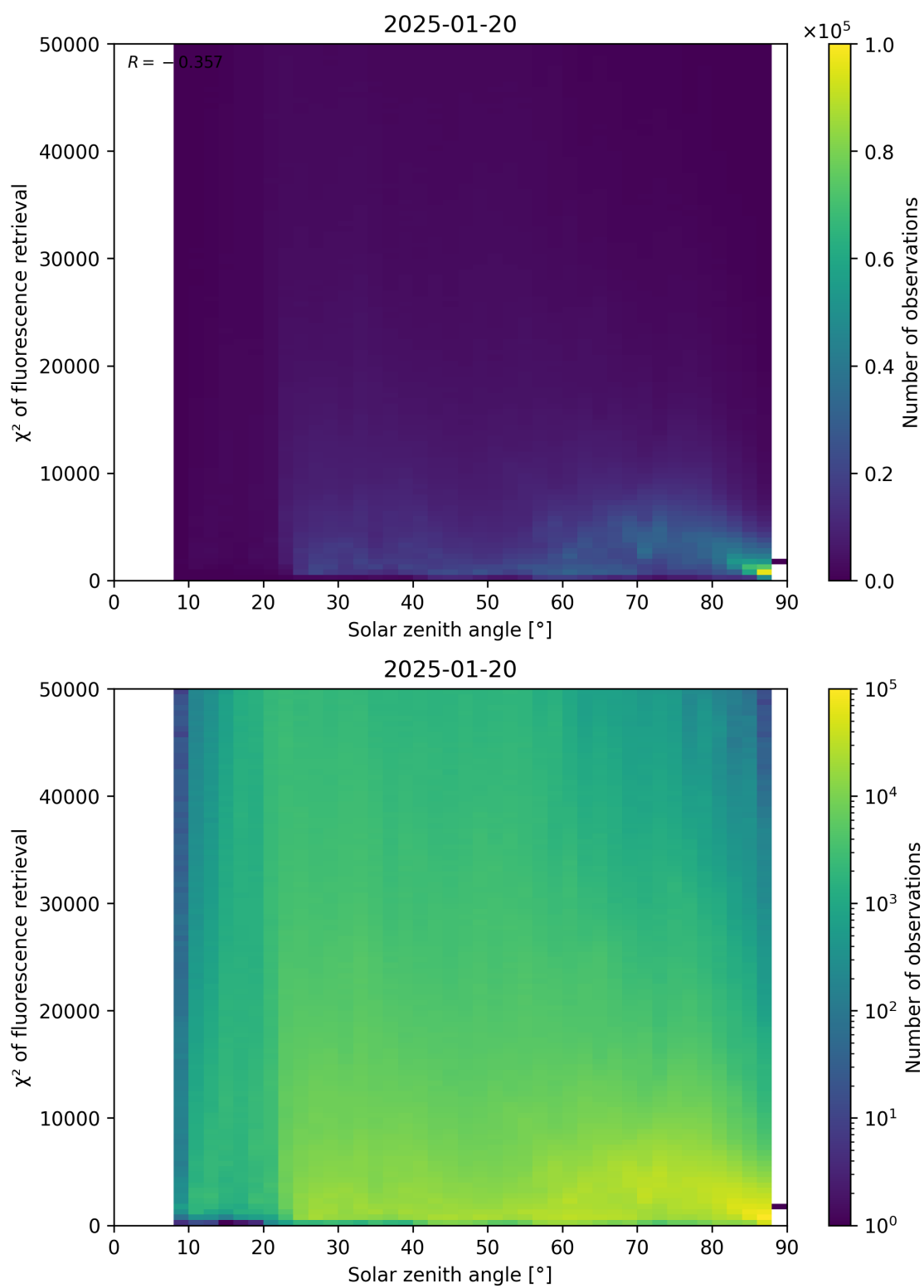
Figure 109: Scatter density plot of “Solar zenith angle” against “ \chi^2 of fluorescence retrieval” for 2025-01-19 to 2025-01-21.
