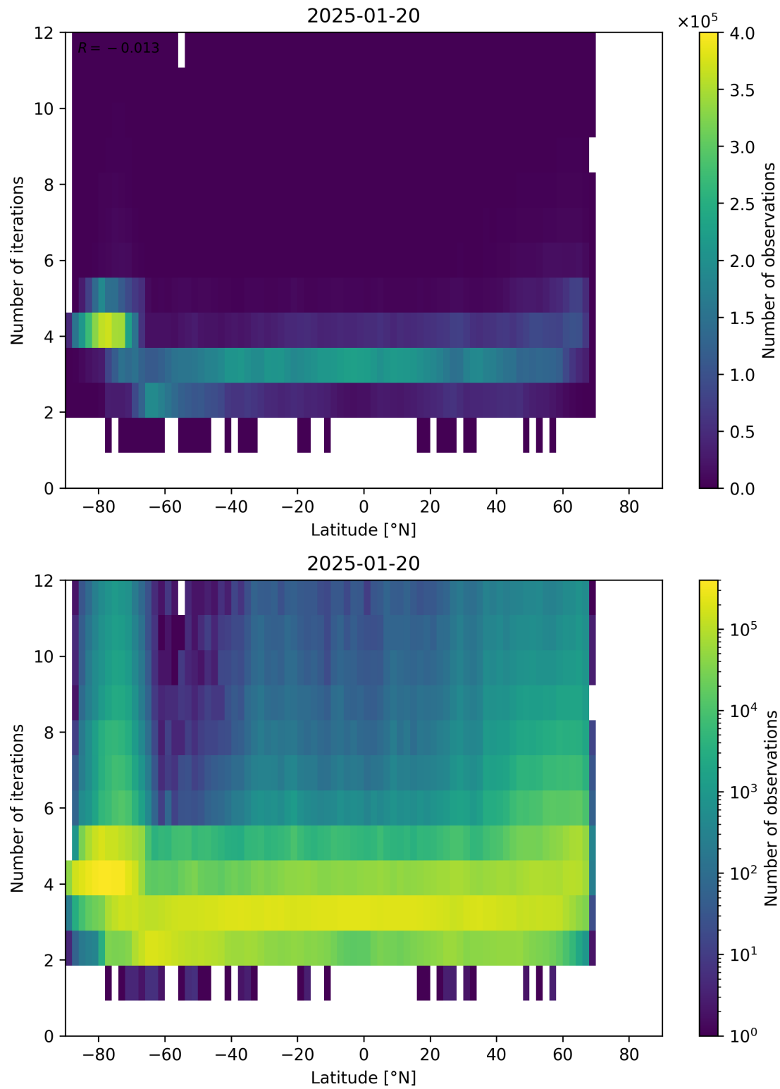
Figure 93: Scatter density plot of “Latitude” against “Number of iterations” for 2025-01-19 to 2025-01-21.
