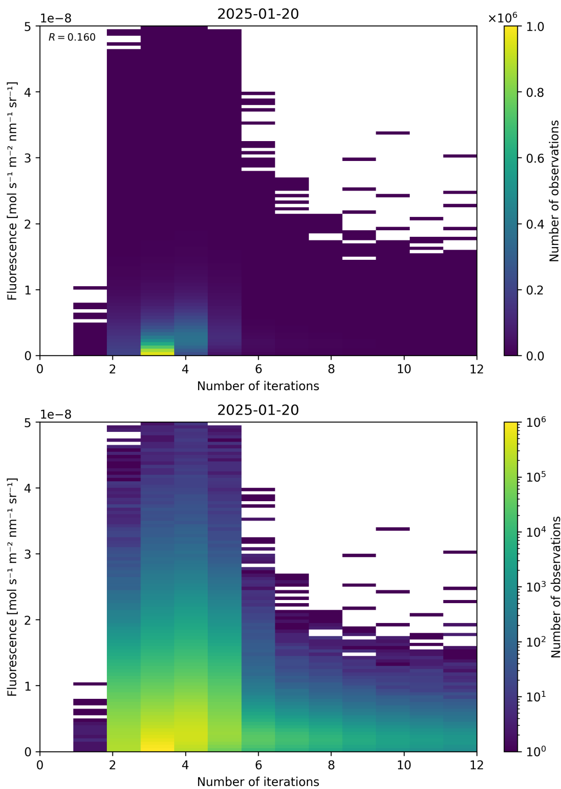
Figure 98: Scatter density plot of “Number of iterations” against “Fluorescence” for 2025-01-19 to 2025-01-21.
