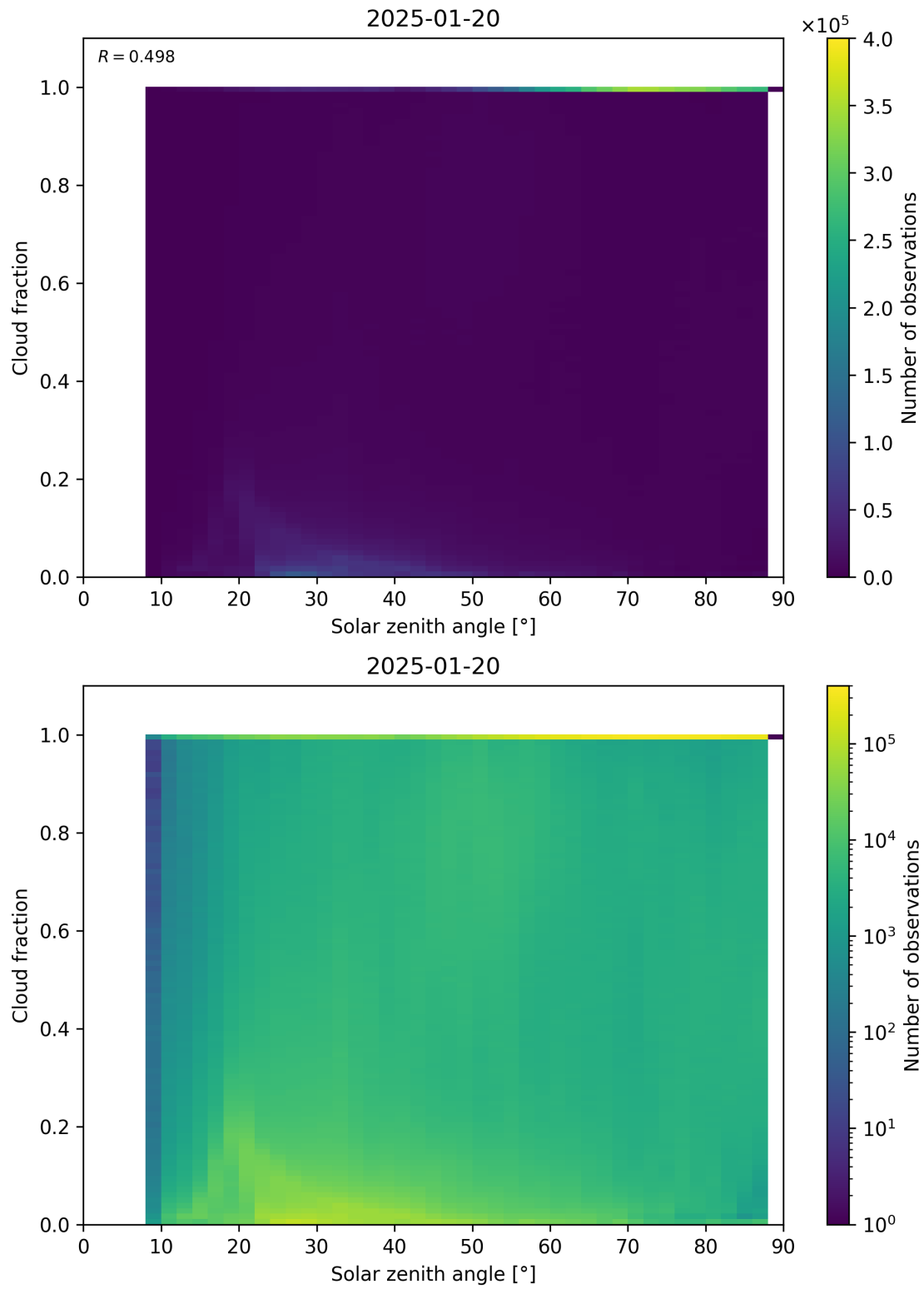
Figure 110: Scatter density plot of “Solar zenith angle” against “Cloud fraction” for 2025-01-19 to 2025-01-21.
