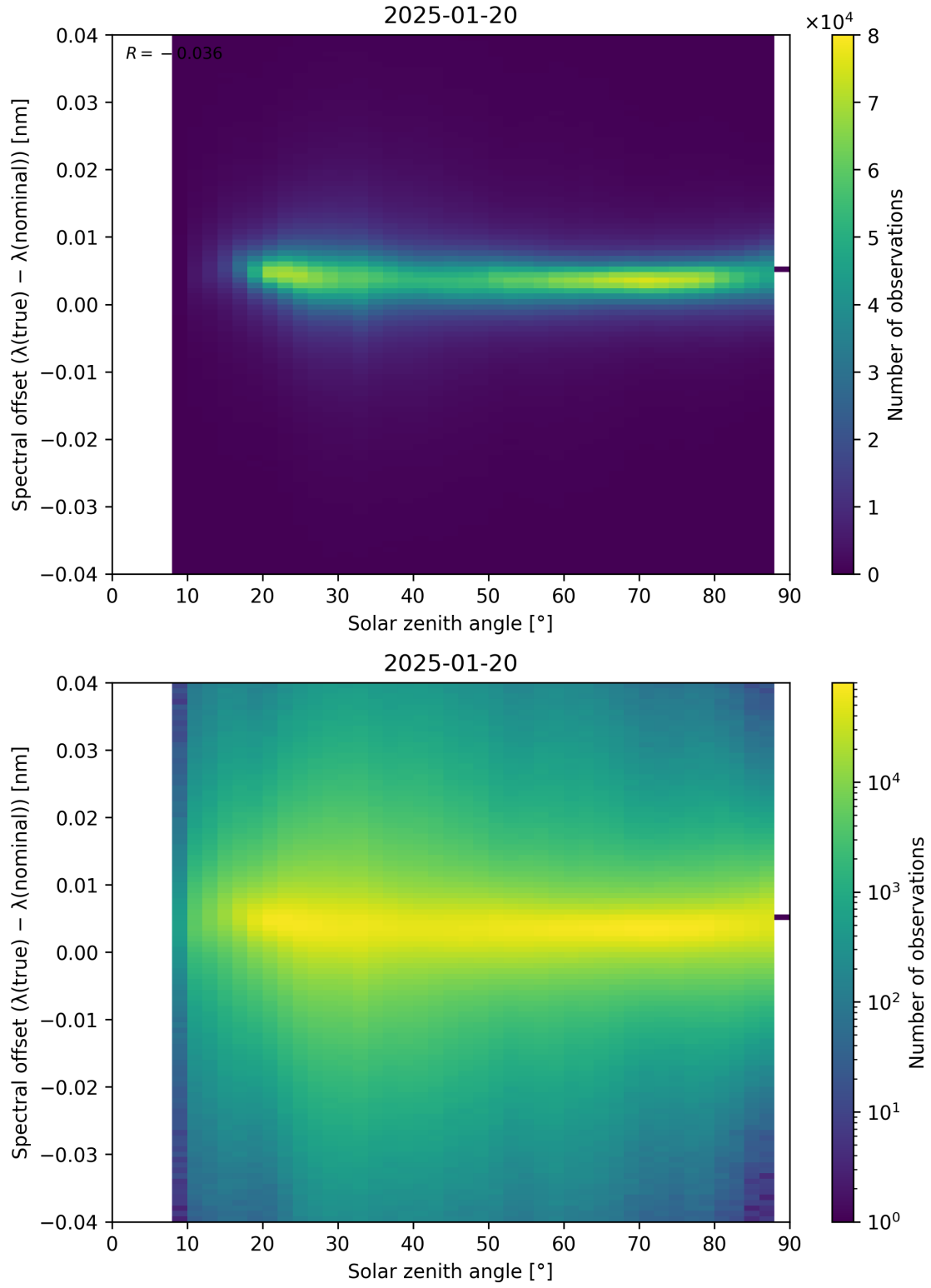
Figure 117: Scatter density plot of “Solar zenith angle” against “Spectral offset ( \lambda_{\text{true}} - \lambda_{\text{nominal}} )” for 2025-01-19 to 2025-01-21.
