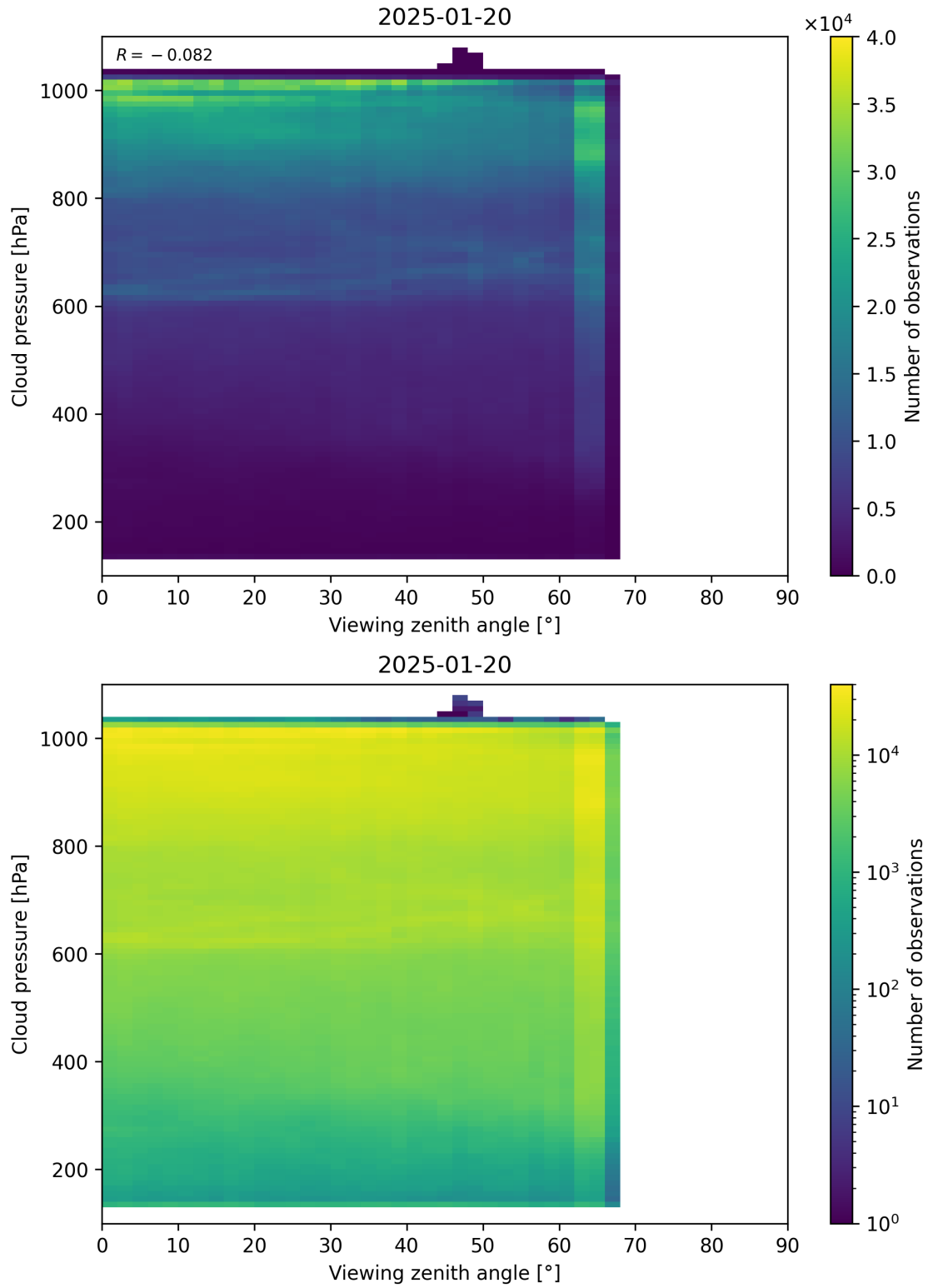
Figure 121: Scatter density plot of “Viewing zenith angle” against “Cloud pressure” for 2025-01-19 to 2025-01-21.
