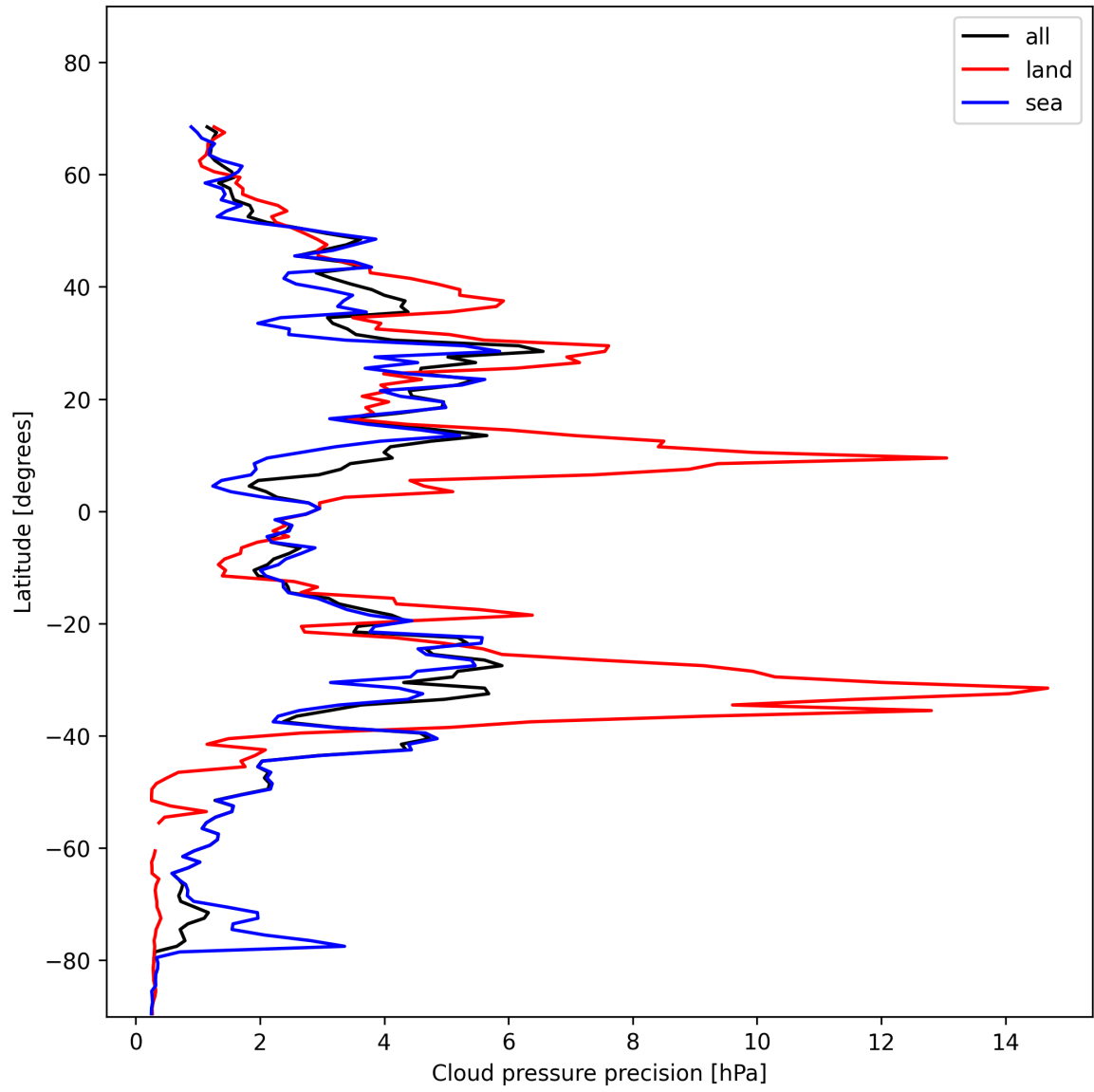
Figure 14: Zonal average of “Cloud pressure precision” for 2025-01-19 to 2025-01-21.
