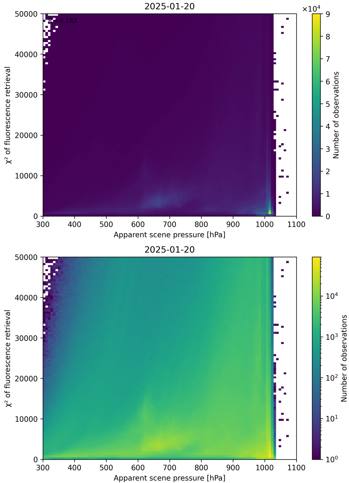
Figure 63: Scatter density plot of “Apparent scene pressure” against “ \chi^2 of fluorescence retrieval” for 2025-01-19 to 2025-01-21.
