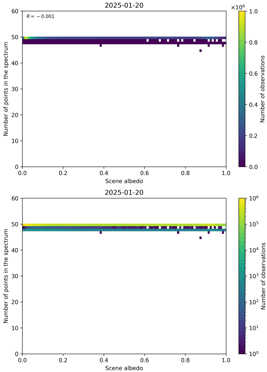
Figure 106: Scatter density plot of “Scene albedo” against “Number of points in the spectrum” for 2025-01-19 to 2025-01-21.
