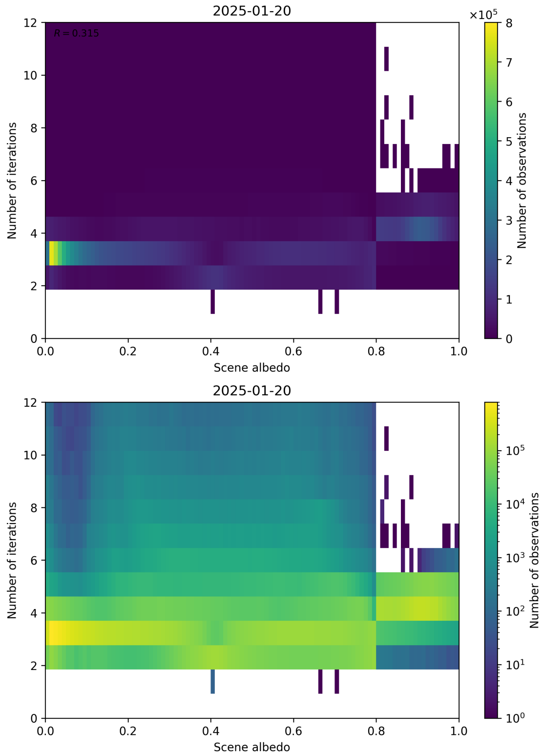
Figure 105: Scatter density plot of “Scene albedo” against “Number of iterations” for 2025-01-19 to 2025-01-21.
