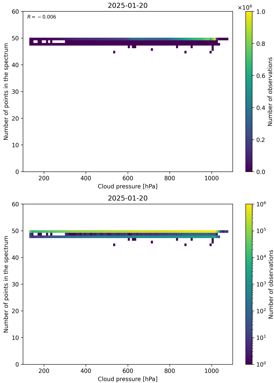
Figure 82: Scatter density plot of “Cloud pressure” against “Number of points in the spectrum” for 2025-01-19 to 2025-01-21.
