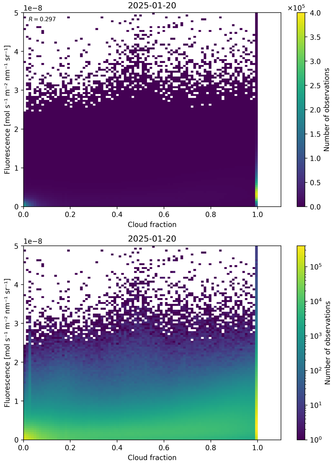
Figure 72: Scatter density plot of “Cloud fraction” against “Fluorescence” for 2025-01-19 to 2025-01-21.
