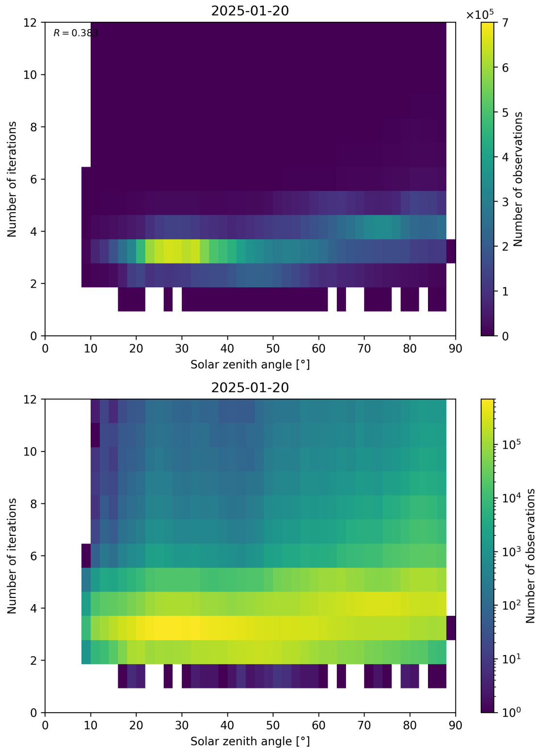
Figure 114: Scatter density plot of “Solar zenith angle” against “Number of iterations” for 2025-01-19 to 2025-01-21.
