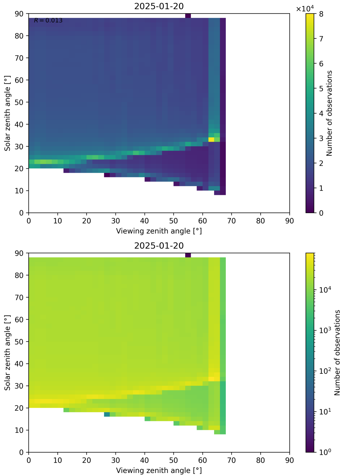
Figure 127: Scatter density plot of “Viewing zenith angle” against “Solar zenith angle” for 2025-01-19 to 2025-01-21.
