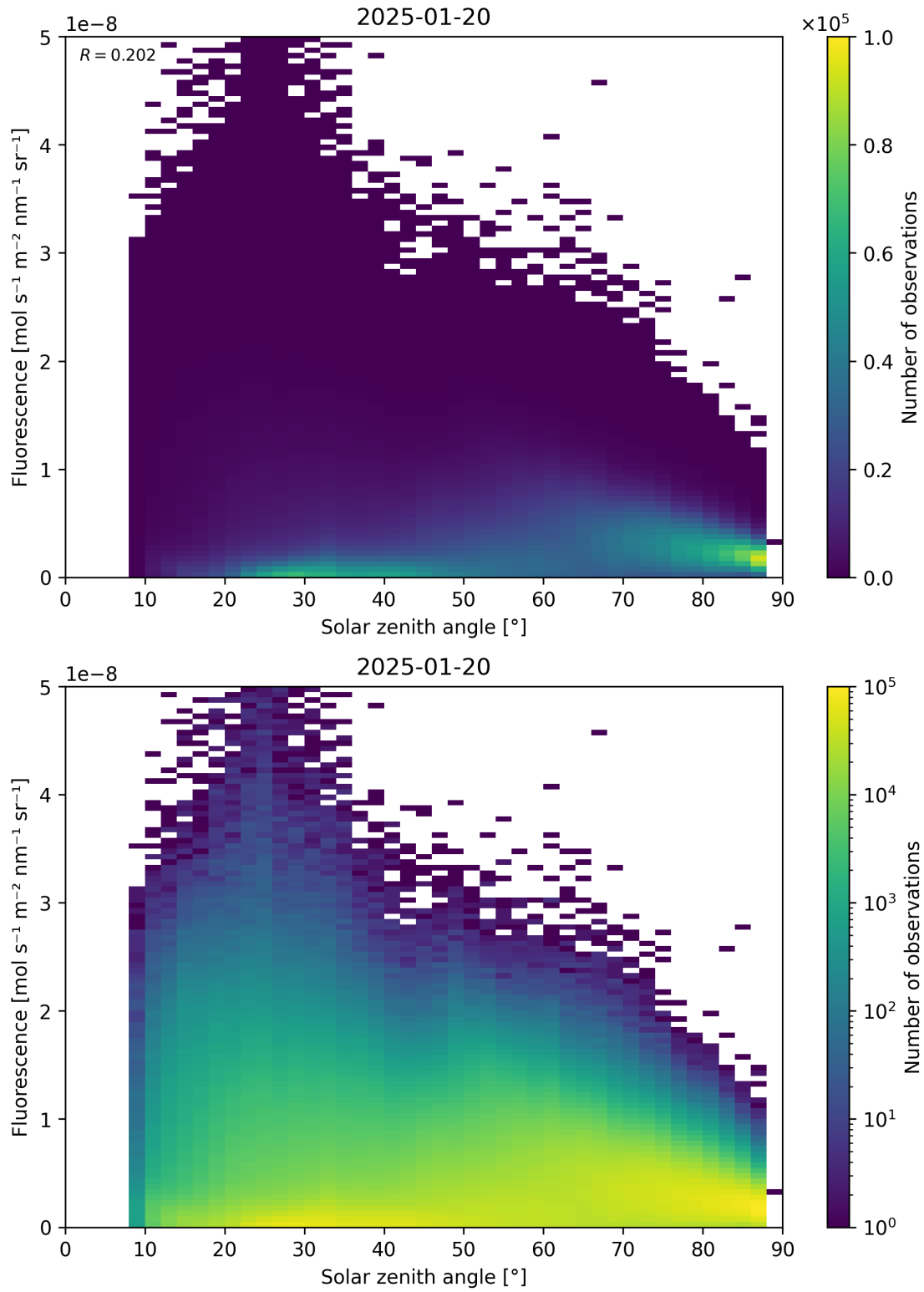
Figure 112: Scatter density plot of “Solar zenith angle” against “Fluorescence” for 2025-01-19 to 2025-01-21.
