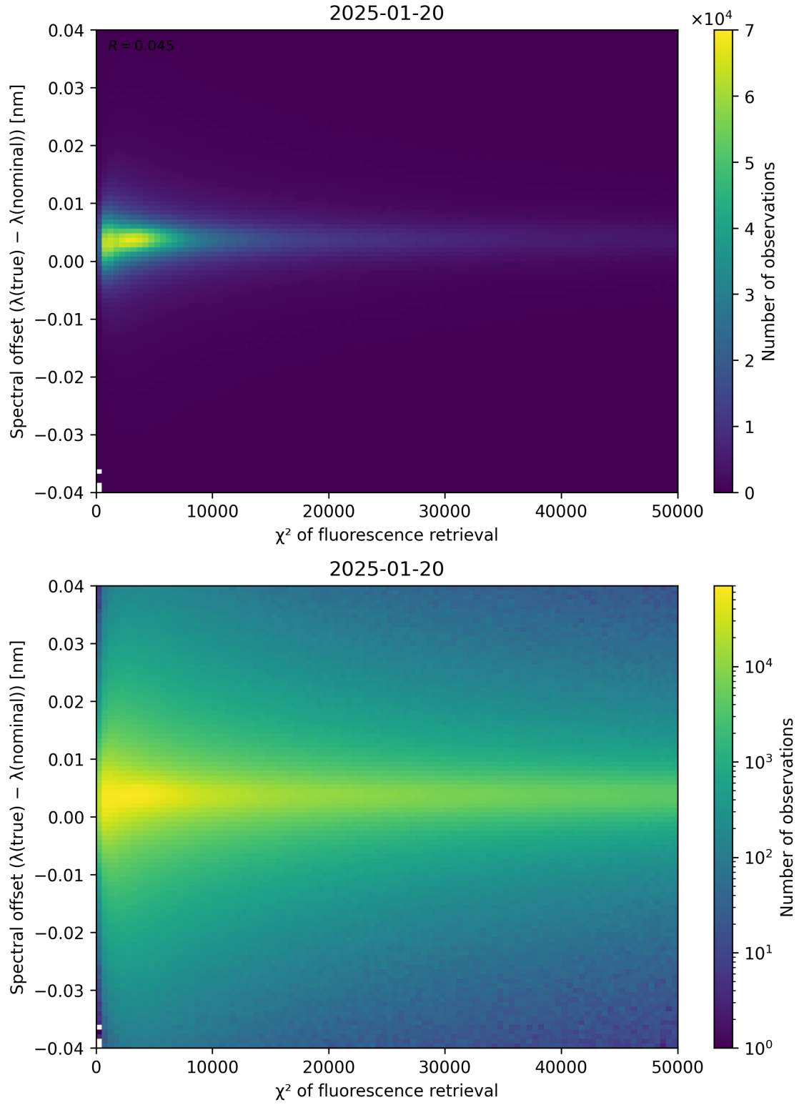
Figure 69: Scatter density plot of “ \chi^2 of fluorescence retrieval” against “Spectral offset ( \lambda_{\text{true}} - \lambda_{\text{nominal}} )” for 2025-01-19 to 2025-01-21.
