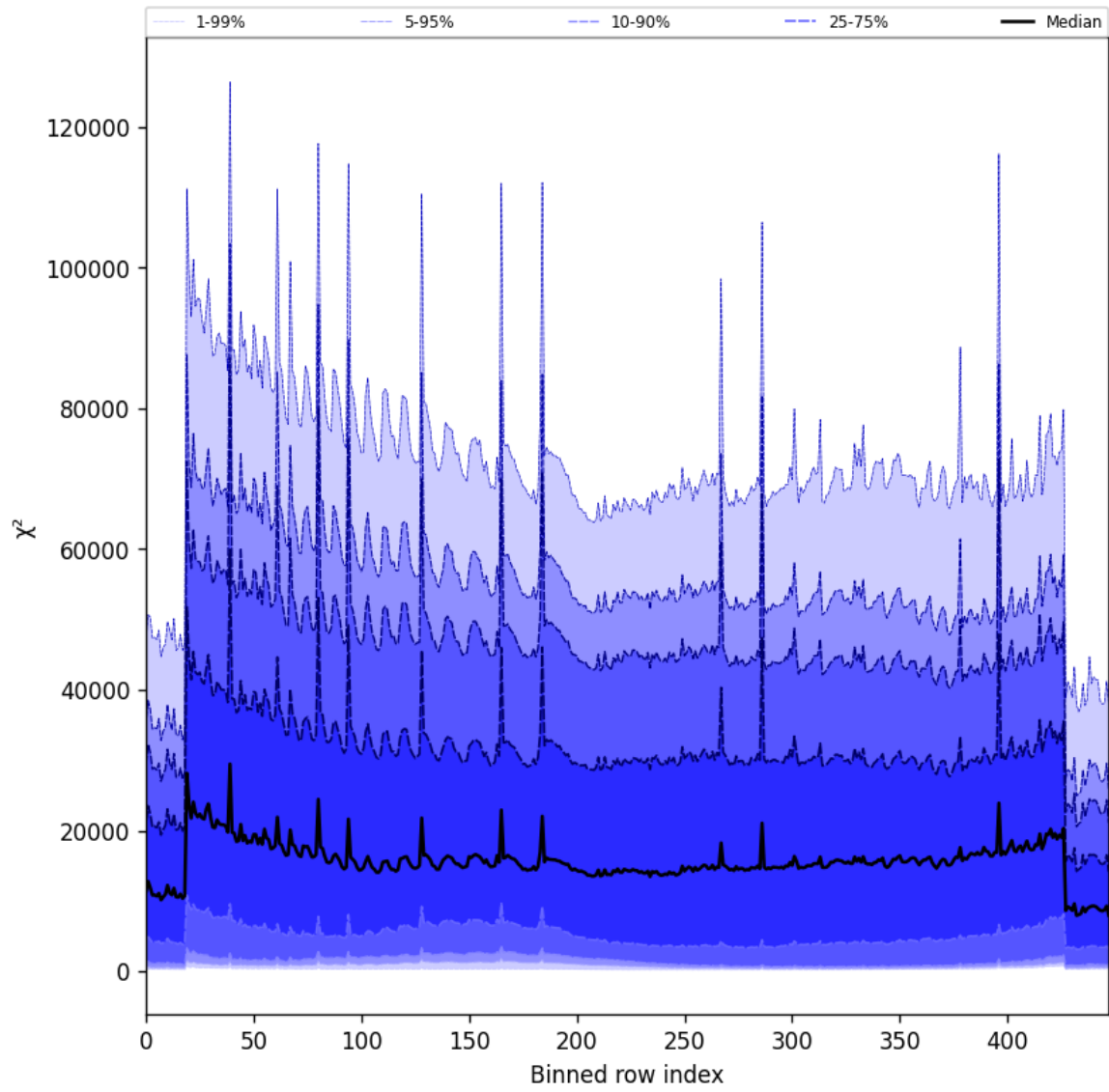
Figure 55: Along track statistics of “ \chi^2 ” for 2025-01-19 to 2025-01-21
