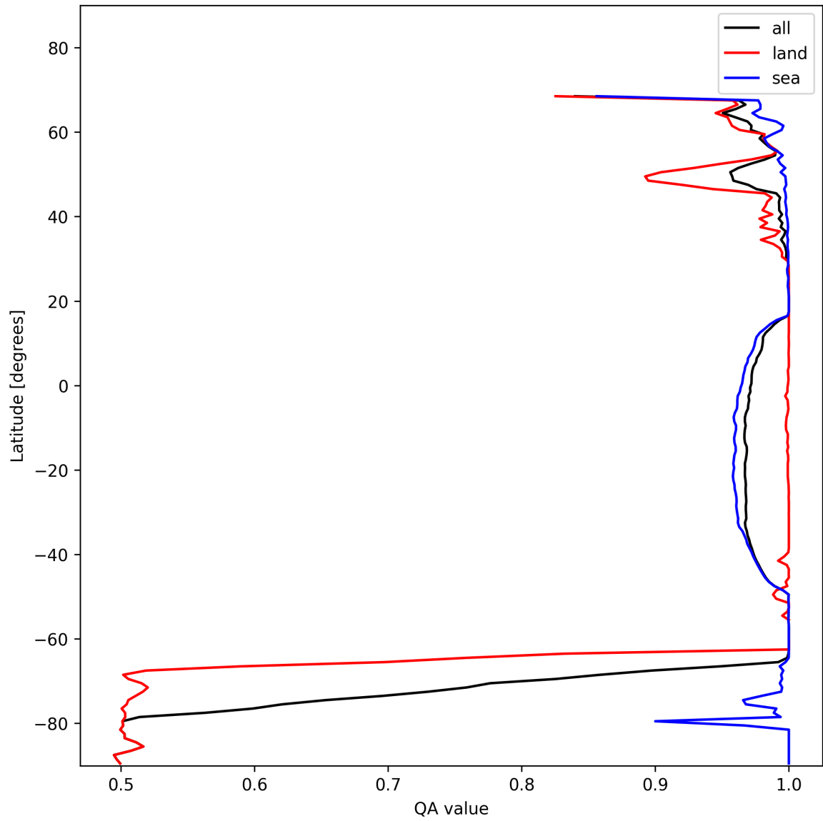
Figure 12: Zonal average of “QA value” for 2025-01-19 to 2025-01-21.
