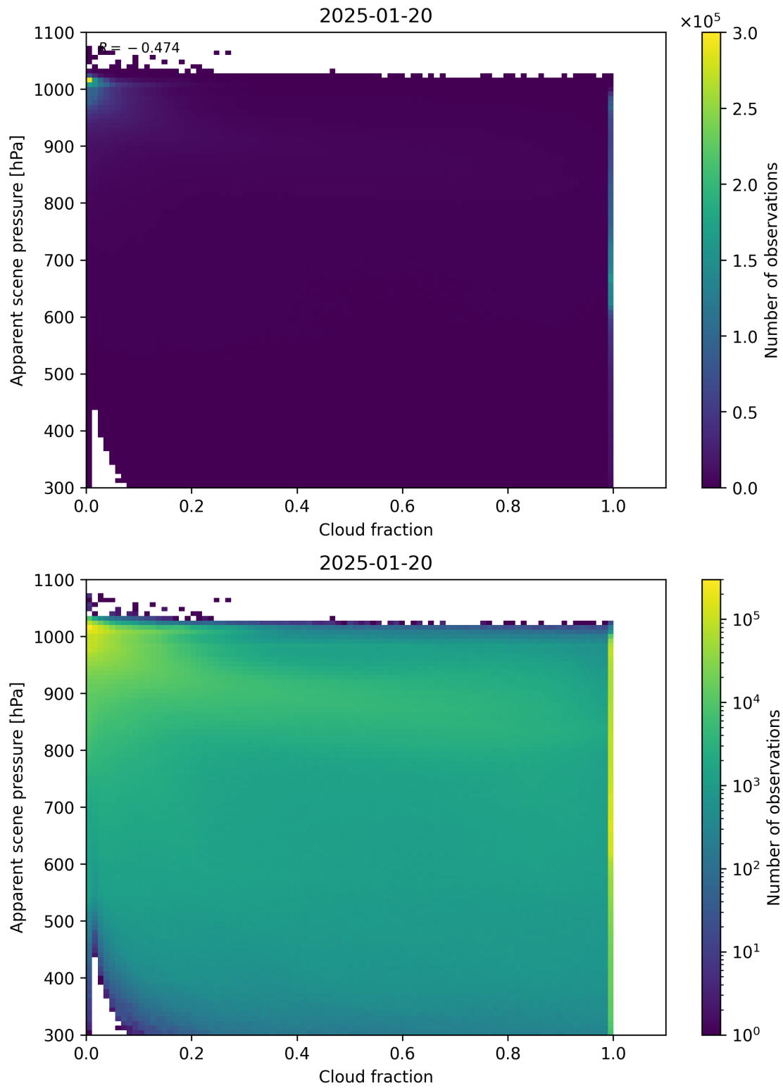
Figure 70: Scatter density plot of “Cloud fraction” against “Apparent scene pressure” for 2025-01-19 to 2025-01-21.
