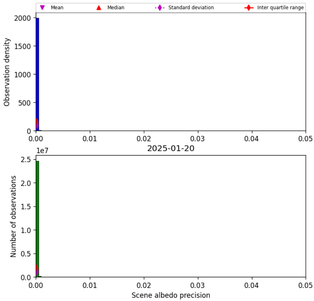
Figure 35: Histogram of “Scene albedo precision” for 2025-01-19 to 2025-01-21
