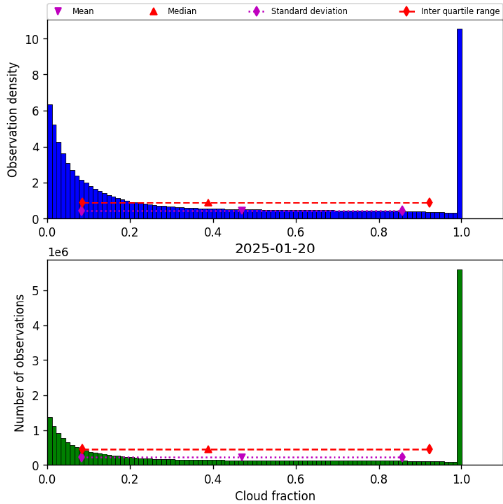
Figure 32: Histogram of “Cloud fraction” for 2025-01-19 to 2025-01-21
