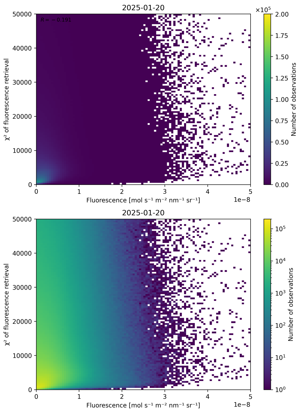
Figure 85: Scatter density plot of “Fluorescence” against “ \chi^2 of fluorescence retrieval” for 2025-01-19 to 2025-01-21.
