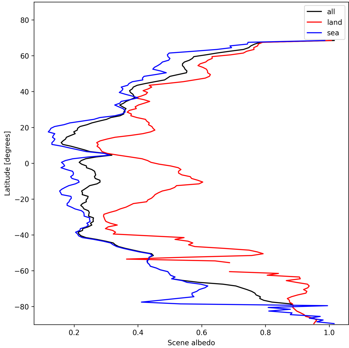
Figure 17: Zonal average of “Scene albedo” for 2025-01-19 to 2025-01-21.
