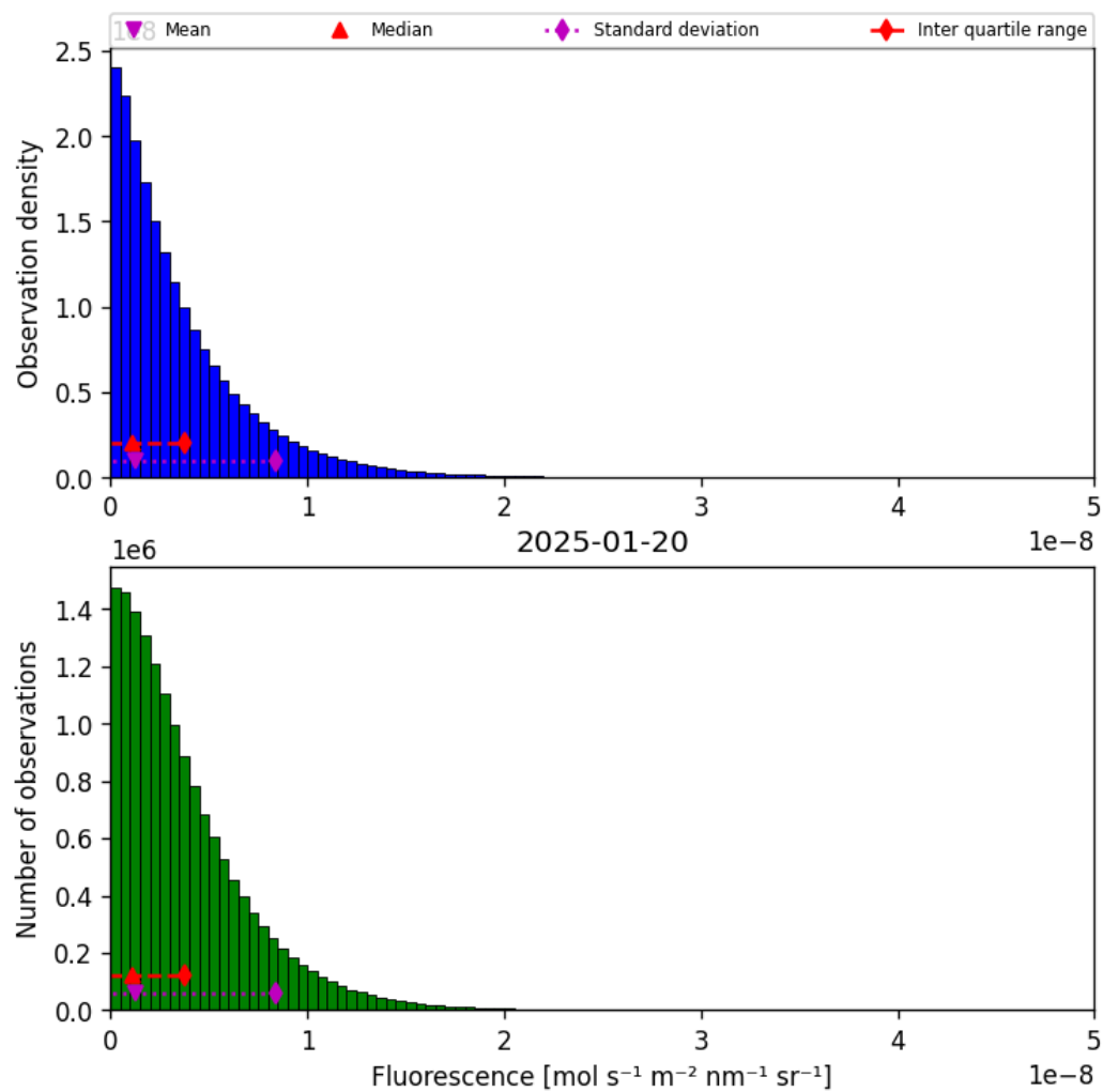
Figure 40: Histogram of “Fluorescence” for 2025-01-19 to 2025-01-21
