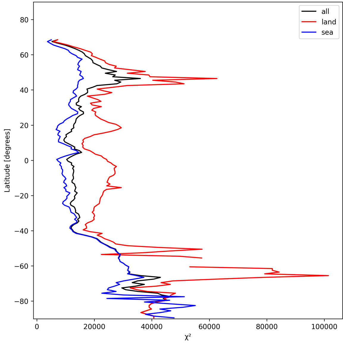
Figure 21: Zonal average of “ \chi^2 ” for 2025-01-19 to 2025-01-21.
