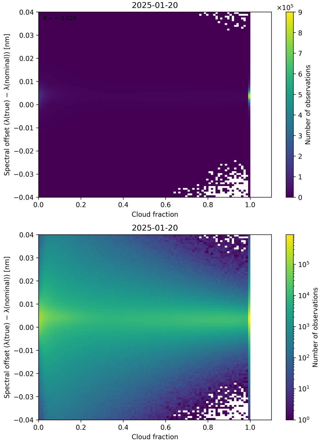
Figure 76: Scatter density plot of “Cloud fraction” against “Spectral offset ( \lambda_{\text{true}} - \lambda_{\text{nominal}} )” for 2025-01-19 to 2025-01-21.
