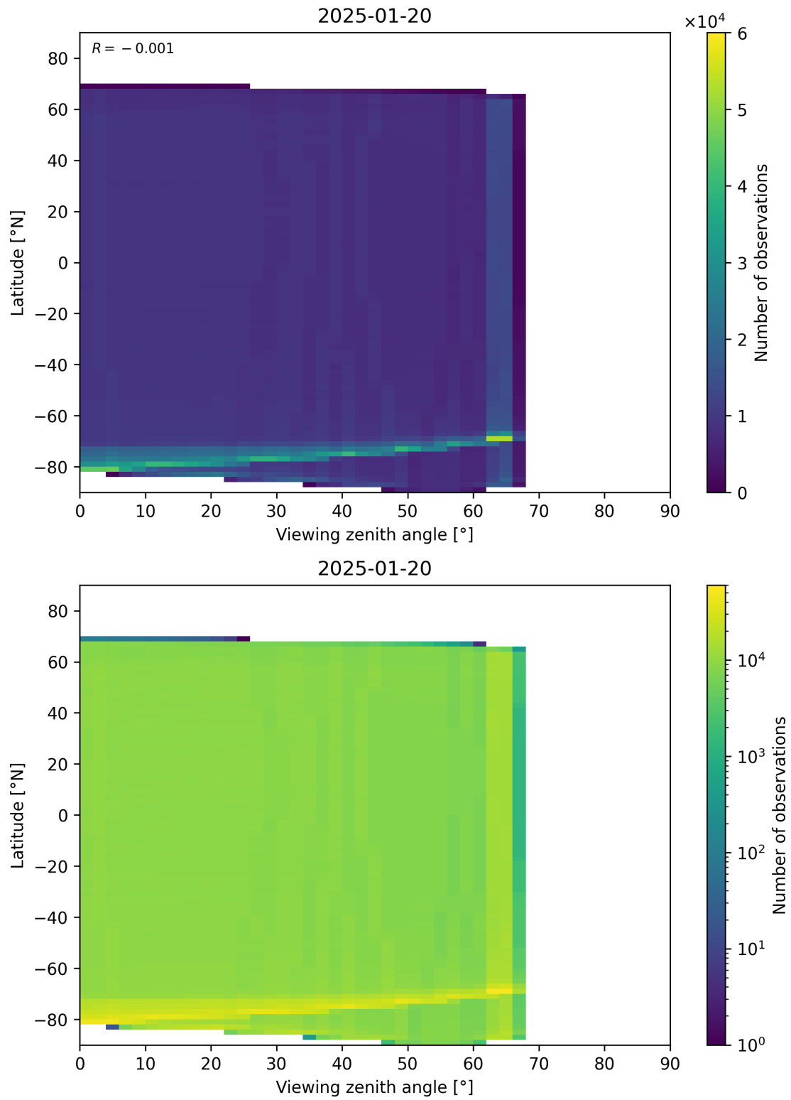
Figure 123: Scatter density plot of “Viewing zenith angle” against “Latitude” for 2025-01-19 to 2025-01-21.
