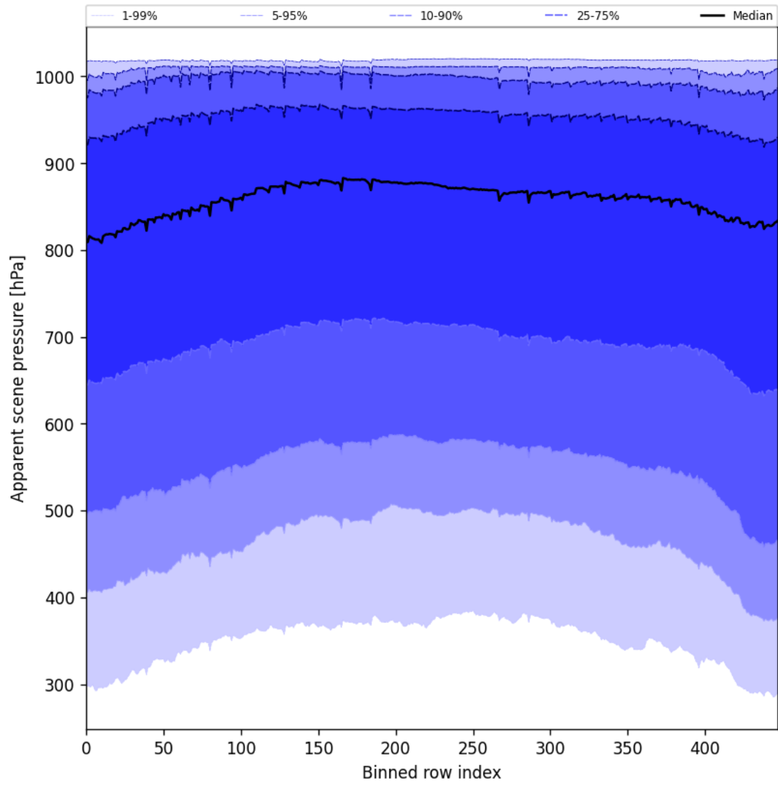
Figure 53: Along track statistics of “Apparent scene pressure” for 2025-01-19 to 2025-01-21
