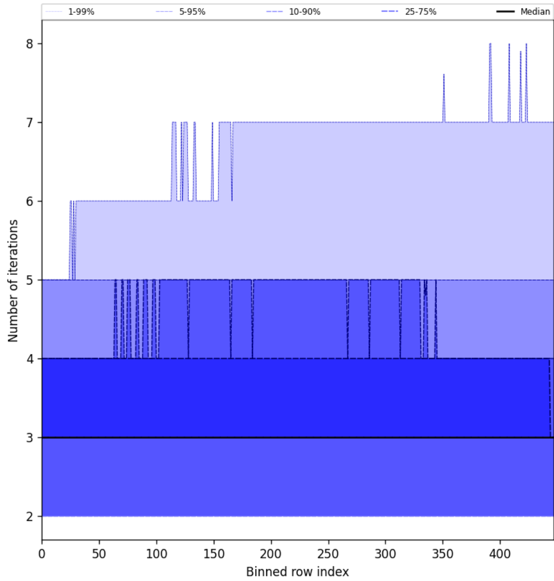
Figure 56: Along track statistics of “Number of iterations” for 2025-01-19 to 2025-01-21
