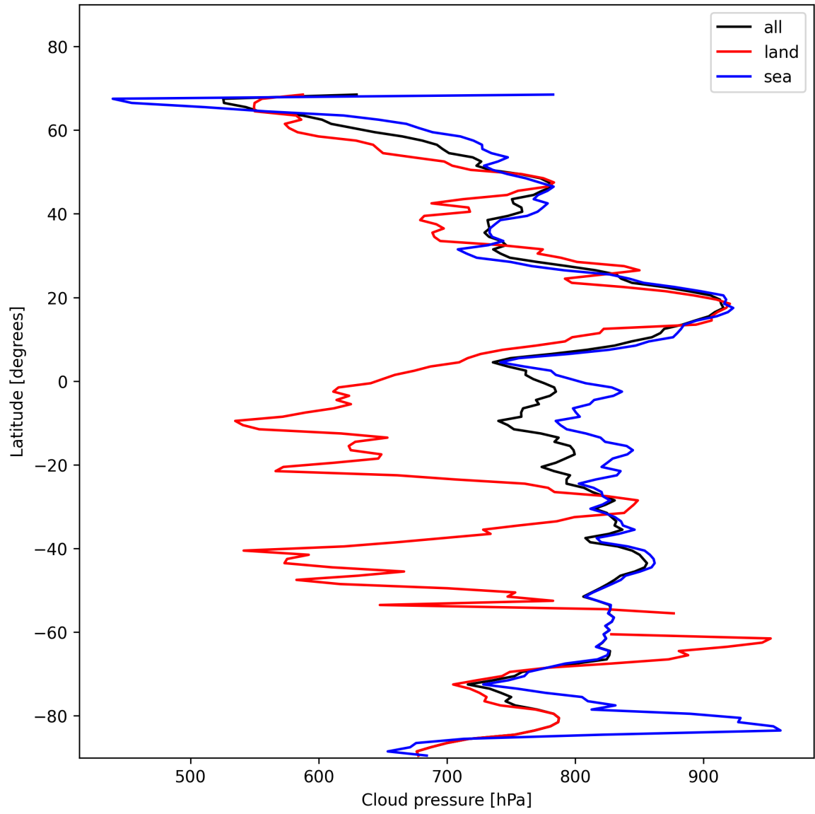
Figure 13: Zonal average of “Cloud pressure” for 2025-01-19 to 2025-01-21.
