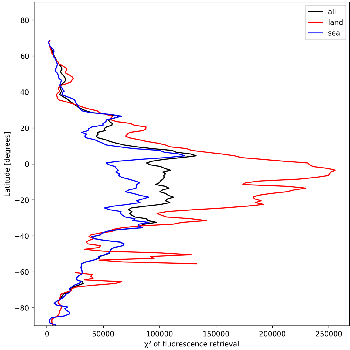
Figure 25: Zonal average of “ \chi^2 of fluorescence retrieval” for 2025-01-19 to 2025-01-21.
