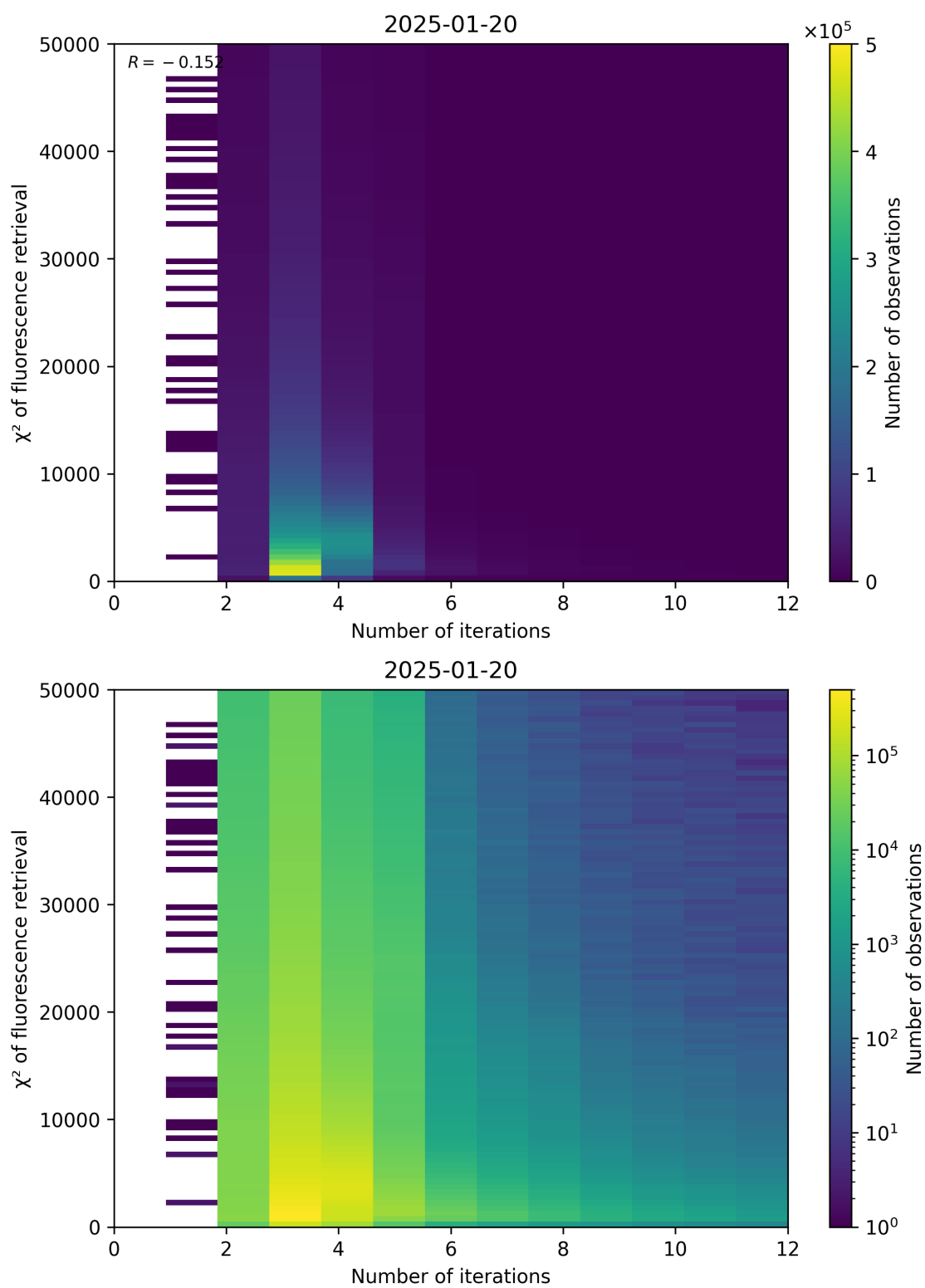
Figure 97: Scatter density plot of “Number of iterations” against “ \chi^2 of fluorescence retrieval” for 2025-01-19 to 2025-01-21.
