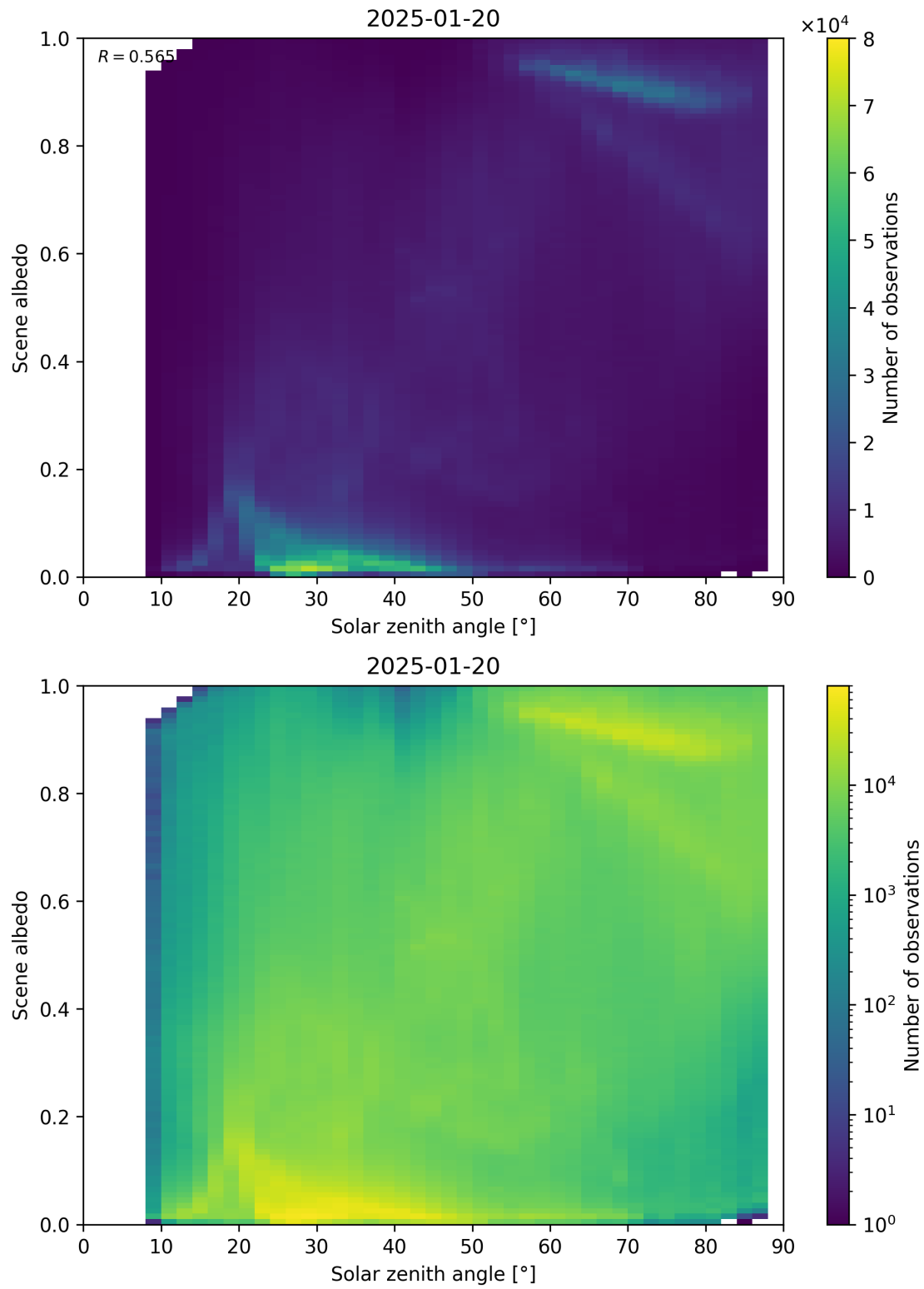
Figure 116: Scatter density plot of “Solar zenith angle” against “Scene albedo” for 2025-01-19 to 2025-01-21.
