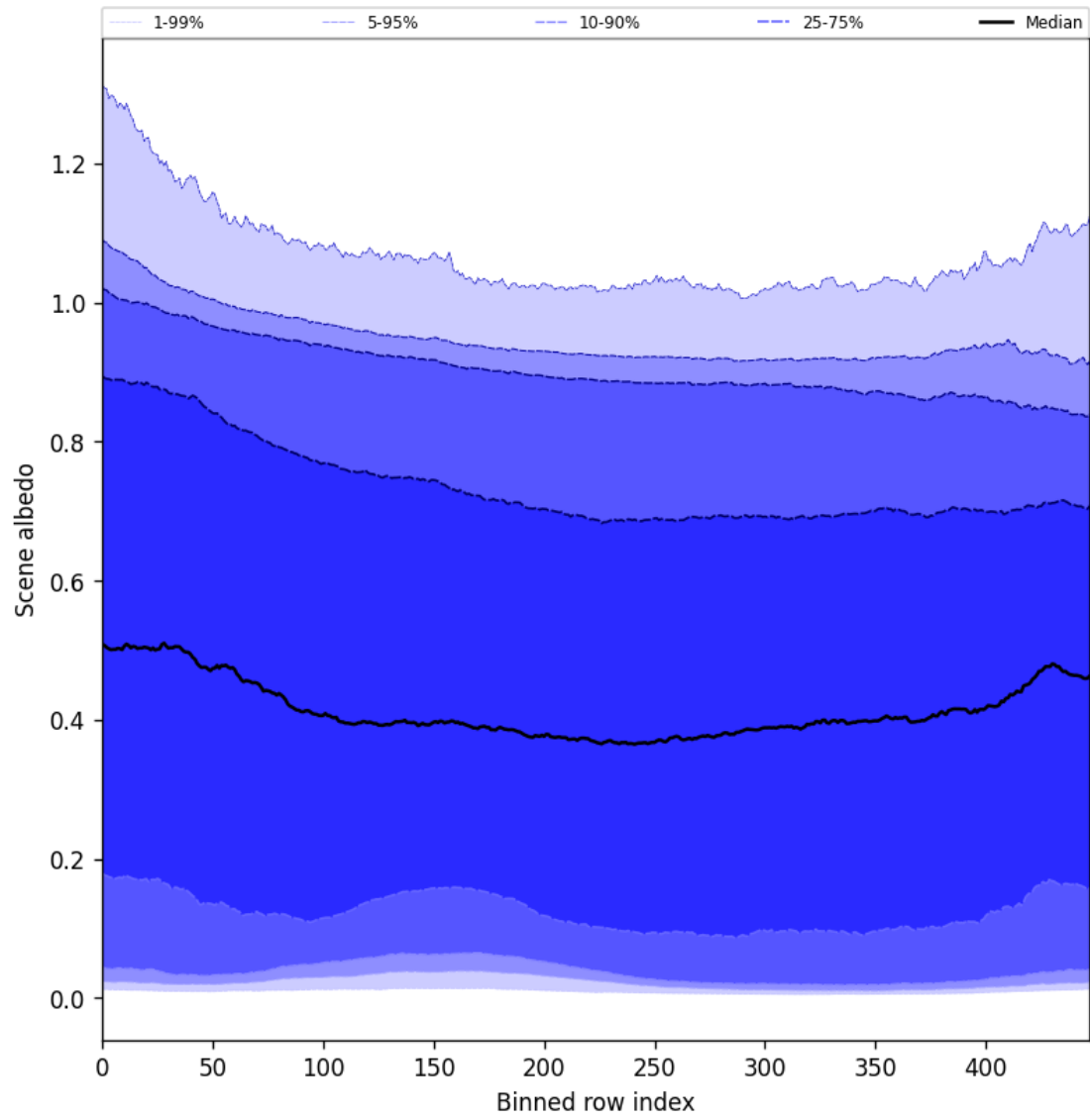
Figure 51: Along track statistics of “Scene albedo” for 2025-01-19 to 2025-01-21
