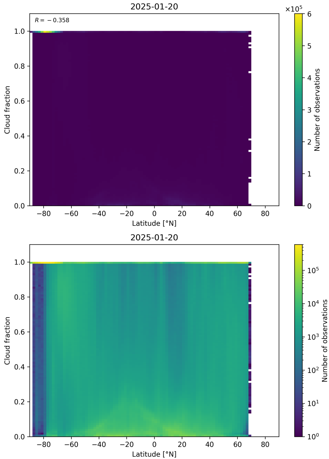
Figure 90: Scatter density plot of “Latitude” against “Cloud fraction” for 2025-01-19 to 2025-01-21.
