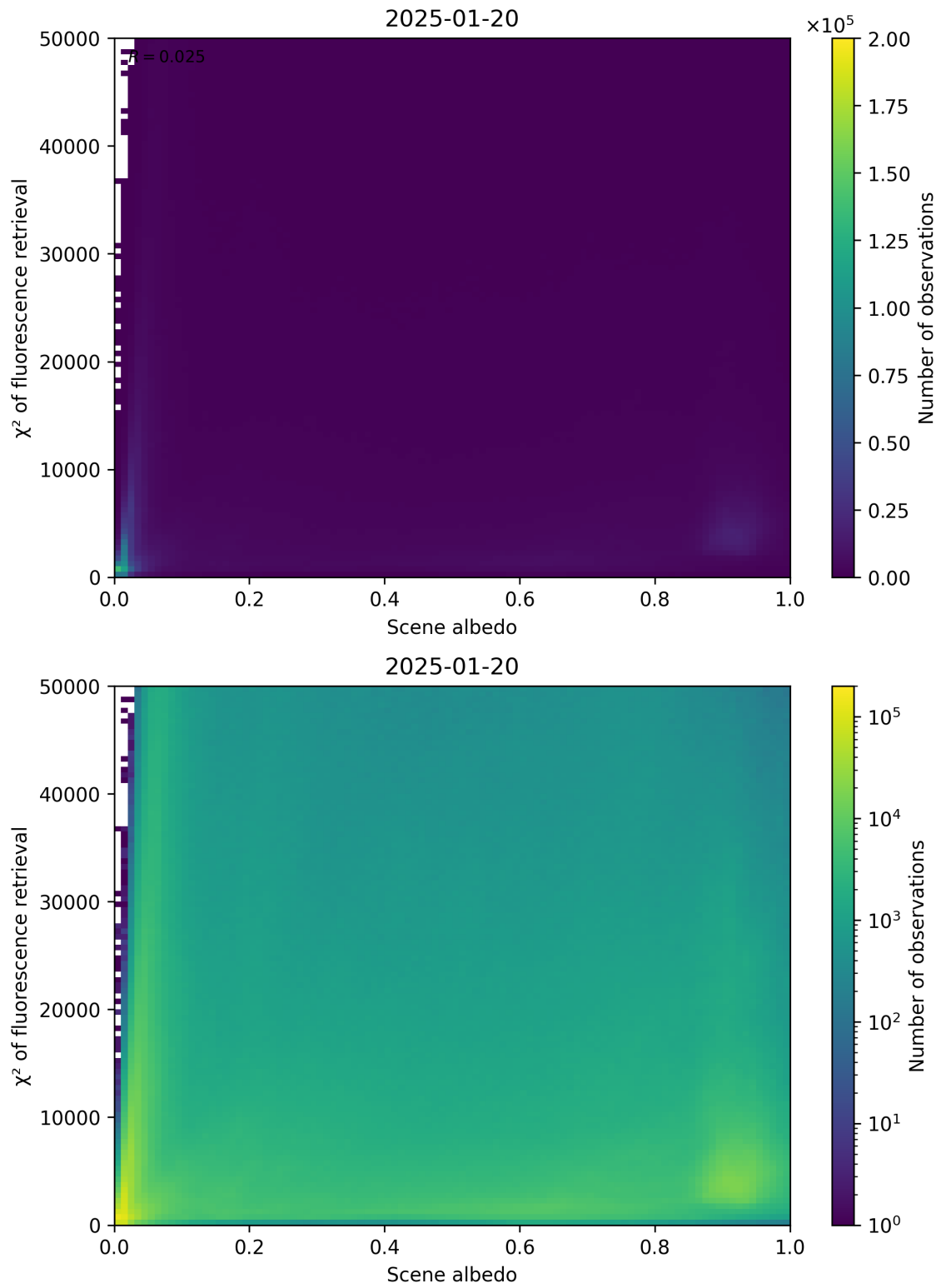
Figure 103: Scatter density plot of “Scene albedo” against “ \chi^2 of fluorescence retrieval” for 2025-01-19 to 2025-01-21.
