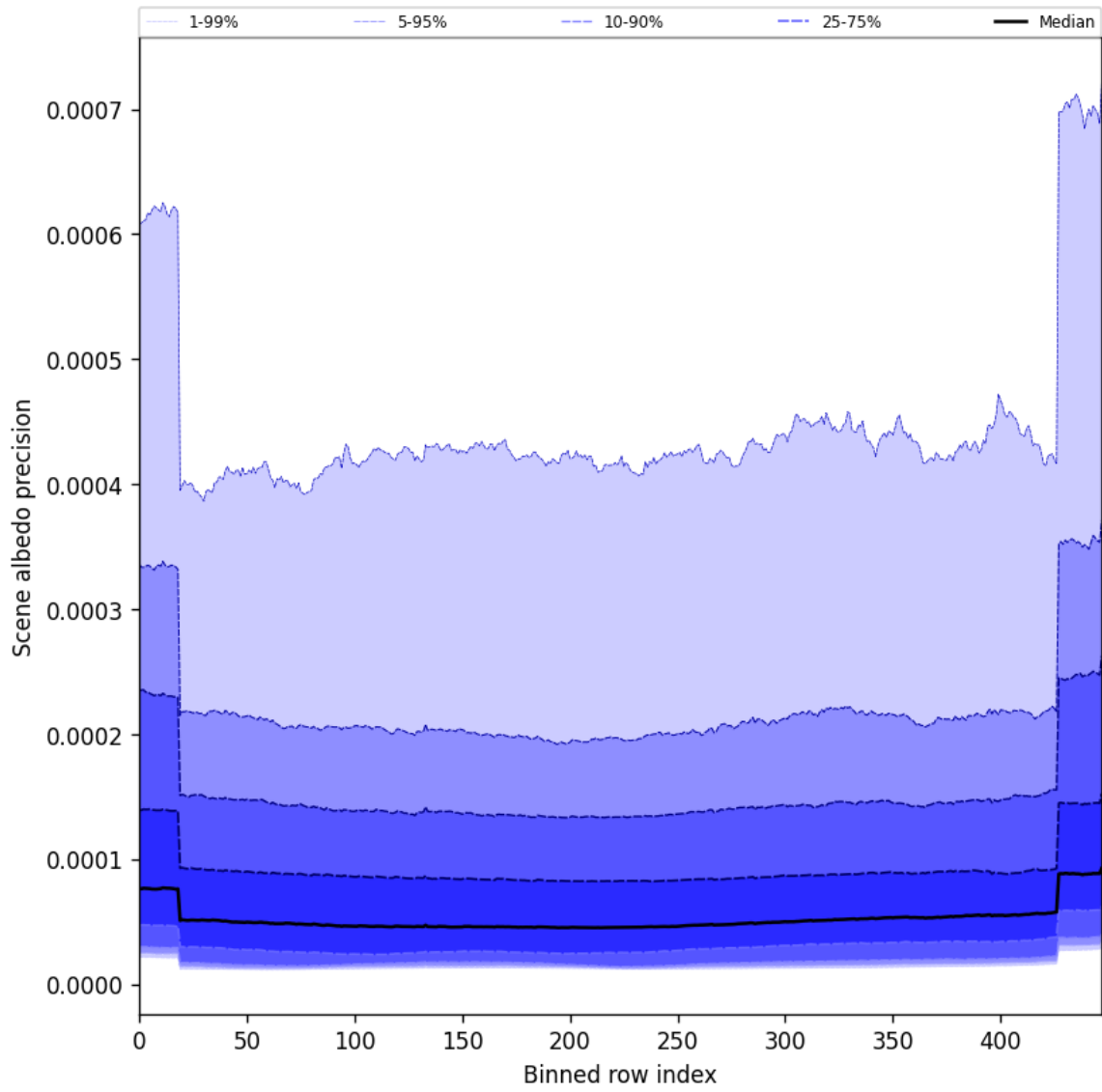
Figure 52: Along track statistics of “Scene albedo precision” for 2025-01-19 to 2025-01-21
