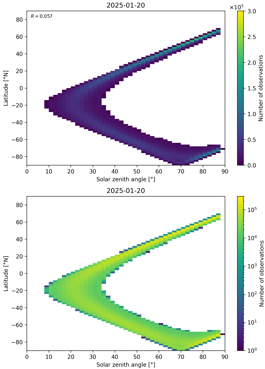
Figure 113: Scatter density plot of “Solar zenith angle” against “Latitude” for 2025-01-19 to 2025-01-21.
