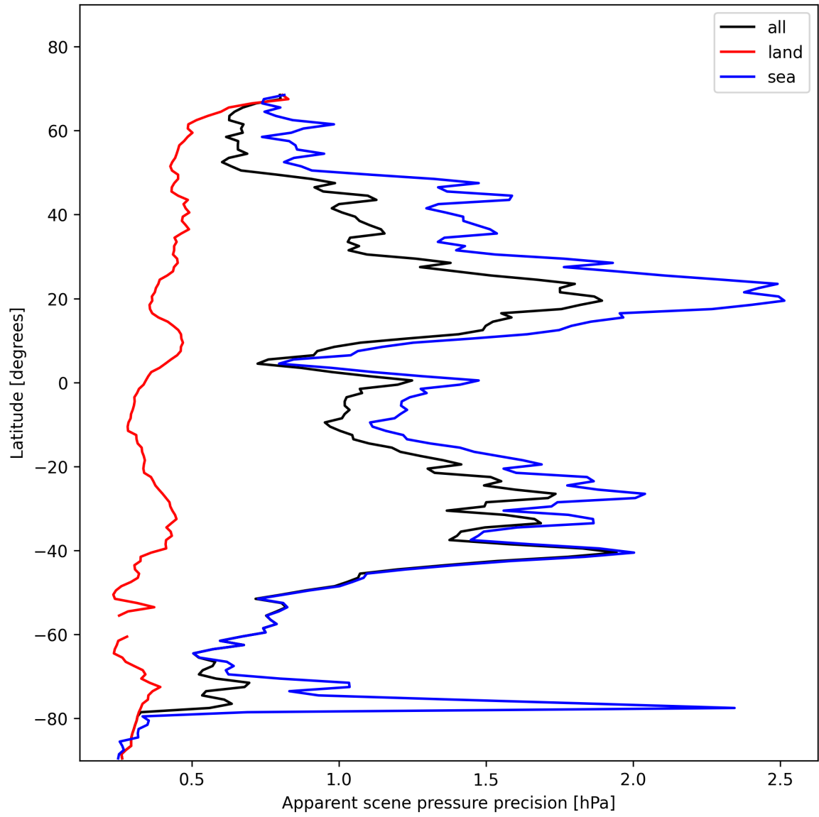
Figure 20: Zonal average of “Apparent scene pressure precision” for 2025-01-19 to 2025-01-21.
