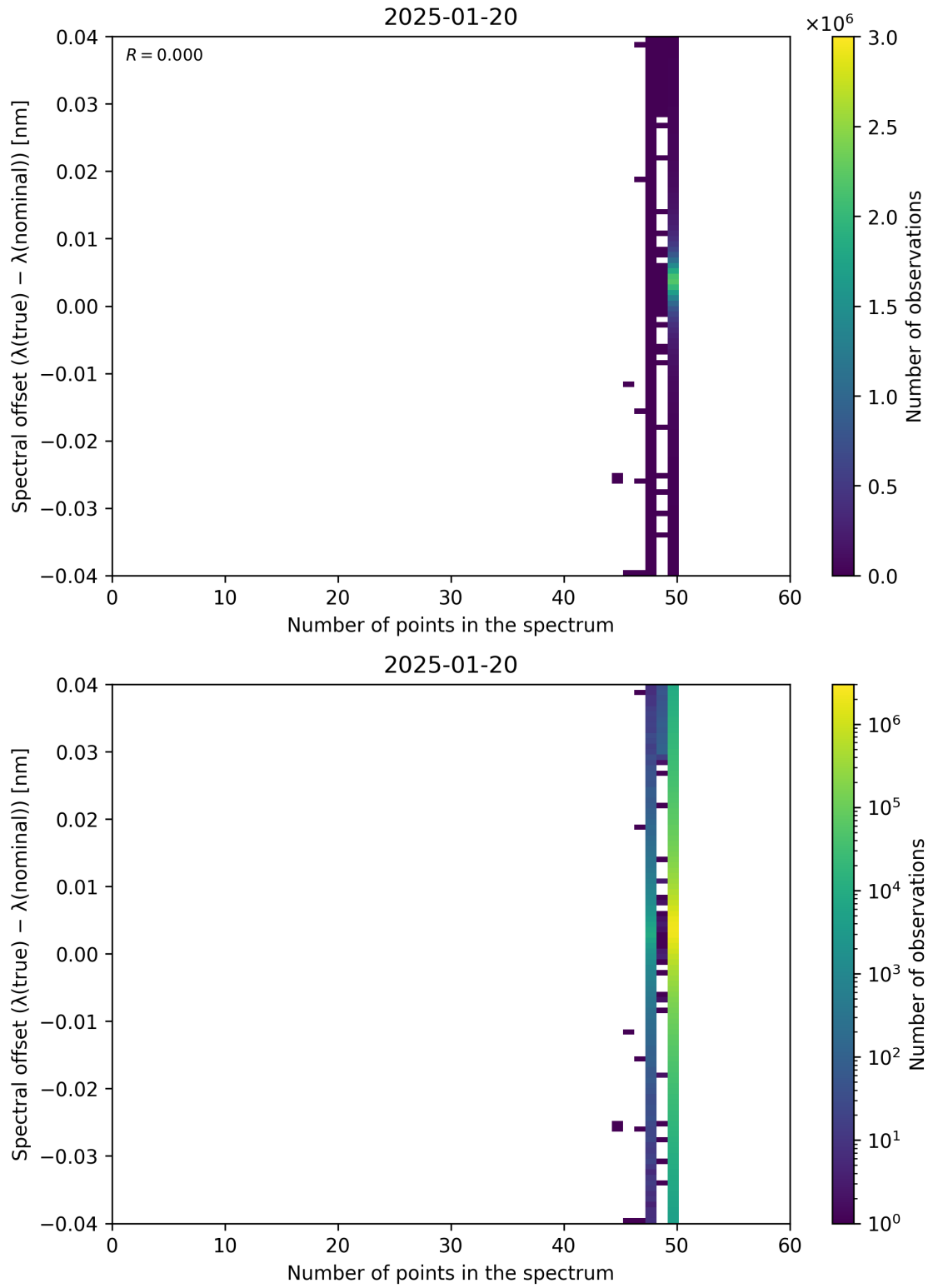
Figure 101: Scatter density plot of “Number of points in the spectrum” against “Spectral offset ( \lambda_{\text{true}} - \lambda_{\text{nominal}} )” for 2025-01-19 to 2025-01-21.
