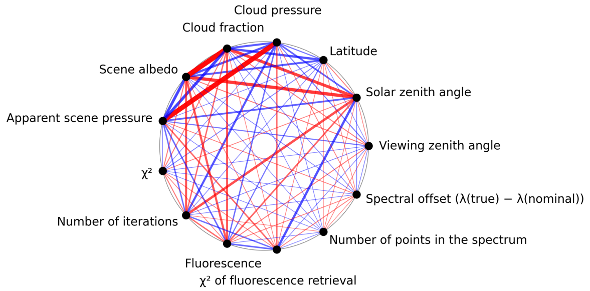
Figure 1: Map of correlation graph for 2025-01-19 to 2025-01-21.
