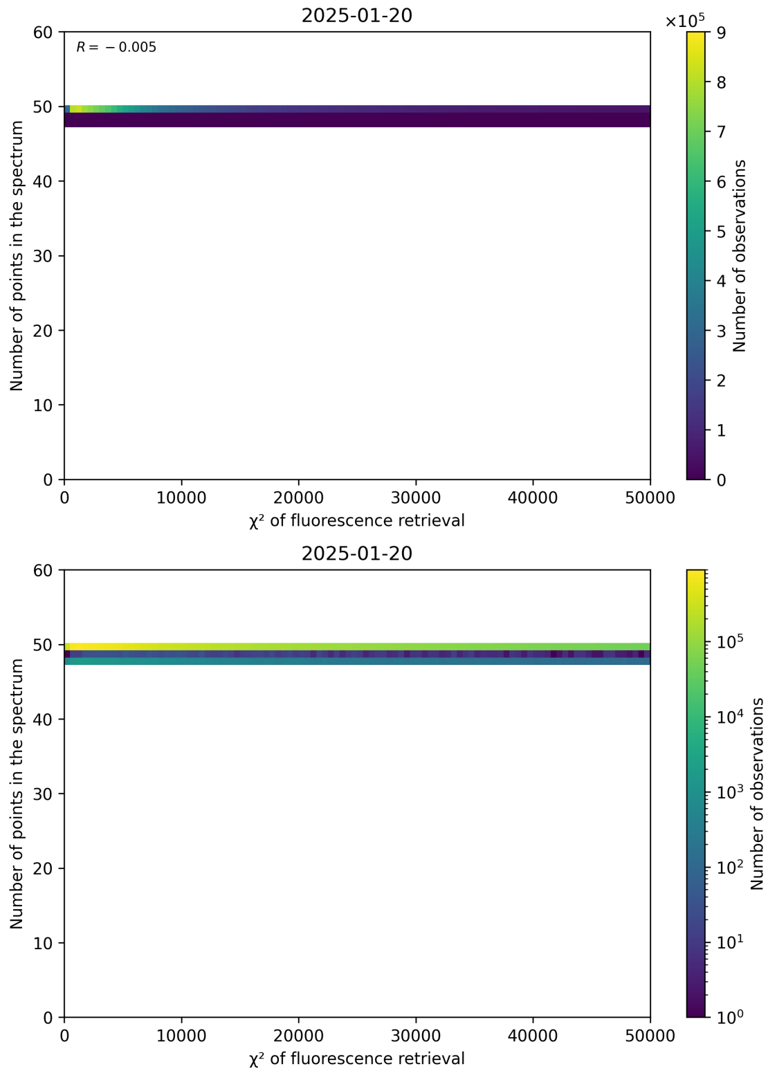
Figure 68: Scatter density plot of “ \chi^2 of fluorescence retrieval” against “Number of points in the spectrum” for 2025-01-19 to 2025-01-21.
