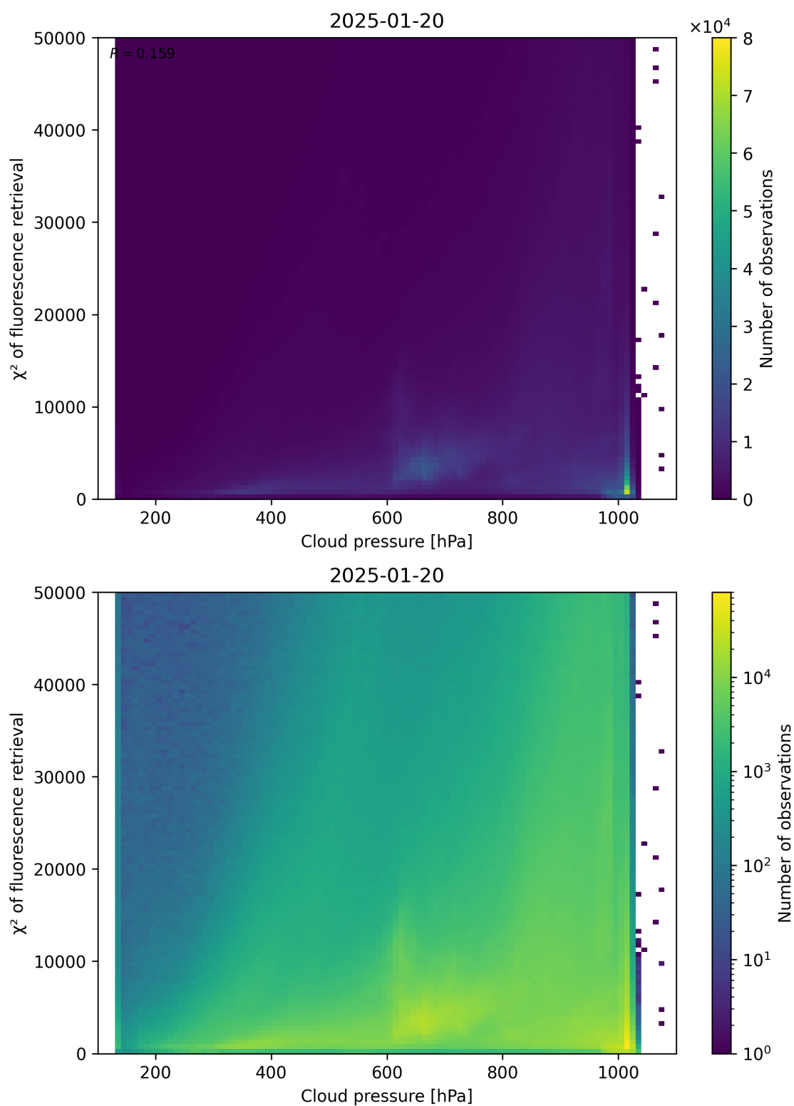
Figure 78: Scatter density plot of “Cloud pressure” against “ \chi^2 of fluorescence retrieval” for 2025-01-19 to 2025-01-21.
