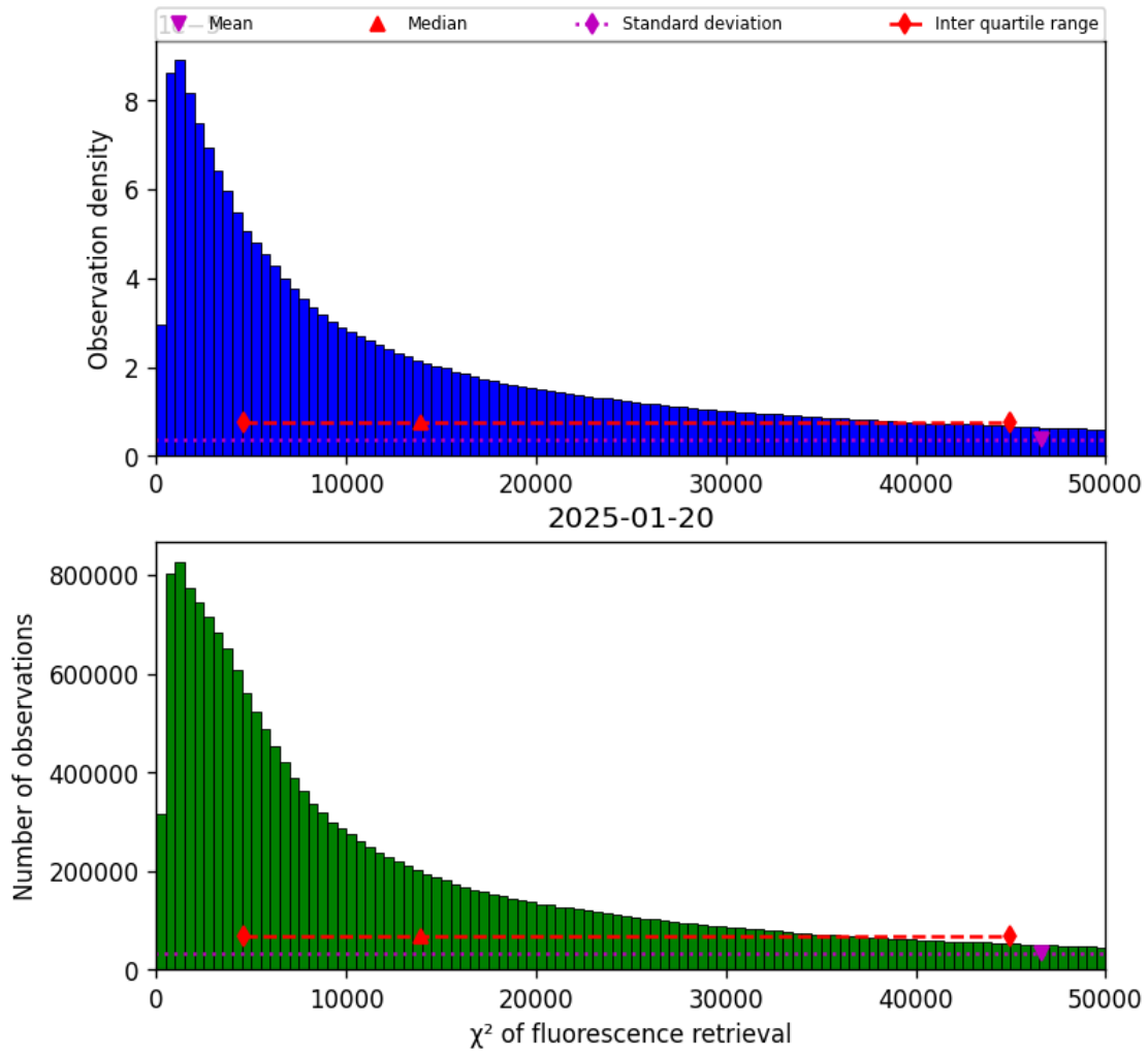
Figure 42: Histogram of “ \chi^2 of fluorescence retrieval” for 2025-01-19 to 2025-01-21
