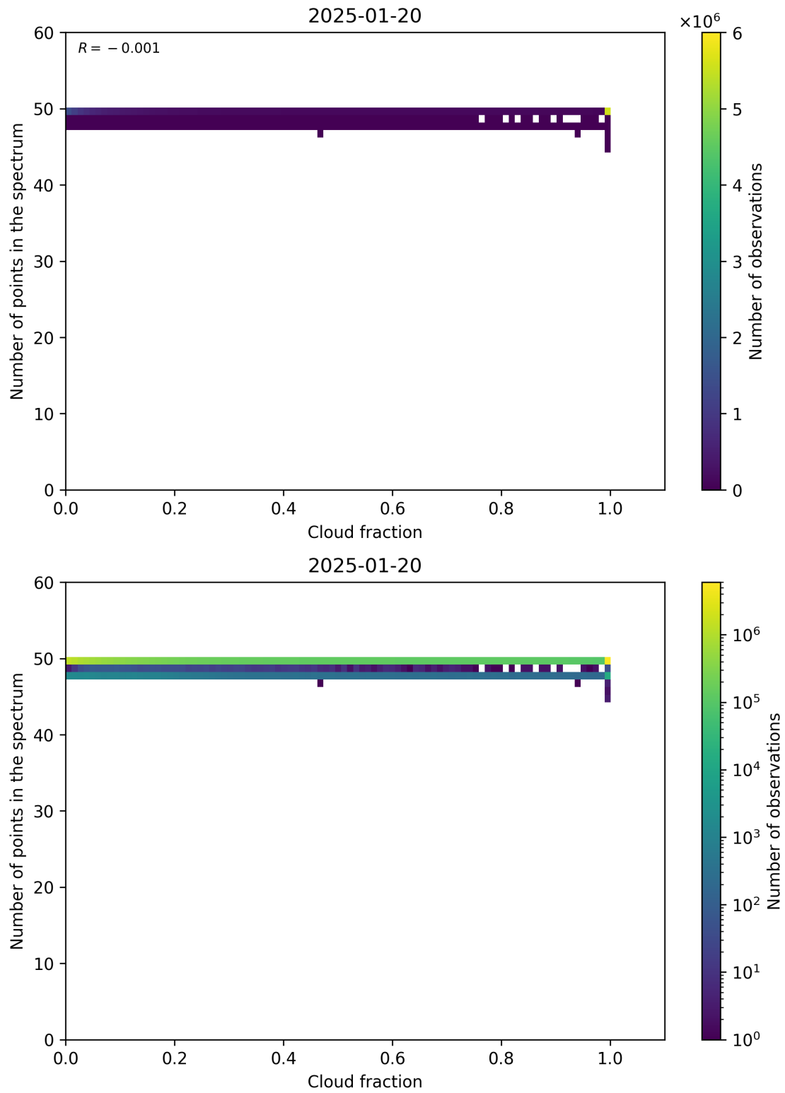
Figure 74: Scatter density plot of “Cloud fraction” against “Number of points in the spectrum” for 2025-01-19 to 2025-01-21.
