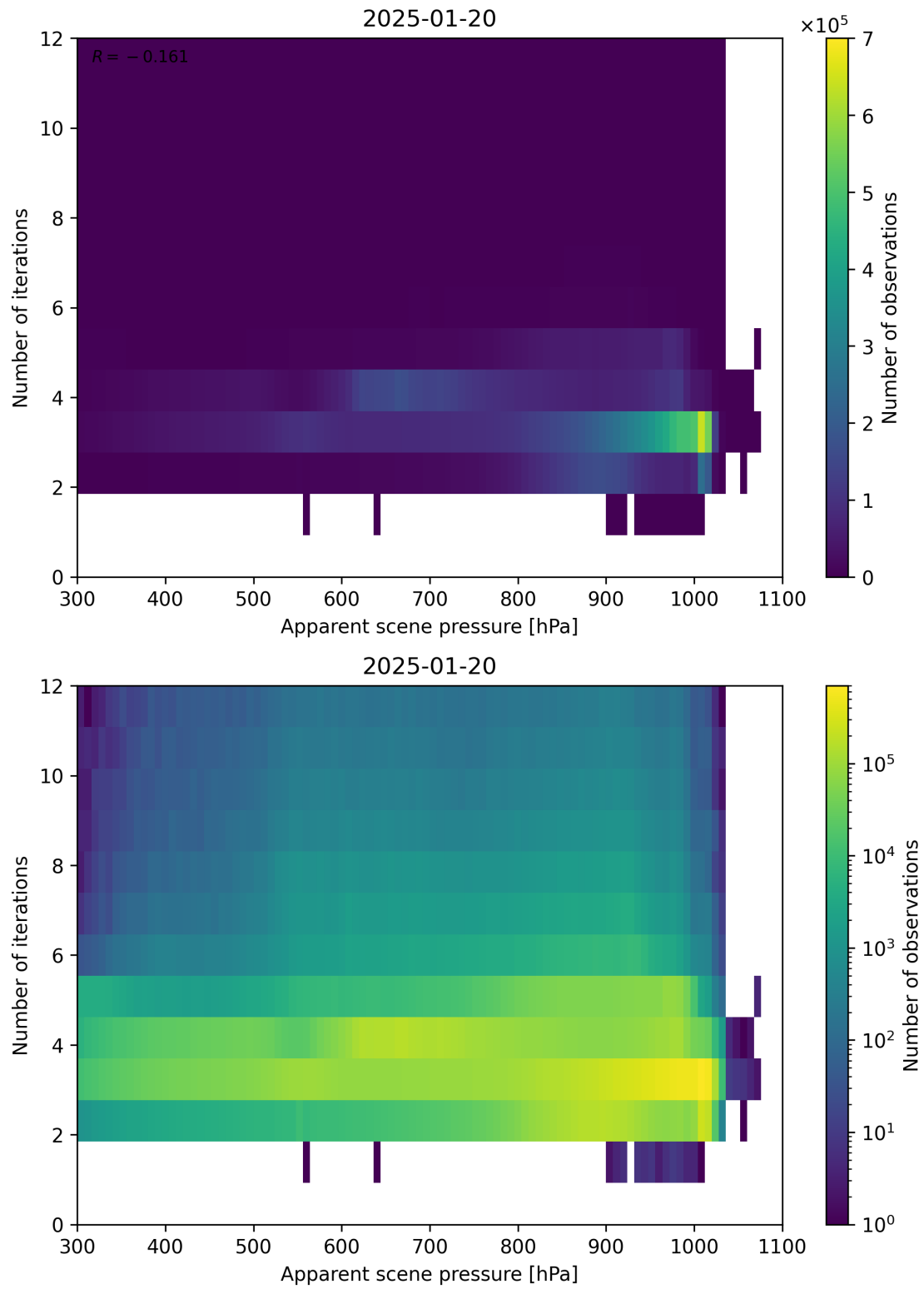
Figure 65: Scatter density plot of “Apparent scene pressure” against “Number of iterations” for 2025-01-19 to 2025-01-21.
