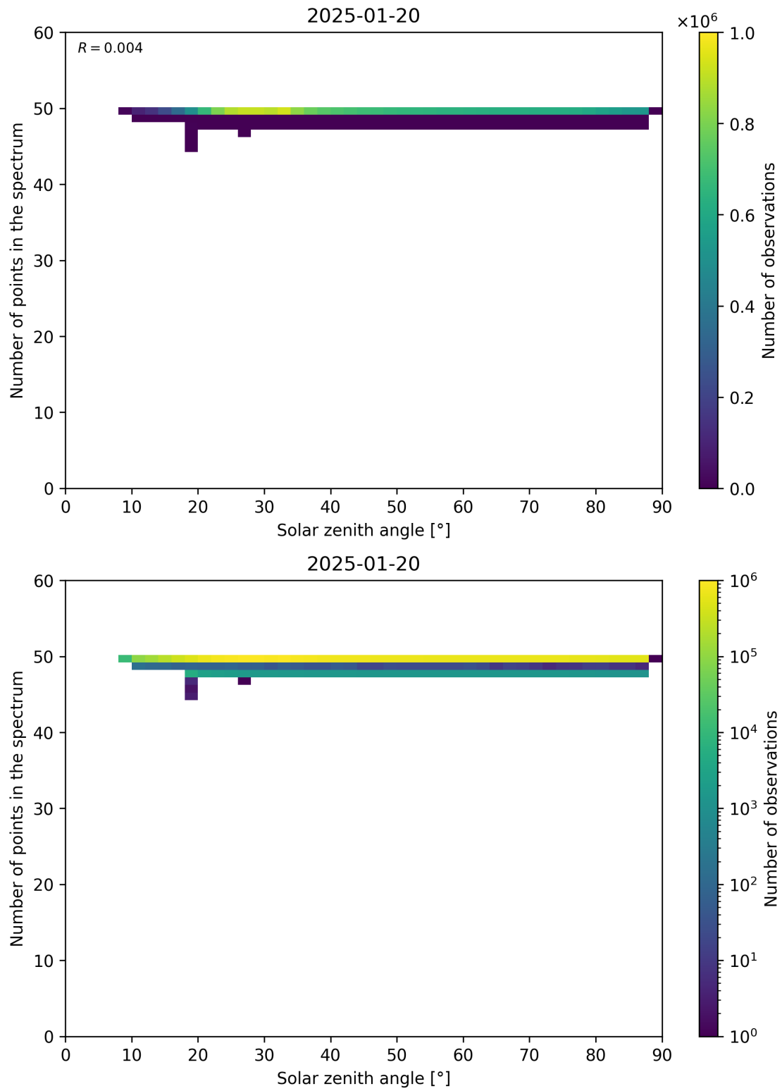
Figure 115: Scatter density plot of “Solar zenith angle” against “Number of points in the spectrum” for 2025-01-19 to 2025-01-21.
