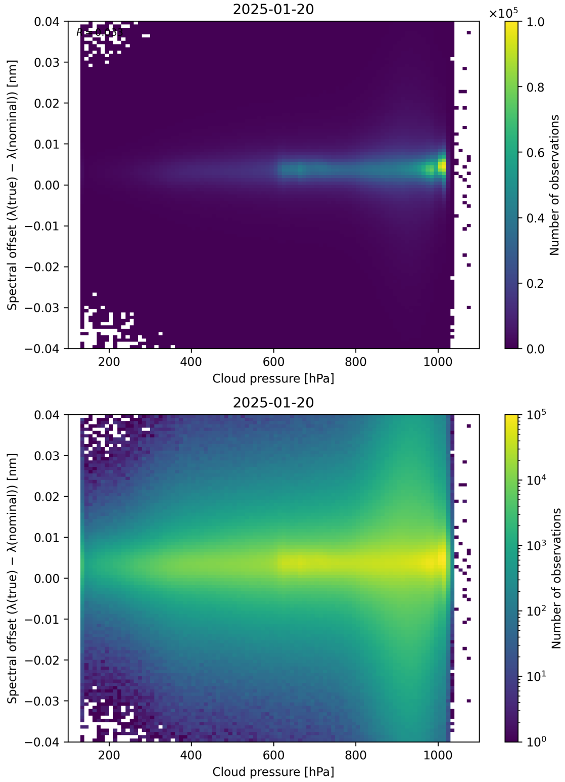
Figure 84: Scatter density plot of “Cloud pressure” against “Spectral offset ( \lambda_{\text{true}} - \lambda_{\text{nominal}} )” for 2025-01-19 to 2025-01-21.
