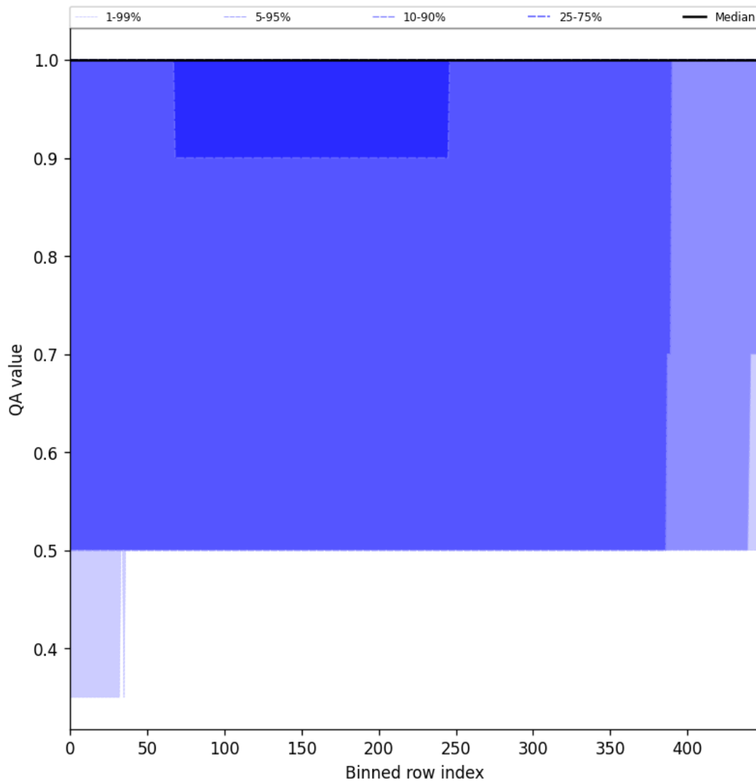
Figure 46: Along track statistics of “QA value” for 2025-01-19 to 2025-01-21
