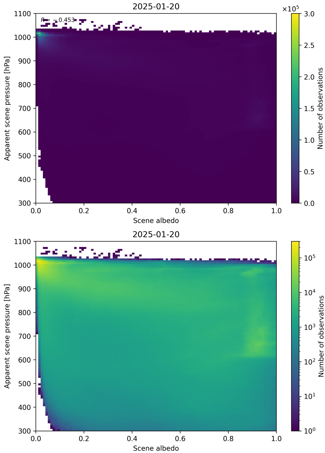
Figure 102: Scatter density plot of “Scene albedo” against “Apparent scene pressure” for 2025-01-19 to 2025-01-21.
