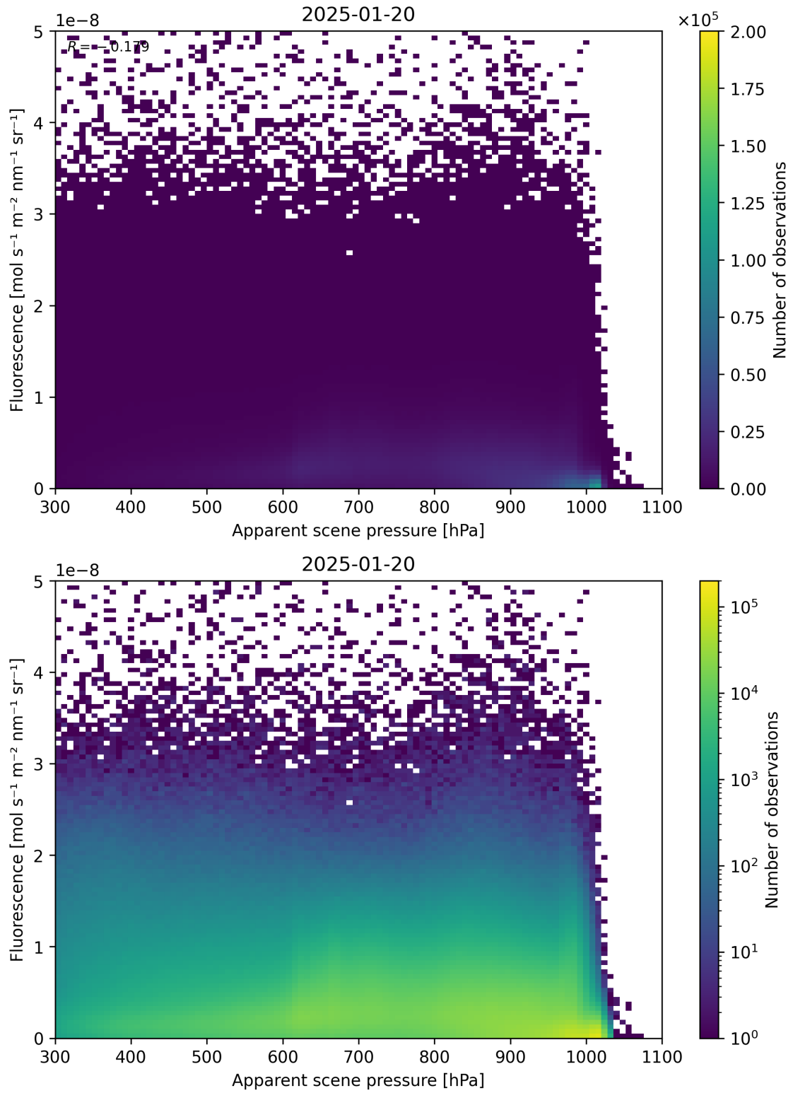
Figure 64: Scatter density plot of “Apparent scene pressure” against “Fluorescence” for 2025-01-19 to 2025-01-21.
