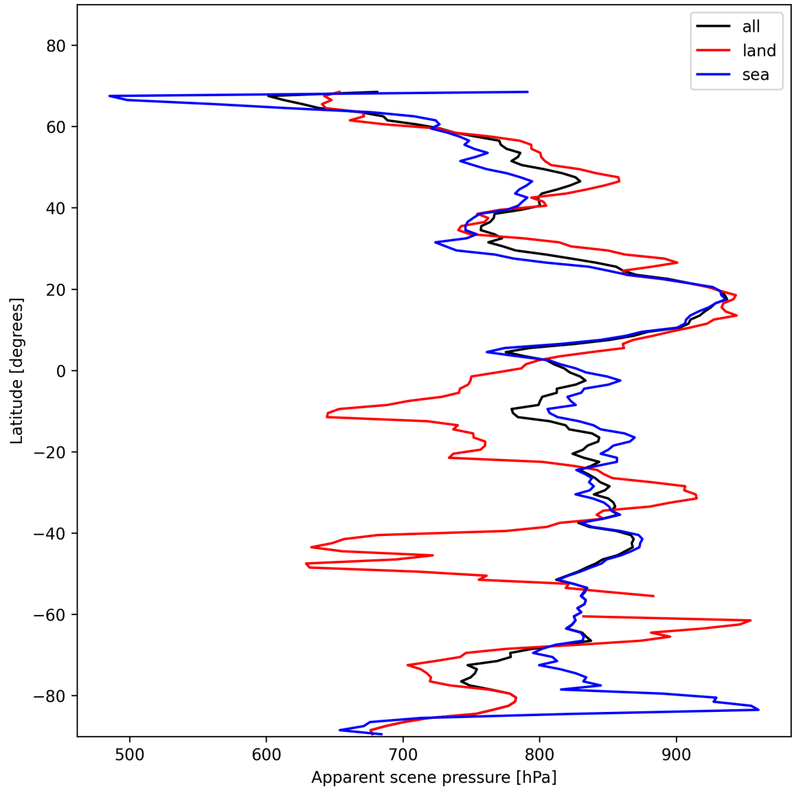
Figure 19: Zonal average of “Apparent scene pressure” for 2025-01-19 to 2025-01-21.
