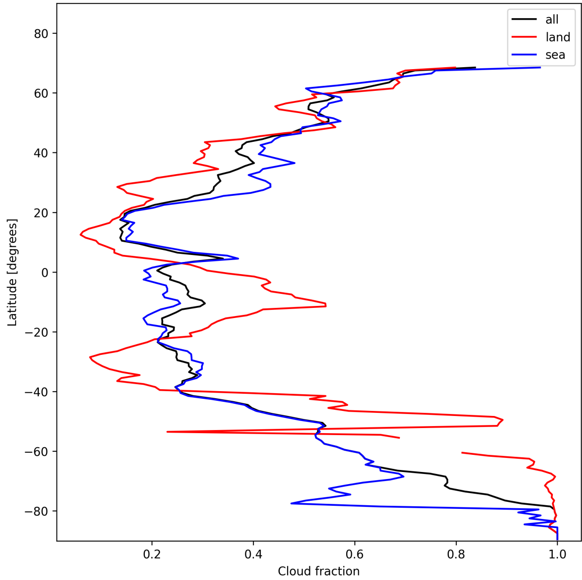
Figure 15: Zonal average of “Cloud fraction” for 2025-01-19 to 2025-01-21.
