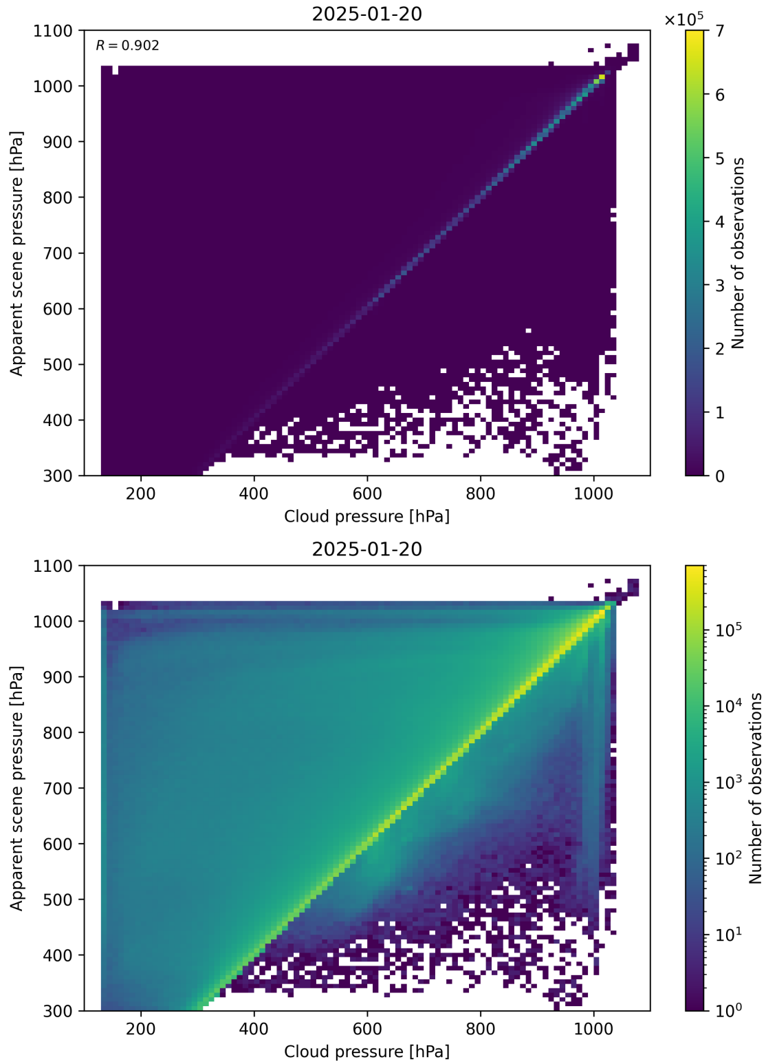
Figure 77: Scatter density plot of “Cloud pressure” against “Apparent scene pressure” for 2025-01-19 to 2025-01-21.
