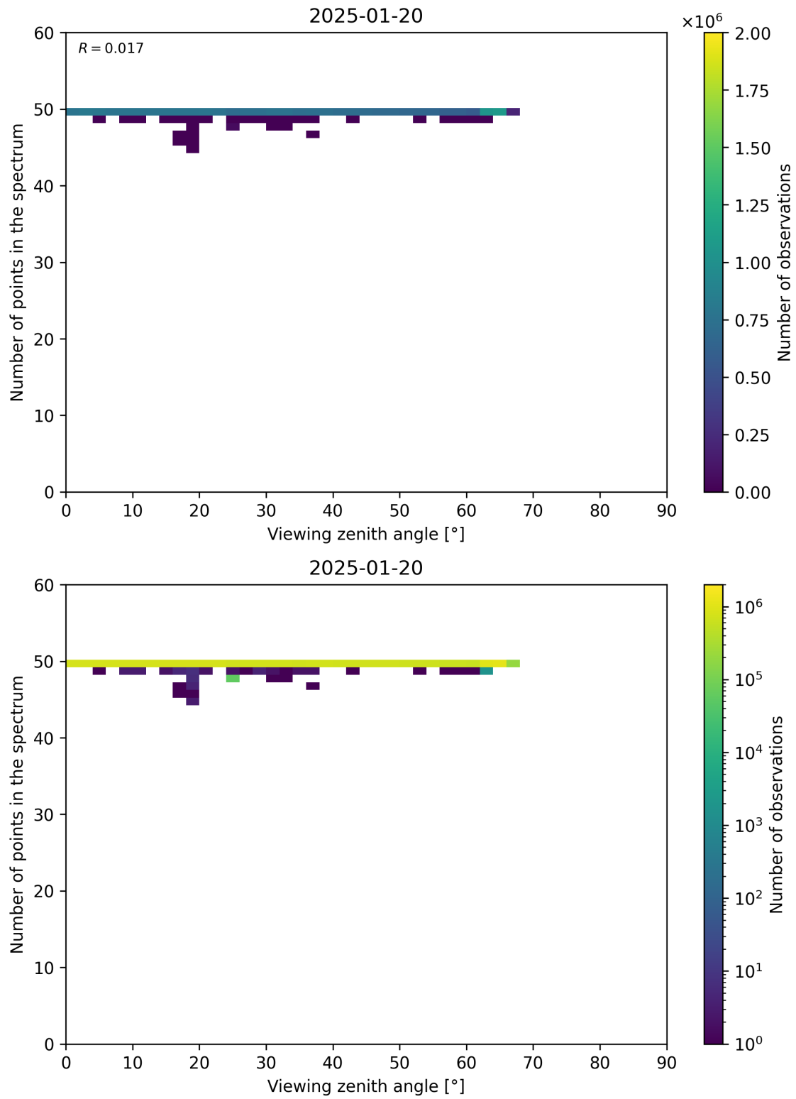
Figure 125: Scatter density plot of “Viewing zenith angle” against “Number of points in the spectrum” for 2025-01-19 to 2025-01-21.
