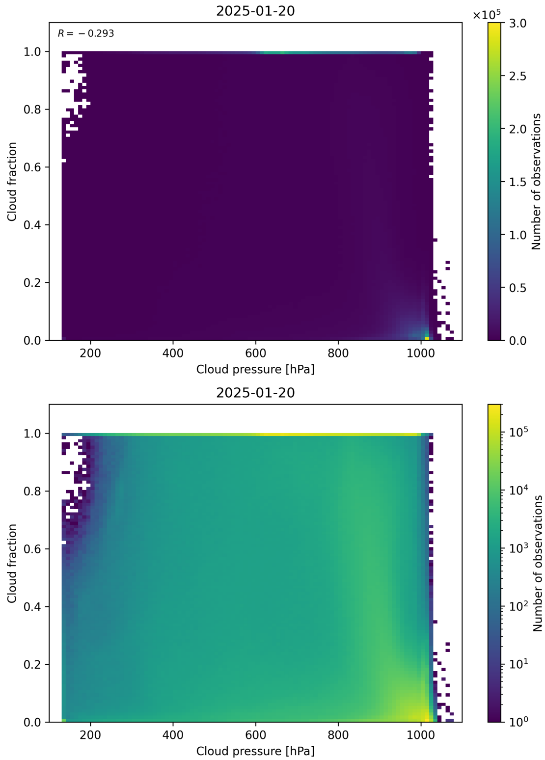
Figure 79: Scatter density plot of “Cloud pressure” against “Cloud fraction” for 2025-01-19 to 2025-01-21.
