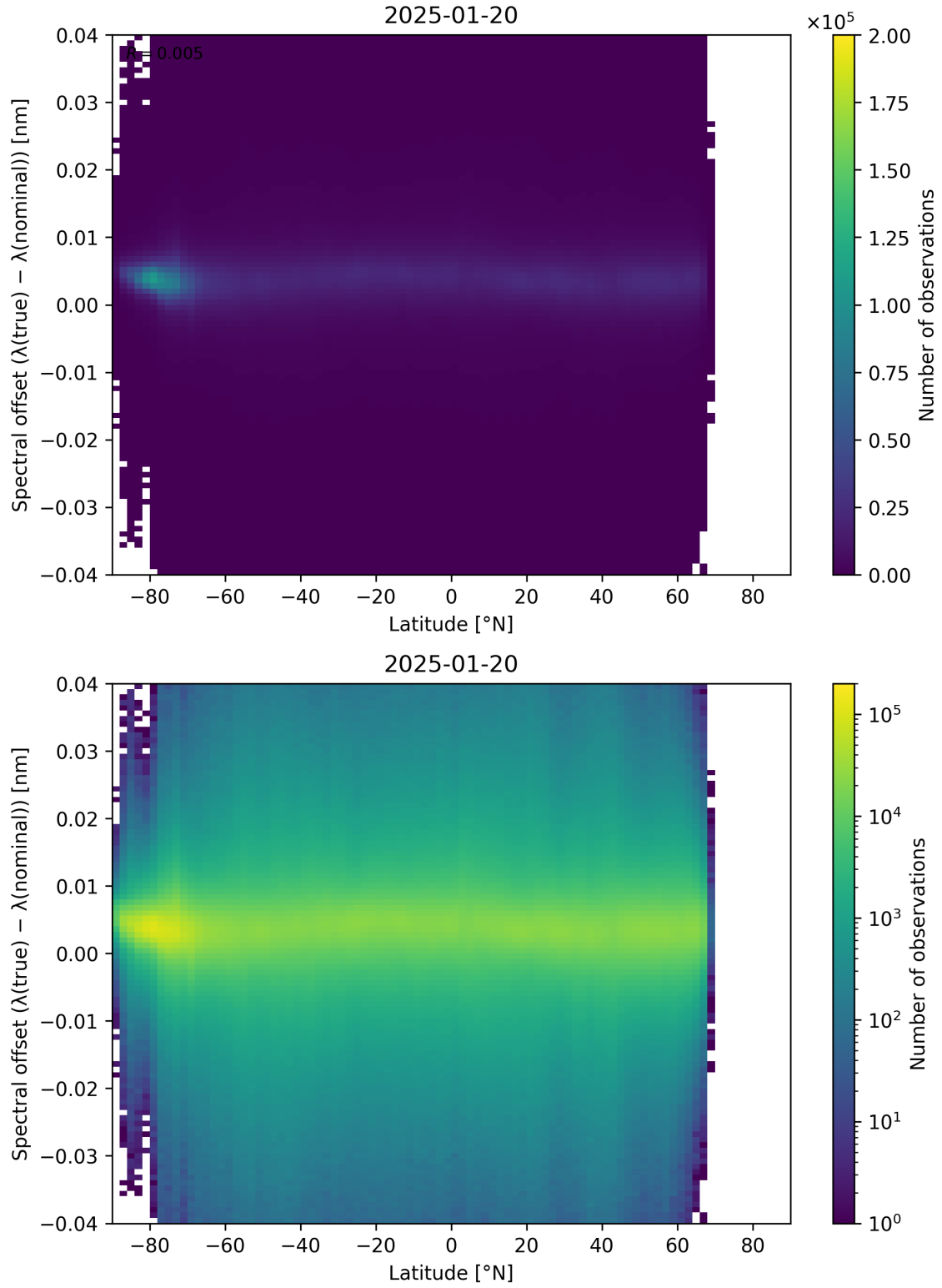
Figure 96: Scatter density plot of “Latitude” against “Spectral offset ( \lambda_{\text{true}} - \lambda_{\text{nominal}} )” for 2025-01-19 to 2025-01-21.
