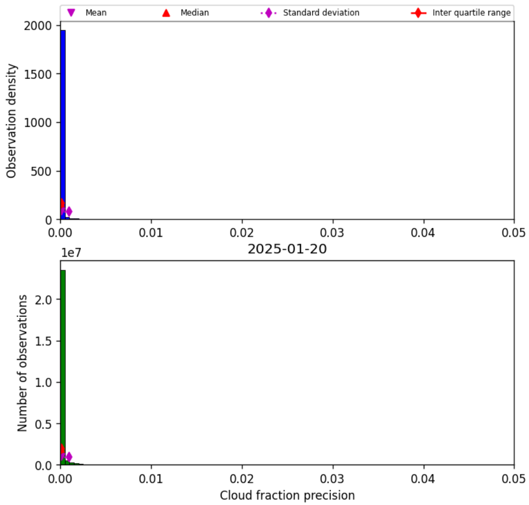
Figure 33: Histogram of “Cloud fraction precision” for 2025-01-19 to 2025-01-21
