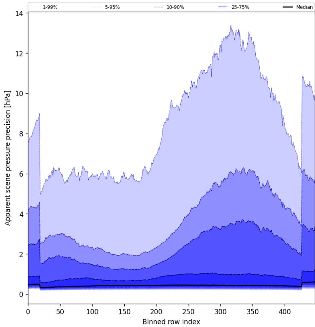
Figure 54: Along track statistics of “Apparent scene pressure precision” for 2025-01-19 to 2025-01-21
