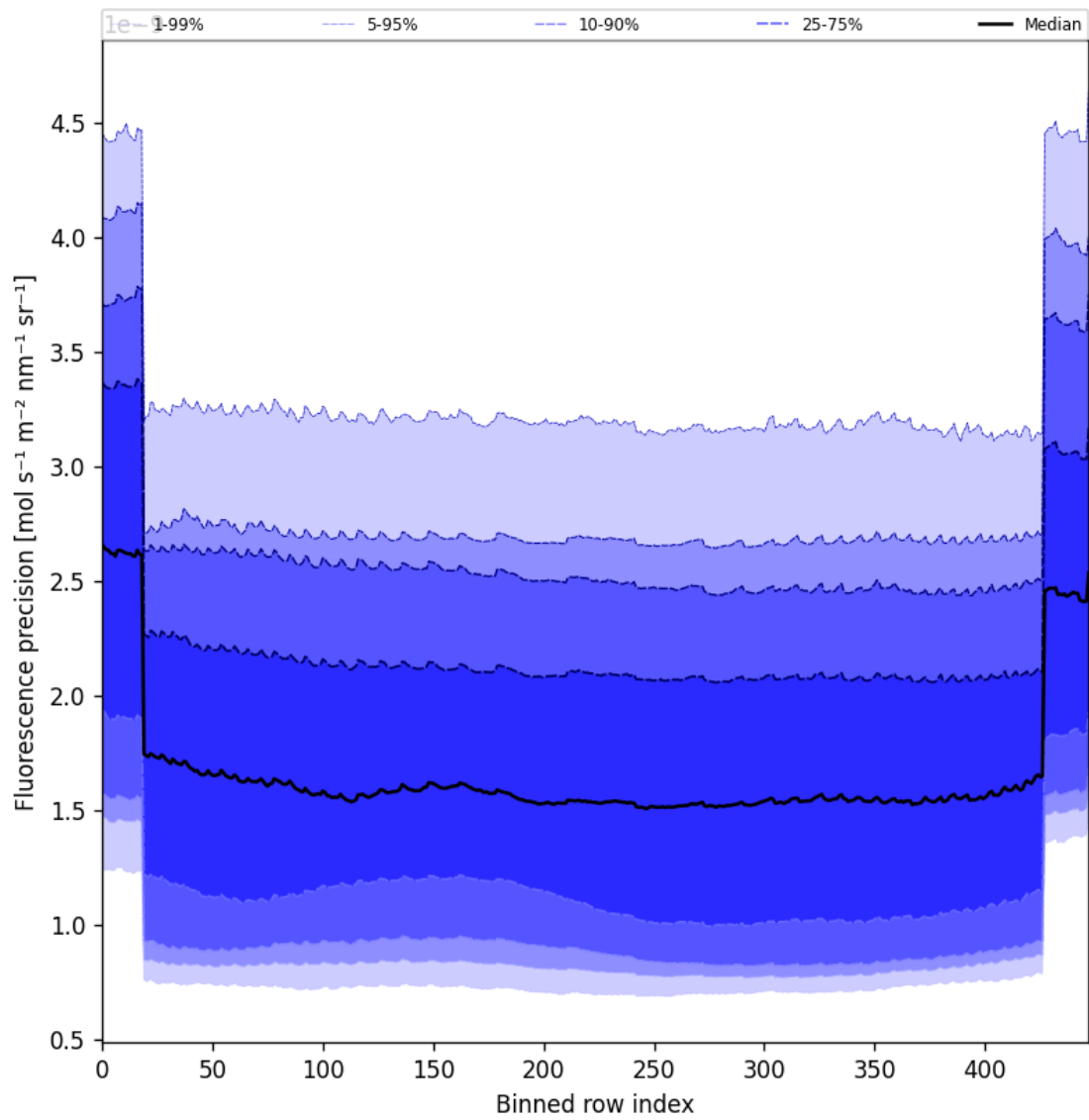
Figure 58: Along track statistics of “Fluorescence precision” for 2025-01-19 to 2025-01-21
