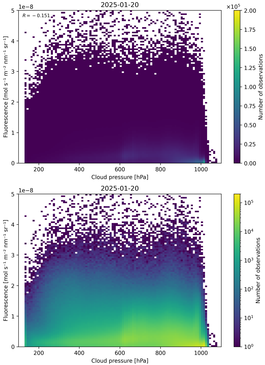
Figure 80: Scatter density plot of “Cloud pressure” against “Fluorescence” for 2025-01-19 to 2025-01-21.
