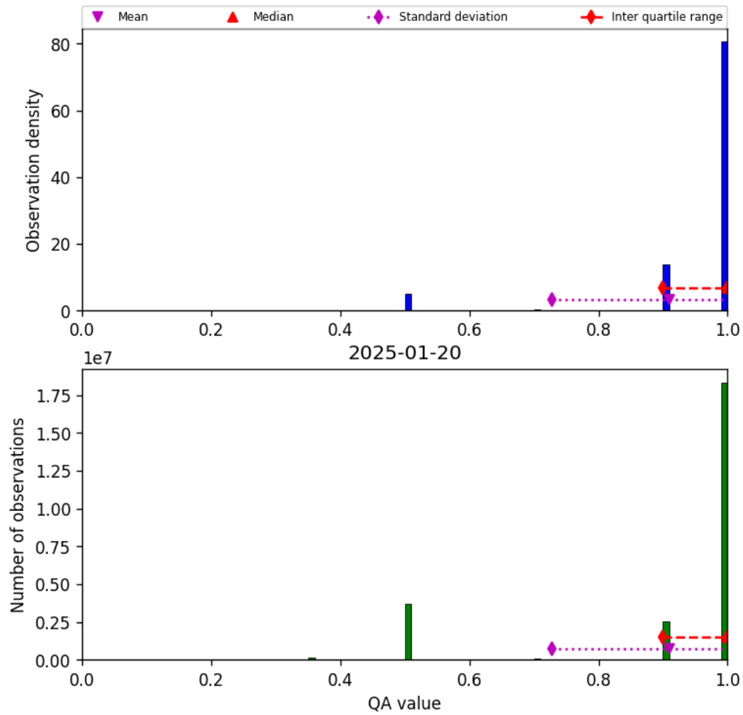
Figure 29: Histogram of “QA value” for 2025-01-19 to 2025-01-21
