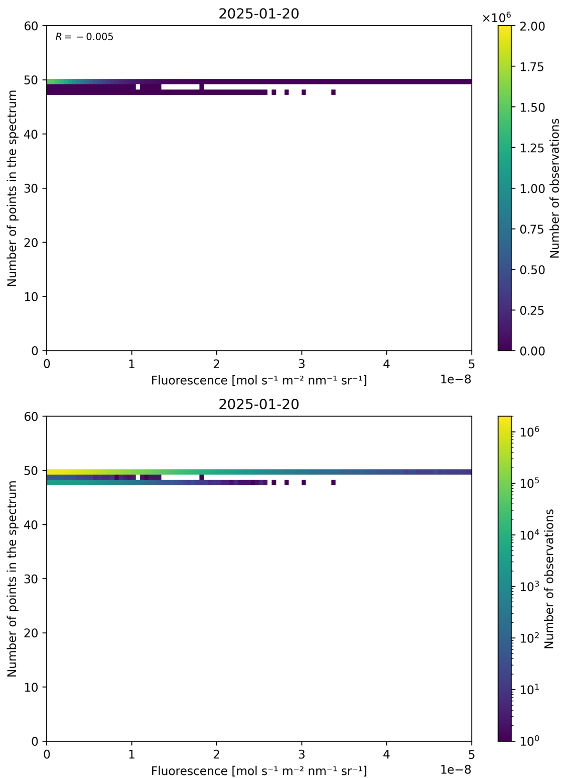
Figure 86: Scatter density plot of “Fluorescence” against “Number of points in the spectrum” for 2025-01-19 to 2025-01-21.
