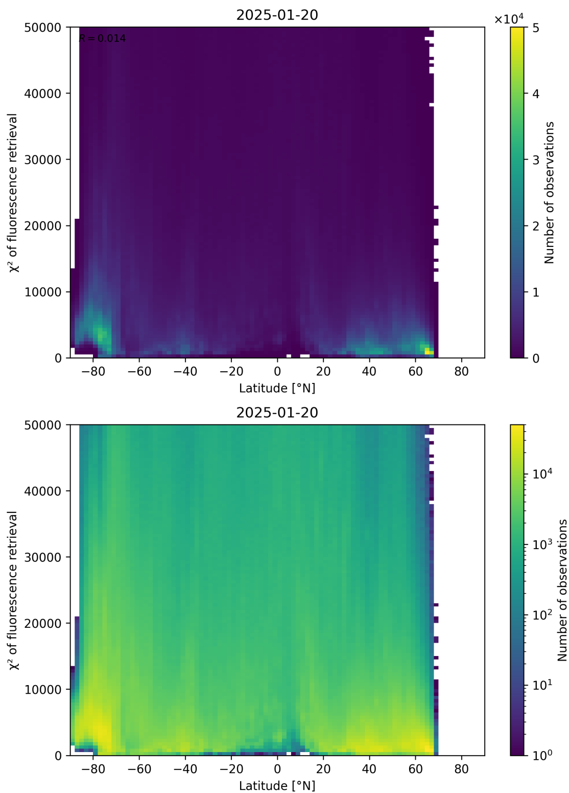
Figure 89: Scatter density plot of “Latitude” against “ \chi^2 of fluorescence retrieval” for 2025-01-19 to 2025-01-21.
