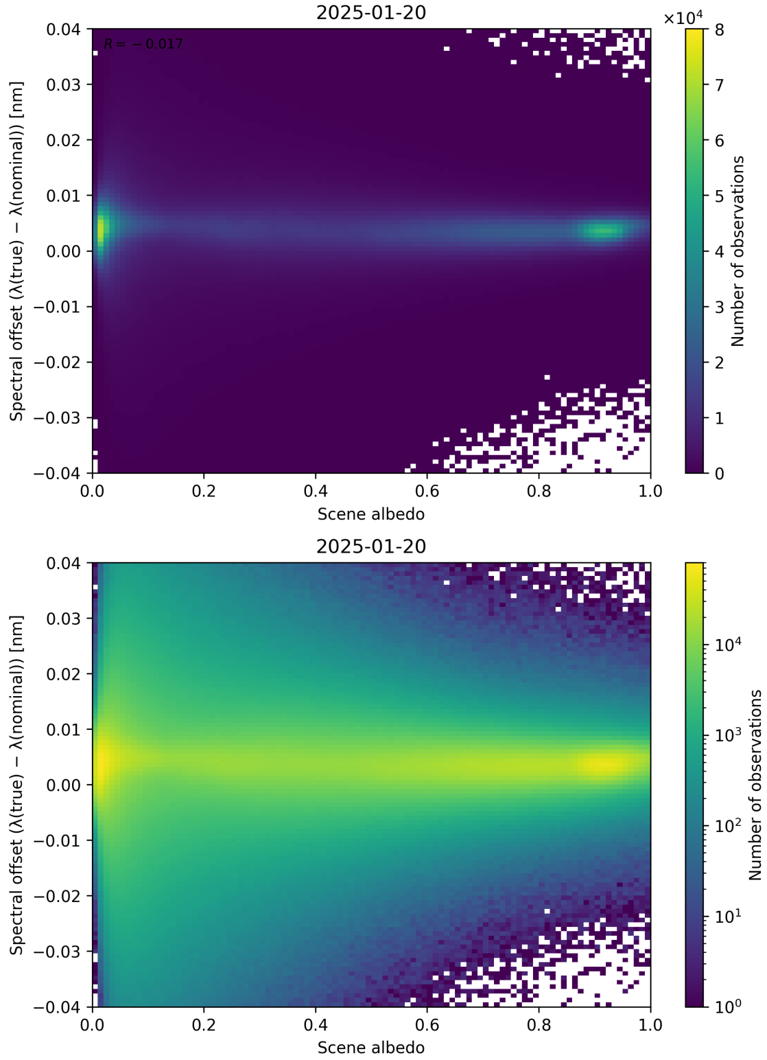
Figure 107: Scatter density plot of “Scene albedo” against “Spectral offset ( \lambda_{\text{true}} - \lambda_{\text{nominal}} )” for 2025-01-19 to 2025-01-21.
