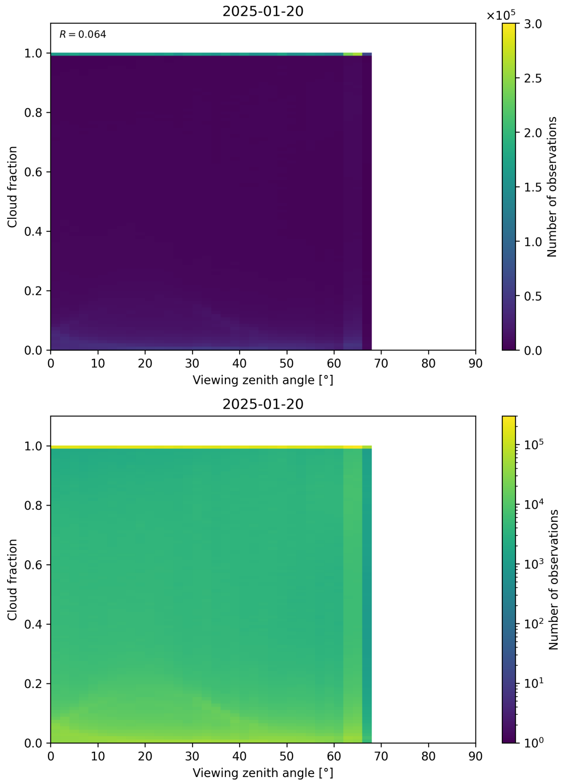
Figure 120: Scatter density plot of “Viewing zenith angle” against “Cloud fraction” for 2025-01-19 to 2025-01-21.
