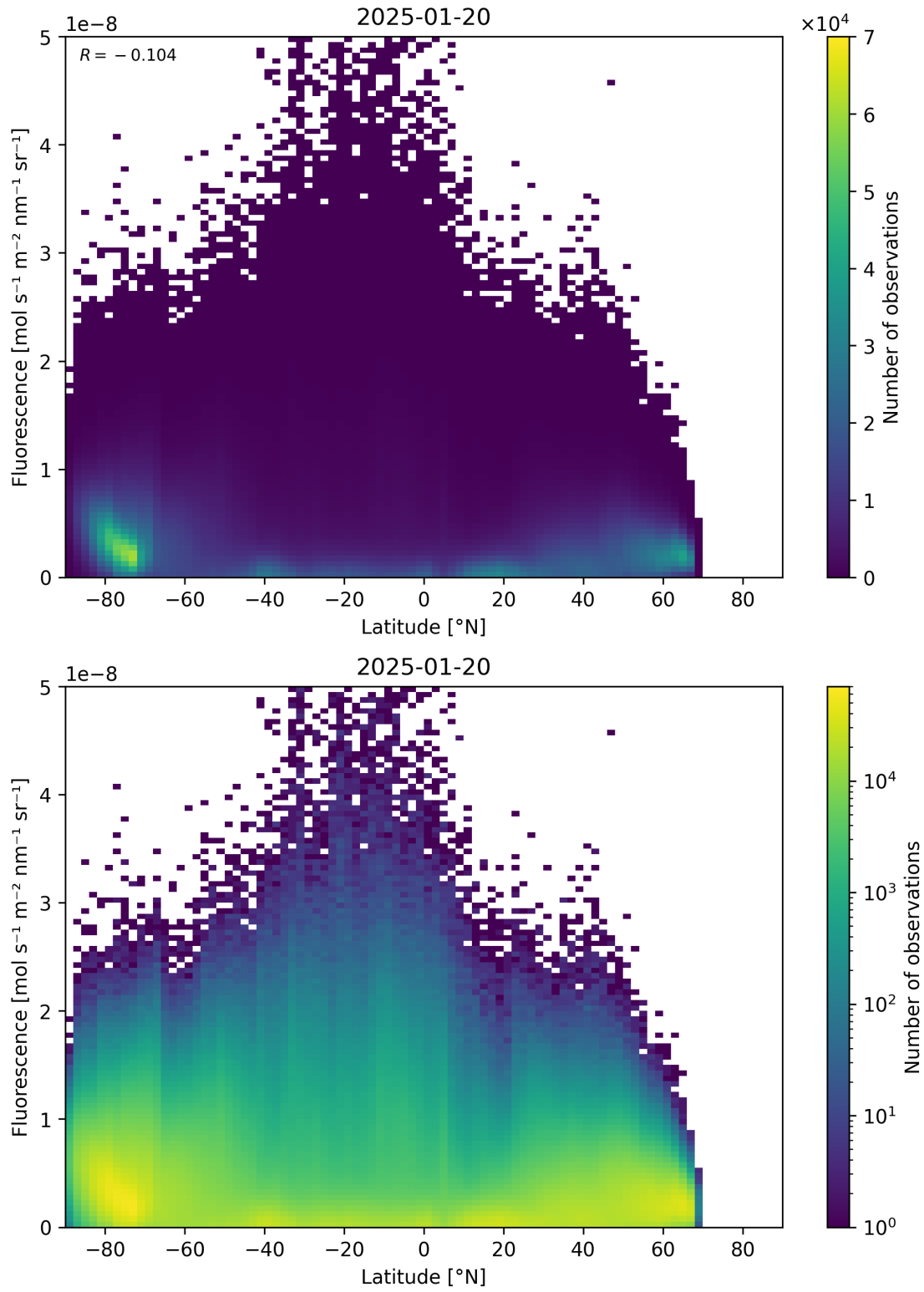
Figure 92: Scatter density plot of “Latitude” against “Fluorescence” for 2025-01-19 to 2025-01-21.
