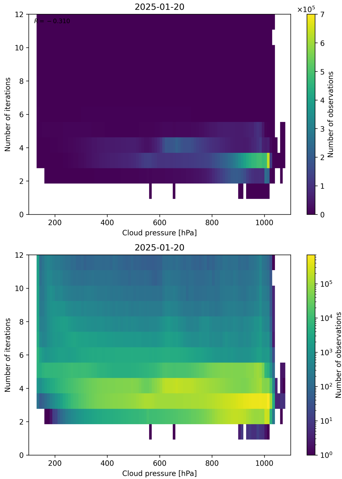
Figure 81: Scatter density plot of “Cloud pressure” against “Number of iterations” for 2025-01-19 to 2025-01-21.
