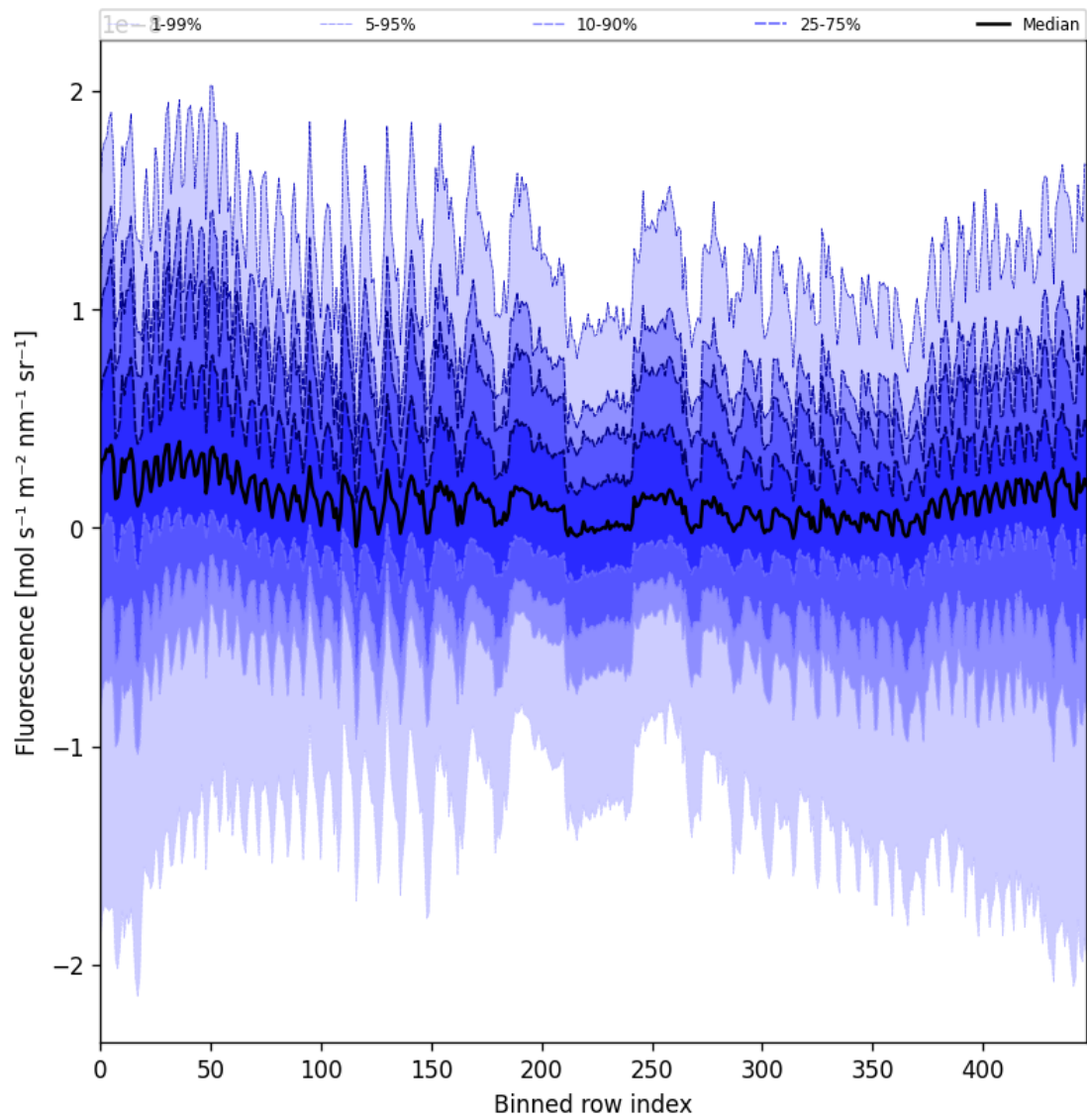
Figure 57: Along track statistics of "Fluorescence" for 2025-01-19 to 2025-01-21
