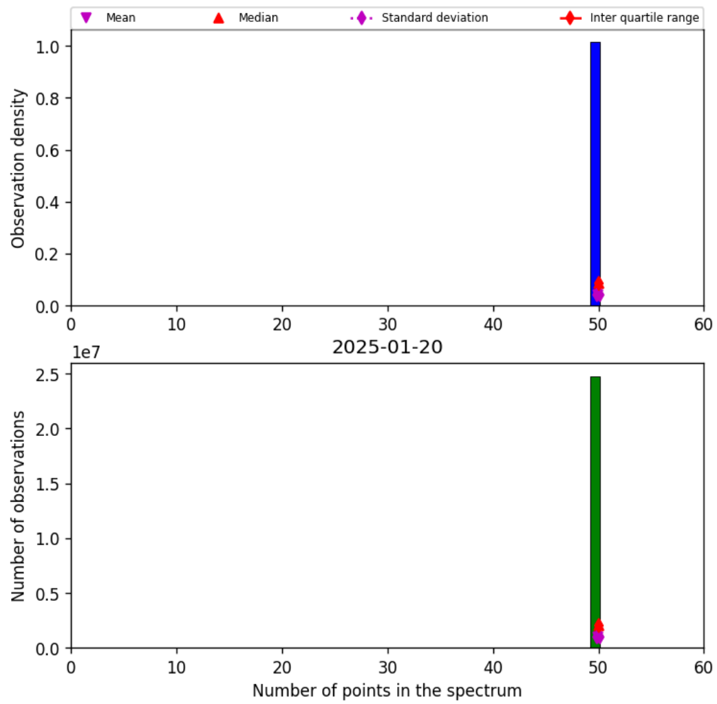
Figure 44: Histogram of “Number of points in the spectrum” for 2025-01-19 to 2025-01-21
