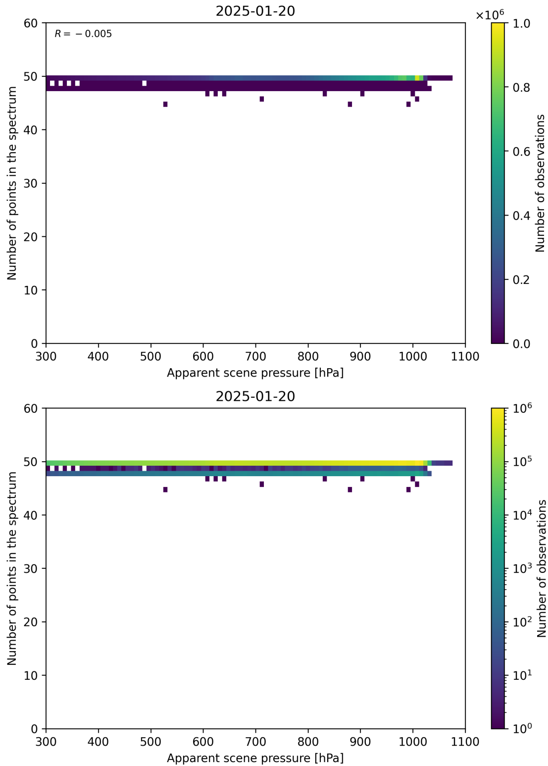
Figure 66: Scatter density plot of “Apparent scene pressure” against “Number of points in the spectrum” for 2025-01-19 to 2025-01-21.
