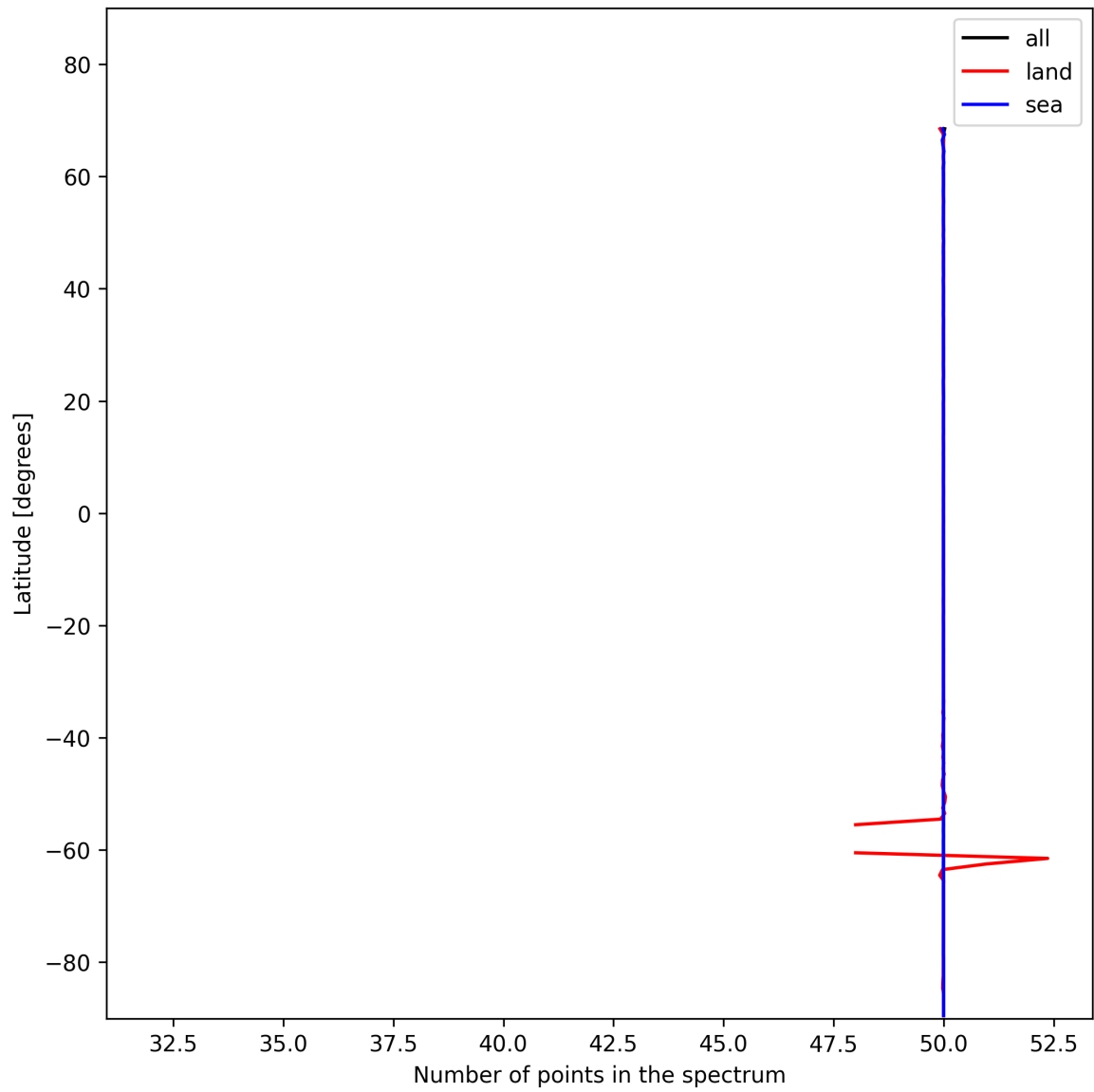
Figure 27: Zonal average of “Number of points in the spectrum” for 2025-01-19 to 2025-01-21.
