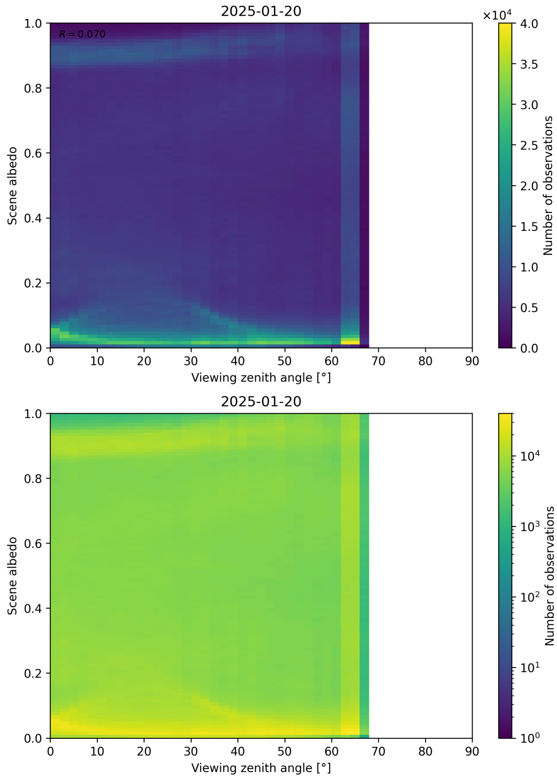
Figure 126: Scatter density plot of “Viewing zenith angle” against “Scene albedo” for 2025-01-19 to 2025-01-21.
