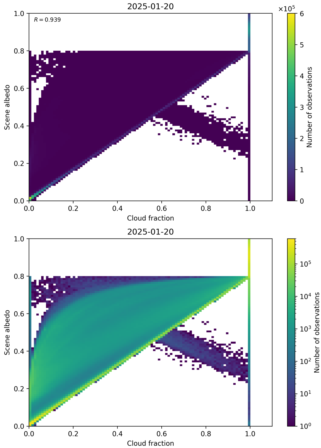
Figure 75: Scatter density plot of “Cloud fraction” against “Scene albedo” for 2025-01-19 to 2025-01-21.
