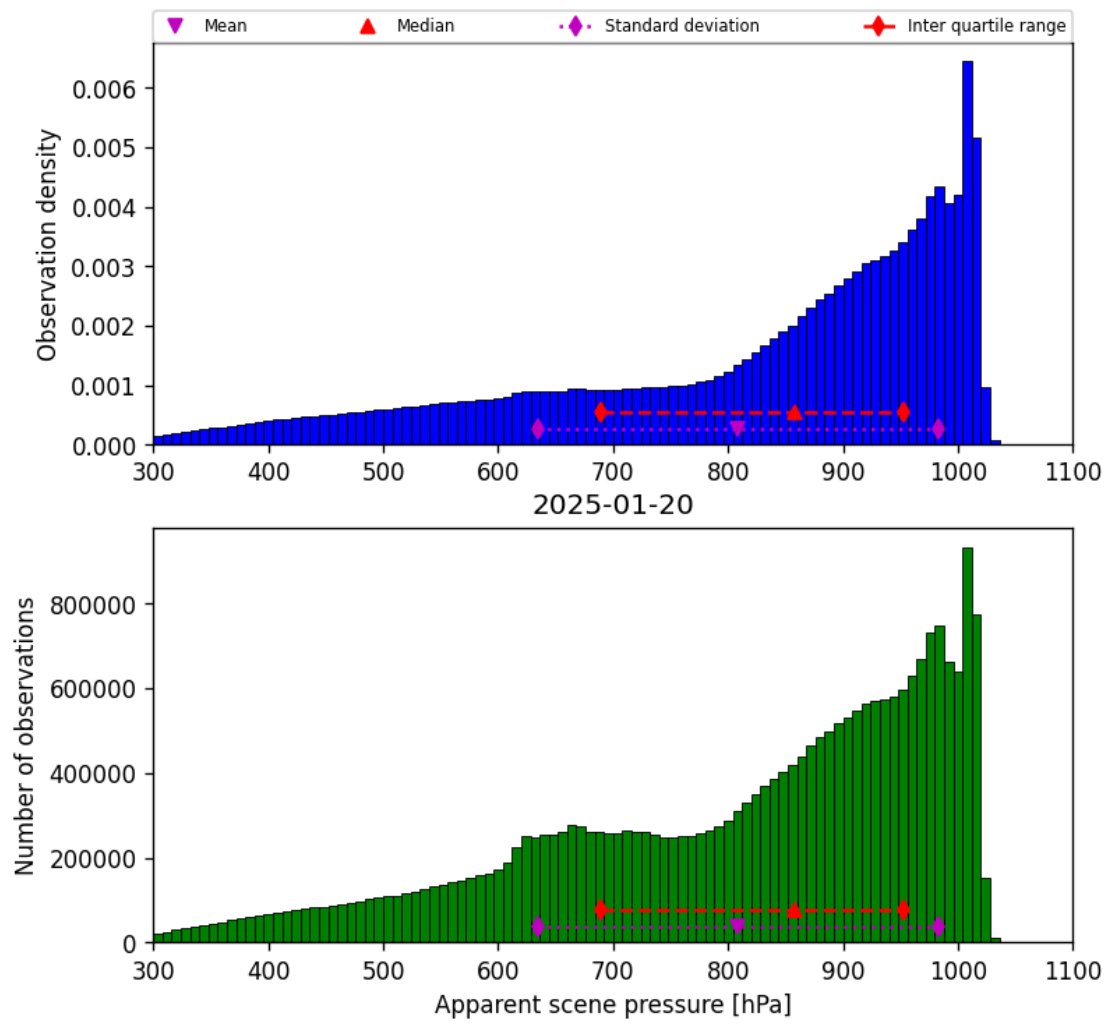
Figure 36: Histogram of “Apparent scene pressure” for 2025-01-19 to 2025-01-21
