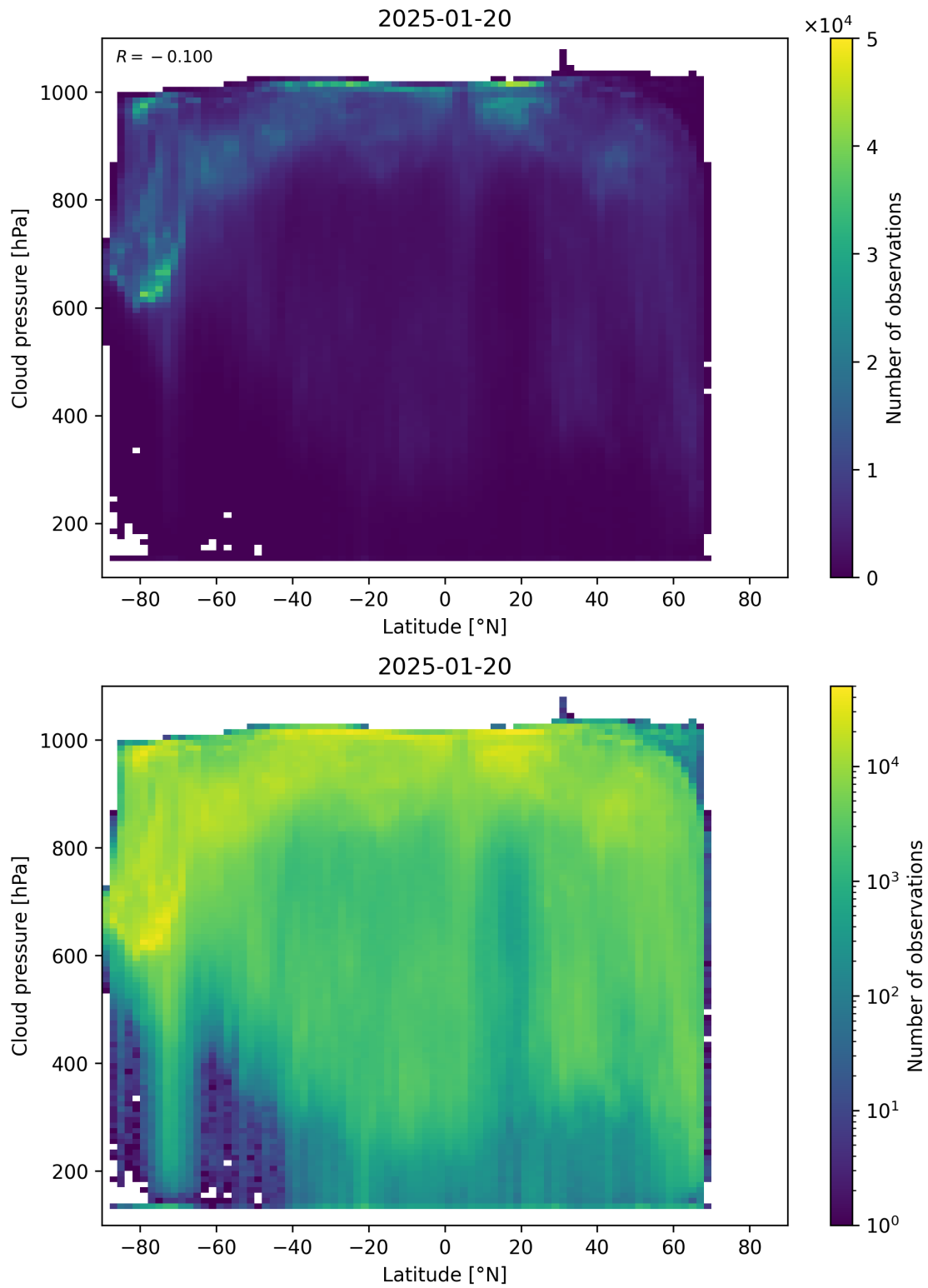
Figure 91: Scatter density plot of “Latitude” against “Cloud pressure” for 2025-01-19 to 2025-01-21.
