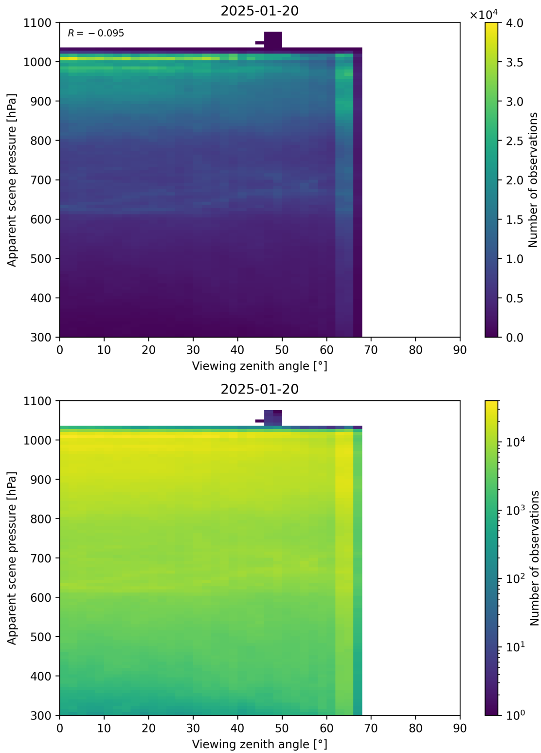
Figure 118: Scatter density plot of “Viewing zenith angle” against “Apparent scene pressure” for 2025-01-19 to 2025-01-21.
