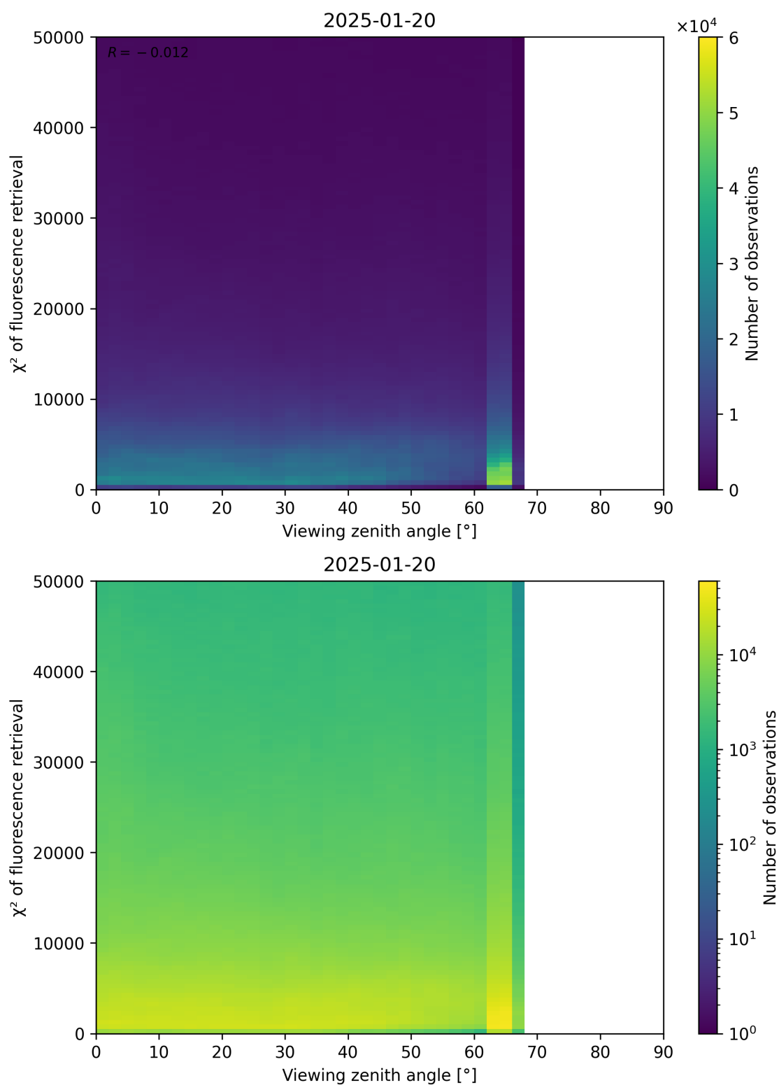
Figure 119: Scatter density plot of “Viewing zenith angle” against “ \chi^2 of fluorescence retrieval” for 2025-01-19 to 2025-01-21.
