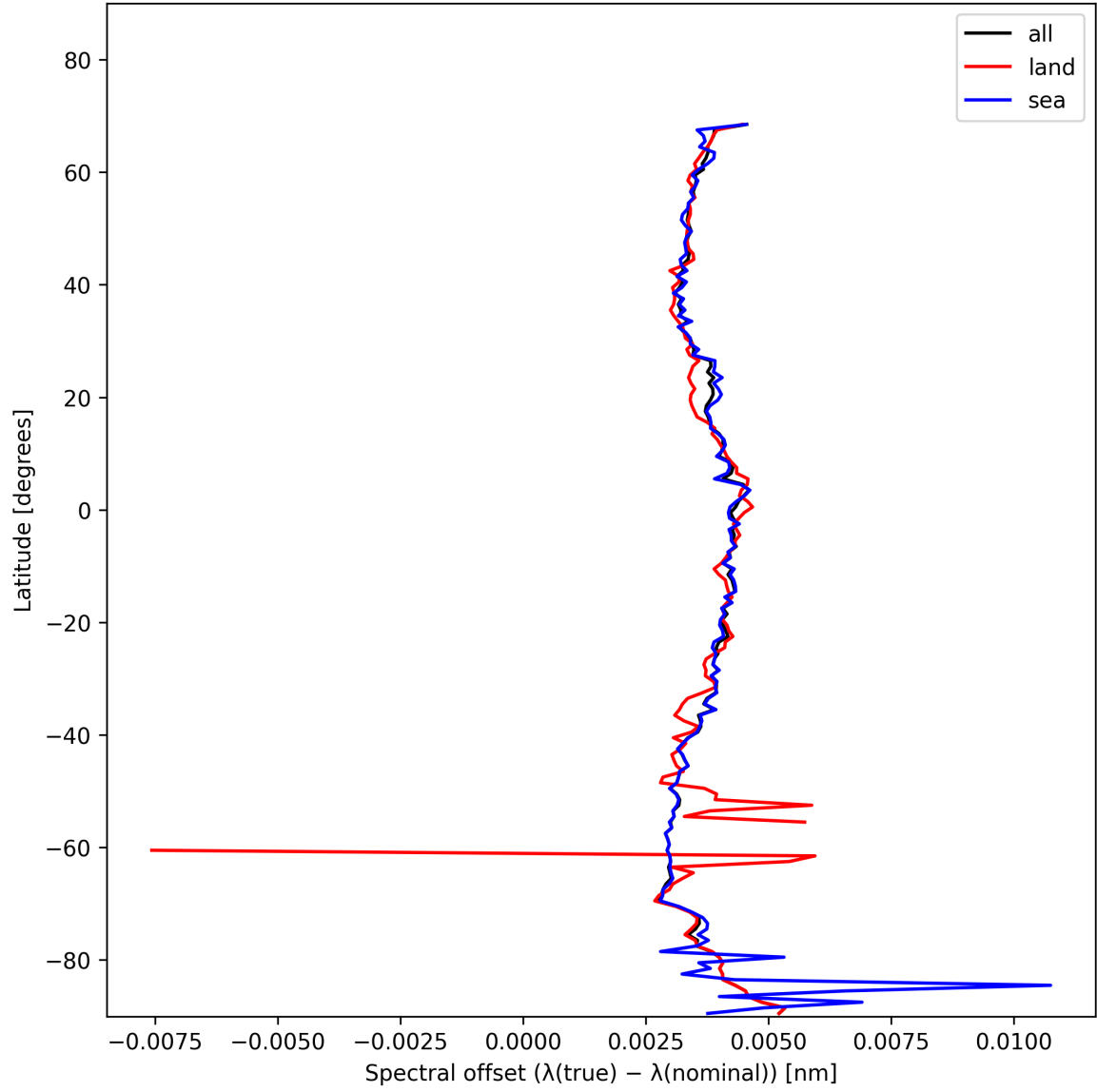
Figure 28: Zonal average of “Spectral offset ( \lambda_{\text{true}} - \lambda_{\text{nominal}} )” for 2025-01-19 to 2025-01-21.
