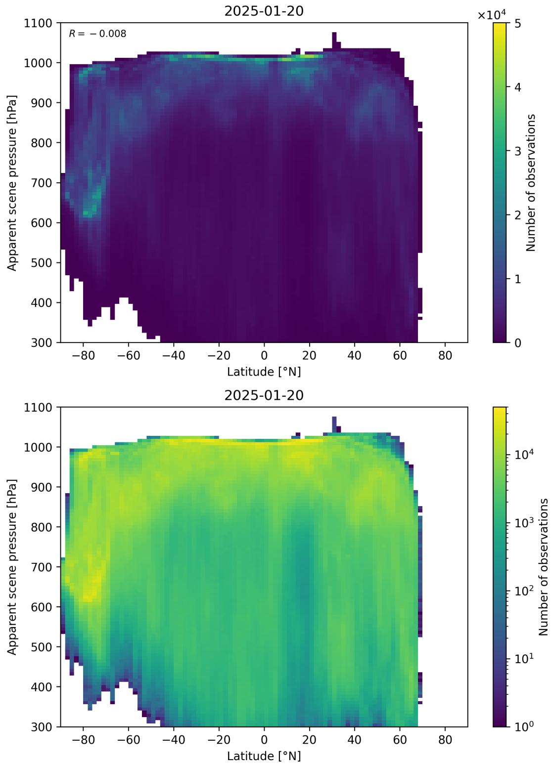
Figure 88: Scatter density plot of “Latitude” against “Apparent scene pressure” for 2025-01-19 to 2025-01-21.
