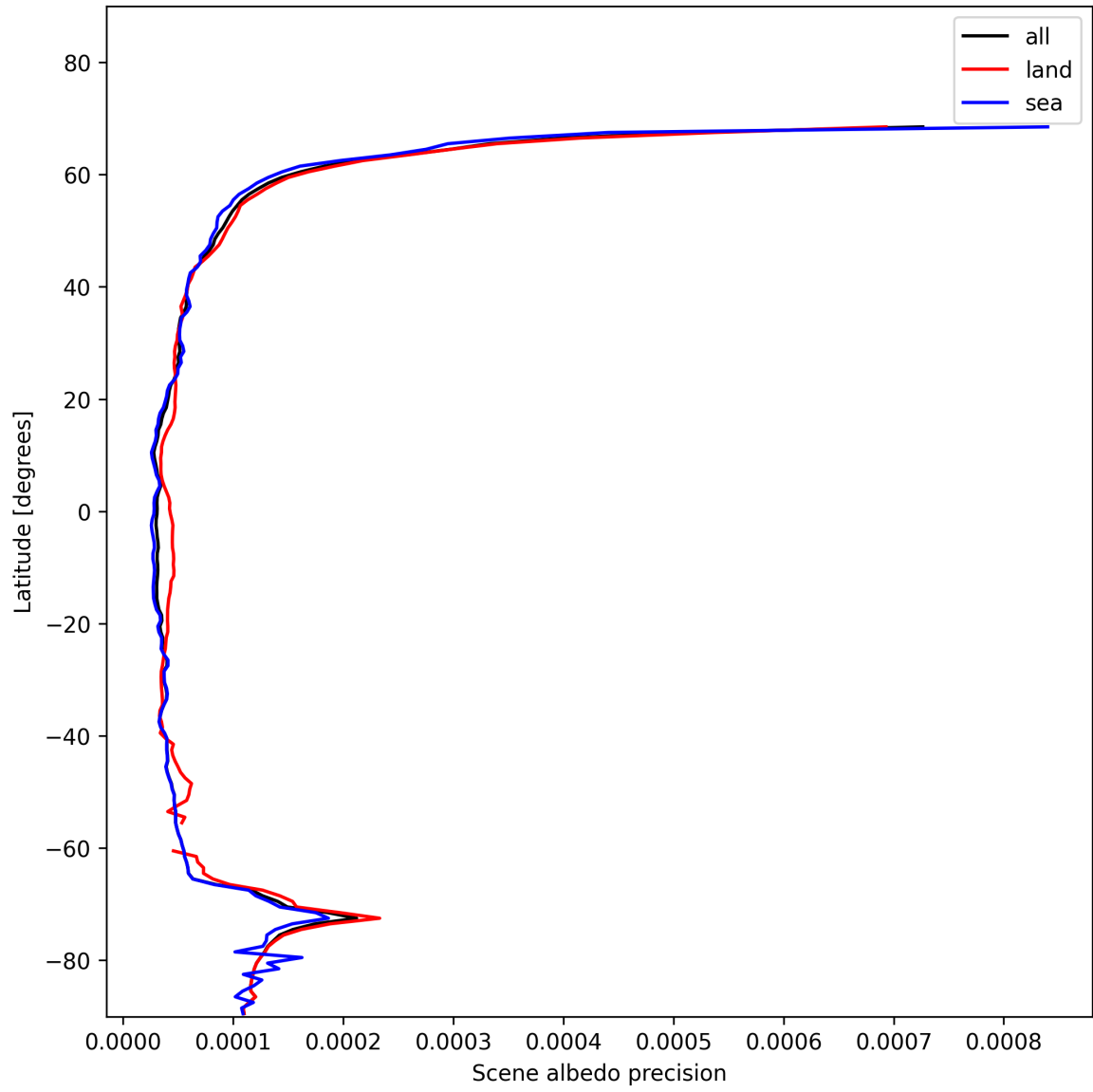
Figure 18: Zonal average of “Scene albedo precision” for 2025-01-19 to 2025-01-21.
