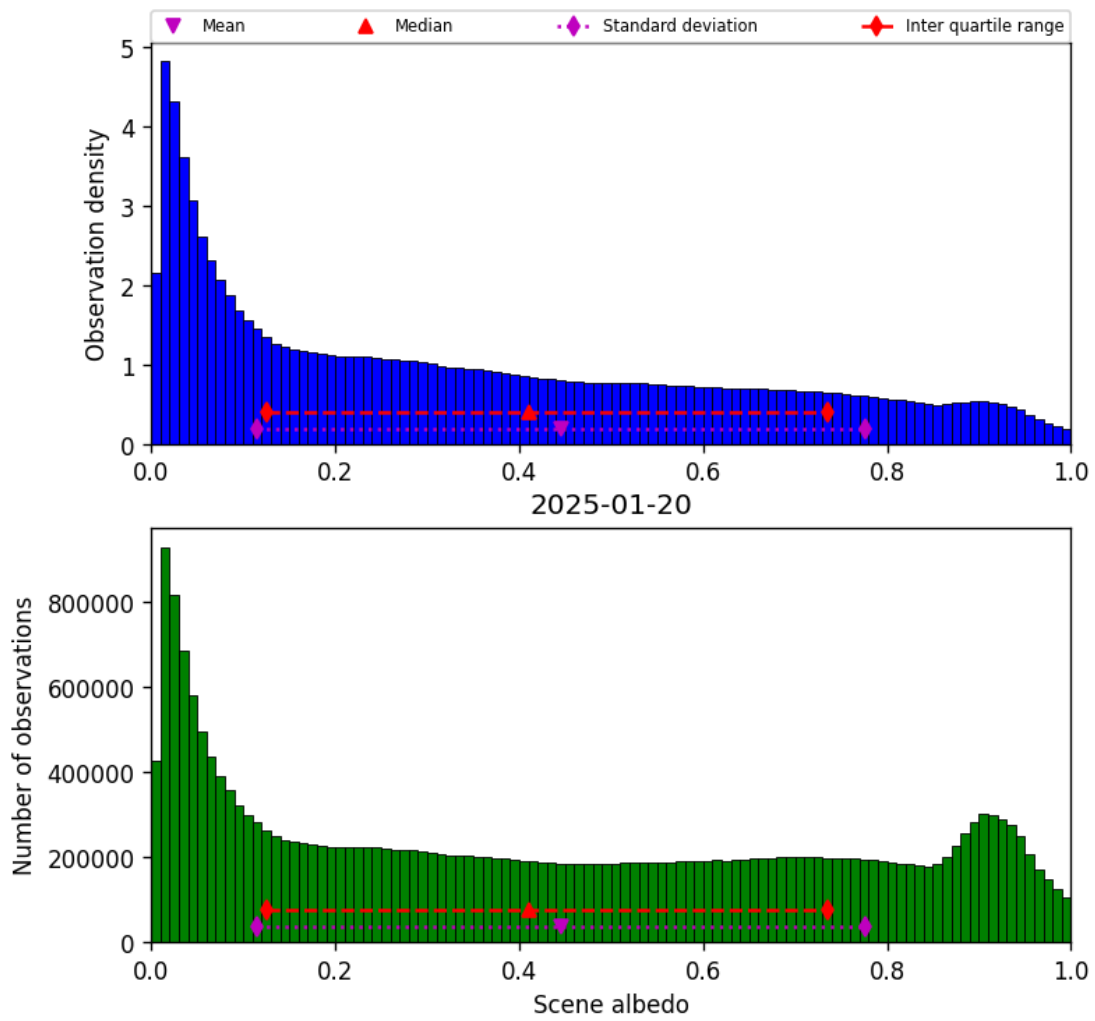
Figure 34: Histogram of “Scene albedo” for 2025-01-19 to 2025-01-21
