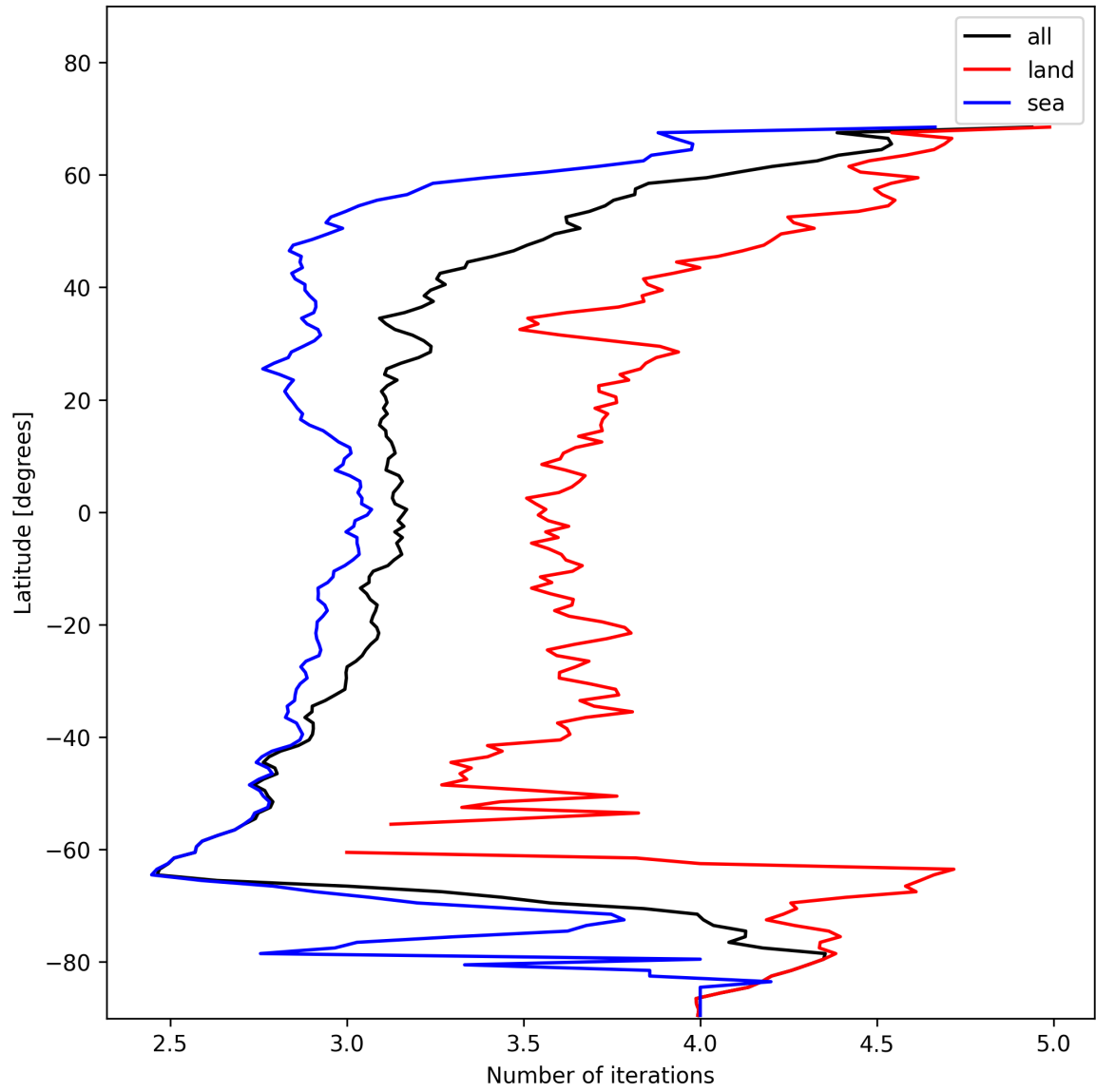
Figure 22: Zonal average of “Number of iterations” for 2025-01-19 to 2025-01-21.
