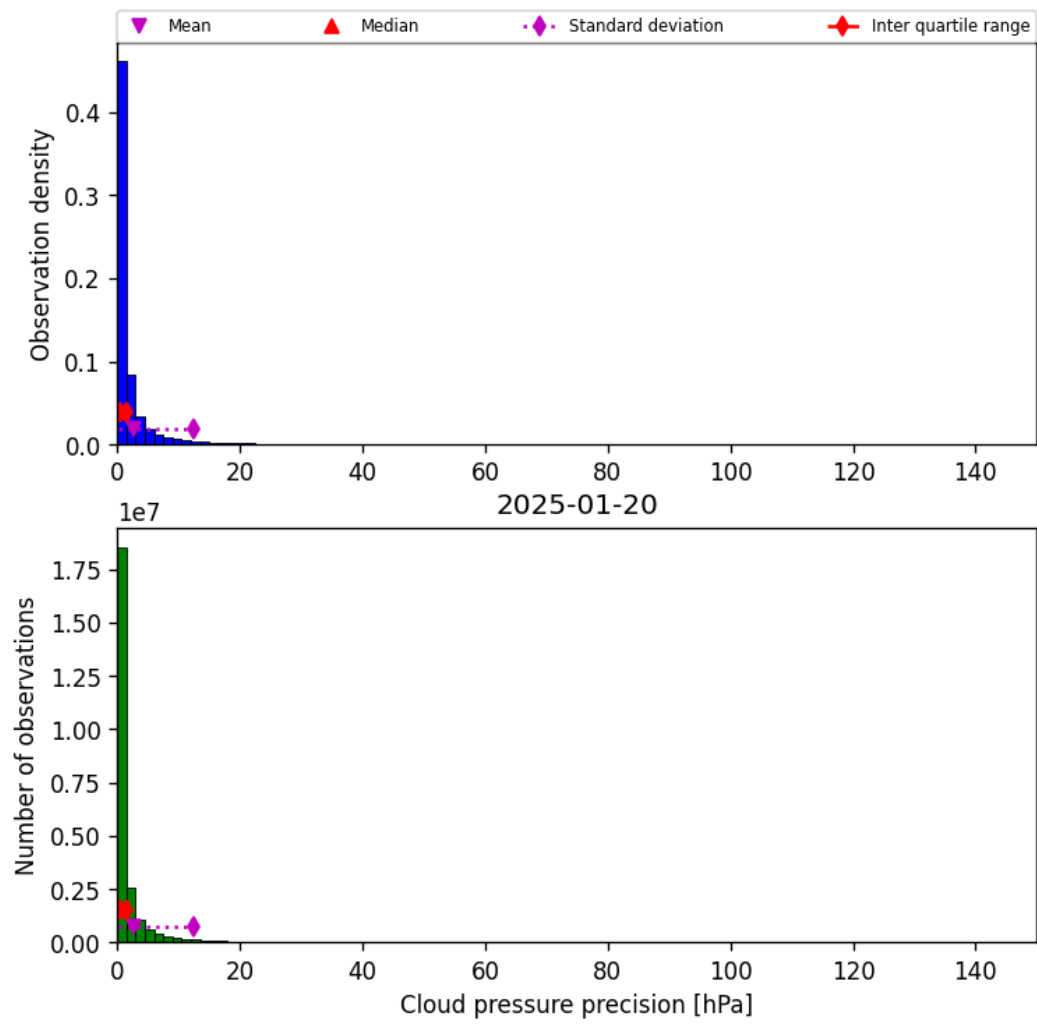
Figure 31: Histogram of “Cloud pressure precision” for 2025-01-19 to 2025-01-21
