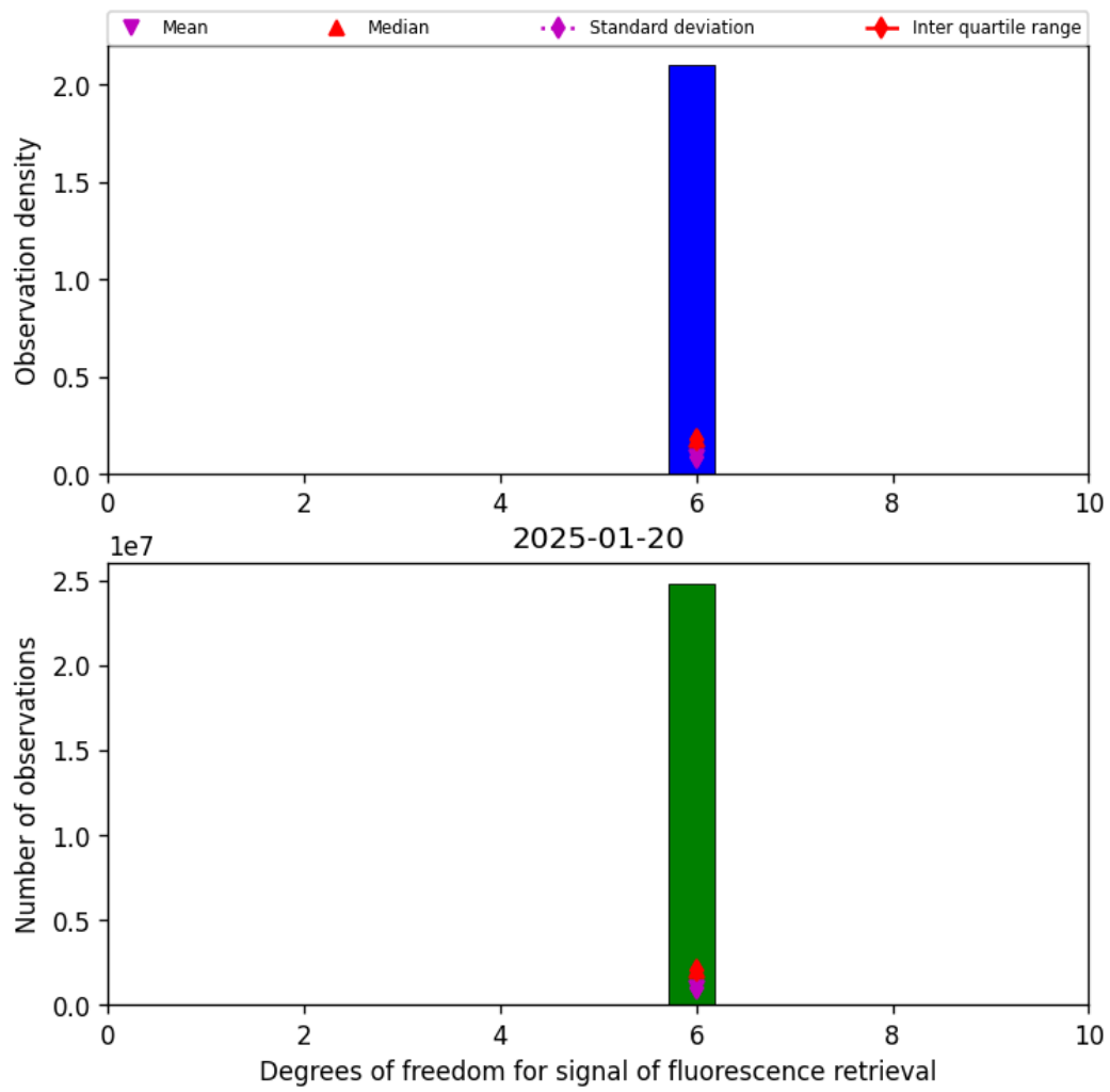
Figure 43: Histogram of "Degrees of freedom for signal of fluorescence retrieval" for 2025-01-19 to 2025-01-21
