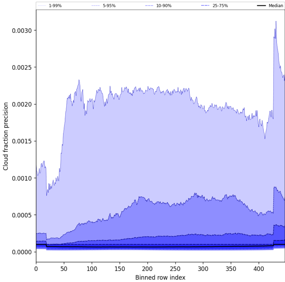
Figure 50: Along track statistics of “Cloud fraction precision” for 2025-01-19 to 2025-01-21
