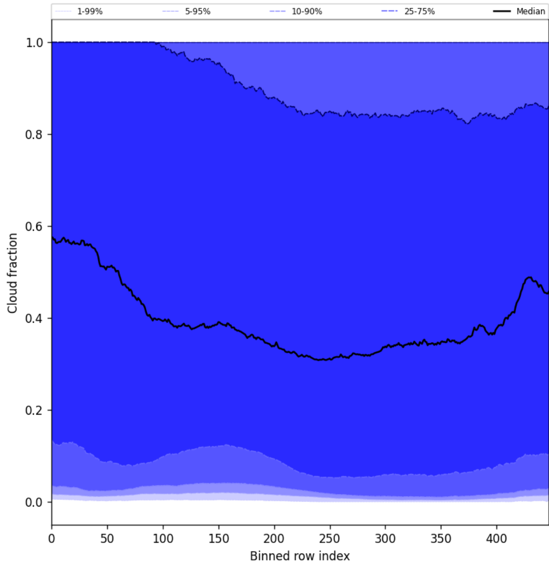
Figure 49: Along track statistics of “Cloud fraction” for 2025-01-19 to 2025-01-21
