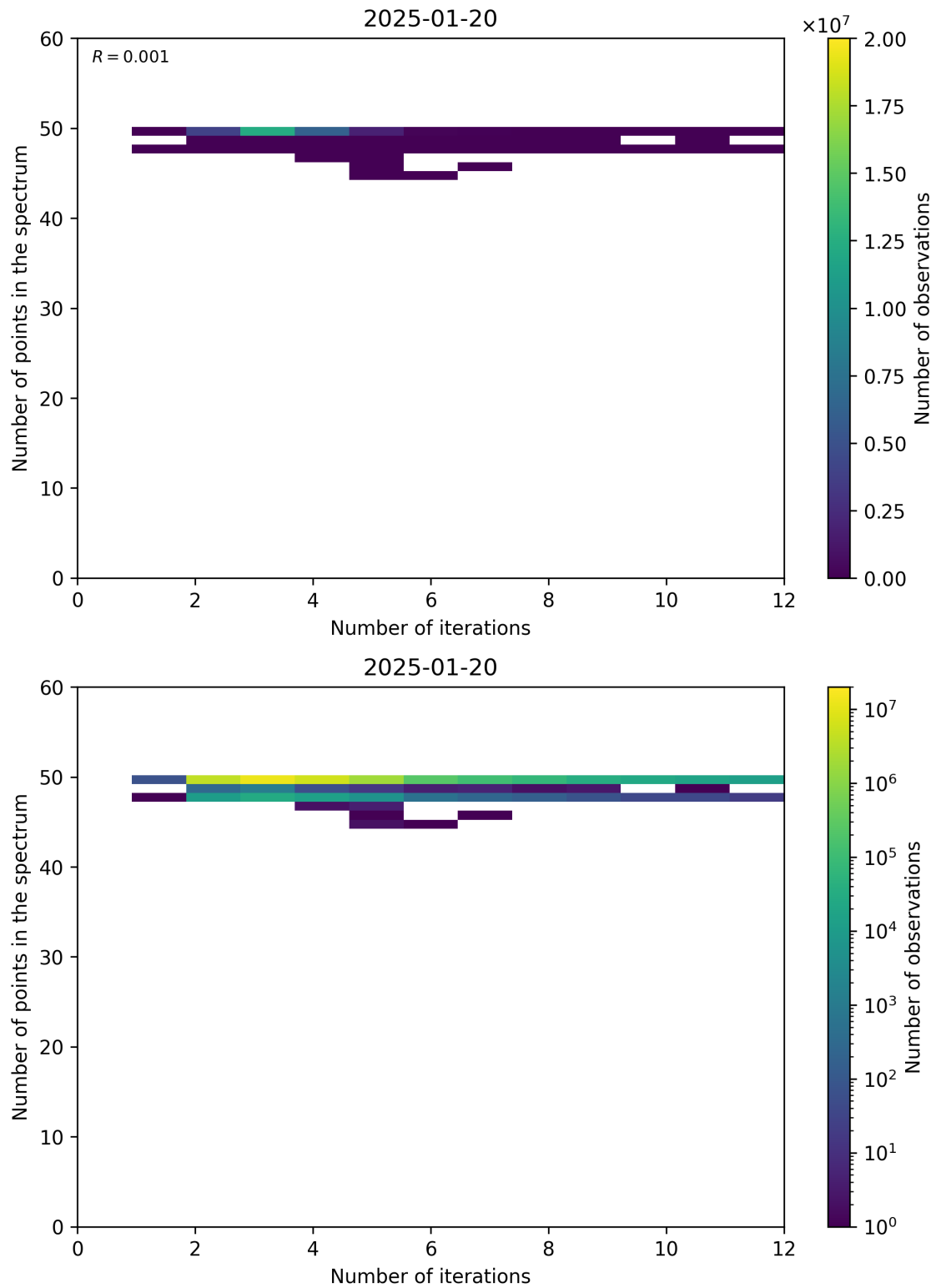
Figure 99: Scatter density plot of “Number of iterations” against “Number of points in the spectrum” for 2025-01-19 to 2025-01-21.
