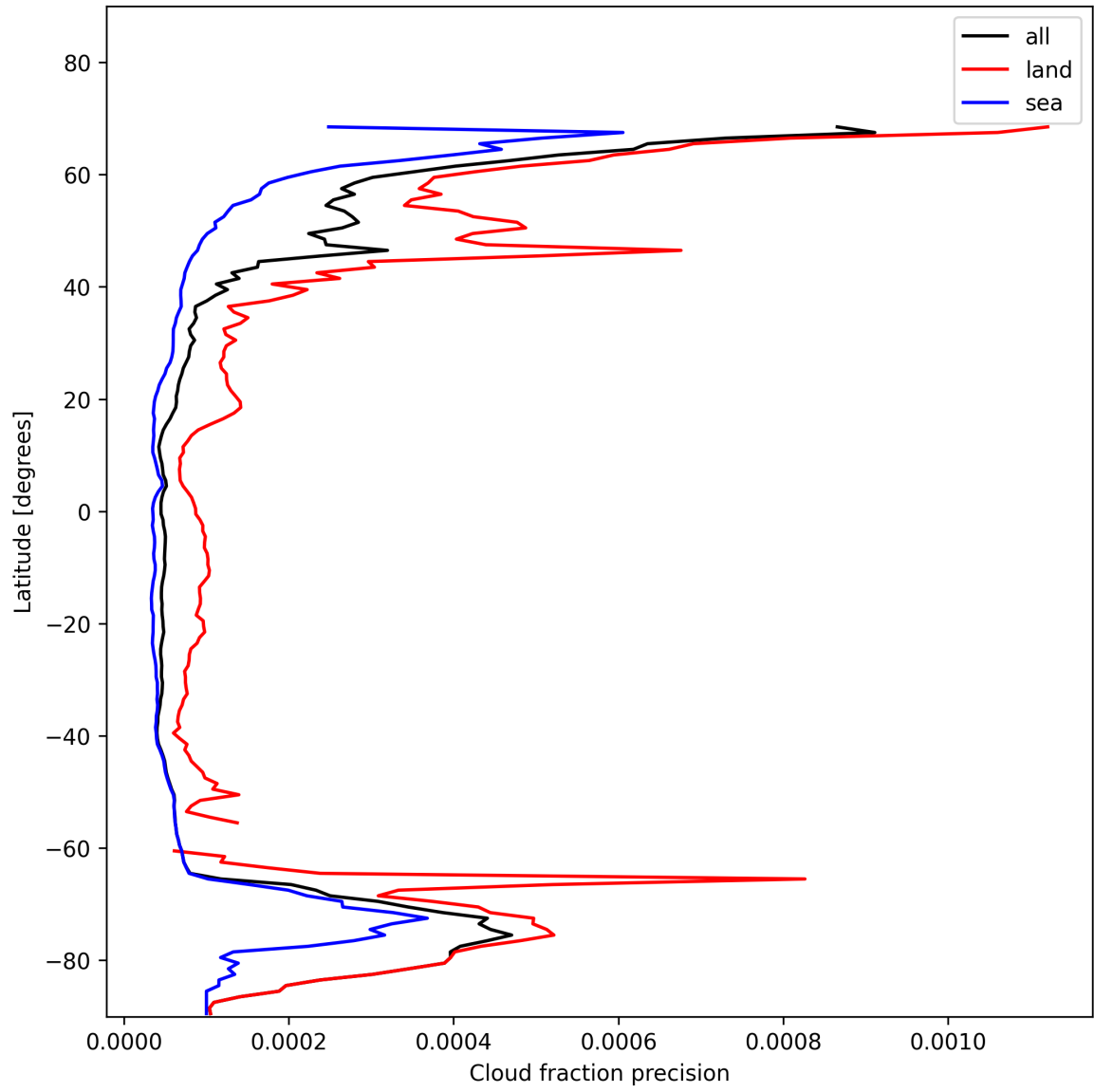
Figure 16: Zonal average of “Cloud fraction precision” for 2025-01-19 to 2025-01-21.
