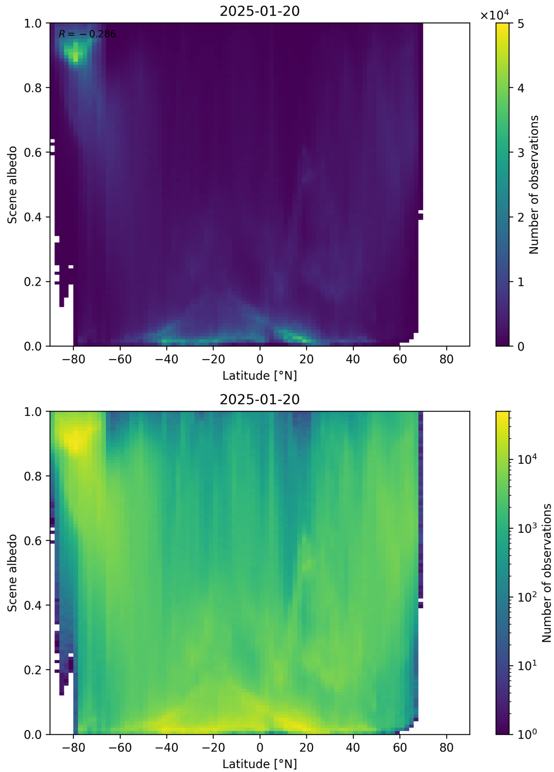
Figure 95: Scatter density plot of “Latitude” against “Scene albedo” for 2025-01-19 to 2025-01-21.
