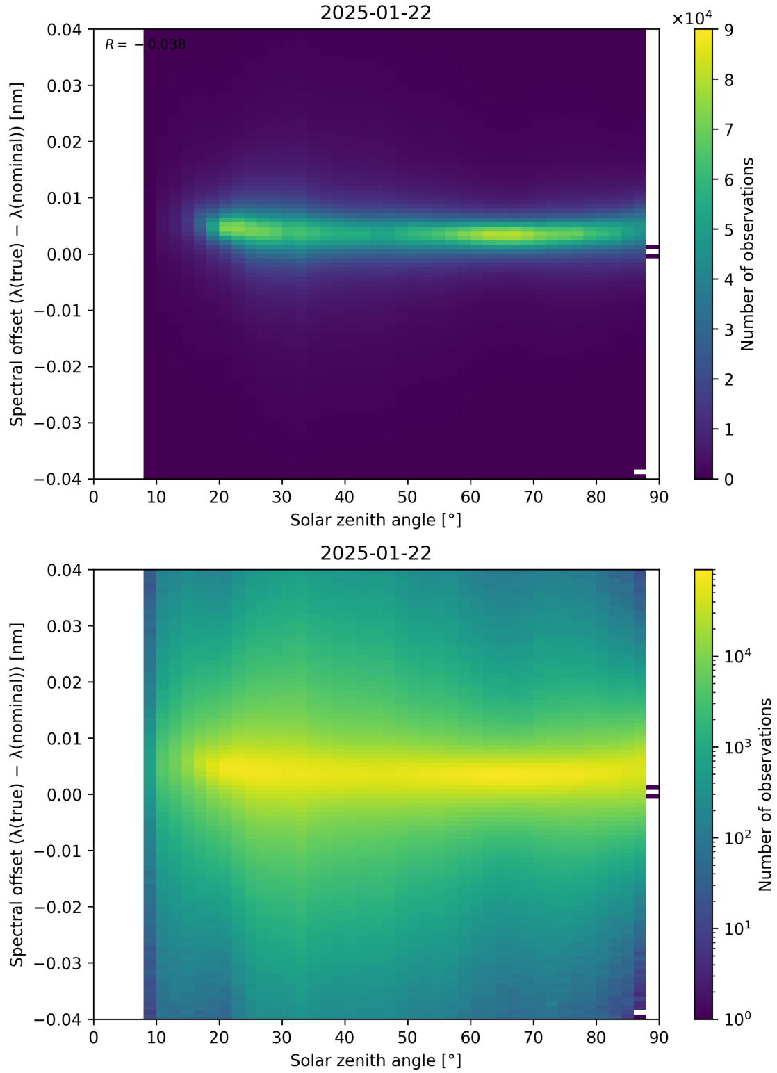
Figure 117: Scatter density plot of “Solar zenith angle” against “Spectral offset ( \lambda_{\text{true}} - \lambda_{\text{nominal}} )” for 2025-01-21 to 2025-01-23.
