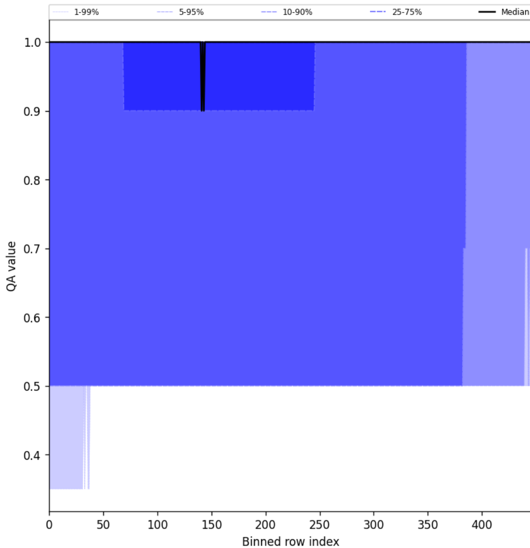
Figure 46: Along track statistics of “QA value” for 2025-01-21 to 2025-01-23
