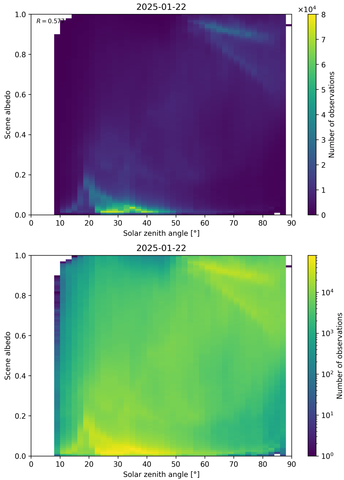
Figure 116: Scatter density plot of “Solar zenith angle” against “Scene albedo” for 2025-01-21 to 2025-01-23.
