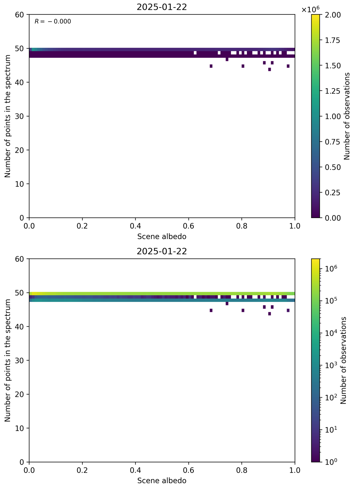
Figure 106: Scatter density plot of “Scene albedo” against “Number of points in the spectrum” for 2025-01-21 to 2025-01-23.
