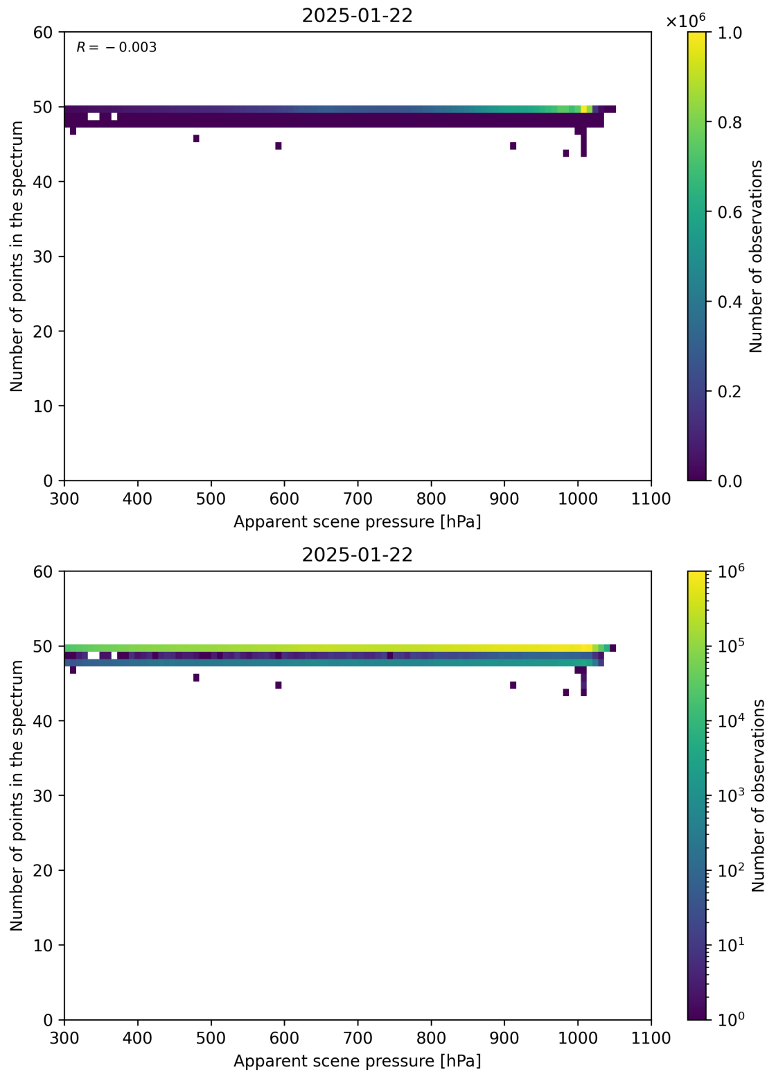
Figure 66: Scatter density plot of “Apparent scene pressure” against “Number of points in the spectrum” for 2025-01-21 to 2025-01-23.
