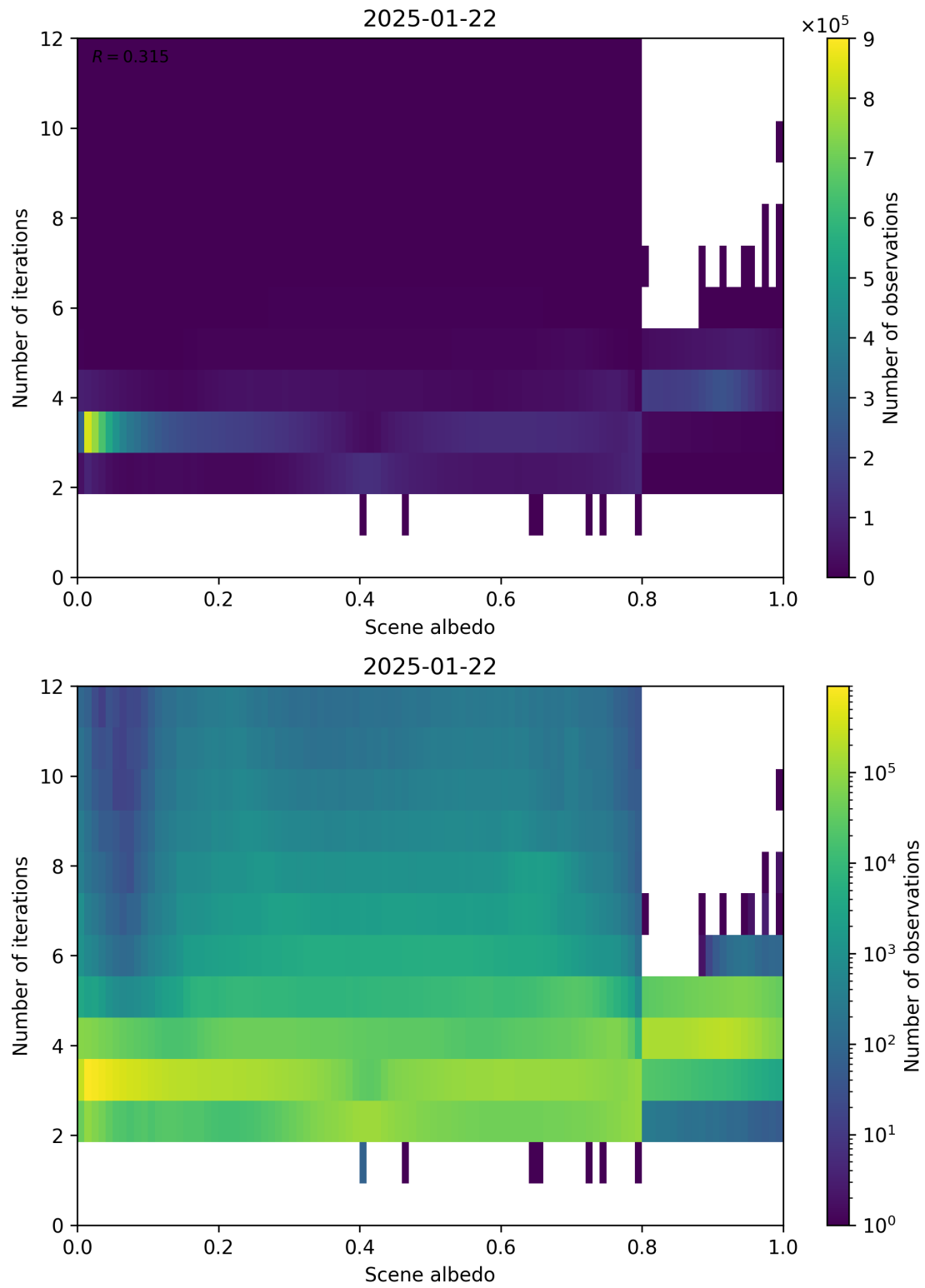
Figure 105: Scatter density plot of “Scene albedo” against “Number of iterations” for 2025-01-21 to 2025-01-23.
