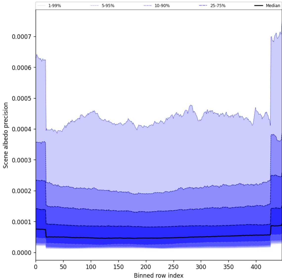
Figure 52: Along track statistics of “Scene albedo precision” for 2025-01-21 to 2025-01-23
