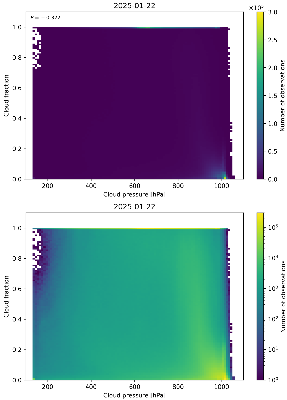
Figure 79: Scatter density plot of “Cloud pressure” against “Cloud fraction” for 2025-01-21 to 2025-01-23.
