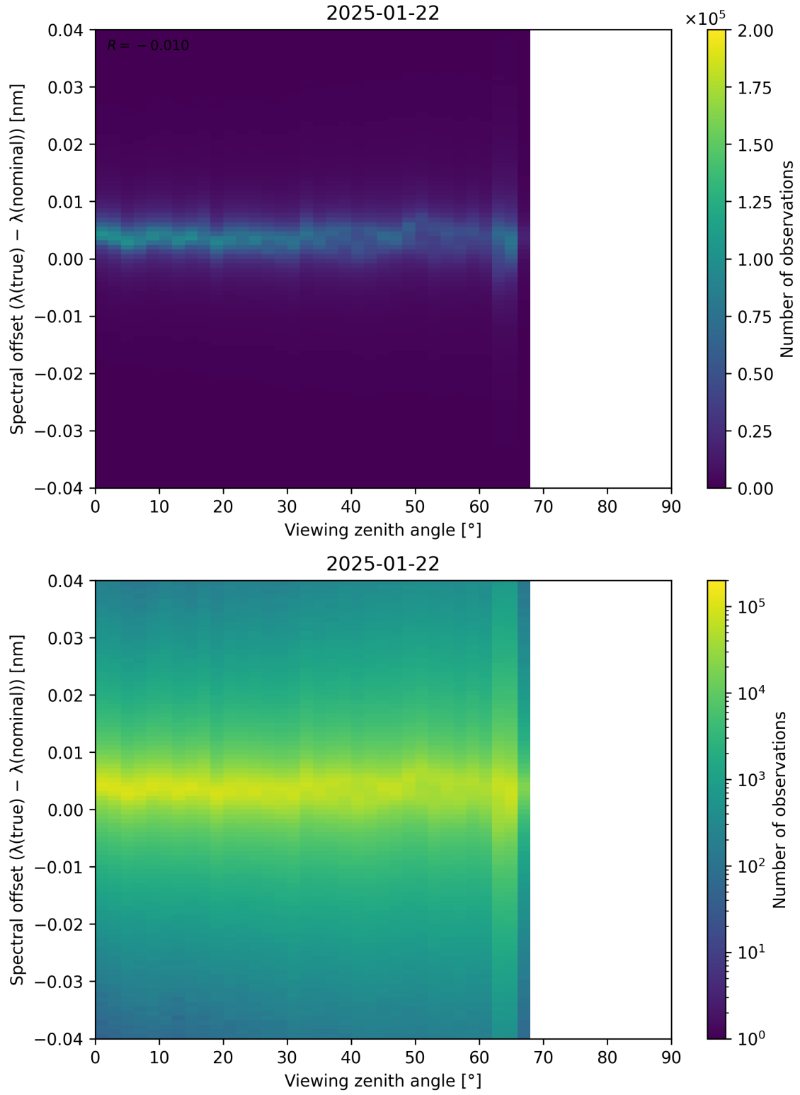
Figure 128: Scatter density plot of “Viewing zenith angle” against “Spectral offset ( \lambda_{\text{true}} - \lambda_{\text{nominal}} )” for 2025-01-21 to 2025-01-23.
