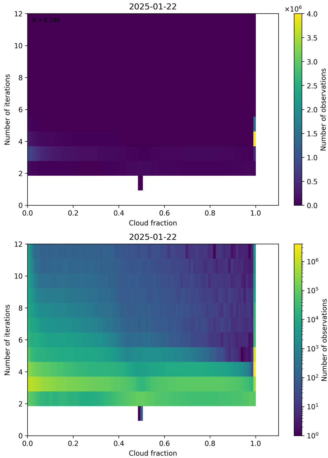
Figure 73: Scatter density plot of “Cloud fraction” against “Number of iterations” for 2025-01-21 to 2025-01-23.
