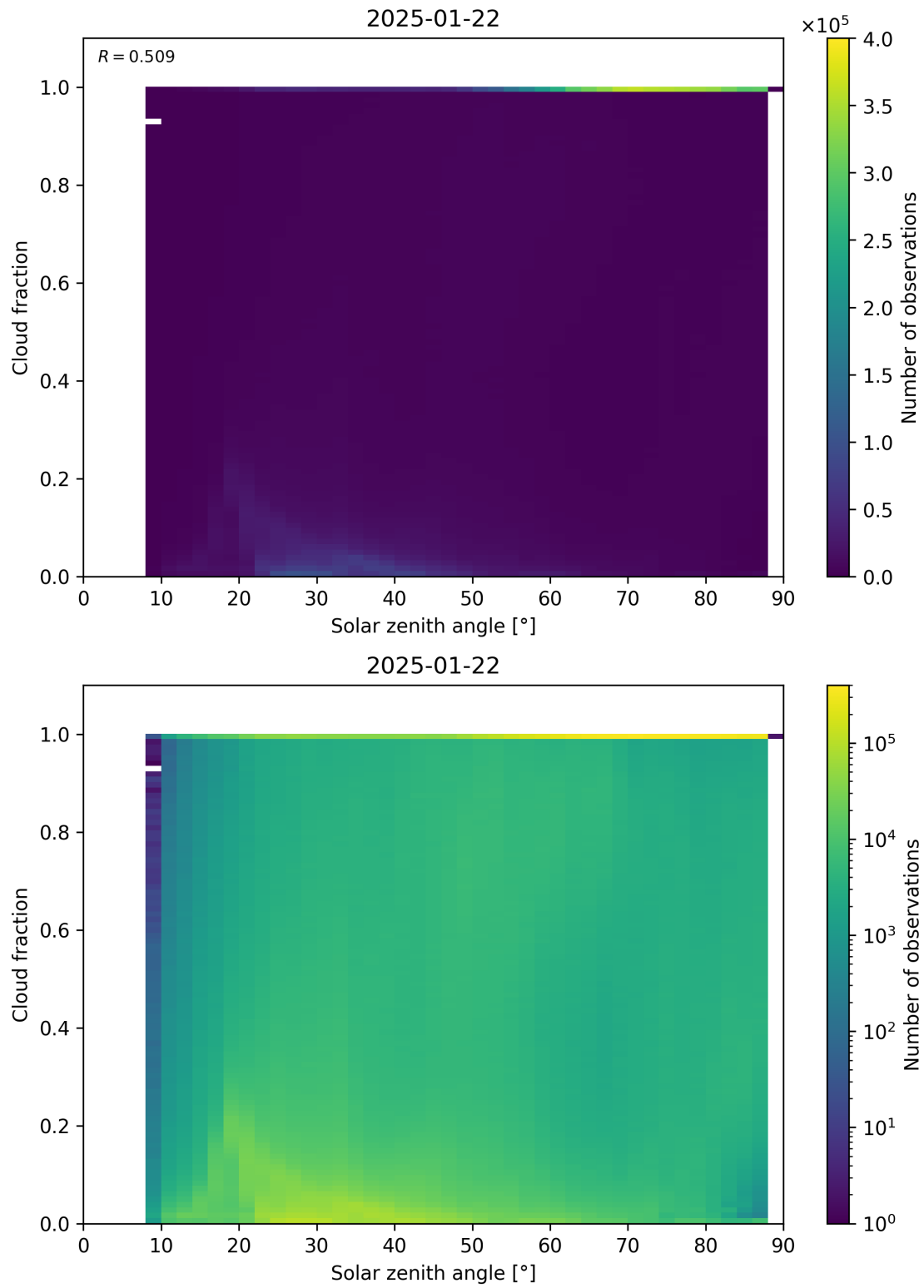
Figure 110: Scatter density plot of “Solar zenith angle” against “Cloud fraction” for 2025-01-21 to 2025-01-23.
