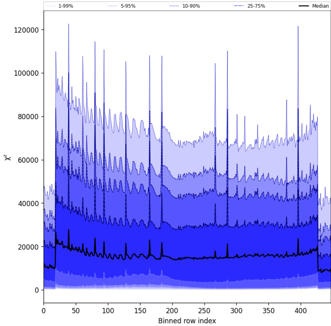
Figure 55: Along track statistics of “ \chi^2 ” for 2025-01-21 to 2025-01-23
