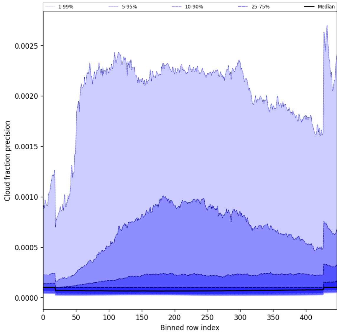
Figure 50: Along track statistics of “Cloud fraction precision” for 2025-01-21 to 2025-01-23
