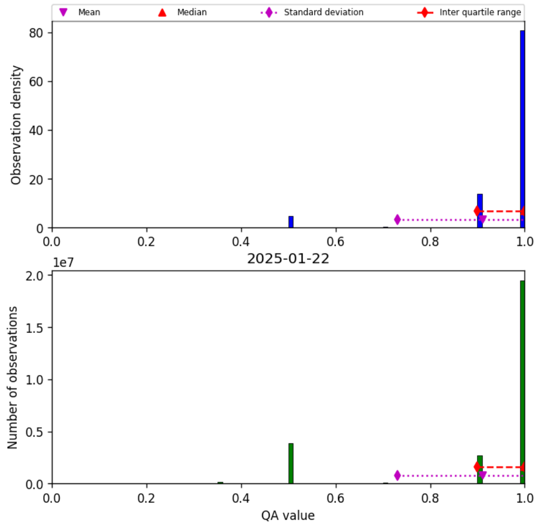
Figure 29: Histogram of “QA value” for 2025-01-21 to 2025-01-23
