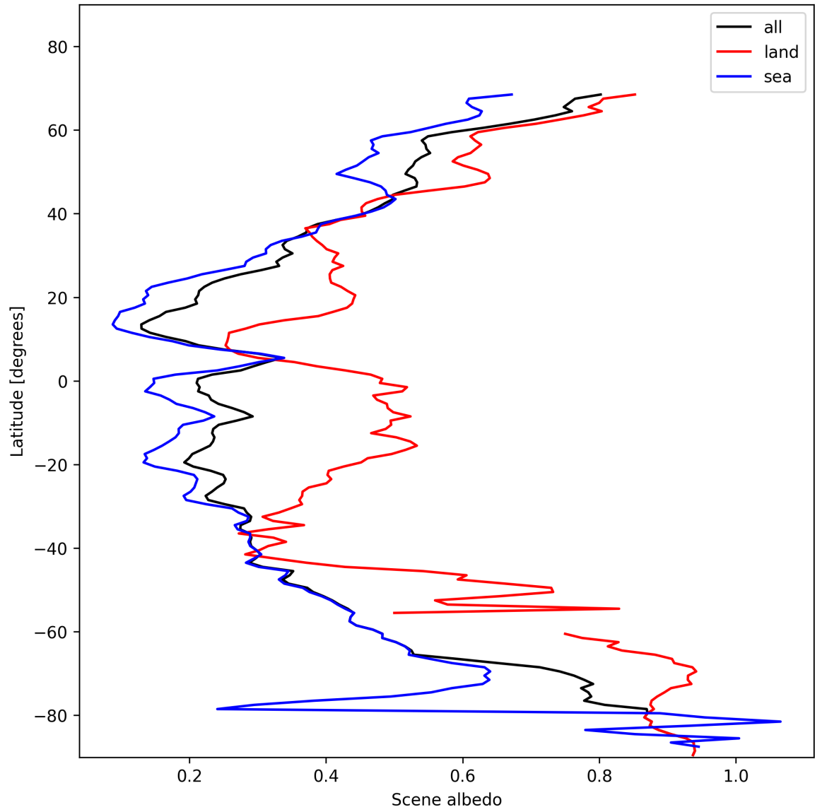
Figure 17: Zonal average of “Scene albedo” for 2025-01-21 to 2025-01-23.
