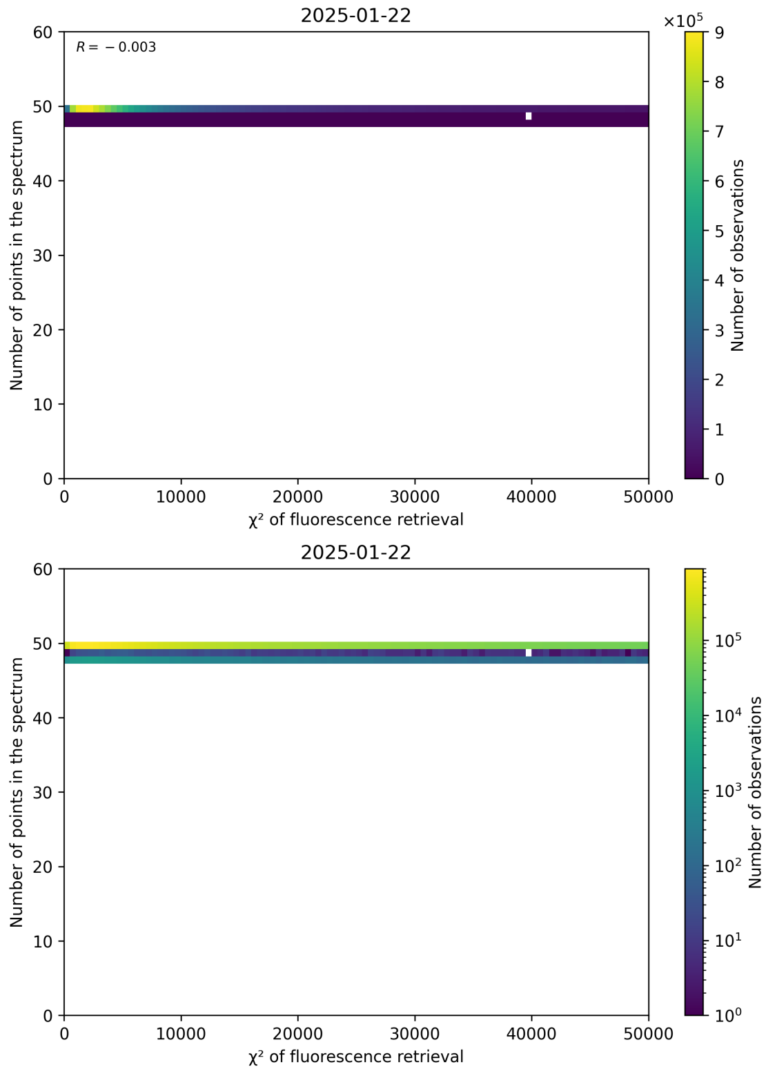
Figure 68: Scatter density plot of “ \chi^2 of fluorescence retrieval” against “Number of points in the spectrum” for 2025-01-21 to 2025-01-23.
