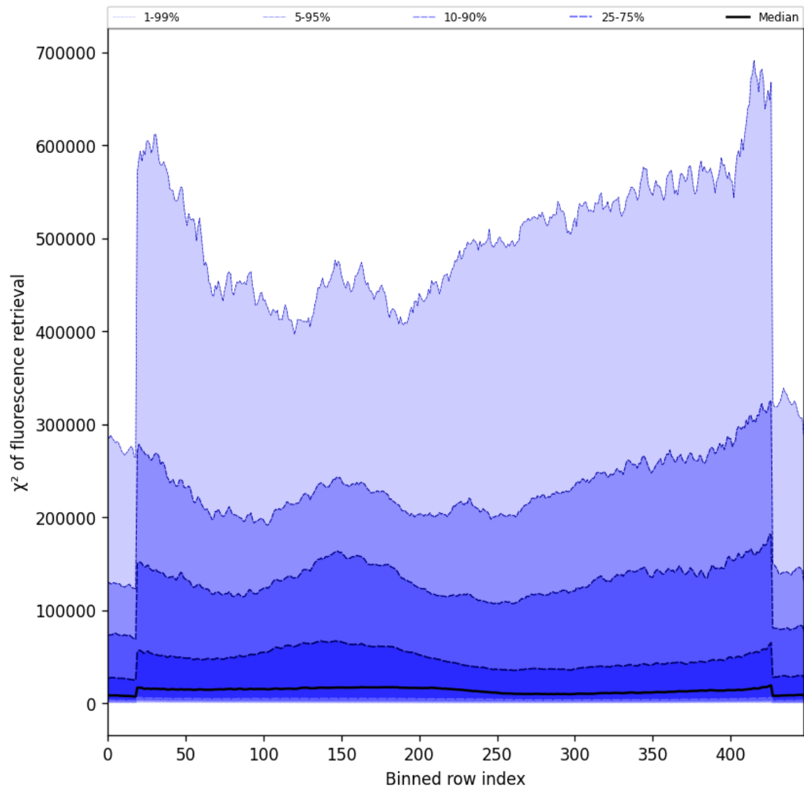
Figure 59: Along track statistics of “ \chi^2 of fluorescence retrieval” for 2025-01-21 to 2025-01-23
