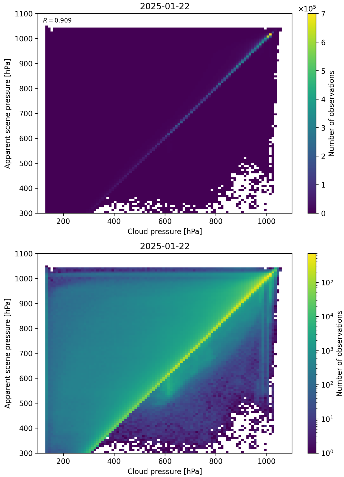
Figure 77: Scatter density plot of “Cloud pressure” against “Apparent scene pressure” for 2025-01-21 to 2025-01-23.
