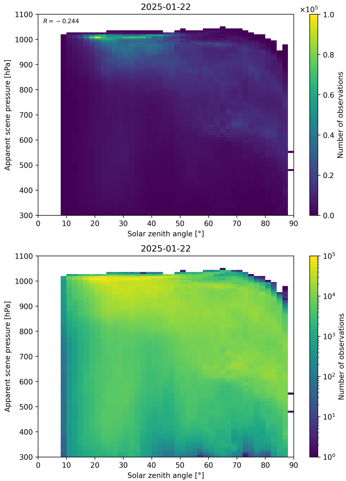
Figure 108: Scatter density plot of “Solar zenith angle” against “Apparent scene pressure” for 2025-01-21 to 2025-01-23.
