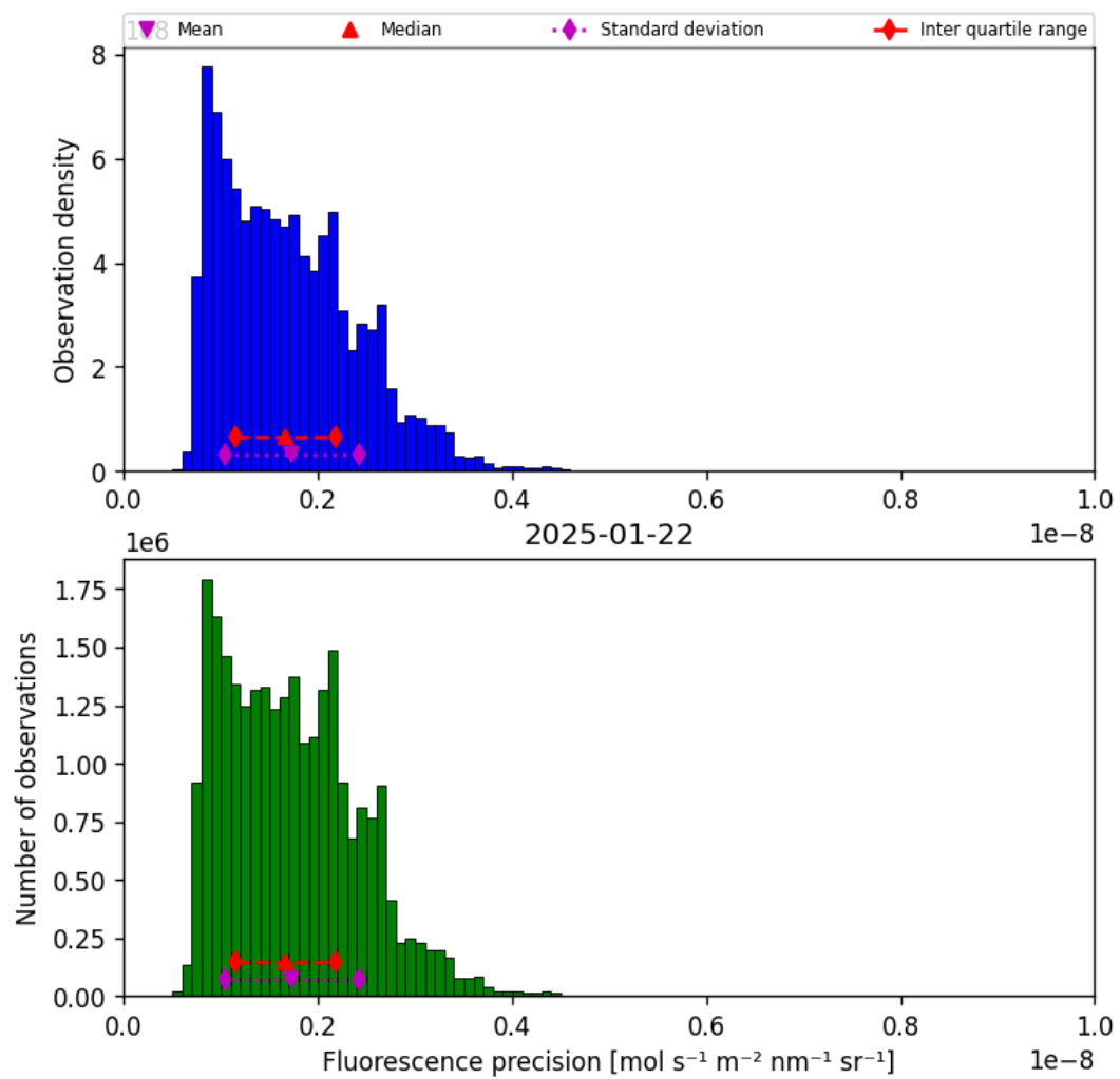
Figure 41: Histogram of “Fluorescence precision” for 2025-01-21 to 2025-01-23
