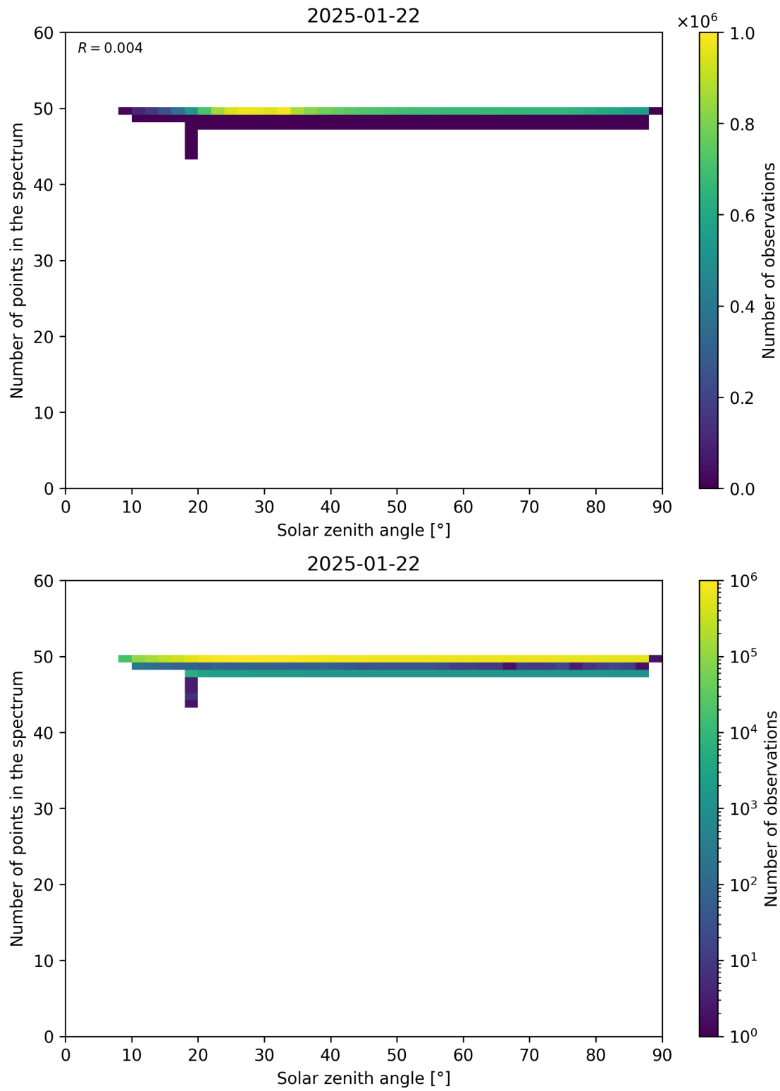
Figure 115: Scatter density plot of “Solar zenith angle” against “Number of points in the spectrum” for 2025-01-21 to 2025-01-23.
