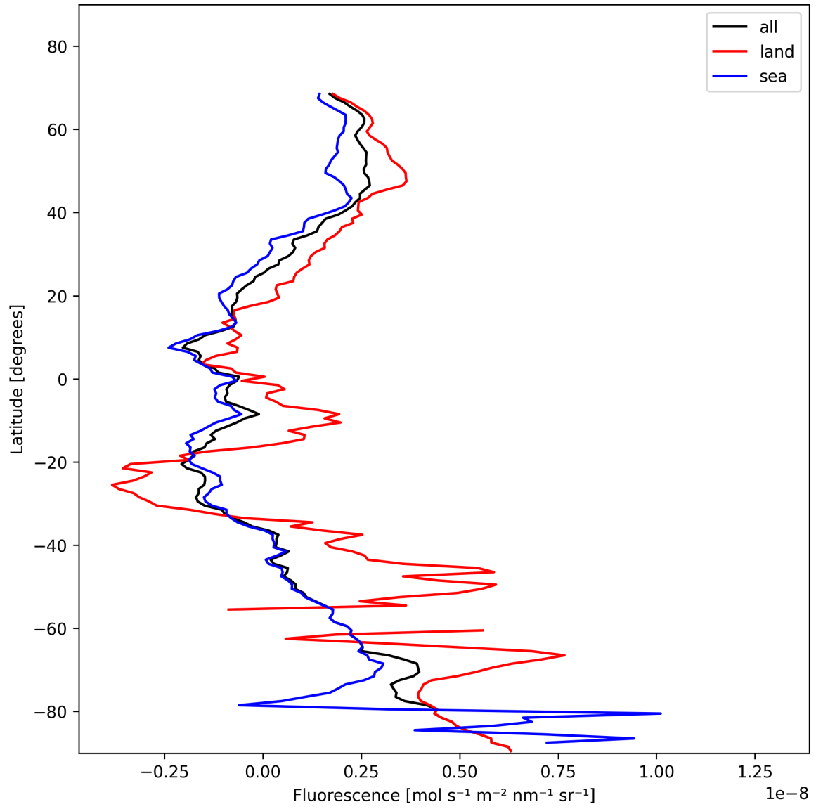
Figure 23: Zonal average of “Fluorescence” for 2025-01-21 to 2025-01-23.
