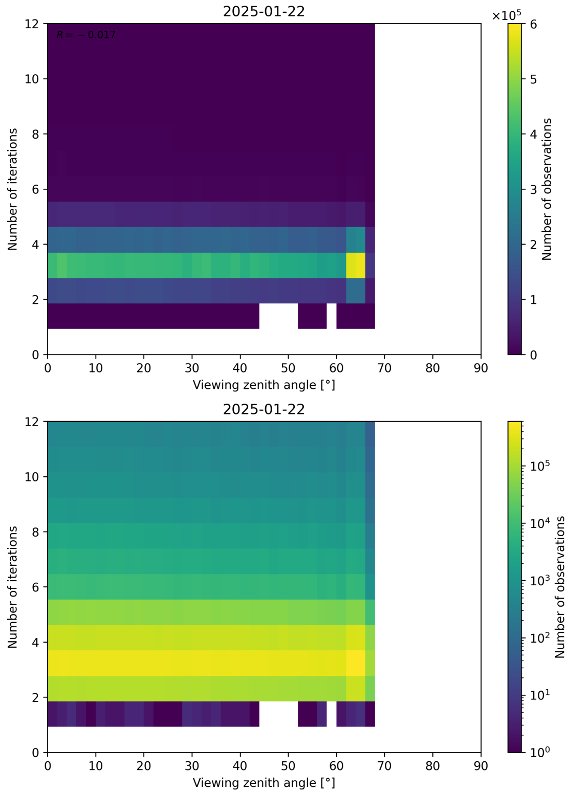
Figure 124: Scatter density plot of “Viewing zenith angle” against “Number of iterations” for 2025-01-21 to 2025-01-23.
