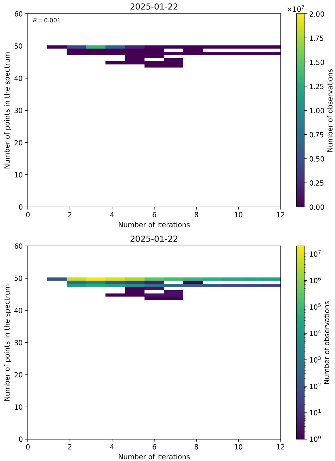
Figure 99: Scatter density plot of “Number of iterations” against “Number of points in the spectrum” for 2025-01-21 to 2025-01-23.
