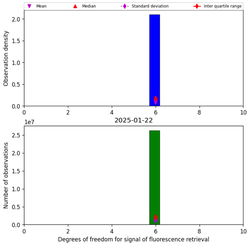
Figure 43: Histogram of "Degrees of freedom for signal of fluorescence retrieval" for 2025-01-21 to 2025-01-23
