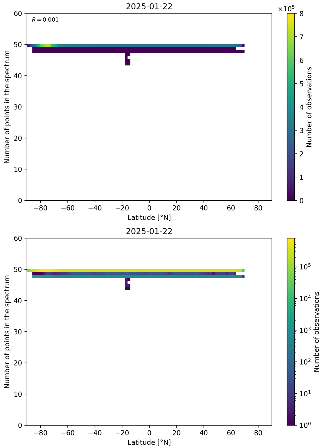
Figure 94: Scatter density plot of “Latitude” against “Number of points in the spectrum” for 2025-01-21 to 2025-01-23.
