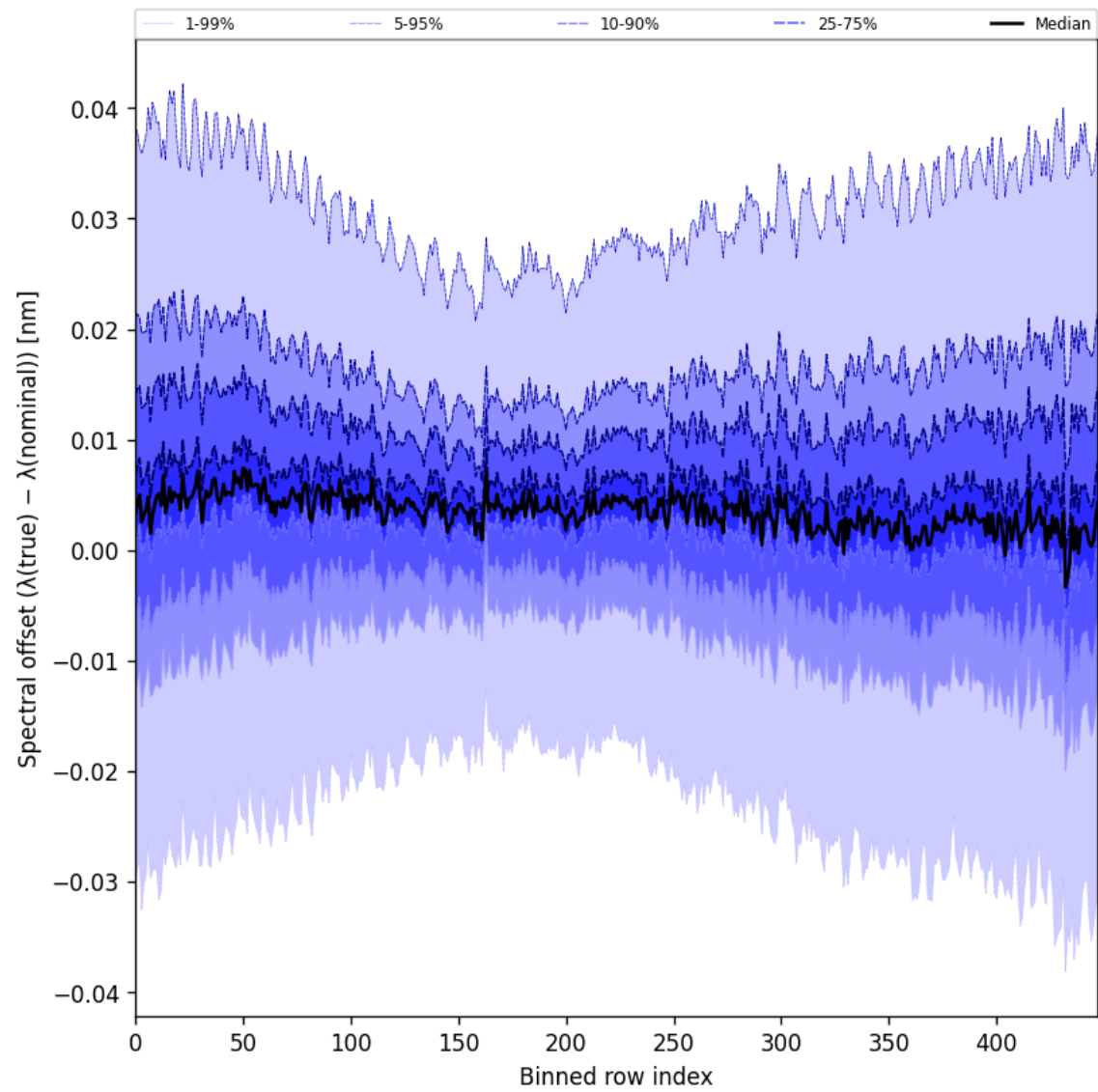
Figure 62: Along track statistics of “Spectral offset ( \lambda_{\text{true}} - \lambda_{\text{nominal}} )” for 2025-01-21 to 2025-01-23
