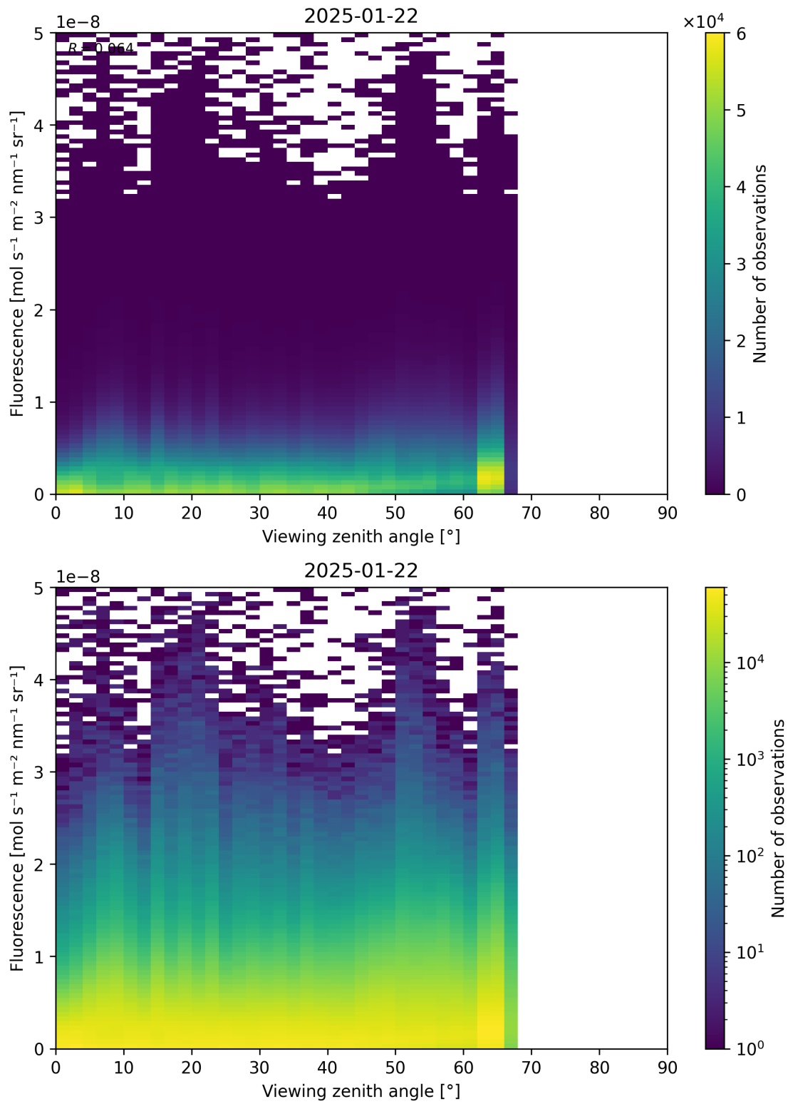
Figure 122: Scatter density plot of “Viewing zenith angle” against “Fluorescence” for 2025-01-21 to 2025-01-23.
