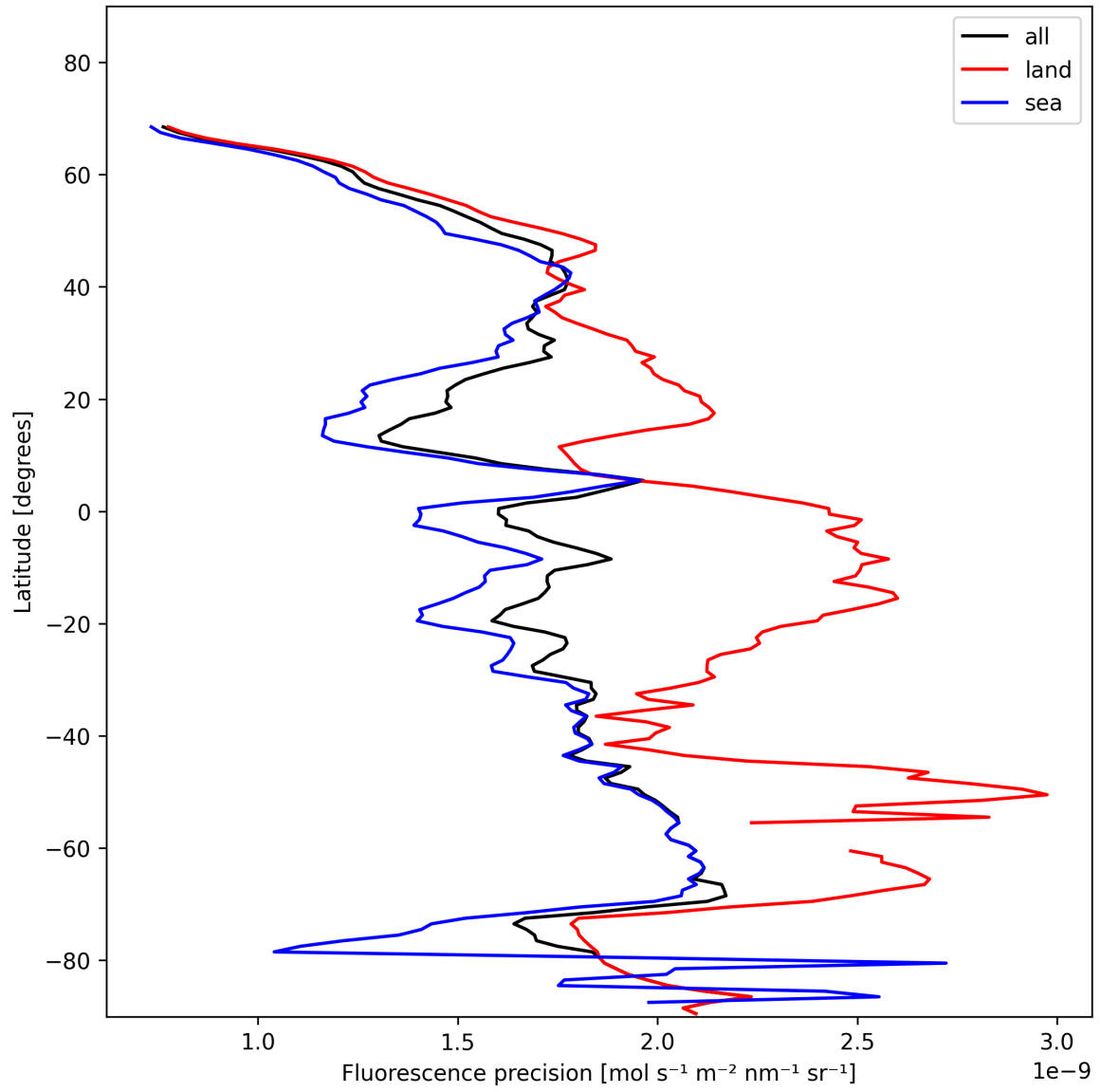
Figure 24: Zonal average of “Fluorescence precision” for 2025-01-21 to 2025-01-23.
