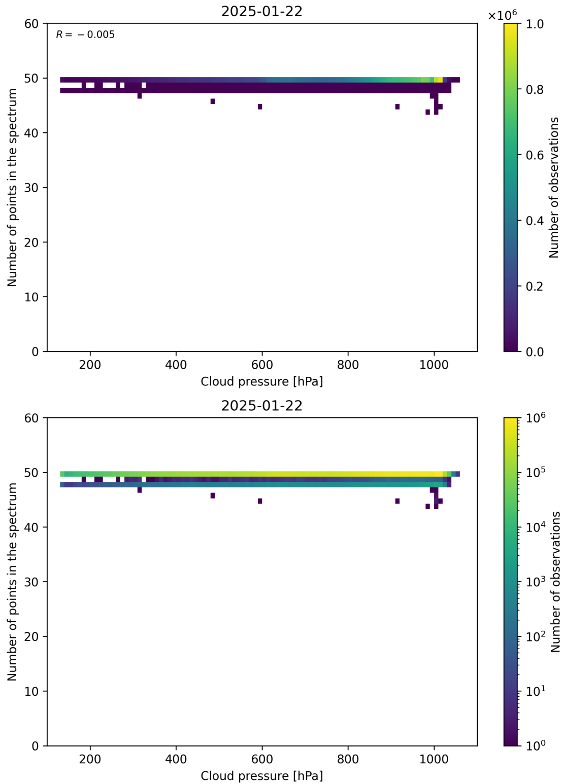
Figure 82: Scatter density plot of “Cloud pressure” against “Number of points in the spectrum” for 2025-01-21 to 2025-01-23.
