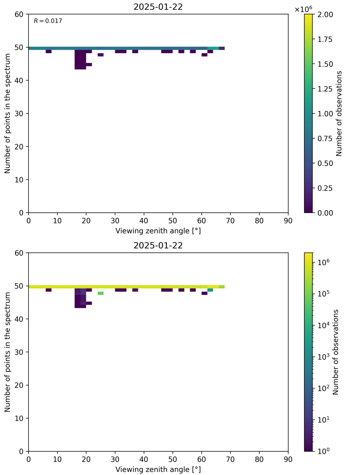
Figure 125: Scatter density plot of “Viewing zenith angle” against “Number of points in the spectrum” for 2025-01-21 to 2025-01-23.
