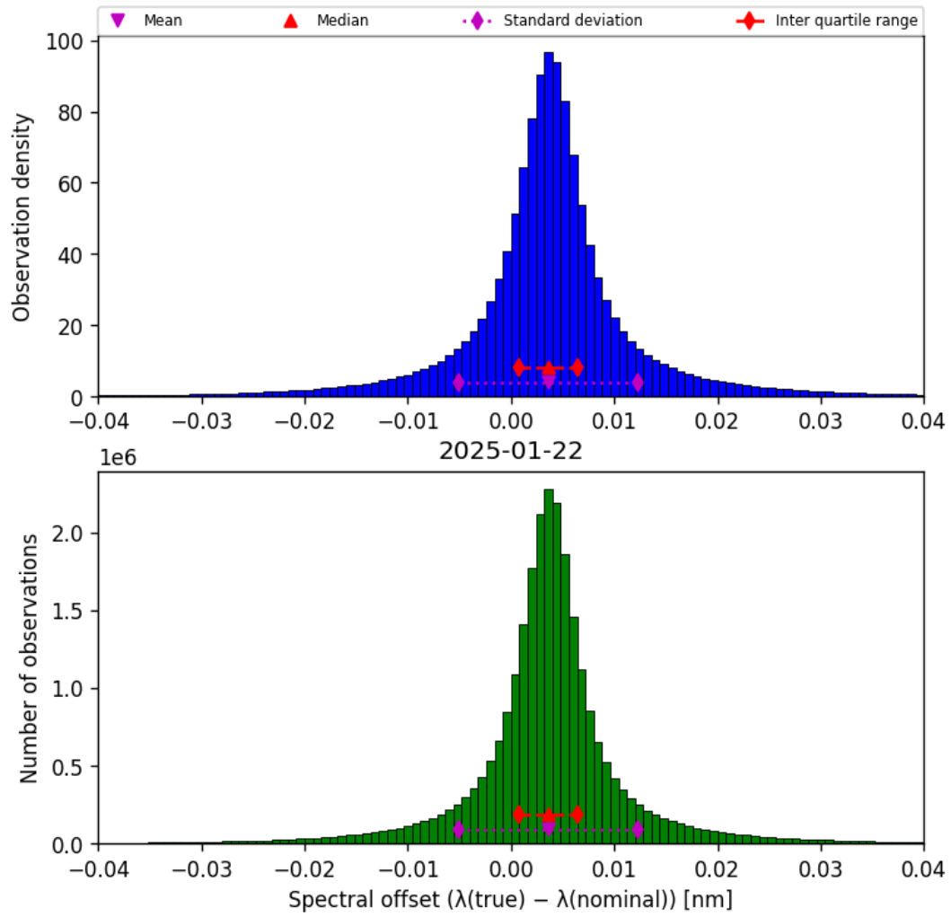
Figure 45: Histogram of “Spectral offset ( \lambda_{\text{true}} - \lambda_{\text{nominal}} )” for 2025-01-21 to 2025-01-23
