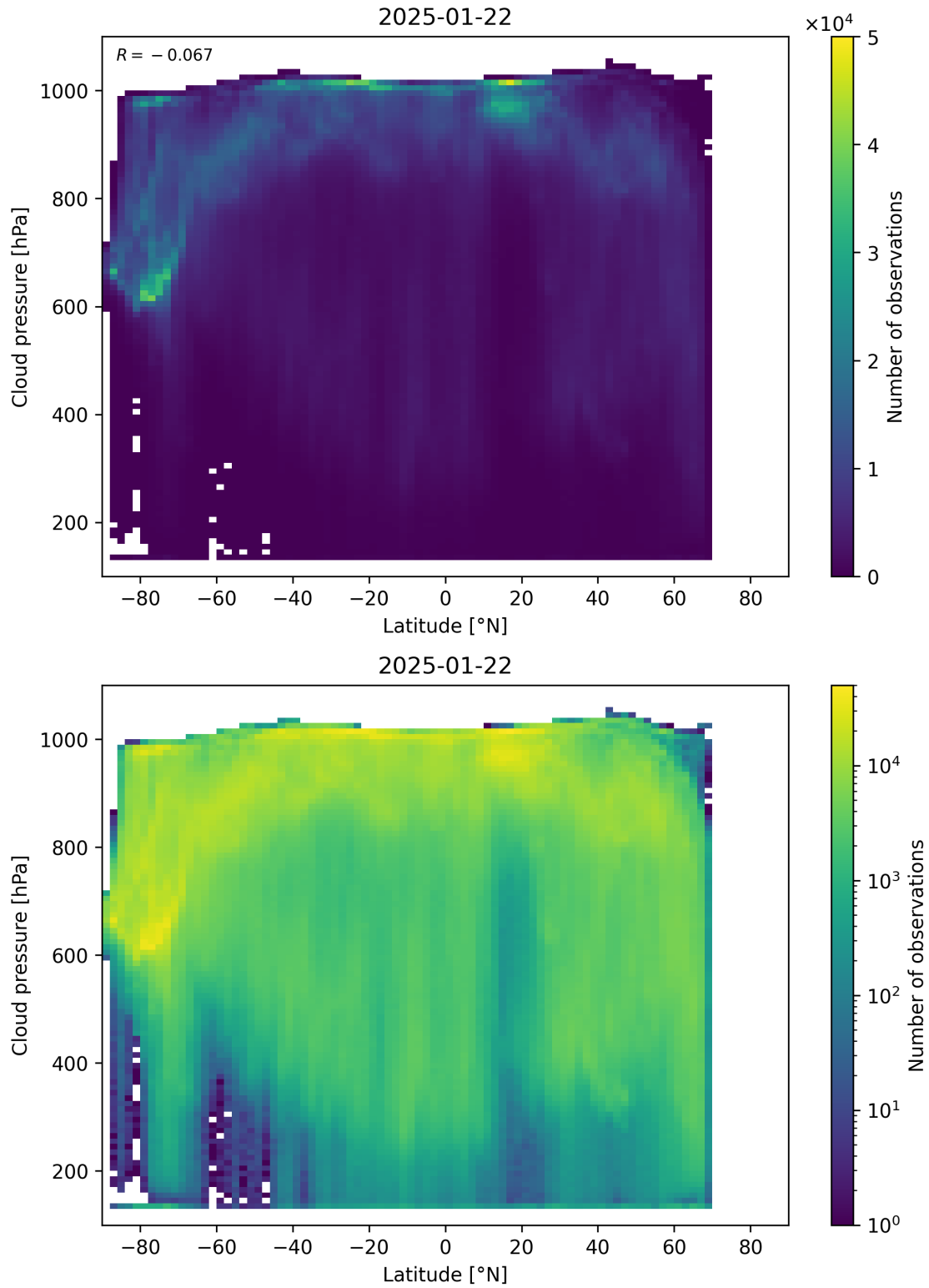
Figure 91: Scatter density plot of “Latitude” against “Cloud pressure” for 2025-01-21 to 2025-01-23.
