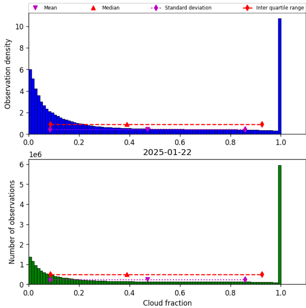
Figure 32: Histogram of “Cloud fraction” for 2025-01-21 to 2025-01-23
