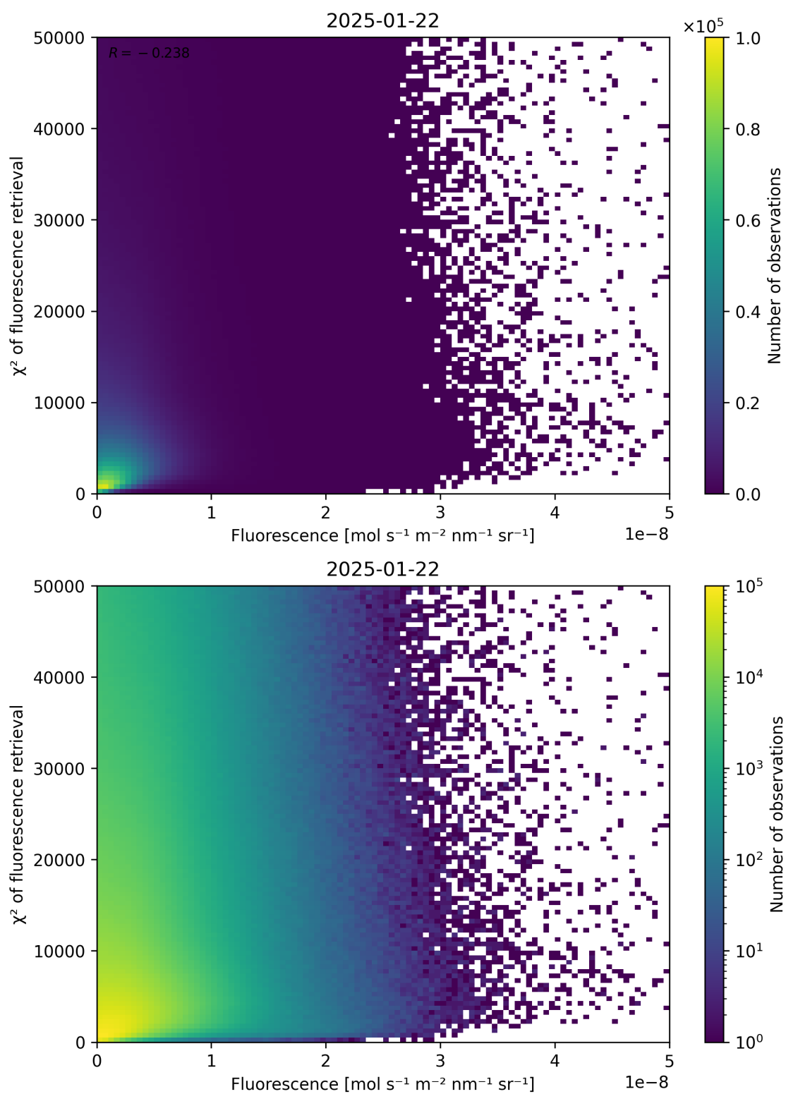
Figure 85: Scatter density plot of “Fluorescence” against “ \chi^2 of fluorescence retrieval” for 2025-01-21 to 2025-01-23.
