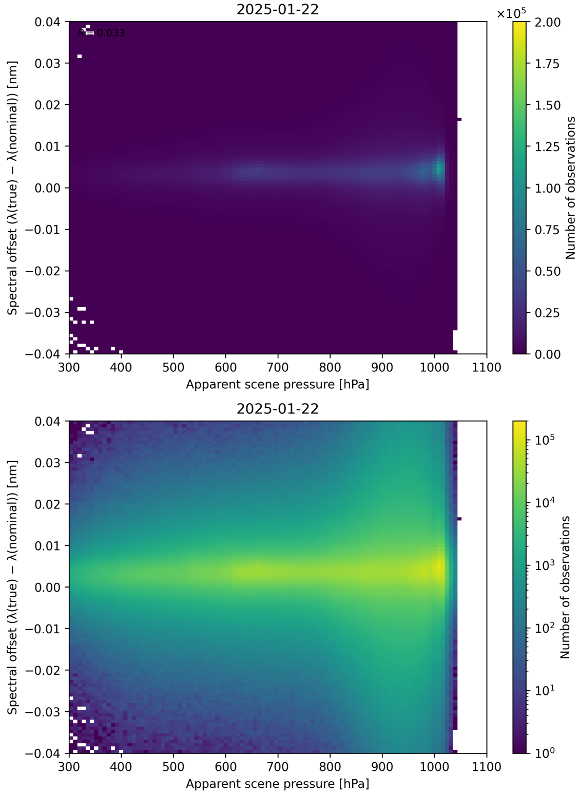
Figure 67: Scatter density plot of “Apparent scene pressure” against “Spectral offset ( \lambda_{\text{true}} - \lambda_{\text{nominal}} )” for 2025-01-21 to 2025-01-23.
