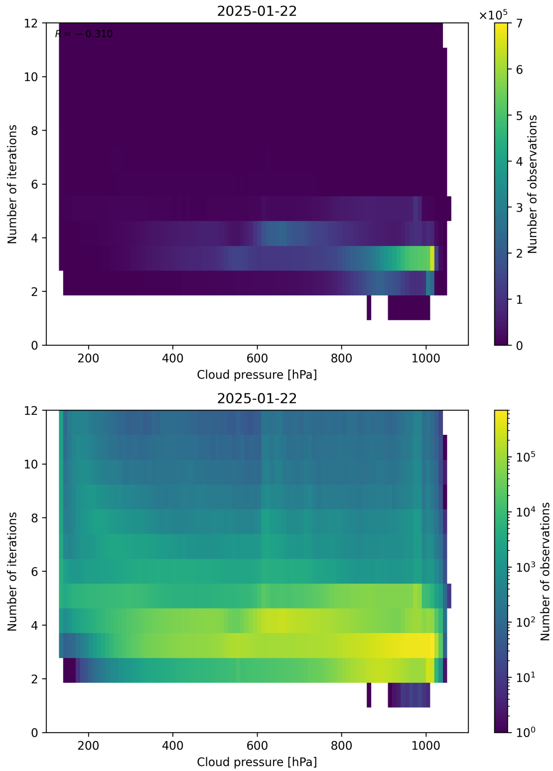
Figure 81: Scatter density plot of “Cloud pressure” against “Number of iterations” for 2025-01-21 to 2025-01-23.
