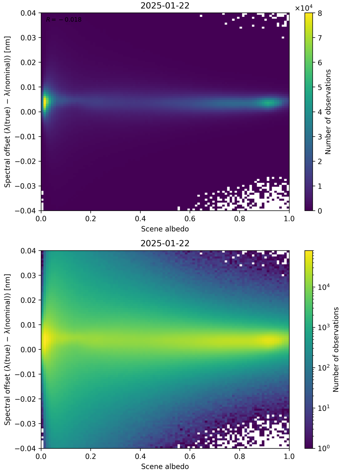
Figure 107: Scatter density plot of “Scene albedo” against “Spectral offset ( \lambda_{\text{true}} - \lambda_{\text{nominal}} )” for 2025-01-21 to 2025-01-23.
