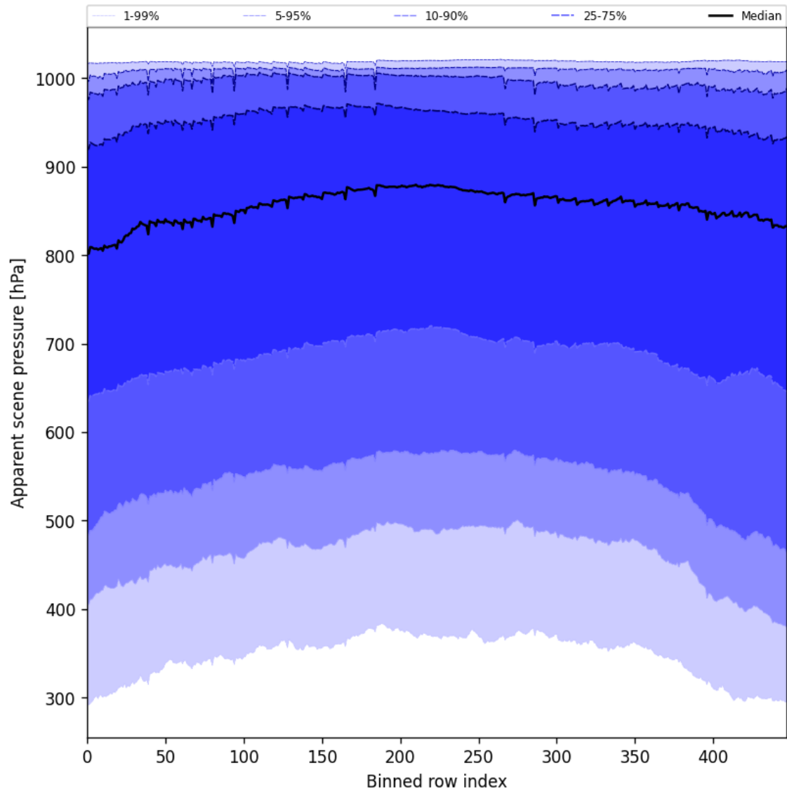
Figure 53: Along track statistics of “Apparent scene pressure” for 2025-01-21 to 2025-01-23
