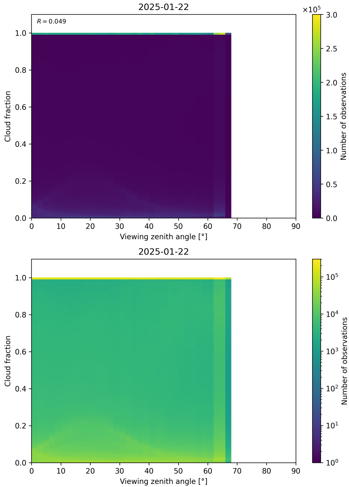
Figure 120: Scatter density plot of “Viewing zenith angle” against “Cloud fraction” for 2025-01-21 to 2025-01-23.
