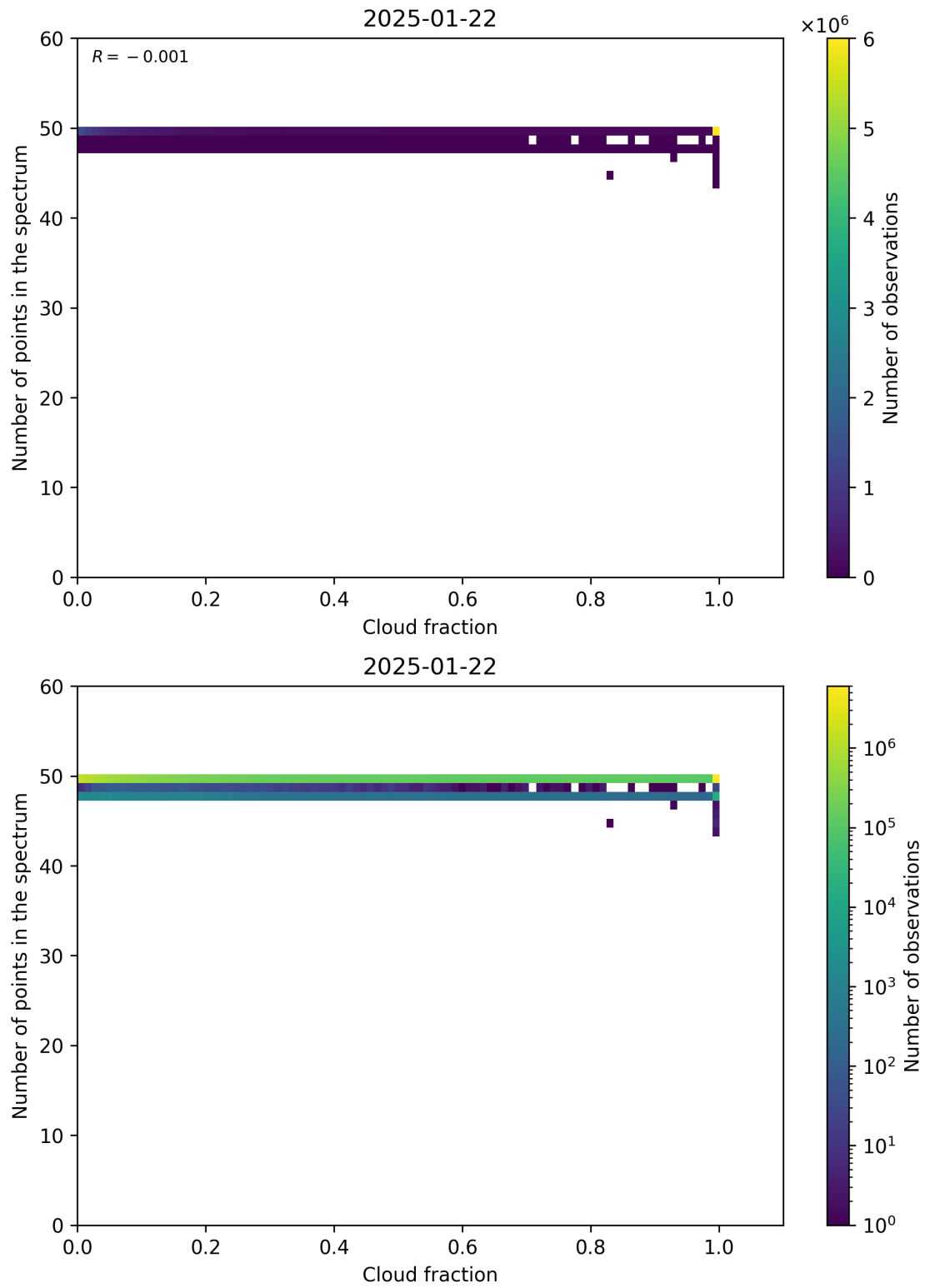
Figure 74: Scatter density plot of “Cloud fraction” against “Number of points in the spectrum” for 2025-01-21 to 2025-01-23.
