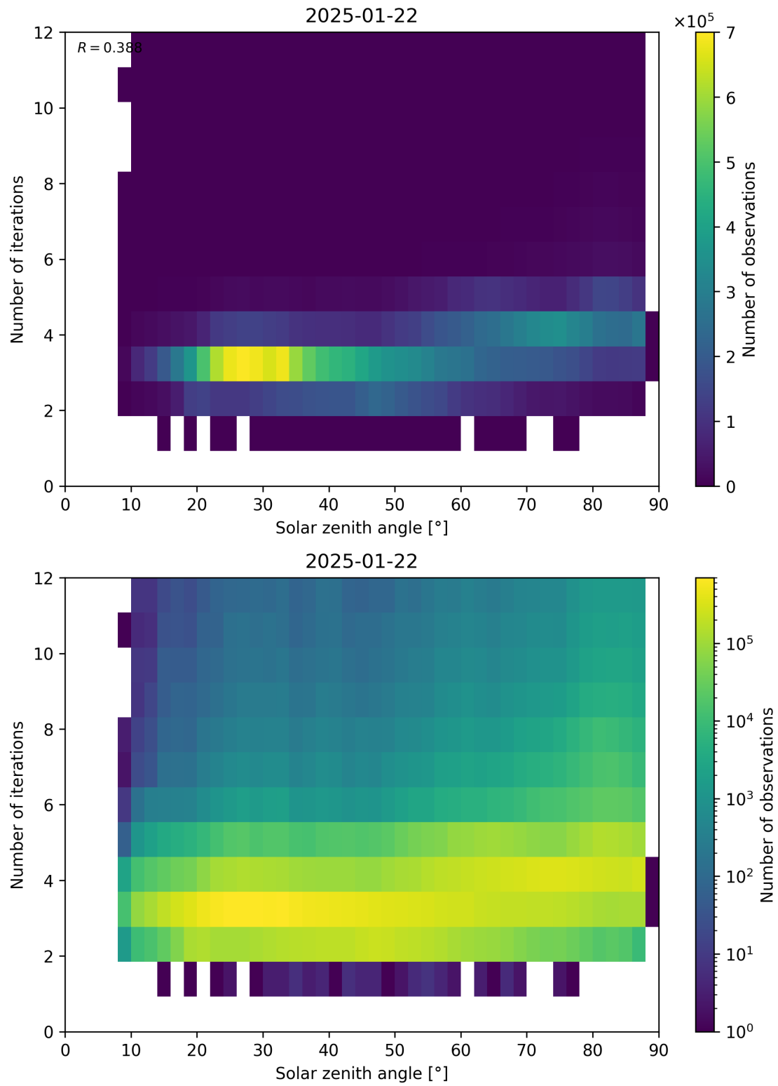
Figure 114: Scatter density plot of “Solar zenith angle” against “Number of iterations” for 2025-01-21 to 2025-01-23.
