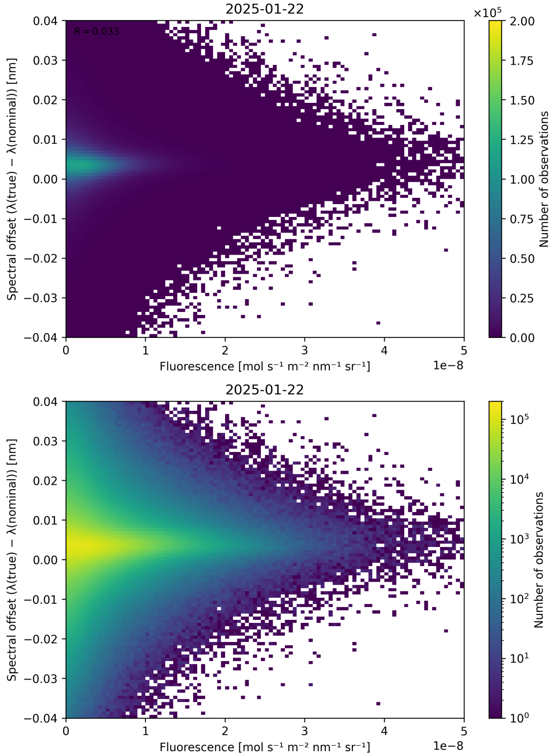
Figure 87: Scatter density plot of “Fluorescence” against “Spectral offset ( \lambda_{\text{true}} - \lambda_{\text{nominal}} )” for 2025-01-21 to 2025-01-23.
