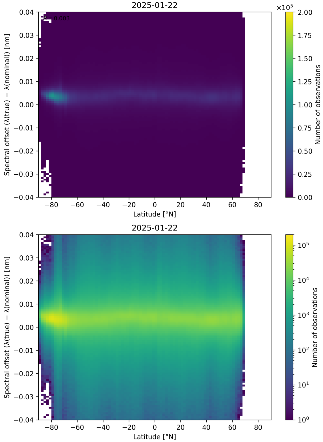
Figure 96: Scatter density plot of “Latitude” against “Spectral offset ( \lambda_{\text{true}} - \lambda_{\text{nominal}} )” for 2025-01-21 to 2025-01-23.
