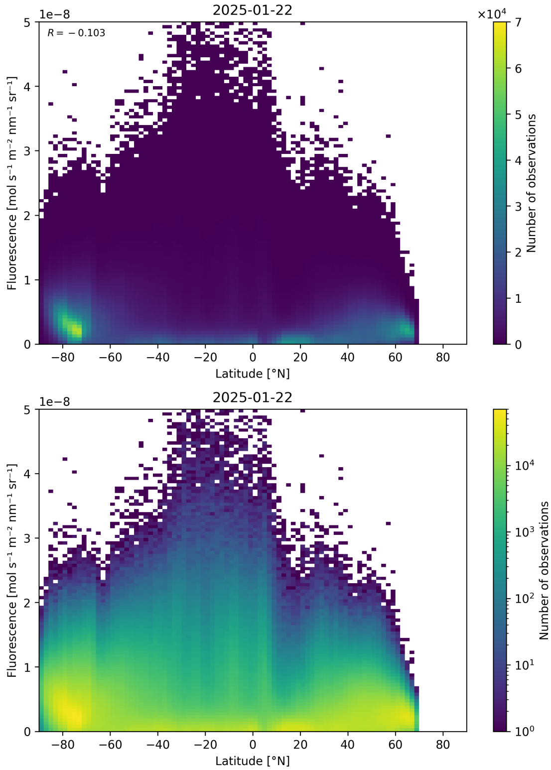
Figure 92: Scatter density plot of “Latitude” against “Fluorescence” for 2025-01-21 to 2025-01-23.
