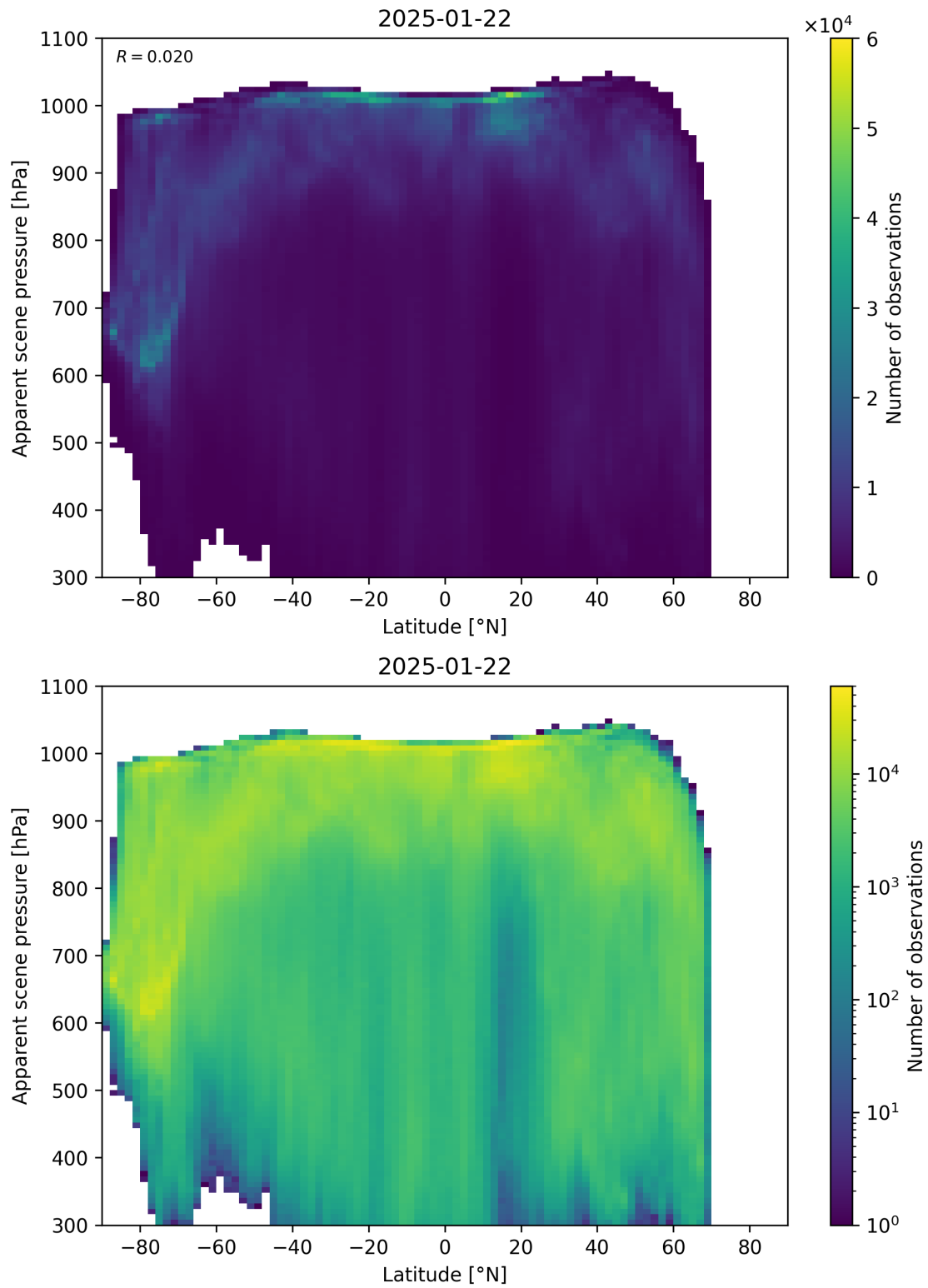
Figure 88: Scatter density plot of “Latitude” against “Apparent scene pressure” for 2025-01-21 to 2025-01-23.
