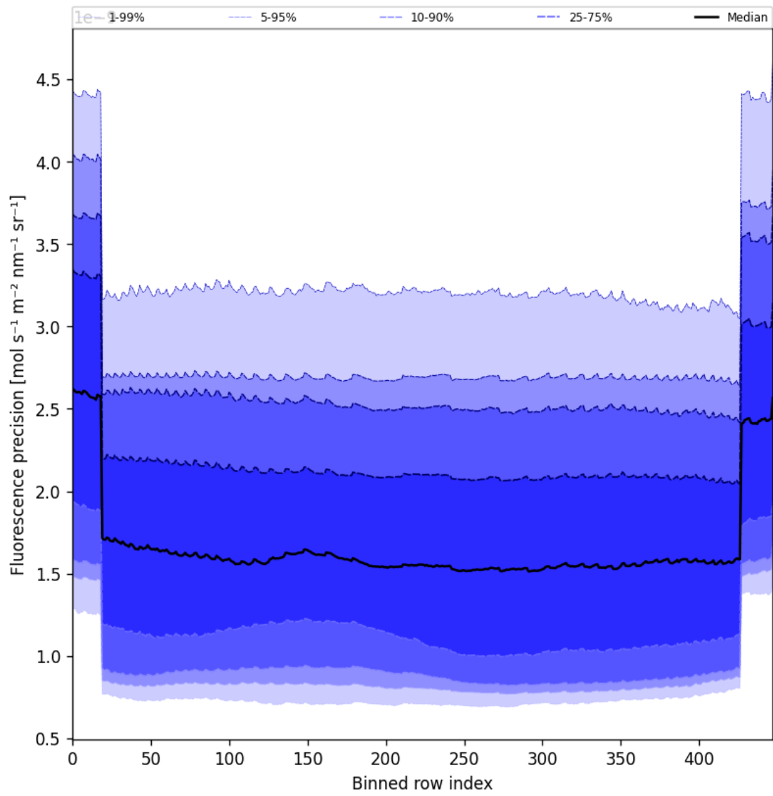
Figure 58: Along track statistics of “Fluorescence precision” for 2025-01-21 to 2025-01-23
