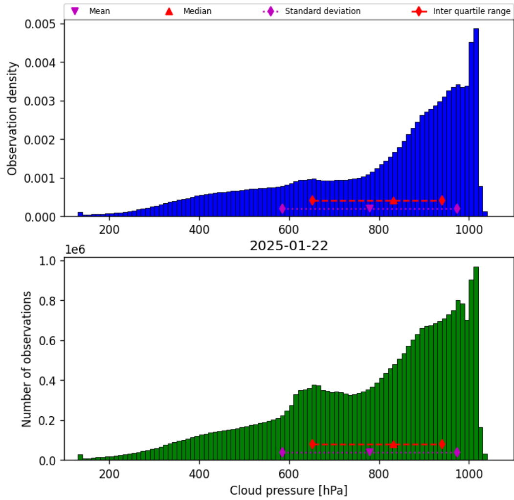
Figure 30: Histogram of “Cloud pressure” for 2025-01-21 to 2025-01-23
