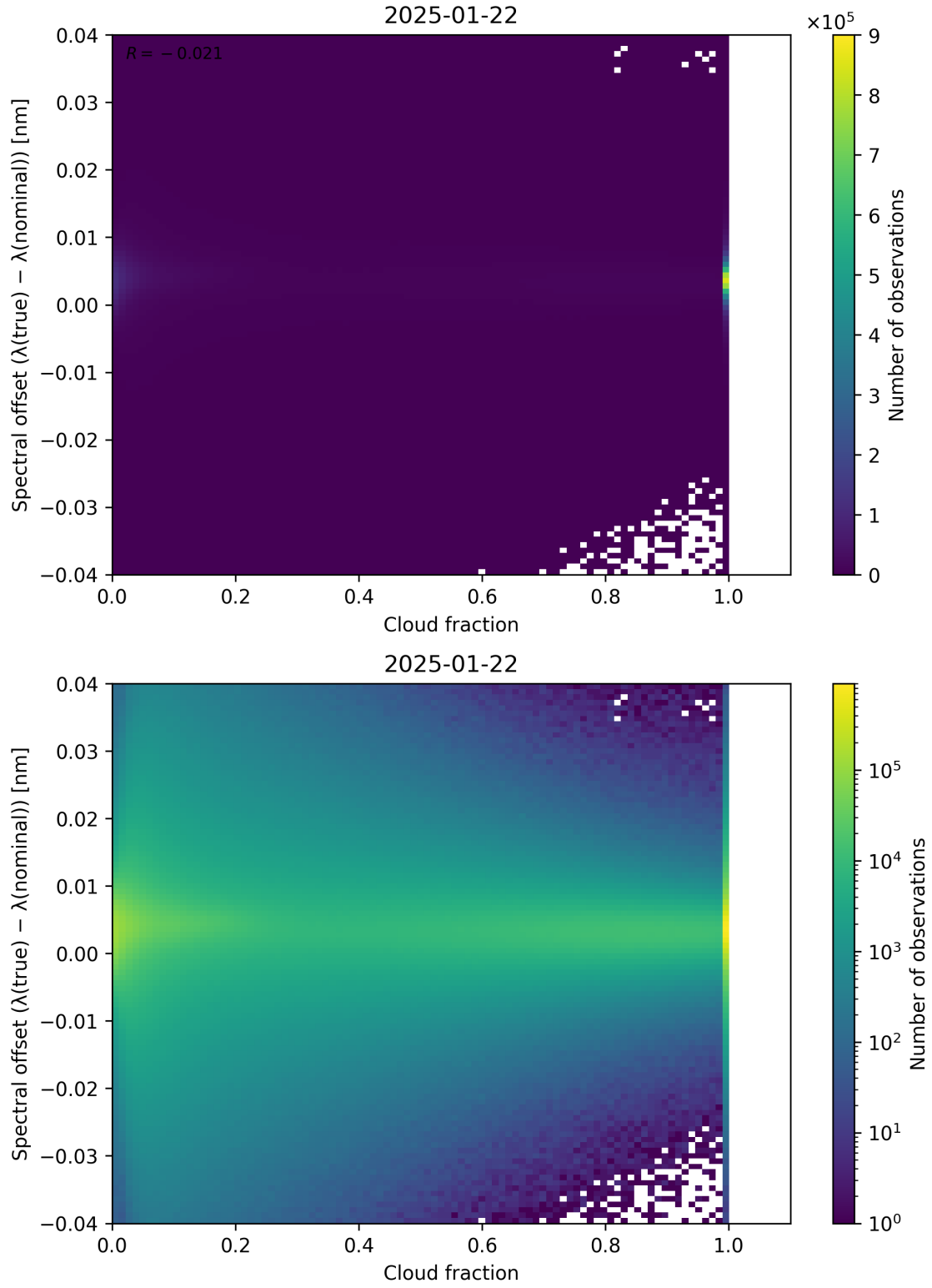
Figure 76: Scatter density plot of “Cloud fraction” against “Spectral offset ( \lambda_{\text{true}} - \lambda_{\text{nominal}} )” for 2025-01-21 to 2025-01-23.
