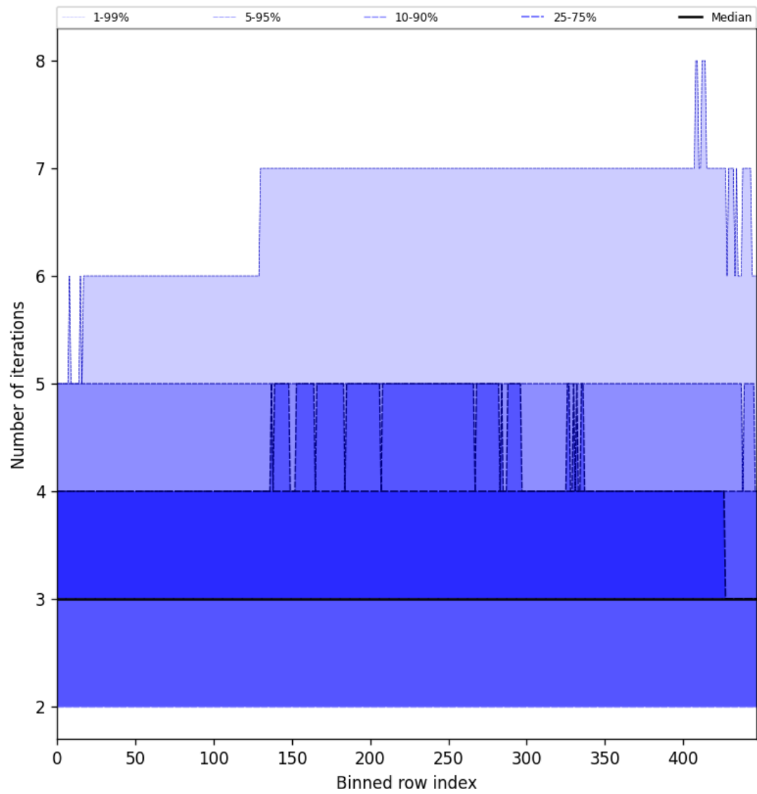
Figure 56: Along track statistics of “Number of iterations” for 2025-01-21 to 2025-01-23
