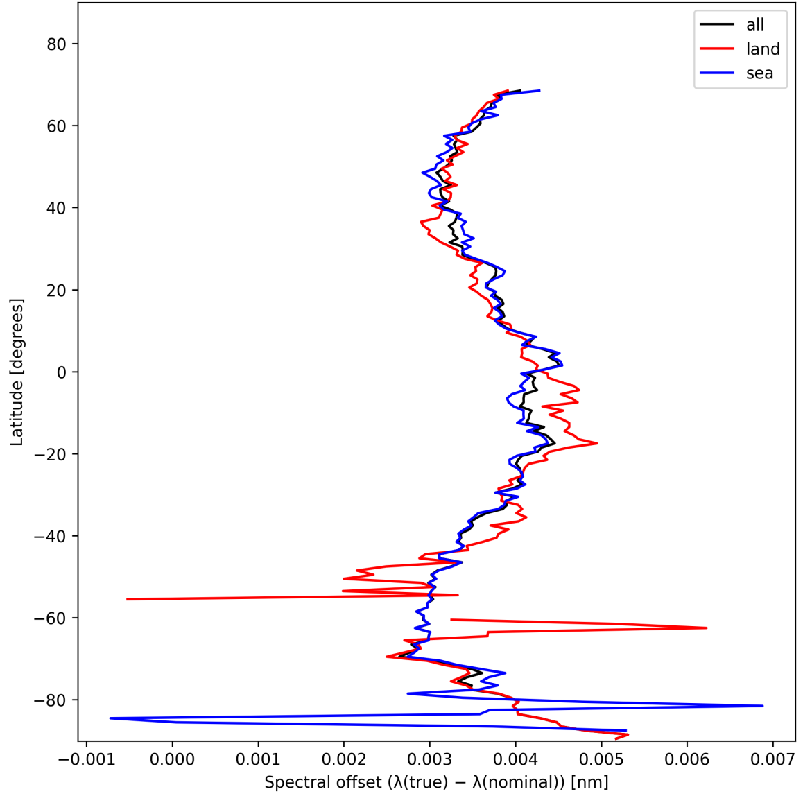
Figure 28: Zonal average of “Spectral offset ( \lambda_{\text{true}} - \lambda_{\text{nominal}} )” for 2025-01-21 to 2025-01-23.
