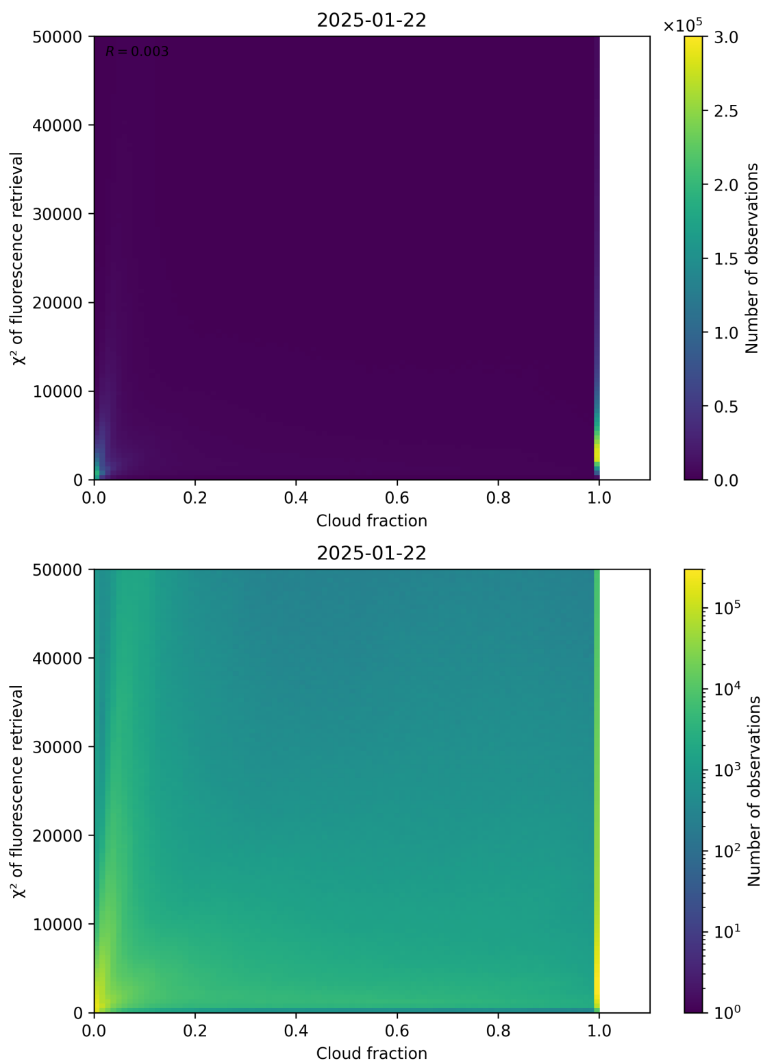
Figure 71: Scatter density plot of “Cloud fraction” against “ \chi^2 of fluorescence retrieval” for 2025-01-21 to 2025-01-23.
