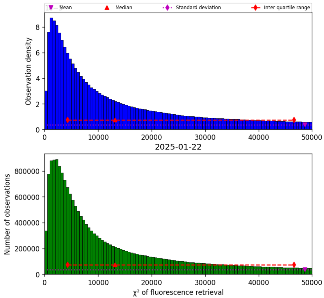
Figure 42: Histogram of “ \chi^2 of fluorescence retrieval” for 2025-01-21 to 2025-01-23
