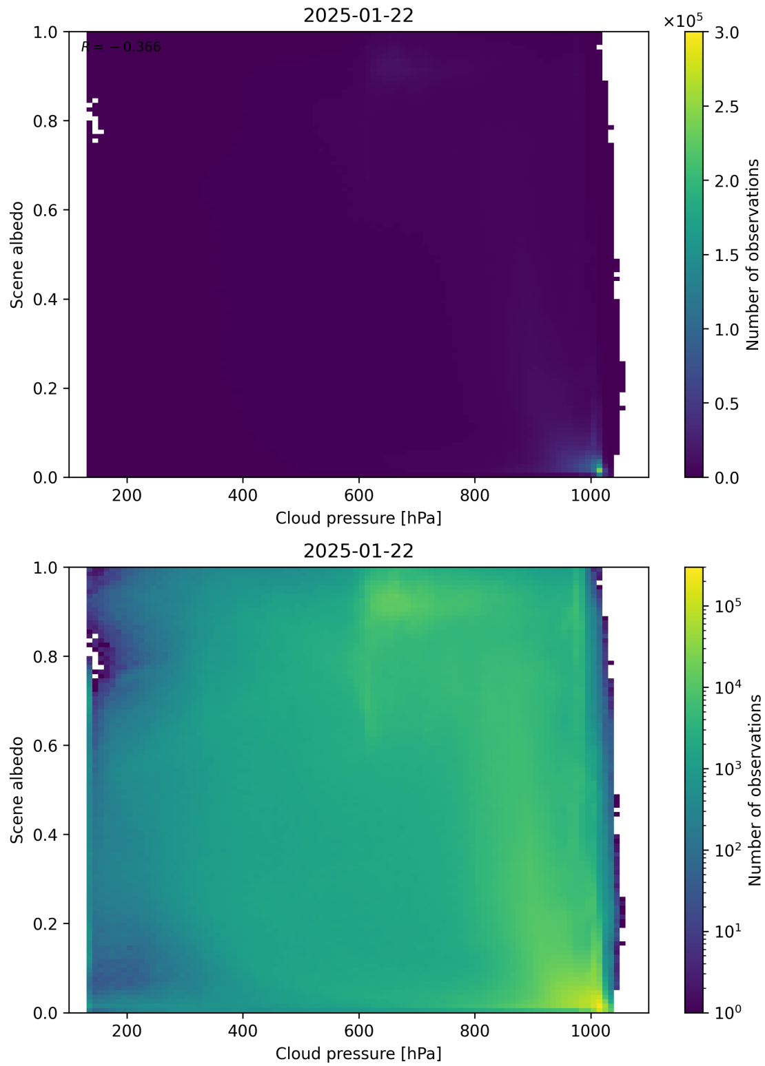
Figure 83: Scatter density plot of “Cloud pressure” against “Scene albedo” for 2025-01-21 to 2025-01-23.
