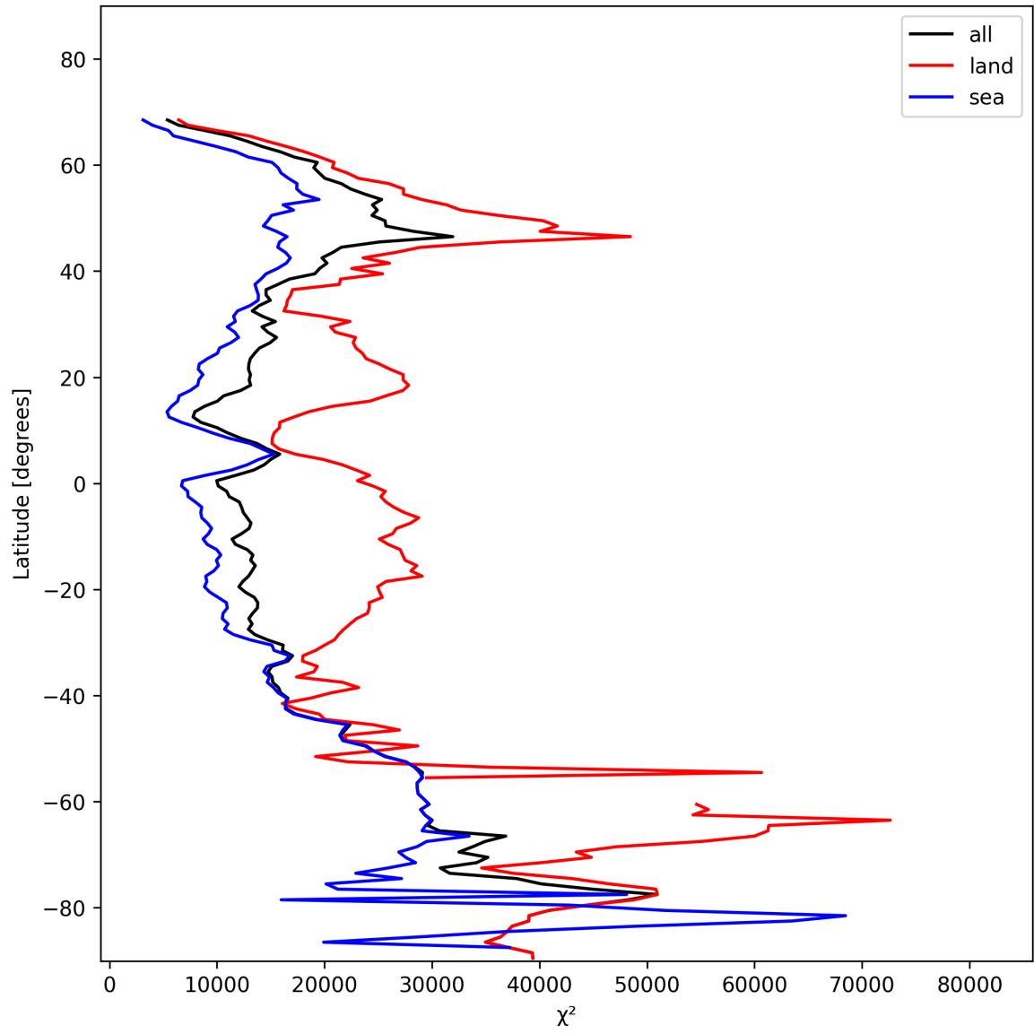
Figure 21: Zonal average of “ \chi^2 ” for 2025-01-21 to 2025-01-23.
