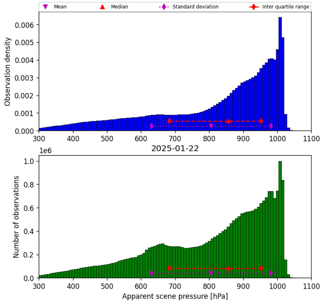
Figure 36: Histogram of “Apparent scene pressure” for 2025-01-21 to 2025-01-23
