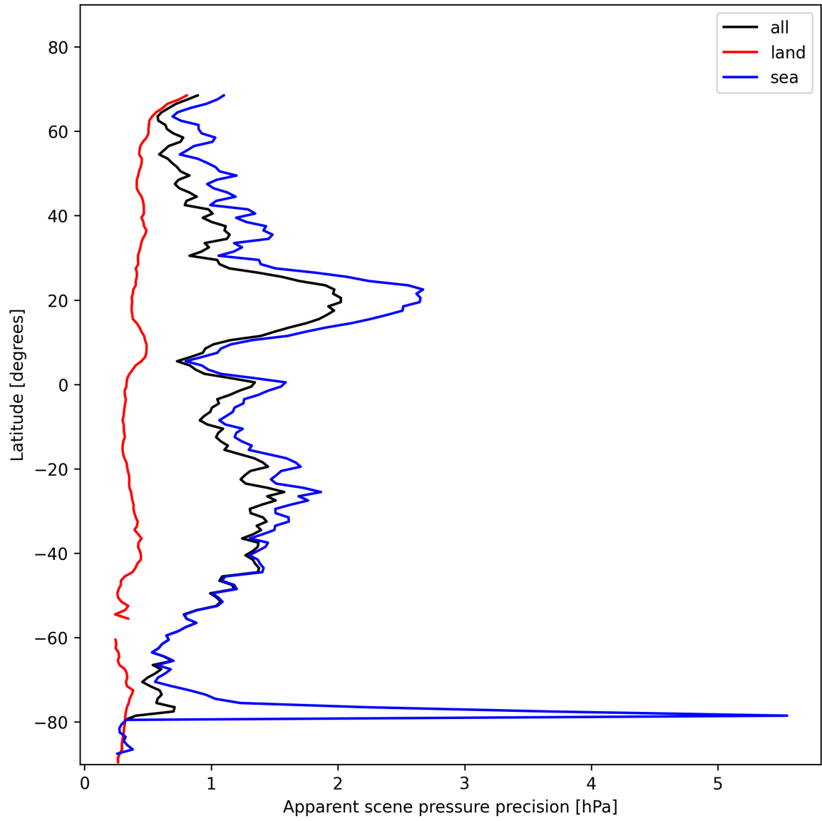
Figure 20: Zonal average of “Apparent scene pressure precision” for 2025-01-21 to 2025-01-23.
