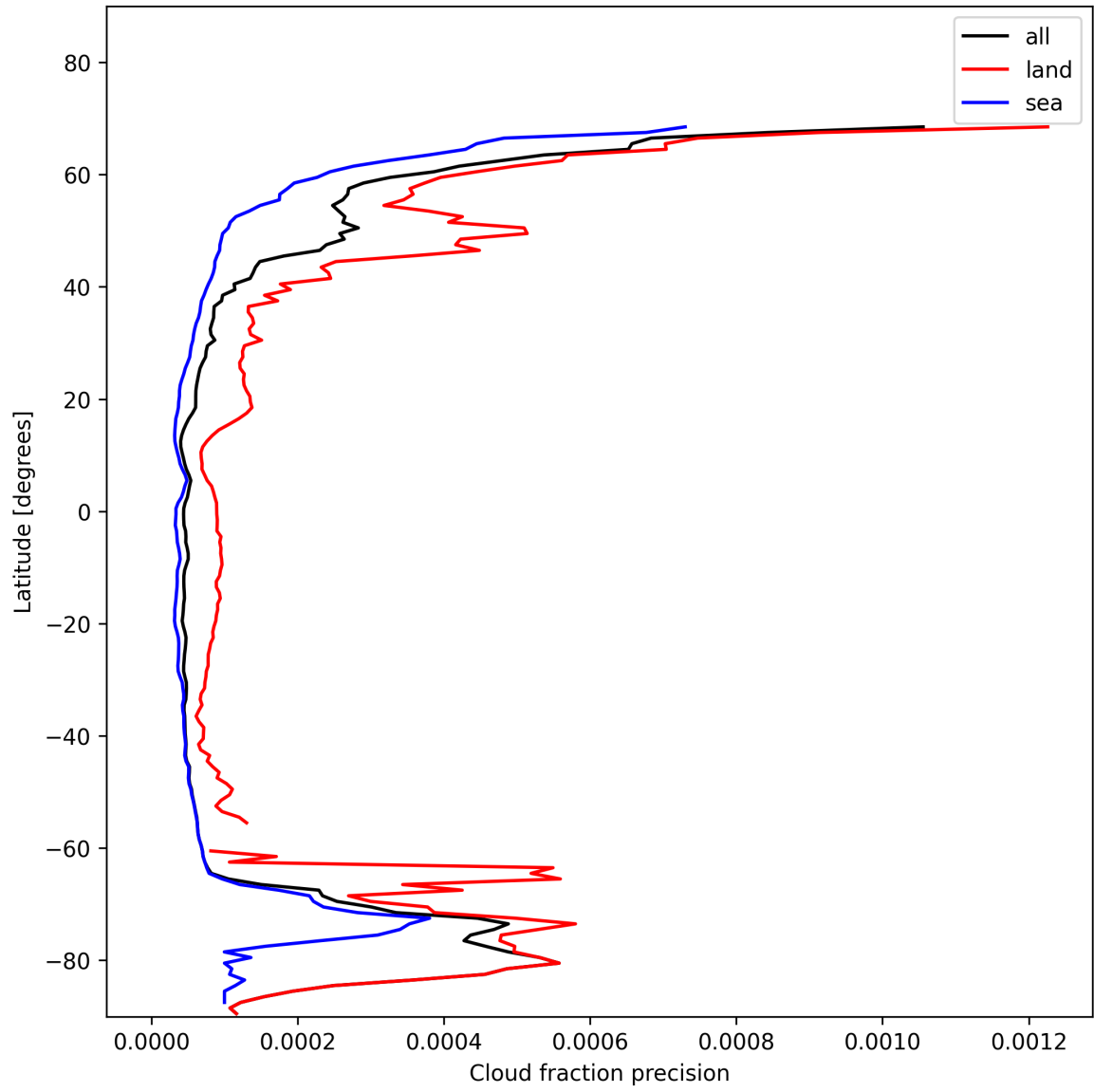
Figure 16: Zonal average of “Cloud fraction precision” for 2025-01-21 to 2025-01-23.
