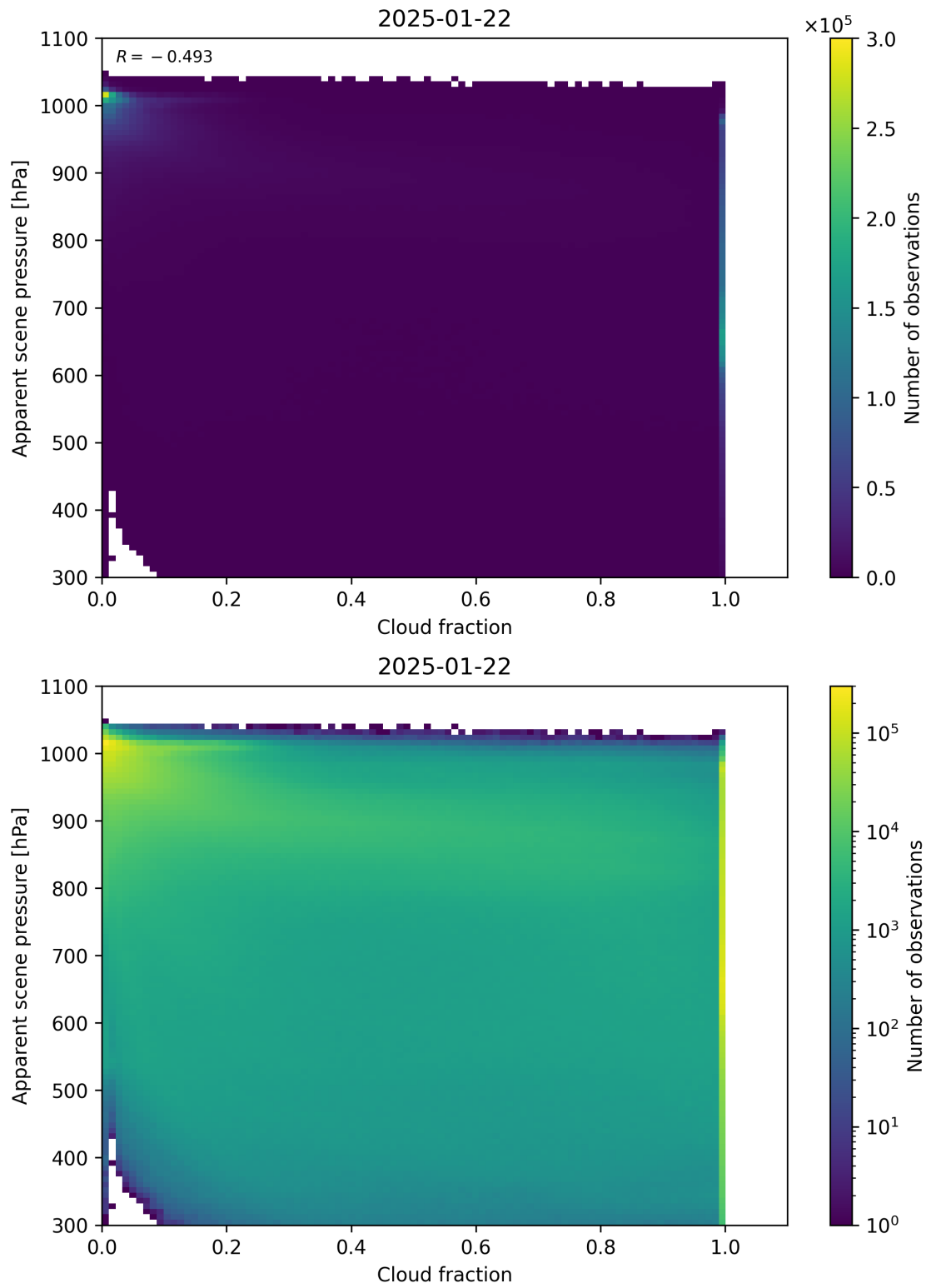
Figure 70: Scatter density plot of “Cloud fraction” against “Apparent scene pressure” for 2025-01-21 to 2025-01-23.
