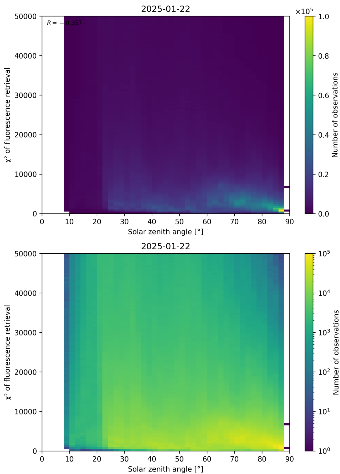
Figure 109: Scatter density plot of “Solar zenith angle” against “ \chi^2 of fluorescence retrieval” for 2025-01-21 to 2025-01-23.
