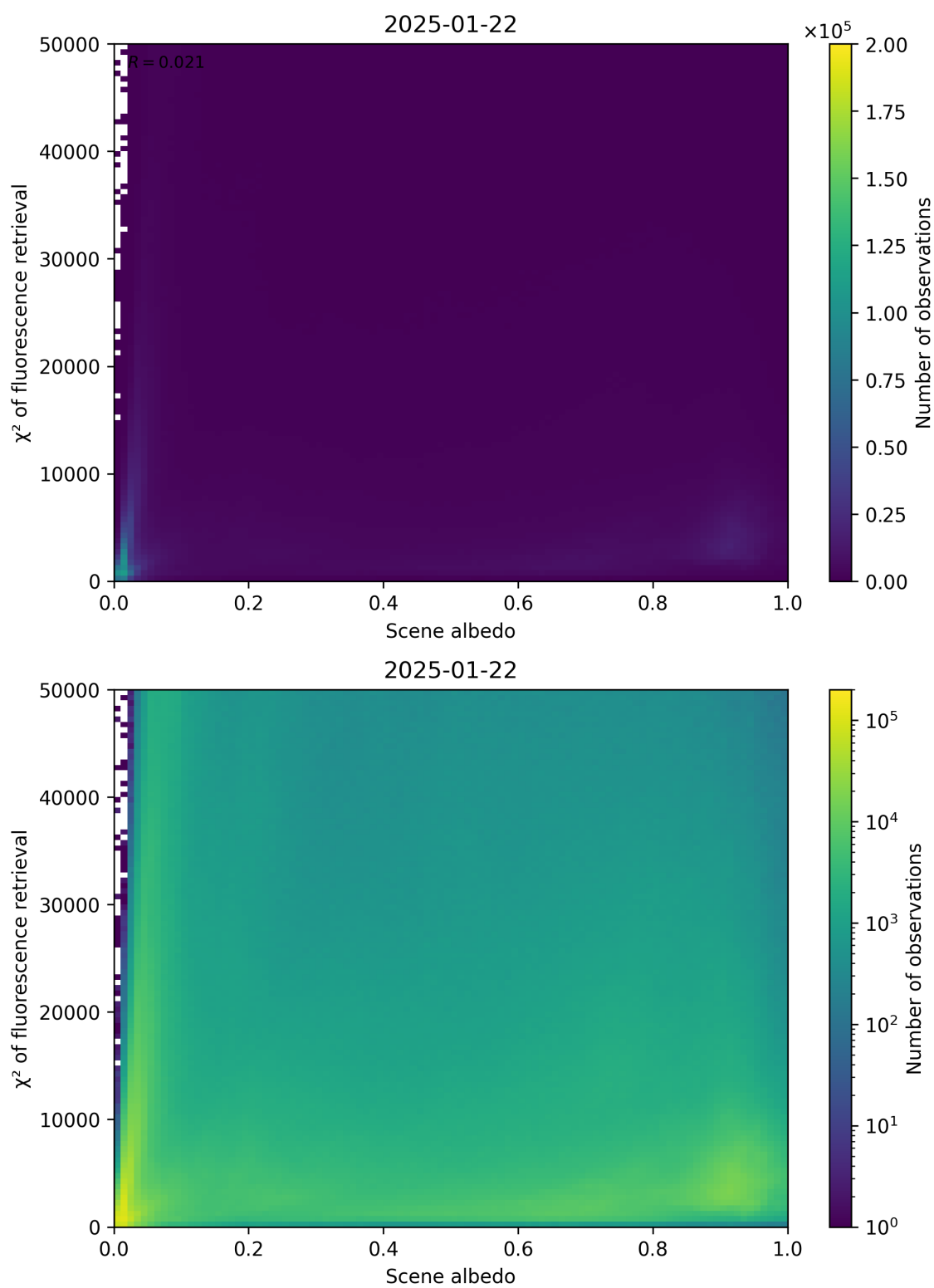
Figure 103: Scatter density plot of “Scene albedo” against “ \chi^2 of fluorescence retrieval” for 2025-01-21 to 2025-01-23.
