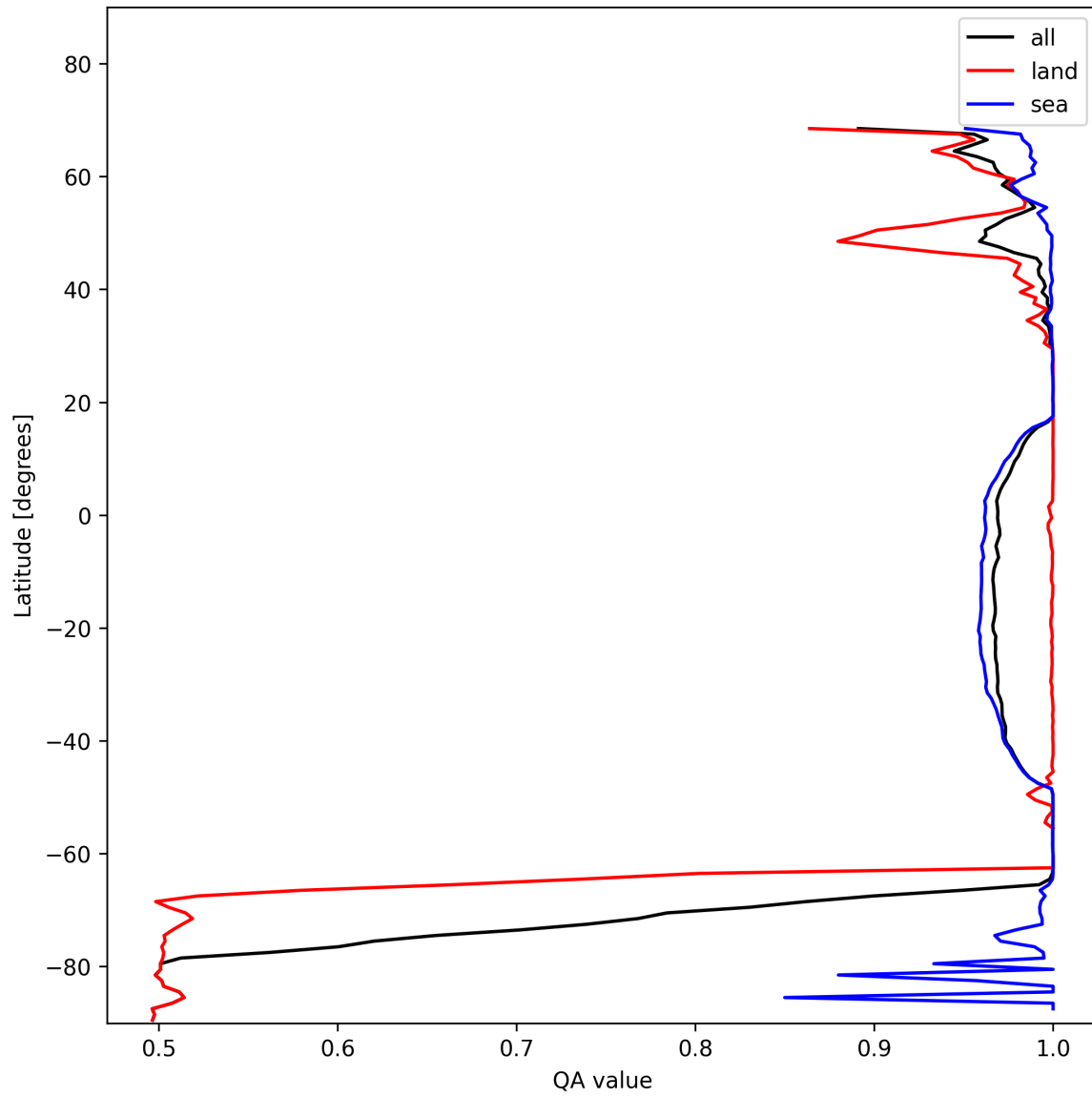
Figure 12: Zonal average of “QA value” for 2025-01-21 to 2025-01-23.
