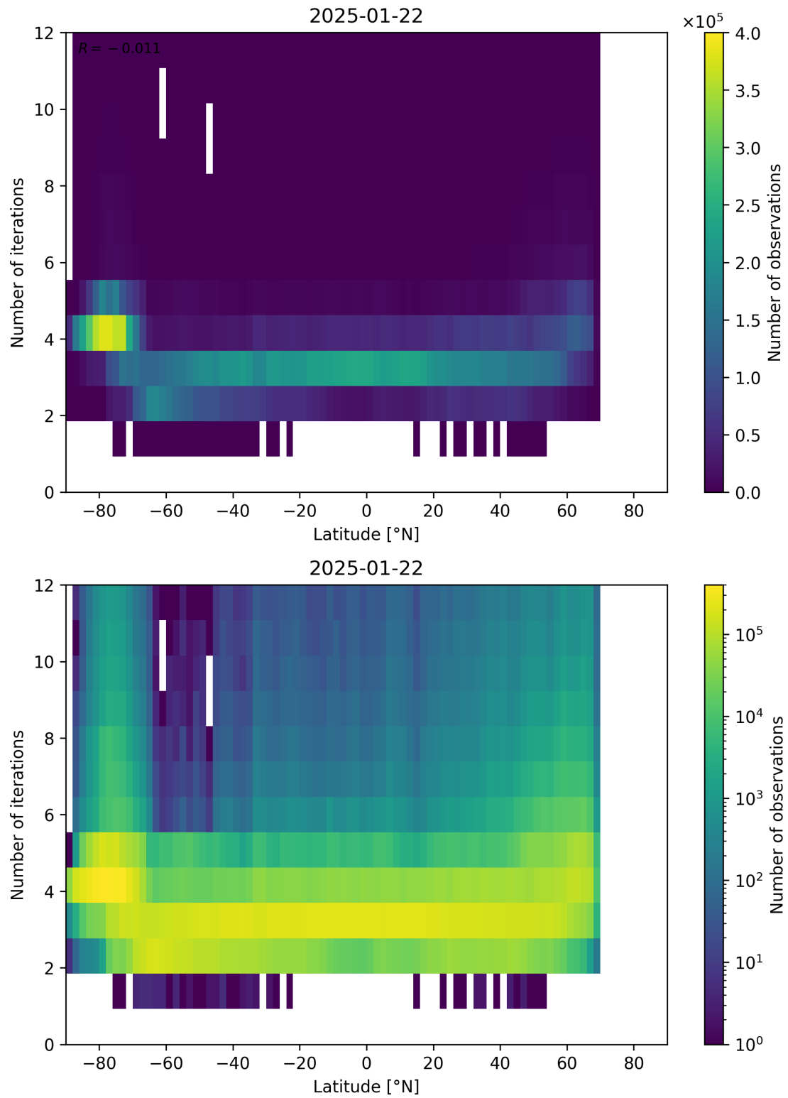
Figure 93: Scatter density plot of “Latitude” against “Number of iterations” for 2025-01-21 to 2025-01-23.
