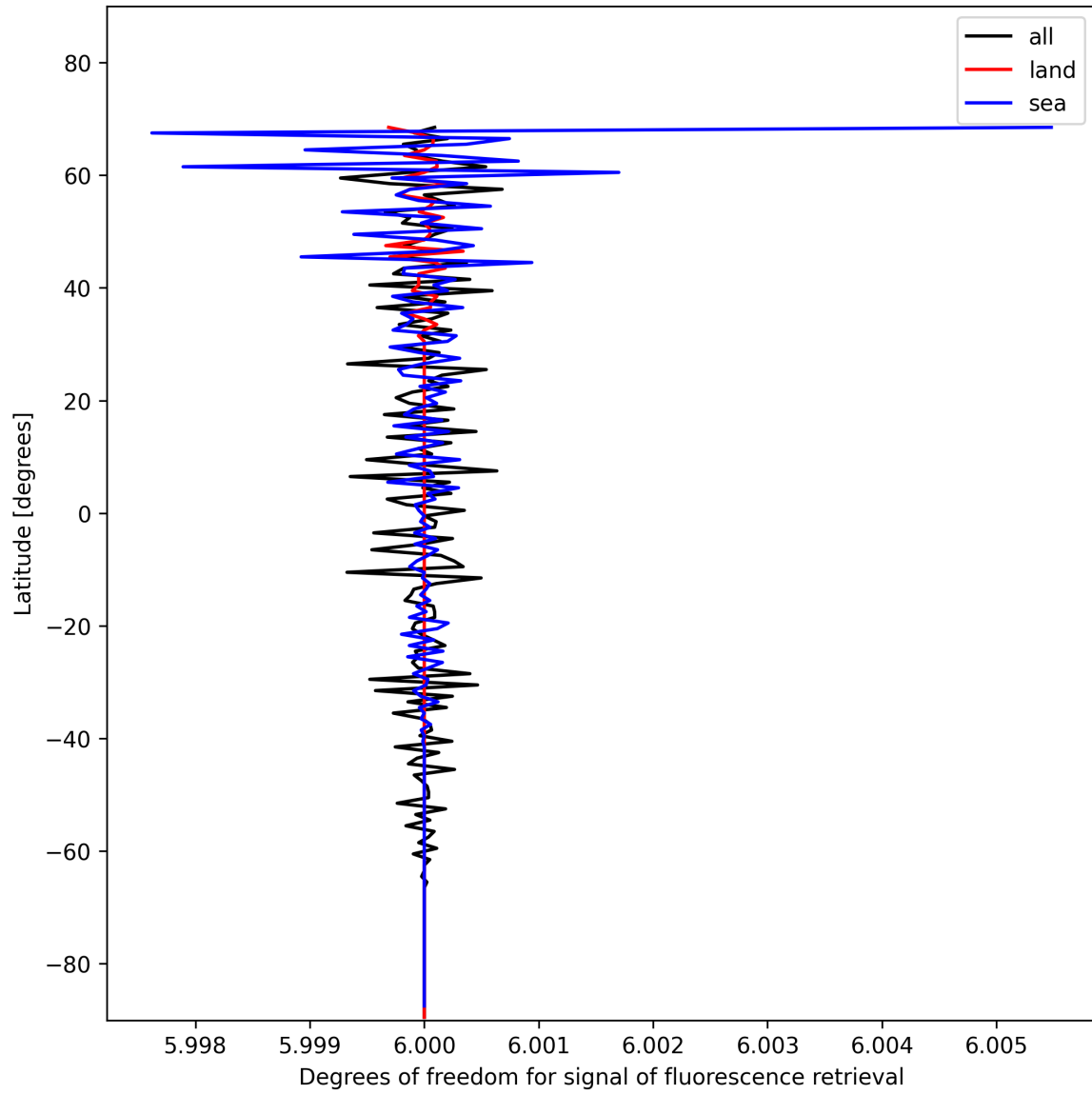
Figure 26: Zonal average of “Degrees of freedom for signal of fluorescence retrieval” for 2025-01-21 to 2025-01-23.
