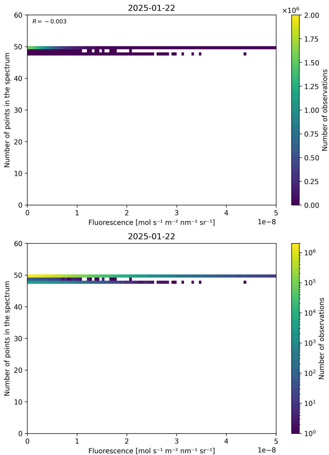
Figure 86: Scatter density plot of “Fluorescence” against “Number of points in the spectrum” for 2025-01-21 to 2025-01-23.
