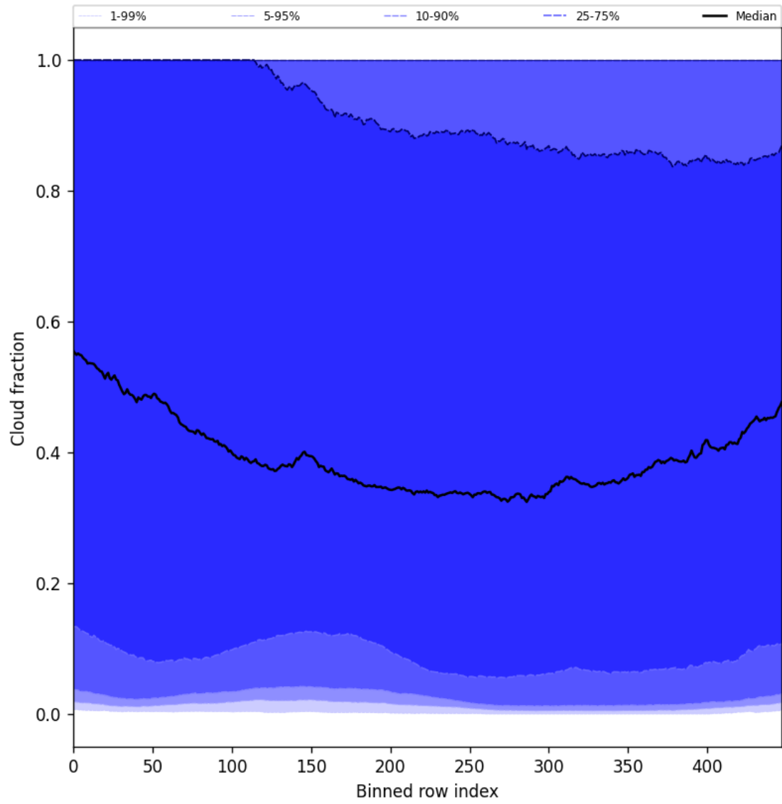
Figure 49: Along track statistics of “Cloud fraction” for 2025-01-21 to 2025-01-23
