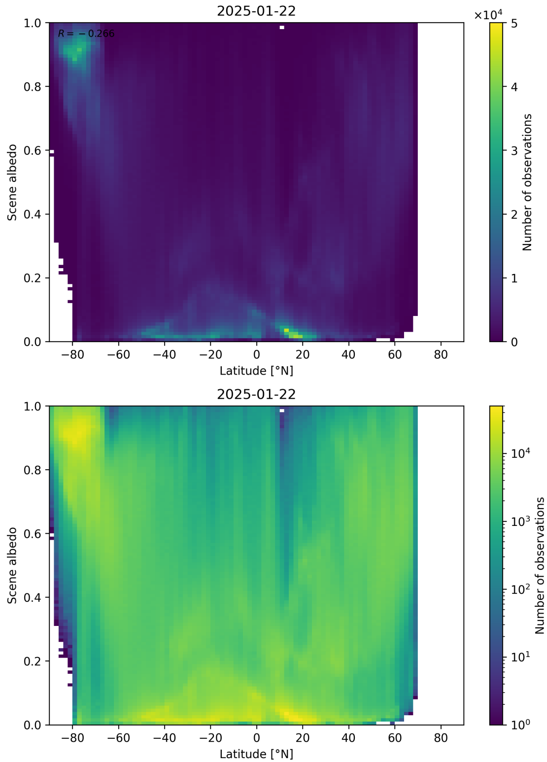
Figure 95: Scatter density plot of “Latitude” against “Scene albedo” for 2025-01-21 to 2025-01-23.
