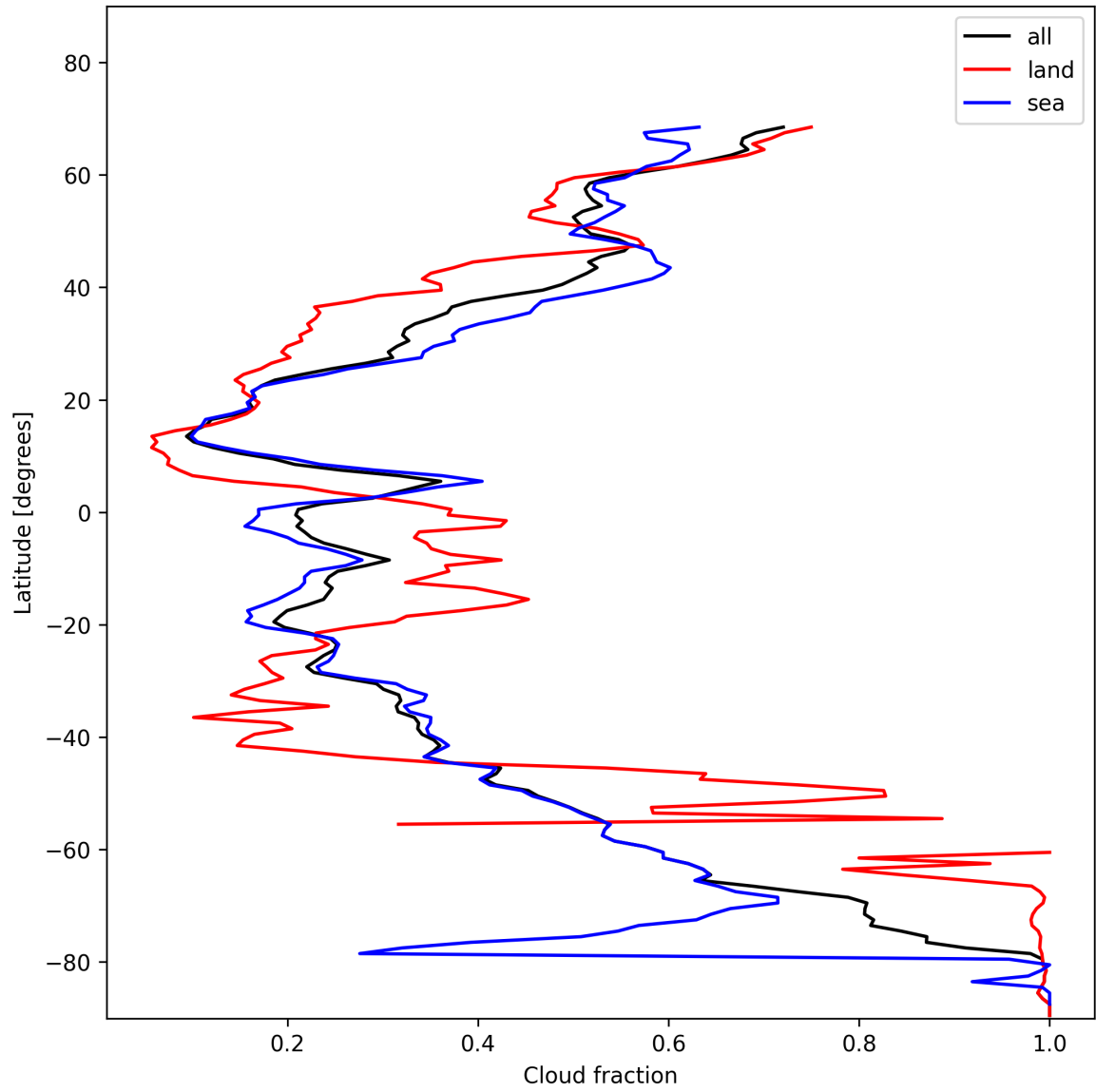
Figure 15: Zonal average of “Cloud fraction” for 2025-01-21 to 2025-01-23.
