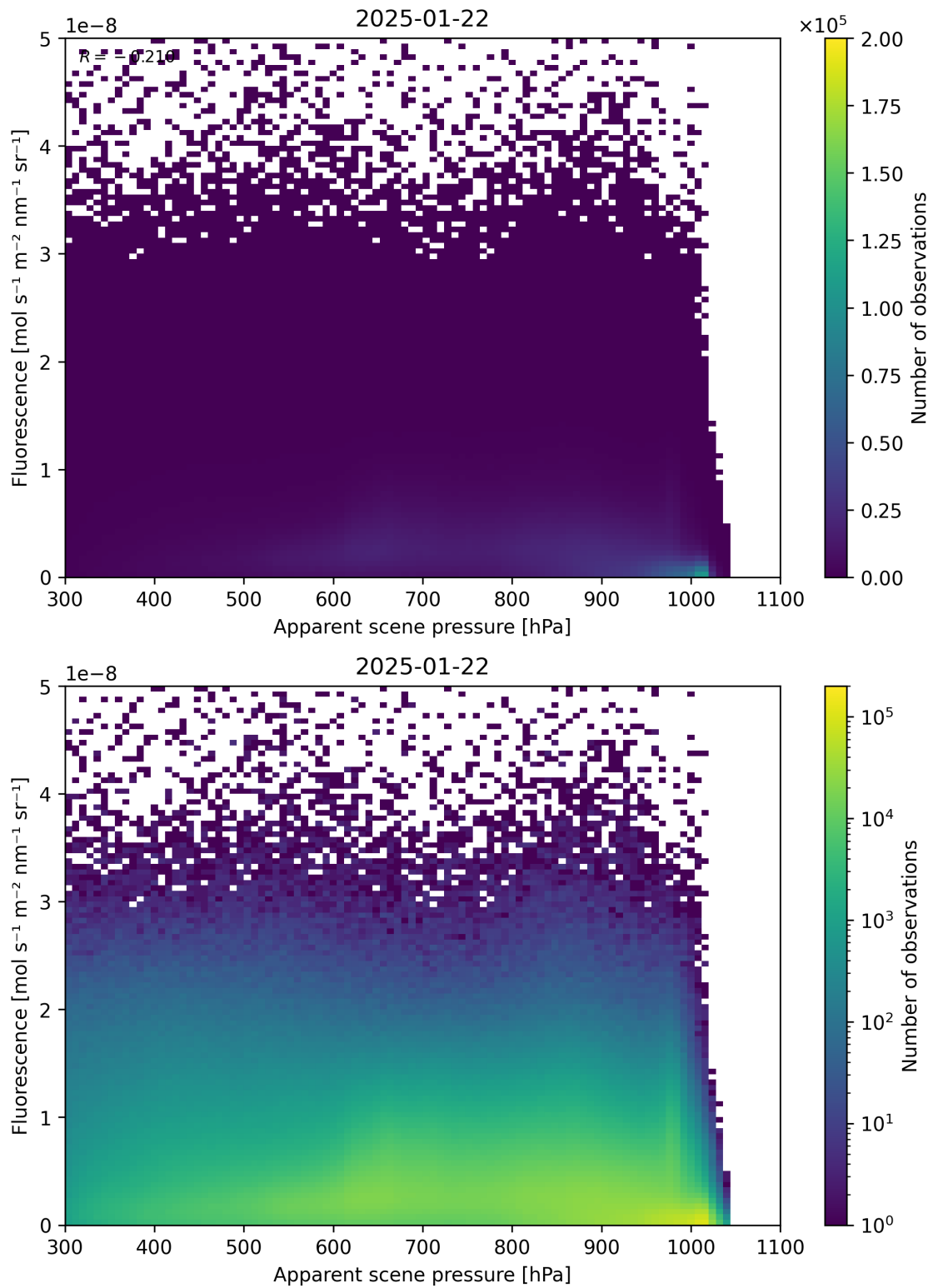
Figure 64: Scatter density plot of “Apparent scene pressure” against “Fluorescence” for 2025-01-21 to 2025-01-23.
