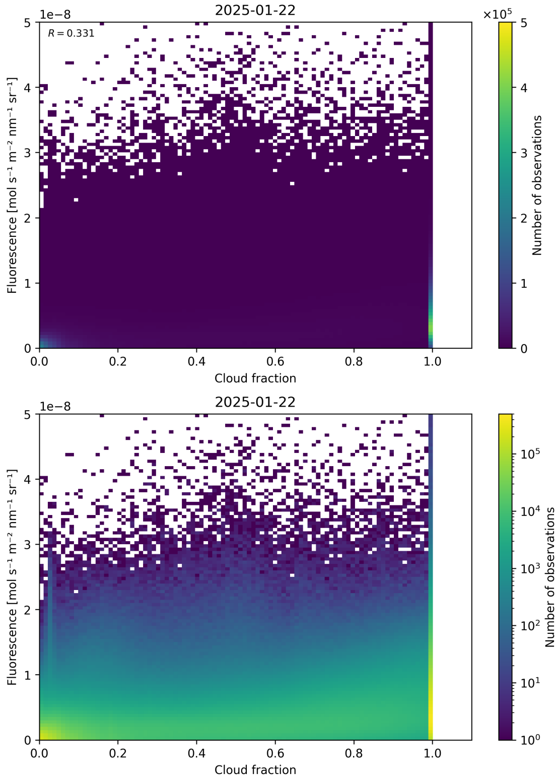
Figure 72: Scatter density plot of “Cloud fraction” against “Fluorescence” for 2025-01-21 to 2025-01-23.
