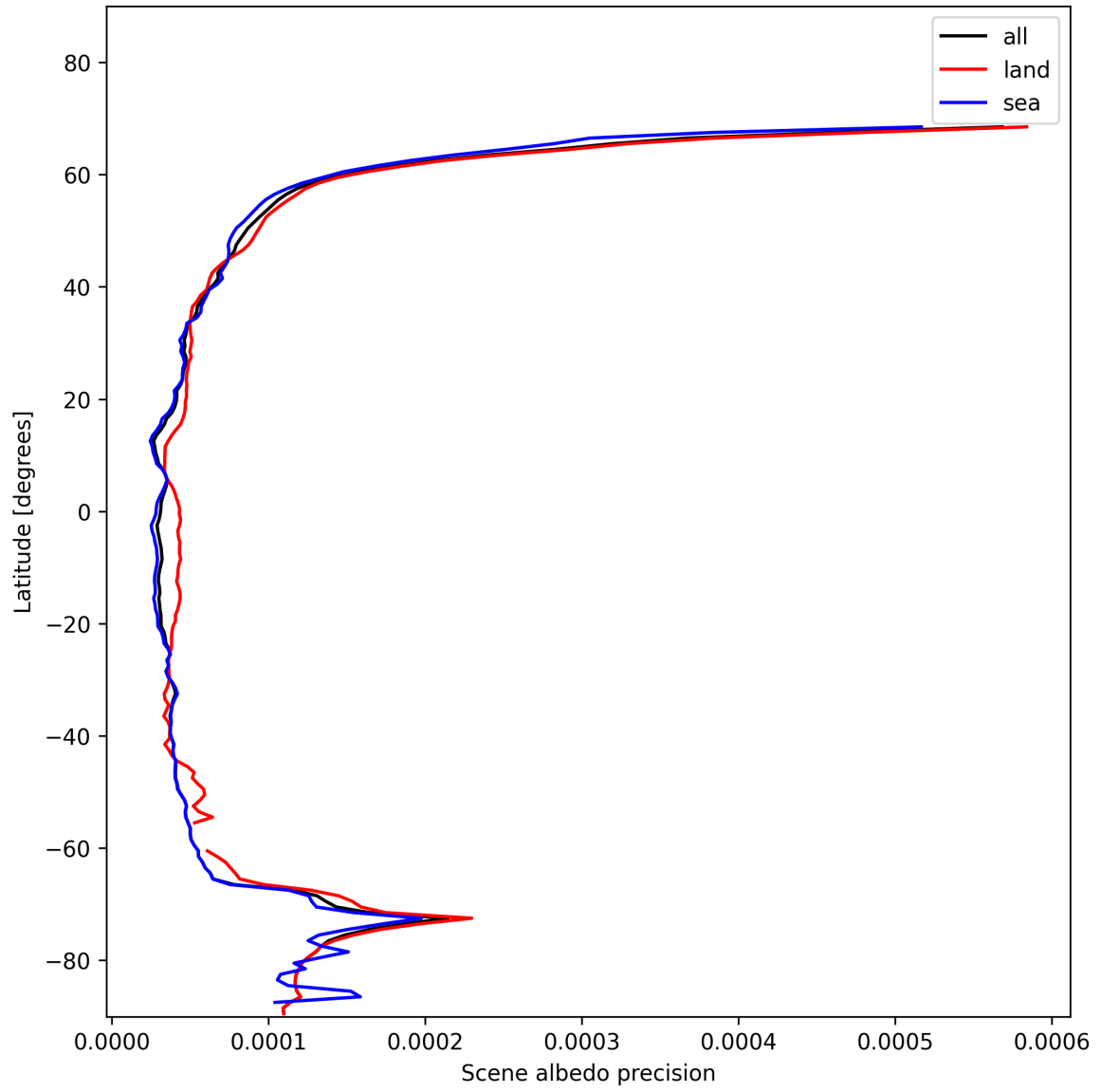
Figure 18: Zonal average of “Scene albedo precision” for 2025-01-21 to 2025-01-23.
