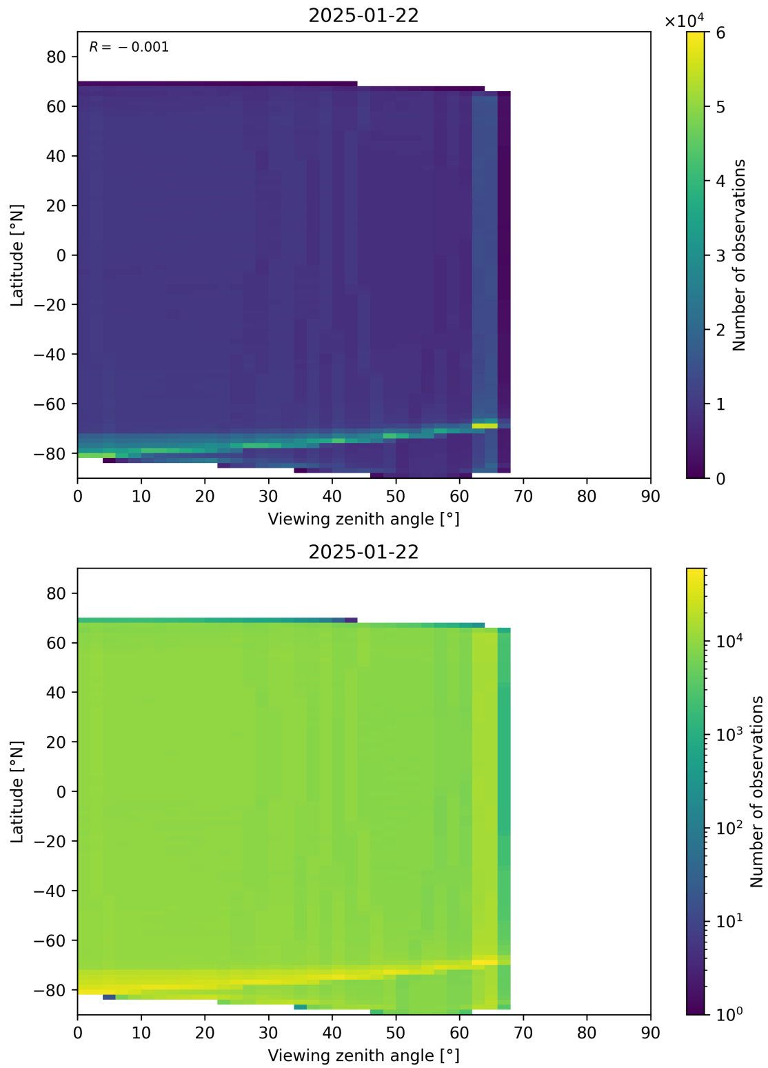
Figure 123: Scatter density plot of “Viewing zenith angle” against “Latitude” for 2025-01-21 to 2025-01-23.
