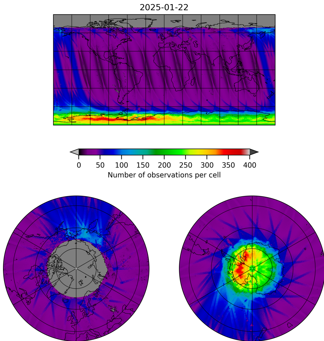
Figure 11: Map of the number of observations for 2025-01-21 to 2025-01-23
