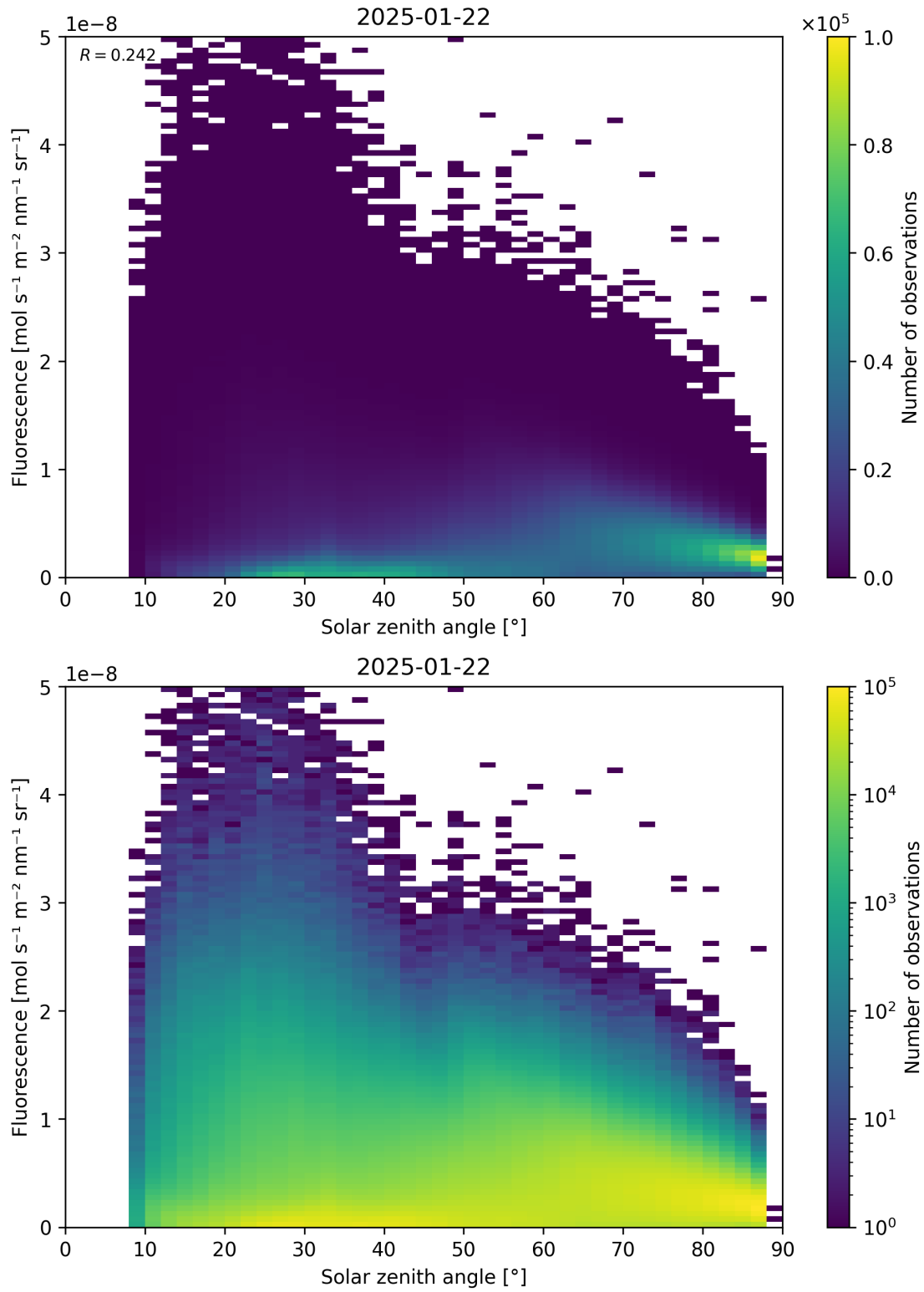
Figure 112: Scatter density plot of “Solar zenith angle” against “Fluorescence” for 2025-01-21 to 2025-01-23.
