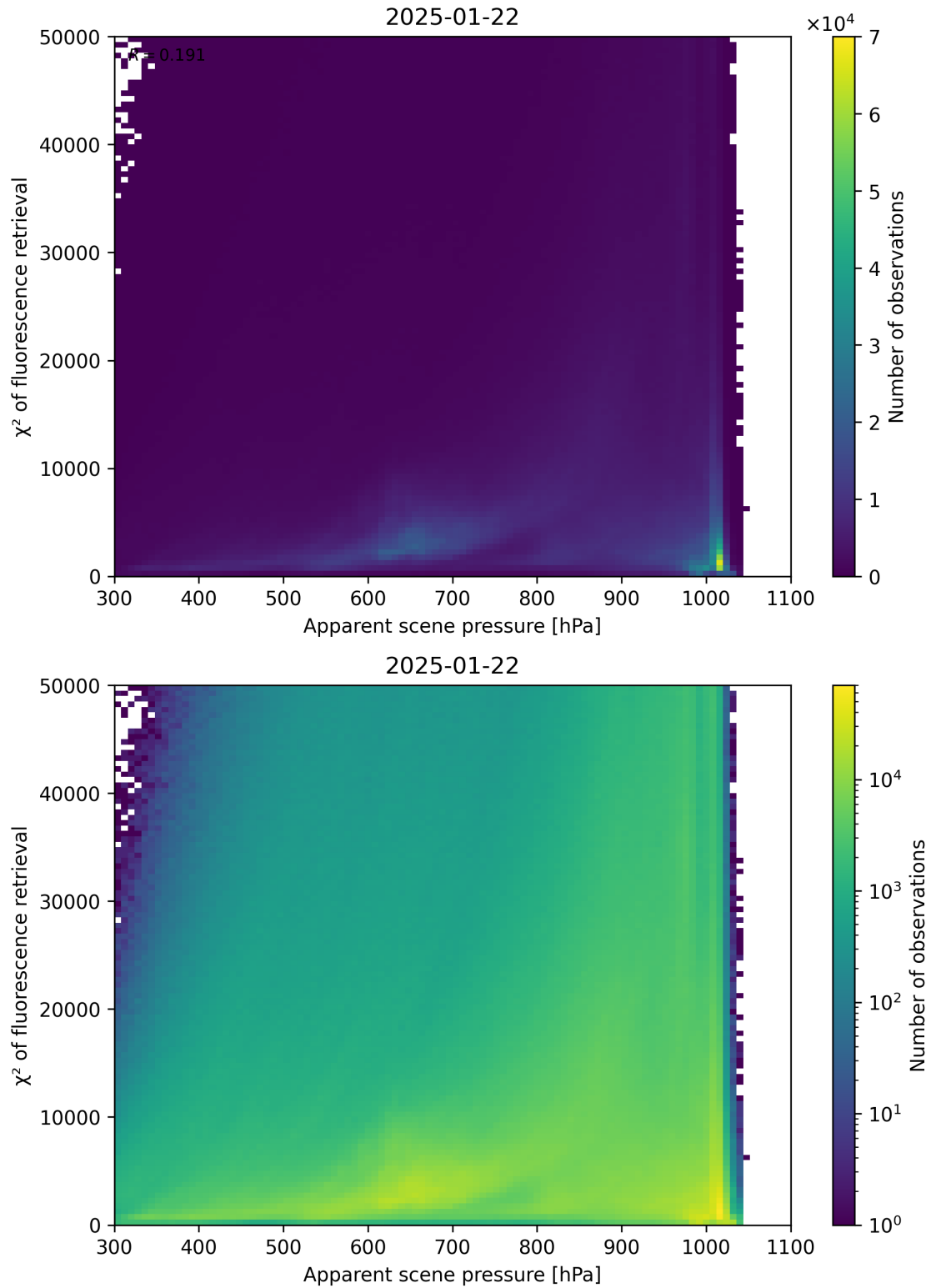
Figure 63: Scatter density plot of “Apparent scene pressure” against “ \chi^2 of fluorescence retrieval” for 2025-01-21 to 2025-01-23.
