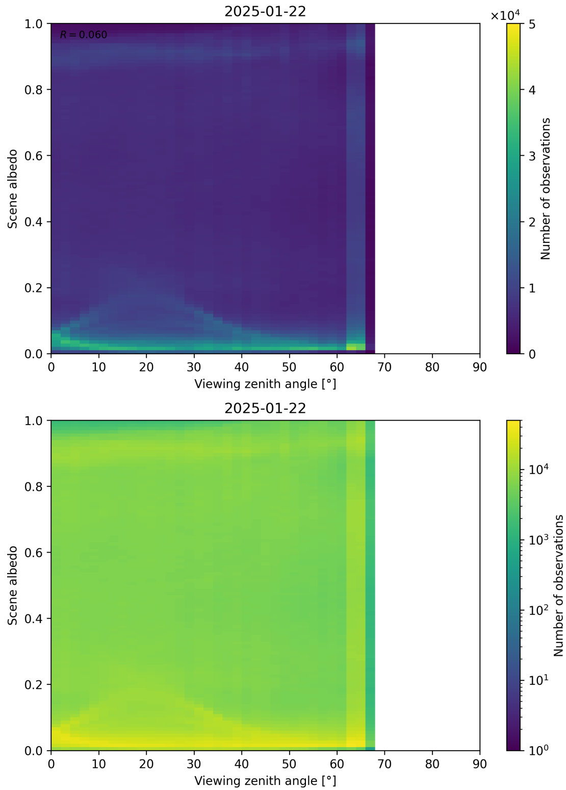
Figure 126: Scatter density plot of “Viewing zenith angle” against “Scene albedo” for 2025-01-21 to 2025-01-23.
