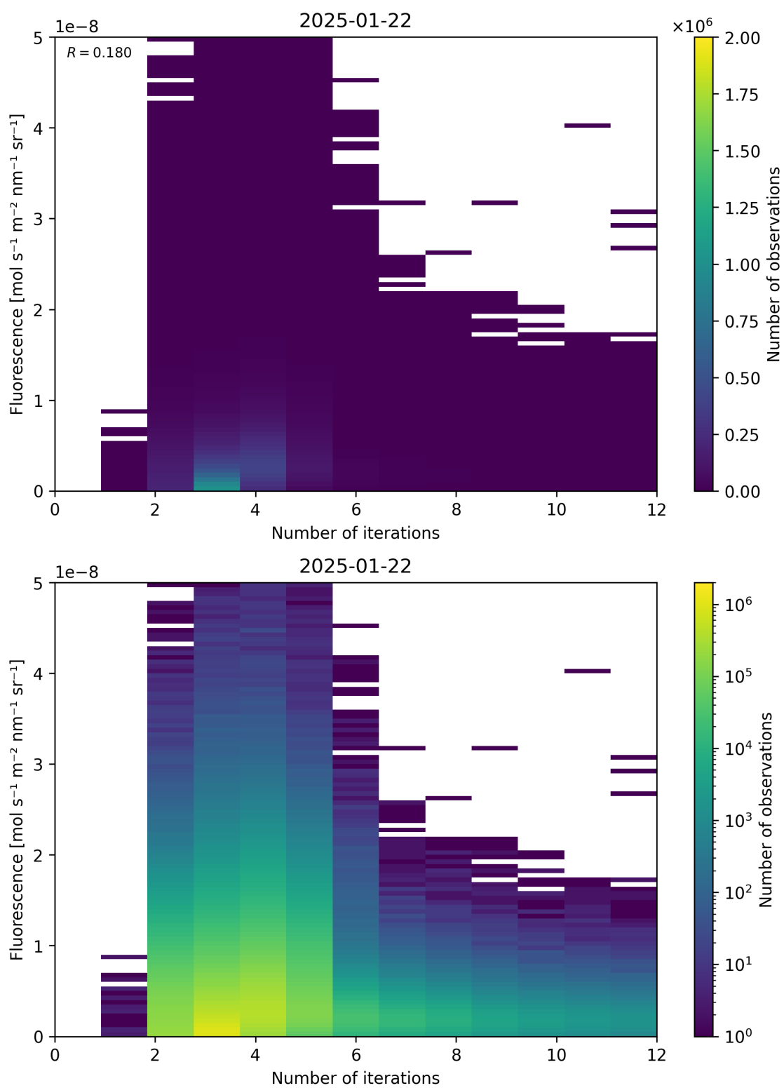
Figure 98: Scatter density plot of “Number of iterations” against “Fluorescence” for 2025-01-21 to 2025-01-23.
