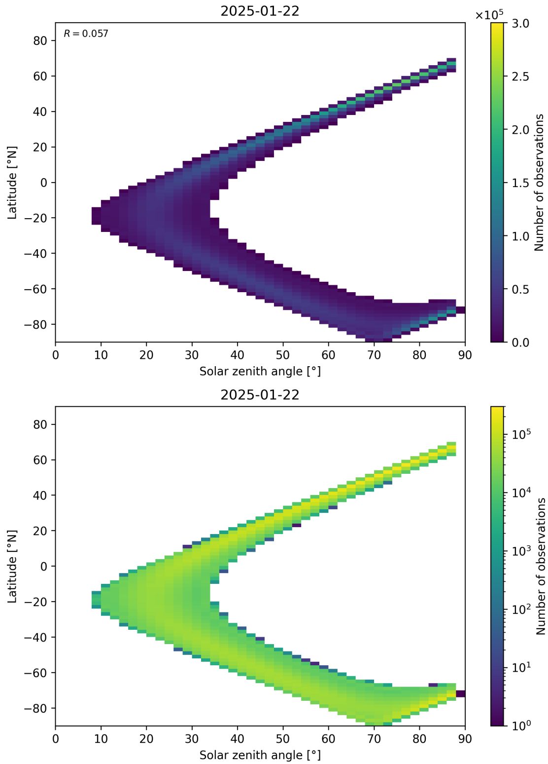
Figure 113: Scatter density plot of “Solar zenith angle” against “Latitude” for 2025-01-21 to 2025-01-23.
