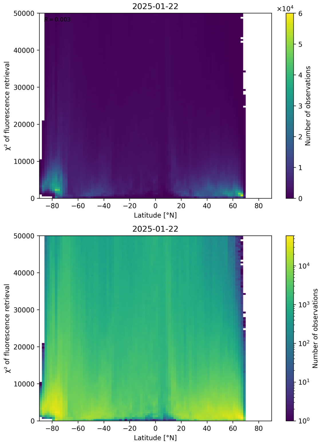
Figure 89: Scatter density plot of “Latitude” against “ \chi^2 of fluorescence retrieval” for 2025-01-21 to 2025-01-23.
