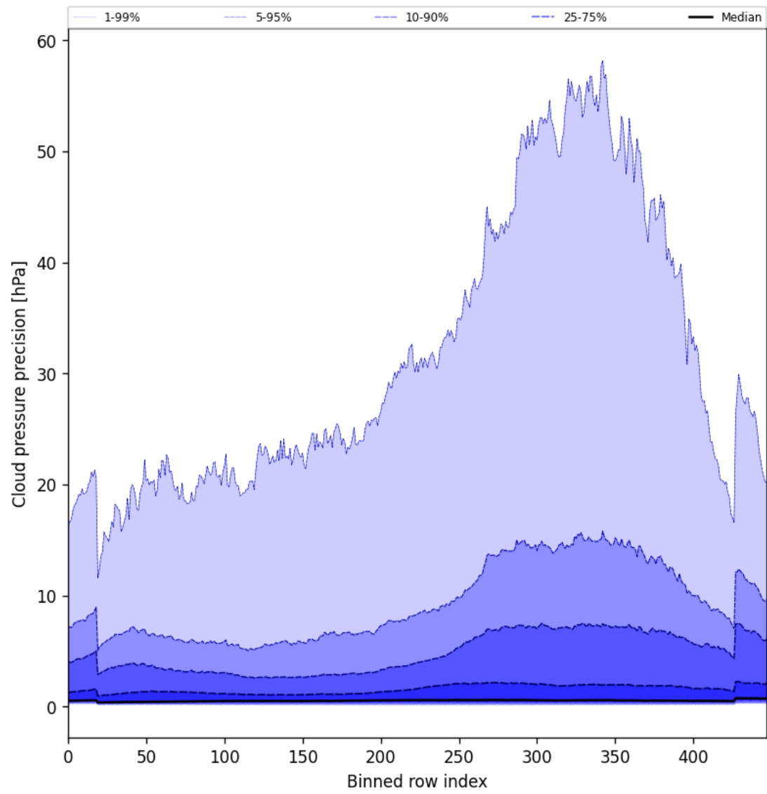
Figure 48: Along track statistics of “Cloud pressure precision” for 2025-01-21 to 2025-01-23
