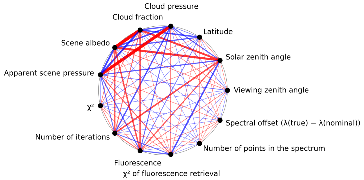
Figure 1: Map of correlation graph for 2025-01-21 to 2025-01-23.
