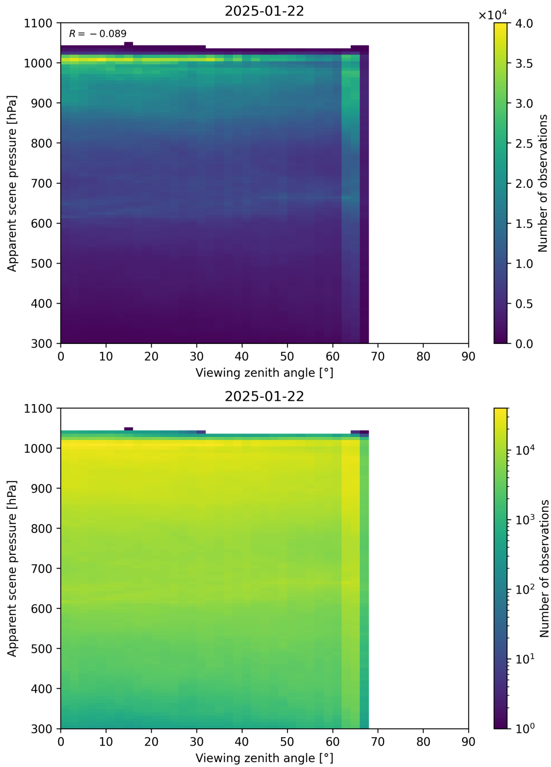
Figure 118: Scatter density plot of “Viewing zenith angle” against “Apparent scene pressure” for 2025-01-21 to 2025-01-23.
