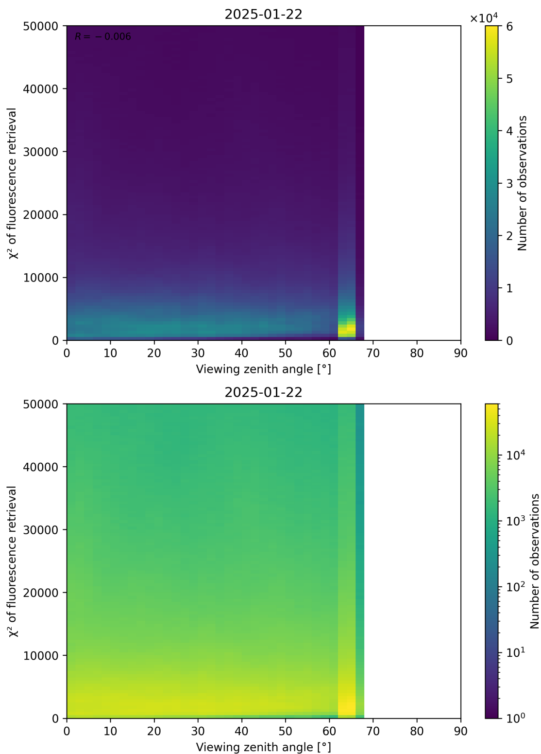
Figure 119: Scatter density plot of “Viewing zenith angle” against “ \chi^2 of fluorescence retrieval” for 2025-01-21 to 2025-01-23.
