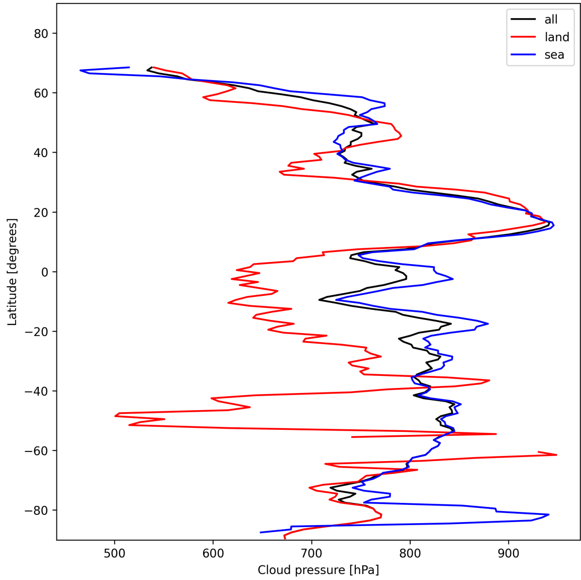
Figure 13: Zonal average of “Cloud pressure” for 2025-01-21 to 2025-01-23.
