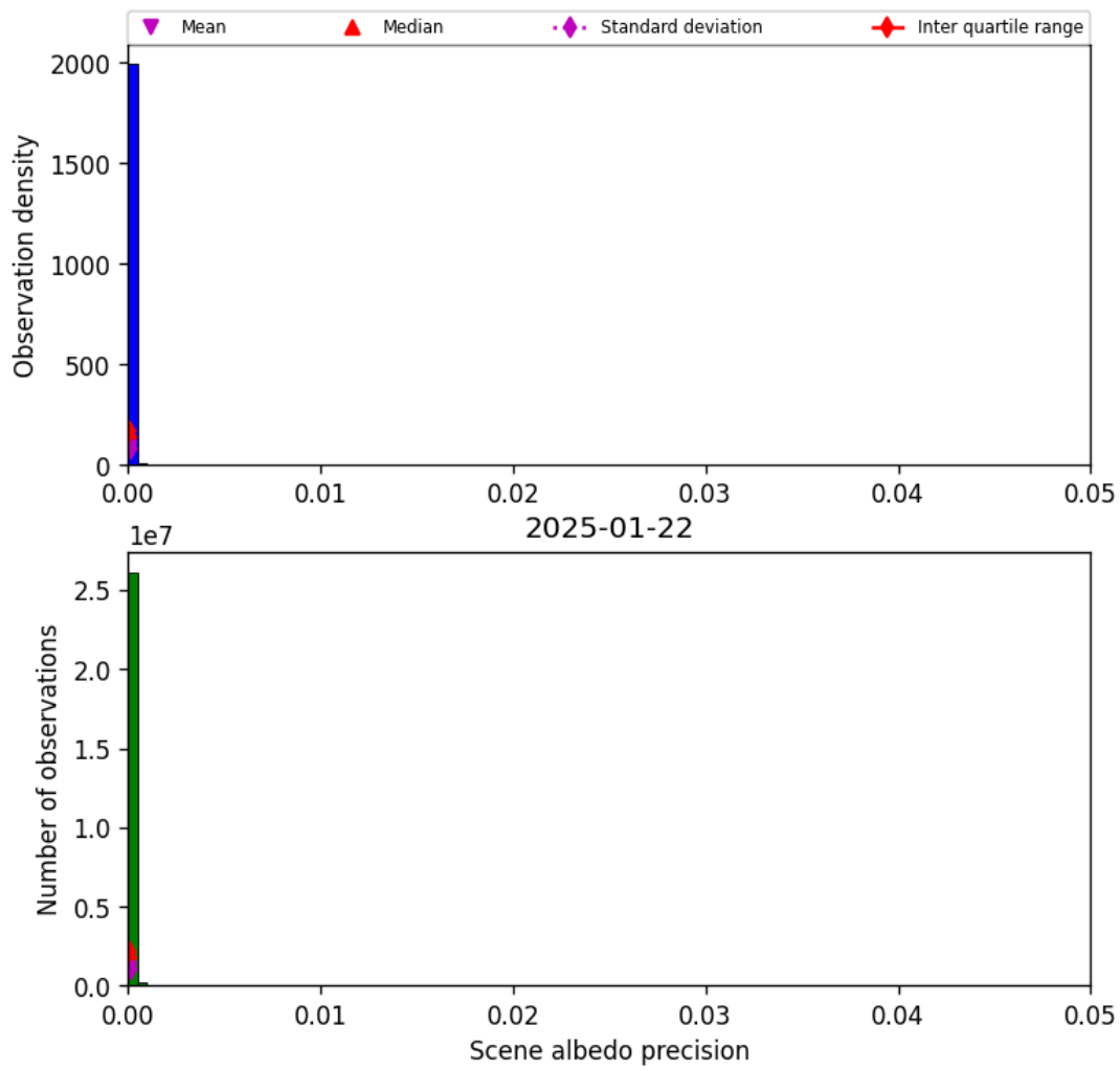
Figure 35: Histogram of “Scene albedo precision” for 2025-01-21 to 2025-01-23
