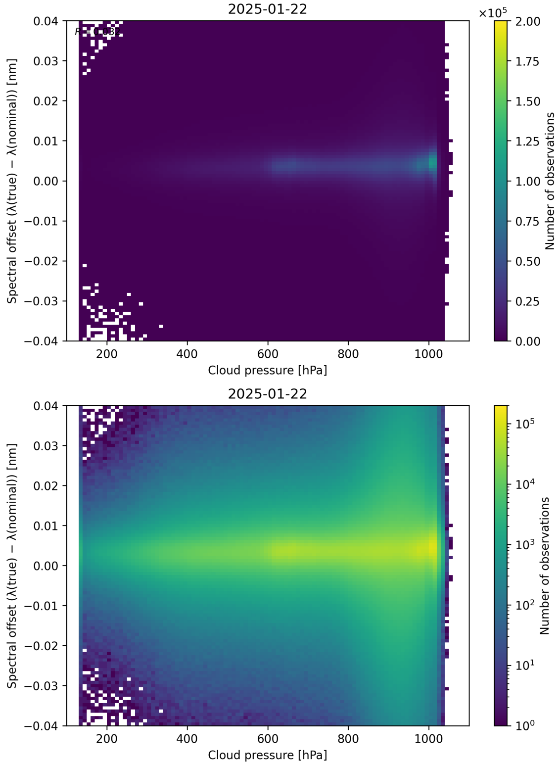
Figure 84: Scatter density plot of “Cloud pressure” against “Spectral offset ( \lambda_{\text{true}} - \lambda_{\text{nominal}} )” for 2025-01-21 to 2025-01-23.
