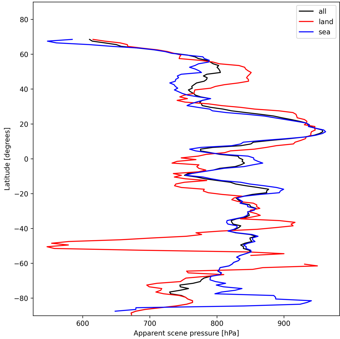
Figure 19: Zonal average of “Apparent scene pressure” for 2025-01-21 to 2025-01-23.
