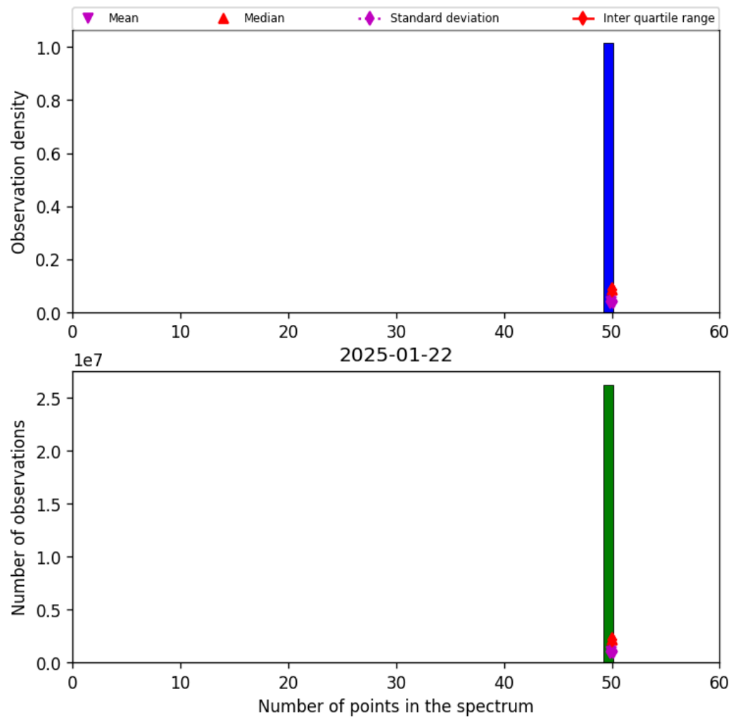
Figure 44: Histogram of “Number of points in the spectrum” for 2025-01-21 to 2025-01-23
