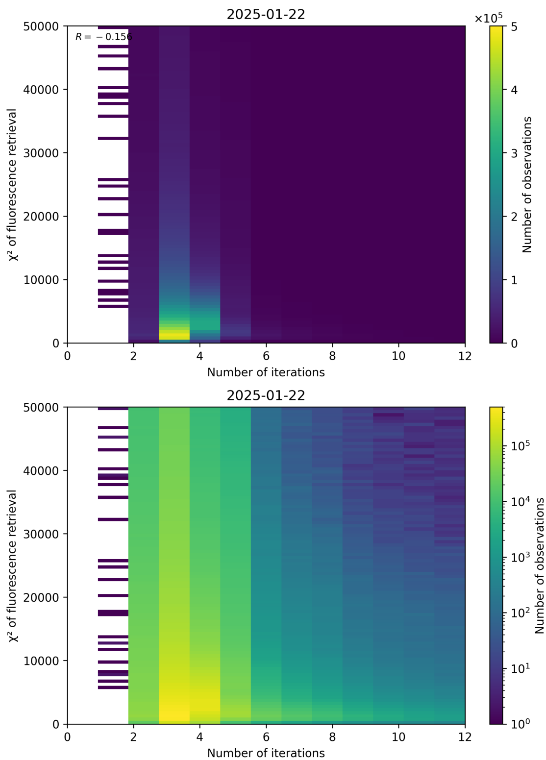
Figure 97: Scatter density plot of “Number of iterations” against “ \chi^2 of fluorescence retrieval” for 2025-01-21 to 2025-01-23.
