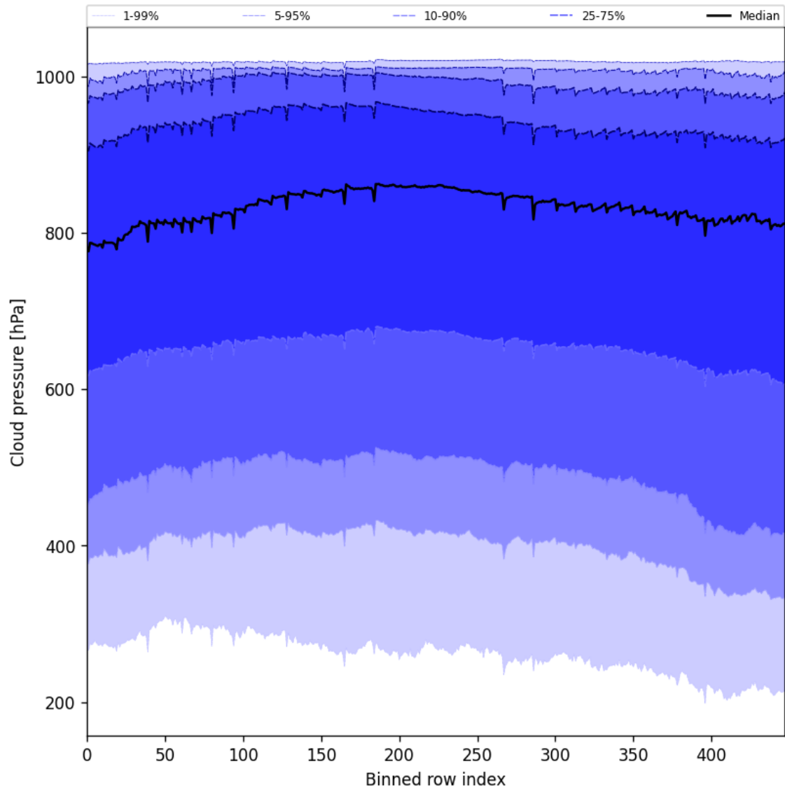
Figure 47: Along track statistics of “Cloud pressure” for 2025-01-21 to 2025-01-23
