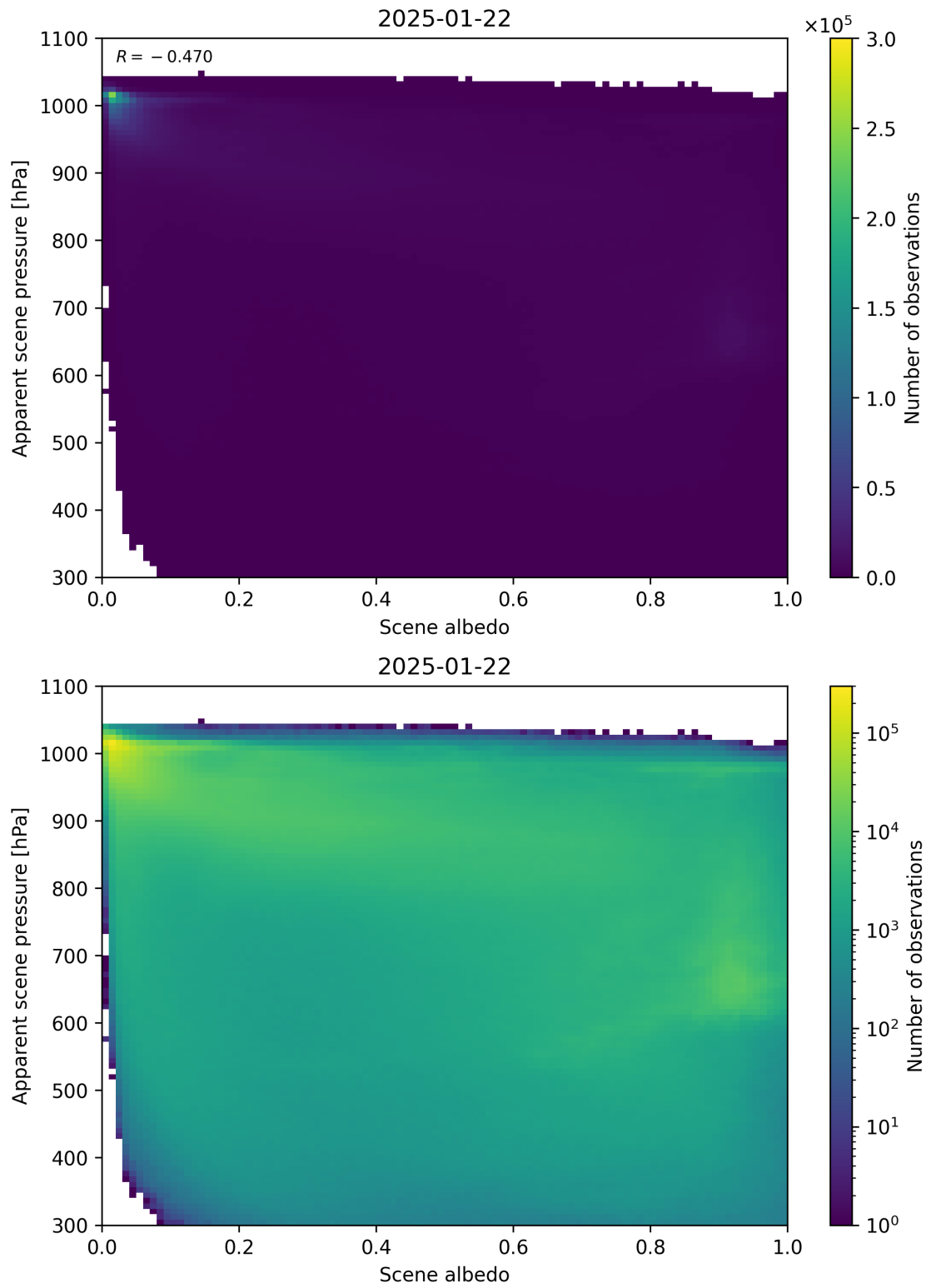
Figure 102: Scatter density plot of “Scene albedo” against “Apparent scene pressure” for 2025-01-21 to 2025-01-23.
