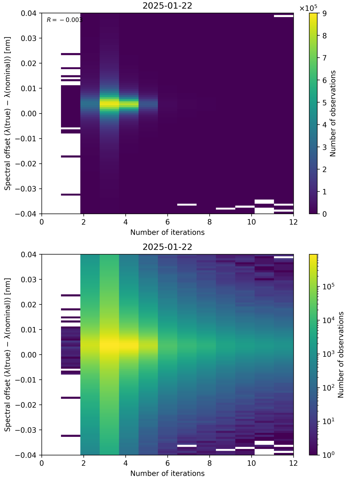
Figure 100: Scatter density plot of “Number of iterations” against “Spectral offset ( \lambda_{\text{true}} - \lambda_{\text{nominal}} )” for 2025-01-21 to 2025-01-23.
