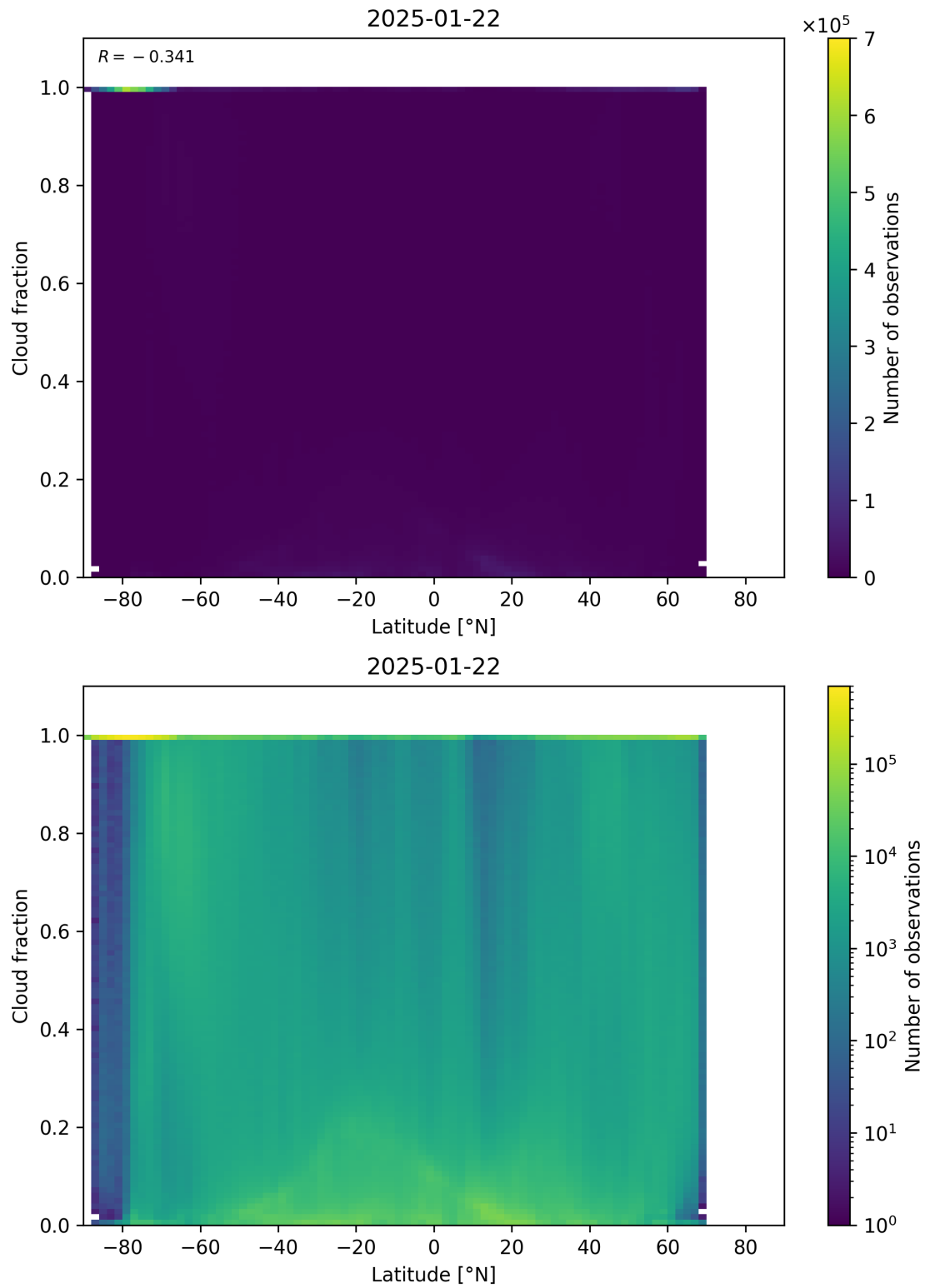
Figure 90: Scatter density plot of “Latitude” against “Cloud fraction” for 2025-01-21 to 2025-01-23.
