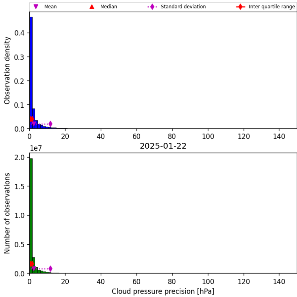
Figure 31: Histogram of “Cloud pressure precision” for 2025-01-21 to 2025-01-23
