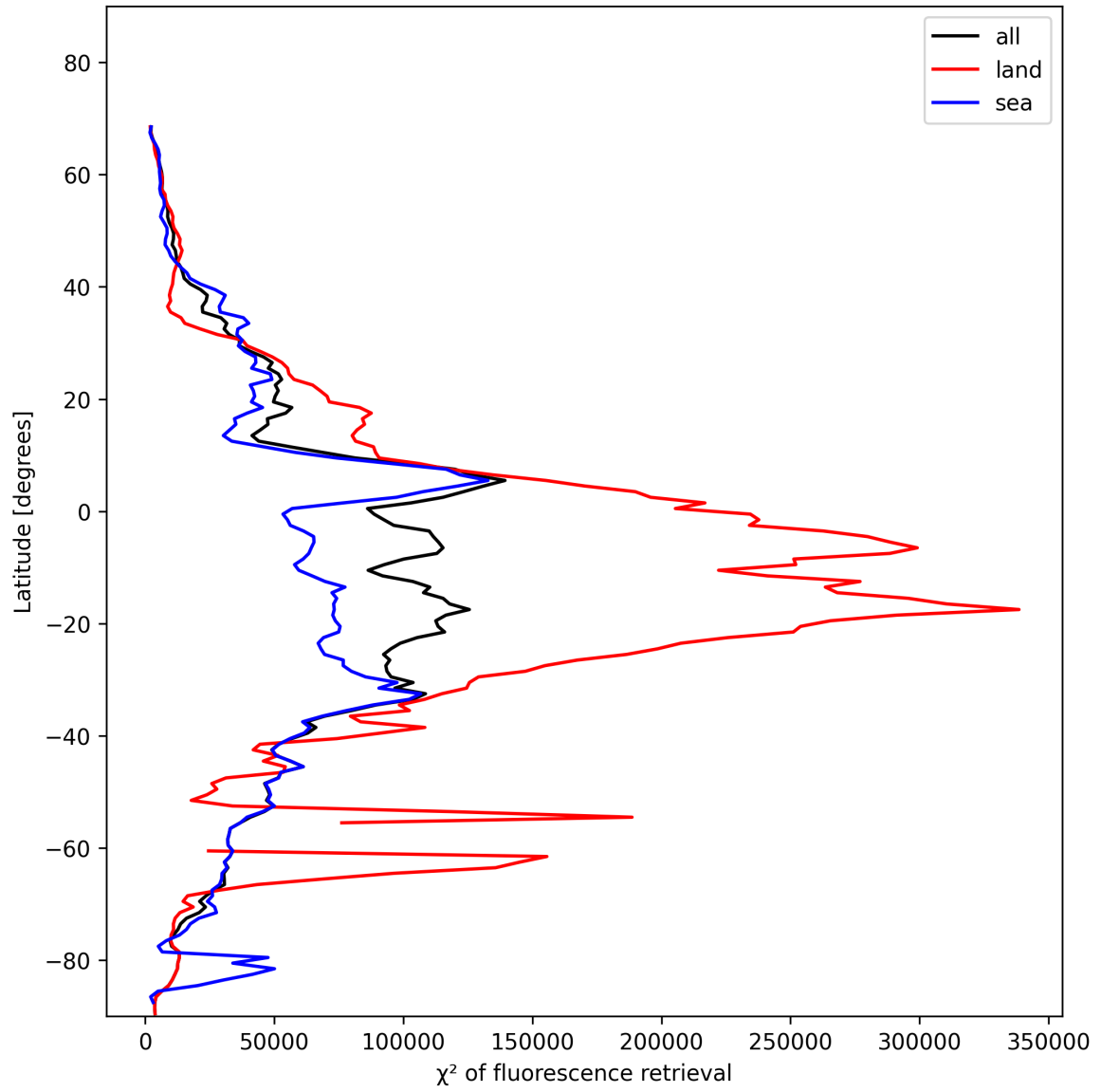
Figure 25: Zonal average of “ \chi^2 of fluorescence retrieval” for 2025-01-21 to 2025-01-23.
