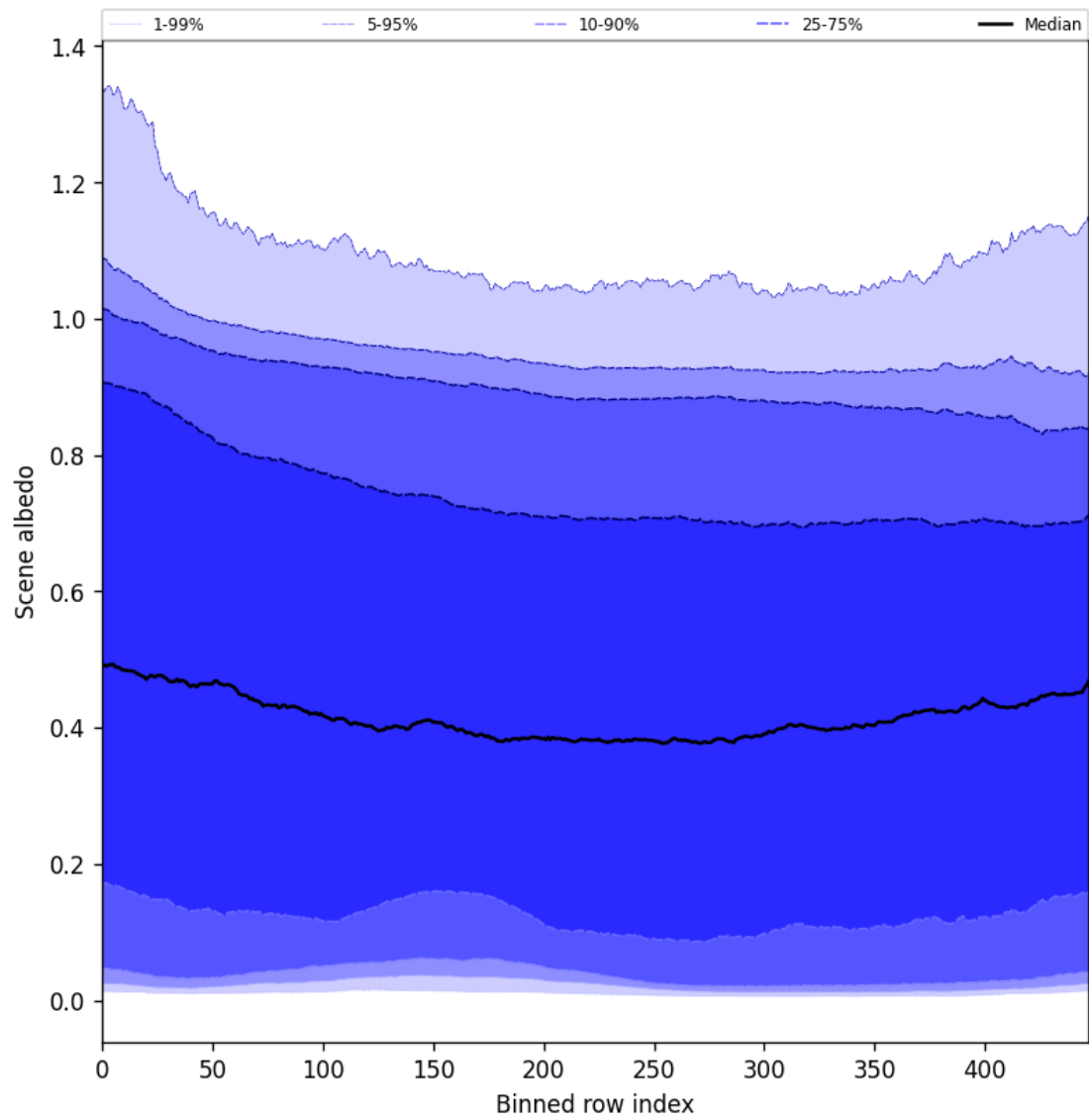
Figure 51: Along track statistics of “Scene albedo” for 2025-01-21 to 2025-01-23
