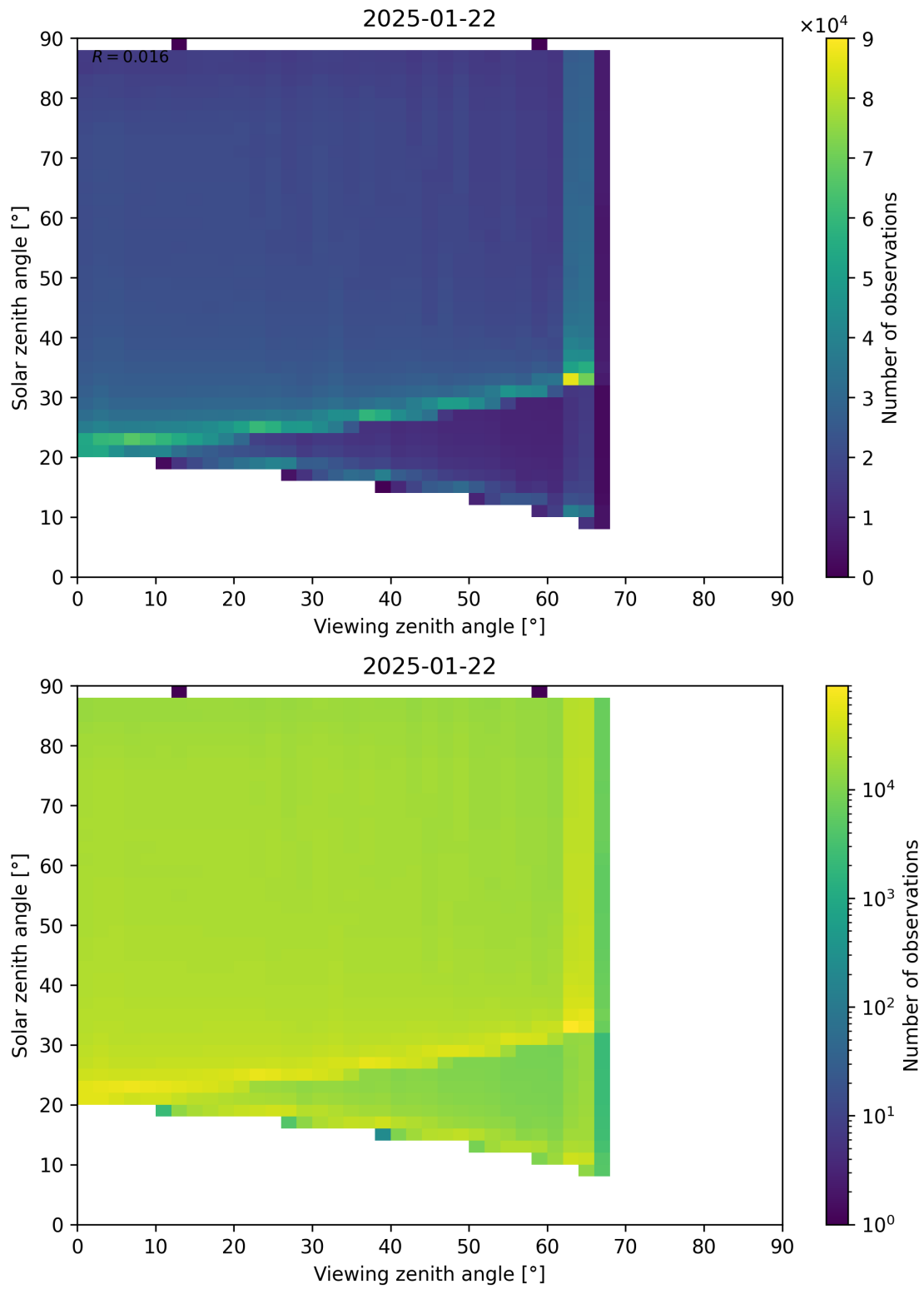
Figure 127: Scatter density plot of “Viewing zenith angle” against “Solar zenith angle” for 2025-01-21 to 2025-01-23.
