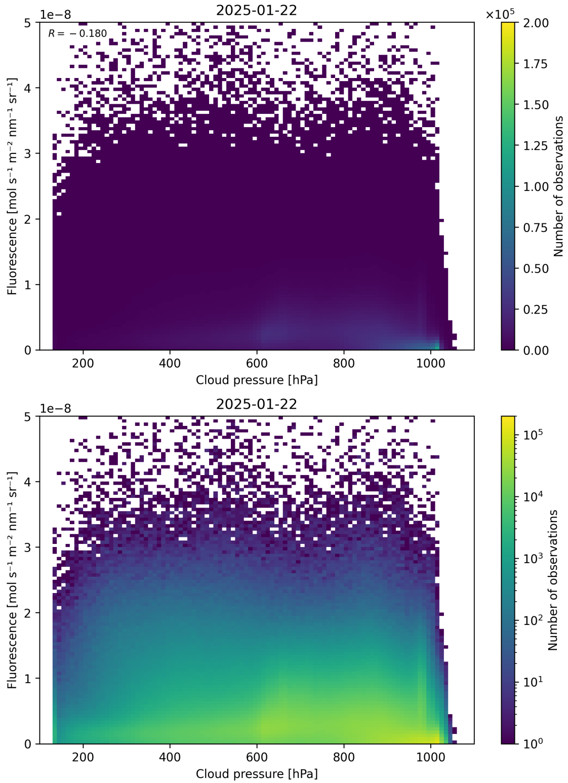
Figure 80: Scatter density plot of “Cloud pressure” against “Fluorescence” for 2025-01-21 to 2025-01-23.
