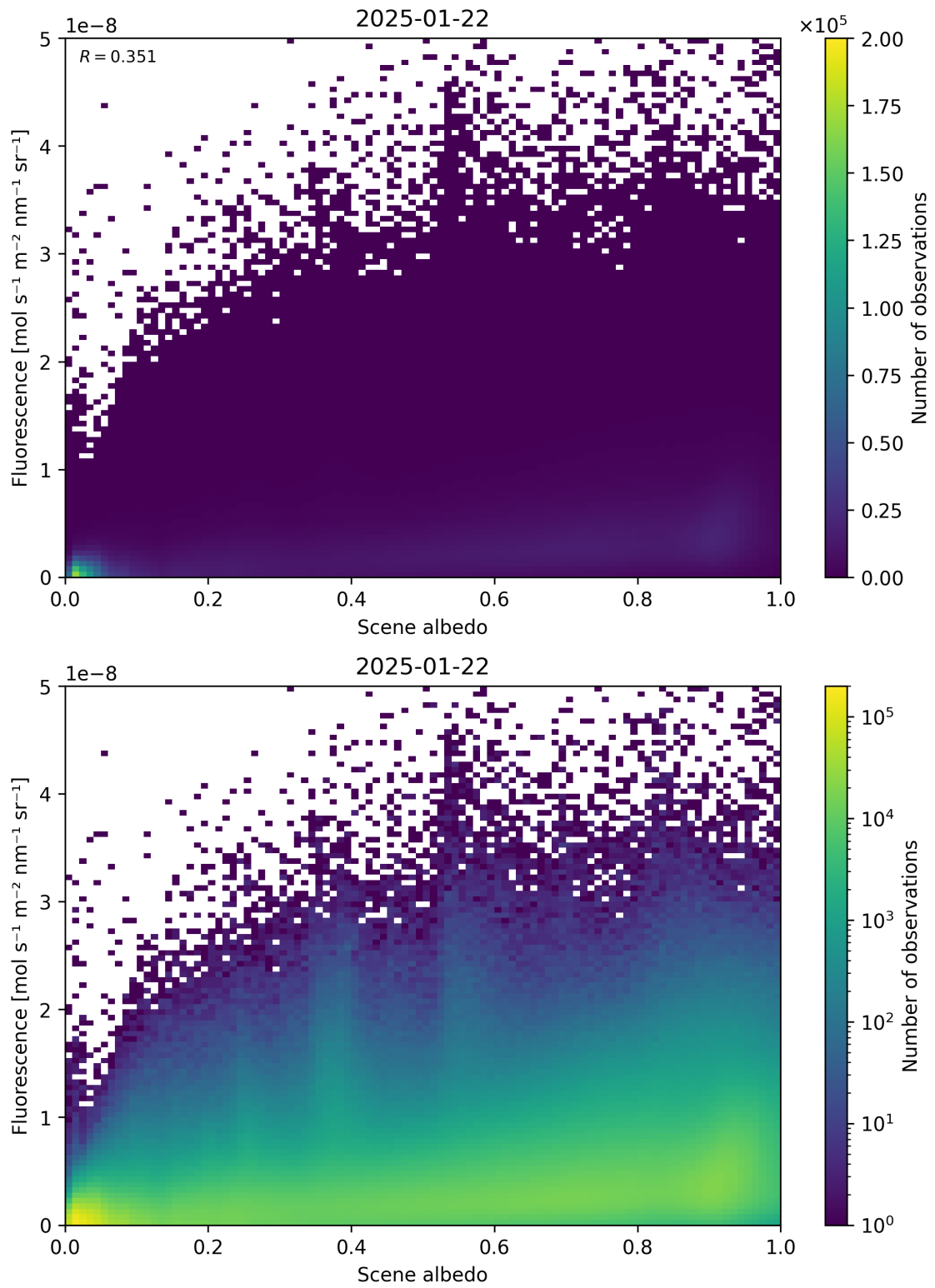
Figure 104: Scatter density plot of “Scene albedo” against “Fluorescence” for 2025-01-21 to 2025-01-23.
