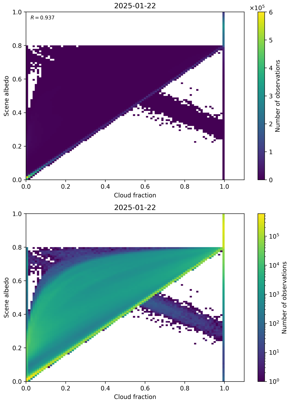
Figure 75: Scatter density plot of “Cloud fraction” against “Scene albedo” for 2025-01-21 to 2025-01-23.
