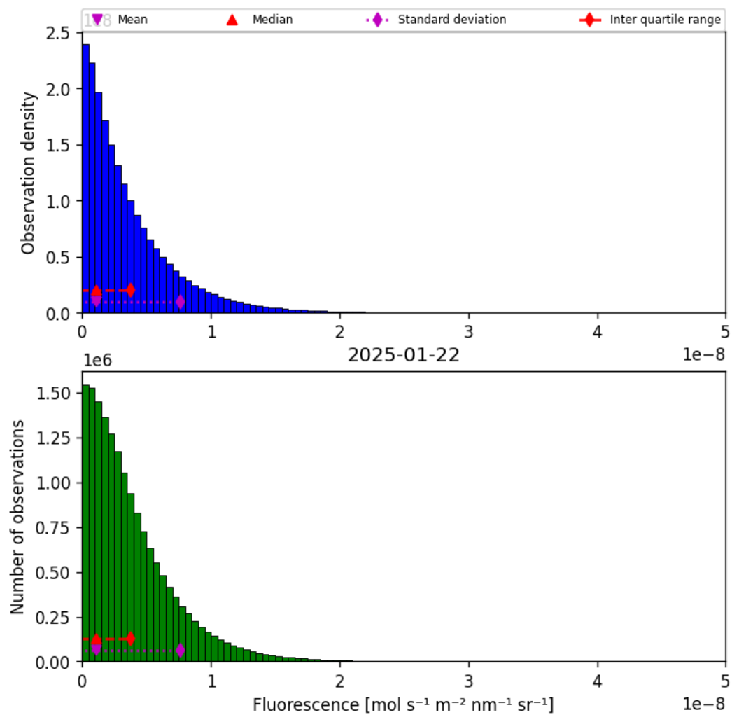
Figure 40: Histogram of “Fluorescence” for 2025-01-21 to 2025-01-23
