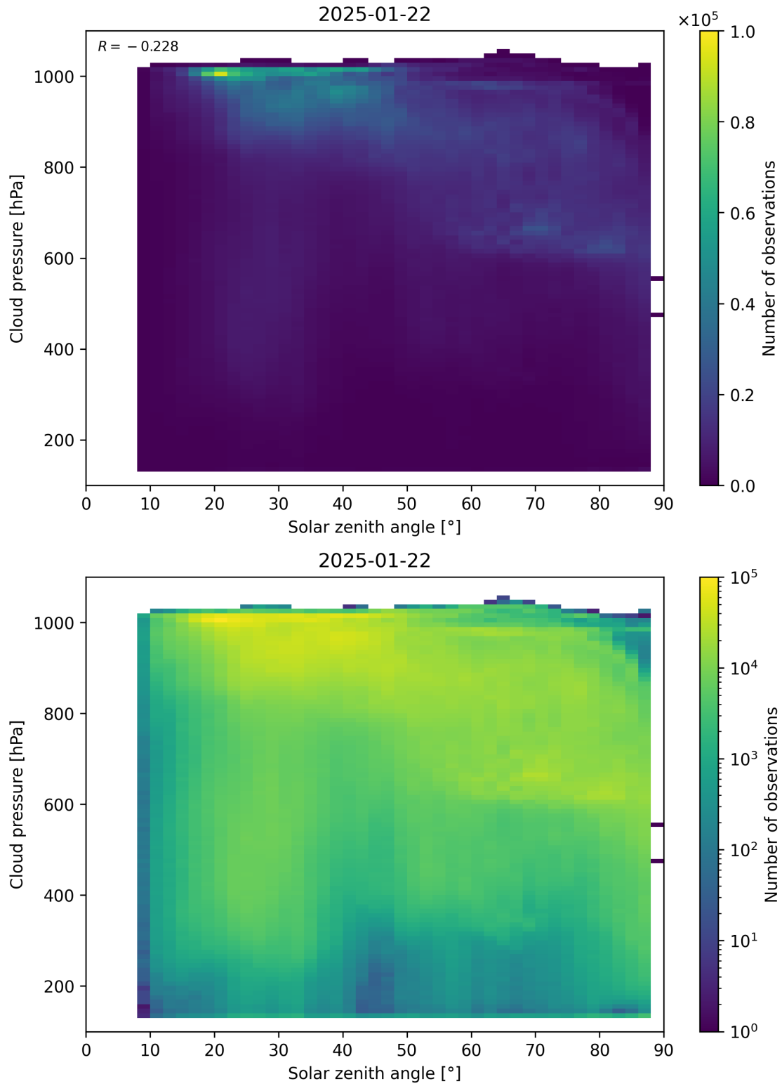
Figure 111: Scatter density plot of “Solar zenith angle” against “Cloud pressure” for 2025-01-21 to 2025-01-23.
