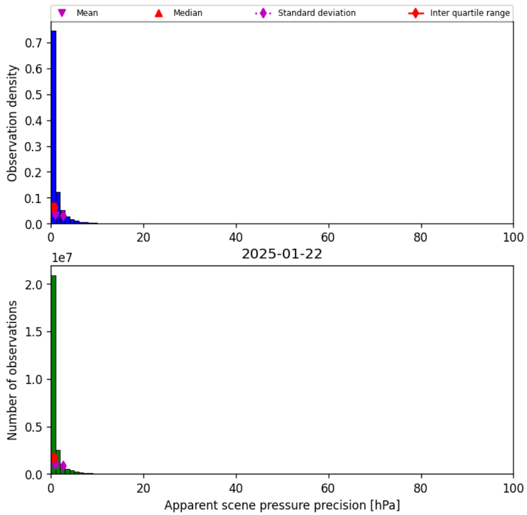
Figure 37: Histogram of “Apparent scene pressure precision” for 2025-01-21 to 2025-01-23
