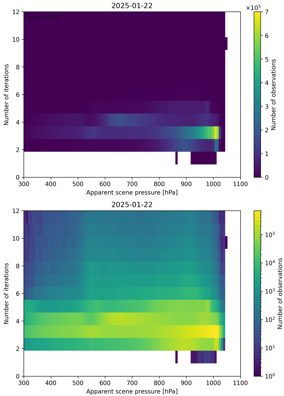
Figure 65: Scatter density plot of “Apparent scene pressure” against “Number of iterations” for 2025-01-21 to 2025-01-23.
