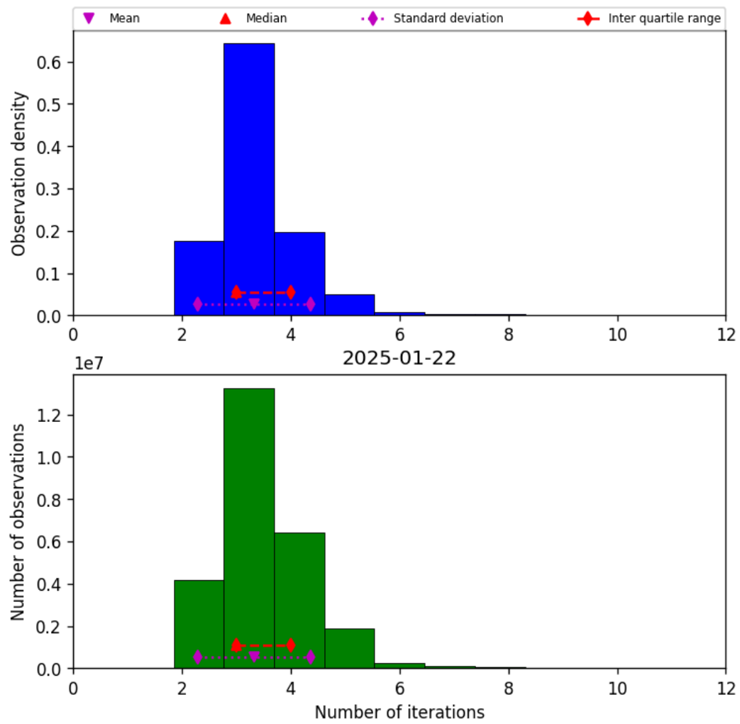
Figure 39: Histogram of “Number of iterations” for 2025-01-21 to 2025-01-23
