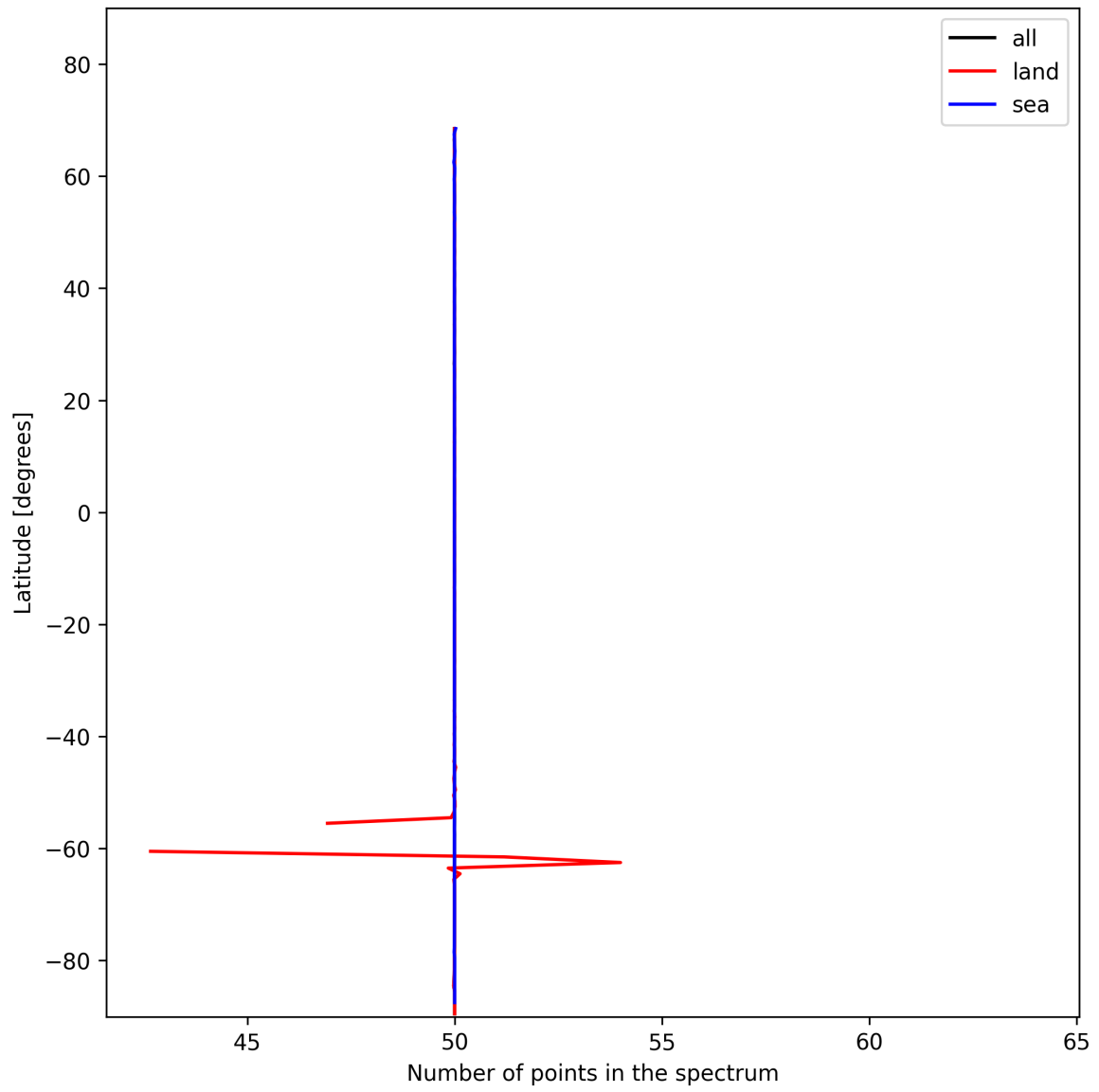
Figure 27: Zonal average of “Number of points in the spectrum” for 2025-01-21 to 2025-01-23.
