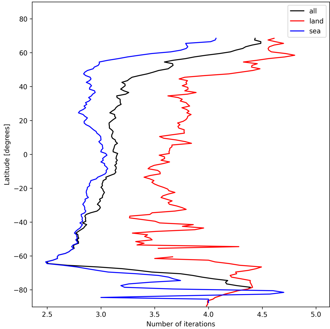
Figure 22: Zonal average of “Number of iterations” for 2025-01-21 to 2025-01-23.
