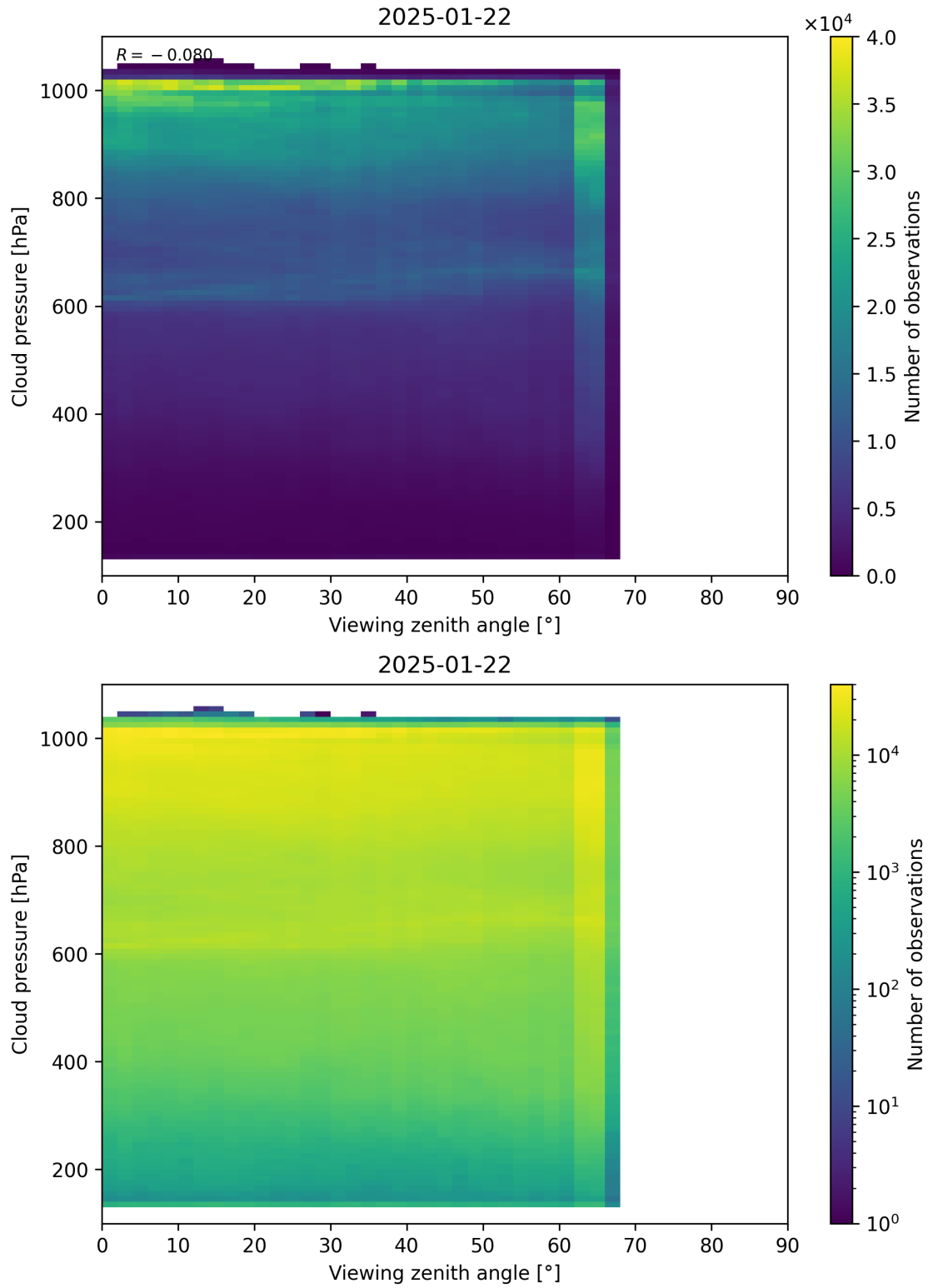
Figure 121: Scatter density plot of “Viewing zenith angle” against “Cloud pressure” for 2025-01-21 to 2025-01-23.
