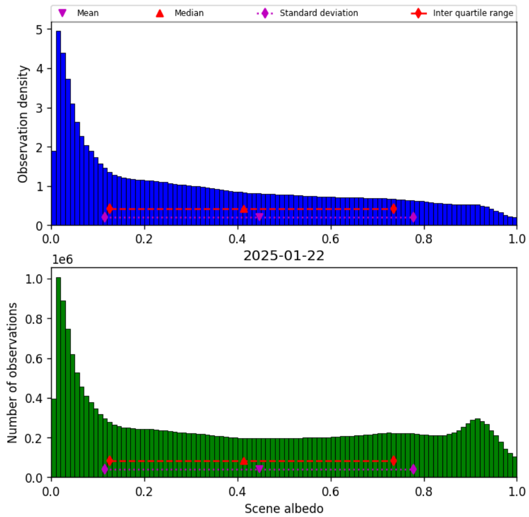
Figure 34: Histogram of “Scene albedo” for 2025-01-21 to 2025-01-23
