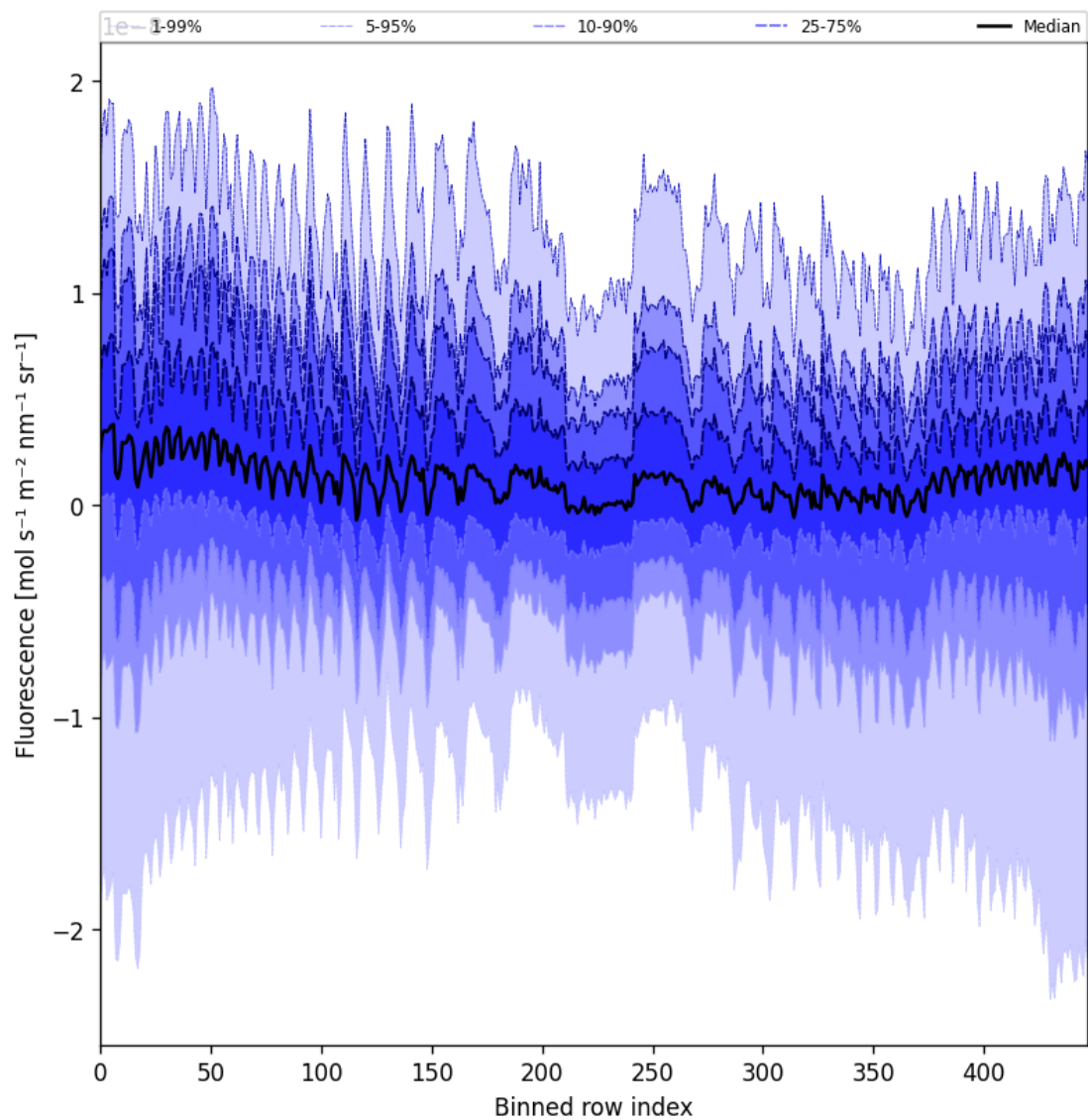
Figure 57: Along track statistics of “Fluorescence” for 2025-01-21 to 2025-01-23
