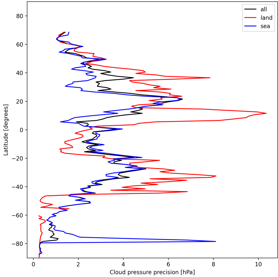
Figure 14: Zonal average of “Cloud pressure precision” for 2025-01-21 to 2025-01-23.
