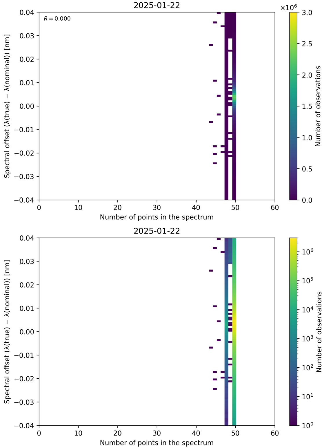
Figure 101: Scatter density plot of “Number of points in the spectrum” against “Spectral offset ( \lambda_{\text{true}} - \lambda_{\text{nominal}} )” for 2025-01-21 to 2025-01-23.
