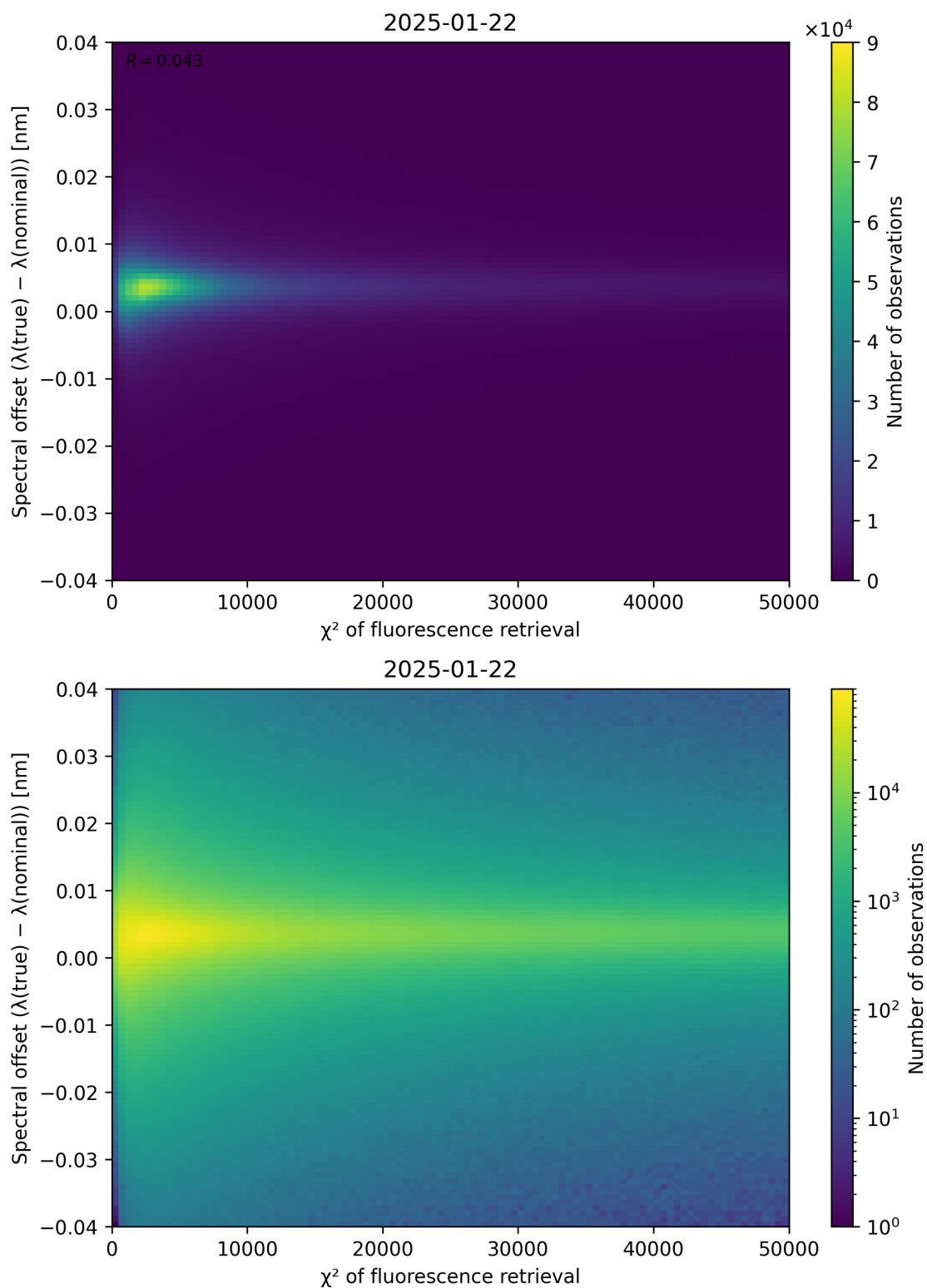
Figure 69: Scatter density plot of “ \chi^2 of fluorescence retrieval” against “Spectral offset ( \lambda_{\text{true}} - \lambda_{\text{nominal}} )” for 2025-01-21 to 2025-01-23.
