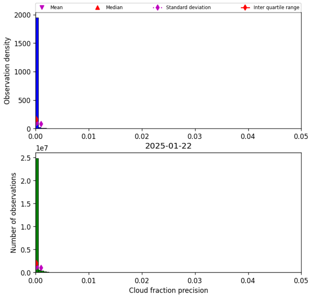
Figure 33: Histogram of “Cloud fraction precision” for 2025-01-21 to 2025-01-23
