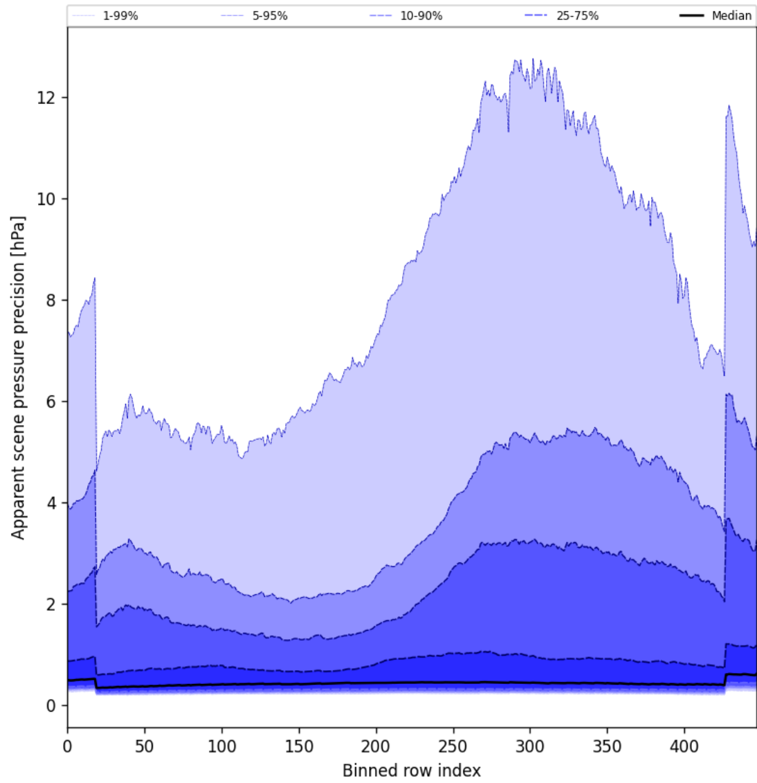
Figure 54: Along track statistics of “Apparent scene pressure precision” for 2025-01-21 to 2025-01-23
