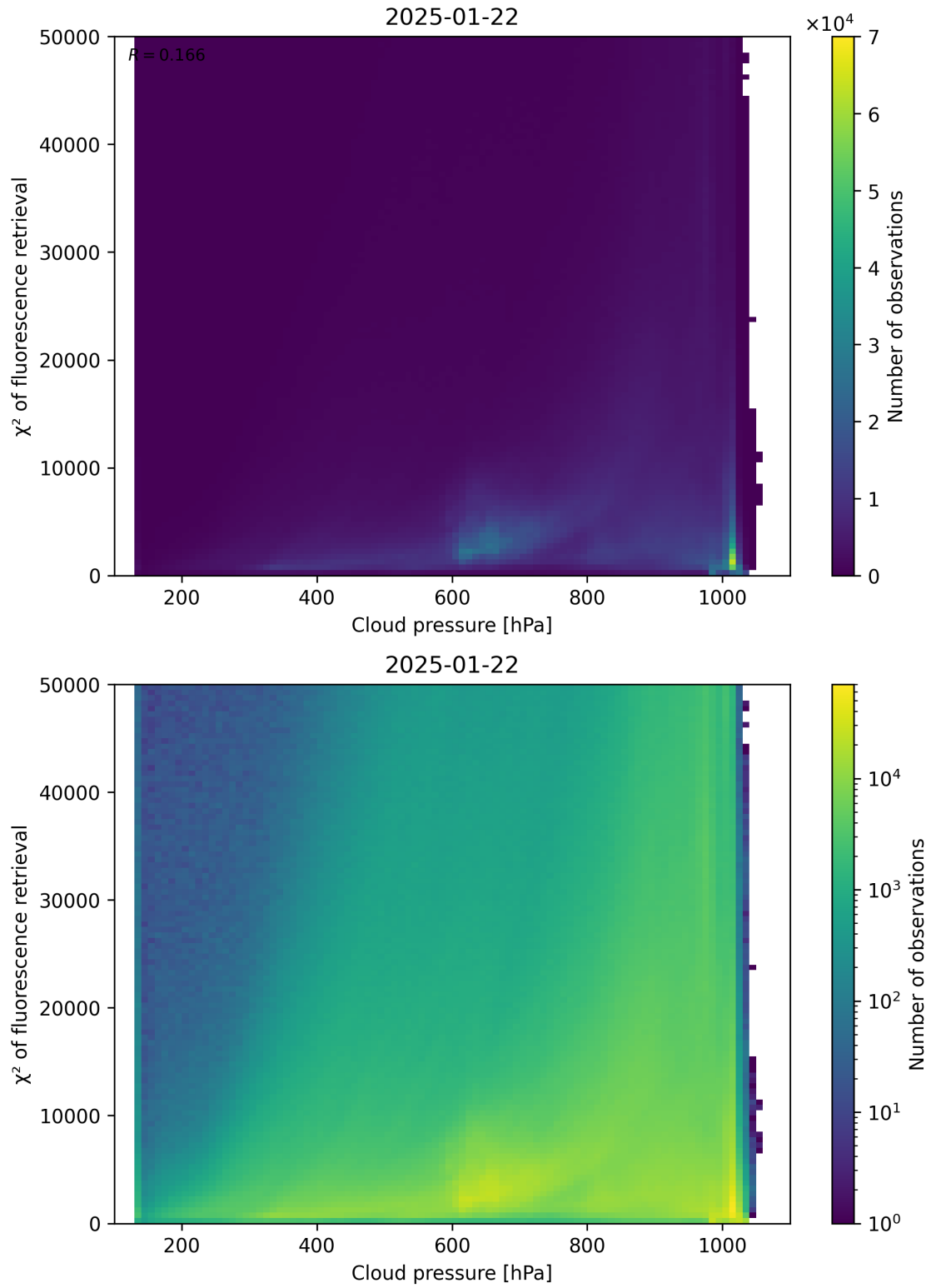
Figure 78: Scatter density plot of “Cloud pressure” against “ \chi^2 of fluorescence retrieval” for 2025-01-21 to 2025-01-23.
