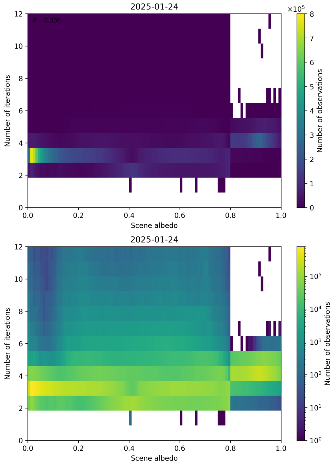
Figure 105: Scatter density plot of “Scene albedo” against “Number of iterations” for 2025-01-23 to 2025-01-25.
