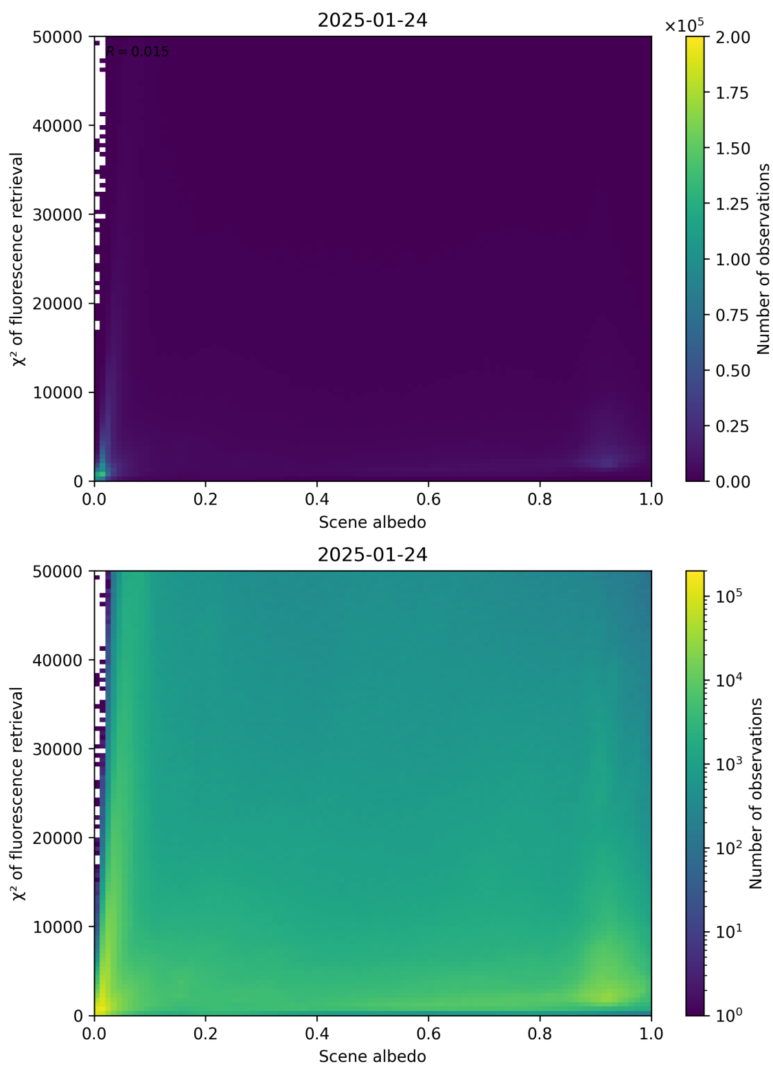
Figure 103: Scatter density plot of “Scene albedo” against “ \chi^2 of fluorescence retrieval” for 2025-01-23 to 2025-01-25.
