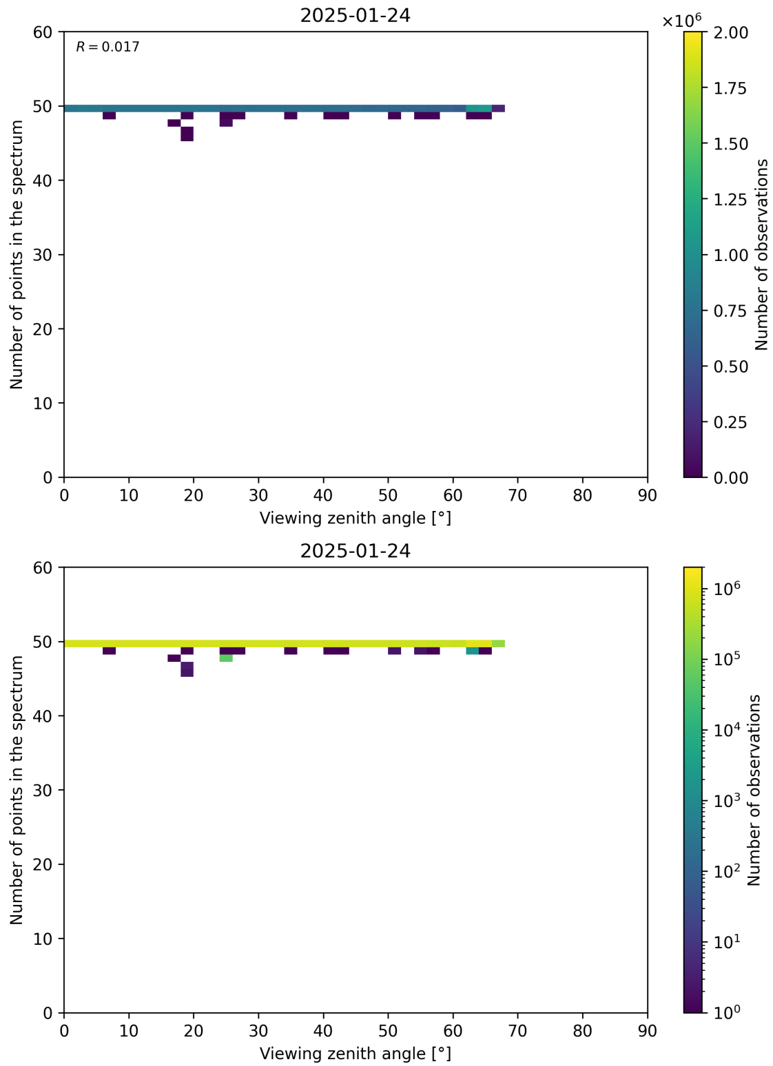
Figure 125: Scatter density plot of “Viewing zenith angle” against “Number of points in the spectrum” for 2025-01-23 to 2025-01-25.
