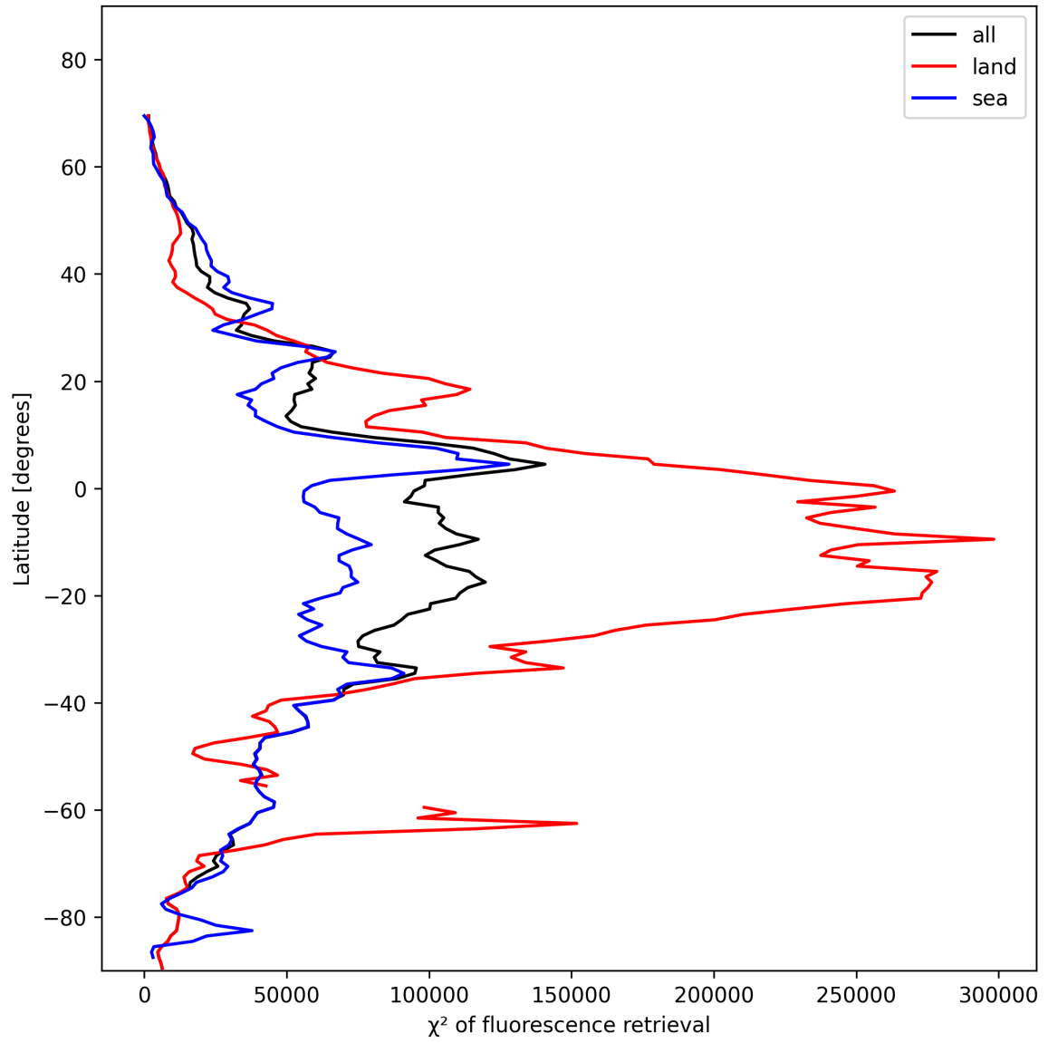
Figure 25: Zonal average of “ \chi^2 of fluorescence retrieval” for 2025-01-23 to 2025-01-25.
