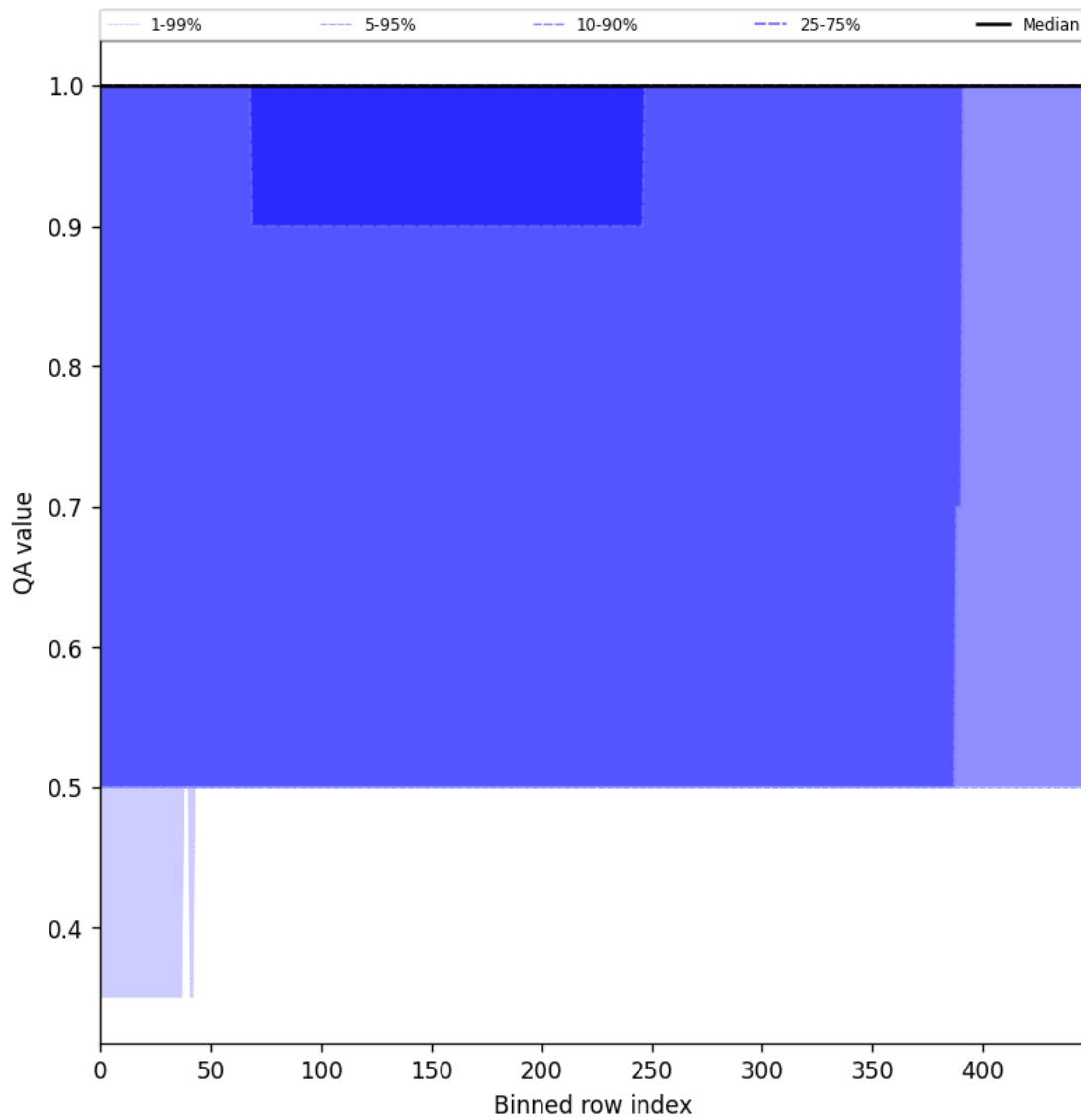
Figure 46: Along track statistics of “QA value” for 2025-01-23 to 2025-01-25
