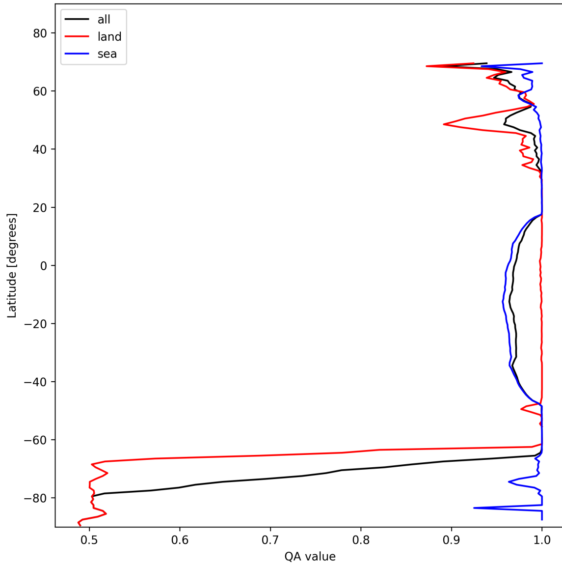
Figure 12: Zonal average of “QA value” for 2025-01-23 to 2025-01-25.
