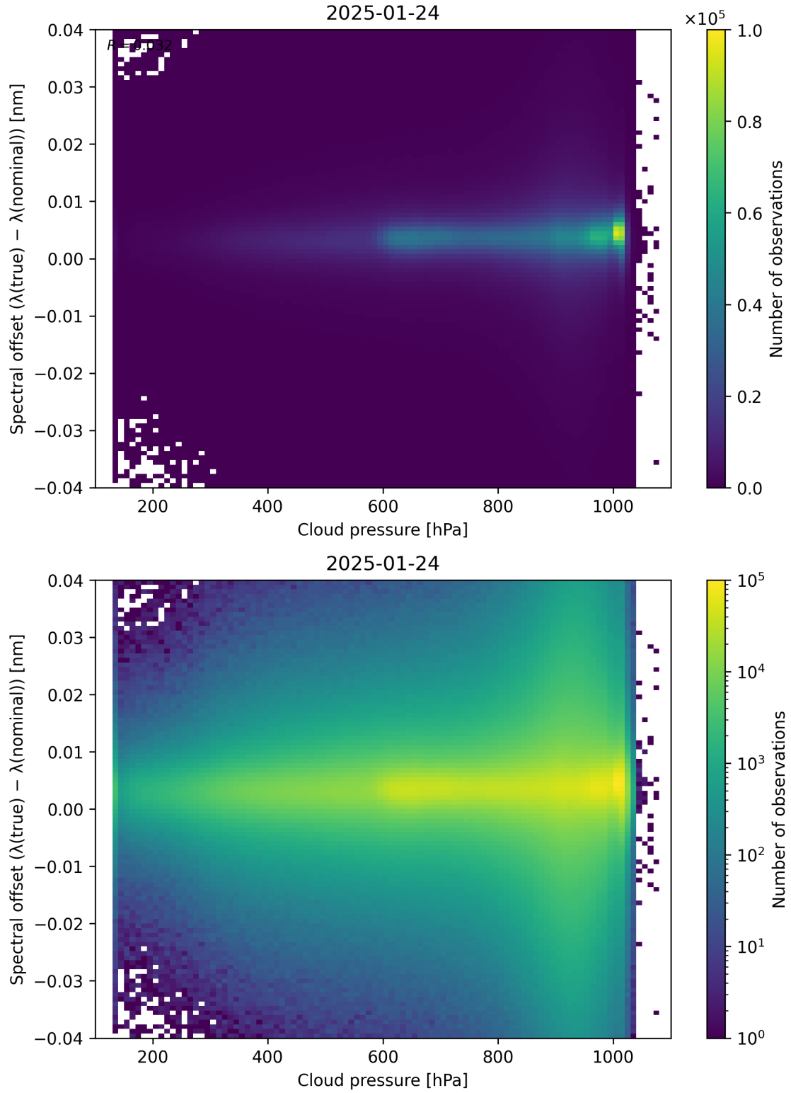
Figure 84: Scatter density plot of “Cloud pressure” against “Spectral offset ( \lambda_{\text{true}} - \lambda_{\text{nominal}} )” for 2025-01-23 to 2025-01-25.
