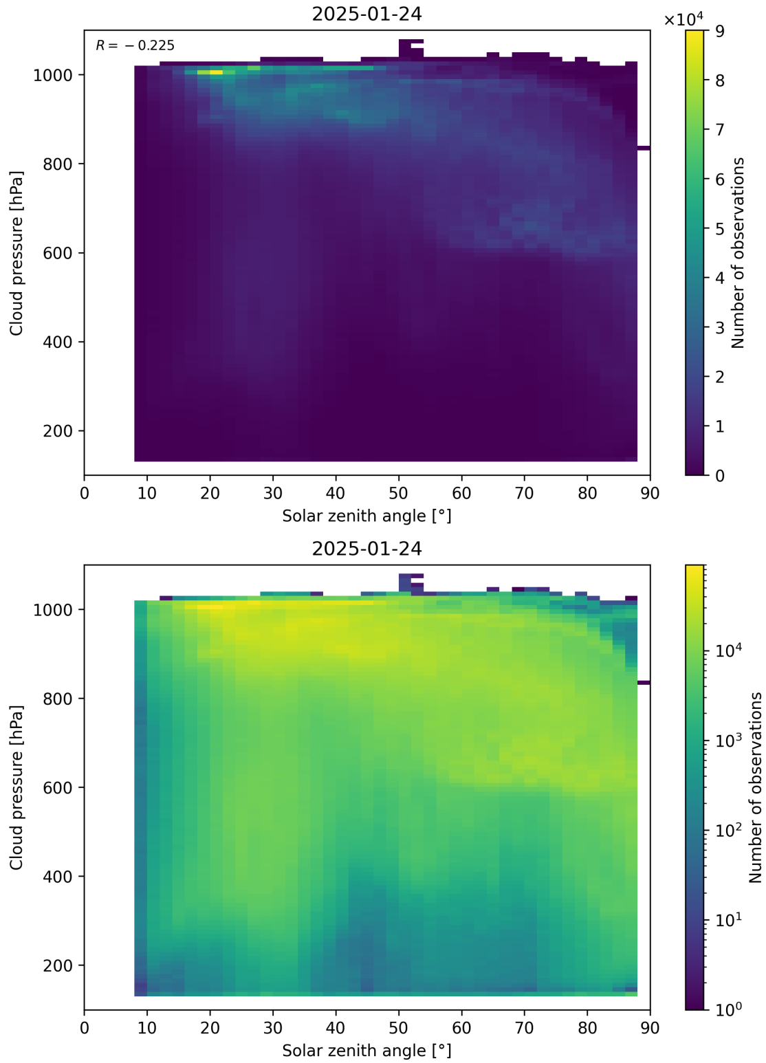
Figure 111: Scatter density plot of “Solar zenith angle” against “Cloud pressure” for 2025-01-23 to 2025-01-25.
