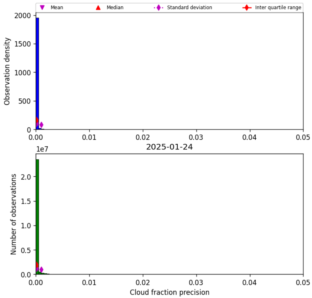
Figure 33: Histogram of “Cloud fraction precision” for 2025-01-23 to 2025-01-25
