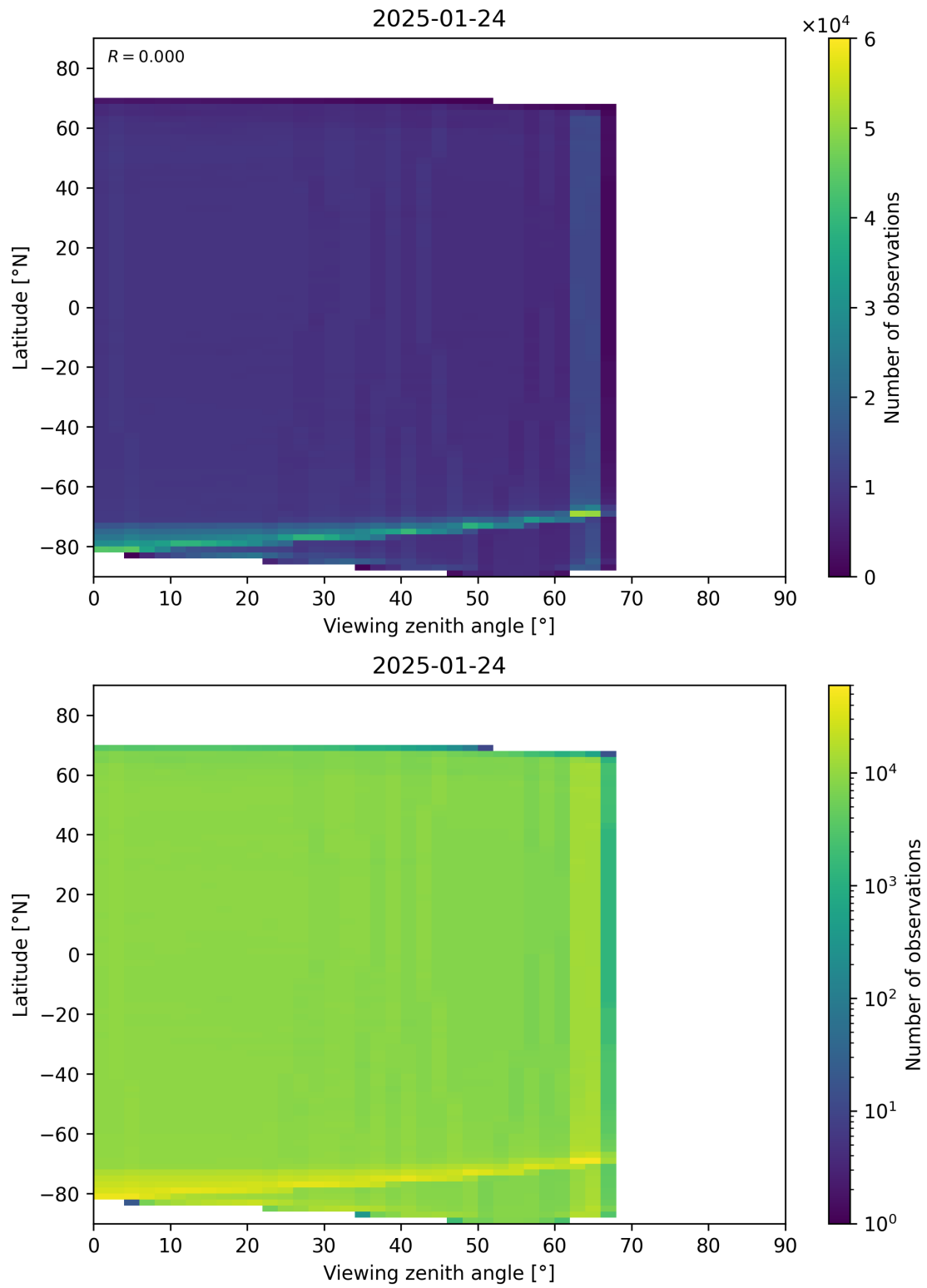
Figure 123: Scatter density plot of “Viewing zenith angle” against “Latitude” for 2025-01-23 to 2025-01-25.
