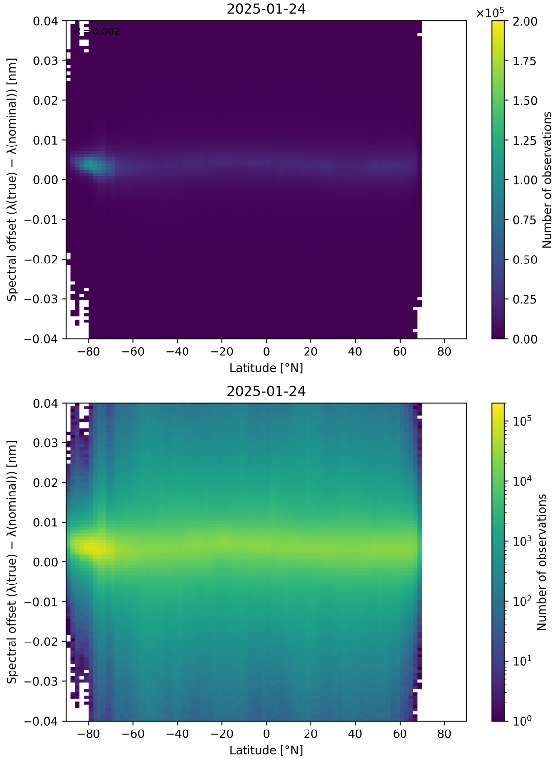
Figure 96: Scatter density plot of “Latitude” against “Spectral offset ( \lambda_{\text{true}} - \lambda_{\text{nominal}} )” for 2025-01-23 to 2025-01-25.
