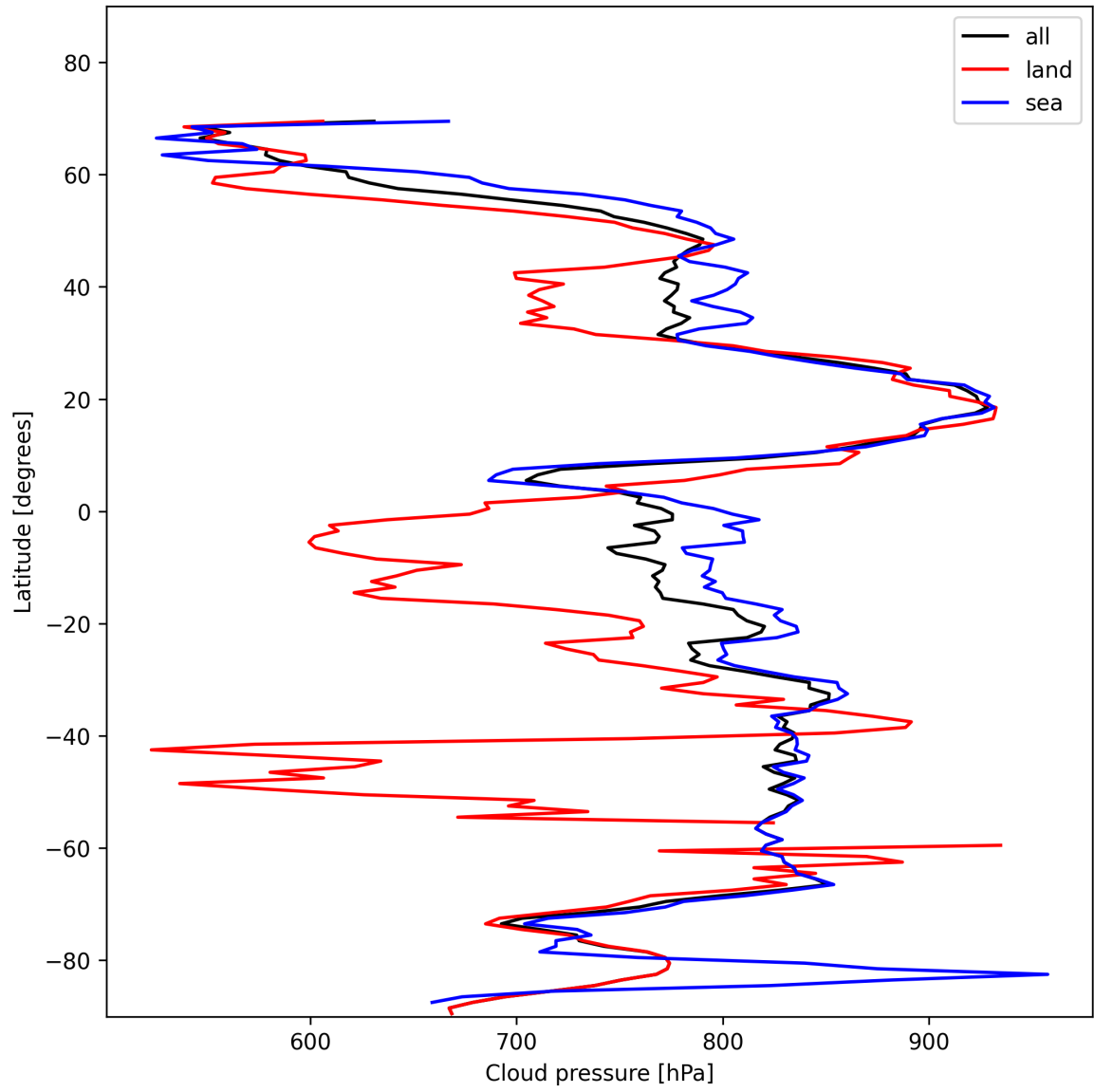
Figure 13: Zonal average of “Cloud pressure” for 2025-01-23 to 2025-01-25.
