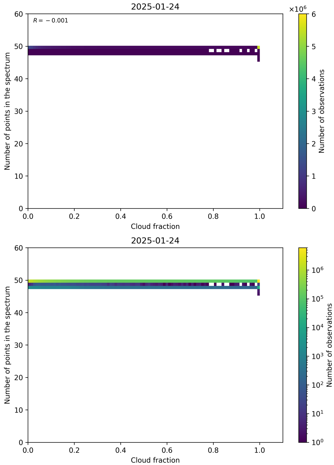
Figure 74: Scatter density plot of “Cloud fraction” against “Number of points in the spectrum” for 2025-01-23 to 2025-01-25.
