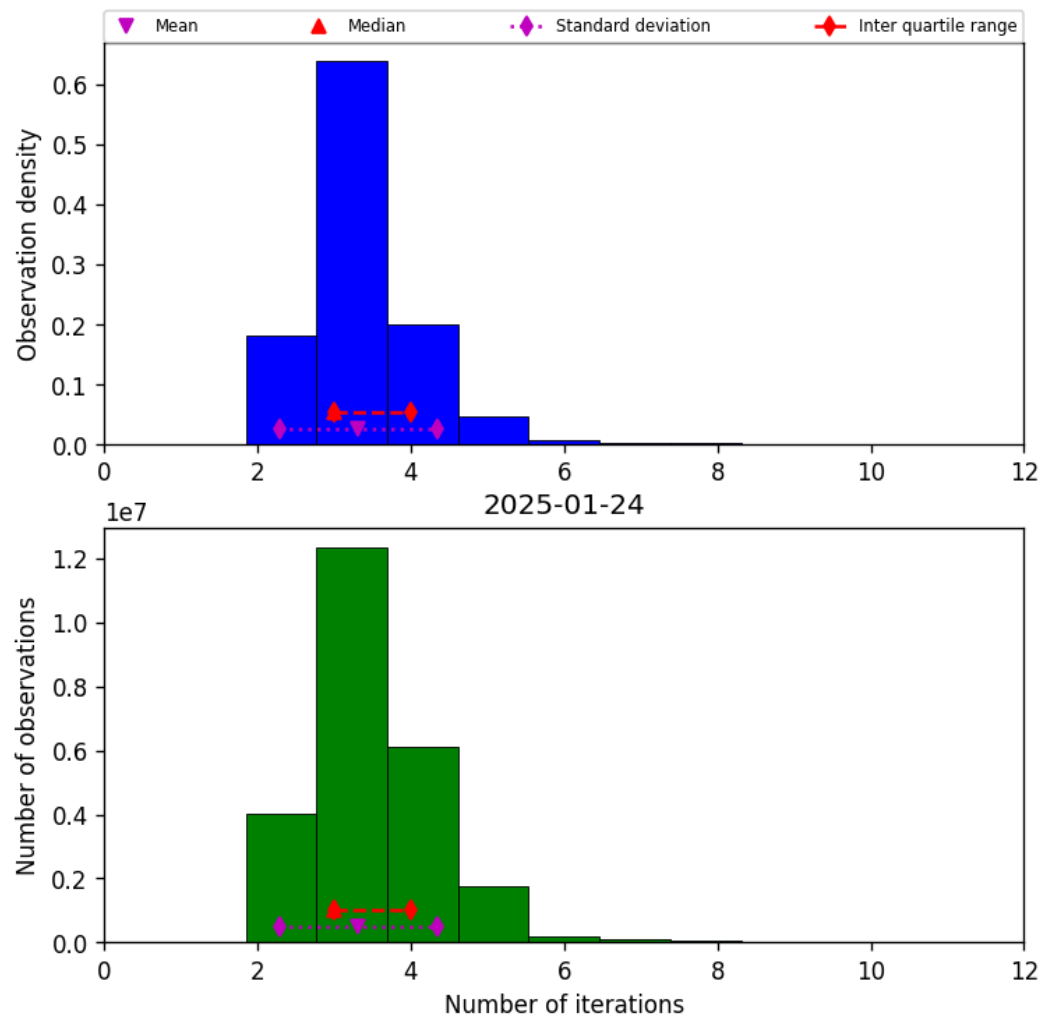
Figure 39: Histogram of “Number of iterations” for 2025-01-23 to 2025-01-25
