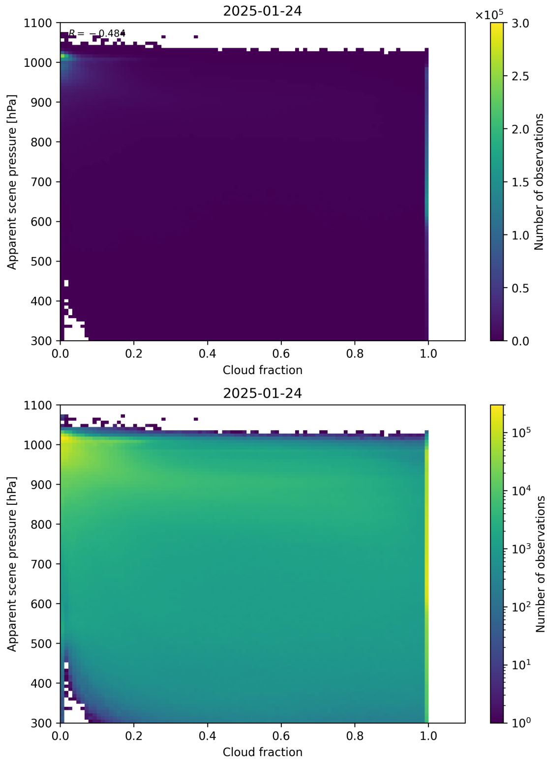
Figure 70: Scatter density plot of “Cloud fraction” against “Apparent scene pressure” for 2025-01-23 to 2025-01-25.
