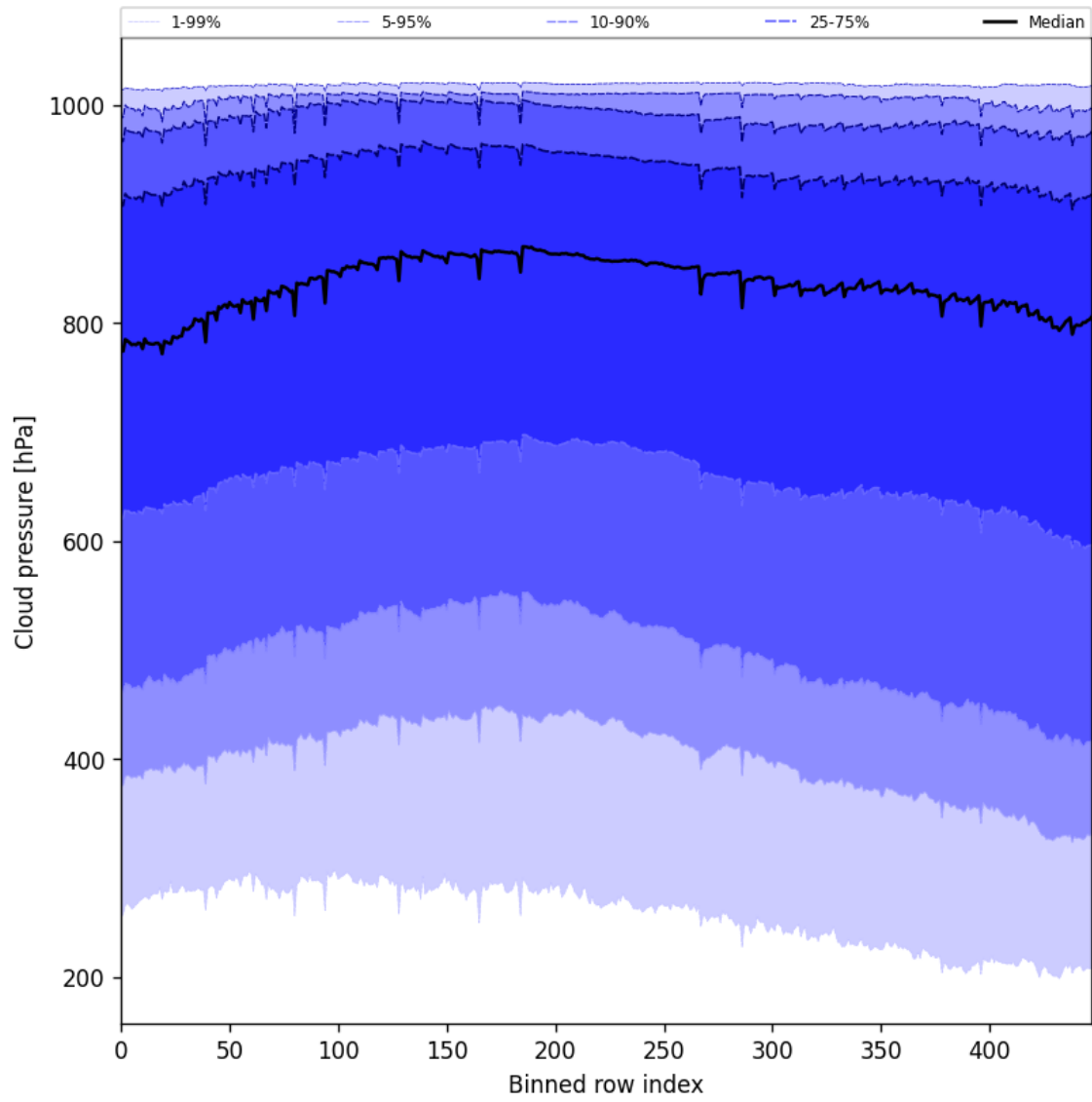
Figure 47: Along track statistics of “Cloud pressure” for 2025-01-23 to 2025-01-25
