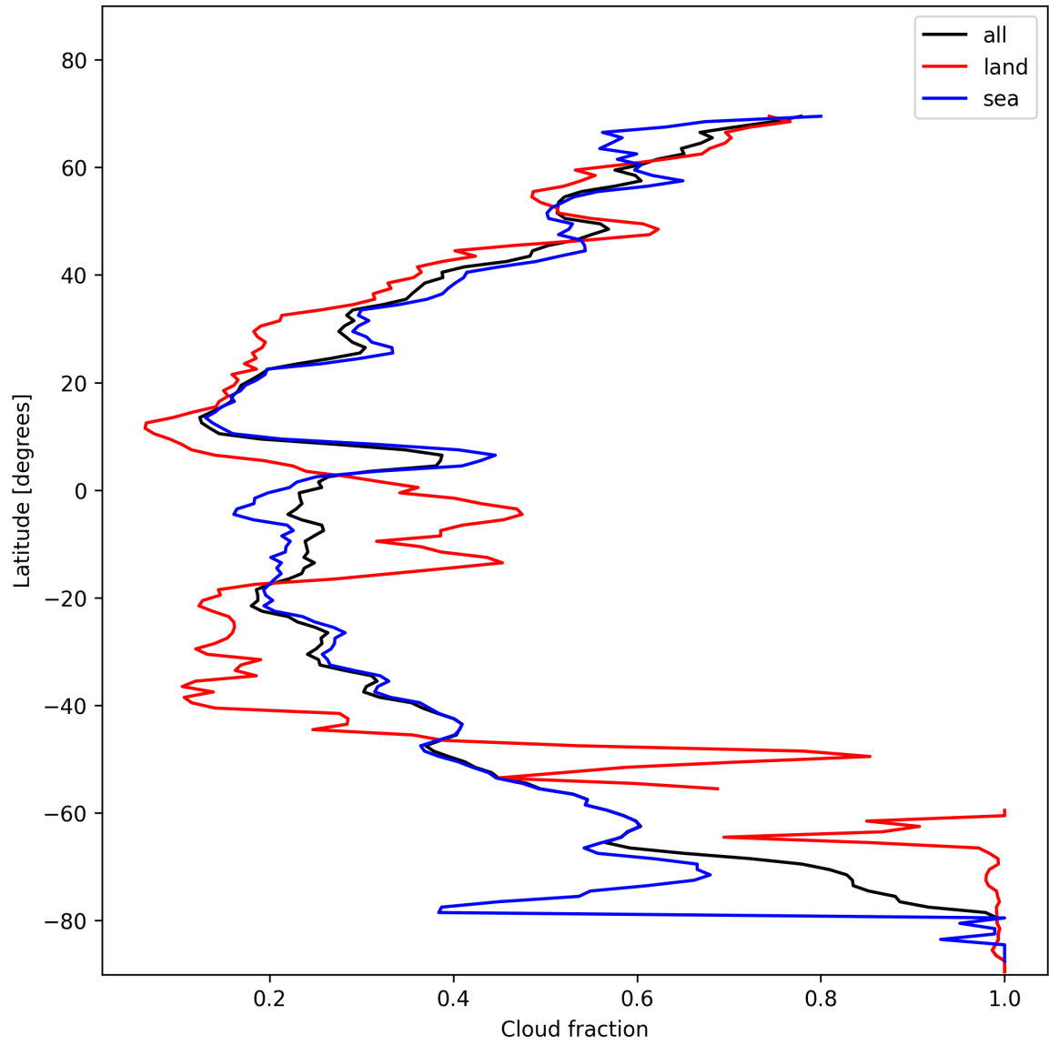
Figure 15: Zonal average of “Cloud fraction” for 2025-01-23 to 2025-01-25.
