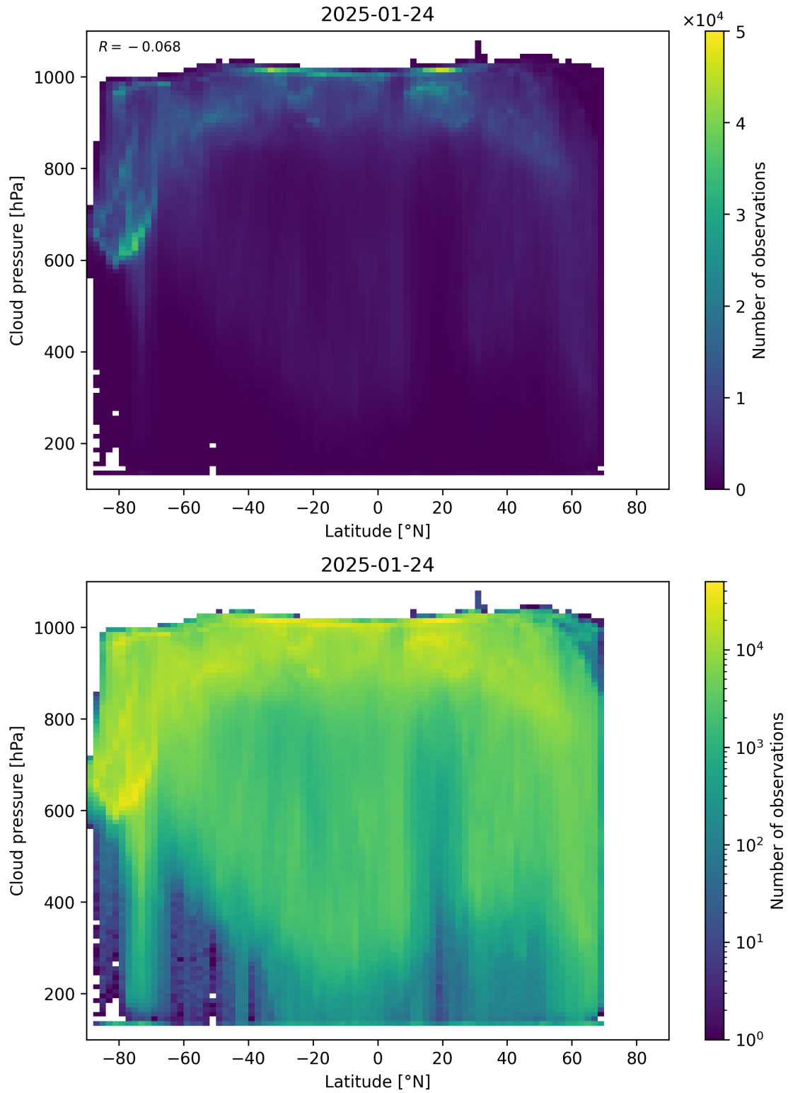
Figure 91: Scatter density plot of “Latitude” against “Cloud pressure” for 2025-01-23 to 2025-01-25.
