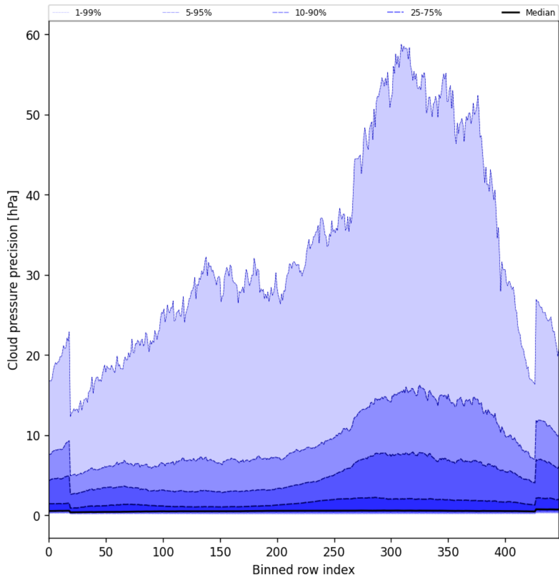
Figure 48: Along track statistics of “Cloud pressure precision” for 2025-01-23 to 2025-01-25
