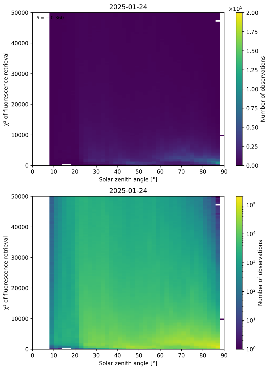
Figure 109: Scatter density plot of “Solar zenith angle” against “ \chi^2 of fluorescence retrieval” for 2025-01-23 to 2025-01-25.
