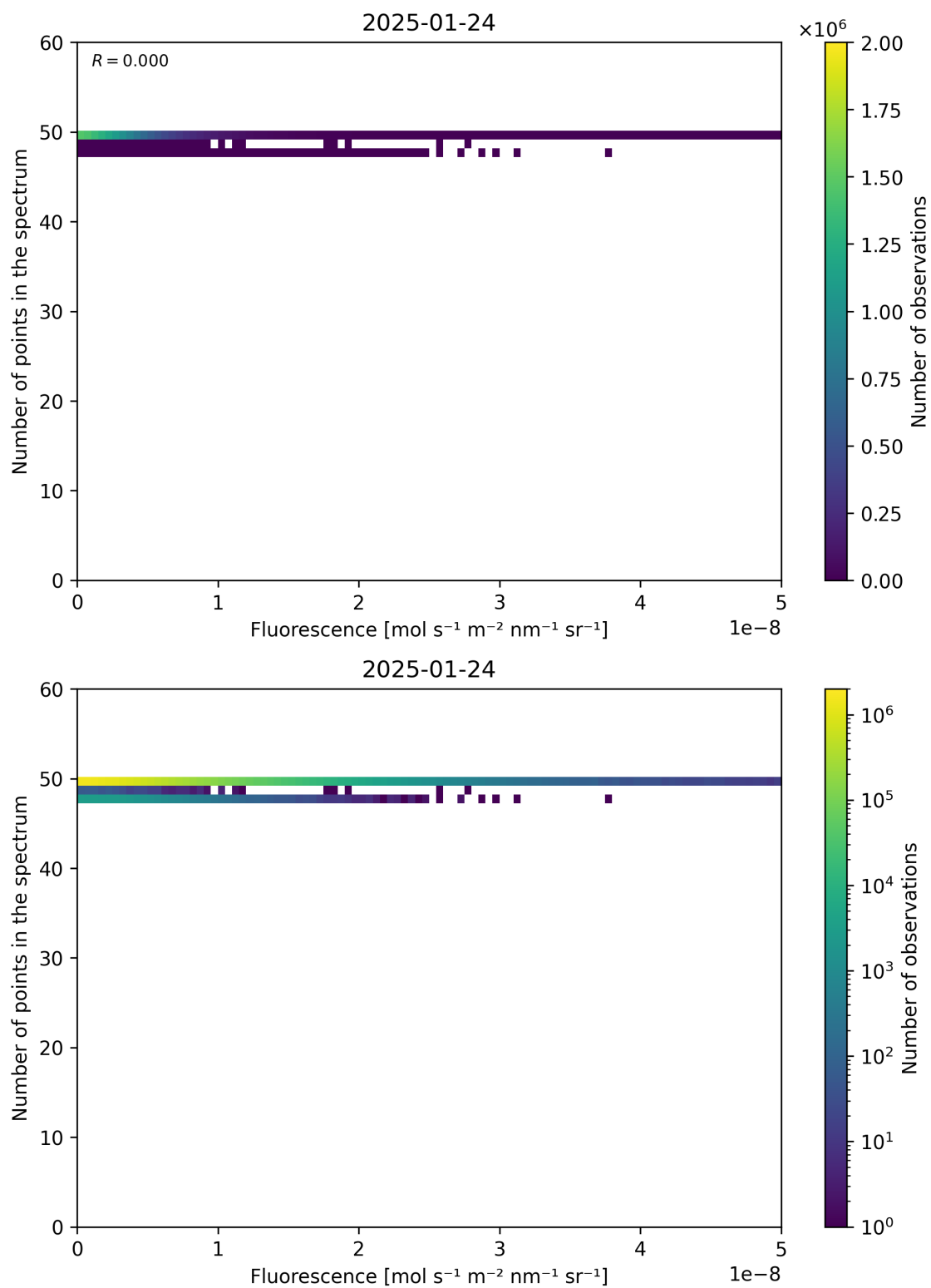
Figure 86: Scatter density plot of “Fluorescence” against “Number of points in the spectrum” for 2025-01-23 to 2025-01-25.
