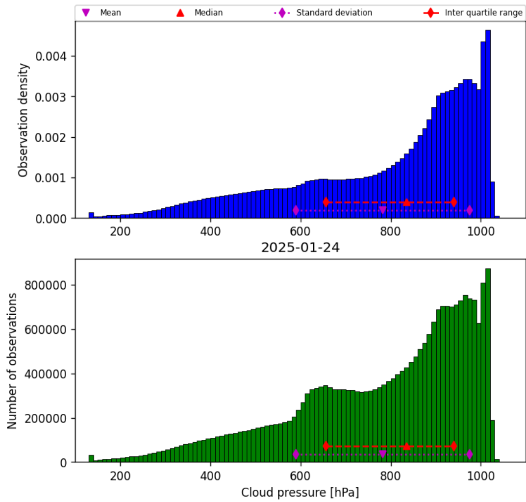
Figure 30: Histogram of “Cloud pressure” for 2025-01-23 to 2025-01-25
