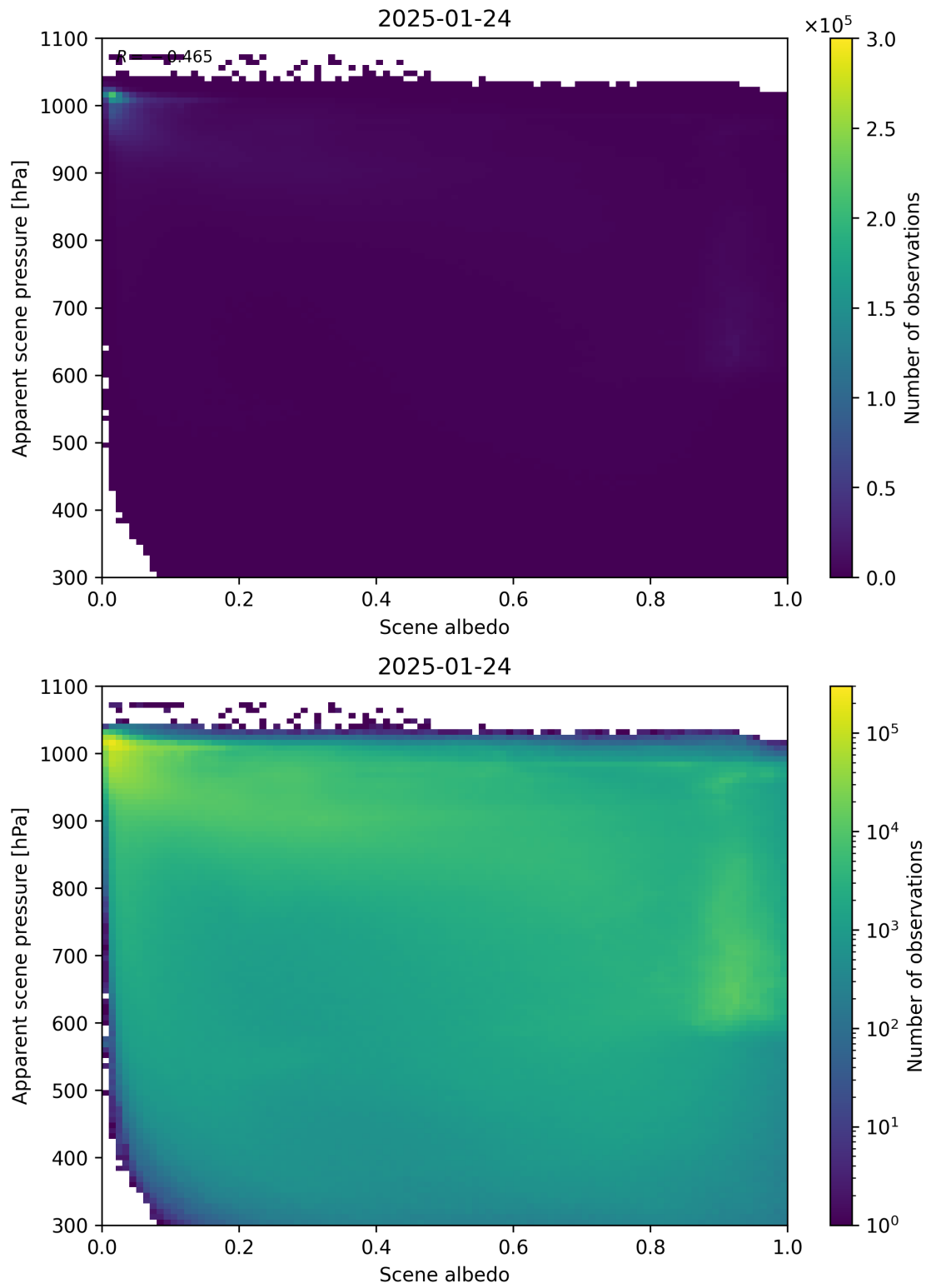
Figure 102: Scatter density plot of “Scene albedo” against “Apparent scene pressure” for 2025-01-23 to 2025-01-25.
