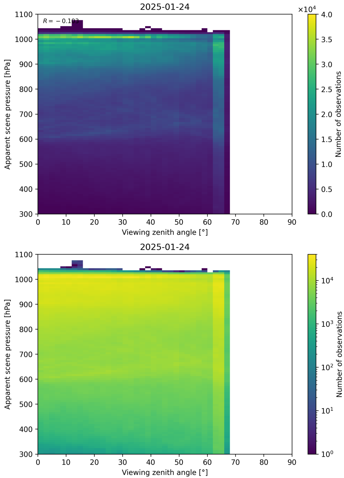
Figure 118: Scatter density plot of “Viewing zenith angle” against “Apparent scene pressure” for 2025-01-23 to 2025-01-25.
