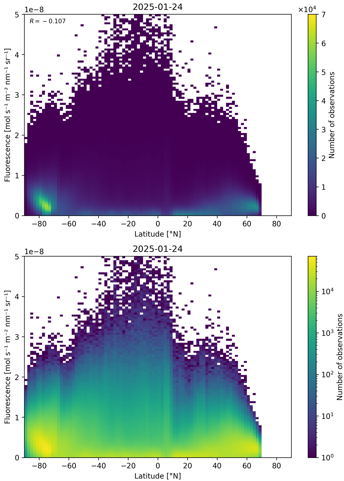
Figure 92: Scatter density plot of “Latitude” against “Fluorescence” for 2025-01-23 to 2025-01-25.
