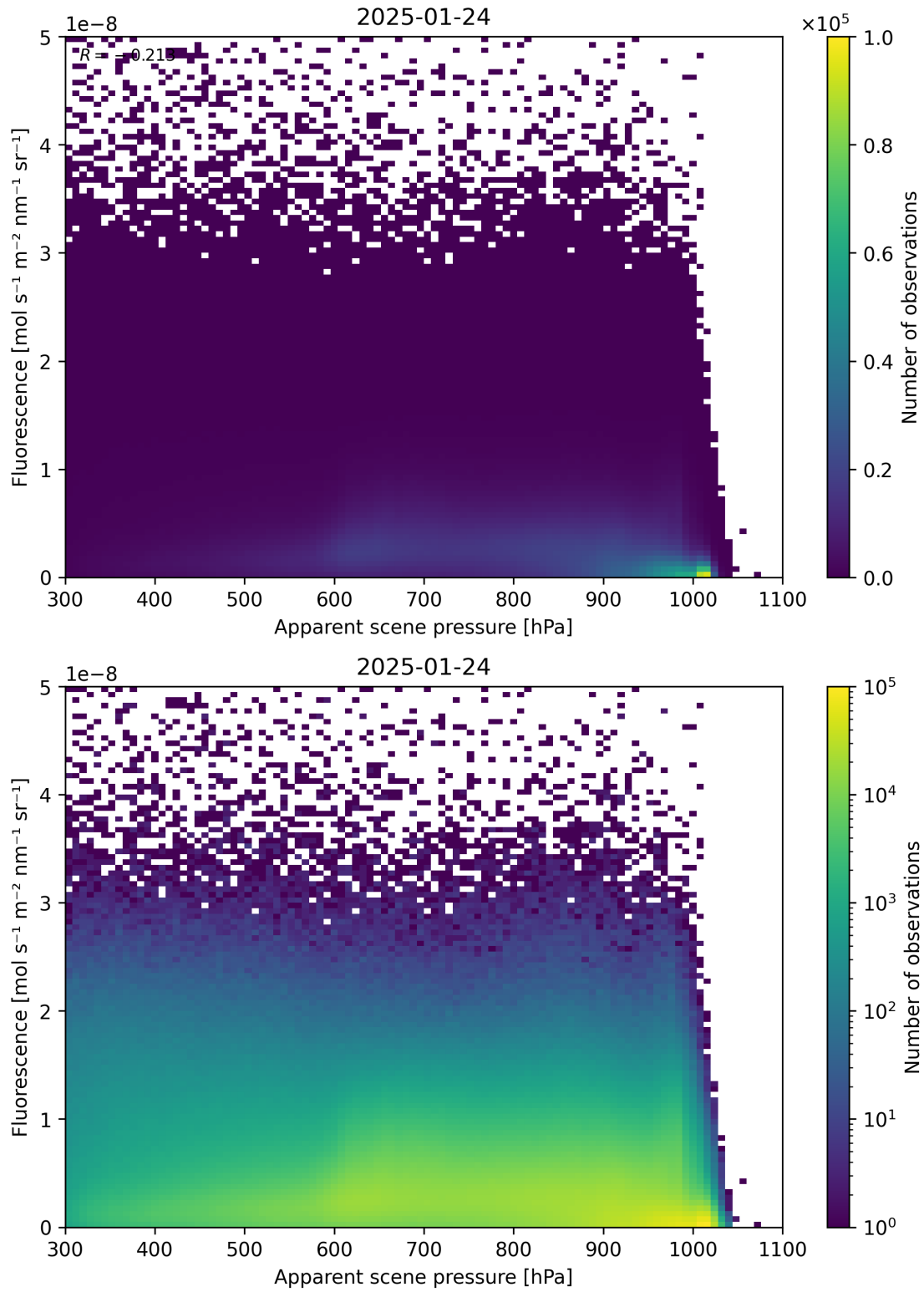
Figure 64: Scatter density plot of “Apparent scene pressure” against “Fluorescence” for 2025-01-23 to 2025-01-25.
