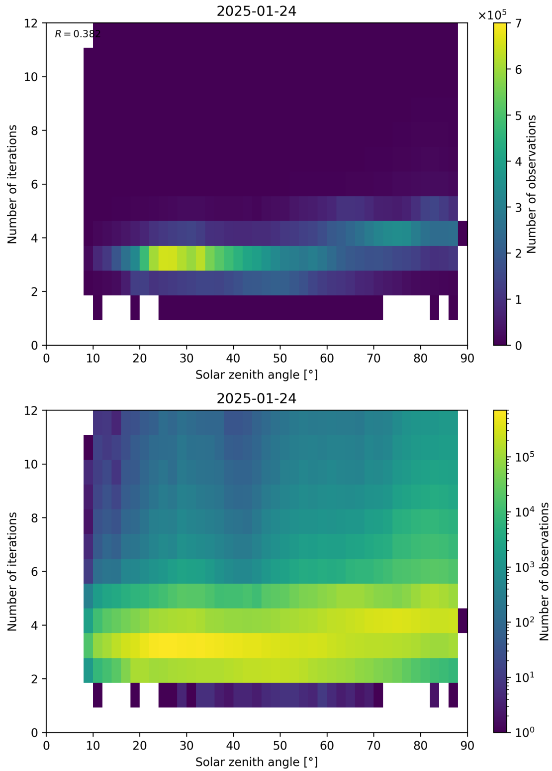
Figure 114: Scatter density plot of “Solar zenith angle” against “Number of iterations” for 2025-01-23 to 2025-01-25.
