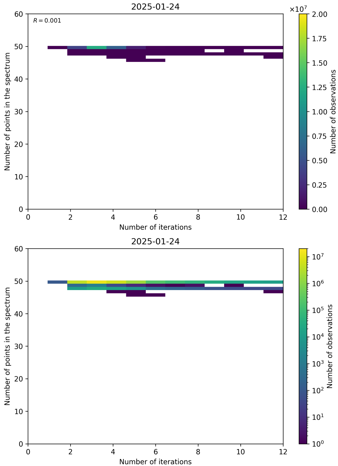
Figure 99: Scatter density plot of “Number of iterations” against “Number of points in the spectrum” for 2025-01-23 to 2025-01-25.
