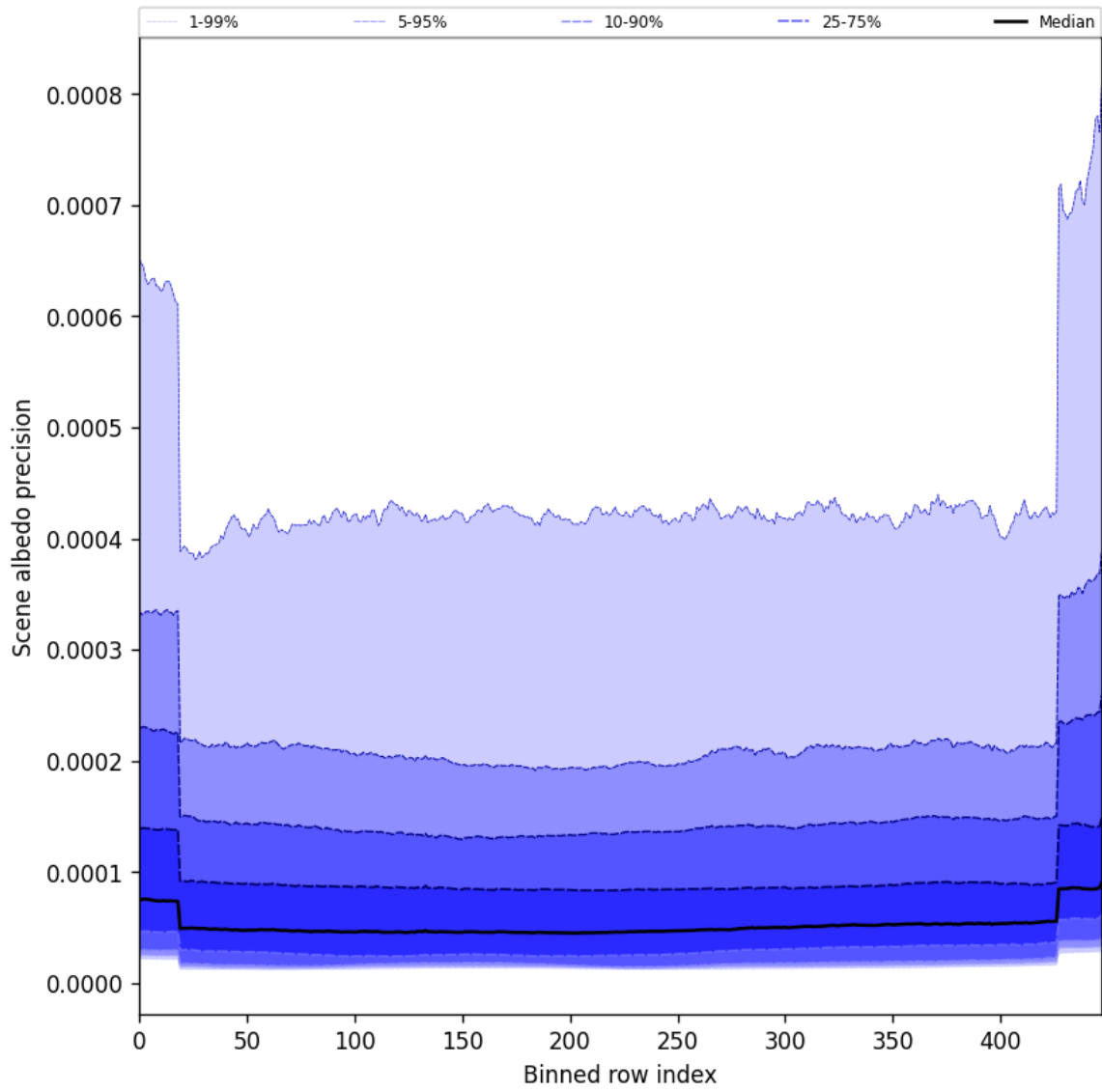
Figure 52: Along track statistics of “Scene albedo precision” for 2025-01-23 to 2025-01-25
