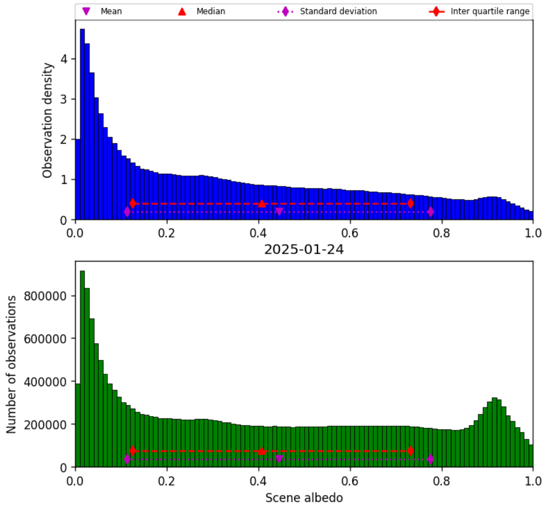
Figure 34: Histogram of “Scene albedo” for 2025-01-23 to 2025-01-25
