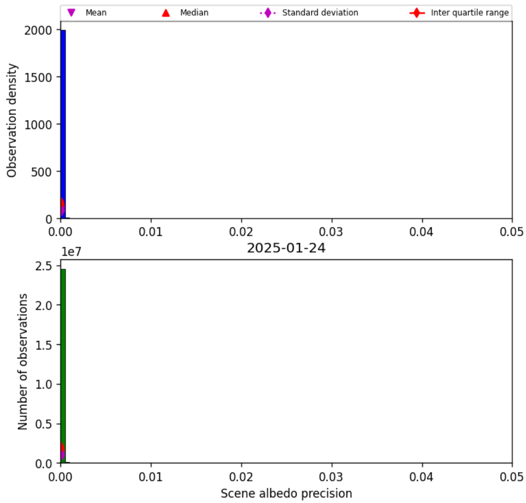
Figure 35: Histogram of “Scene albedo precision” for 2025-01-23 to 2025-01-25
