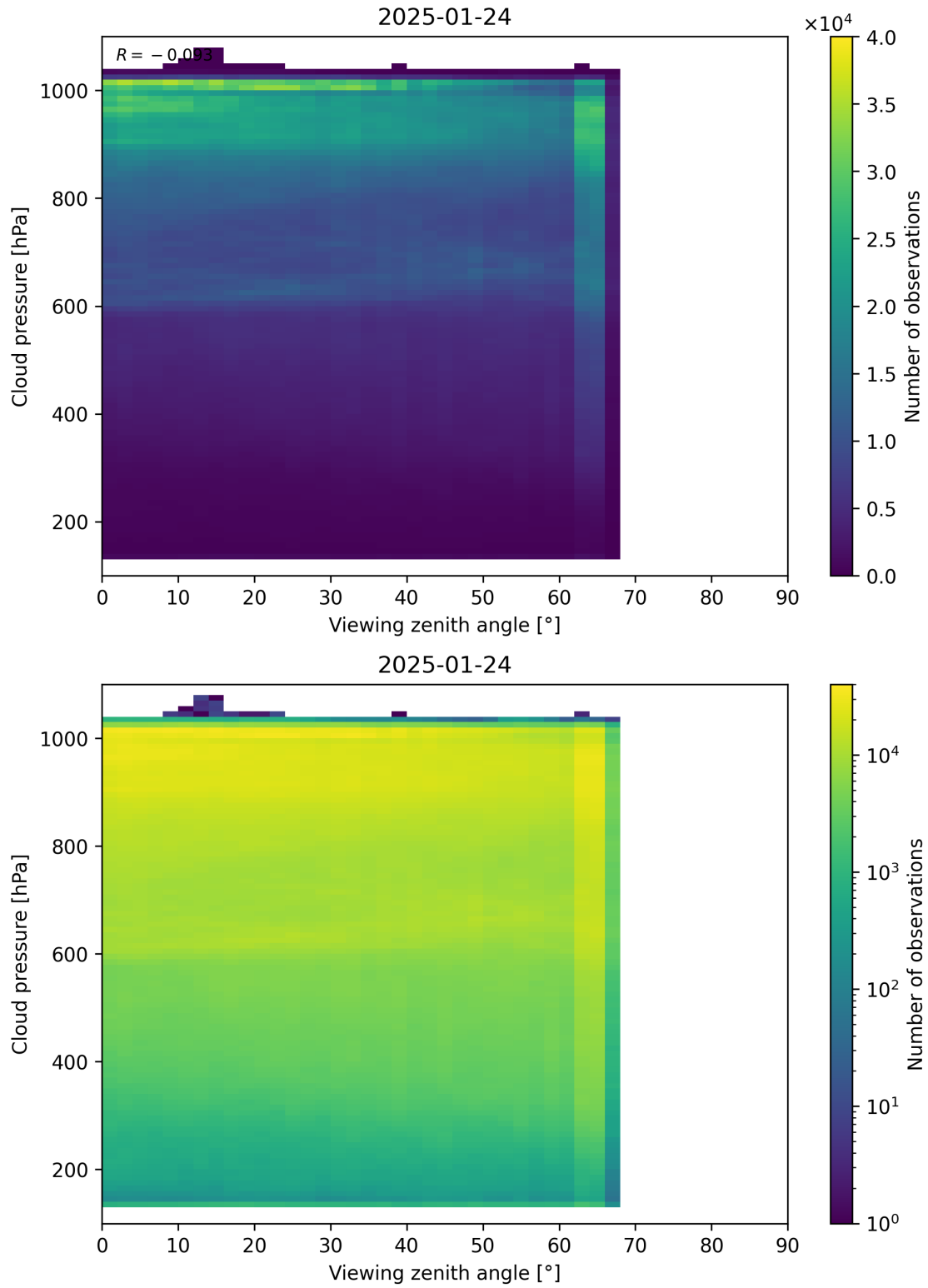
Figure 121: Scatter density plot of “Viewing zenith angle” against “Cloud pressure” for 2025-01-23 to 2025-01-25.
