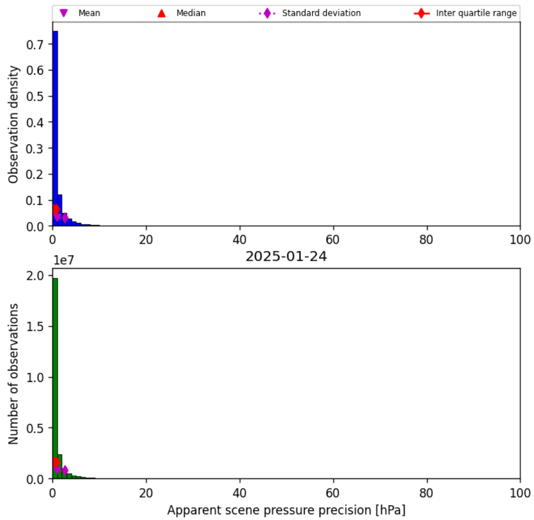
Figure 37: Histogram of “Apparent scene pressure precision” for 2025-01-23 to 2025-01-25
