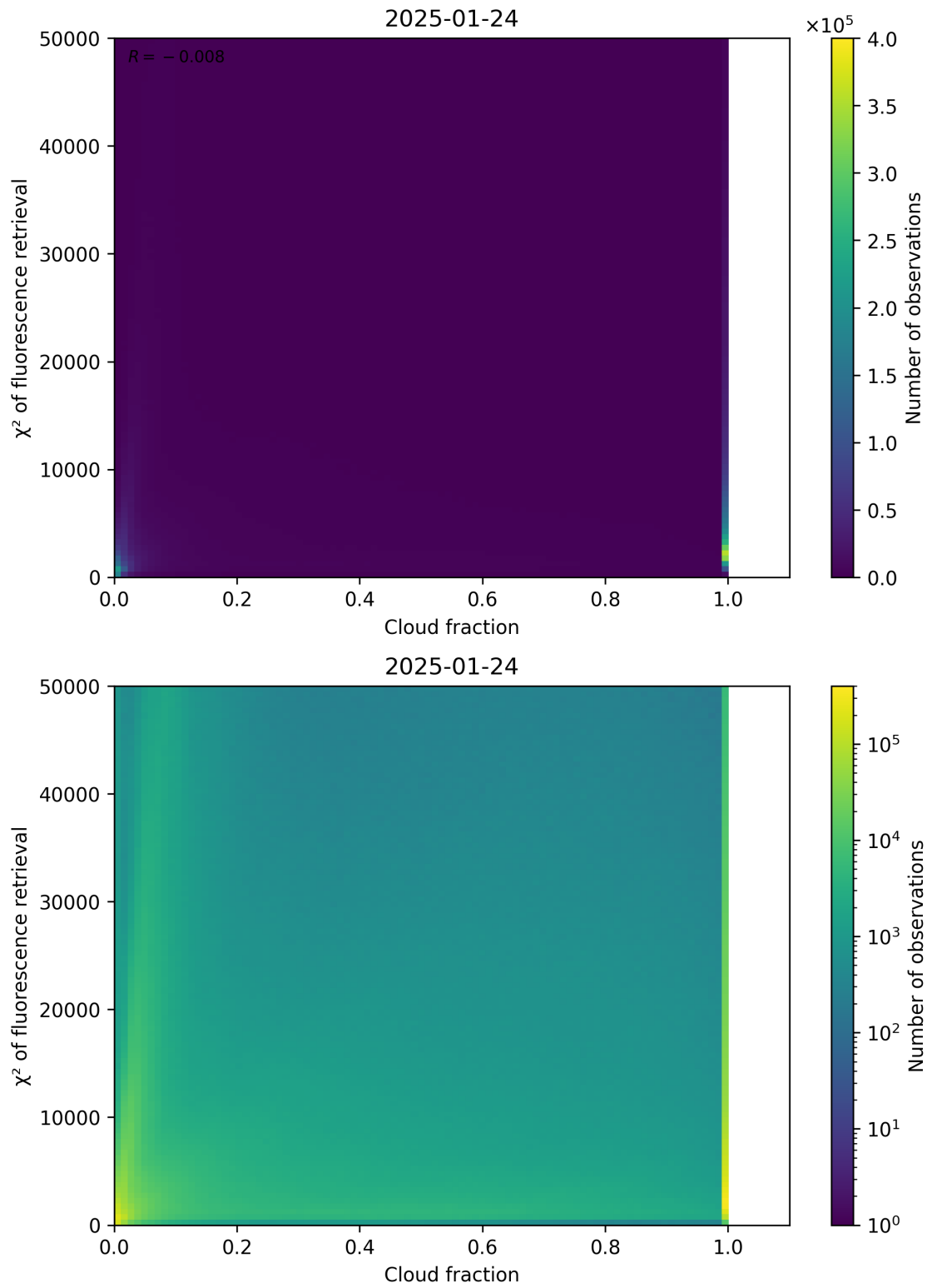
Figure 71: Scatter density plot of “Cloud fraction” against “ \chi^2 of fluorescence retrieval” for 2025-01-23 to 2025-01-25.
