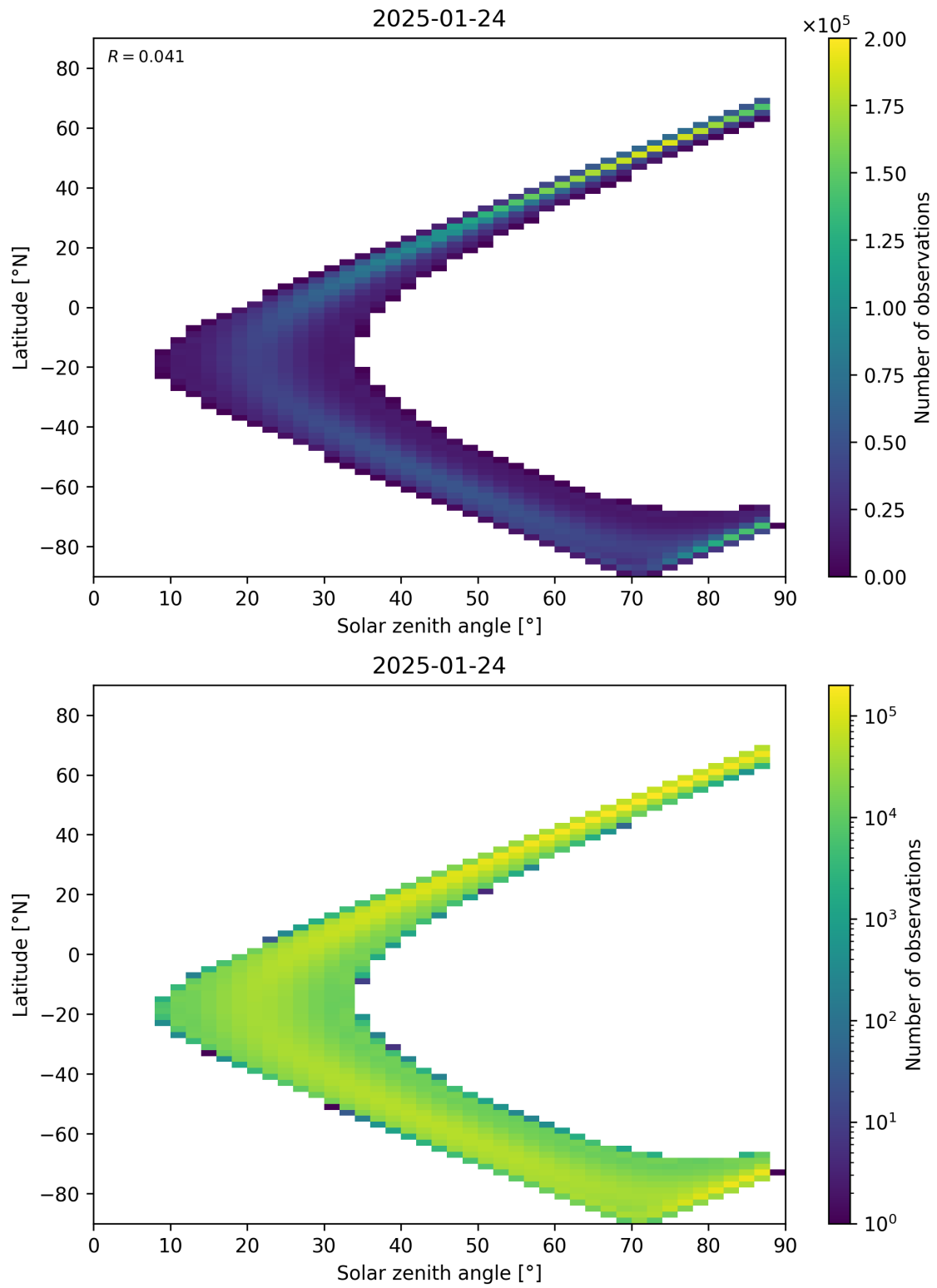
Figure 113: Scatter density plot of “Solar zenith angle” against “Latitude” for 2025-01-23 to 2025-01-25.
