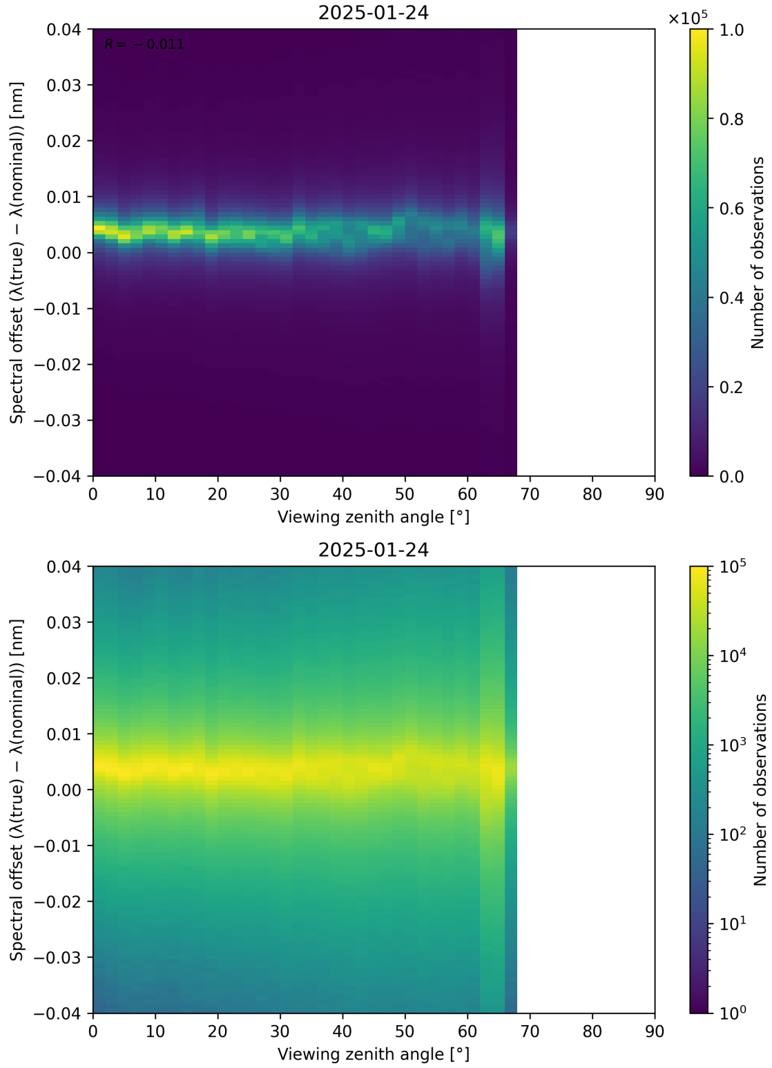
Figure 128: Scatter density plot of “Viewing zenith angle” against “Spectral offset ( \lambda_{\text{true}} - \lambda_{\text{nominal}} )” for 2025-01-23 to 2025-01-25.
