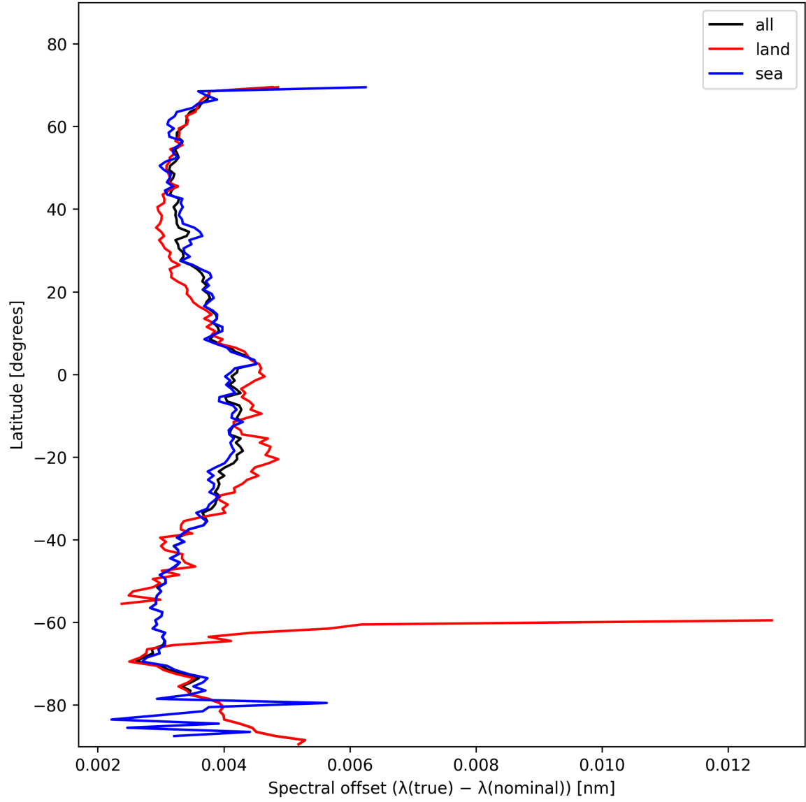
Figure 28: Zonal average of “Spectral offset ( \lambda_{\text{true}} - \lambda_{\text{nominal}} )” for 2025-01-23 to 2025-01-25.
