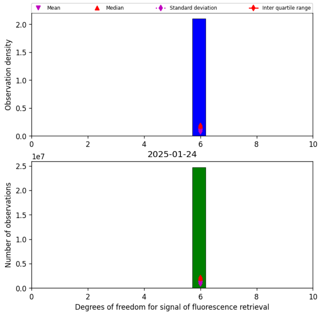
Figure 43: Histogram of “Degrees of freedom for signal of fluorescence retrieval” for 2025-01-23 to 2025-01-25
