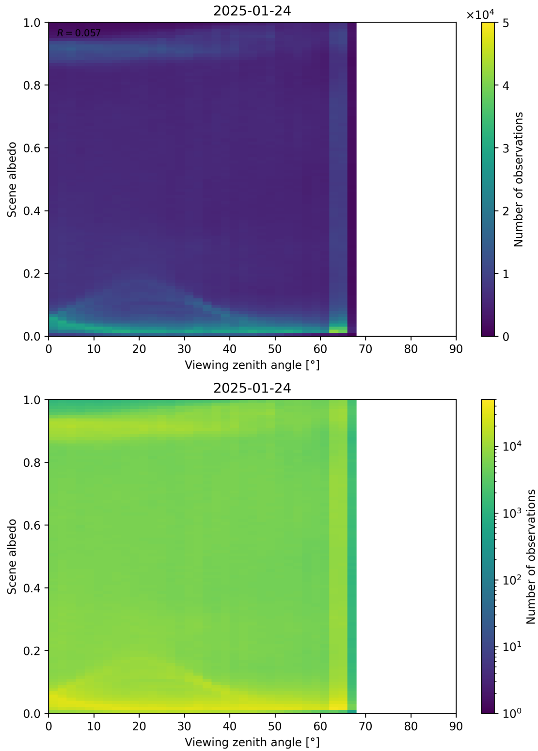
Figure 126: Scatter density plot of “Viewing zenith angle” against “Scene albedo” for 2025-01-23 to 2025-01-25.
