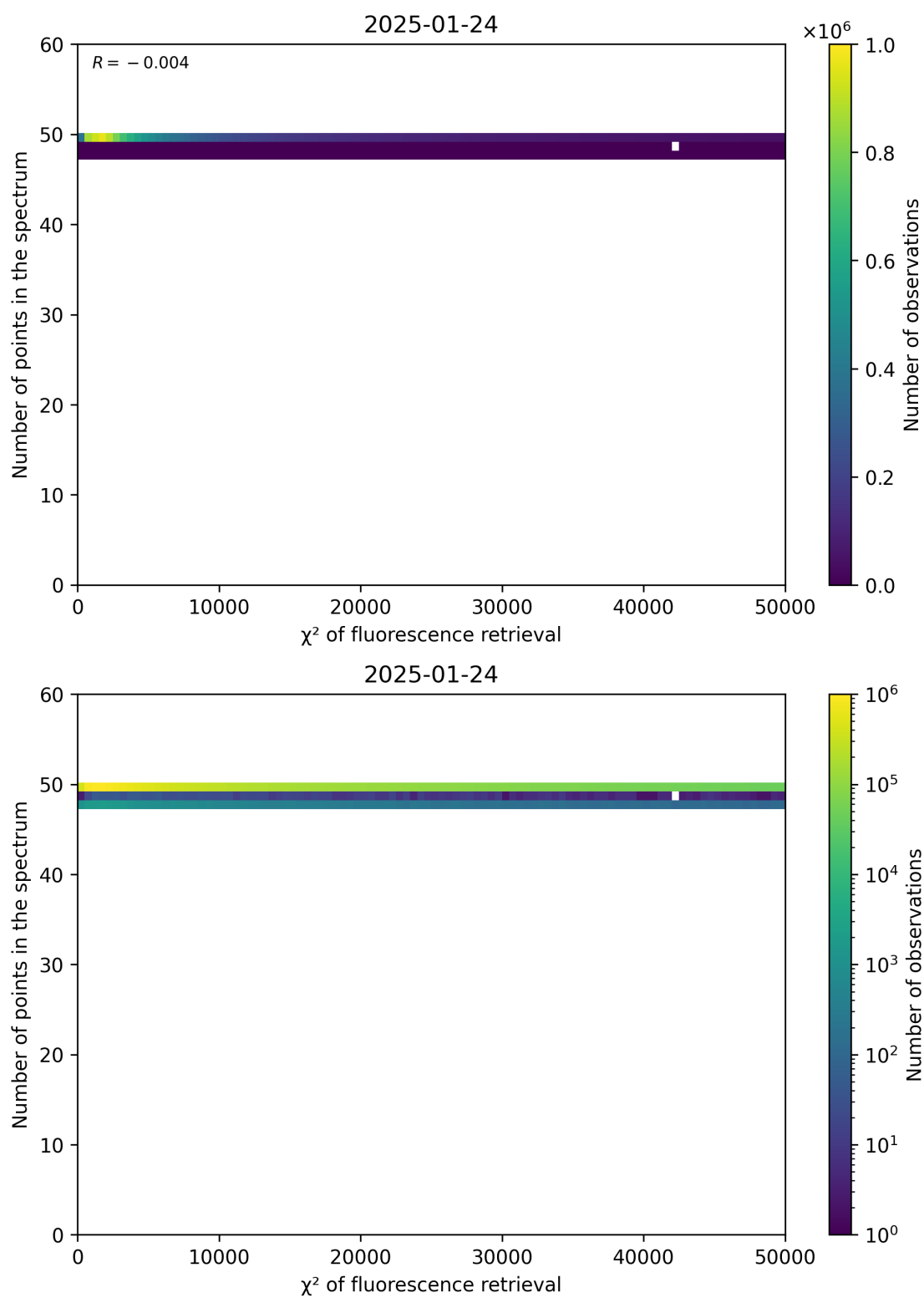
Figure 68: Scatter density plot of “ \chi^2 of fluorescence retrieval” against “Number of points in the spectrum” for 2025-01-23 to 2025-01-25.
