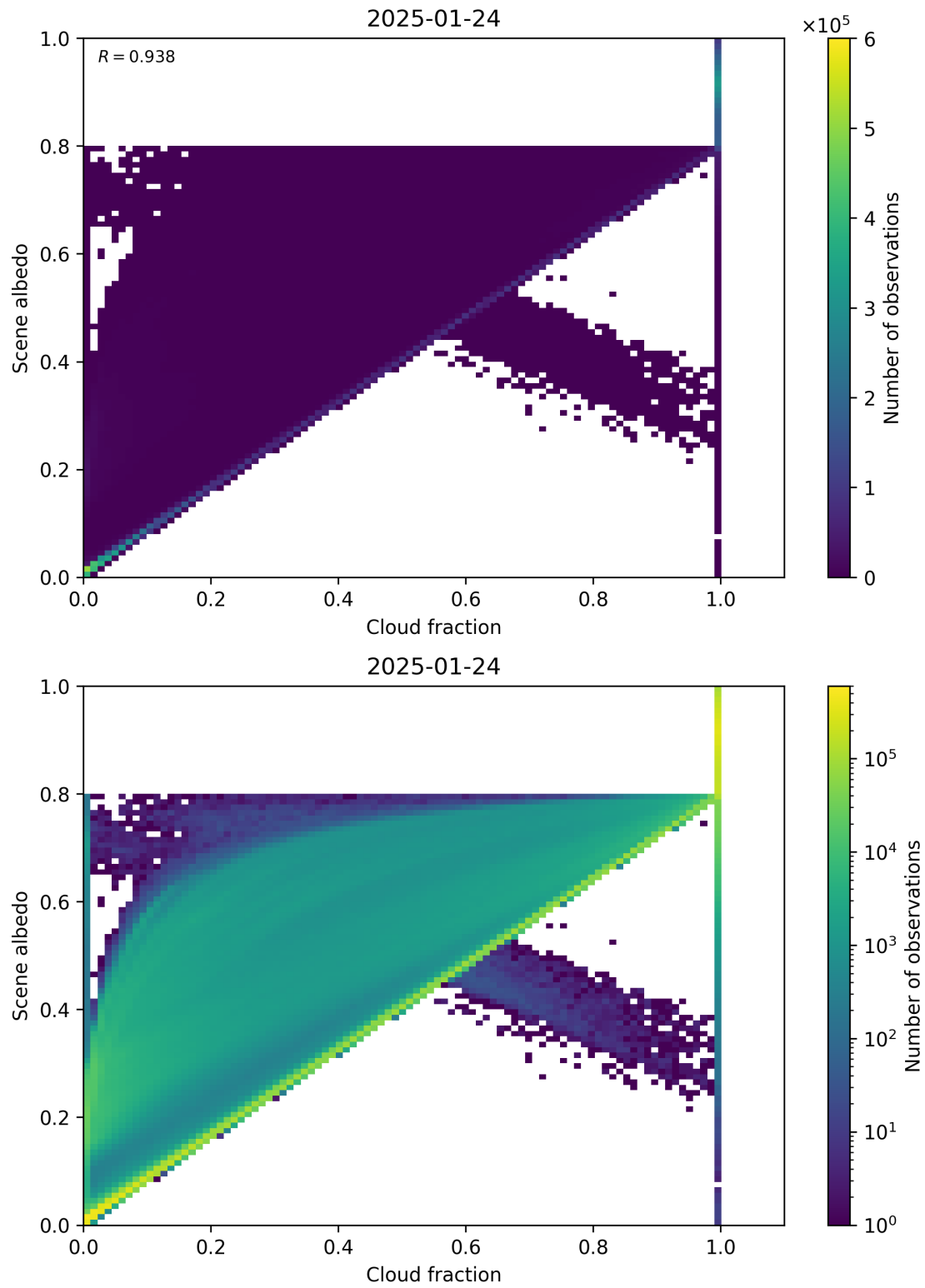
Figure 75: Scatter density plot of “Cloud fraction” against “Scene albedo” for 2025-01-23 to 2025-01-25.
