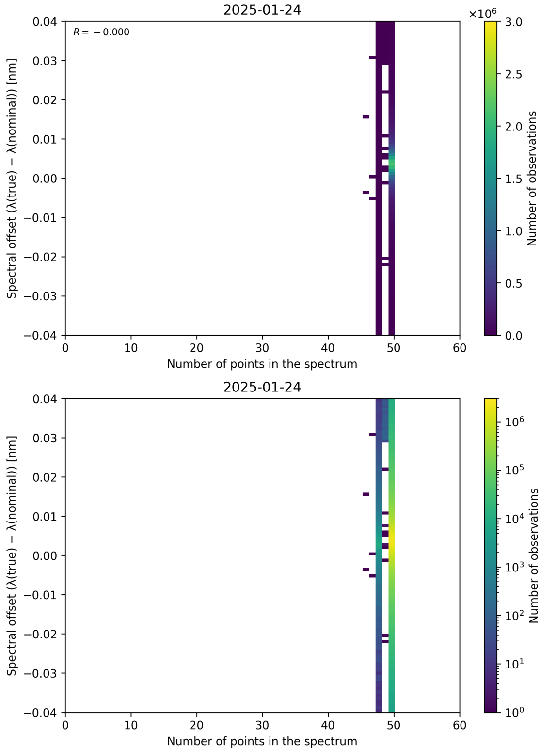
Figure 101: Scatter density plot of “Number of points in the spectrum” against “Spectral offset ( \lambda_{\text{true}} - \lambda_{\text{nominal}} )” for 2025-01-23 to 2025-01-25.
