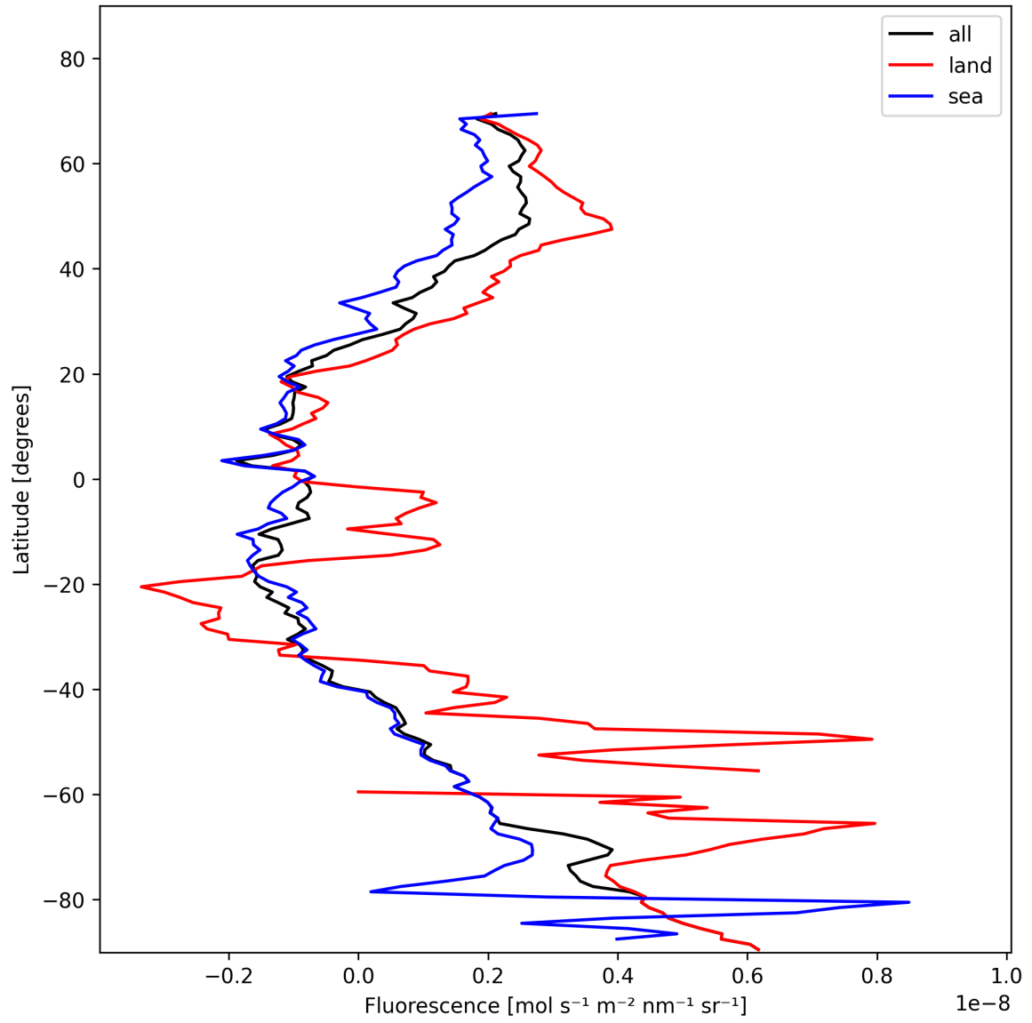
Figure 23: Zonal average of “Fluorescence” for 2025-01-23 to 2025-01-25.
