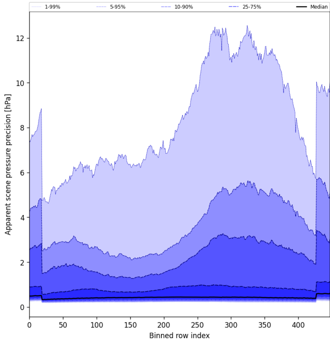
Figure 54: Along track statistics of “Apparent scene pressure precision” for 2025-01-23 to 2025-01-25
