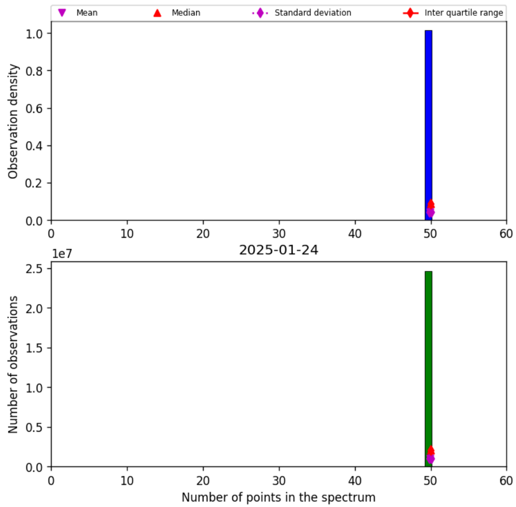
Figure 44: Histogram of "Number of points in the spectrum" for 2025-01-23 to 2025-01-25
