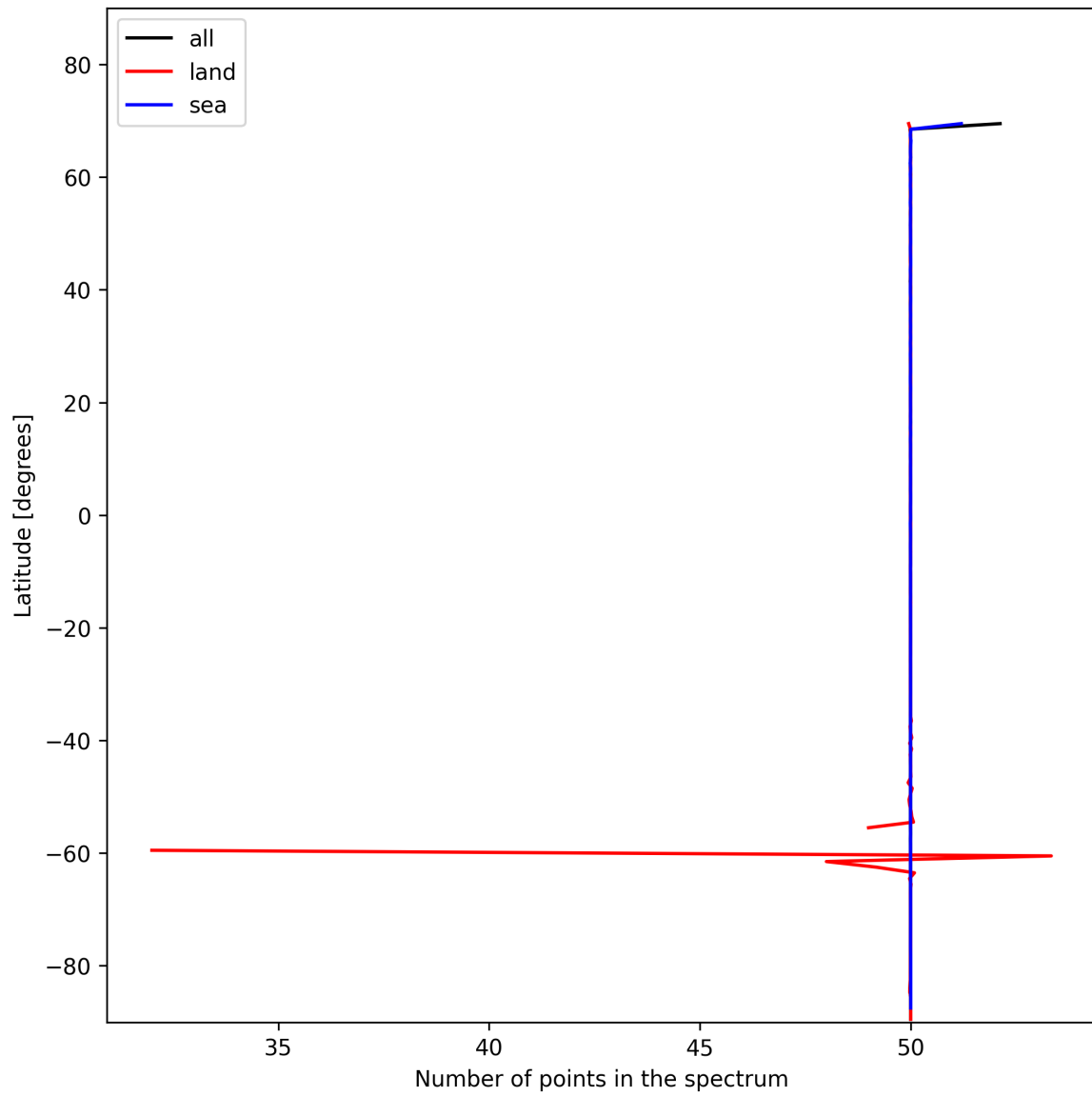
Figure 27: Zonal average of “Number of points in the spectrum” for 2025-01-23 to 2025-01-25.
