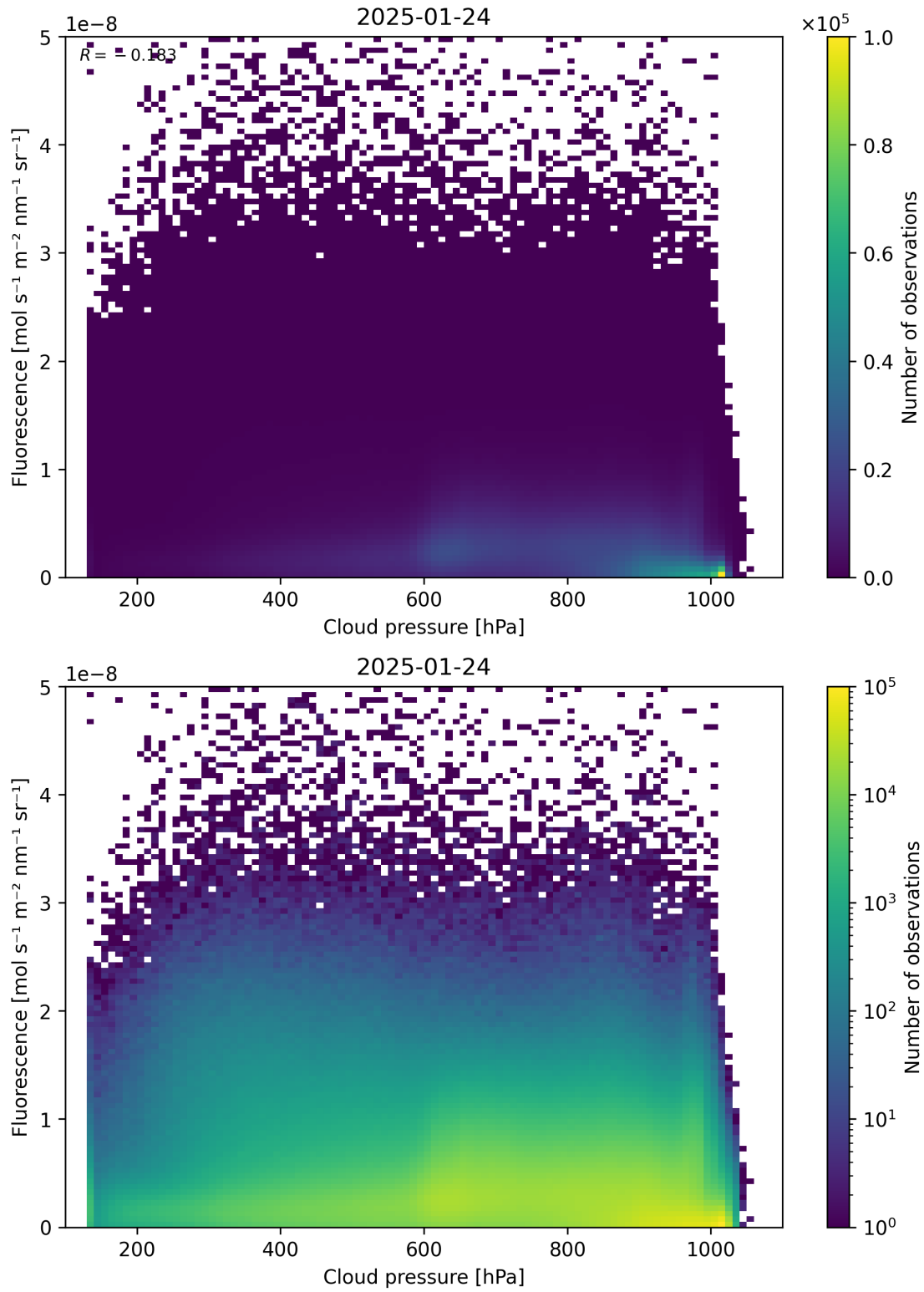
Figure 80: Scatter density plot of “Cloud pressure” against “Fluorescence” for 2025-01-23 to 2025-01-25.
