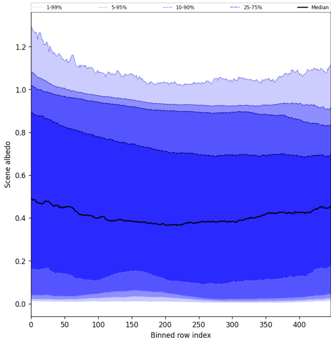
Figure 51: Along track statistics of “Scene albedo” for 2025-01-23 to 2025-01-25
