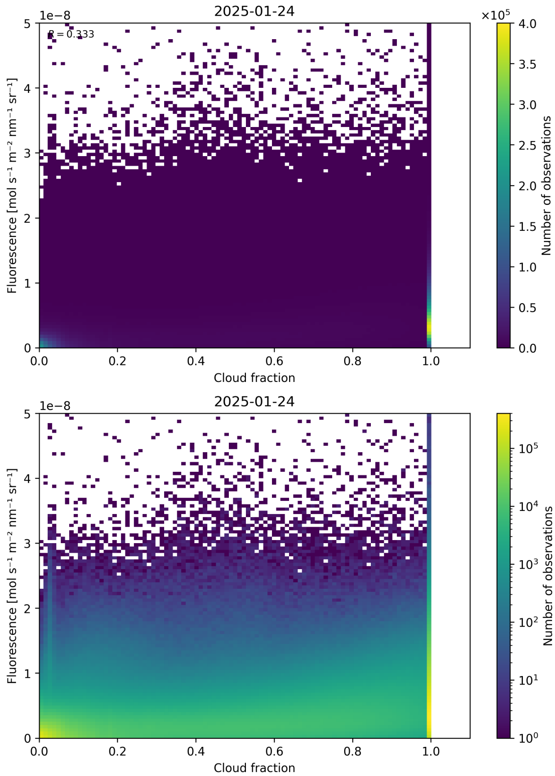
Figure 72: Scatter density plot of “Cloud fraction” against “Fluorescence” for 2025-01-23 to 2025-01-25.
