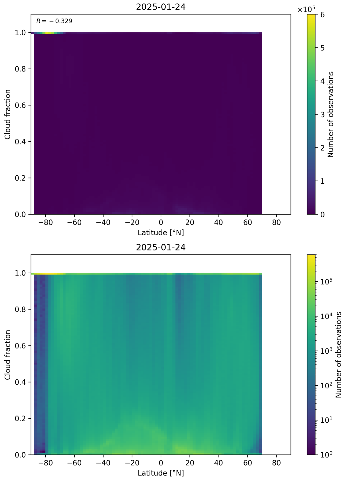
Figure 90: Scatter density plot of “Latitude” against “Cloud fraction” for 2025-01-23 to 2025-01-25.
