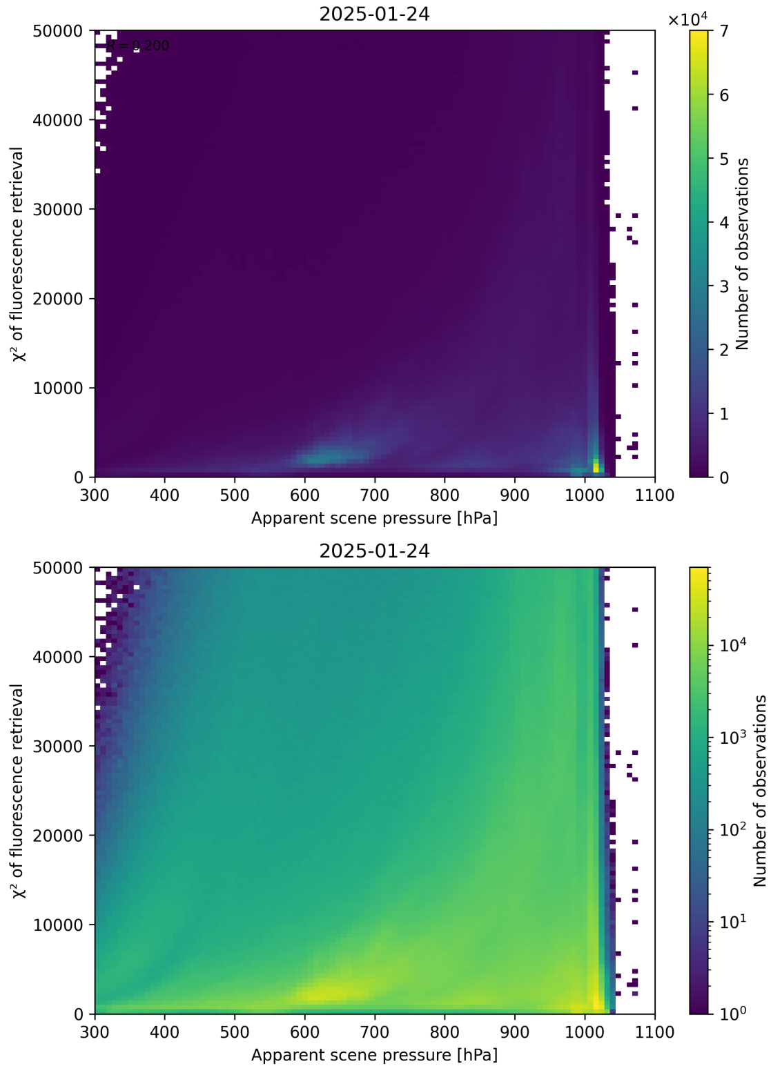
Figure 63: Scatter density plot of “Apparent scene pressure” against “ \chi^2 of fluorescence retrieval” for 2025-01-23 to 2025-01-25.
