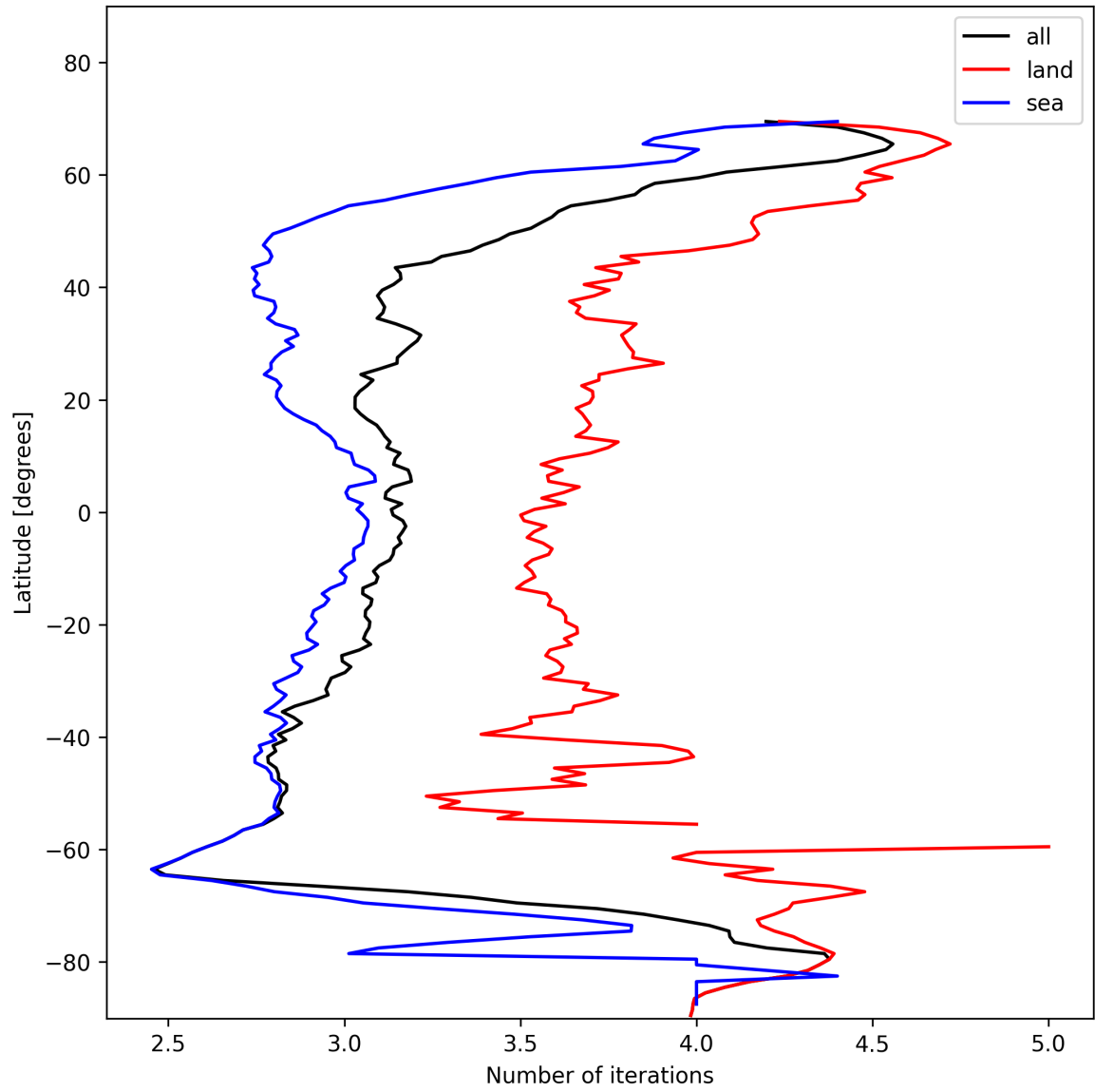
Figure 22: Zonal average of “Number of iterations” for 2025-01-23 to 2025-01-25.
