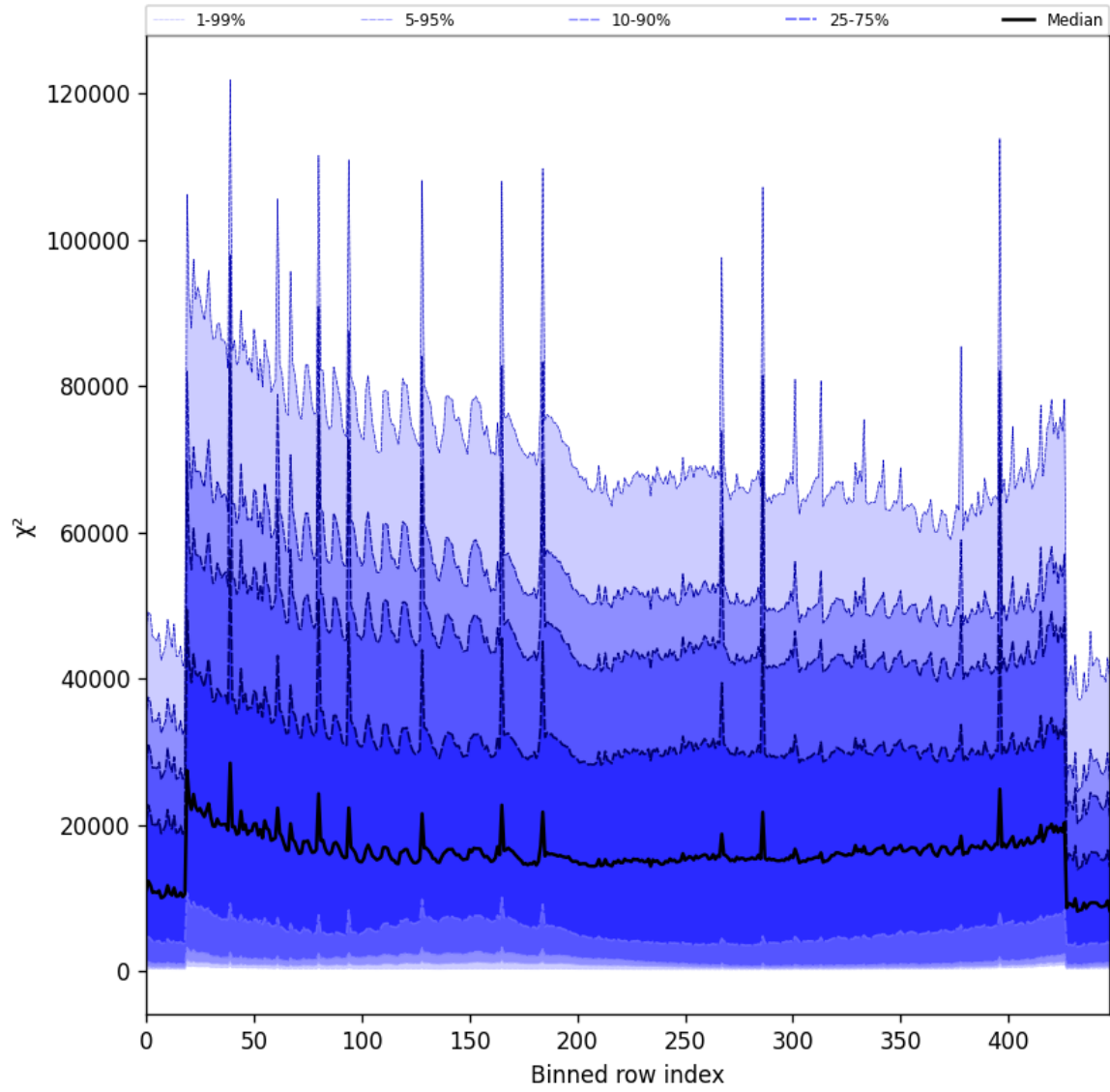
Figure 55: Along track statistics of “ \chi^2 ” for 2025-01-23 to 2025-01-25
