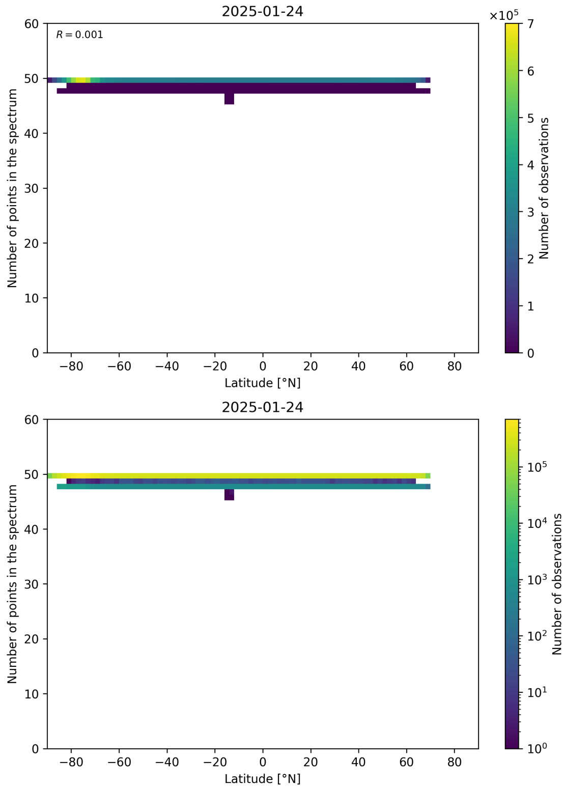
Figure 94: Scatter density plot of “Latitude” against “Number of points in the spectrum” for 2025-01-23 to 2025-01-25.
