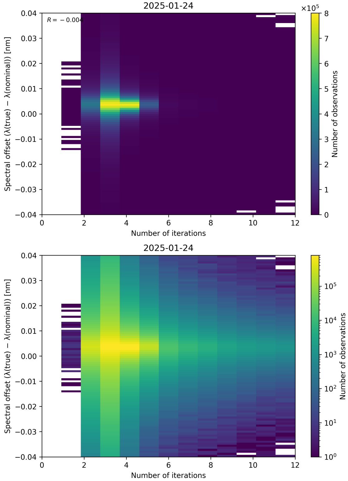
Figure 100: Scatter density plot of “Number of iterations” against “Spectral offset ( \lambda_{\text{true}} - \lambda_{\text{nominal}} )” for 2025-01-23 to 2025-01-25.
