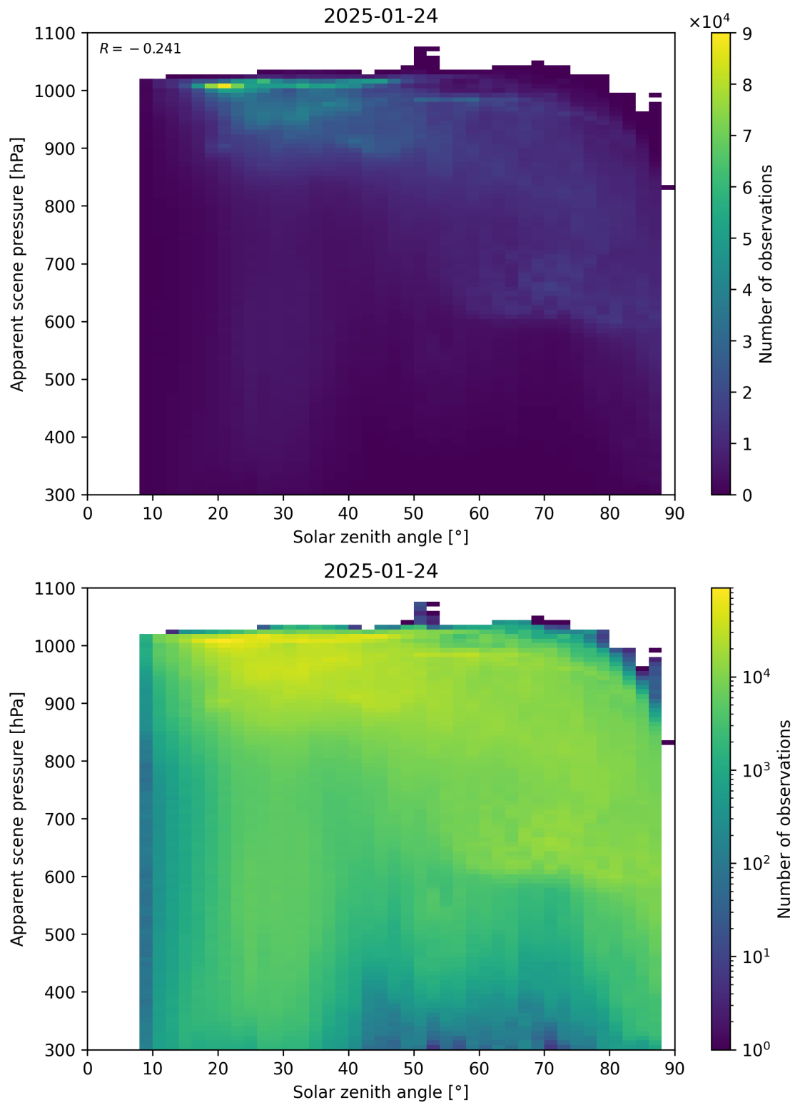
Figure 108: Scatter density plot of “Solar zenith angle” against “Apparent scene pressure” for 2025-01-23 to 2025-01-25.
