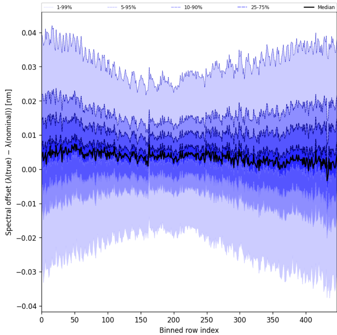
Figure 62: Along track statistics of “Spectral offset ( \lambda_{\text{true}} - \lambda_{\text{nominal}} )” for 2025-01-23 to 2025-01-25
