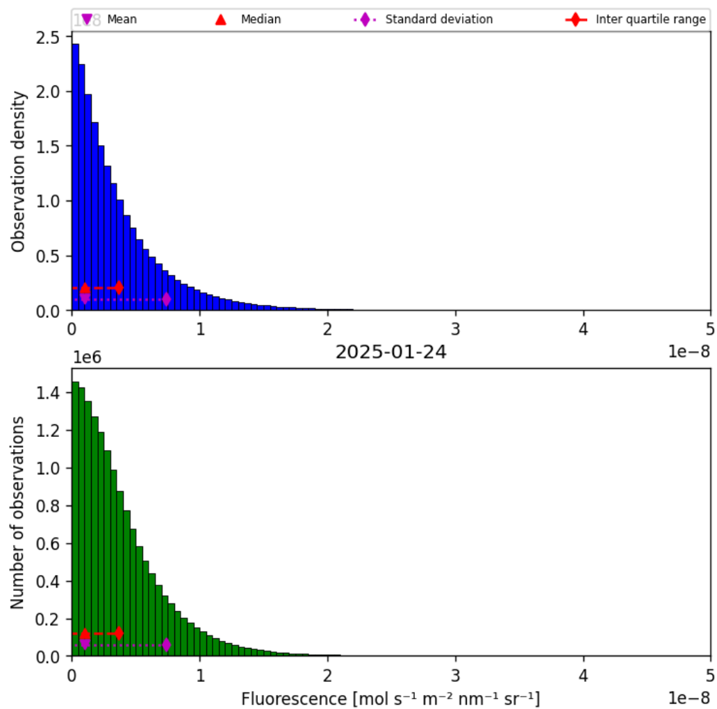
Figure 40: Histogram of “Fluorescence” for 2025-01-23 to 2025-01-25
