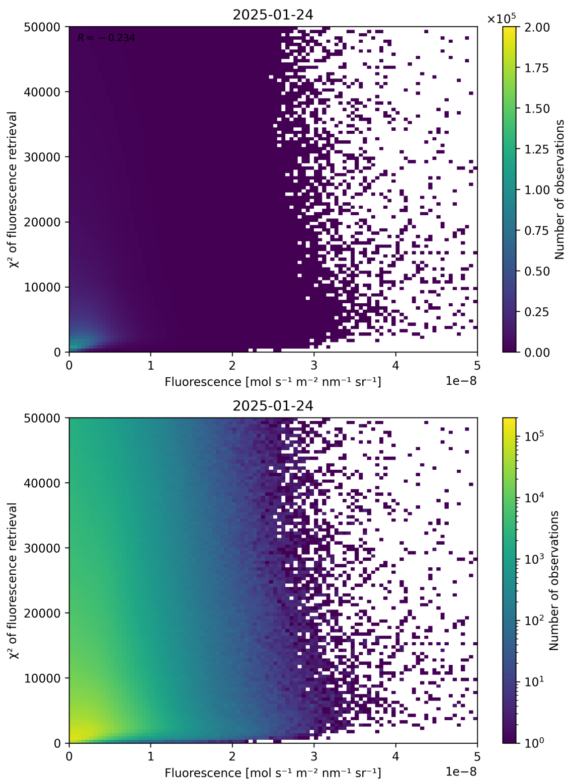
Figure 85: Scatter density plot of “Fluorescence” against “ \chi^2 of fluorescence retrieval” for 2025-01-23 to 2025-01-25.
