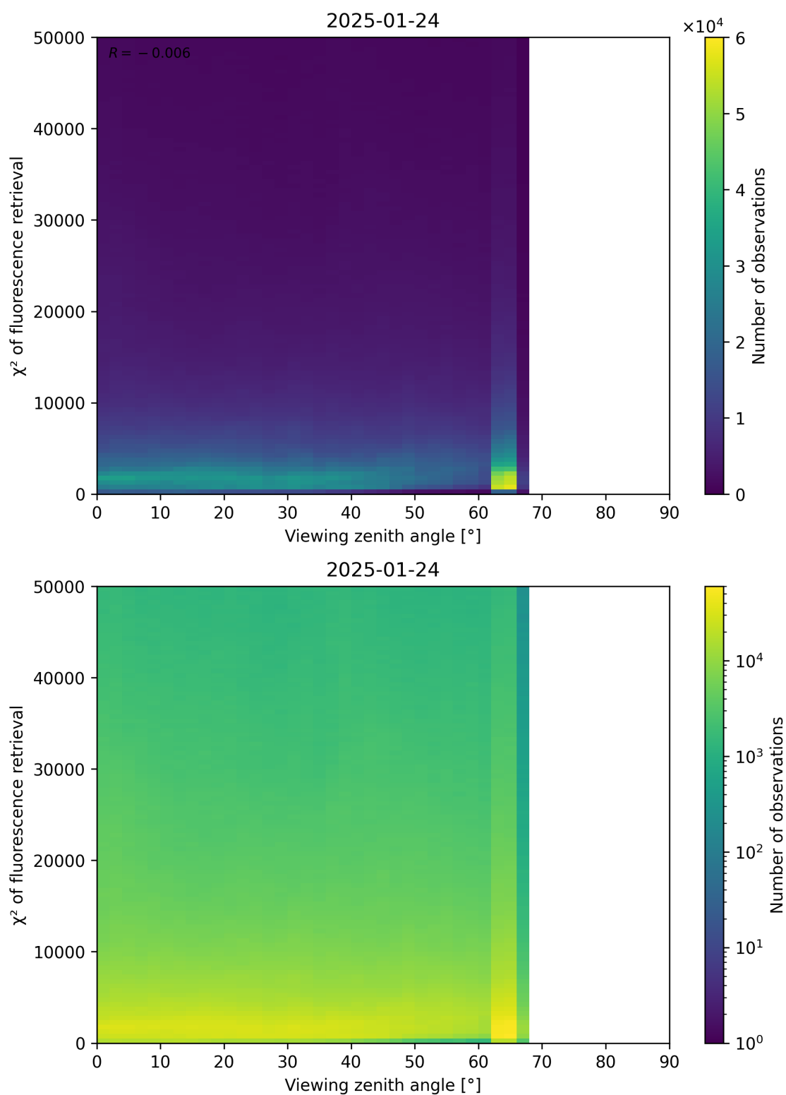
Figure 119: Scatter density plot of “Viewing zenith angle” against “ \chi^2 of fluorescence retrieval” for 2025-01-23 to 2025-01-25.
