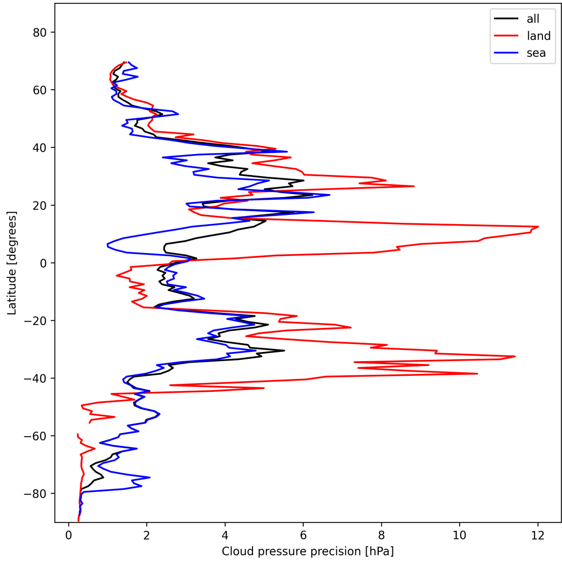
Figure 14: Zonal average of “Cloud pressure precision” for 2025-01-23 to 2025-01-25.
