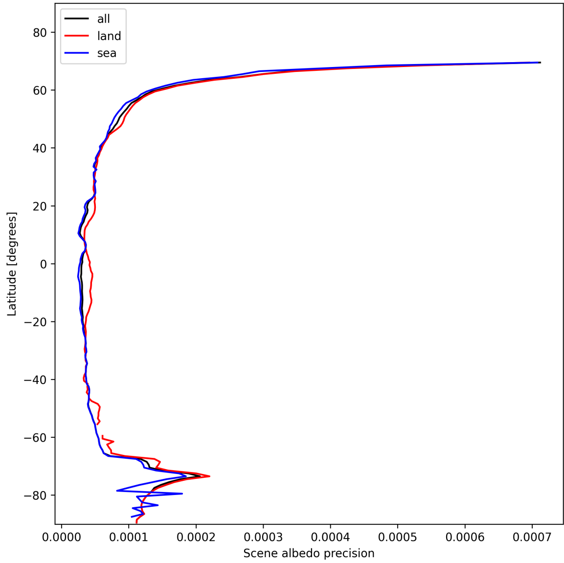
Figure 18: Zonal average of “Scene albedo precision” for 2025-01-23 to 2025-01-25.
