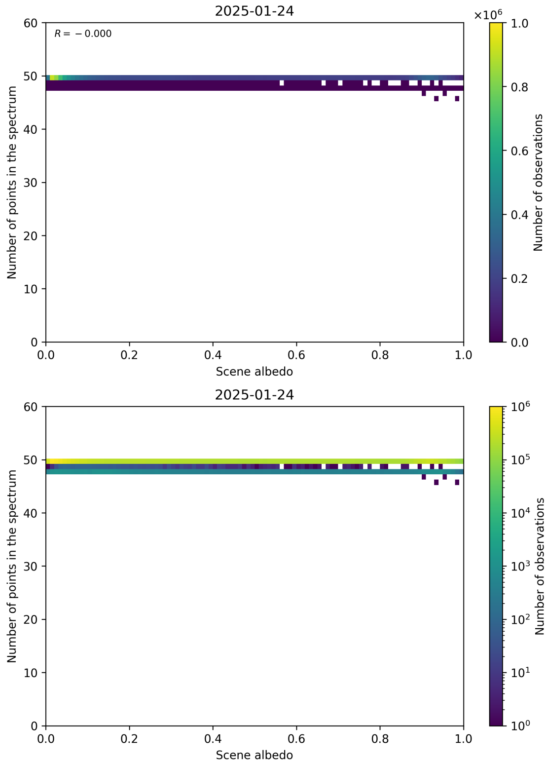
Figure 106: Scatter density plot of “Scene albedo” against “Number of points in the spectrum” for 2025-01-23 to 2025-01-25.
