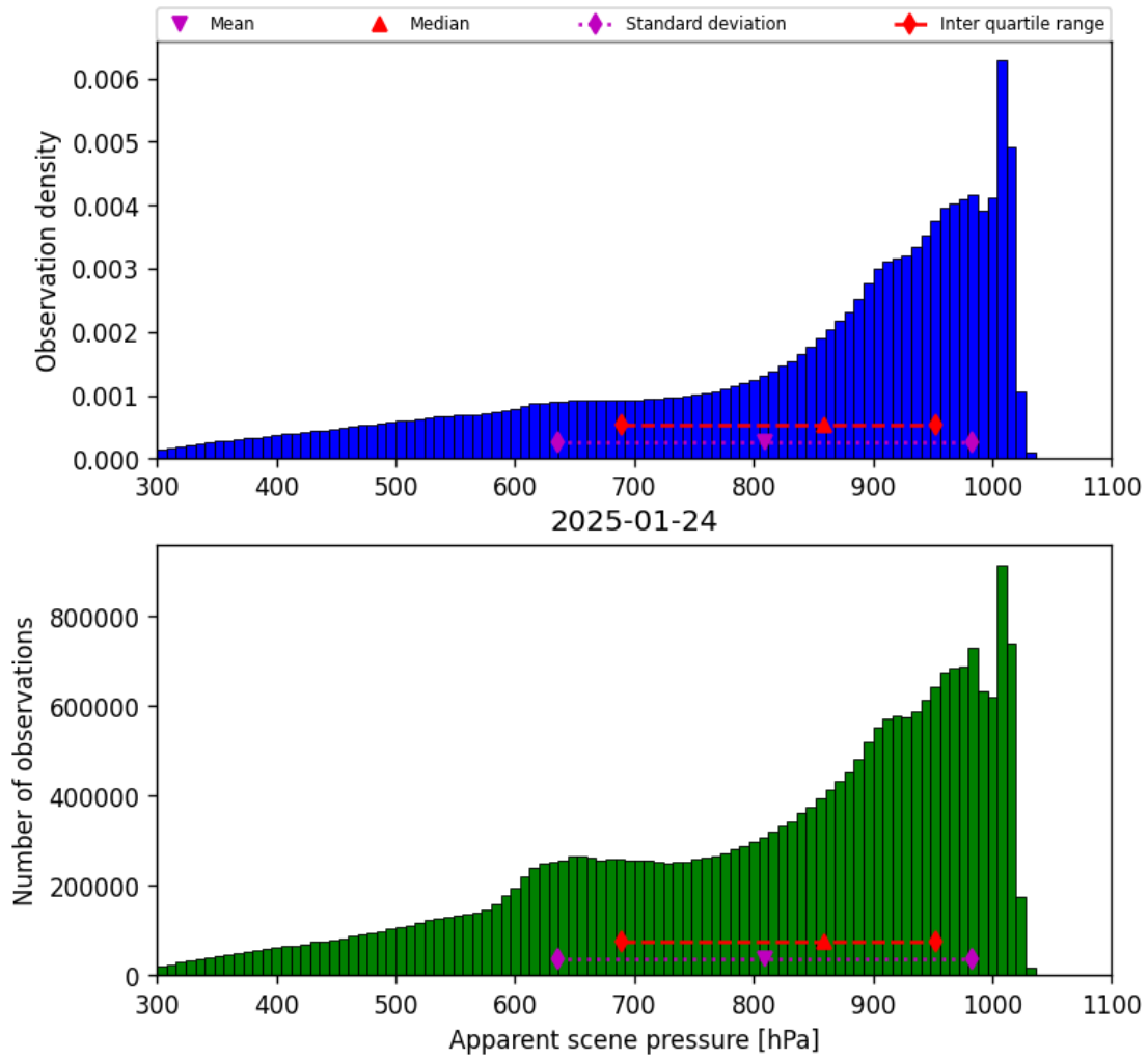
Figure 36: Histogram of “Apparent scene pressure” for 2025-01-23 to 2025-01-25
