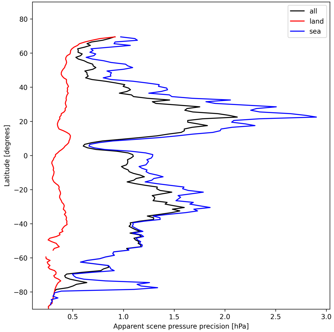
Figure 20: Zonal average of “Apparent scene pressure precision” for 2025-01-23 to 2025-01-25.
