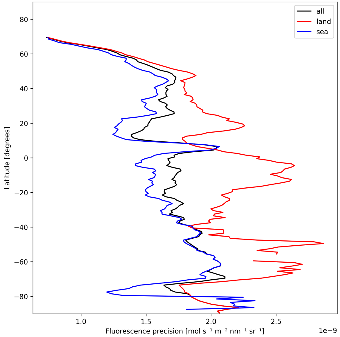
Figure 24: Zonal average of “Fluorescence precision” for 2025-01-23 to 2025-01-25.
