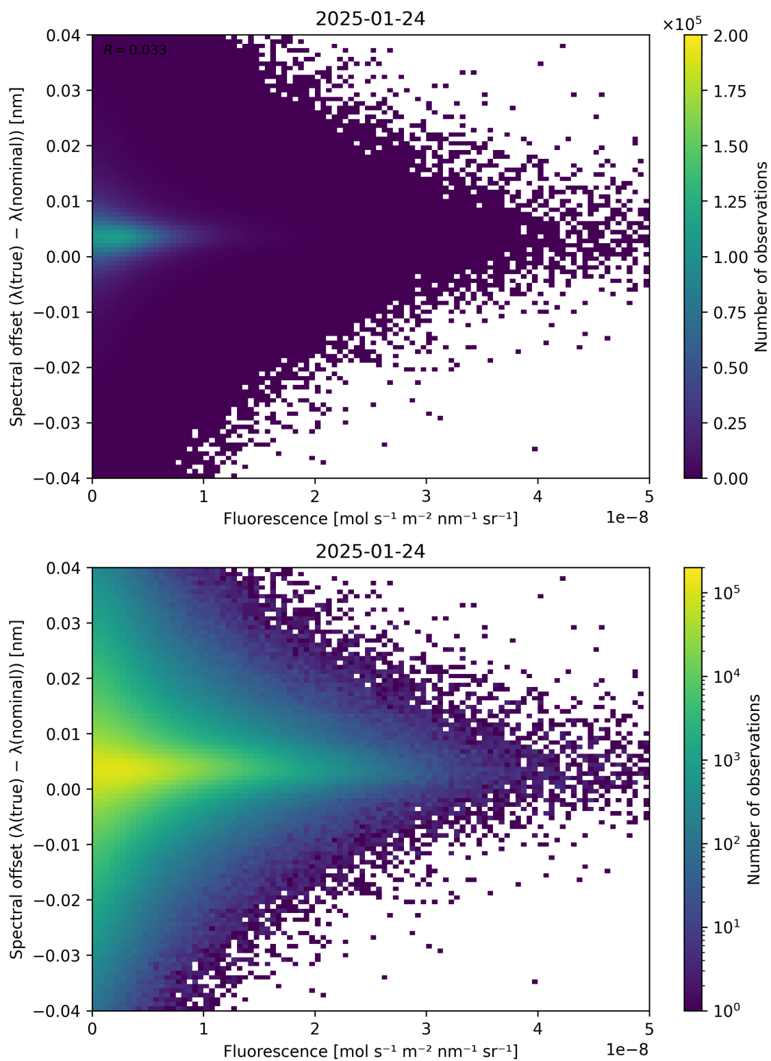
Figure 87: Scatter density plot of “Fluorescence” against “Spectral offset ( \lambda_{\text{true}} - \lambda_{\text{nominal}} )” for 2025-01-23 to 2025-01-25.
