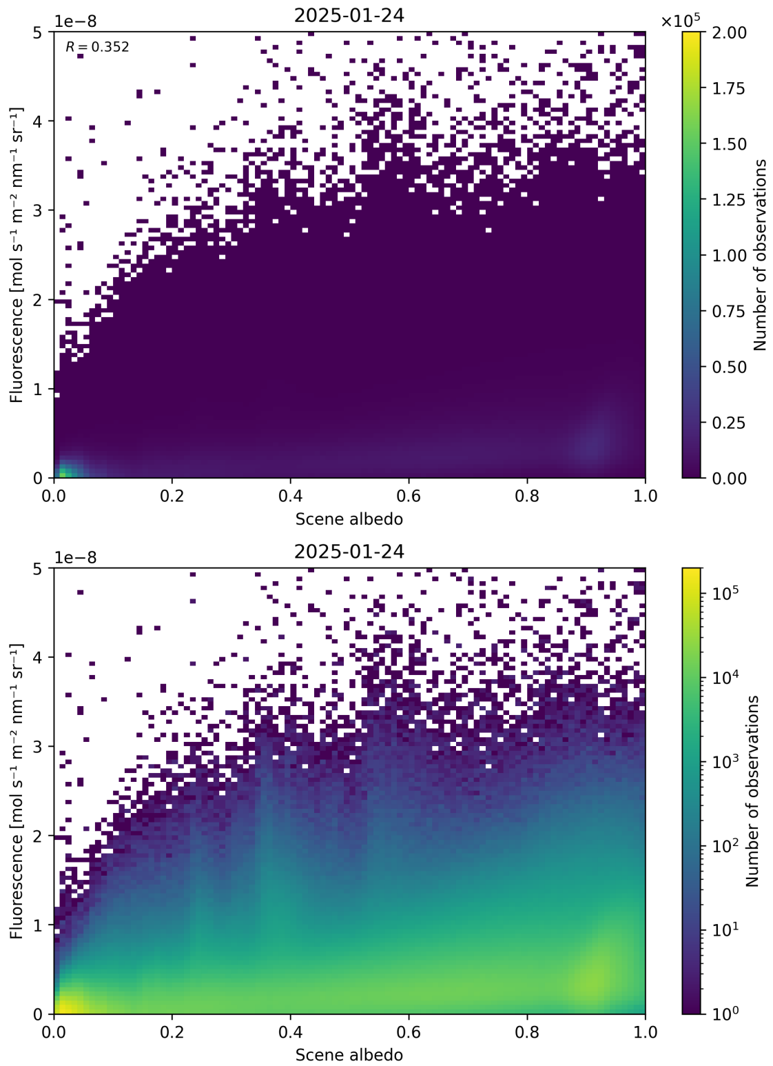
Figure 104: Scatter density plot of “Scene albedo” against “Fluorescence” for 2025-01-23 to 2025-01-25.
