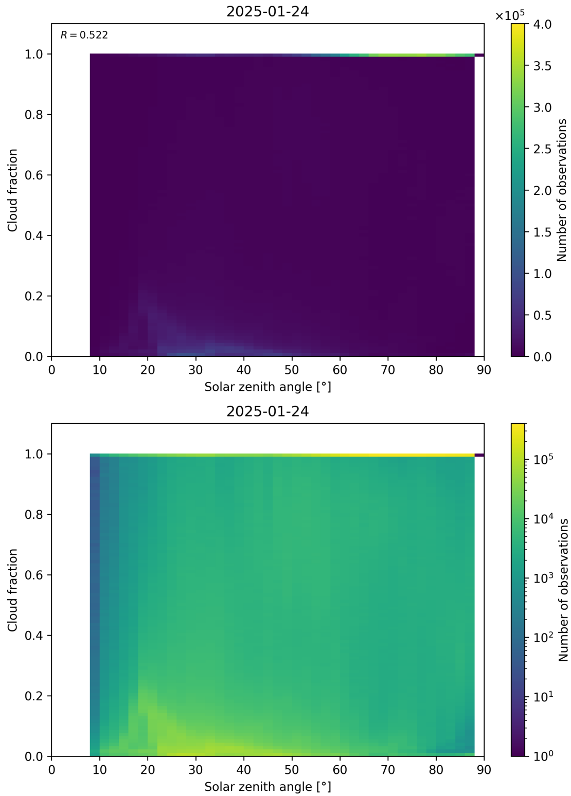
Figure 110: Scatter density plot of “Solar zenith angle” against “Cloud fraction” for 2025-01-23 to 2025-01-25.
