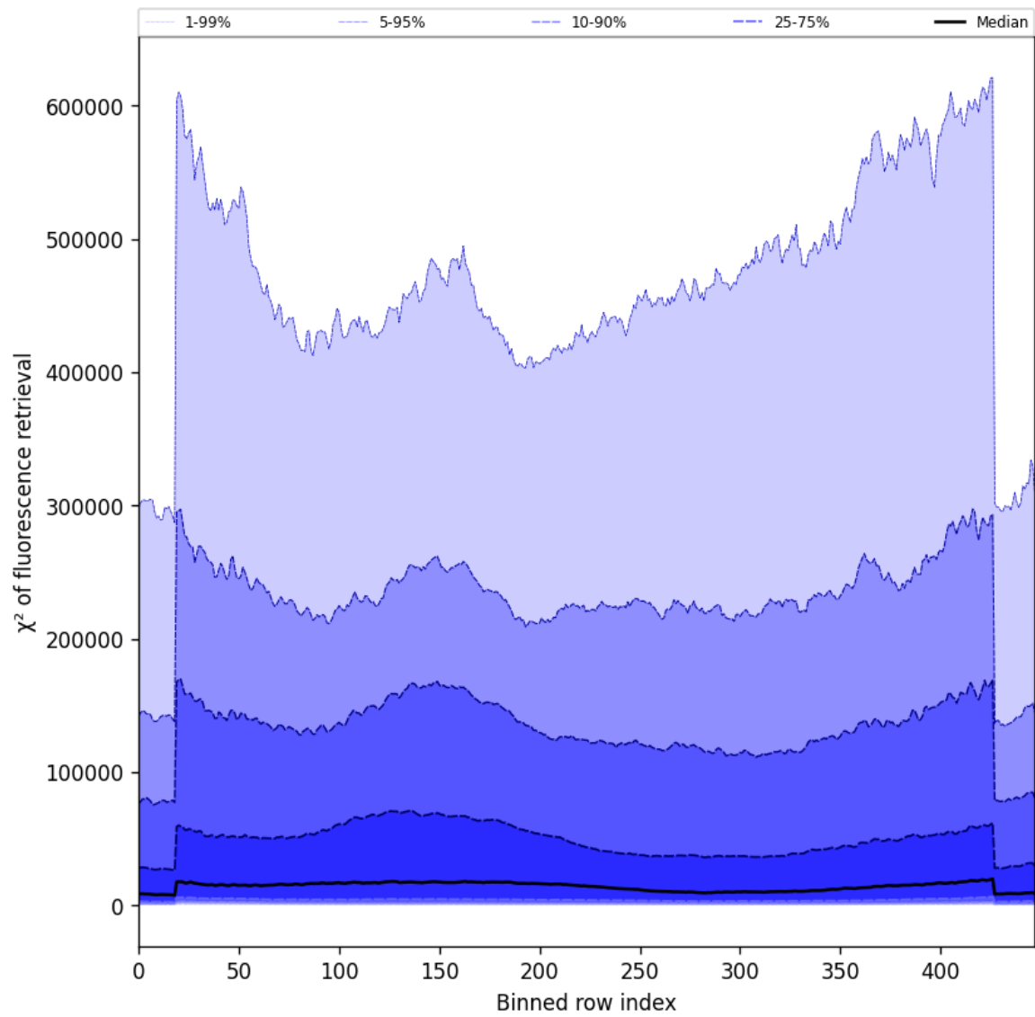
Figure 59: Along track statistics of “ \chi^2 of fluorescence retrieval” for 2025-01-23 to 2025-01-25
