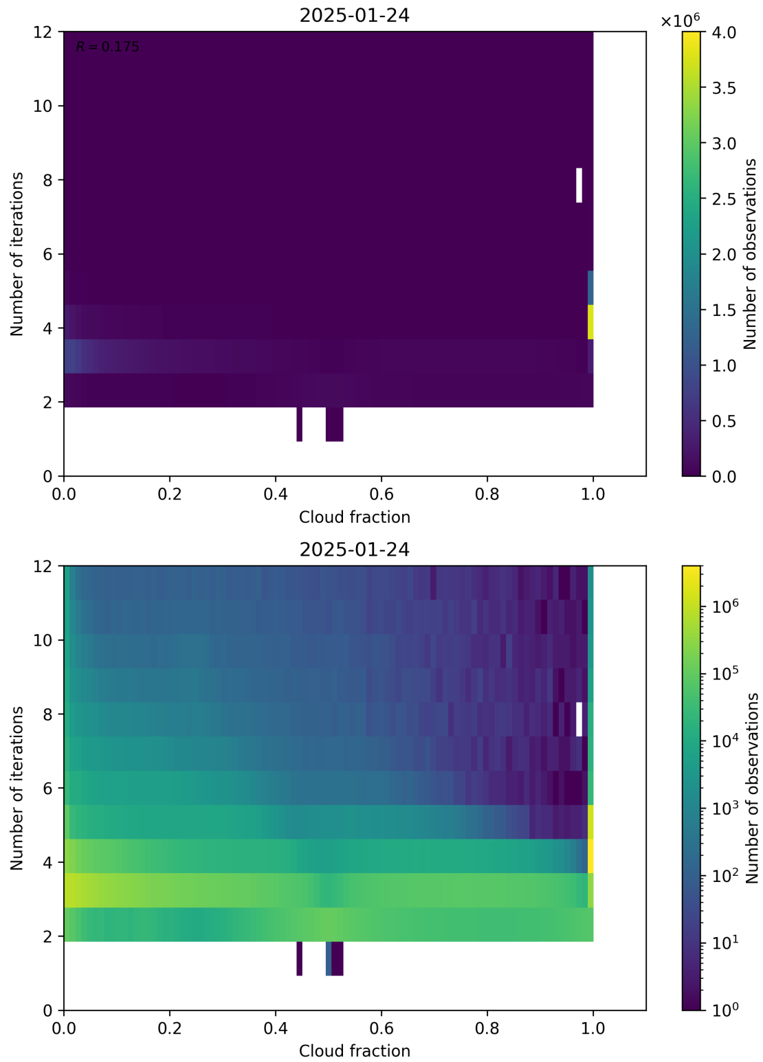
Figure 73: Scatter density plot of “Cloud fraction” against “Number of iterations” for 2025-01-23 to 2025-01-25.
