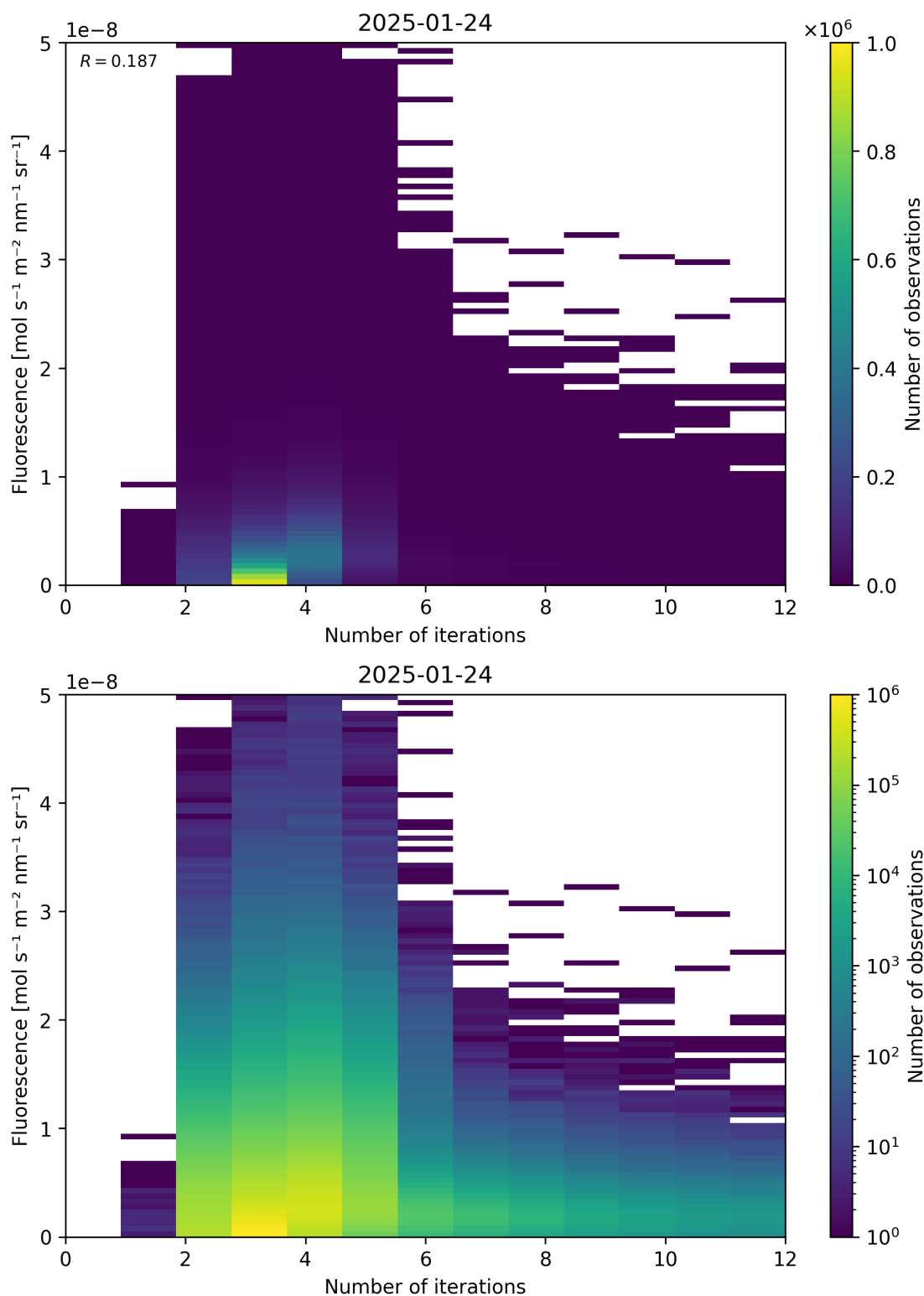
Figure 98: Scatter density plot of “Number of iterations” against “Fluorescence” for 2025-01-23 to 2025-01-25.
