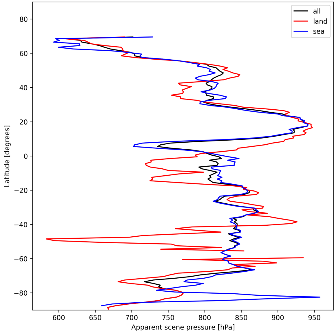
Figure 19: Zonal average of “Apparent scene pressure” for 2025-01-23 to 2025-01-25.
