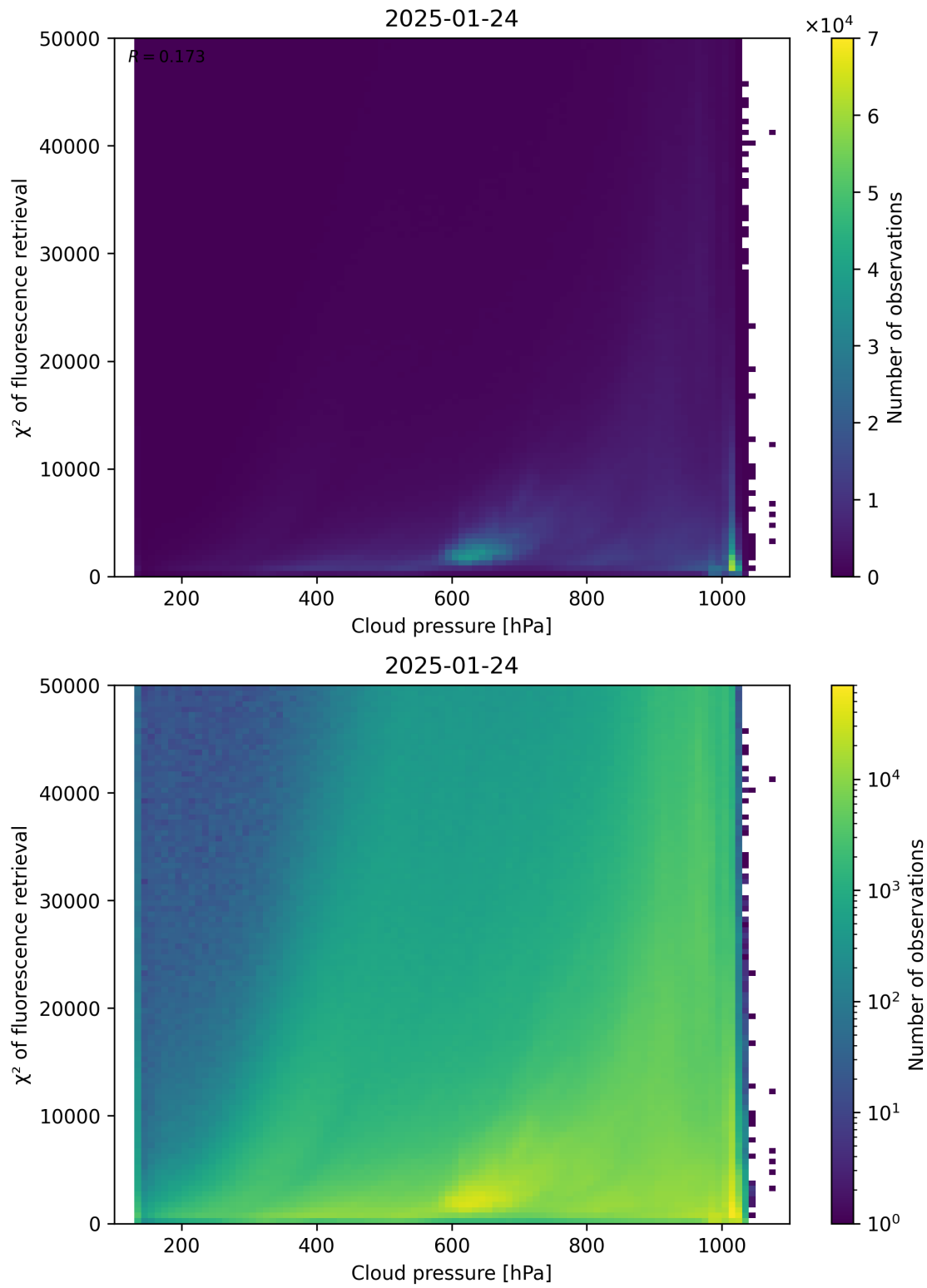
Figure 78: Scatter density plot of “Cloud pressure” against “ \chi^2 of fluorescence retrieval” for 2025-01-23 to 2025-01-25.
