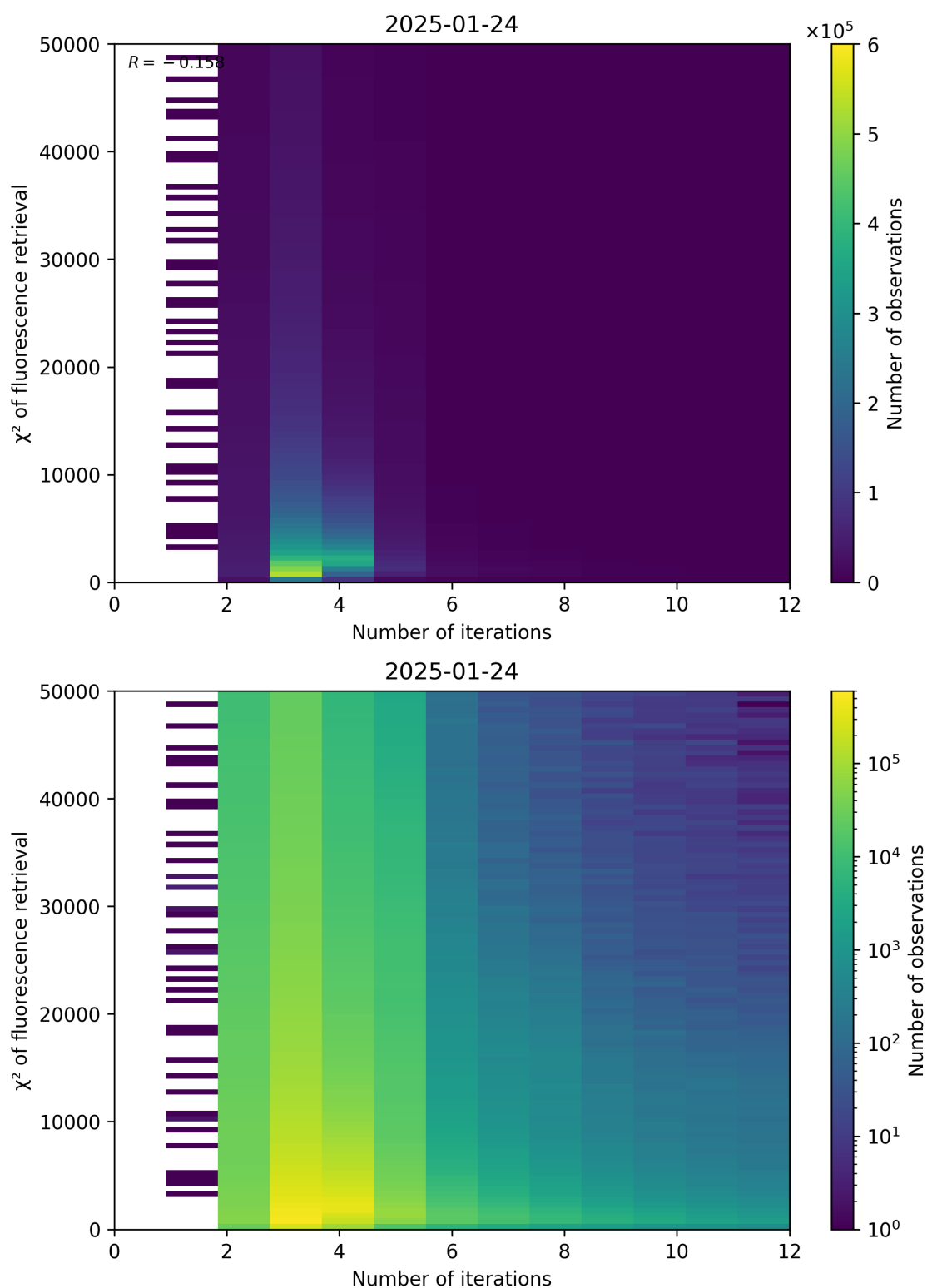
Figure 97: Scatter density plot of “Number of iterations” against “ \chi^2 of fluorescence retrieval” for 2025-01-23 to 2025-01-25.
