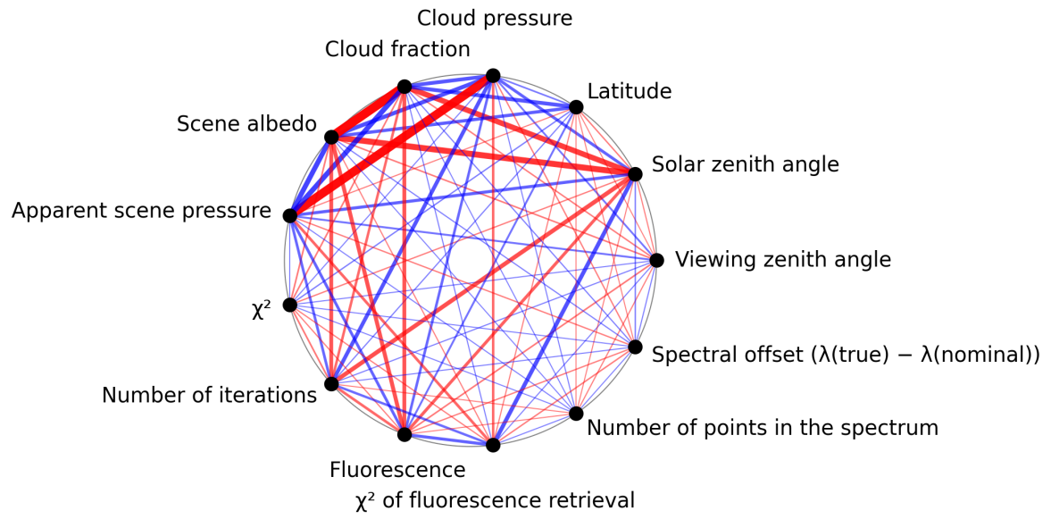
Figure 1: Map of correlation graph for 2025-01-23 to 2025-01-25.
