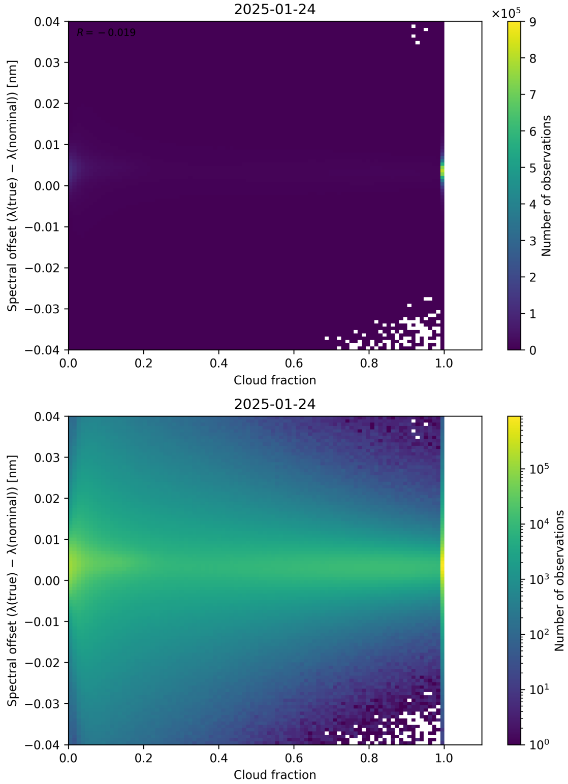
Figure 76: Scatter density plot of “Cloud fraction” against “Spectral offset ( \lambda_{\text{true}} - \lambda_{\text{nominal}} )” for 2025-01-23 to 2025-01-25.
