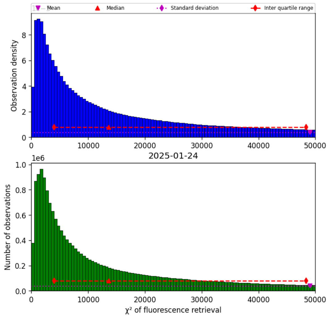
Figure 42: Histogram of “ \chi^2 of fluorescence retrieval” for 2025-01-23 to 2025-01-25
