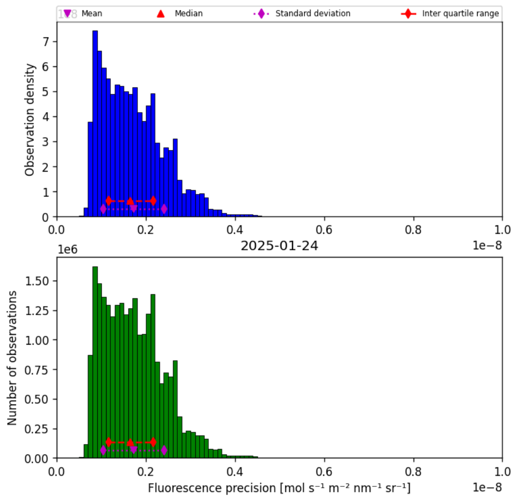
Figure 41: Histogram of “Fluorescence precision” for 2025-01-23 to 2025-01-25
