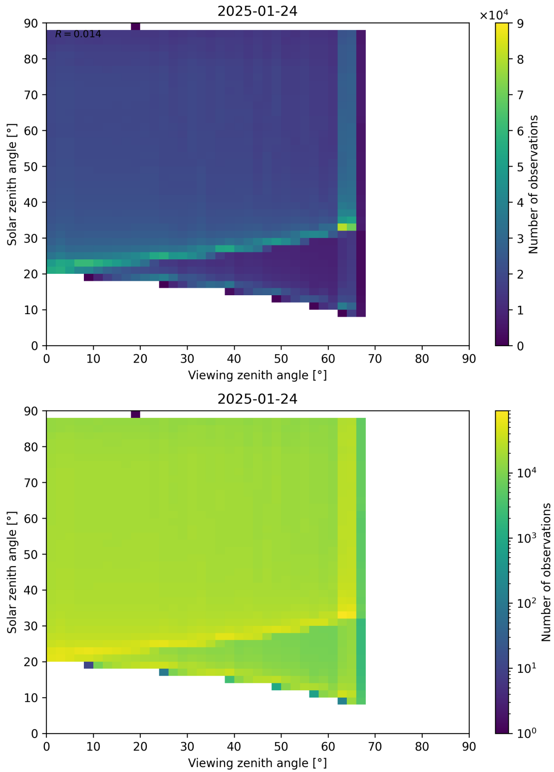
Figure 127: Scatter density plot of “Viewing zenith angle” against “Solar zenith angle” for 2025-01-23 to 2025-01-25.
