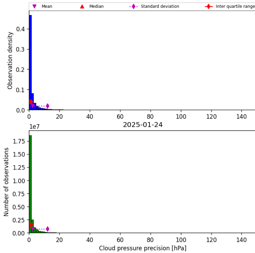
Figure 31: Histogram of “Cloud pressure precision” for 2025-01-23 to 2025-01-25
