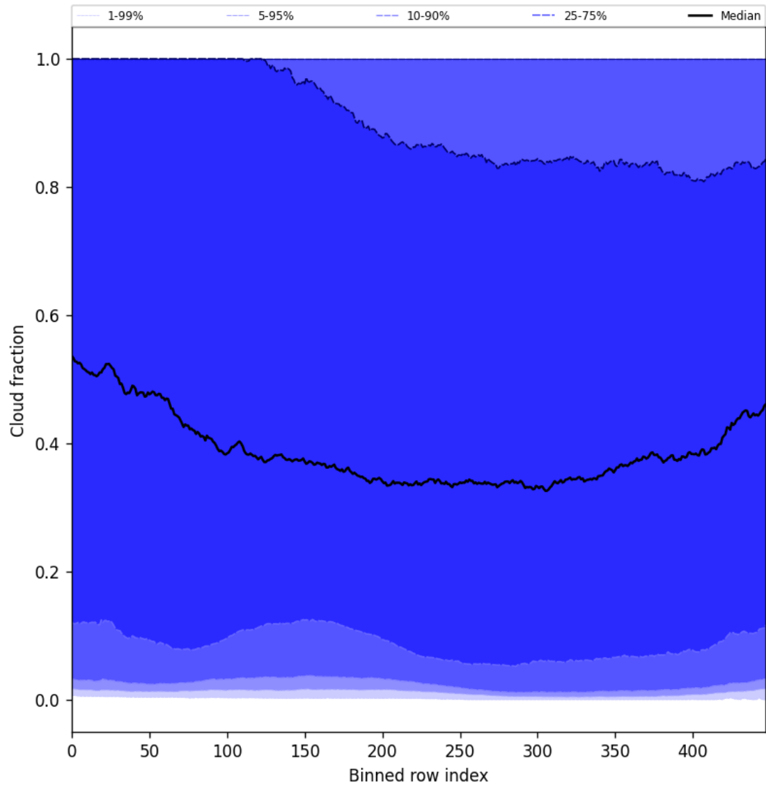
Figure 49: Along track statistics of “Cloud fraction” for 2025-01-23 to 2025-01-25
