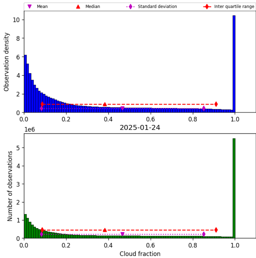
Figure 32: Histogram of “Cloud fraction” for 2025-01-23 to 2025-01-25
