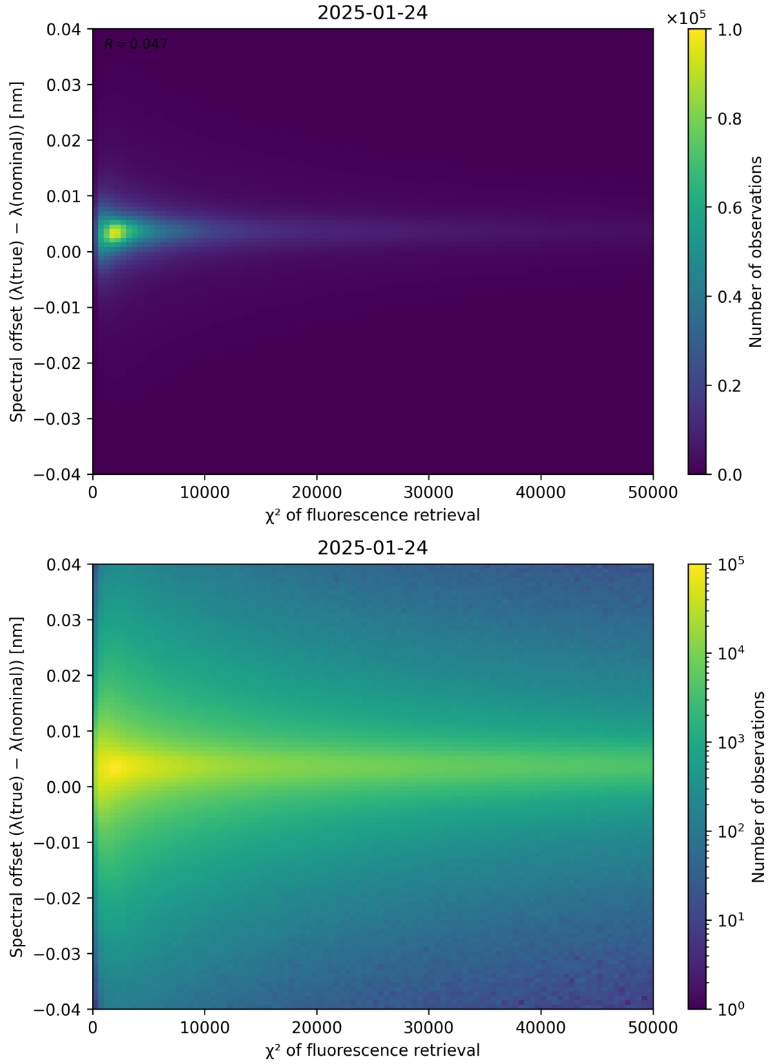
Figure 69: Scatter density plot of “ \chi^2 of fluorescence retrieval” against “Spectral offset ( \lambda_{\text{true}} - \lambda_{\text{nominal}} )” for 2025-01-23 to 2025-01-25.
