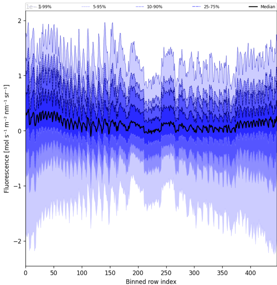
Figure 57: Along track statistics of “Fluorescence” for 2025-01-23 to 2025-01-25
