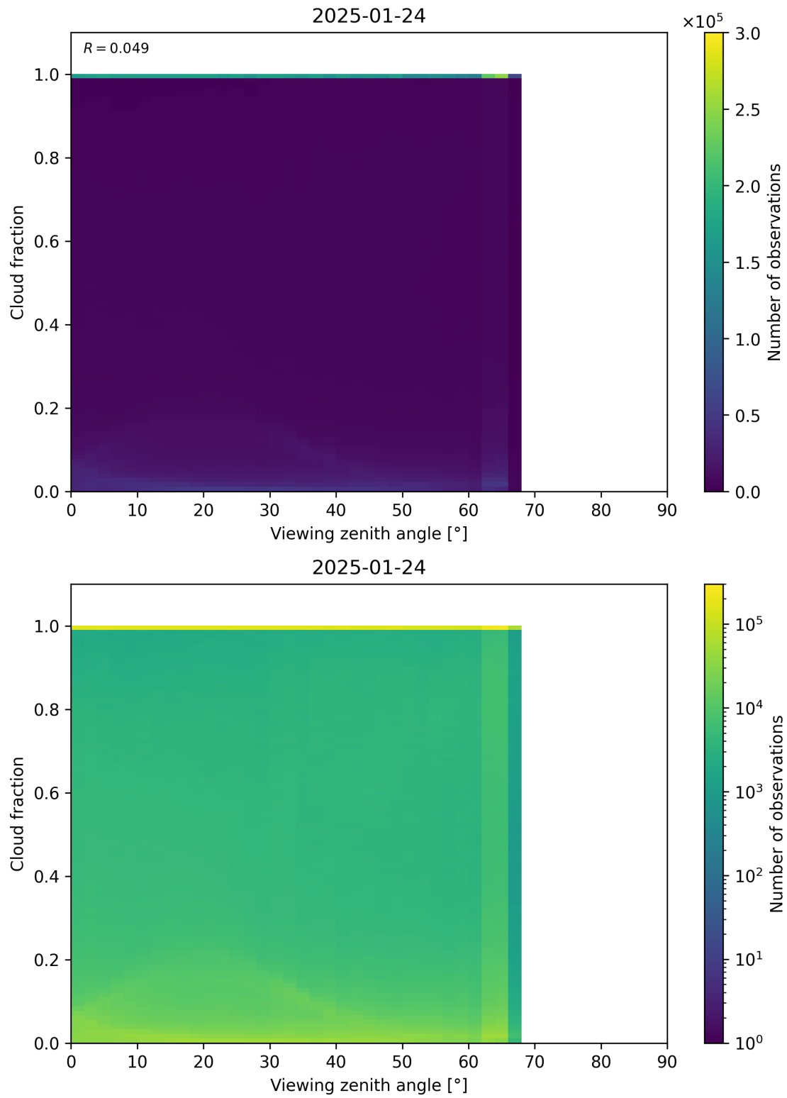
Figure 120: Scatter density plot of “Viewing zenith angle” against “Cloud fraction” for 2025-01-23 to 2025-01-25.
