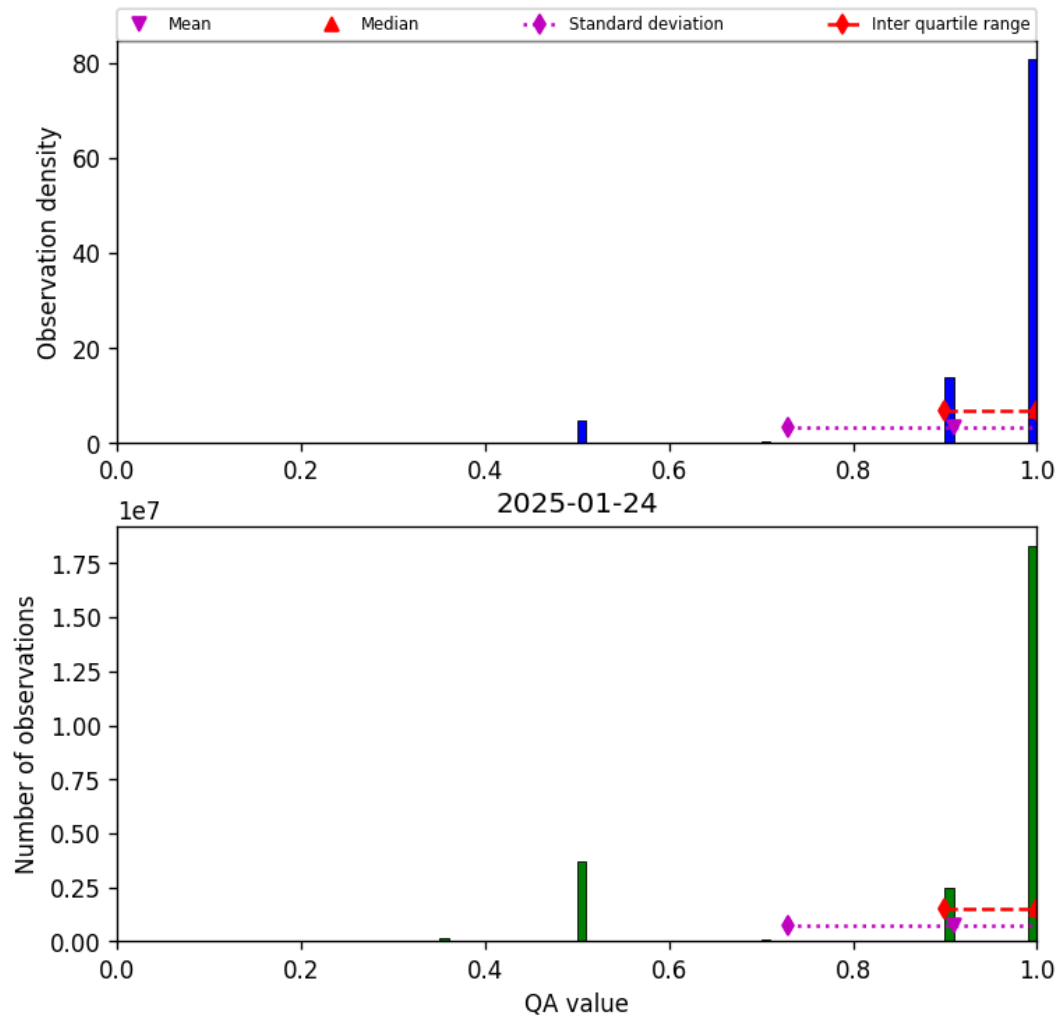
Figure 29: Histogram of “QA value” for 2025-01-23 to 2025-01-25
