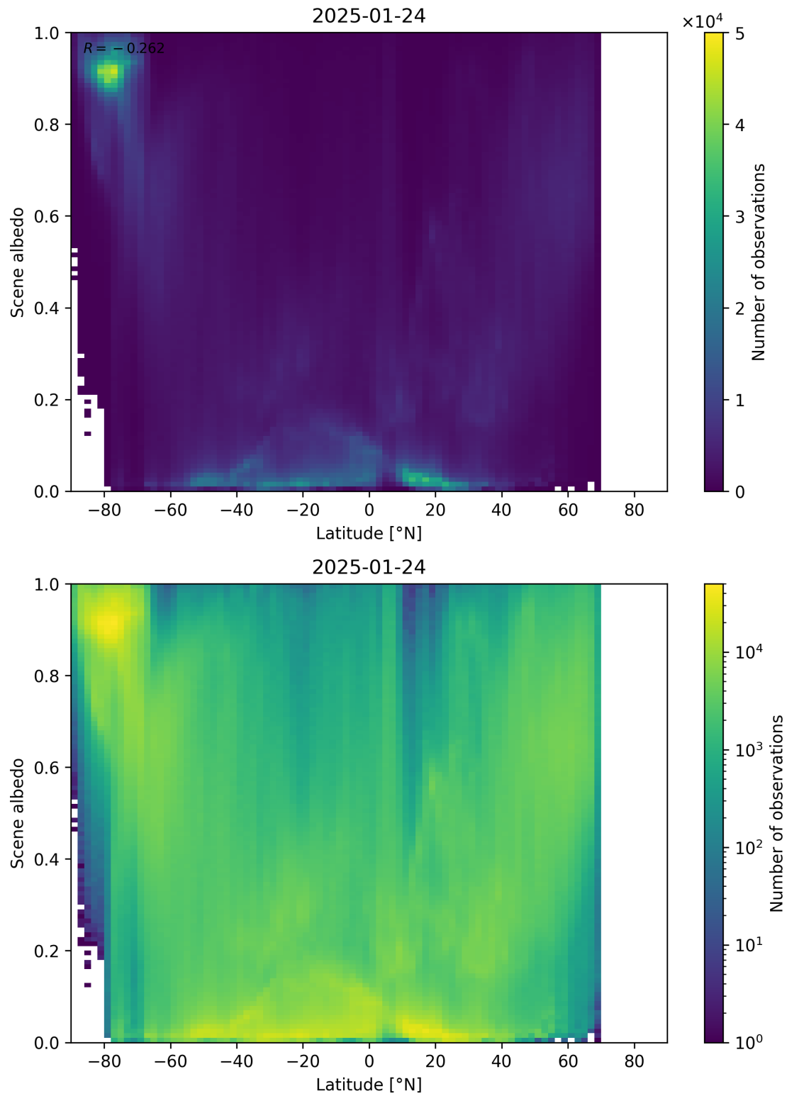
Figure 95: Scatter density plot of “Latitude” against “Scene albedo” for 2025-01-23 to 2025-01-25.
