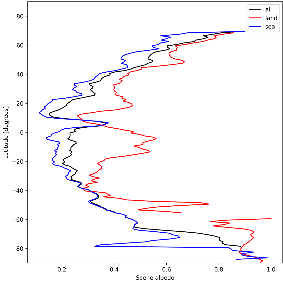
Figure 17: Zonal average of “Scene albedo” for 2025-01-23 to 2025-01-25.
