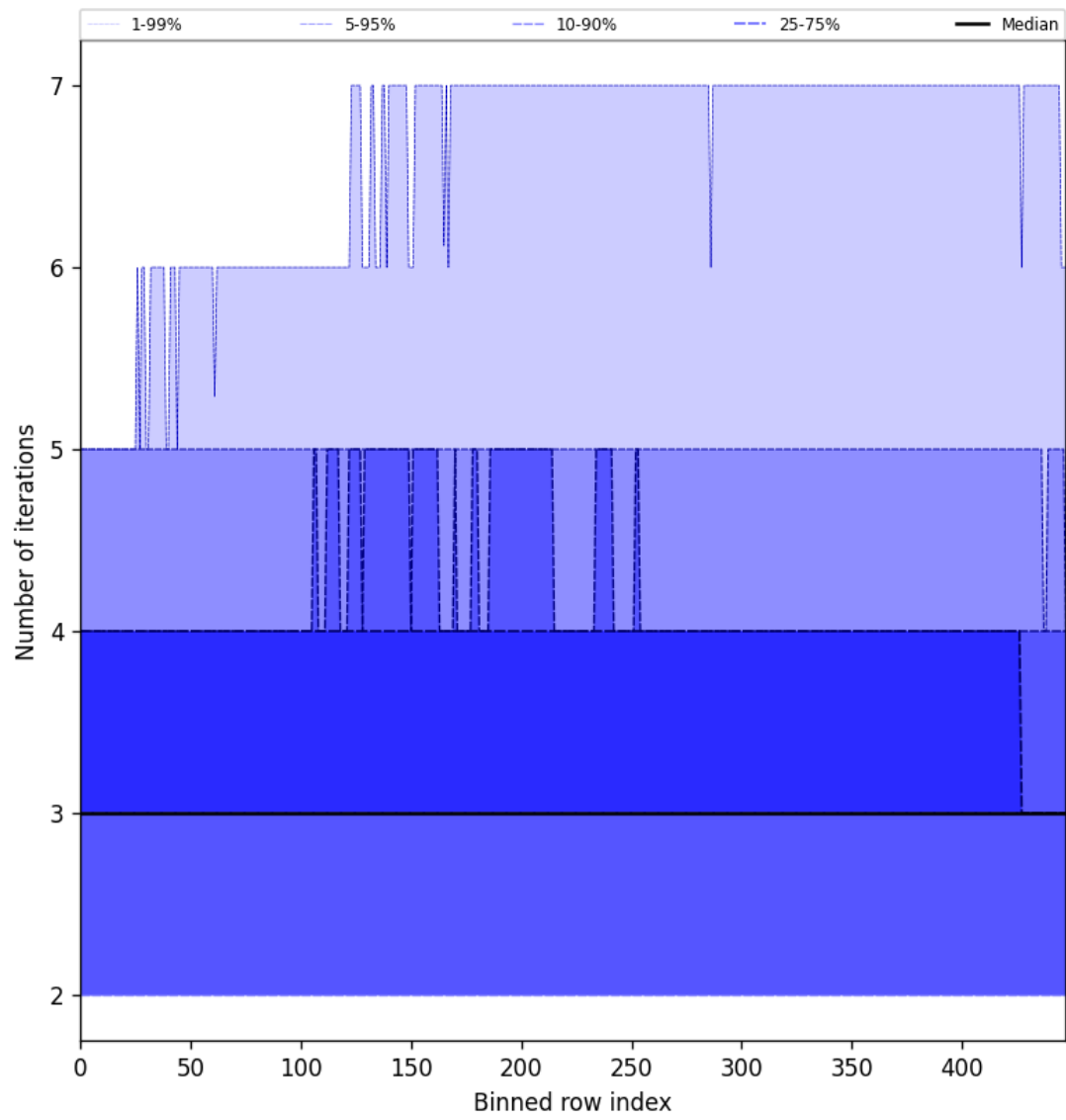
Figure 56: Along track statistics of “Number of iterations” for 2025-01-23 to 2025-01-25
