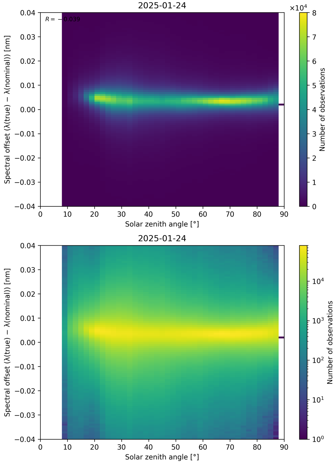
Figure 117: Scatter density plot of “Solar zenith angle” against “Spectral offset ( \lambda_{\text{true}} - \lambda_{\text{nominal}} )” for 2025-01-23 to 2025-01-25.
