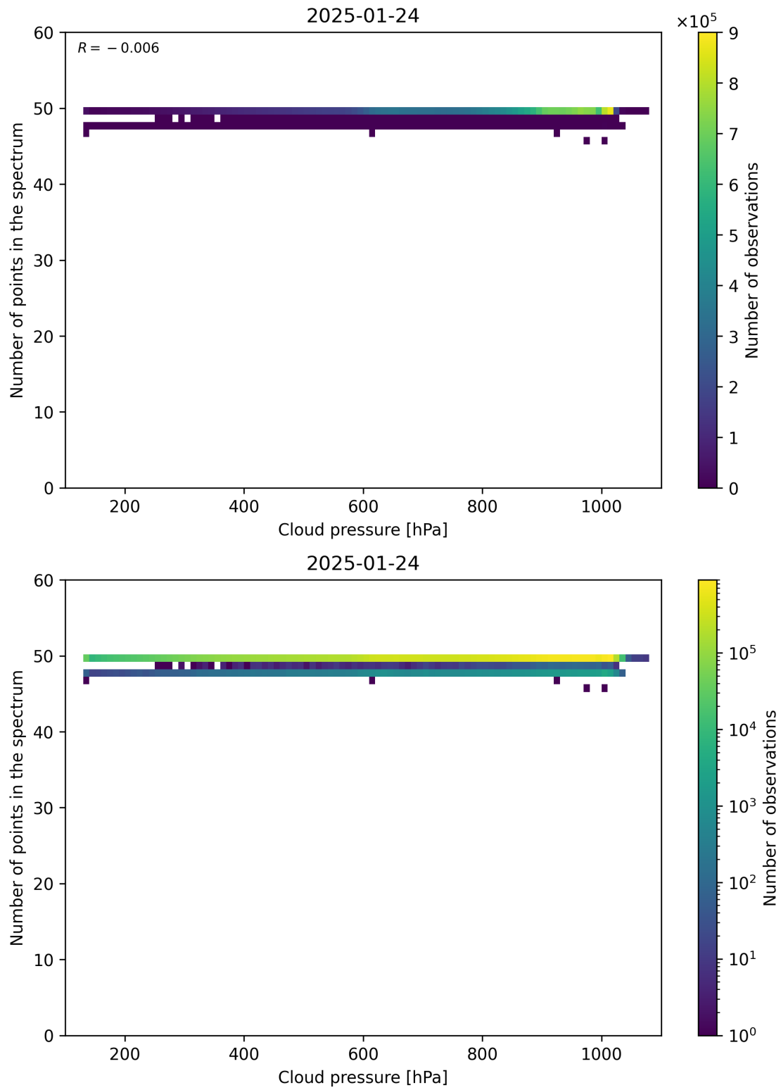
Figure 82: Scatter density plot of “Cloud pressure” against “Number of points in the spectrum” for 2025-01-23 to 2025-01-25.
