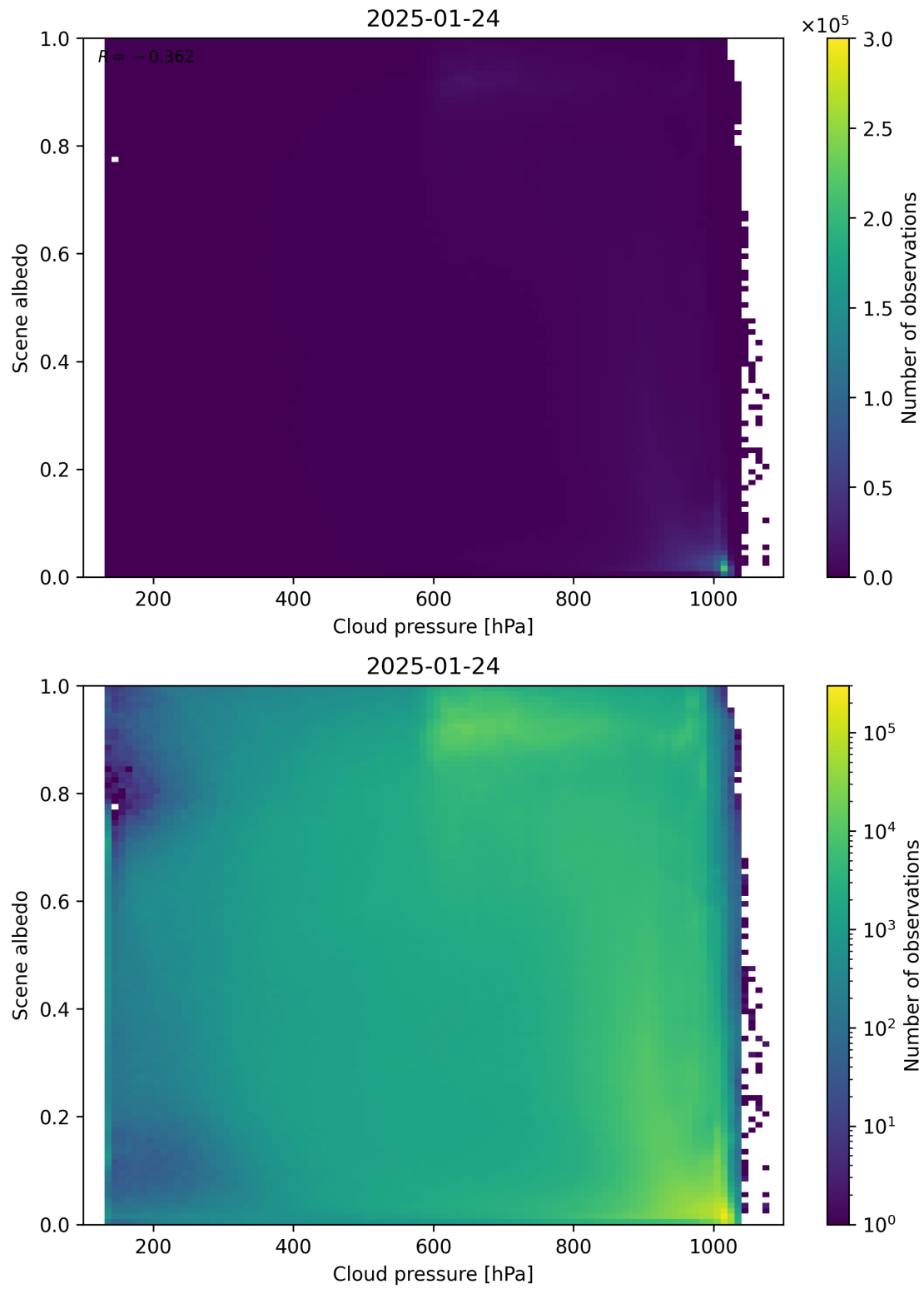
Figure 83: Scatter density plot of “Cloud pressure” against “Scene albedo” for 2025-01-23 to 2025-01-25.
