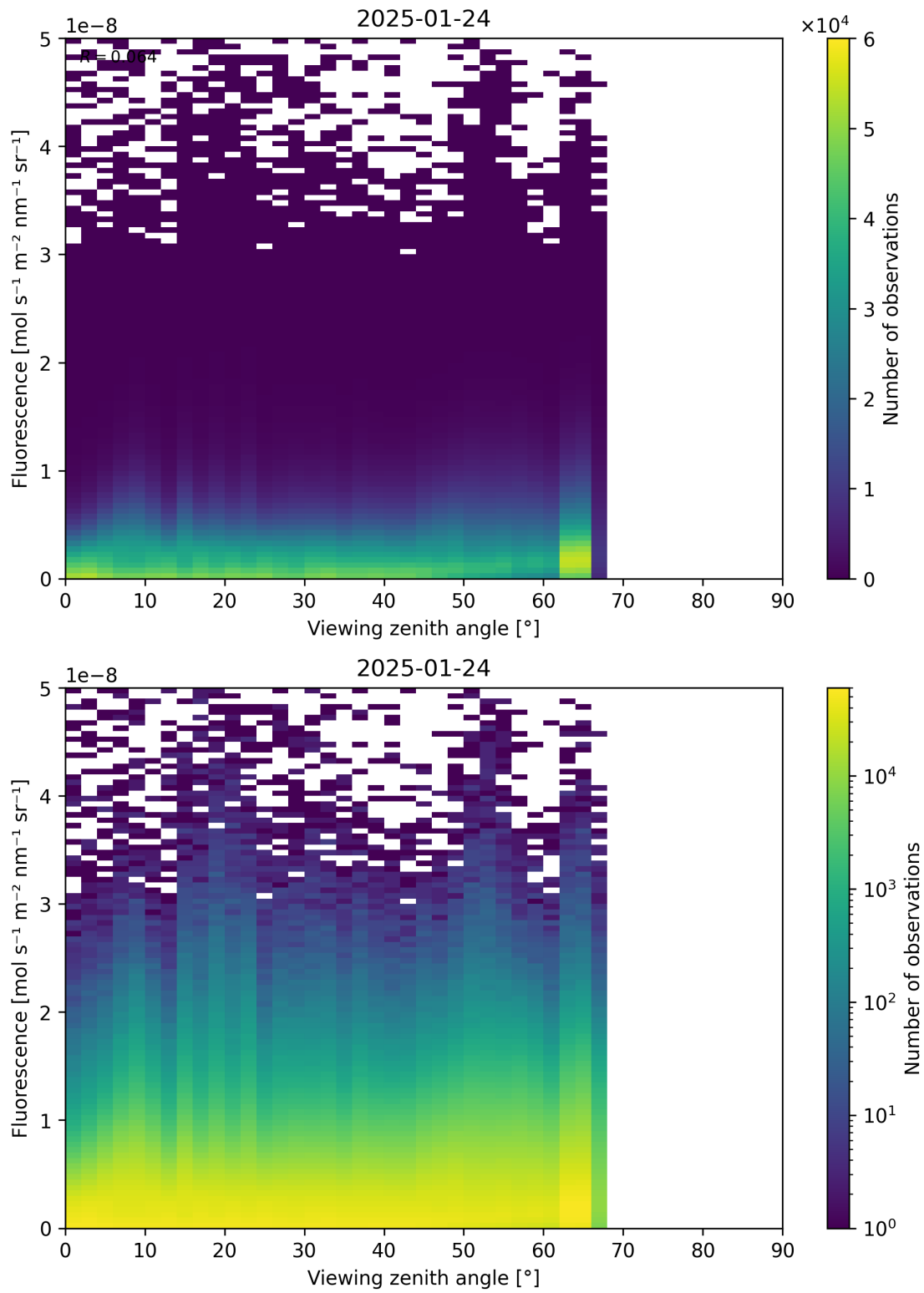
Figure 122: Scatter density plot of “Viewing zenith angle” against “Fluorescence” for 2025-01-23 to 2025-01-25.
