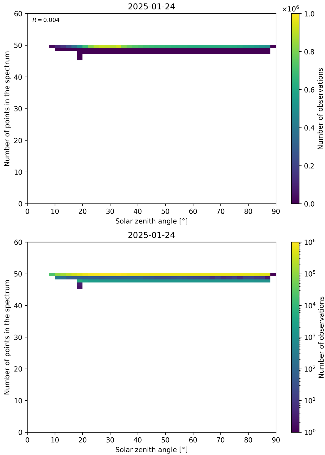
Figure 115: Scatter density plot of “Solar zenith angle” against “Number of points in the spectrum” for 2025-01-23 to 2025-01-25.
