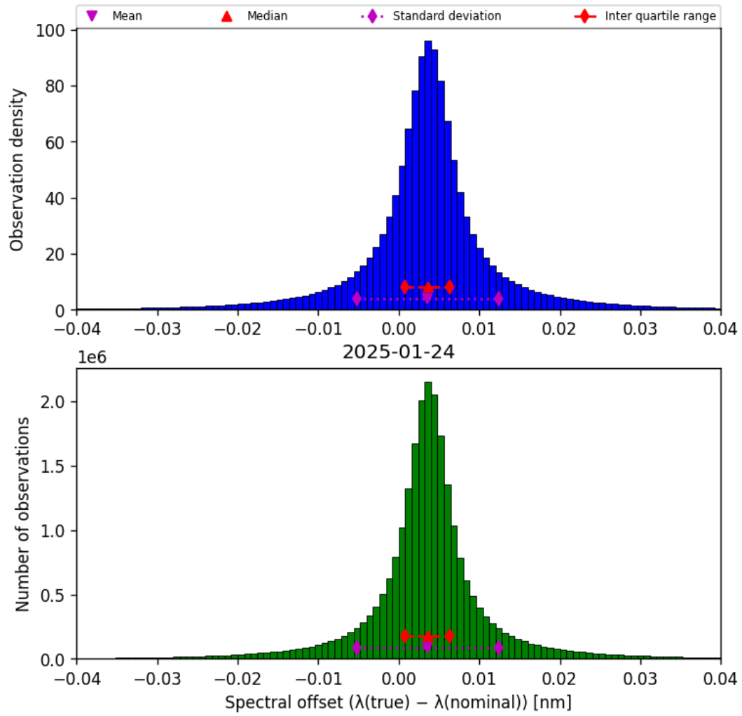
Figure 45: Histogram of “Spectral offset ( \lambda_{\text{true}} - \lambda_{\text{nominal}} )” for 2025-01-23 to 2025-01-25
