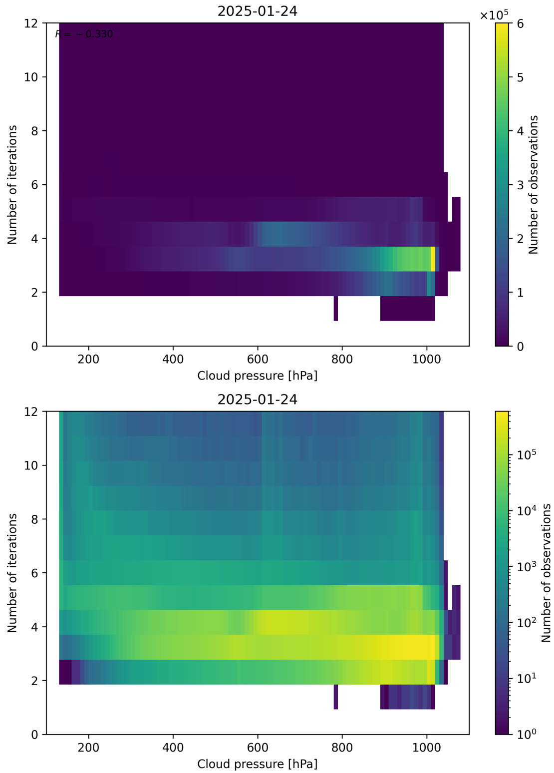
Figure 81: Scatter density plot of “Cloud pressure” against “Number of iterations” for 2025-01-23 to 2025-01-25.
