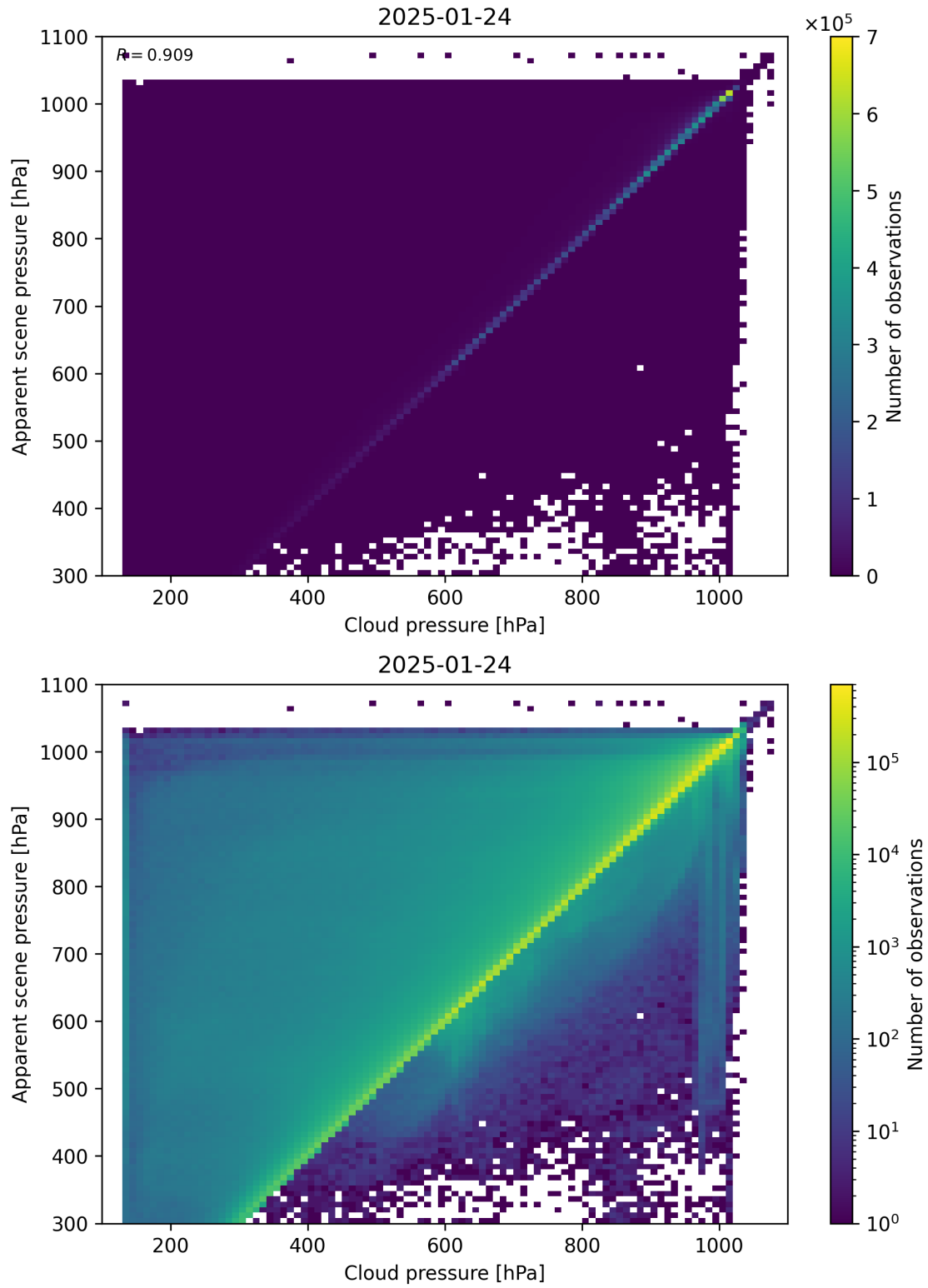
Figure 77: Scatter density plot of “Cloud pressure” against “Apparent scene pressure” for 2025-01-23 to 2025-01-25.
