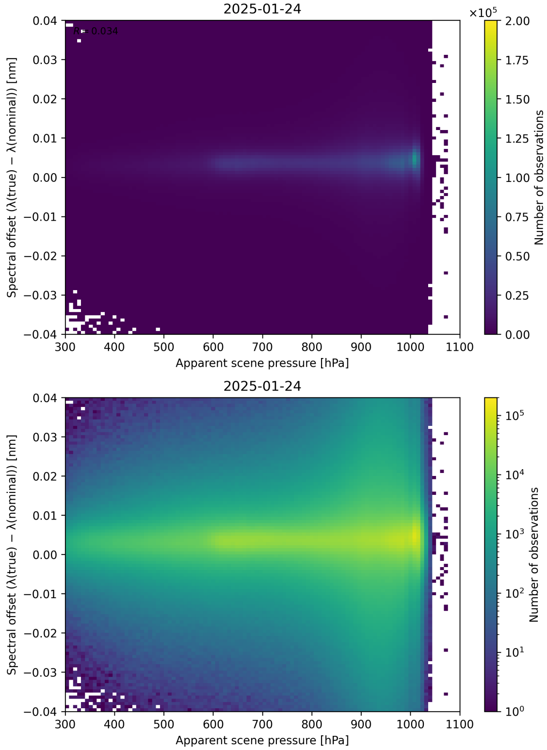
Figure 67: Scatter density plot of “Apparent scene pressure” against “Spectral offset ( \lambda_{\text{true}} - \lambda_{\text{nominal}} )” for 2025-01-23 to 2025-01-25.
