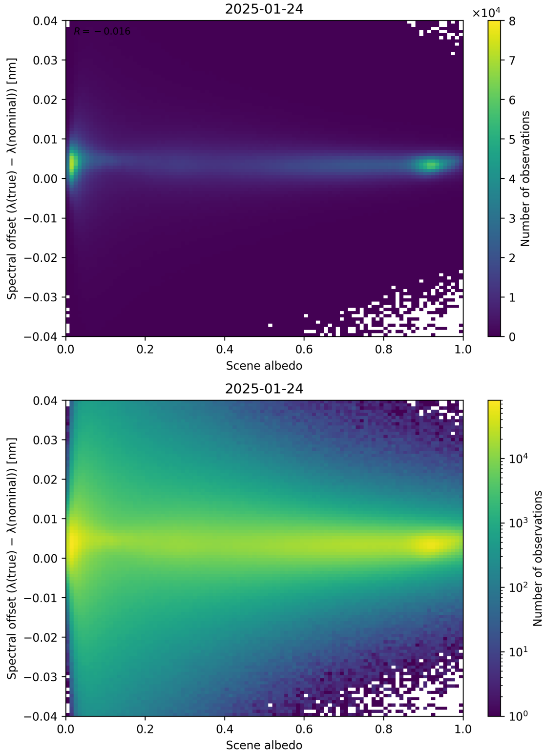
Figure 107: Scatter density plot of “Scene albedo” against “Spectral offset ( \lambda_{\text{true}} - \lambda_{\text{nominal}} )” for 2025-01-23 to 2025-01-25.
