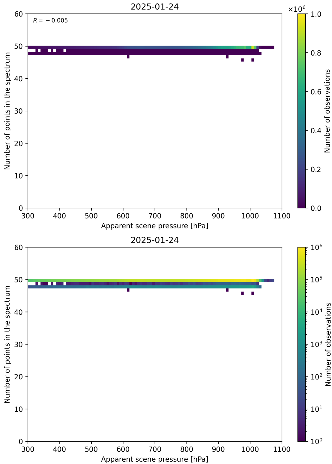
Figure 66: Scatter density plot of “Apparent scene pressure” against “Number of points in the spectrum” for 2025-01-23 to 2025-01-25.
