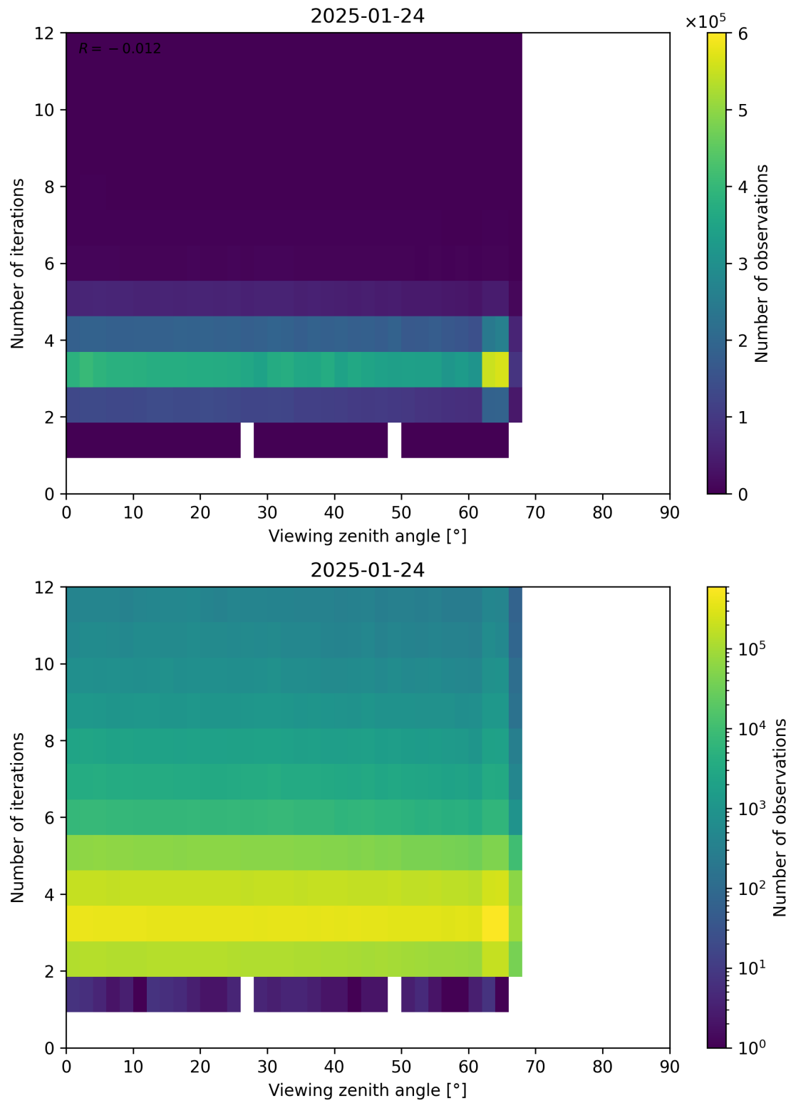
Figure 124: Scatter density plot of “Viewing zenith angle” against “Number of iterations” for 2025-01-23 to 2025-01-25.
