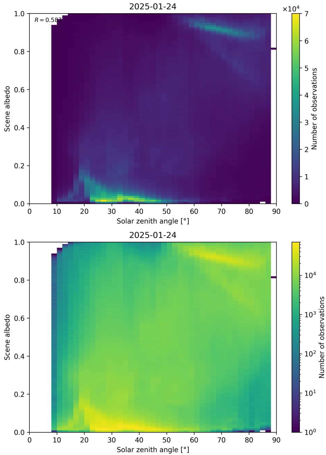
Figure 116: Scatter density plot of “Solar zenith angle” against “Scene albedo” for 2025-01-23 to 2025-01-25.
