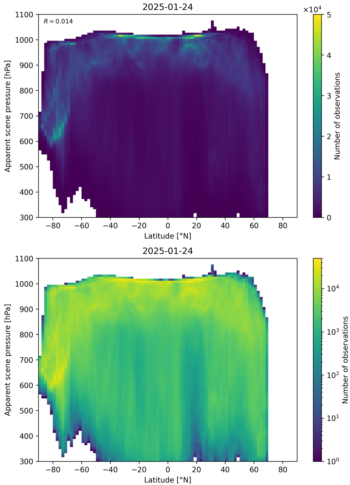
Figure 88: Scatter density plot of “Latitude” against “Apparent scene pressure” for 2025-01-23 to 2025-01-25.
