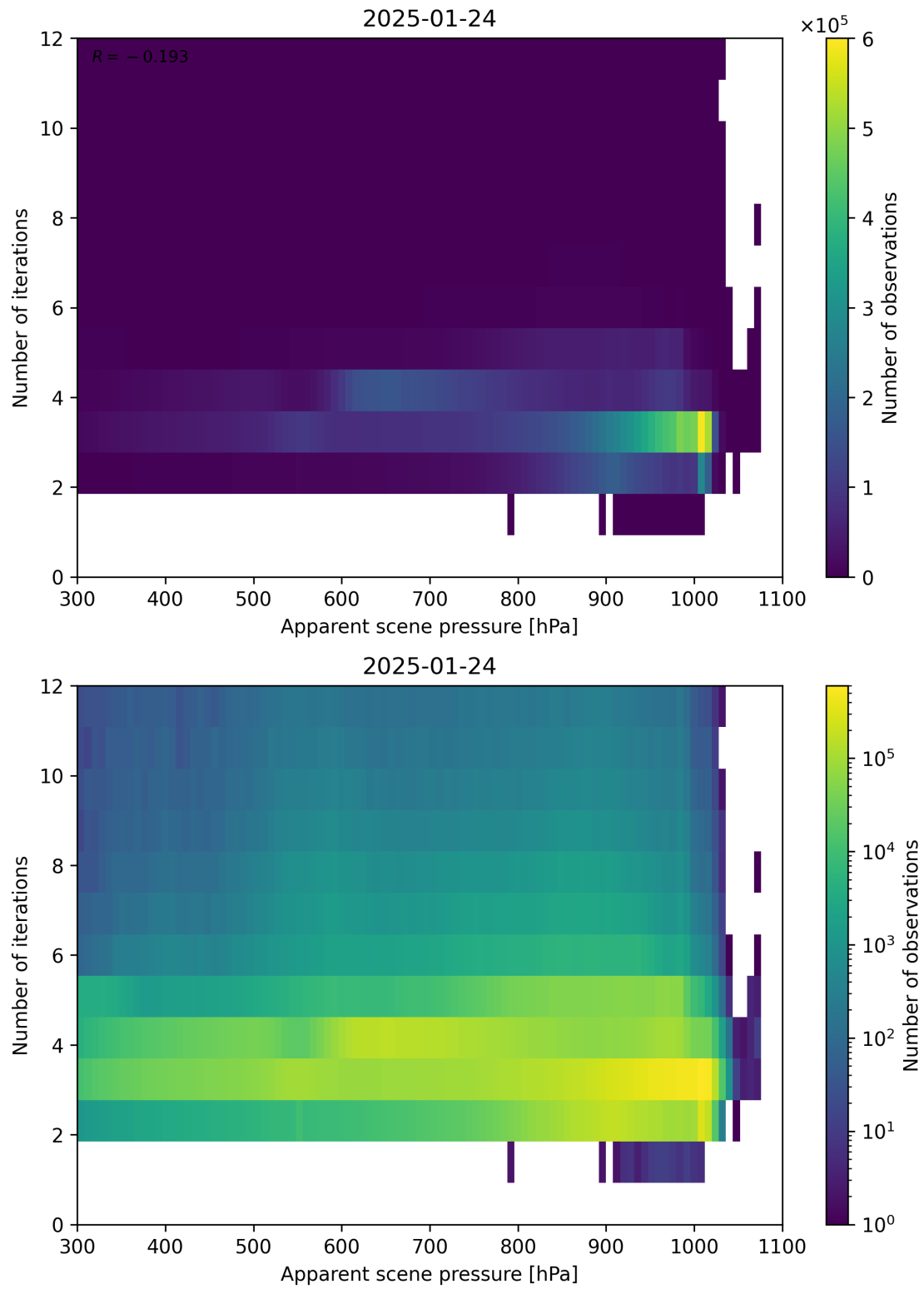
Figure 65: Scatter density plot of “Apparent scene pressure” against “Number of iterations” for 2025-01-23 to 2025-01-25.
