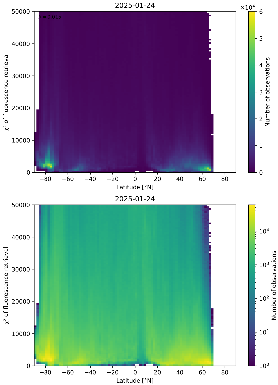
Figure 89: Scatter density plot of “Latitude” against “ \chi^2 of fluorescence retrieval” for 2025-01-23 to 2025-01-25.
