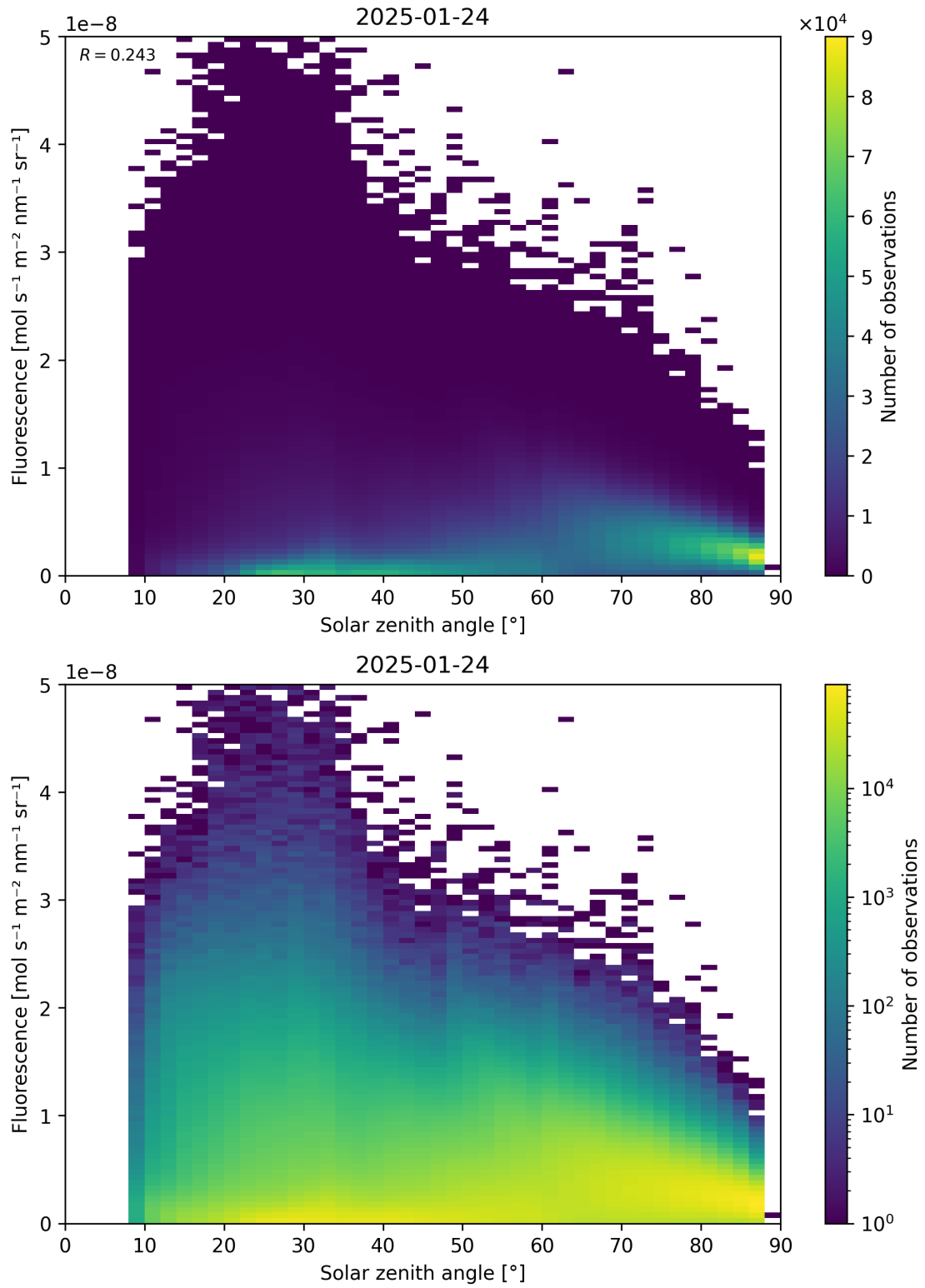
Figure 112: Scatter density plot of “Solar zenith angle” against “Fluorescence” for 2025-01-23 to 2025-01-25.
