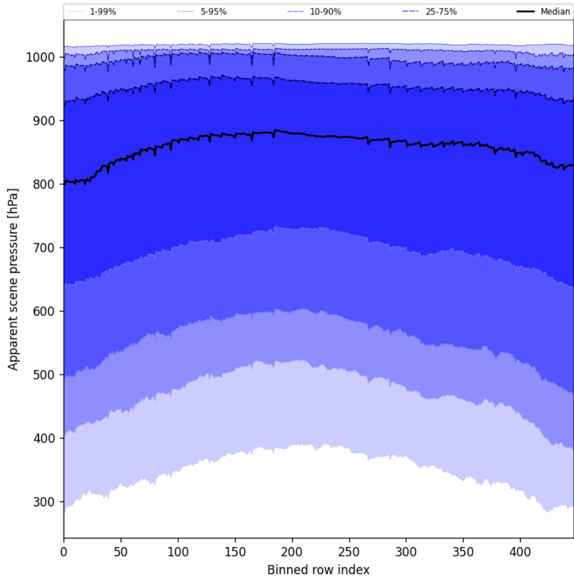
Figure 53: Along track statistics of “Apparent scene pressure” for 2025-01-23 to 2025-01-25
