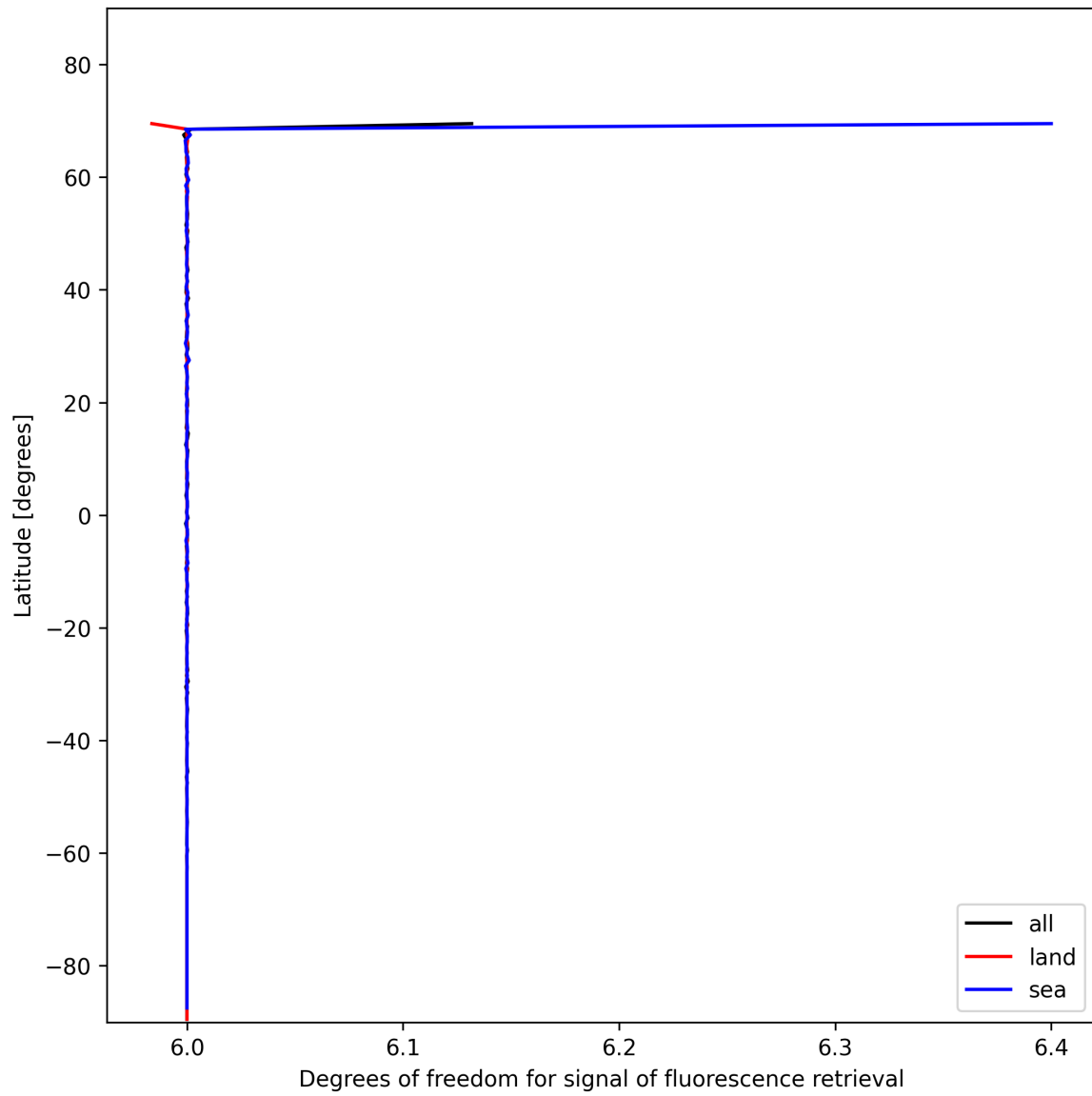
Figure 26: Zonal average of “Degrees of freedom for signal of fluorescence retrieval” for 2025-01-23 to 2025-01-25.
