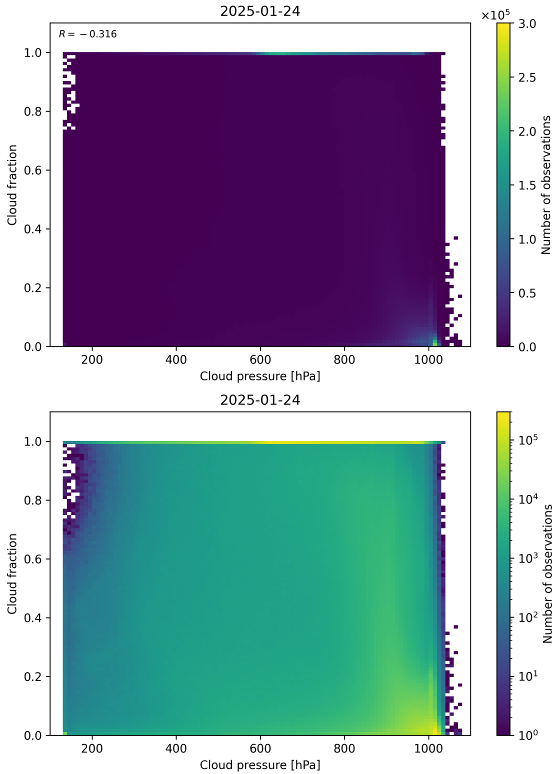
Figure 79: Scatter density plot of “Cloud pressure” against “Cloud fraction” for 2025-01-23 to 2025-01-25.
