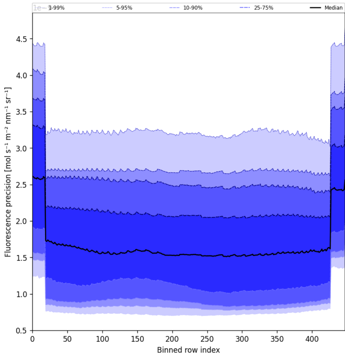
Figure 58: Along track statistics of “Fluorescence precision” for 2025-01-23 to 2025-01-25
