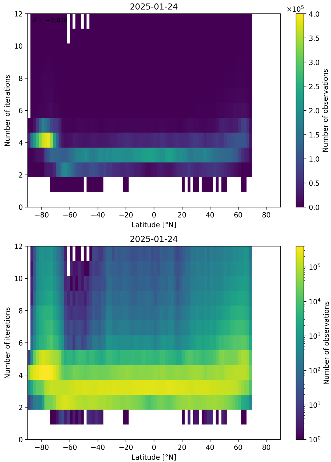
Figure 93: Scatter density plot of “Latitude” against “Number of iterations” for 2025-01-23 to 2025-01-25.
