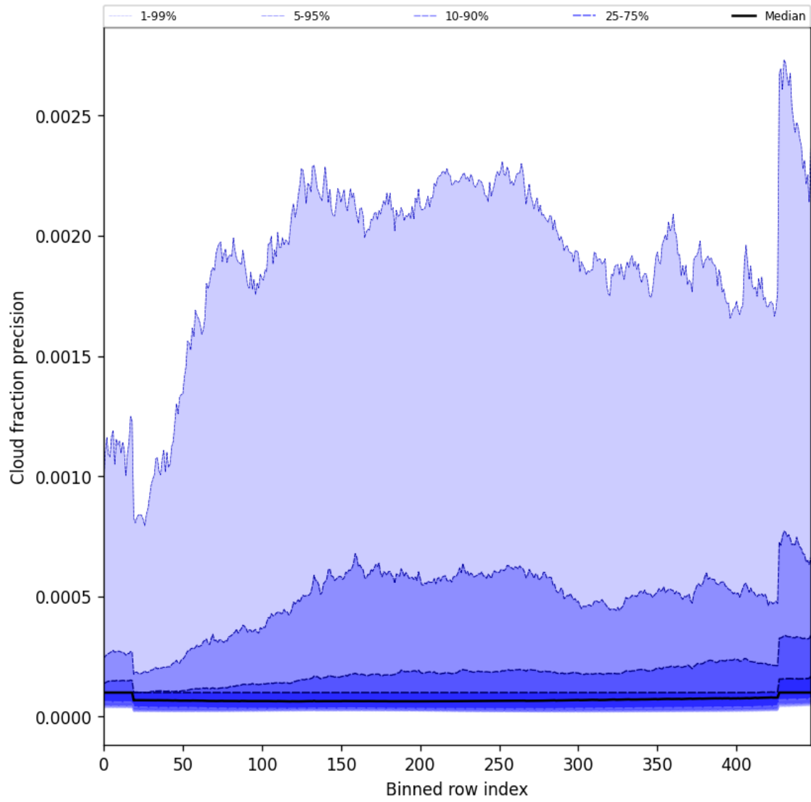
Figure 50: Along track statistics of “Cloud fraction precision” for 2025-01-23 to 2025-01-25
