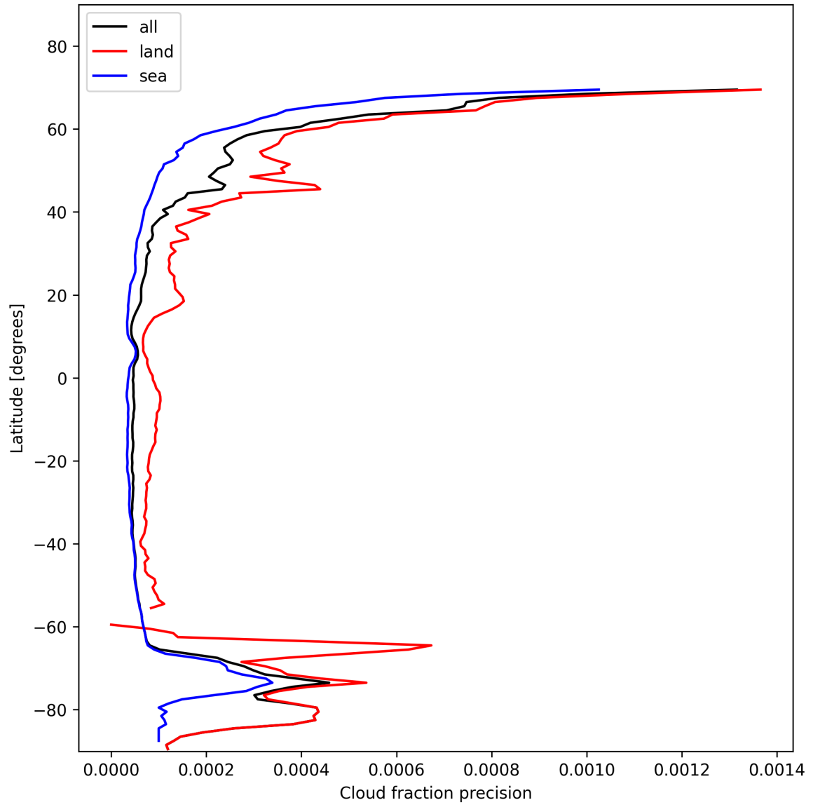
Figure 16: Zonal average of “Cloud fraction precision” for 2025-01-23 to 2025-01-25.
