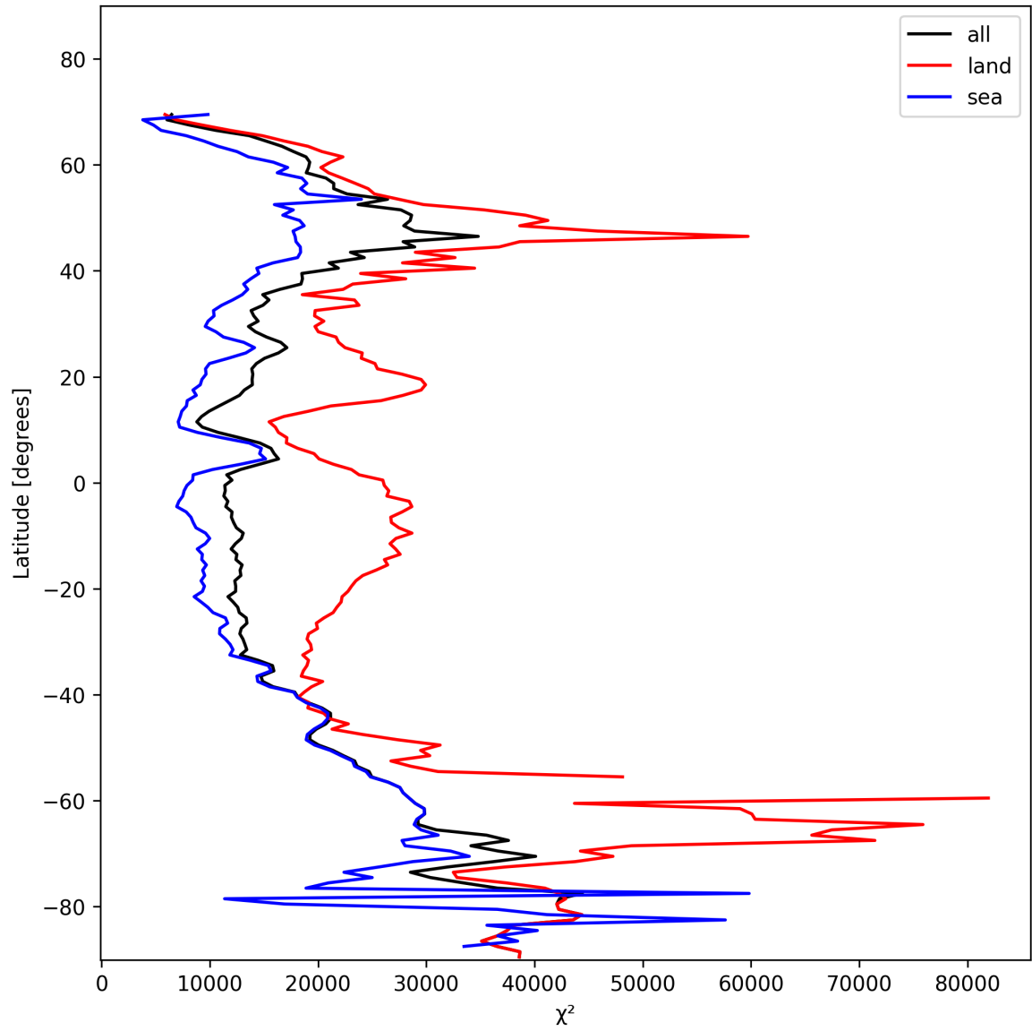
Figure 21: Zonal average of “ \chi^2 ” for 2025-01-23 to 2025-01-25.
