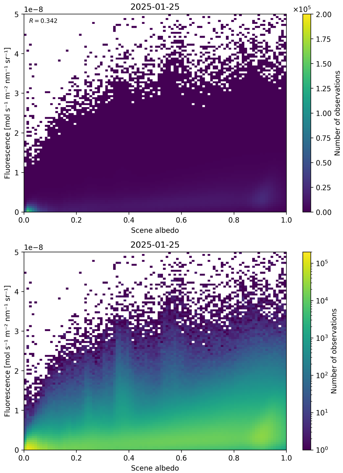
Figure 104: Scatter density plot of “Scene albedo” against “Fluorescence” for 2025-01-24 to 2025-01-26.
