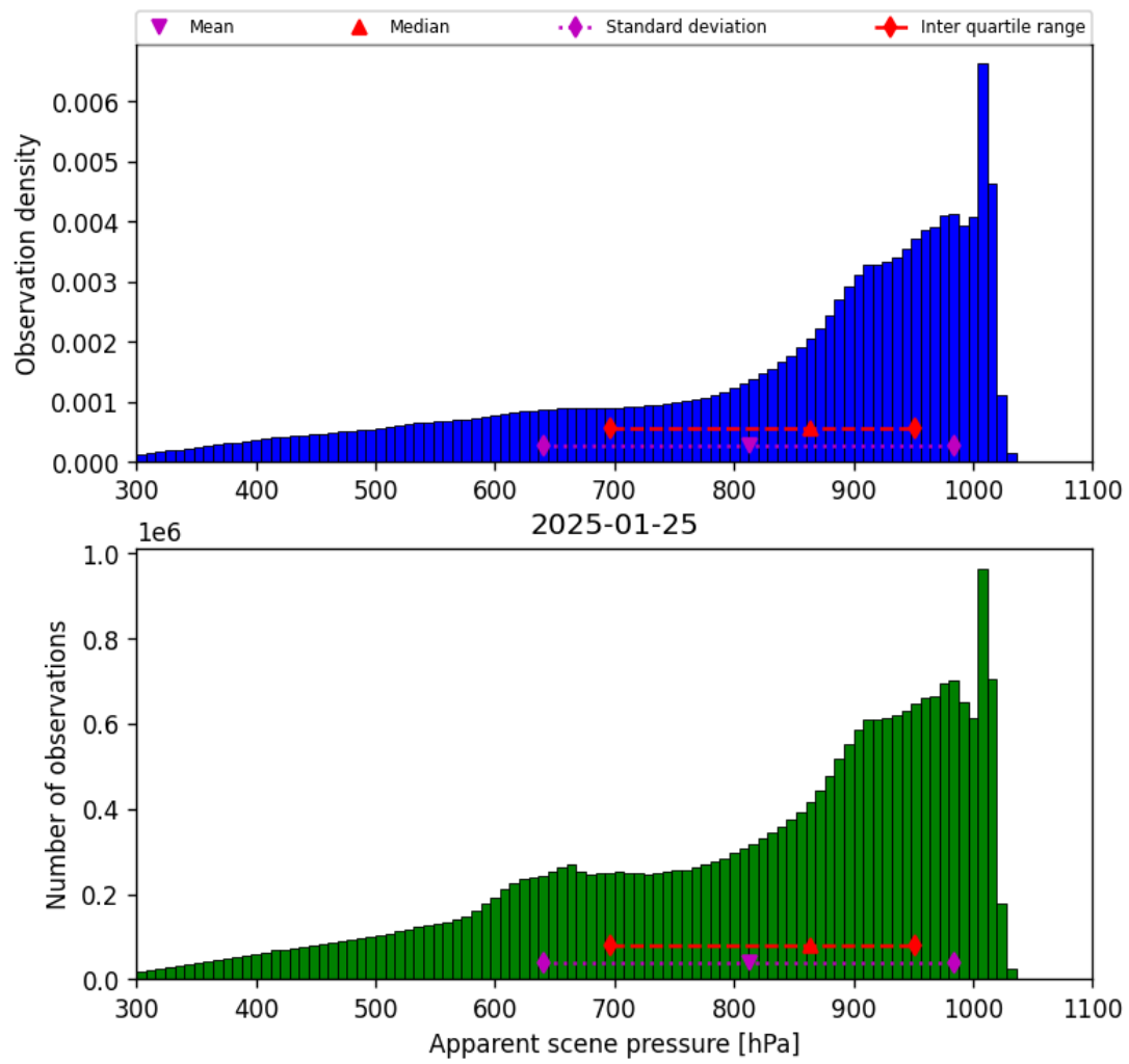
Figure 36: Histogram of “Apparent scene pressure” for 2025-01-24 to 2025-01-26
