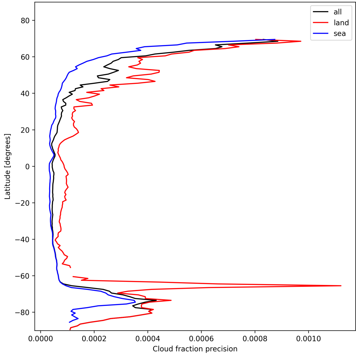
Figure 16: Zonal average of “Cloud fraction precision” for 2025-01-24 to 2025-01-26.
