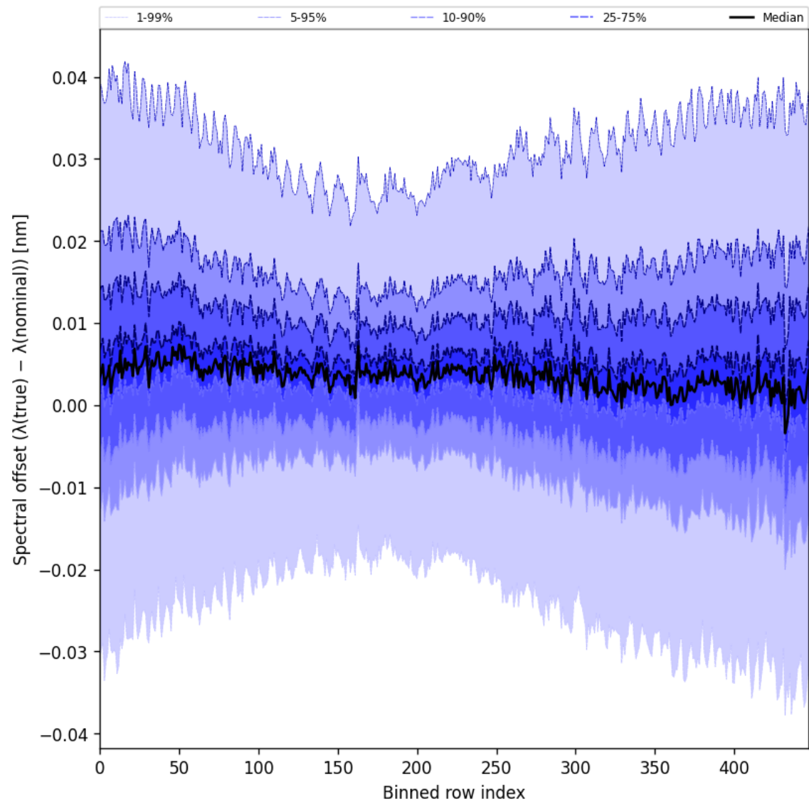
Figure 62: Along track statistics of “Spectral offset ( \lambda_{\text{true}} - \lambda_{\text{nominal}} )” for 2025-01-24 to 2025-01-26
