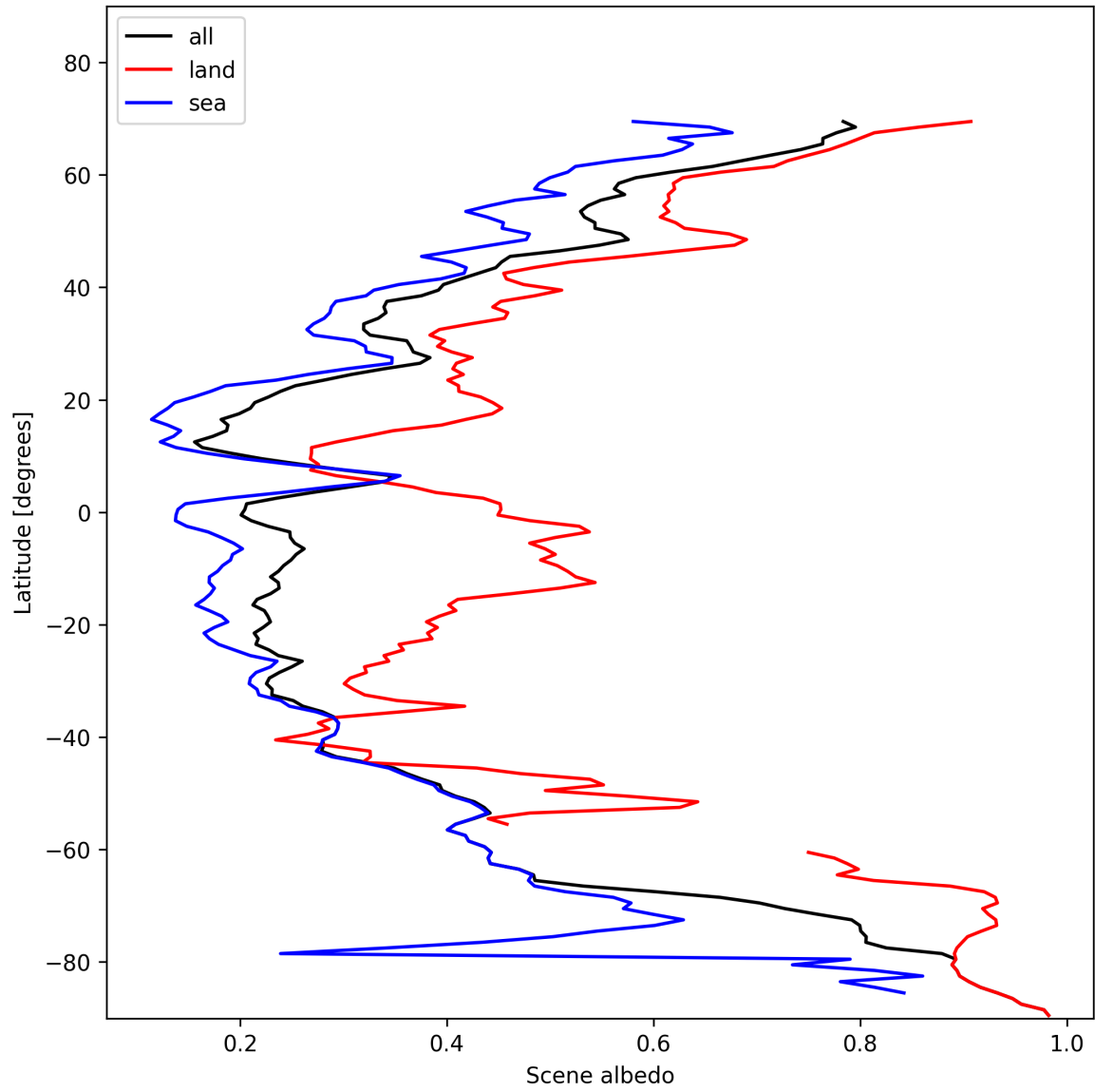
Figure 17: Zonal average of “Scene albedo” for 2025-01-24 to 2025-01-26.
