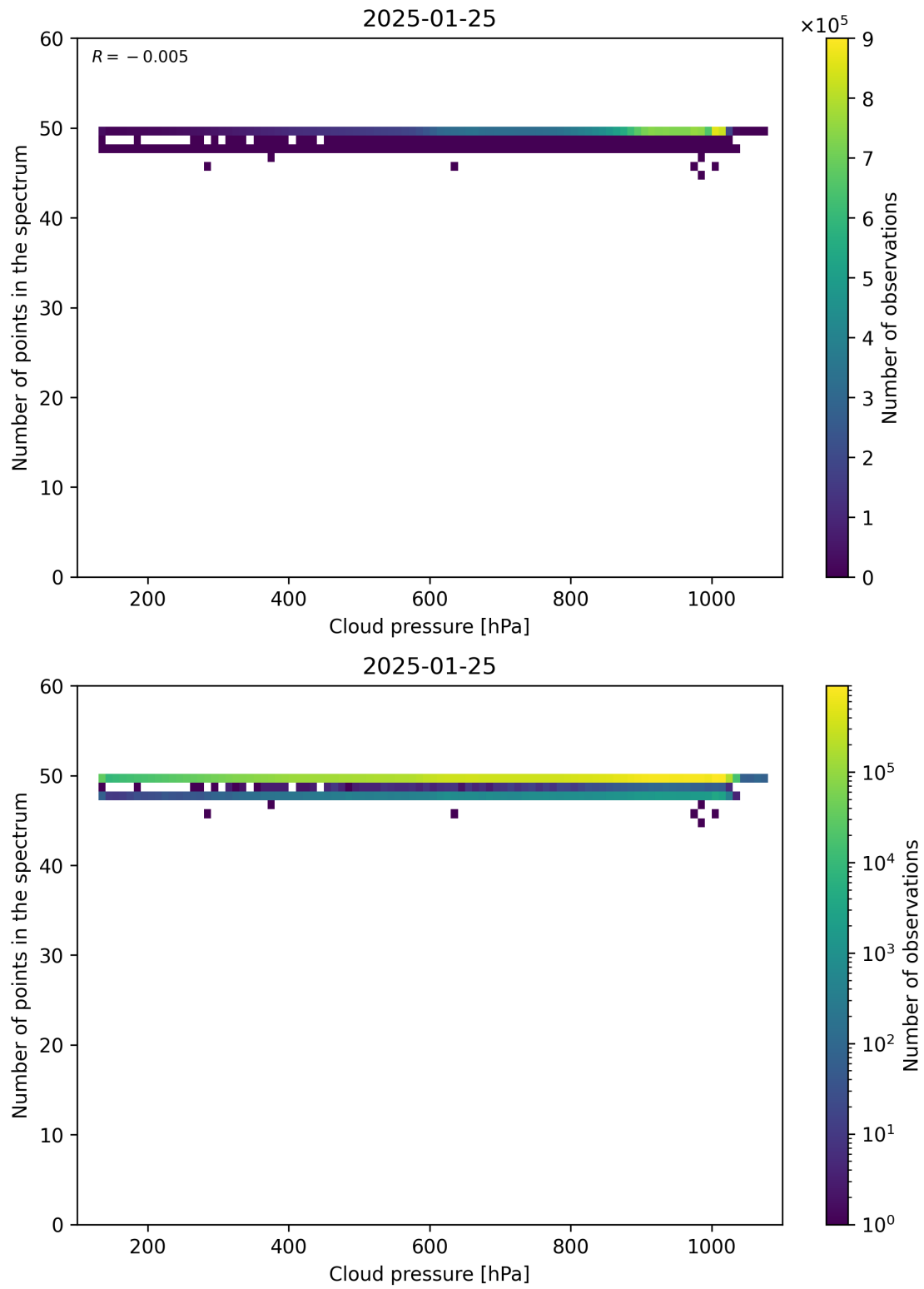
Figure 82: Scatter density plot of “Cloud pressure” against “Number of points in the spectrum” for 2025-01-24 to 2025-01-26.
