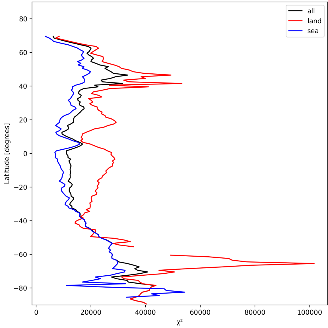
Figure 21: Zonal average of “ \chi^2 ” for 2025-01-24 to 2025-01-26.
