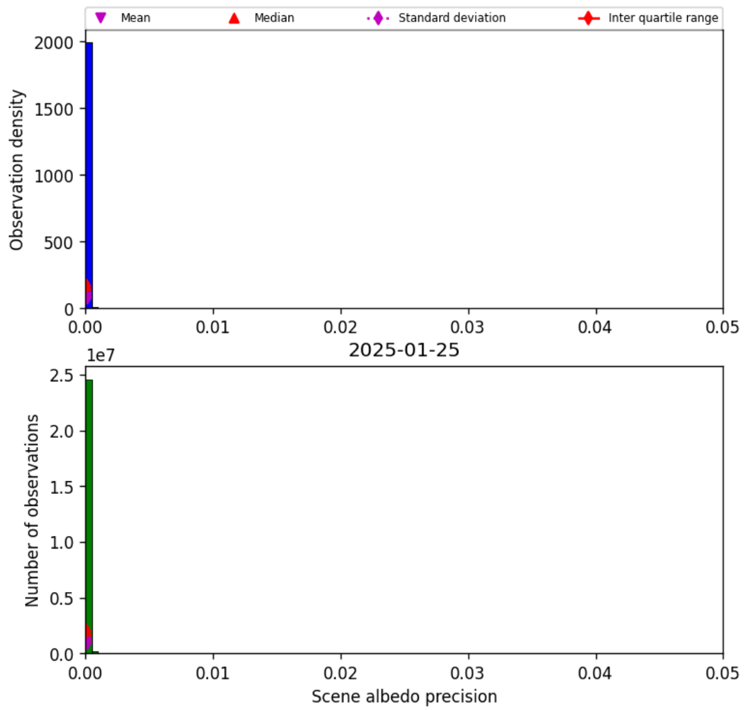
Figure 35: Histogram of “Scene albedo precision” for 2025-01-24 to 2025-01-26
