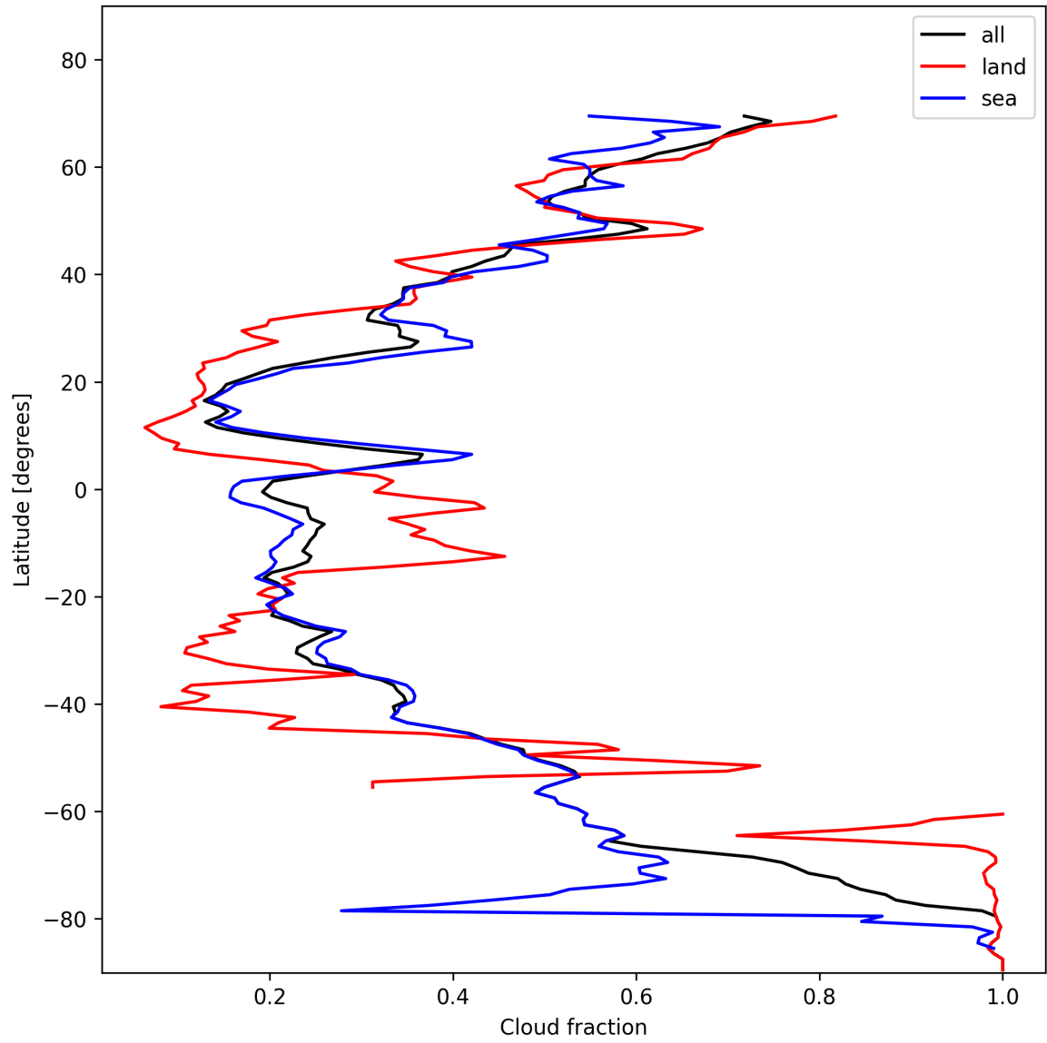
Figure 15: Zonal average of “Cloud fraction” for 2025-01-24 to 2025-01-26.
