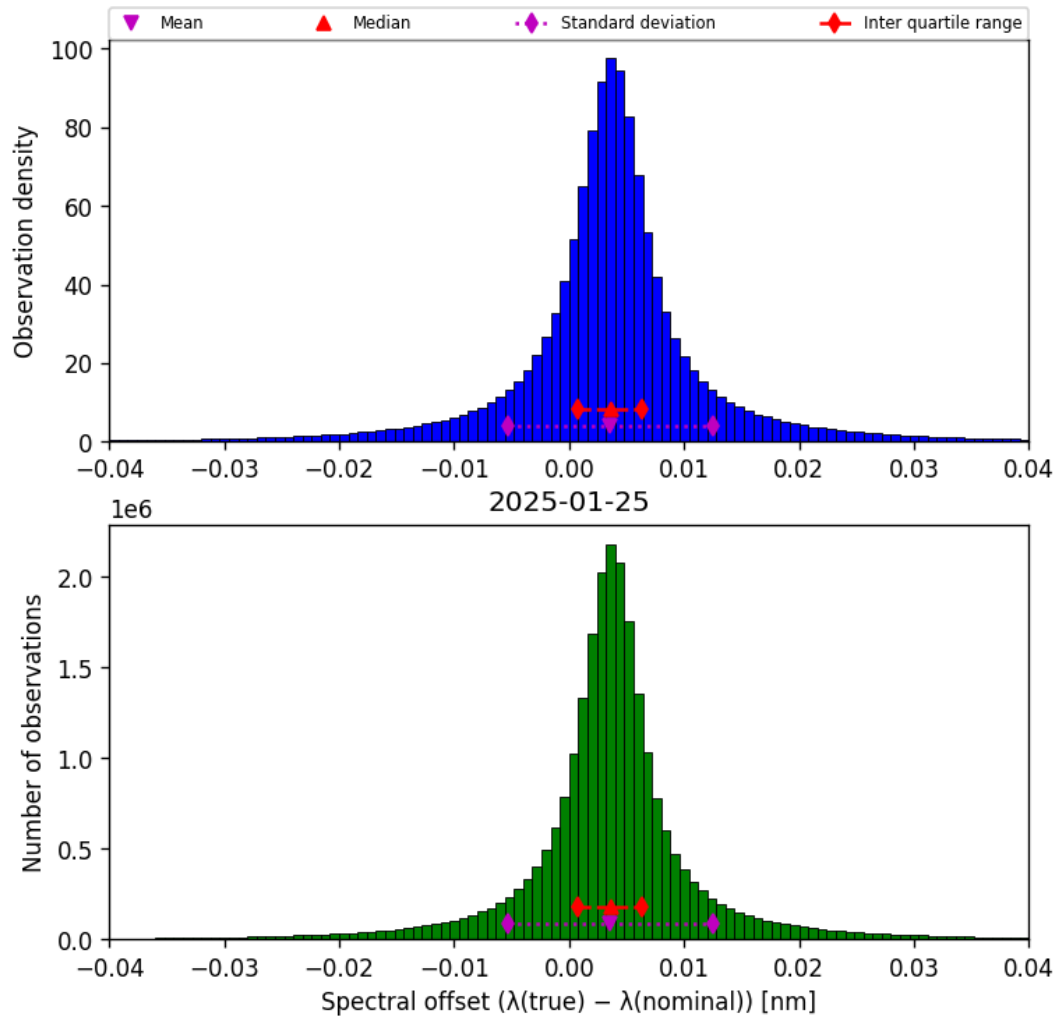
Figure 45: Histogram of “Spectral offset ( \lambda_{\text{true}} - \lambda_{\text{nominal}} )” for 2025-01-24 to 2025-01-26
