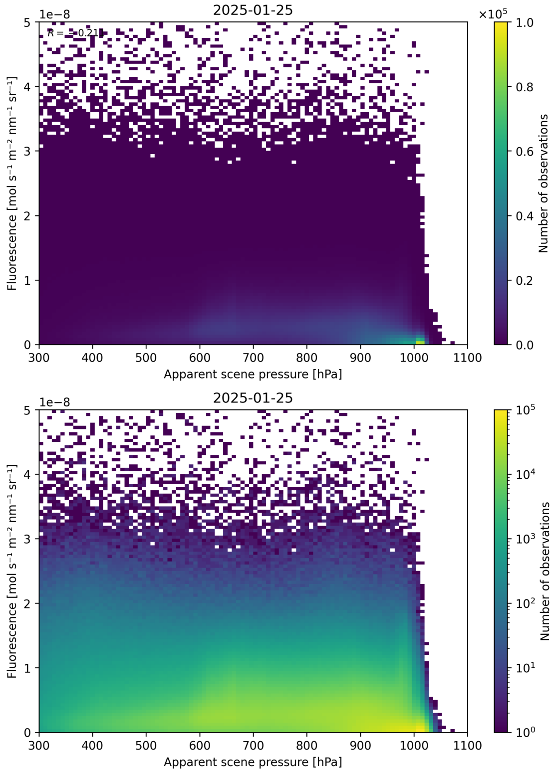
Figure 64: Scatter density plot of “Apparent scene pressure” against “Fluorescence” for 2025-01-24 to 2025-01-26.
