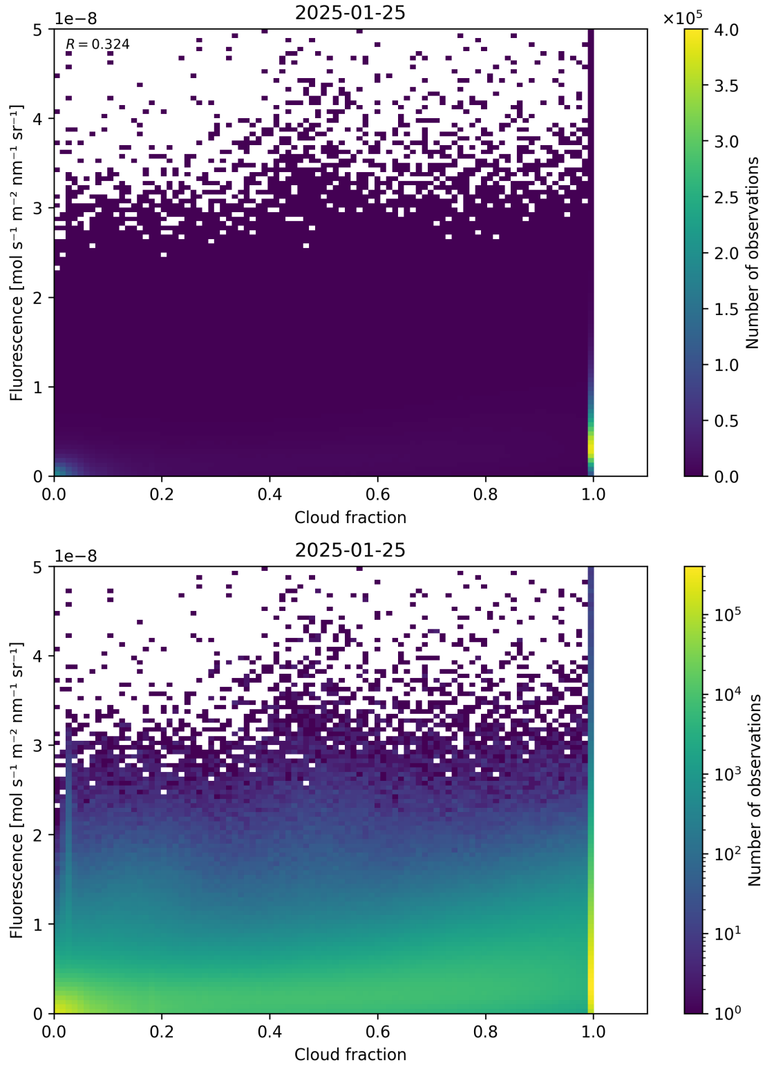
Figure 72: Scatter density plot of “Cloud fraction” against “Fluorescence” for 2025-01-24 to 2025-01-26.
