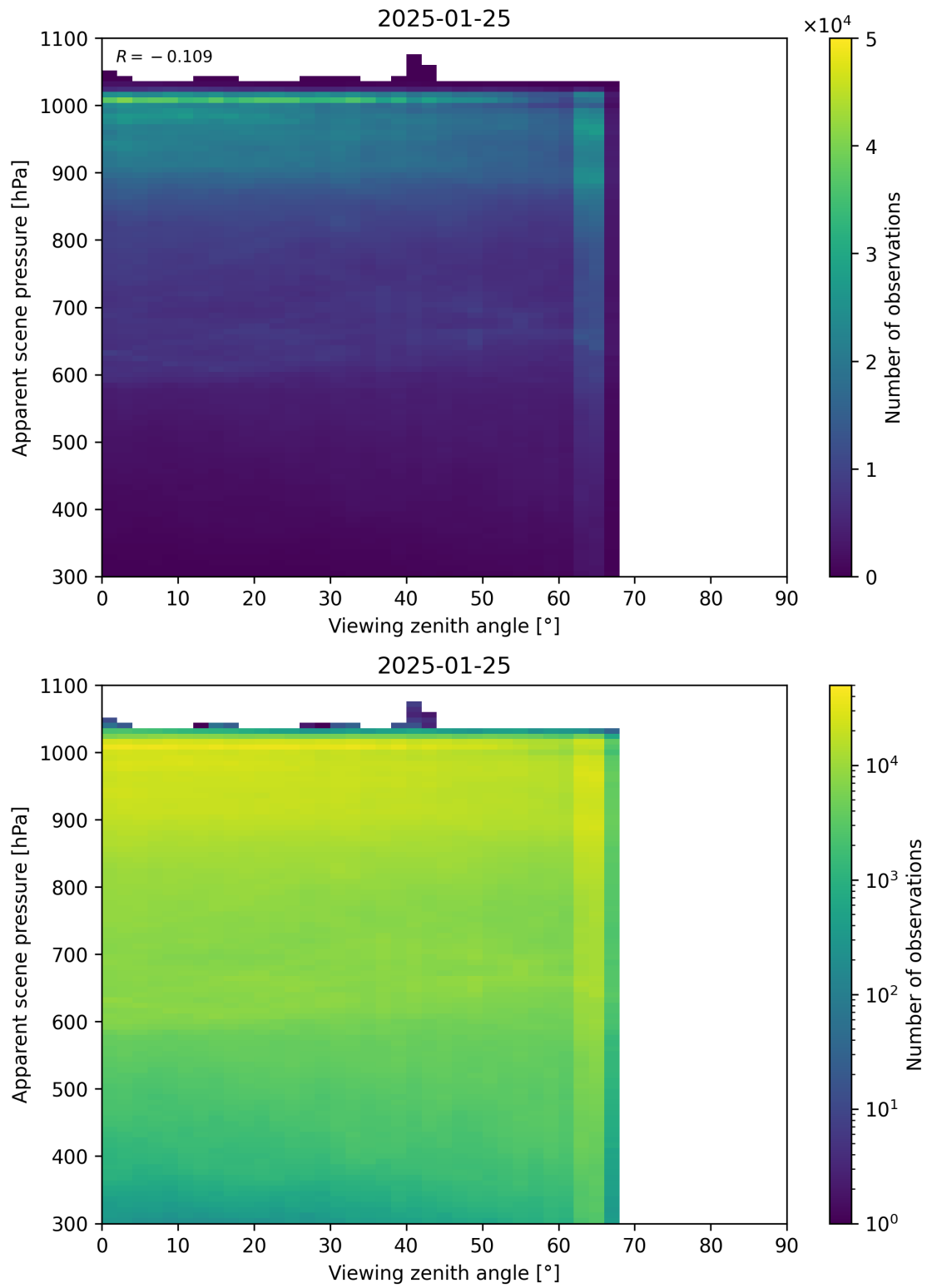
Figure 118: Scatter density plot of “Viewing zenith angle” against “Apparent scene pressure” for 2025-01-24 to 2025-01-26.
