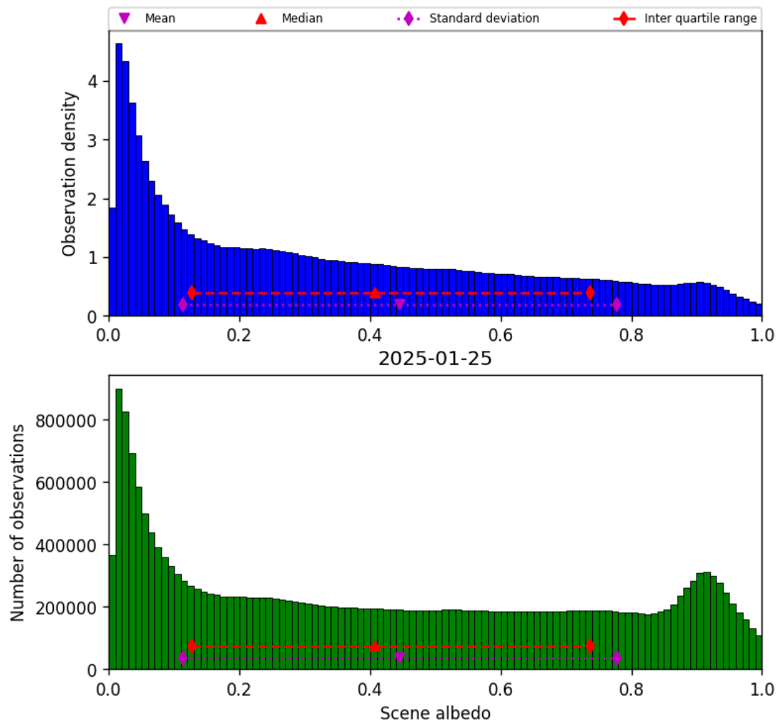
Figure 34: Histogram of “Scene albedo” for 2025-01-24 to 2025-01-26
