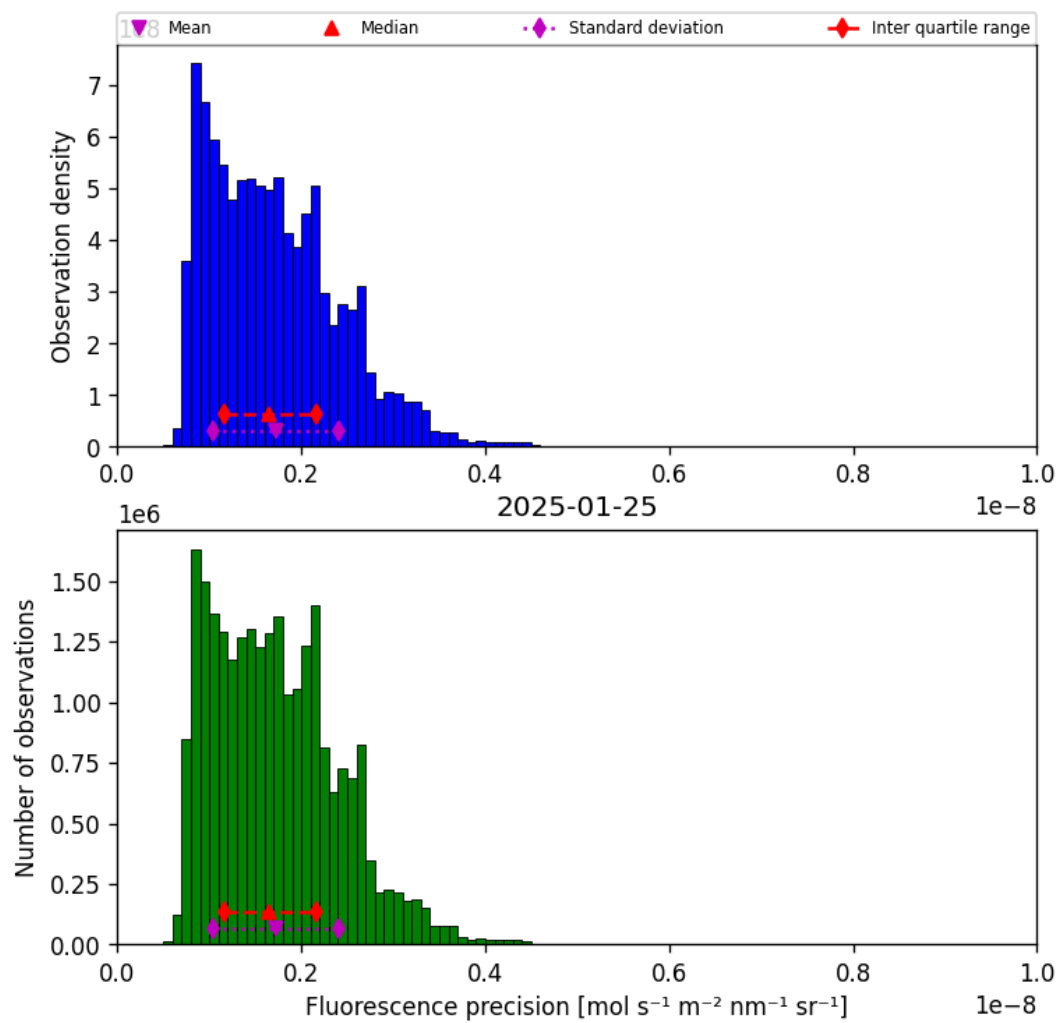
Figure 41: Histogram of “Fluorescence precision” for 2025-01-24 to 2025-01-26
