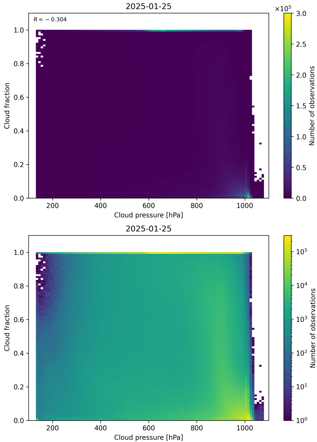
Figure 79: Scatter density plot of “Cloud pressure” against “Cloud fraction” for 2025-01-24 to 2025-01-26.
