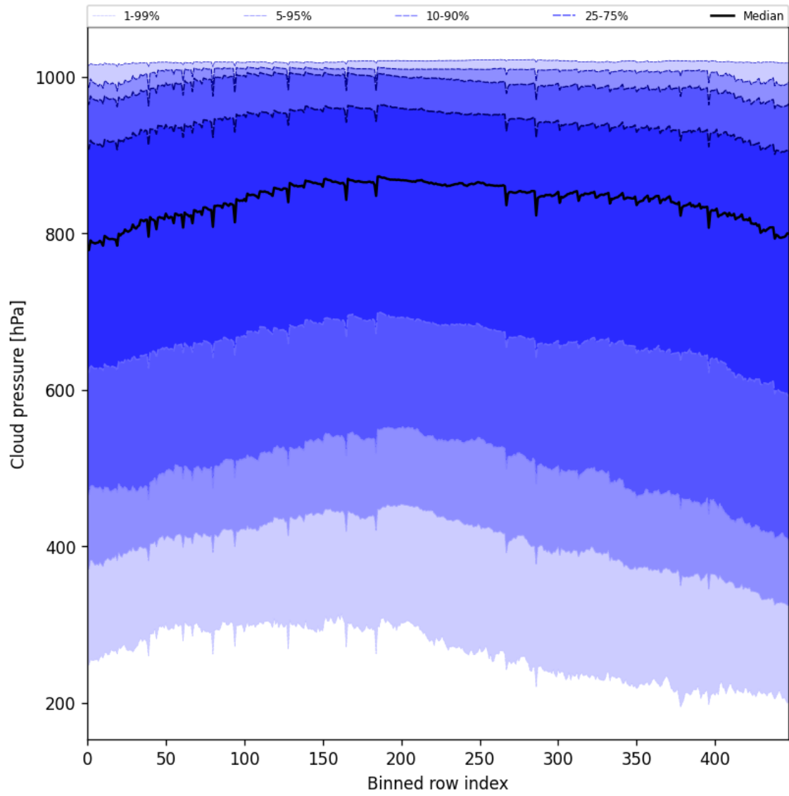
Figure 47: Along track statistics of “Cloud pressure” for 2025-01-24 to 2025-01-26
