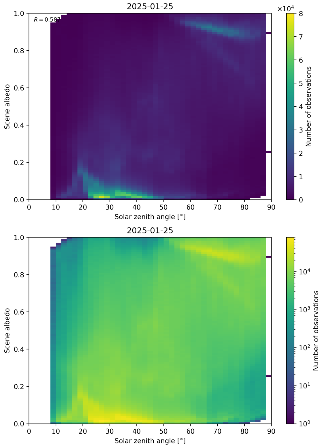
Figure 116: Scatter density plot of “Solar zenith angle” against “Scene albedo” for 2025-01-24 to 2025-01-26.
