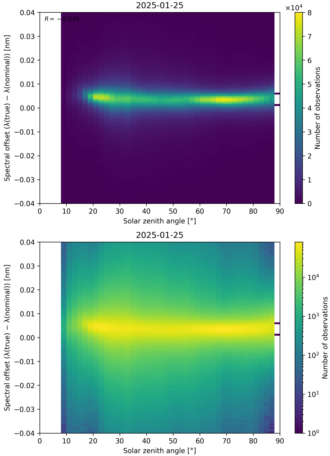
Figure 117: Scatter density plot of “Solar zenith angle” against “Spectral offset ( \lambda_{\text{true}} - \lambda_{\text{nominal}} )” for 2025-01-24 to 2025-01-26.
