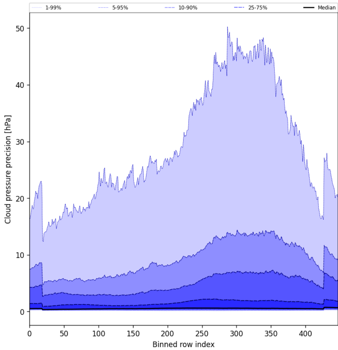
Figure 48: Along track statistics of “Cloud pressure precision” for 2025-01-24 to 2025-01-26
