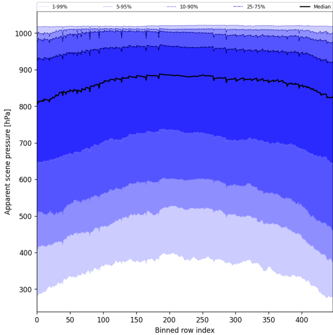
Figure 53: Along track statistics of “Apparent scene pressure” for 2025-01-24 to 2025-01-26
