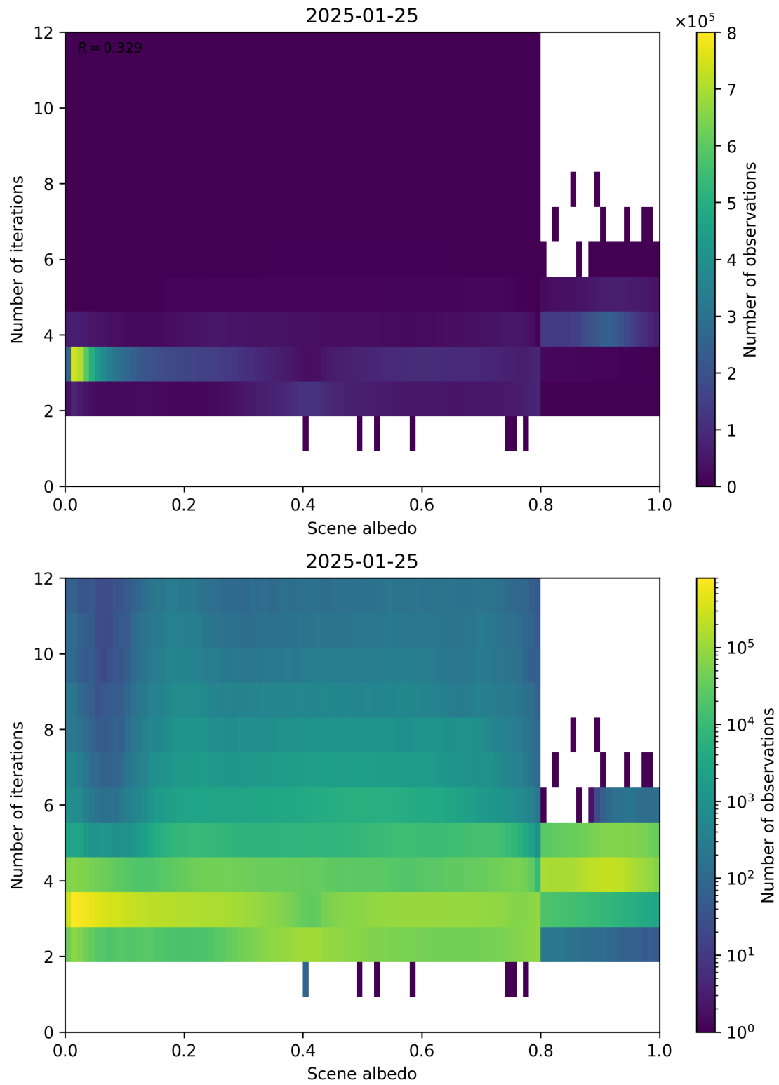
Figure 105: Scatter density plot of “Scene albedo” against “Number of iterations” for 2025-01-24 to 2025-01-26.
