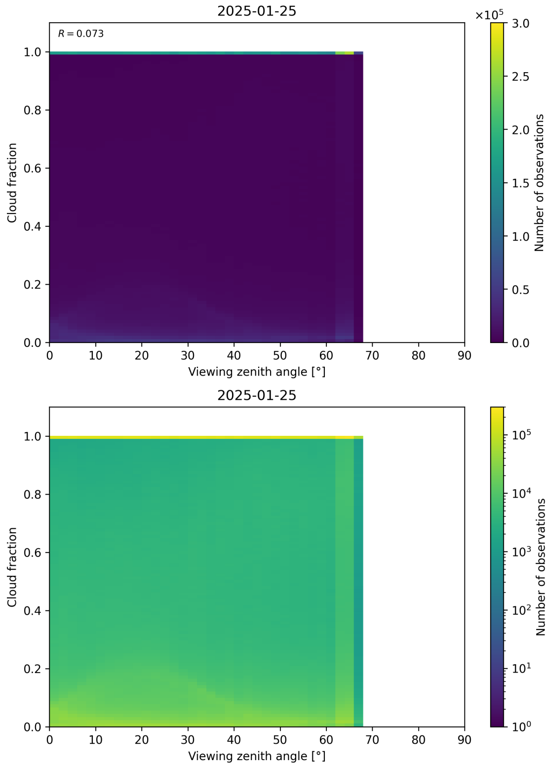
Figure 120: Scatter density plot of “Viewing zenith angle” against “Cloud fraction” for 2025-01-24 to 2025-01-26.
