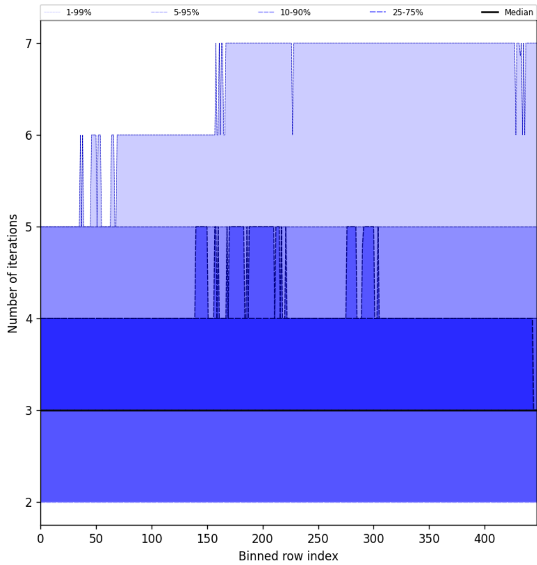
Figure 56: Along track statistics of “Number of iterations” for 2025-01-24 to 2025-01-26
