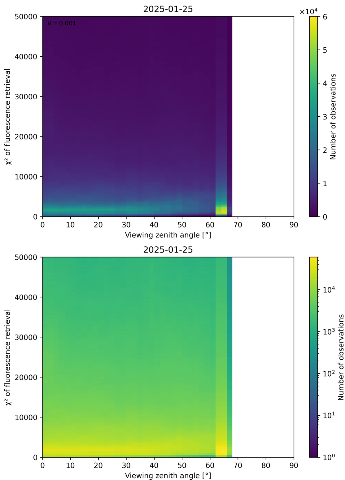
Figure 119: Scatter density plot of “Viewing zenith angle” against “ \chi^2 of fluorescence retrieval” for 2025-01-24 to 2025-01-26.
