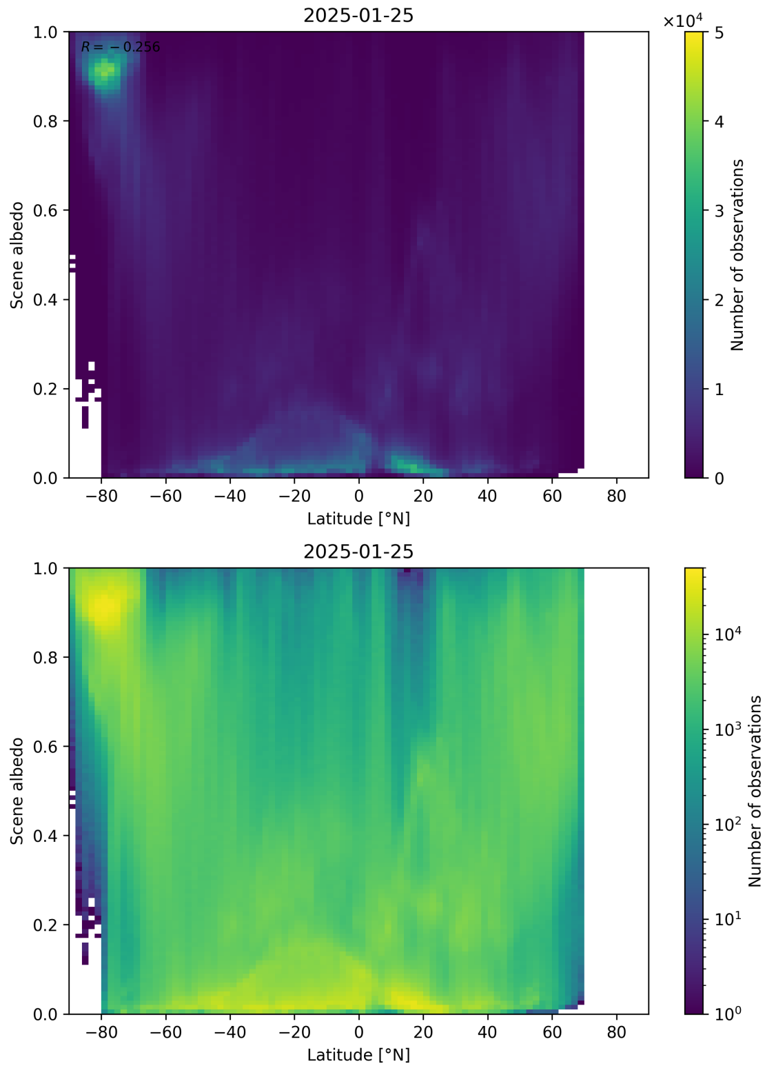
Figure 95: Scatter density plot of “Latitude” against “Scene albedo” for 2025-01-24 to 2025-01-26.
