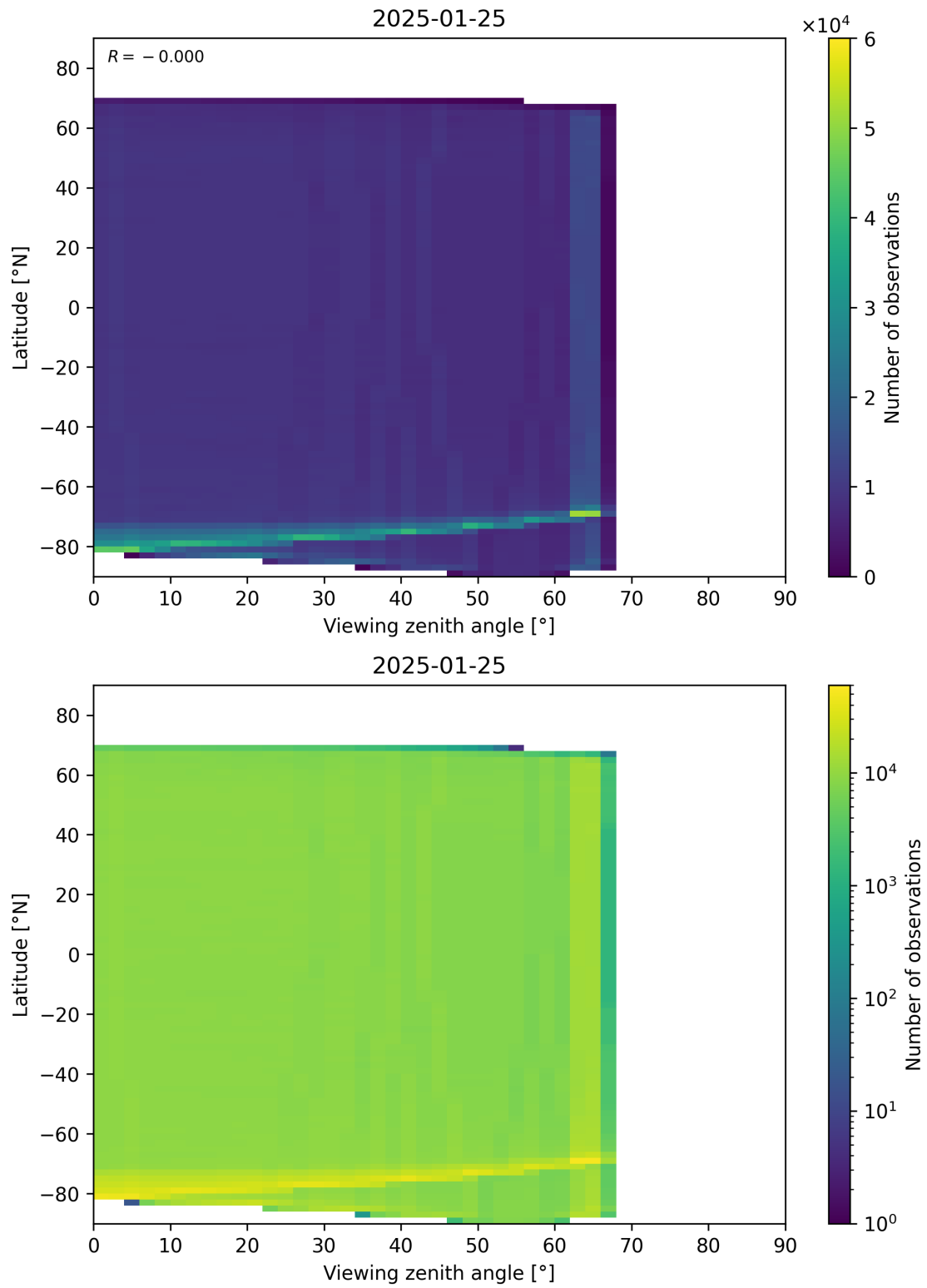
Figure 123: Scatter density plot of “Viewing zenith angle” against “Latitude” for 2025-01-24 to 2025-01-26.
