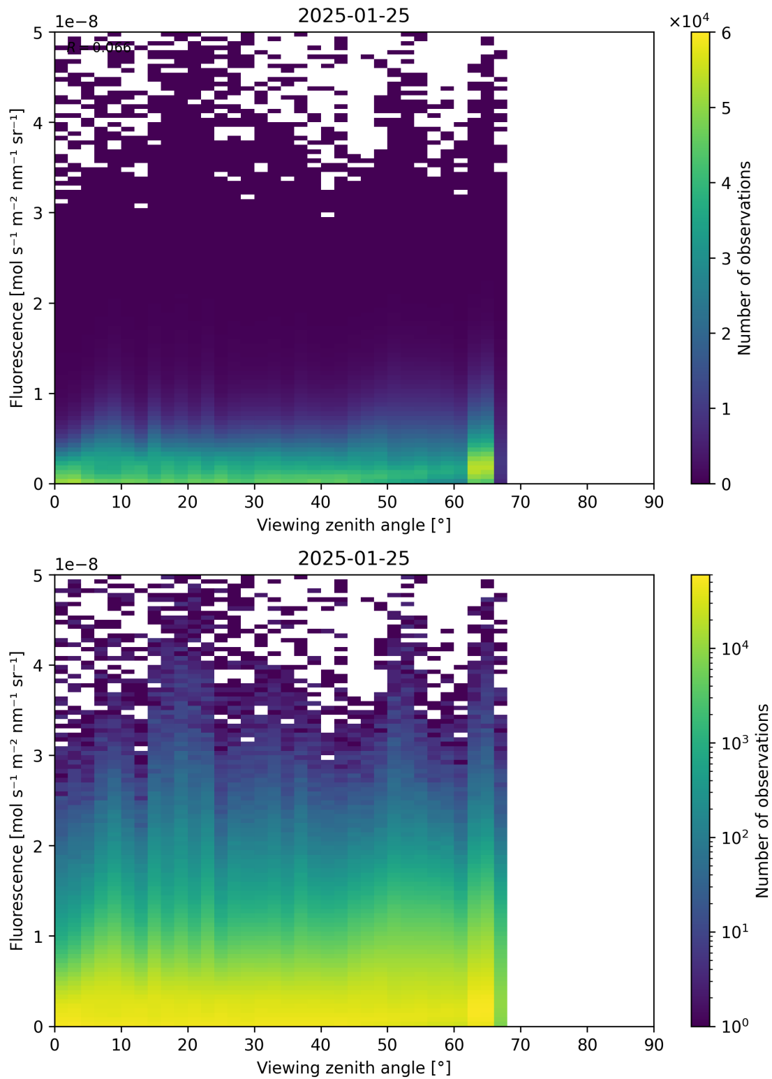
Figure 122: Scatter density plot of “Viewing zenith angle” against “Fluorescence” for 2025-01-24 to 2025-01-26.
