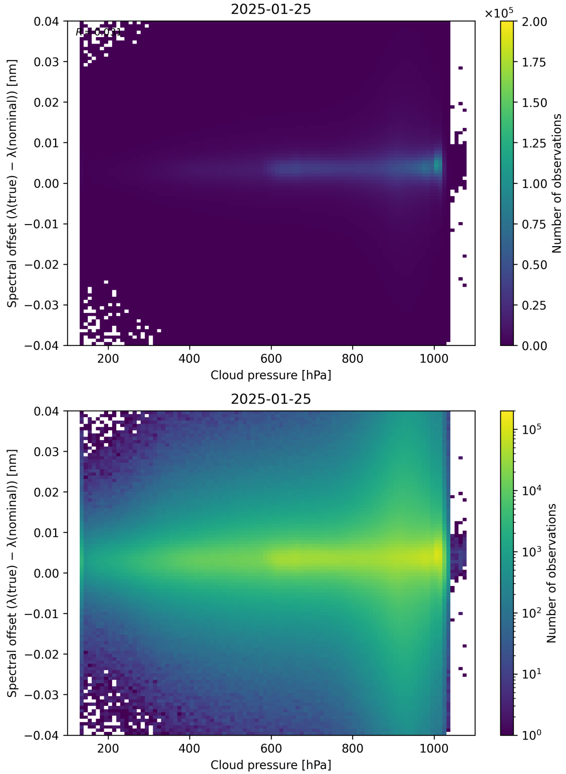
Figure 84: Scatter density plot of “Cloud pressure” against “Spectral offset ( \lambda_{\text{true}} - \lambda_{\text{nominal}} )” for 2025-01-24 to 2025-01-26.
