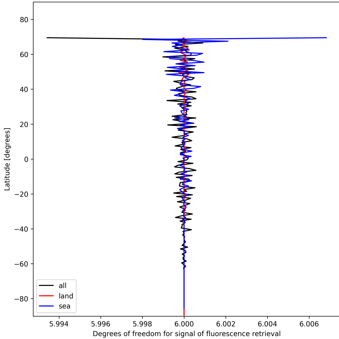
Figure 26: Zonal average of “Degrees of freedom for signal of fluorescence retrieval” for 2025-01-24 to 2025-01-26.
