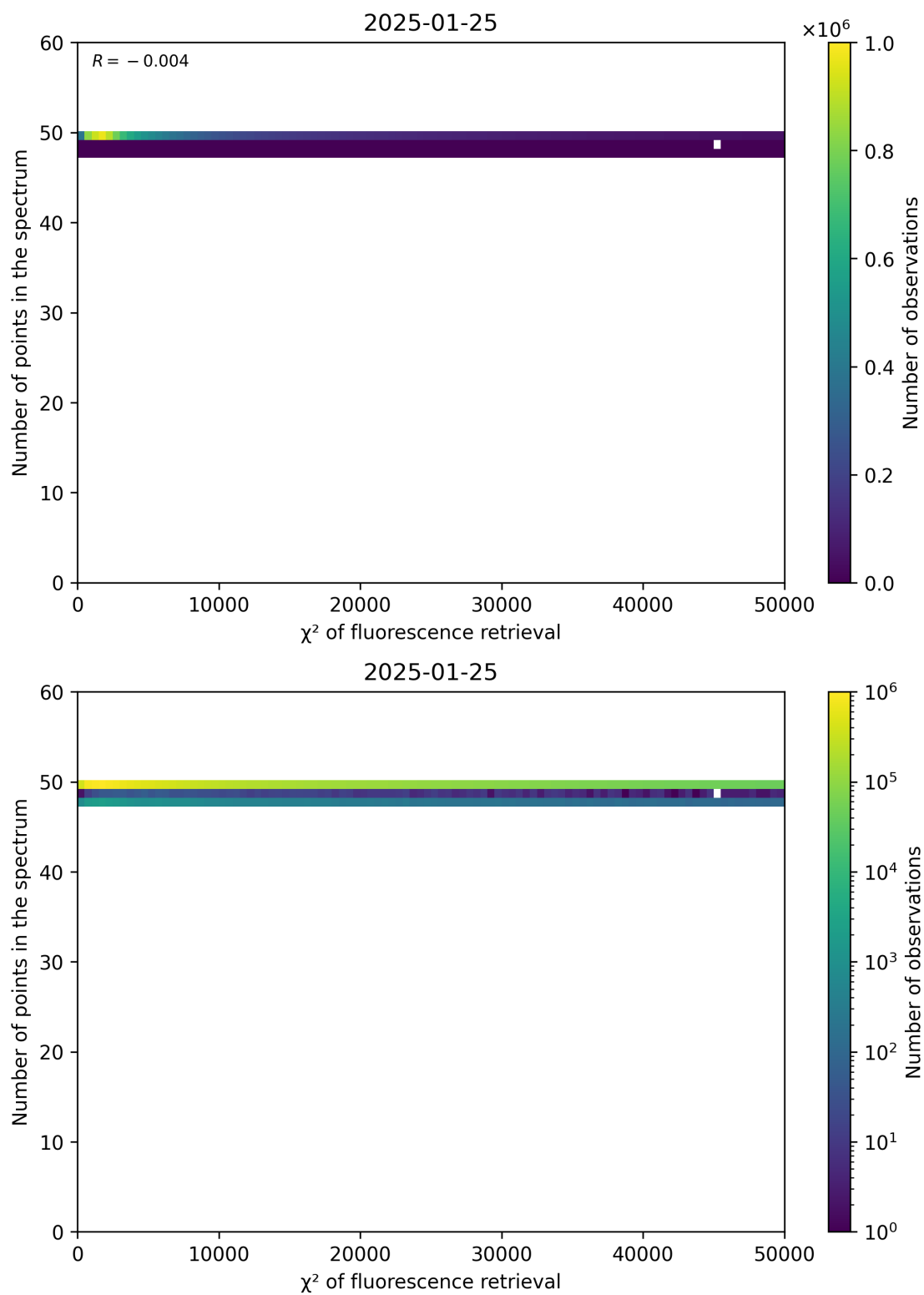
Figure 68: Scatter density plot of “ \chi^2 of fluorescence retrieval” against “Number of points in the spectrum” for 2025-01-24 to 2025-01-26.
