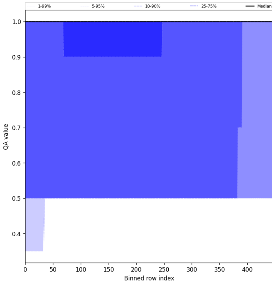
Figure 46: Along track statistics of “QA value” for 2025-01-24 to 2025-01-26
