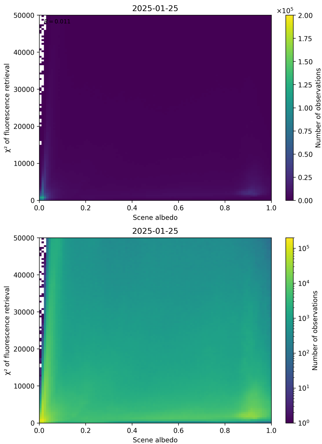
Figure 103: Scatter density plot of “Scene albedo” against “ \chi^2 of fluorescence retrieval” for 2025-01-24 to 2025-01-26.
