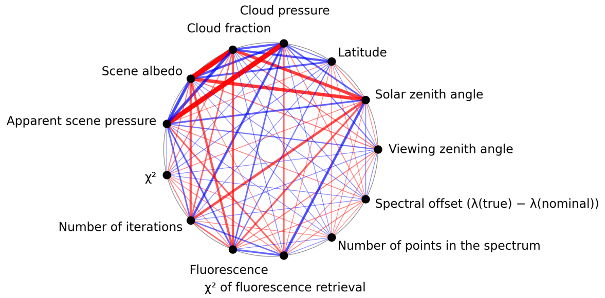
Figure 1: Map of correlation graph for 2025-01-24 to 2025-01-26.
