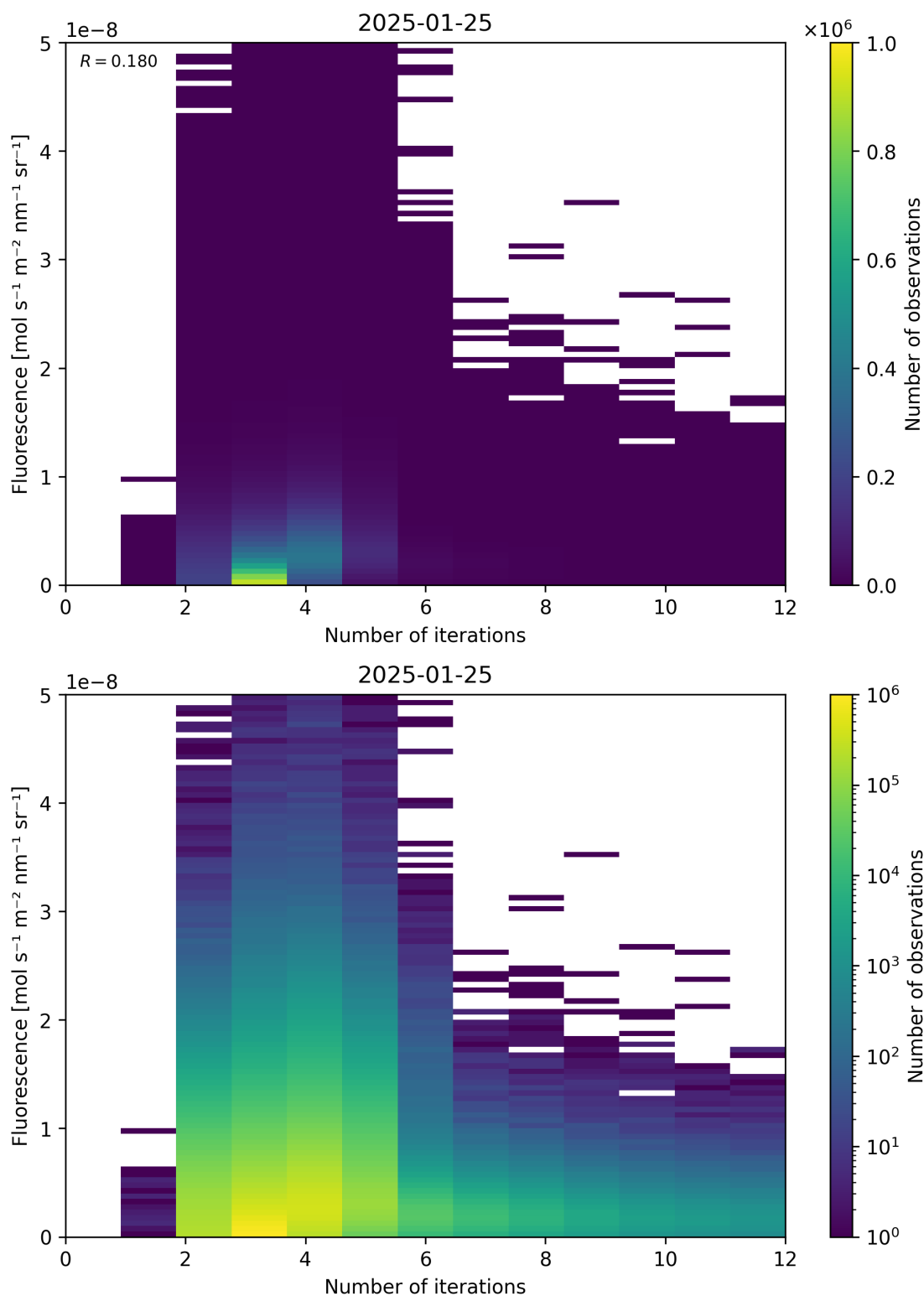
Figure 98: Scatter density plot of “Number of iterations” against “Fluorescence” for 2025-01-24 to 2025-01-26.
