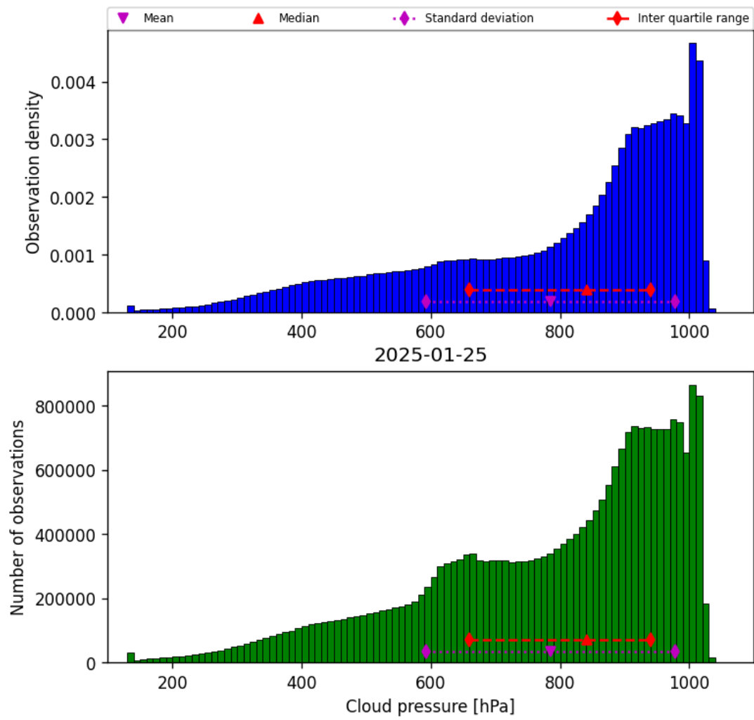
Figure 30: Histogram of “Cloud pressure” for 2025-01-24 to 2025-01-26
