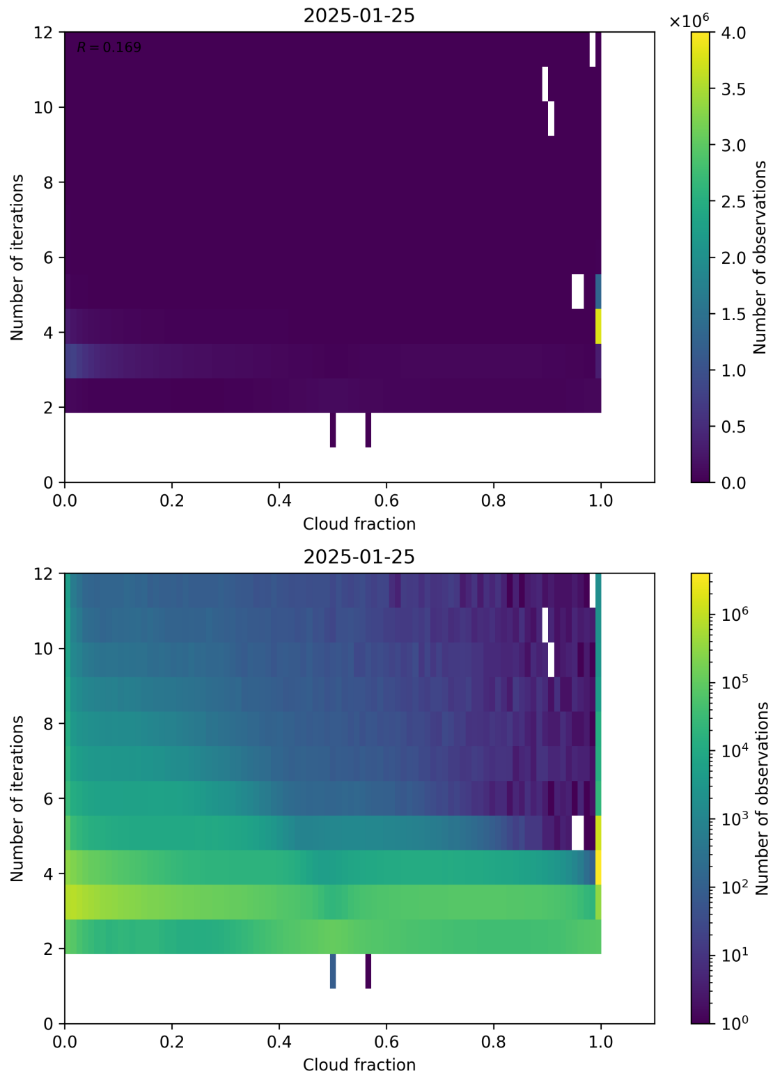
Figure 73: Scatter density plot of “Cloud fraction” against “Number of iterations” for 2025-01-24 to 2025-01-26.
