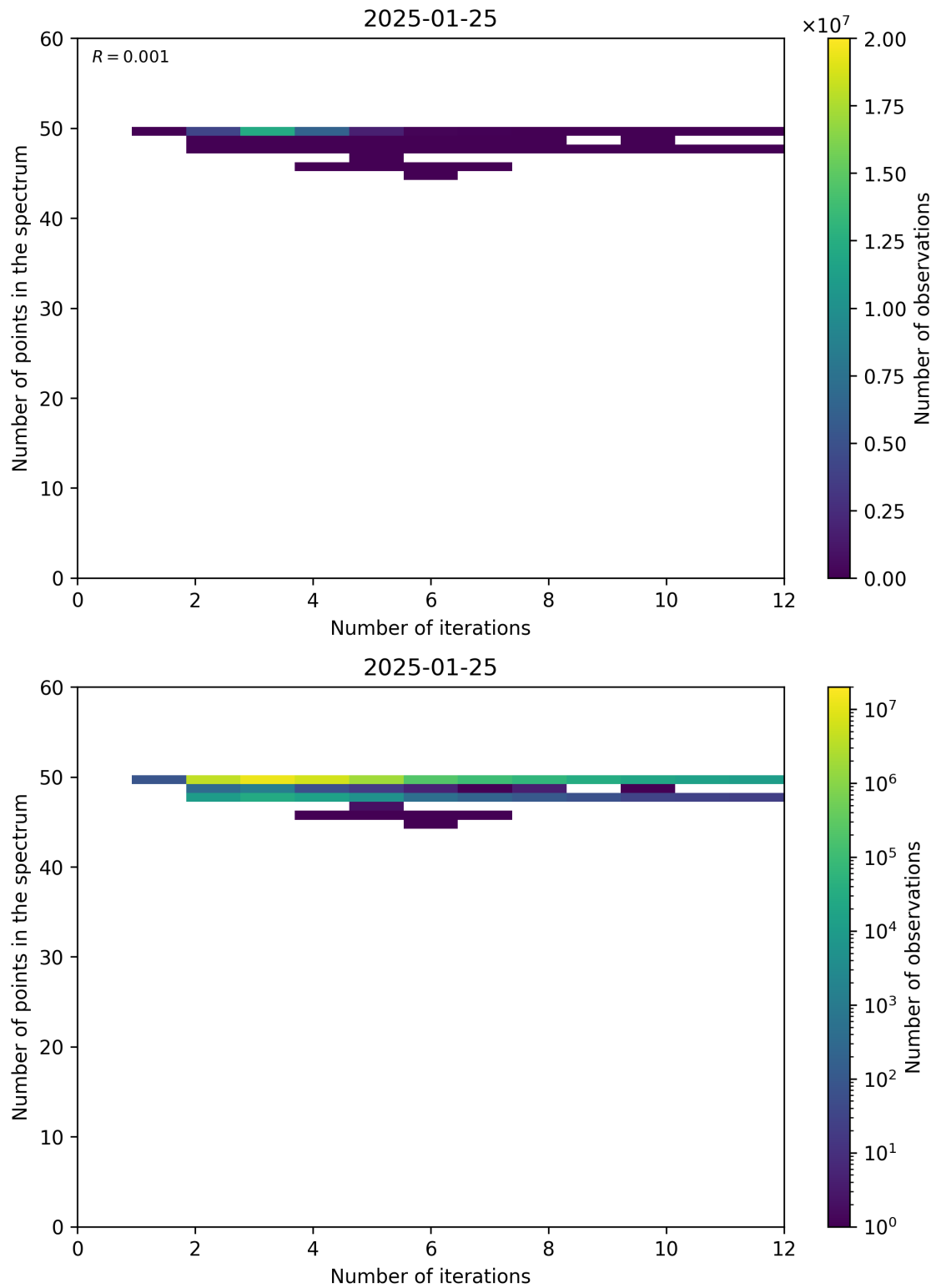
Figure 99: Scatter density plot of “Number of iterations” against “Number of points in the spectrum” for 2025-01-24 to 2025-01-26.
