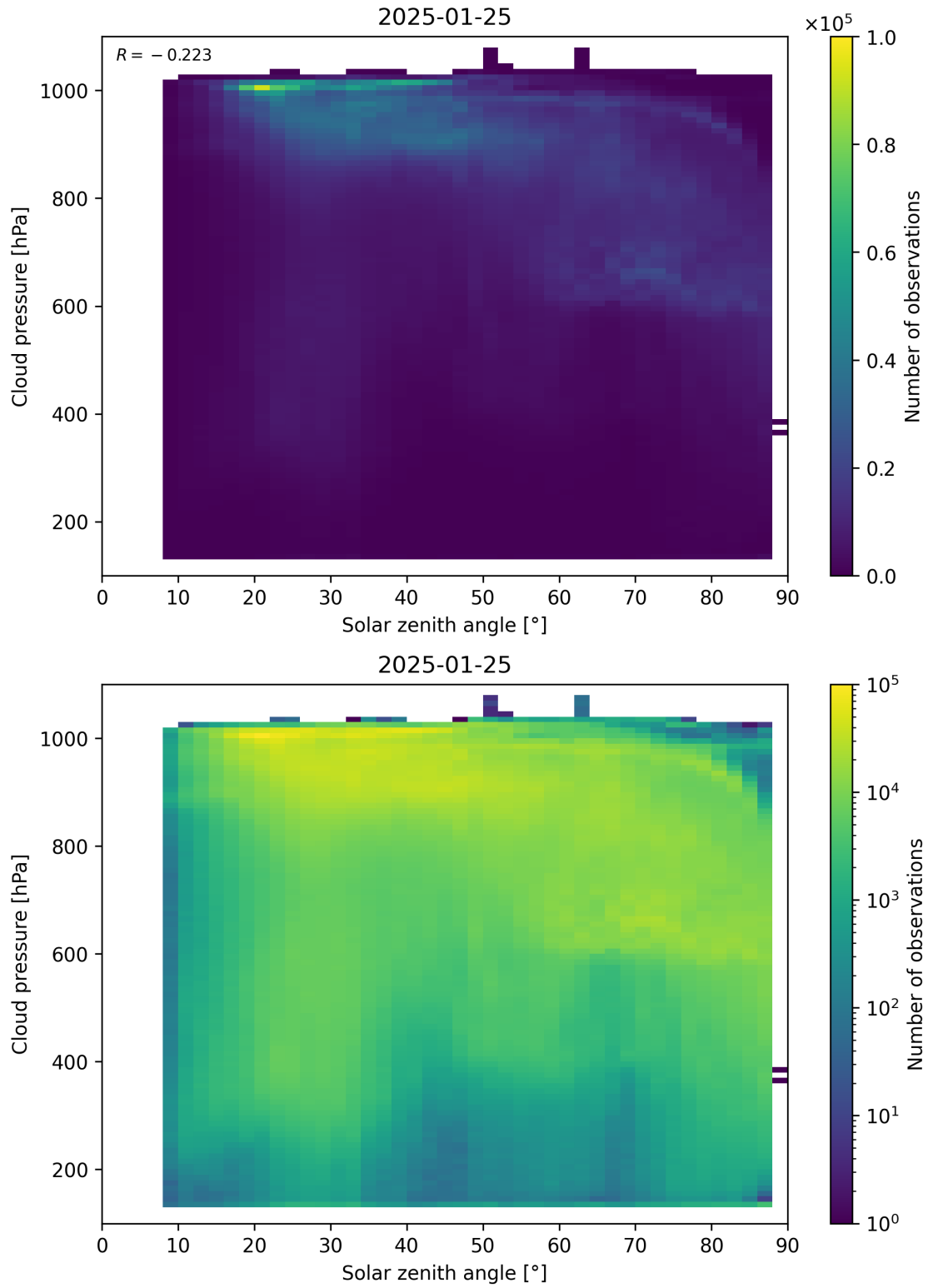
Figure 111: Scatter density plot of “Solar zenith angle” against “Cloud pressure” for 2025-01-24 to 2025-01-26.
