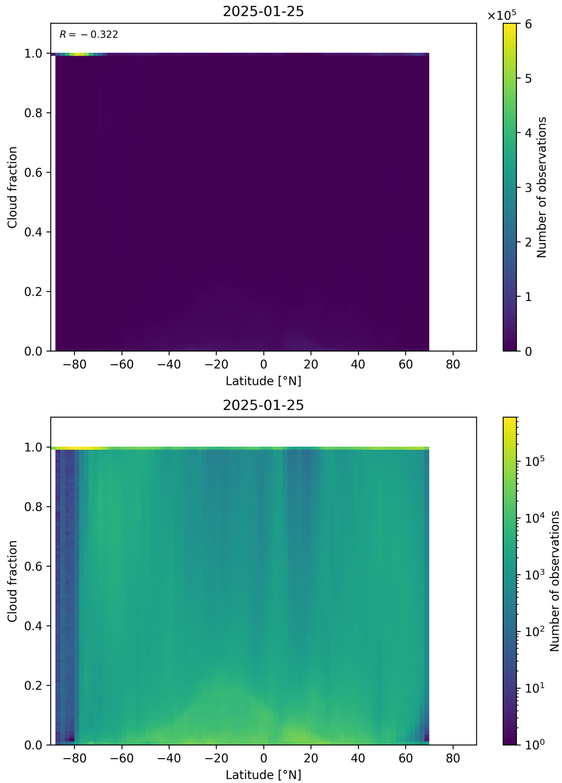
Figure 90: Scatter density plot of “Latitude” against “Cloud fraction” for 2025-01-24 to 2025-01-26.
