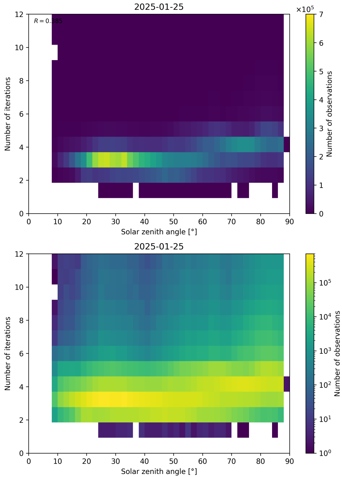
Figure 114: Scatter density plot of “Solar zenith angle” against “Number of iterations” for 2025-01-24 to 2025-01-26.
