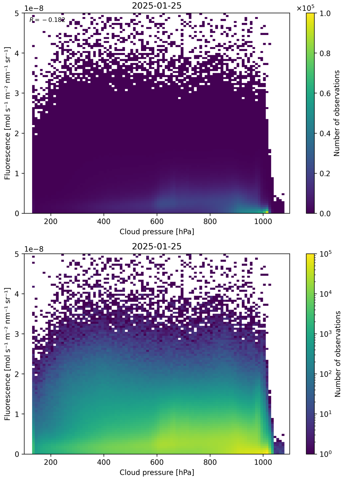
Figure 80: Scatter density plot of “Cloud pressure” against “Fluorescence” for 2025-01-24 to 2025-01-26.
