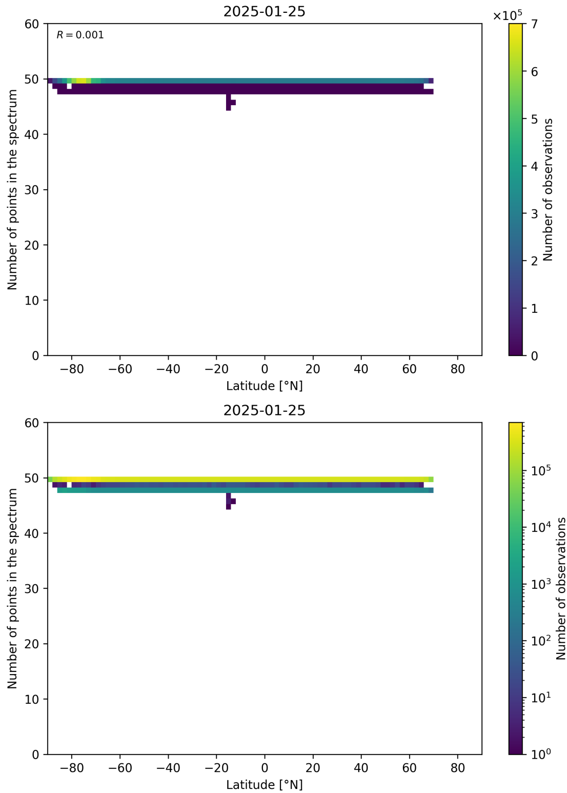
Figure 94: Scatter density plot of “Latitude” against “Number of points in the spectrum” for 2025-01-24 to 2025-01-26.
