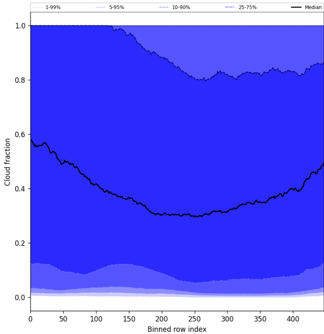
Figure 49: Along track statistics of “Cloud fraction” for 2025-01-24 to 2025-01-26
