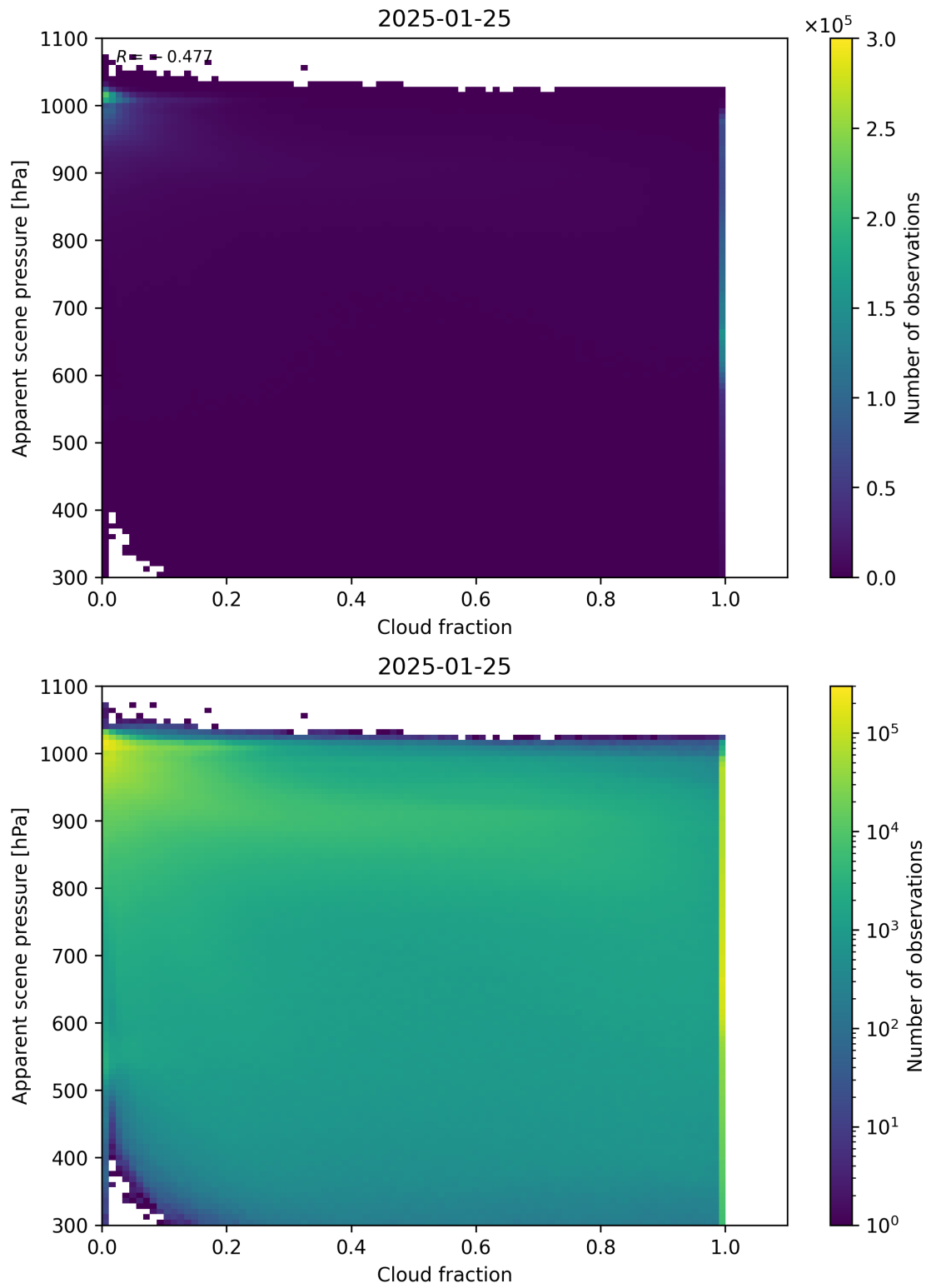
Figure 70: Scatter density plot of “Cloud fraction” against “Apparent scene pressure” for 2025-01-24 to 2025-01-26.
