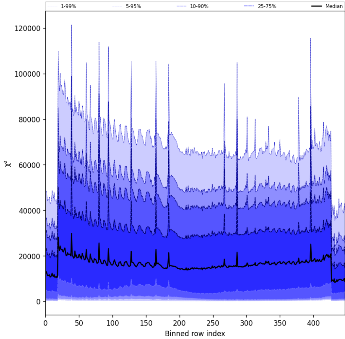
Figure 55: Along track statistics of “ \chi^2 ” for 2025-01-24 to 2025-01-26
