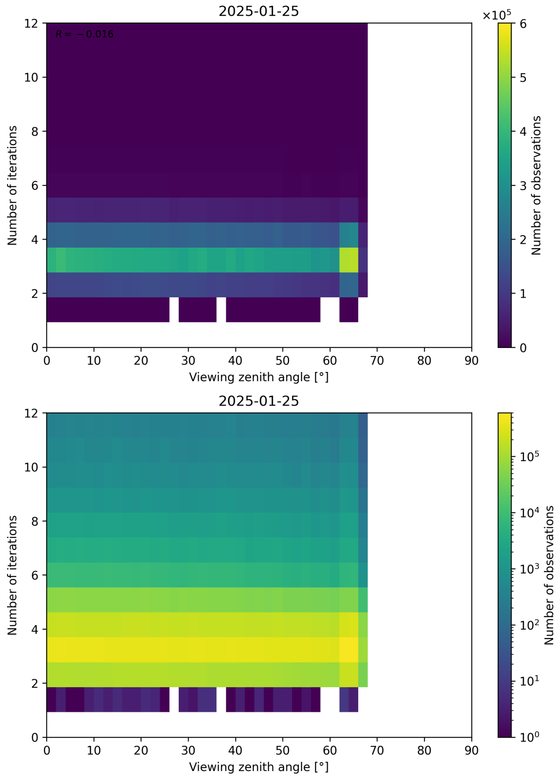
Figure 124: Scatter density plot of “Viewing zenith angle” against “Number of iterations” for 2025-01-24 to 2025-01-26.
