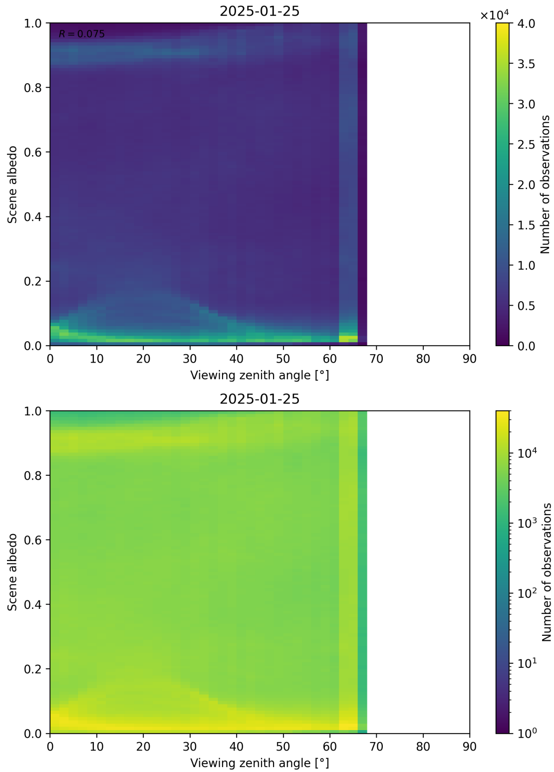
Figure 126: Scatter density plot of “Viewing zenith angle” against “Scene albedo” for 2025-01-24 to 2025-01-26.
