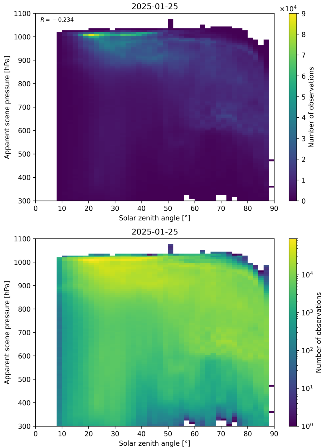
Figure 108: Scatter density plot of “Solar zenith angle” against “Apparent scene pressure” for 2025-01-24 to 2025-01-26.
