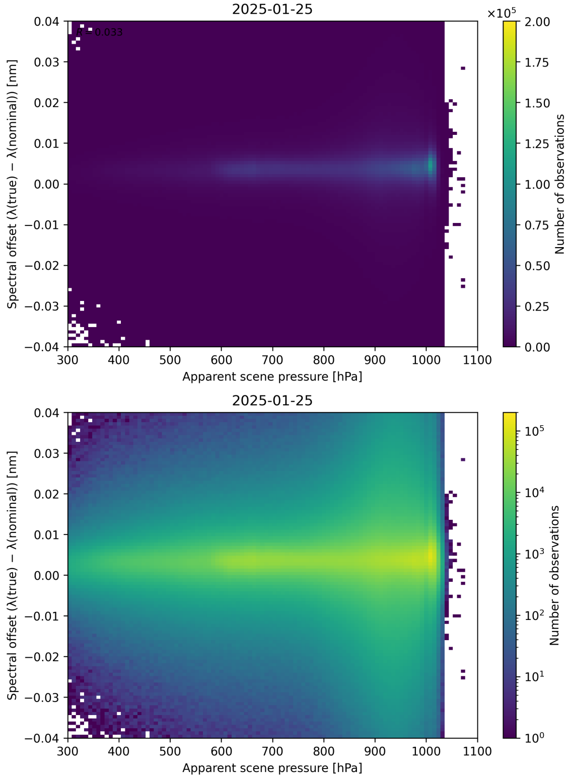
Figure 67: Scatter density plot of “Apparent scene pressure” against “Spectral offset ( \lambda_{\text{true}} - \lambda_{\text{nominal}} )” for 2025-01-24 to 2025-01-26.
