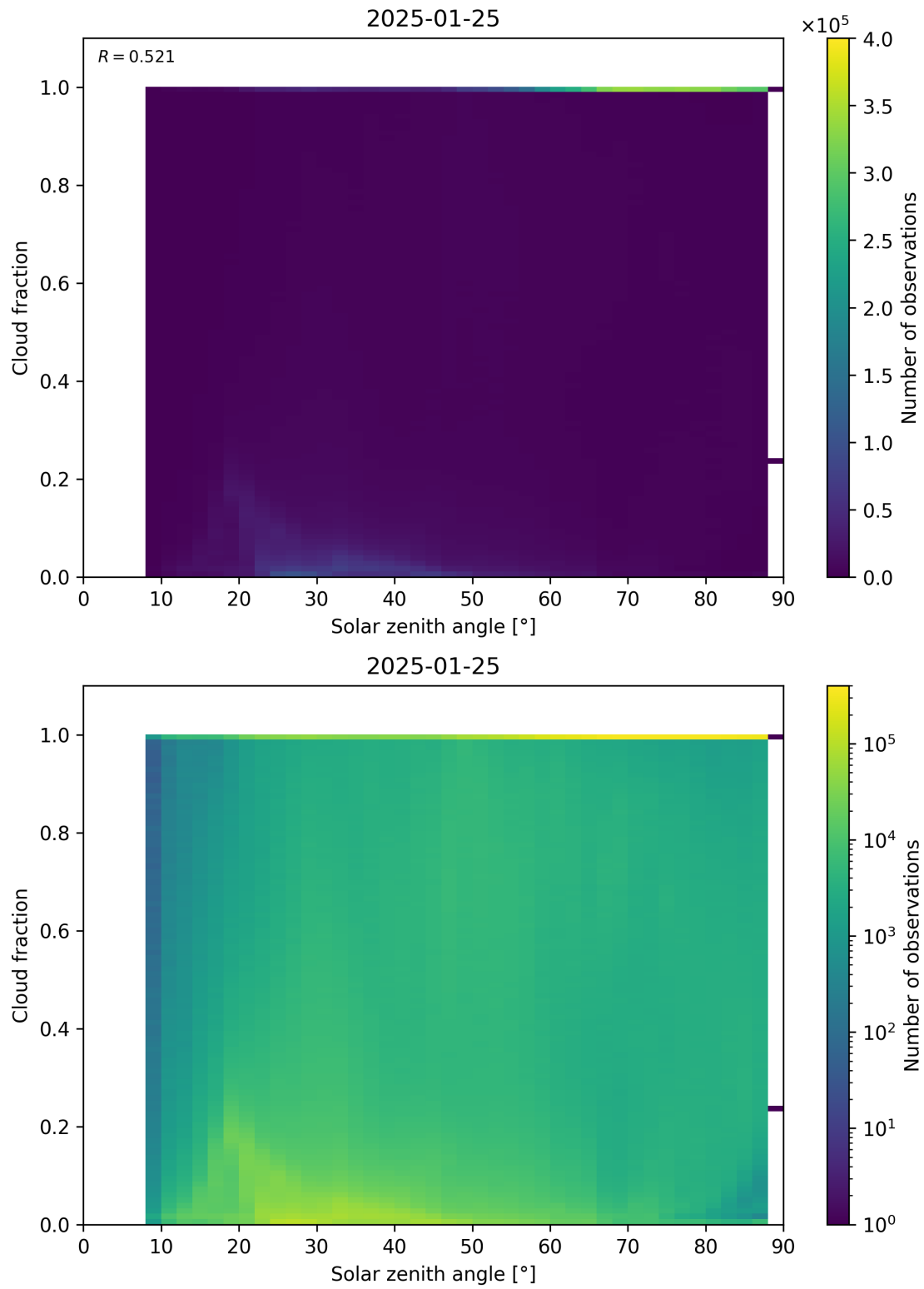
Figure 110: Scatter density plot of “Solar zenith angle” against “Cloud fraction” for 2025-01-24 to 2025-01-26.
