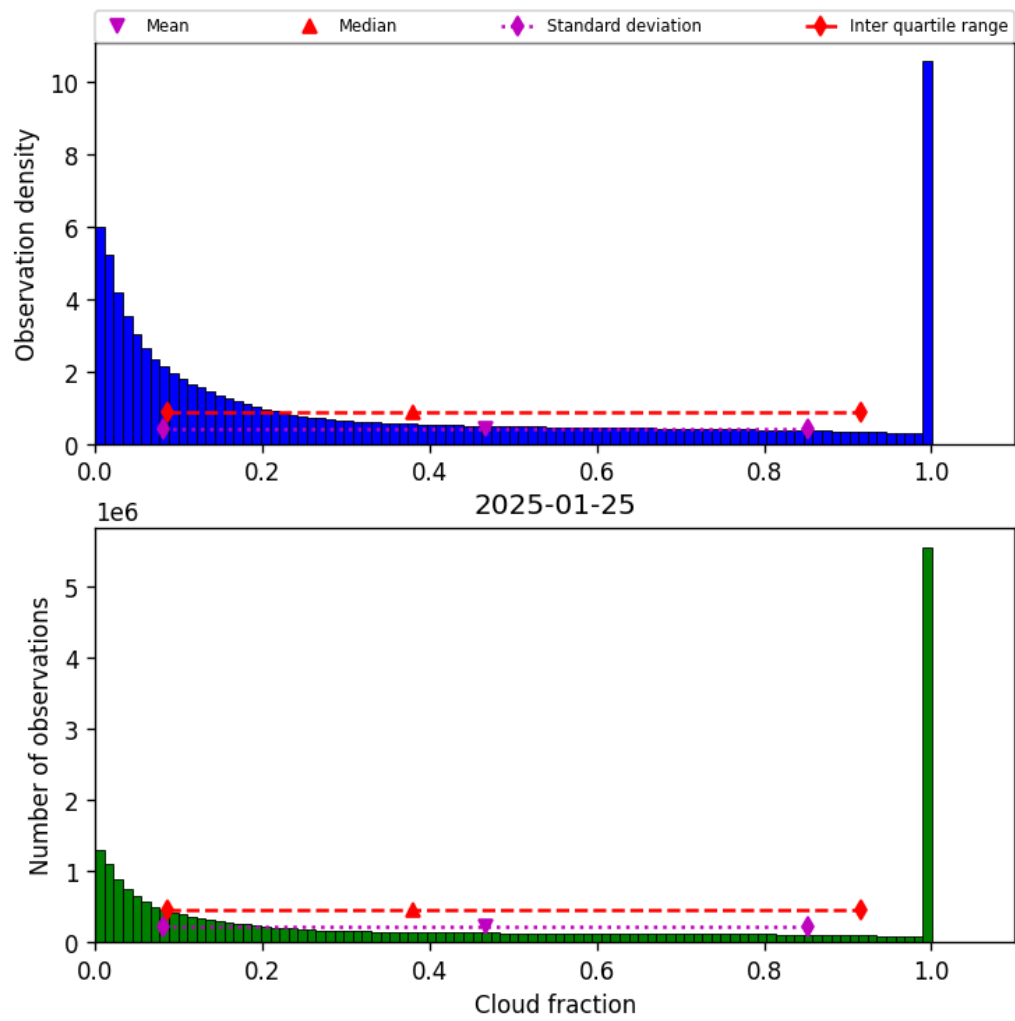
Figure 32: Histogram of “Cloud fraction” for 2025-01-24 to 2025-01-26
