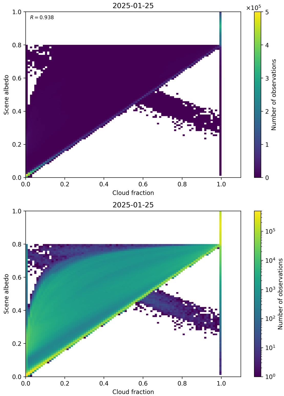
Figure 75: Scatter density plot of “Cloud fraction” against “Scene albedo” for 2025-01-24 to 2025-01-26.
