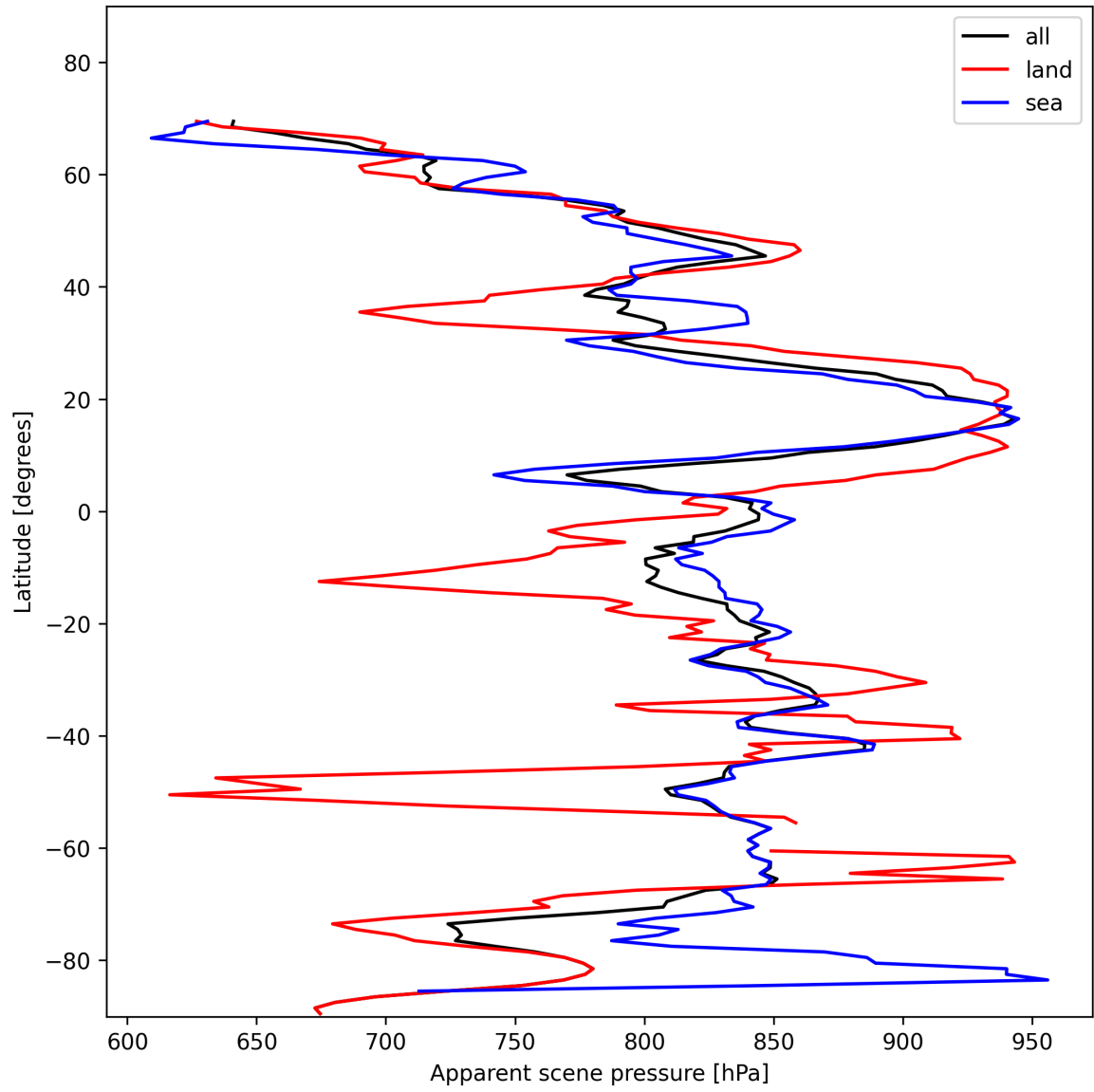
Figure 19: Zonal average of “Apparent scene pressure” for 2025-01-24 to 2025-01-26.
