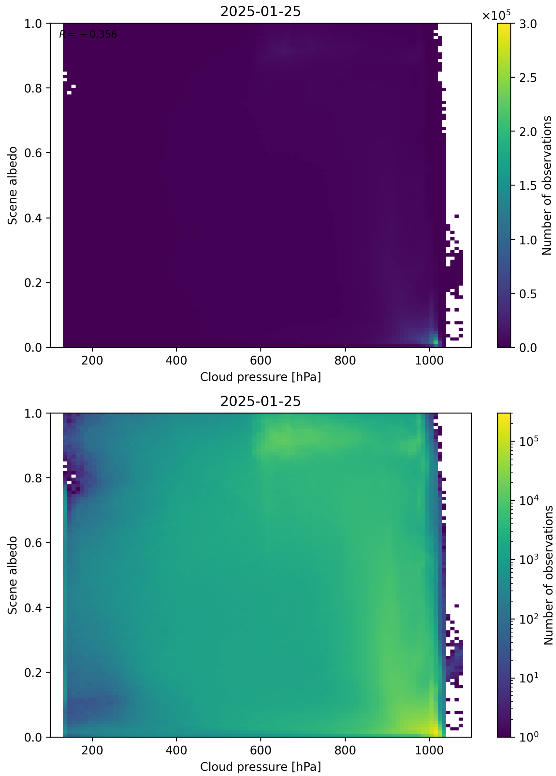
Figure 83: Scatter density plot of “Cloud pressure” against “Scene albedo” for 2025-01-24 to 2025-01-26.
