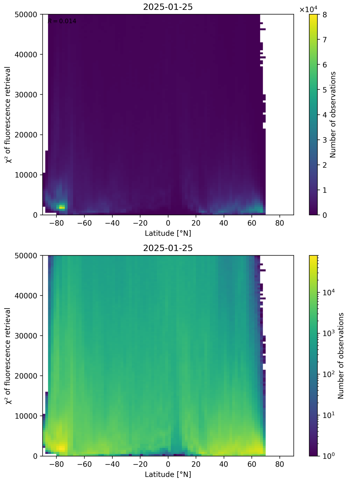
Figure 89: Scatter density plot of “Latitude” against “ \chi^2 of fluorescence retrieval” for 2025-01-24 to 2025-01-26.
