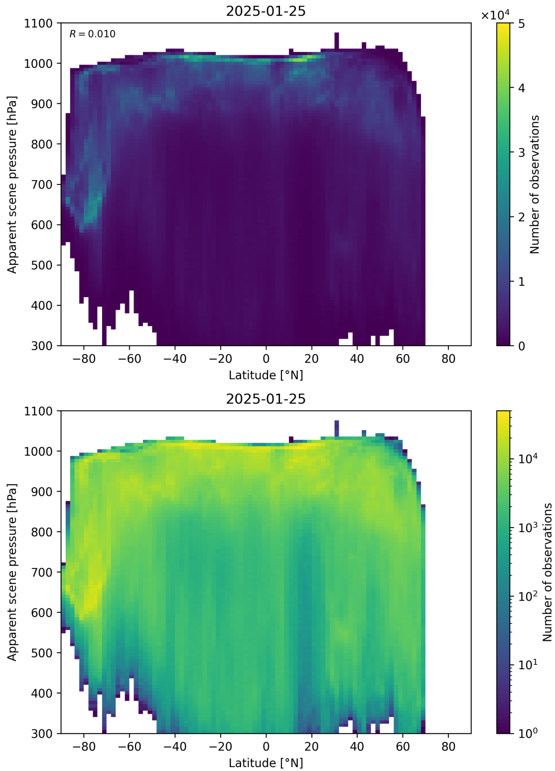
Figure 88: Scatter density plot of “Latitude” against “Apparent scene pressure” for 2025-01-24 to 2025-01-26.
