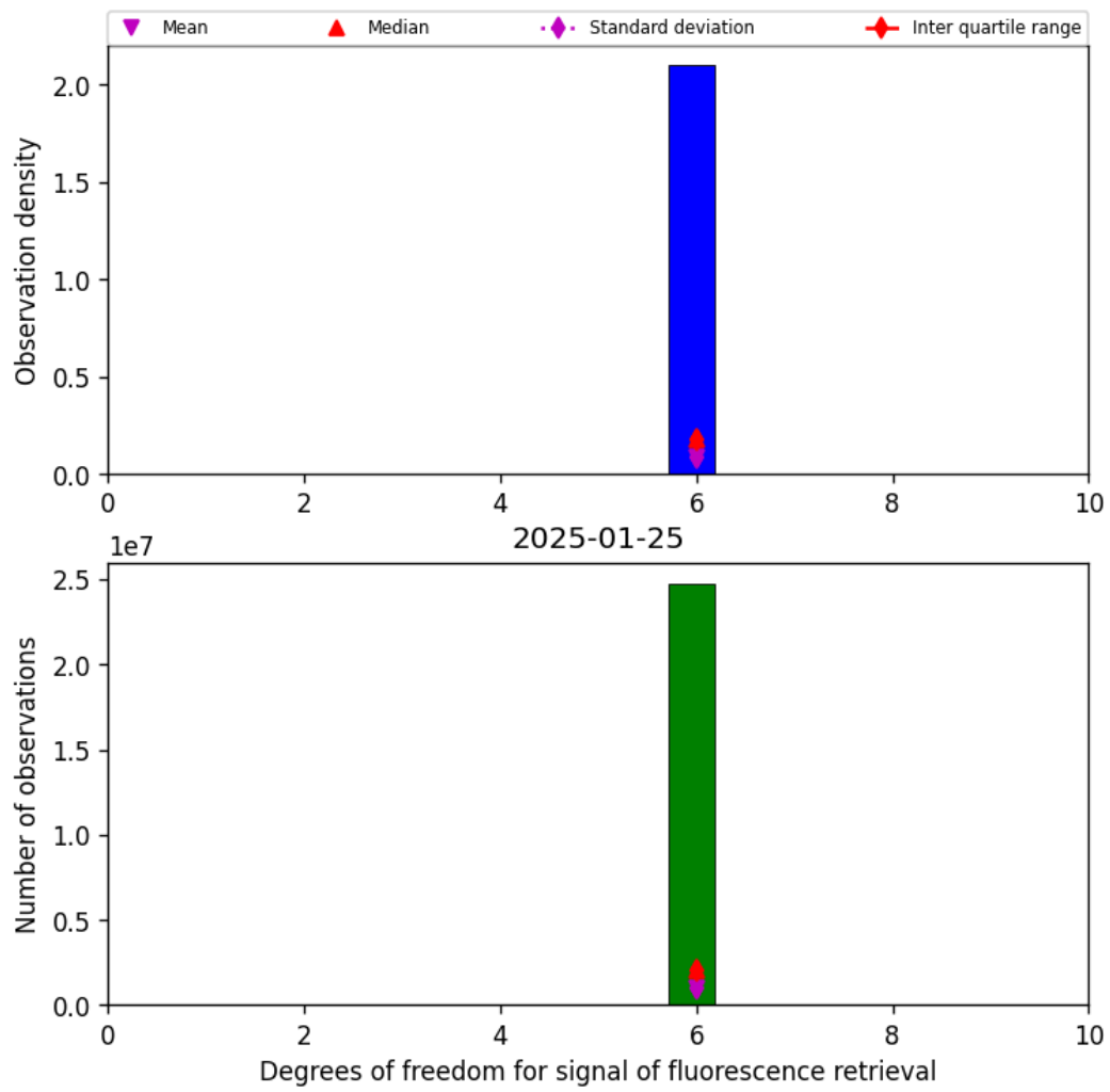
Figure 43: Histogram of “Degrees of freedom for signal of fluorescence retrieval” for 2025-01-24 to 2025-01-26
