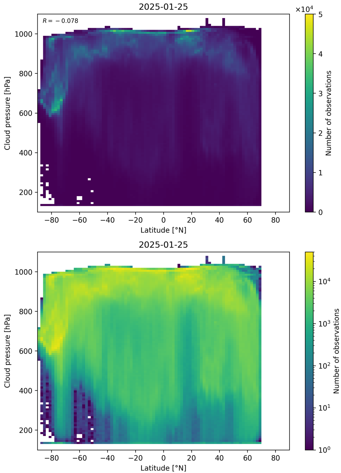
Figure 91: Scatter density plot of “Latitude” against “Cloud pressure” for 2025-01-24 to 2025-01-26.
