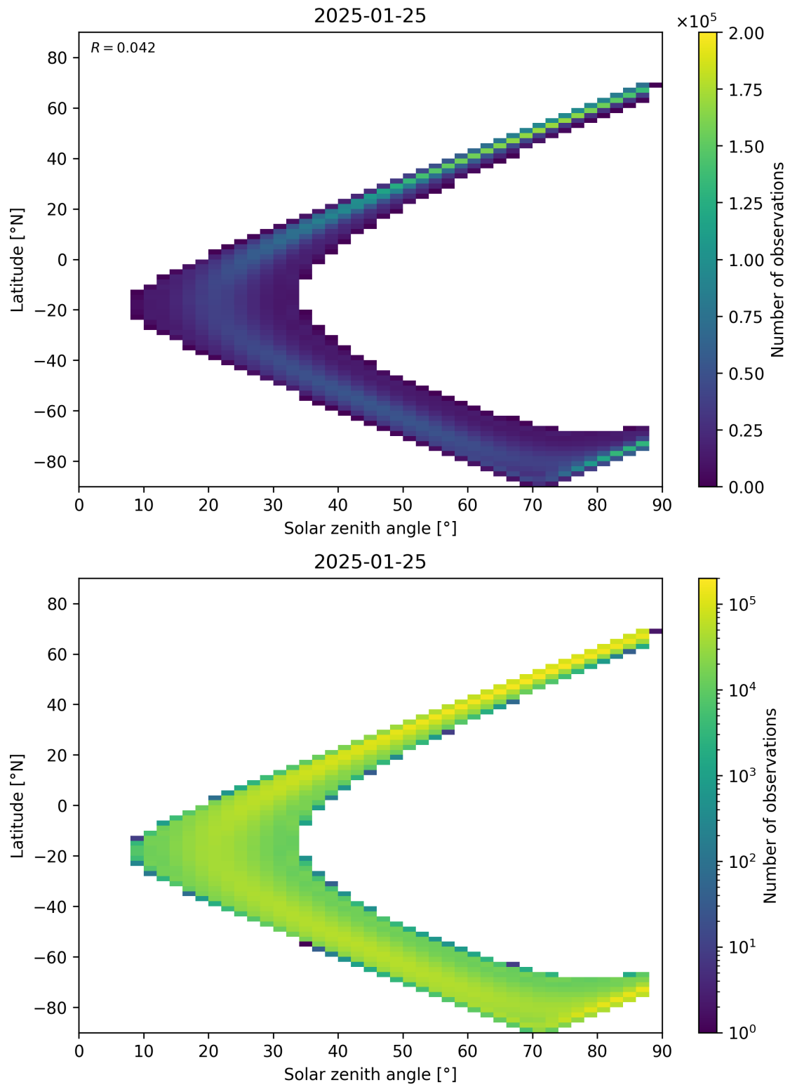
Figure 113: Scatter density plot of “Solar zenith angle” against “Latitude” for 2025-01-24 to 2025-01-26.
