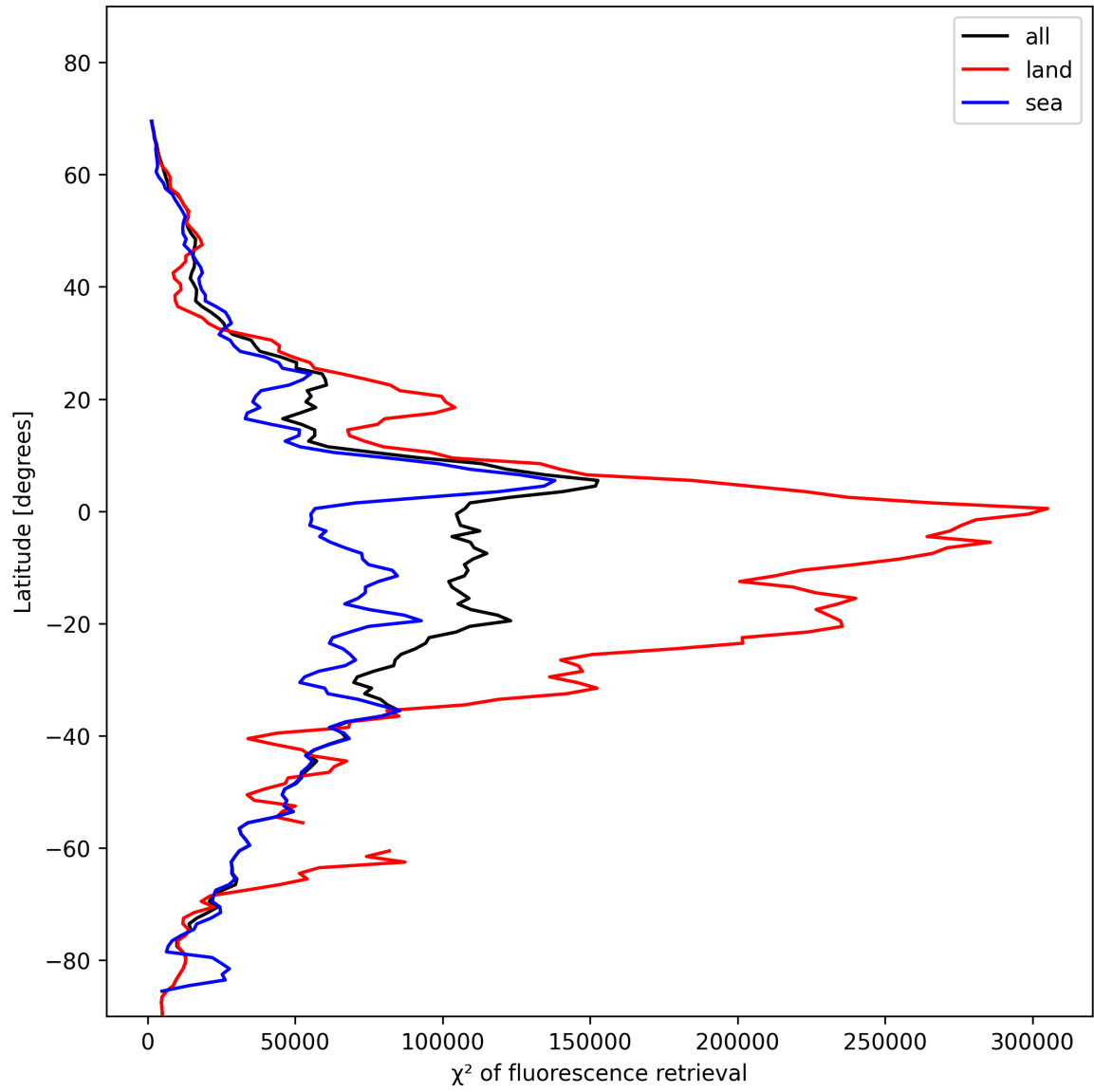
Figure 25: Zonal average of “ \chi^2 of fluorescence retrieval” for 2025-01-24 to 2025-01-26.
