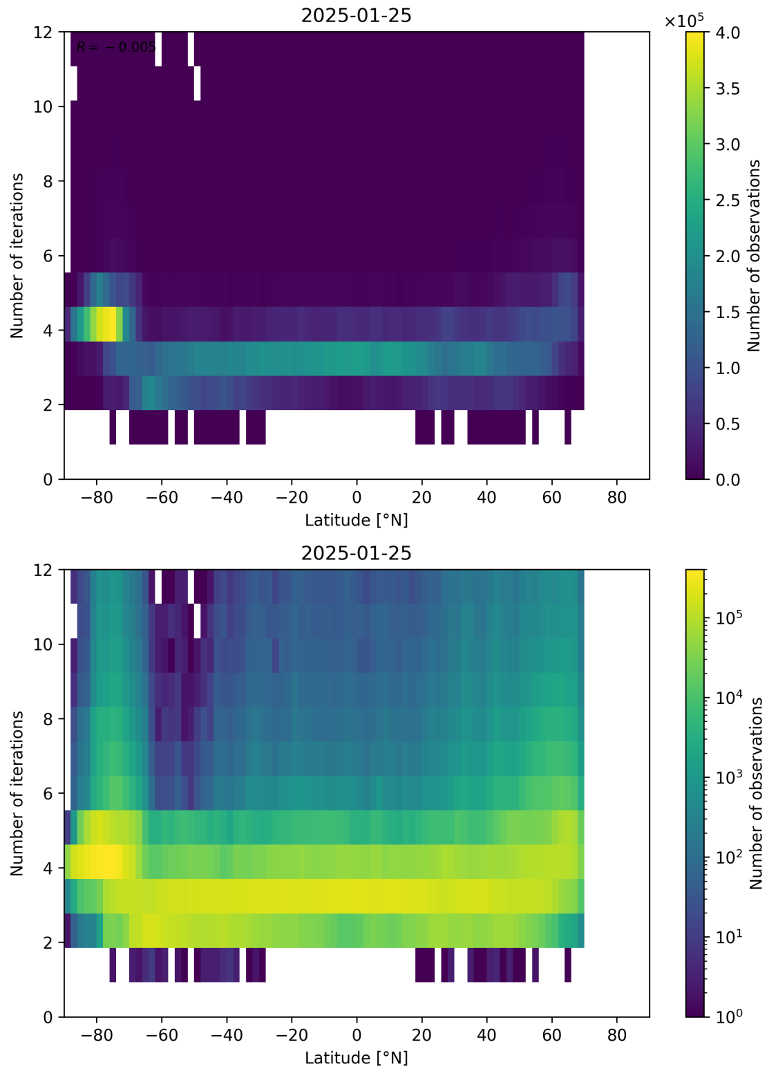
Figure 93: Scatter density plot of “Latitude” against “Number of iterations” for 2025-01-24 to 2025-01-26.
