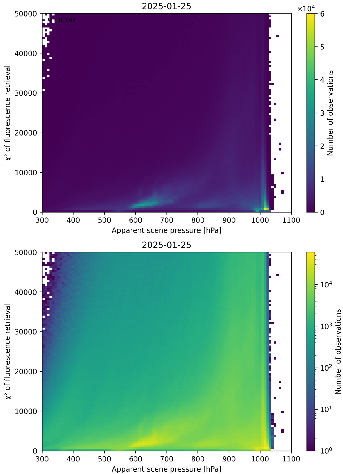
Figure 63: Scatter density plot of “Apparent scene pressure” against “ \chi^2 of fluorescence retrieval” for 2025-01-24 to 2025-01-26.
