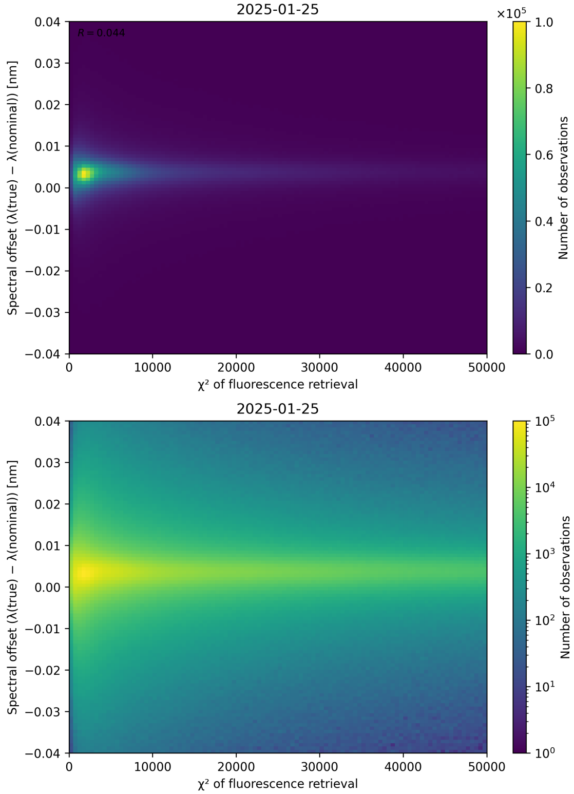
Figure 69: Scatter density plot of “ \chi^2 of fluorescence retrieval” against “Spectral offset ( \lambda_{\text{true}} - \lambda_{\text{nominal}} )” for 2025-01-24 to 2025-01-26.
