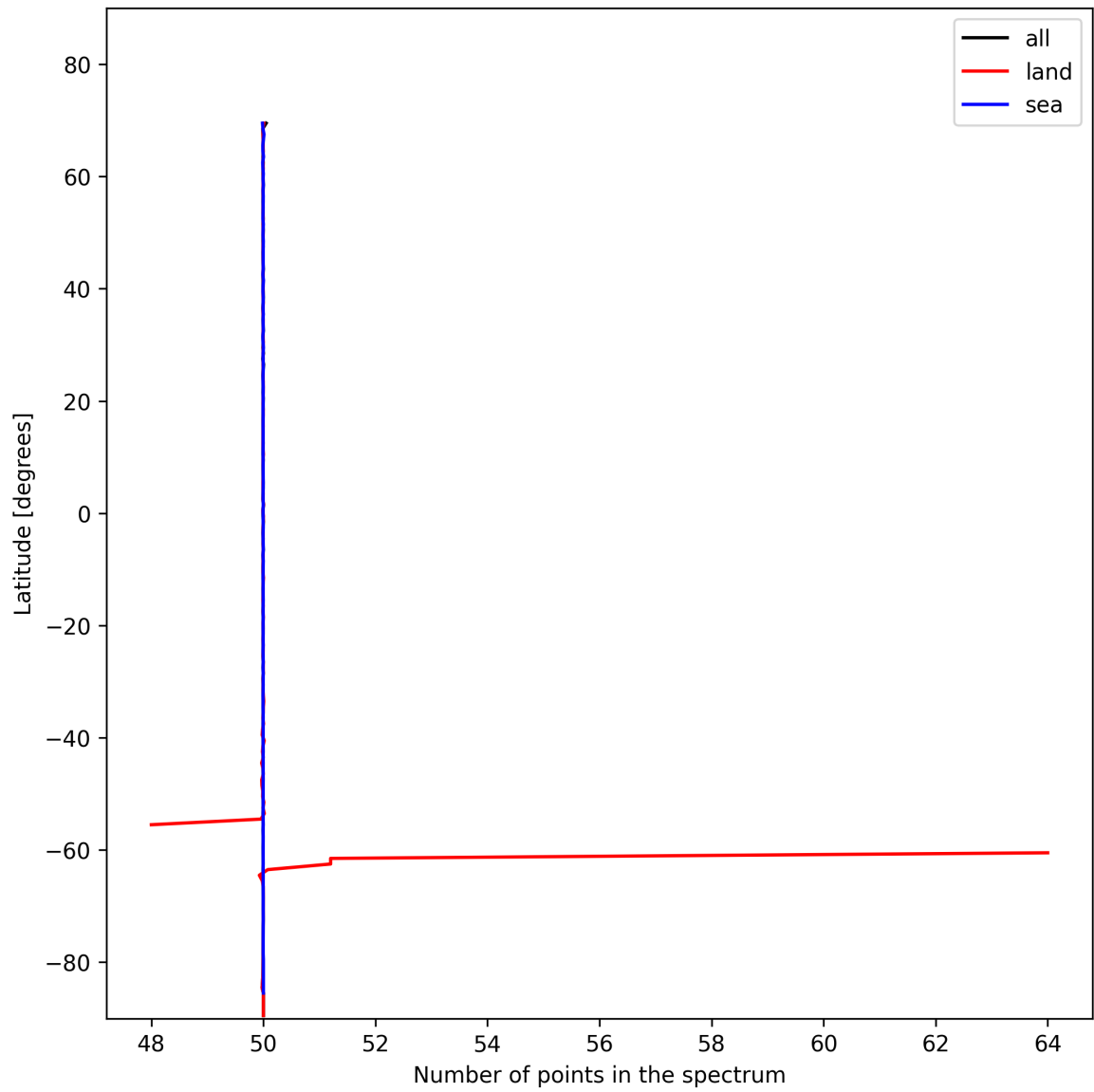
Figure 27: Zonal average of “Number of points in the spectrum” for 2025-01-24 to 2025-01-26.
