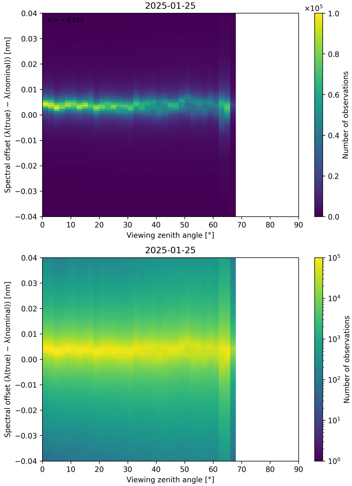
Figure 128: Scatter density plot of “Viewing zenith angle” against “Spectral offset ( \lambda_{\text{true}} - \lambda_{\text{nominal}} )” for 2025-01-24 to 2025-01-26.
