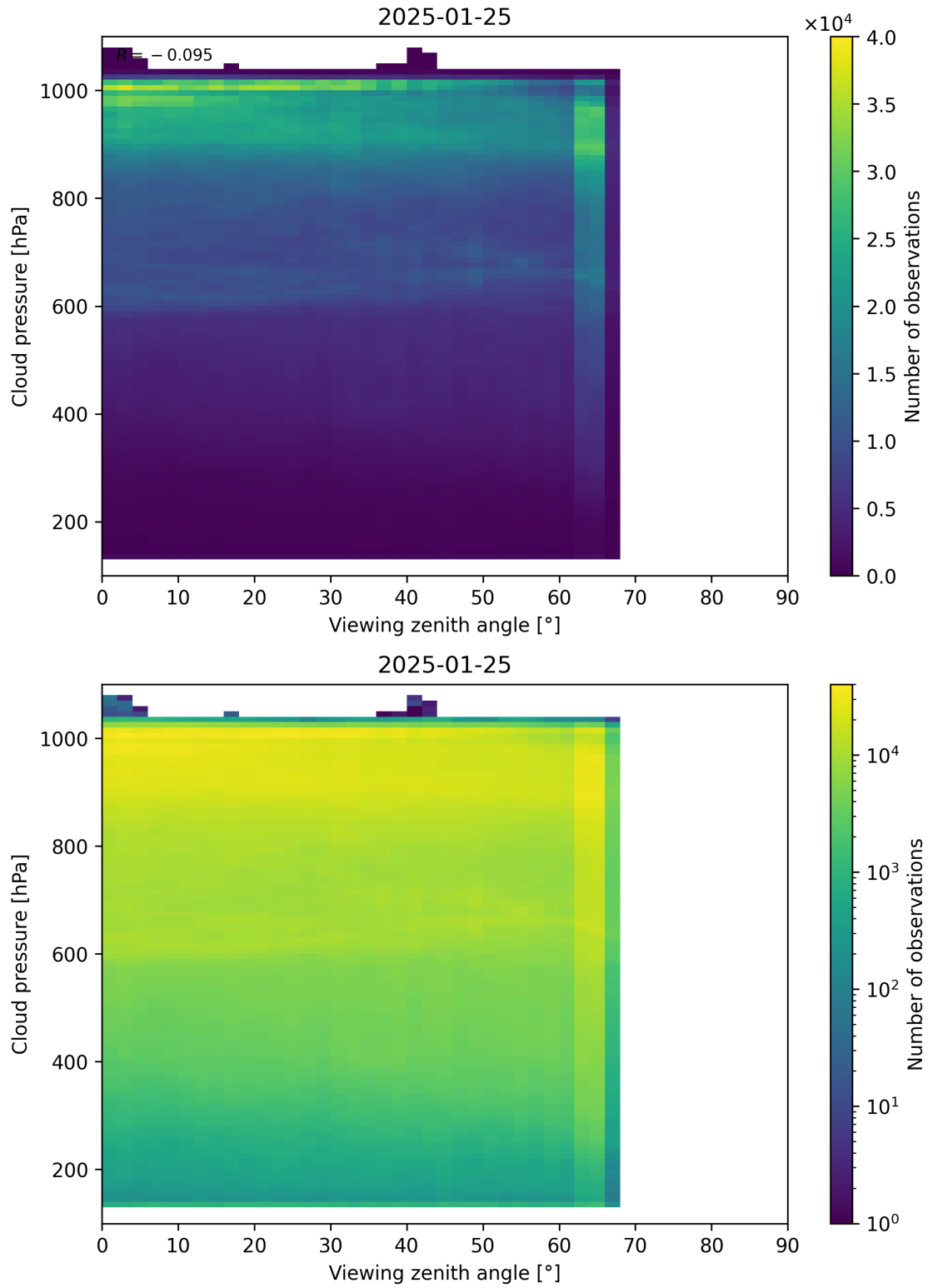
Figure 121: Scatter density plot of “Viewing zenith angle” against “Cloud pressure” for 2025-01-24 to 2025-01-26.
