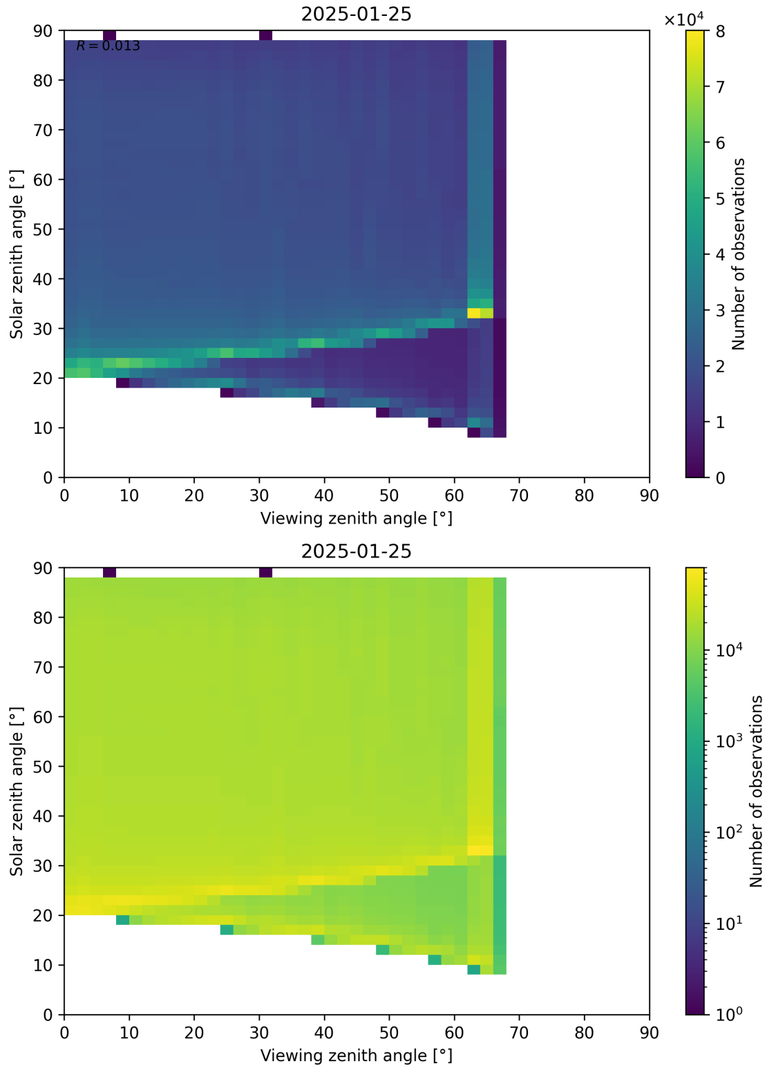
Figure 127: Scatter density plot of “Viewing zenith angle” against “Solar zenith angle” for 2025-01-24 to 2025-01-26.
