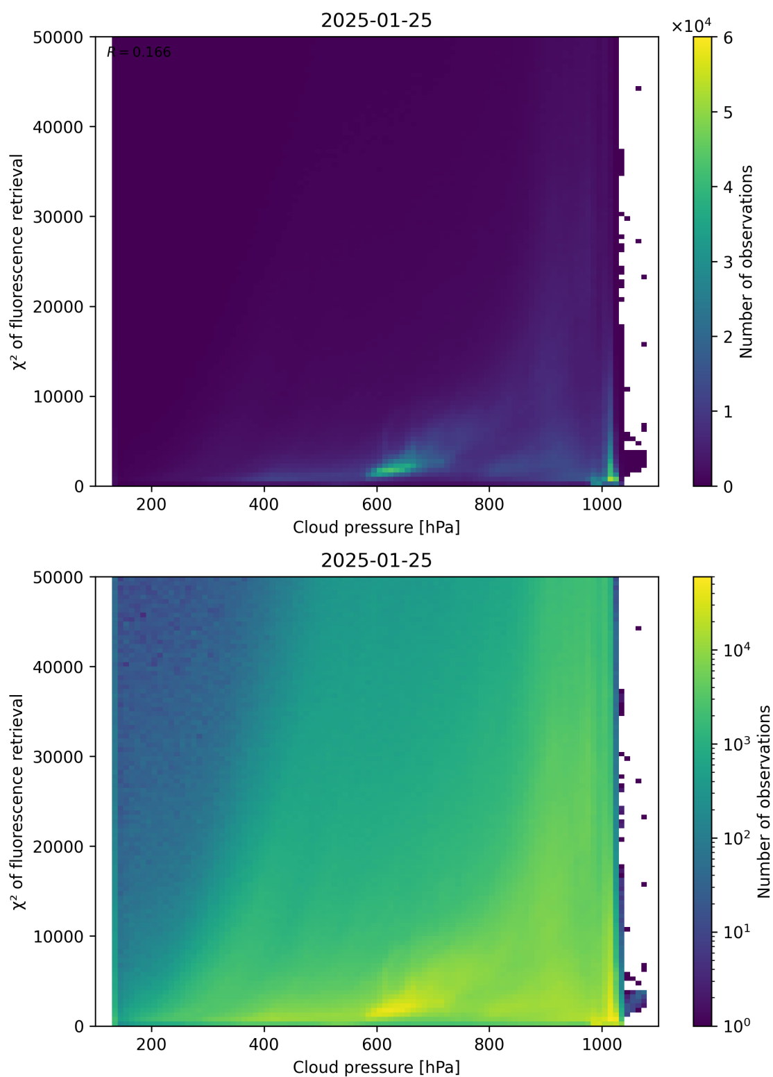
Figure 78: Scatter density plot of “Cloud pressure” against “ \chi^2 of fluorescence retrieval” for 2025-01-24 to 2025-01-26.
