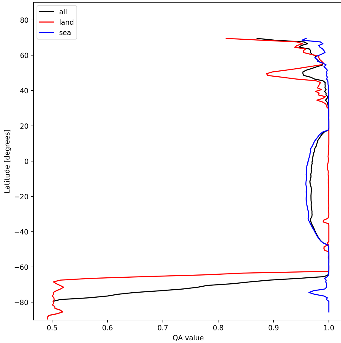
Figure 12: Zonal average of “QA value” for 2025-01-24 to 2025-01-26.
