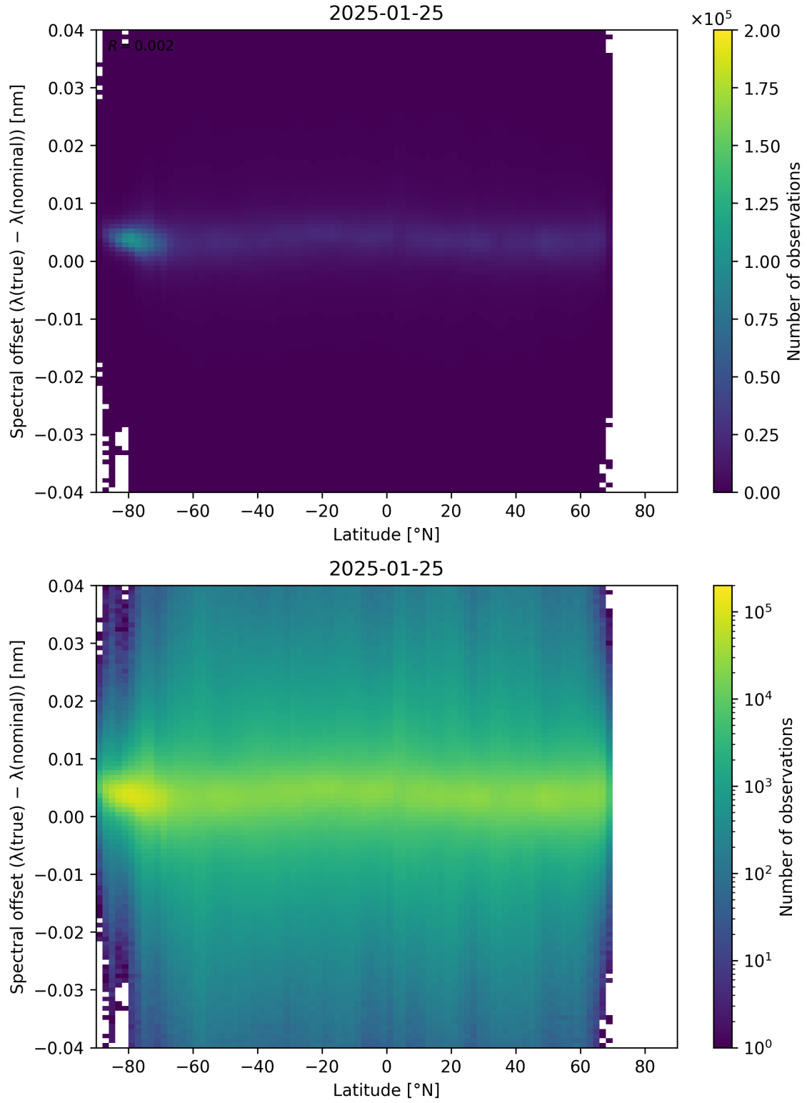
Figure 96: Scatter density plot of “Latitude” against “Spectral offset ( \lambda_{\text{true}} - \lambda_{\text{nominal}} )” for 2025-01-24 to 2025-01-26.
