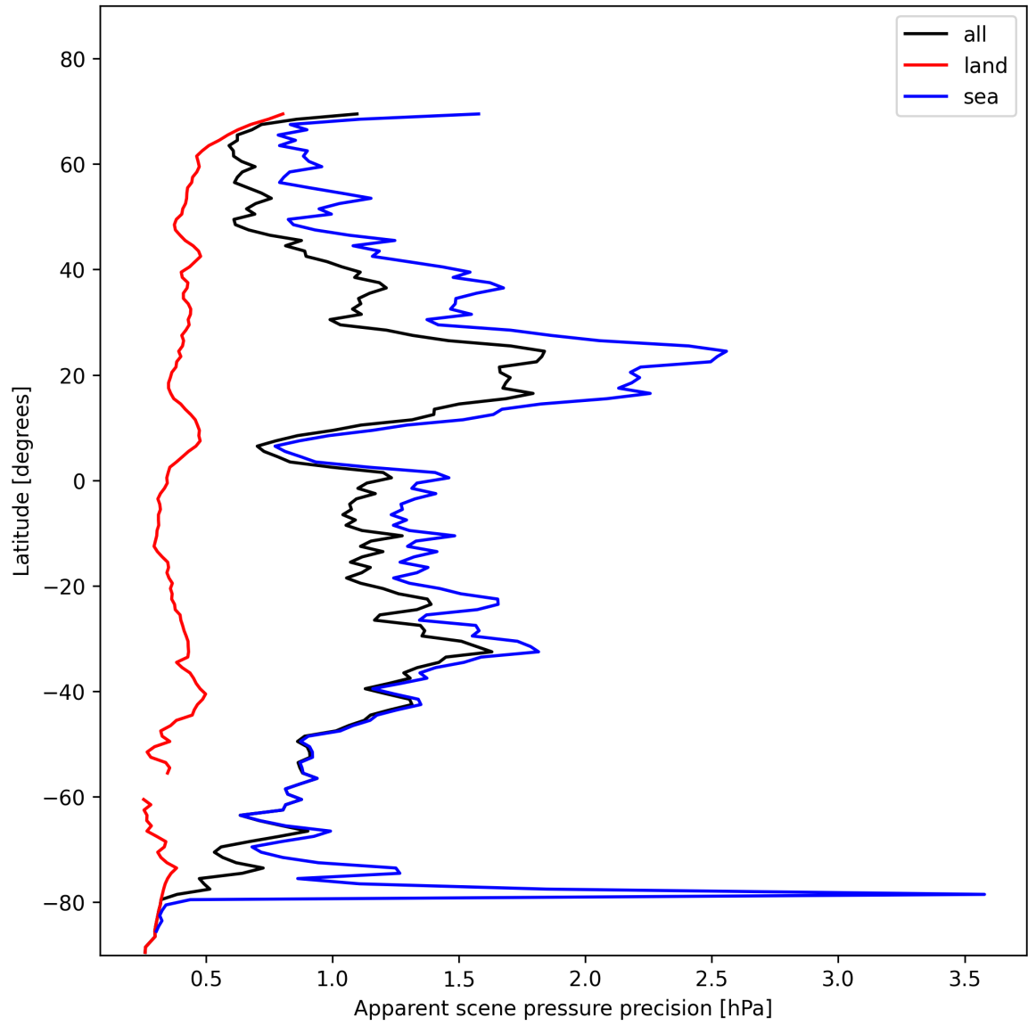
Figure 20: Zonal average of “Apparent scene pressure precision” for 2025-01-24 to 2025-01-26.
