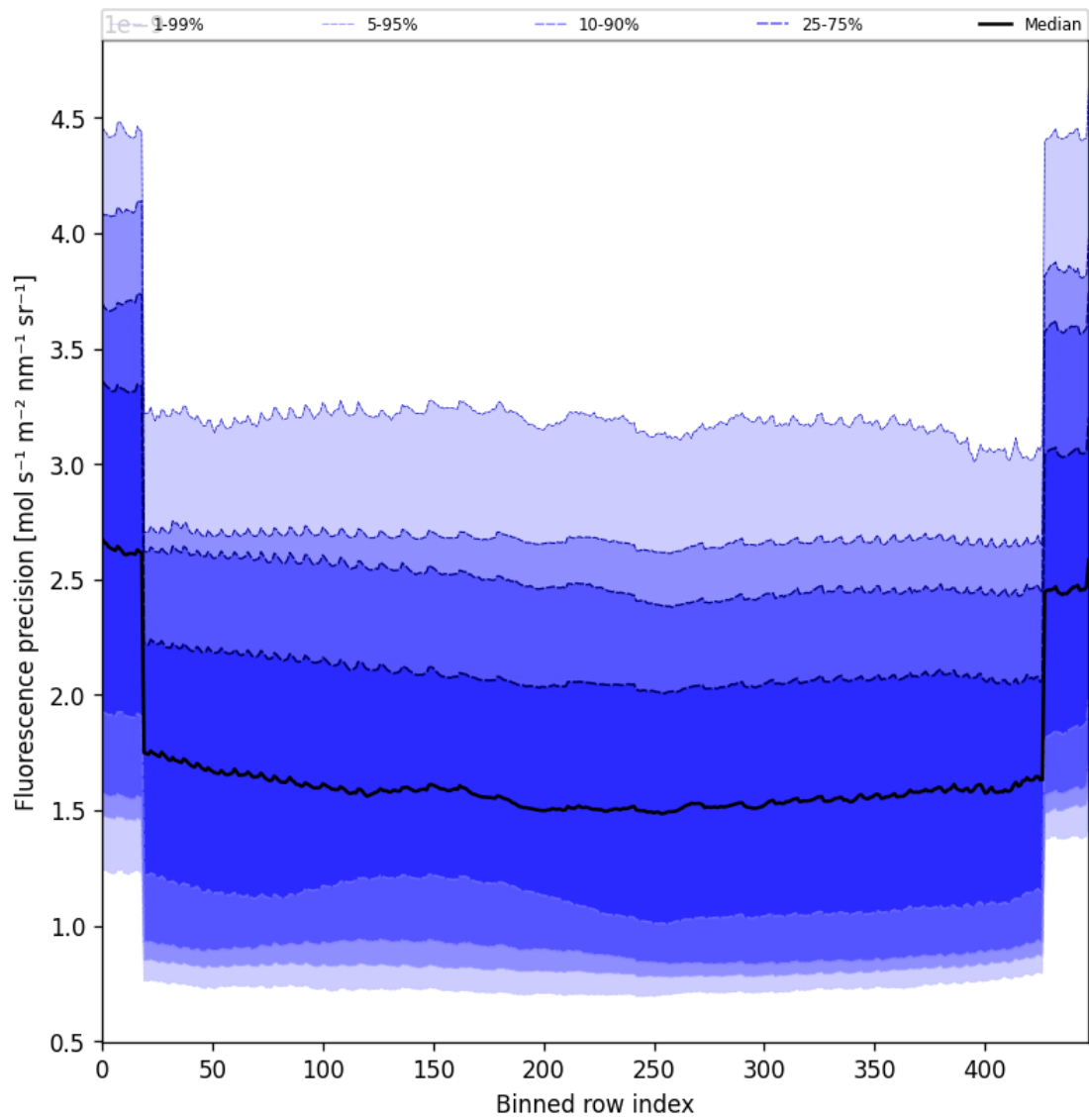
Figure 58: Along track statistics of “Fluorescence precision” for 2025-01-24 to 2025-01-26
