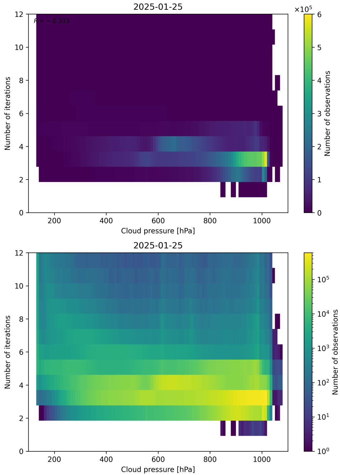
Figure 81: Scatter density plot of “Cloud pressure” against “Number of iterations” for 2025-01-24 to 2025-01-26.
