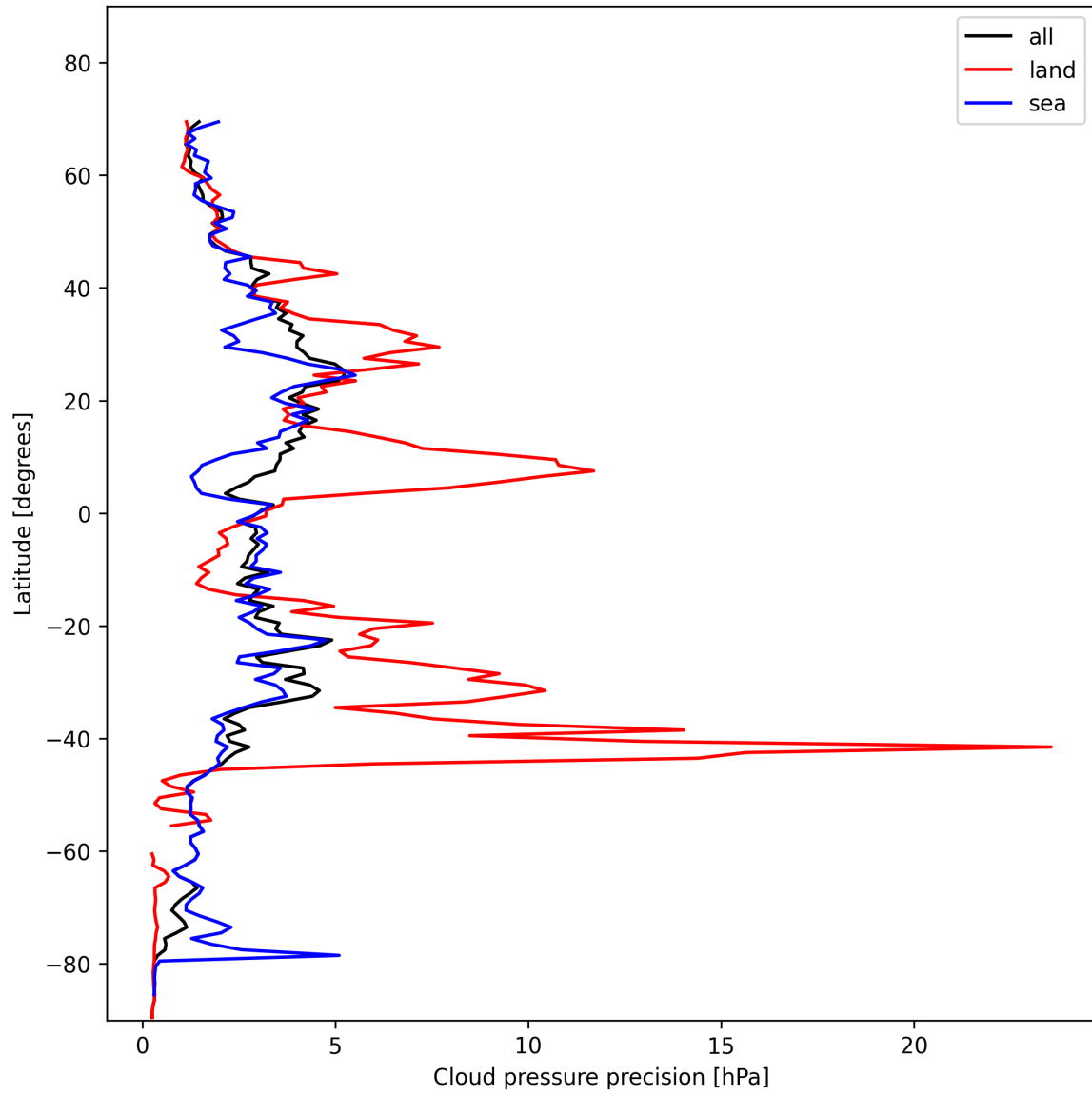
Figure 14: Zonal average of “Cloud pressure precision” for 2025-01-24 to 2025-01-26.
