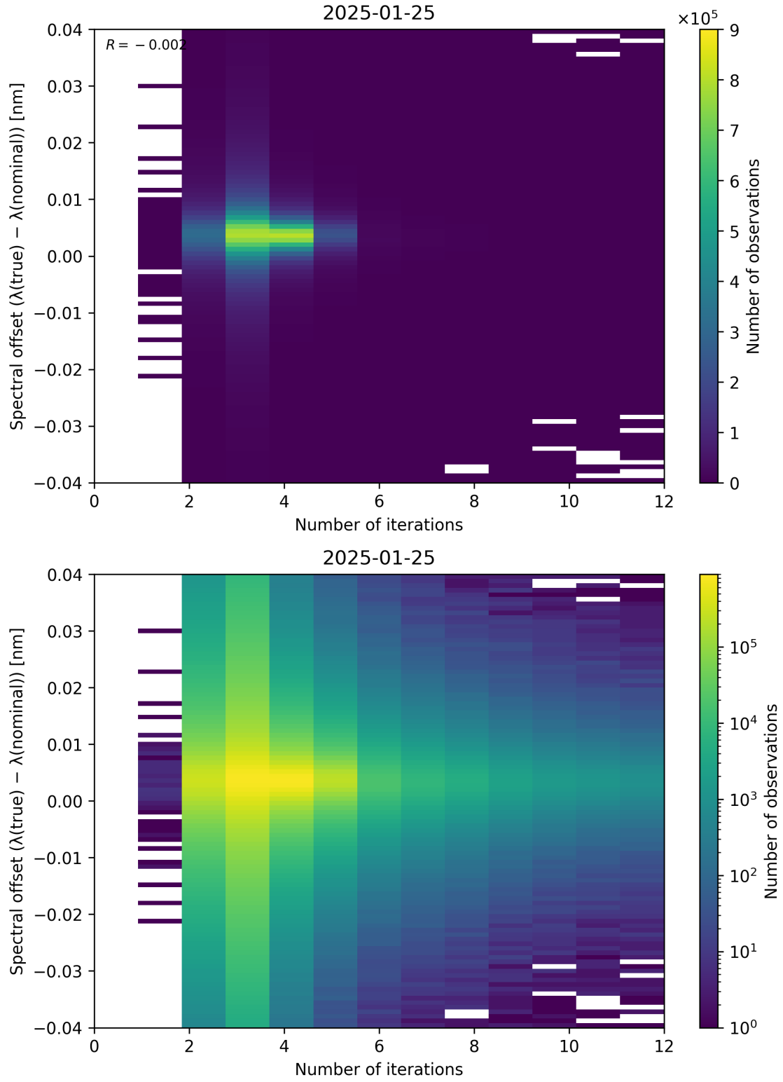
Figure 100: Scatter density plot of “Number of iterations” against “Spectral offset ( \lambda_{\text{true}} - \lambda_{\text{nominal}} )” for 2025-01-24 to 2025-01-26.
