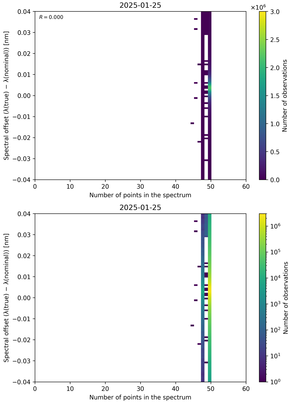
Figure 101: Scatter density plot of “Number of points in the spectrum” against “Spectral offset ( \lambda_{\text{true}} - \lambda_{\text{nominal}} )” for 2025-01-24 to 2025-01-26.
