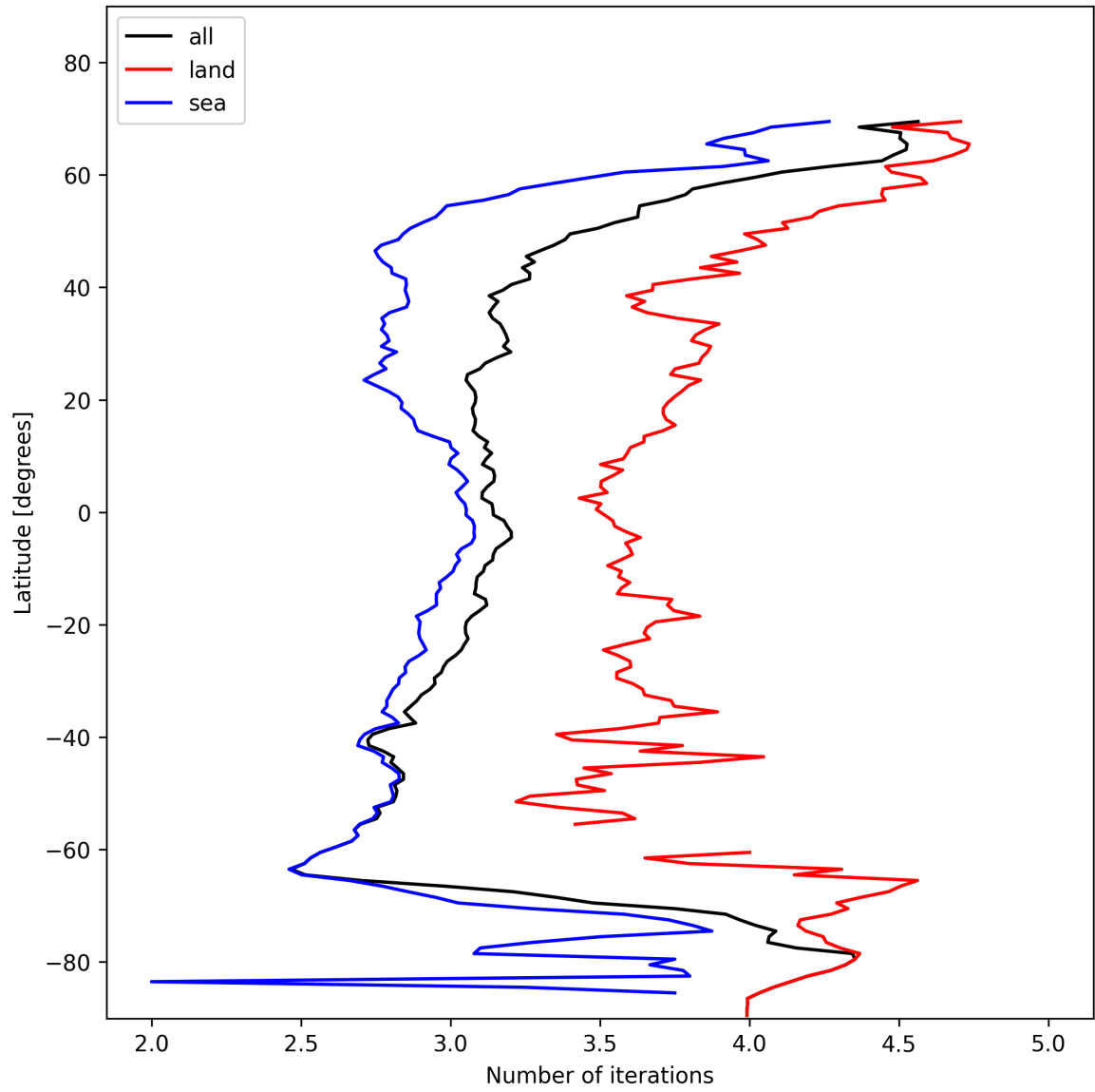
Figure 22: Zonal average of “Number of iterations” for 2025-01-24 to 2025-01-26.
