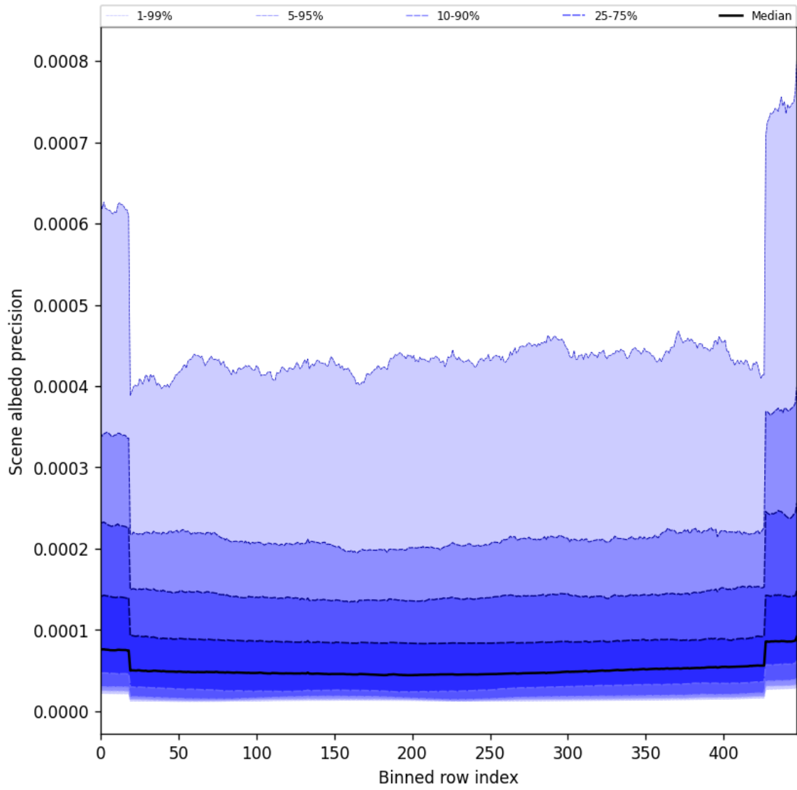
Figure 52: Along track statistics of “Scene albedo precision” for 2025-01-24 to 2025-01-26
