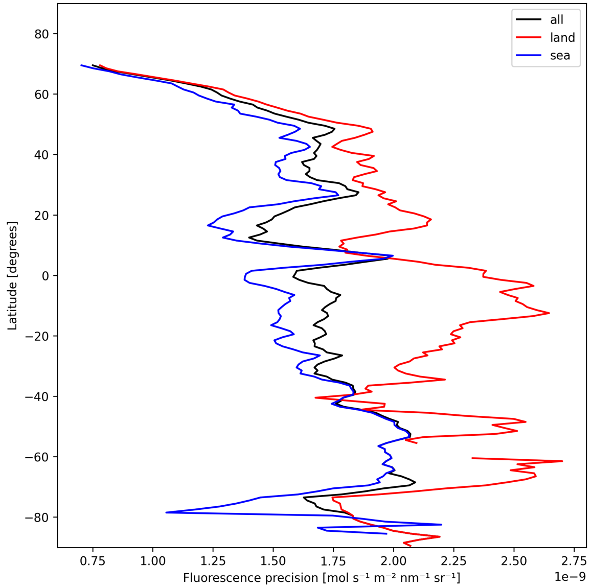
Figure 24: Zonal average of “Fluorescence precision” for 2025-01-24 to 2025-01-26.
