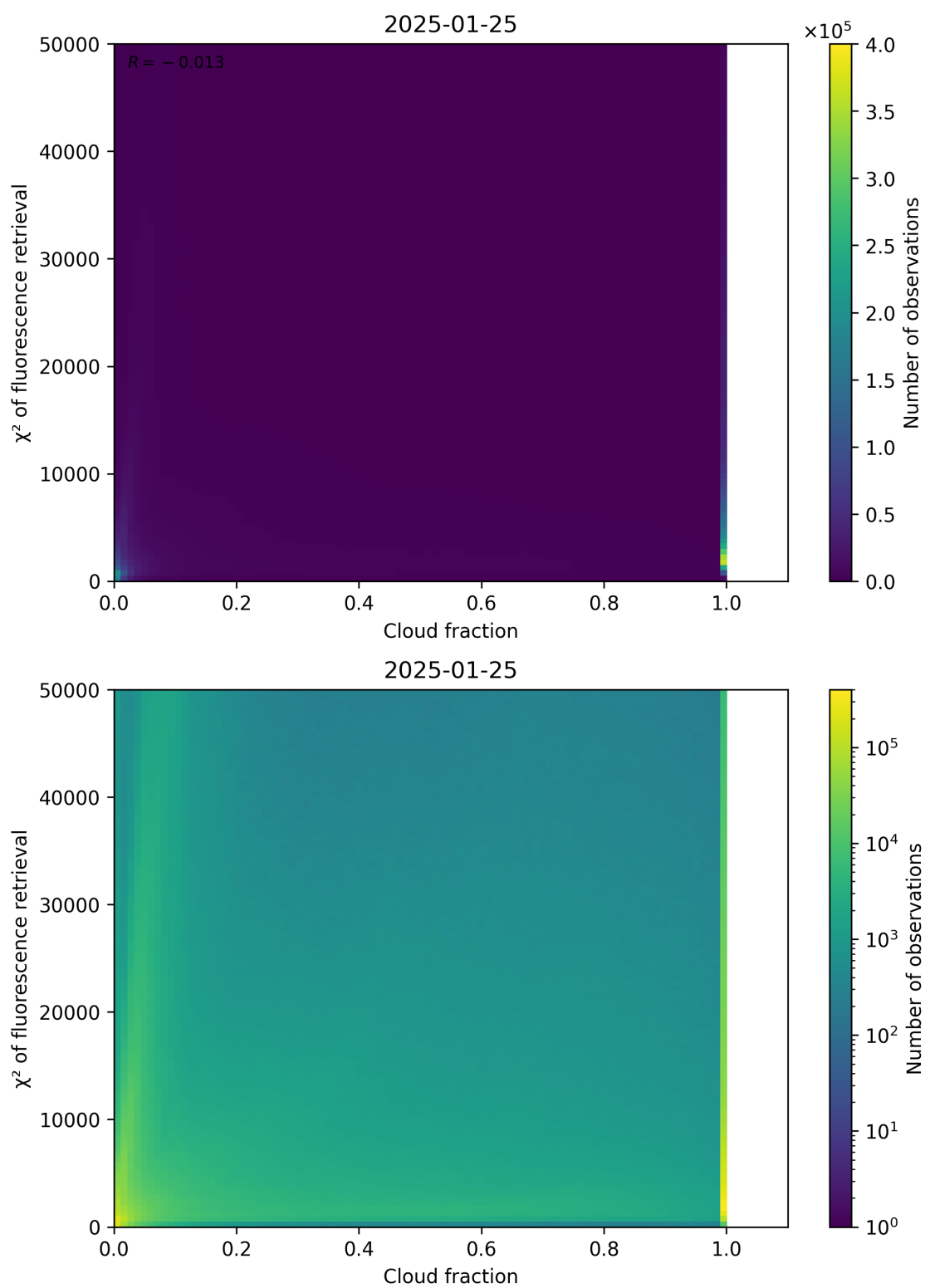
Figure 71: Scatter density plot of “Cloud fraction” against “ \chi^2 of fluorescence retrieval” for 2025-01-24 to 2025-01-26.
