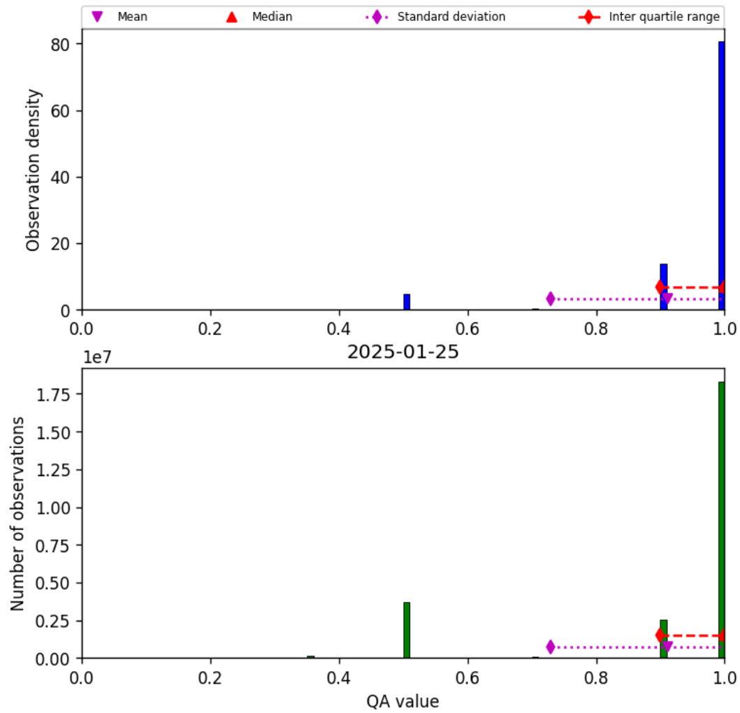
Figure 29: Histogram of “QA value” for 2025-01-24 to 2025-01-26
