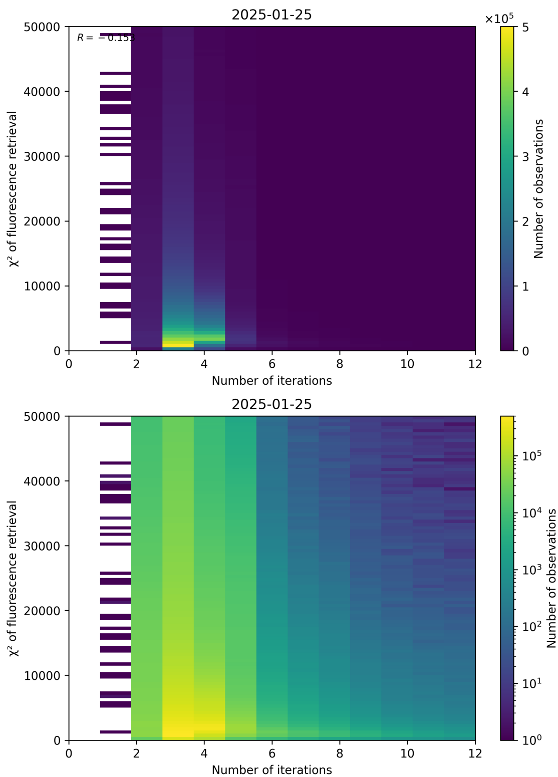
Figure 97: Scatter density plot of “Number of iterations” against “ \chi^2 of fluorescence retrieval” for 2025-01-24 to 2025-01-26.
