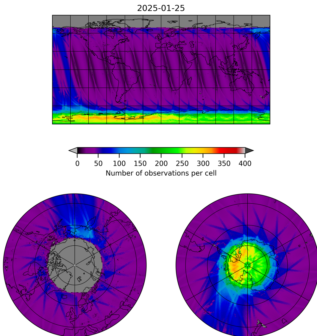
Figure 11: Map of the number of observations for 2025-01-24 to 2025-01-26
