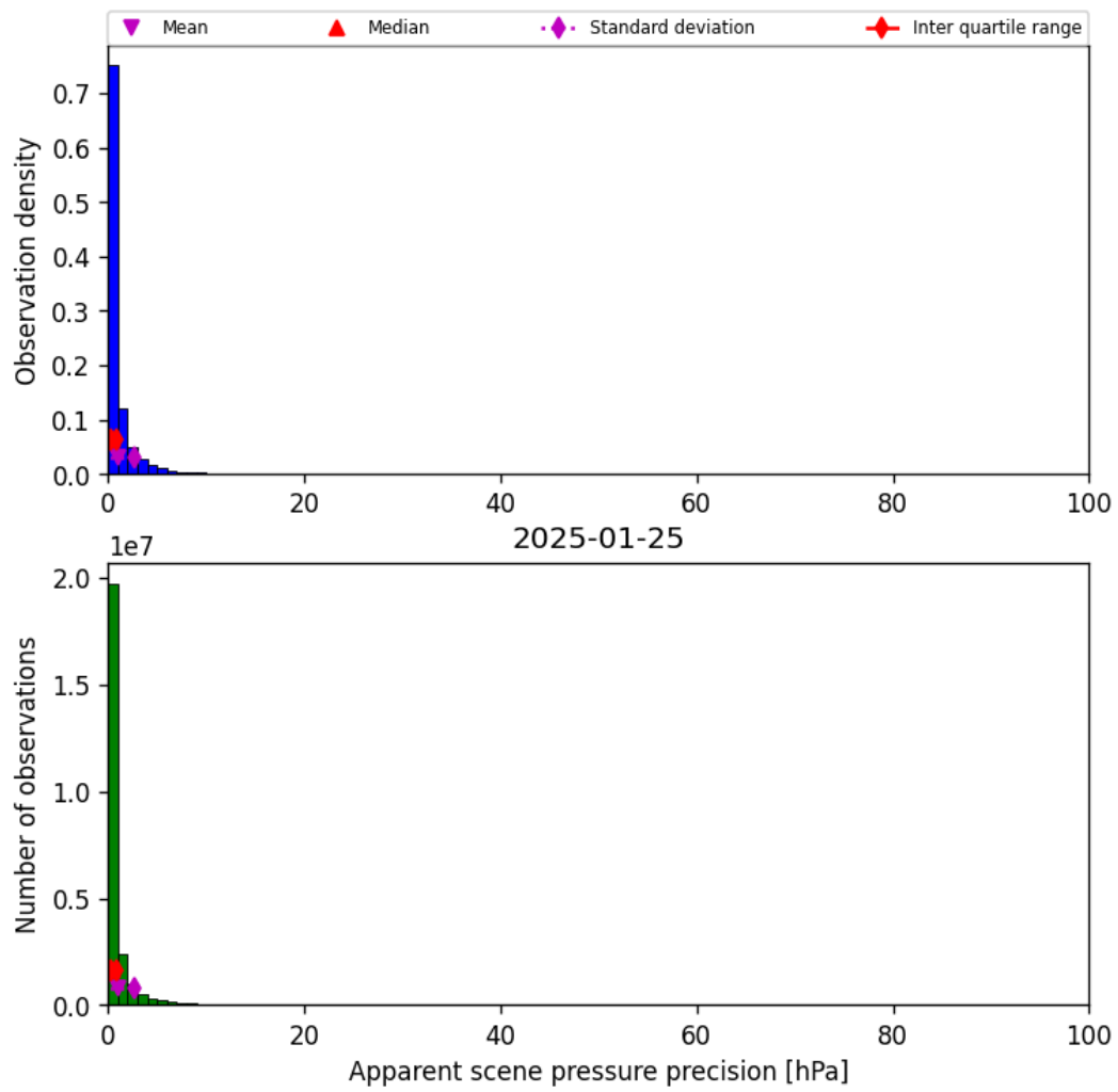
Figure 37: Histogram of “Apparent scene pressure precision” for 2025-01-24 to 2025-01-26
