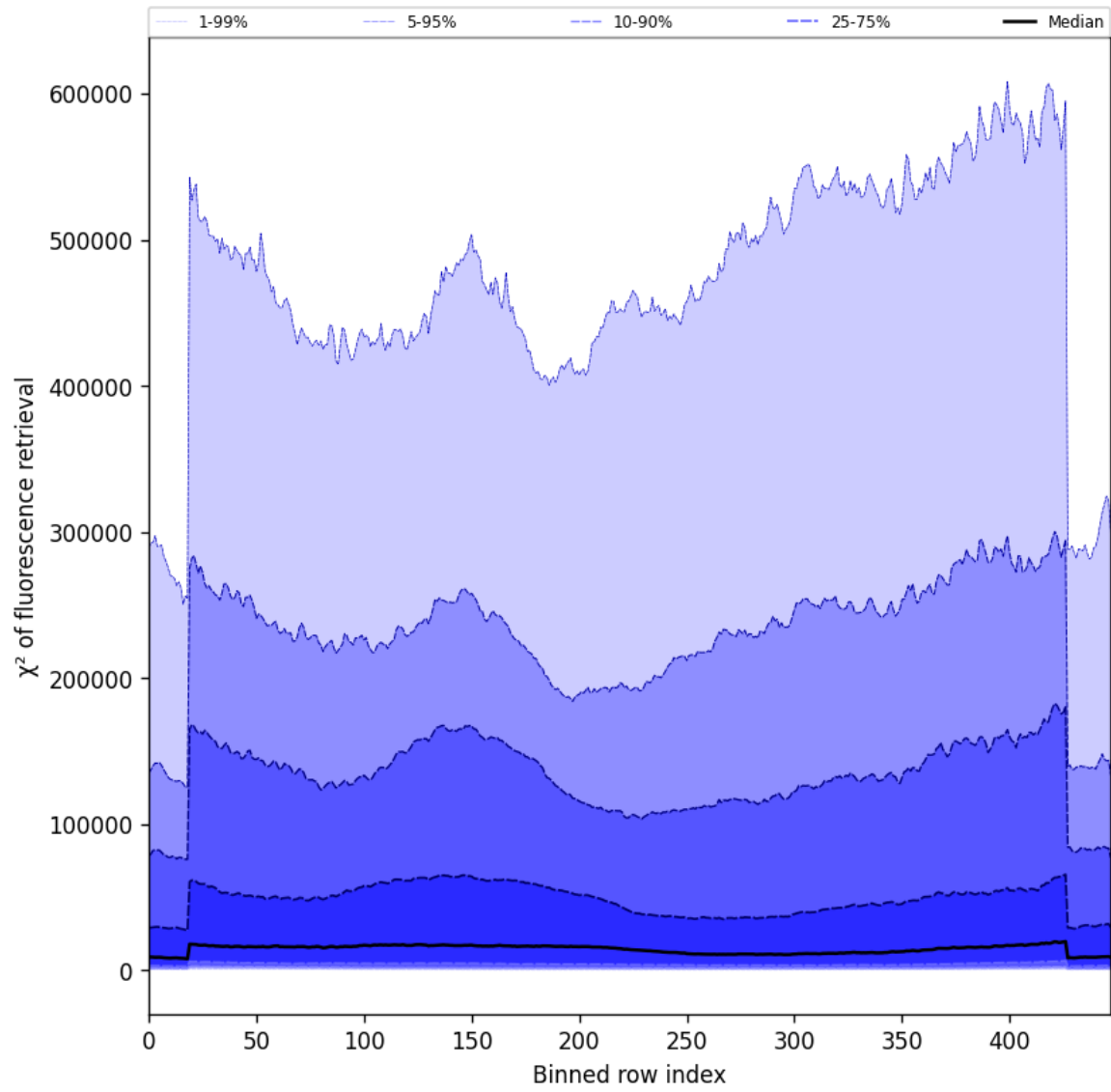
Figure 59: Along track statistics of “ \chi^2 of fluorescence retrieval” for 2025-01-24 to 2025-01-26
