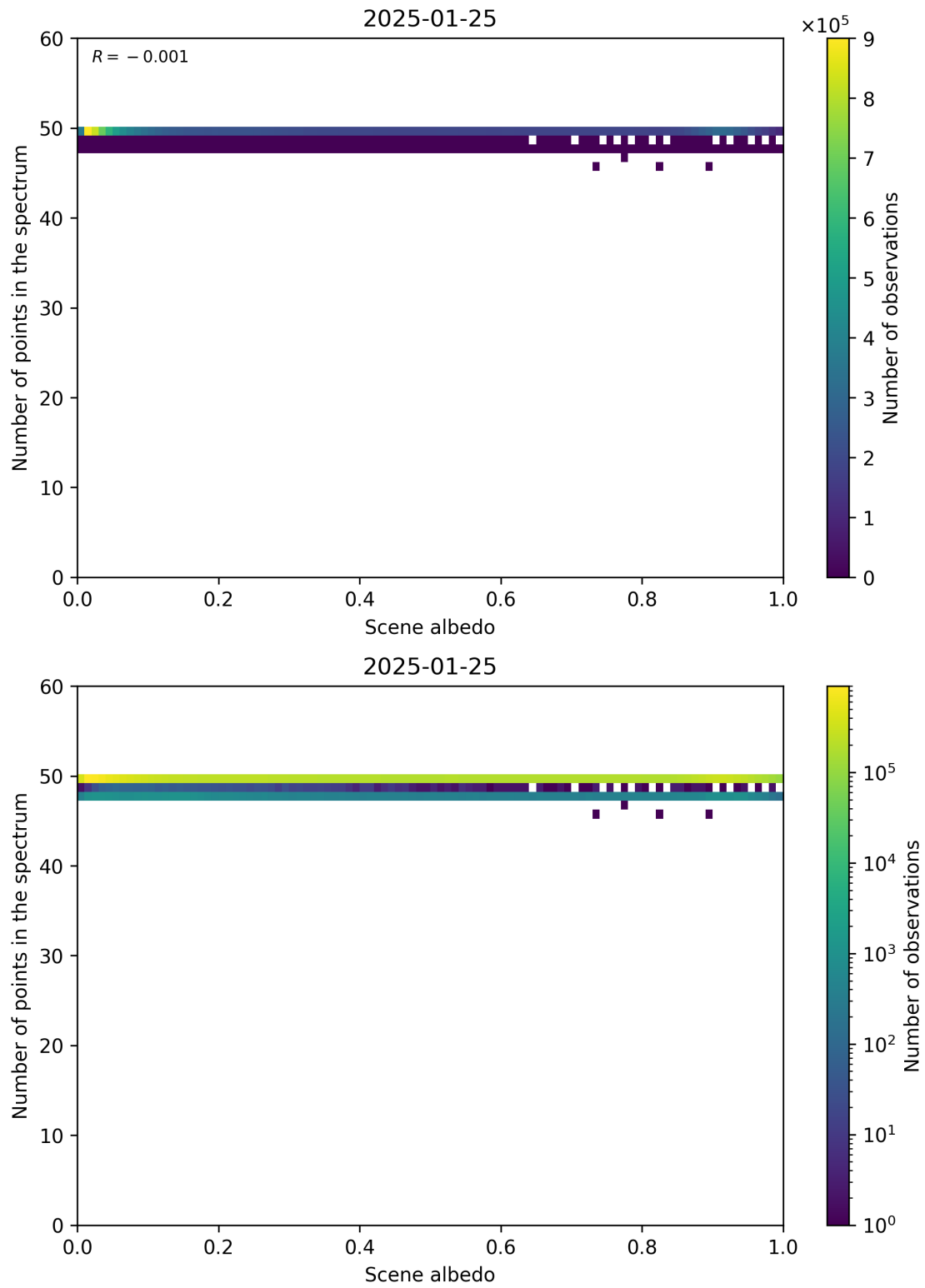
Figure 106: Scatter density plot of “Scene albedo” against “Number of points in the spectrum” for 2025-01-24 to 2025-01-26.
