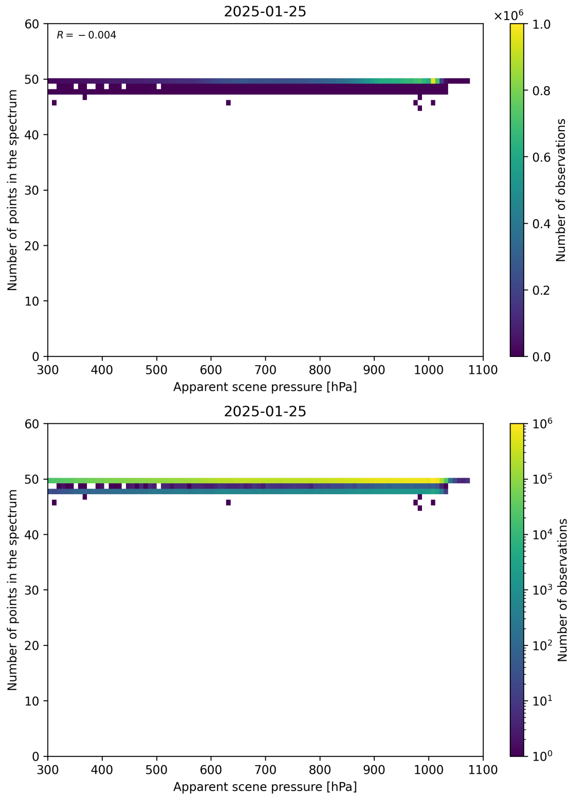
Figure 66: Scatter density plot of “Apparent scene pressure” against “Number of points in the spectrum” for 2025-01-24 to 2025-01-26.
