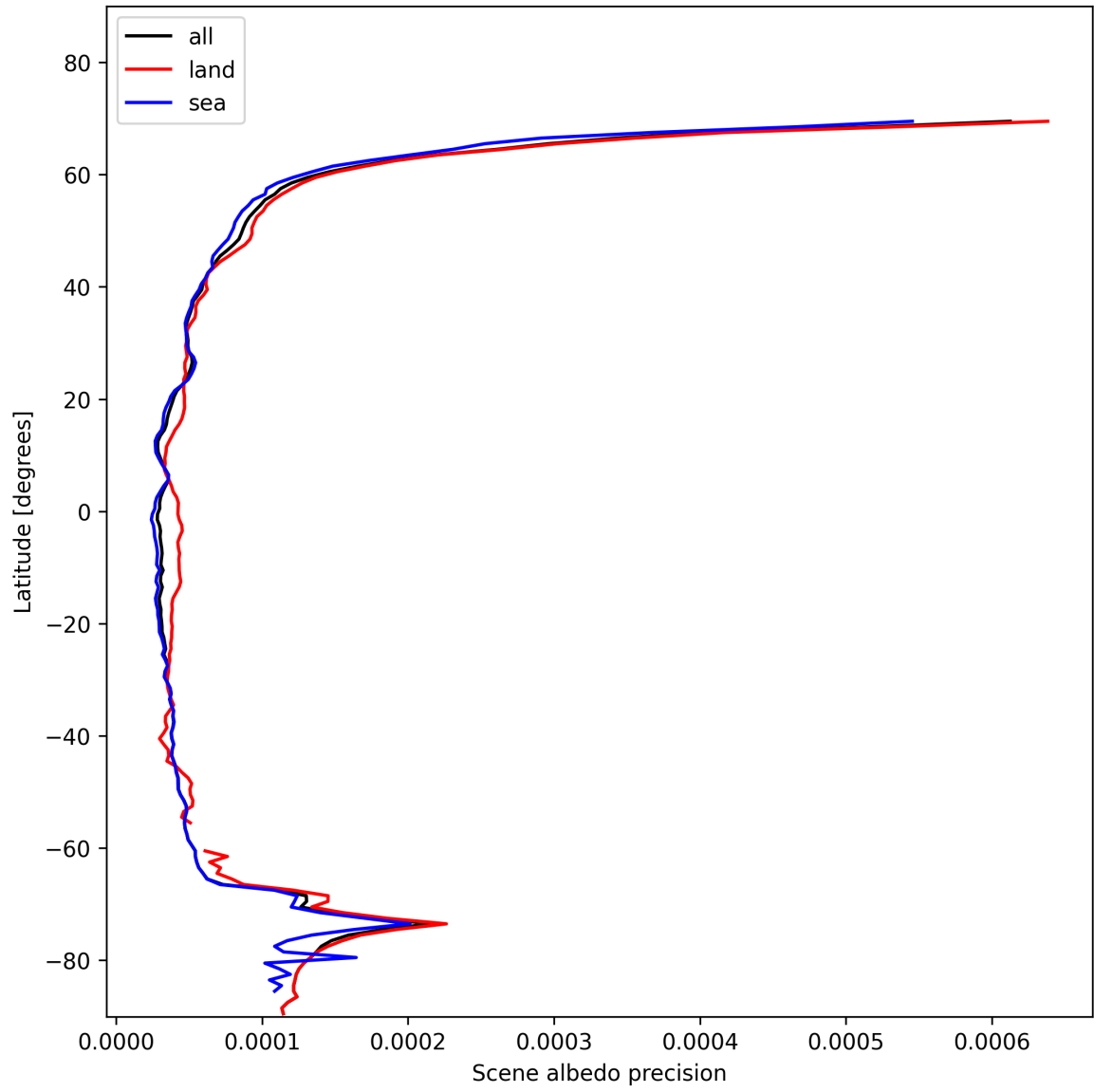
Figure 18: Zonal average of “Scene albedo precision” for 2025-01-24 to 2025-01-26.
