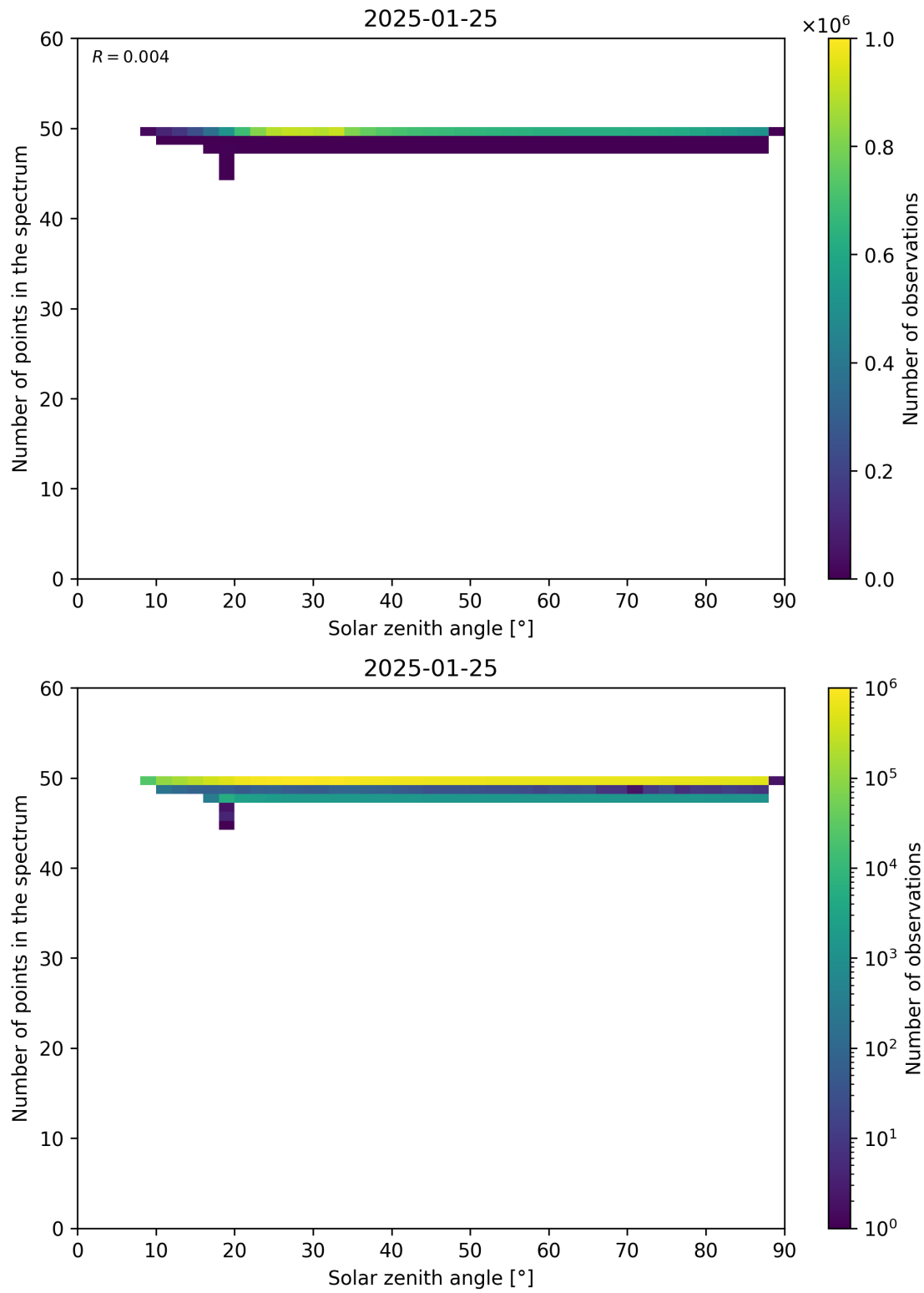
Figure 115: Scatter density plot of “Solar zenith angle” against “Number of points in the spectrum” for 2025-01-24 to 2025-01-26.
