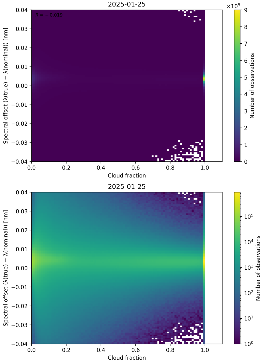
Figure 76: Scatter density plot of “Cloud fraction” against “Spectral offset ( \lambda_{\text{true}} - \lambda_{\text{nominal}} )” for 2025-01-24 to 2025-01-26.
