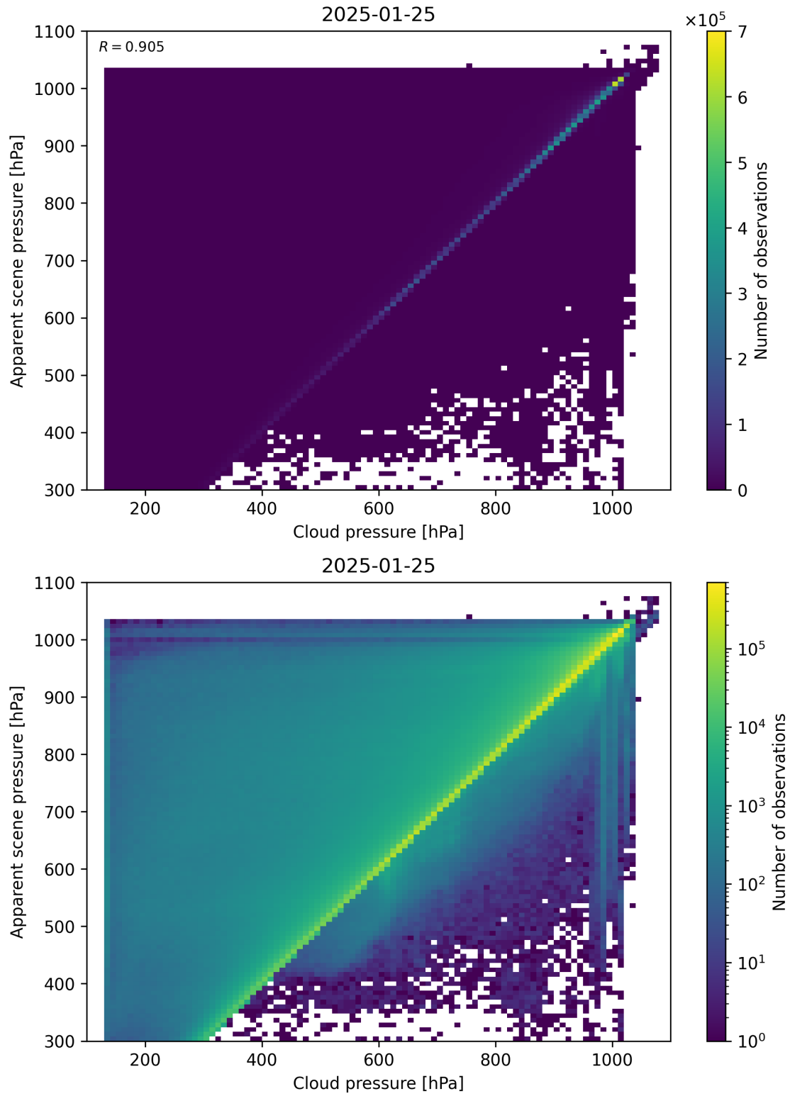
Figure 77: Scatter density plot of “Cloud pressure” against “Apparent scene pressure” for 2025-01-24 to 2025-01-26.
