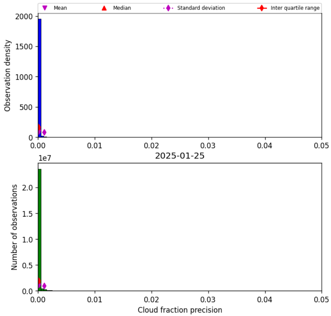
Figure 33: Histogram of “Cloud fraction precision” for 2025-01-24 to 2025-01-26
