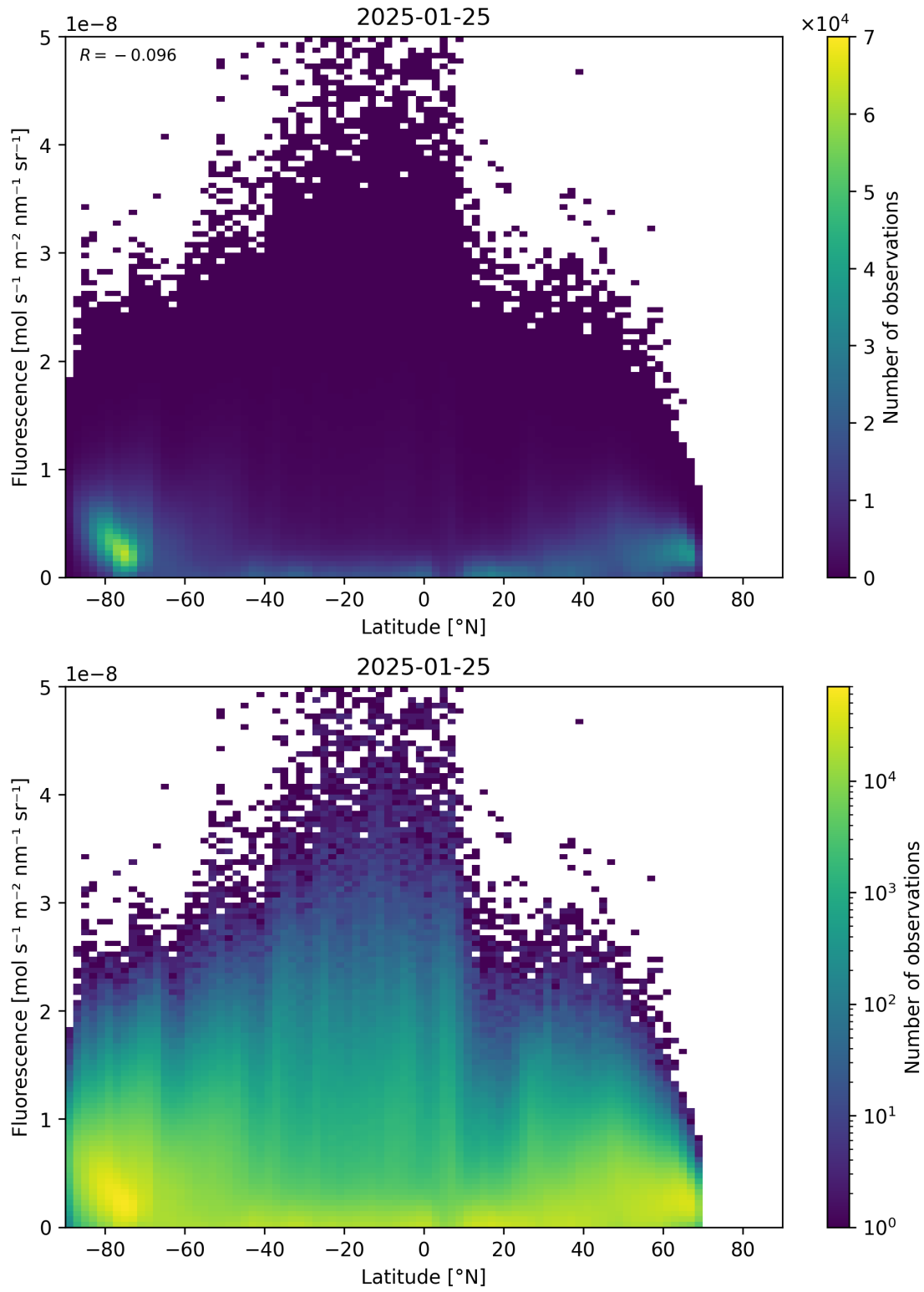
Figure 92: Scatter density plot of “Latitude” against “Fluorescence” for 2025-01-24 to 2025-01-26.
