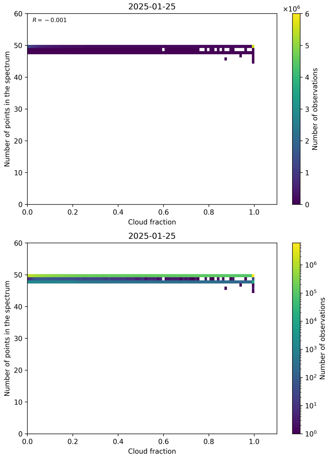
Figure 74: Scatter density plot of “Cloud fraction” against “Number of points in the spectrum” for 2025-01-24 to 2025-01-26.
