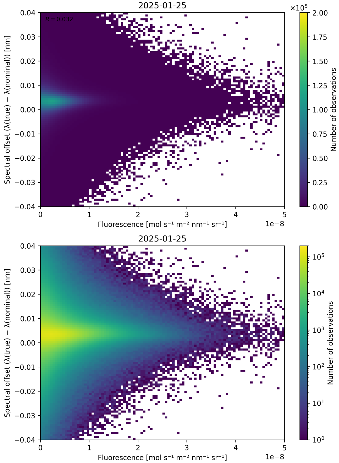
Figure 87: Scatter density plot of “Fluorescence” against “Spectral offset ( \lambda_{\text{true}} - \lambda_{\text{nominal}} )” for 2025-01-24 to 2025-01-26.
