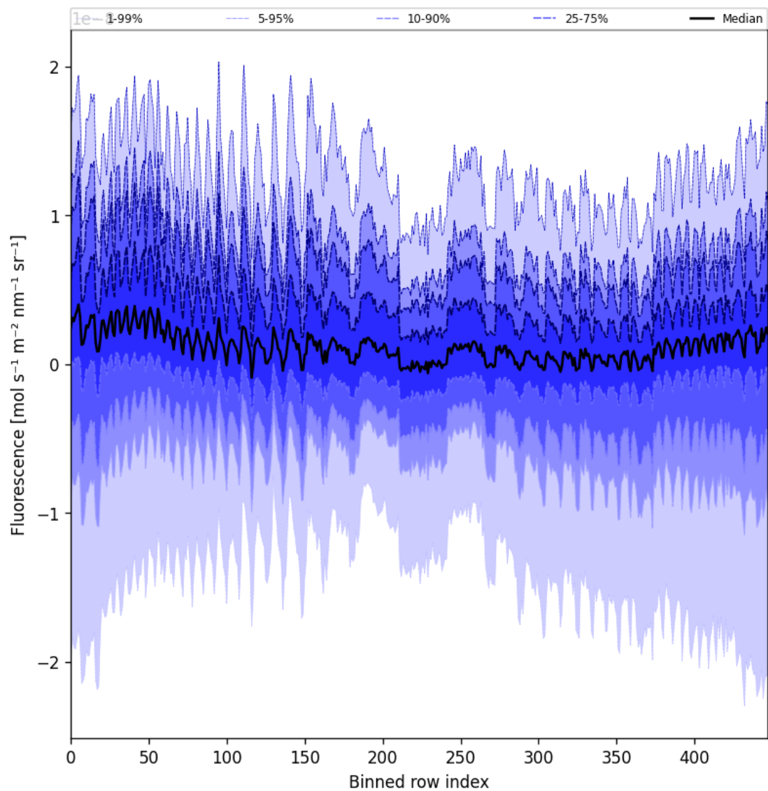
Figure 57: Along track statistics of “Fluorescence” for 2025-01-24 to 2025-01-26
