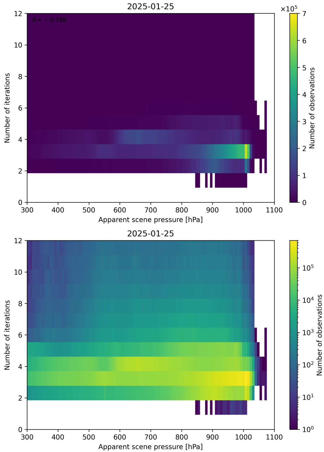
Figure 65: Scatter density plot of “Apparent scene pressure” against “Number of iterations” for 2025-01-24 to 2025-01-26.
