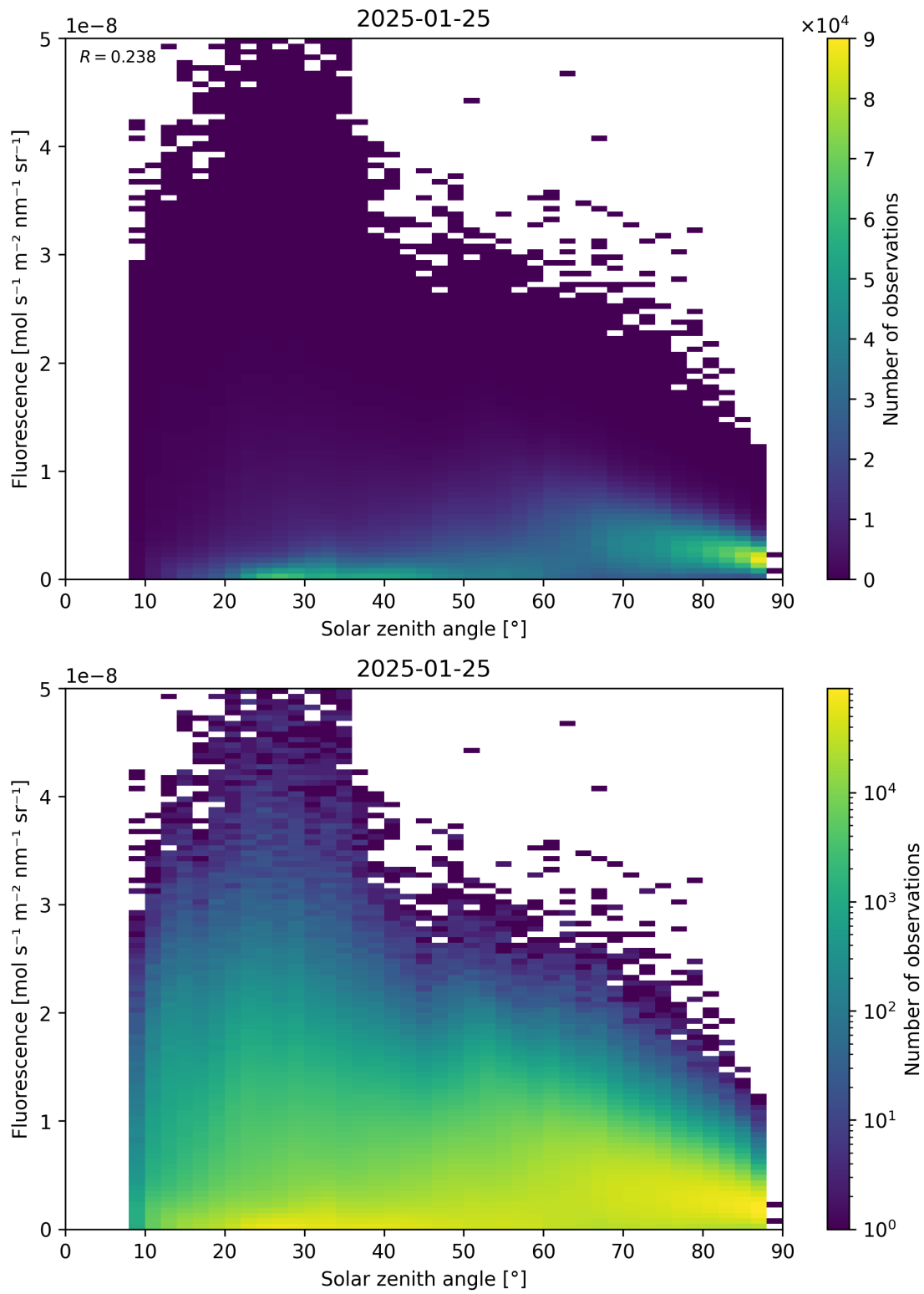
Figure 112: Scatter density plot of “Solar zenith angle” against “Fluorescence” for 2025-01-24 to 2025-01-26.
