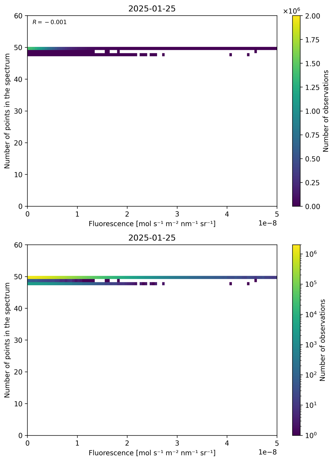
Figure 86: Scatter density plot of “Fluorescence” against “Number of points in the spectrum” for 2025-01-24 to 2025-01-26.
