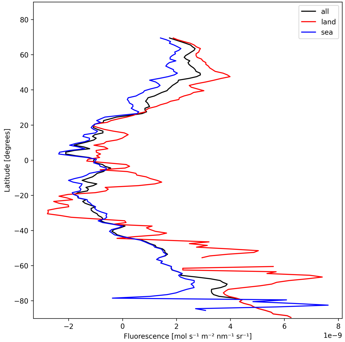
Figure 23: Zonal average of “Fluorescence” for 2025-01-24 to 2025-01-26.
