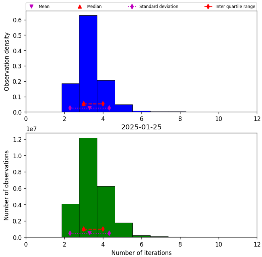
Figure 39: Histogram of “Number of iterations” for 2025-01-24 to 2025-01-26
