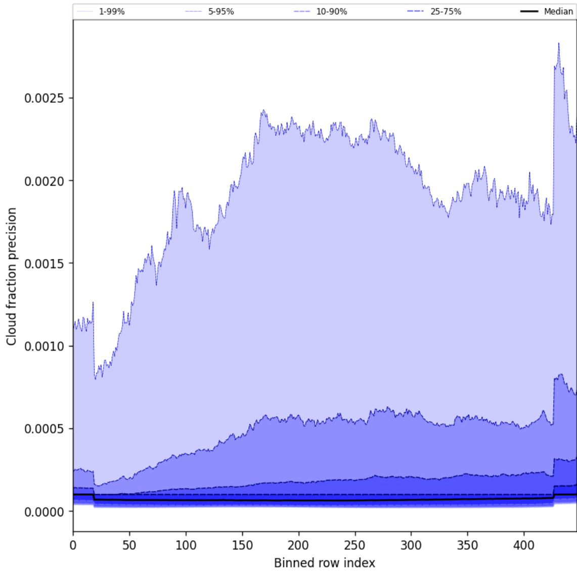
Figure 50: Along track statistics of “Cloud fraction precision” for 2025-01-24 to 2025-01-26
