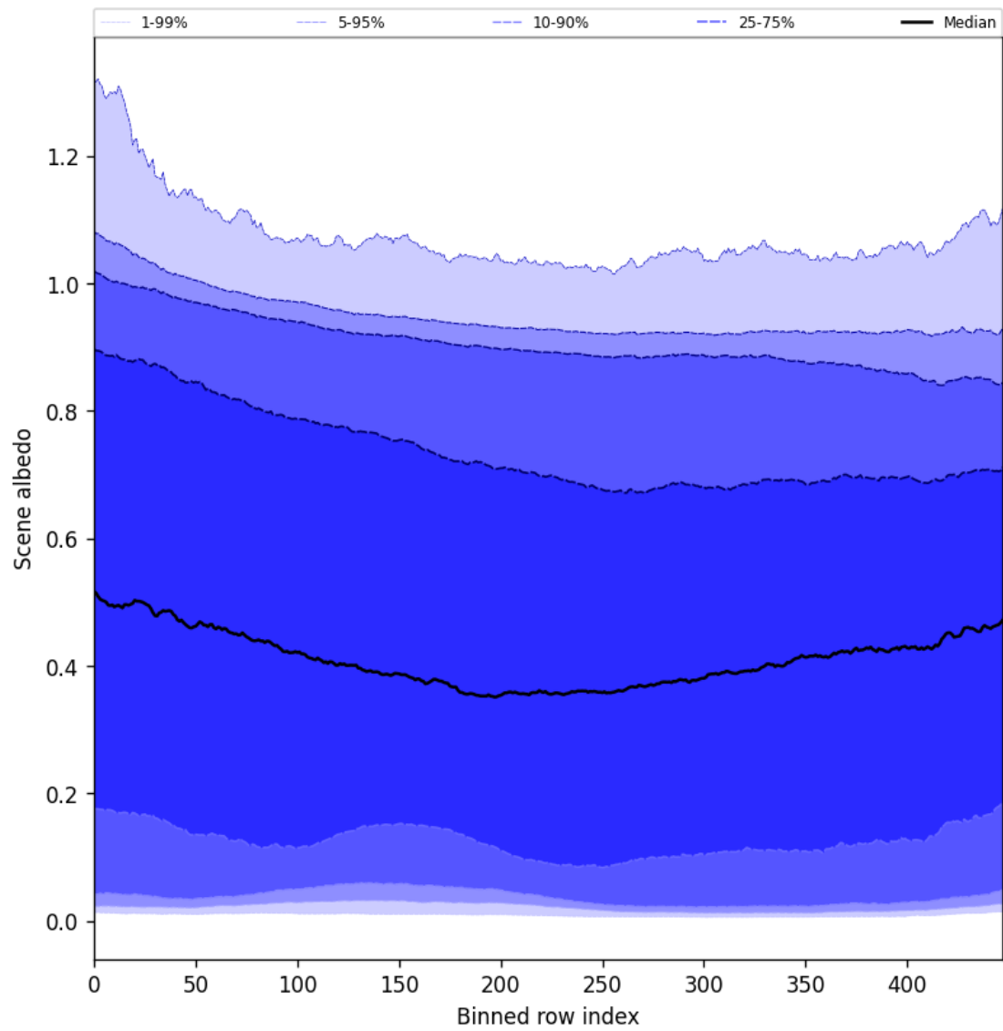
Figure 51: Along track statistics of “Scene albedo” for 2025-01-24 to 2025-01-26
