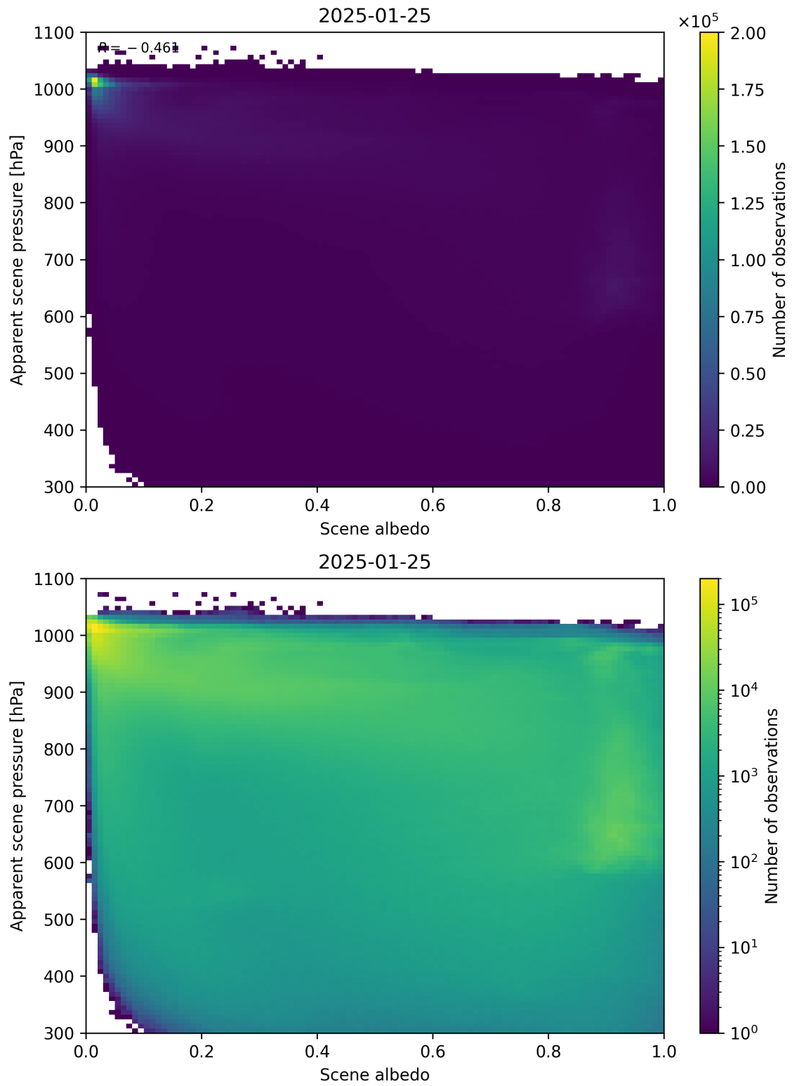
Figure 102: Scatter density plot of “Scene albedo” against “Apparent scene pressure” for 2025-01-24 to 2025-01-26.
