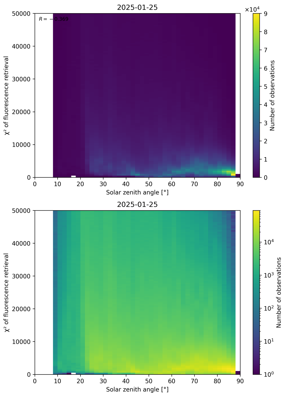
Figure 109: Scatter density plot of “Solar zenith angle” against “ \chi^2 of fluorescence retrieval” for 2025-01-24 to 2025-01-26.
