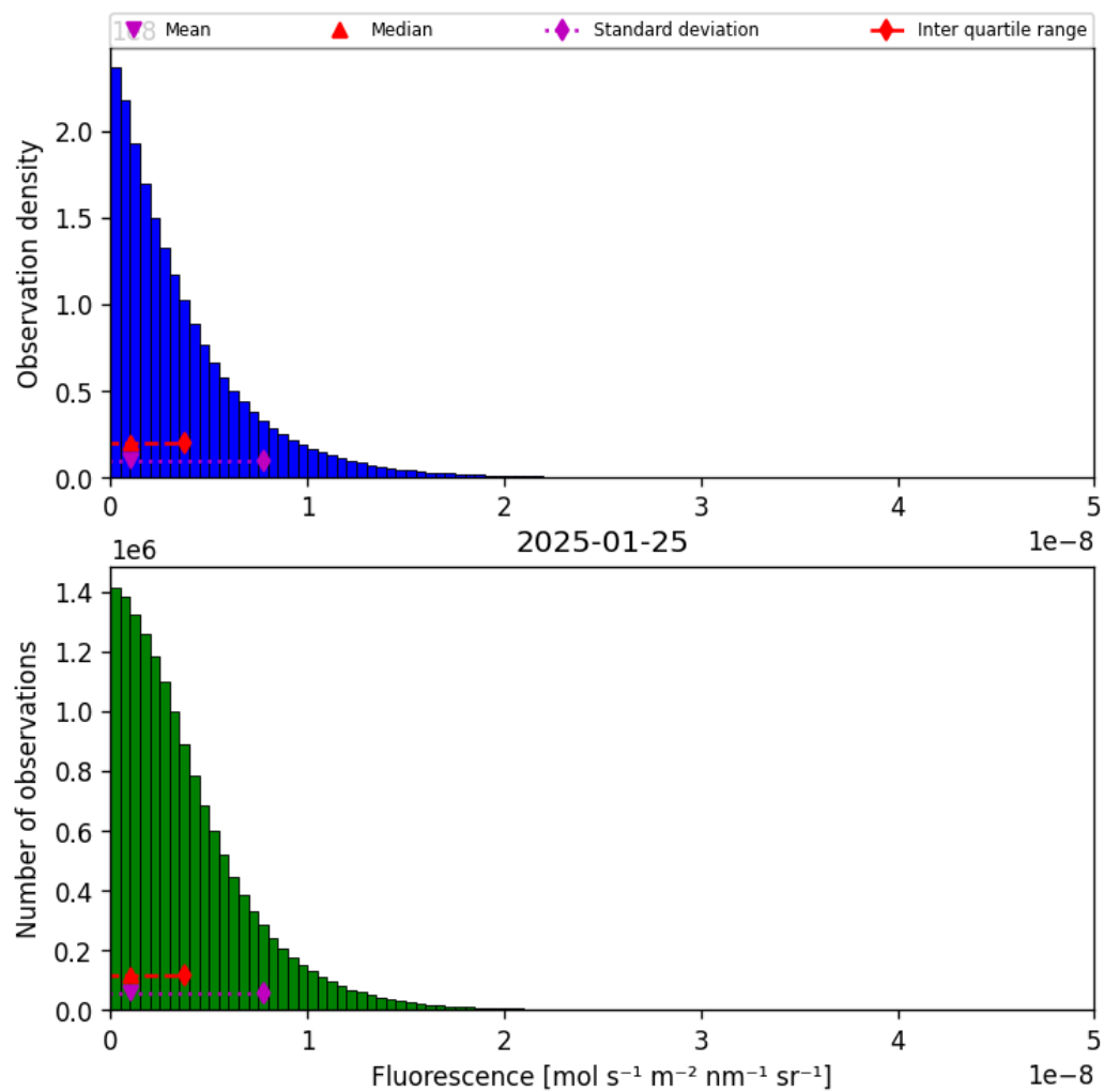
Figure 40: Histogram of “Fluorescence” for 2025-01-24 to 2025-01-26
