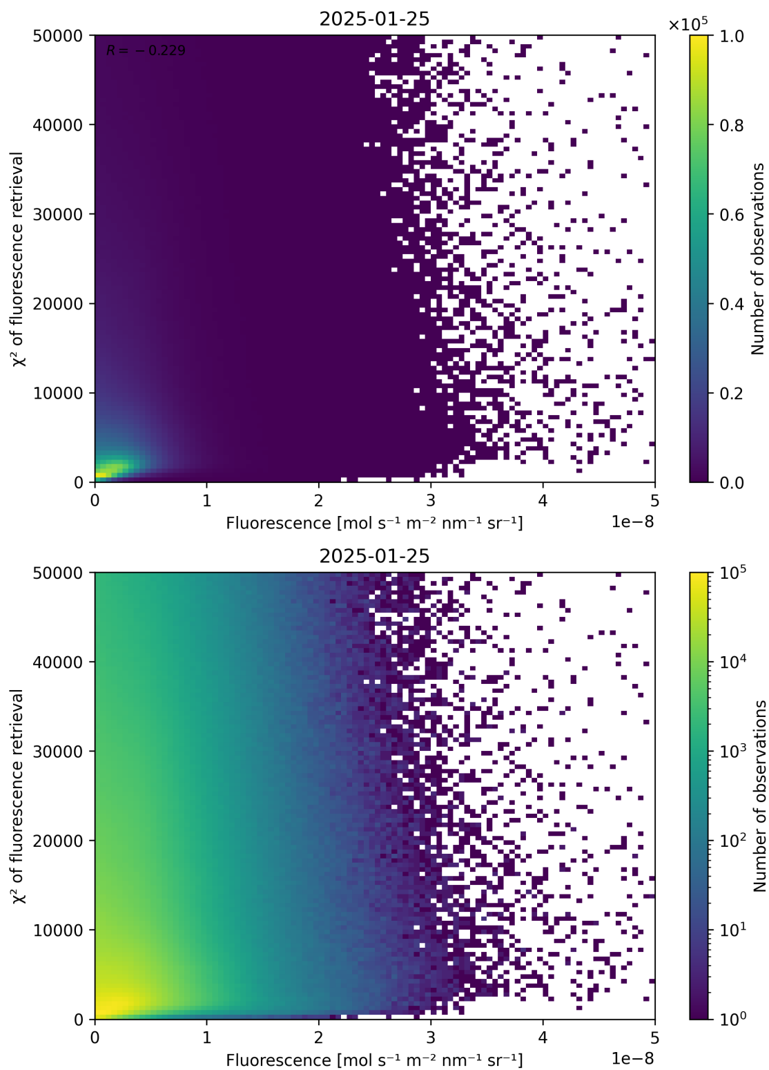
Figure 85: Scatter density plot of “Fluorescence” against “ \chi^2 of fluorescence retrieval” for 2025-01-24 to 2025-01-26.
