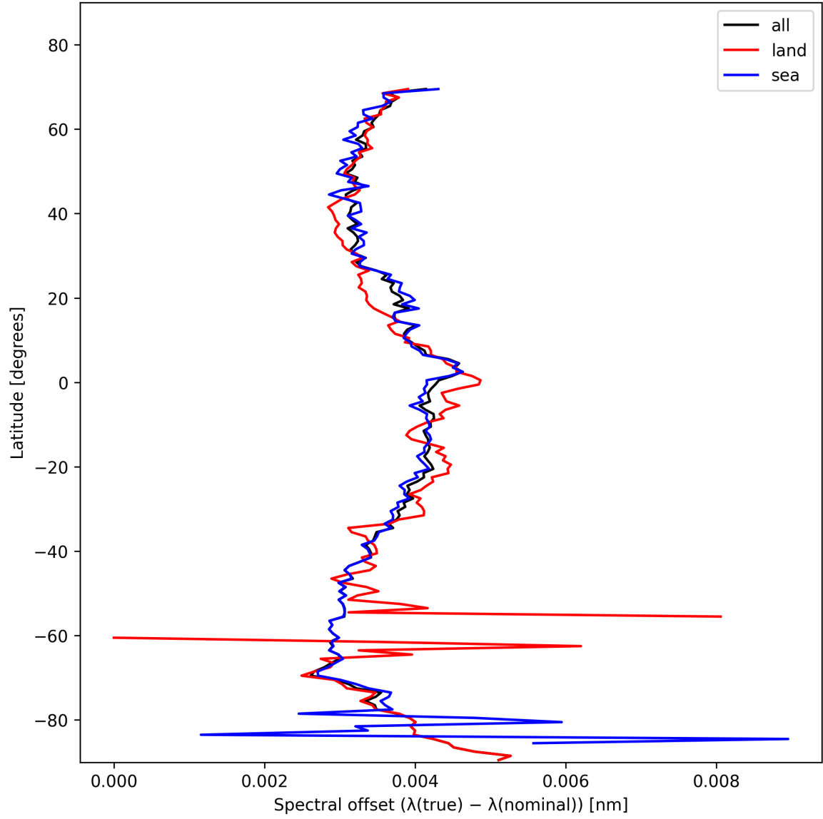
Figure 28: Zonal average of “Spectral offset ( \lambda_{\text{true}} - \lambda_{\text{nominal}} )” for 2025-01-24 to 2025-01-26.
