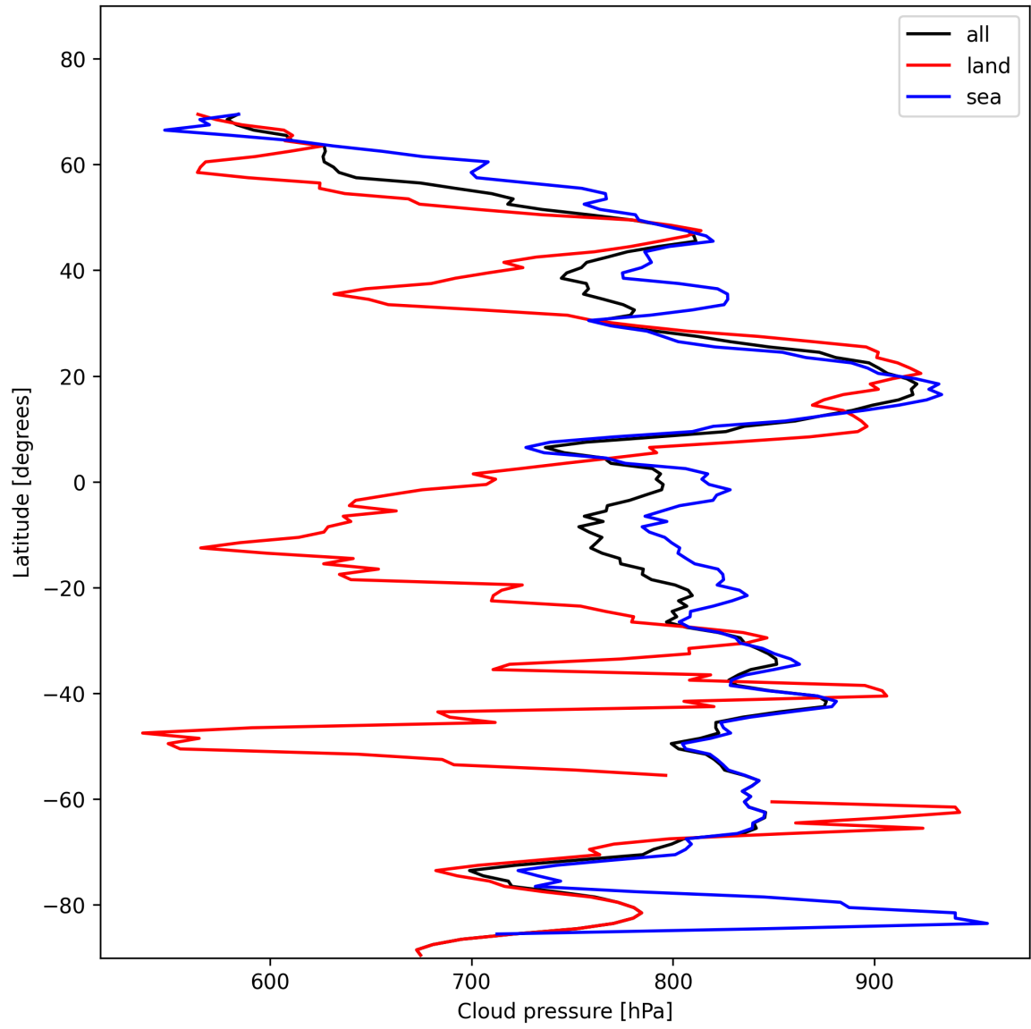
Figure 13: Zonal average of “Cloud pressure” for 2025-01-24 to 2025-01-26.
