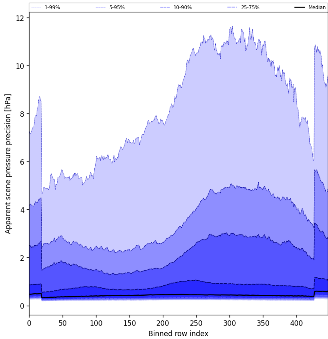
Figure 54: Along track statistics of “Apparent scene pressure precision” for 2025-01-24 to 2025-01-26
