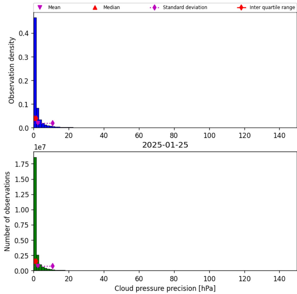
Figure 31: Histogram of “Cloud pressure precision” for 2025-01-24 to 2025-01-26
