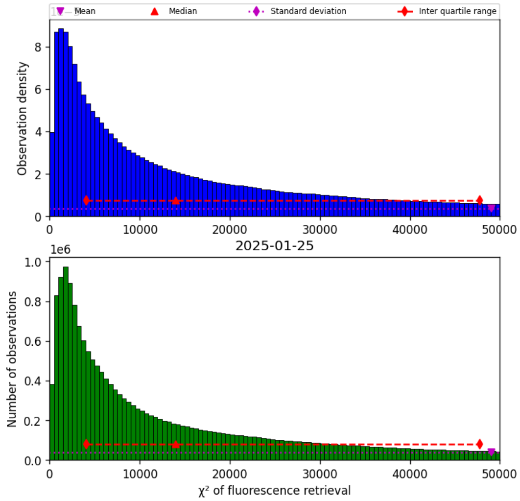
Figure 42: Histogram of “ \chi^2 of fluorescence retrieval” for 2025-01-24 to 2025-01-26
