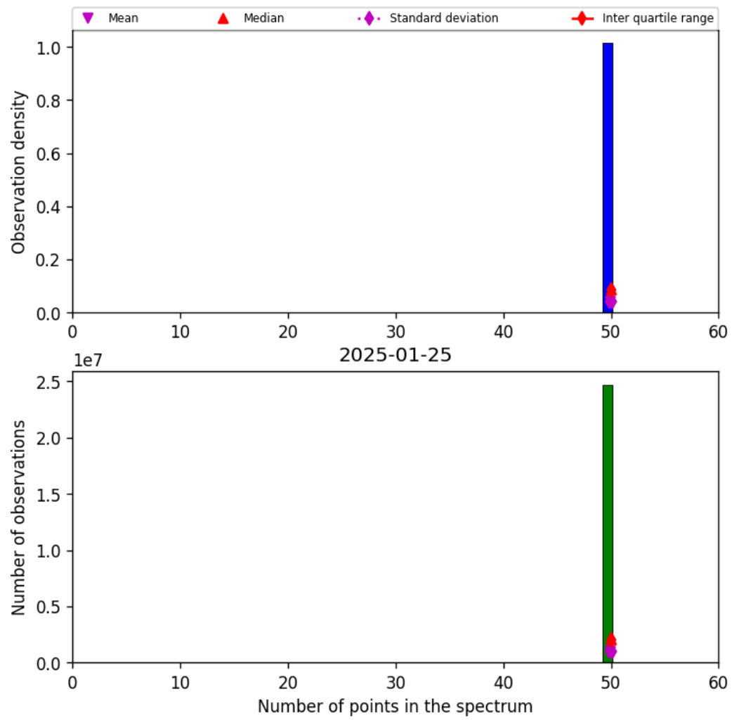
Figure 44: Histogram of “Number of points in the spectrum” for 2025-01-24 to 2025-01-26
