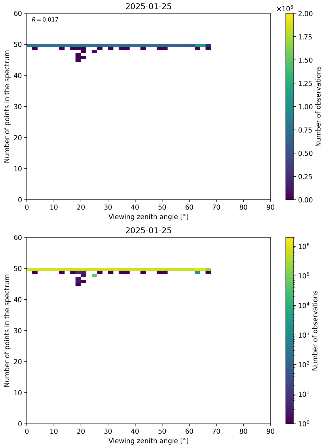
Figure 125: Scatter density plot of “Viewing zenith angle” against “Number of points in the spectrum” for 2025-01-24 to 2025-01-26.
