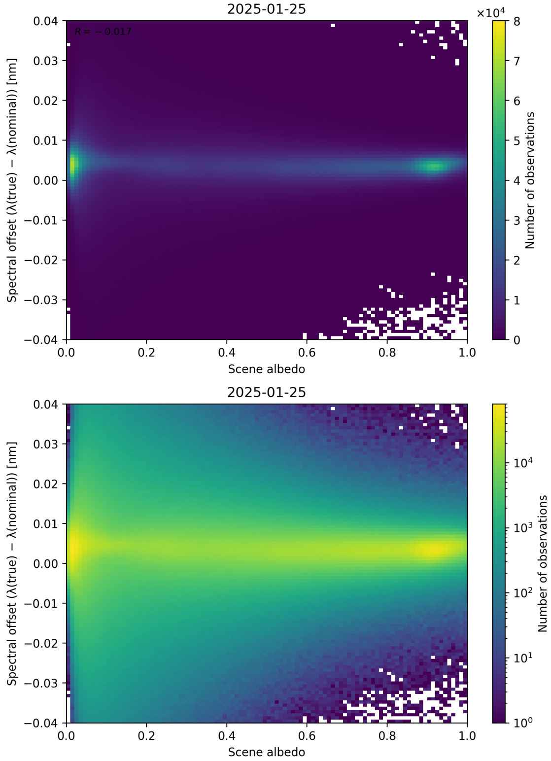
Figure 107: Scatter density plot of “Scene albedo” against “Spectral offset ( \lambda_{\text{true}} - \lambda_{\text{nominal}} )” for 2025-01-24 to 2025-01-26.
