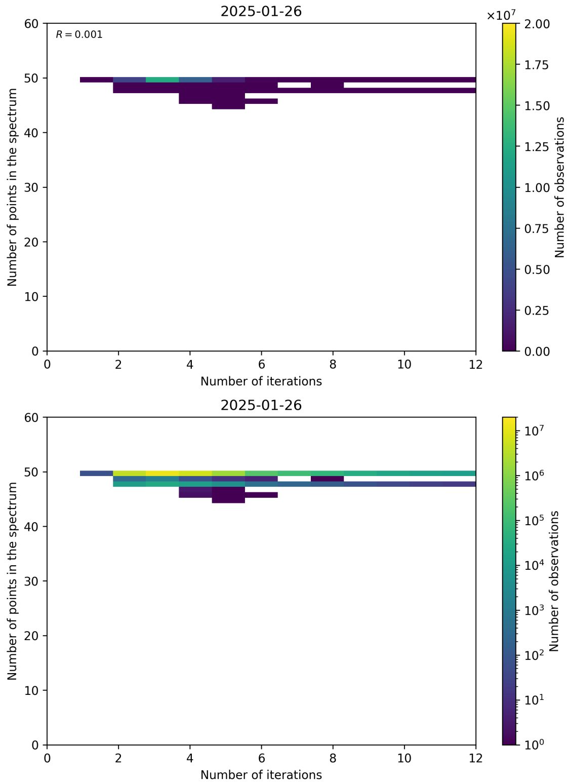
Figure 99: Scatter density plot of “Number of iterations” against “Number of points in the spectrum” for 2025-01-25 to 2025-01-27.
