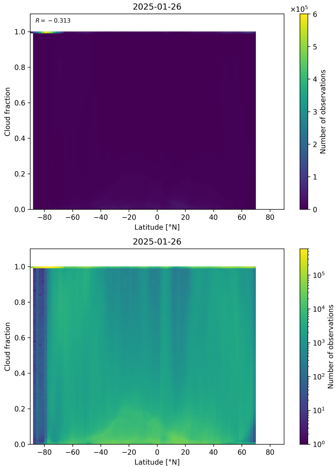
Figure 90: Scatter density plot of “Latitude” against “Cloud fraction” for 2025-01-25 to 2025-01-27.
