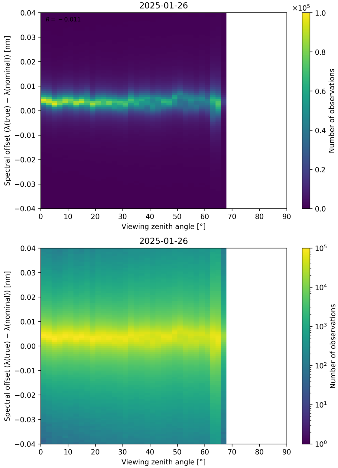
Figure 128: Scatter density plot of “Viewing zenith angle” against “Spectral offset ( \lambda_{\text{true}} - \lambda_{\text{nominal}} )” for 2025-01-25 to 2025-01-27.
