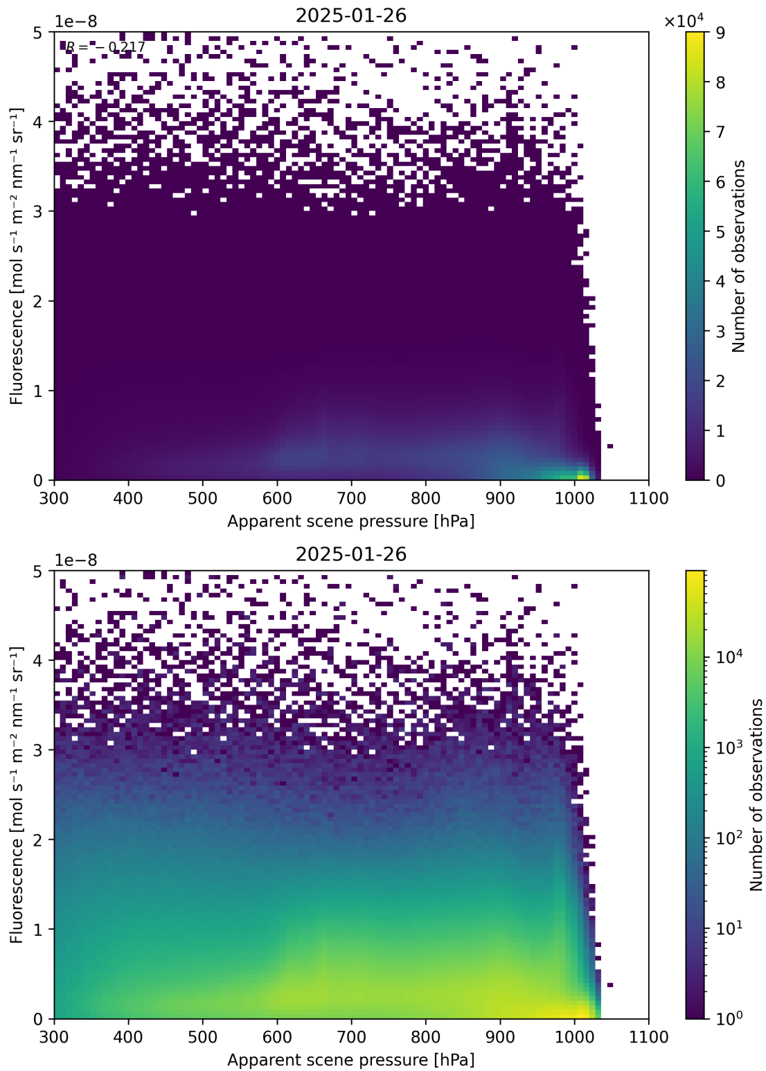
Figure 64: Scatter density plot of “Apparent scene pressure” against “Fluorescence” for 2025-01-25 to 2025-01-27.
