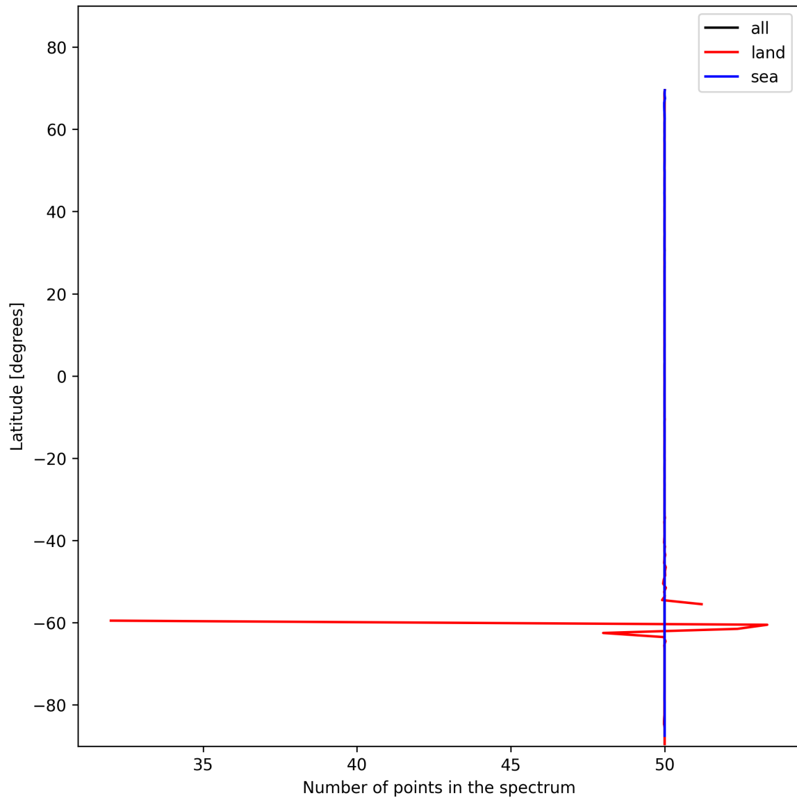
Figure 27: Zonal average of “Number of points in the spectrum” for 2025-01-25 to 2025-01-27.
