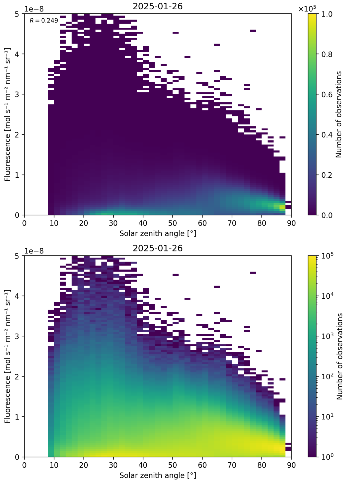
Figure 112: Scatter density plot of “Solar zenith angle” against “Fluorescence” for 2025-01-25 to 2025-01-27.
