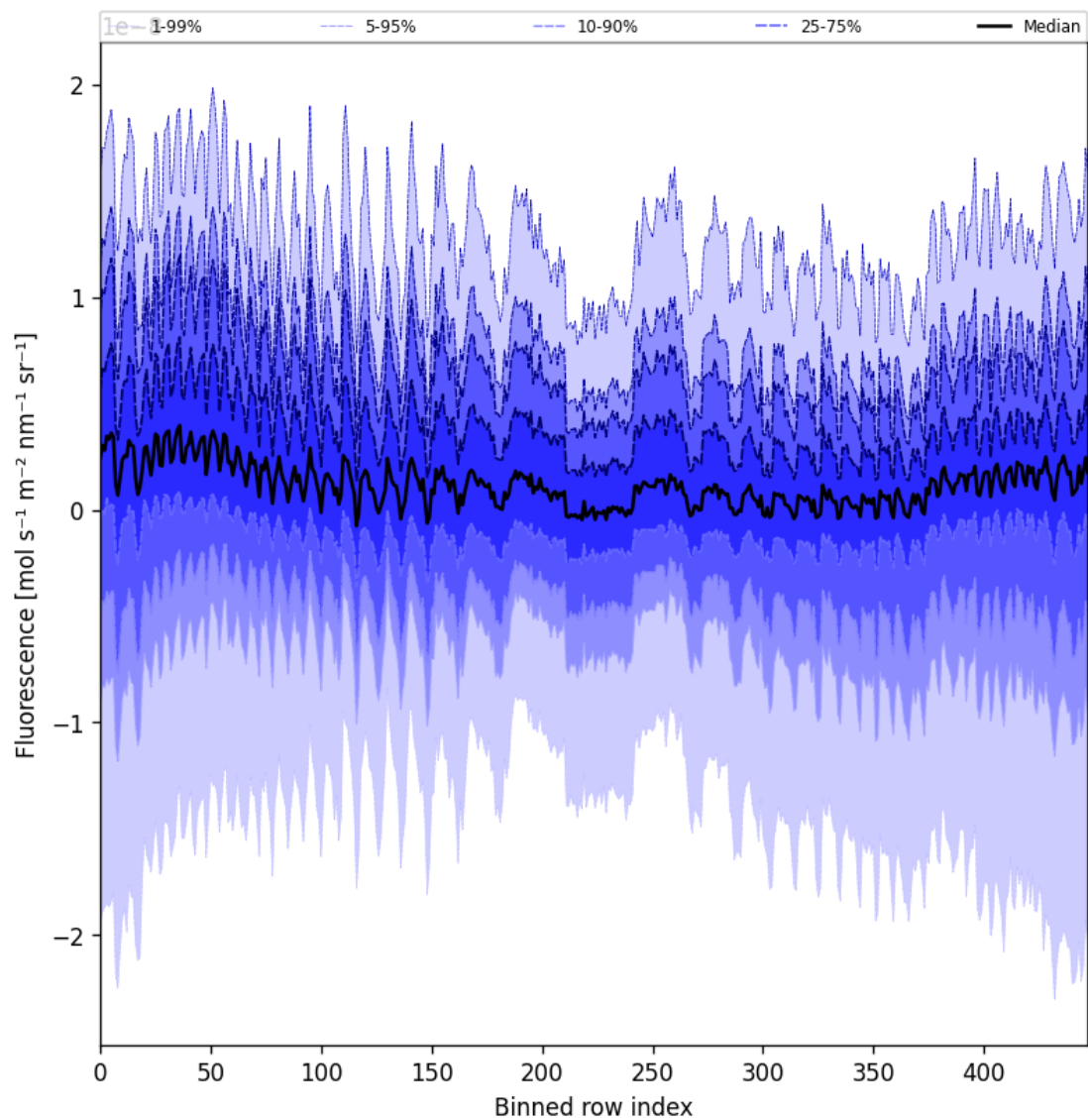
Figure 57: Along track statistics of “Fluorescence” for 2025-01-25 to 2025-01-27
