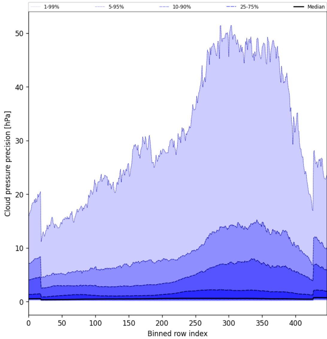
Figure 48: Along track statistics of “Cloud pressure precision” for 2025-01-25 to 2025-01-27
