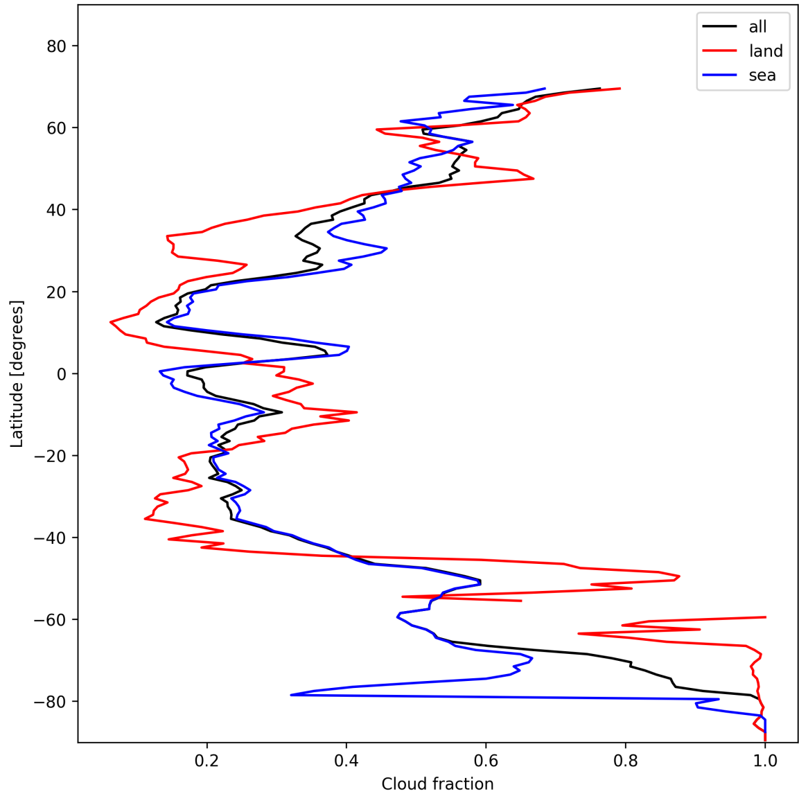
Figure 15: Zonal average of “Cloud fraction” for 2025-01-25 to 2025-01-27.
