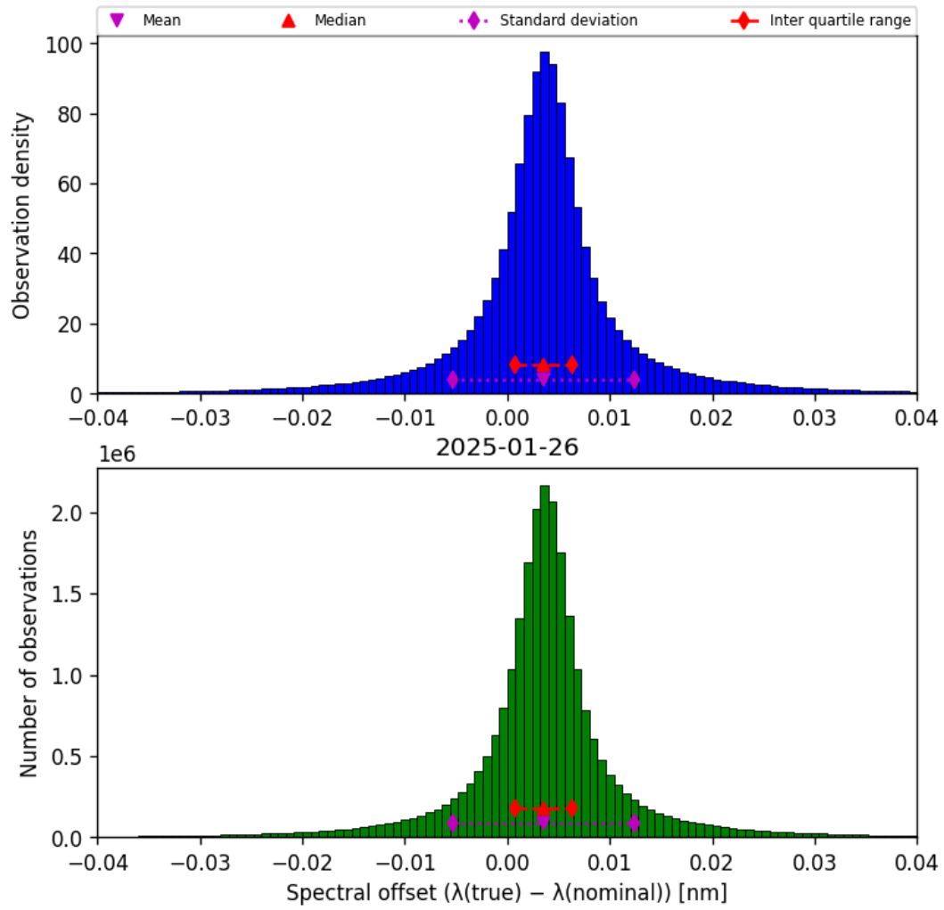
Figure 45: Histogram of “Spectral offset ( \lambda_{\text{true}} - \lambda_{\text{nominal}} )” for 2025-01-25 to 2025-01-27
