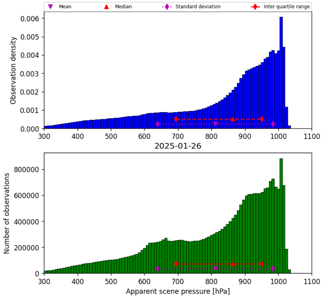
Figure 36: Histogram of “Apparent scene pressure” for 2025-01-25 to 2025-01-27
