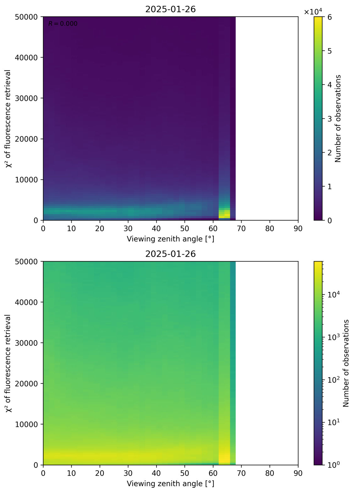
Figure 119: Scatter density plot of “Viewing zenith angle” against “ \chi^2 of fluorescence retrieval” for 2025-01-25 to 2025-01-27.
