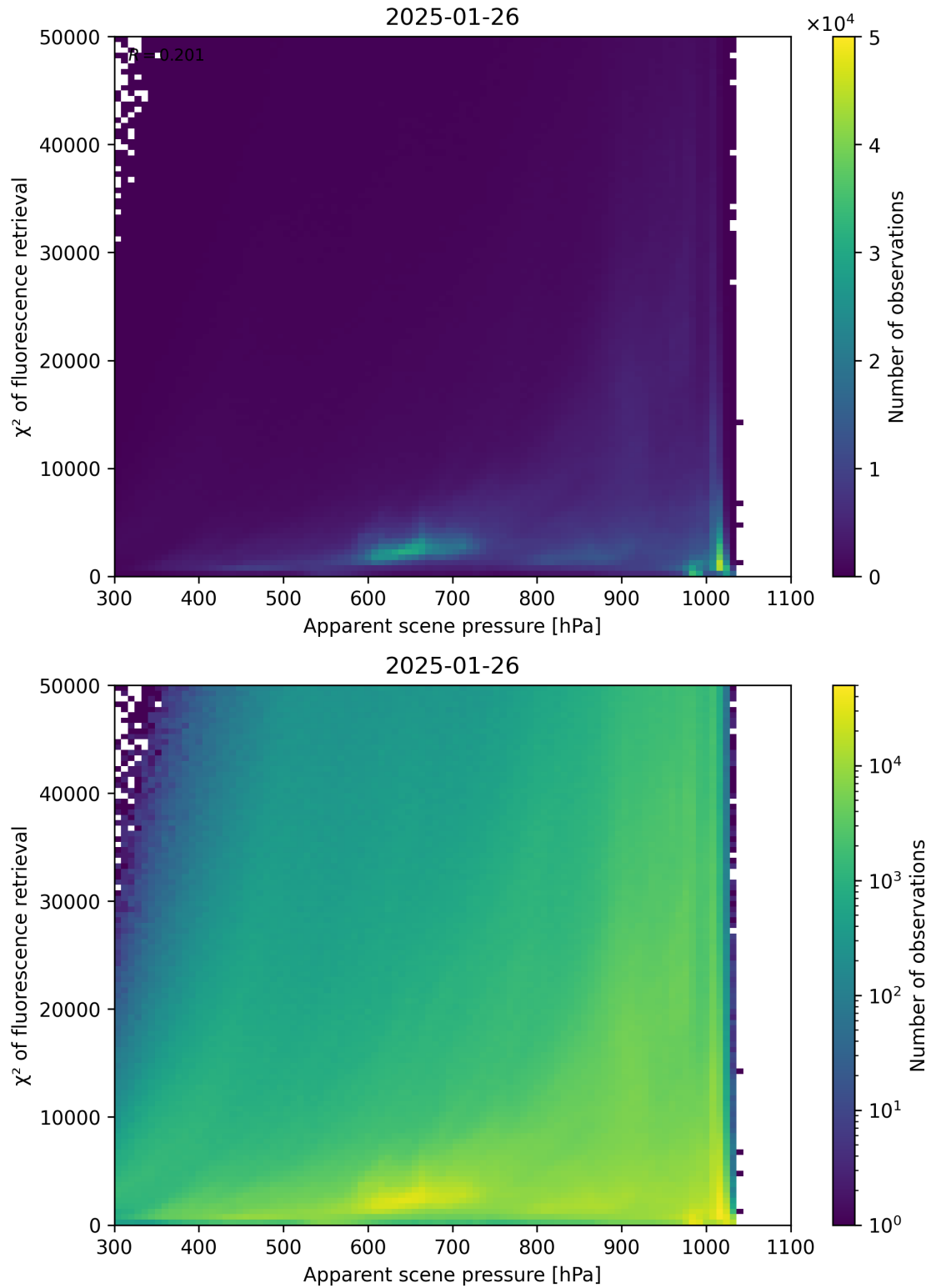
Figure 63: Scatter density plot of “Apparent scene pressure” against “ \chi^2 of fluorescence retrieval” for 2025-01-25 to 2025-01-27.
