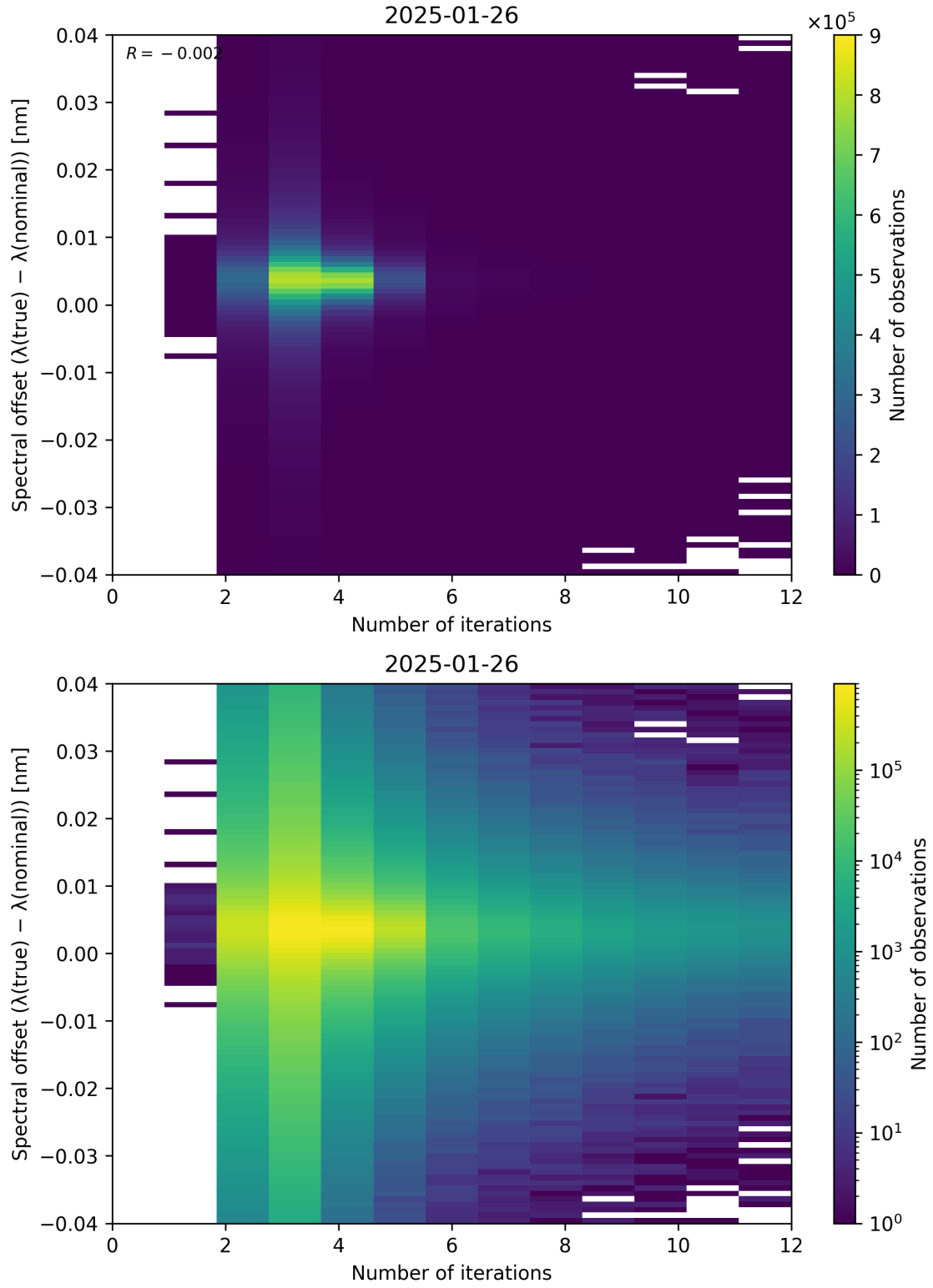
Figure 100: Scatter density plot of “Number of iterations” against “Spectral offset ( \lambda_{\text{true}} - \lambda_{\text{nominal}} )” for 2025-01-25 to 2025-01-27.
