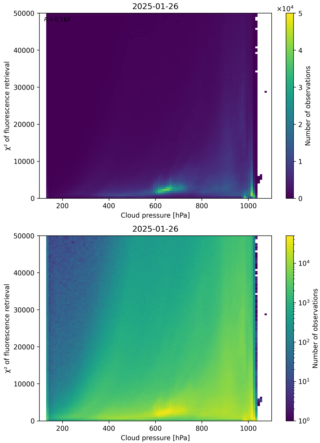
Figure 78: Scatter density plot of “Cloud pressure” against “ \chi^2 of fluorescence retrieval” for 2025-01-25 to 2025-01-27.
