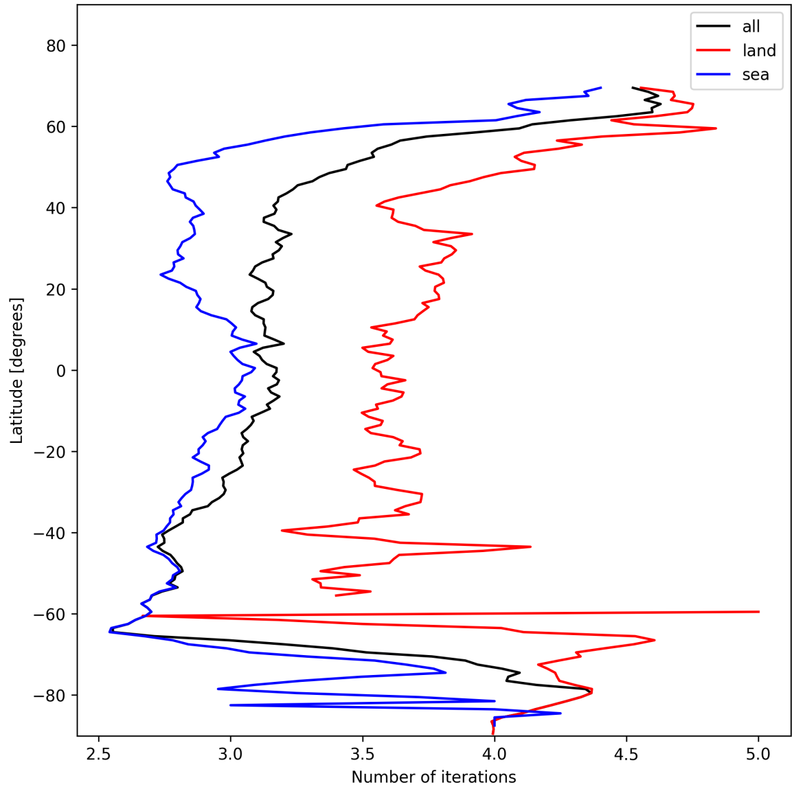
Figure 22: Zonal average of “Number of iterations” for 2025-01-25 to 2025-01-27.
