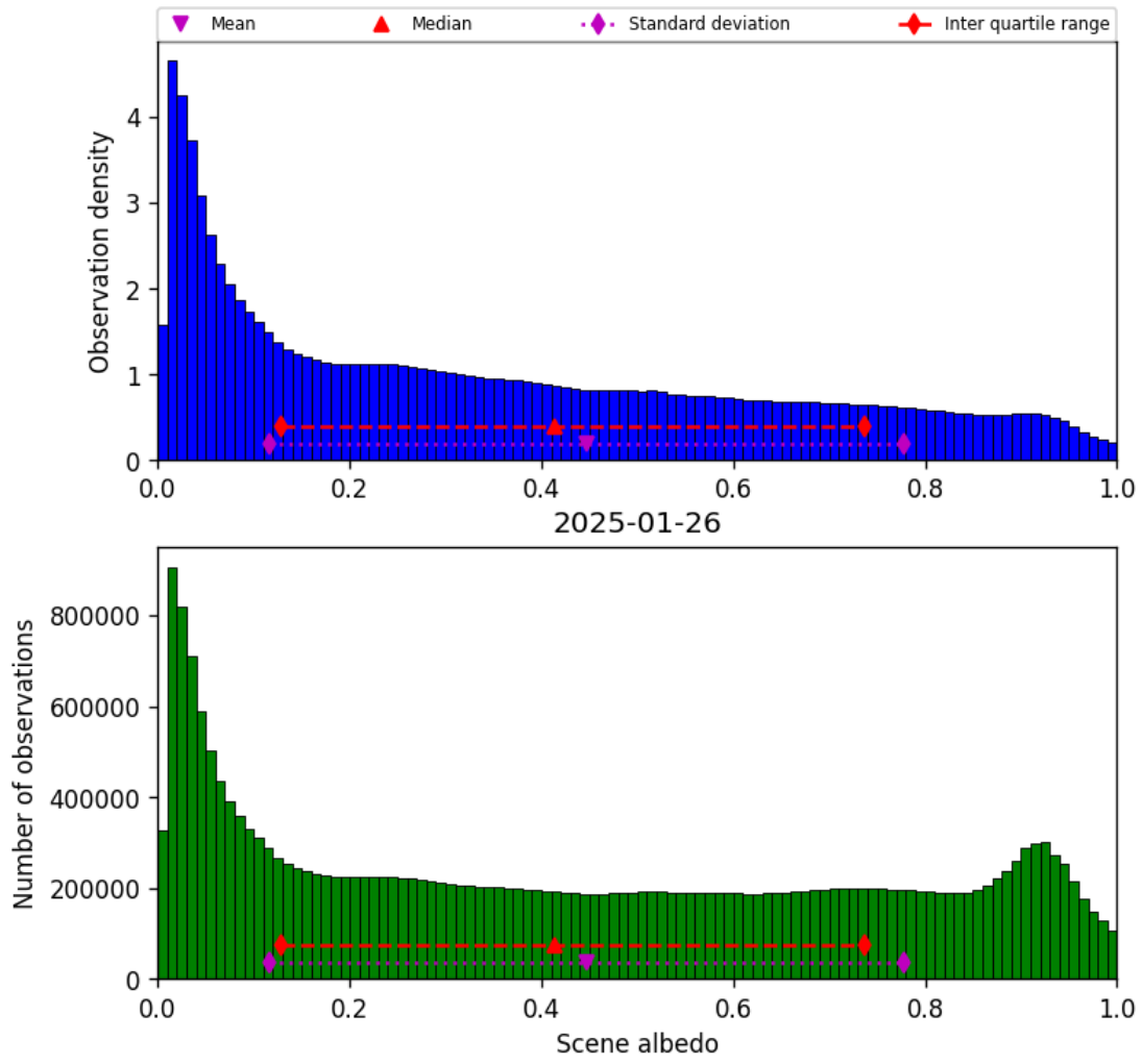
Figure 34: Histogram of “Scene albedo” for 2025-01-25 to 2025-01-27
