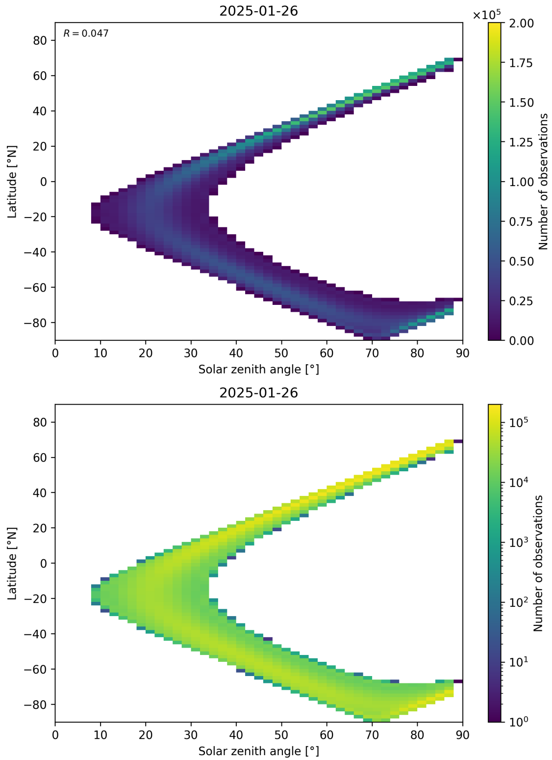
Figure 113: Scatter density plot of “Solar zenith angle” against “Latitude” for 2025-01-25 to 2025-01-27.
