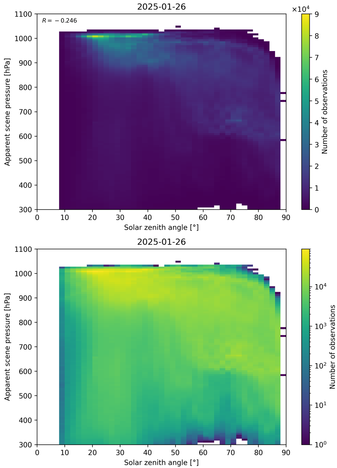
Figure 108: Scatter density plot of “Solar zenith angle” against “Apparent scene pressure” for 2025-01-25 to 2025-01-27.
