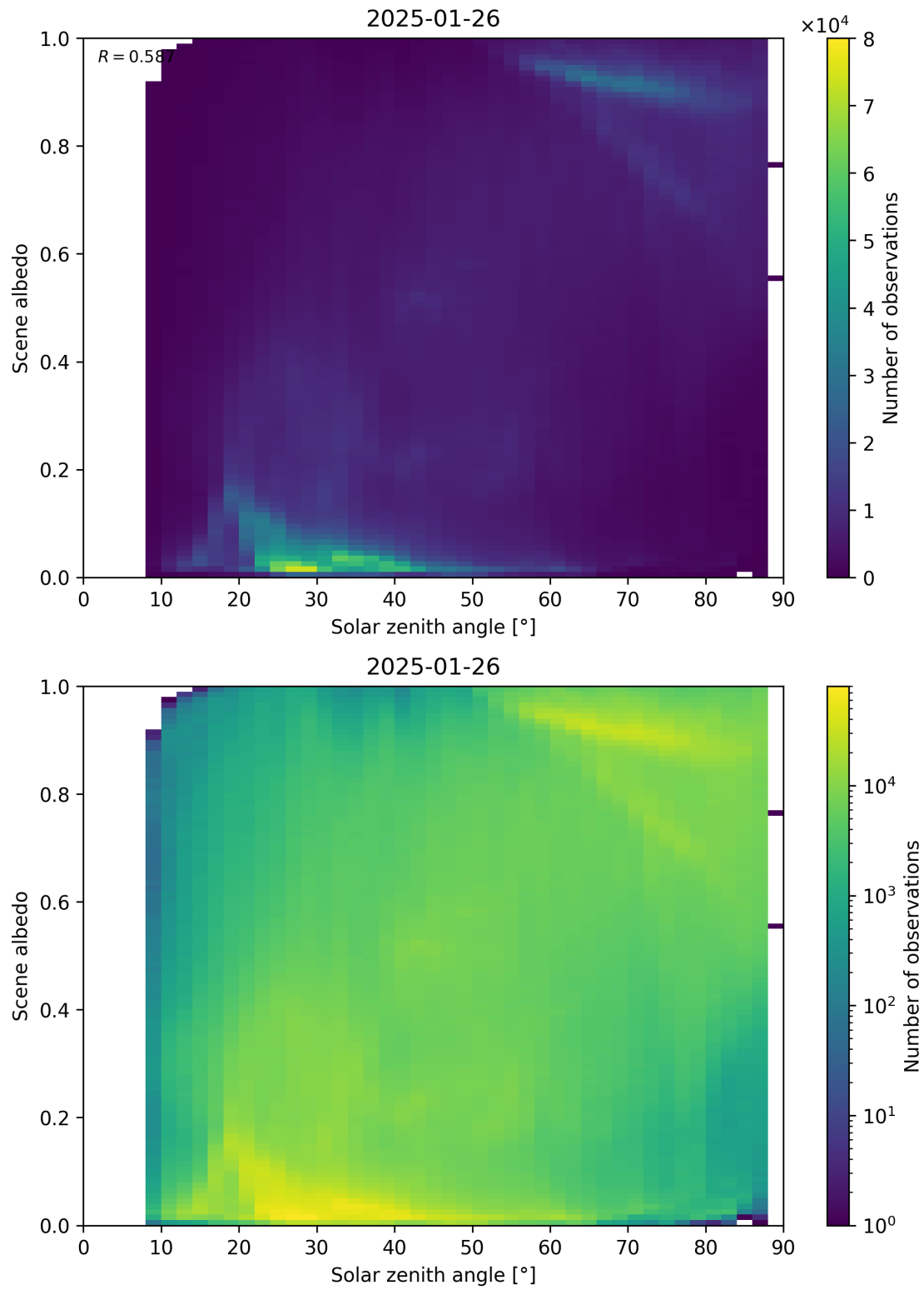
Figure 116: Scatter density plot of “Solar zenith angle” against “Scene albedo” for 2025-01-25 to 2025-01-27.
