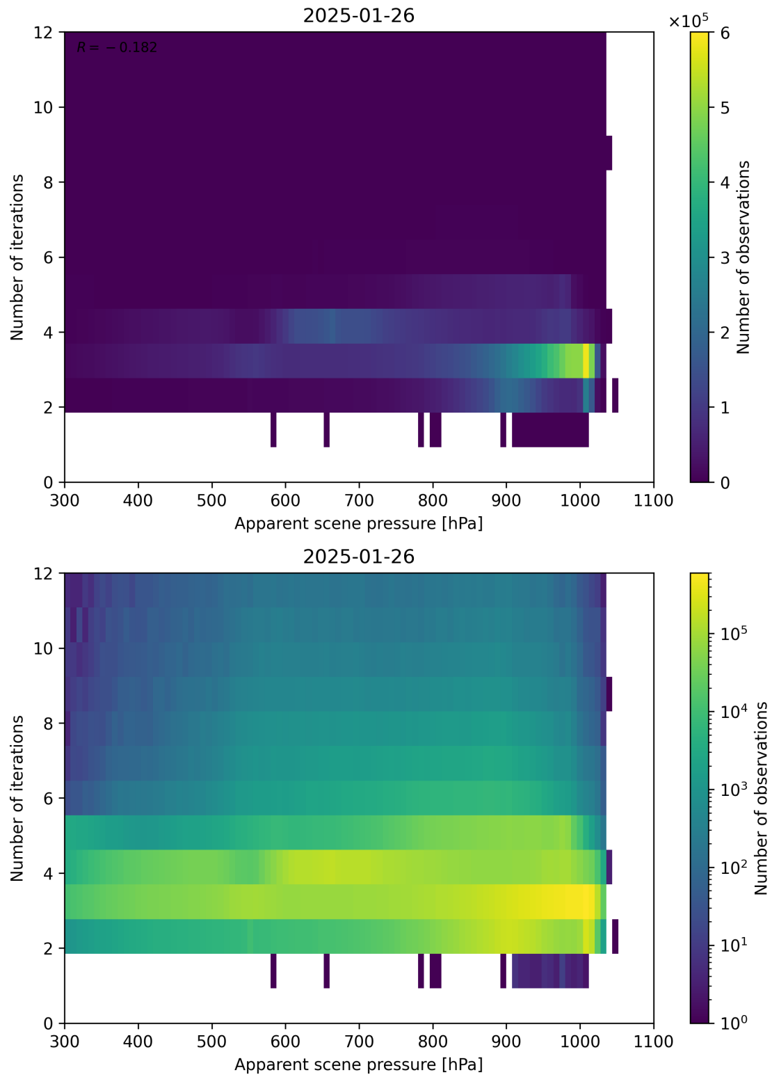
Figure 65: Scatter density plot of “Apparent scene pressure” against “Number of iterations” for 2025-01-25 to 2025-01-27.
