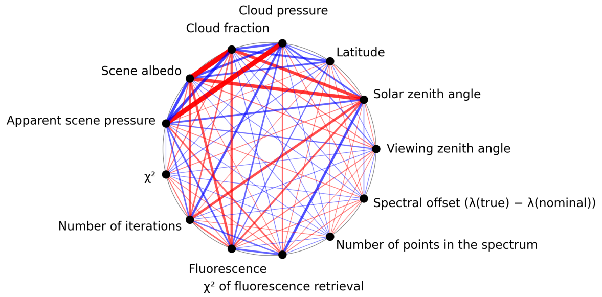
Figure 1: Map of correlation graph for 2025-01-25 to 2025-01-27.
