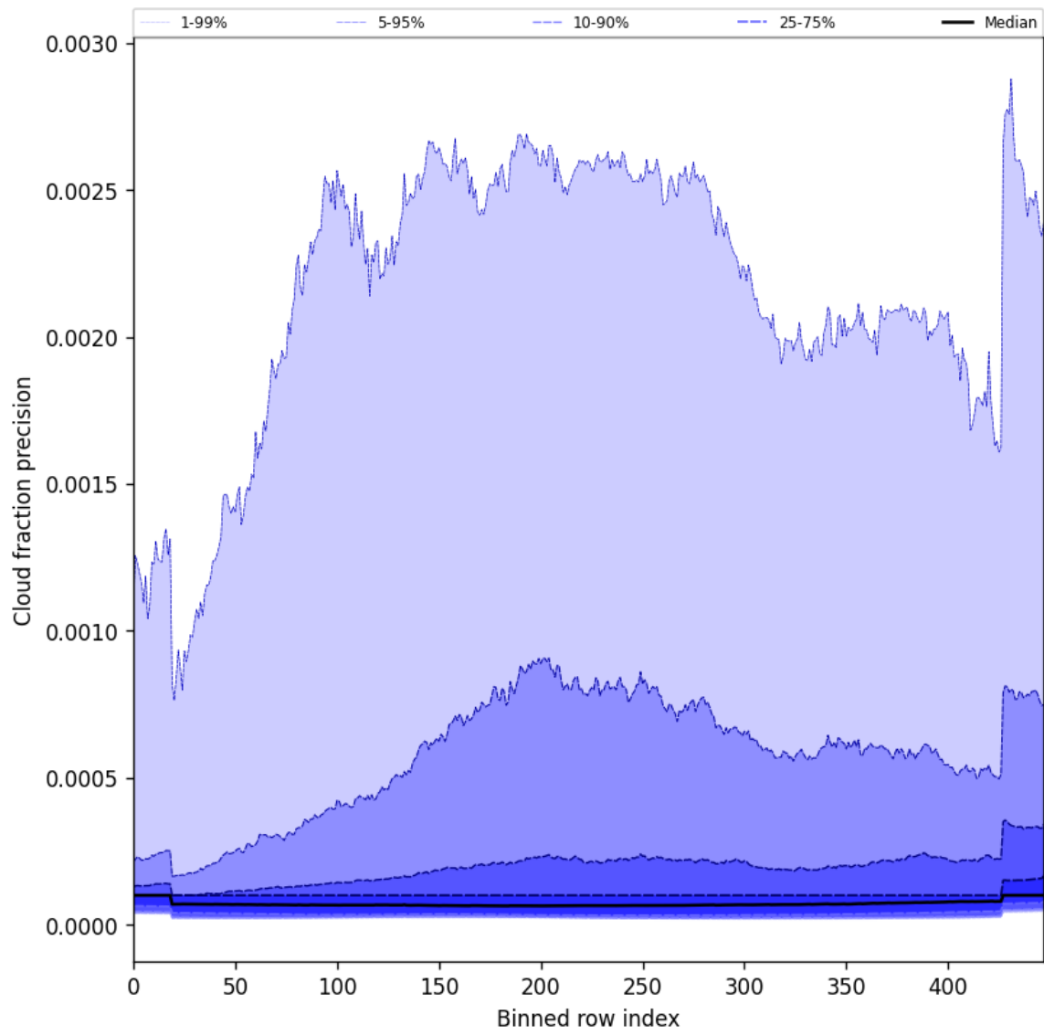
Figure 50: Along track statistics of “Cloud fraction precision” for 2025-01-25 to 2025-01-27
