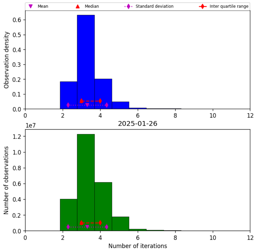
Figure 39: Histogram of “Number of iterations” for 2025-01-25 to 2025-01-27
