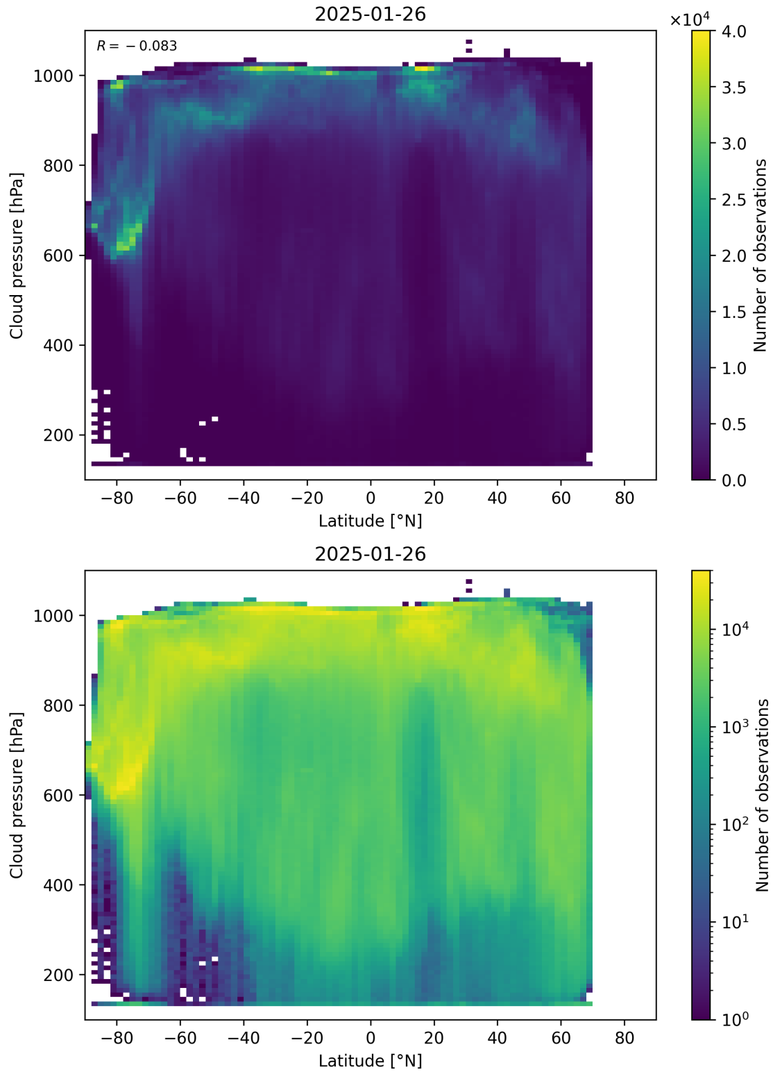
Figure 91: Scatter density plot of “Latitude” against “Cloud pressure” for 2025-01-25 to 2025-01-27.
