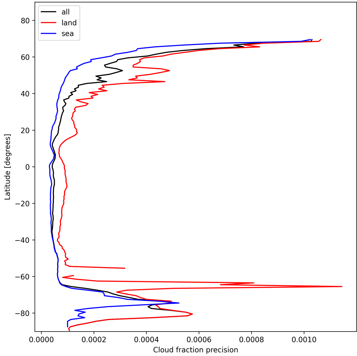
Figure 16: Zonal average of “Cloud fraction precision” for 2025-01-25 to 2025-01-27.
