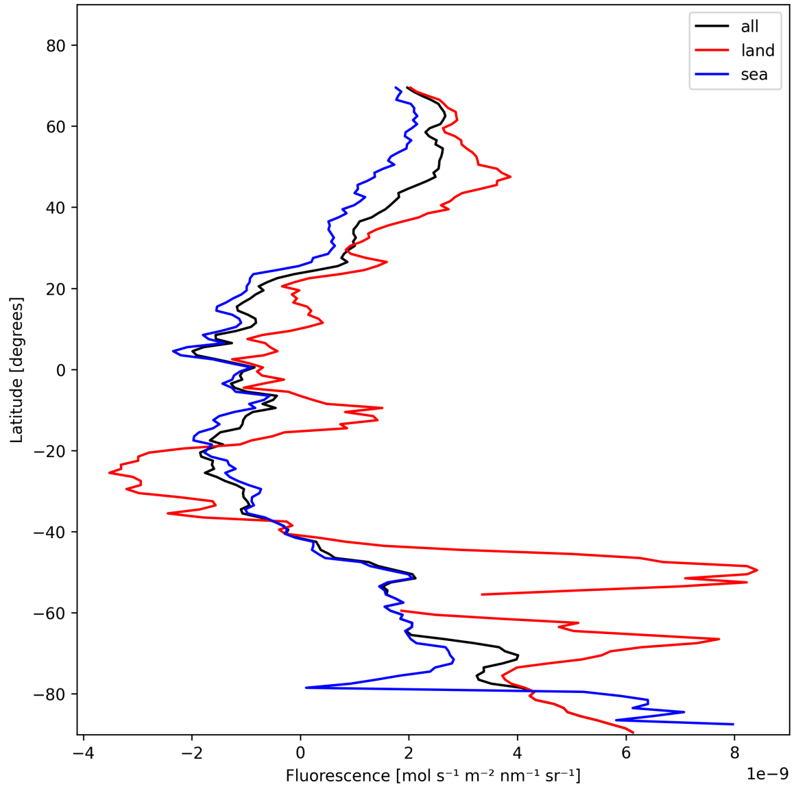
Figure 23: Zonal average of “Fluorescence” for 2025-01-25 to 2025-01-27.
