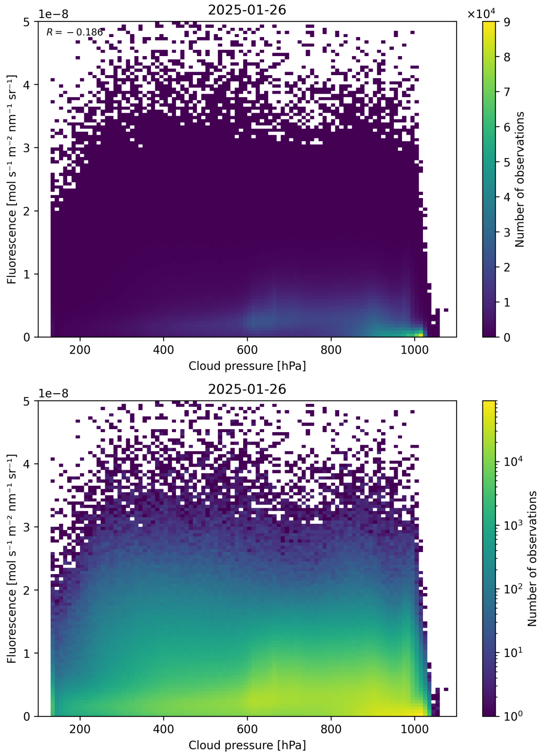
Figure 80: Scatter density plot of “Cloud pressure” against “Fluorescence” for 2025-01-25 to 2025-01-27.
