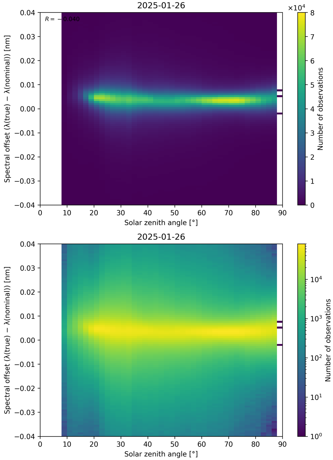
Figure 117: Scatter density plot of “Solar zenith angle” against “Spectral offset ( \lambda_{\text{true}} - \lambda_{\text{nominal}} )” for 2025-01-25 to 2025-01-27.
