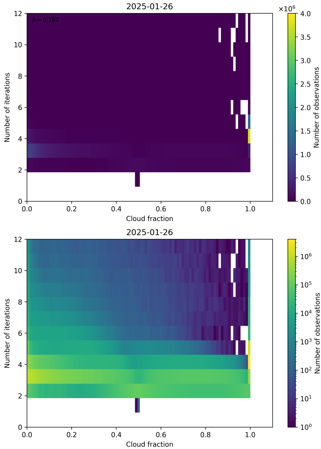
Figure 73: Scatter density plot of “Cloud fraction” against “Number of iterations” for 2025-01-25 to 2025-01-27.
