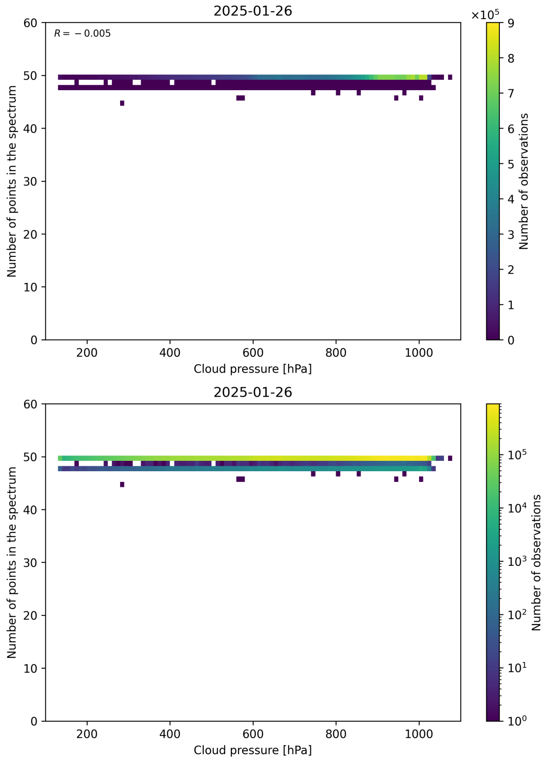
Figure 82: Scatter density plot of “Cloud pressure” against “Number of points in the spectrum” for 2025-01-25 to 2025-01-27.
