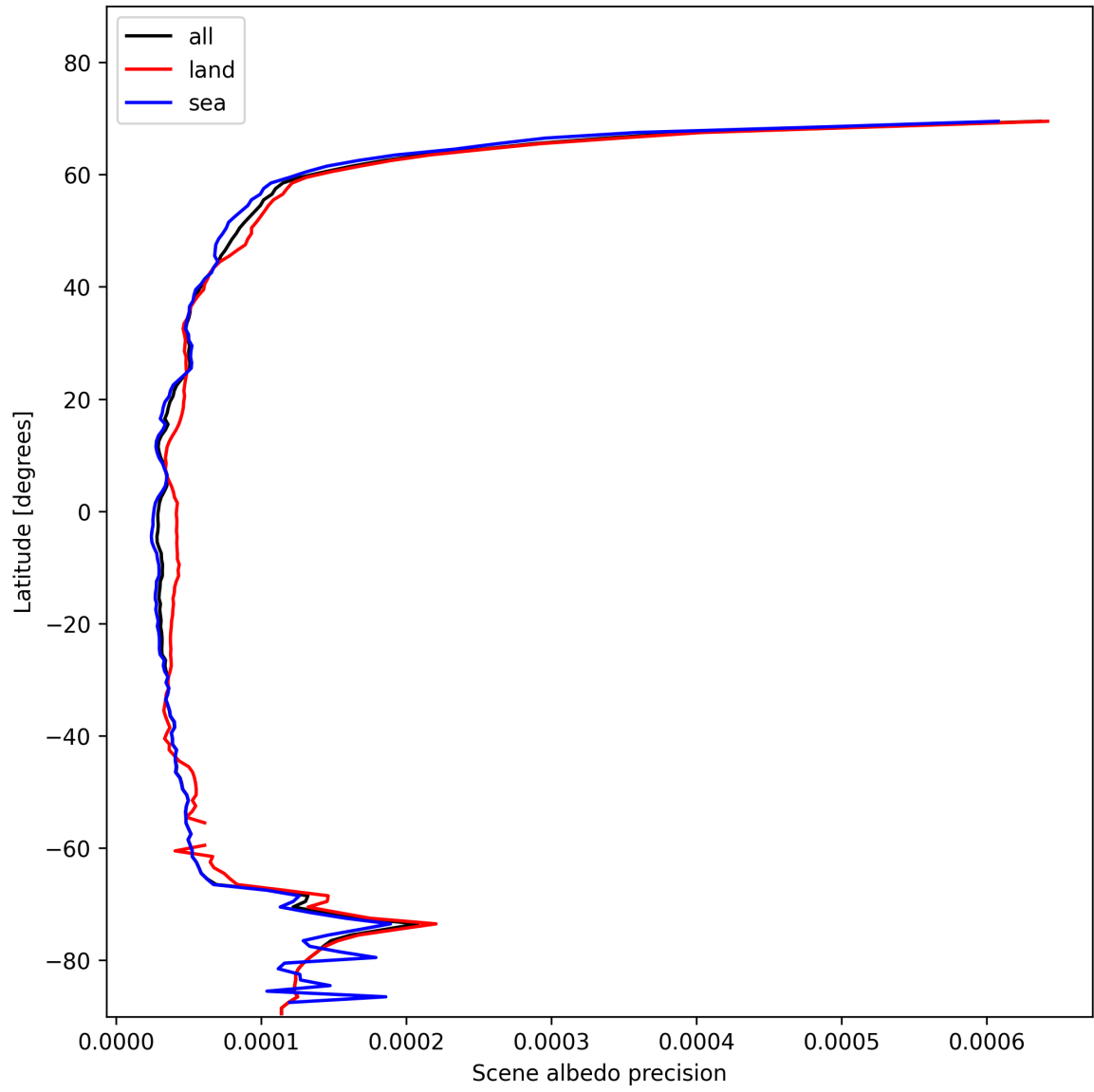
Figure 18: Zonal average of “Scene albedo precision” for 2025-01-25 to 2025-01-27.
