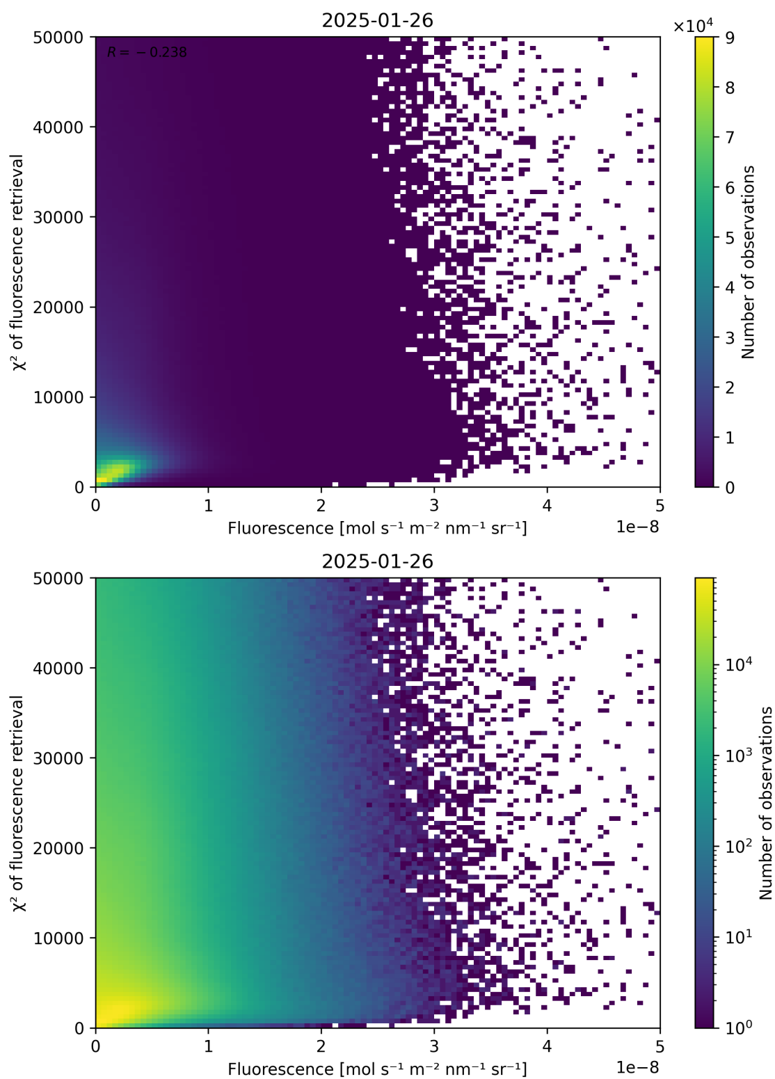
Figure 85: Scatter density plot of “Fluorescence” against “ \chi^2 of fluorescence retrieval” for 2025-01-25 to 2025-01-27.
