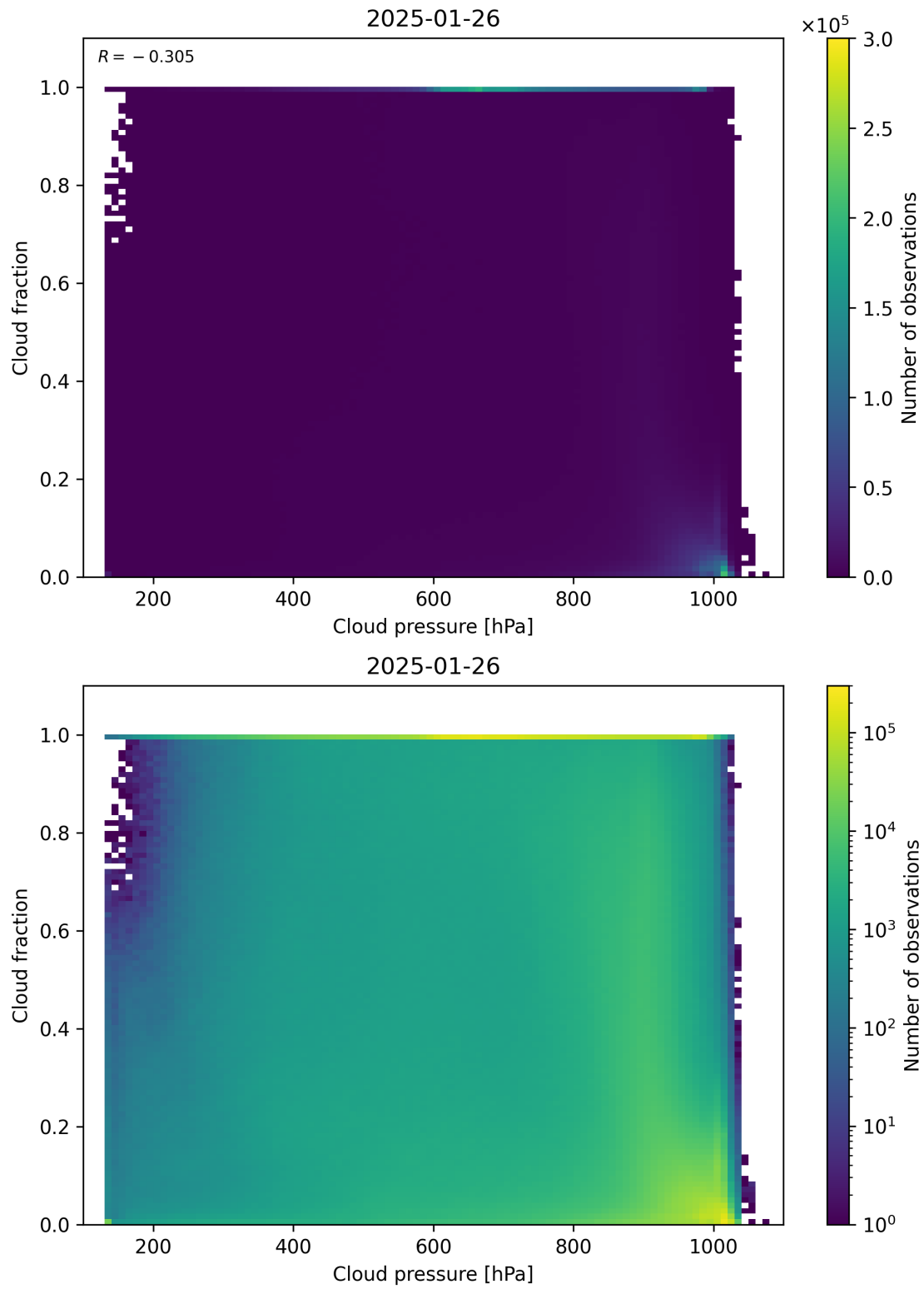
Figure 79: Scatter density plot of “Cloud pressure” against “Cloud fraction” for 2025-01-25 to 2025-01-27.
