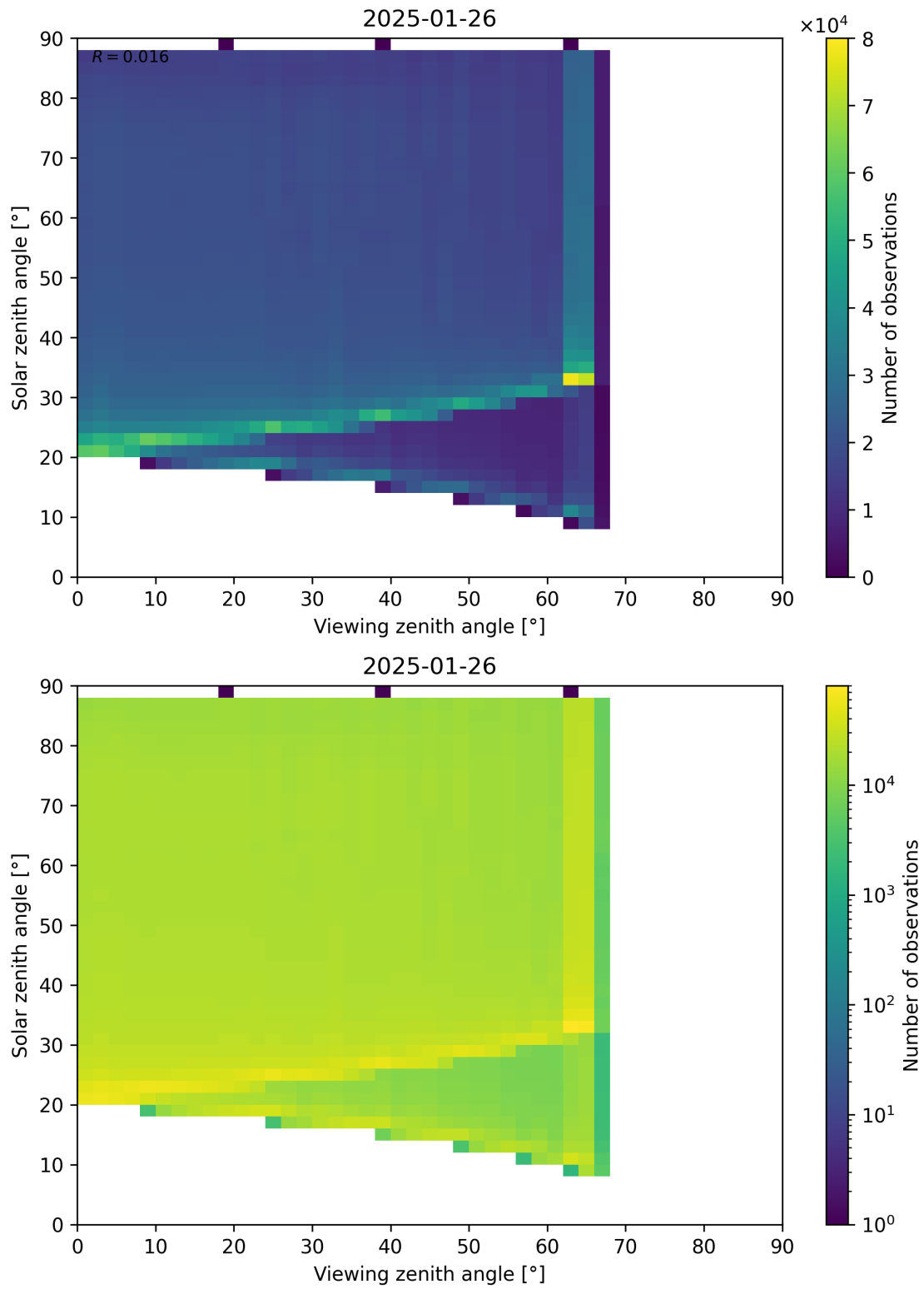
Figure 127: Scatter density plot of “Viewing zenith angle” against “Solar zenith angle” for 2025-01-25 to 2025-01-27.
