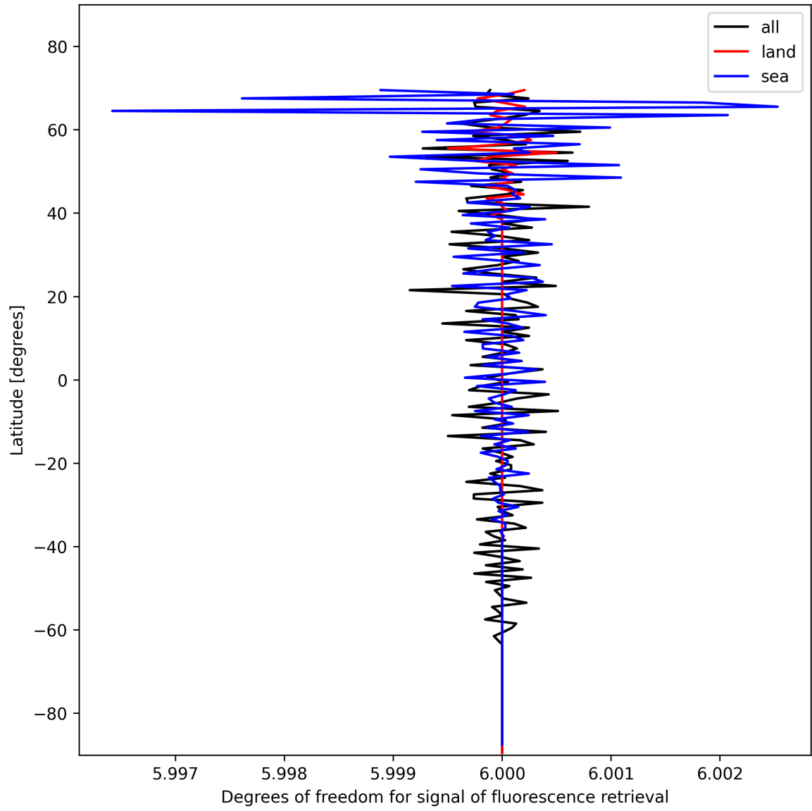
Figure 26: Zonal average of “Degrees of freedom for signal of fluorescence retrieval” for 2025-01-25 to 2025-01-27.
