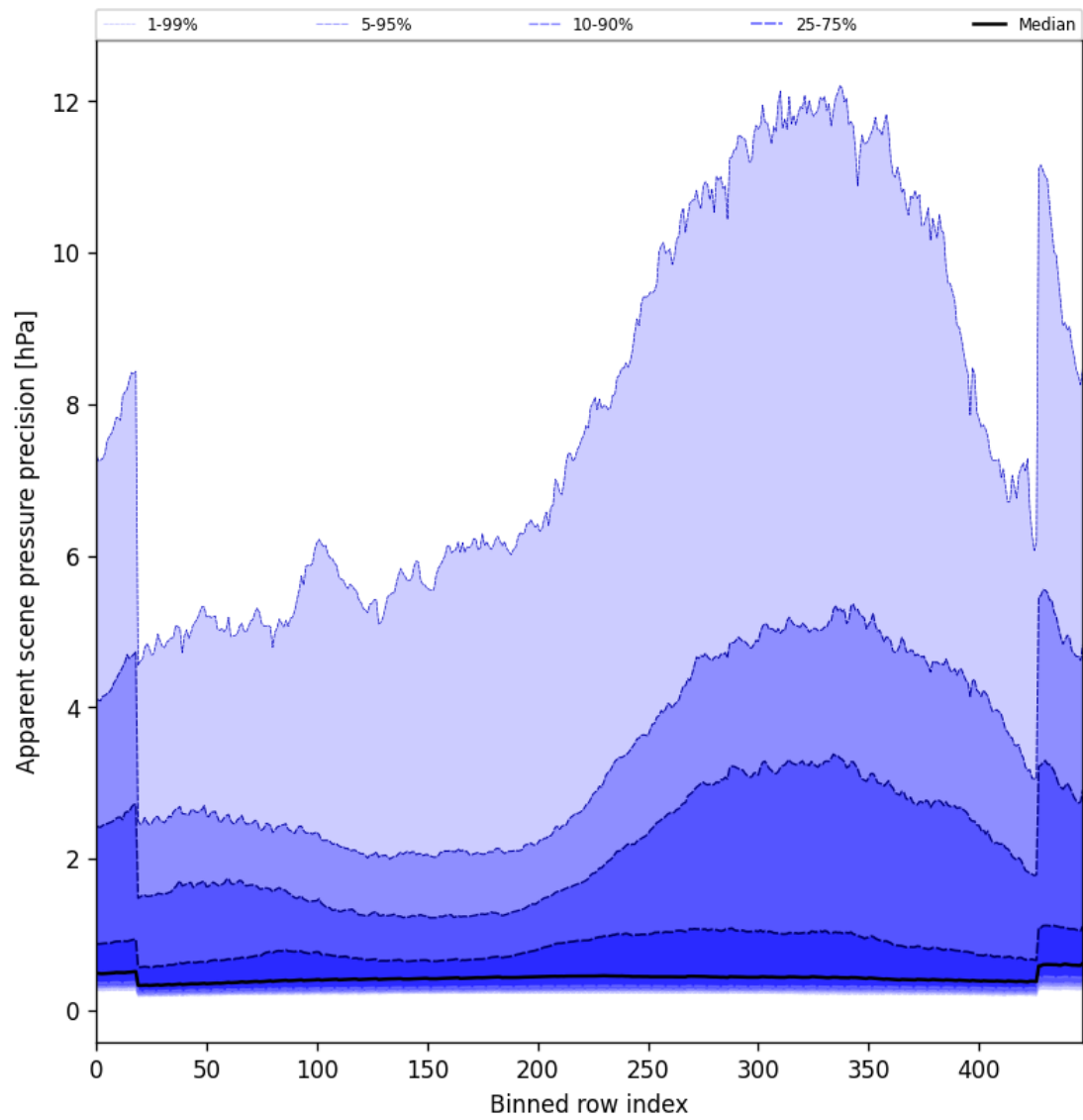
Figure 54: Along track statistics of “Apparent scene pressure precision” for 2025-01-25 to 2025-01-27
