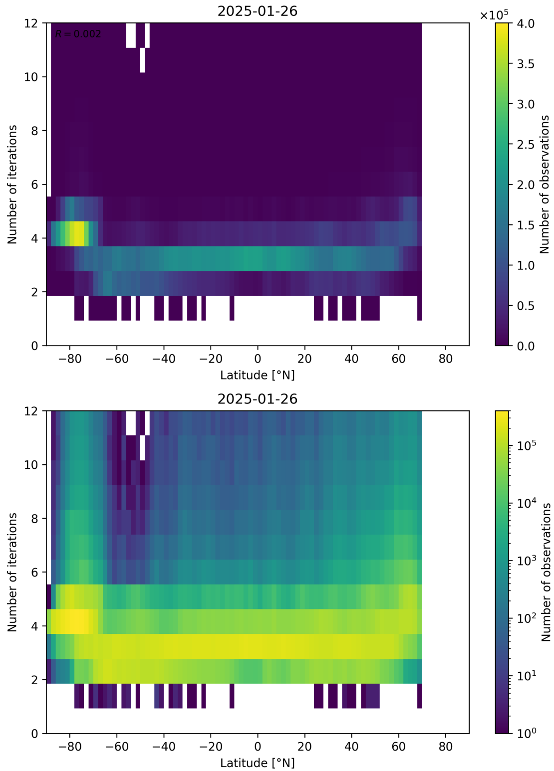
Figure 93: Scatter density plot of “Latitude” against “Number of iterations” for 2025-01-25 to 2025-01-27.
