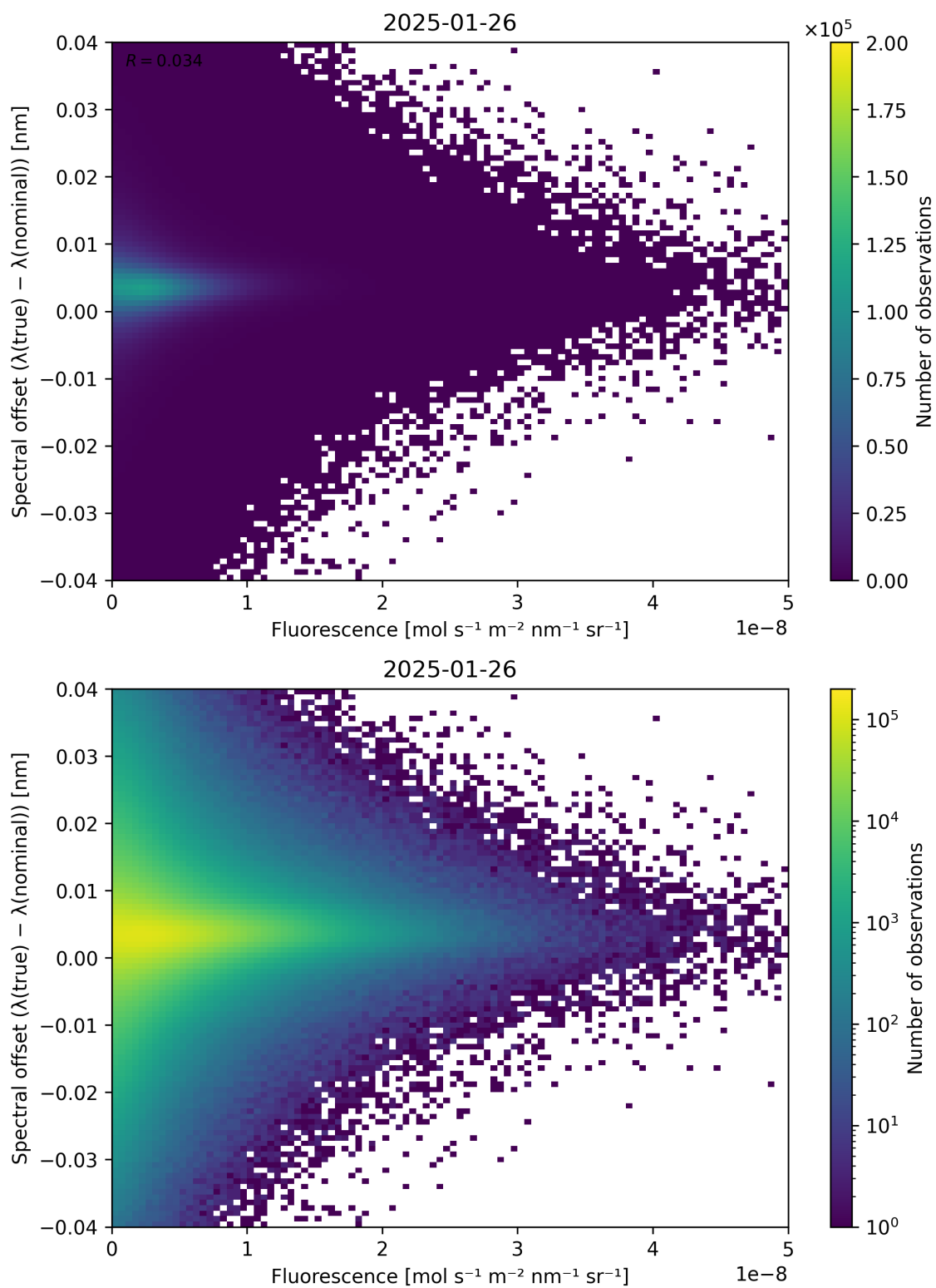
Figure 87: Scatter density plot of “Fluorescence” against “Spectral offset ( \lambda_{\text{true}} - \lambda_{\text{nominal}} )” for 2025-01-25 to 2025-01-27.
