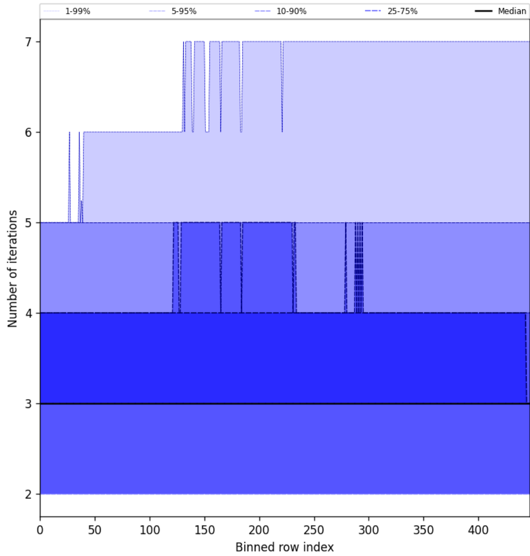
Figure 56: Along track statistics of “Number of iterations” for 2025-01-25 to 2025-01-27
