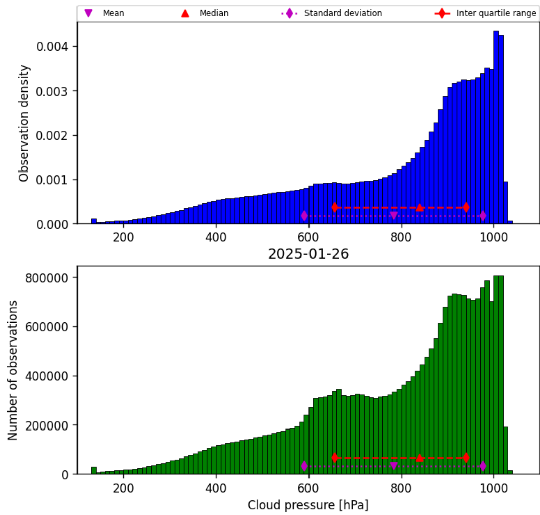
Figure 30: Histogram of “Cloud pressure” for 2025-01-25 to 2025-01-27
