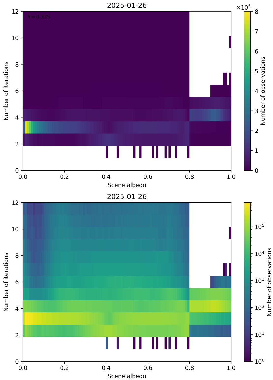
Figure 105: Scatter density plot of “Scene albedo” against “Number of iterations” for 2025-01-25 to 2025-01-27.
