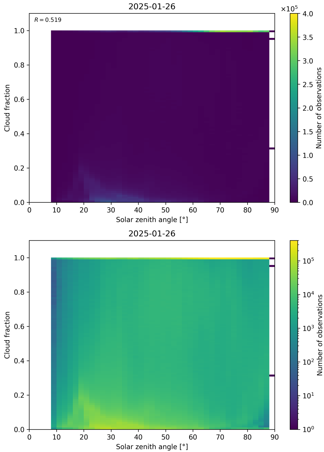
Figure 110: Scatter density plot of “Solar zenith angle” against “Cloud fraction” for 2025-01-25 to 2025-01-27.
