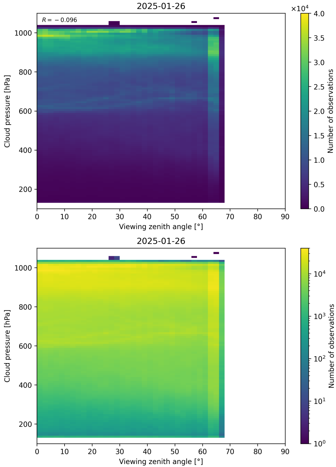
Figure 121: Scatter density plot of “Viewing zenith angle” against “Cloud pressure” for 2025-01-25 to 2025-01-27.
