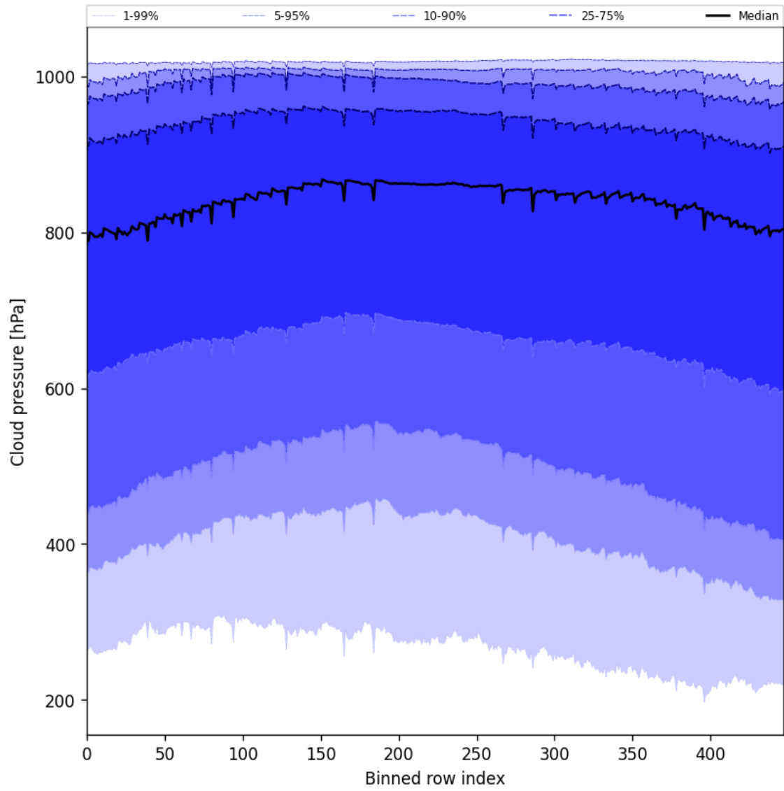
Figure 47: Along track statistics of “Cloud pressure” for 2025-01-25 to 2025-01-27
