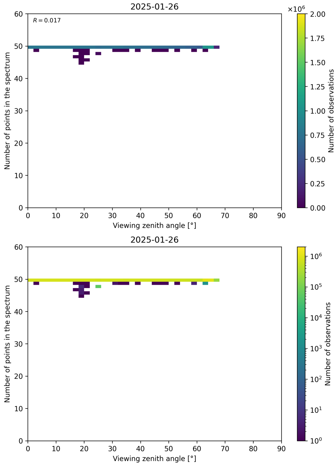
Figure 125: Scatter density plot of “Viewing zenith angle” against “Number of points in the spectrum” for 2025-01-25 to 2025-01-27.
