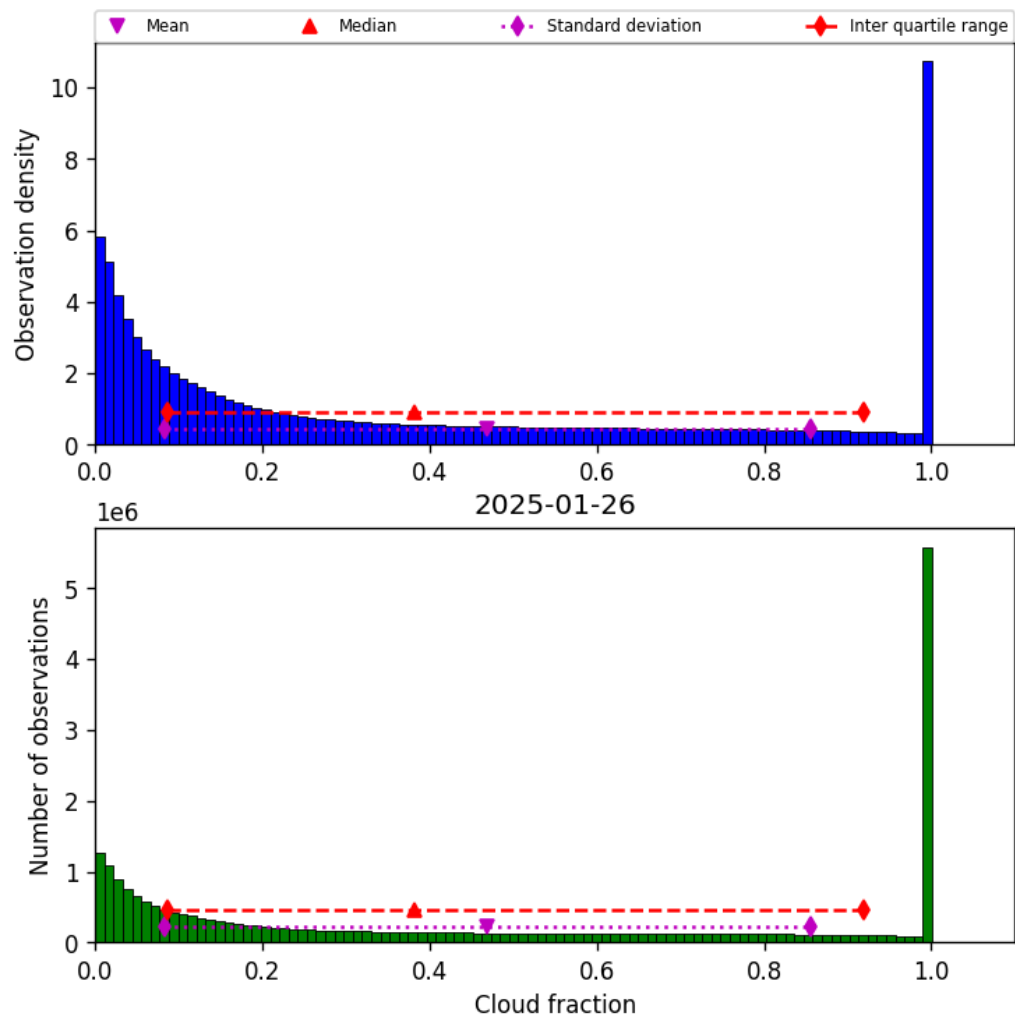
Figure 32: Histogram of “Cloud fraction” for 2025-01-25 to 2025-01-27
