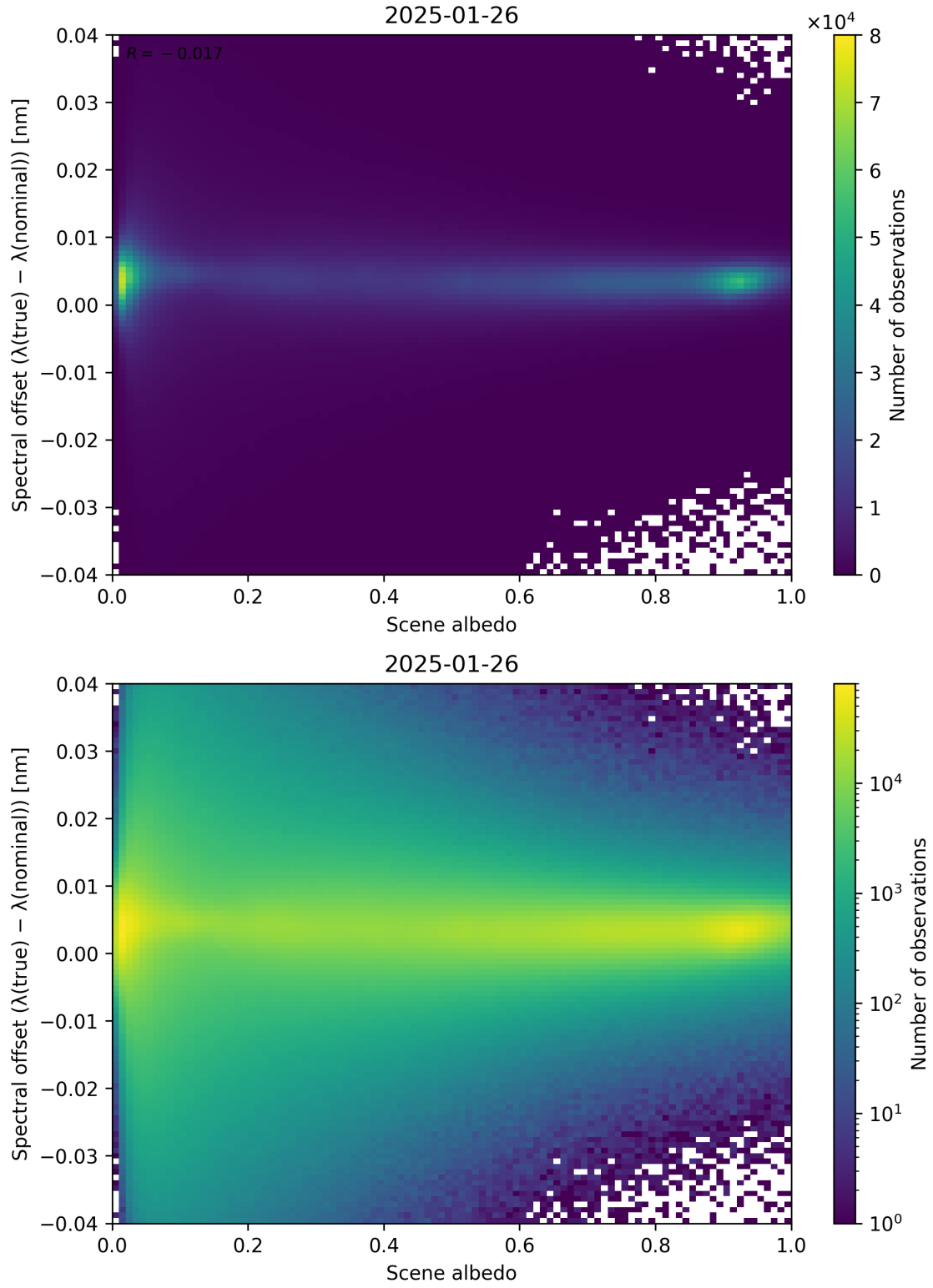
Figure 107: Scatter density plot of “Scene albedo” against “Spectral offset ( \lambda_{\text{true}} - \lambda_{\text{nominal}} )” for 2025-01-25 to 2025-01-27.
