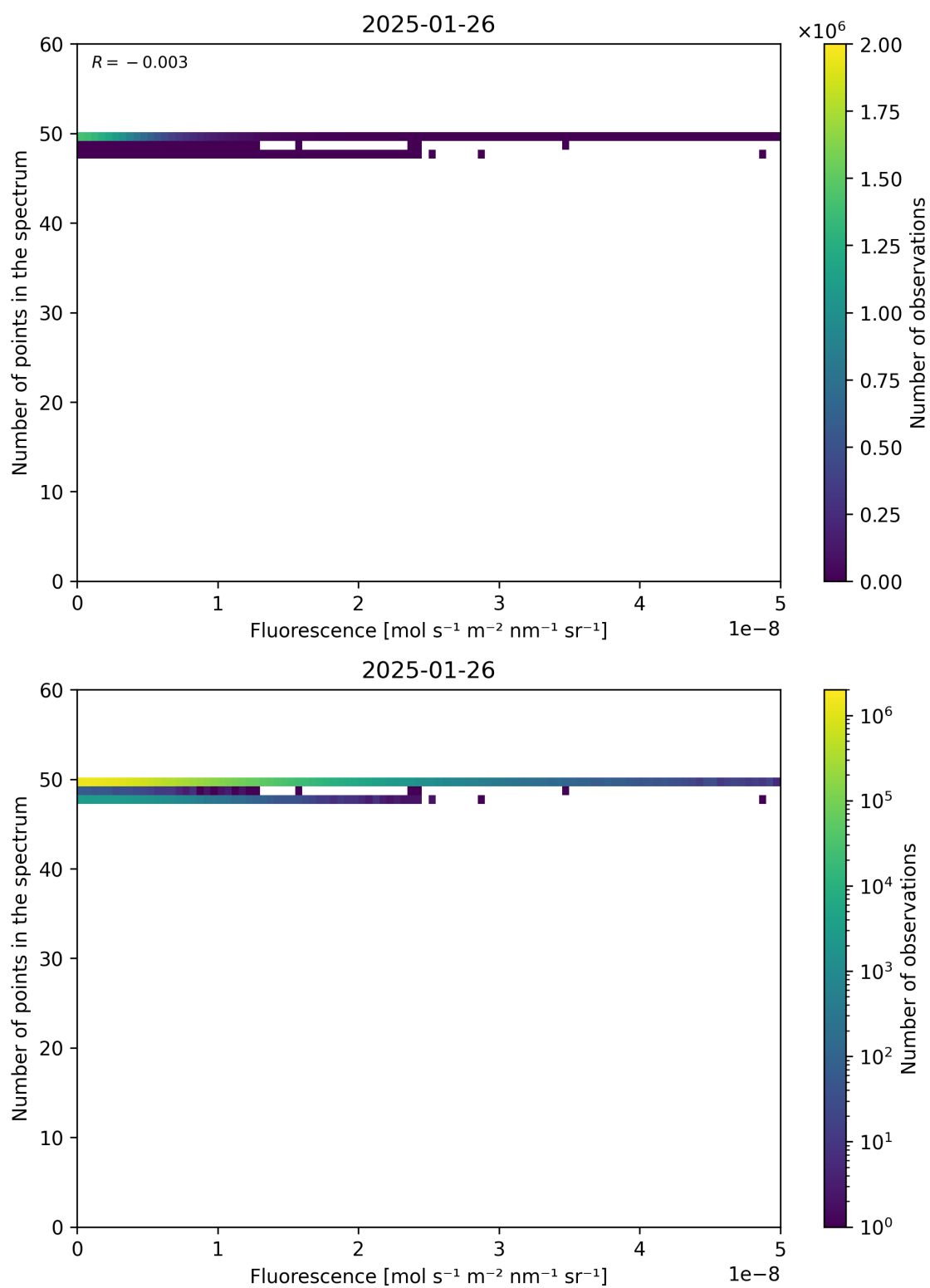
Figure 86: Scatter density plot of “Fluorescence” against “Number of points in the spectrum” for 2025-01-25 to 2025-01-27.
