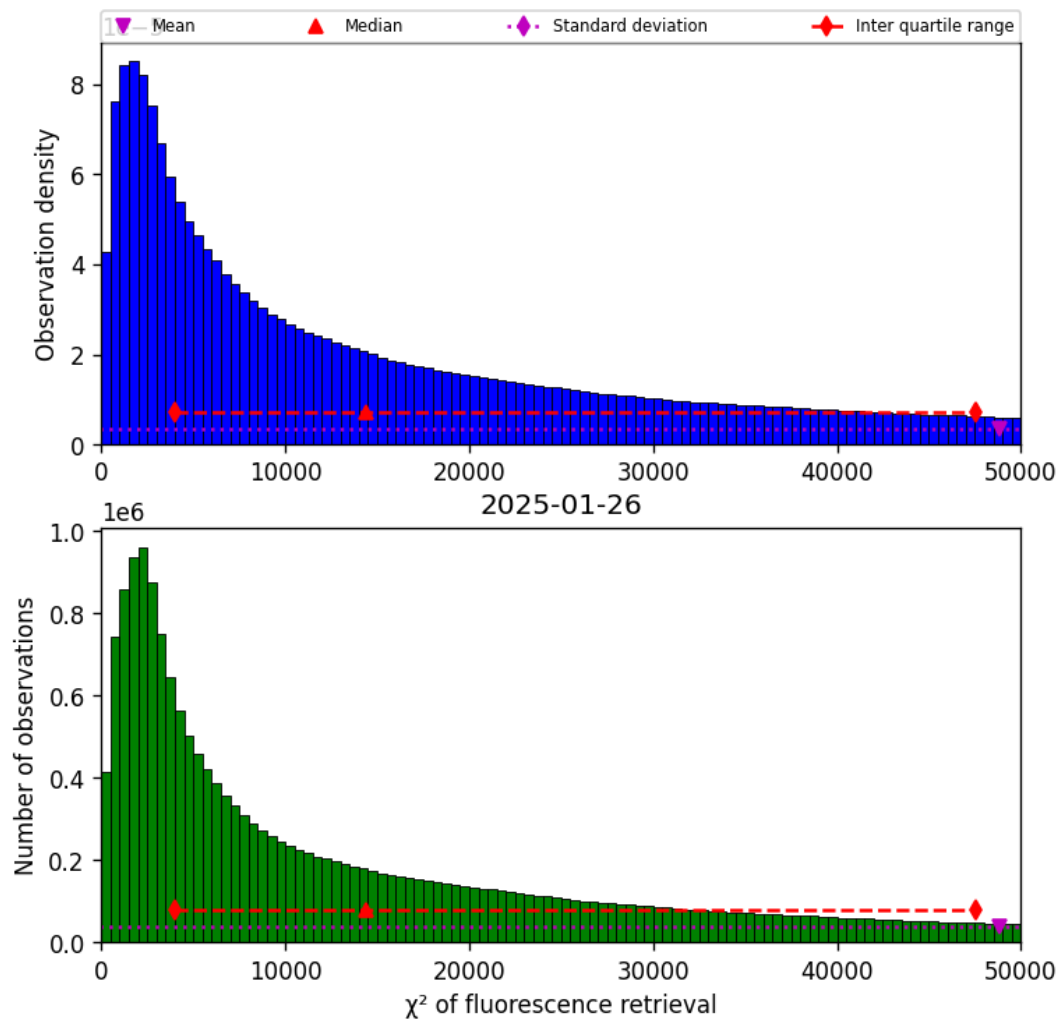
Figure 42: Histogram of “ \chi^2 of fluorescence retrieval” for 2025-01-25 to 2025-01-27
