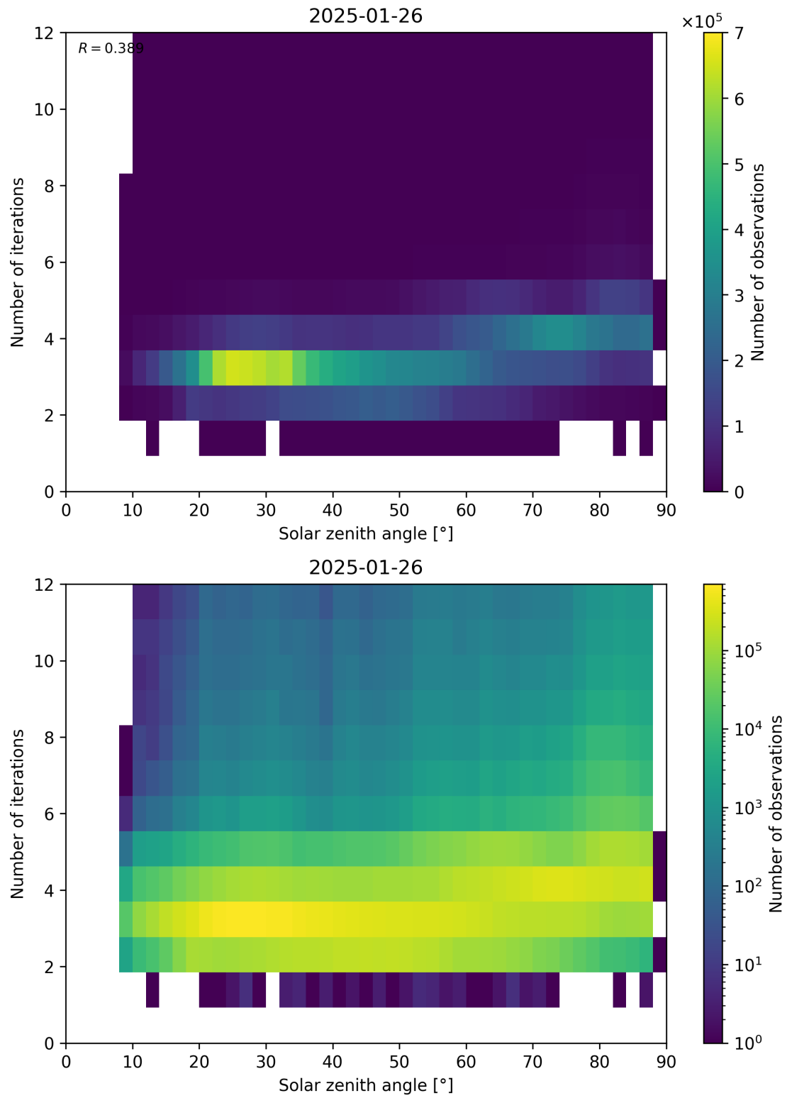
Figure 114: Scatter density plot of “Solar zenith angle” against “Number of iterations” for 2025-01-25 to 2025-01-27.
