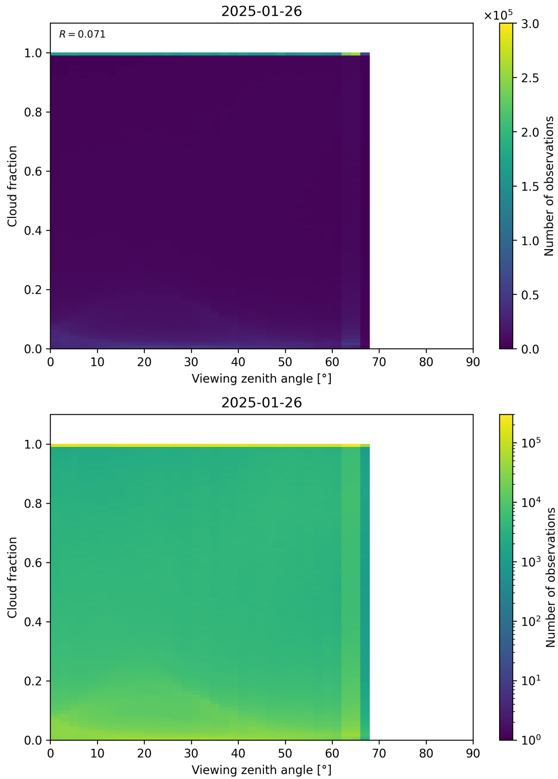
Figure 120: Scatter density plot of “Viewing zenith angle” against “Cloud fraction” for 2025-01-25 to 2025-01-27.
