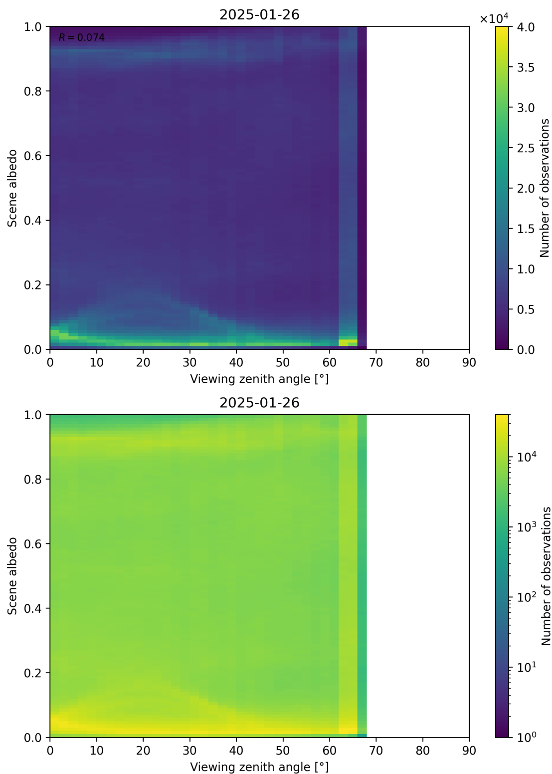
Figure 126: Scatter density plot of “Viewing zenith angle” against “Scene albedo” for 2025-01-25 to 2025-01-27.
