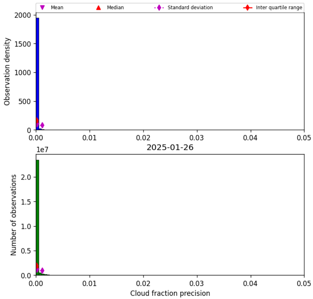
Figure 33: Histogram of “Cloud fraction precision” for 2025-01-25 to 2025-01-27
