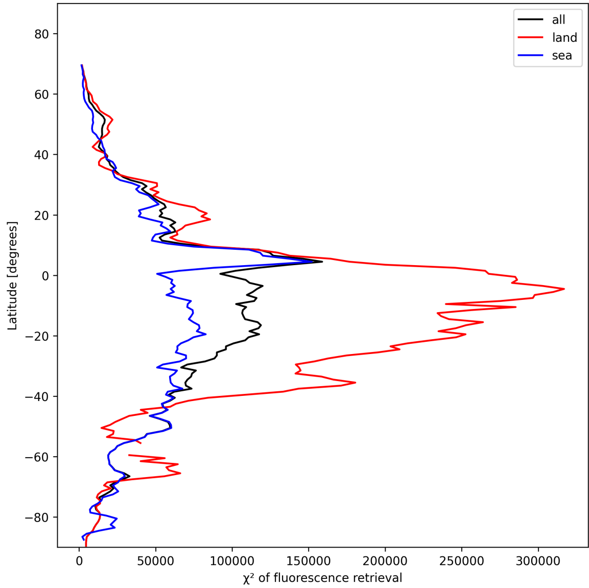
Figure 25: Zonal average of “ \chi^2 of fluorescence retrieval” for 2025-01-25 to 2025-01-27.
