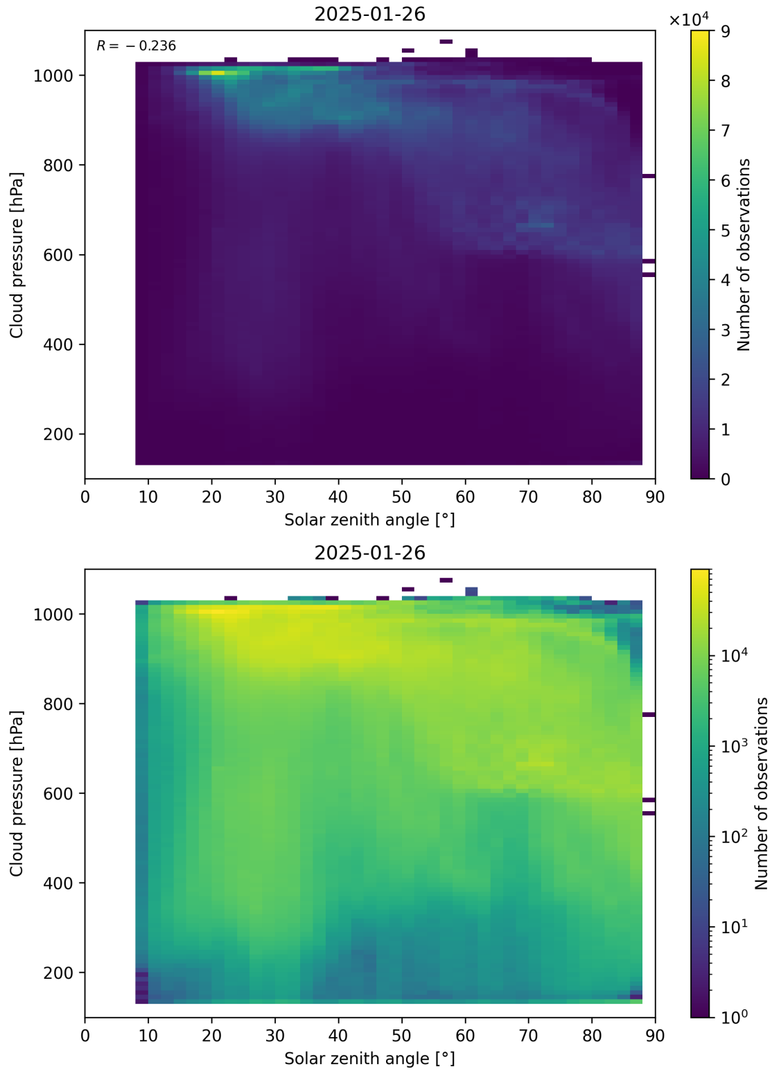
Figure 111: Scatter density plot of “Solar zenith angle” against “Cloud pressure” for 2025-01-25 to 2025-01-27.
