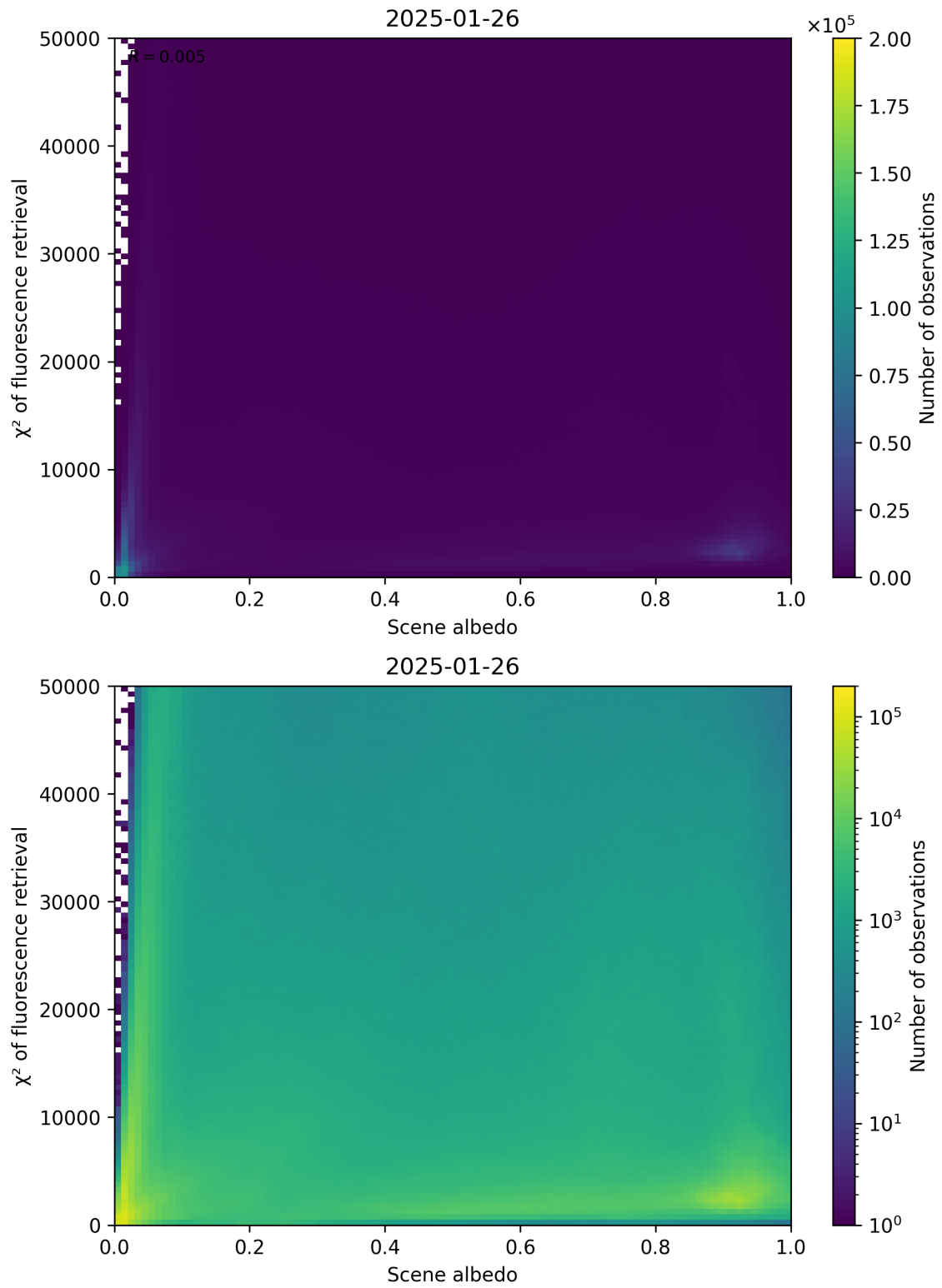
Figure 103: Scatter density plot of “Scene albedo” against “ \chi^2 of fluorescence retrieval” for 2025-01-25 to 2025-01-27.
