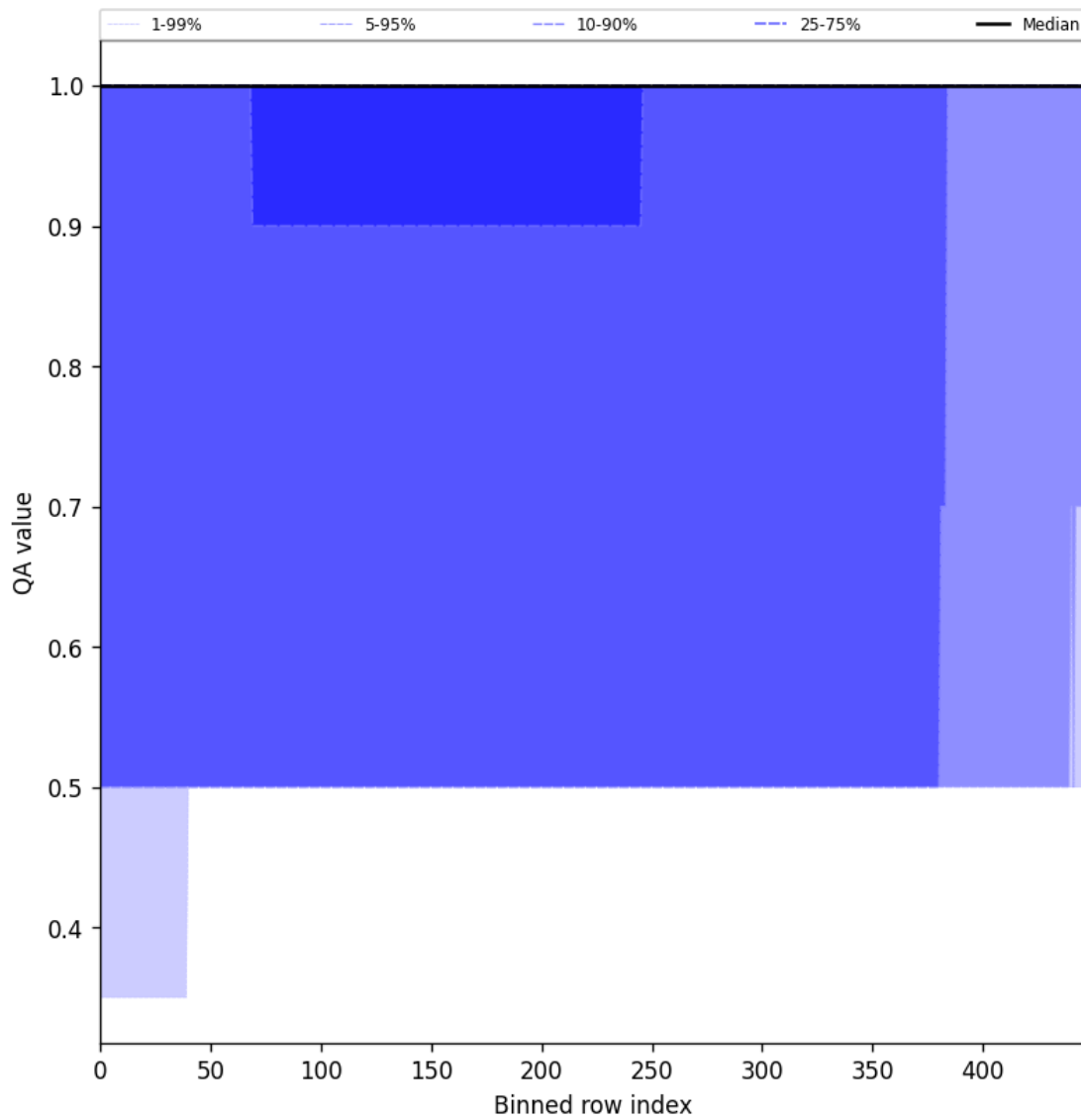
Figure 46: Along track statistics of “QA value” for 2025-01-25 to 2025-01-27
