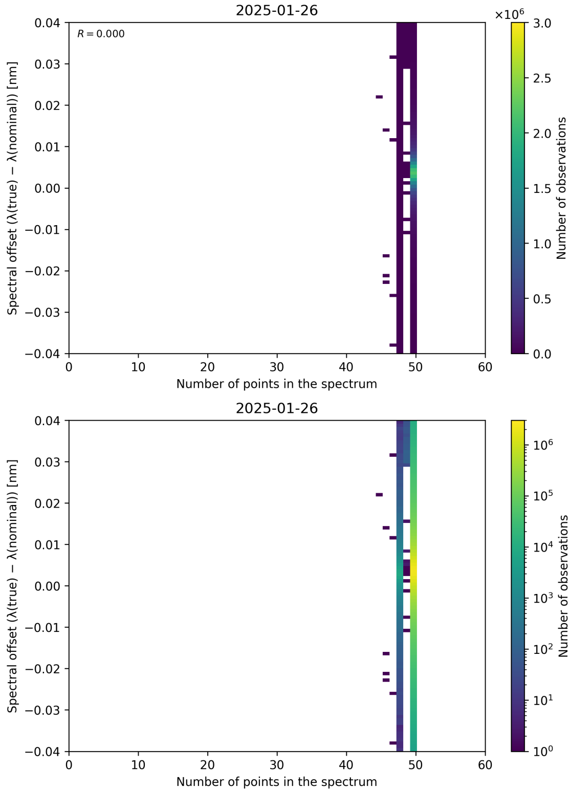
Figure 101: Scatter density plot of “Number of points in the spectrum” against “Spectral offset ( \lambda_{\text{true}} - \lambda_{\text{nominal}} )” for 2025-01-25 to 2025-01-27.
