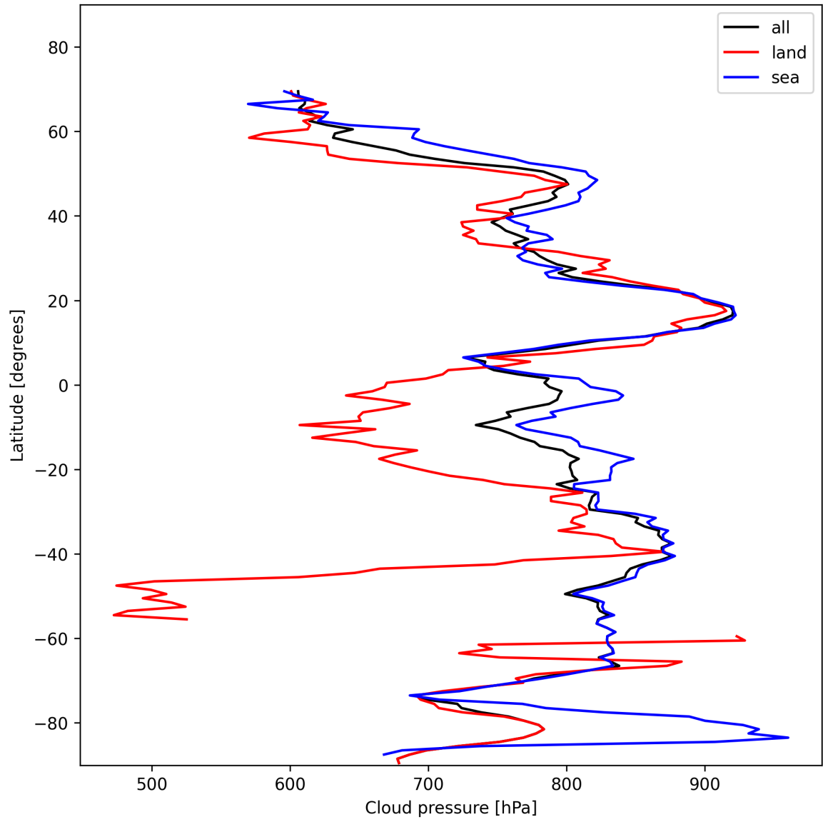
Figure 13: Zonal average of “Cloud pressure” for 2025-01-25 to 2025-01-27.
