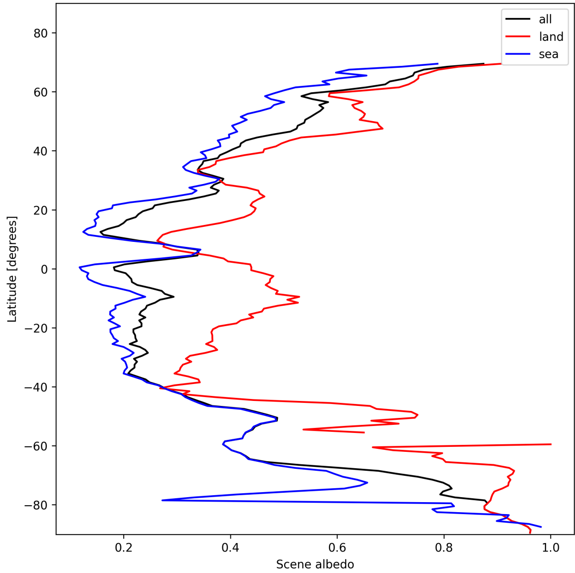
Figure 17: Zonal average of “Scene albedo” for 2025-01-25 to 2025-01-27.
