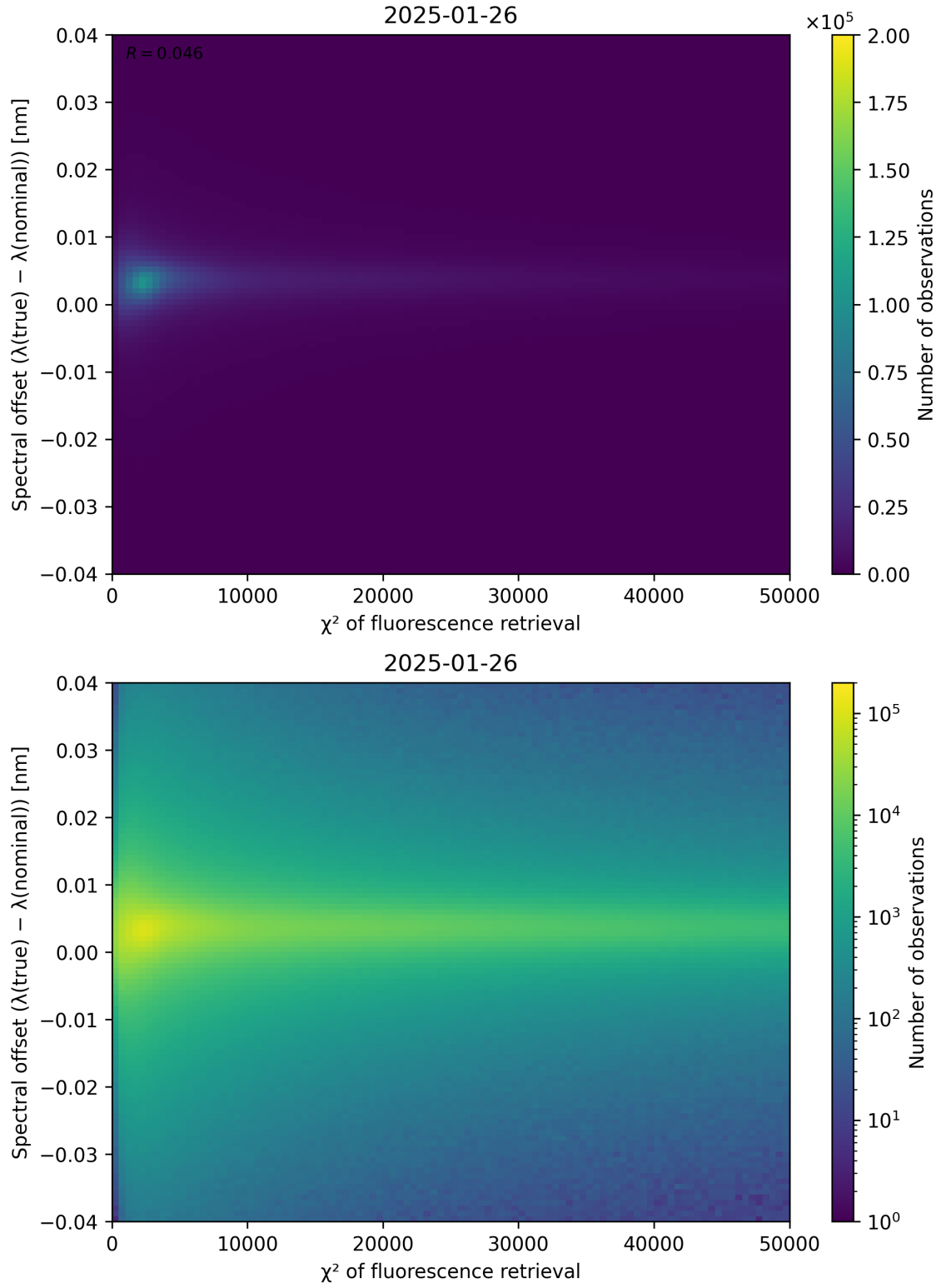
Figure 69: Scatter density plot of “ \chi^2 of fluorescence retrieval” against “Spectral offset ( \lambda_{\text{true}} - \lambda_{\text{nominal}} )” for 2025-01-25 to 2025-01-27.
