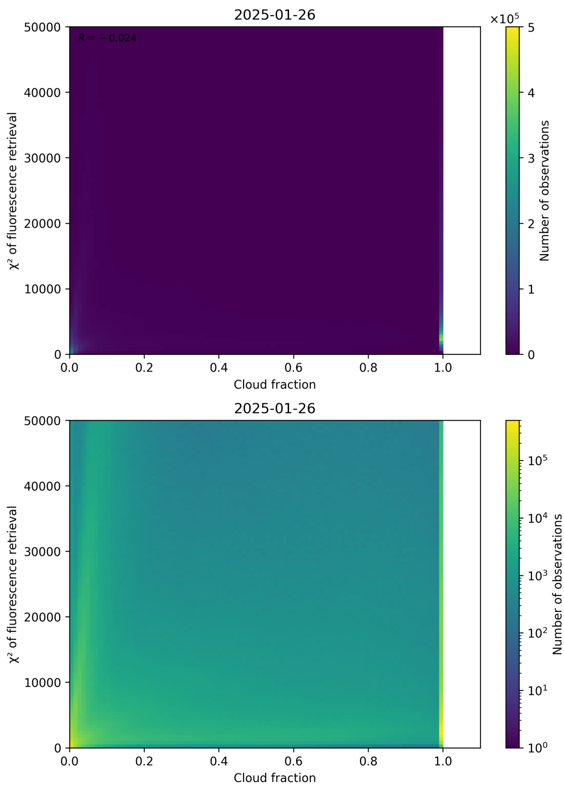
Figure 71: Scatter density plot of “Cloud fraction” against “ \chi^2 of fluorescence retrieval” for 2025-01-25 to 2025-01-27.
