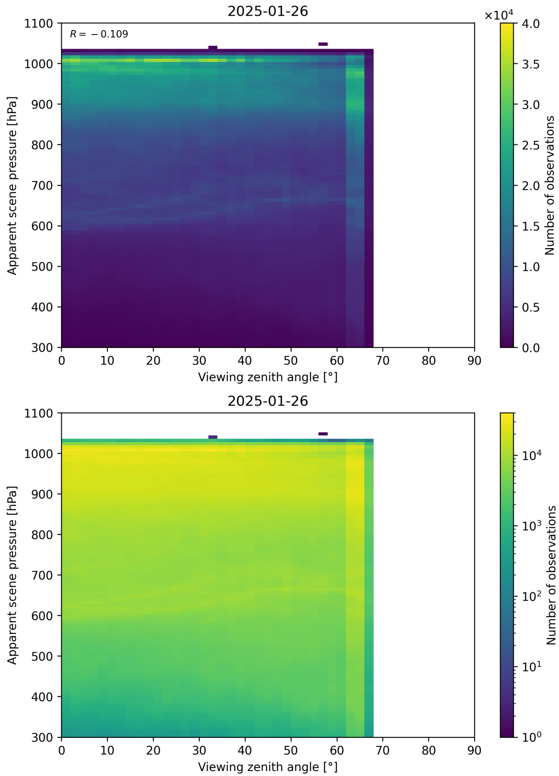
Figure 118: Scatter density plot of “Viewing zenith angle” against “Apparent scene pressure” for 2025-01-25 to 2025-01-27.
