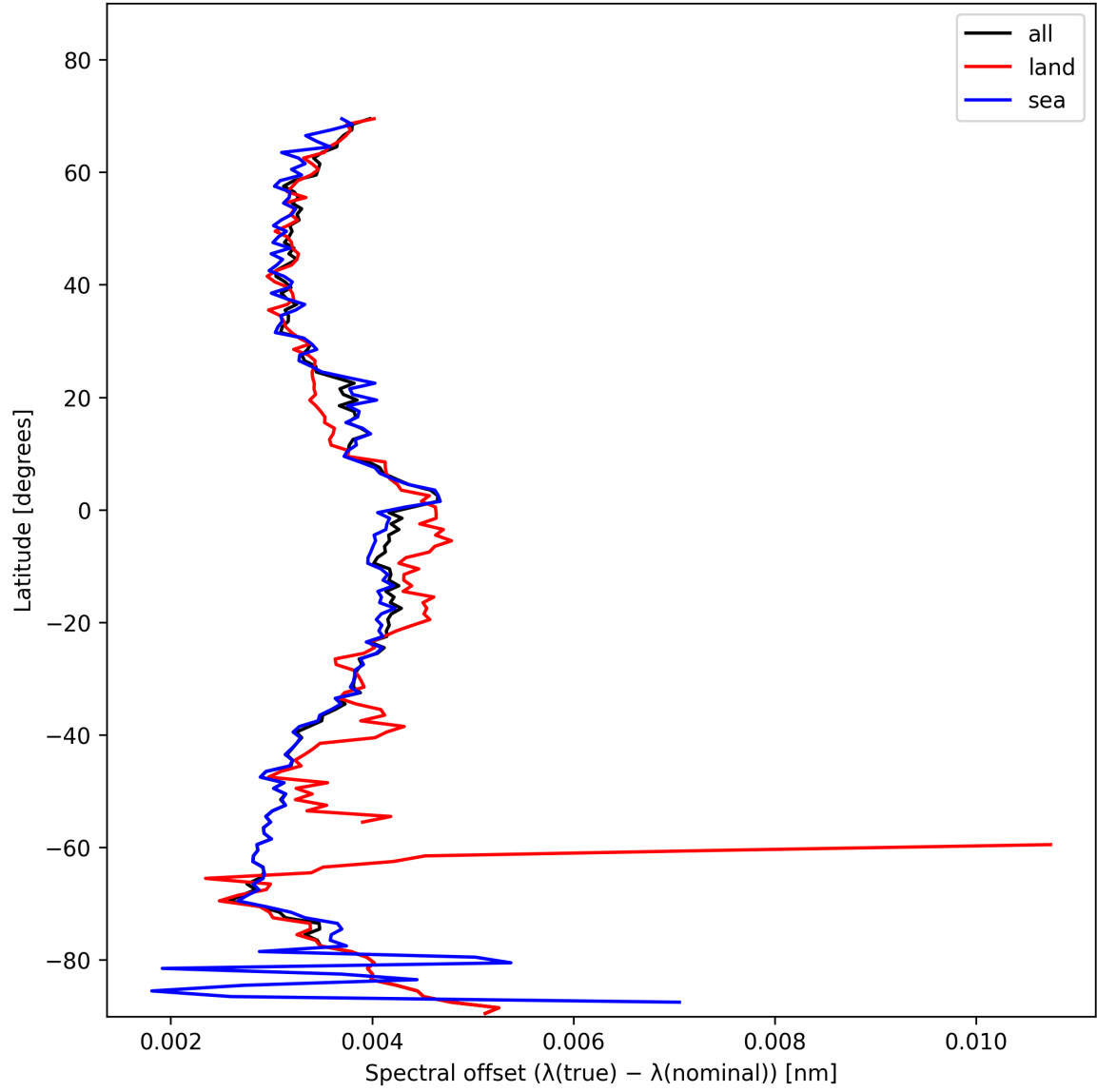
Figure 28: Zonal average of “Spectral offset ( \lambda_{\text{true}} - \lambda_{\text{nominal}} )” for 2025-01-25 to 2025-01-27.
