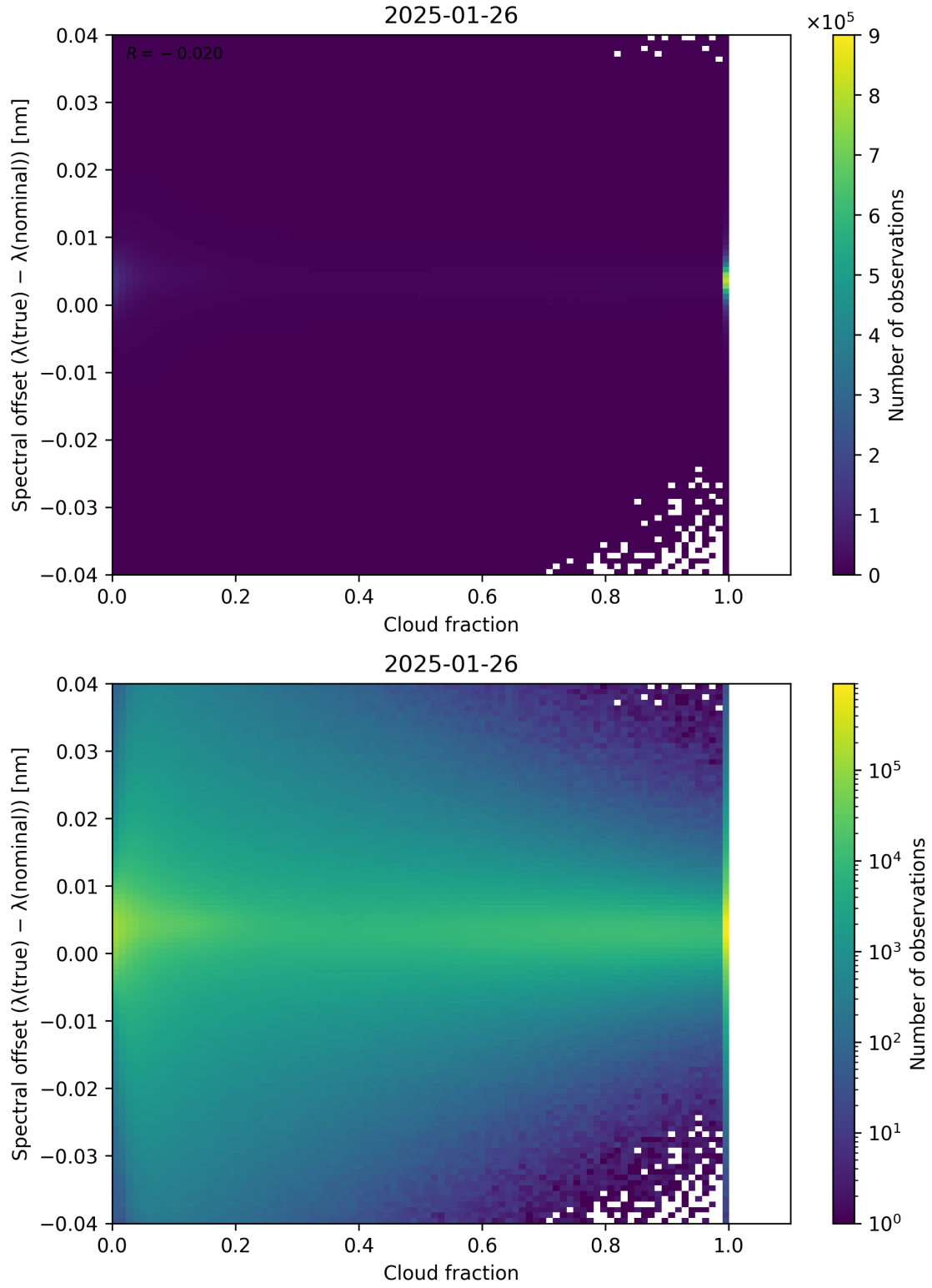
Figure 76: Scatter density plot of “Cloud fraction” against “Spectral offset ( \lambda_{\text{true}} - \lambda_{\text{nominal}} )” for 2025-01-25 to 2025-01-27.
