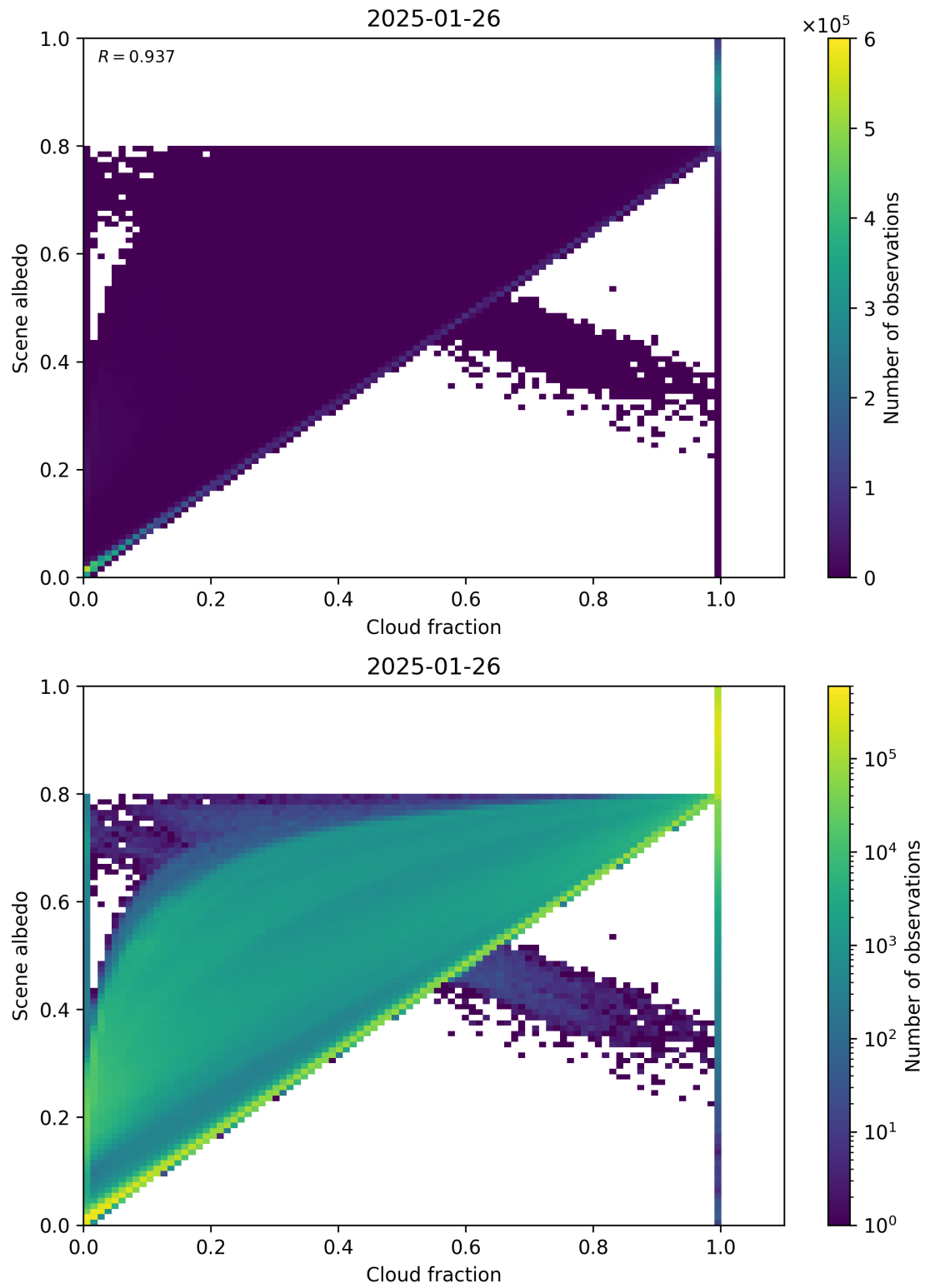
Figure 75: Scatter density plot of “Cloud fraction” against “Scene albedo” for 2025-01-25 to 2025-01-27.
