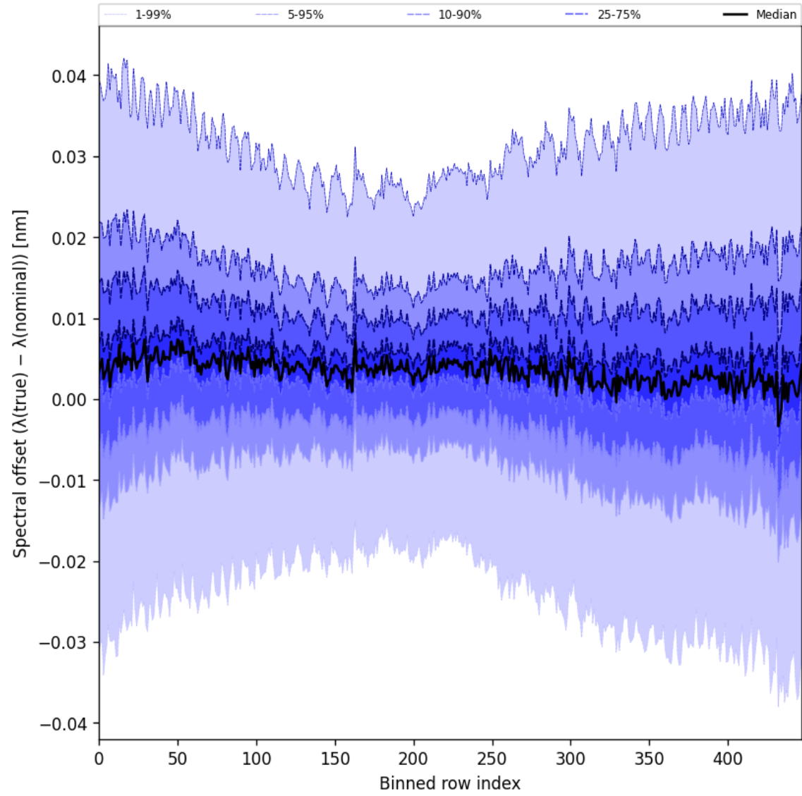
Figure 62: Along track statistics of “Spectral offset ( \lambda_{\text{true}} - \lambda_{\text{nominal}} )” for 2025-01-25 to 2025-01-27
