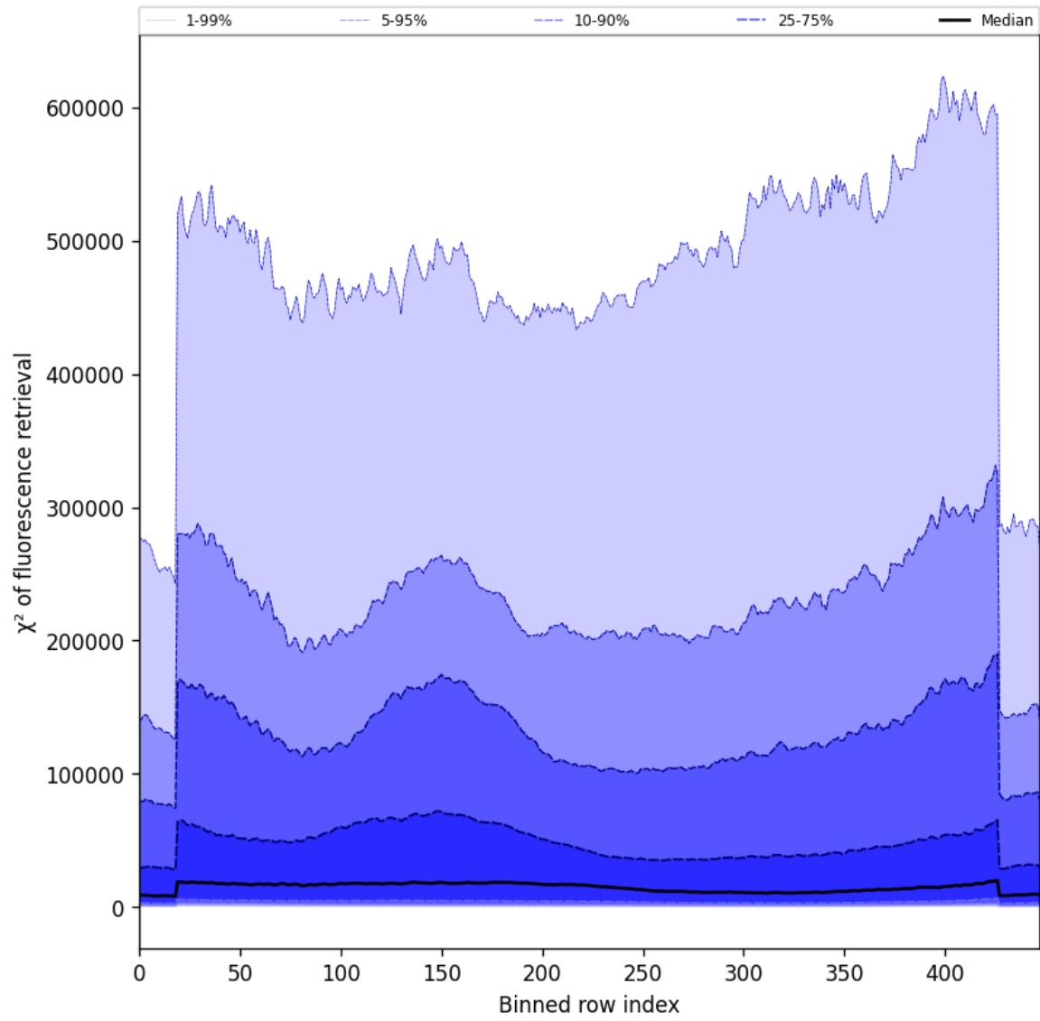
Figure 59: Along track statistics of “ \chi^2 of fluorescence retrieval” for 2025-01-25 to 2025-01-27
