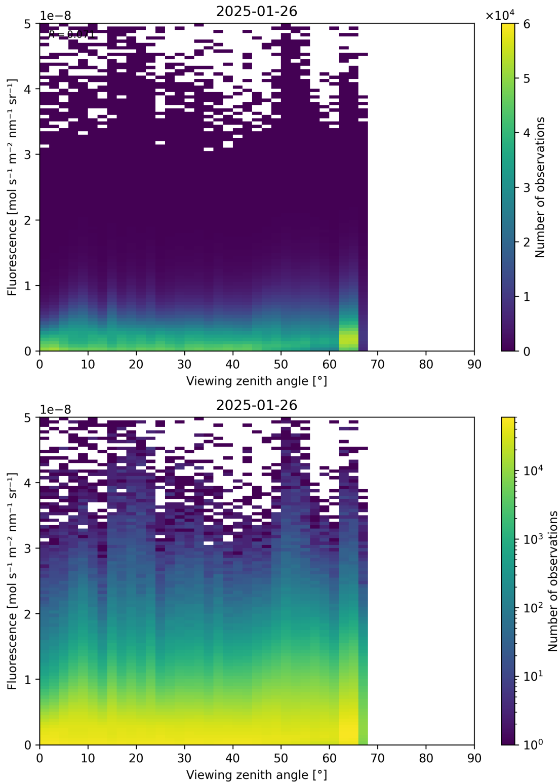
Figure 122: Scatter density plot of "Viewing zenith angle" against "Fluorescence" for 2025-01-25 to 2025-01-27.
