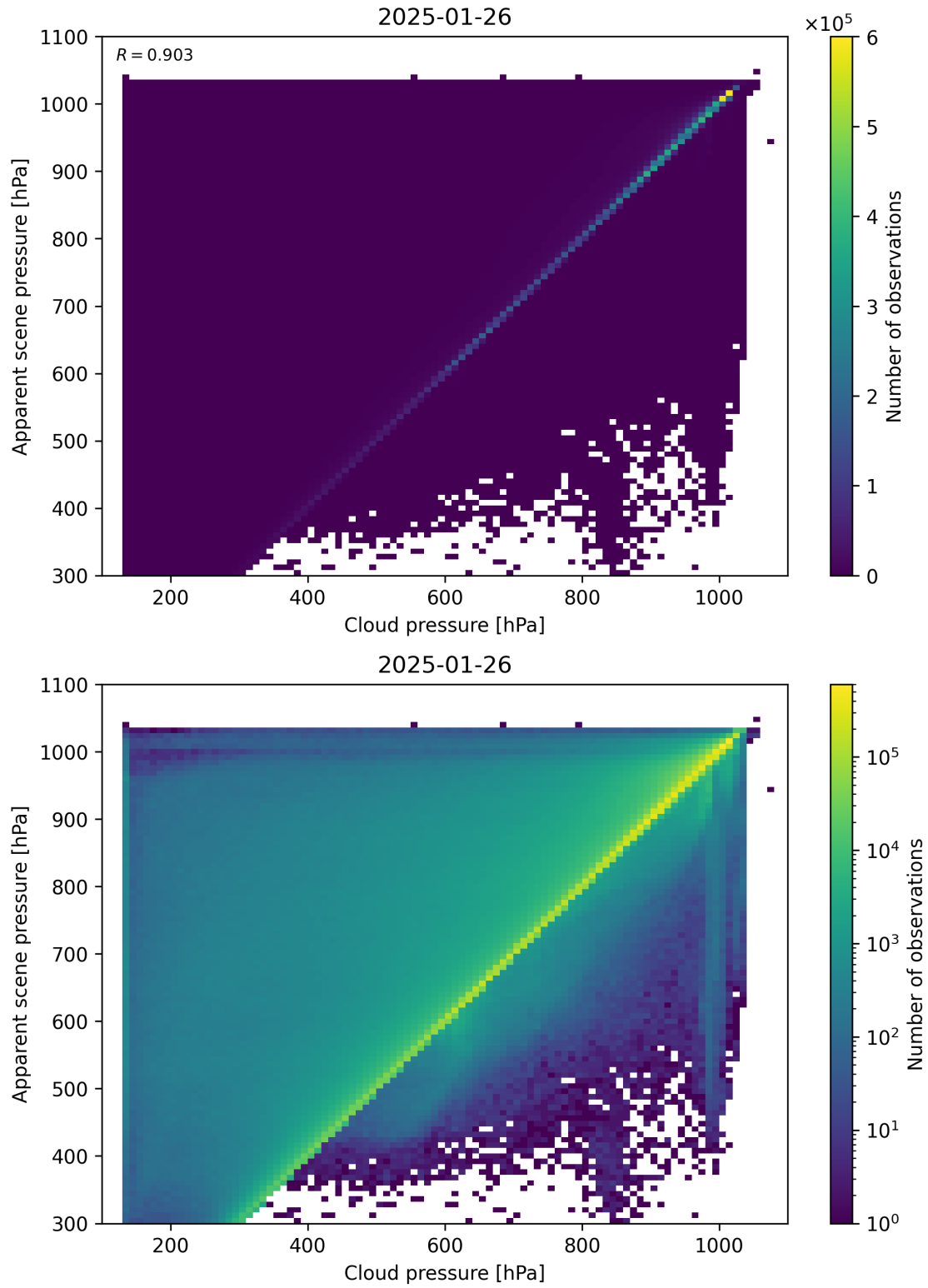
Figure 77: Scatter density plot of “Cloud pressure” against “Apparent scene pressure” for 2025-01-25 to 2025-01-27.
