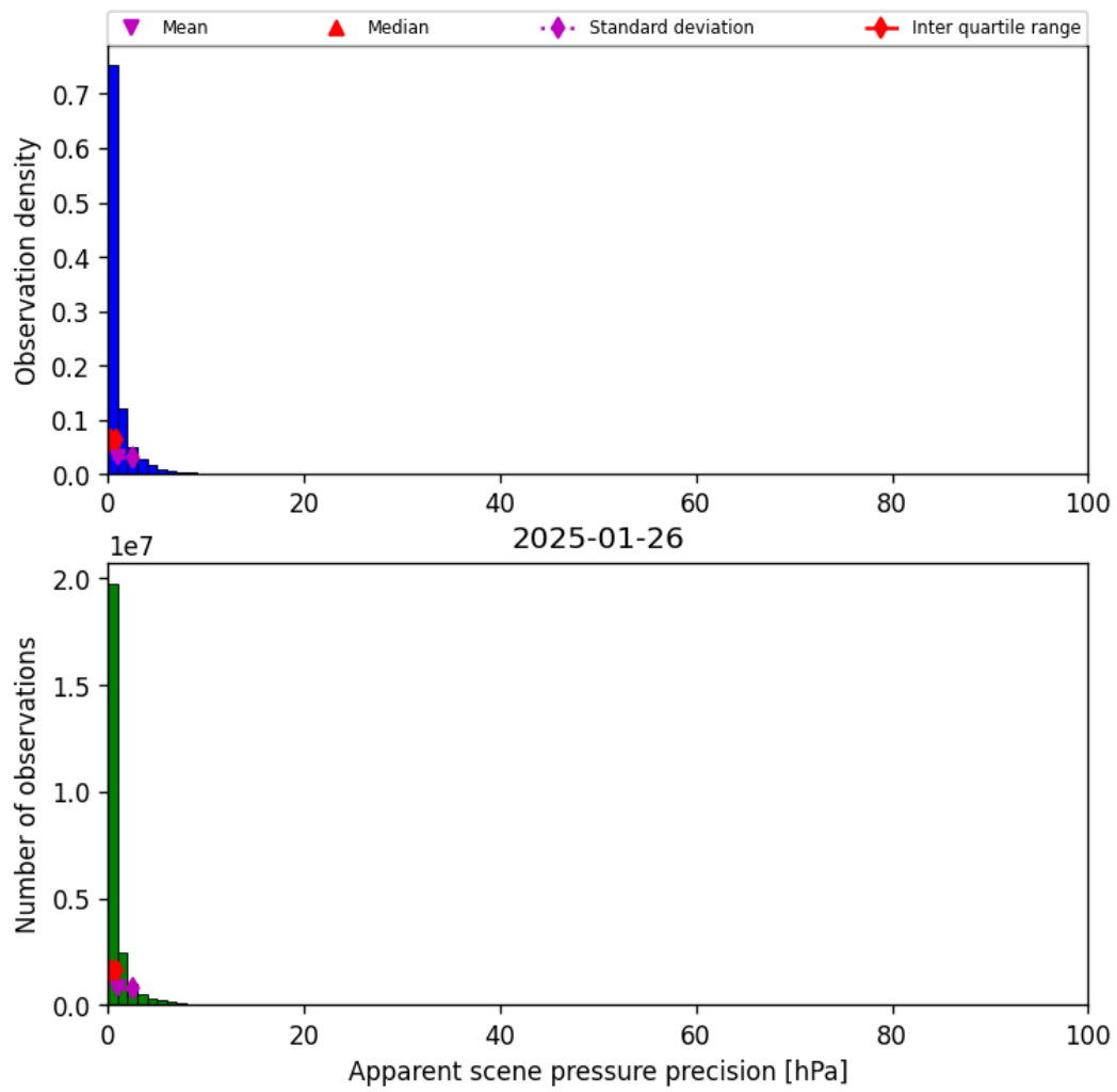
Figure 37: Histogram of “Apparent scene pressure precision” for 2025-01-25 to 2025-01-27
