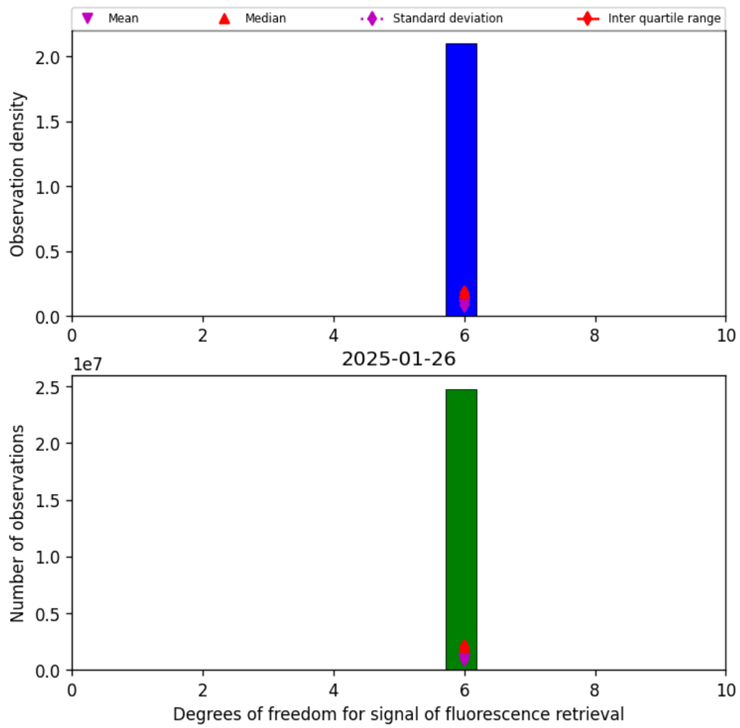
Figure 43: Histogram of “Degrees of freedom for signal of fluorescence retrieval” for 2025-01-25 to 2025-01-27
