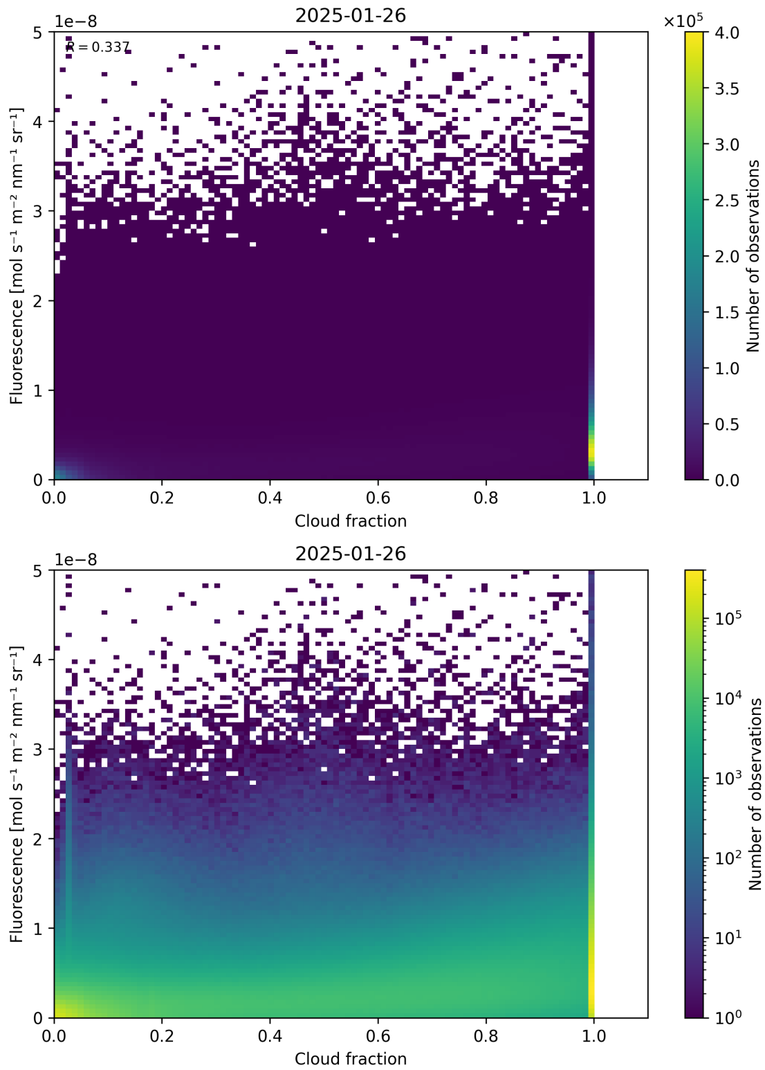
Figure 72: Scatter density plot of “Cloud fraction” against “Fluorescence” for 2025-01-25 to 2025-01-27.
