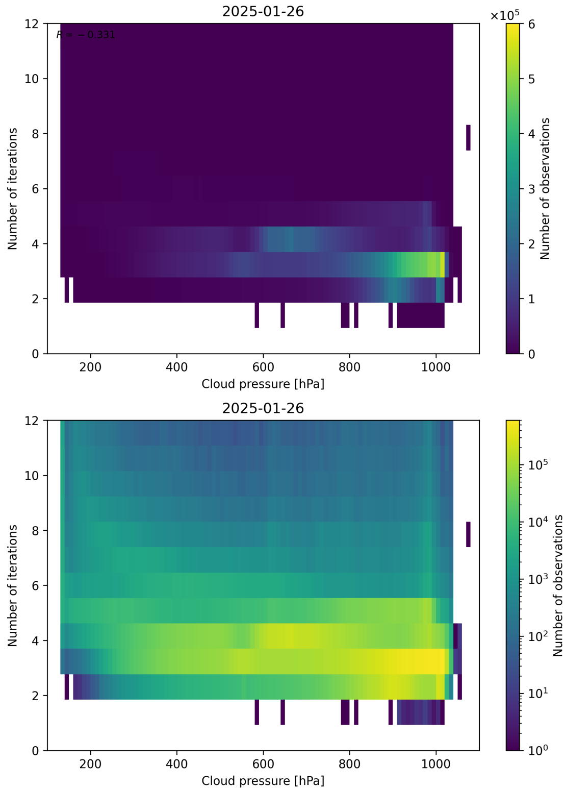
Figure 81: Scatter density plot of “Cloud pressure” against “Number of iterations” for 2025-01-25 to 2025-01-27.
