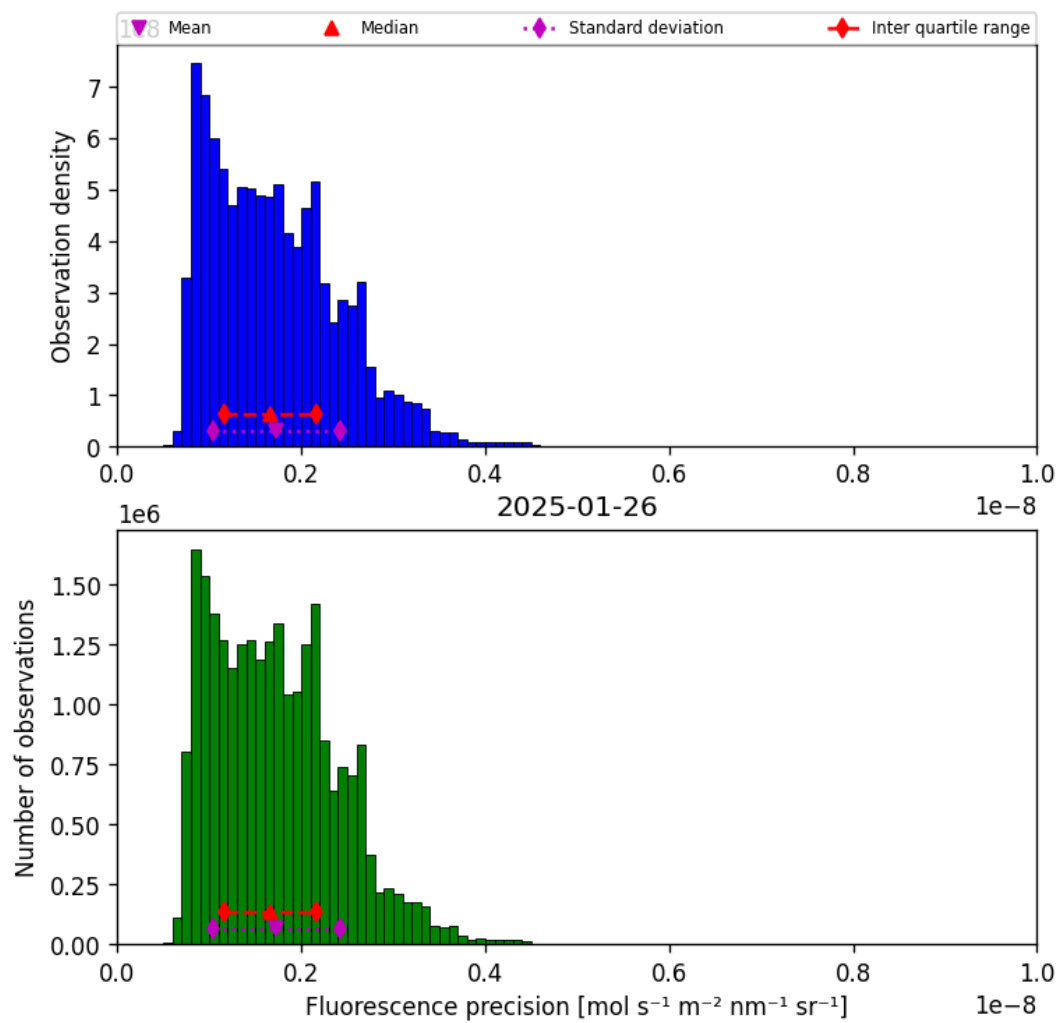
Figure 41: Histogram of “Fluorescence precision” for 2025-01-25 to 2025-01-27
