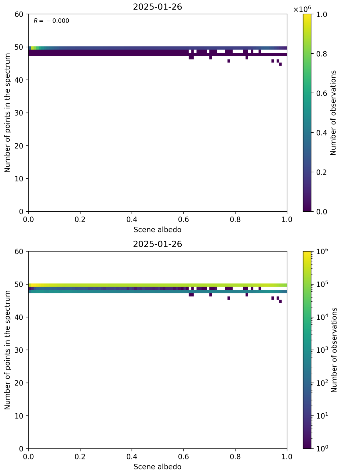
Figure 106: Scatter density plot of “Scene albedo” against “Number of points in the spectrum” for 2025-01-25 to 2025-01-27.
