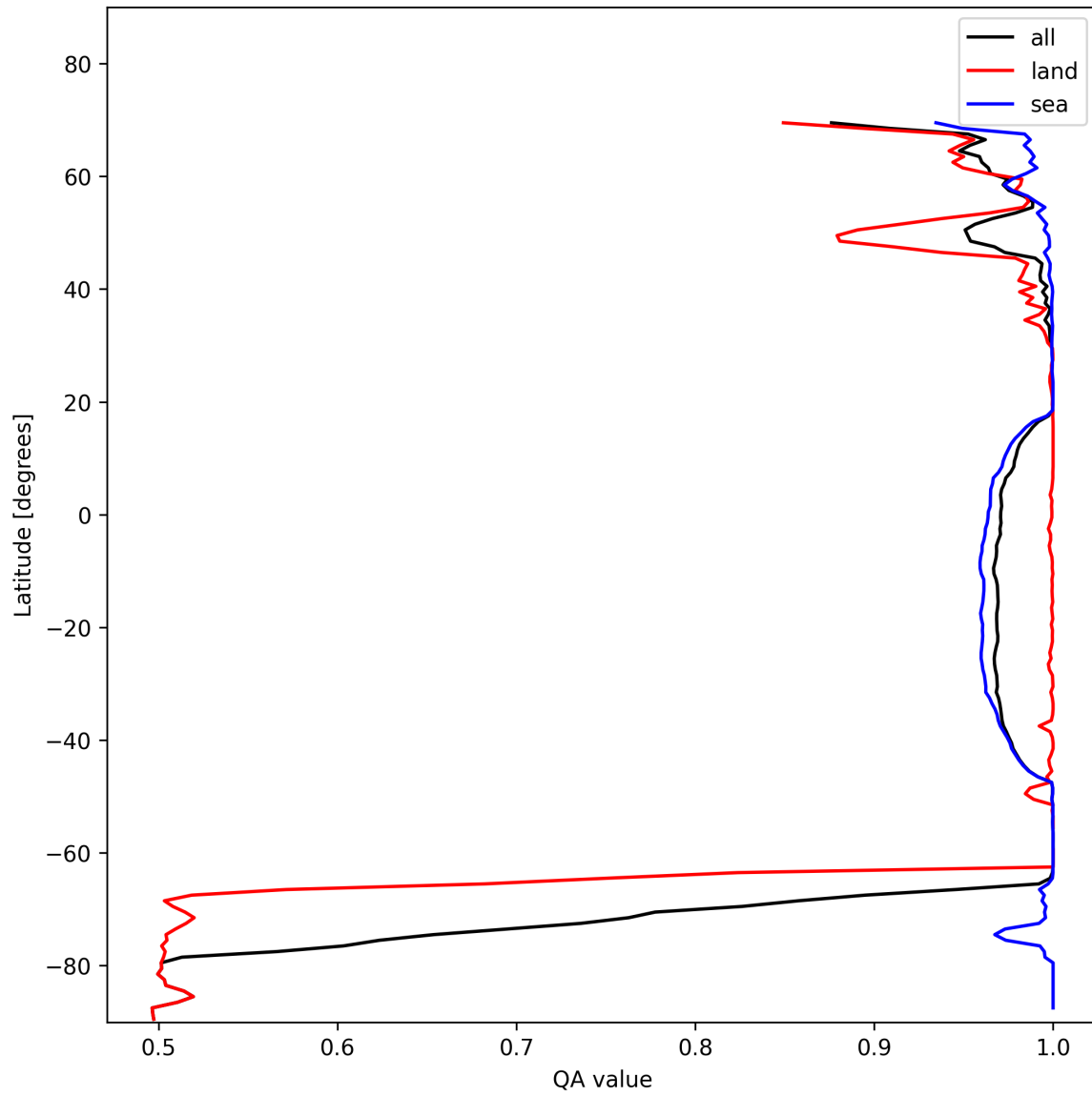
Figure 12: Zonal average of “QA value” for 2025-01-25 to 2025-01-27.
