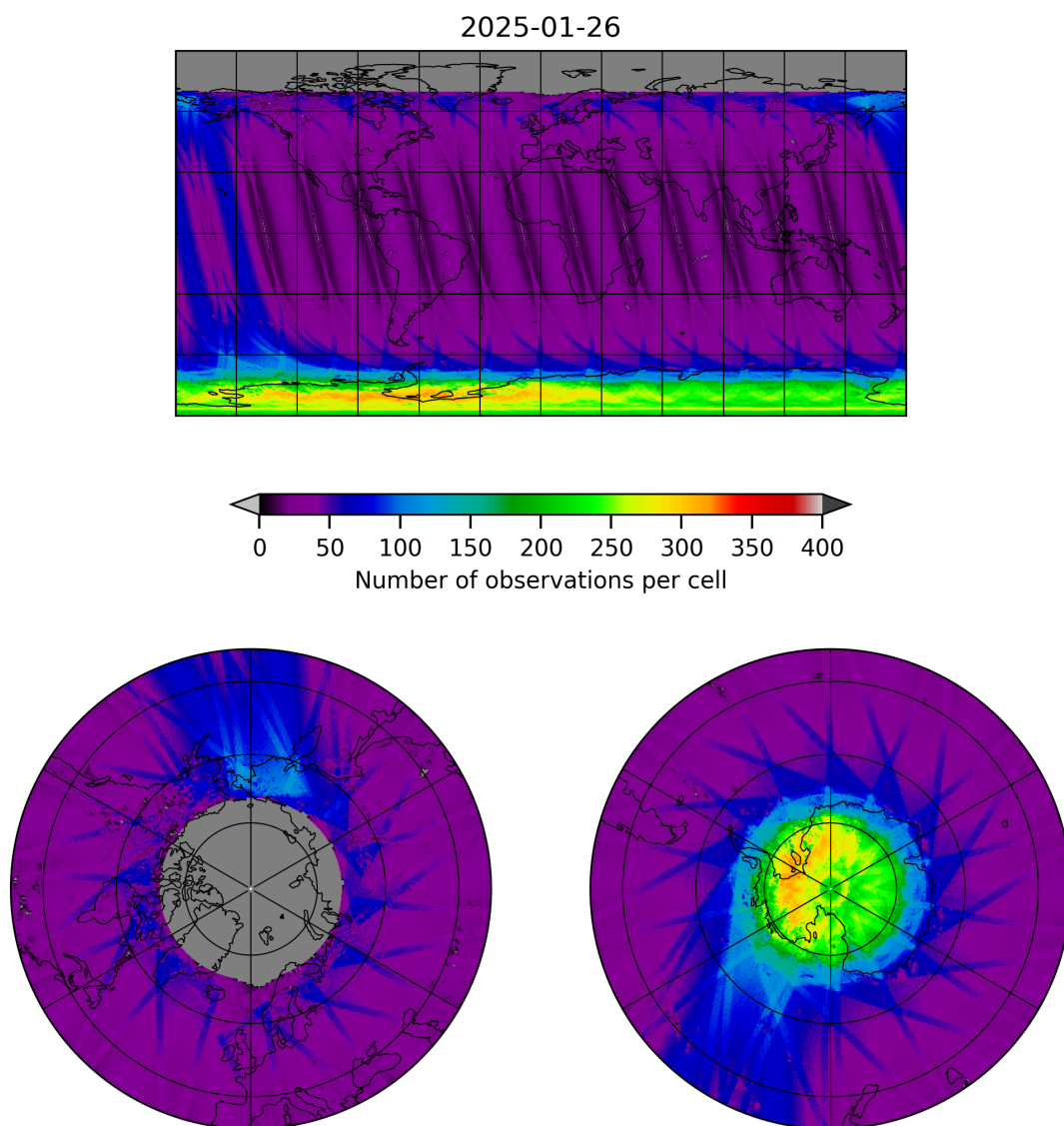
Figure 11: Map of the number of observations for 2025-01-25 to 2025-01-27
