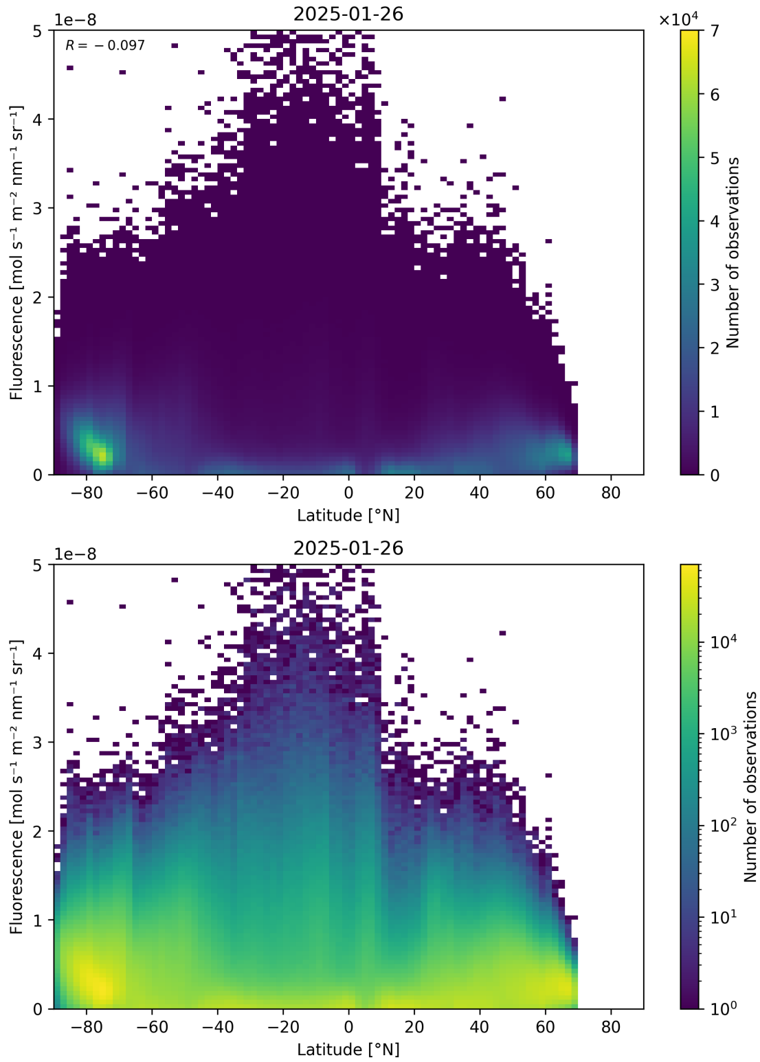
Figure 92: Scatter density plot of “Latitude” against “Fluorescence” for 2025-01-25 to 2025-01-27.
