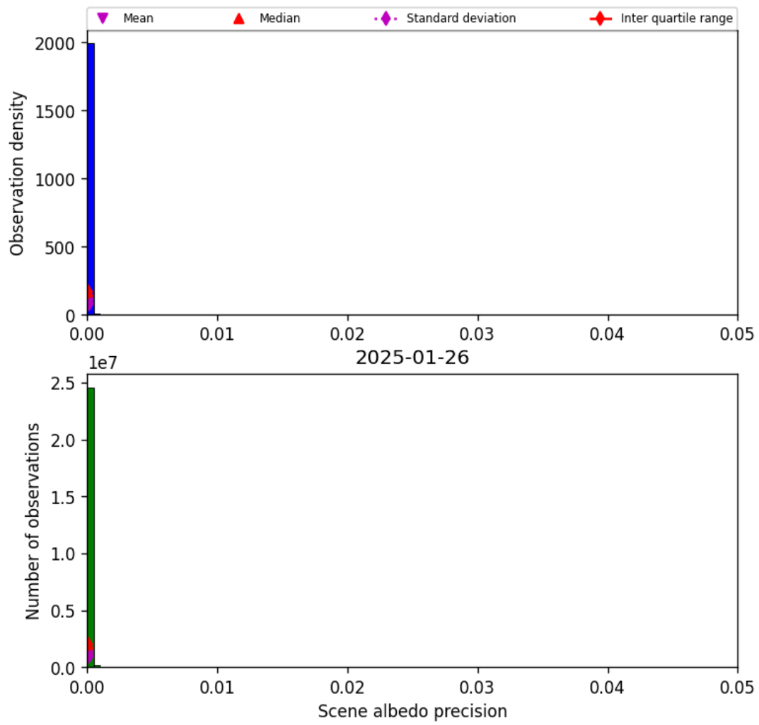
Figure 35: Histogram of “Scene albedo precision” for 2025-01-25 to 2025-01-27
