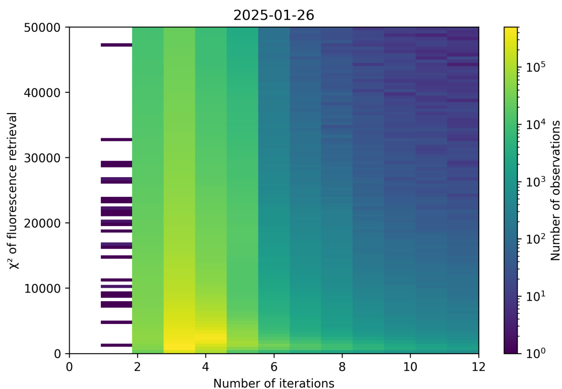
Figure 97: Scatter density plot of “Number of iterations” against “ \chi^2 of fluorescence retrieval” for 2025-01-25 to 2025-01-27.
