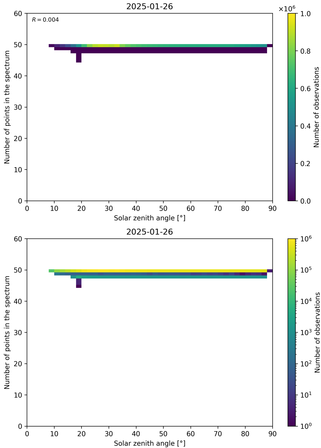
Figure 115: Scatter density plot of “Solar zenith angle” against “Number of points in the spectrum” for 2025-01-25 to 2025-01-27.
