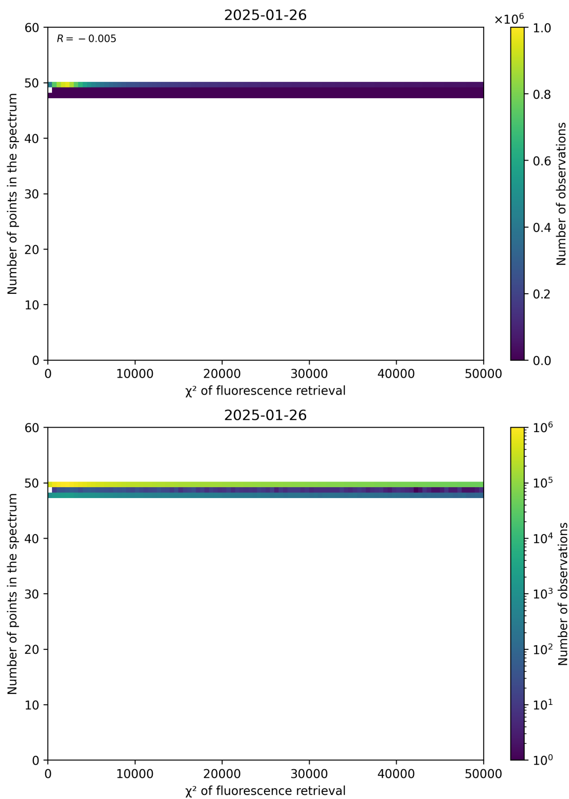
Figure 68: Scatter density plot of " \chi^2 of fluorescence retrieval" against "Number of points in the spectrum" for 2025-01-25 to 2025-01-27.
