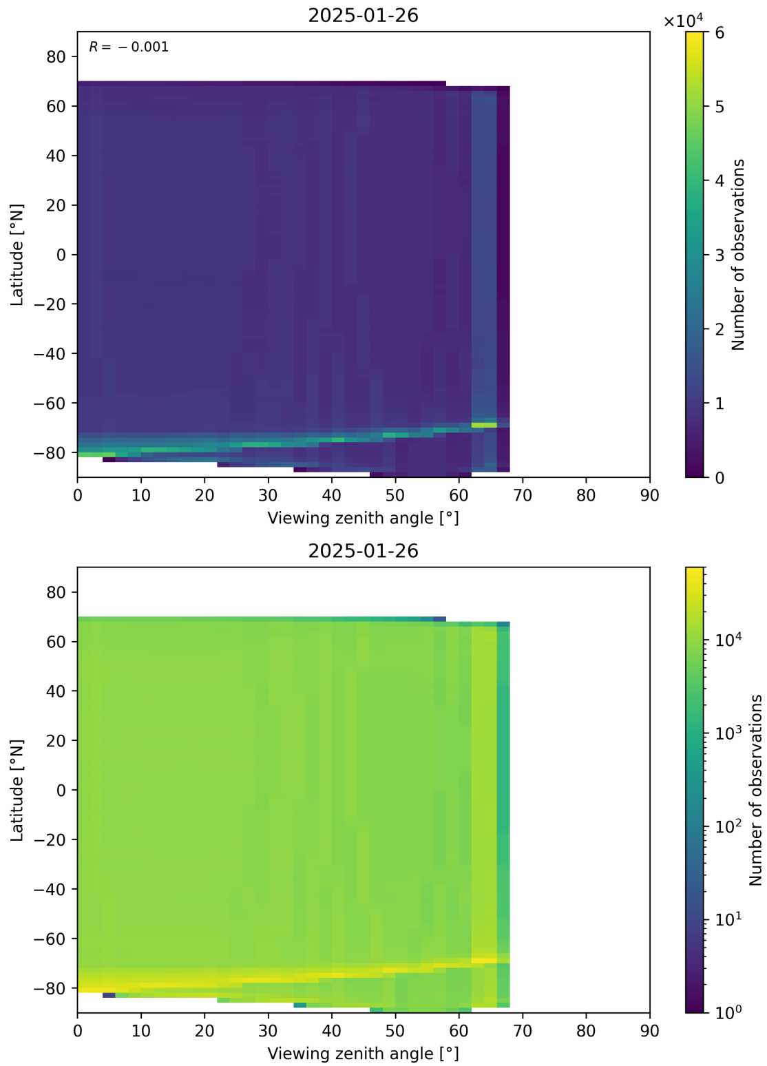
Figure 123: Scatter density plot of “Viewing zenith angle” against “Latitude” for 2025-01-25 to 2025-01-27.
