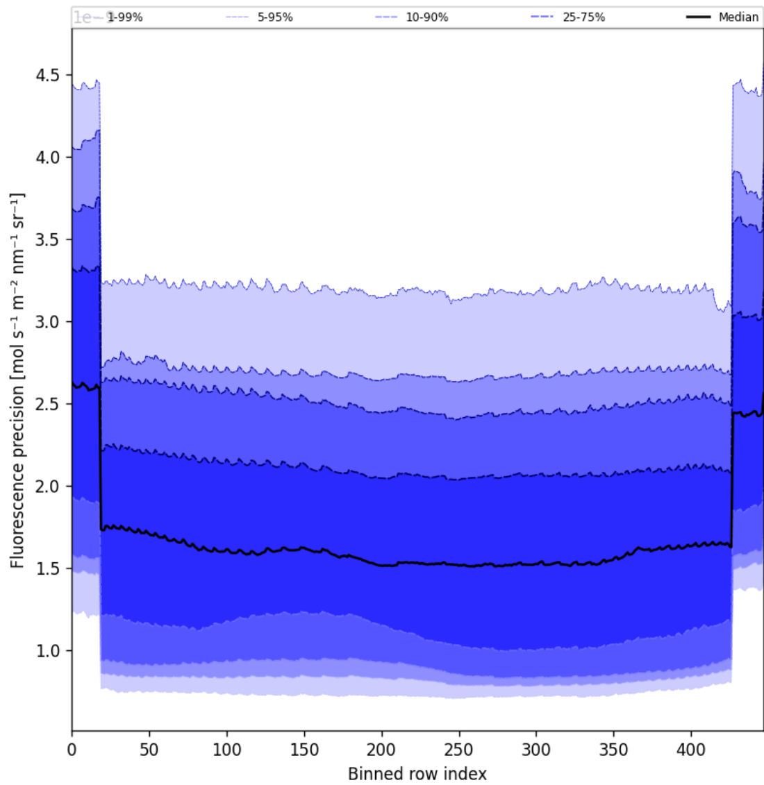
Figure 58: Along track statistics of “Fluorescence precision” for 2025-01-25 to 2025-01-27
