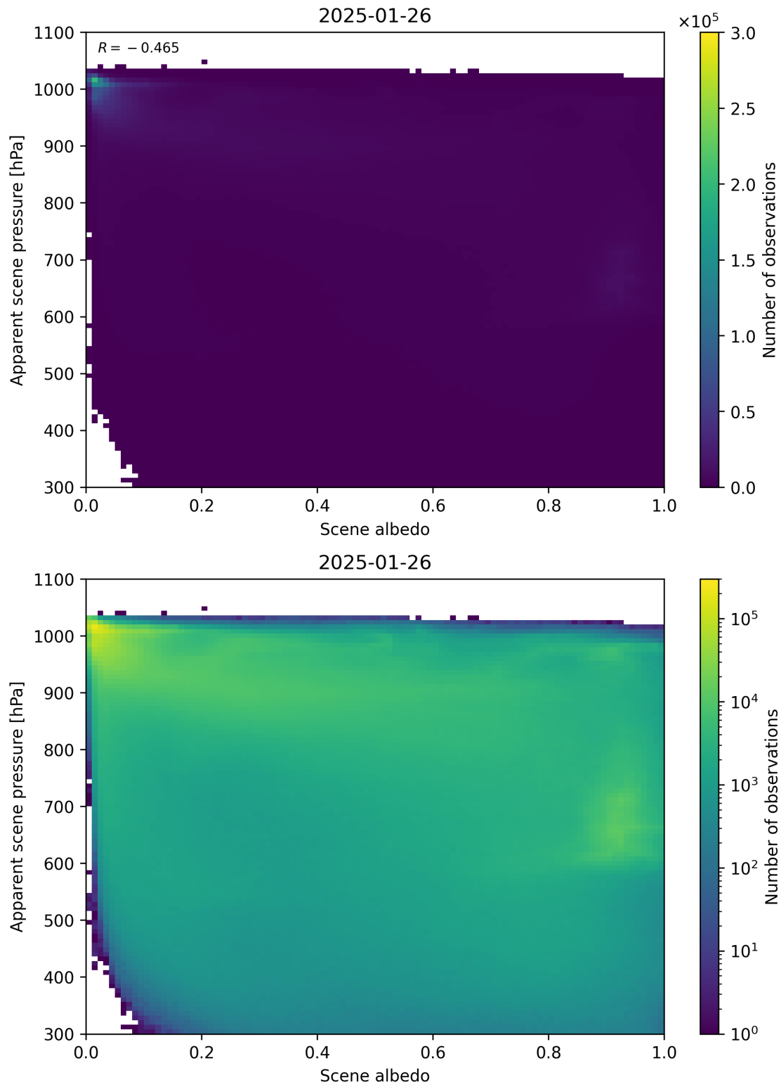
Figure 102: Scatter density plot of “Scene albedo” against “Apparent scene pressure” for 2025-01-25 to 2025-01-27.
