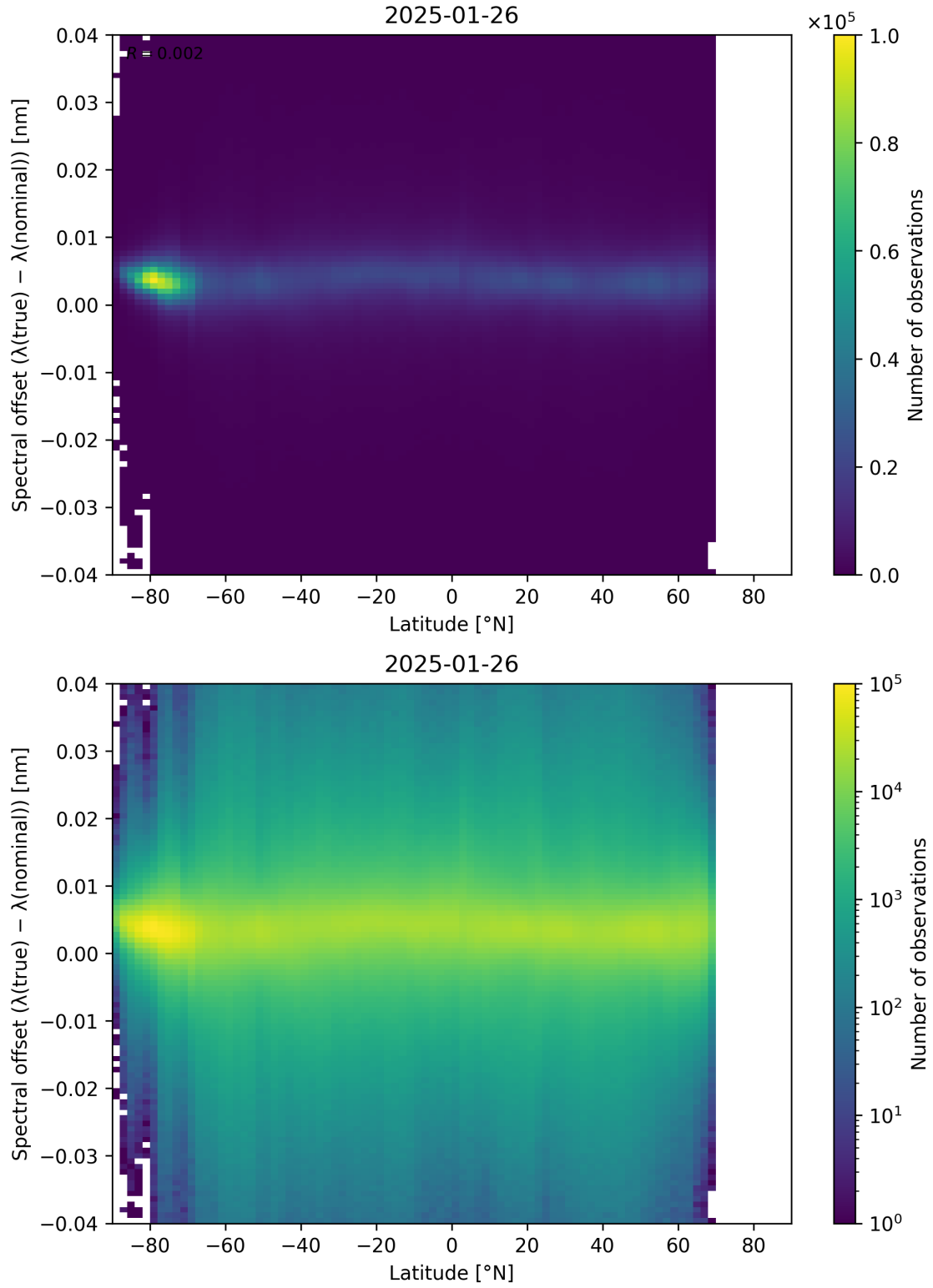
Figure 96: Scatter density plot of “Latitude” against “Spectral offset ( \lambda_{\text{true}} - \lambda_{\text{nominal}} )” for 2025-01-25 to 2025-01-27.
