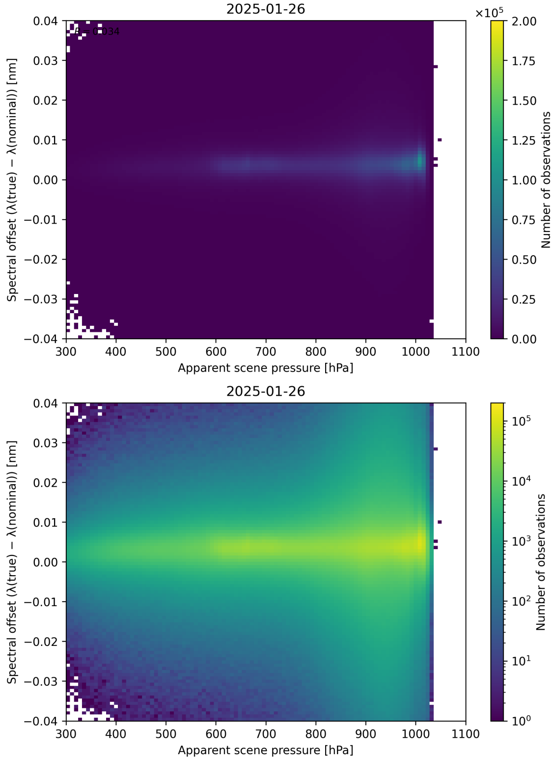
Figure 67: Scatter density plot of “Apparent scene pressure” against “Spectral offset ( \lambda_{\text{true}} - \lambda_{\text{nominal}} )” for 2025-01-25 to 2025-01-27.
