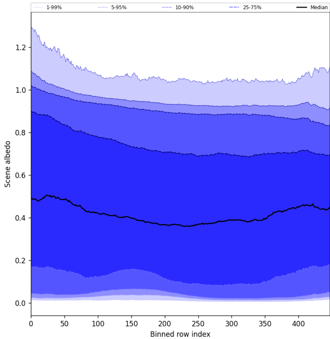
Figure 51: Along track statistics of “Scene albedo” for 2025-01-25 to 2025-01-27
