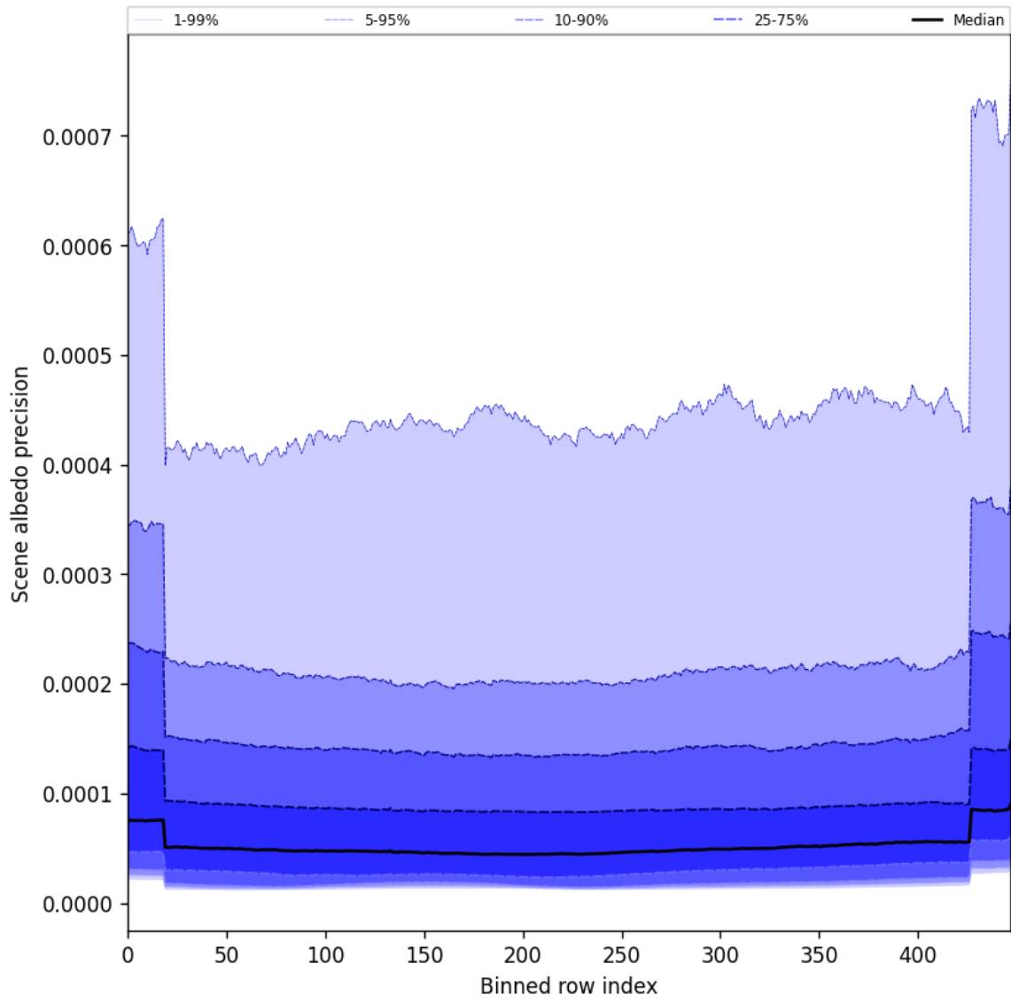
Figure 52: Along track statistics of “Scene albedo precision” for 2025-01-25 to 2025-01-27
