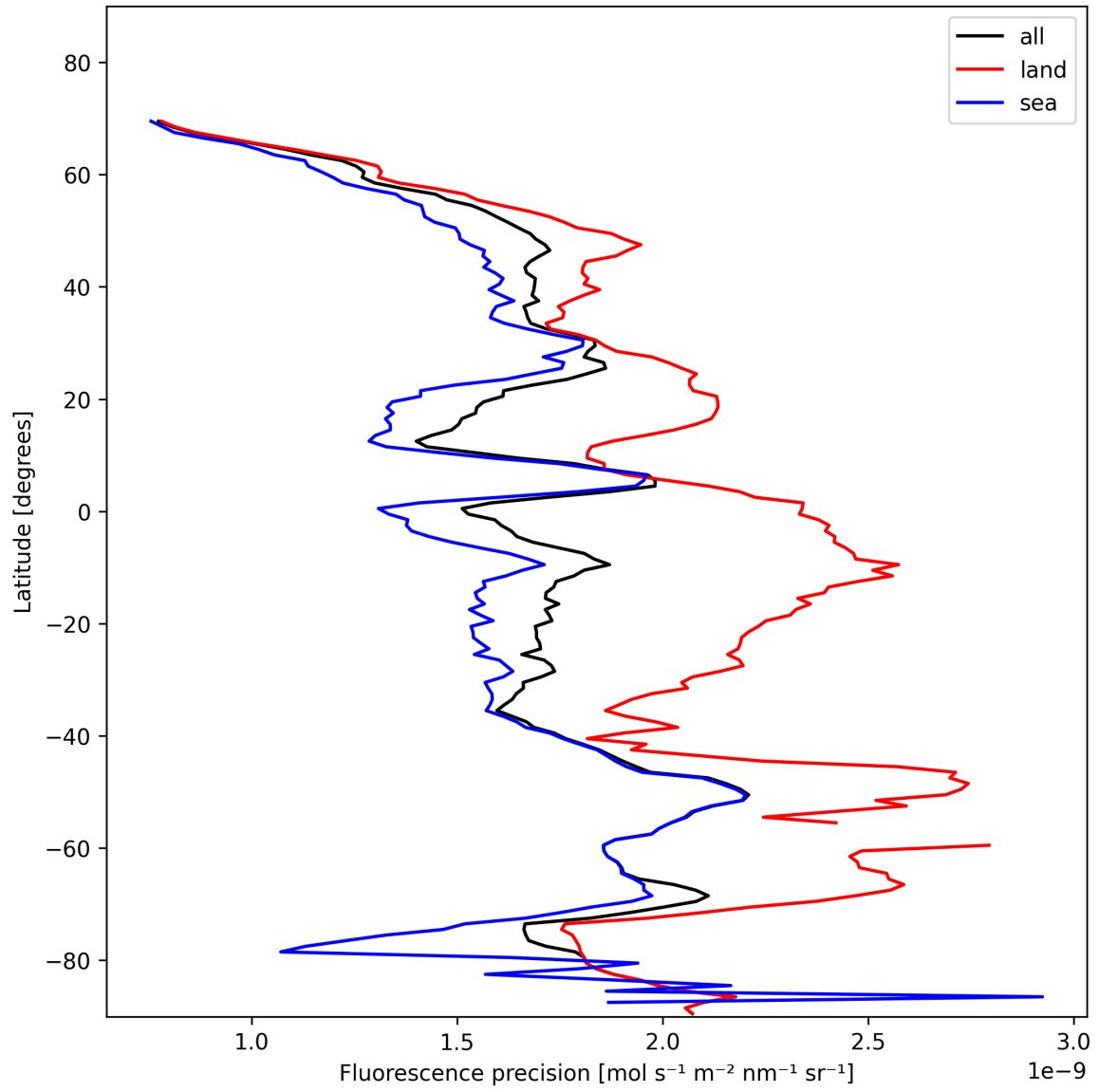
Figure 24: Zonal average of “Fluorescence precision” for 2025-01-25 to 2025-01-27.
