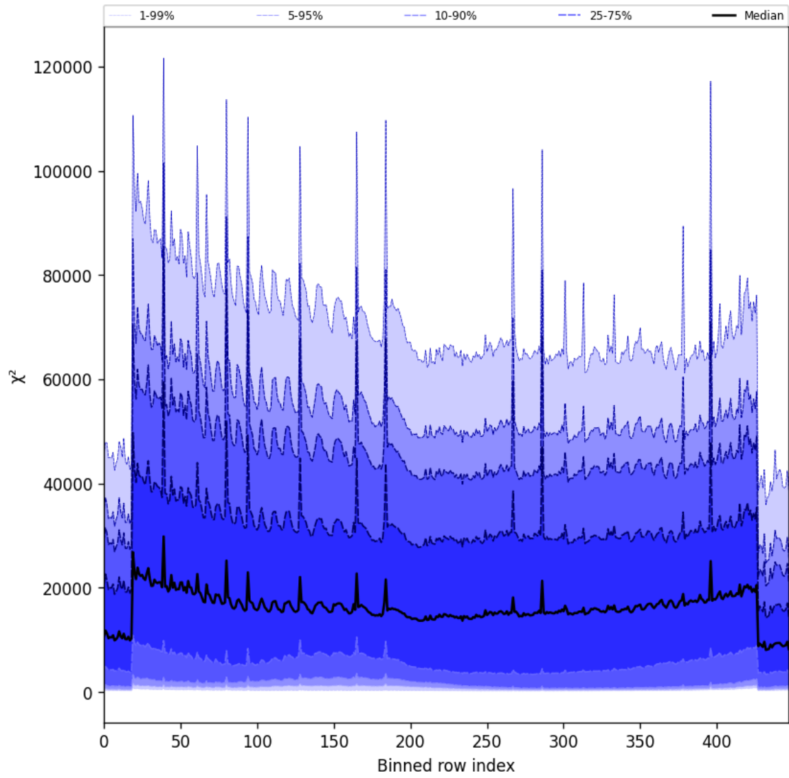
Figure 55: Along track statistics of “ \chi^2 ” for 2025-01-25 to 2025-01-27
