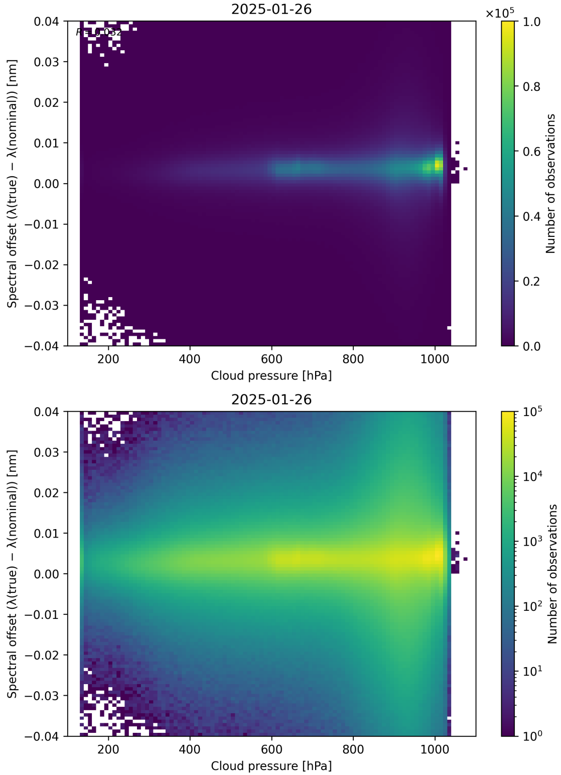
Figure 84: Scatter density plot of “Cloud pressure” against “Spectral offset ( \lambda_{\text{true}} - \lambda_{\text{nominal}} )” for 2025-01-25 to 2025-01-27.
