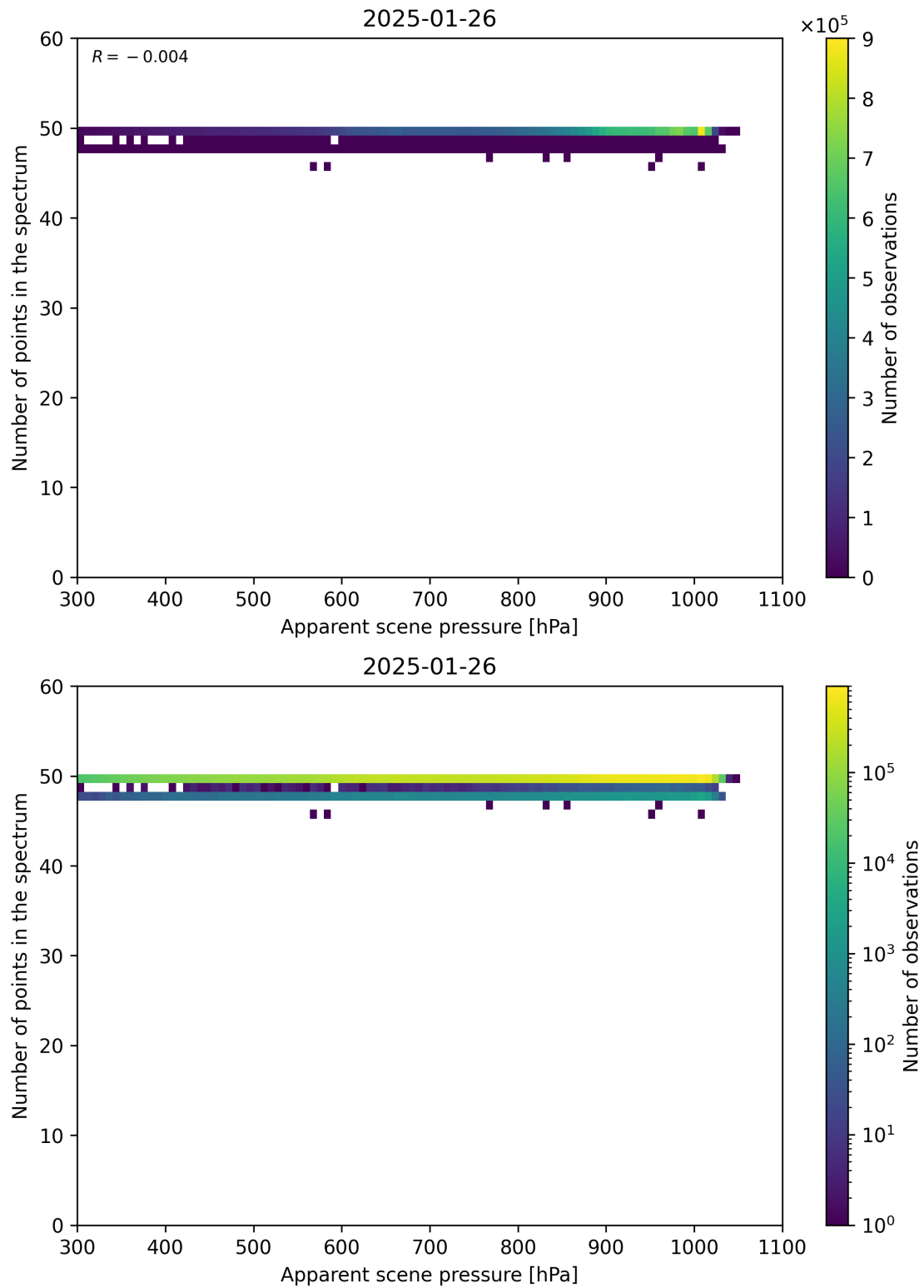
Figure 66: Scatter density plot of “Apparent scene pressure” against “Number of points in the spectrum” for 2025-01-25 to 2025-01-27.
