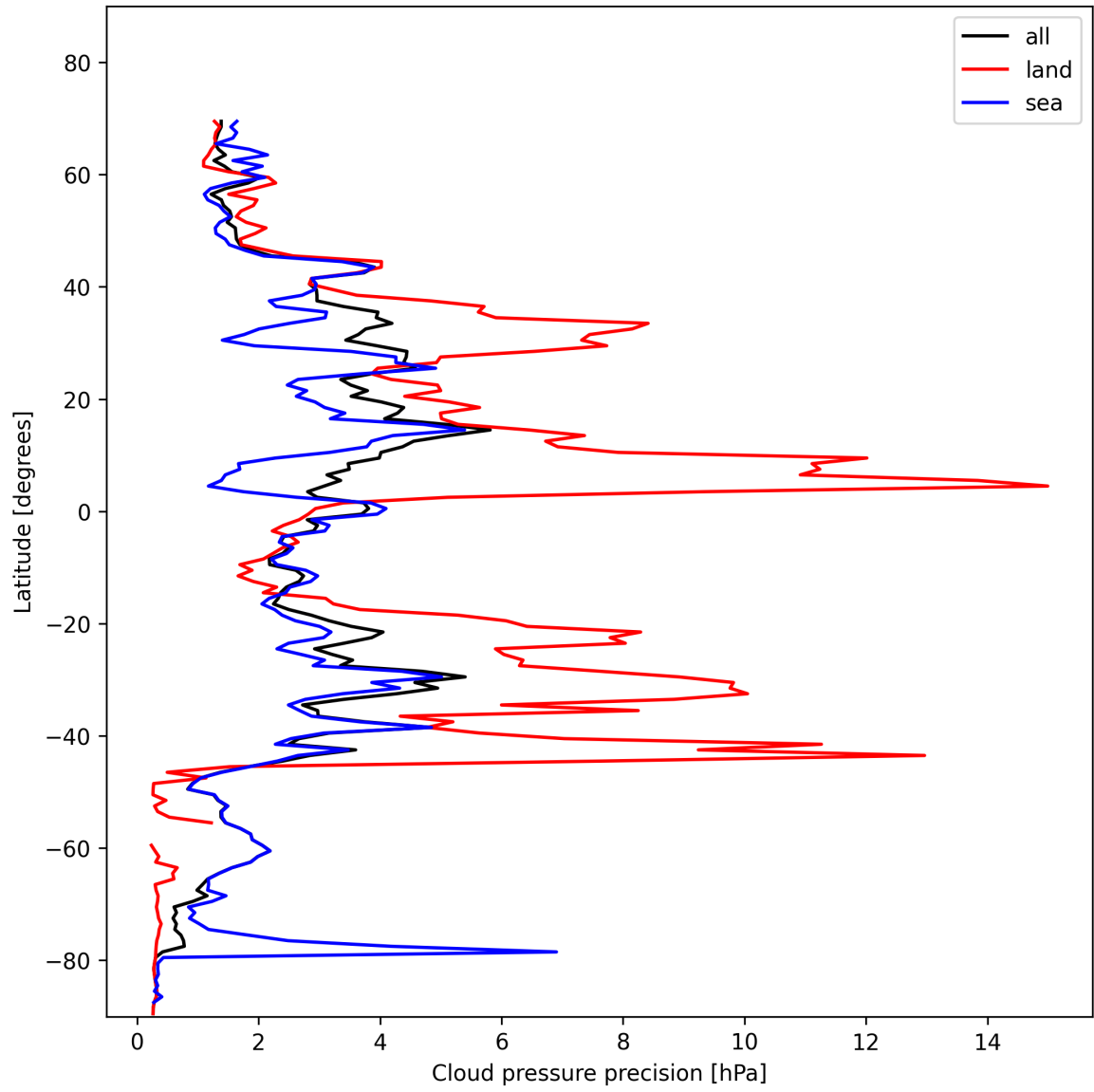
Figure 14: Zonal average of “Cloud pressure precision” for 2025-01-25 to 2025-01-27.
