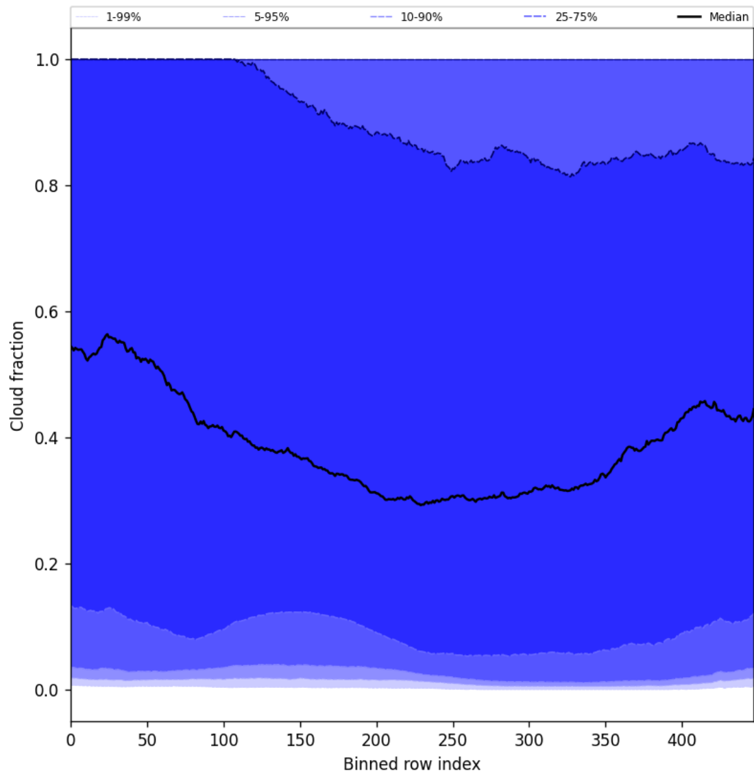
Figure 49: Along track statistics of “Cloud fraction” for 2025-01-25 to 2025-01-27
