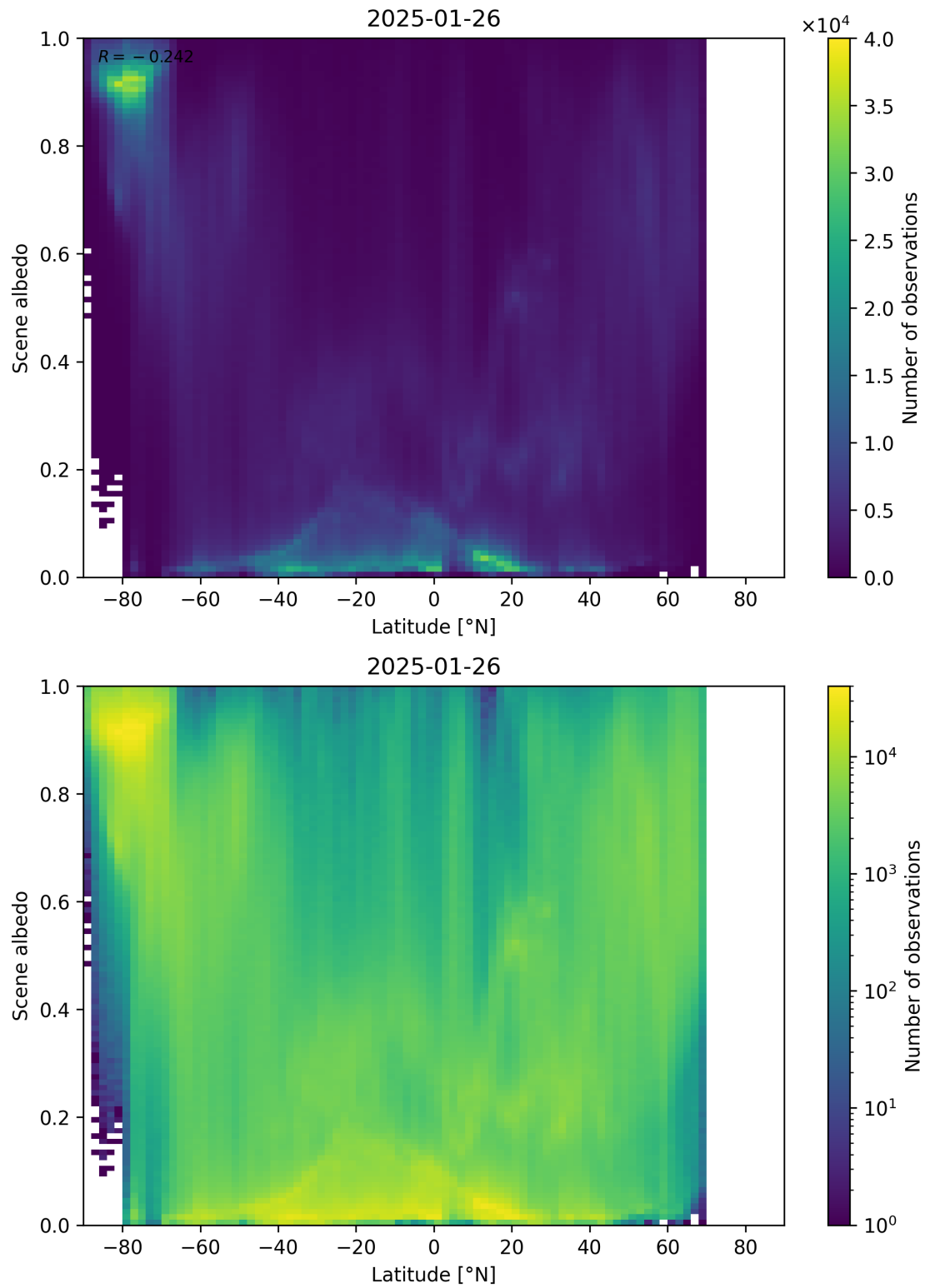
Figure 95: Scatter density plot of “Latitude” against “Scene albedo” for 2025-01-25 to 2025-01-27.
