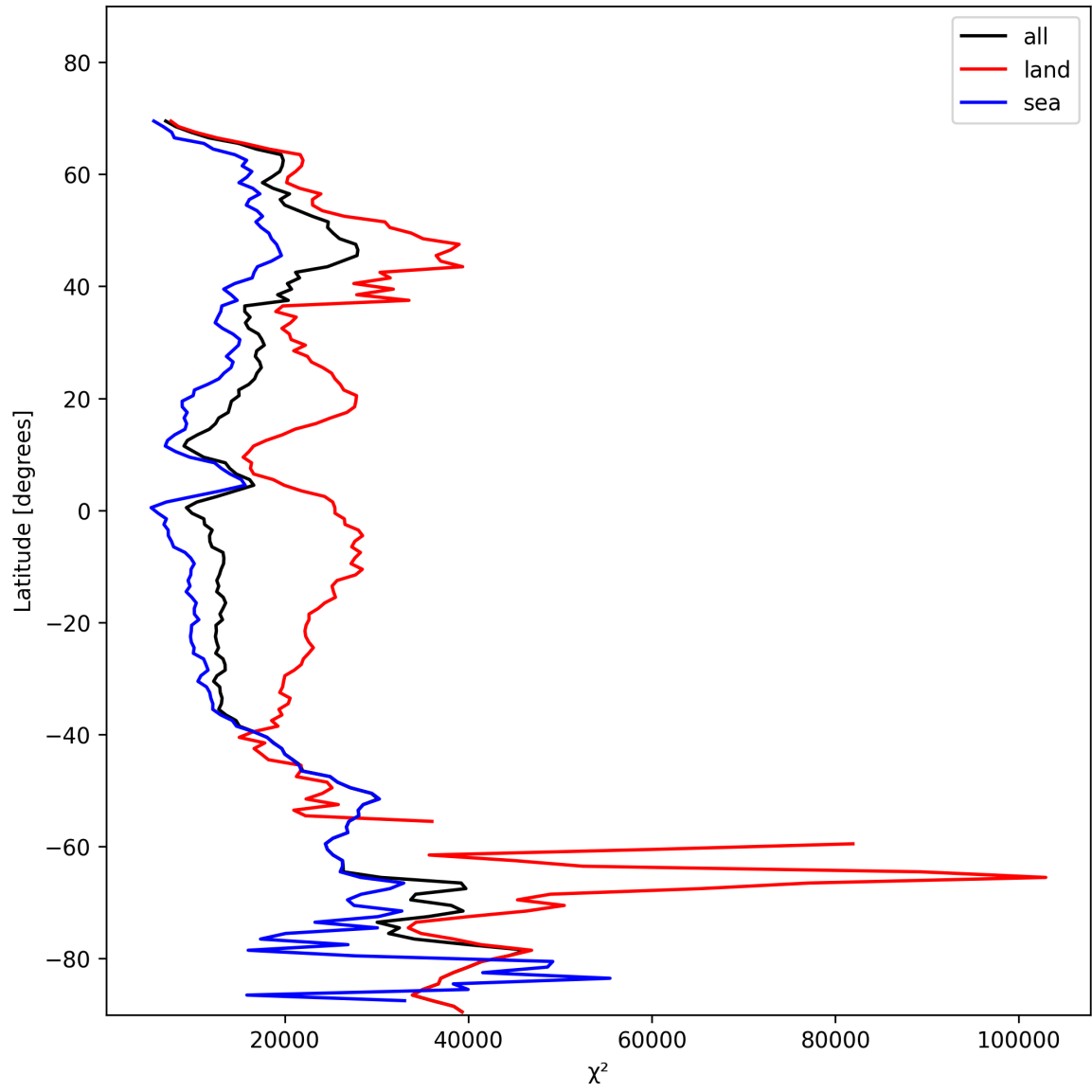
Figure 21: Zonal average of “ \chi^2 ” for 2025-01-25 to 2025-01-27.
