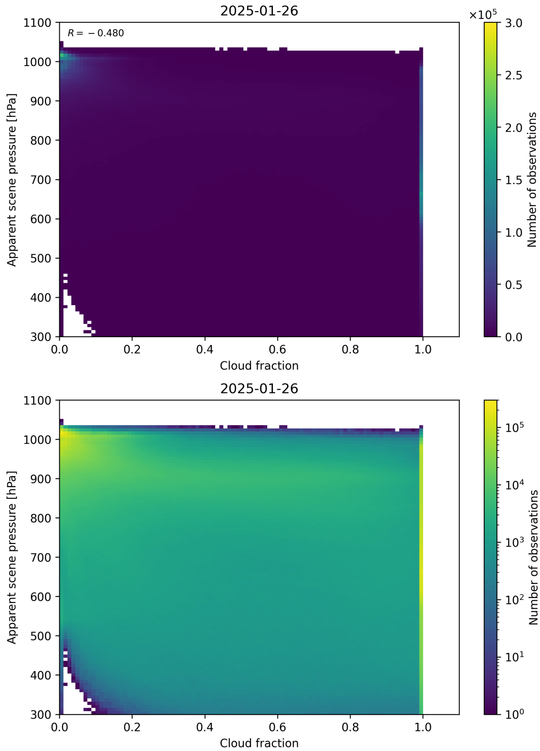
Figure 70: Scatter density plot of “Cloud fraction” against “Apparent scene pressure” for 2025-01-25 to 2025-01-27.
