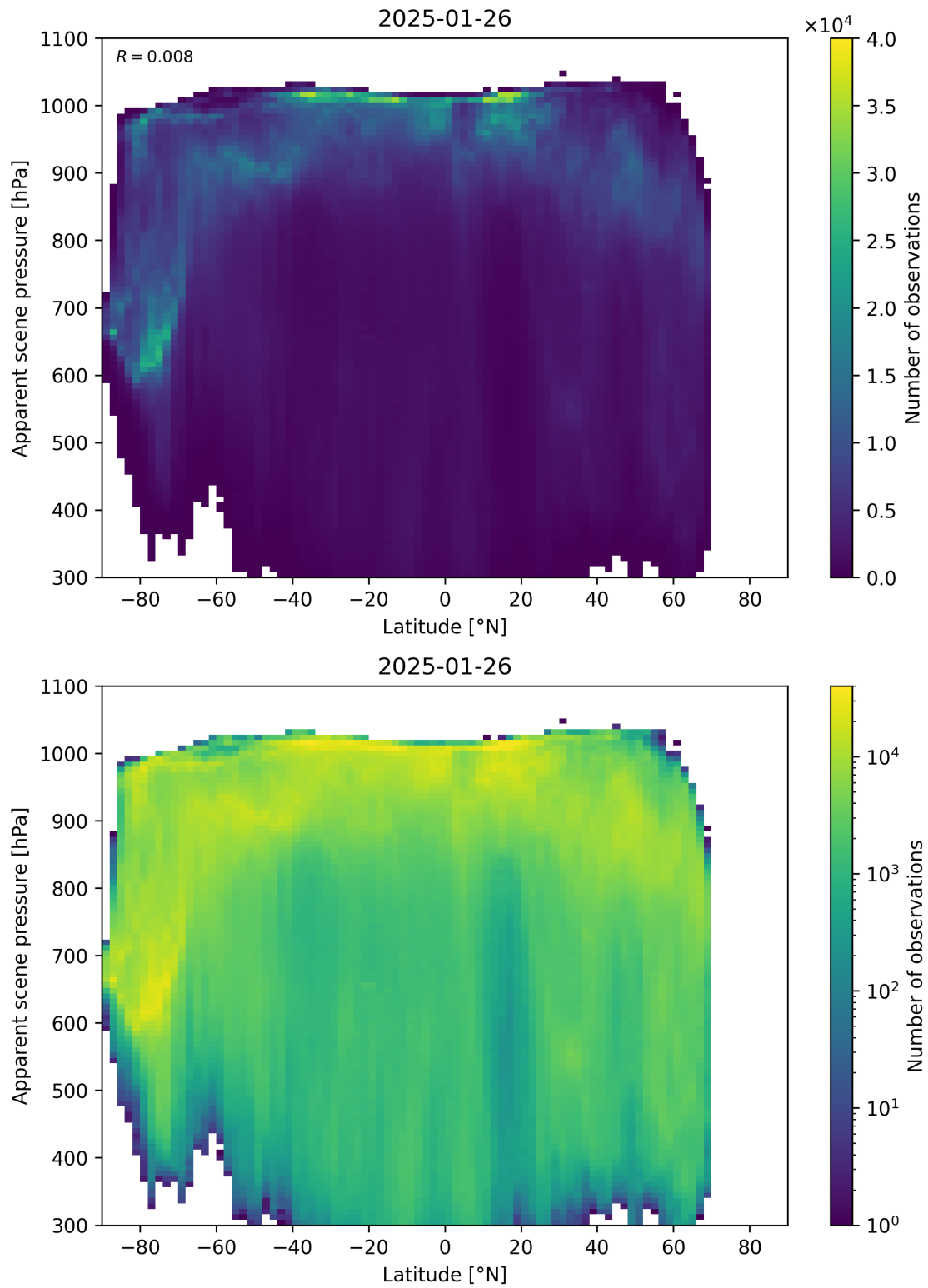
Figure 88: Scatter density plot of “Latitude” against “Apparent scene pressure” for 2025-01-25 to 2025-01-27.
