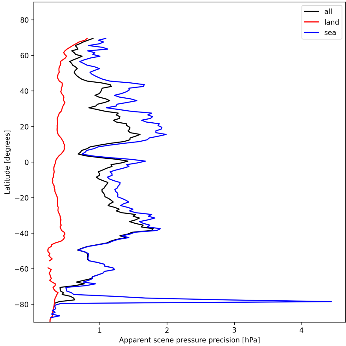
Figure 20: Zonal average of “Apparent scene pressure precision” for 2025-01-25 to 2025-01-27.
