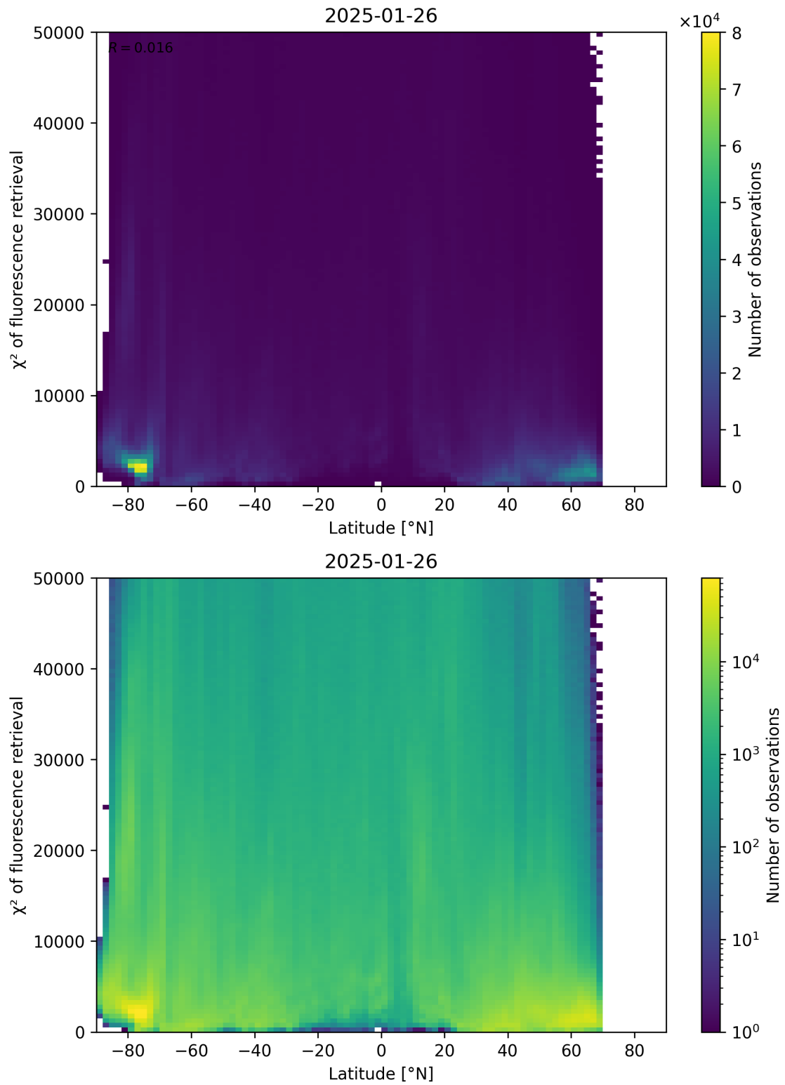
Figure 89: Scatter density plot of “Latitude” against “ \chi^2 of fluorescence retrieval” for 2025-01-25 to 2025-01-27.
