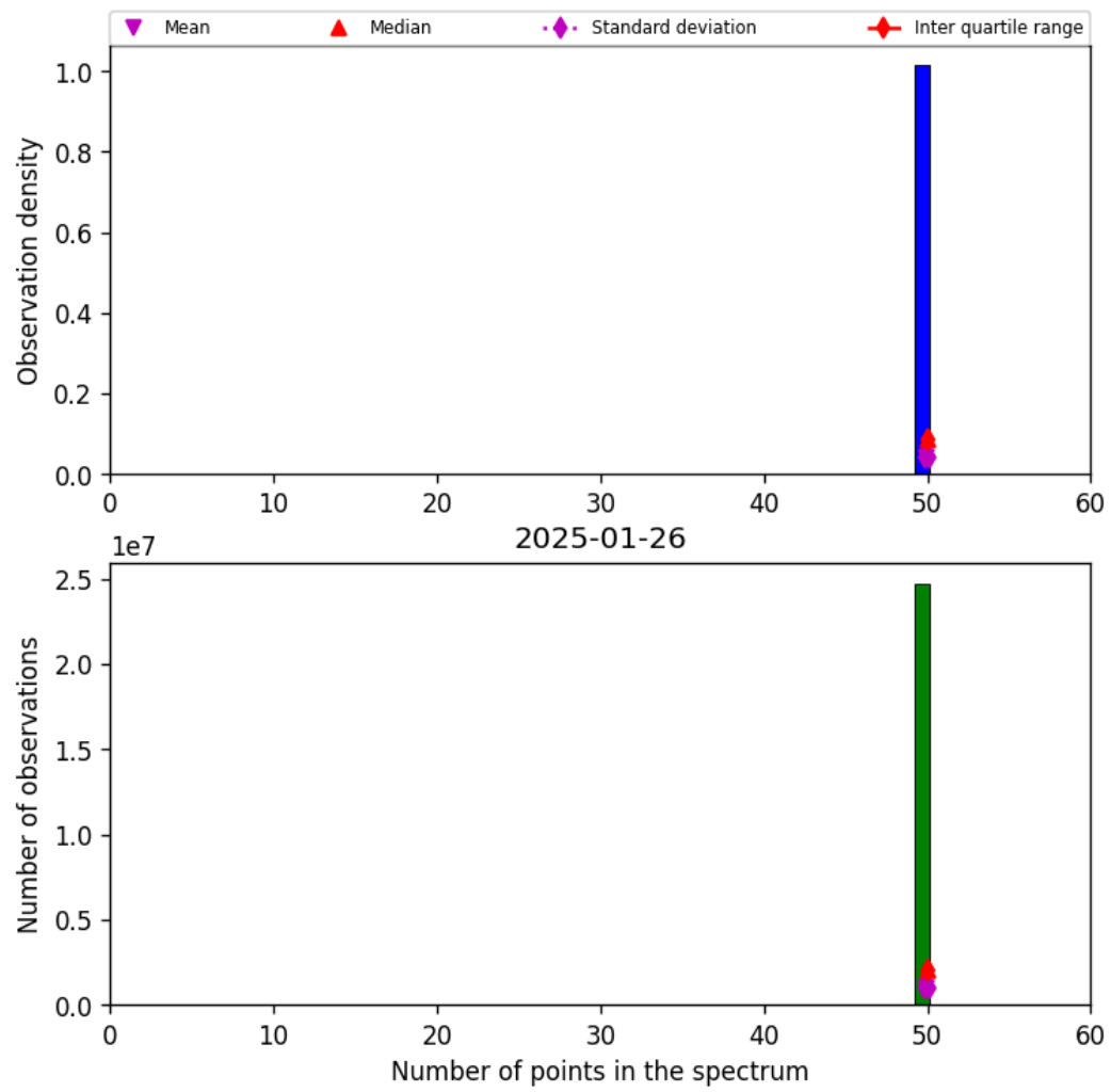
Figure 44: Histogram of “Number of points in the spectrum” for 2025-01-25 to 2025-01-27
