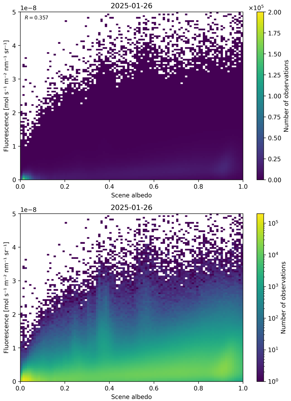
Figure 104: Scatter density plot of "Scene albedo" against "Fluorescence" for 2025-01-25 to 2025-01-27.
