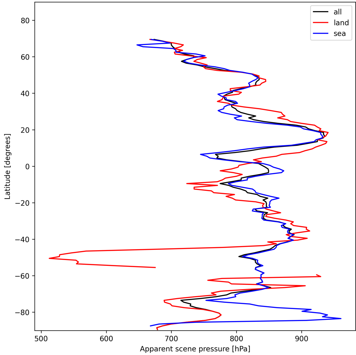
Figure 19: Zonal average of “Apparent scene pressure” for 2025-01-25 to 2025-01-27.
