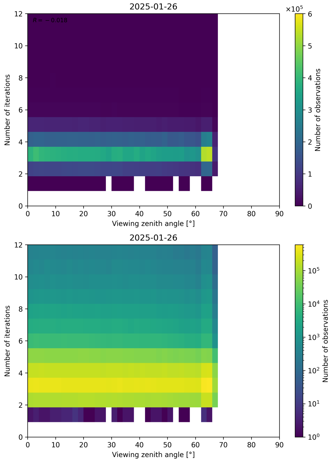
Figure 124: Scatter density plot of “Viewing zenith angle” against “Number of iterations” for 2025-01-25 to 2025-01-27.
