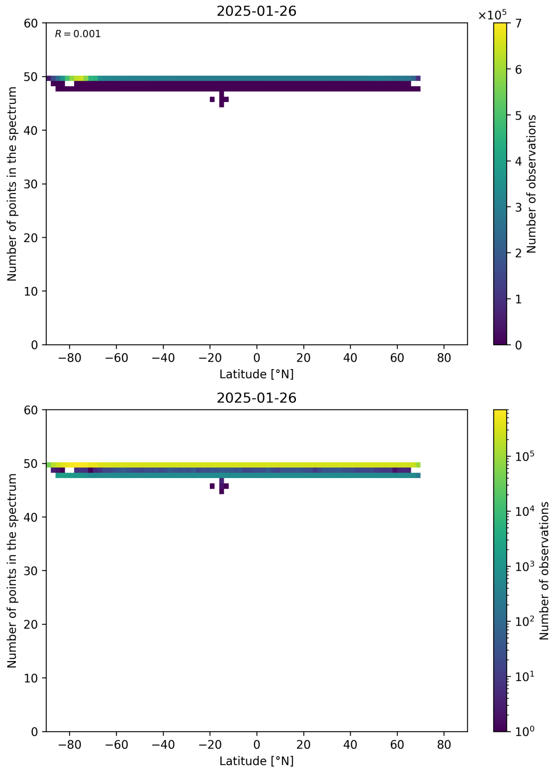
Figure 94: Scatter density plot of “Latitude” against “Number of points in the spectrum” for 2025-01-25 to 2025-01-27.
