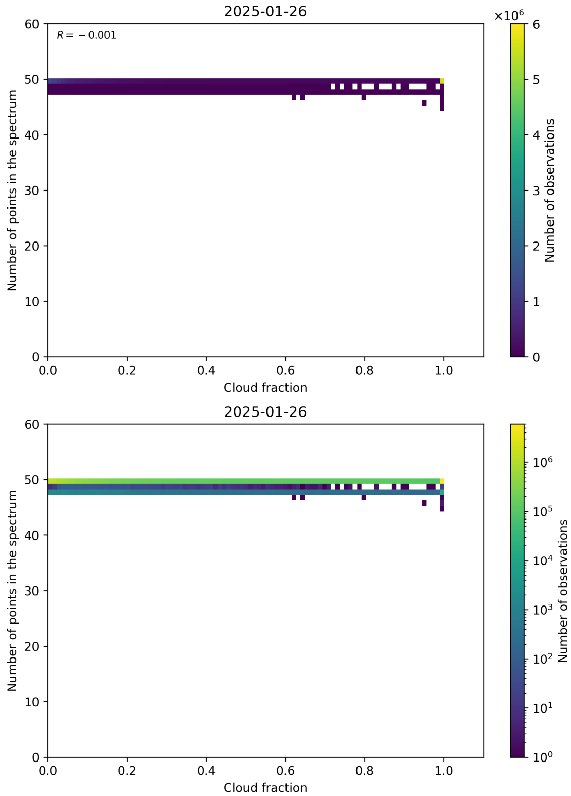
Figure 74: Scatter density plot of “Cloud fraction” against “Number of points in the spectrum” for 2025-01-25 to 2025-01-27.
