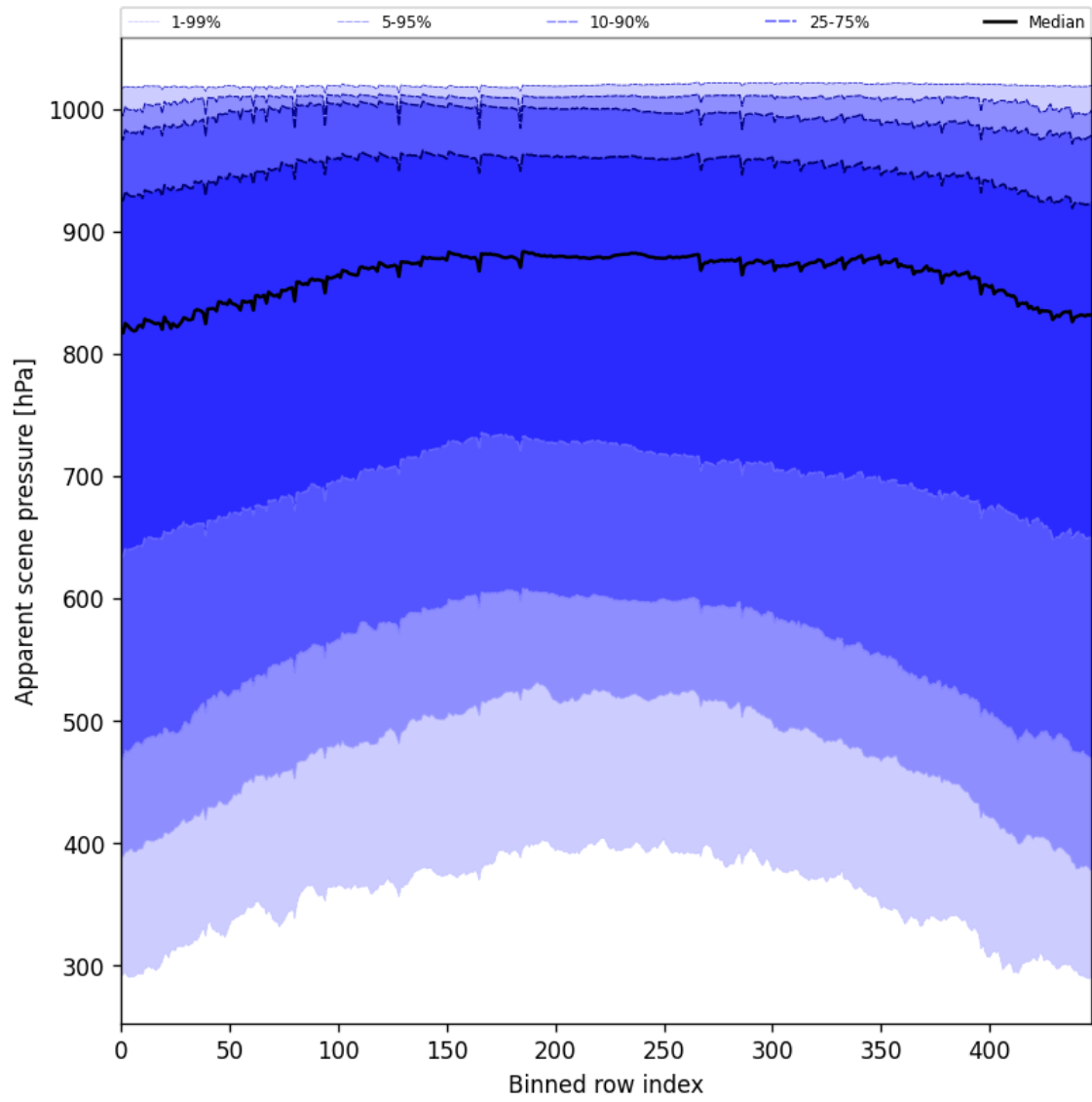
Figure 53: Along track statistics of “Apparent scene pressure” for 2025-01-25 to 2025-01-27
