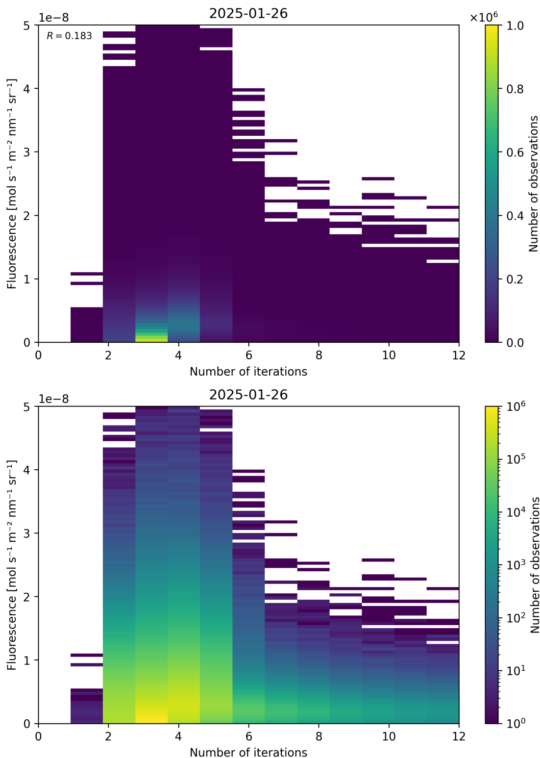
Figure 98: Scatter density plot of “Number of iterations” against “Fluorescence” for 2025-01-25 to 2025-01-27.
