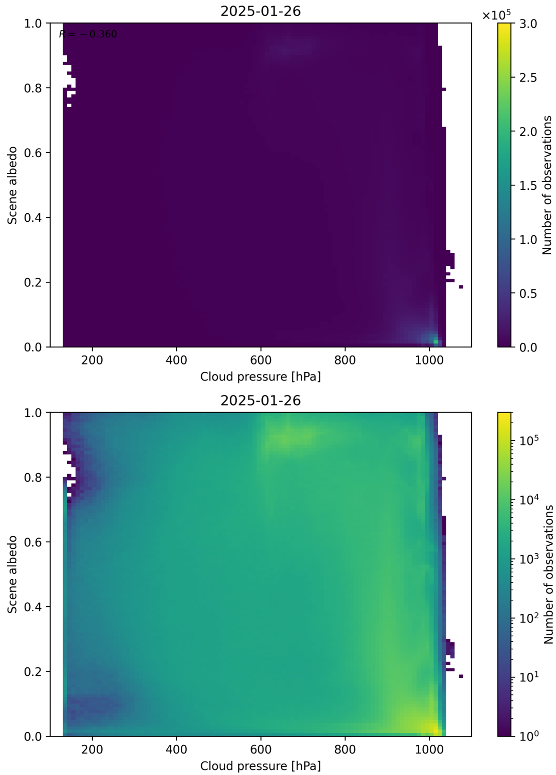
Figure 83: Scatter density plot of “Cloud pressure” against “Scene albedo” for 2025-01-25 to 2025-01-27.
