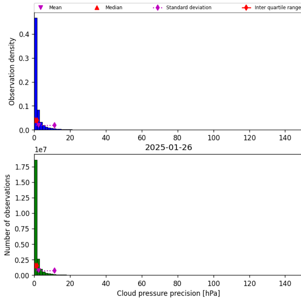
Figure 31: Histogram of “Cloud pressure precision” for 2025-01-25 to 2025-01-27
