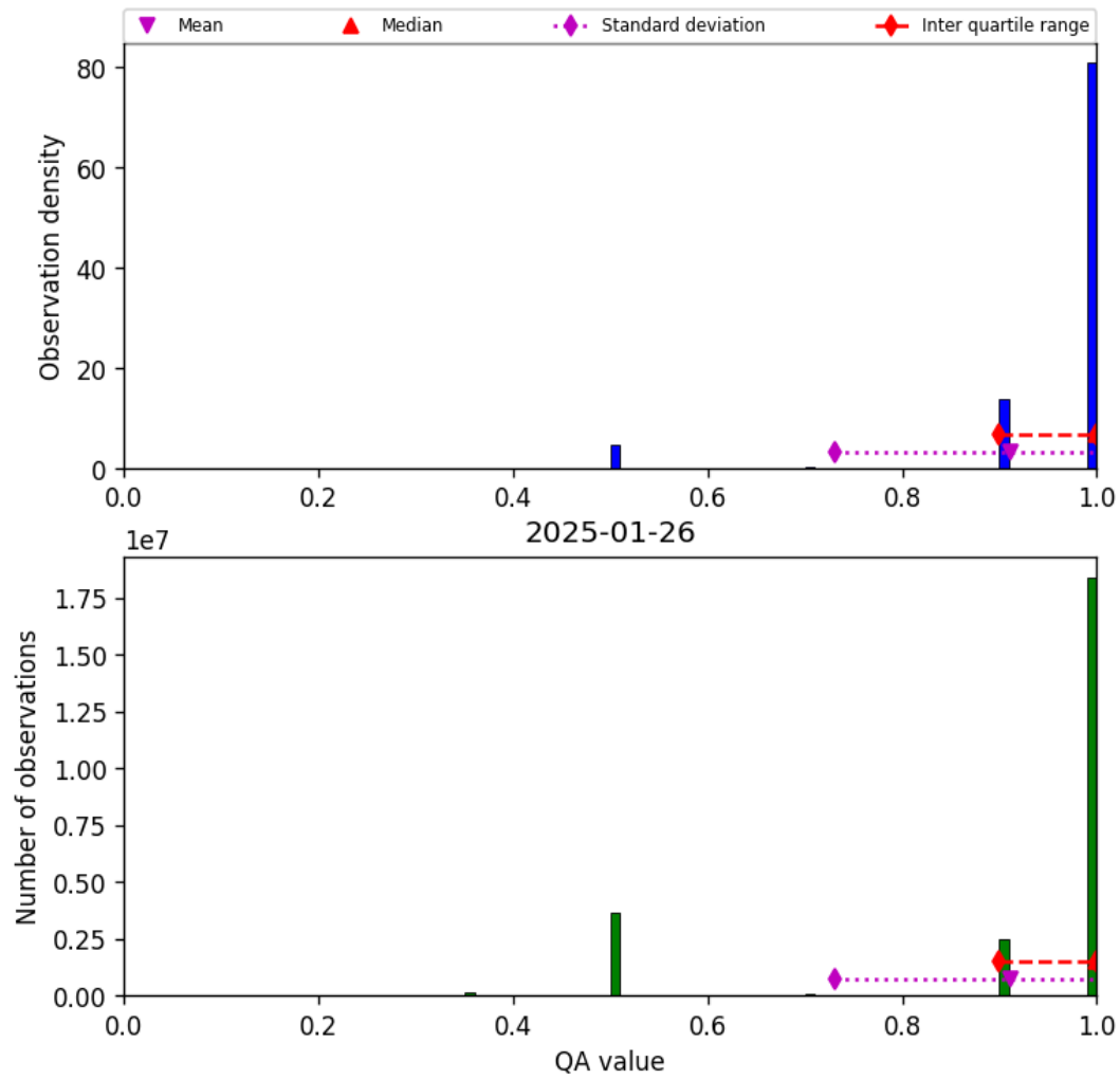
Figure 29: Histogram of “QA value” for 2025-01-25 to 2025-01-27
