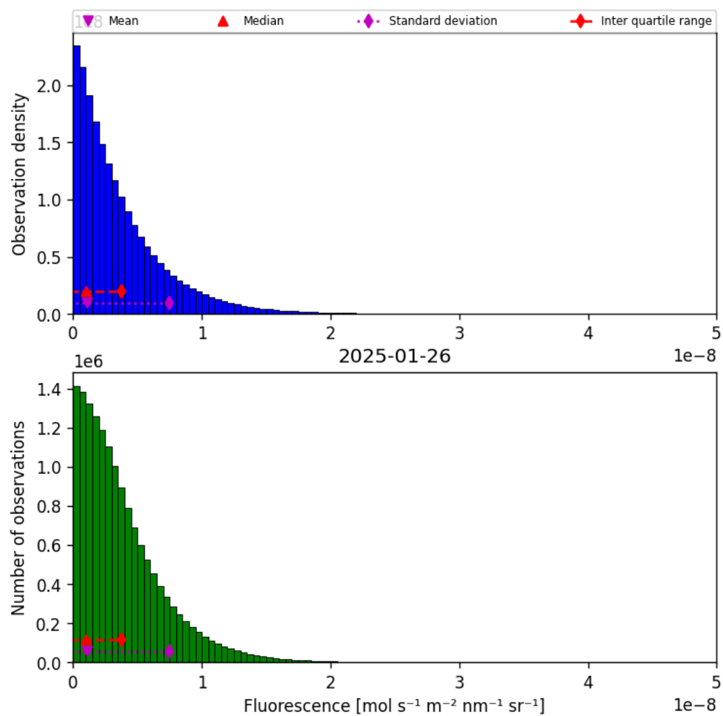
Figure 40: Histogram of “Fluorescence” for 2025-01-25 to 2025-01-27
