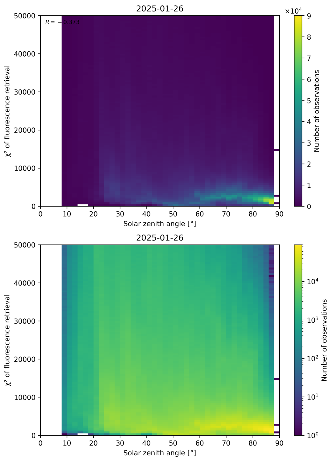
Figure 109: Scatter density plot of “Solar zenith angle” against “ \chi^2 of fluorescence retrieval” for 2025-01-25 to 2025-01-27.
