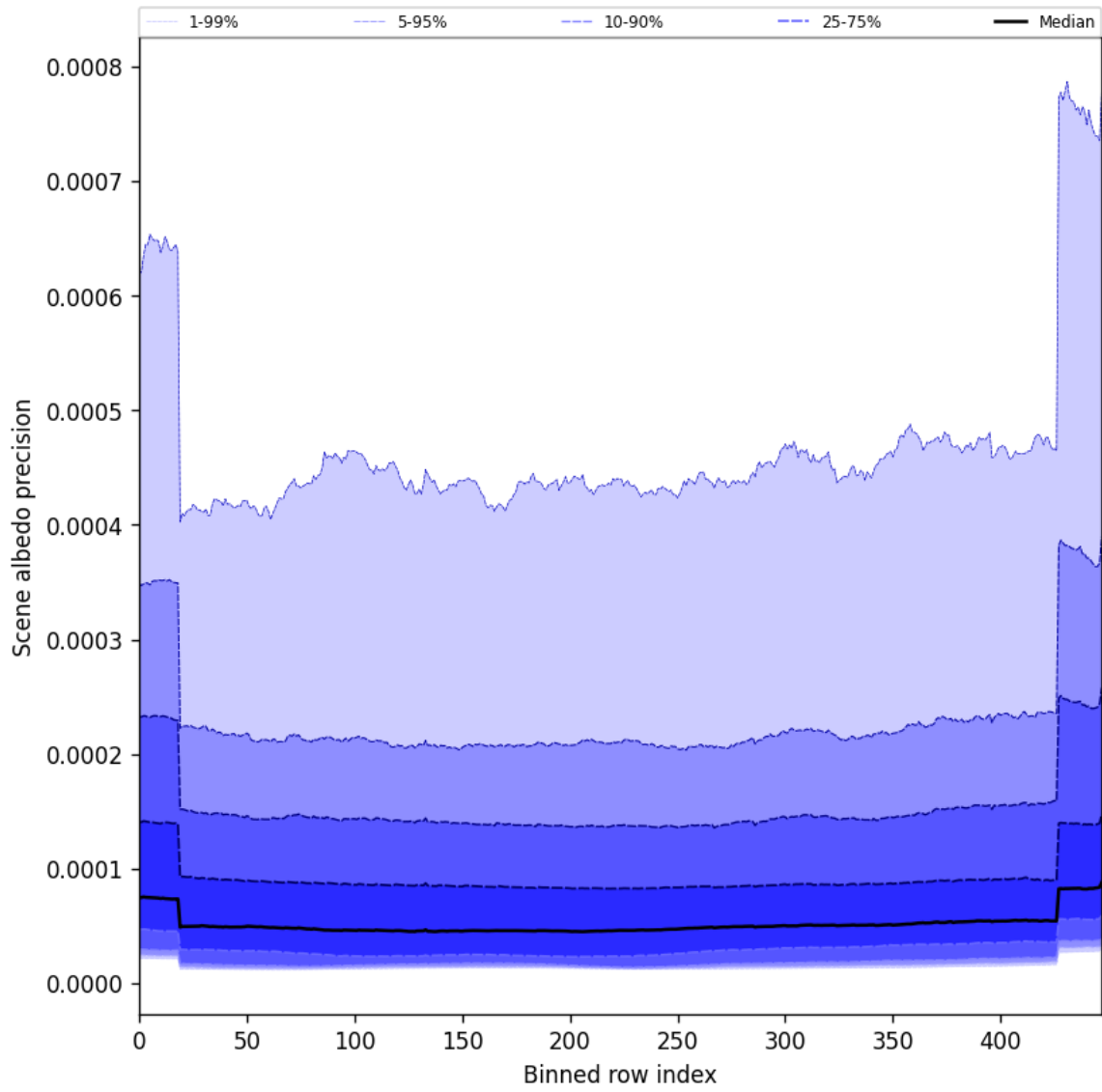
Figure 52: Along track statistics of “Scene albedo precision” for 2025-01-26 to 2025-01-28
