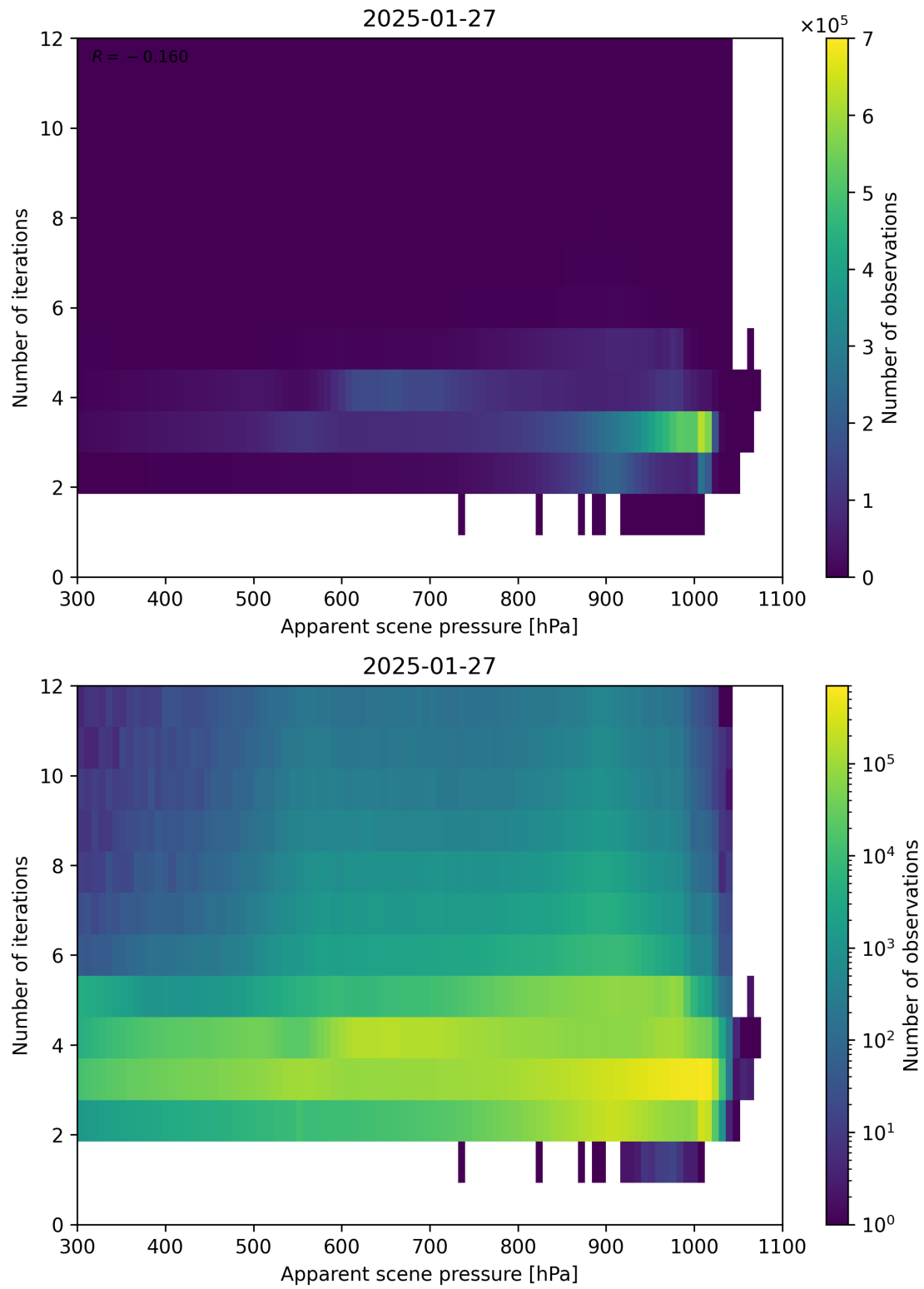
Figure 65: Scatter density plot of “Apparent scene pressure” against “Number of iterations” for 2025-01-26 to 2025-01-28.
