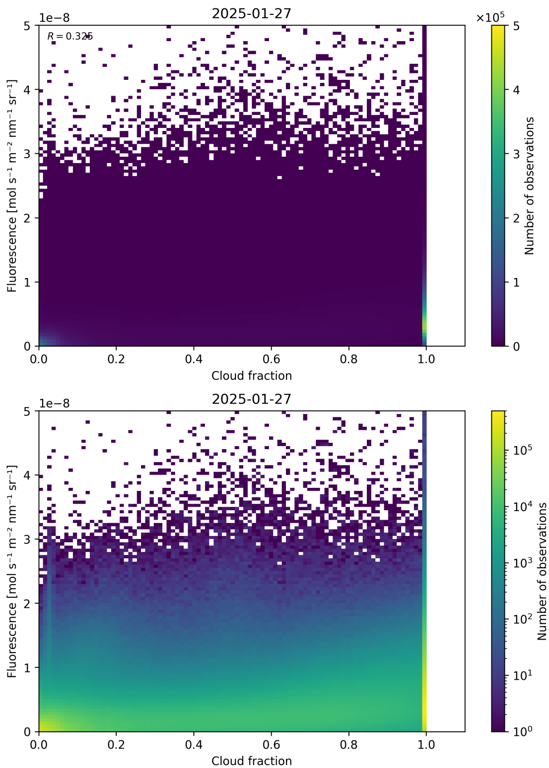
Figure 72: Scatter density plot of “Cloud fraction” against “Fluorescence” for 2025-01-26 to 2025-01-28.
