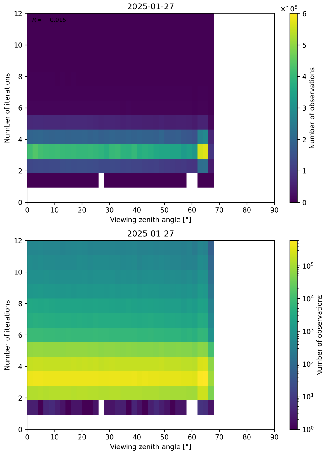
Figure 124: Scatter density plot of “Viewing zenith angle” against “Number of iterations” for 2025-01-26 to 2025-01-28.
