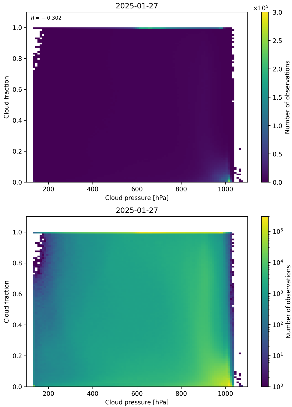
Figure 79: Scatter density plot of “Cloud pressure” against “Cloud fraction” for 2025-01-26 to 2025-01-28.
