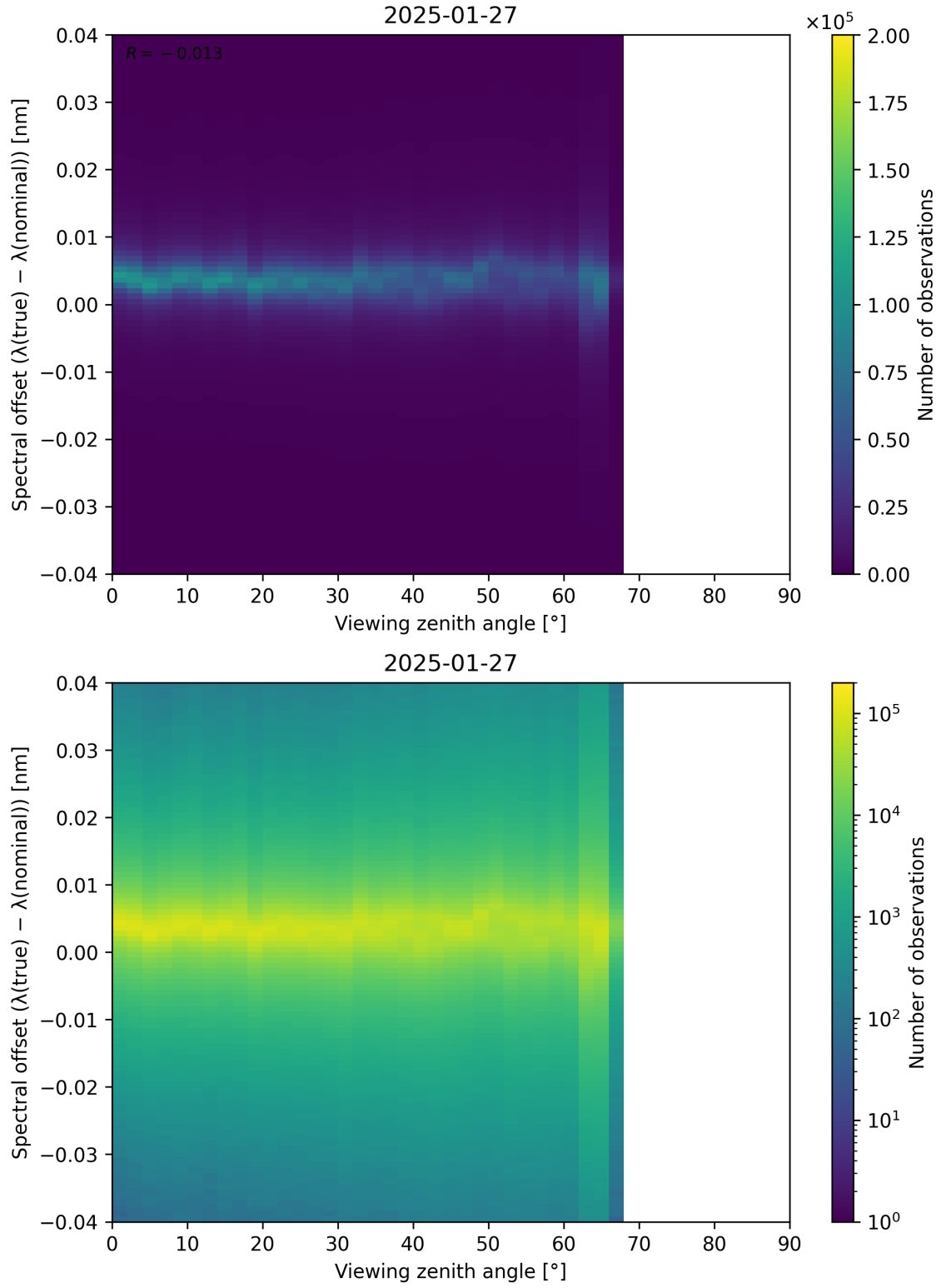
Figure 128: Scatter density plot of “Viewing zenith angle” against “Spectral offset ( \lambda_{\text{true}} - \lambda_{\text{nominal}} )” for 2025-01-26 to 2025-01-28.
