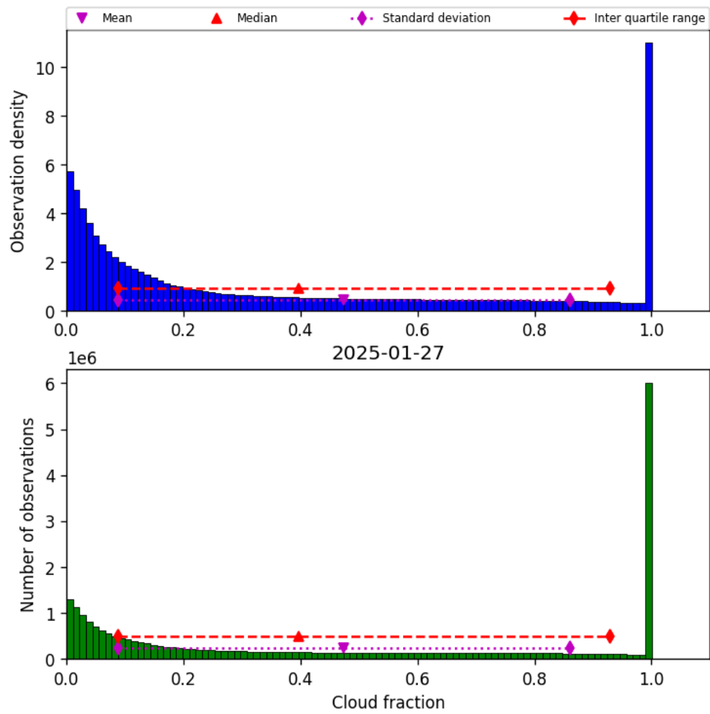
Figure 32: Histogram of “Cloud fraction” for 2025-01-26 to 2025-01-28
