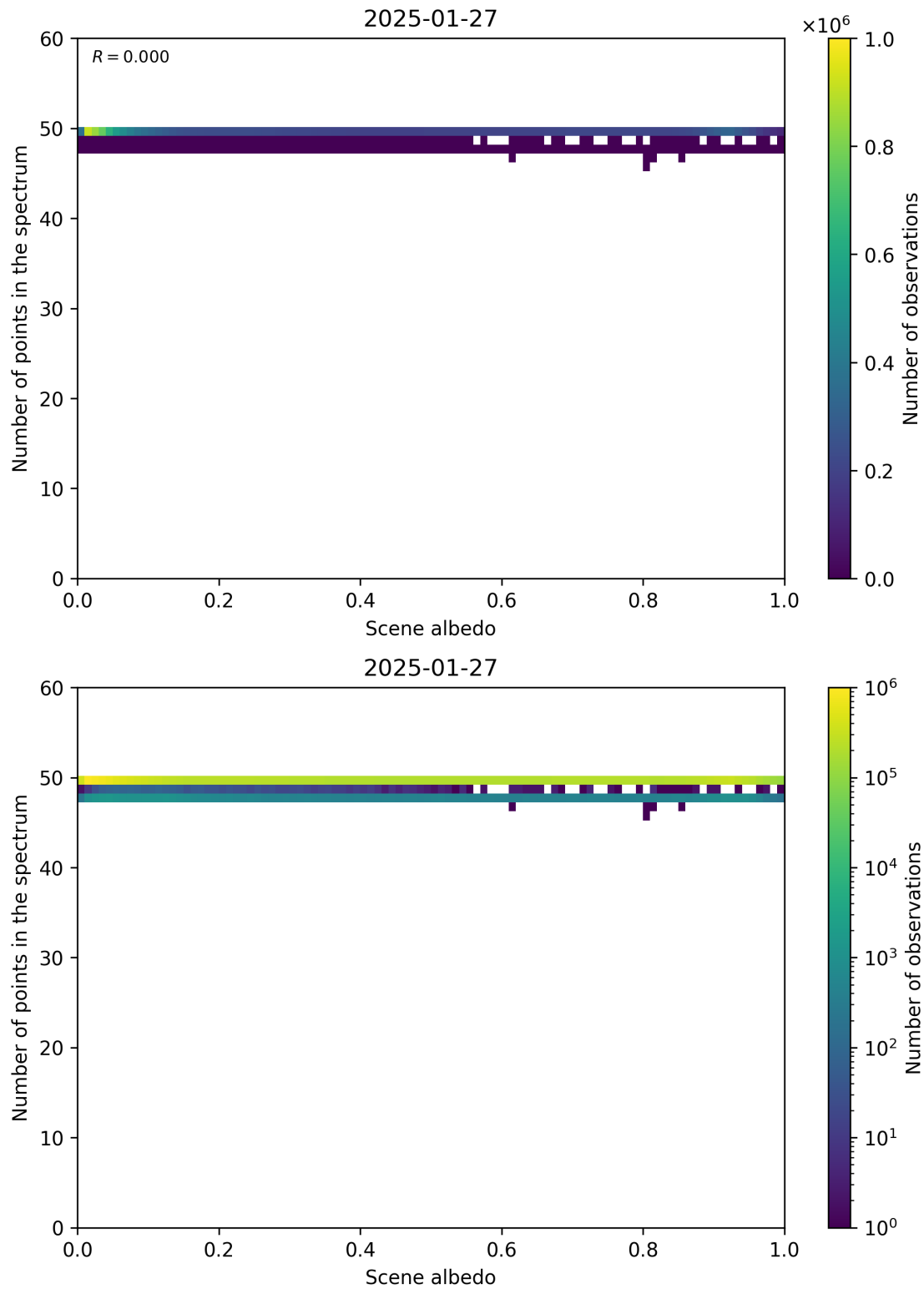
Figure 106: Scatter density plot of “Scene albedo” against “Number of points in the spectrum” for 2025-01-26 to 2025-01-28.
