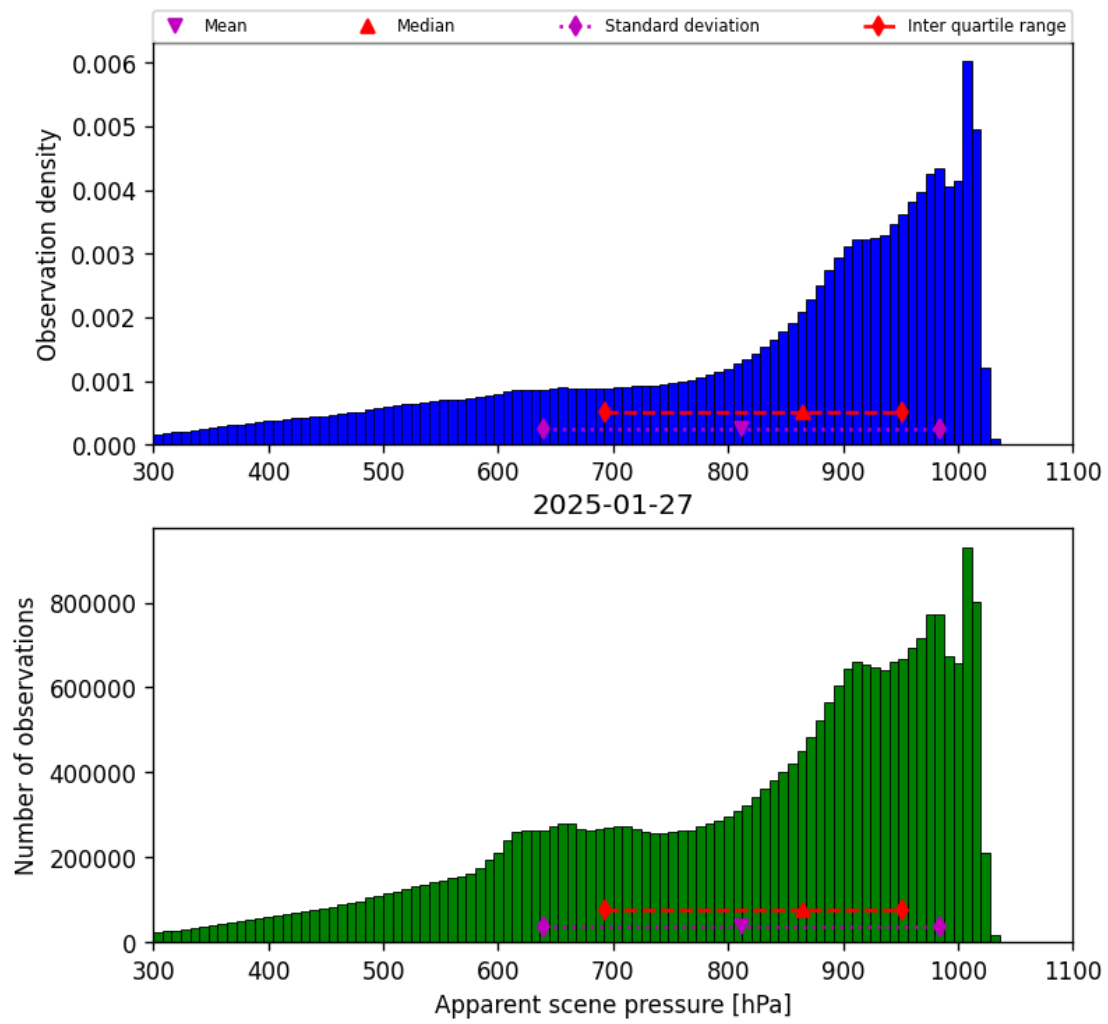
Figure 36: Histogram of “Apparent scene pressure” for 2025-01-26 to 2025-01-28
