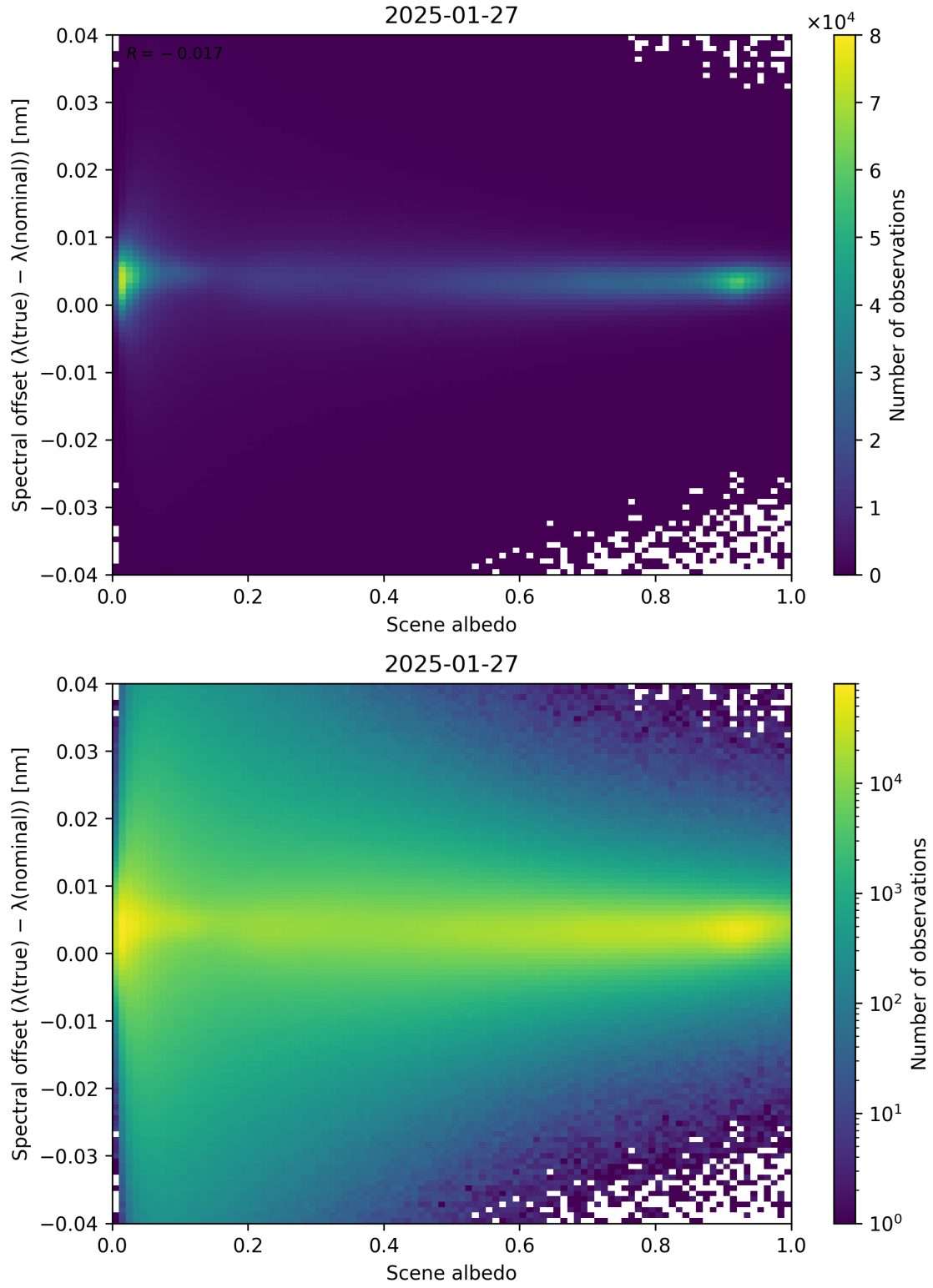
Figure 107: Scatter density plot of “Scene albedo” against “Spectral offset ( \lambda_{\text{true}} - \lambda_{\text{nominal}} )” for 2025-01-26 to 2025-01-28.
