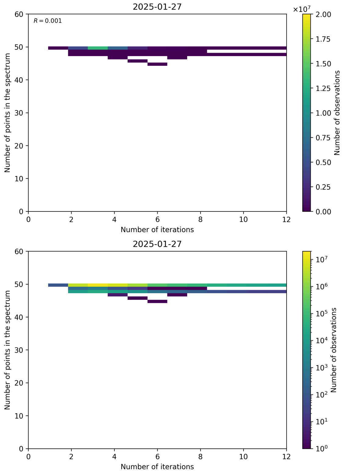
Figure 99: Scatter density plot of “Number of iterations” against “Number of points in the spectrum” for 2025-01-26 to 2025-01-28.
