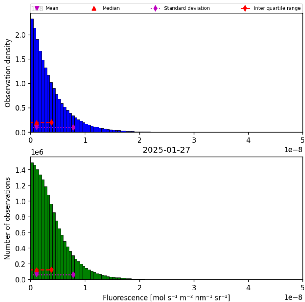
Figure 40: Histogram of “Fluorescence” for 2025-01-26 to 2025-01-28
