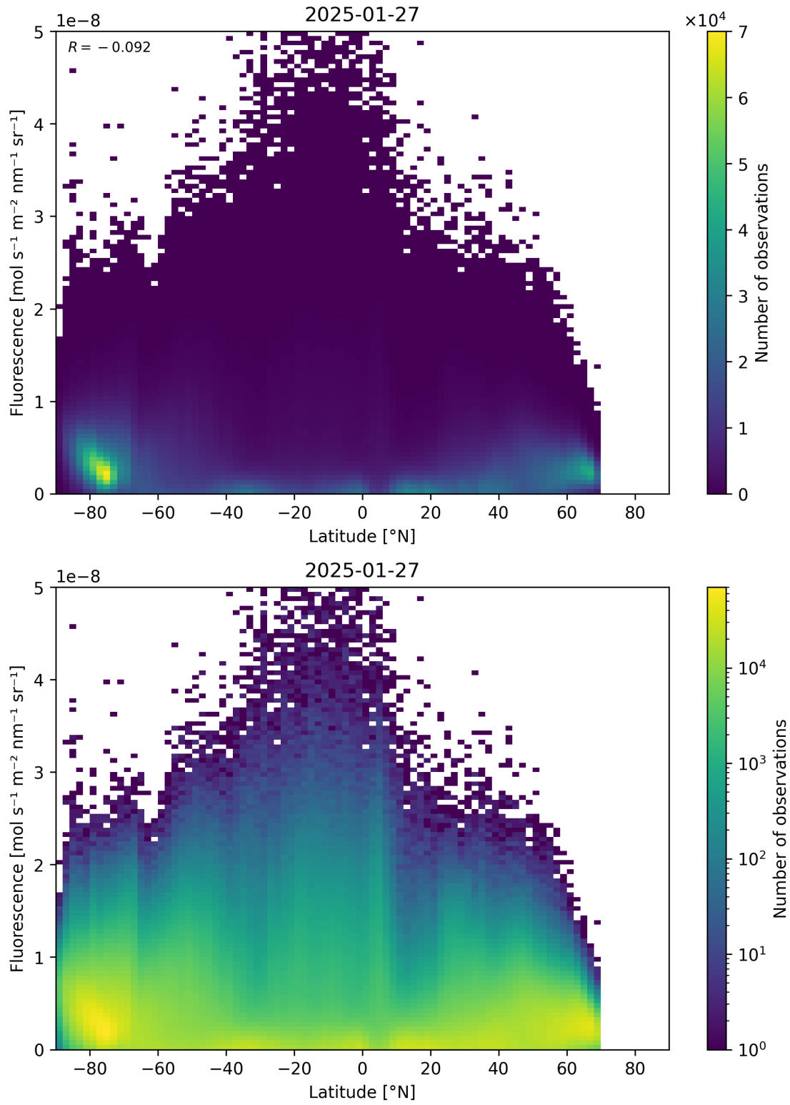
Figure 92: Scatter density plot of “Latitude” against “Fluorescence” for 2025-01-26 to 2025-01-28.
