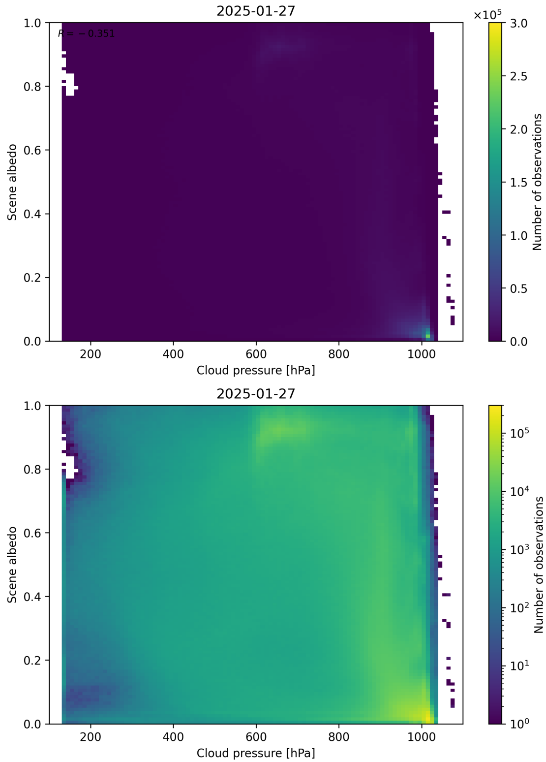
Figure 83: Scatter density plot of “Cloud pressure” against “Scene albedo” for 2025-01-26 to 2025-01-28.
