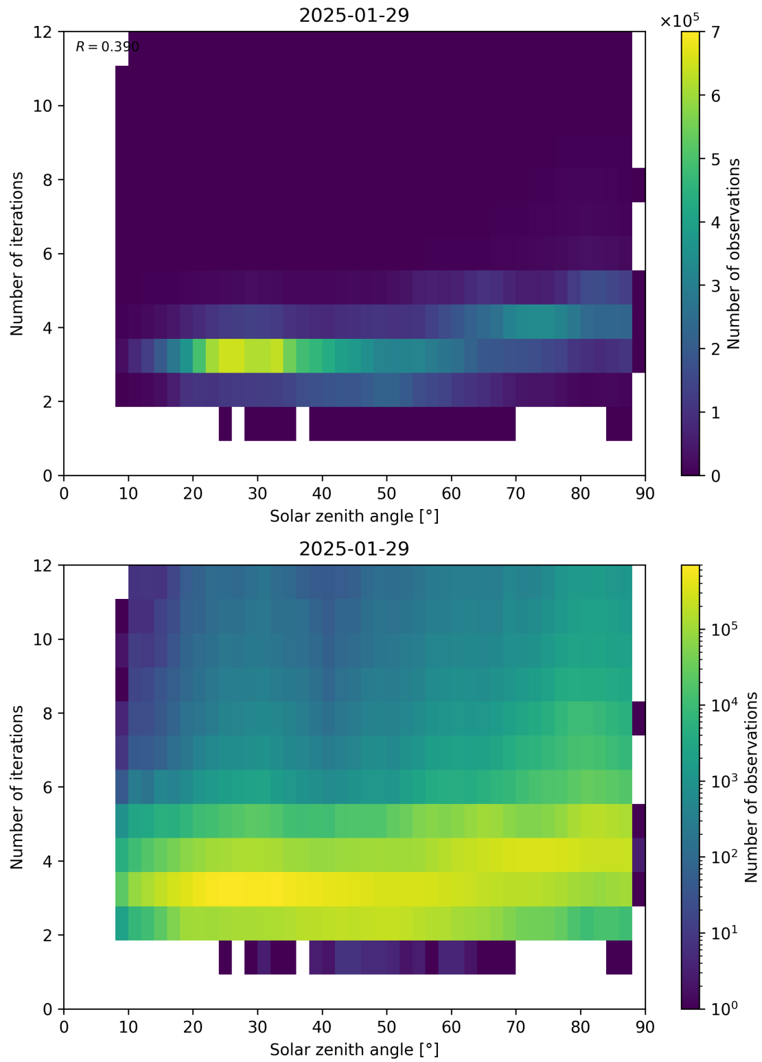
Figure 114: Scatter density plot of “Solar zenith angle” against “Number of iterations” for 2025-01-28 to 2025-01-30.
