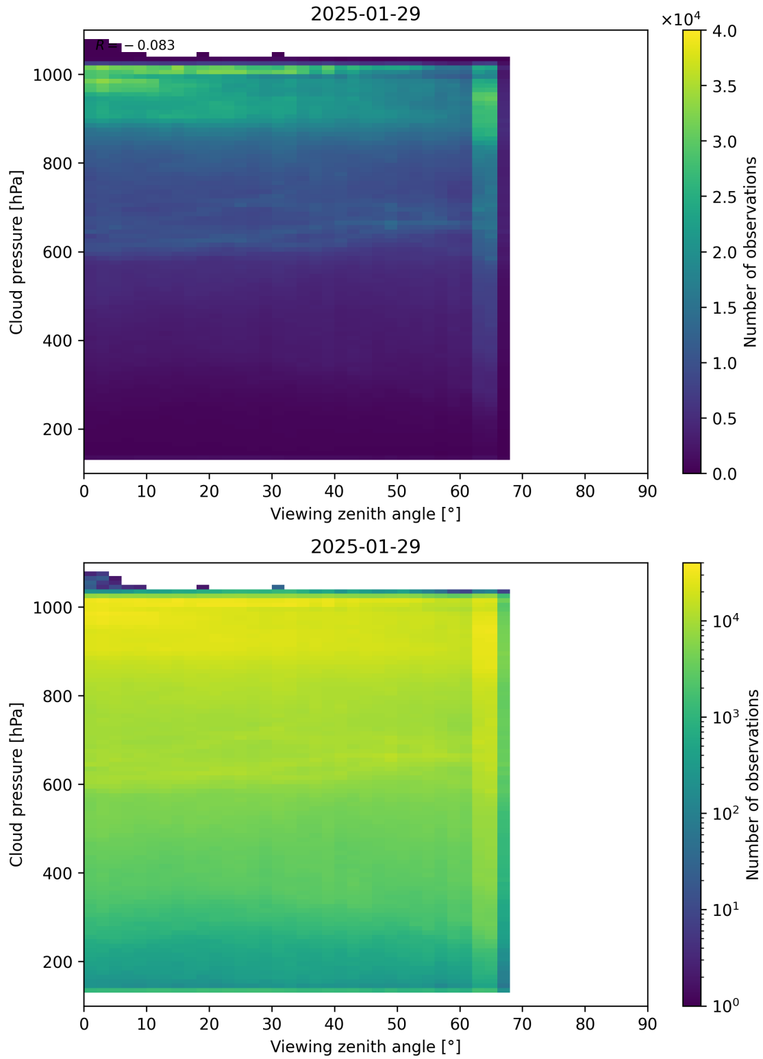
Figure 121: Scatter density plot of “Viewing zenith angle” against “Cloud pressure” for 2025-01-28 to 2025-01-30.
