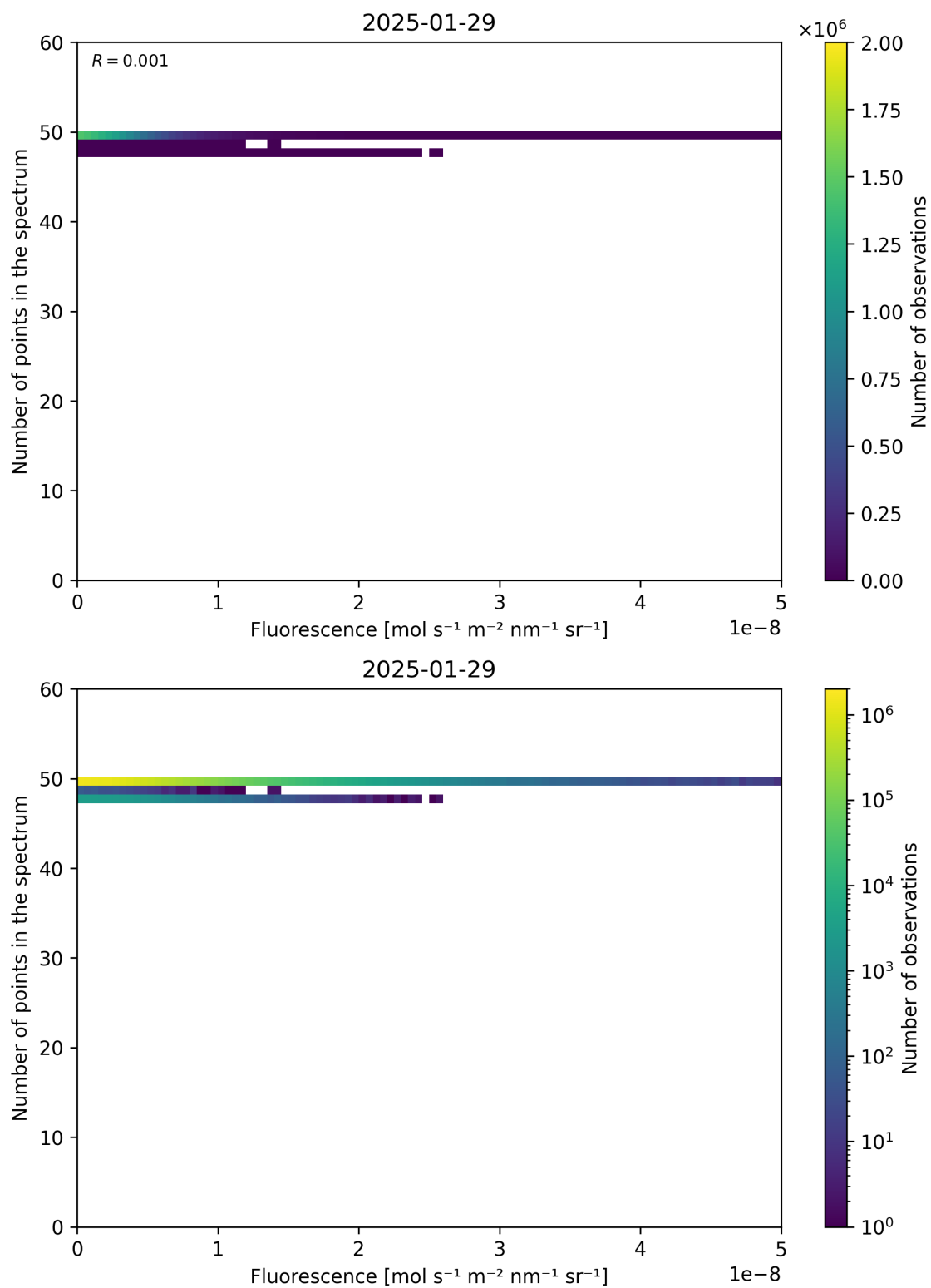
Figure 86: Scatter density plot of “Fluorescence” against “Number of points in the spectrum” for 2025-01-28 to 2025-01-30.
