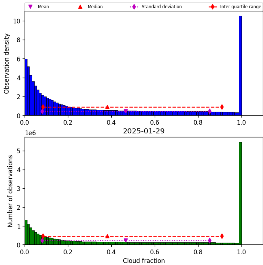
Figure 32: Histogram of “Cloud fraction” for 2025-01-28 to 2025-01-30
