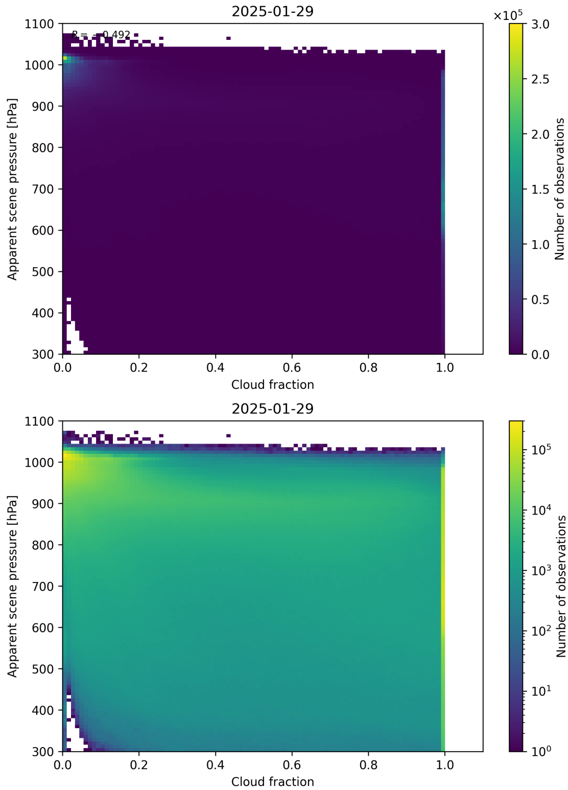
Figure 70: Scatter density plot of “Cloud fraction” against “Apparent scene pressure” for 2025-01-28 to 2025-01-30.
