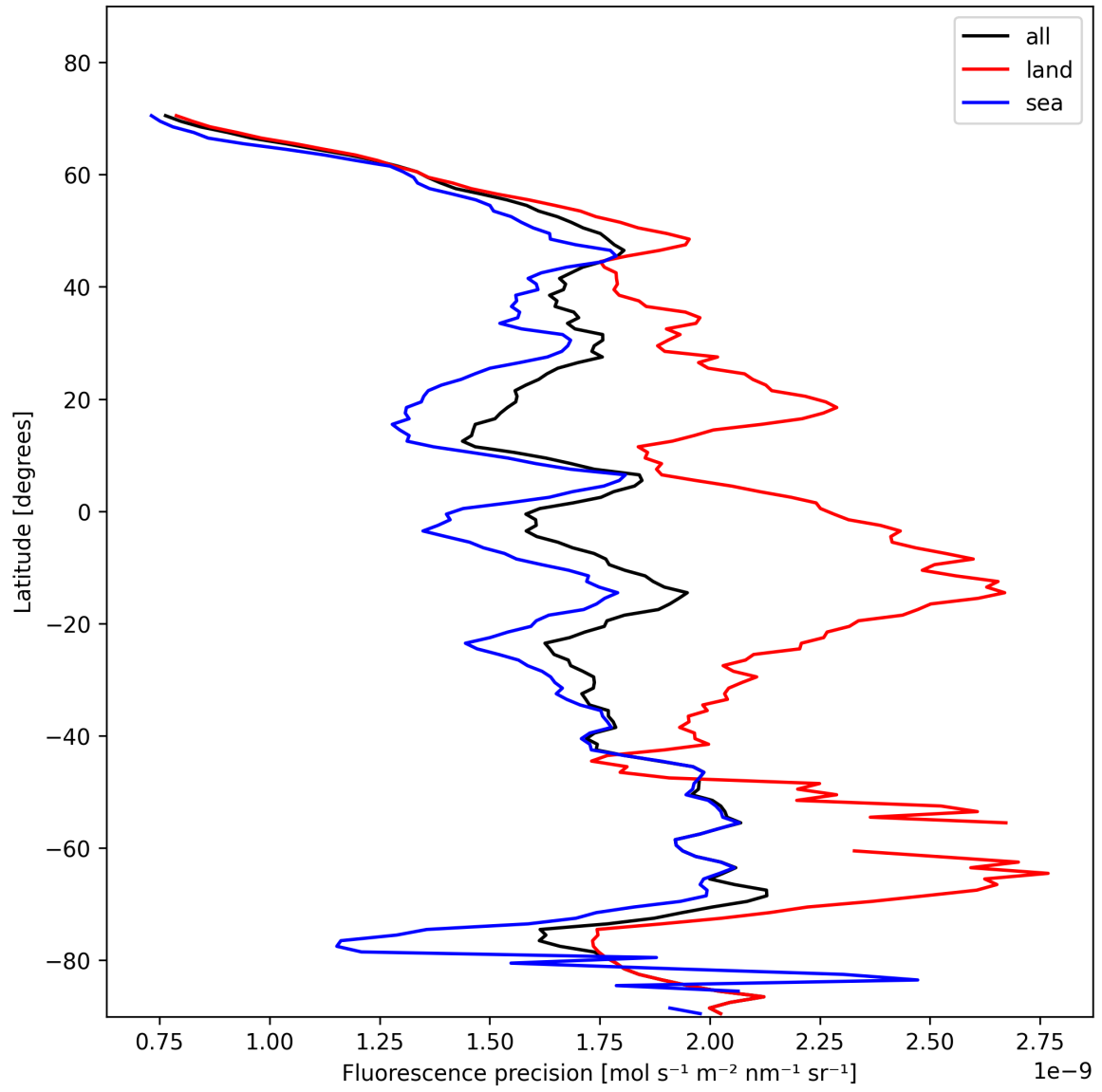
Figure 24: Zonal average of “Fluorescence precision” for 2025-01-28 to 2025-01-30.
