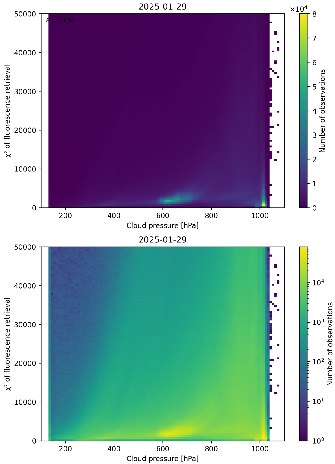
Figure 78: Scatter density plot of “Cloud pressure” against “ \chi^2 of fluorescence retrieval” for 2025-01-28 to 2025-01-30.
