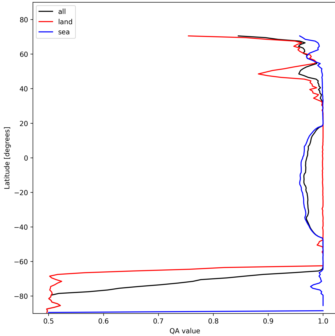
Figure 12: Zonal average of “QA value” for 2025-01-28 to 2025-01-30.
