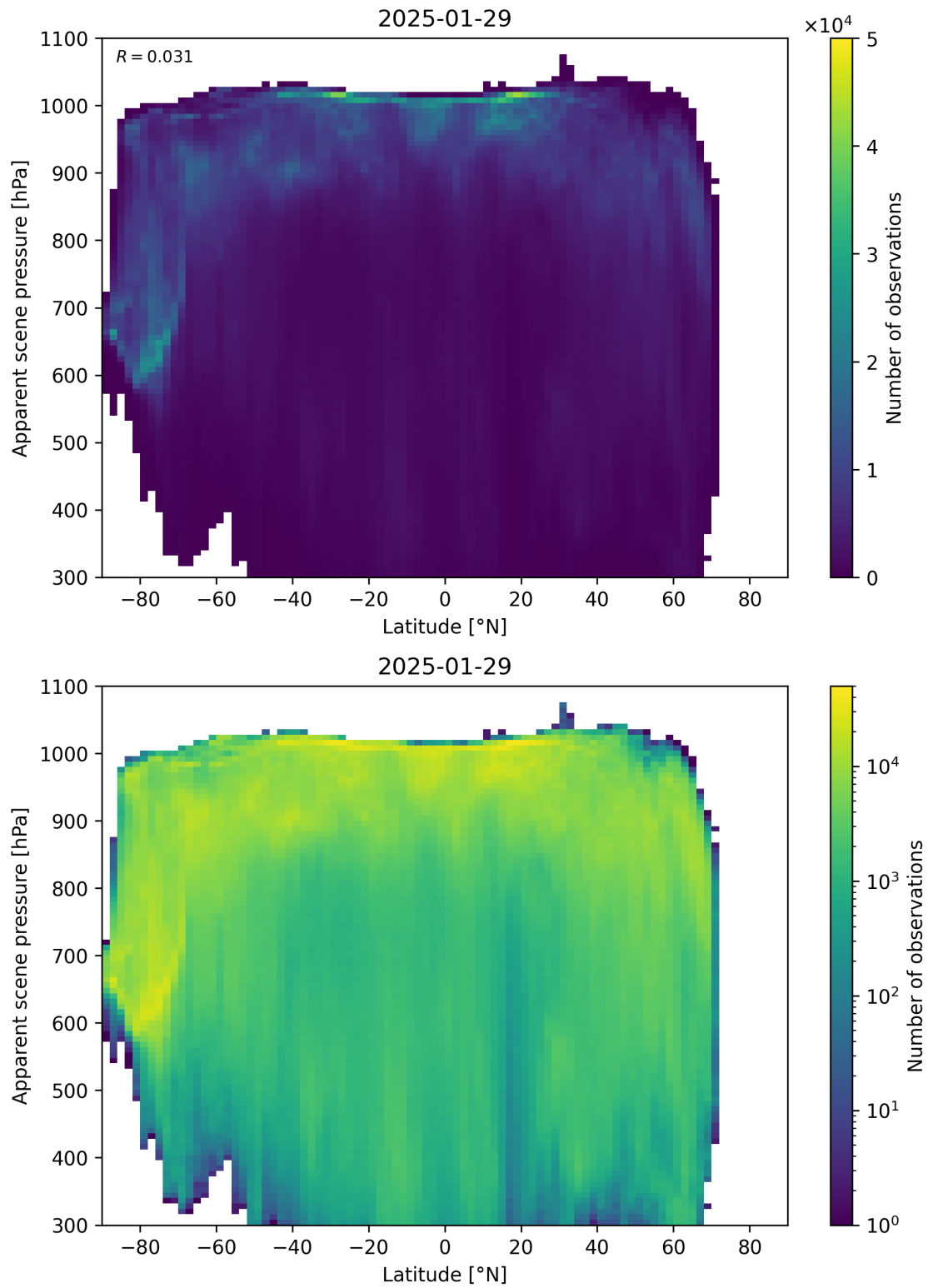
Figure 88: Scatter density plot of “Latitude” against “Apparent scene pressure” for 2025-01-28 to 2025-01-30.
