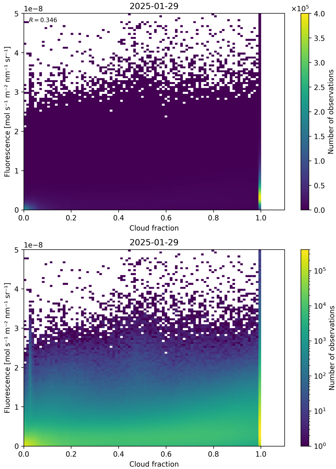
Figure 72: Scatter density plot of “Cloud fraction” against “Fluorescence” for 2025-01-28 to 2025-01-30.
