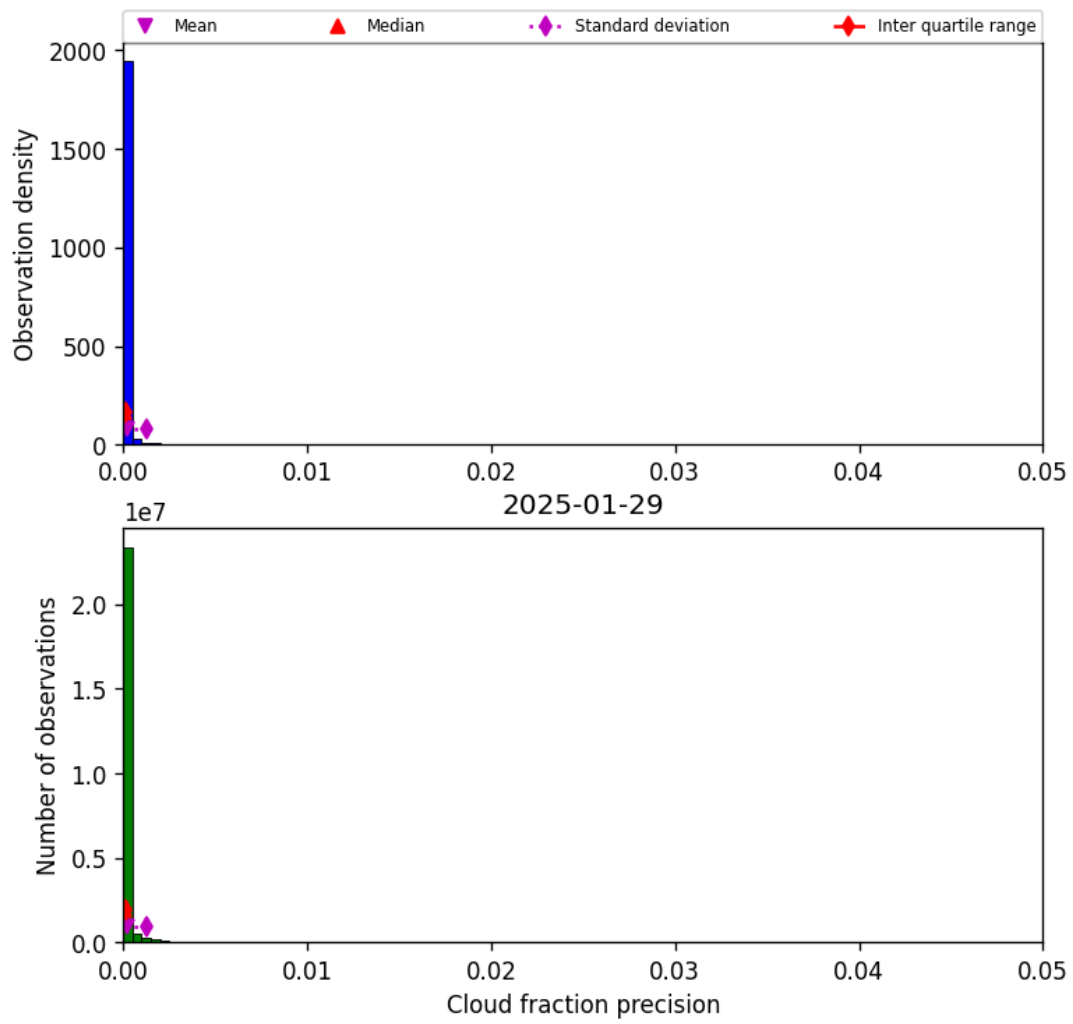
Figure 33: Histogram of “Cloud fraction precision” for 2025-01-28 to 2025-01-30
