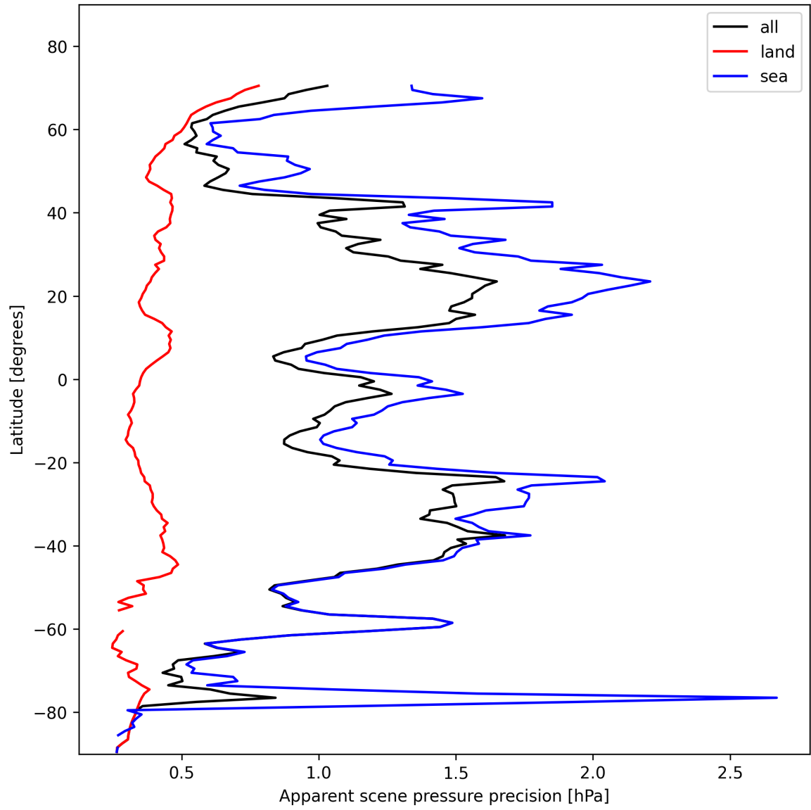
Figure 20: Zonal average of “Apparent scene pressure precision” for 2025-01-28 to 2025-01-30.
