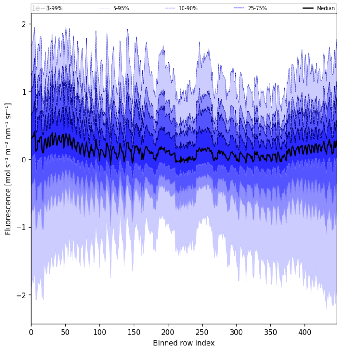
Figure 57: Along track statistics of “Fluorescence” for 2025-01-28 to 2025-01-30
