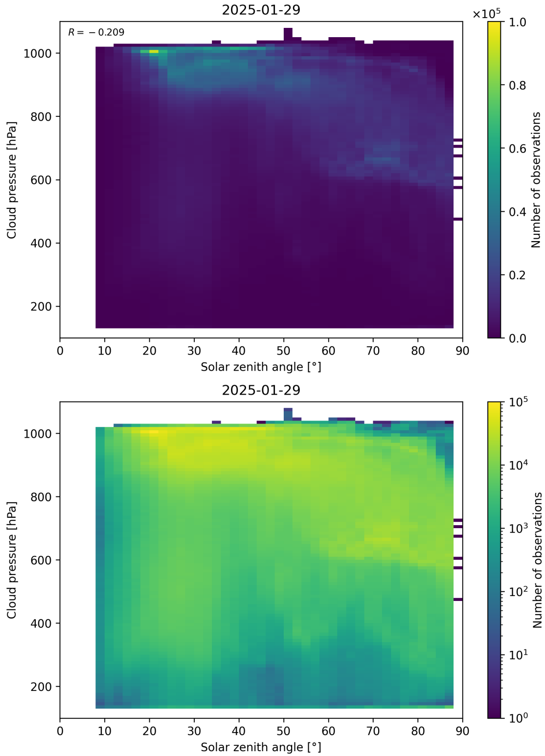
Figure 111: Scatter density plot of “Solar zenith angle” against “Cloud pressure” for 2025-01-28 to 2025-01-30.
