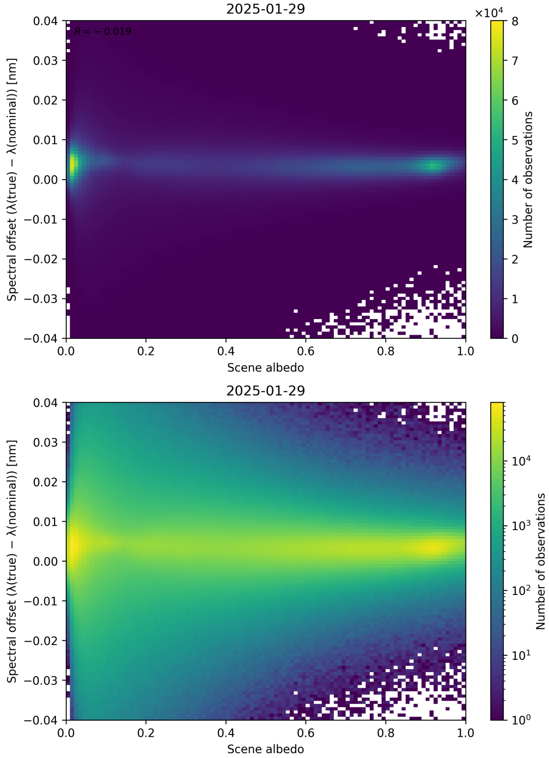
Figure 107: Scatter density plot of “Scene albedo” against “Spectral offset ( \lambda_{\text{true}} - \lambda_{\text{nominal}} )” for 2025-01-28 to 2025-01-30.
