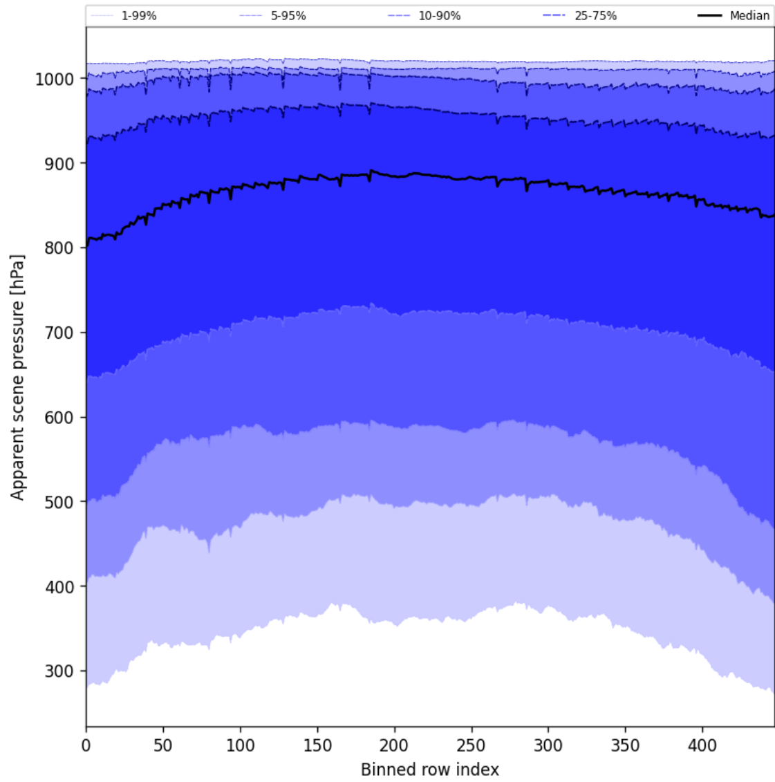
Figure 53: Along track statistics of “Apparent scene pressure” for 2025-01-28 to 2025-01-30
