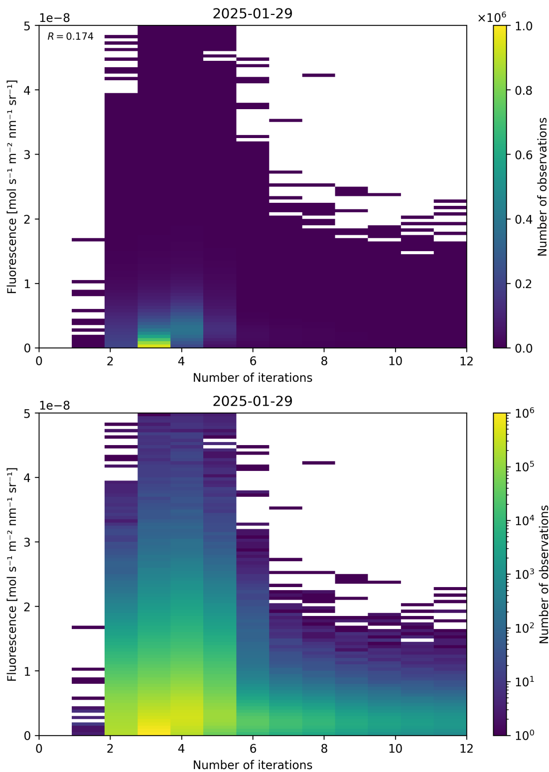
Figure 98: Scatter density plot of “Number of iterations” against “Fluorescence” for 2025-01-28 to 2025-01-30.
