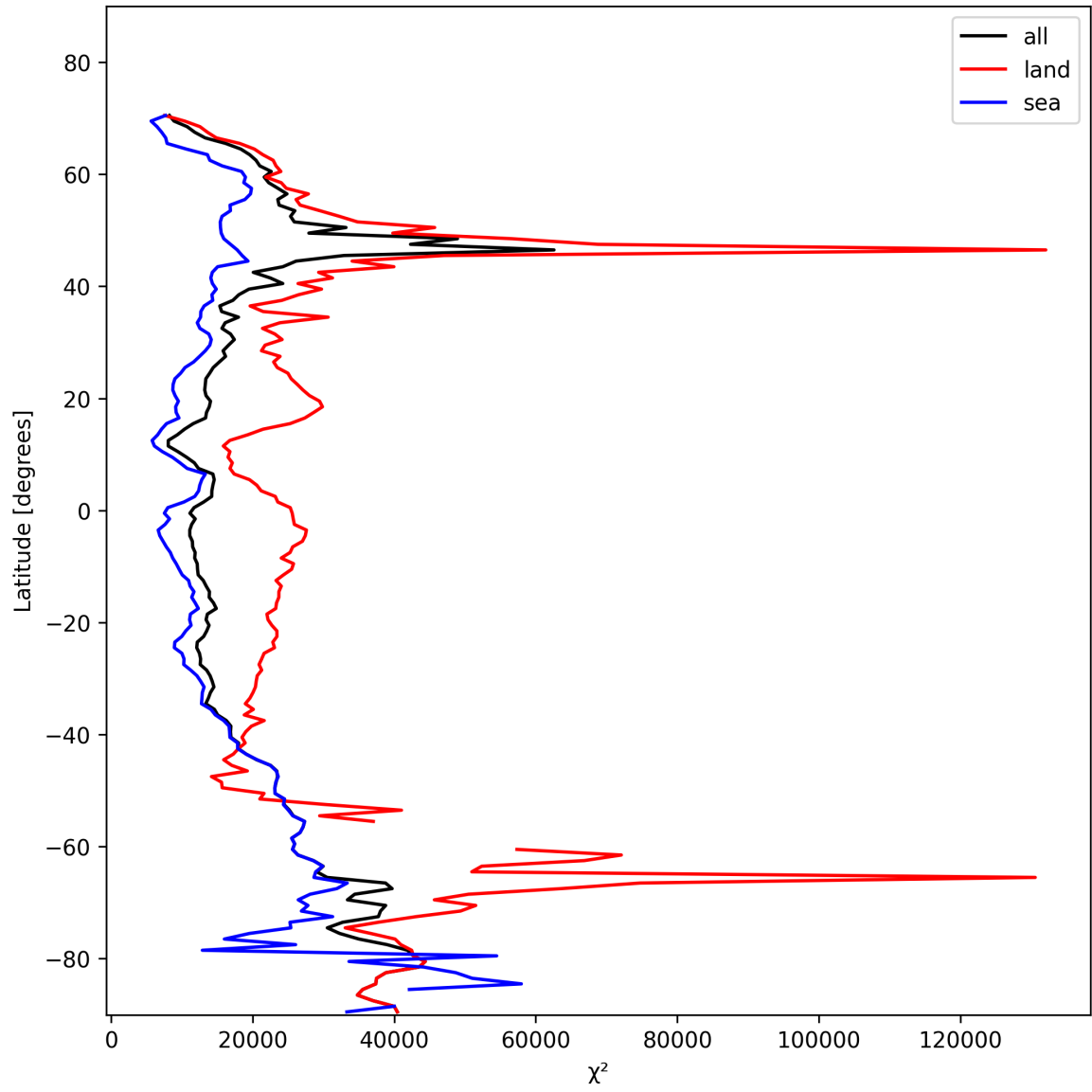
Figure 21: Zonal average of “ \chi^2 ” for 2025-01-28 to 2025-01-30.
