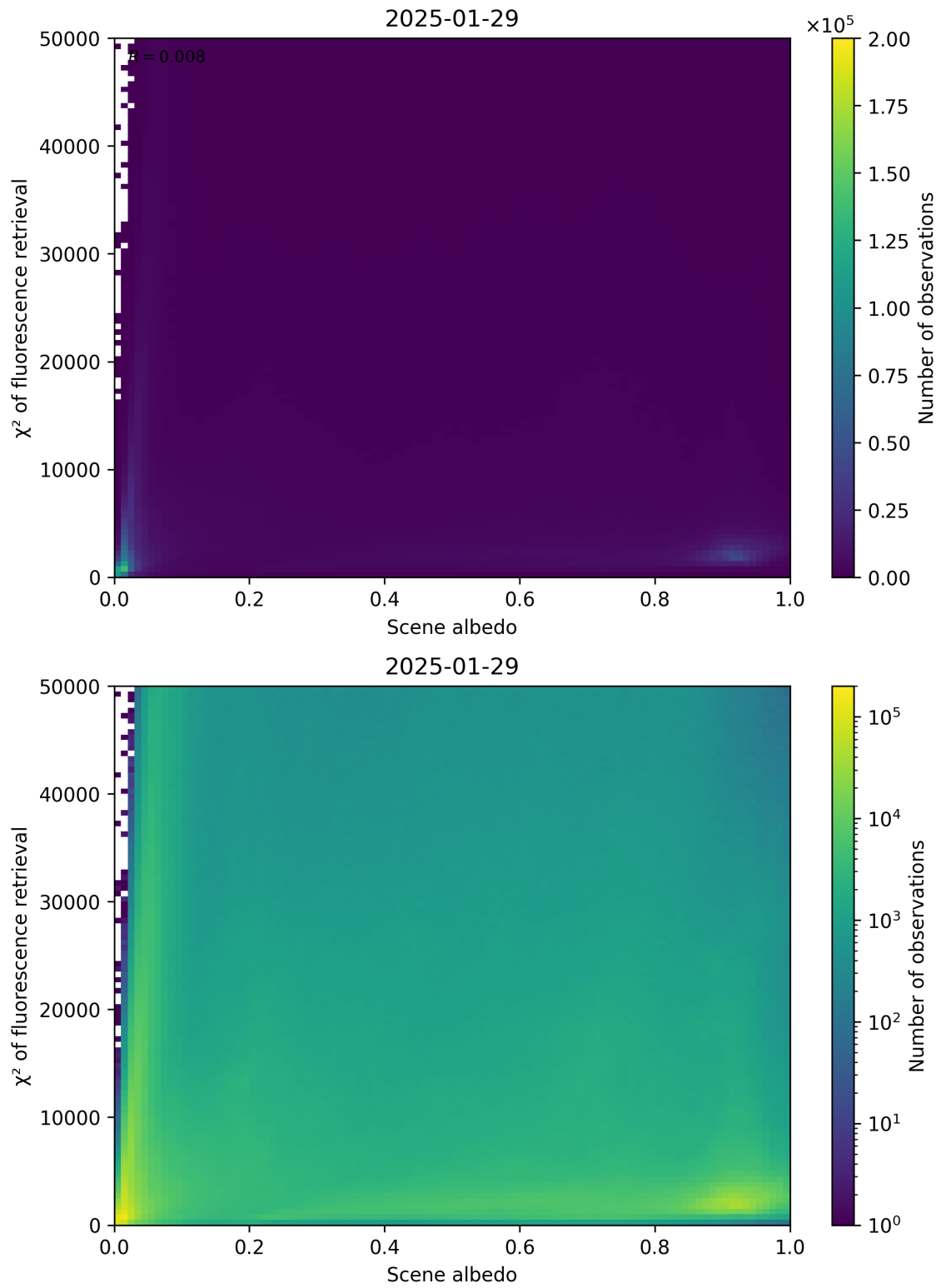
Figure 103: Scatter density plot of “Scene albedo” against “ \chi^2 of fluorescence retrieval” for 2025-01-28 to 2025-01-30.
