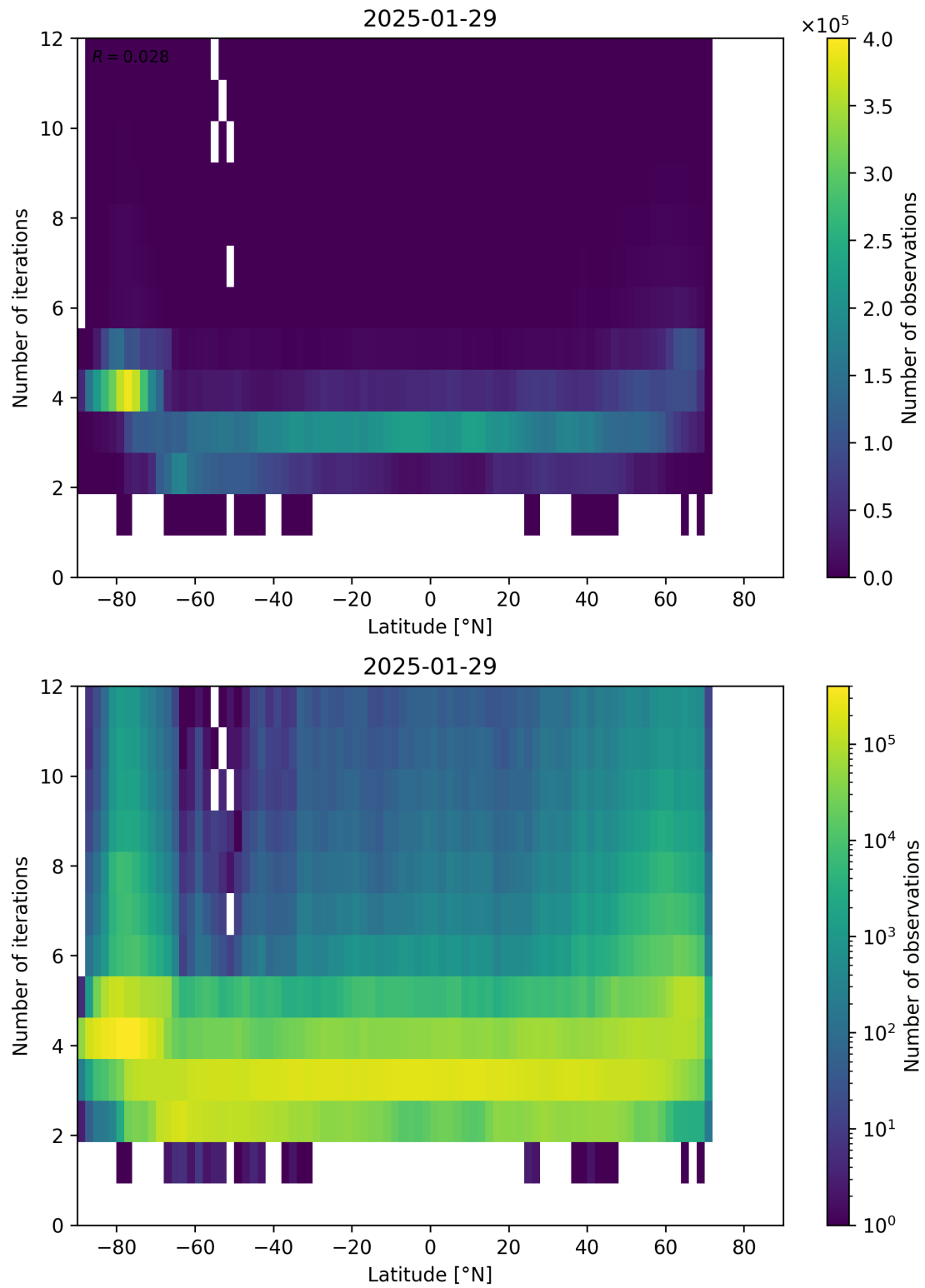
Figure 93: Scatter density plot of “Latitude” against “Number of iterations” for 2025-01-28 to 2025-01-30.
