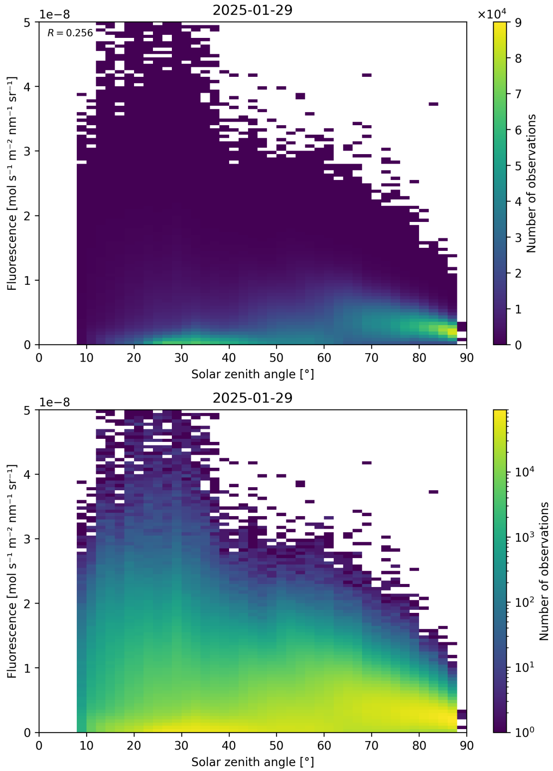
Figure 112: Scatter density plot of “Solar zenith angle” against “Fluorescence” for 2025-01-28 to 2025-01-30.
