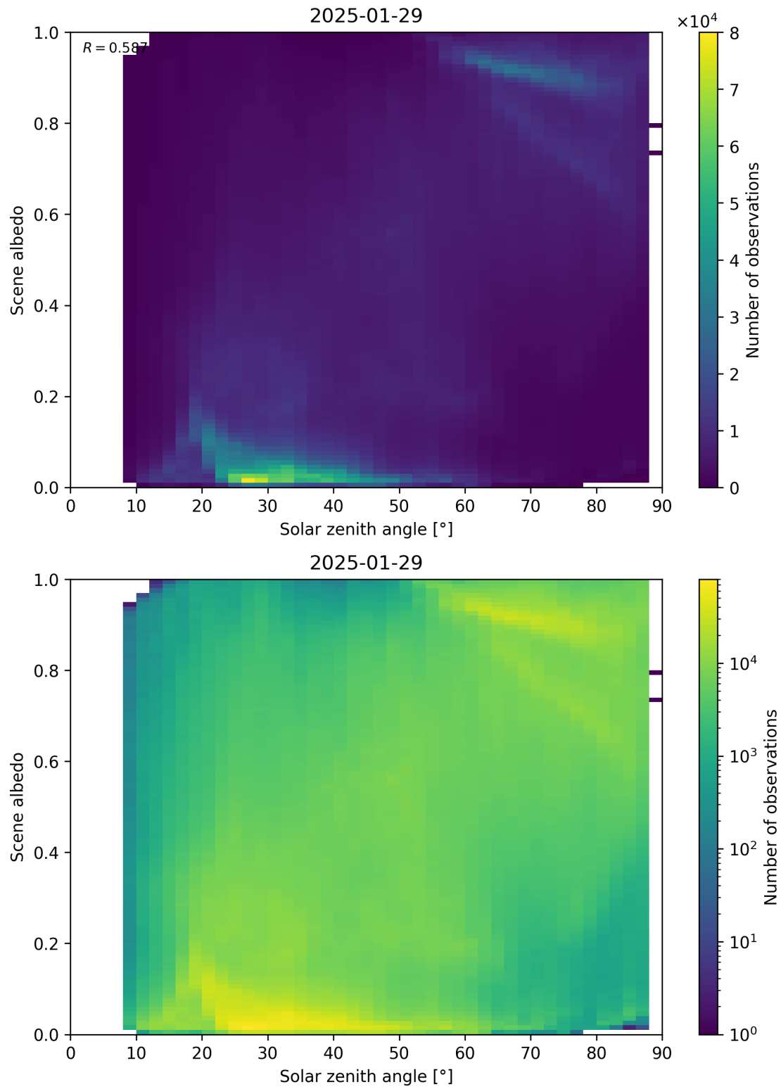
Figure 116: Scatter density plot of “Solar zenith angle” against “Scene albedo” for 2025-01-28 to 2025-01-30.
