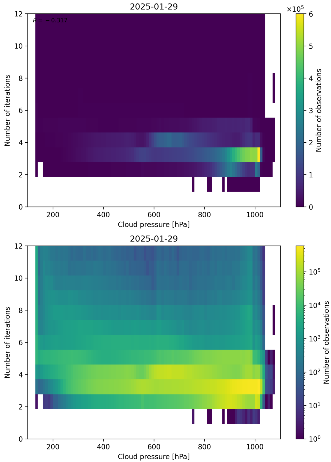
Figure 81: Scatter density plot of “Cloud pressure” against “Number of iterations” for 2025-01-28 to 2025-01-30.
