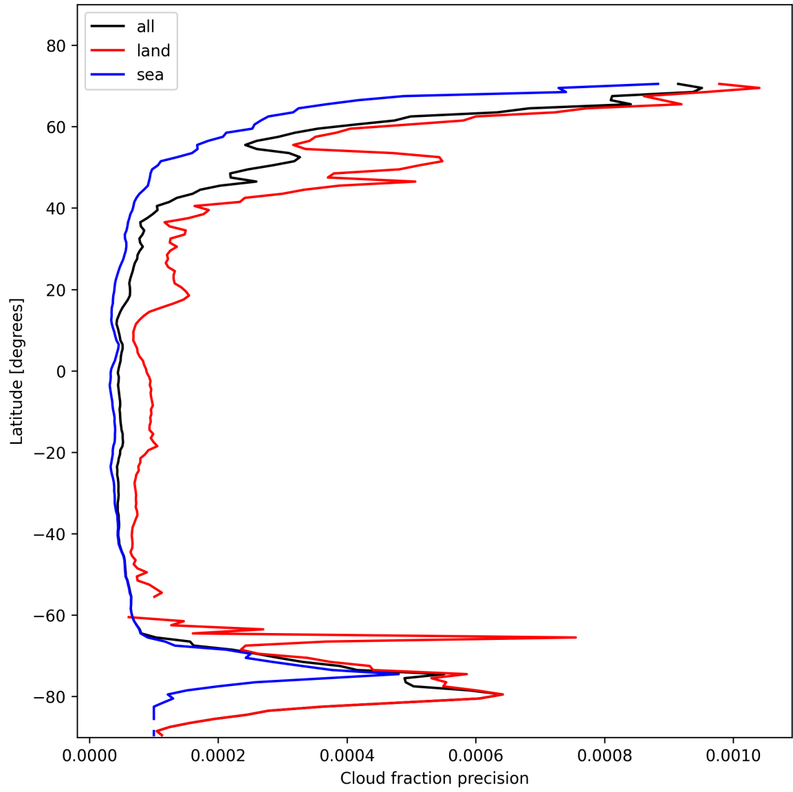
Figure 16: Zonal average of “Cloud fraction precision” for 2025-01-28 to 2025-01-30.
