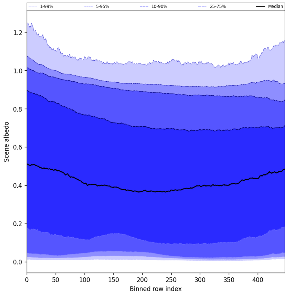
Figure 51: Along track statistics of “Scene albedo” for 2025-01-28 to 2025-01-30
