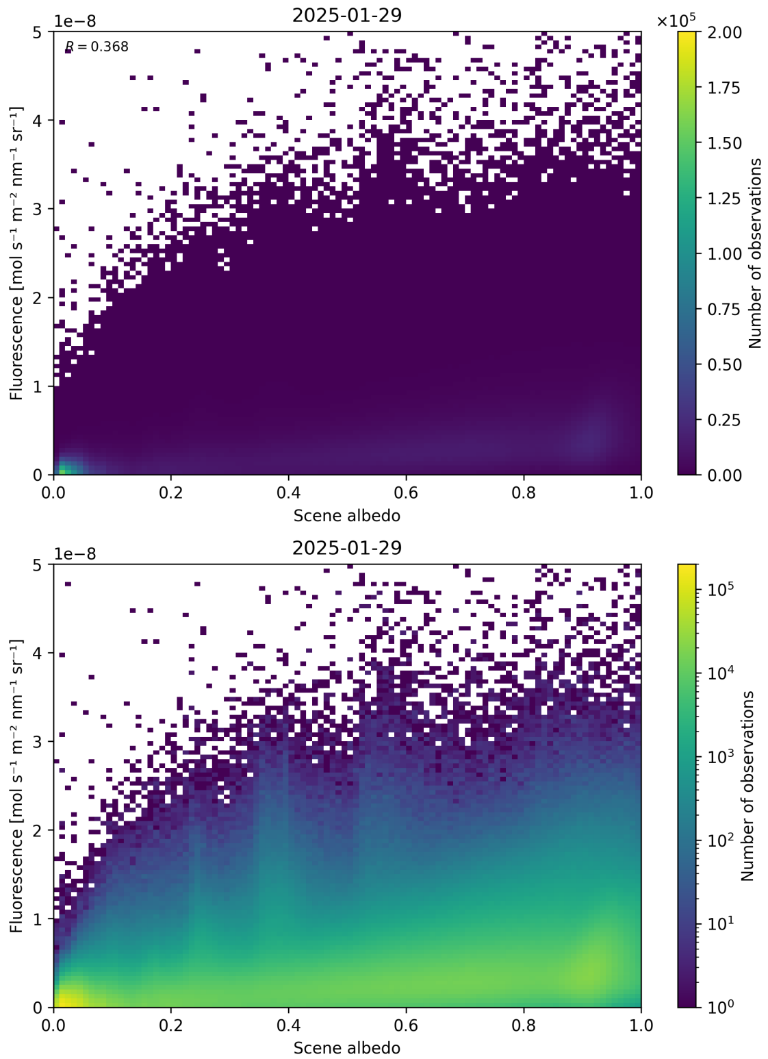
Figure 104: Scatter density plot of “Scene albedo” against “Fluorescence” for 2025-01-28 to 2025-01-30.
