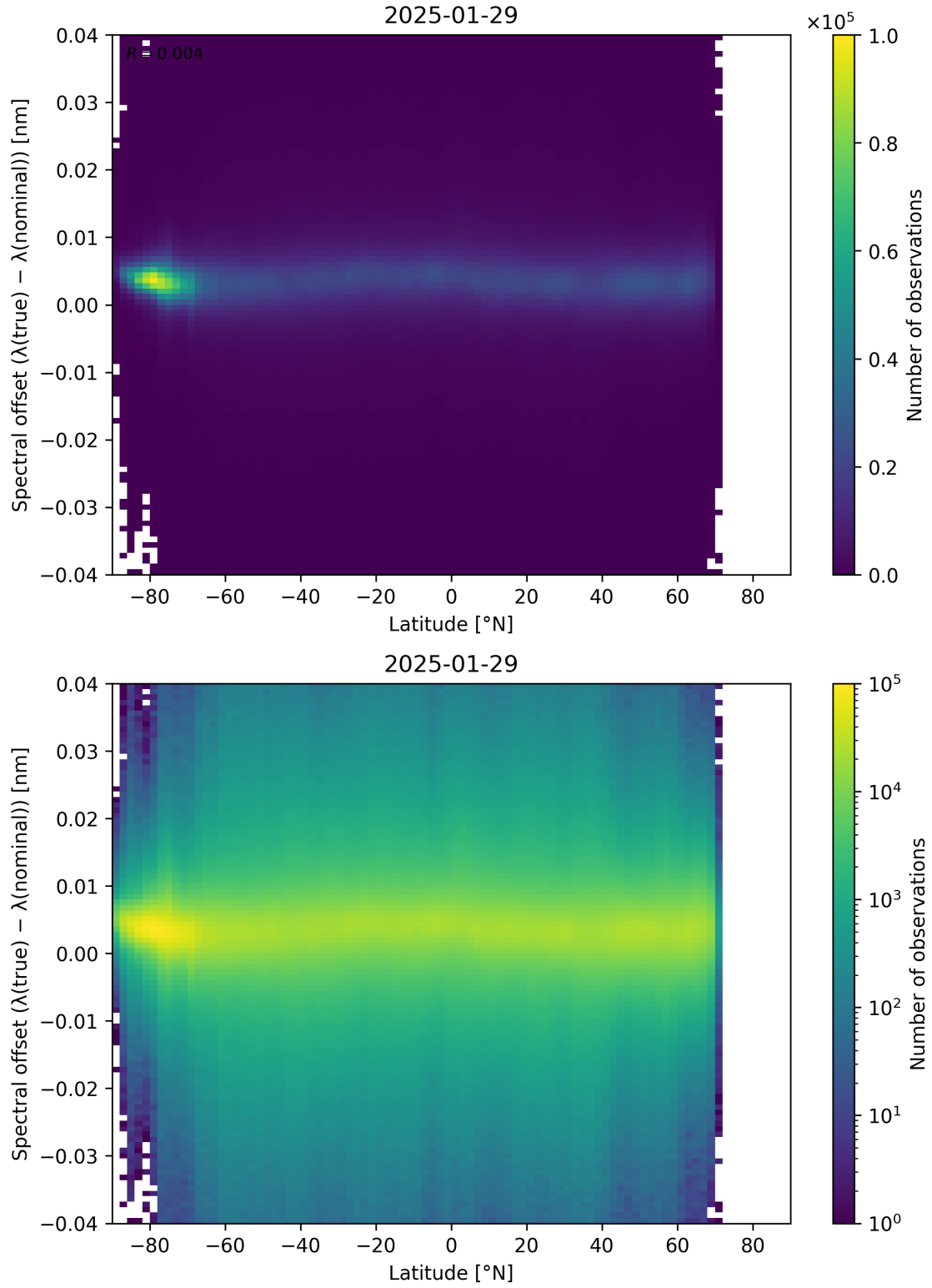
Figure 96: Scatter density plot of “Latitude” against “Spectral offset ( \lambda_{\text{true}} - \lambda_{\text{nominal}} )” for 2025-01-28 to 2025-01-30.
