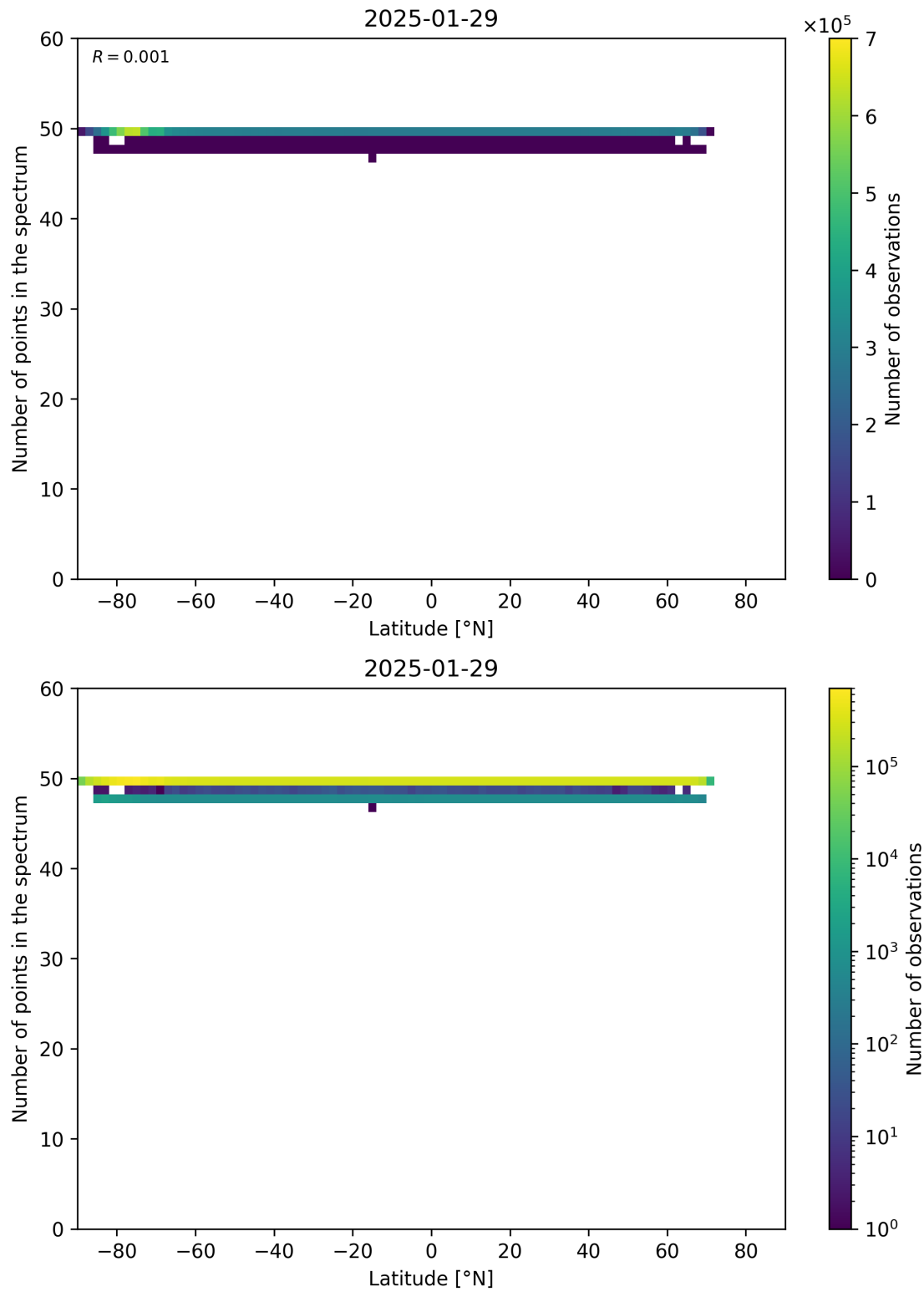
Figure 94: Scatter density plot of “Latitude” against “Number of points in the spectrum” for 2025-01-28 to 2025-01-30.
