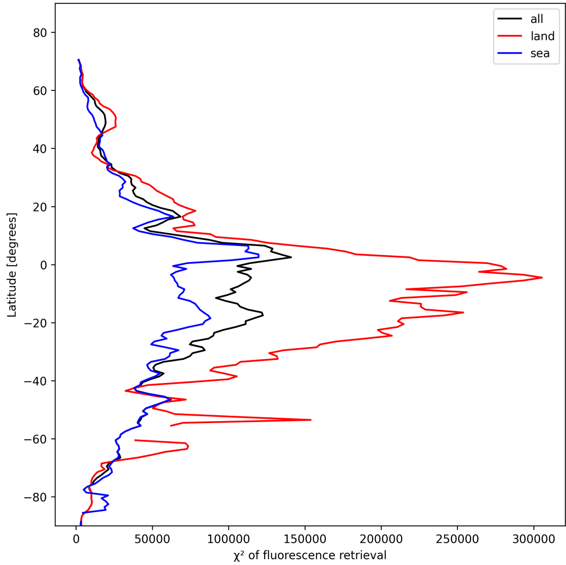
Figure 25: Zonal average of “ \chi^2 of fluorescence retrieval” for 2025-01-28 to 2025-01-30.
