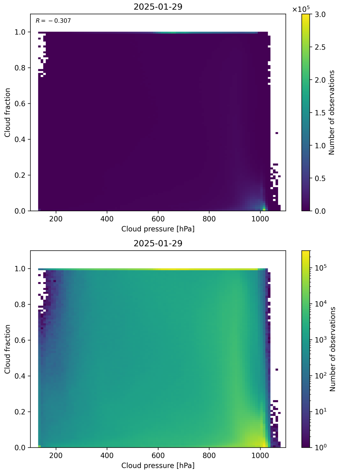
Figure 79: Scatter density plot of “Cloud pressure” against “Cloud fraction” for 2025-01-28 to 2025-01-30.
