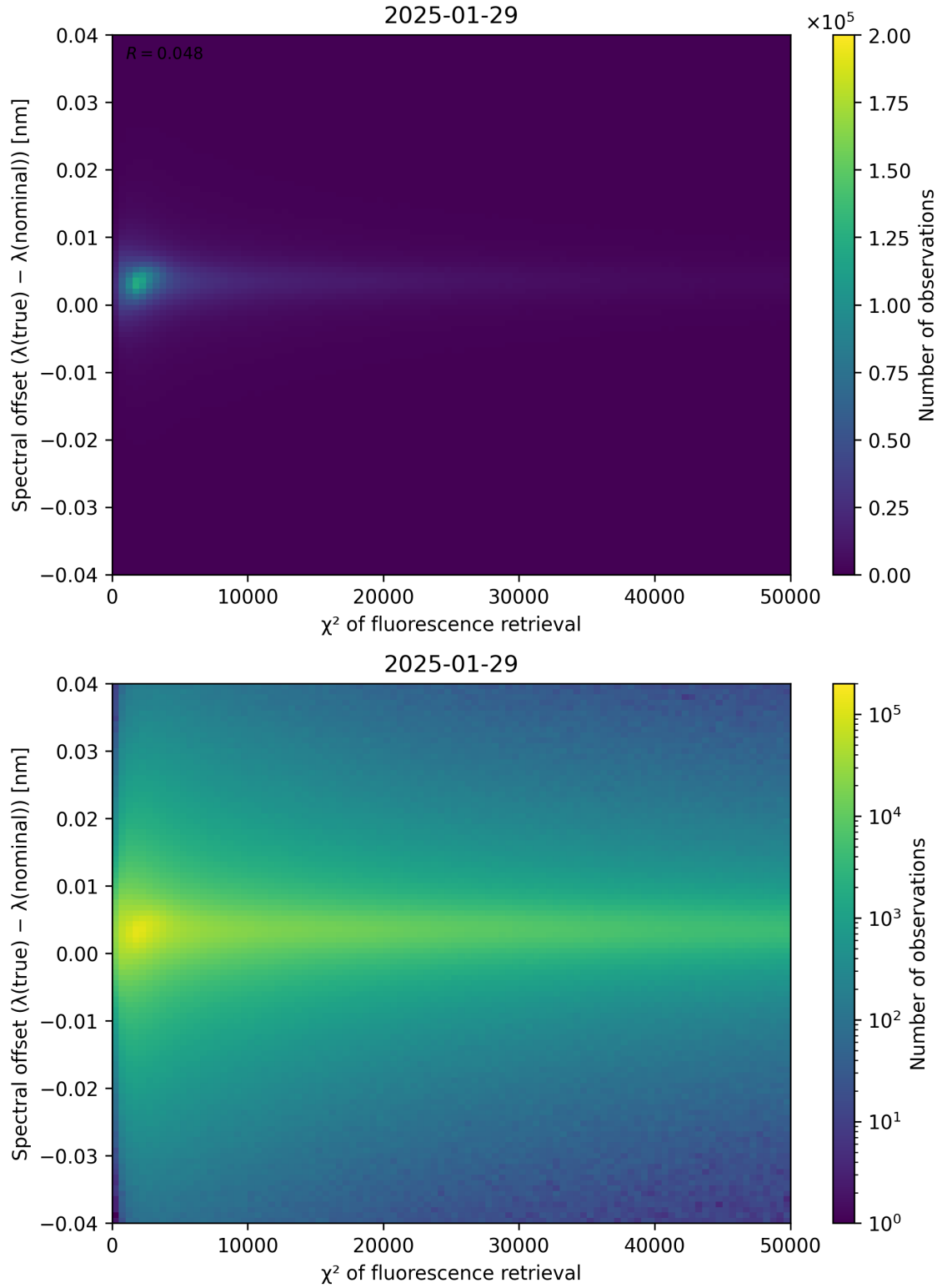
Figure 69: Scatter density plot of “ \chi^2 of fluorescence retrieval” against “Spectral offset ( \lambda_{\text{true}} - \lambda_{\text{nominal}} )” for 2025-01-28 to 2025-01-30.
