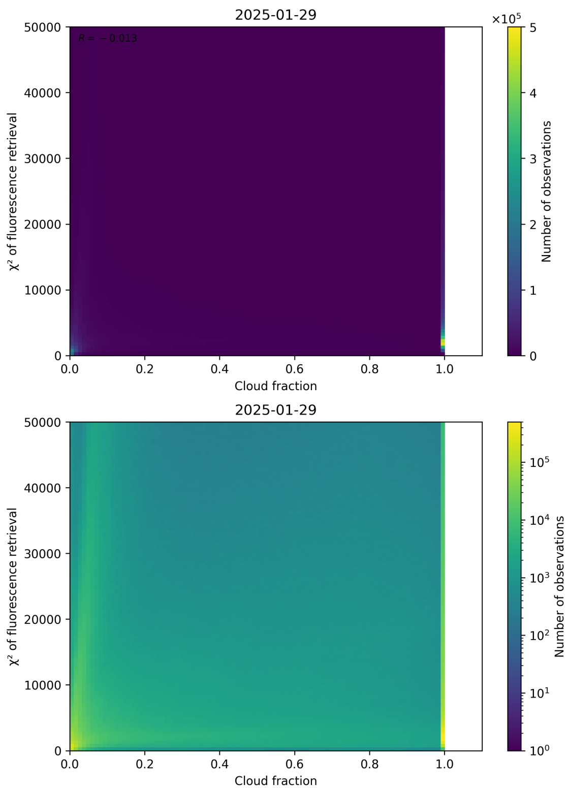
Figure 71: Scatter density plot of “Cloud fraction” against “ \chi^2 of fluorescence retrieval” for 2025-01-28 to 2025-01-30.
