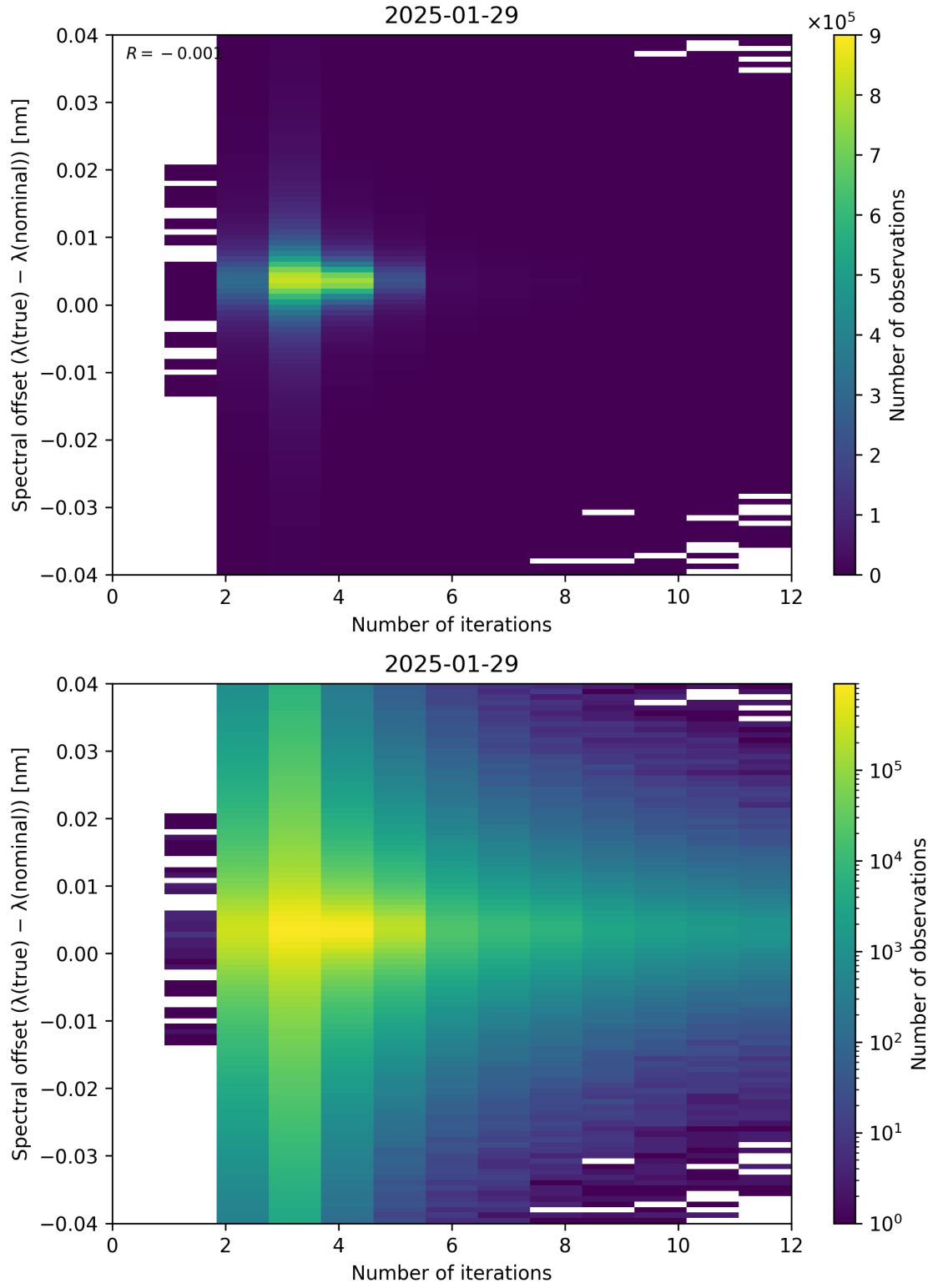
Figure 100: Scatter density plot of “Number of iterations” against “Spectral offset ( \lambda_{\text{true}} - \lambda_{\text{nominal}} )” for 2025-01-28 to 2025-01-30.
