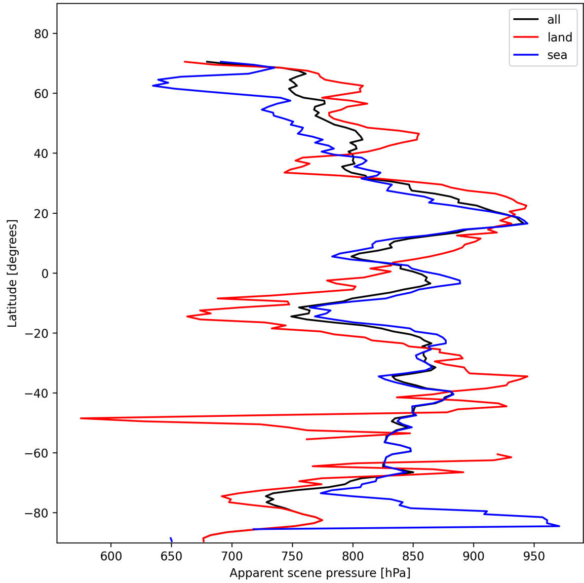
Figure 19: Zonal average of “Apparent scene pressure” for 2025-01-28 to 2025-01-30.
