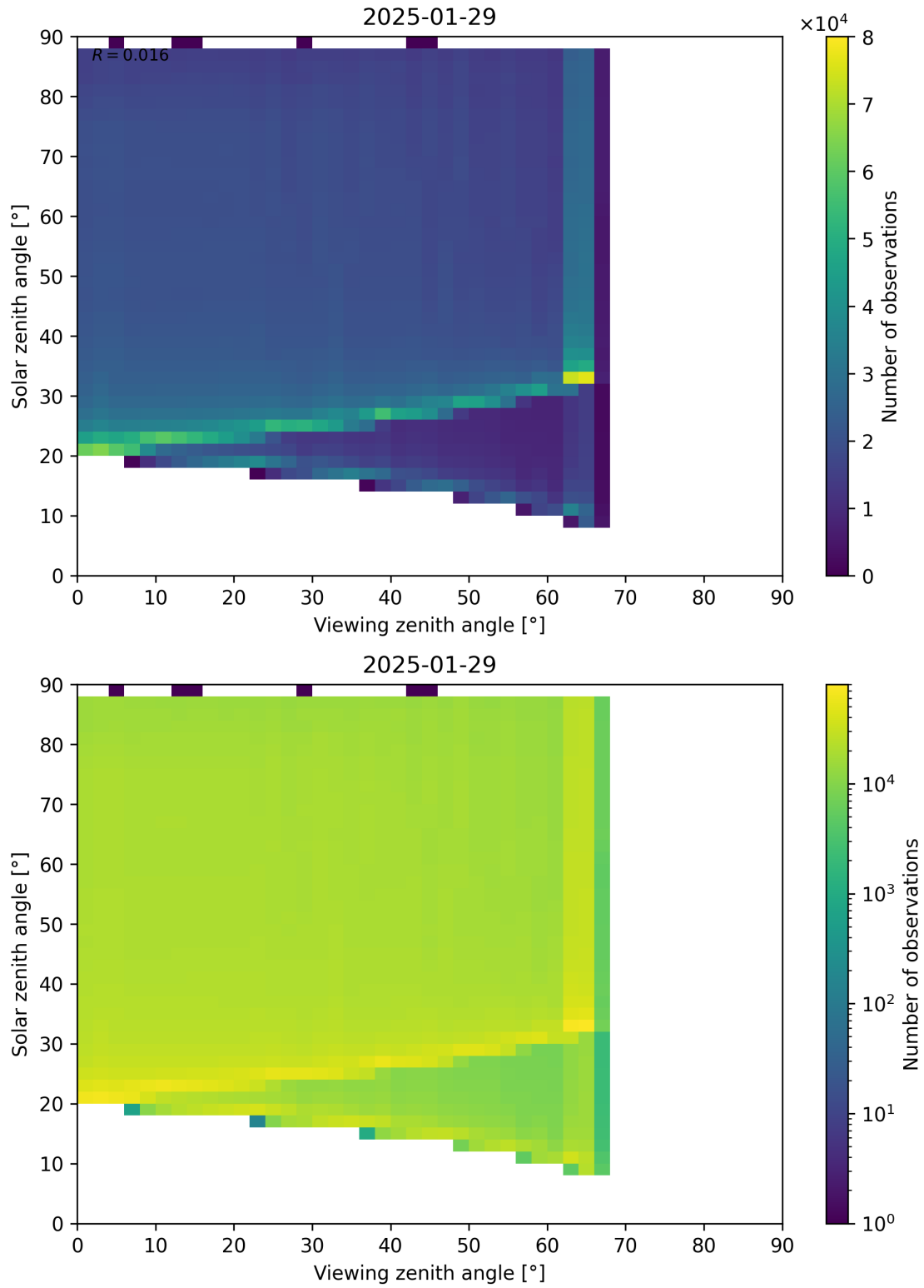
Figure 127: Scatter density plot of “Viewing zenith angle” against “Solar zenith angle” for 2025-01-28 to 2025-01-30.
