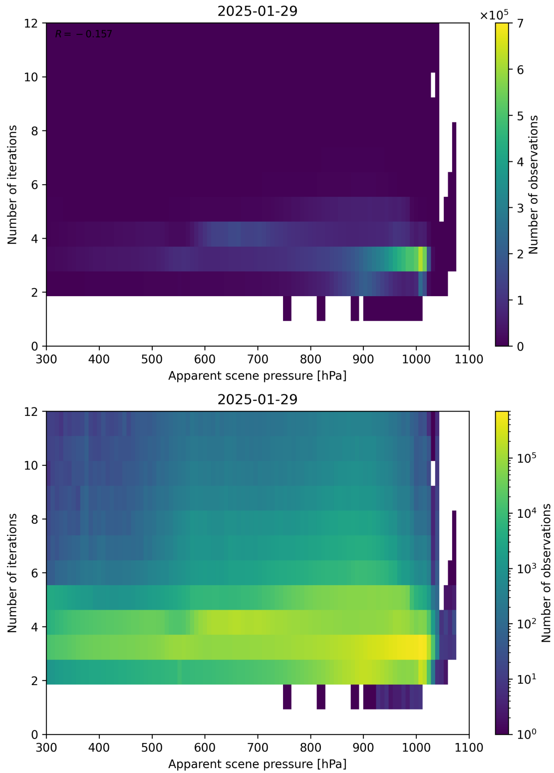
Figure 65: Scatter density plot of “Apparent scene pressure” against “Number of iterations” for 2025-01-28 to 2025-01-30.
