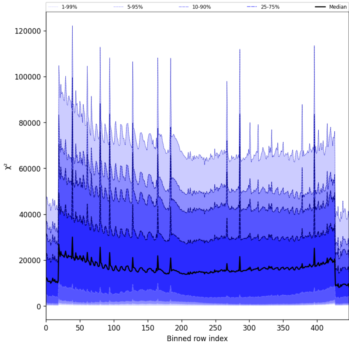
Figure 55: Along track statistics of “ \chi^2 ” for 2025-01-28 to 2025-01-30
