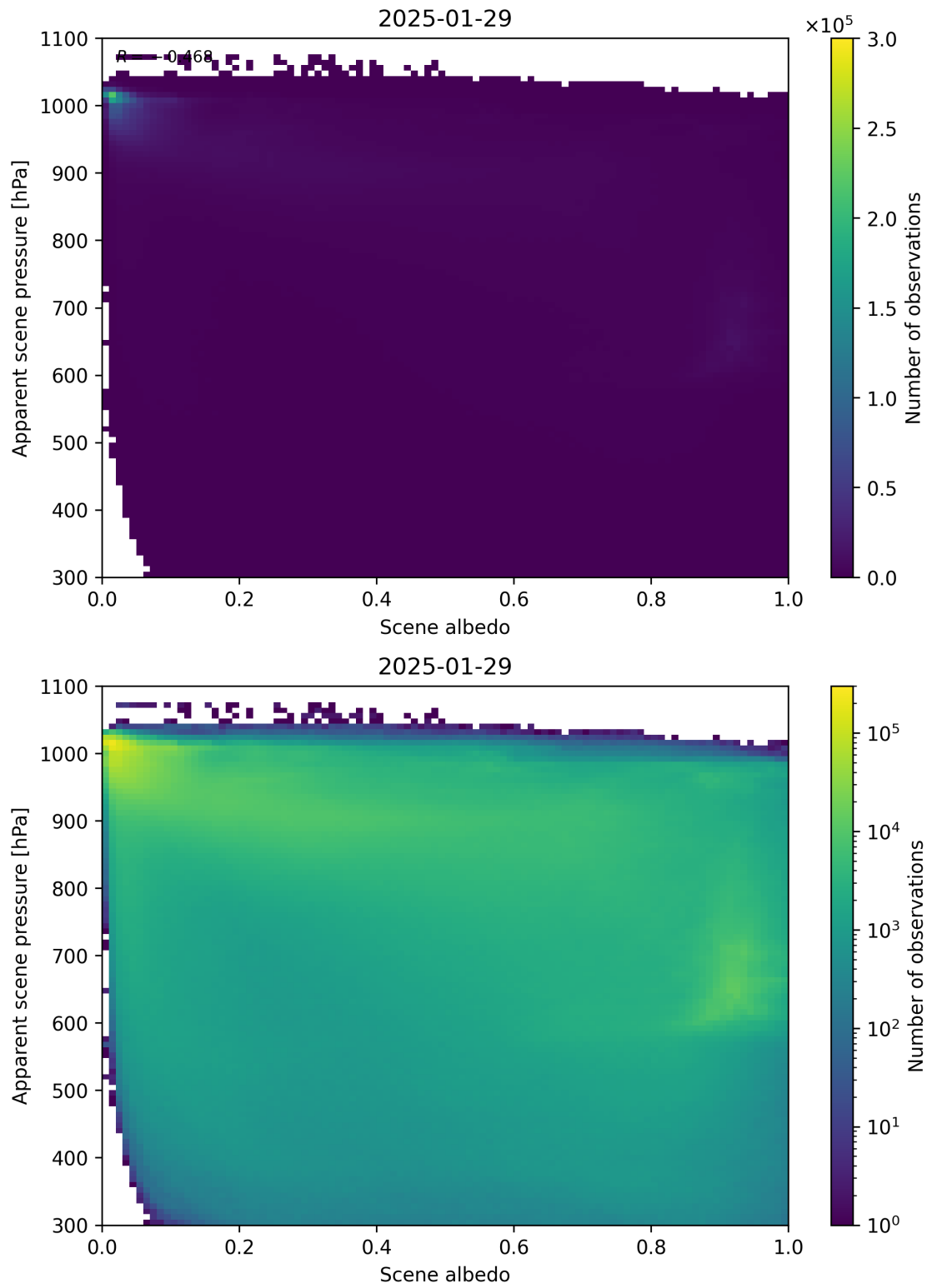
Figure 102: Scatter density plot of “Scene albedo” against “Apparent scene pressure” for 2025-01-28 to 2025-01-30.
