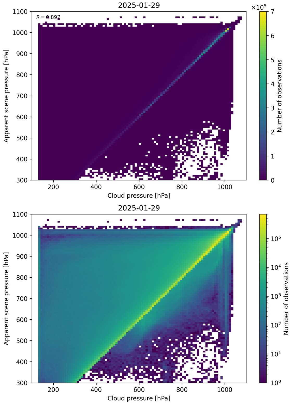
Figure 77: Scatter density plot of “Cloud pressure” against “Apparent scene pressure” for 2025-01-28 to 2025-01-30.
