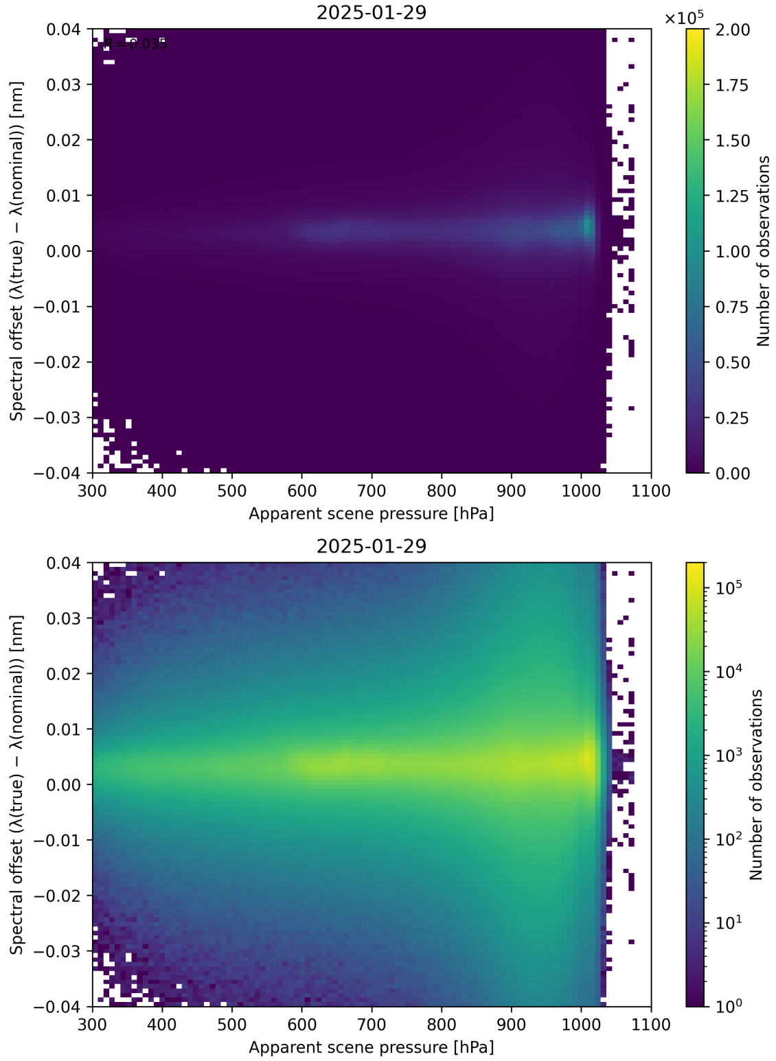
Figure 67: Scatter density plot of “Apparent scene pressure” against “Spectral offset ( \lambda_{\text{true}} - \lambda_{\text{nominal}} )” for 2025-01-28 to 2025-01-30.
