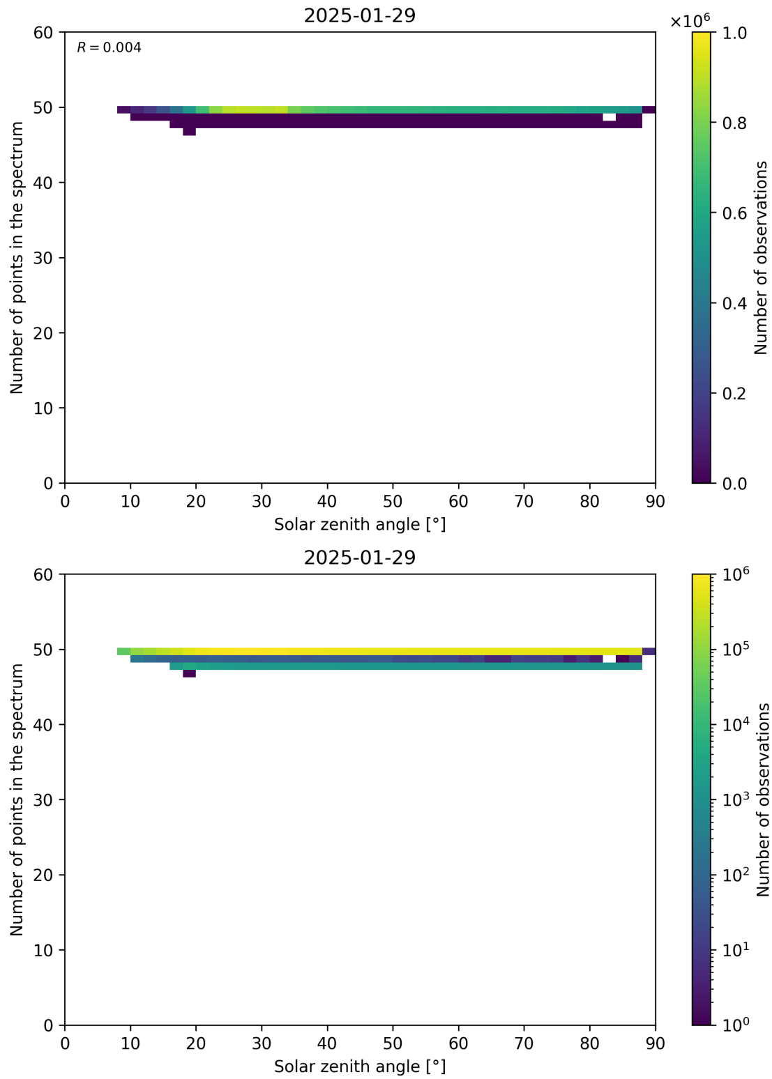
Figure 115: Scatter density plot of “Solar zenith angle” against “Number of points in the spectrum” for 2025-01-28 to 2025-01-30.
