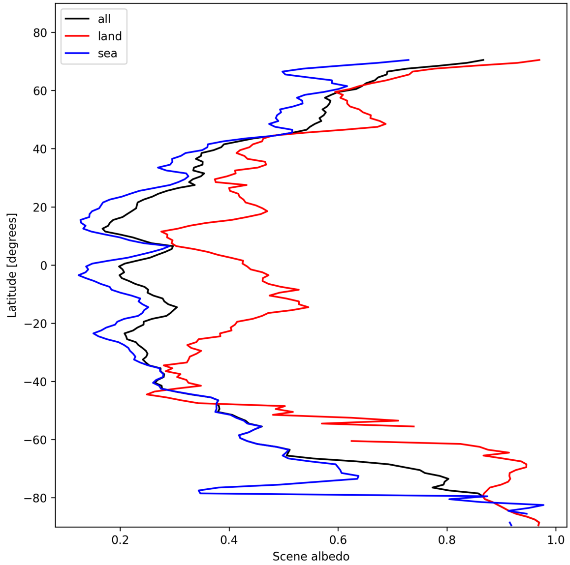
Figure 17: Zonal average of “Scene albedo” for 2025-01-28 to 2025-01-30.
