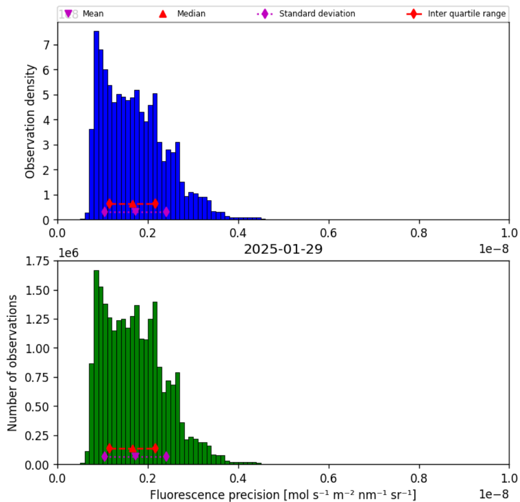
Figure 41: Histogram of “Fluorescence precision” for 2025-01-28 to 2025-01-30
