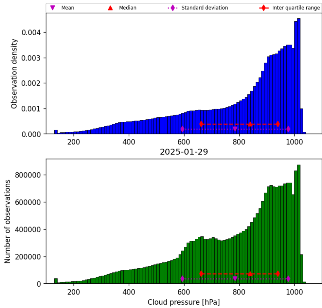
Figure 30: Histogram of “Cloud pressure” for 2025-01-28 to 2025-01-30
