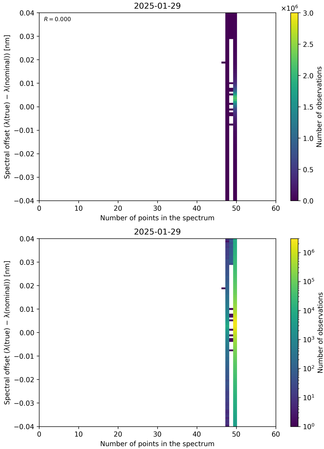
Figure 101: Scatter density plot of “Number of points in the spectrum” against “Spectral offset ( \lambda_{\text{true}} - \lambda_{\text{nominal}} )” for 2025-01-28 to 2025-01-30.
