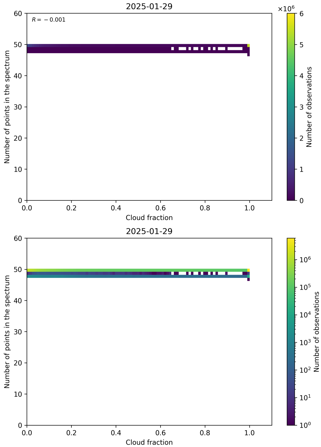
Figure 74: Scatter density plot of “Cloud fraction” against “Number of points in the spectrum” for 2025-01-28 to 2025-01-30.
