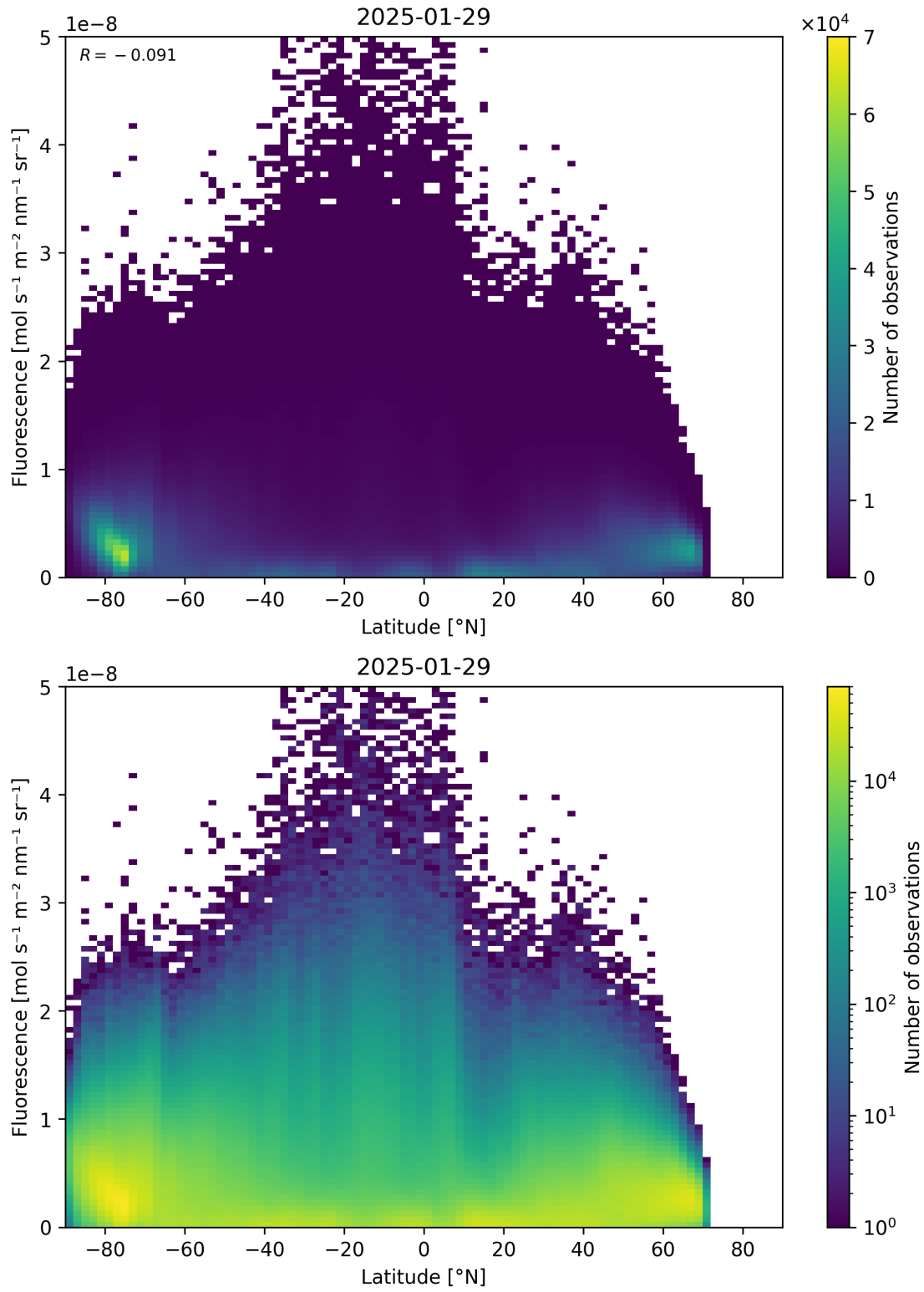
Figure 92: Scatter density plot of “Latitude” against “Fluorescence” for 2025-01-28 to 2025-01-30.
