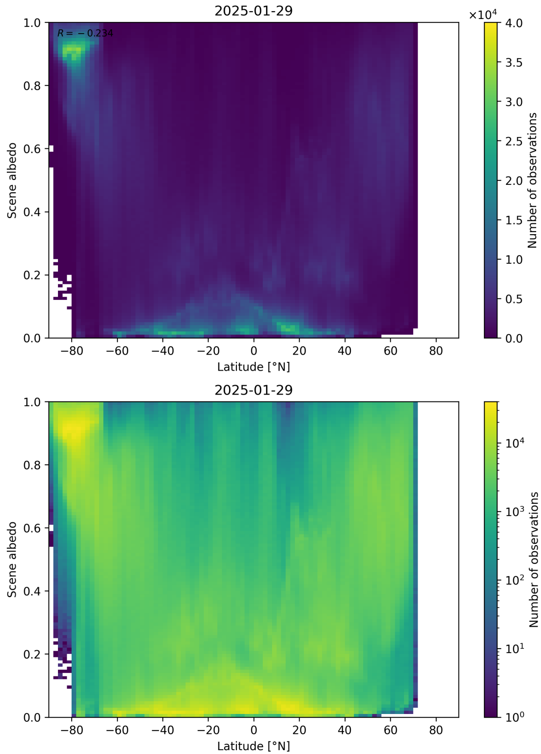
Figure 95: Scatter density plot of “Latitude” against “Scene albedo” for 2025-01-28 to 2025-01-30.
