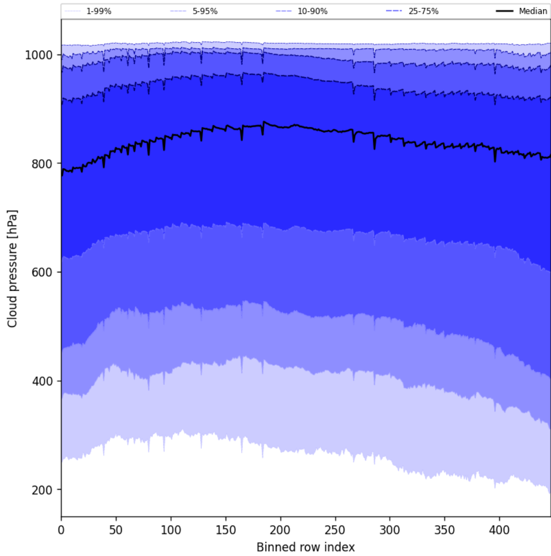
Figure 47: Along track statistics of “Cloud pressure” for 2025-01-28 to 2025-01-30
