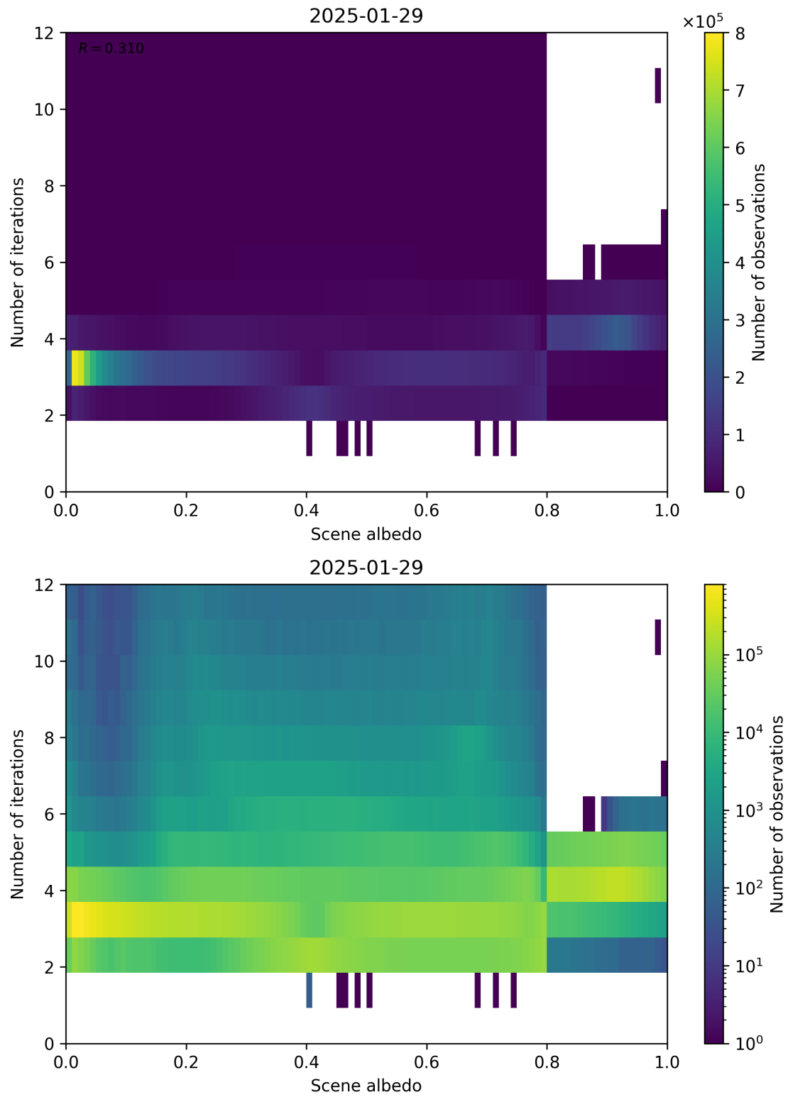
Figure 105: Scatter density plot of “Scene albedo” against “Number of iterations” for 2025-01-28 to 2025-01-30.
