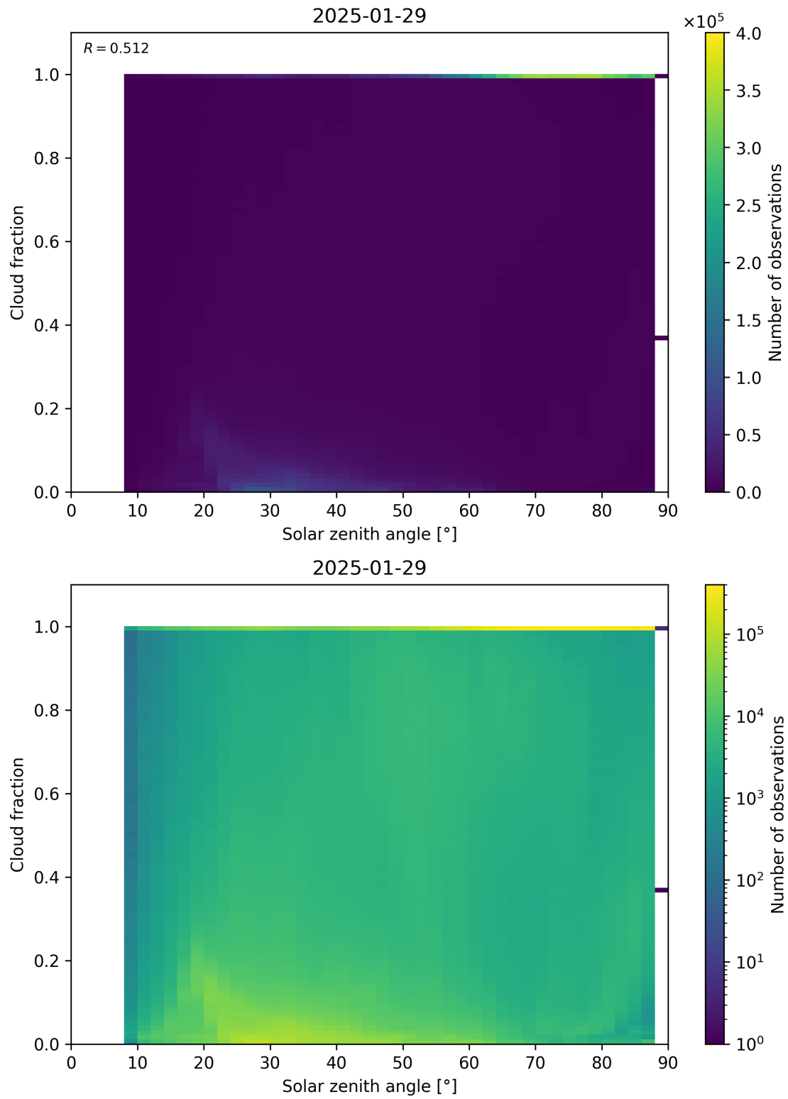
Figure 110: Scatter density plot of “Solar zenith angle” against “Cloud fraction” for 2025-01-28 to 2025-01-30.
