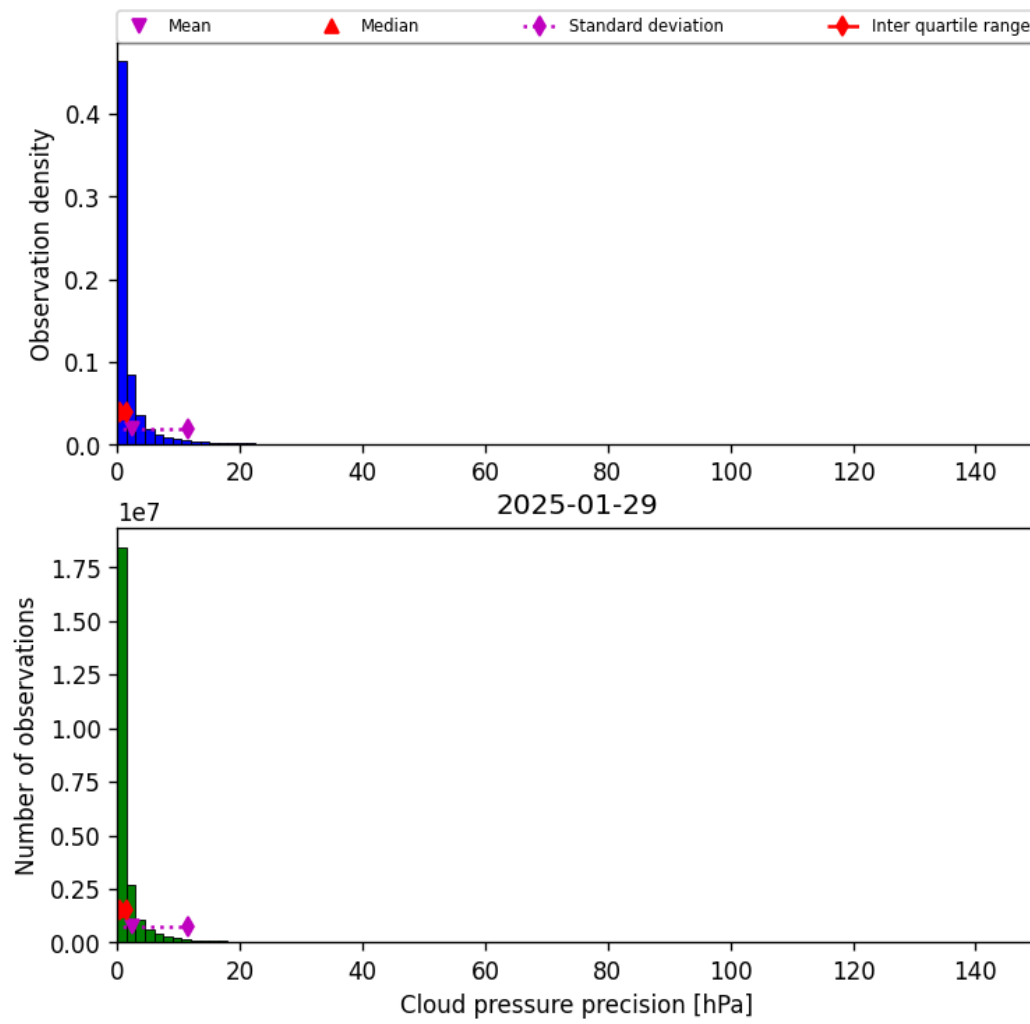
Figure 31: Histogram of “Cloud pressure precision” for 2025-01-28 to 2025-01-30
