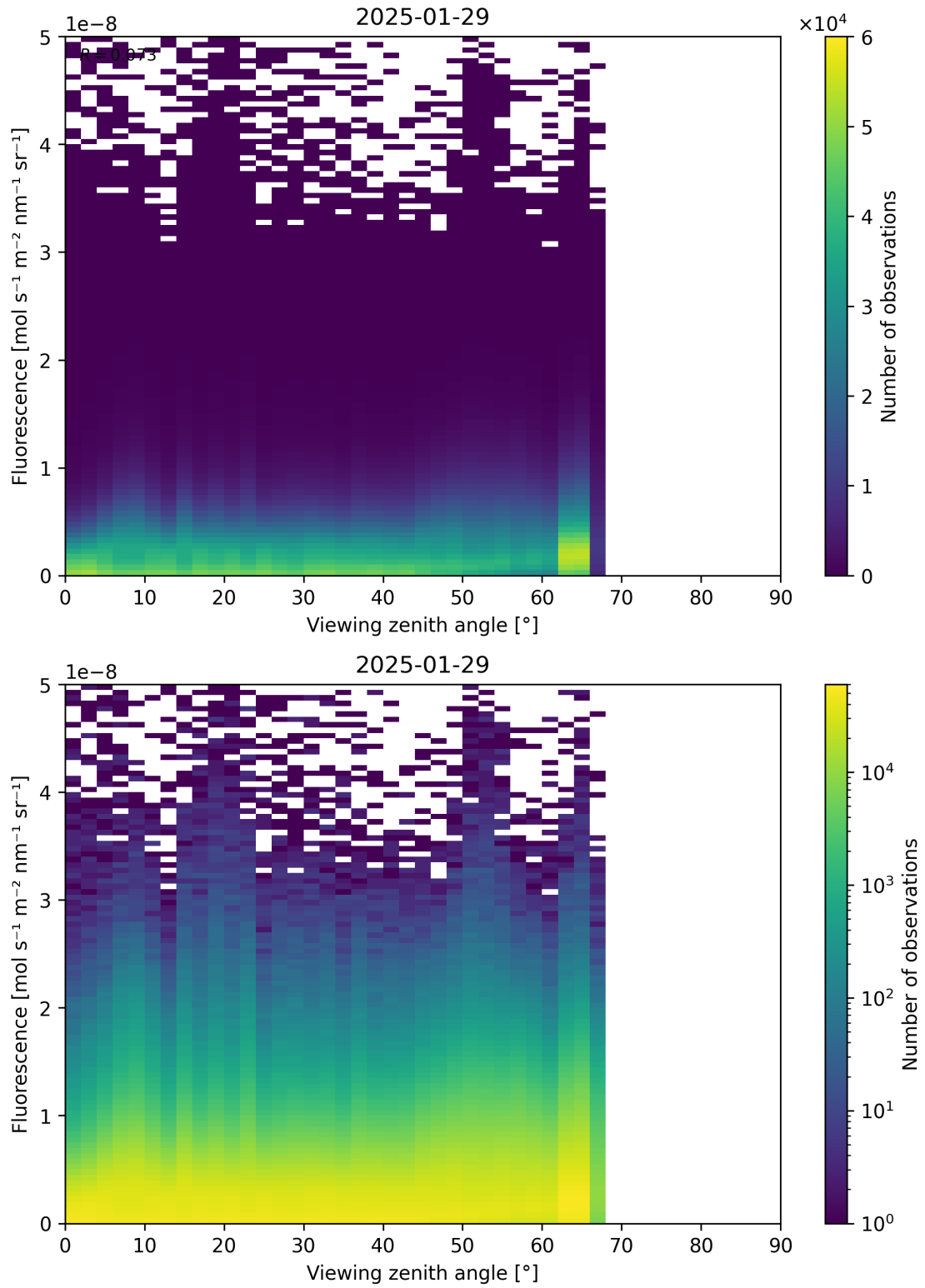
Figure 122: Scatter density plot of “Viewing zenith angle” against “Fluorescence” for 2025-01-28 to 2025-01-30.
