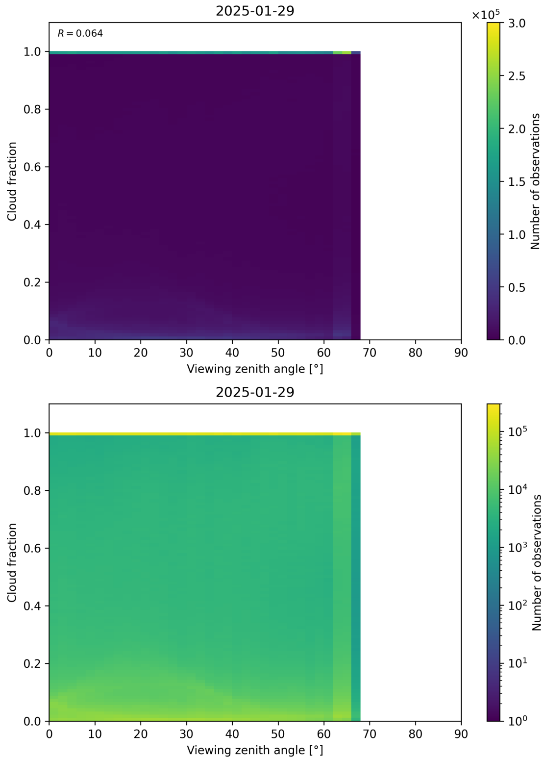
Figure 120: Scatter density plot of “Viewing zenith angle” against “Cloud fraction” for 2025-01-28 to 2025-01-30.
