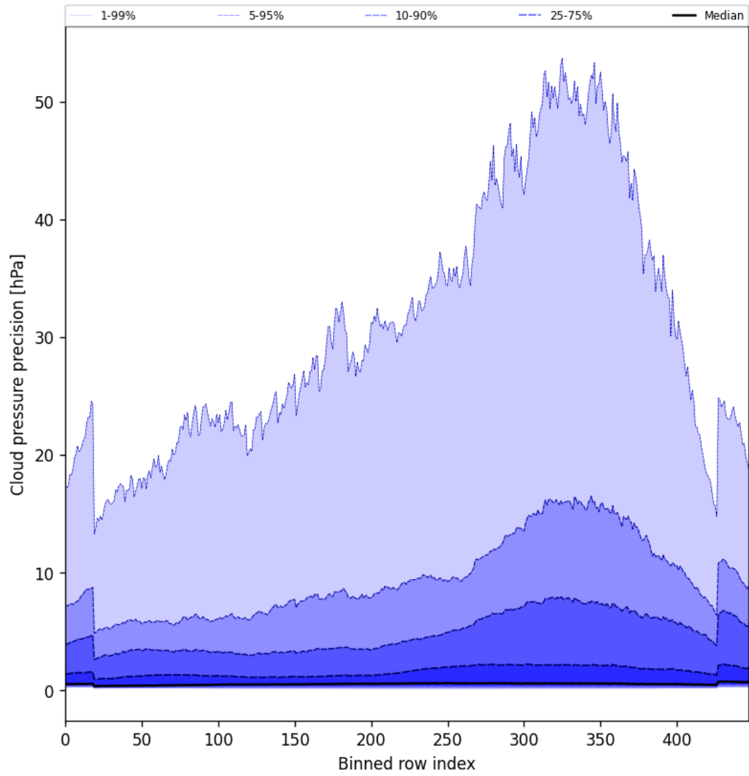
Figure 48: Along track statistics of “Cloud pressure precision” for 2025-01-28 to 2025-01-30
