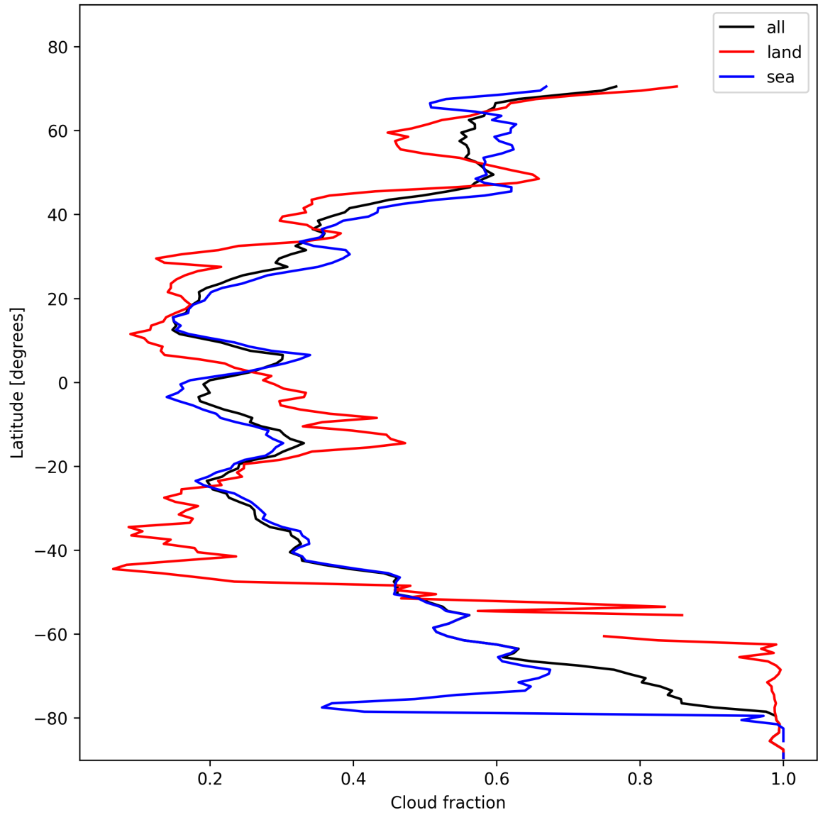
Figure 15: Zonal average of “Cloud fraction” for 2025-01-28 to 2025-01-30.
