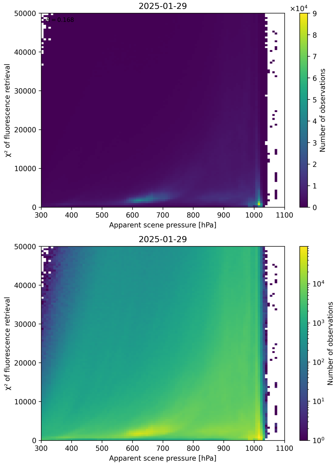
Figure 63: Scatter density plot of “Apparent scene pressure” against “ \chi^2 of fluorescence retrieval” for 2025-01-28 to 2025-01-30.
