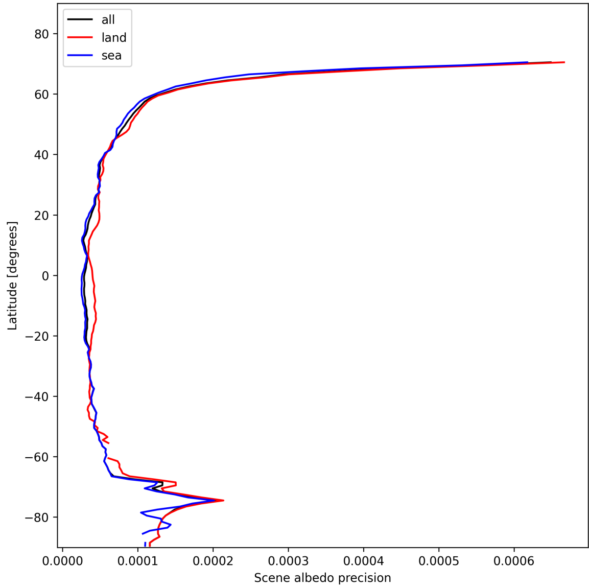
Figure 18: Zonal average of “Scene albedo precision” for 2025-01-28 to 2025-01-30.
