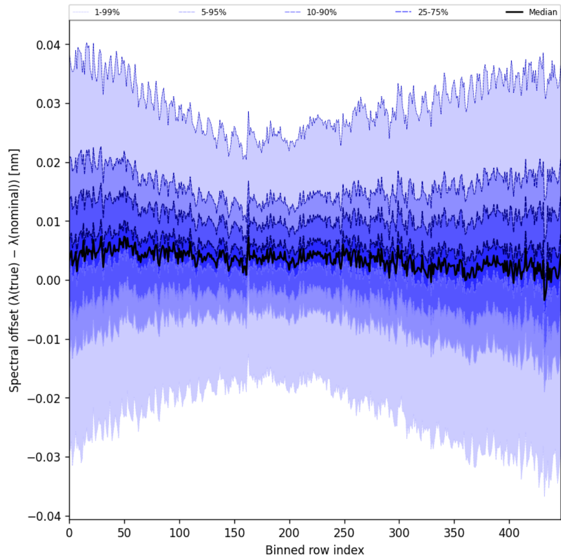
Figure 62: Along track statistics of “Spectral offset ( \lambda_{\text{true}} - \lambda_{\text{nominal}} )” for 2025-01-28 to 2025-01-30
