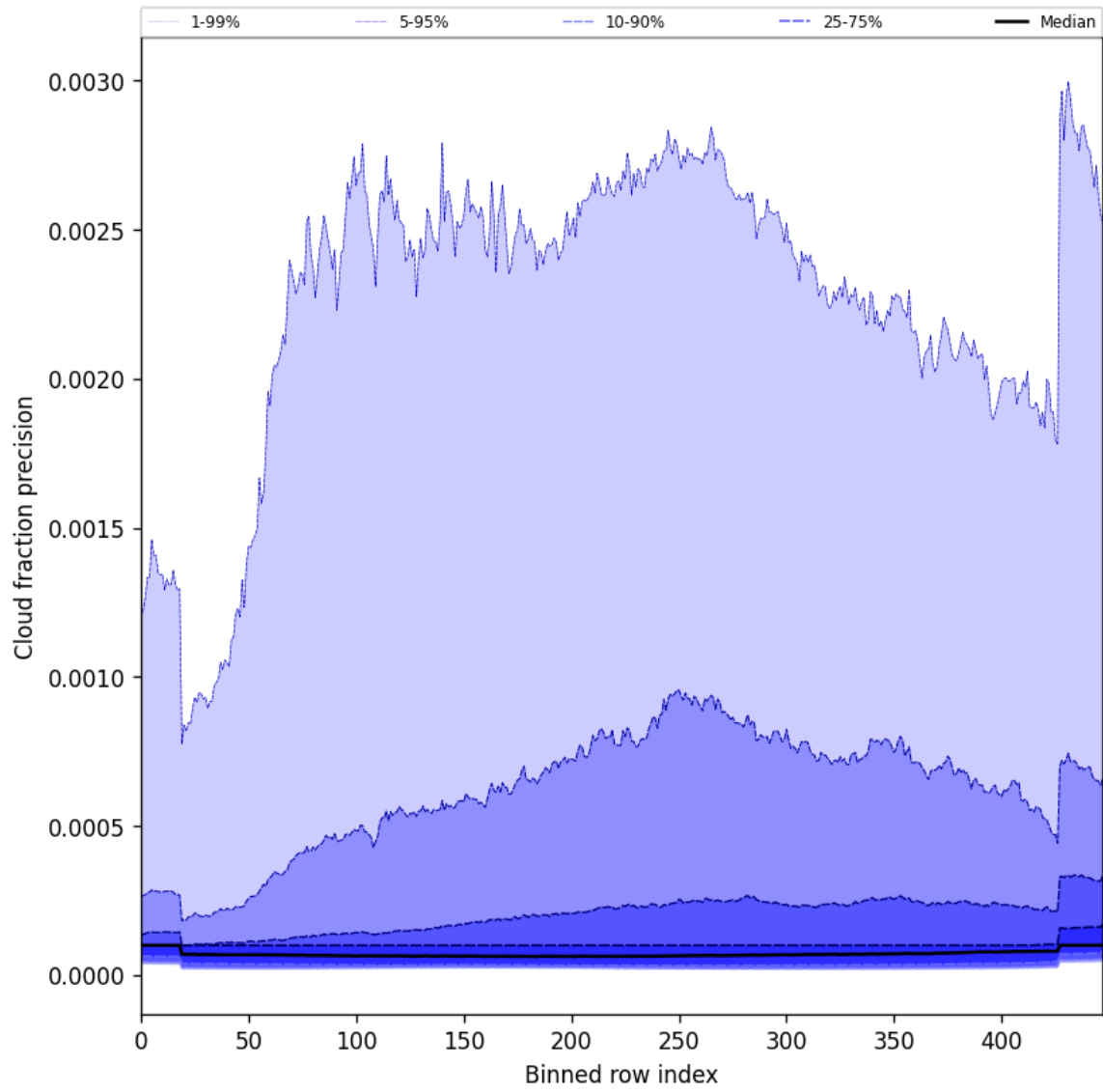
Figure 50: Along track statistics of “Cloud fraction precision” for 2025-01-28 to 2025-01-30
