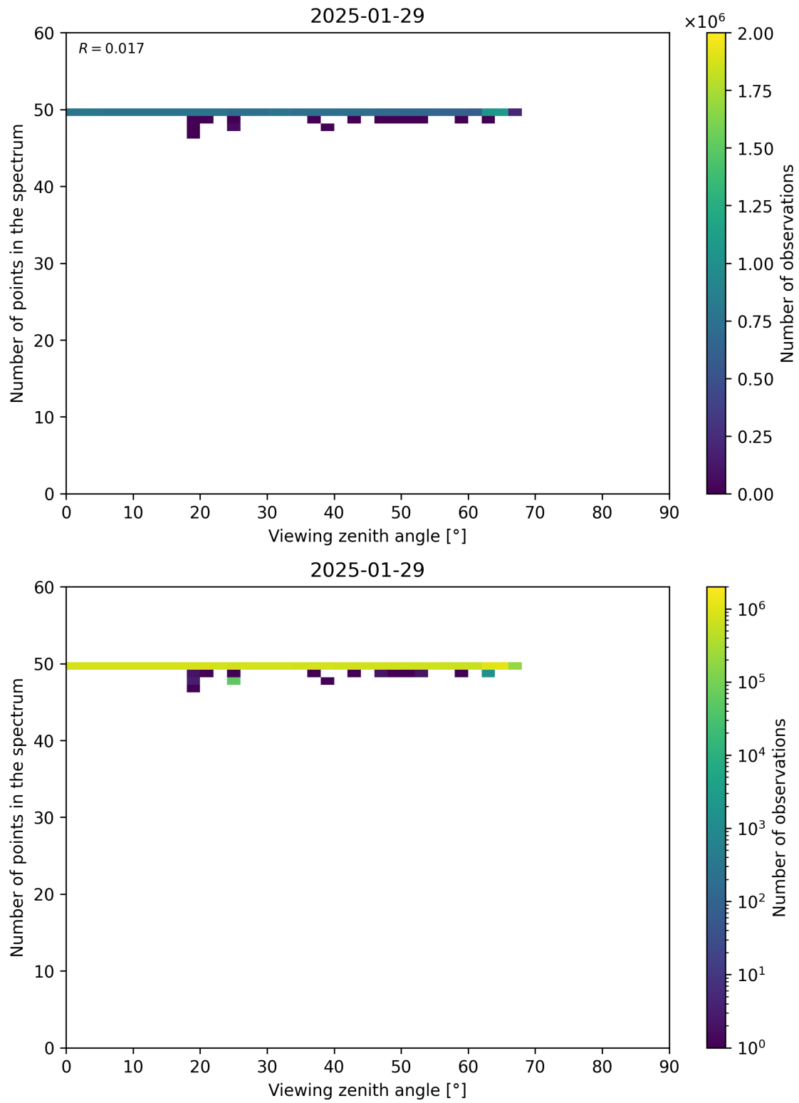
Figure 125: Scatter density plot of “Viewing zenith angle” against “Number of points in the spectrum” for 2025-01-28 to 2025-01-30.
