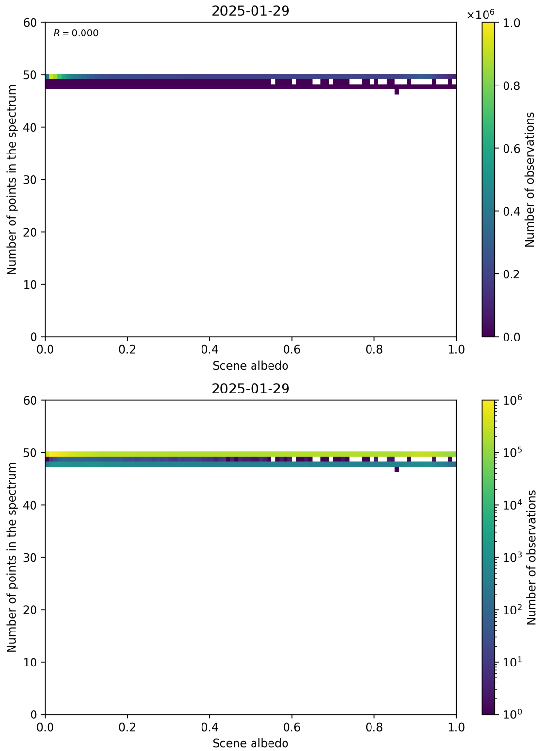
Figure 106: Scatter density plot of “Scene albedo” against “Number of points in the spectrum” for 2025-01-28 to 2025-01-30.
