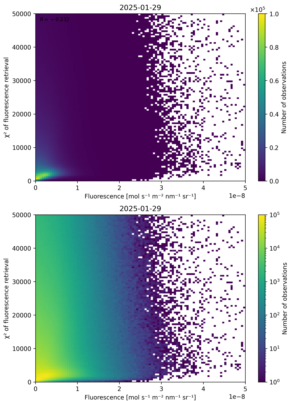
Figure 85: Scatter density plot of “Fluorescence” against “ \chi^2 of fluorescence retrieval” for 2025-01-28 to 2025-01-30.
