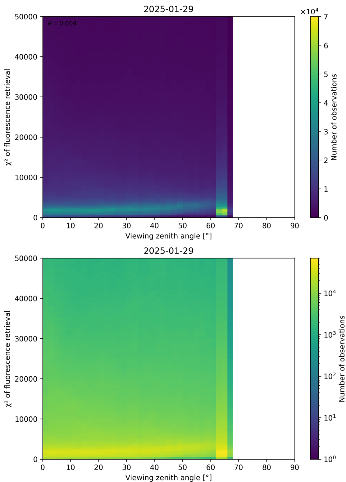
Figure 119: Scatter density plot of “Viewing zenith angle” against “ \chi^2 of fluorescence retrieval” for 2025-01-28 to 2025-01-30.
