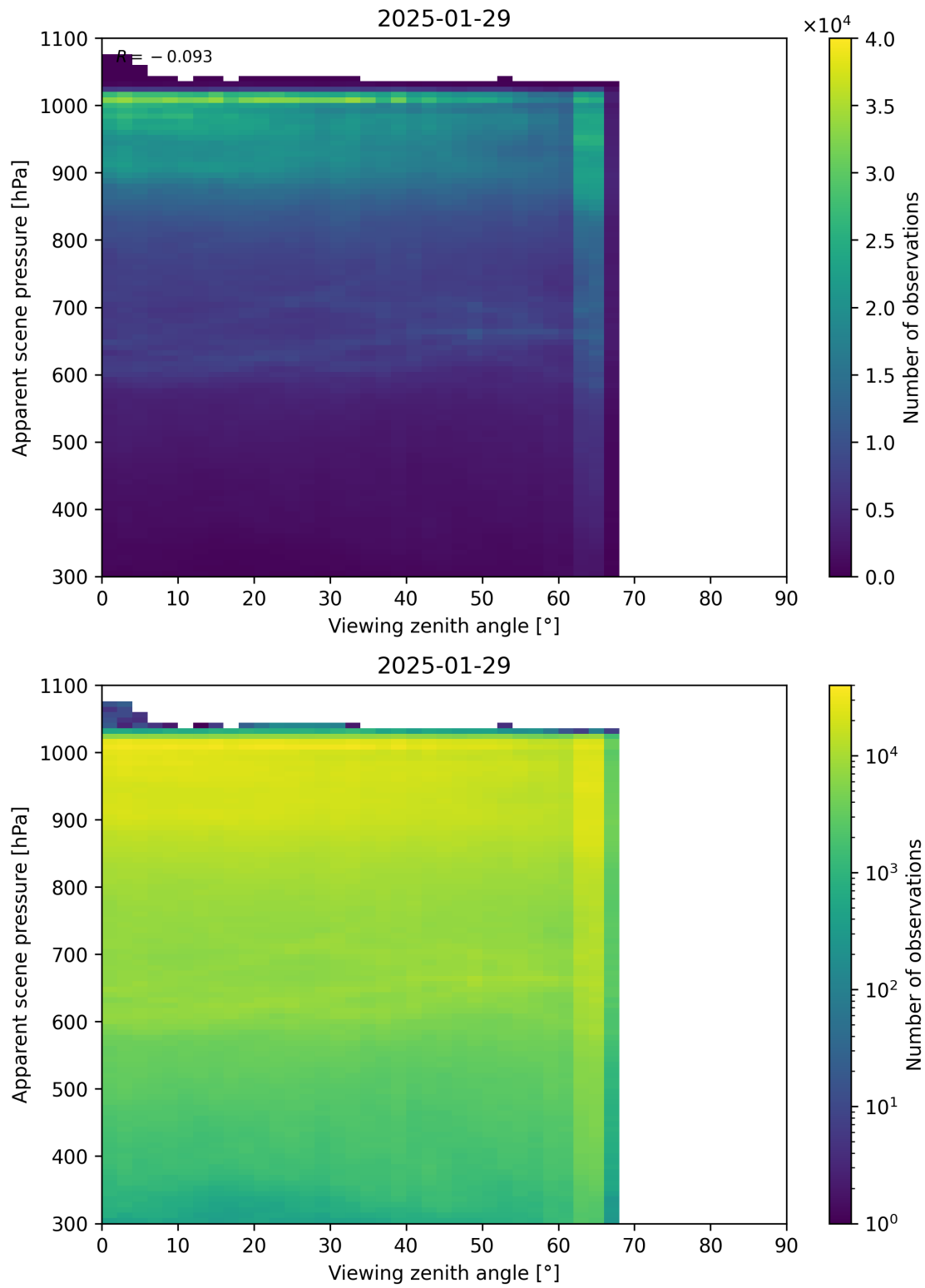
Figure 118: Scatter density plot of “Viewing zenith angle” against “Apparent scene pressure” for 2025-01-28 to 2025-01-30.
