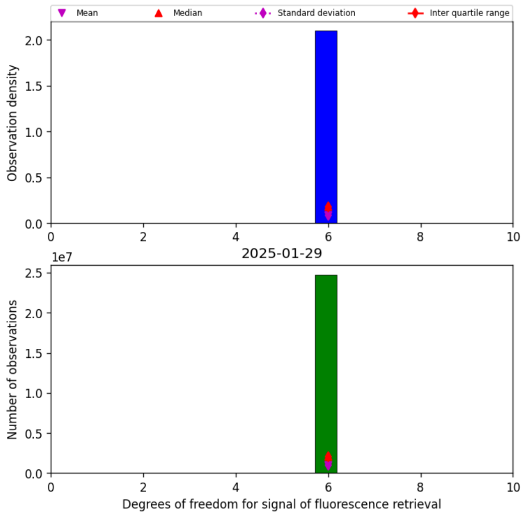
Figure 43: Histogram of "Degrees of freedom for signal of fluorescence retrieval" for 2025-01-28 to 2025-01-30
