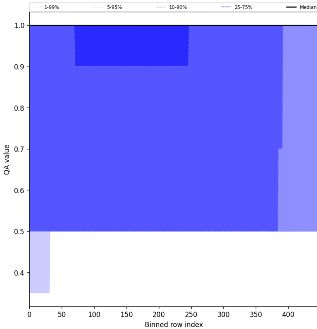
Figure 46: Along track statistics of “QA value” for 2025-01-28 to 2025-01-30
