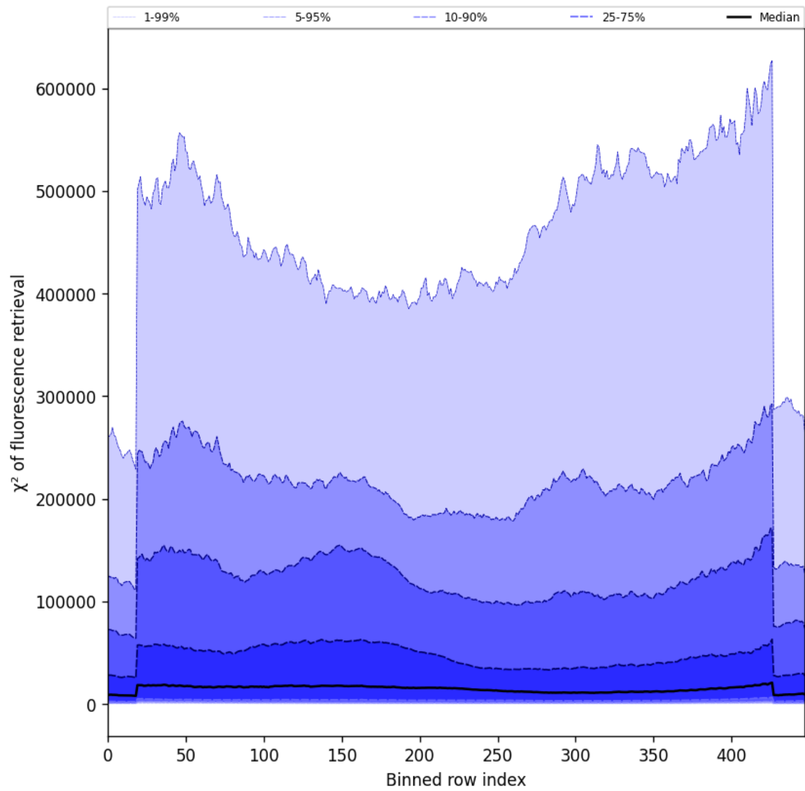
Figure 59: Along track statistics of “ \chi^2 of fluorescence retrieval” for 2025-01-28 to 2025-01-30
