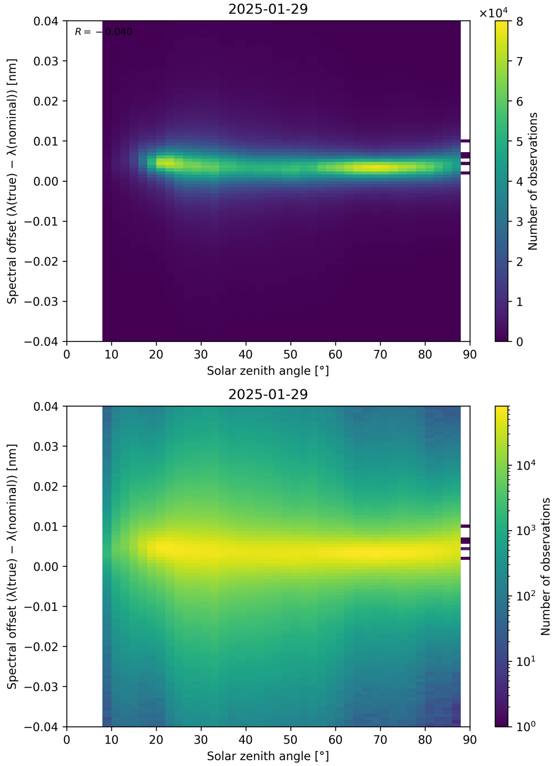
Figure 117: Scatter density plot of “Solar zenith angle” against “Spectral offset ( \lambda_{\text{true}} - \lambda_{\text{nominal}} )” for 2025-01-28 to 2025-01-30.
