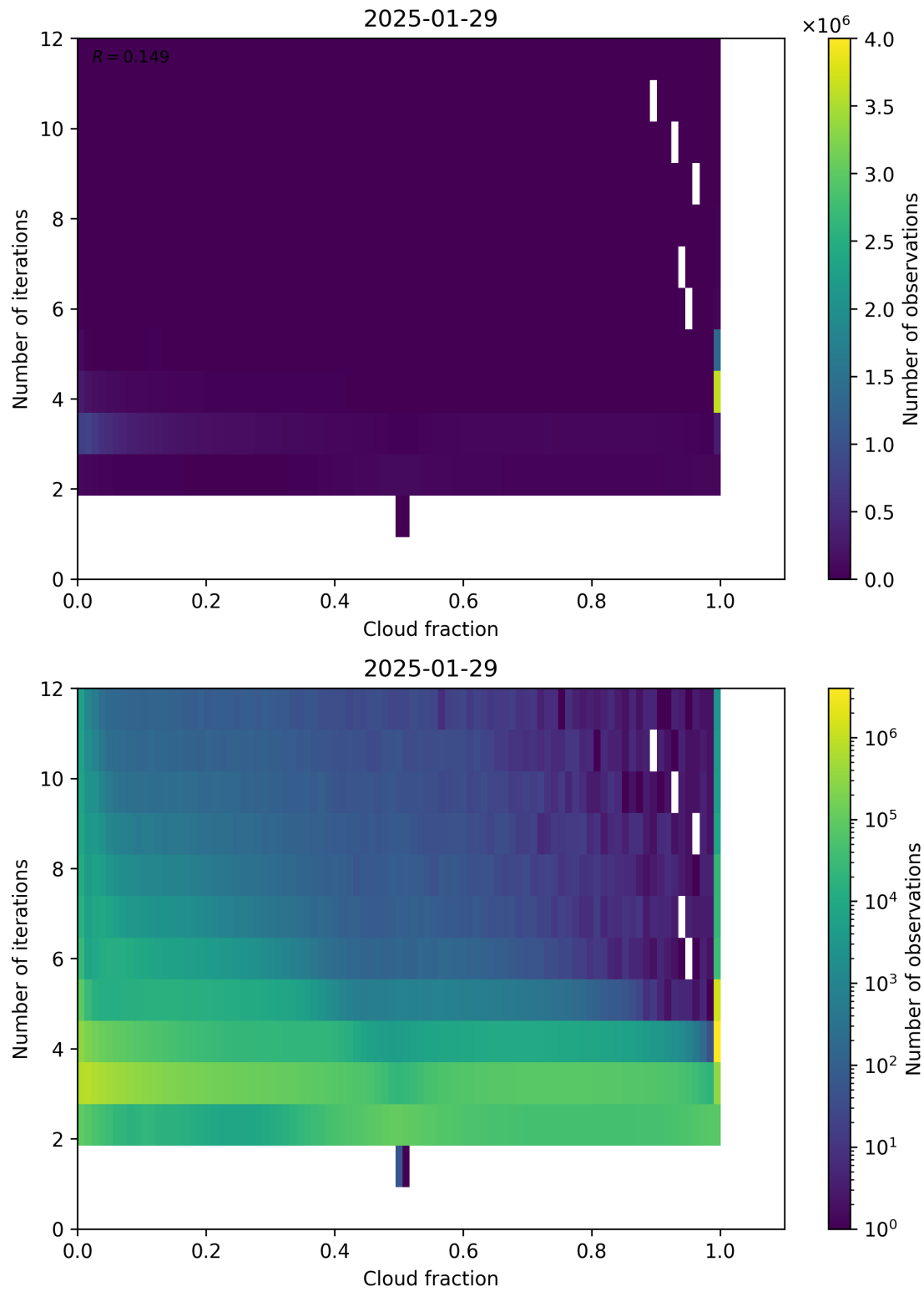
Figure 73: Scatter density plot of “Cloud fraction” against “Number of iterations” for 2025-01-28 to 2025-01-30.
