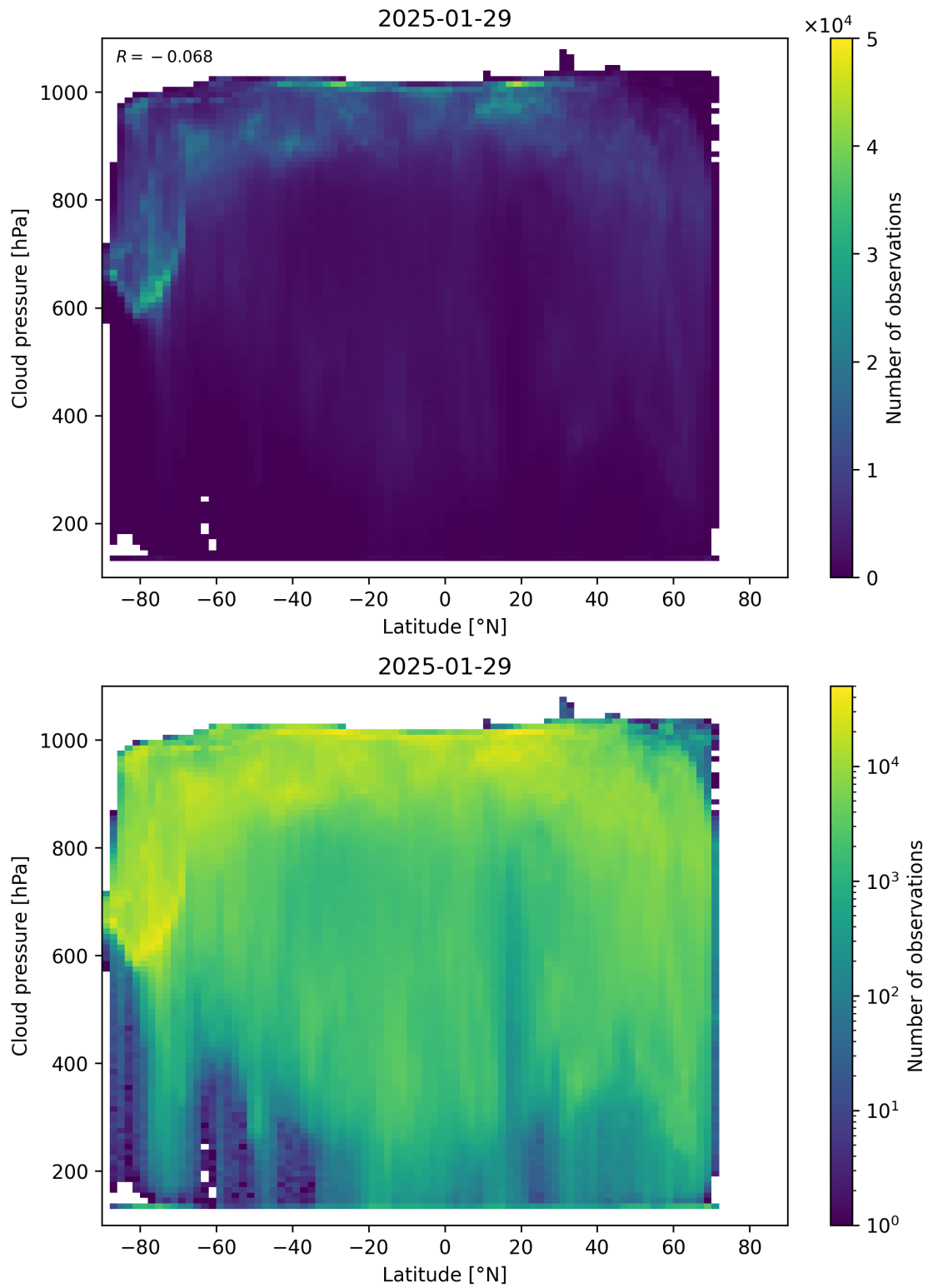
Figure 91: Scatter density plot of “Latitude” against “Cloud pressure” for 2025-01-28 to 2025-01-30.
