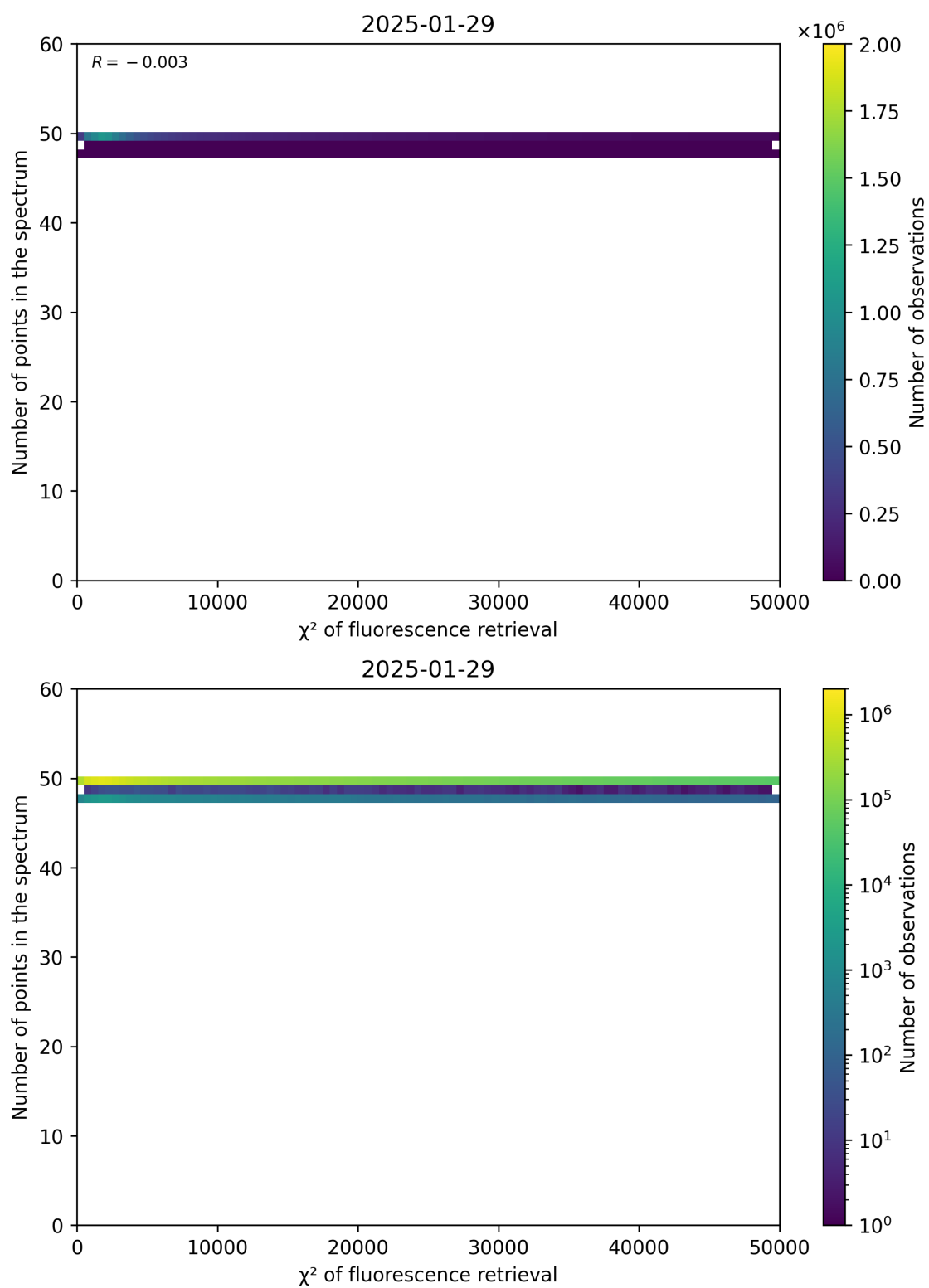
Figure 68: Scatter density plot of “ \chi^2 of fluorescence retrieval” against “Number of points in the spectrum” for 2025-01-28 to 2025-01-30.
