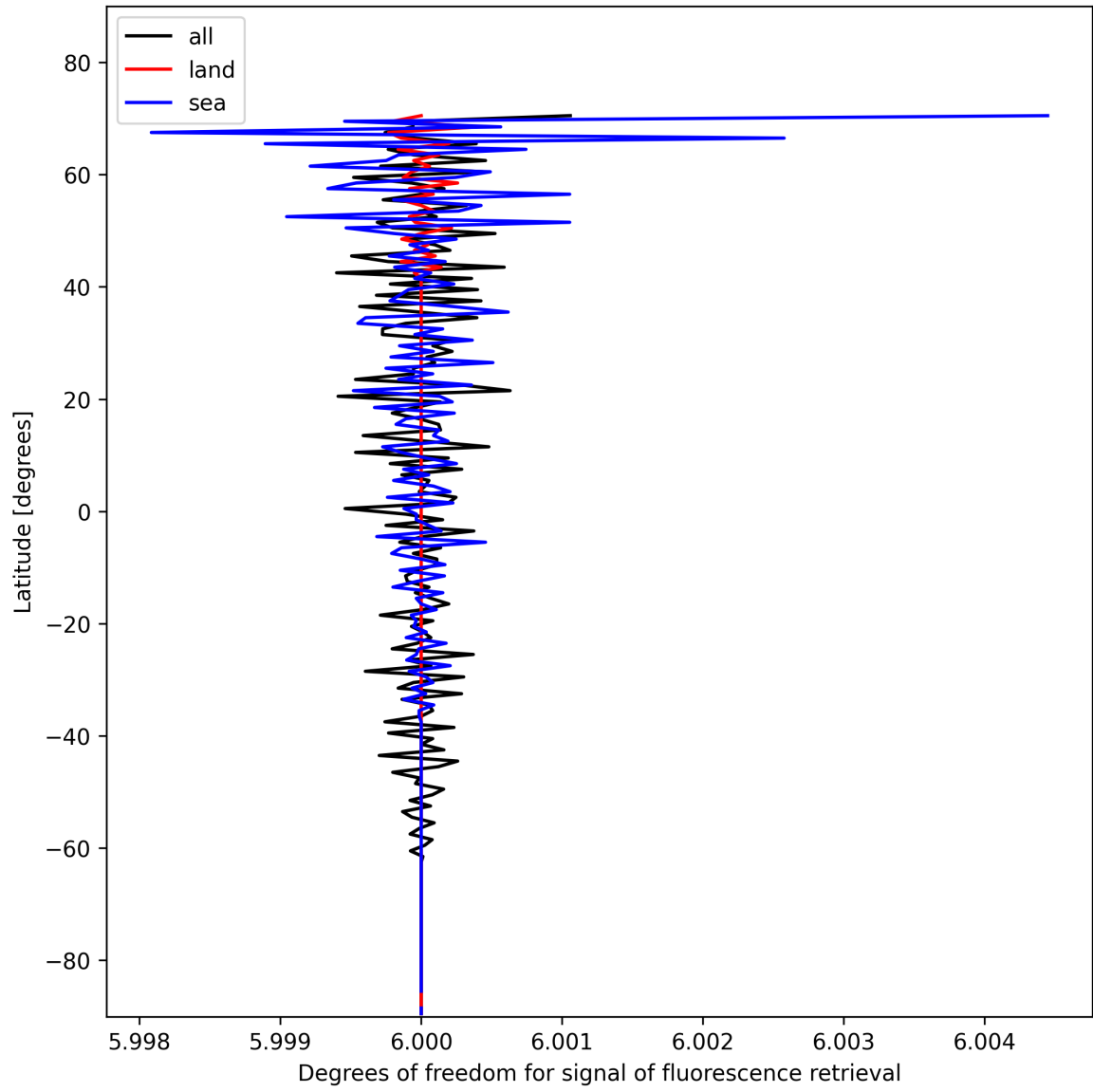
Figure 26: Zonal average of “Degrees of freedom for signal of fluorescence retrieval” for 2025-01-28 to 2025-01-30.
