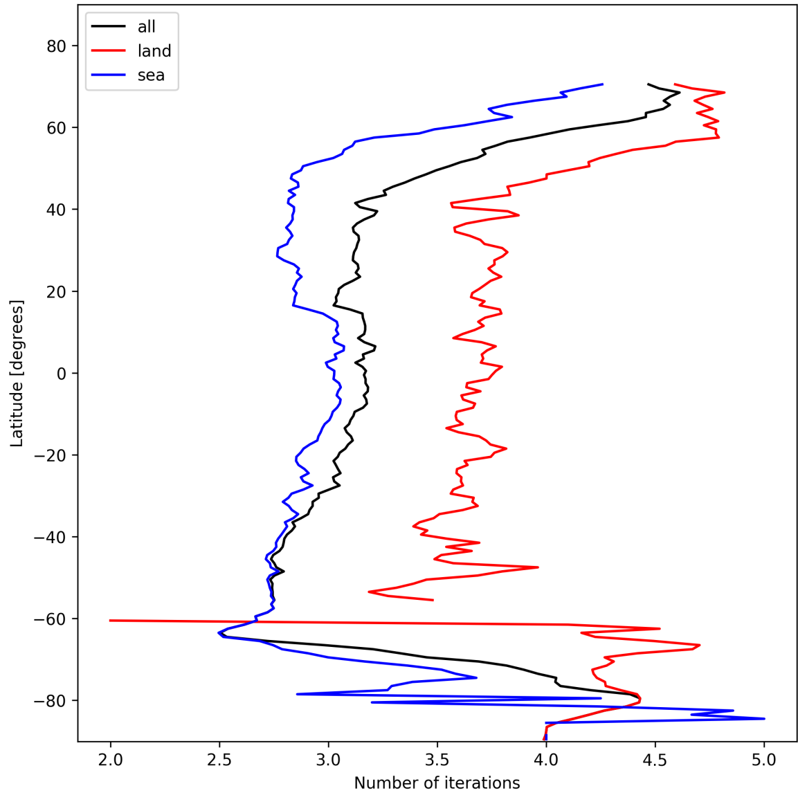
Figure 22: Zonal average of “Number of iterations” for 2025-01-28 to 2025-01-30.
