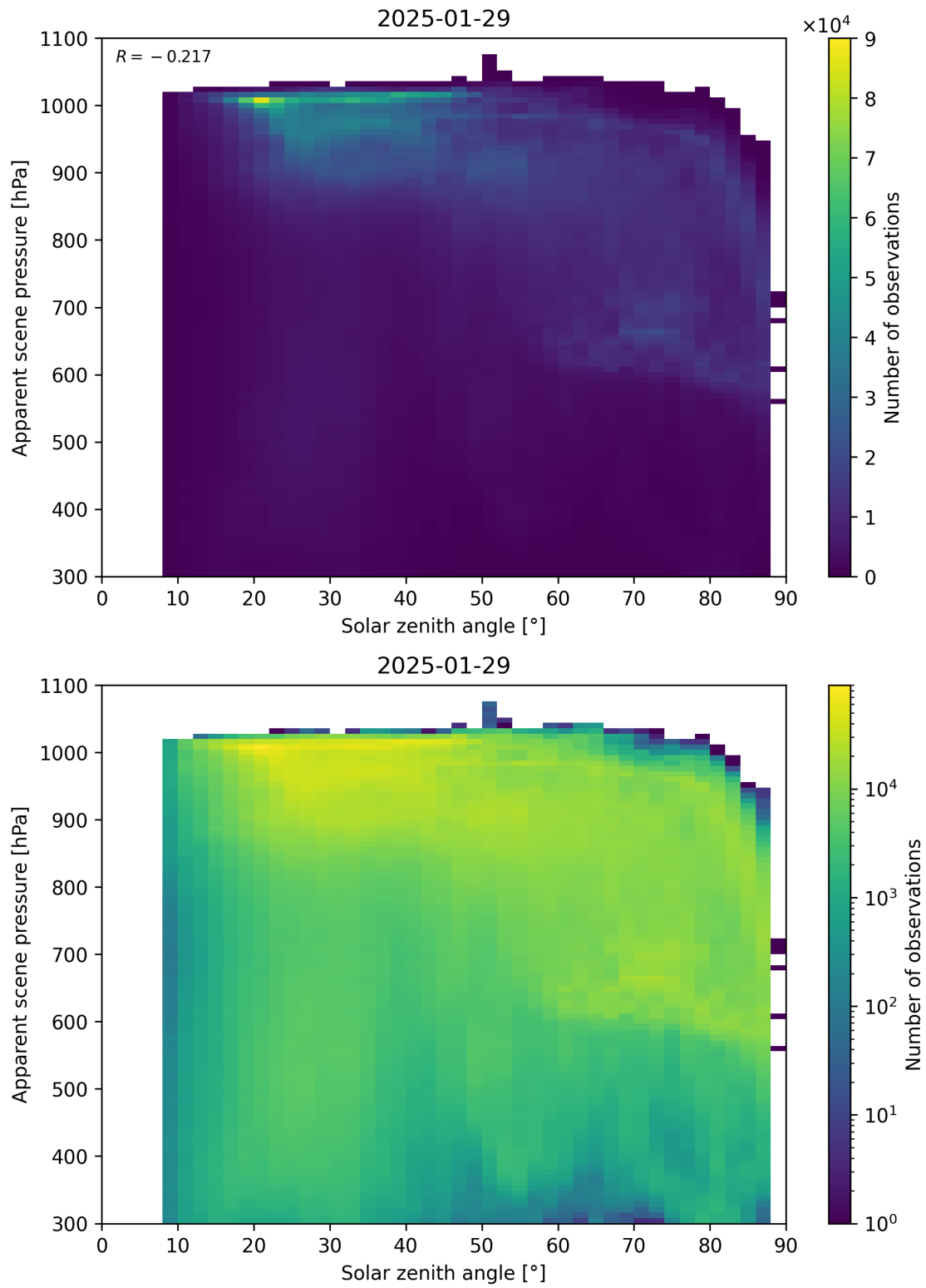
Figure 108: Scatter density plot of “Solar zenith angle” against “Apparent scene pressure” for 2025-01-28 to 2025-01-30.
