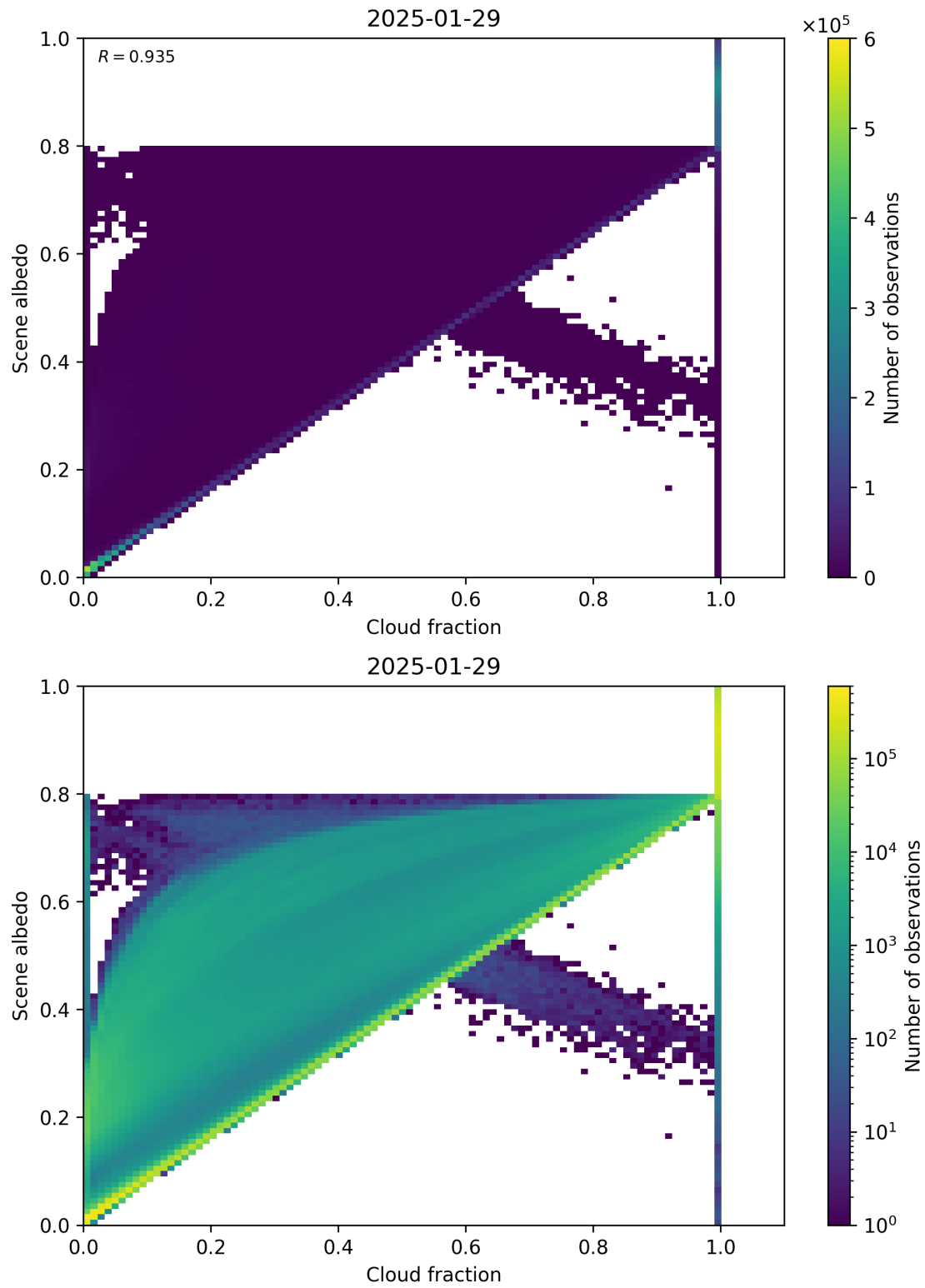
Figure 75: Scatter density plot of “Cloud fraction” against “Scene albedo” for 2025-01-28 to 2025-01-30.
