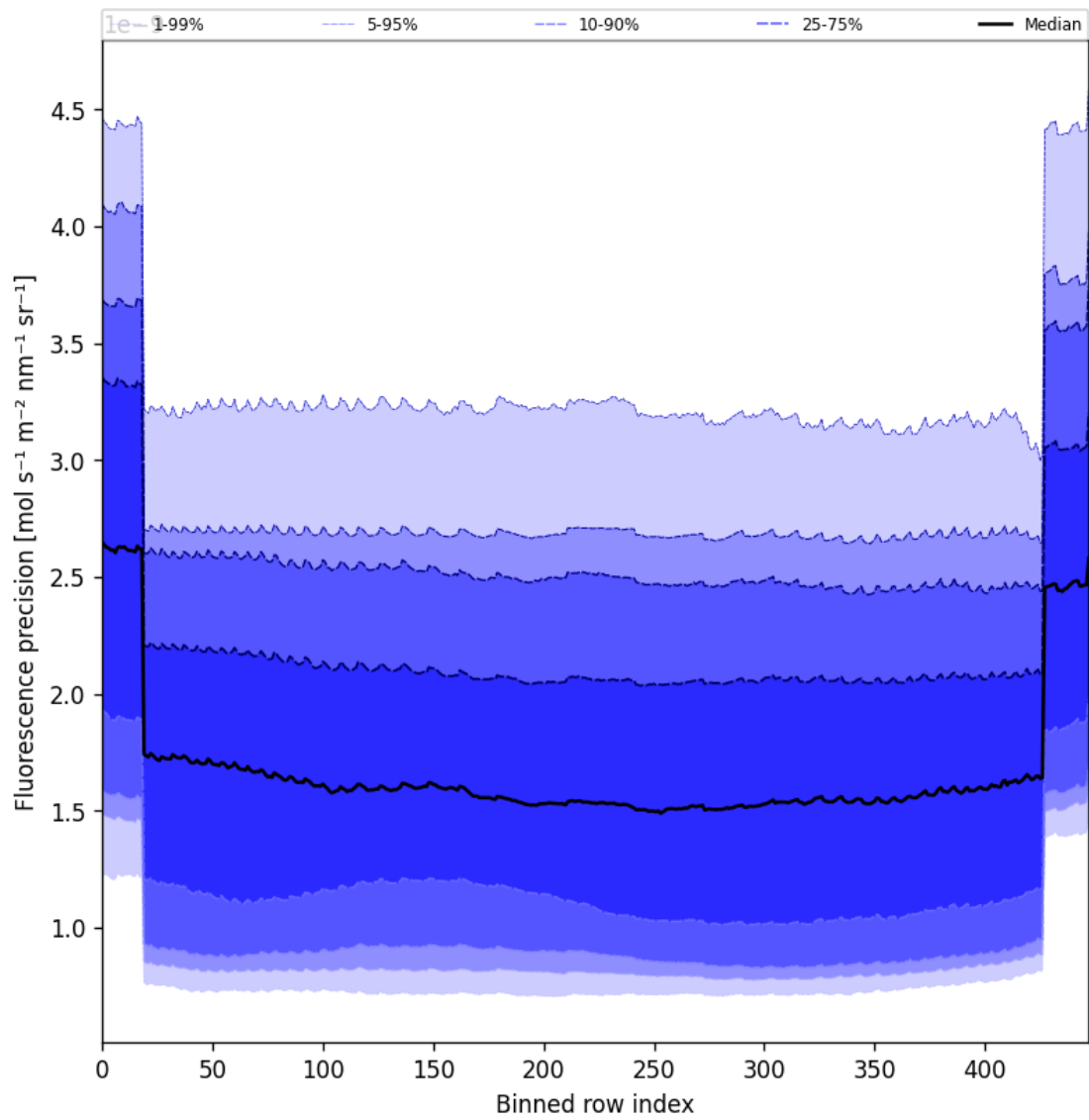
Figure 58: Along track statistics of “Fluorescence precision” for 2025-01-28 to 2025-01-30
