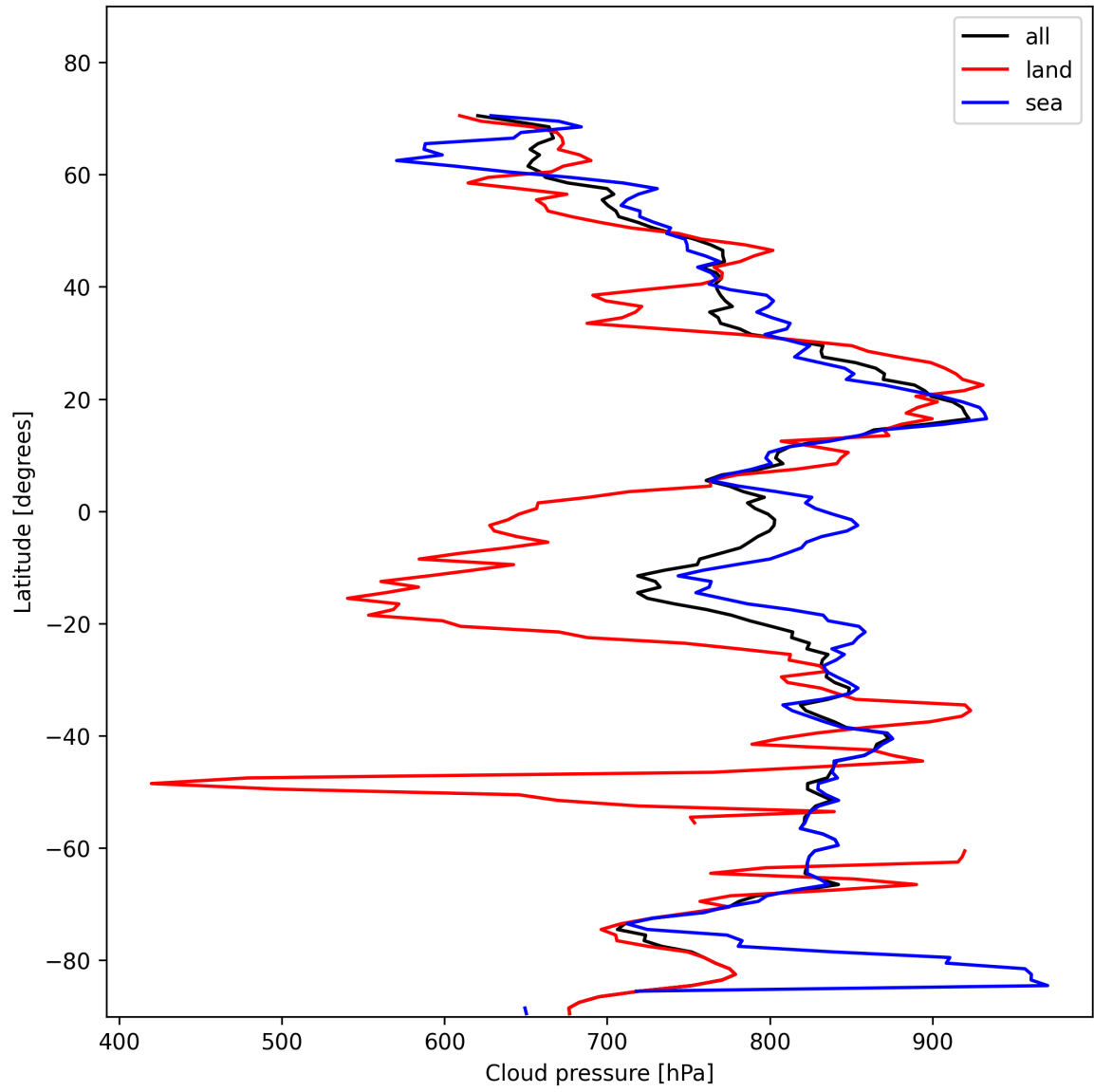
Figure 13: Zonal average of “Cloud pressure” for 2025-01-28 to 2025-01-30.
