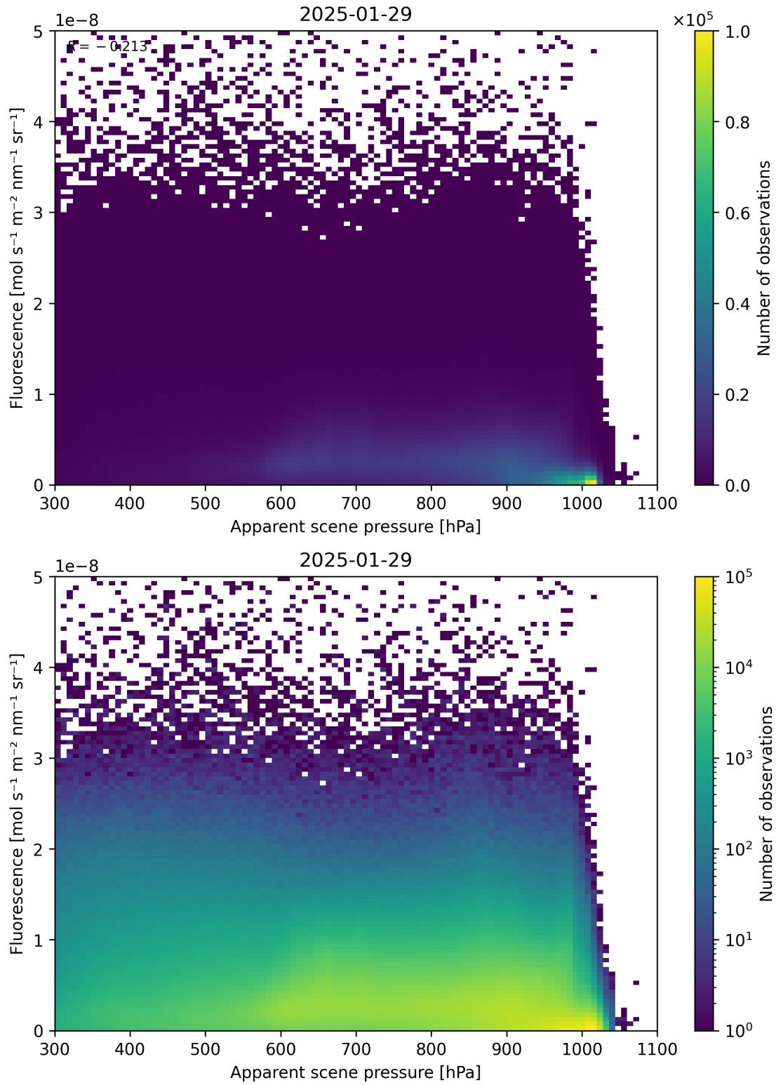
Figure 64: Scatter density plot of “Apparent scene pressure” against “Fluorescence” for 2025-01-28 to 2025-01-30.
