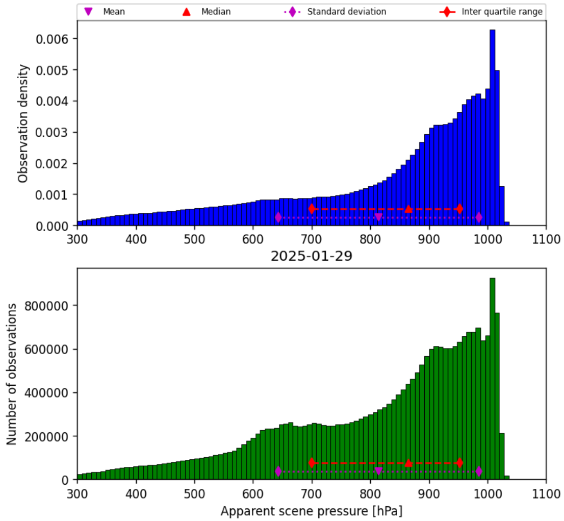
Figure 36: Histogram of “Apparent scene pressure” for 2025-01-28 to 2025-01-30
