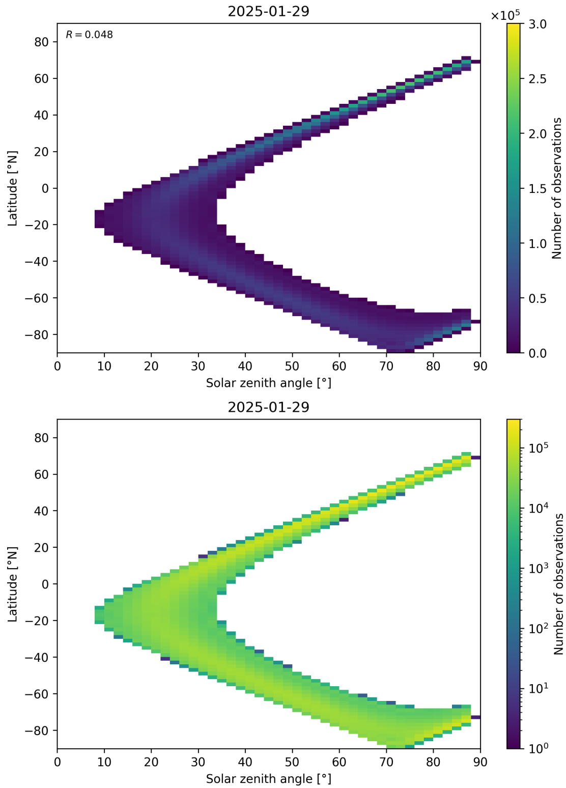
Figure 113: Scatter density plot of “Solar zenith angle” against “Latitude” for 2025-01-28 to 2025-01-30.
