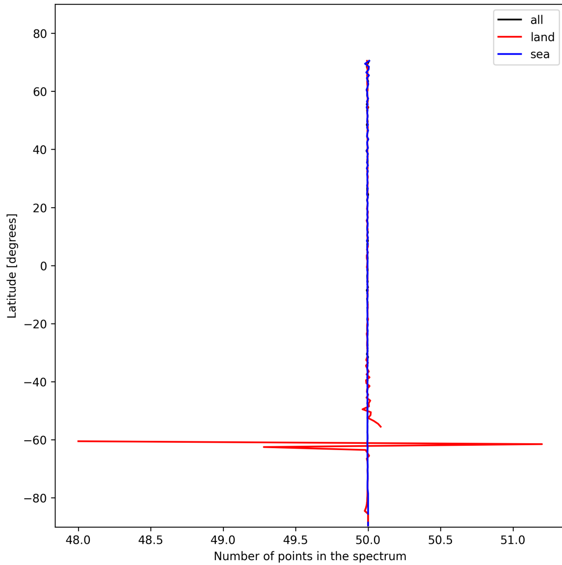
Figure 27: Zonal average of “Number of points in the spectrum” for 2025-01-28 to 2025-01-30.
