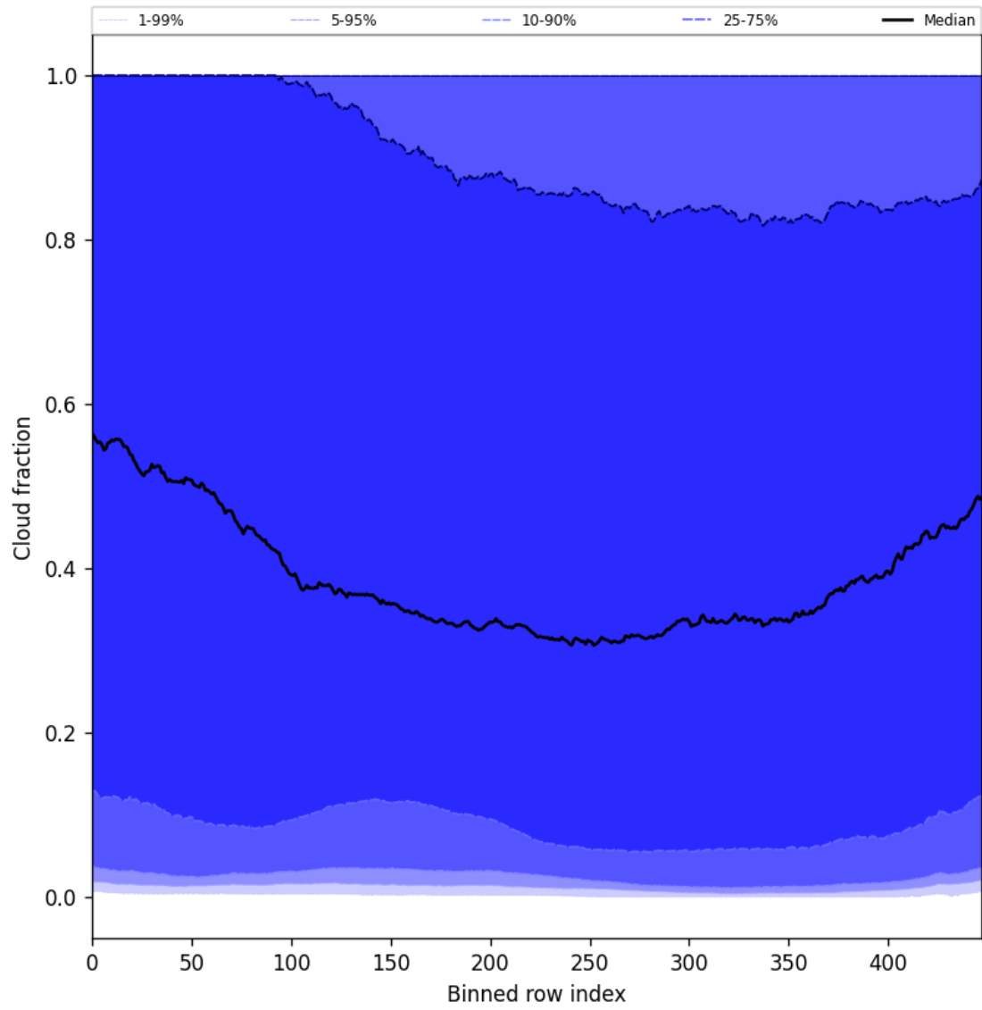
Figure 49: Along track statistics of “Cloud fraction” for 2025-01-28 to 2025-01-30
