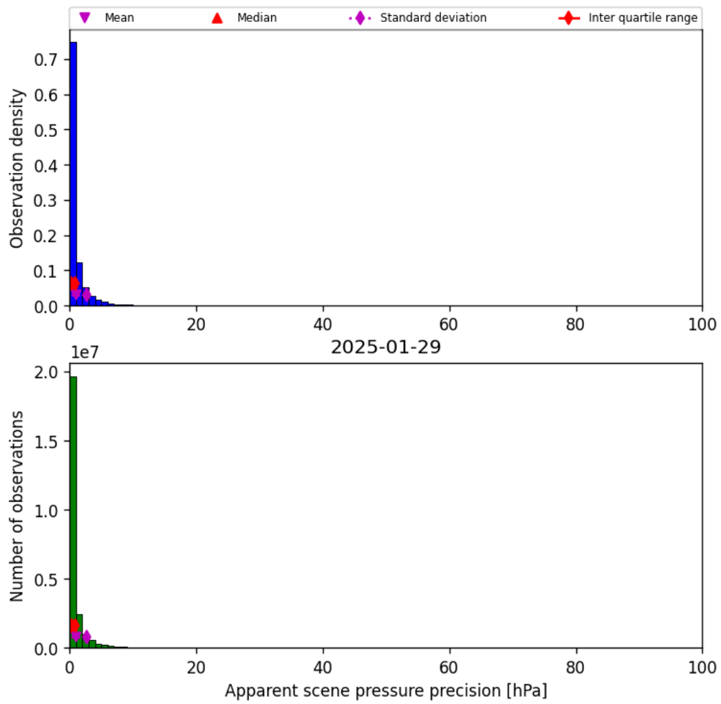
Figure 37: Histogram of “Apparent scene pressure precision” for 2025-01-28 to 2025-01-30
