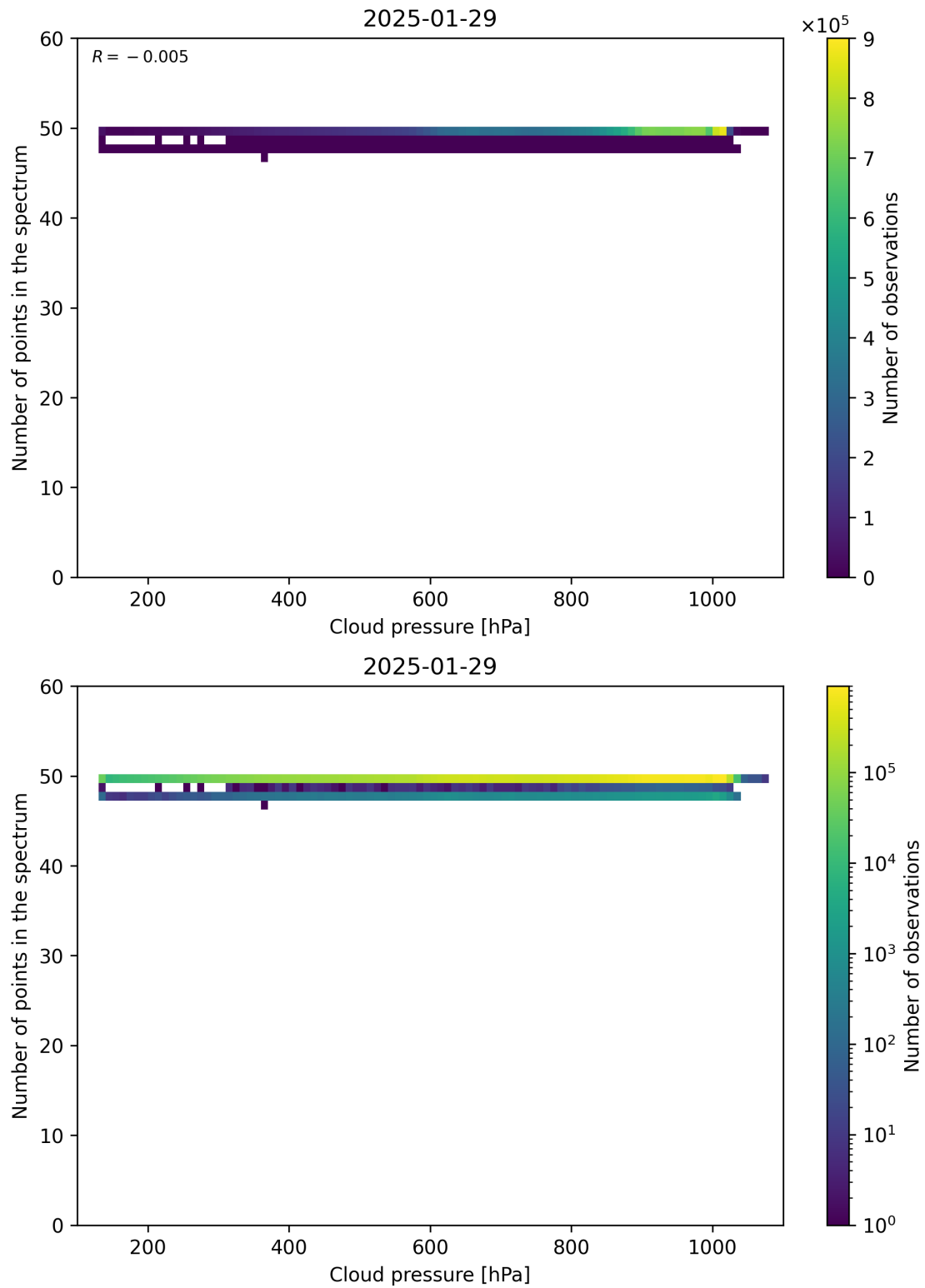
Figure 82: Scatter density plot of “Cloud pressure” against “Number of points in the spectrum” for 2025-01-28 to 2025-01-30.
