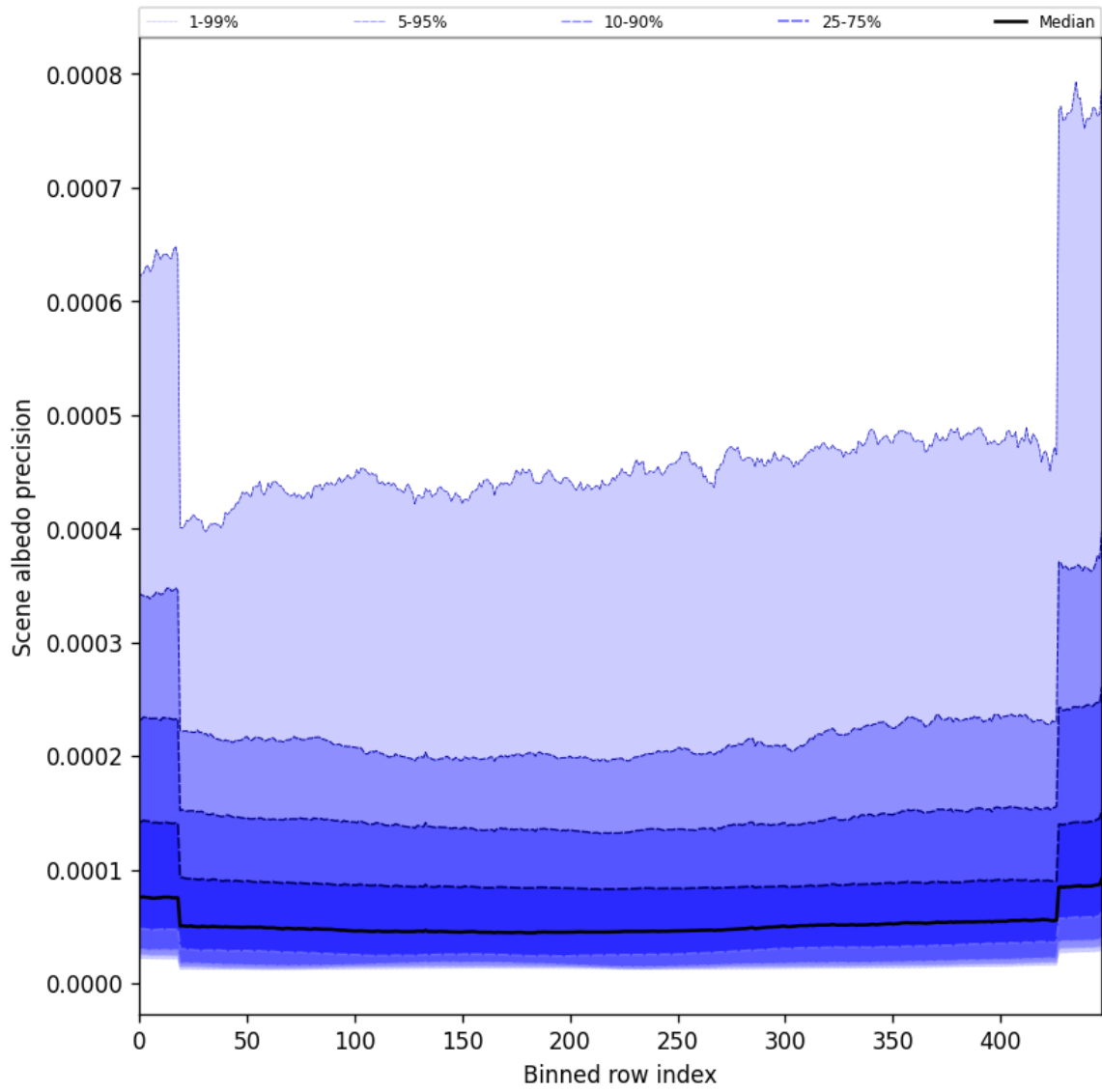
Figure 52: Along track statistics of “Scene albedo precision” for 2025-01-28 to 2025-01-30
