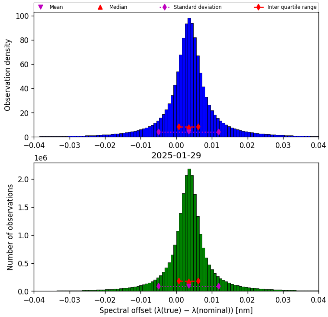
Figure 45: Histogram of “Spectral offset ( \lambda_{\text{true}} - \lambda_{\text{nominal}} )” for 2025-01-28 to 2025-01-30
