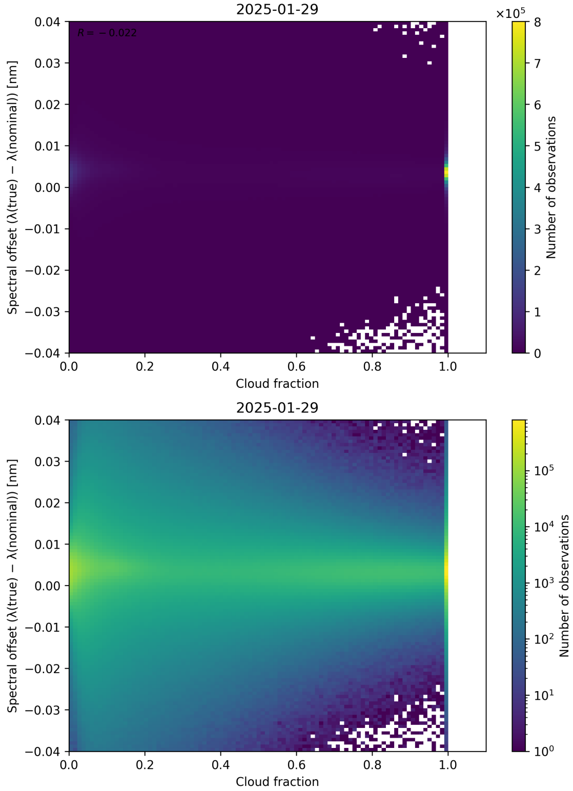
Figure 76: Scatter density plot of “Cloud fraction” against “Spectral offset ( \lambda_{\text{true}} - \lambda_{\text{nominal}} )” for 2025-01-28 to 2025-01-30.
