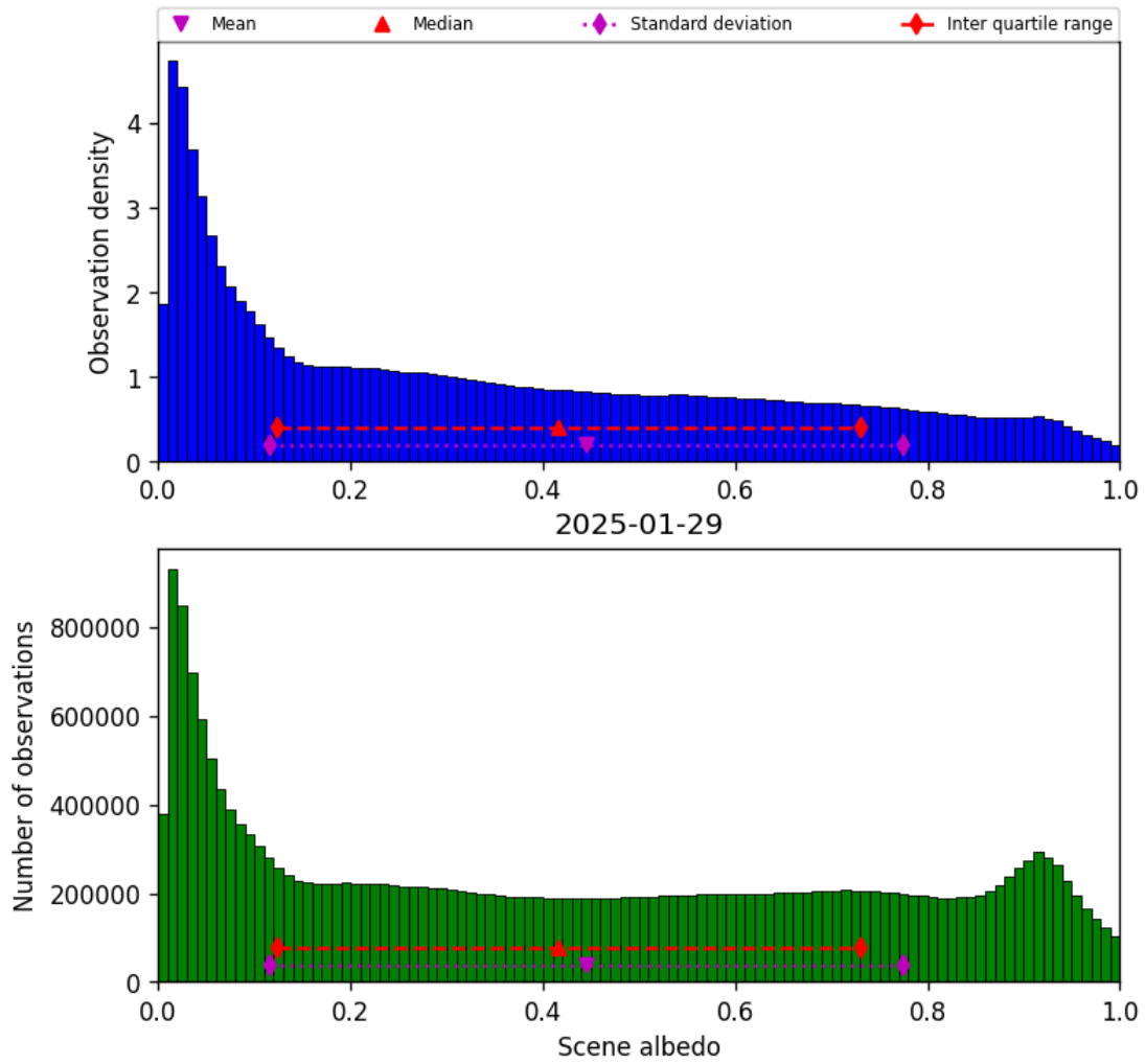
Figure 34: Histogram of “Scene albedo” for 2025-01-28 to 2025-01-30
