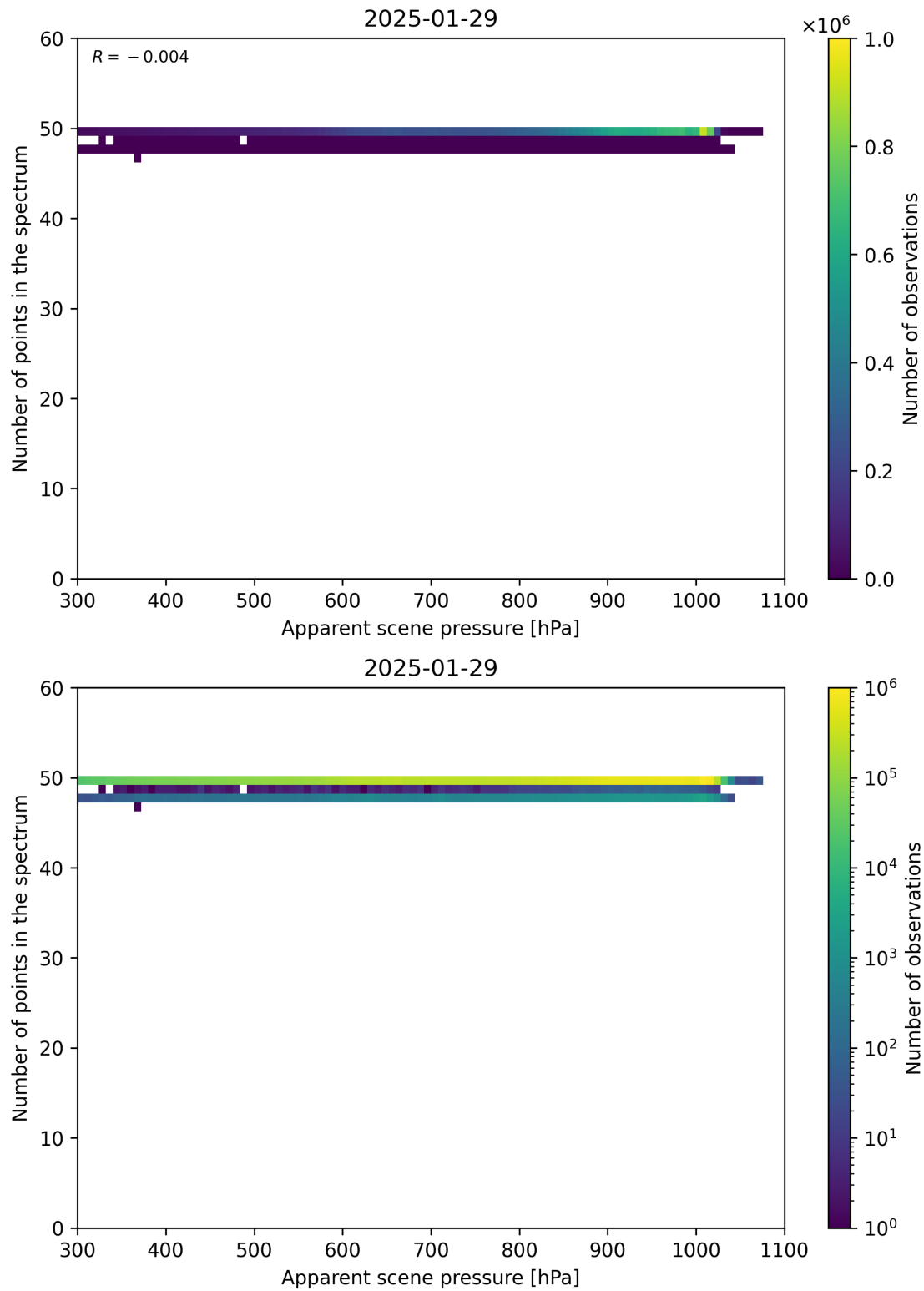
Figure 66: Scatter density plot of “Apparent scene pressure” against “Number of points in the spectrum” for 2025-01-28 to 2025-01-30.
