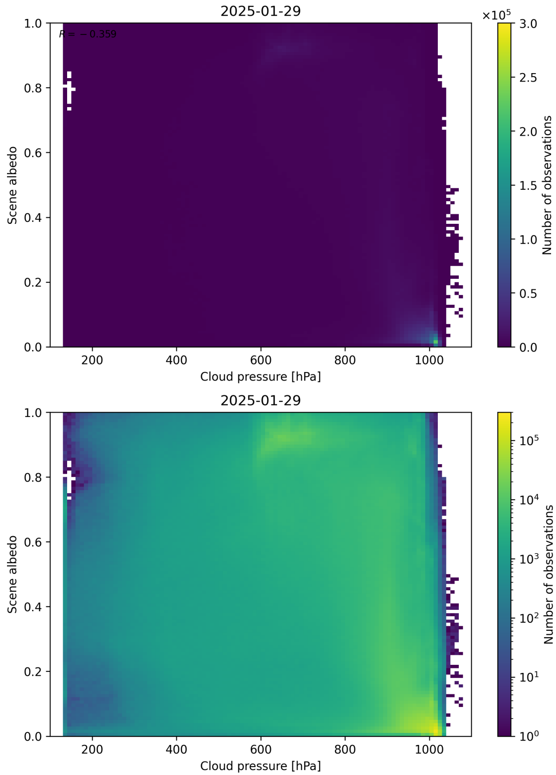
Figure 83: Scatter density plot of “Cloud pressure” against “Scene albedo” for 2025-01-28 to 2025-01-30.
