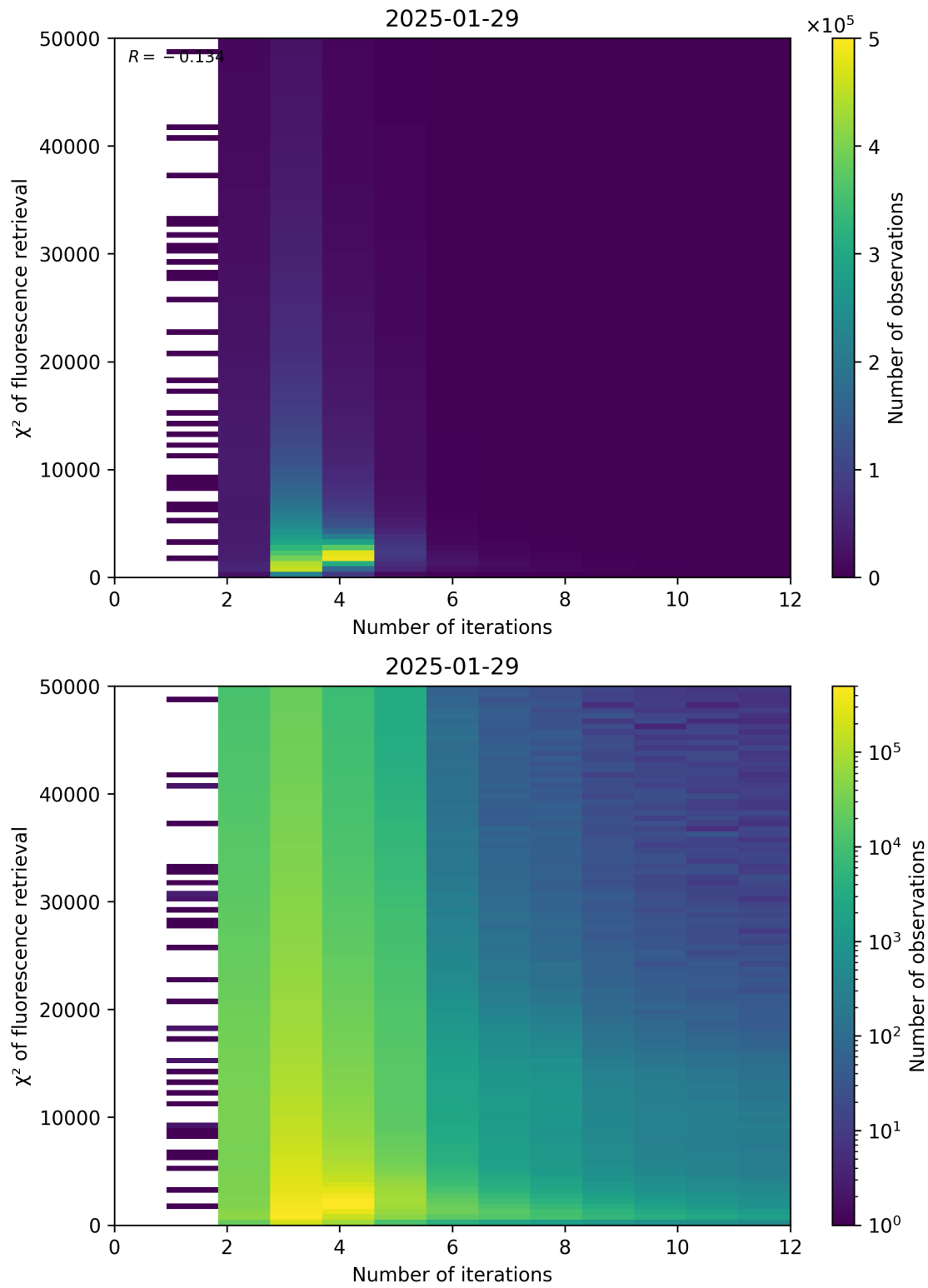
Figure 97: Scatter density plot of “Number of iterations” against “ \chi^2 of fluorescence retrieval” for 2025-01-28 to 2025-01-30.
