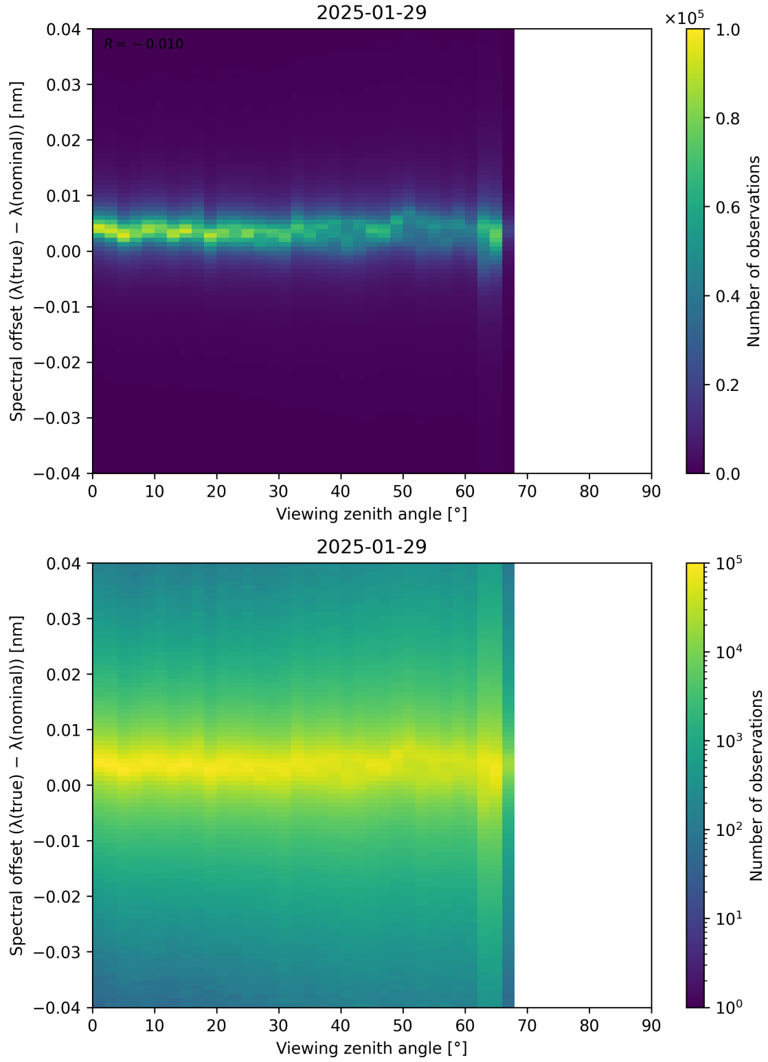
Figure 128: Scatter density plot of “Viewing zenith angle” against “Spectral offset ( \lambda_{\text{true}} - \lambda_{\text{nominal}} )” for 2025-01-28 to 2025-01-30.
