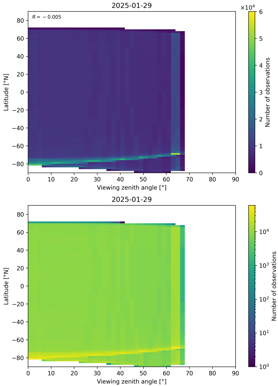
Figure 123: Scatter density plot of “Viewing zenith angle” against “Latitude” for 2025-01-28 to 2025-01-30.
