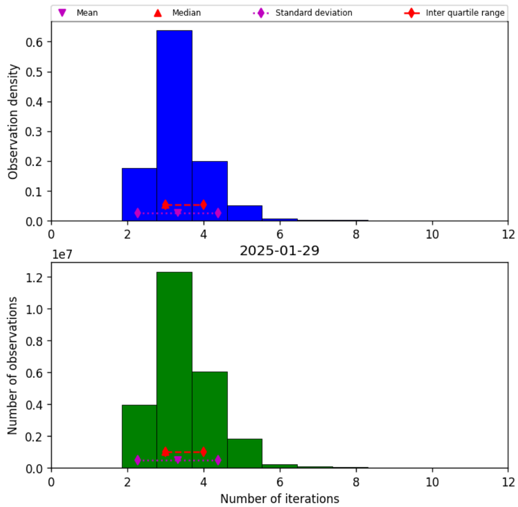
Figure 39: Histogram of “Number of iterations” for 2025-01-28 to 2025-01-30
