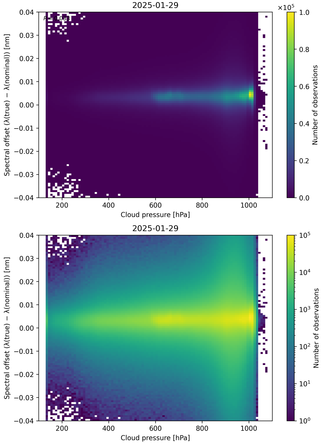
Figure 84: Scatter density plot of “Cloud pressure” against “Spectral offset ( \lambda_{\text{true}} - \lambda_{\text{nominal}} )” for 2025-01-28 to 2025-01-30.
