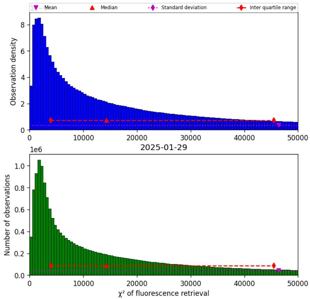
Figure 42: Histogram of “ \chi^2 of fluorescence retrieval” for 2025-01-28 to 2025-01-30
