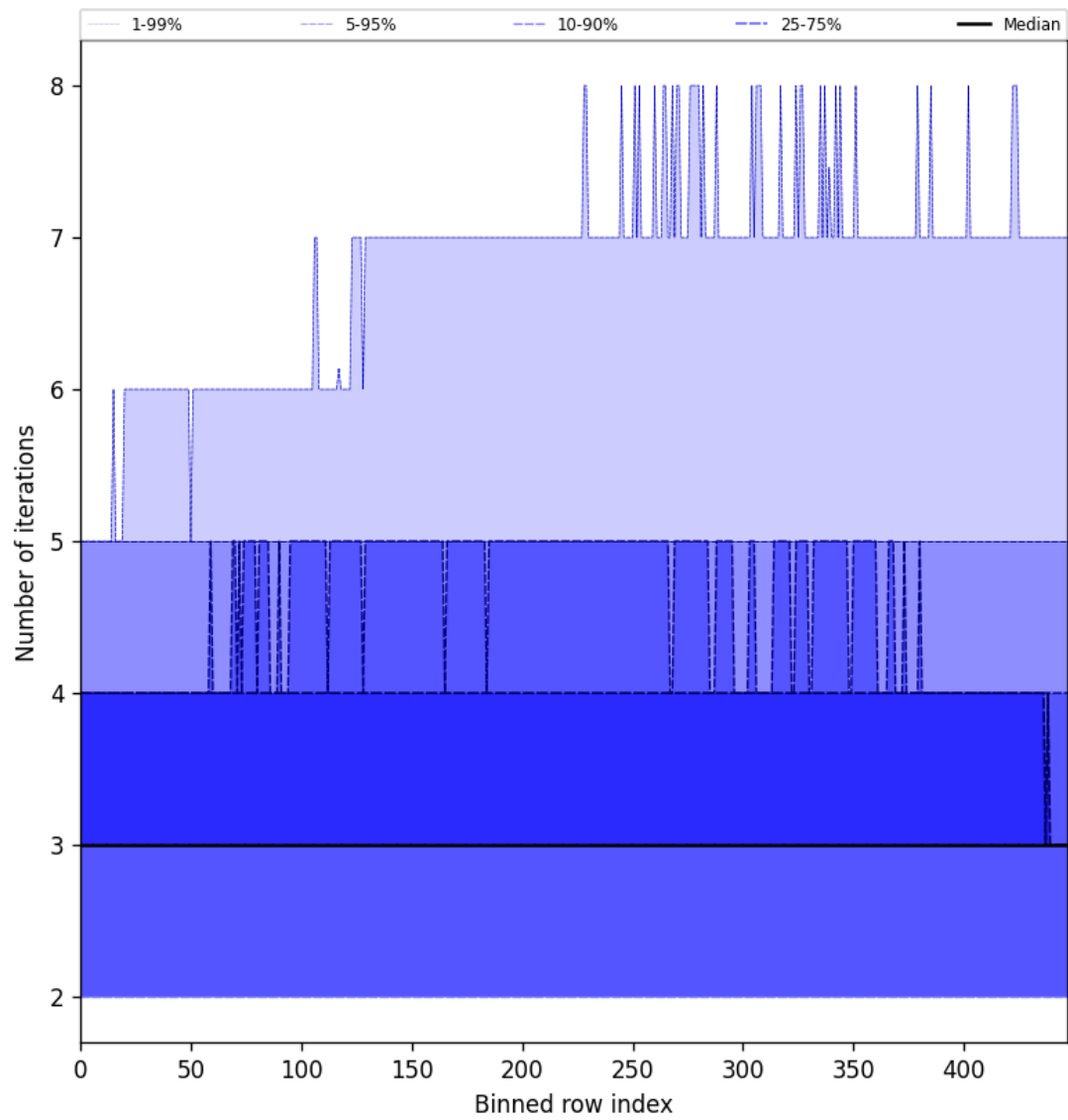
Figure 56: Along track statistics of “Number of iterations” for 2025-01-28 to 2025-01-30
