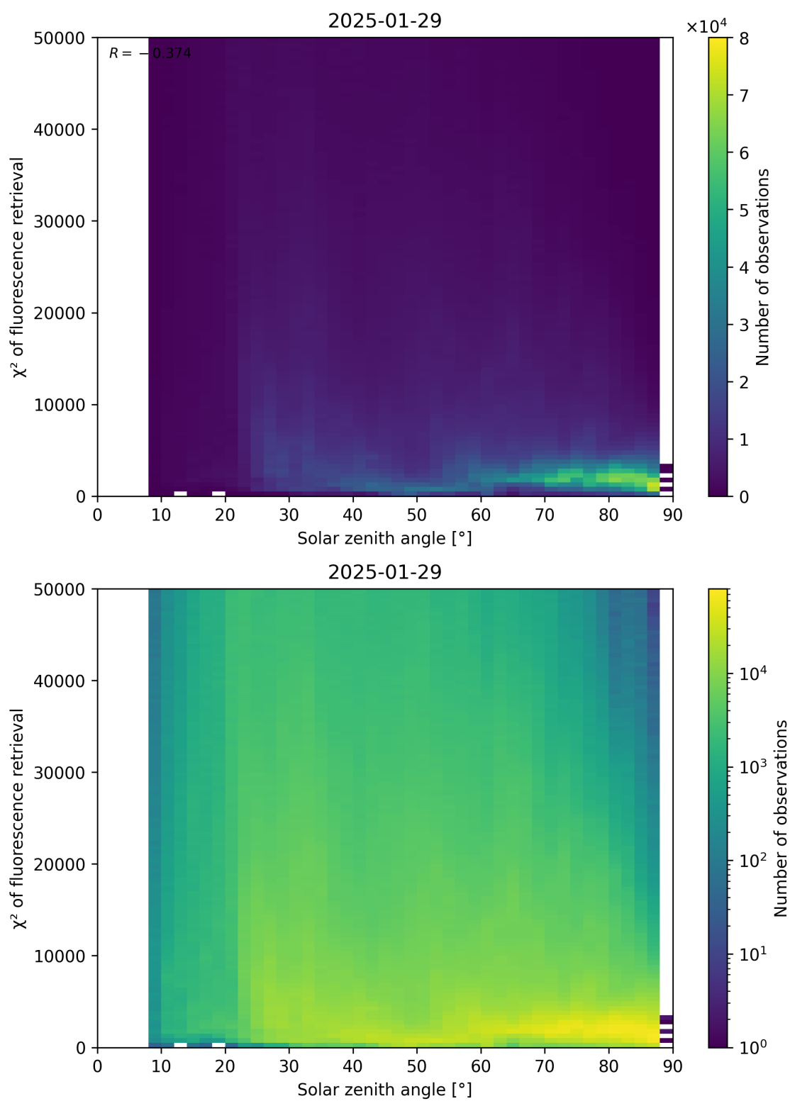
Figure 109: Scatter density plot of “Solar zenith angle” against “ \chi^2 of fluorescence retrieval” for 2025-01-28 to 2025-01-30.
