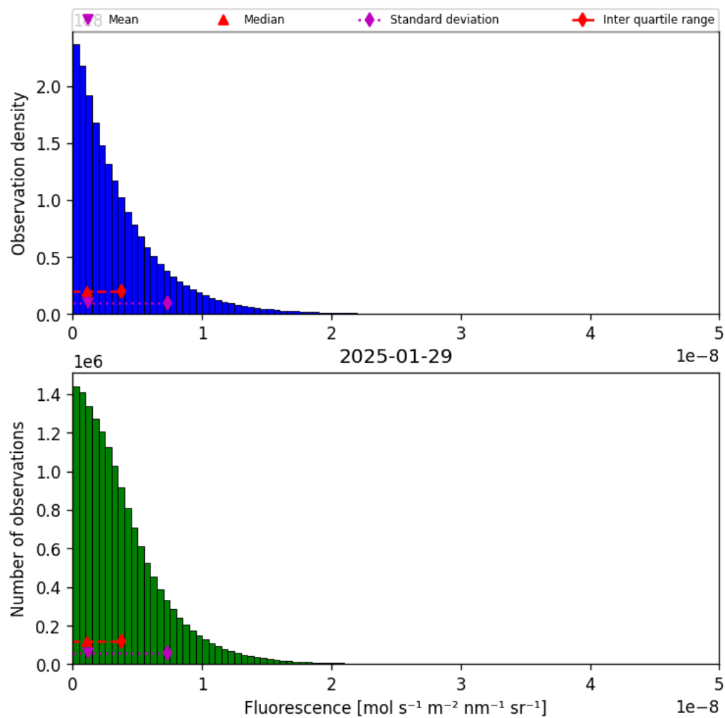
Figure 40: Histogram of “Fluorescence” for 2025-01-28 to 2025-01-30
