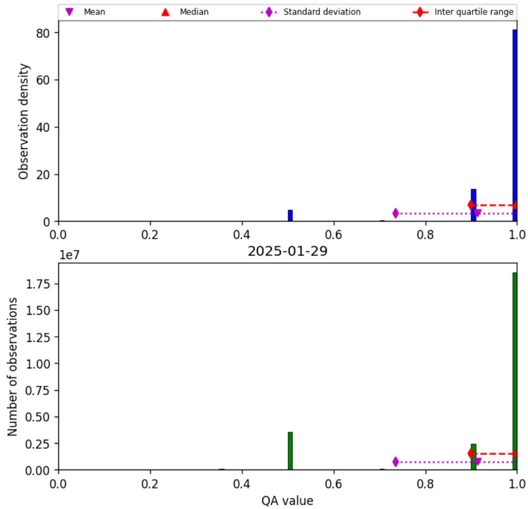
Figure 29: Histogram of “QA value” for 2025-01-28 to 2025-01-30
