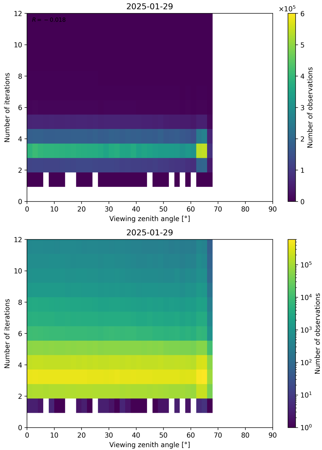
Figure 124: Scatter density plot of “Viewing zenith angle” against “Number of iterations” for 2025-01-28 to 2025-01-30.
