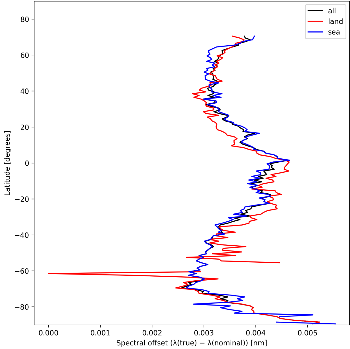
Figure 28: Zonal average of “Spectral offset ( \lambda_{\text{true}} - \lambda_{\text{nominal}} )” for 2025-01-28 to 2025-01-30.
