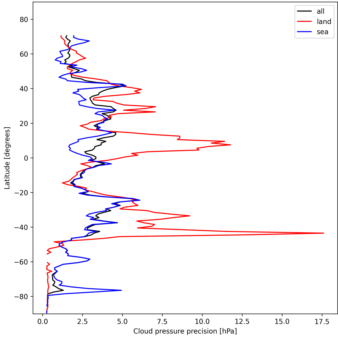
Figure 14: Zonal average of "Cloud pressure precision" for 2025-01-28 to 2025-01-30.
