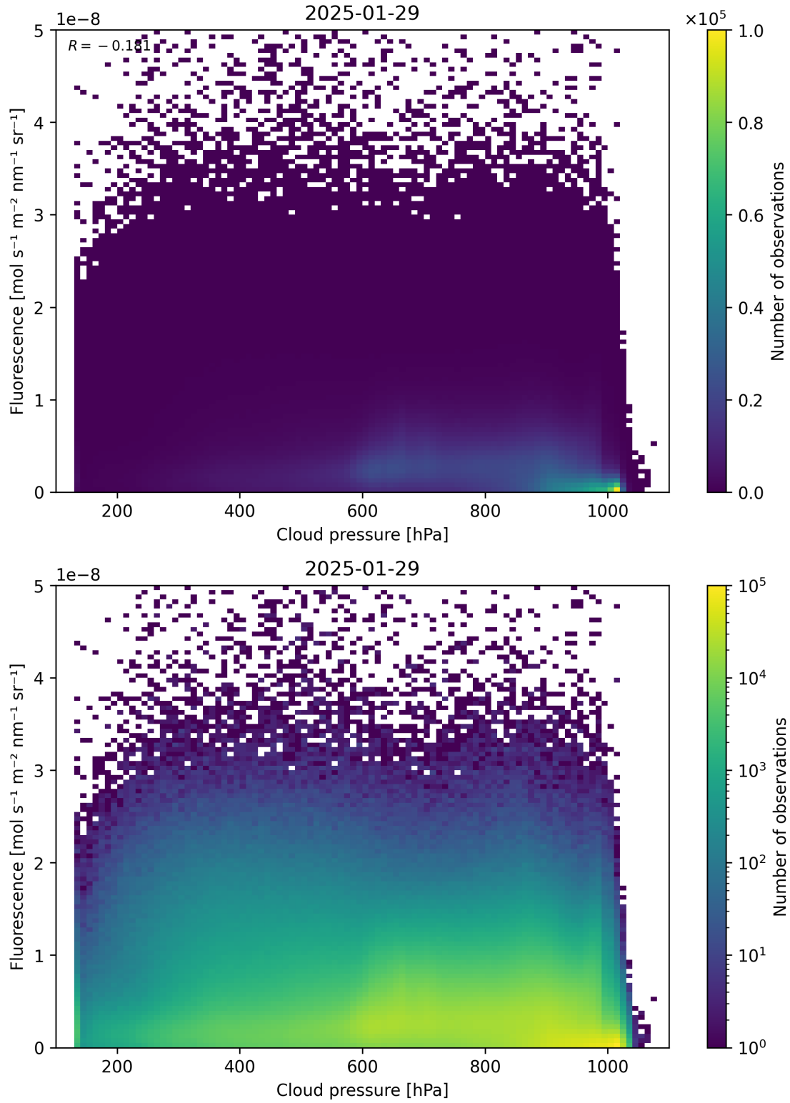
Figure 80: Scatter density plot of “Cloud pressure” against “Fluorescence” for 2025-01-28 to 2025-01-30.
