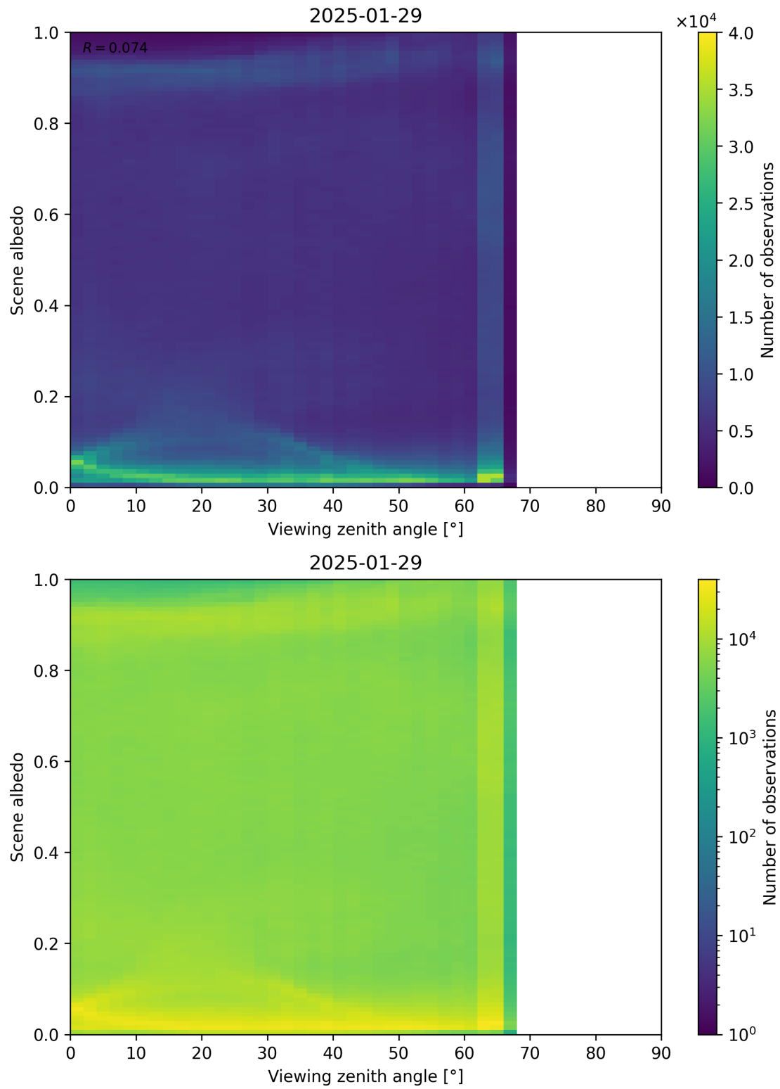
Figure 126: Scatter density plot of “Viewing zenith angle” against “Scene albedo” for 2025-01-28 to 2025-01-30.
