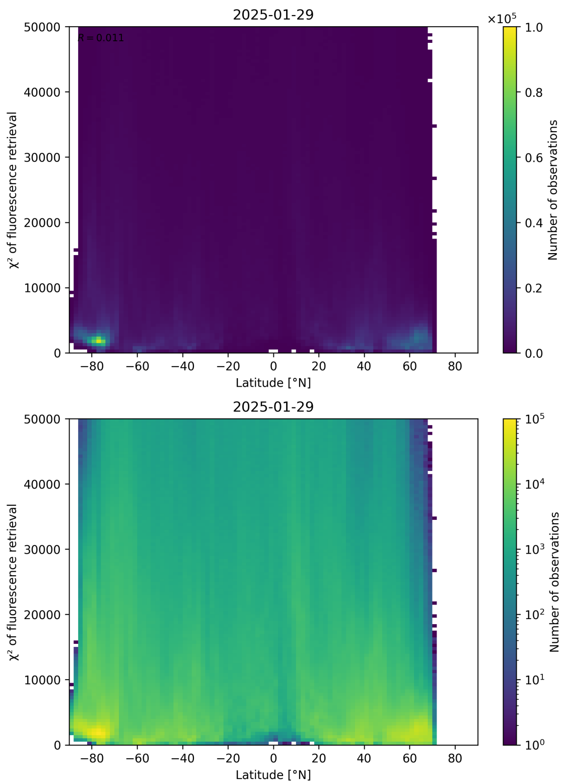
Figure 89: Scatter density plot of “Latitude” against “ \chi^2 of fluorescence retrieval” for 2025-01-28 to 2025-01-30.
