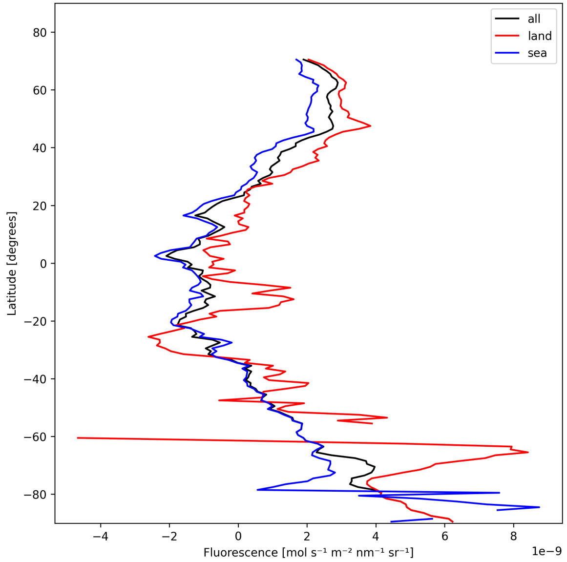
Figure 23: Zonal average of “Fluorescence” for 2025-01-28 to 2025-01-30.
