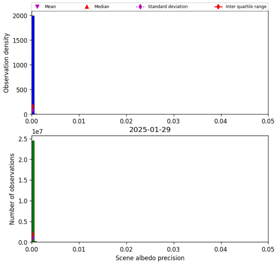
Figure 35: Histogram of “Scene albedo precision” for 2025-01-28 to 2025-01-30
