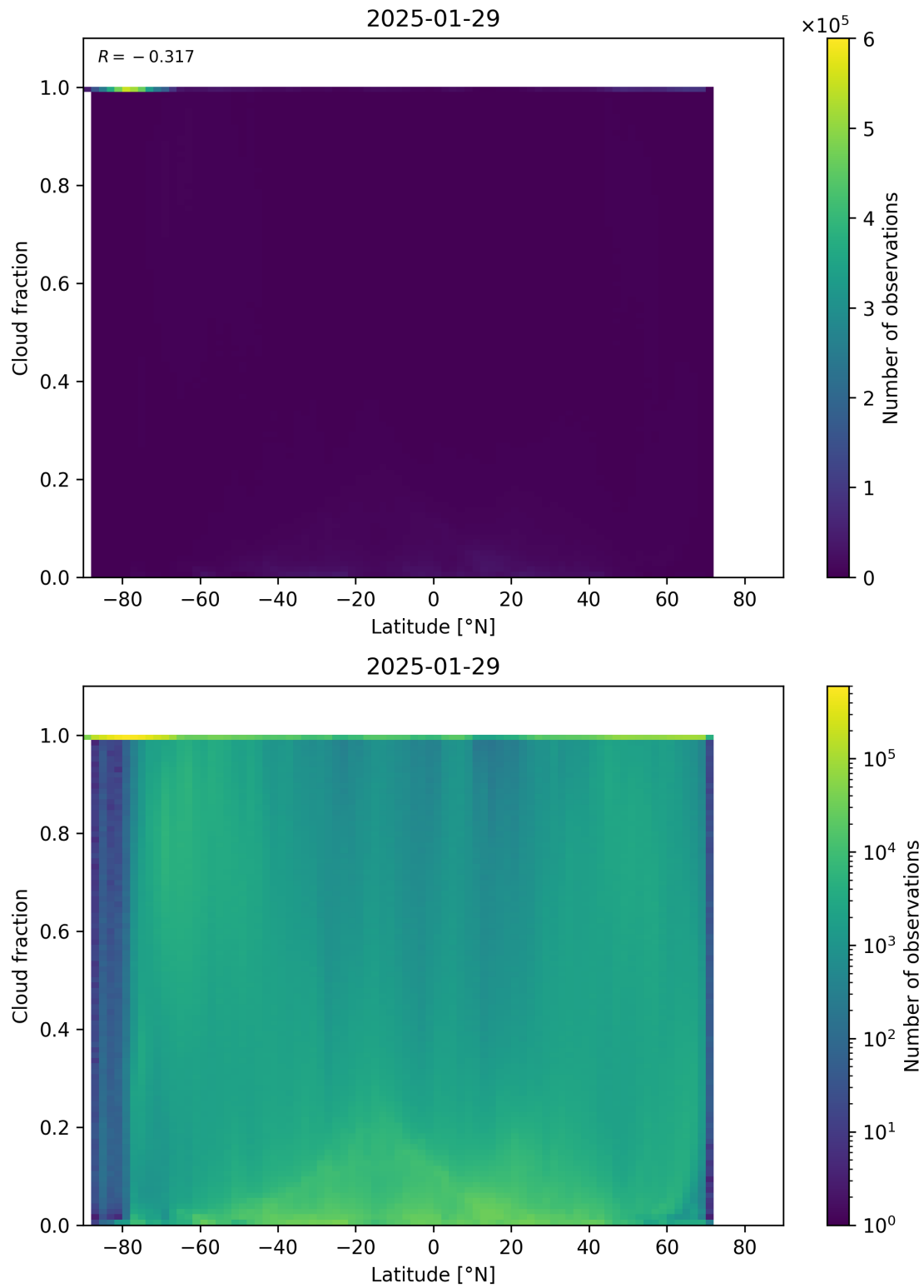
Figure 90: Scatter density plot of “Latitude” against “Cloud fraction” for 2025-01-28 to 2025-01-30.
