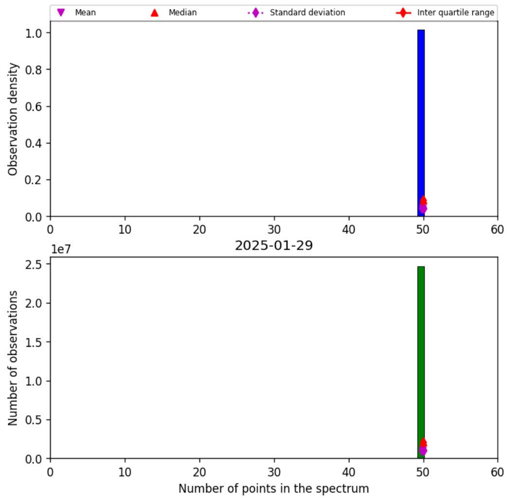
Figure 44: Histogram of “Number of points in the spectrum” for 2025-01-28 to 2025-01-30
