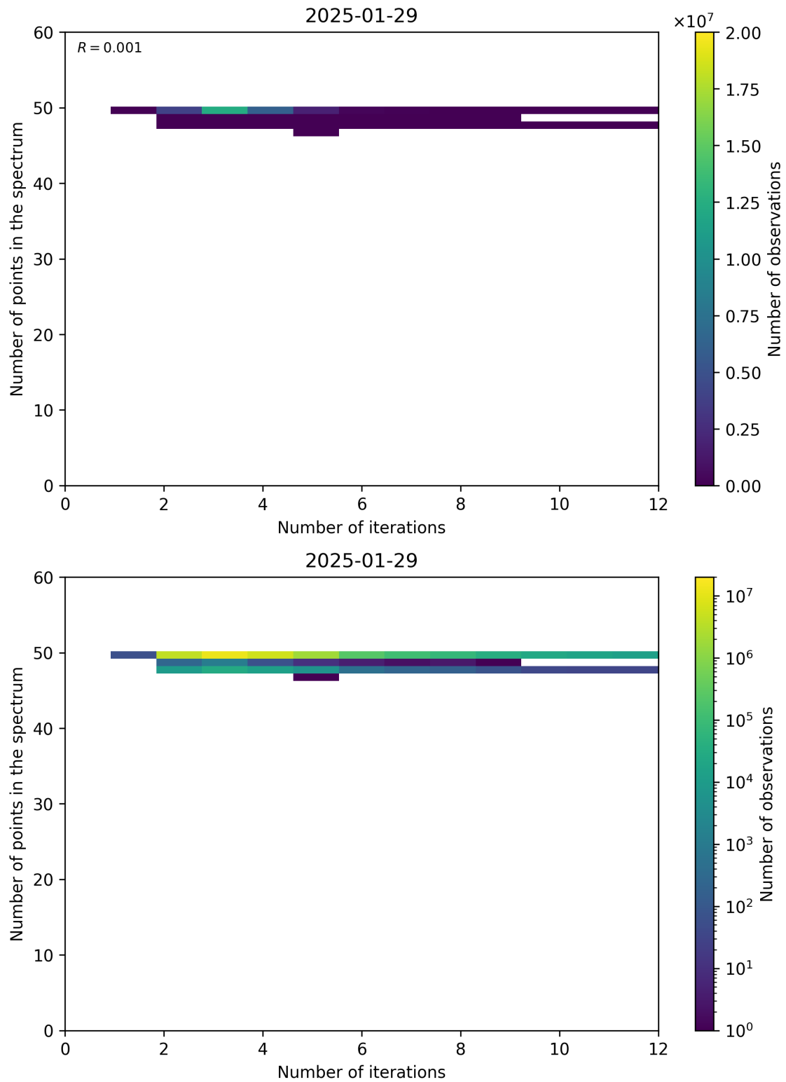
Figure 99: Scatter density plot of “Number of iterations” against “Number of points in the spectrum” for 2025-01-28 to 2025-01-30.
