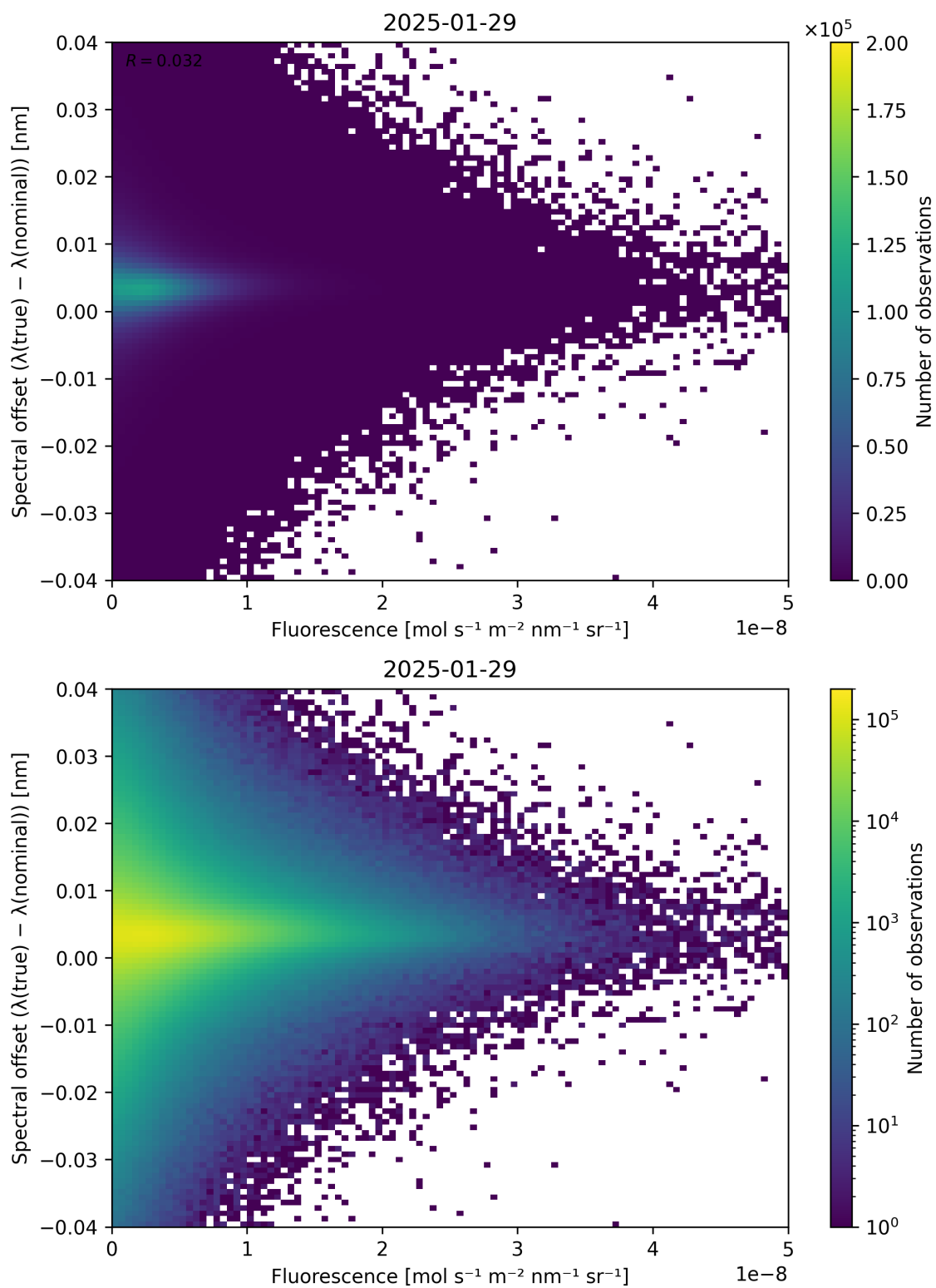
Figure 87: Scatter density plot of “Fluorescence” against “Spectral offset ( \lambda_{\text{true}} - \lambda_{\text{nominal}} )” for 2025-01-28 to 2025-01-30.
