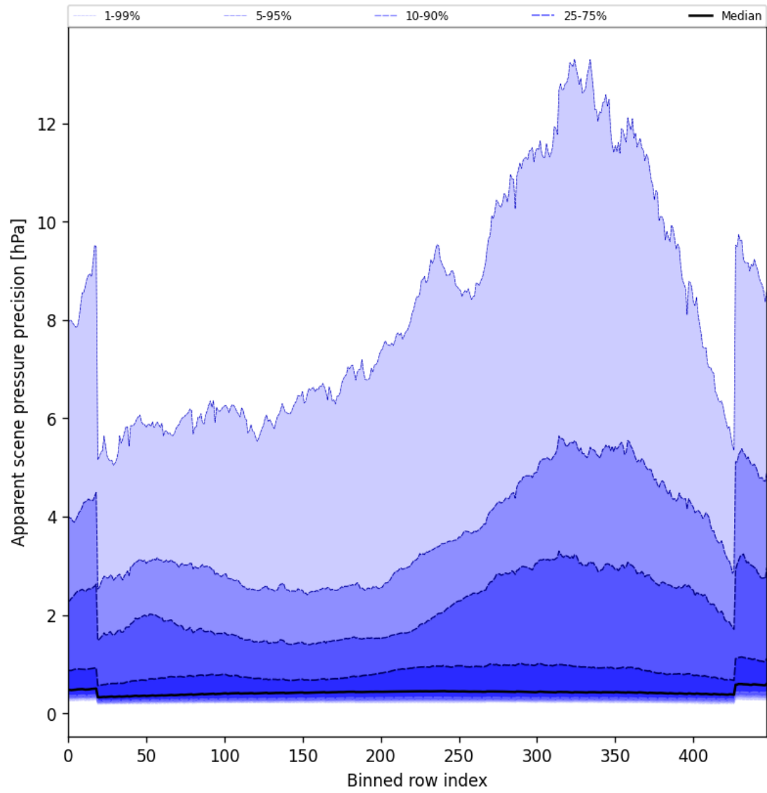
Figure 54: Along track statistics of “Apparent scene pressure precision” for 2025-01-28 to 2025-01-30
