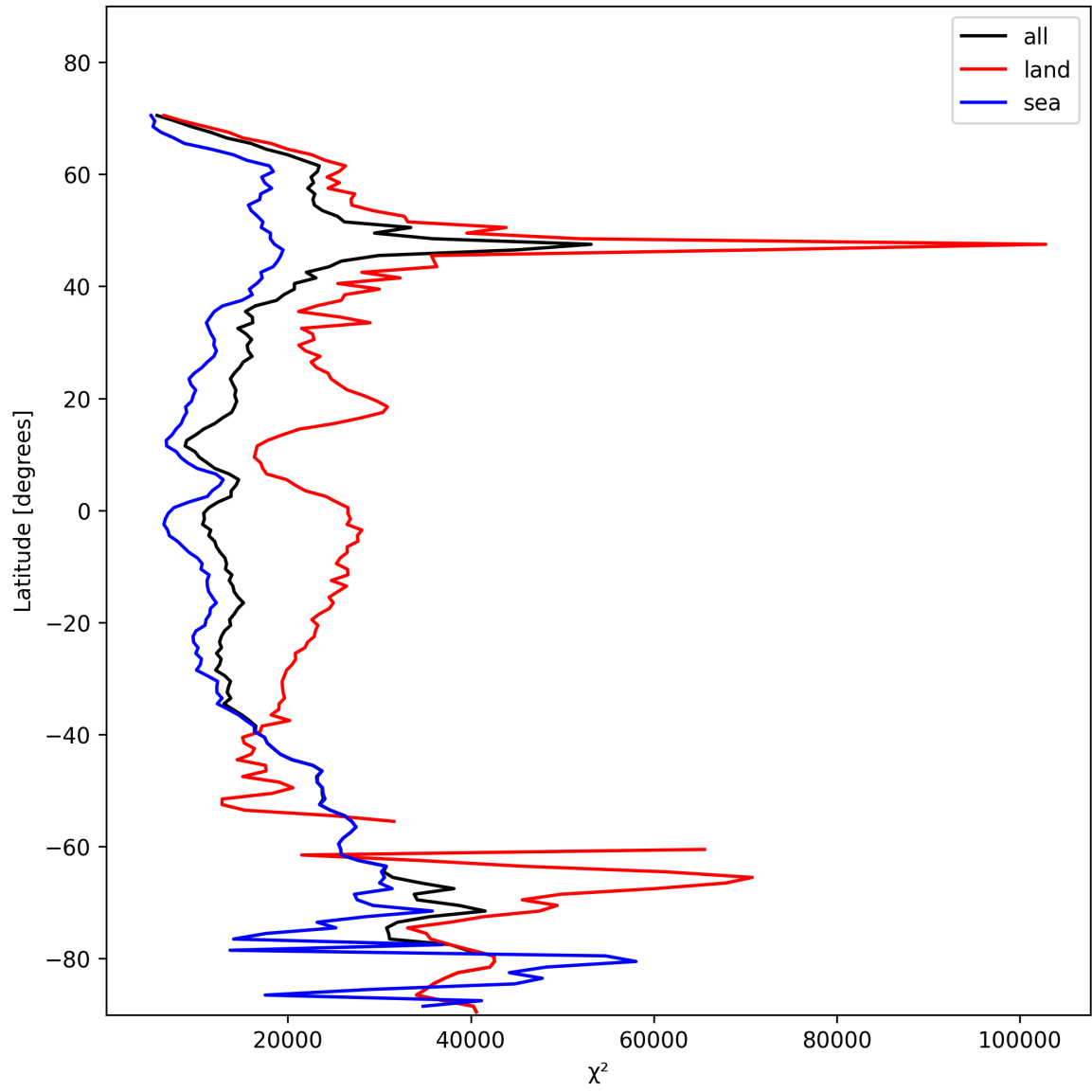
Figure 21: Zonal average of “ \chi^2 ” for 2025-01-29 to 2025-01-31.
