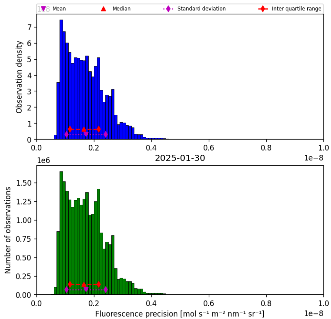
Figure 41: Histogram of “Fluorescence precision” for 2025-01-29 to 2025-01-31
