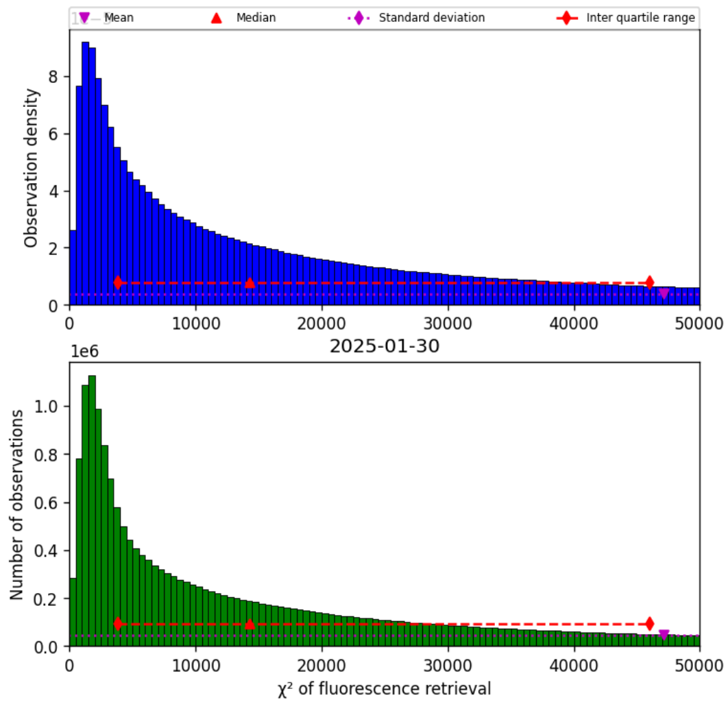
Figure 42: Histogram of “ \chi^2 of fluorescence retrieval” for 2025-01-29 to 2025-01-31
