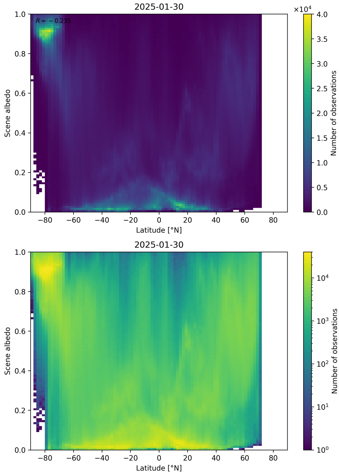
Figure 95: Scatter density plot of “Latitude” against “Scene albedo” for 2025-01-29 to 2025-01-31.
