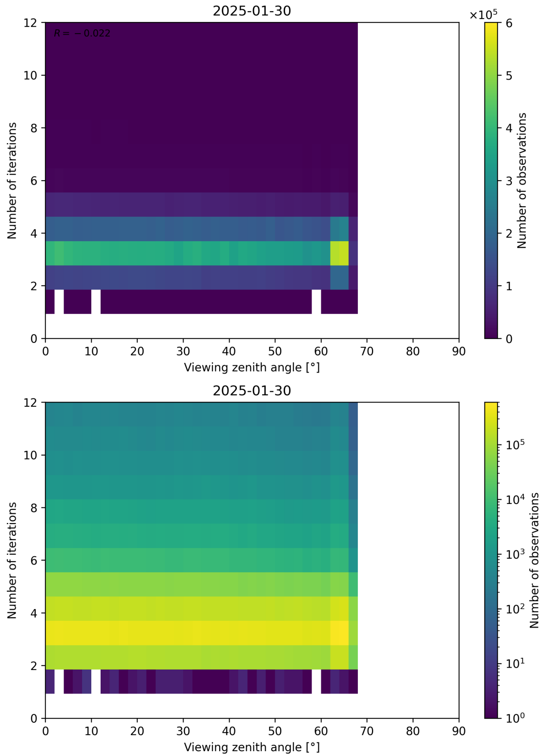
Figure 124: Scatter density plot of “Viewing zenith angle” against “Number of iterations” for 2025-01-29 to 2025-01-31.
