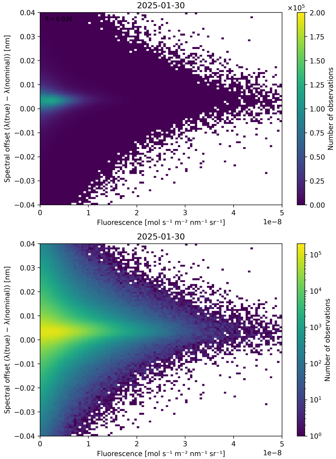
Figure 87: Scatter density plot of “Fluorescence” against “Spectral offset ( \lambda_{\text{true}} - \lambda_{\text{nominal}} )” for 2025-01-29 to 2025-01-31.
