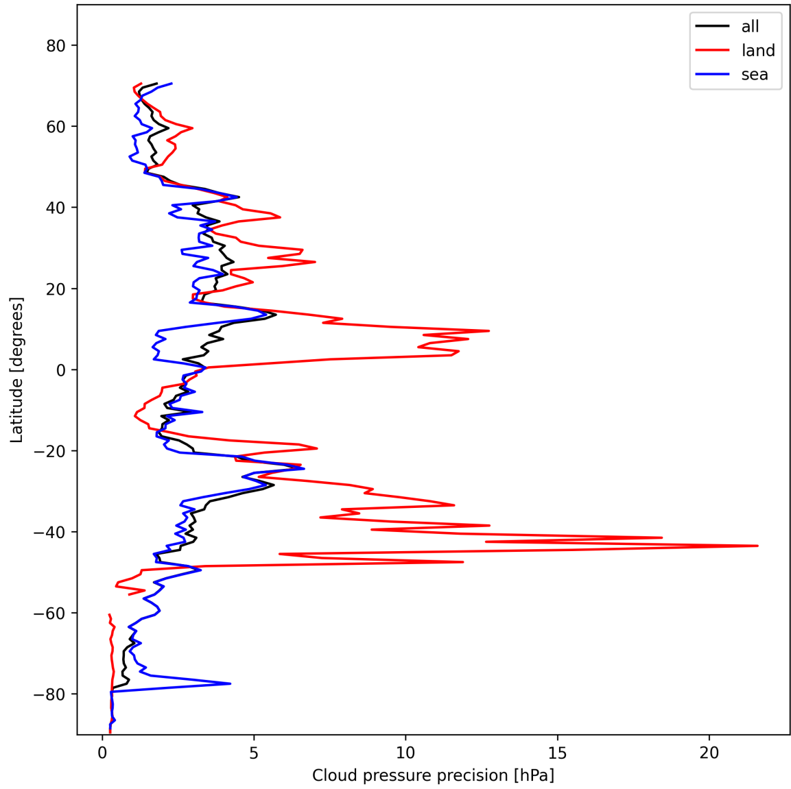
Figure 14: Zonal average of “Cloud pressure precision” for 2025-01-29 to 2025-01-31.
