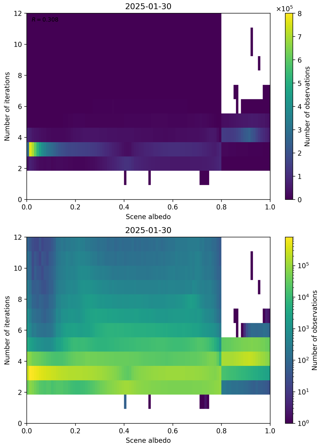
Figure 105: Scatter density plot of “Scene albedo” against “Number of iterations” for 2025-01-29 to 2025-01-31.
