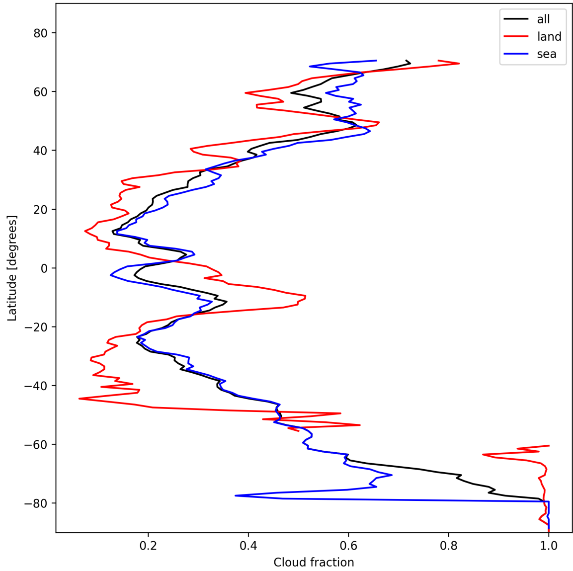
Figure 15: Zonal average of “Cloud fraction” for 2025-01-29 to 2025-01-31.
