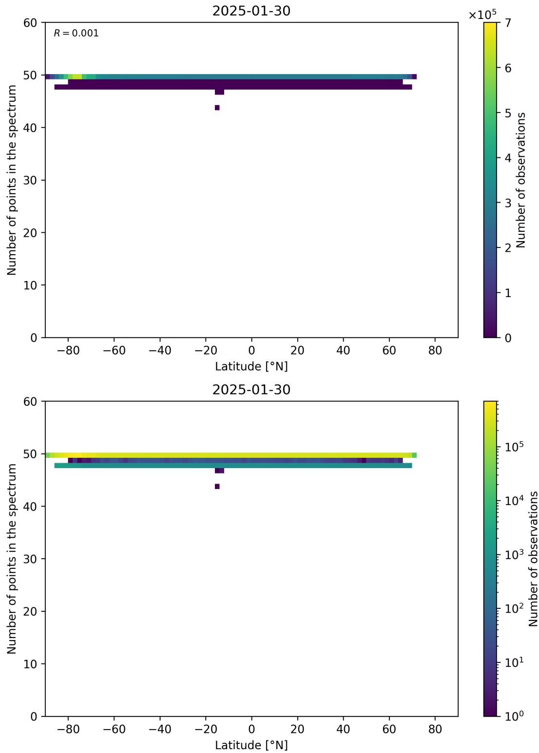
Figure 94: Scatter density plot of “Latitude” against “Number of points in the spectrum” for 2025-01-29 to 2025-01-31.
