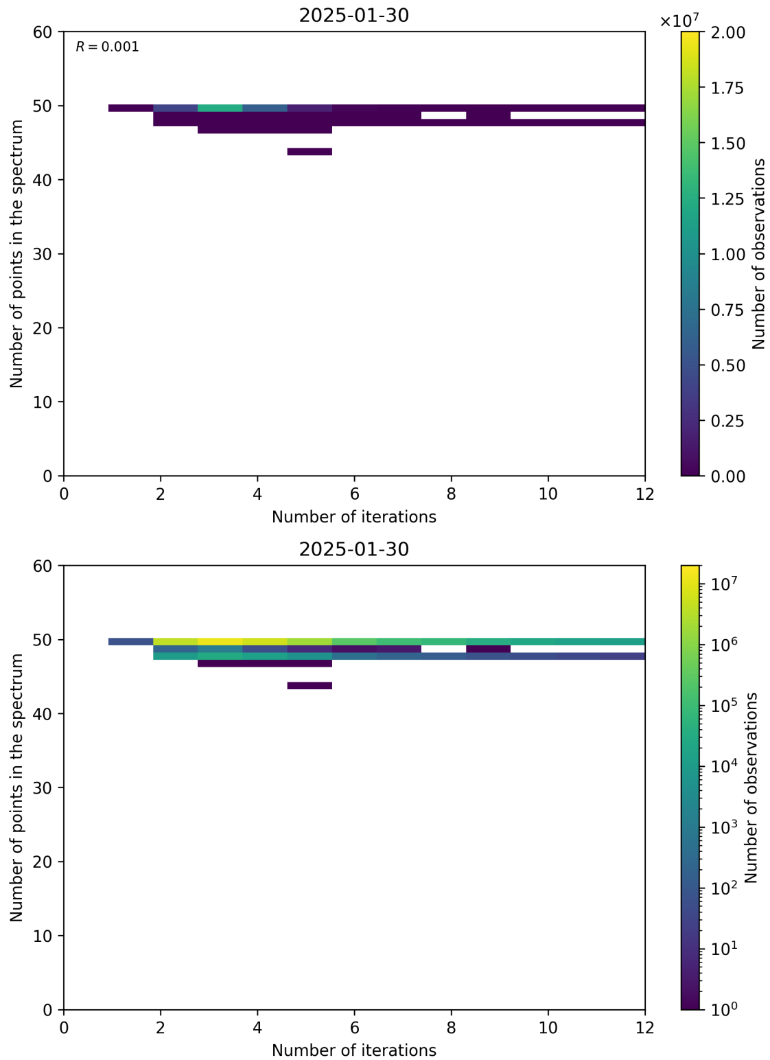
Figure 99: Scatter density plot of “Number of iterations” against “Number of points in the spectrum” for 2025-01-29 to 2025-01-31.
