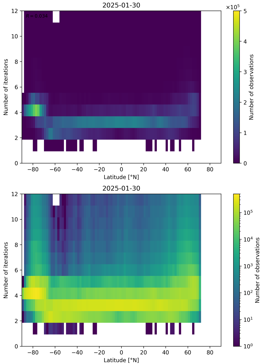
Figure 93: Scatter density plot of “Latitude” against “Number of iterations” for 2025-01-29 to 2025-01-31.
