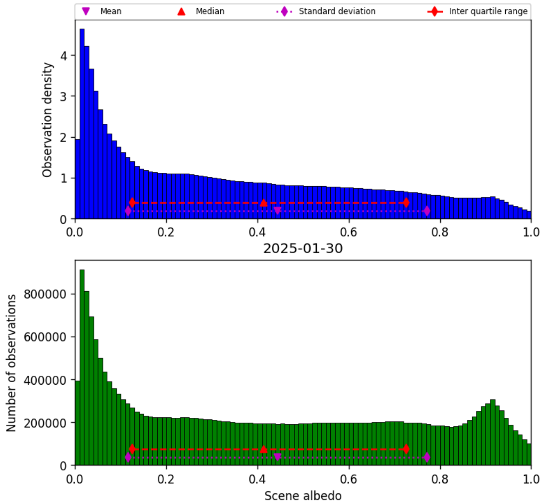
Figure 34: Histogram of “Scene albedo” for 2025-01-29 to 2025-01-31
