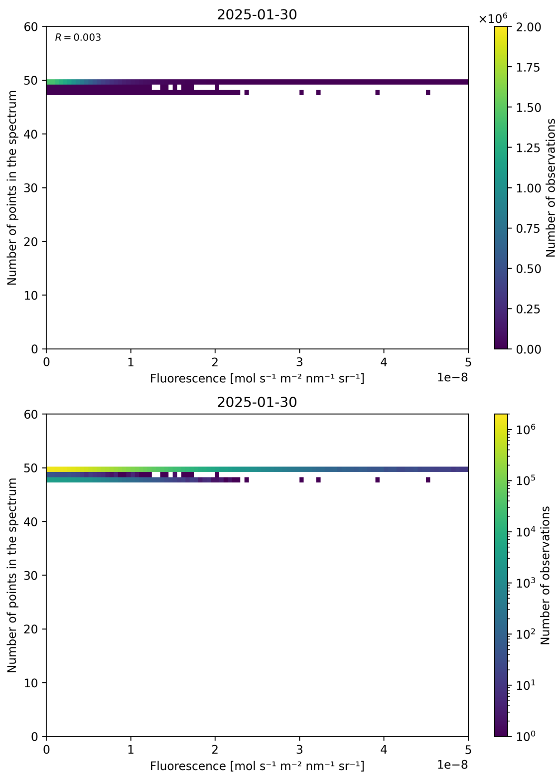
Figure 86: Scatter density plot of “Fluorescence” against “Number of points in the spectrum” for 2025-01-29 to 2025-01-31.
