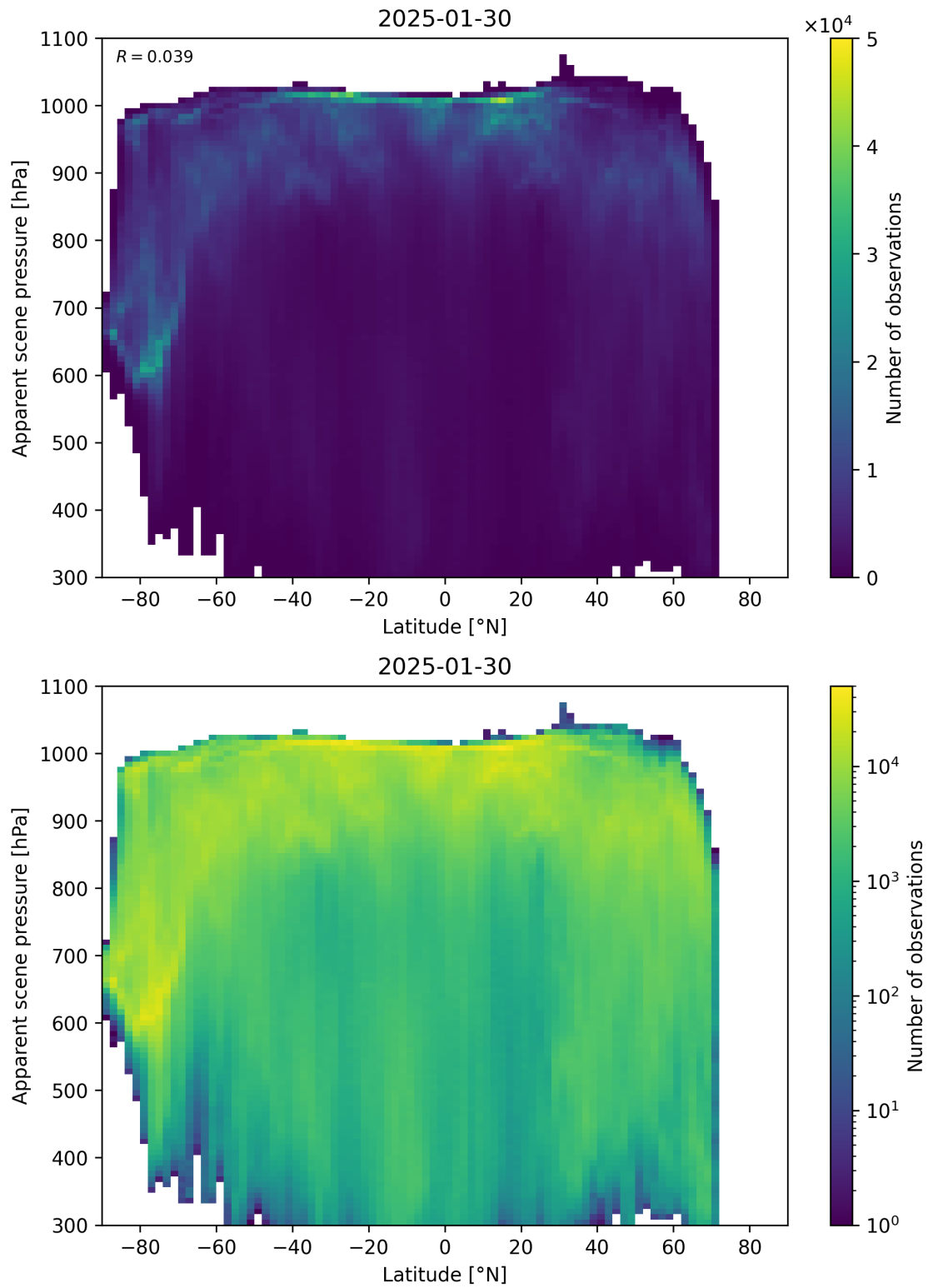
Figure 88: Scatter density plot of “Latitude” against “Apparent scene pressure” for 2025-01-29 to 2025-01-31.
