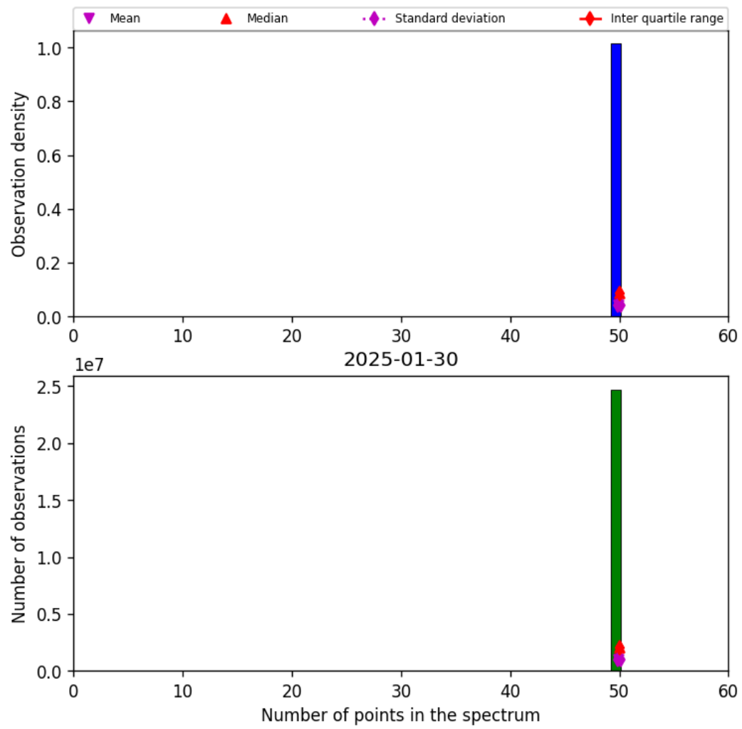
Figure 44: Histogram of “Number of points in the spectrum” for 2025-01-29 to 2025-01-31
