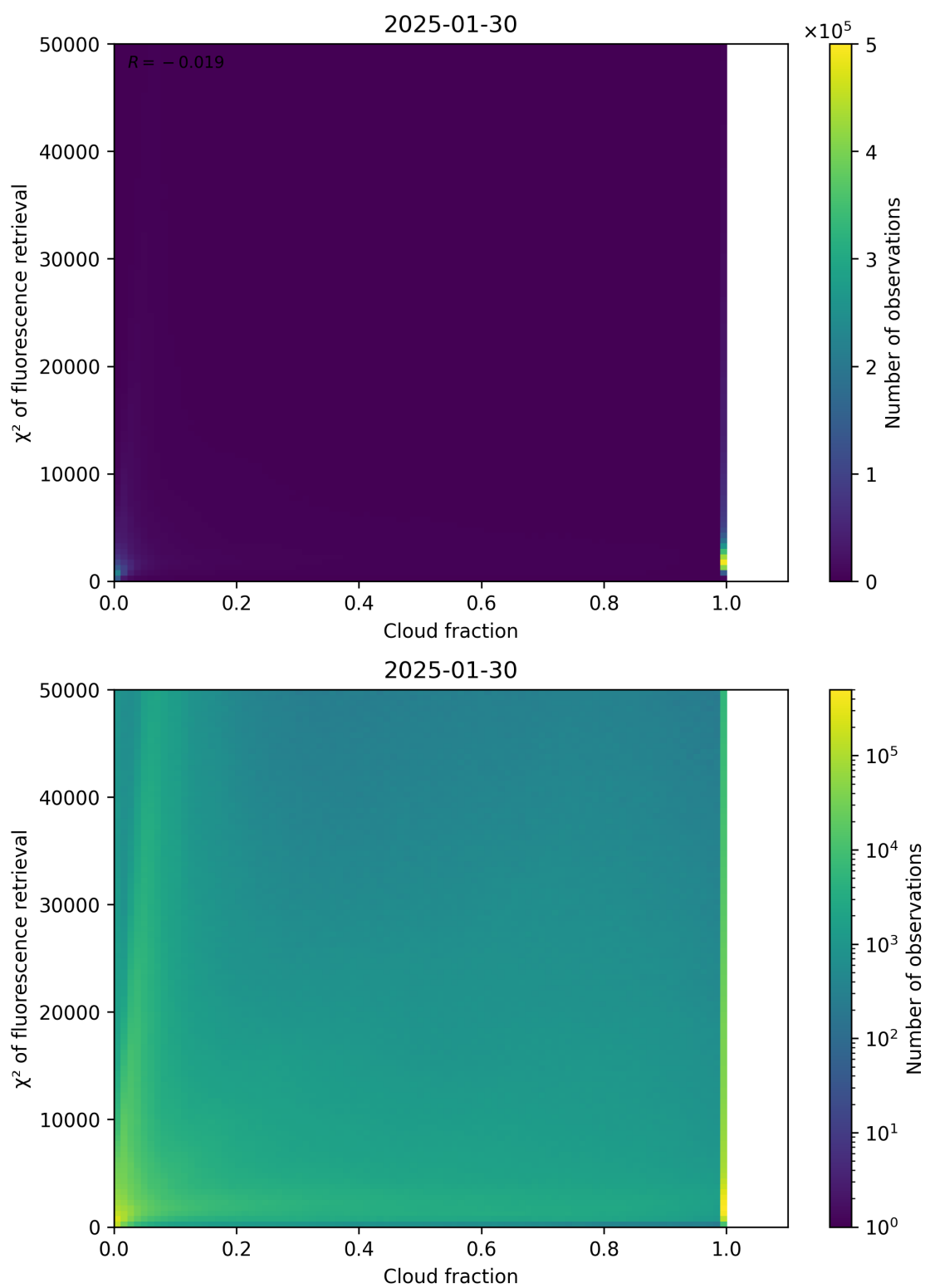
Figure 71: Scatter density plot of “Cloud fraction” against “ \chi^2 of fluorescence retrieval” for 2025-01-29 to 2025-01-31.
