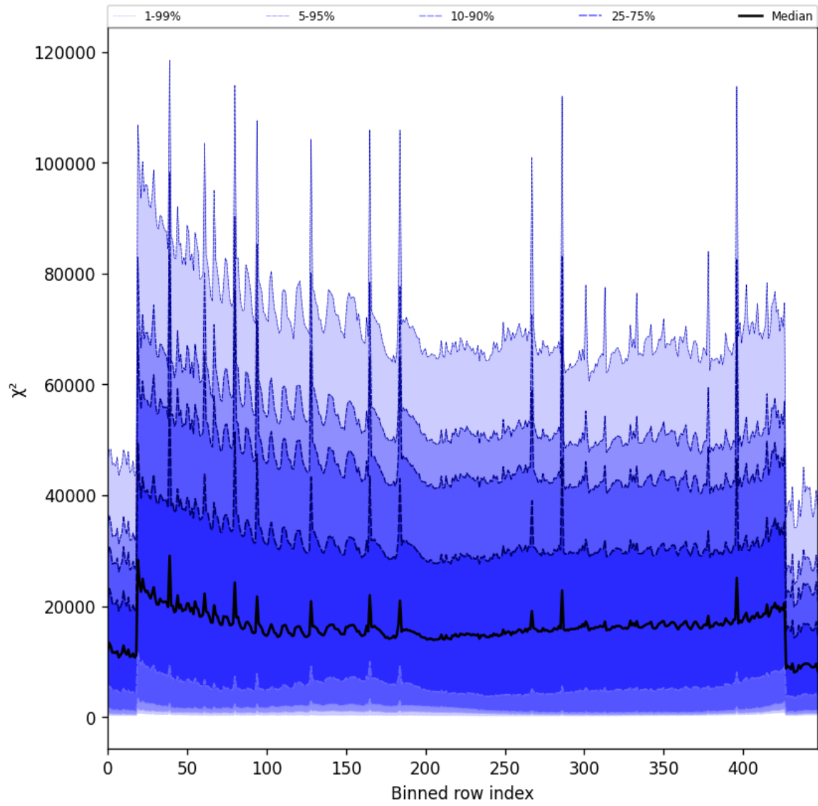
Figure 55: Along track statistics of " \chi^2 " for 2025-01-29 to 2025-01-31
