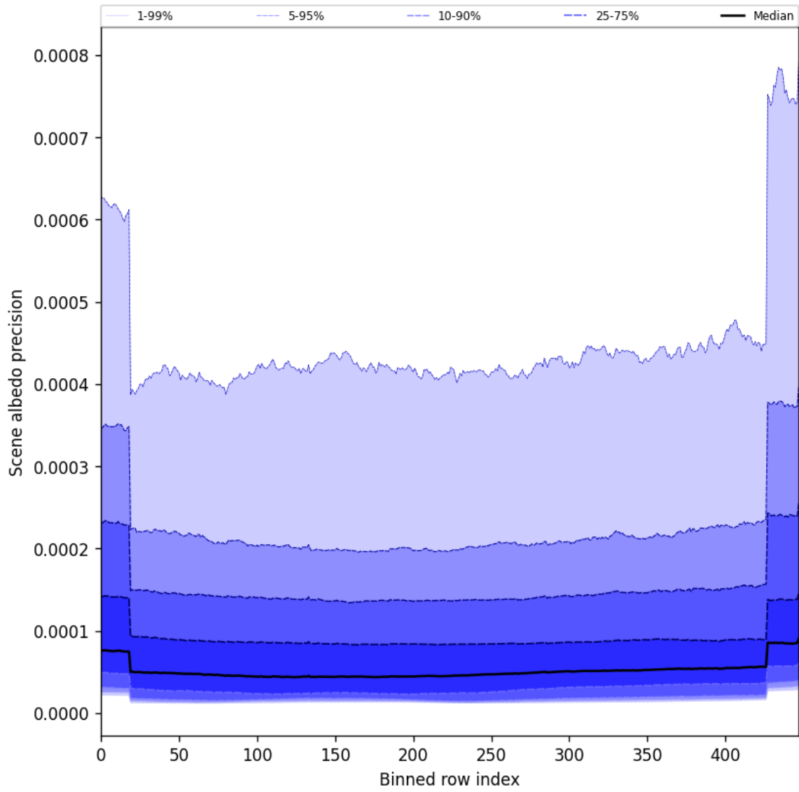
Figure 52: Along track statistics of “Scene albedo precision” for 2025-01-29 to 2025-01-31
