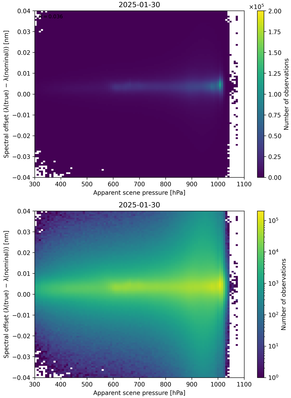
Figure 67: Scatter density plot of “Apparent scene pressure” against “Spectral offset ( \lambda_{\text{true}} - \lambda_{\text{nominal}} )” for 2025-01-29 to 2025-01-31.
