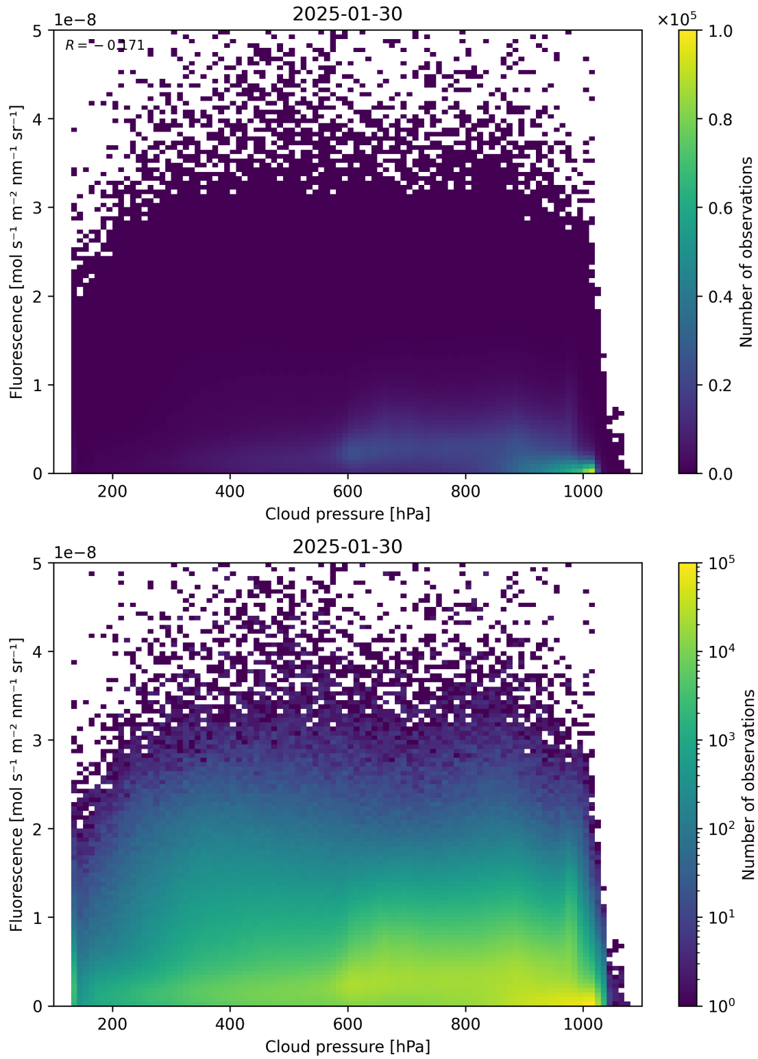
Figure 80: Scatter density plot of “Cloud pressure” against “Fluorescence” for 2025-01-29 to 2025-01-31.
