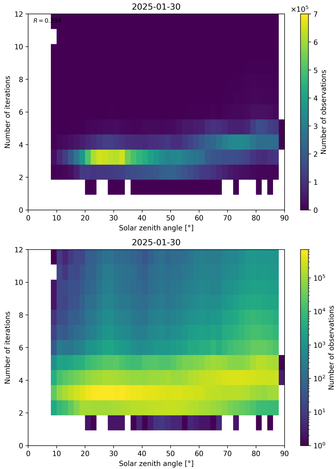
Figure 114: Scatter density plot of “Solar zenith angle” against “Number of iterations” for 2025-01-29 to 2025-01-31.
