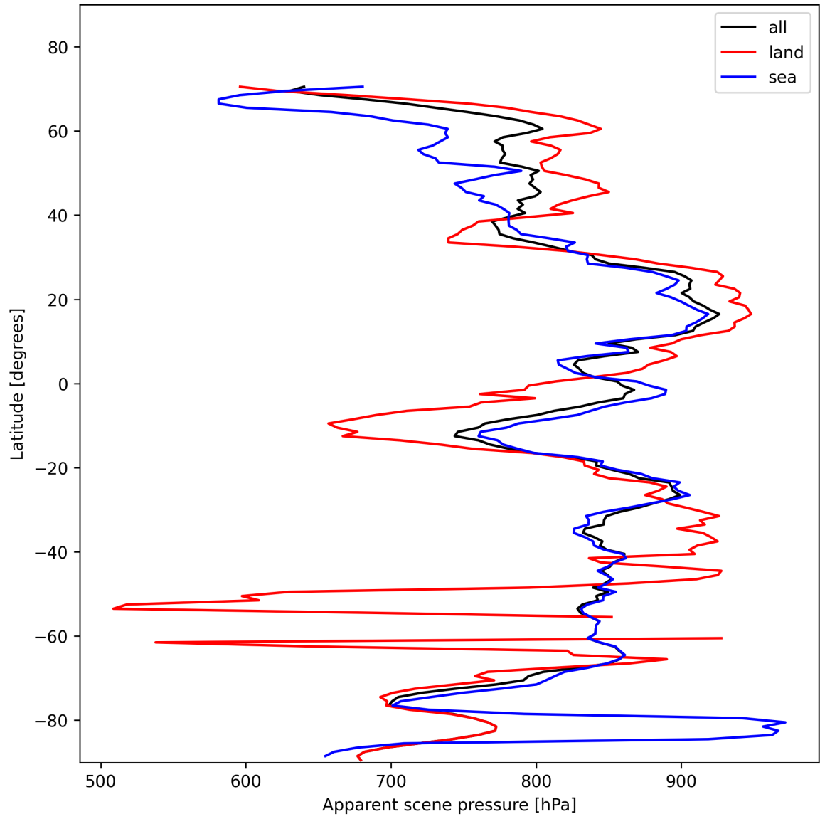
Figure 19: Zonal average of “Apparent scene pressure” for 2025-01-29 to 2025-01-31.
