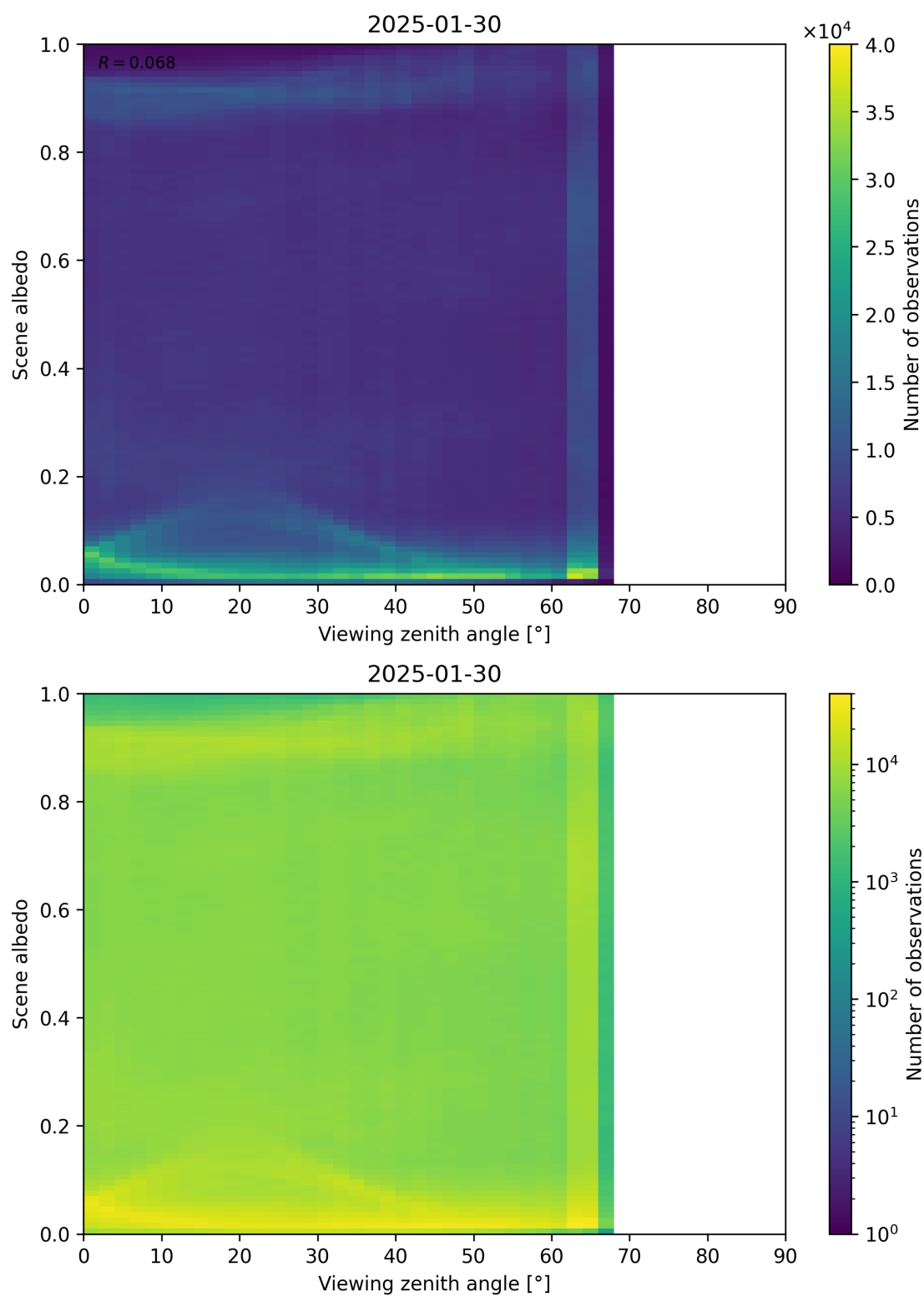
Figure 126: Scatter density plot of “Viewing zenith angle” against “Scene albedo” for 2025-01-29 to 2025-01-31.
