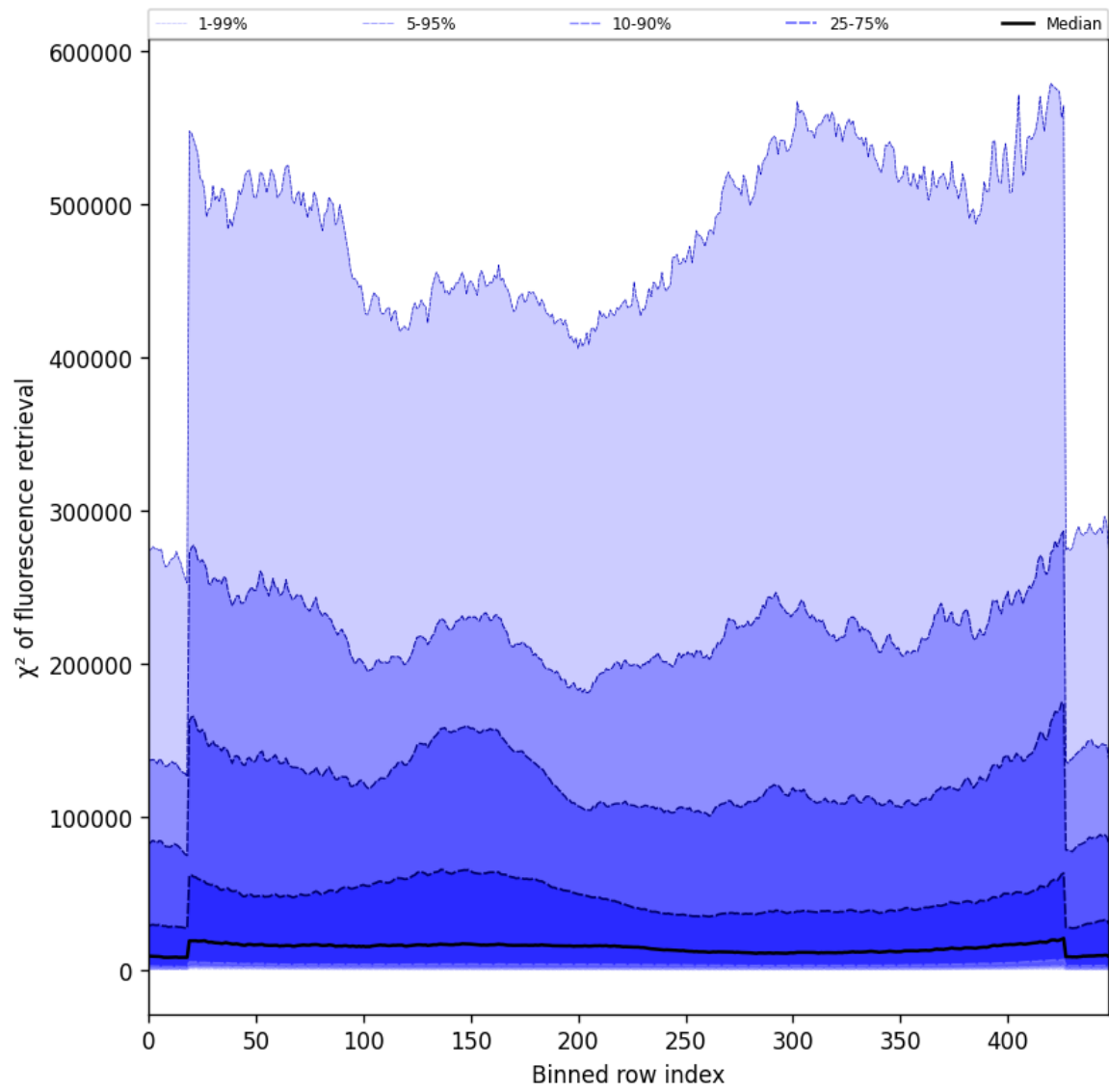
Figure 59: Along track statistics of “ \chi^2 of fluorescence retrieval” for 2025-01-29 to 2025-01-31
