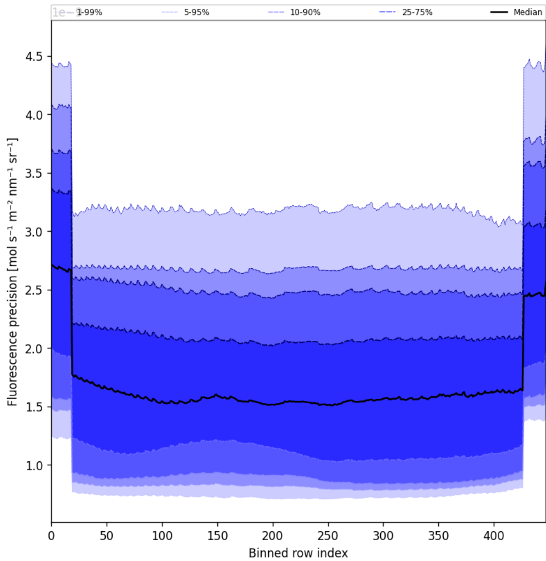
Figure 58: Along track statistics of “Fluorescence precision” for 2025-01-29 to 2025-01-31
