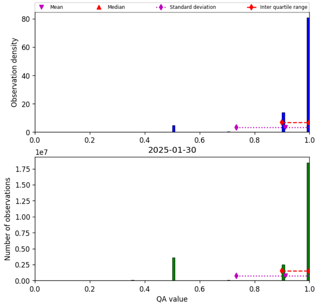
Figure 29: Histogram of “QA value” for 2025-01-29 to 2025-01-31
