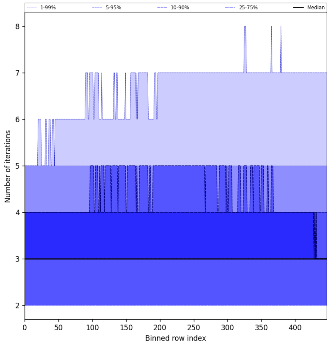
Figure 56: Along track statistics of “Number of iterations” for 2025-01-29 to 2025-01-31
