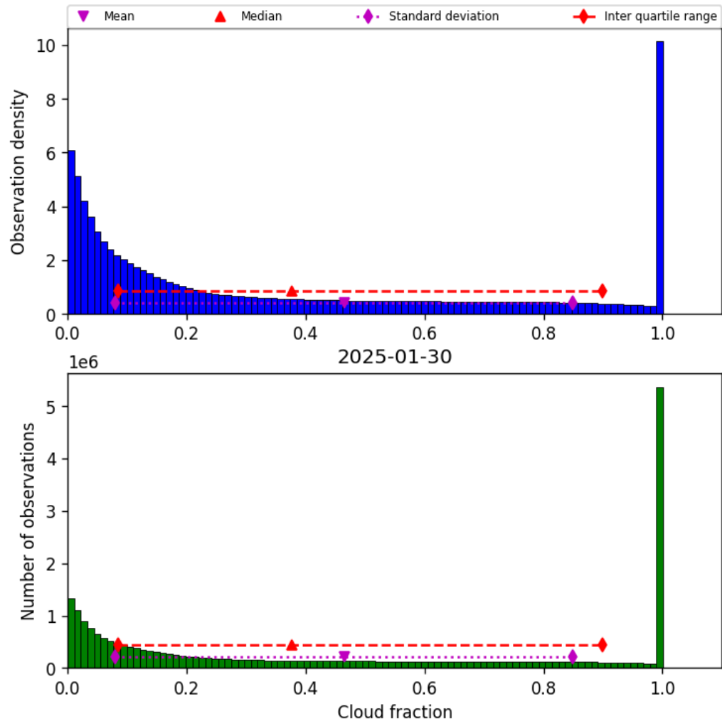
Figure 32: Histogram of “Cloud fraction” for 2025-01-29 to 2025-01-31
