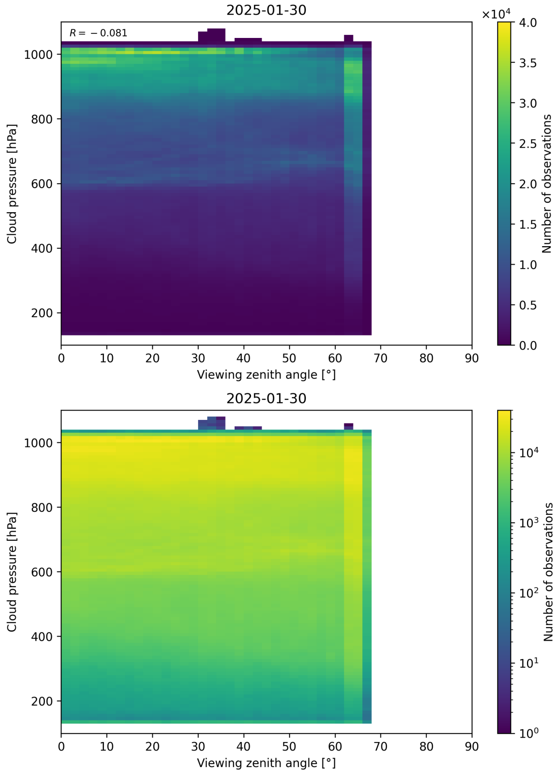
Figure 121: Scatter density plot of “Viewing zenith angle” against “Cloud pressure” for 2025-01-29 to 2025-01-31.
