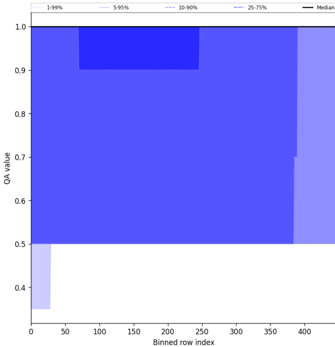
Figure 46: Along track statistics of “QA value” for 2025-01-29 to 2025-01-31
