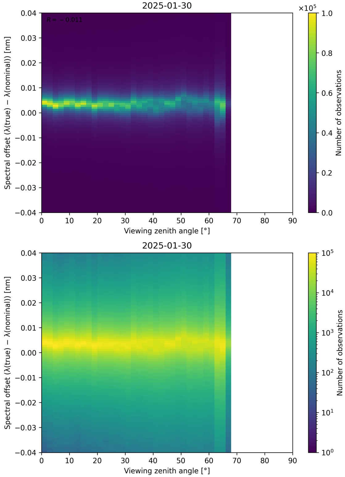
Figure 128: Scatter density plot of “Viewing zenith angle” against “Spectral offset ( \lambda_{\text{true}} - \lambda_{\text{nominal}} )” for 2025-01-29 to 2025-01-31.
