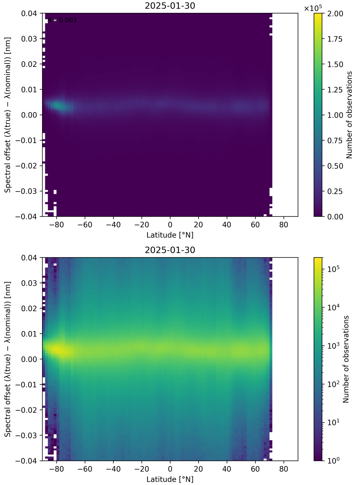
Figure 96: Scatter density plot of “Latitude” against “Spectral offset ( \lambda_{\text{true}} - \lambda_{\text{nominal}} )” for 2025-01-29 to 2025-01-31.
