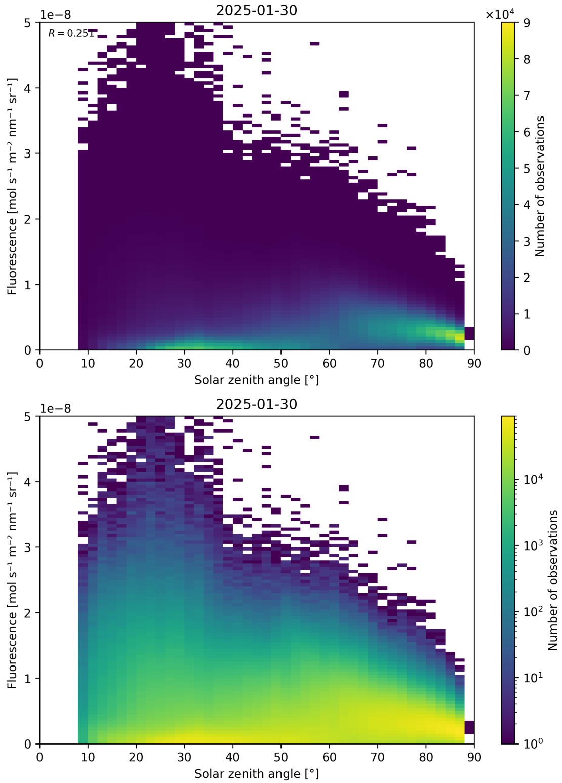
Figure 112: Scatter density plot of “Solar zenith angle” against “Fluorescence” for 2025-01-29 to 2025-01-31.
