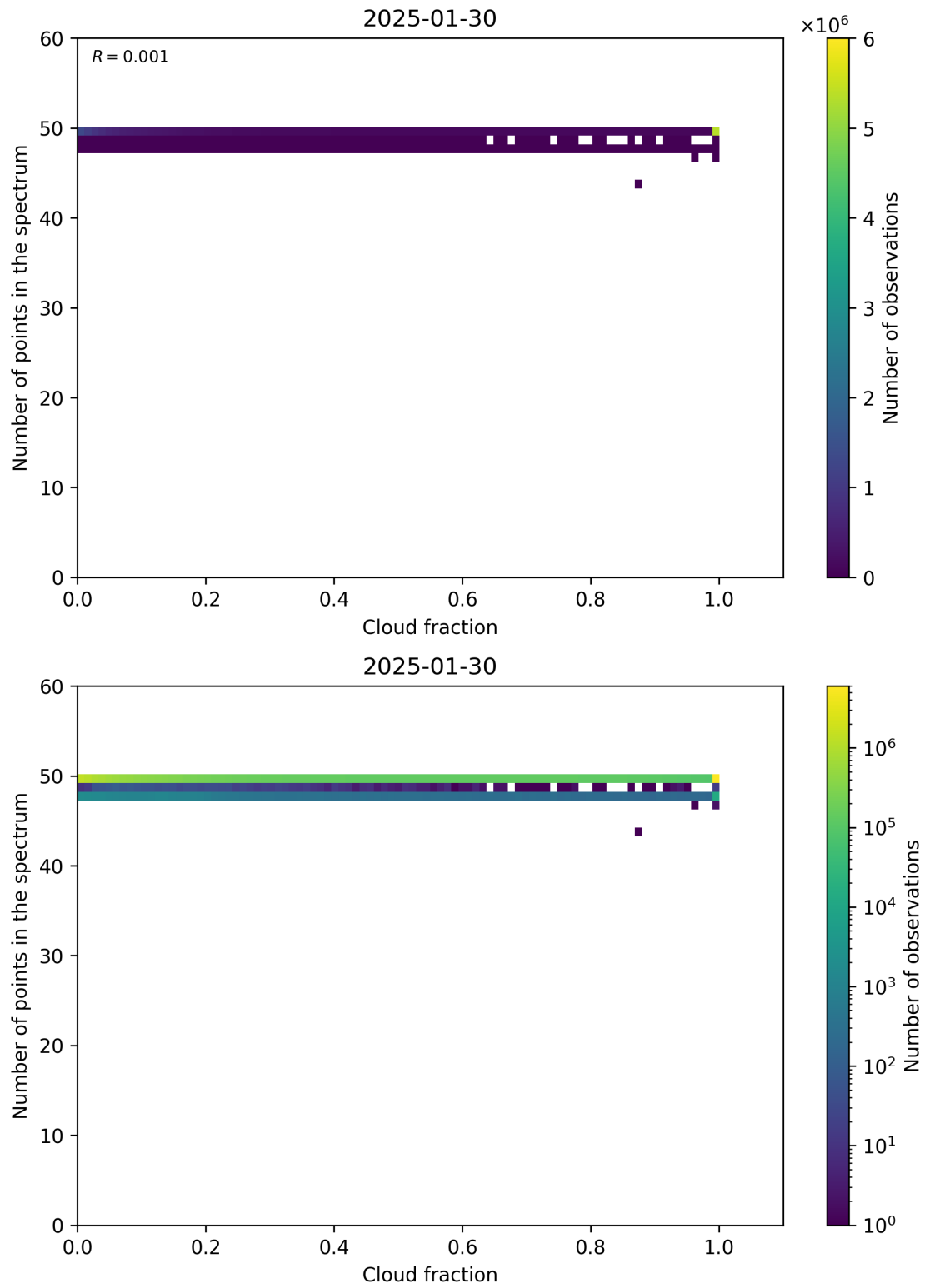
Figure 74: Scatter density plot of “Cloud fraction” against “Number of points in the spectrum” for 2025-01-29 to 2025-01-31.
