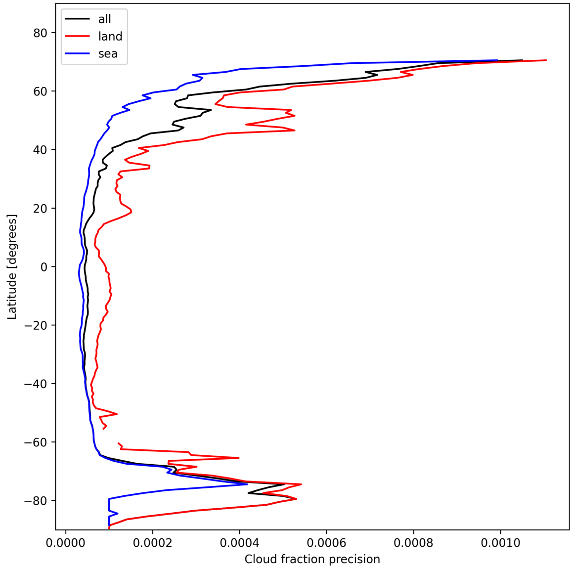
Figure 16: Zonal average of “Cloud fraction precision” for 2025-01-29 to 2025-01-31.
