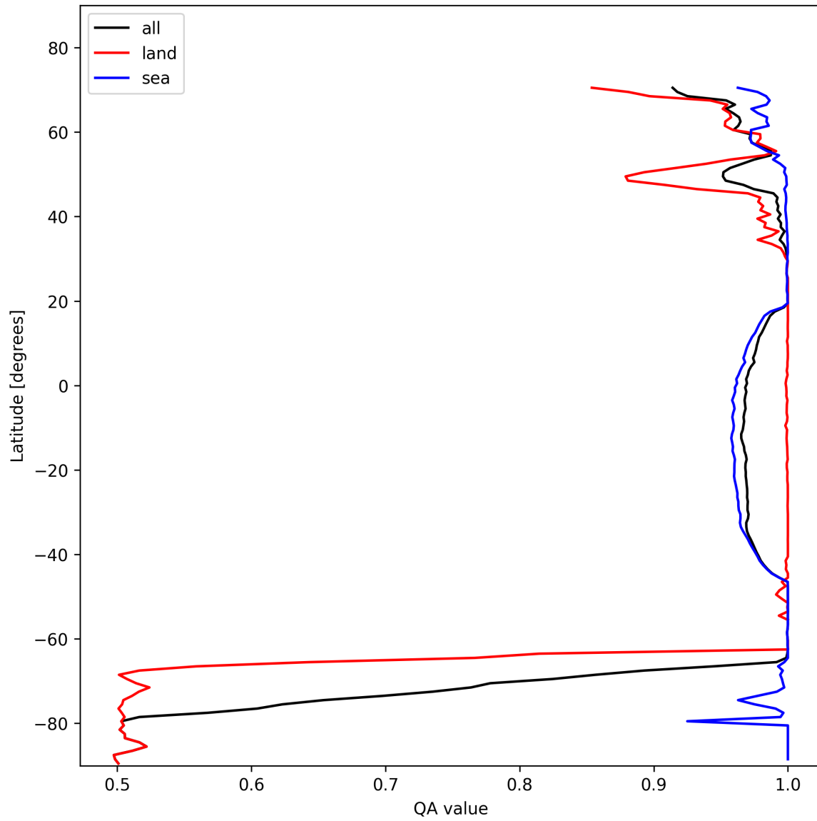
Figure 12: Zonal average of “QA value” for 2025-01-29 to 2025-01-31.
