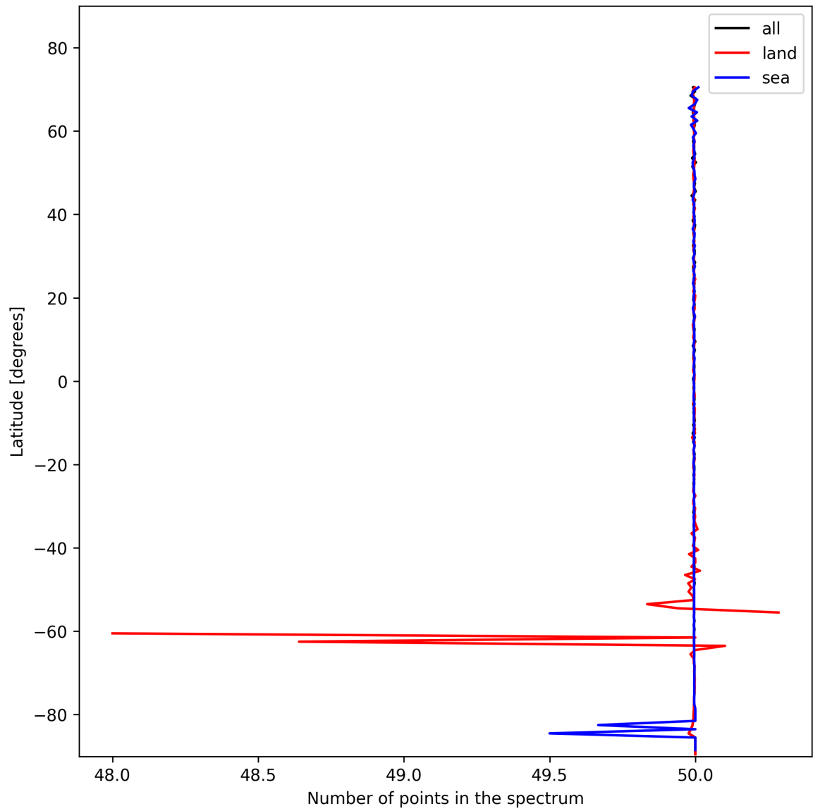
Figure 27: Zonal average of “Number of points in the spectrum” for 2025-01-29 to 2025-01-31.
