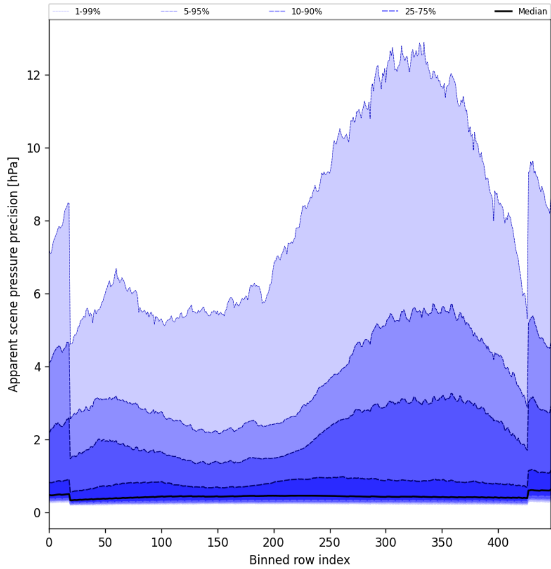
Figure 54: Along track statistics of “Apparent scene pressure precision” for 2025-01-29 to 2025-01-31
