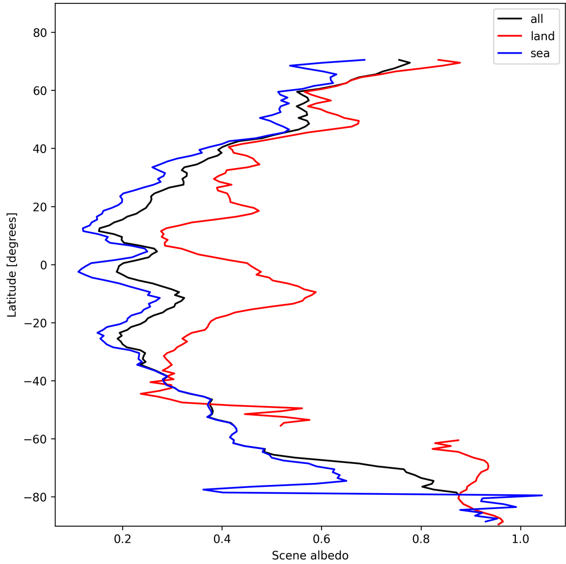
Figure 17: Zonal average of “Scene albedo” for 2025-01-29 to 2025-01-31.
