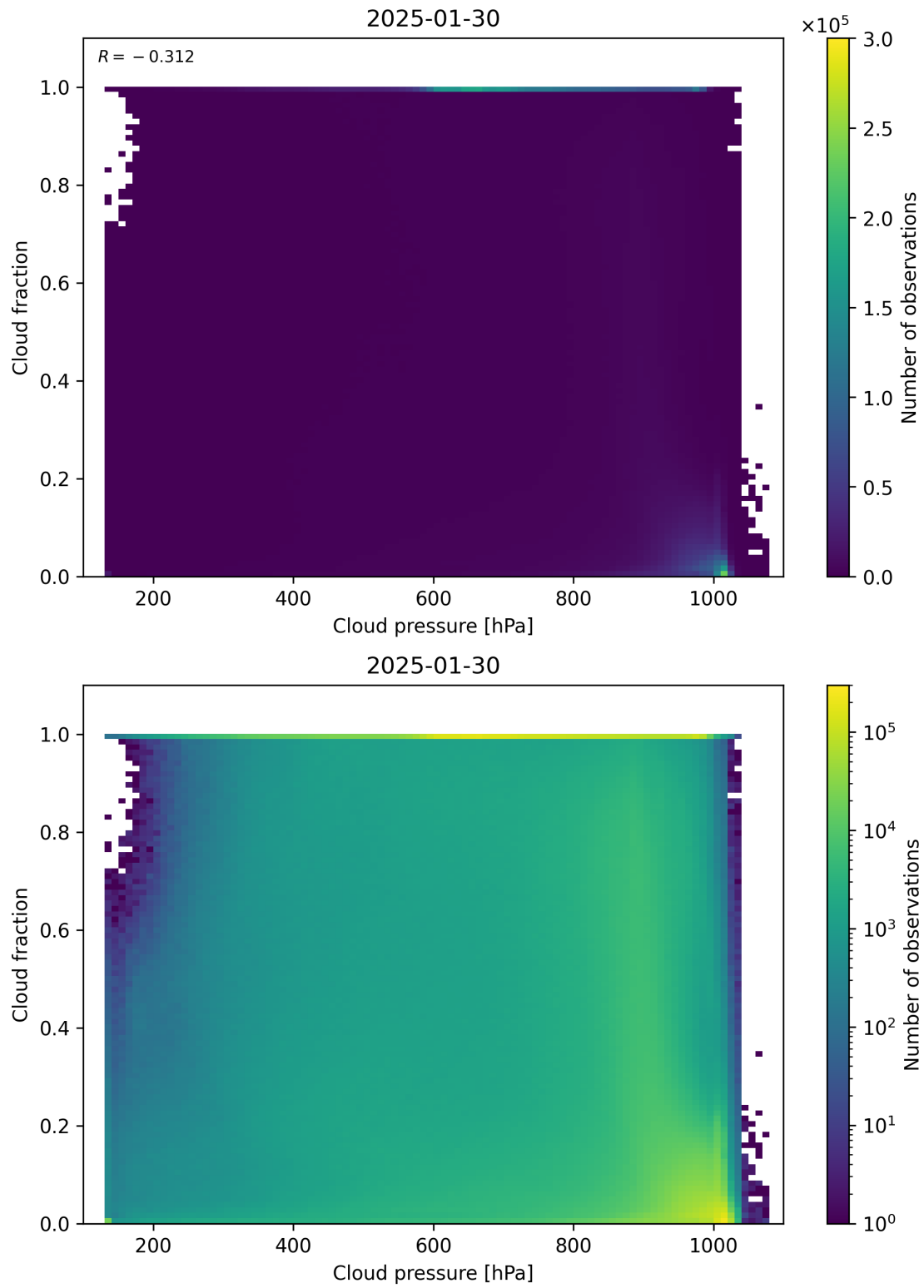
Figure 79: Scatter density plot of “Cloud pressure” against “Cloud fraction” for 2025-01-29 to 2025-01-31.
