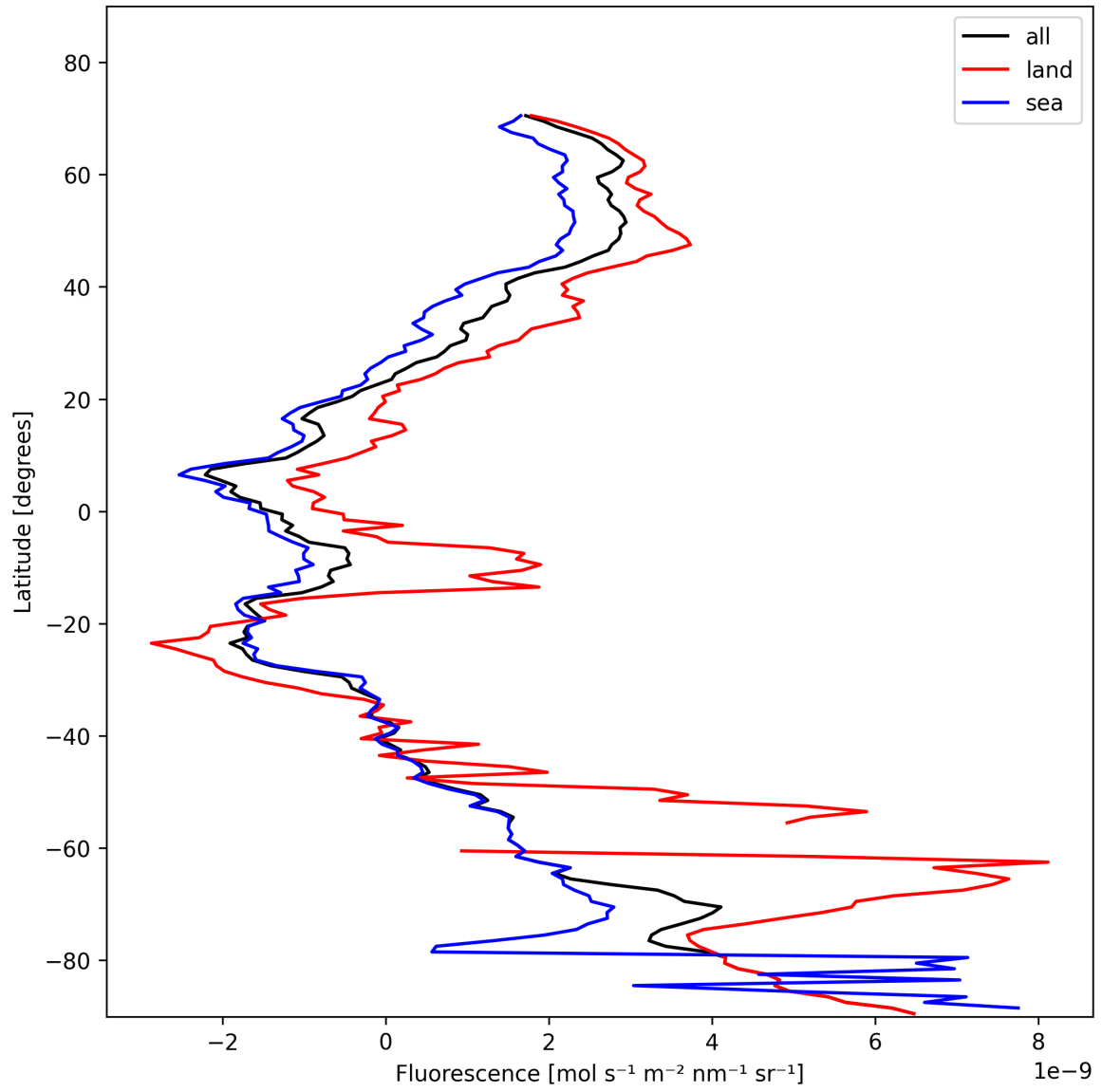
Figure 23: Zonal average of “Fluorescence” for 2025-01-29 to 2025-01-31.
