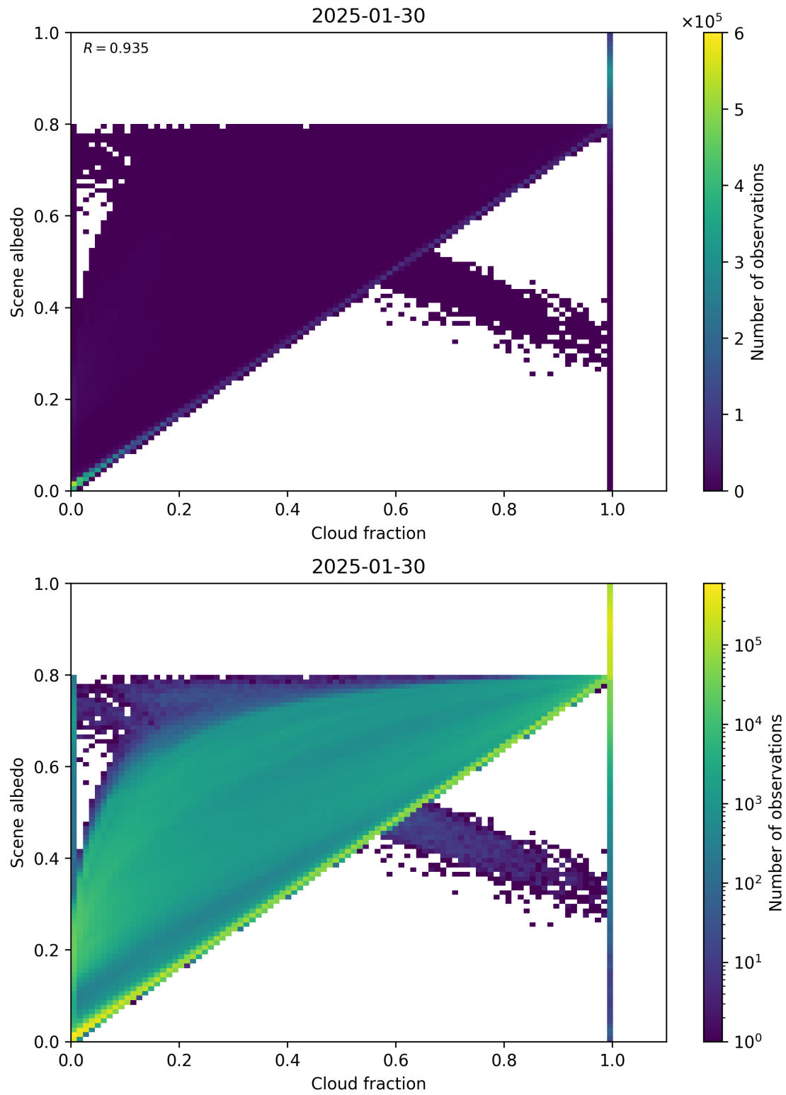
Figure 75: Scatter density plot of “Cloud fraction” against “Scene albedo” for 2025-01-29 to 2025-01-31.
