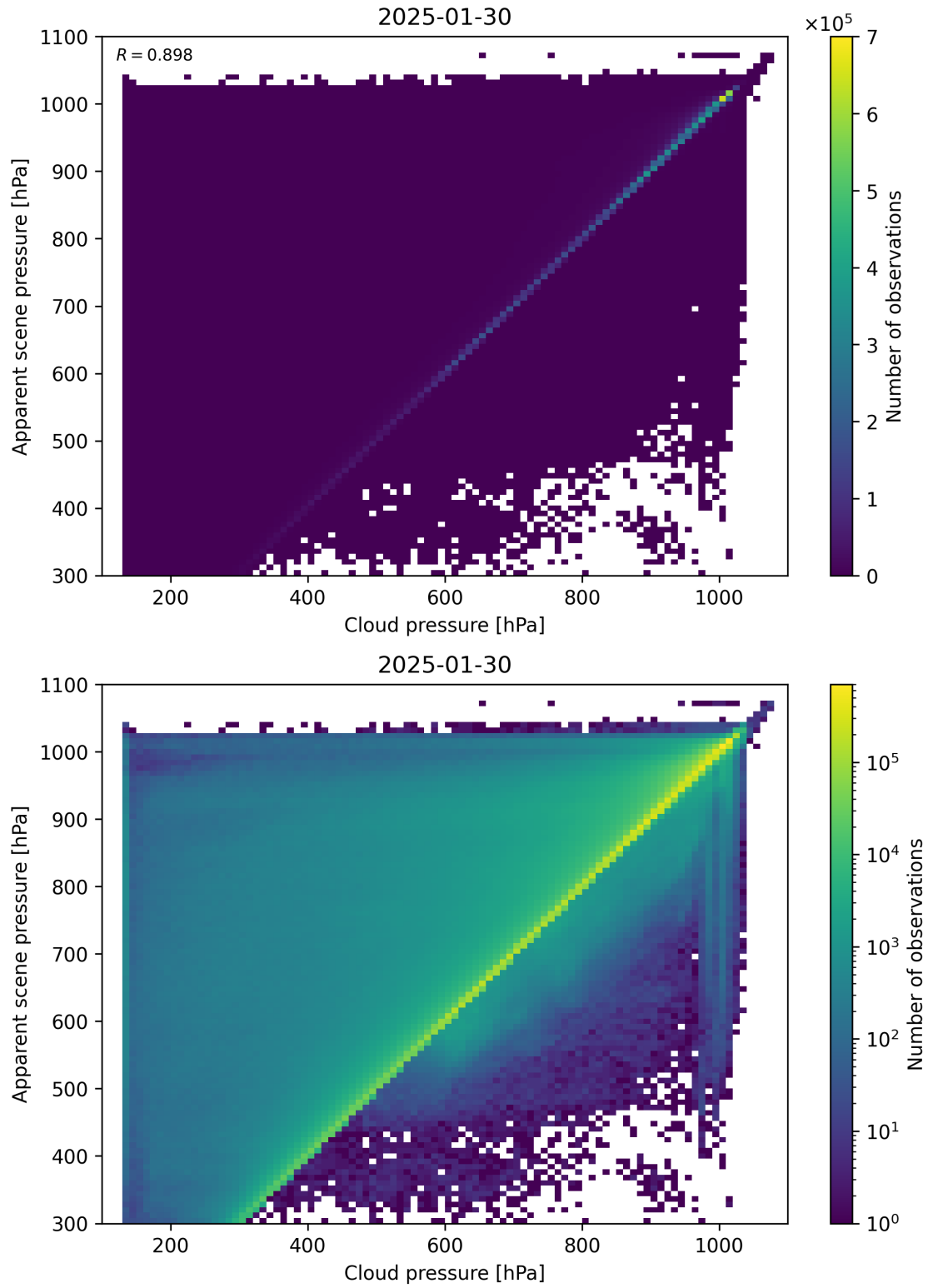
Figure 77: Scatter density plot of “Cloud pressure” against “Apparent scene pressure” for 2025-01-29 to 2025-01-31.
