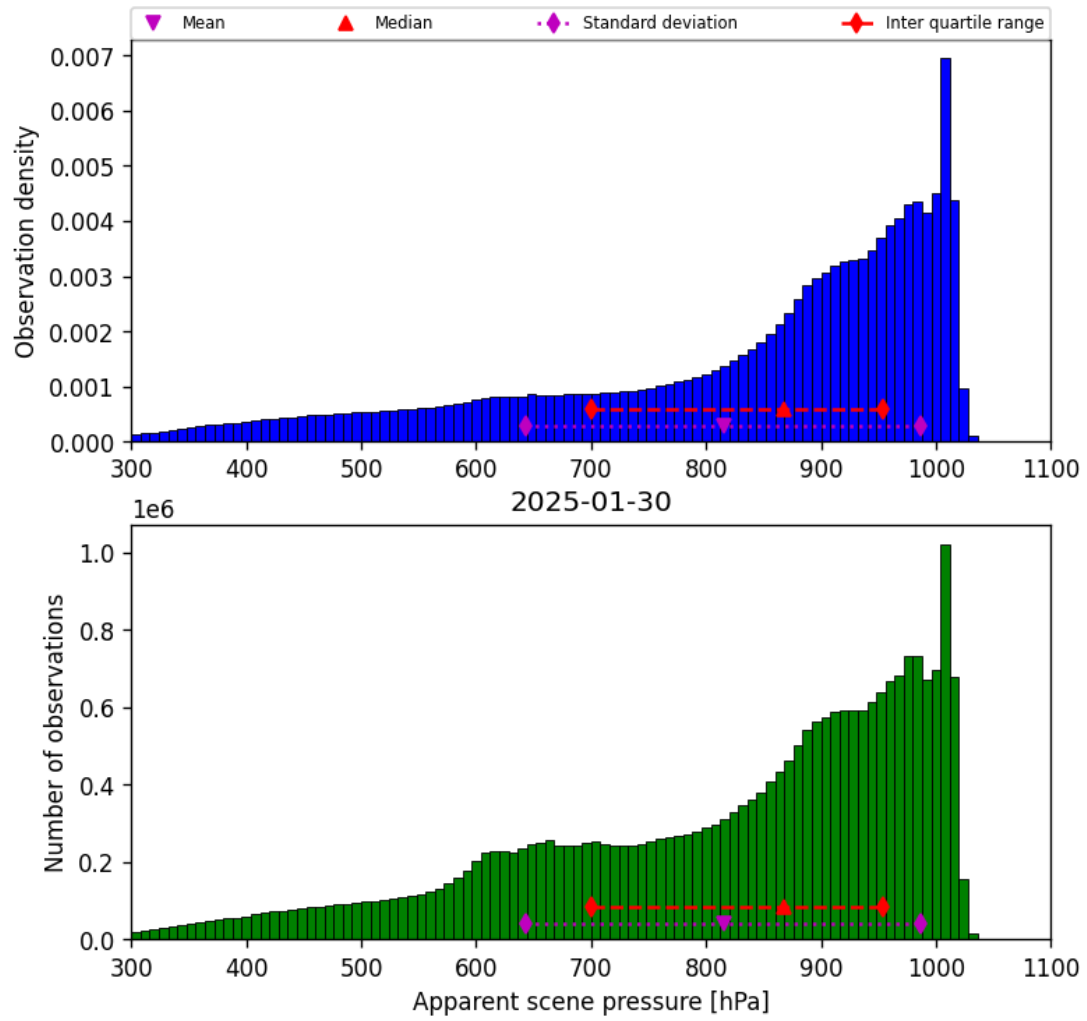
Figure 36: Histogram of “Apparent scene pressure” for 2025-01-29 to 2025-01-31
