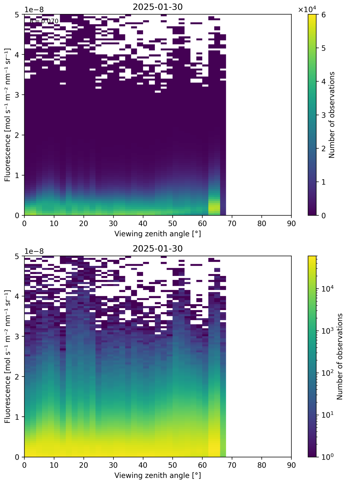
Figure 122: Scatter density plot of “Viewing zenith angle” against “Fluorescence” for 2025-01-29 to 2025-01-31.
