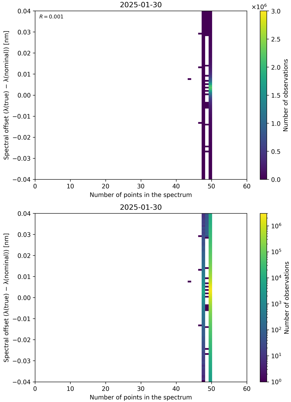
Figure 101: Scatter density plot of “Number of points in the spectrum” against “Spectral offset ( \lambda_{\text{true}} - \lambda_{\text{nominal}} )” for 2025-01-29 to 2025-01-31.
