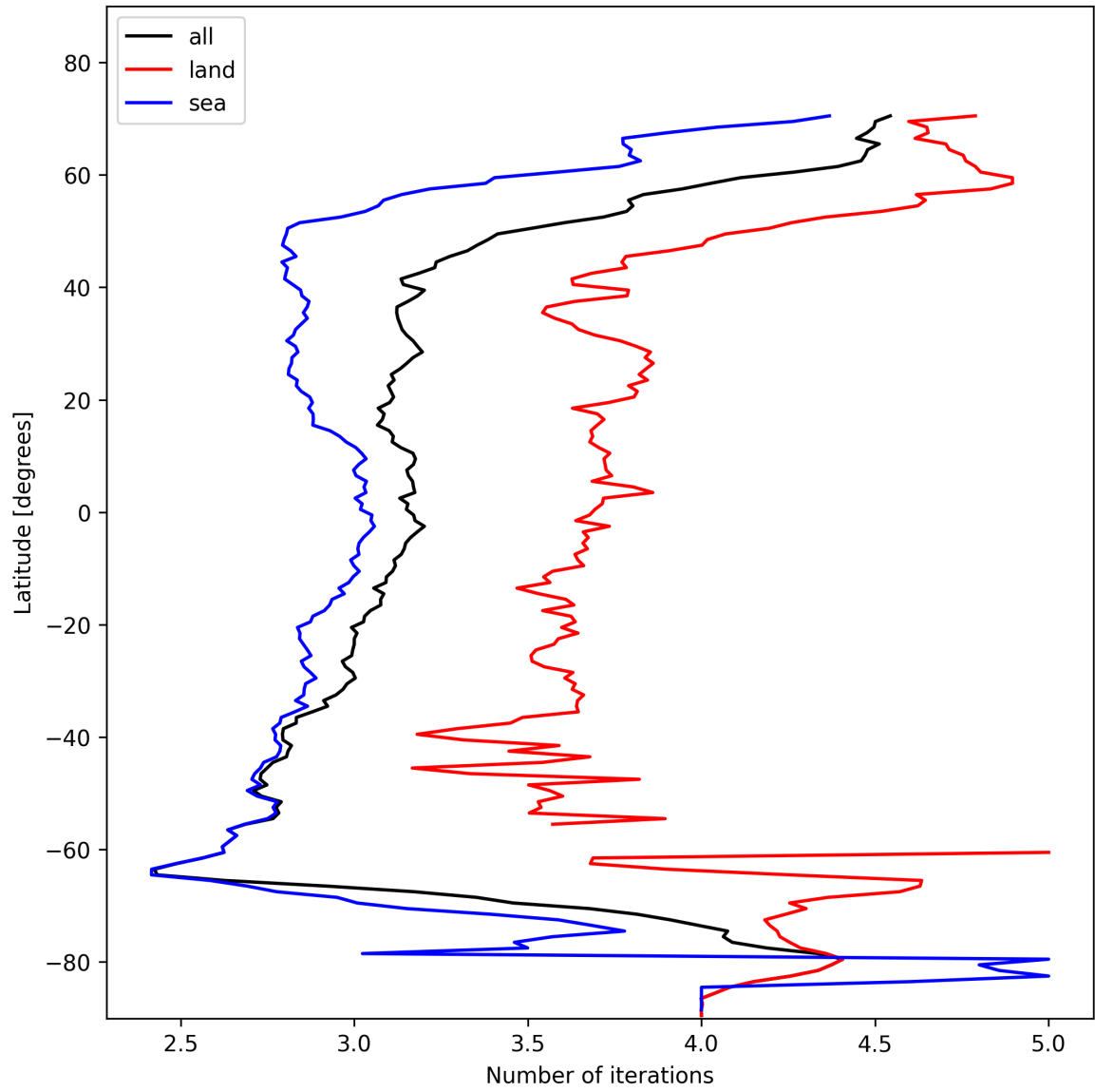
Figure 22: Zonal average of “Number of iterations” for 2025-01-29 to 2025-01-31.
