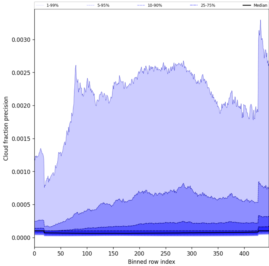
Figure 50: Along track statistics of “Cloud fraction precision” for 2025-01-29 to 2025-01-31
