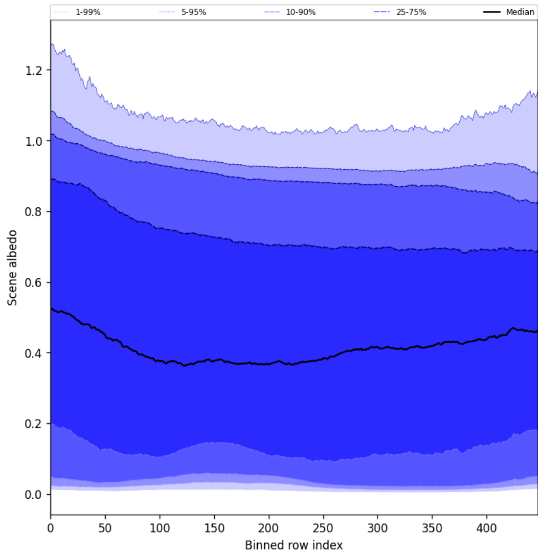
Figure 51: Along track statistics of “Scene albedo” for 2025-01-29 to 2025-01-31
