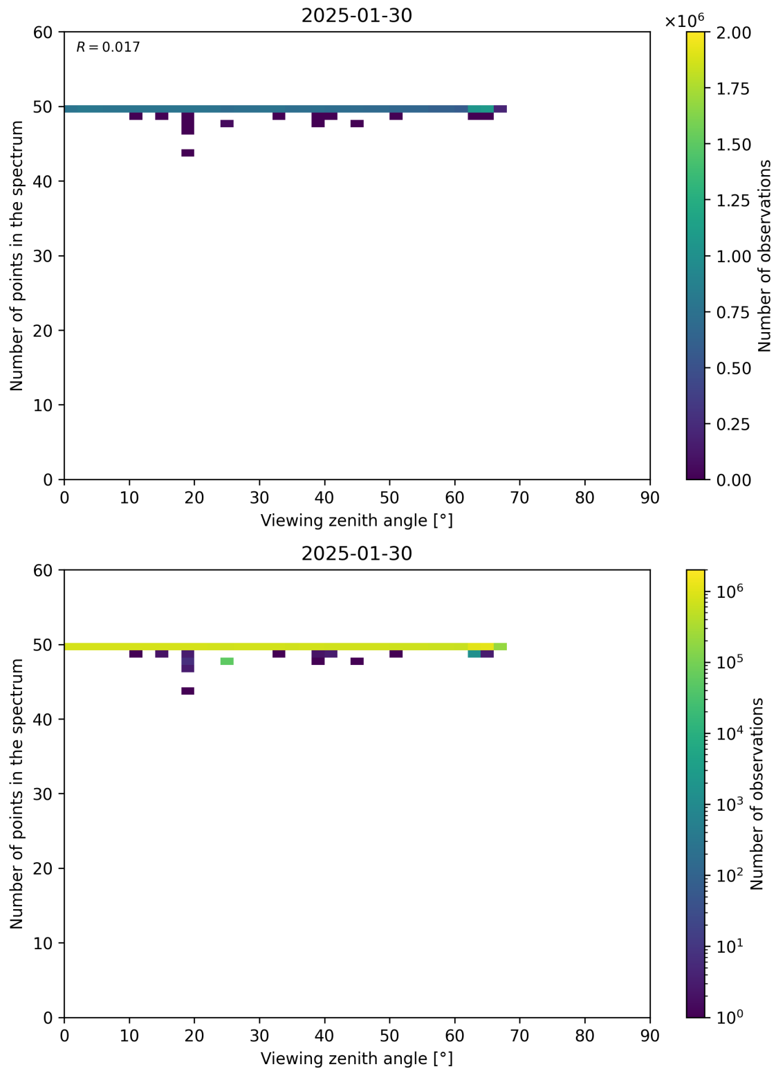
Figure 125: Scatter density plot of “Viewing zenith angle” against “Number of points in the spectrum” for 2025-01-29 to 2025-01-31.
