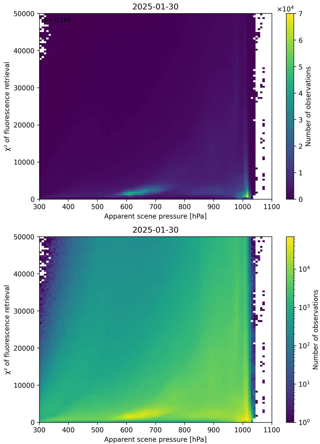
Figure 63: Scatter density plot of “Apparent scene pressure” against “ \chi^2 of fluorescence retrieval” for 2025-01-29 to 2025-01-31.
