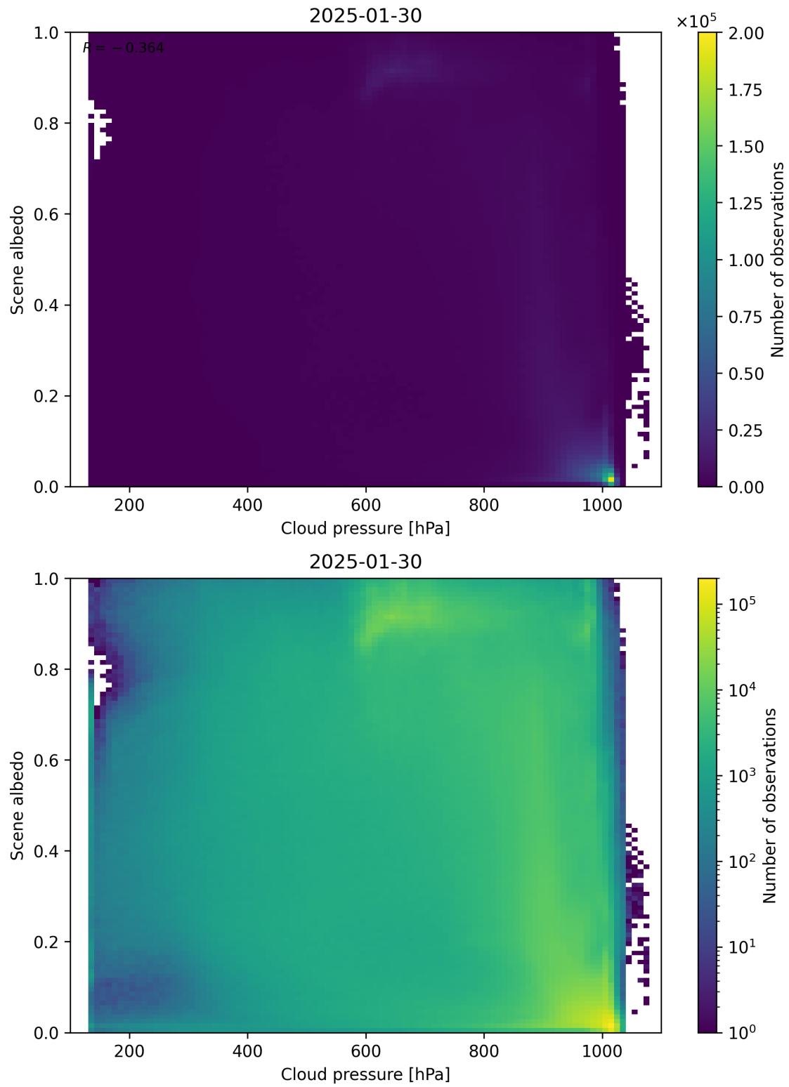
Figure 83: Scatter density plot of “Cloud pressure” against “Scene albedo” for 2025-01-29 to 2025-01-31.
