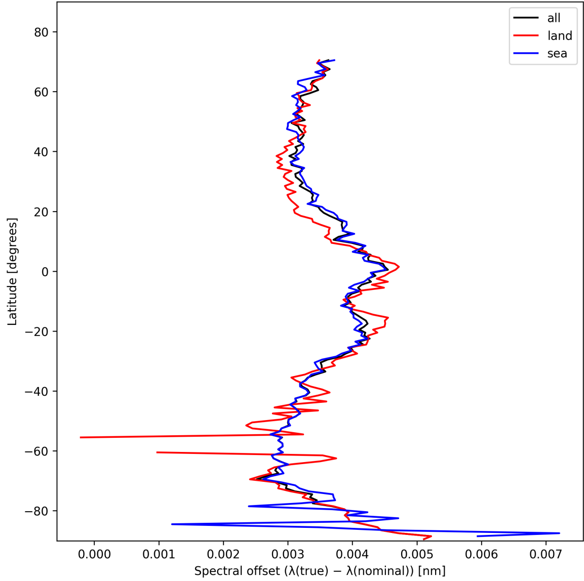
Figure 28: Zonal average of “Spectral offset ( \lambda_{\text{true}} - \lambda_{\text{nominal}} )” for 2025-01-29 to 2025-01-31.
