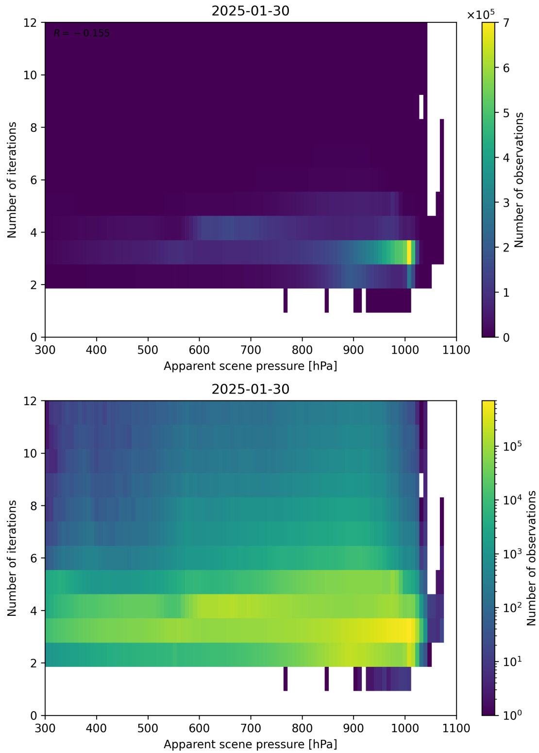
Figure 65: Scatter density plot of “Apparent scene pressure” against “Number of iterations” for 2025-01-29 to 2025-01-31.
