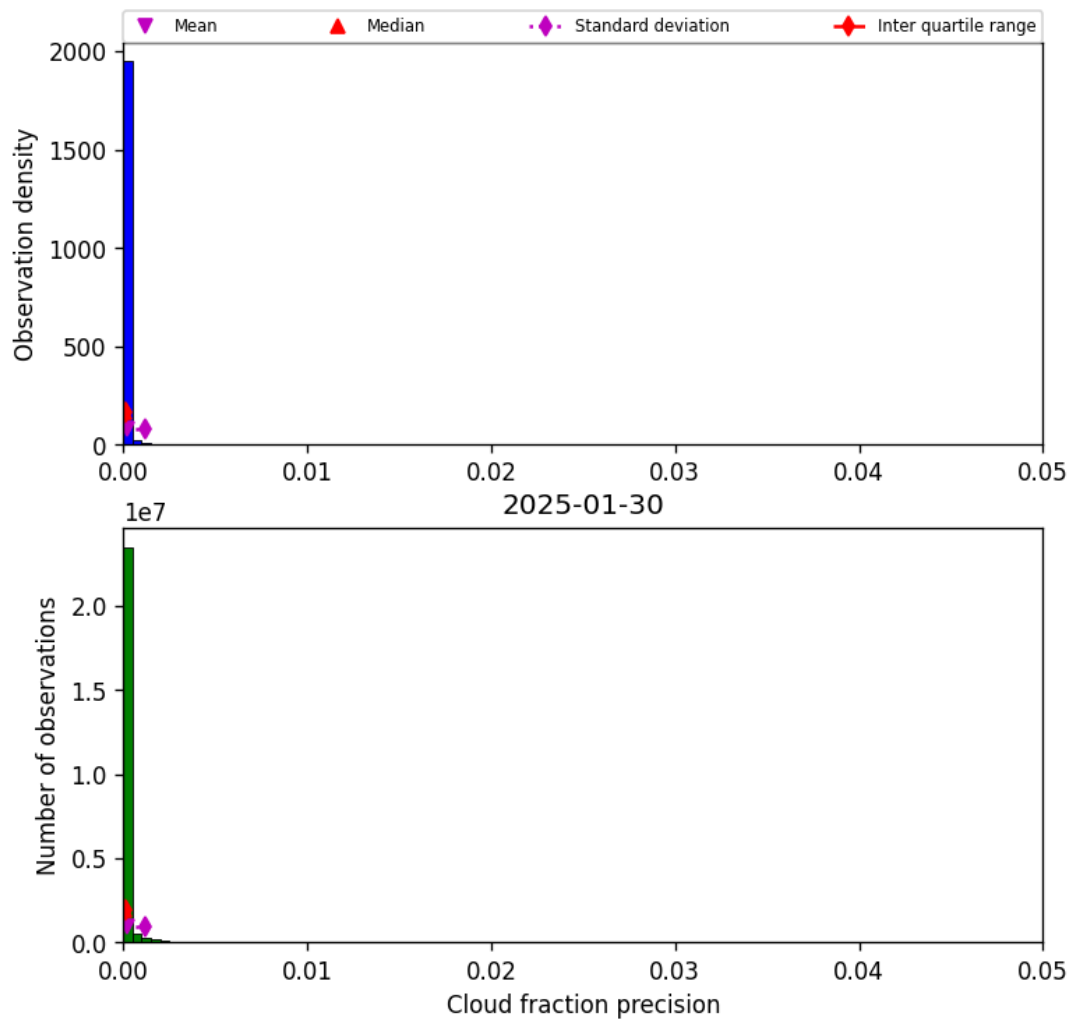
Figure 33: Histogram of “Cloud fraction precision” for 2025-01-29 to 2025-01-31
