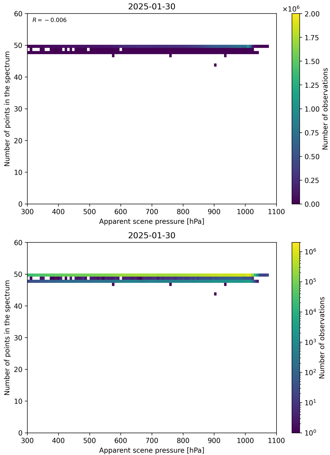
Figure 66: Scatter density plot of “Apparent scene pressure” against “Number of points in the spectrum” for 2025-01-29 to 2025-01-31.
