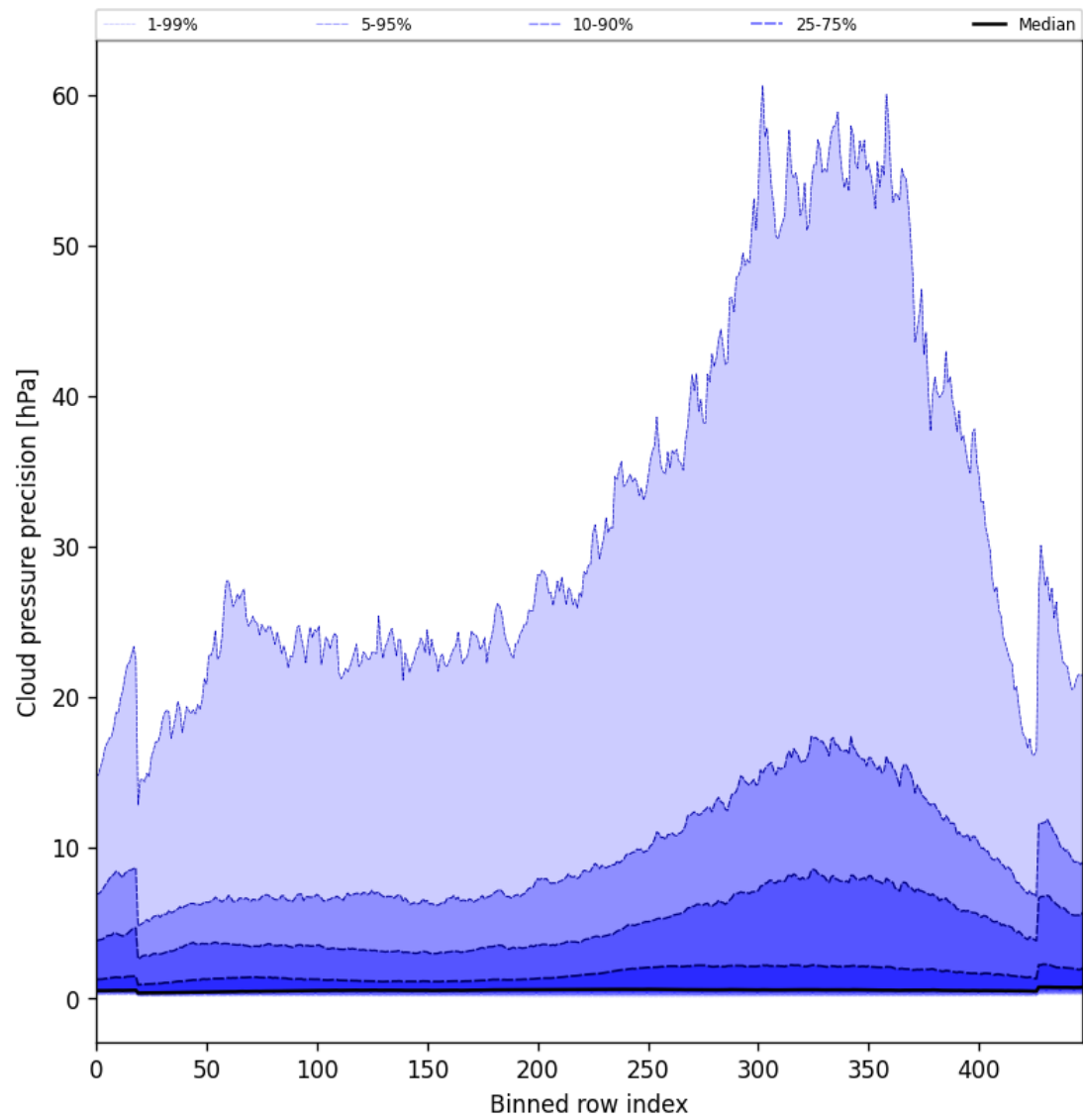
Figure 48: Along track statistics of “Cloud pressure precision” for 2025-01-29 to 2025-01-31
