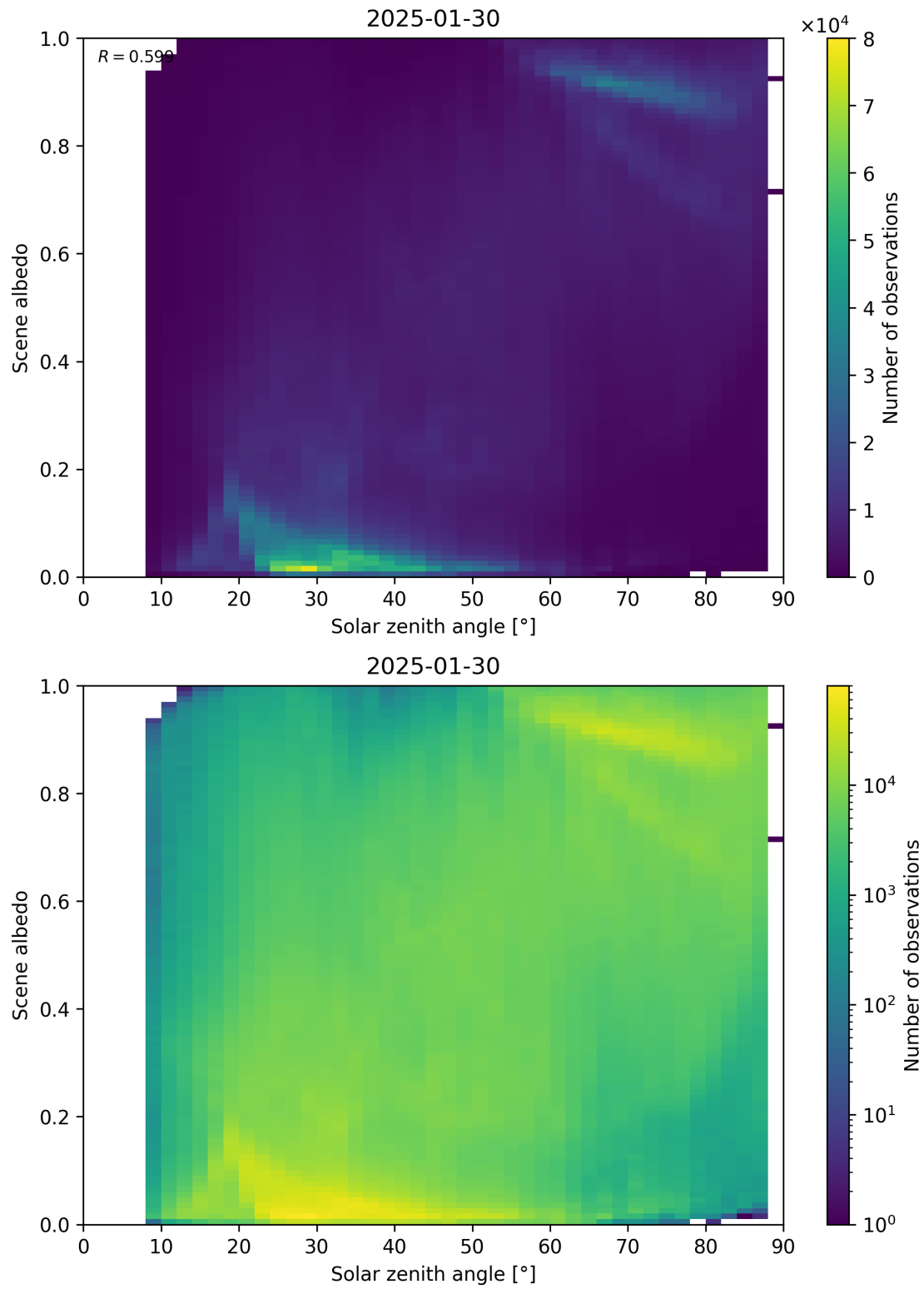
Figure 116: Scatter density plot of “Solar zenith angle” against “Scene albedo” for 2025-01-29 to 2025-01-31.
