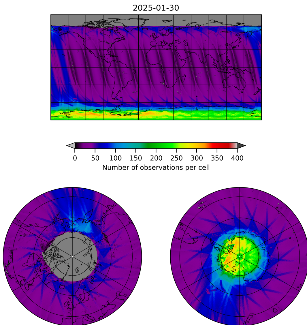
Figure 11: Map of the number of observations for 2025-01-29 to 2025-01-31
