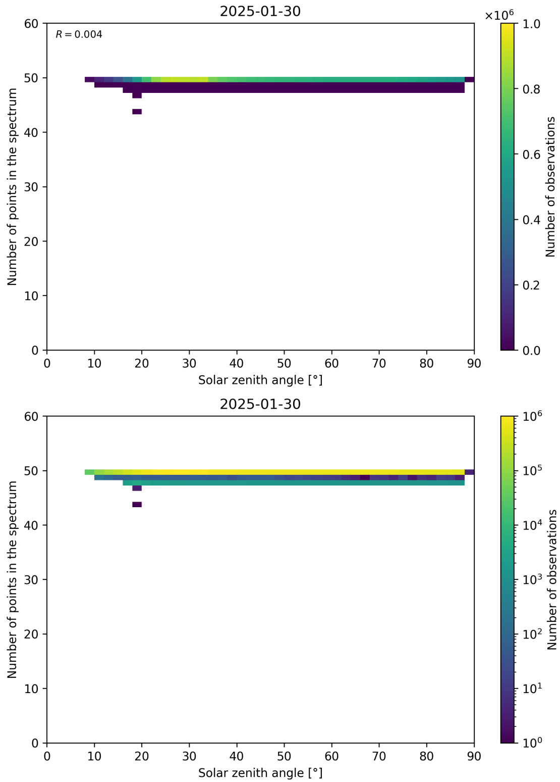
Figure 115: Scatter density plot of “Solar zenith angle” against “Number of points in the spectrum” for 2025-01-29 to 2025-01-31.
