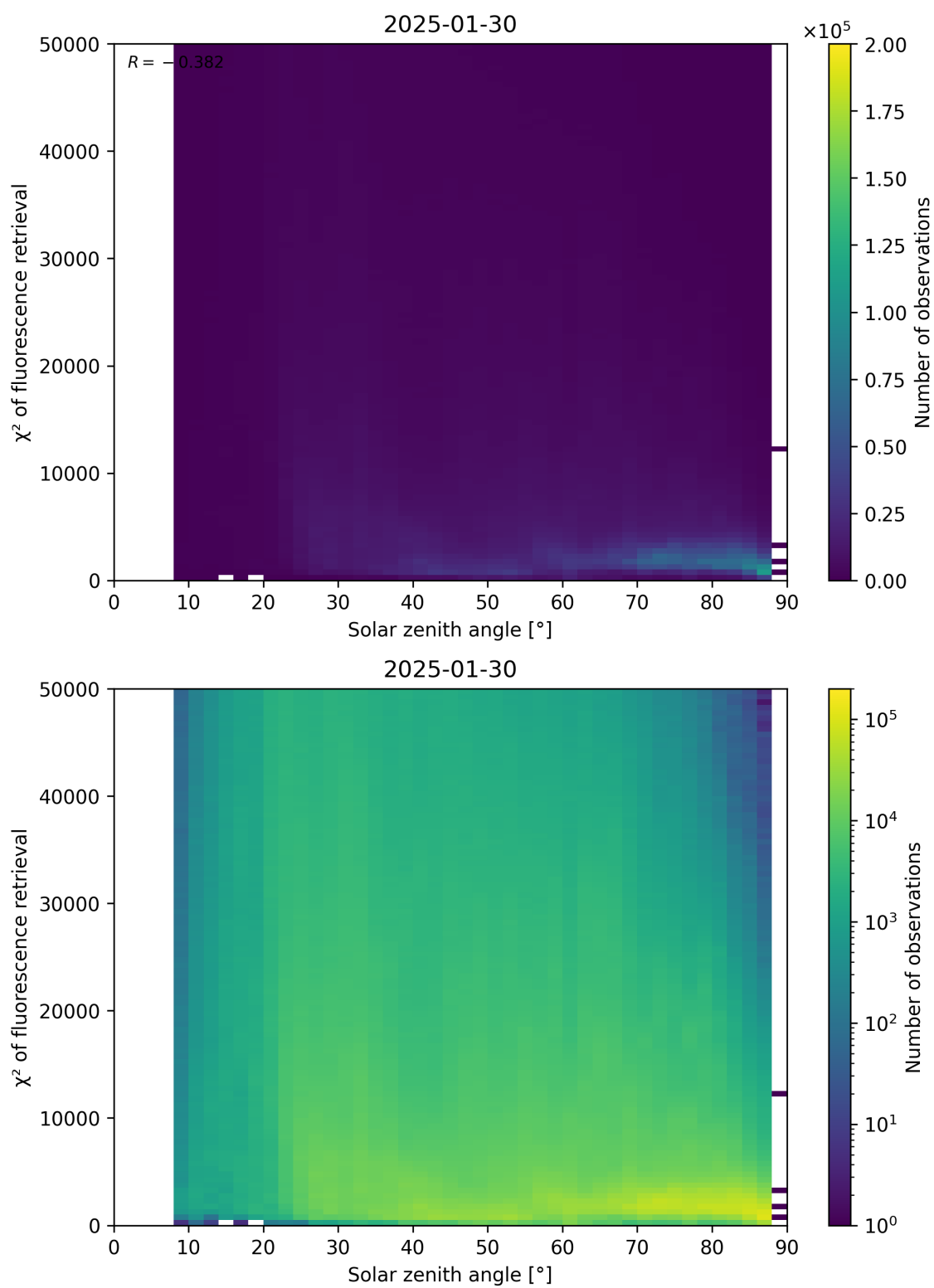
Figure 109: Scatter density plot of “Solar zenith angle” against “ \chi^2 of fluorescence retrieval” for 2025-01-29 to 2025-01-31.
