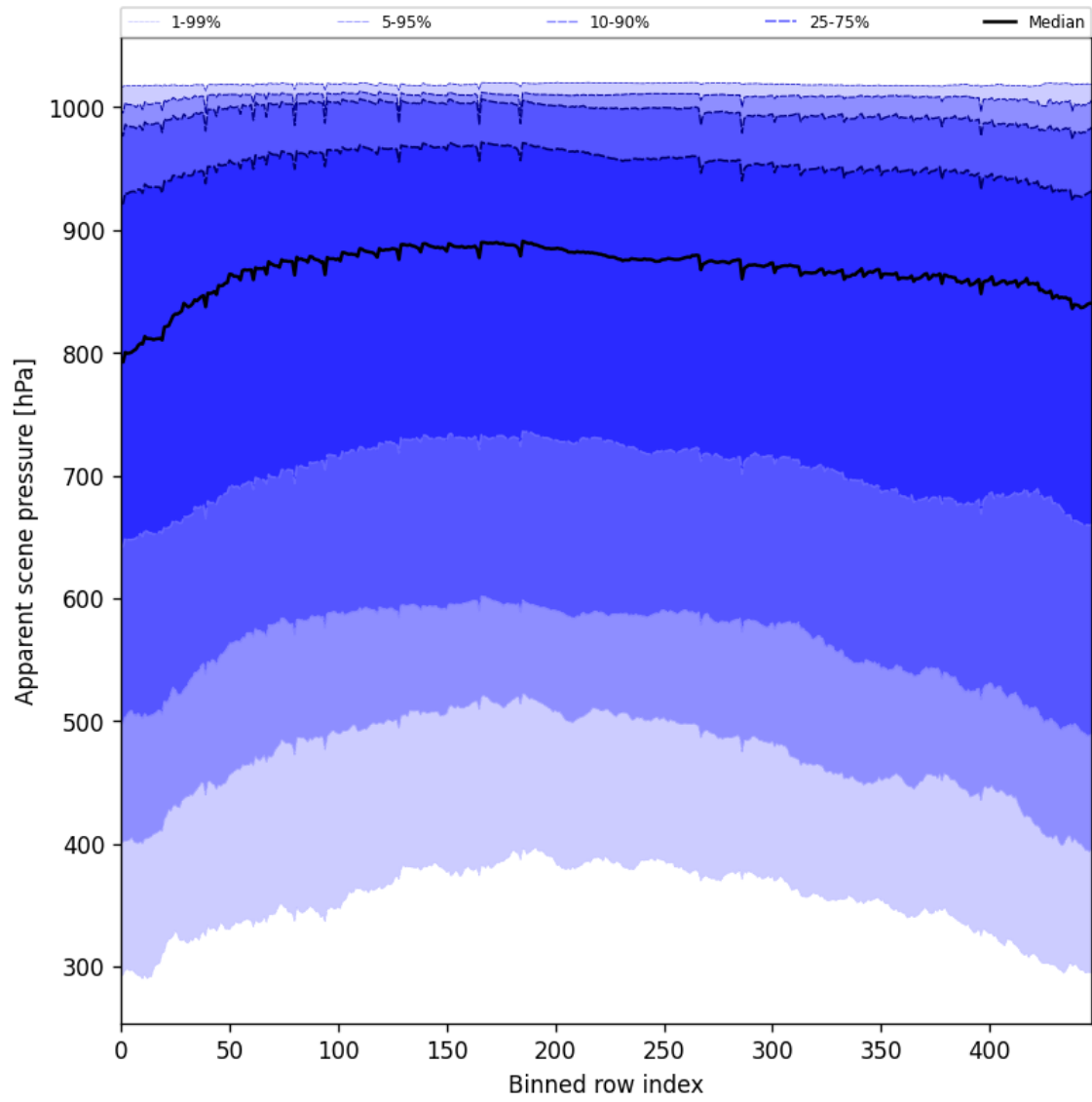
Figure 53: Along track statistics of “Apparent scene pressure” for 2025-01-29 to 2025-01-31
