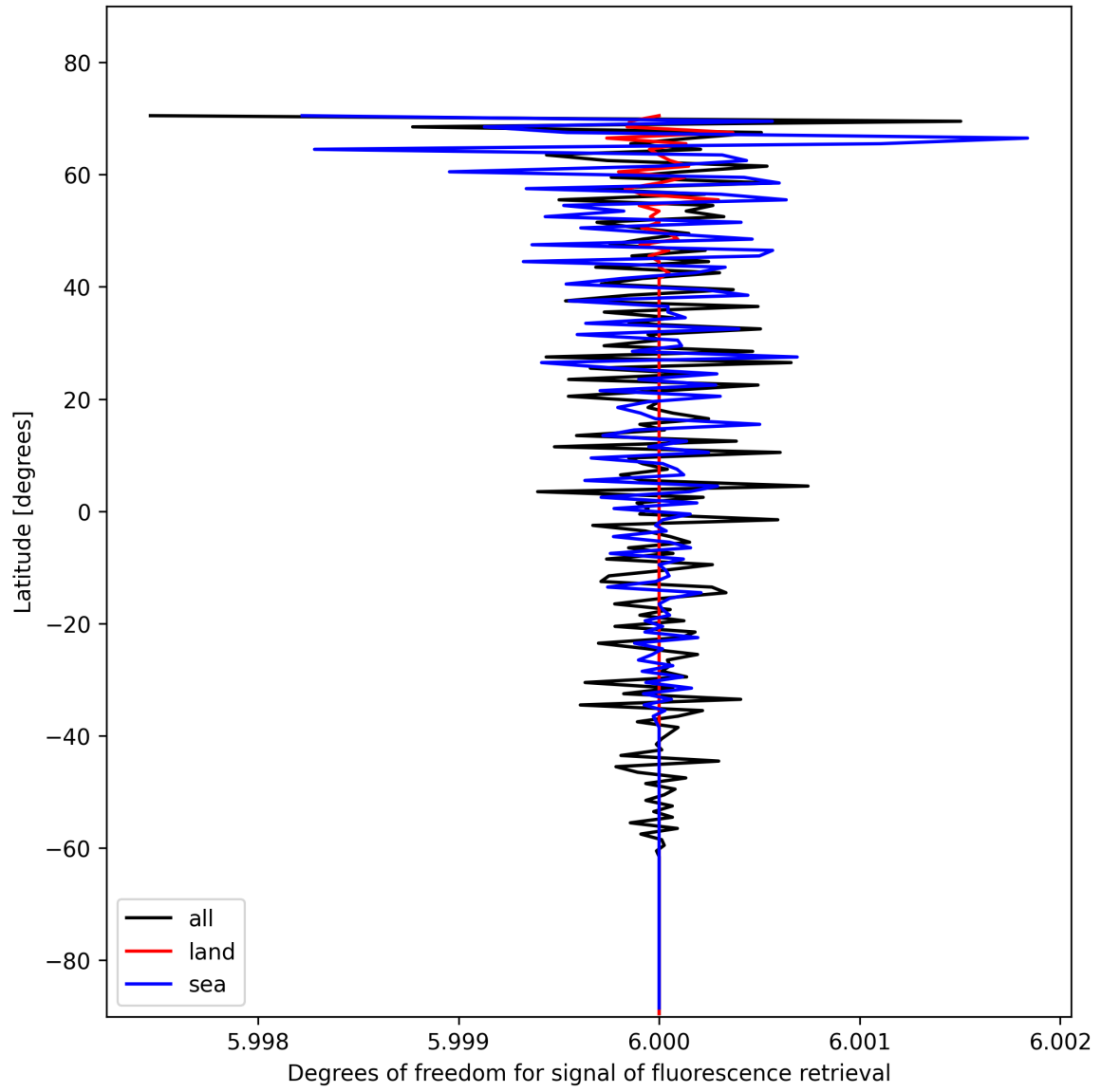
Figure 26: Zonal average of “Degrees of freedom for signal of fluorescence retrieval” for 2025-01-29 to 2025-01-31.
