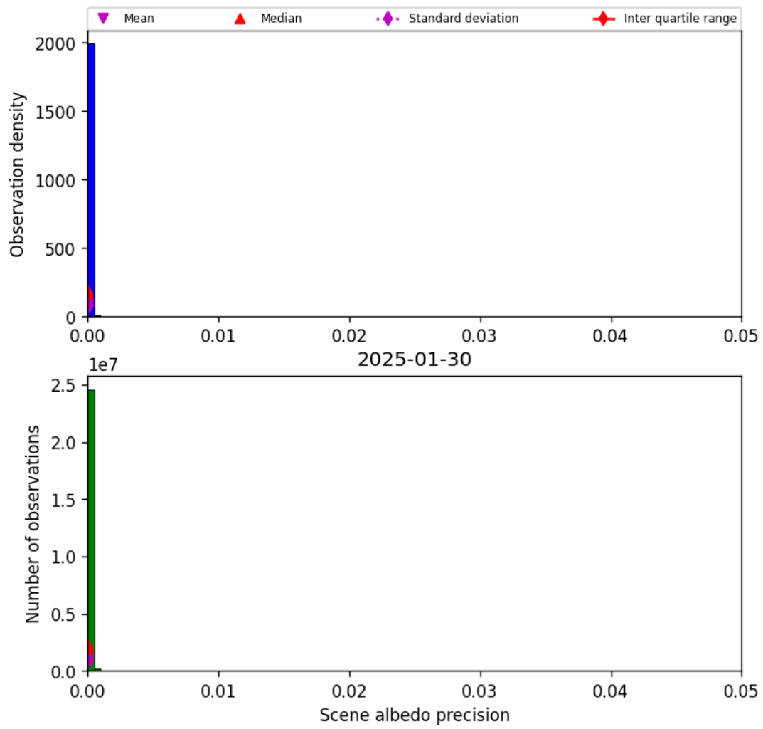
Figure 35: Histogram of “Scene albedo precision” for 2025-01-29 to 2025-01-31
