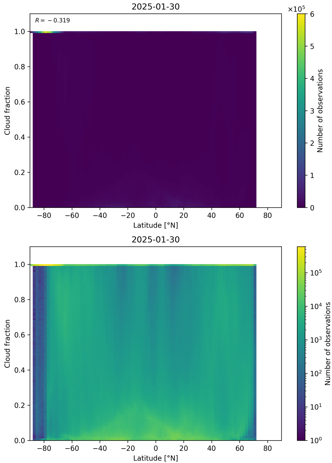
Figure 90: Scatter density plot of “Latitude” against “Cloud fraction” for 2025-01-29 to 2025-01-31.
