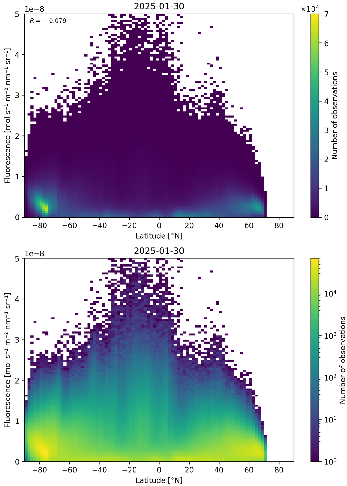
Figure 92: Scatter density plot of “Latitude” against “Fluorescence” for 2025-01-29 to 2025-01-31.
