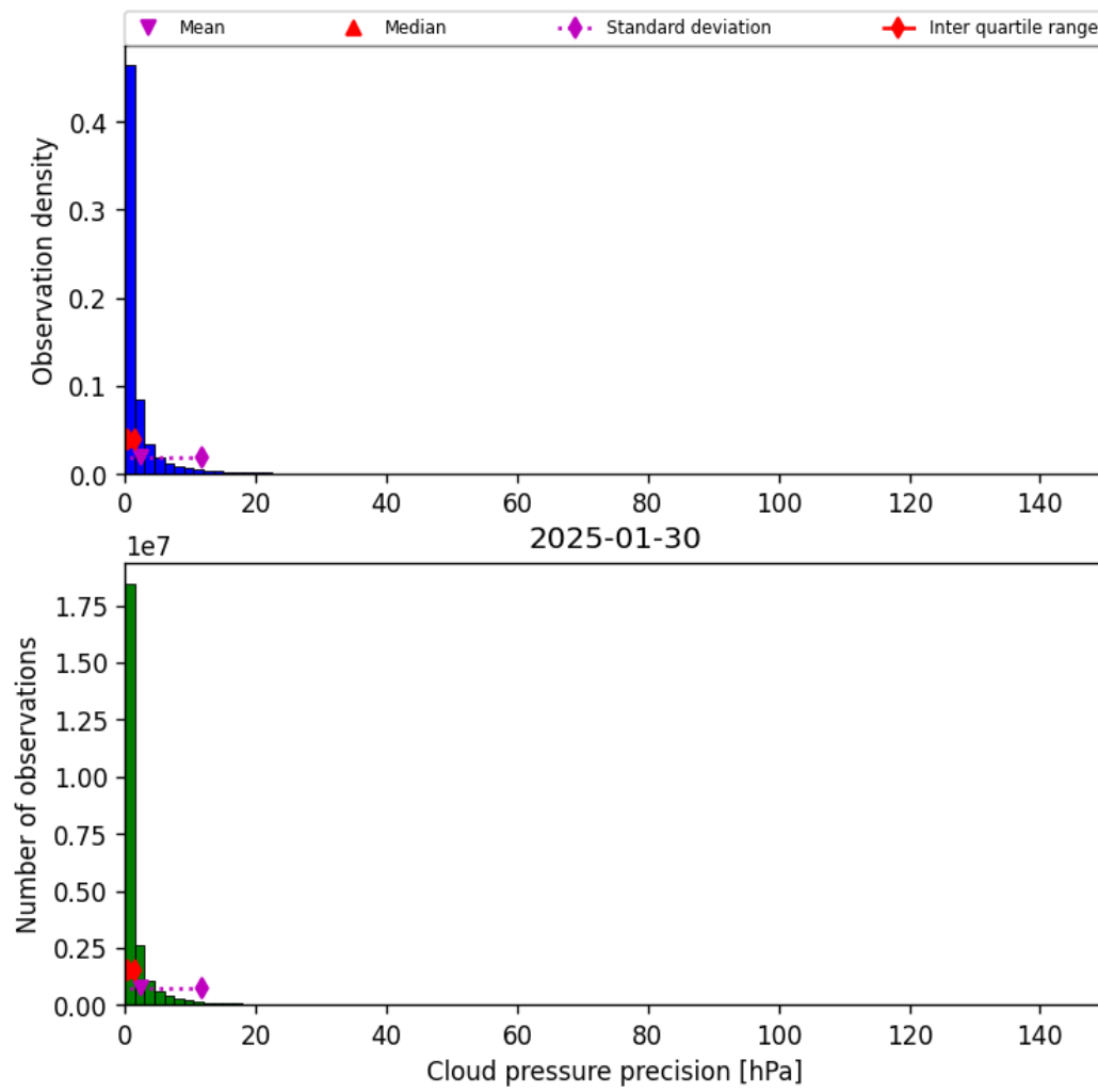
Figure 31: Histogram of “Cloud pressure precision” for 2025-01-29 to 2025-01-31
