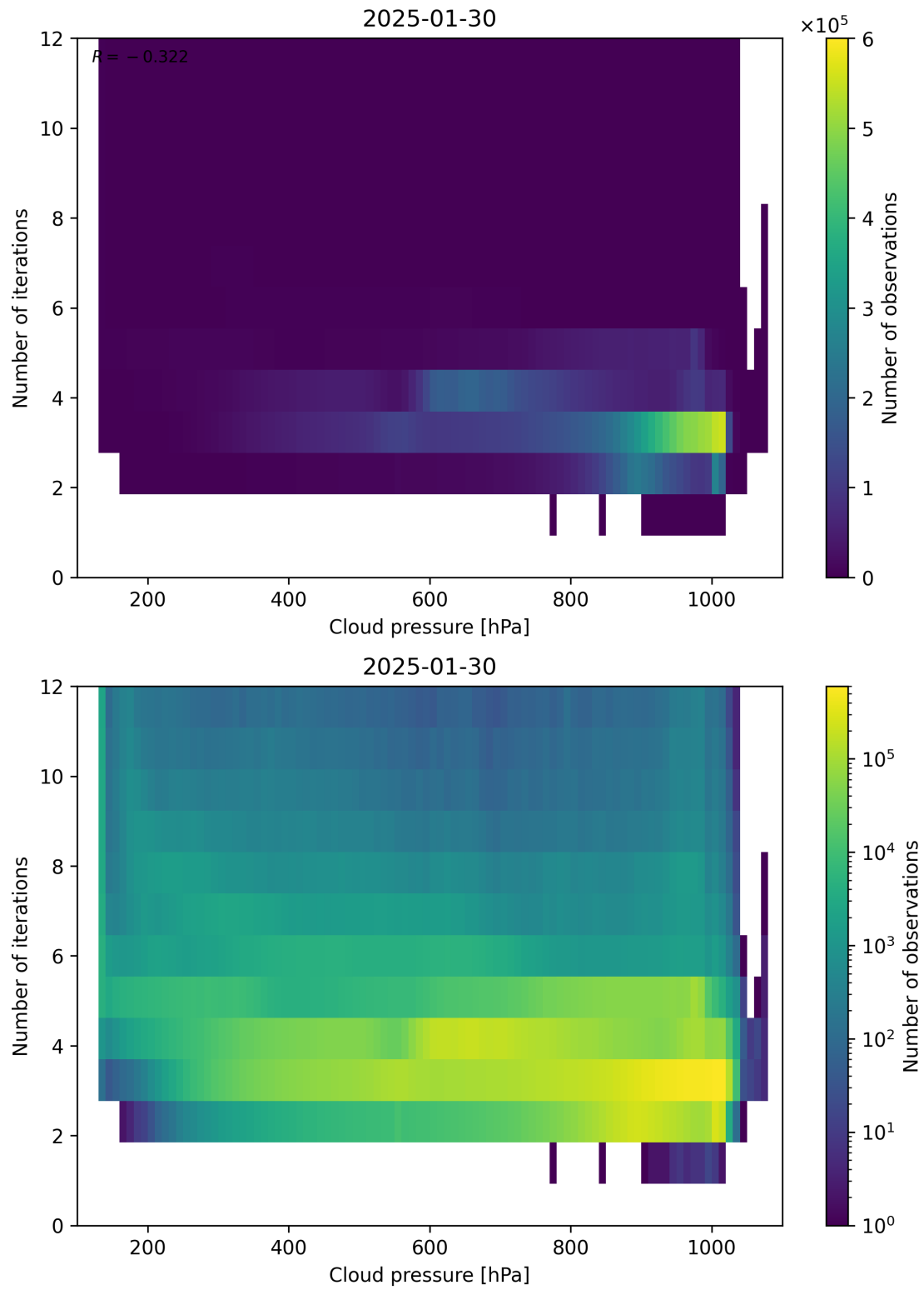
Figure 81: Scatter density plot of “Cloud pressure” against “Number of iterations” for 2025-01-29 to 2025-01-31.
