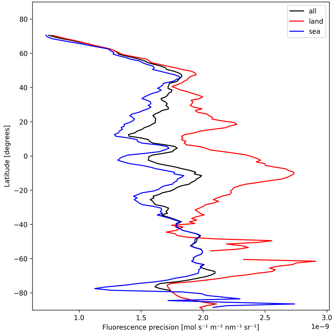
Figure 24: Zonal average of “Fluorescence precision” for 2025-01-29 to 2025-01-31.
