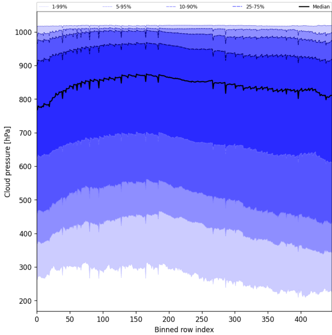
Figure 47: Along track statistics of “Cloud pressure” for 2025-01-29 to 2025-01-31
