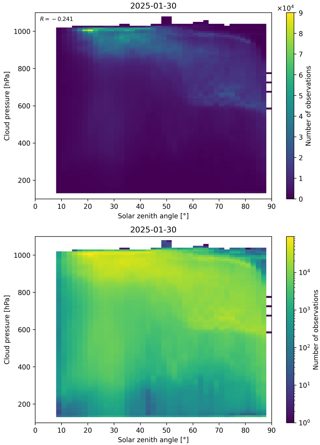
Figure 111: Scatter density plot of “Solar zenith angle” against “Cloud pressure” for 2025-01-29 to 2025-01-31.
