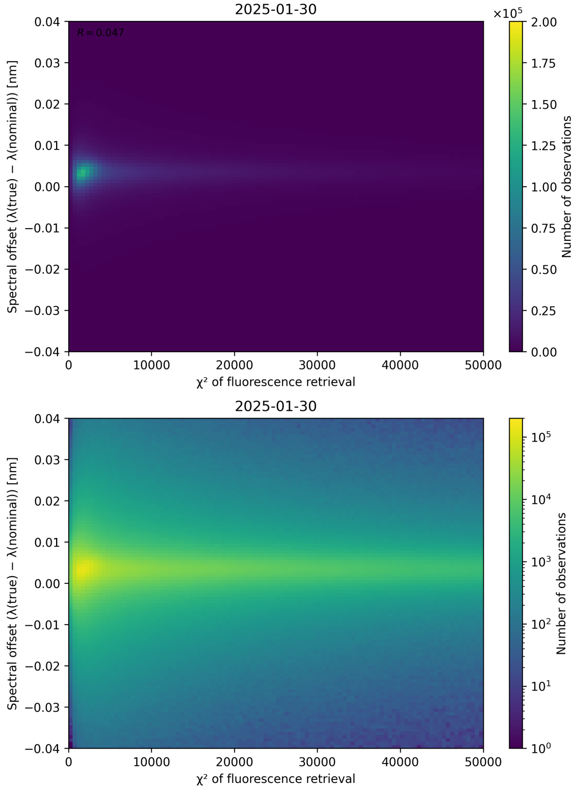
Figure 69: Scatter density plot of “ \chi^2 of fluorescence retrieval” against “Spectral offset ( \lambda_{\text{true}} - \lambda_{\text{nominal}} )” for 2025-01-29 to 2025-01-31.
