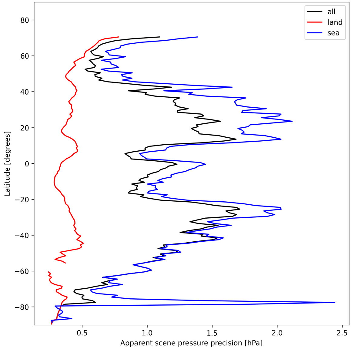
Figure 20: Zonal average of “Apparent scene pressure precision” for 2025-01-29 to 2025-01-31.
