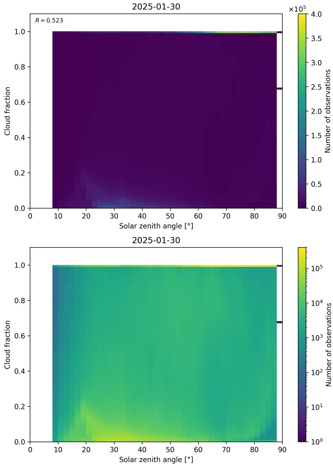
Figure 110: Scatter density plot of “Solar zenith angle” against “Cloud fraction” for 2025-01-29 to 2025-01-31.
