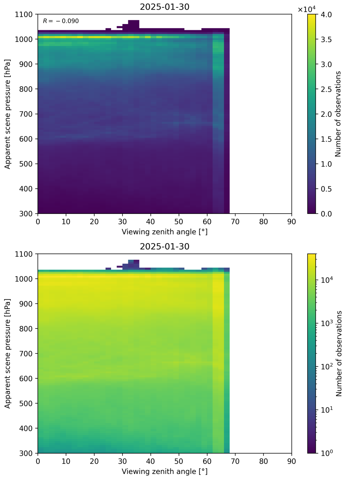
Figure 118: Scatter density plot of “Viewing zenith angle” against “Apparent scene pressure” for 2025-01-29 to 2025-01-31.
