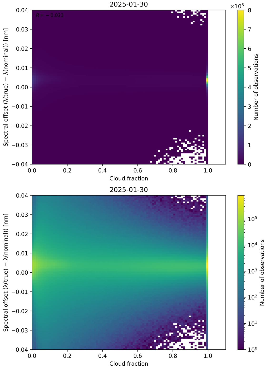
Figure 76: Scatter density plot of “Cloud fraction” against “Spectral offset ( \lambda_{\text{true}} - \lambda_{\text{nominal}} )” for 2025-01-29 to 2025-01-31.
