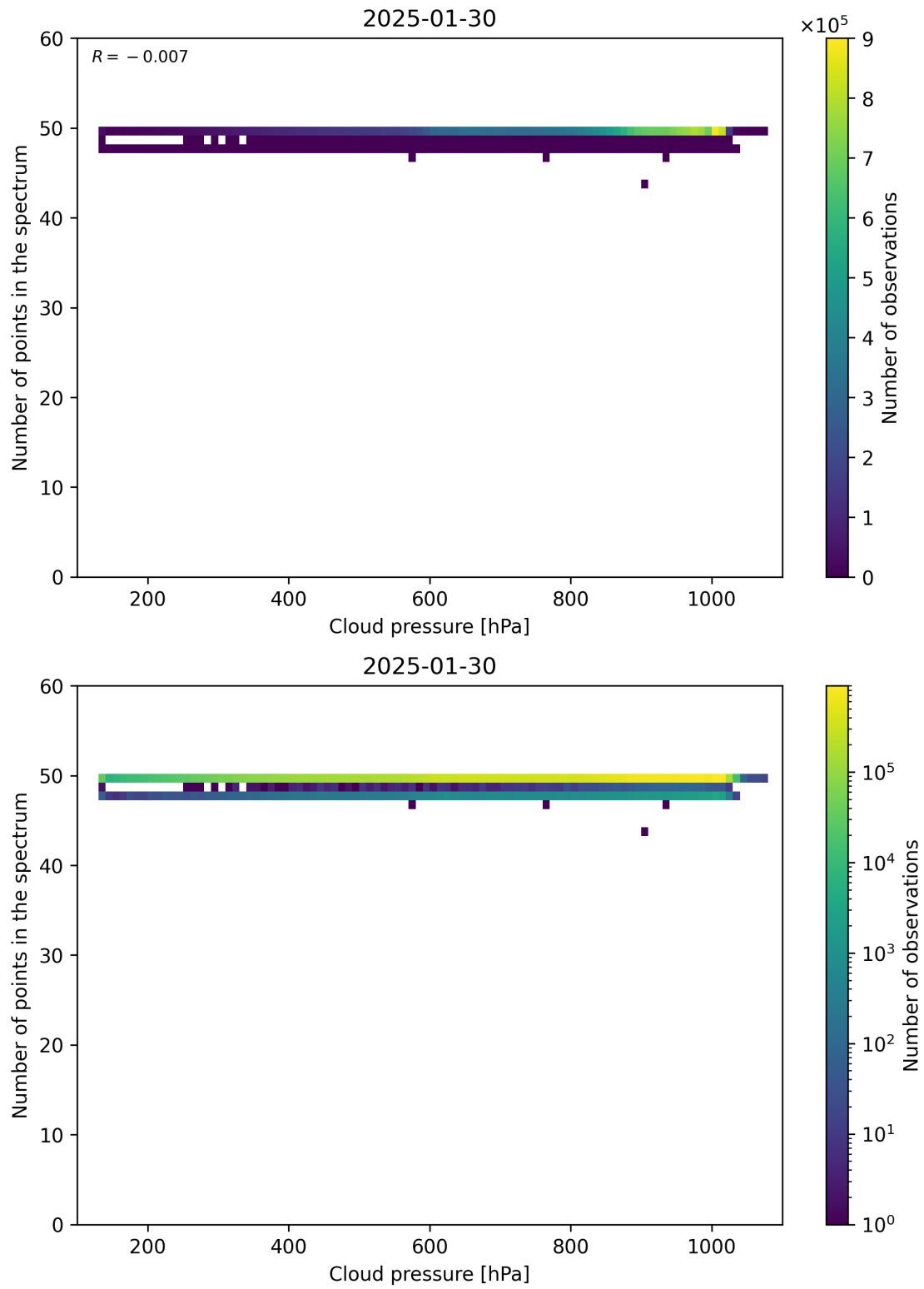
Figure 82: Scatter density plot of “Cloud pressure” against “Number of points in the spectrum” for 2025-01-29 to 2025-01-31.
