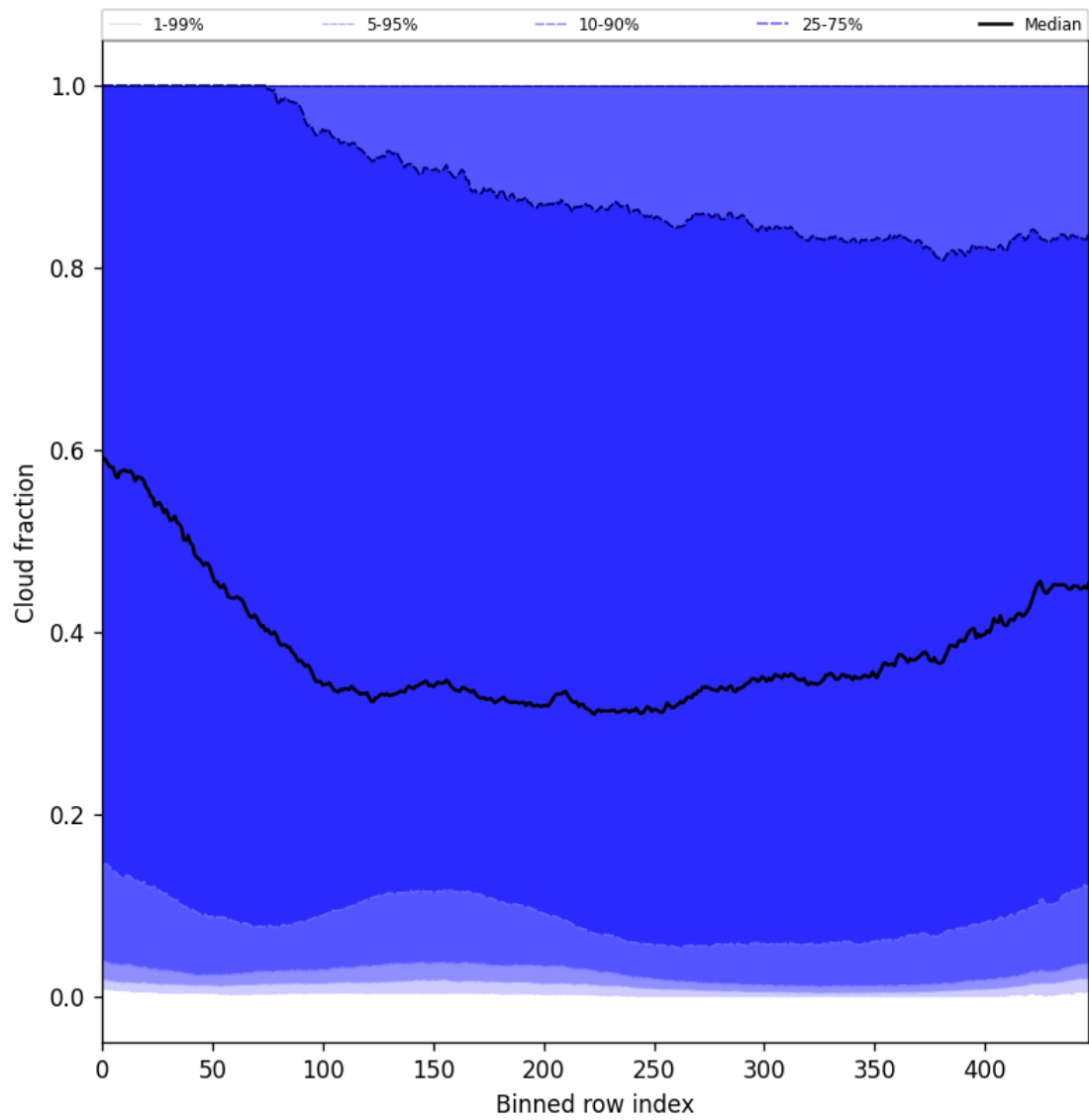
Figure 49: Along track statistics of “Cloud fraction” for 2025-01-29 to 2025-01-31
