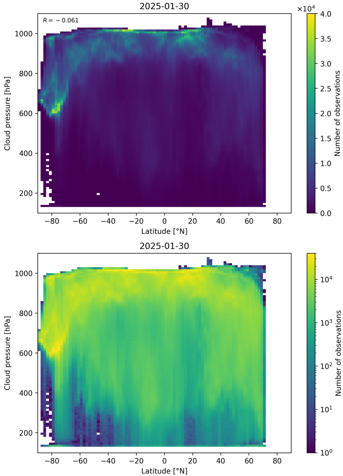
Figure 91: Scatter density plot of “Latitude” against “Cloud pressure” for 2025-01-29 to 2025-01-31.
