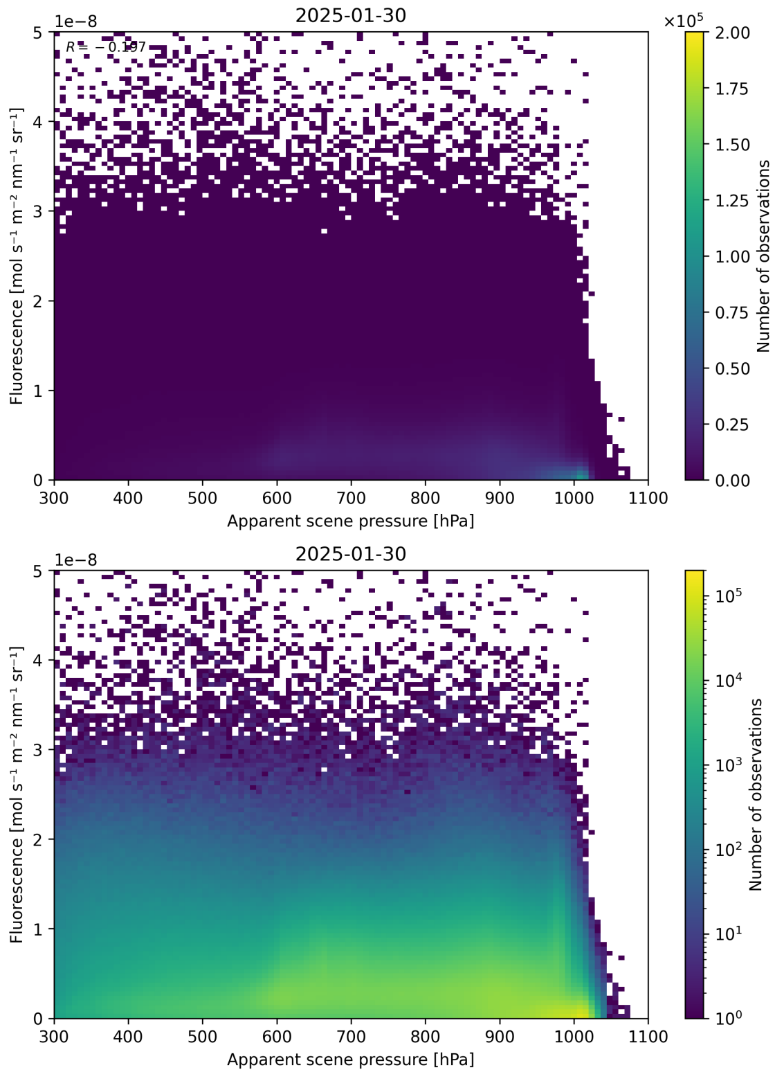
Figure 64: Scatter density plot of “Apparent scene pressure” against “Fluorescence” for 2025-01-29 to 2025-01-31.
