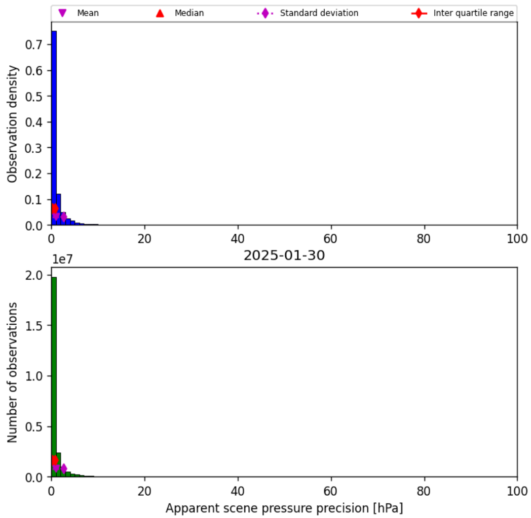
Figure 37: Histogram of “Apparent scene pressure precision” for 2025-01-29 to 2025-01-31
