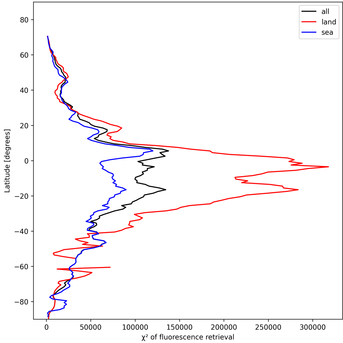
Figure 25: Zonal average of “ \chi^2 of fluorescence retrieval” for 2025-01-29 to 2025-01-31.
