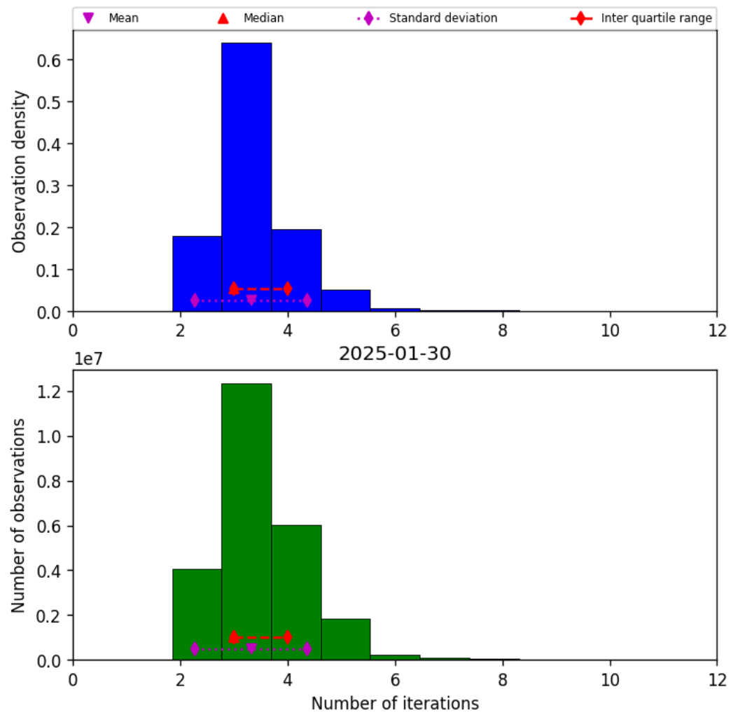
Figure 39: Histogram of “Number of iterations” for 2025-01-29 to 2025-01-31
