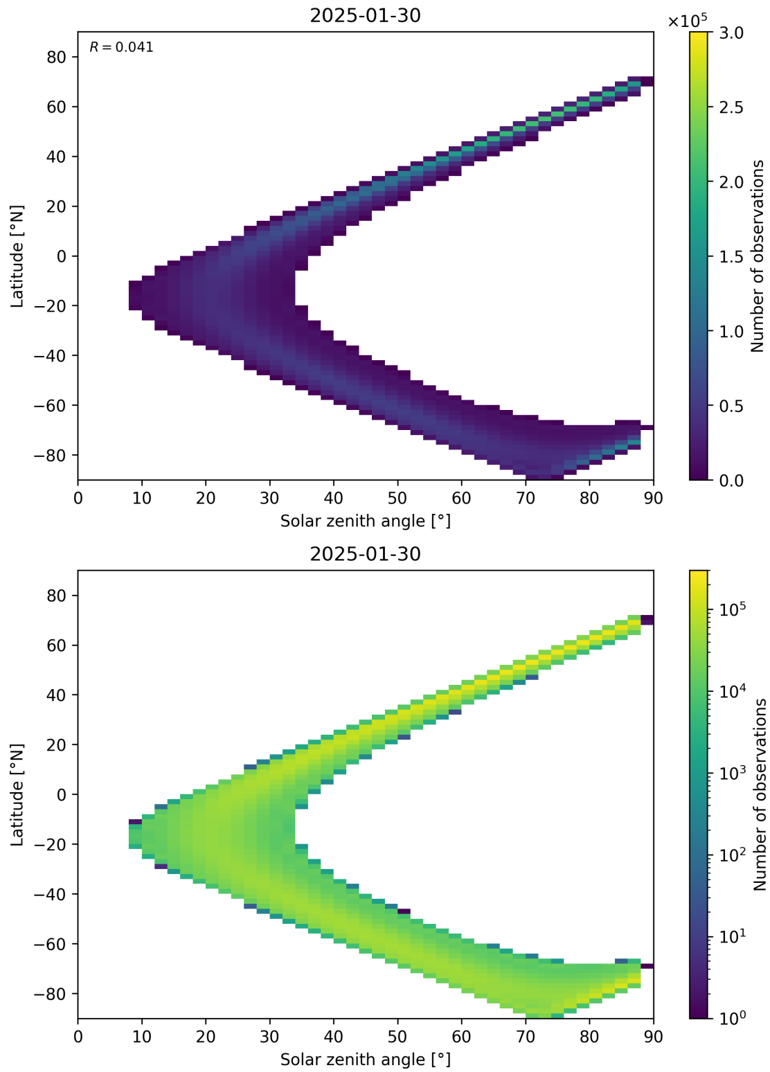
Figure 113: Scatter density plot of “Solar zenith angle” against “Latitude” for 2025-01-29 to 2025-01-31.
