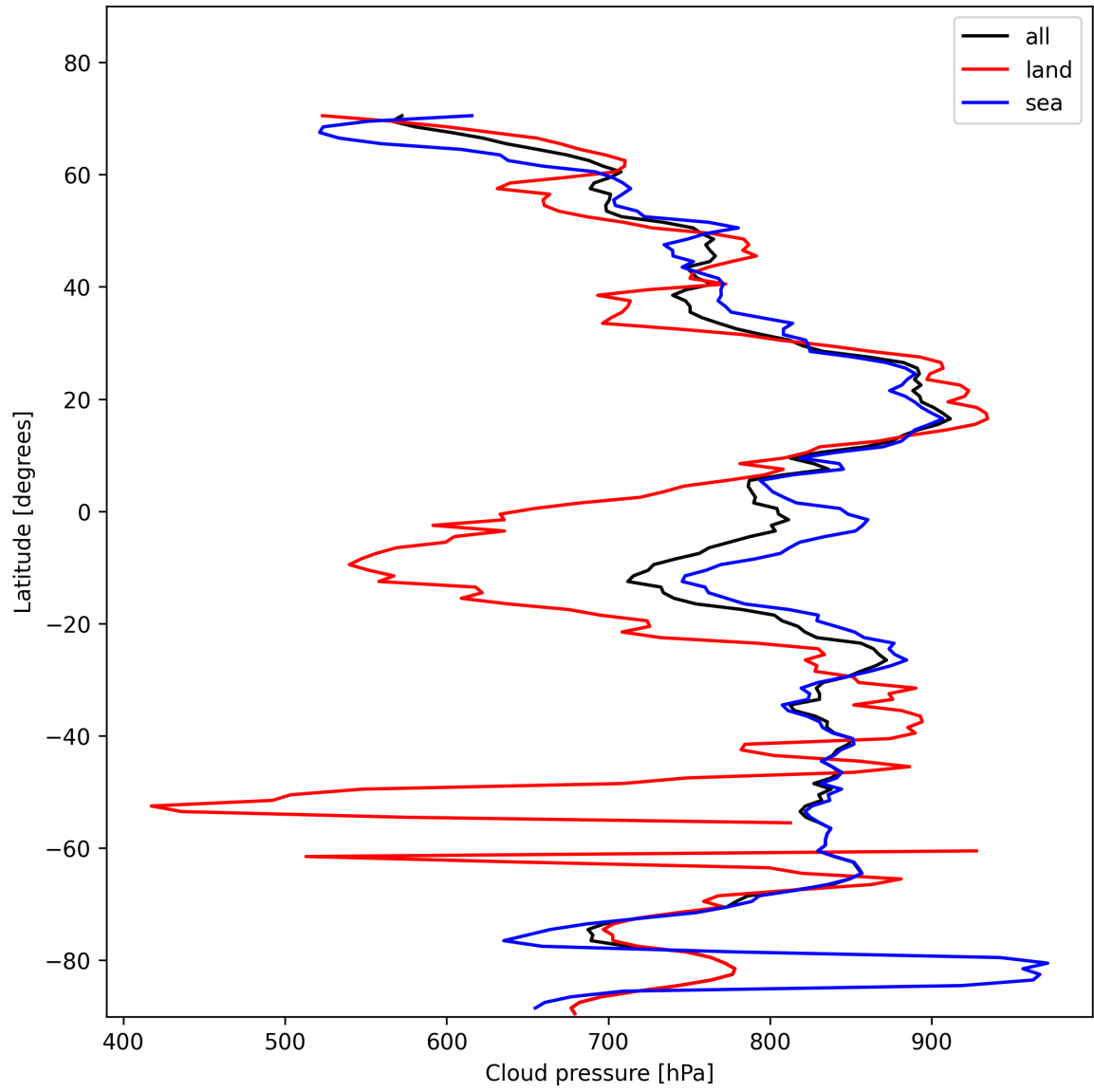
Figure 13: Zonal average of “Cloud pressure” for 2025-01-29 to 2025-01-31.
