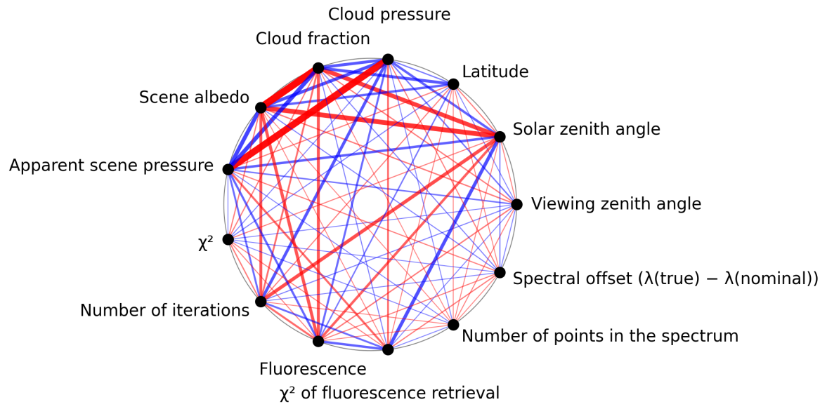
Figure 1: Map of correlation graph for 2025-01-29 to 2025-01-31.
