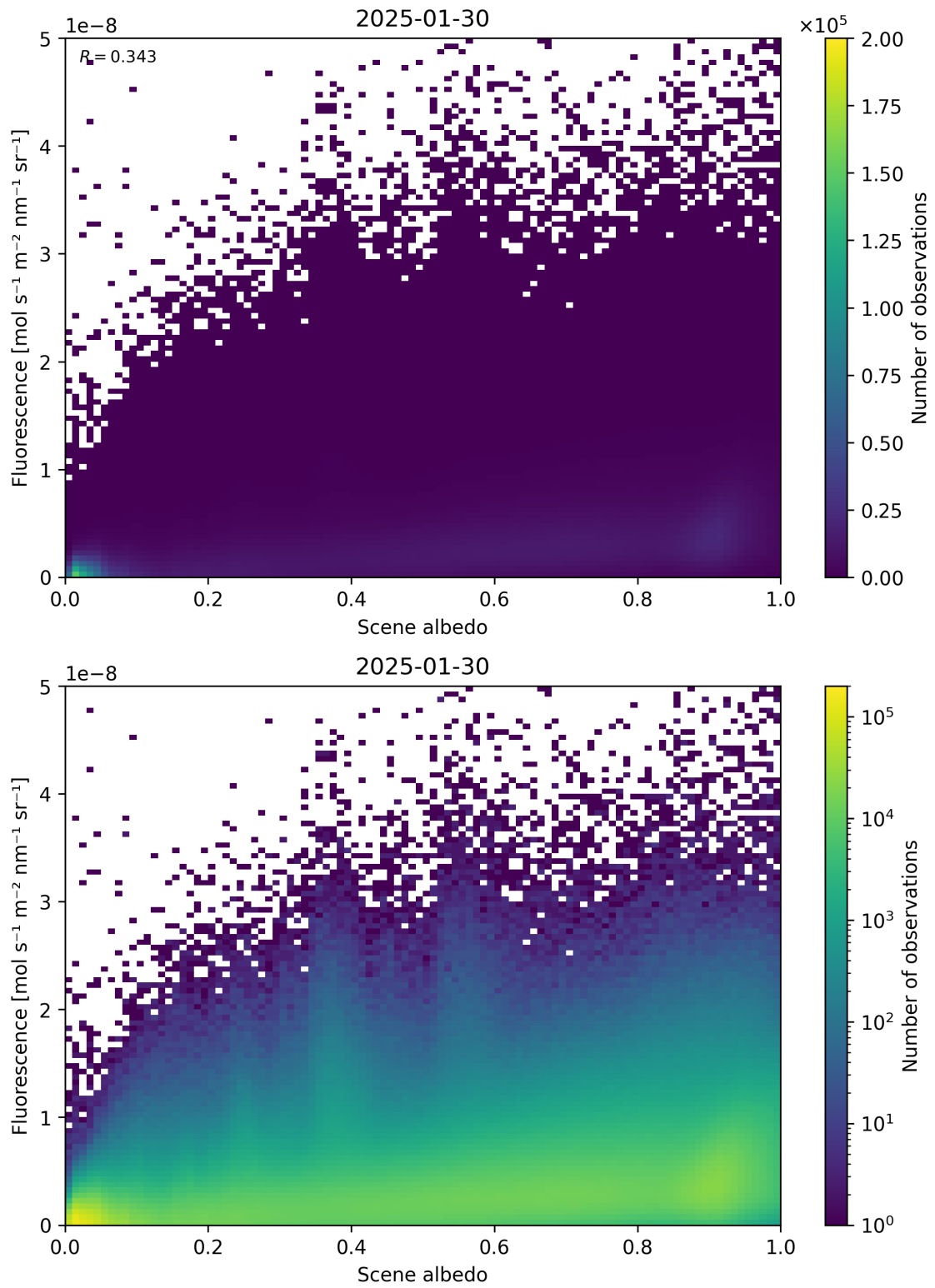
Figure 104: Scatter density plot of "Scene albedo" against "Fluorescence" for 2025-01-29 to 2025-01-31.
