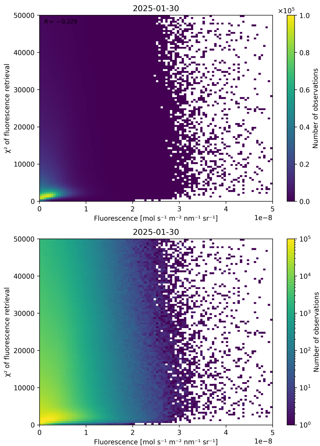
Figure 85: Scatter density plot of “Fluorescence” against “ \chi^2 of fluorescence retrieval” for 2025-01-29 to 2025-01-31.
