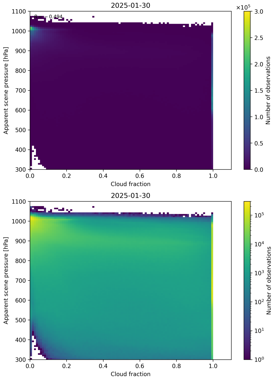
Figure 70: Scatter density plot of “Cloud fraction” against “Apparent scene pressure” for 2025-01-29 to 2025-01-31.
