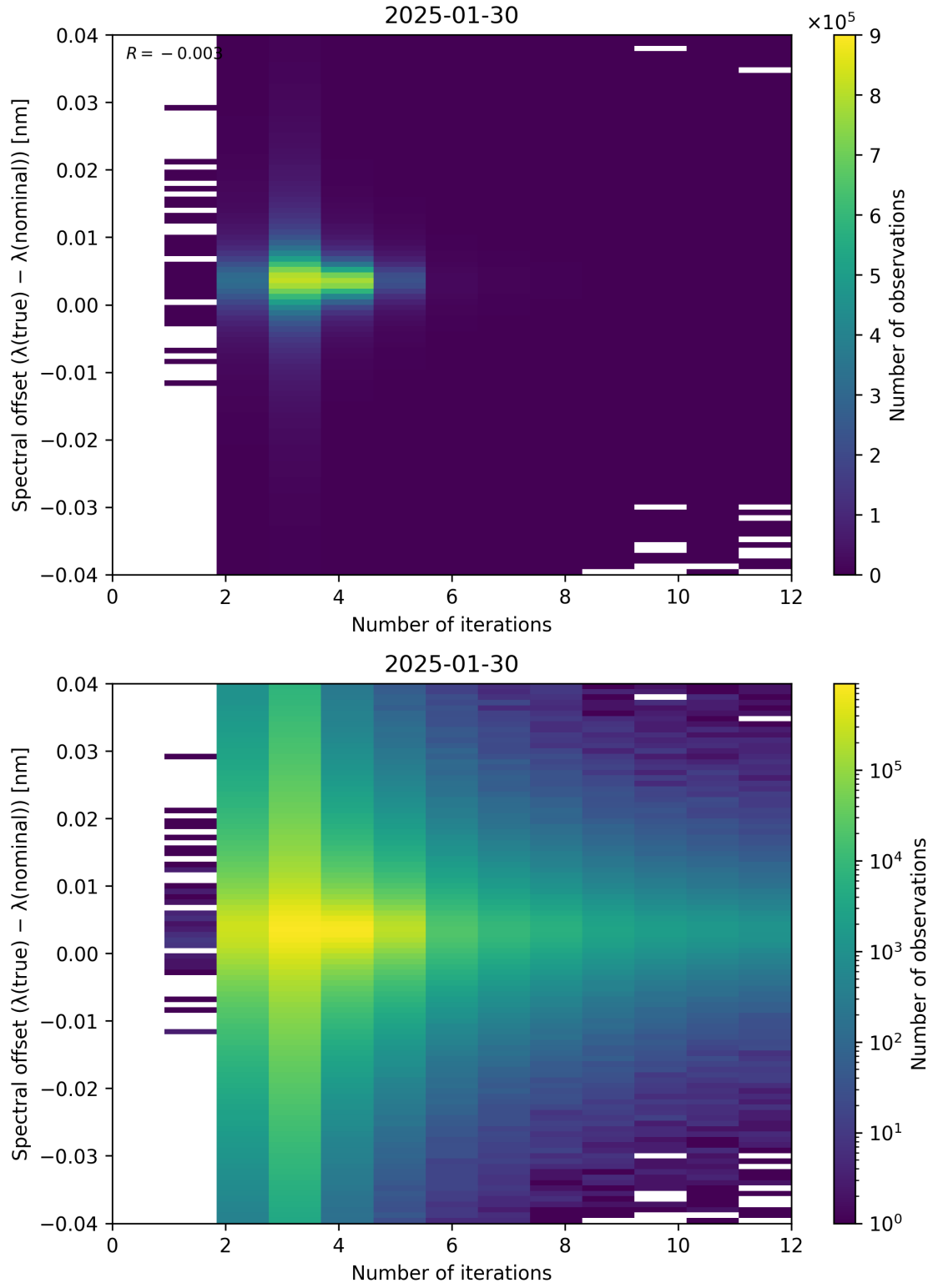
Figure 100: Scatter density plot of “Number of iterations” against “Spectral offset ( \lambda_{\text{true}} - \lambda_{\text{nominal}} )” for 2025-01-29 to 2025-01-31.
