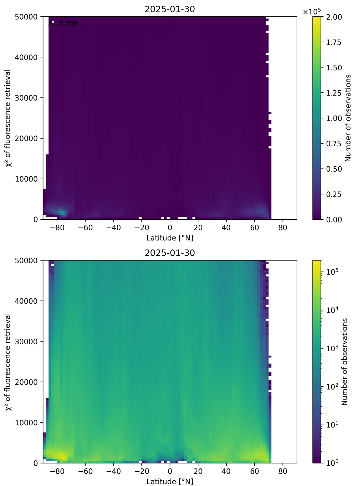
Figure 89: Scatter density plot of “Latitude” against “ \chi^2 of fluorescence retrieval” for 2025-01-29 to 2025-01-31.
