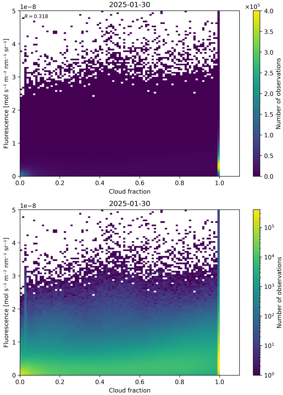
Figure 72: Scatter density plot of “Cloud fraction” against “Fluorescence” for 2025-01-29 to 2025-01-31.
