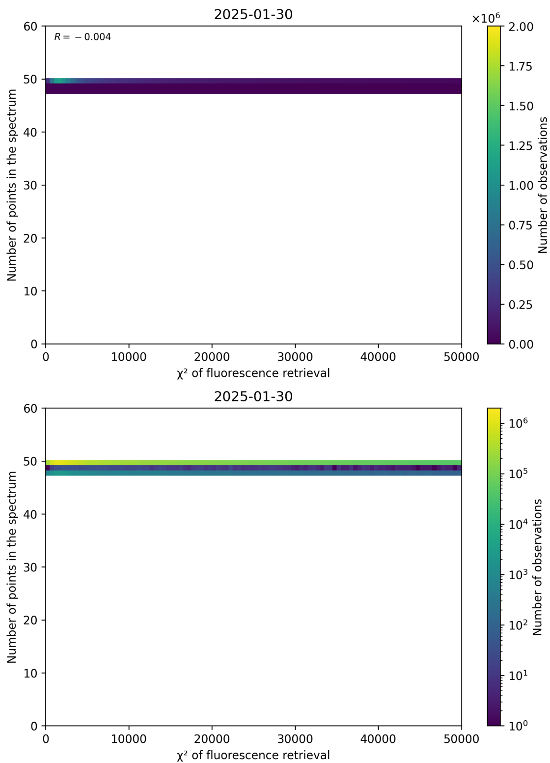
Figure 68: Scatter density plot of “ \chi^2 of fluorescence retrieval” against “Number of points in the spectrum” for 2025-01-29 to 2025-01-31.
