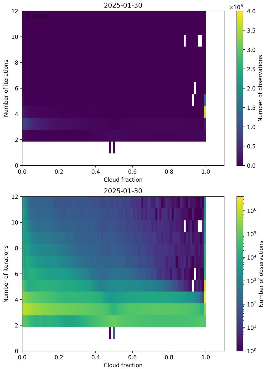
Figure 73: Scatter density plot of “Cloud fraction” against “Number of iterations” for 2025-01-29 to 2025-01-31.
