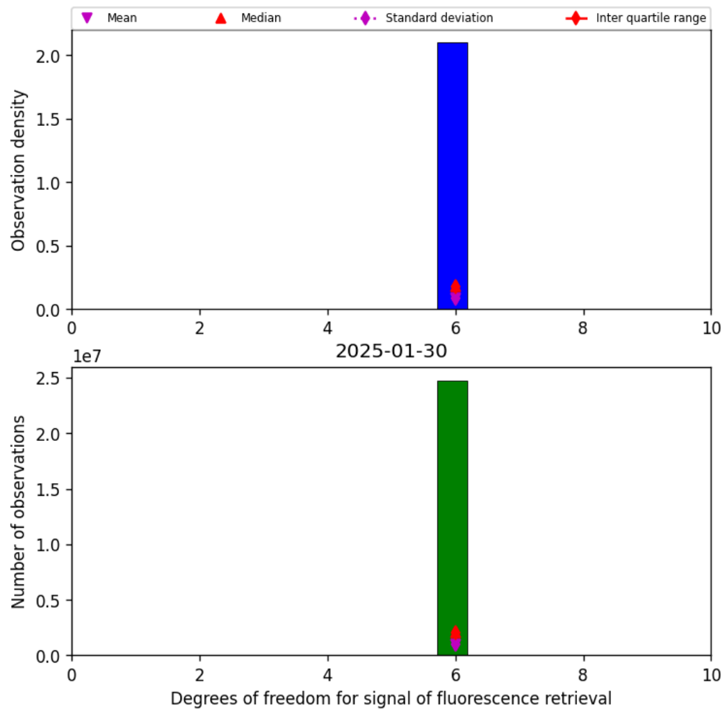
Figure 43: Histogram of "Degrees of freedom for signal of fluorescence retrieval" for 2025-01-29 to 2025-01-31
