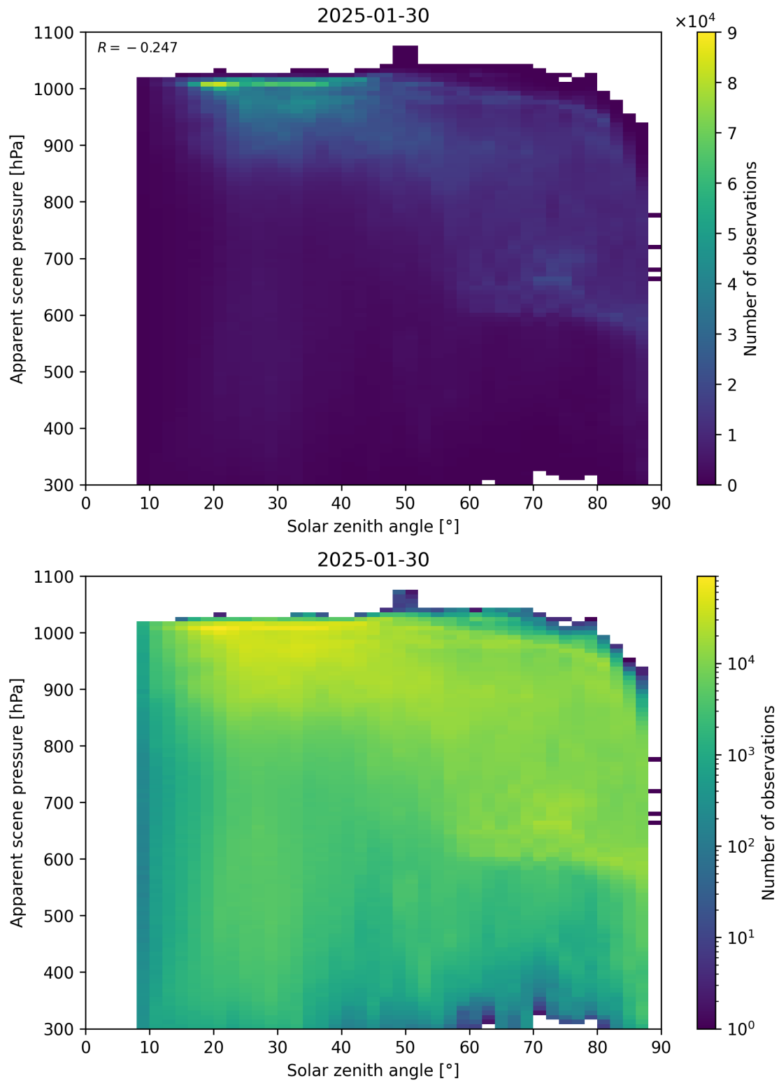
Figure 108: Scatter density plot of “Solar zenith angle” against “Apparent scene pressure” for 2025-01-29 to 2025-01-31.
