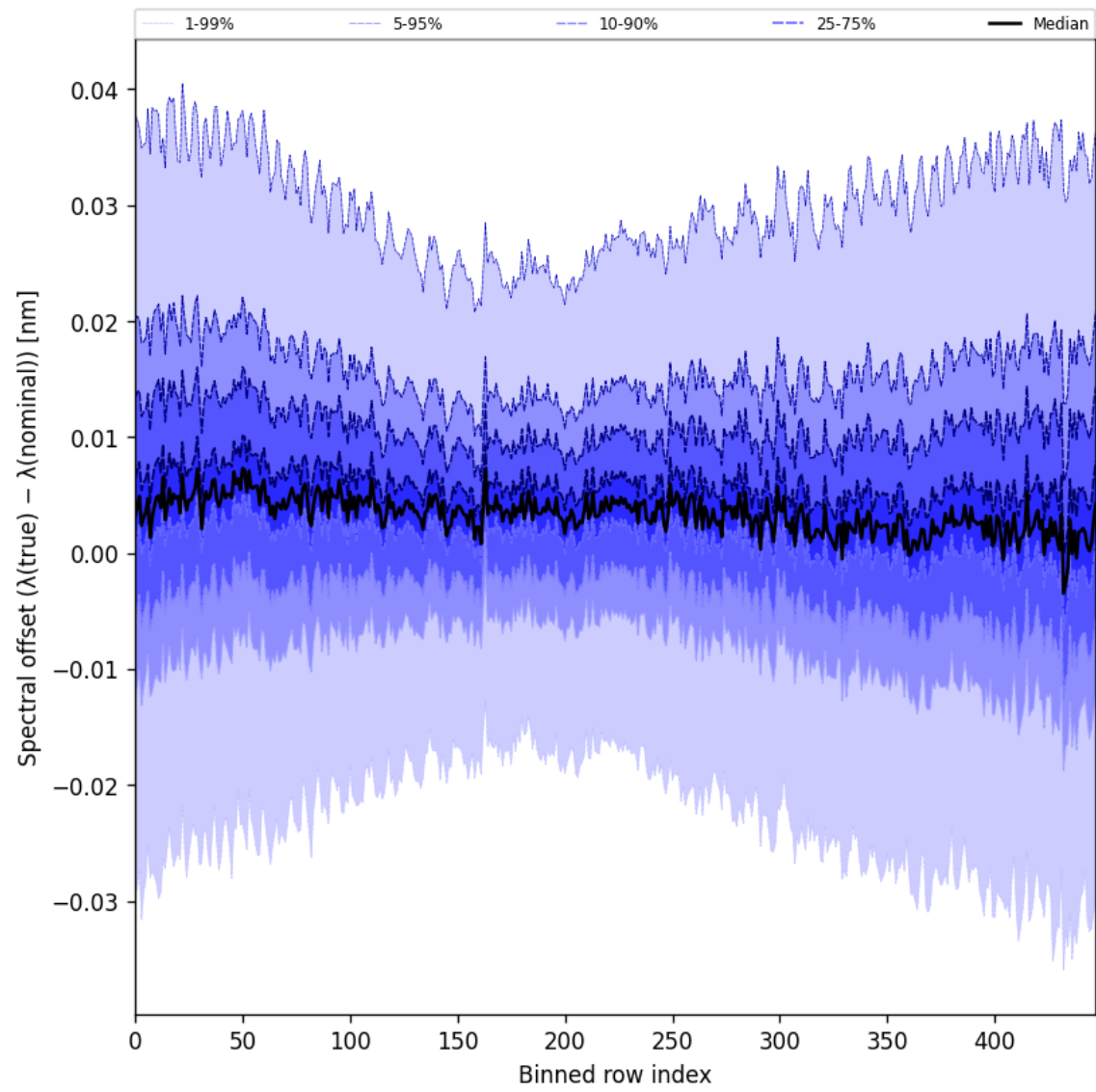
Figure 62: Along track statistics of “Spectral offset ( \lambda_{\text{true}} - \lambda_{\text{nominal}} )” for 2025-01-29 to 2025-01-31
