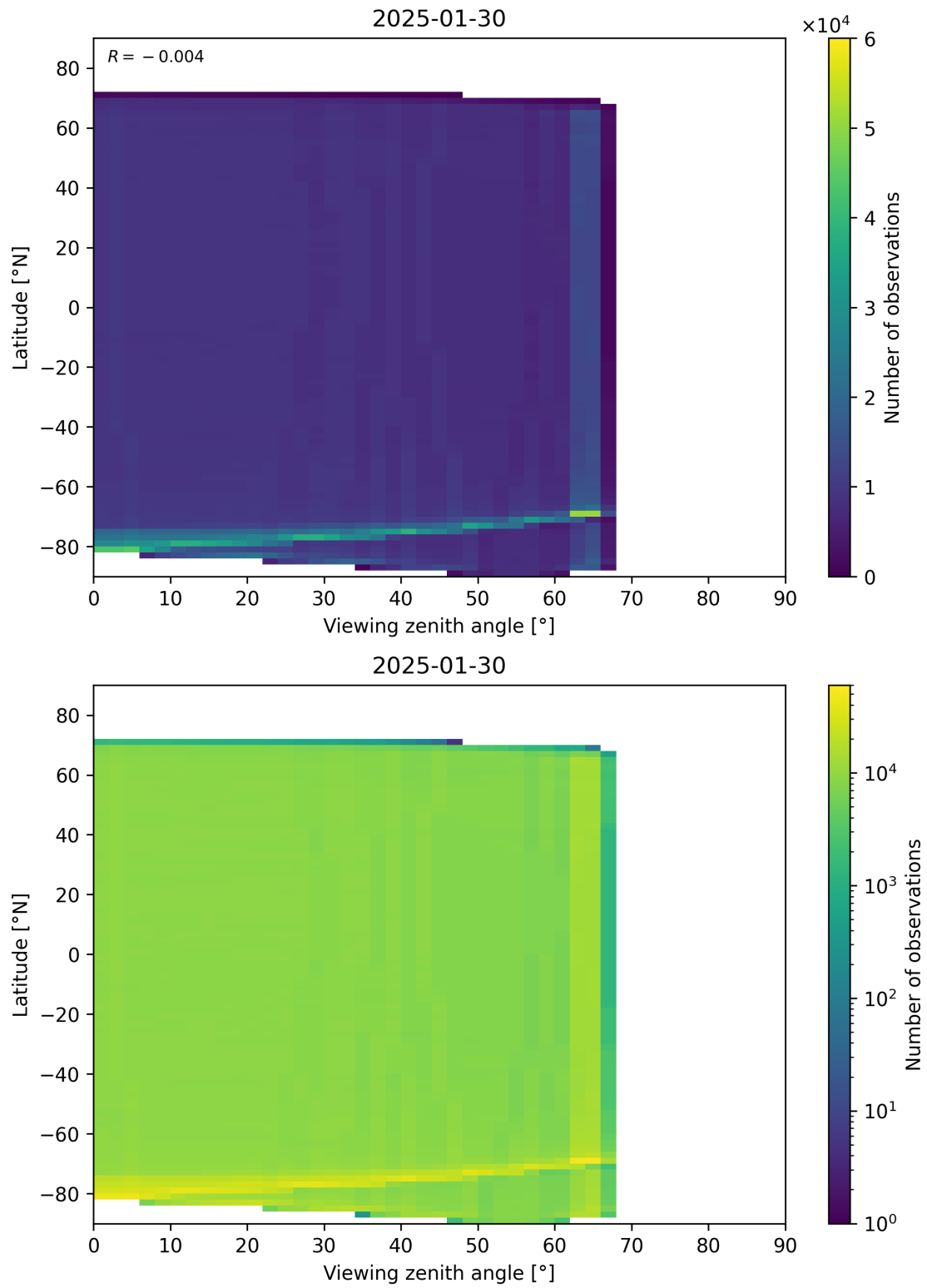
Figure 123: Scatter density plot of “Viewing zenith angle” against “Latitude” for 2025-01-29 to 2025-01-31.
