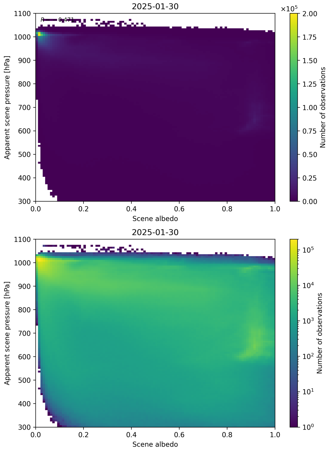
Figure 102: Scatter density plot of “Scene albedo” against “Apparent scene pressure” for 2025-01-29 to 2025-01-31.
