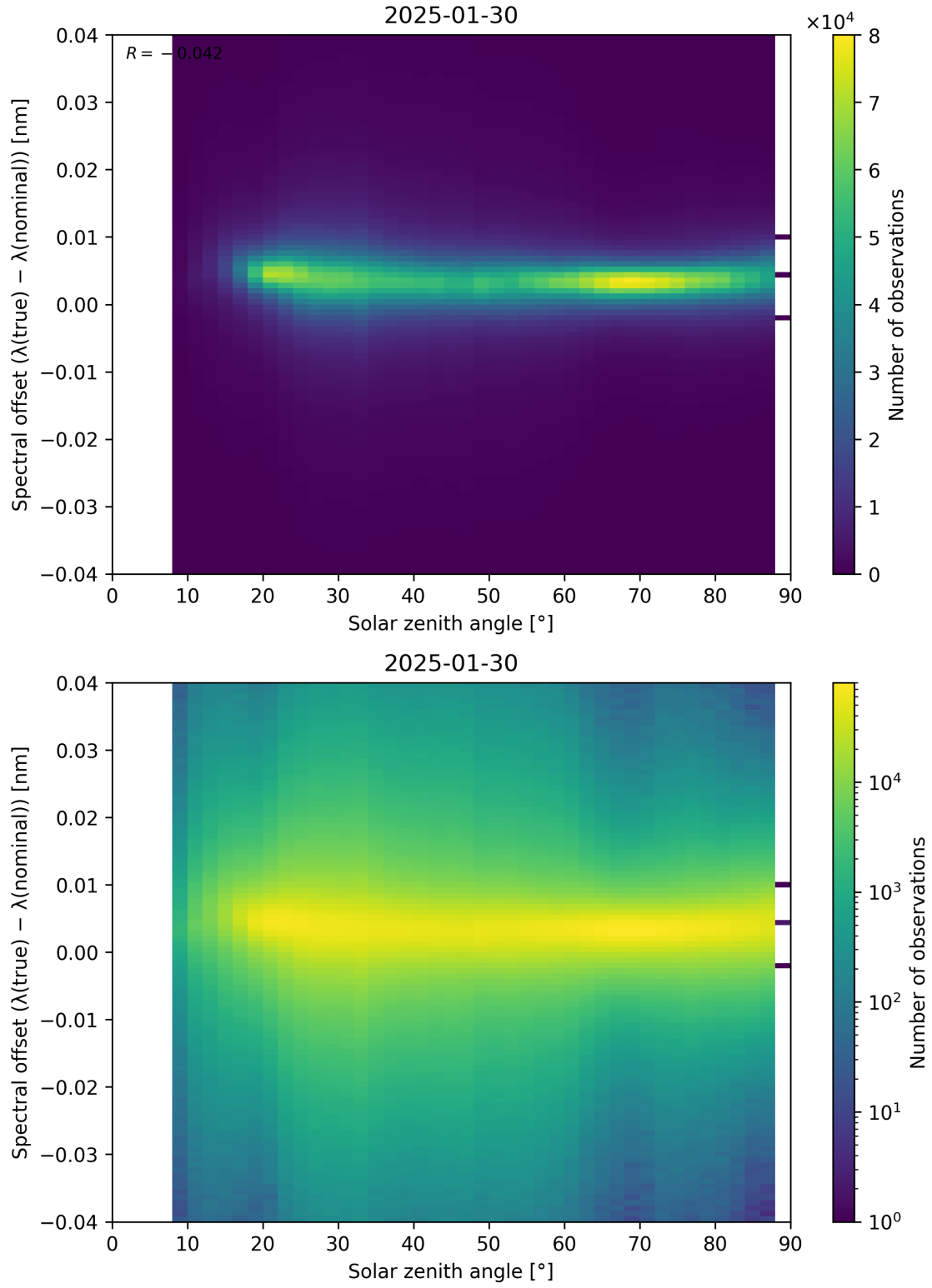
Figure 117: Scatter density plot of “Solar zenith angle” against “Spectral offset ( \lambda_{\text{true}} - \lambda_{\text{nominal}} )” for 2025-01-29 to 2025-01-31.
