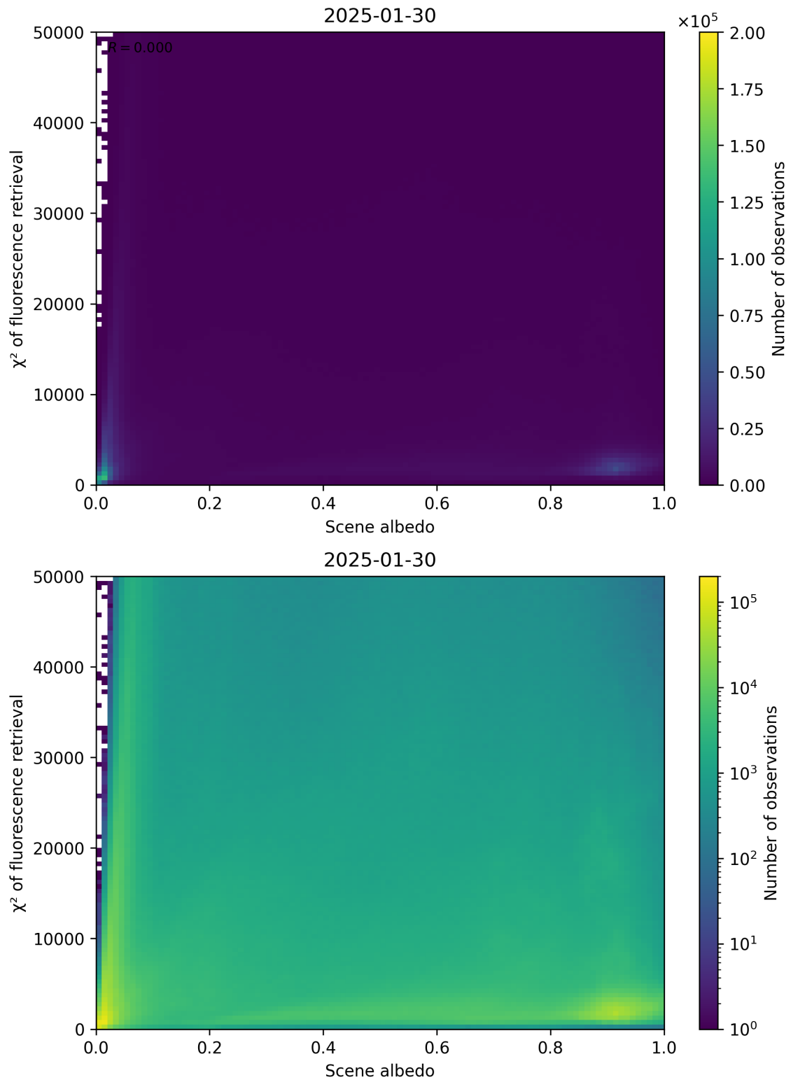
Figure 103: Scatter density plot of “Scene albedo” against “ \chi^2 of fluorescence retrieval” for 2025-01-29 to 2025-01-31.
