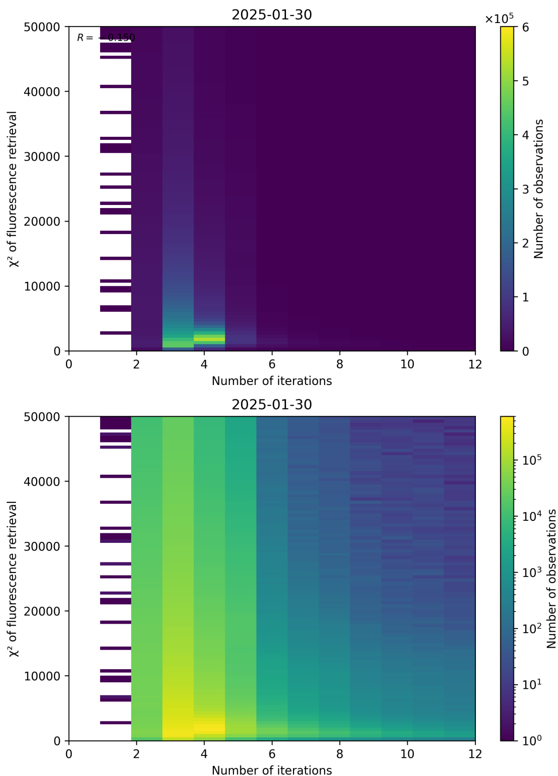
Figure 97: Scatter density plot of “Number of iterations” against “ \chi^2 of fluorescence retrieval” for 2025-01-29 to 2025-01-31.
