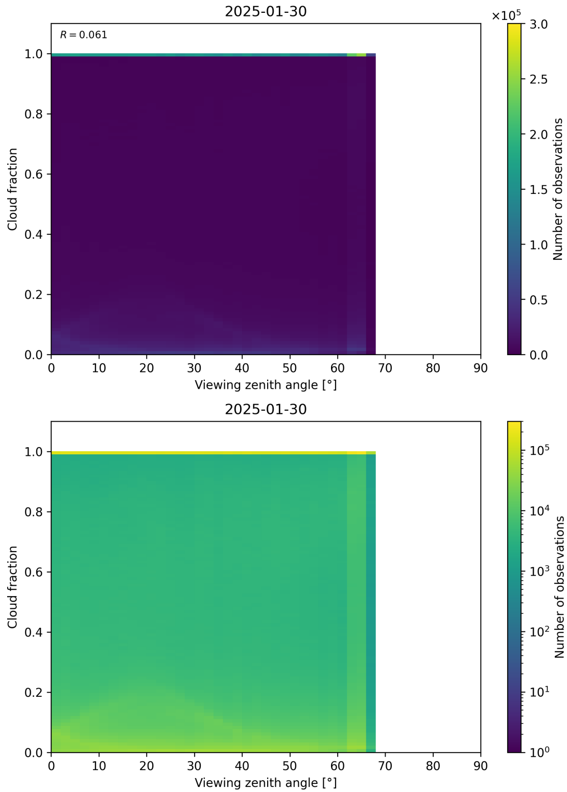
Figure 120: Scatter density plot of “Viewing zenith angle” against “Cloud fraction” for 2025-01-29 to 2025-01-31.
