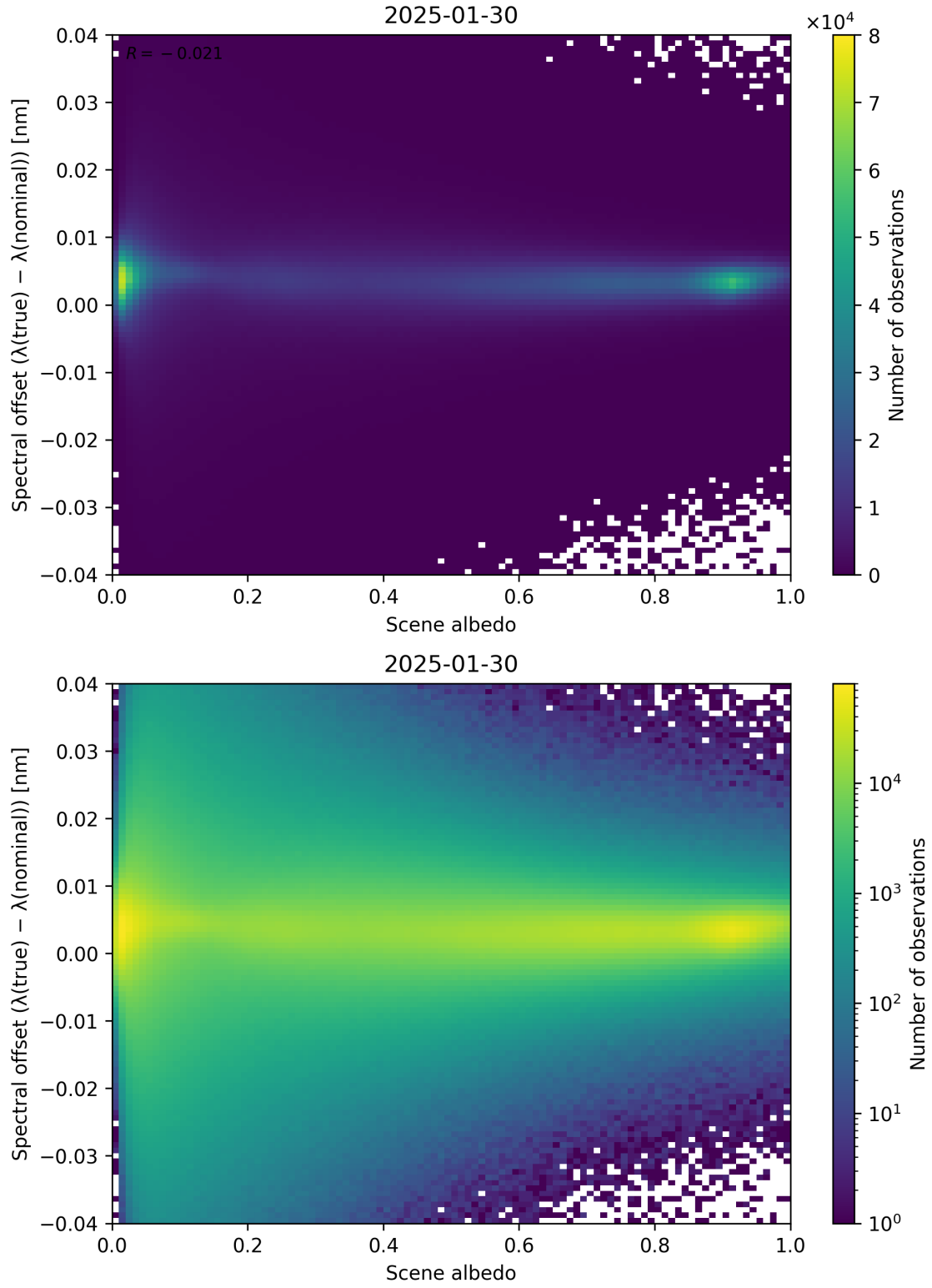
Figure 107: Scatter density plot of “Scene albedo” against “Spectral offset ( \lambda_{\text{true}} - \lambda_{\text{nominal}} )” for 2025-01-29 to 2025-01-31.
