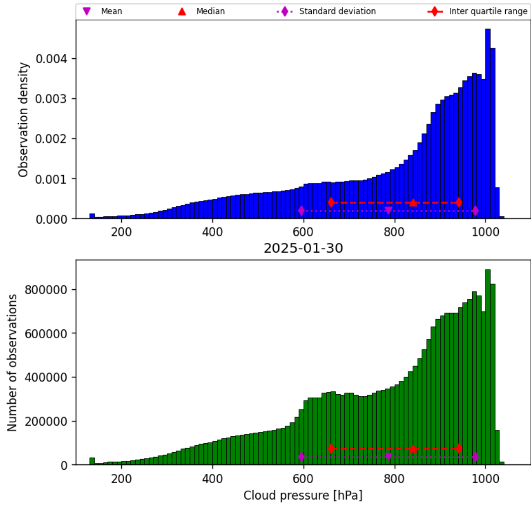
Figure 30: Histogram of “Cloud pressure” for 2025-01-29 to 2025-01-31
