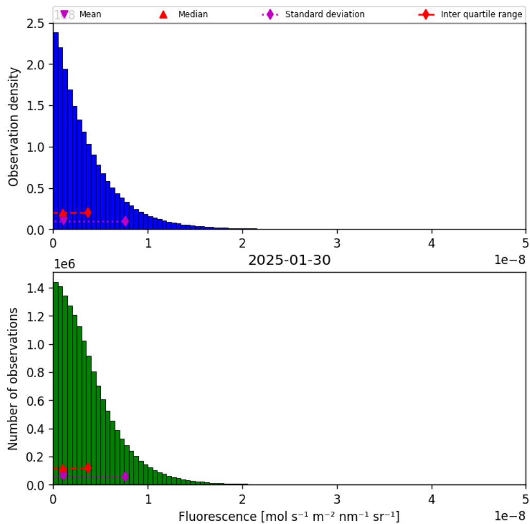
Figure 40: Histogram of “Fluorescence” for 2025-01-29 to 2025-01-31
