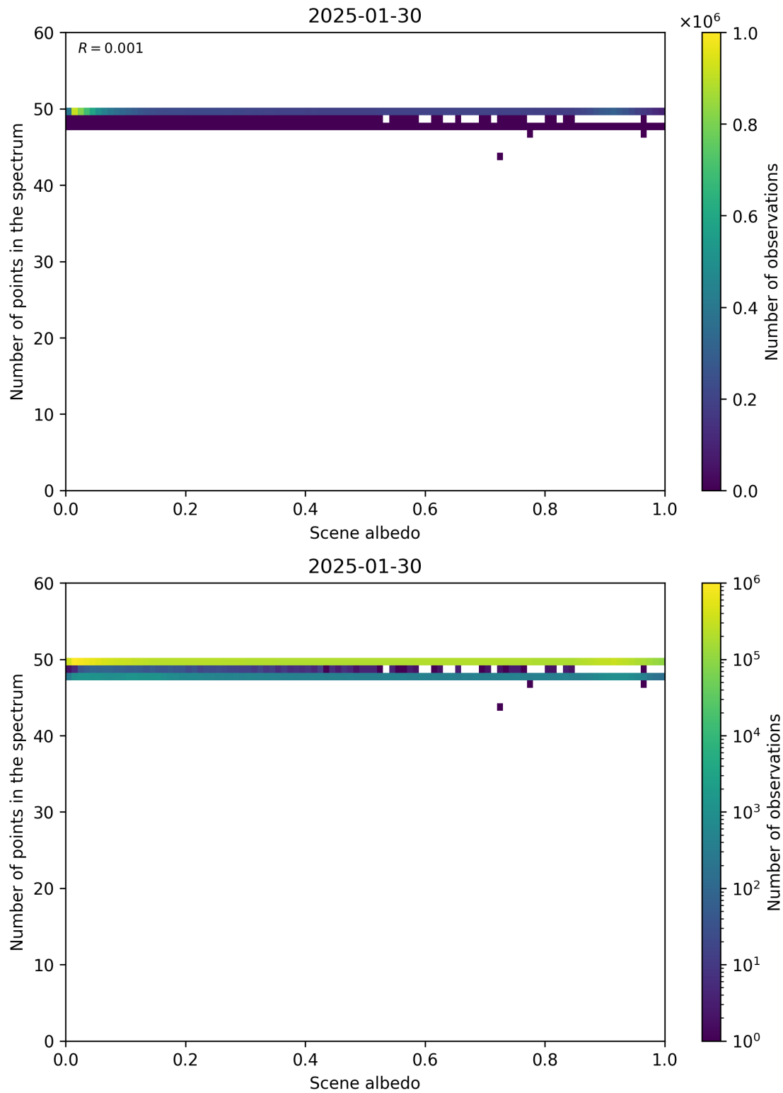
Figure 106: Scatter density plot of “Scene albedo” against “Number of points in the spectrum” for 2025-01-29 to 2025-01-31.
