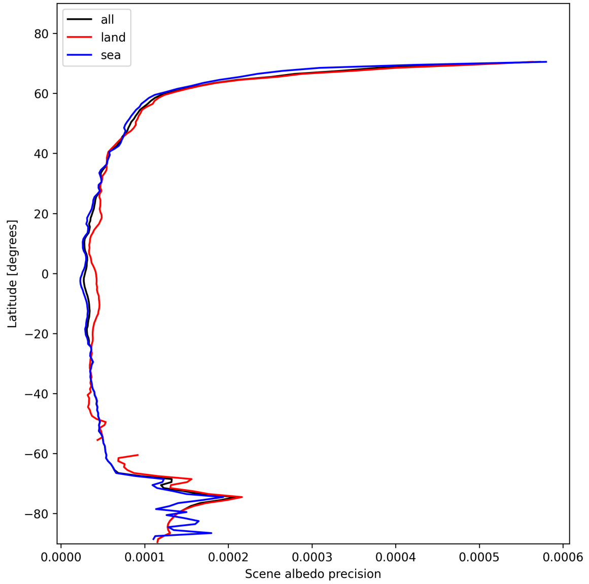
Figure 18: Zonal average of “Scene albedo precision” for 2025-01-29 to 2025-01-31.
