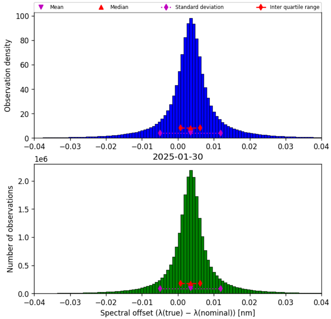
Figure 45: Histogram of “Spectral offset ( \lambda_{\text{true}} - \lambda_{\text{nominal}} )” for 2025-01-29 to 2025-01-31
