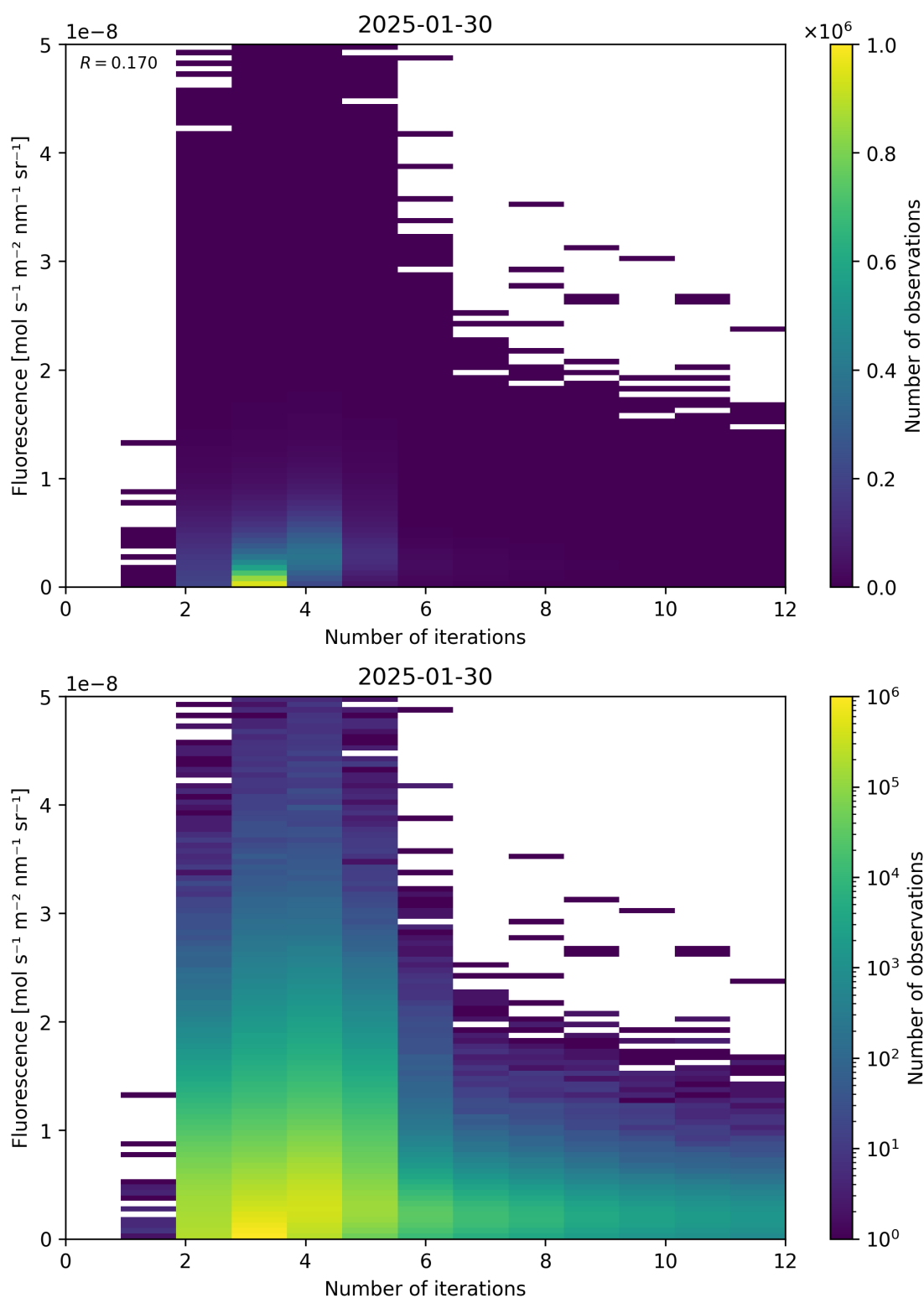
Figure 98: Scatter density plot of "Number of iterations" against "Fluorescence" for 2025-01-29 to 2025-01-31.
