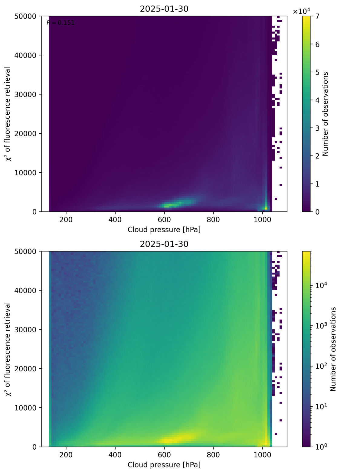
Figure 78: Scatter density plot of “Cloud pressure” against “ \chi^2 of fluorescence retrieval” for 2025-01-29 to 2025-01-31.
