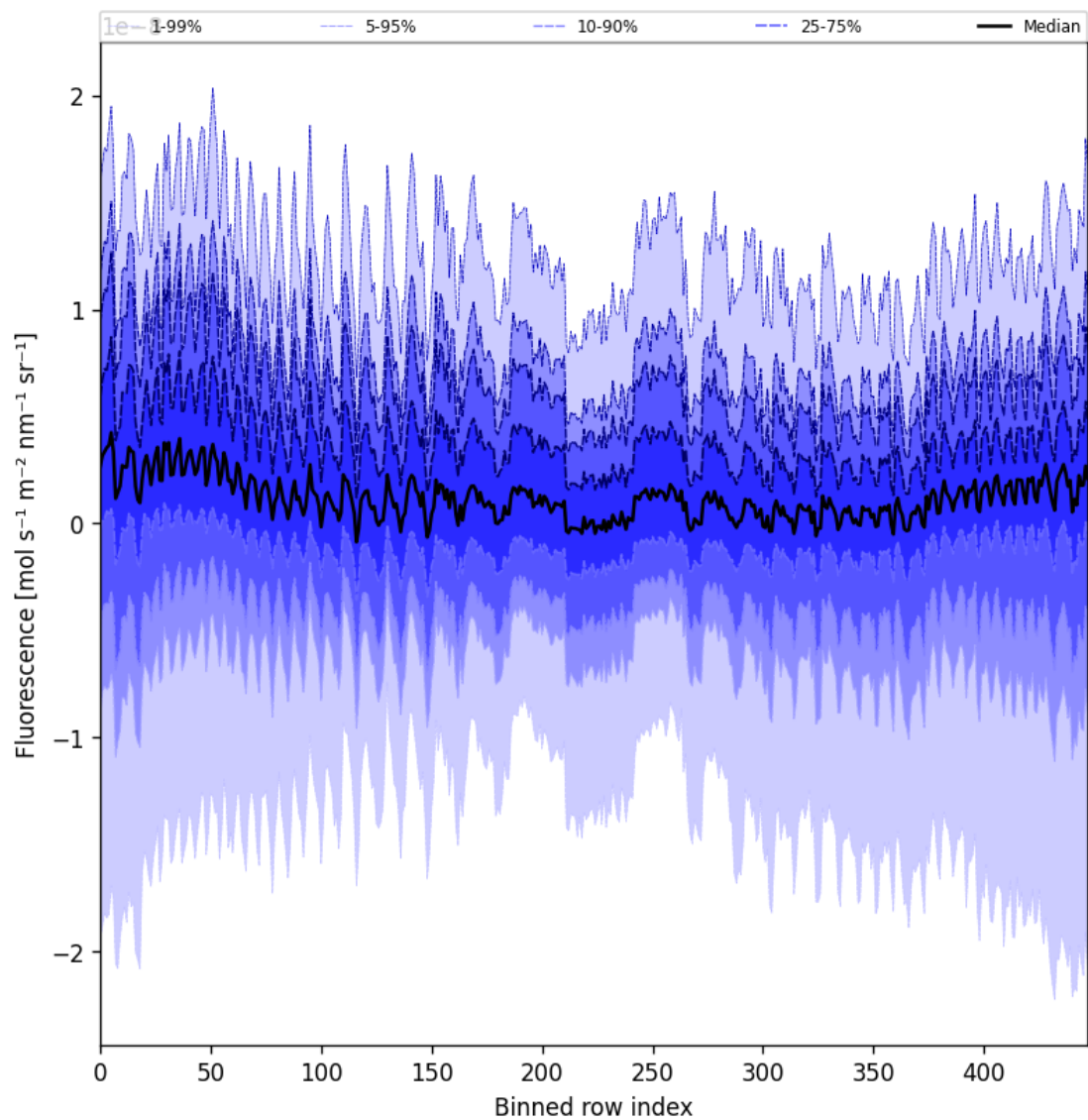
Figure 57: Along track statistics of “Fluorescence” for 2025-01-29 to 2025-01-31
