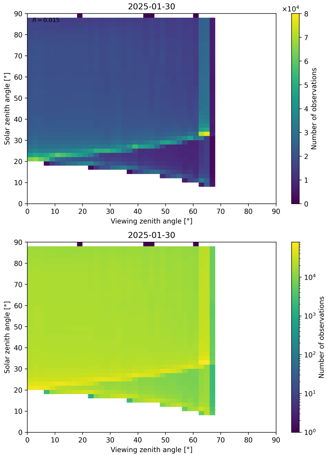
Figure 127: Scatter density plot of “Viewing zenith angle” against “Solar zenith angle” for 2025-01-29 to 2025-01-31.
