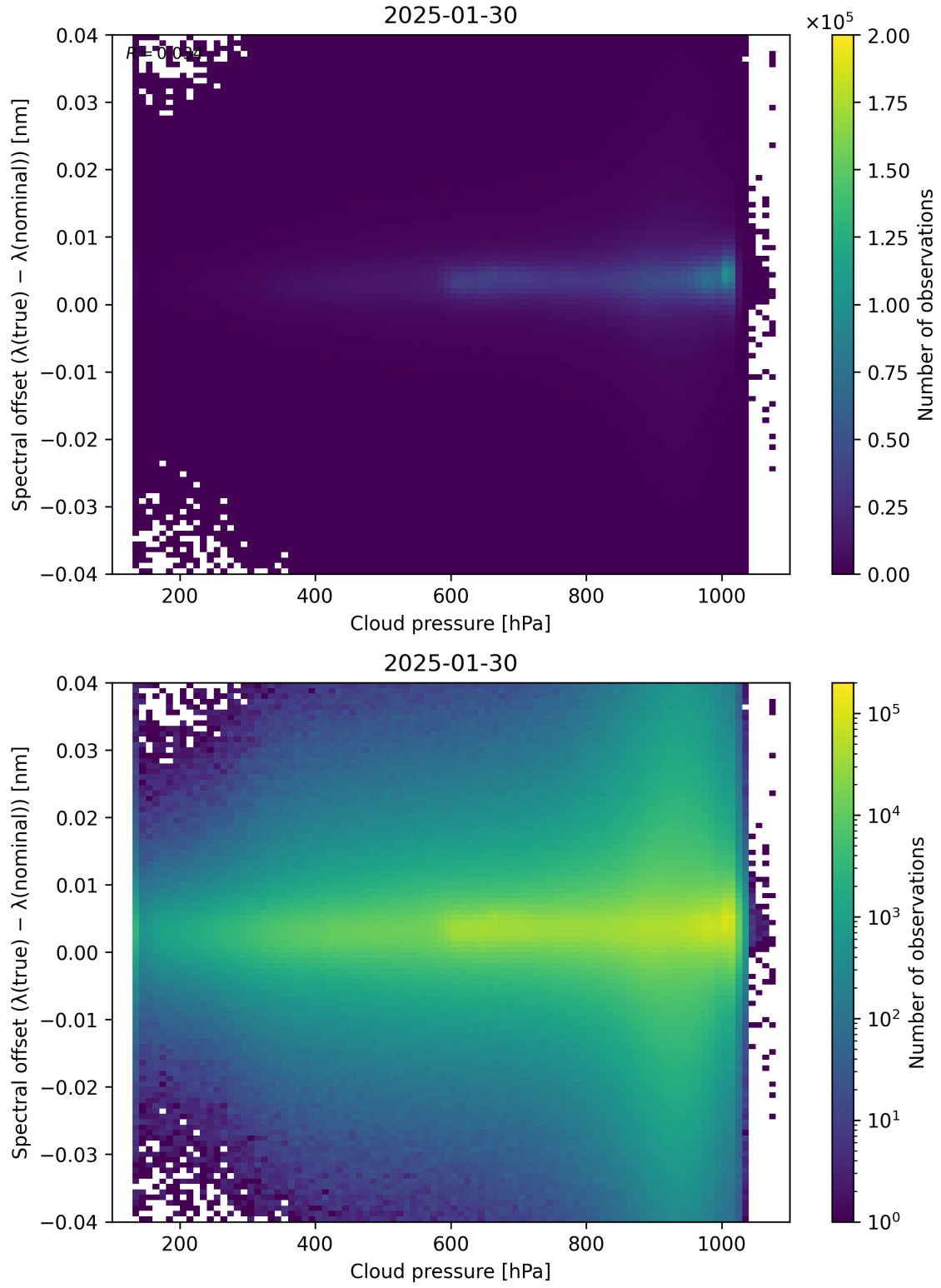
Figure 84: Scatter density plot of “Cloud pressure” against “Spectral offset ( \lambda_{\text{true}} - \lambda_{\text{nominal}} )” for 2025-01-29 to 2025-01-31.
