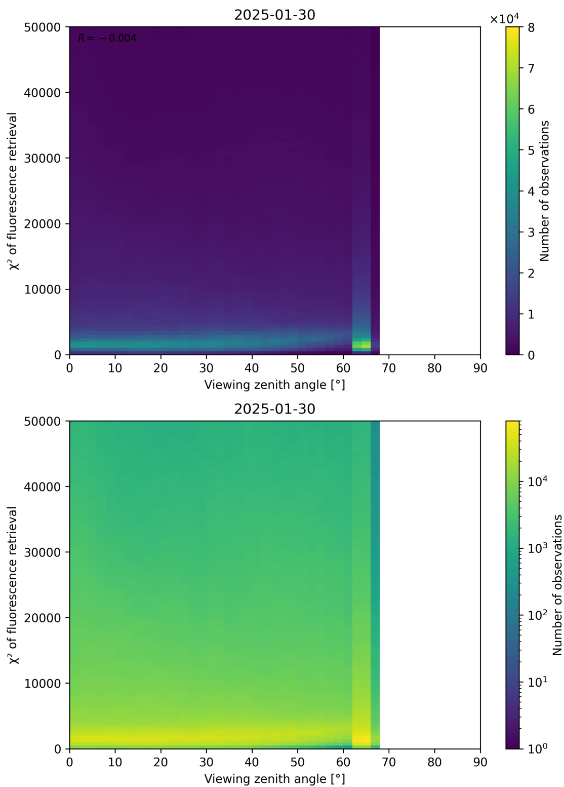
Figure 119: Scatter density plot of “Viewing zenith angle” against “ \chi^2 of fluorescence retrieval” for 2025-01-29 to 2025-01-31.
