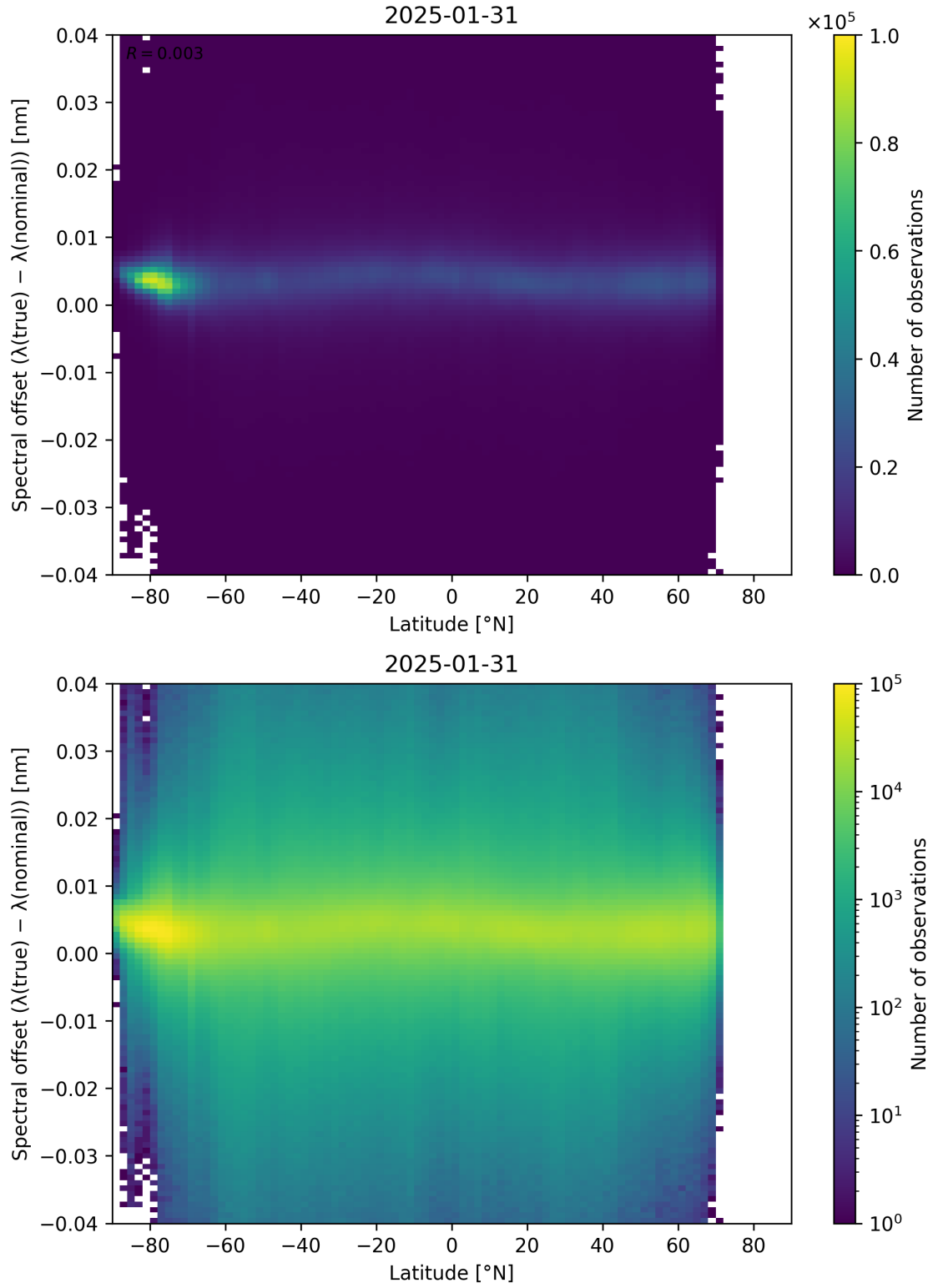
Figure 96: Scatter density plot of “Latitude” against “Spectral offset ( \lambda_{\text{true}} - \lambda_{\text{nominal}} )” for 2025-01-30 to 2025-02-01.
