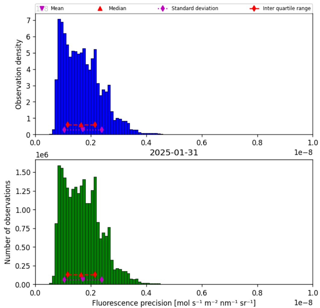
Figure 41: Histogram of “Fluorescence precision” for 2025-01-30 to 2025-02-01
