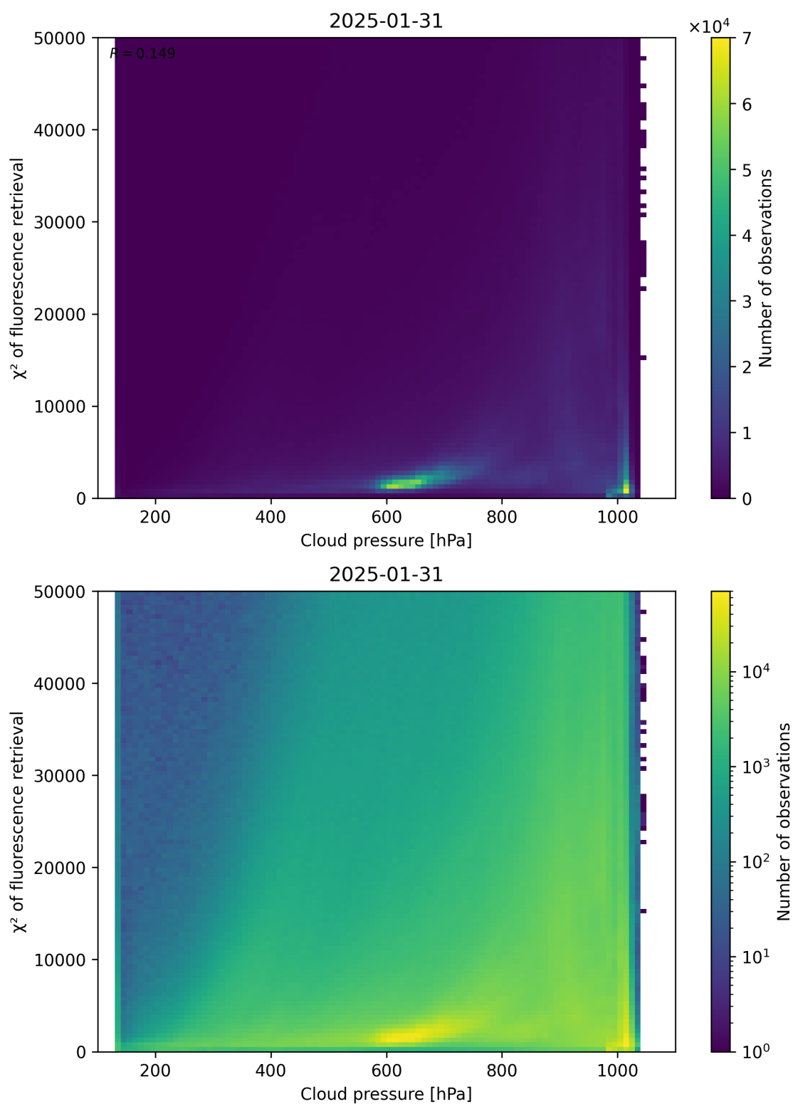
Figure 78: Scatter density plot of “Cloud pressure” against “ \chi^2 of fluorescence retrieval” for 2025-01-30 to 2025-02-01.
