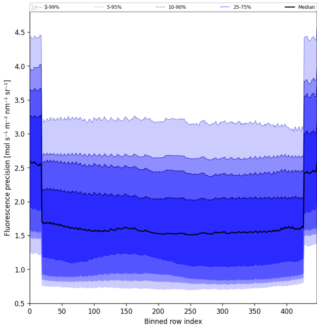
Figure 58: Along track statistics of “Fluorescence precision” for 2025-01-30 to 2025-02-01
