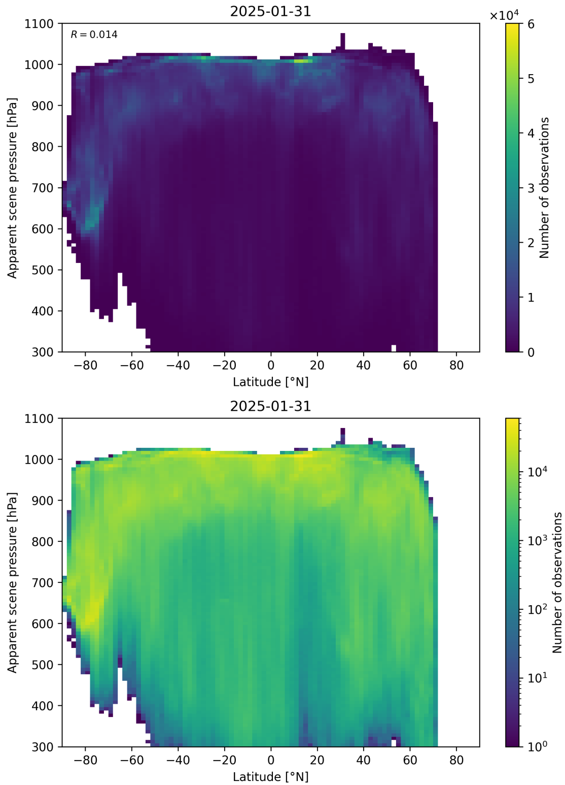
Figure 88: Scatter density plot of “Latitude” against “Apparent scene pressure” for 2025-01-30 to 2025-02-01.
