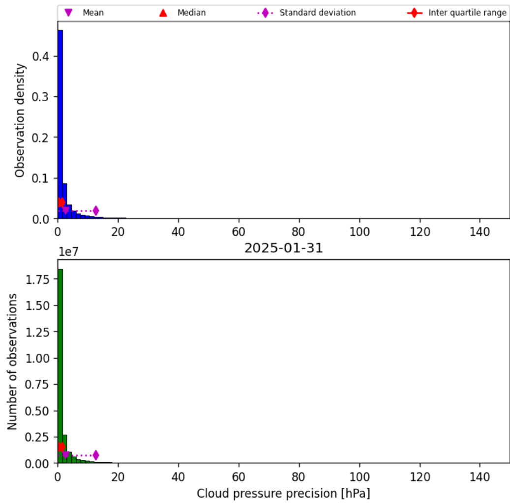
Figure 31: Histogram of “Cloud pressure precision” for 2025-01-30 to 2025-02-01
