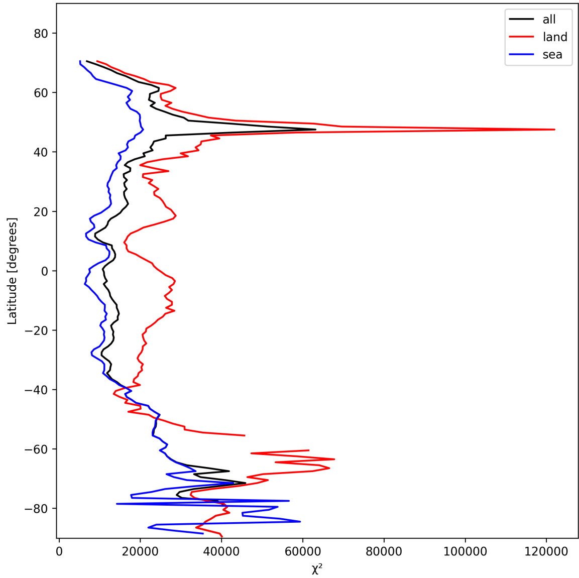
Figure 21: Zonal average of “ \chi^2 ” for 2025-01-30 to 2025-02-01.
