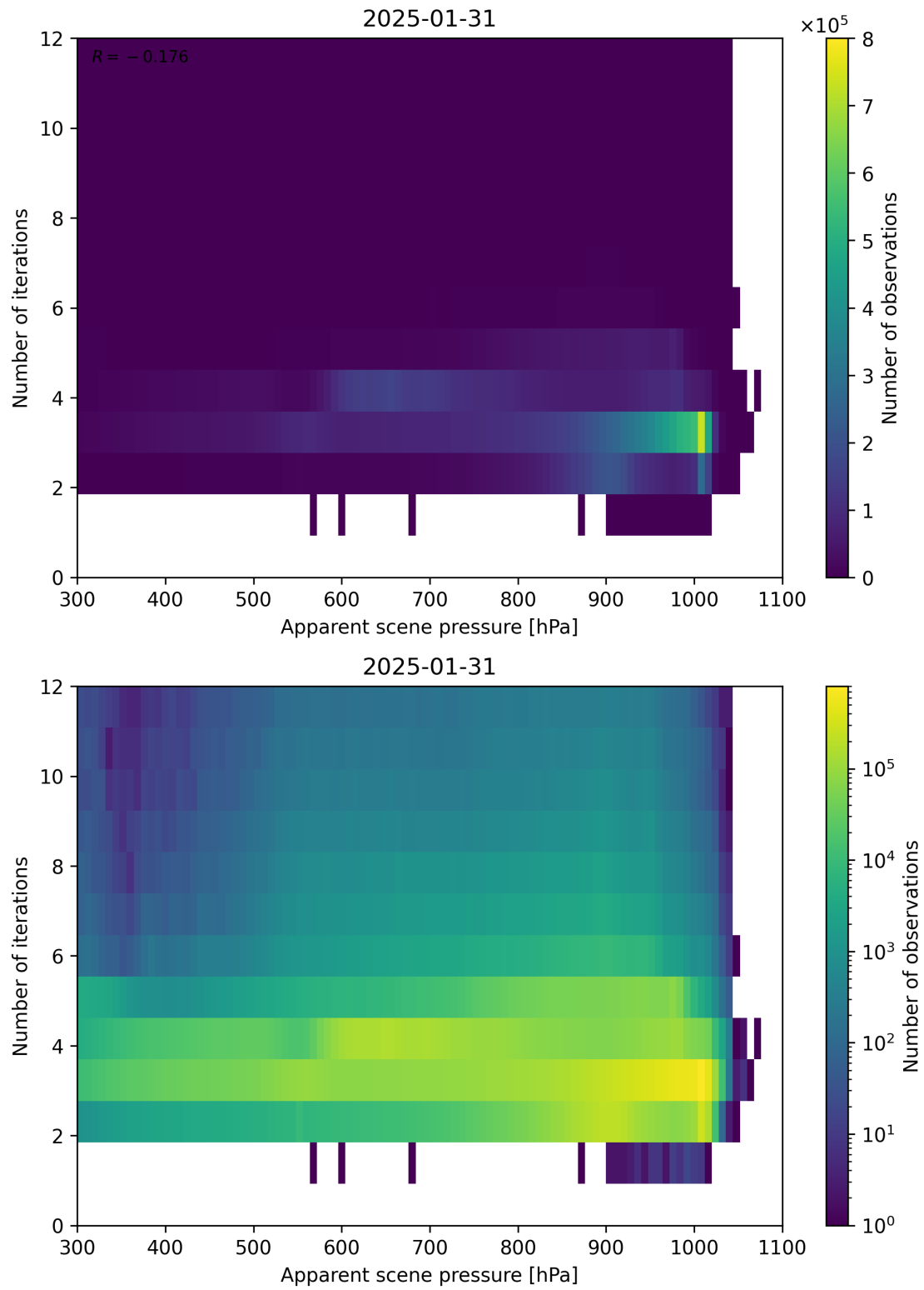
Figure 65: Scatter density plot of “Apparent scene pressure” against “Number of iterations” for 2025-01-30 to 2025-02-01.
