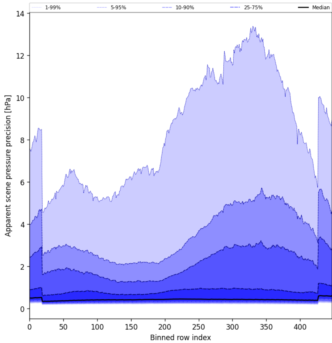
Figure 54: Along track statistics of “Apparent scene pressure precision” for 2025-01-30 to 2025-02-01
