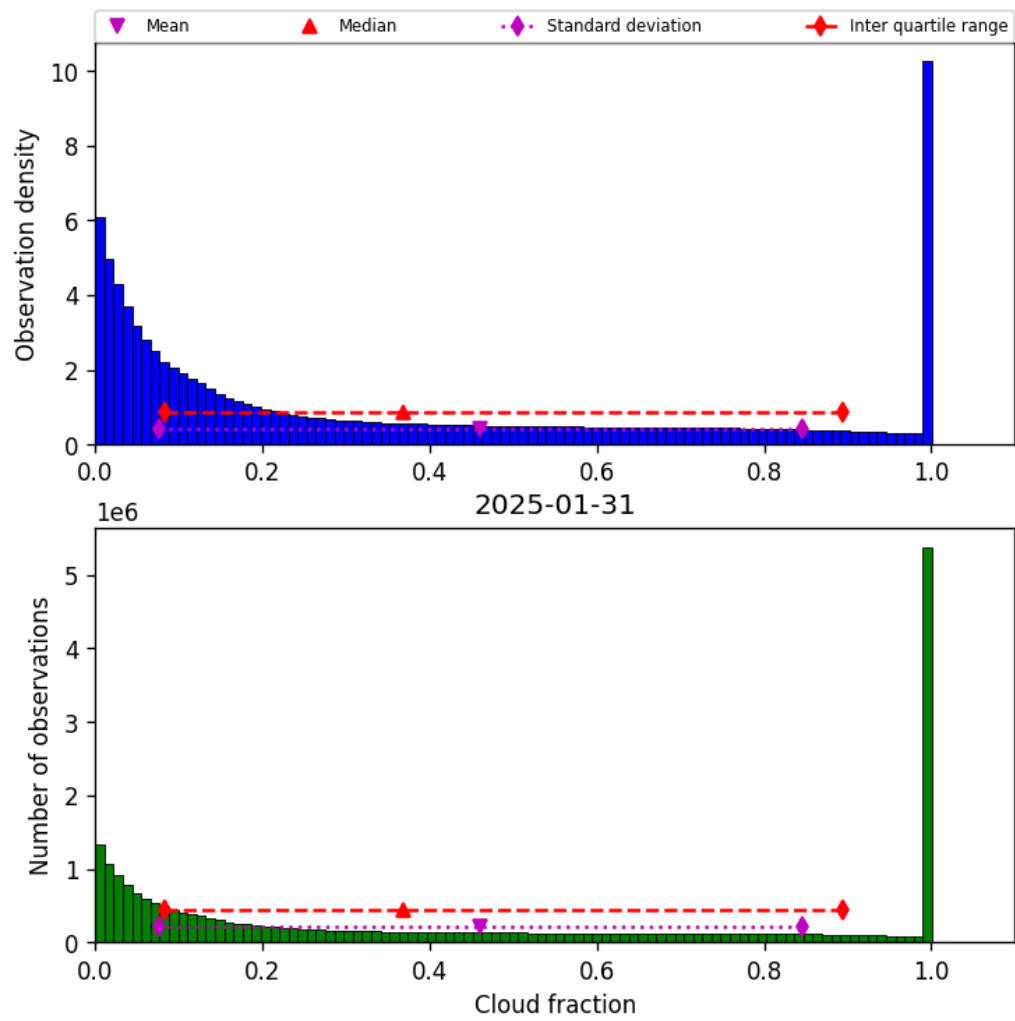
Figure 32: Histogram of “Cloud fraction” for 2025-01-30 to 2025-02-01
