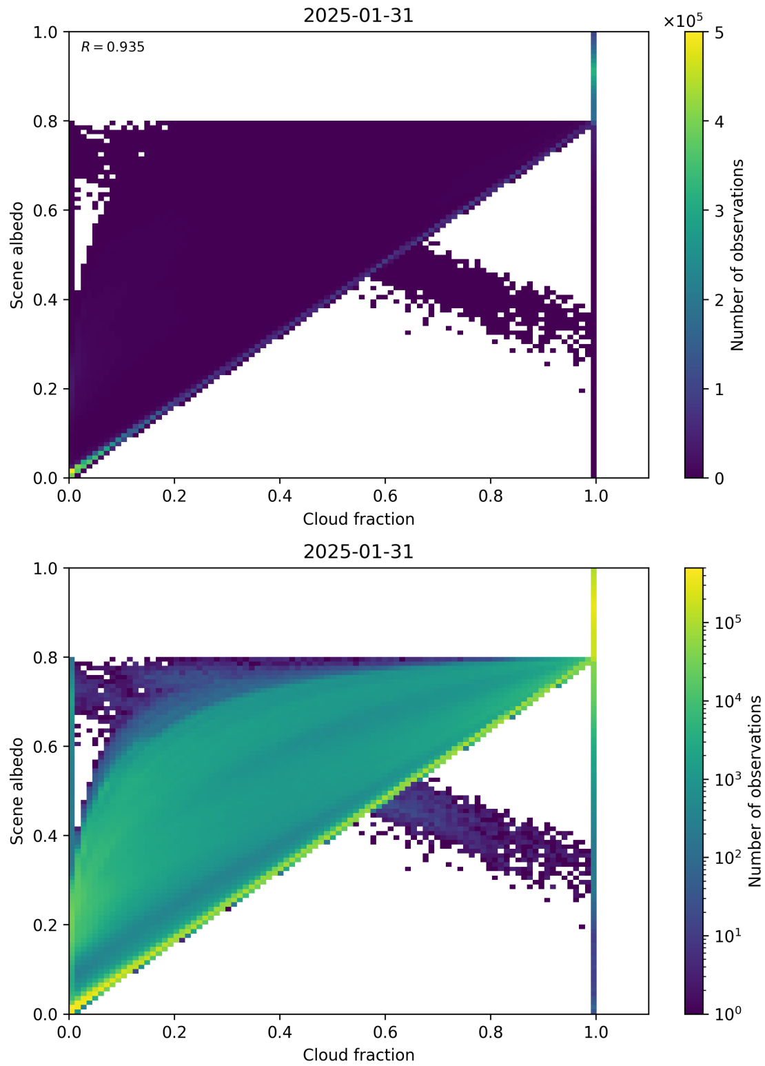
Figure 75: Scatter density plot of “Cloud fraction” against “Scene albedo” for 2025-01-30 to 2025-02-01.
