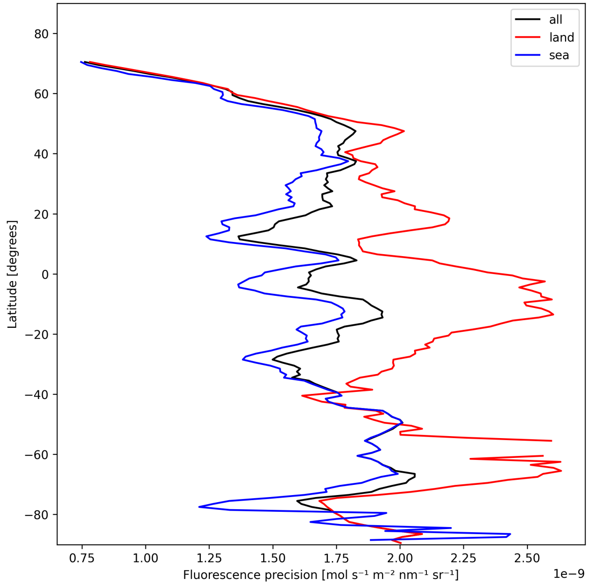
Figure 24: Zonal average of “Fluorescence precision” for 2025-01-30 to 2025-02-01.
