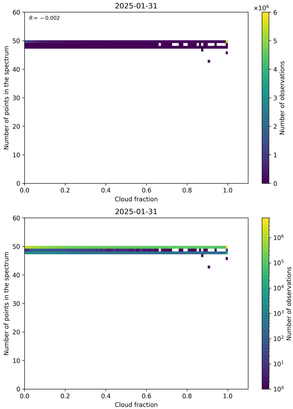
Figure 74: Scatter density plot of “Cloud fraction” against “Number of points in the spectrum” for 2025-01-30 to 2025-02-01.
