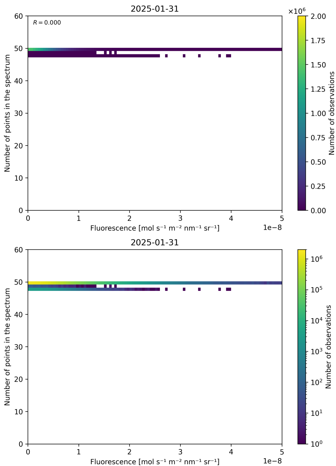
Figure 86: Scatter density plot of “Fluorescence” against “Number of points in the spectrum” for 2025-01-30 to 2025-02-01.
