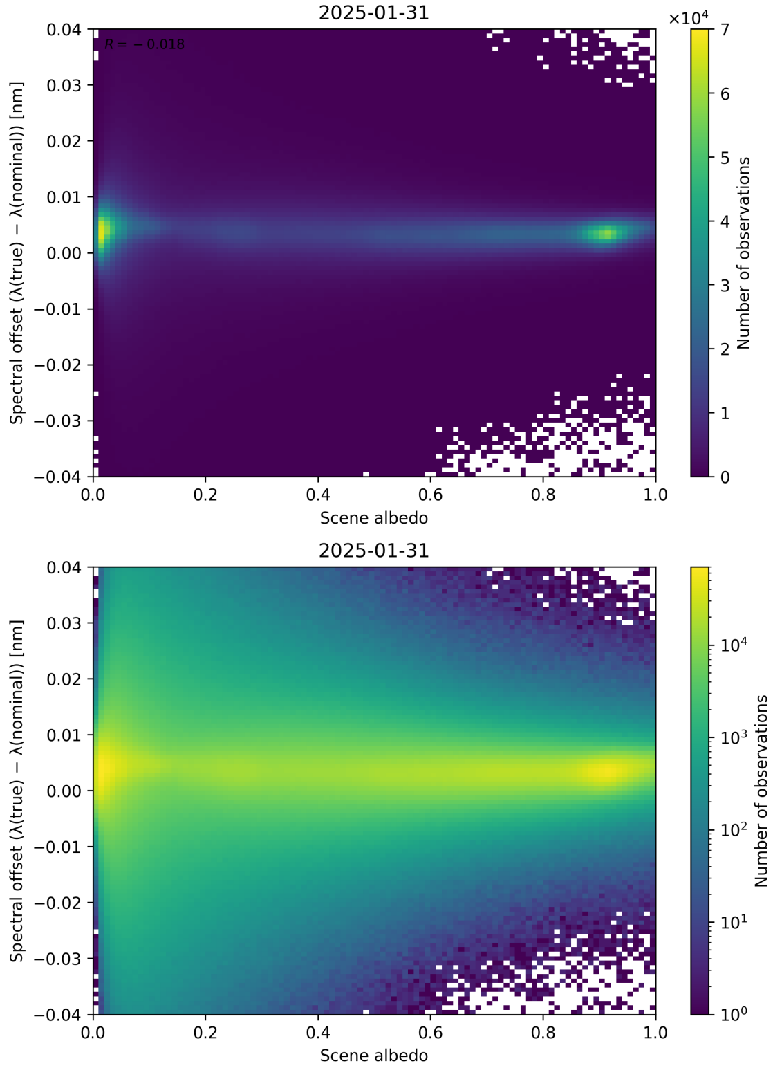
Figure 107: Scatter density plot of “Scene albedo” against “Spectral offset ( \lambda_{\text{true}} - \lambda_{\text{nominal}} )” for 2025-01-30 to 2025-02-01.
