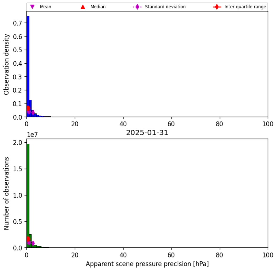
Figure 37: Histogram of “Apparent scene pressure precision” for 2025-01-30 to 2025-02-01
