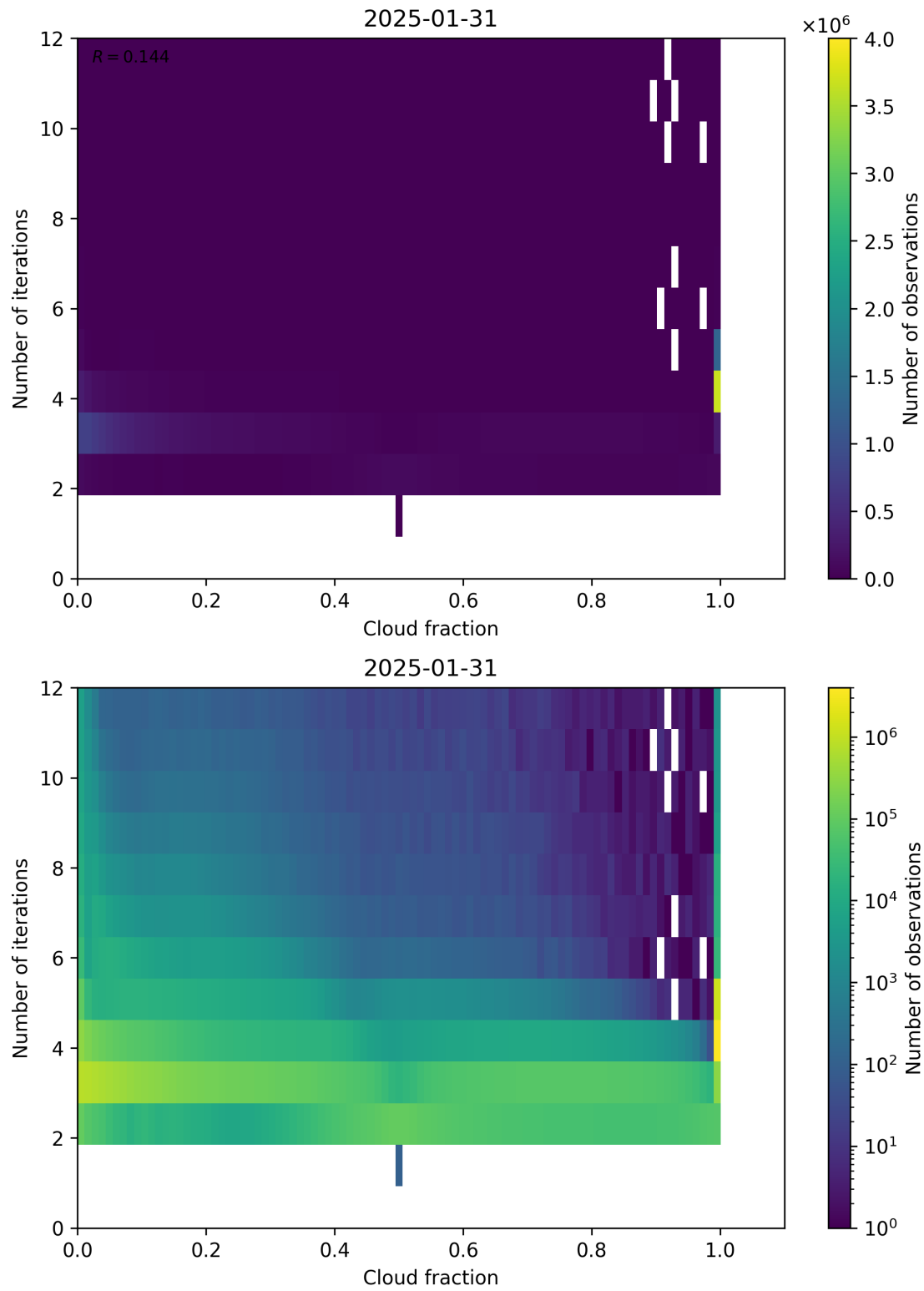
Figure 73: Scatter density plot of “Cloud fraction” against “Number of iterations” for 2025-01-30 to 2025-02-01.
