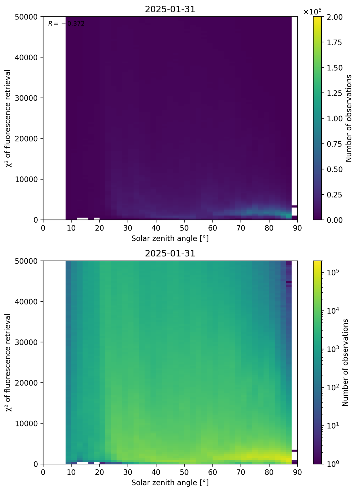
Figure 109: Scatter density plot of “Solar zenith angle” against “ \chi^2 of fluorescence retrieval” for 2025-01-30 to 2025-02-01.
