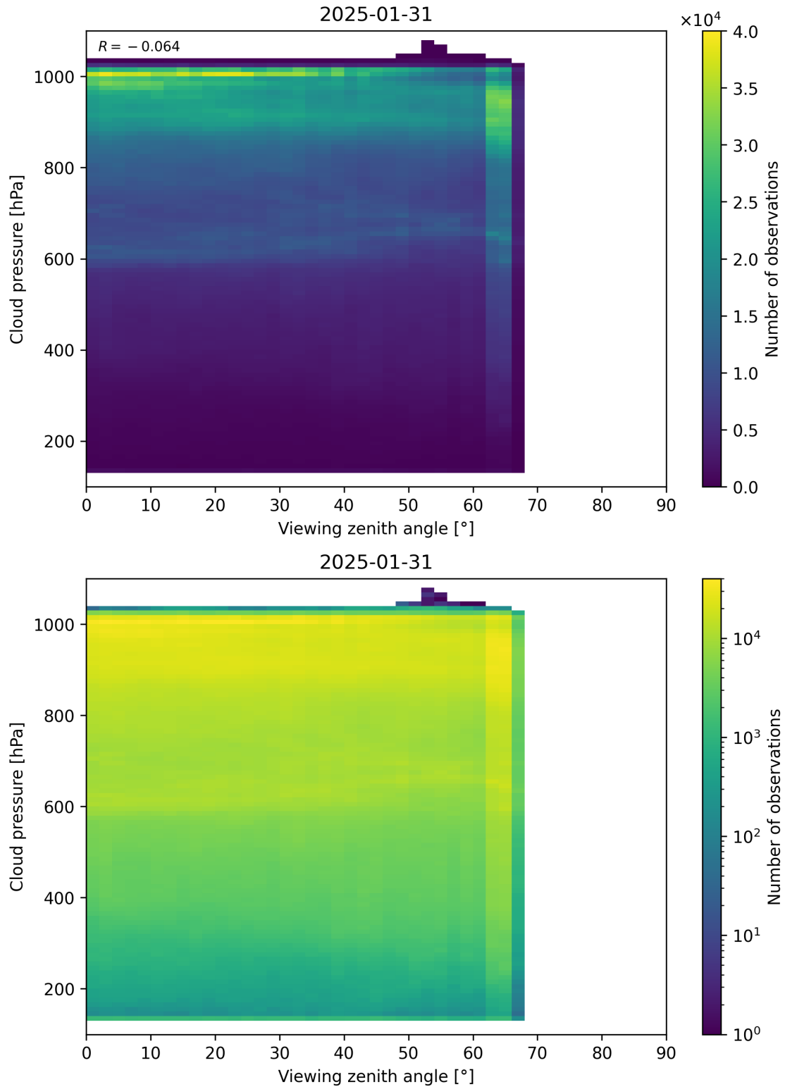
Figure 121: Scatter density plot of “Viewing zenith angle” against “Cloud pressure” for 2025-01-30 to 2025-02-01.
