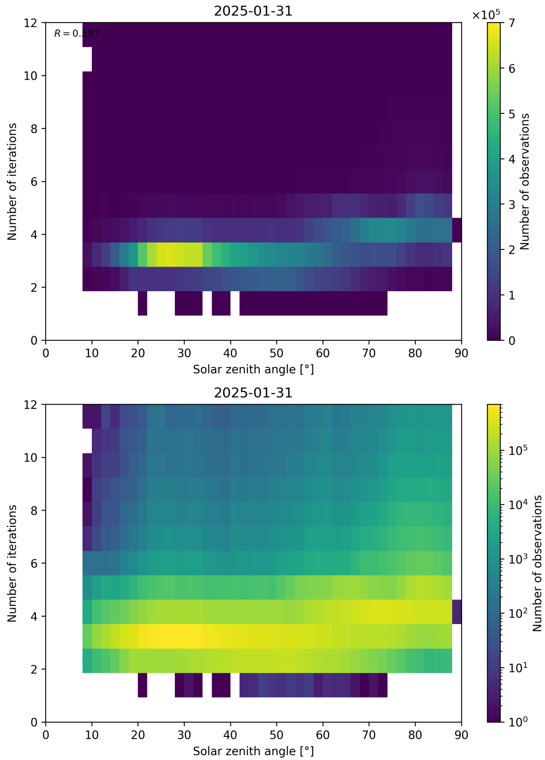
Figure 114: Scatter density plot of “Solar zenith angle” against “Number of iterations” for 2025-01-30 to 2025-02-01.
