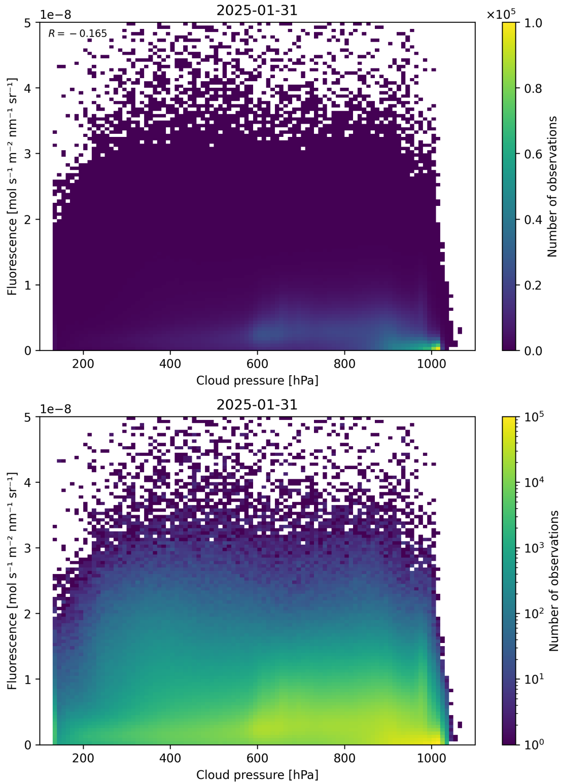
Figure 80: Scatter density plot of “Cloud pressure” against “Fluorescence” for 2025-01-30 to 2025-02-01.
