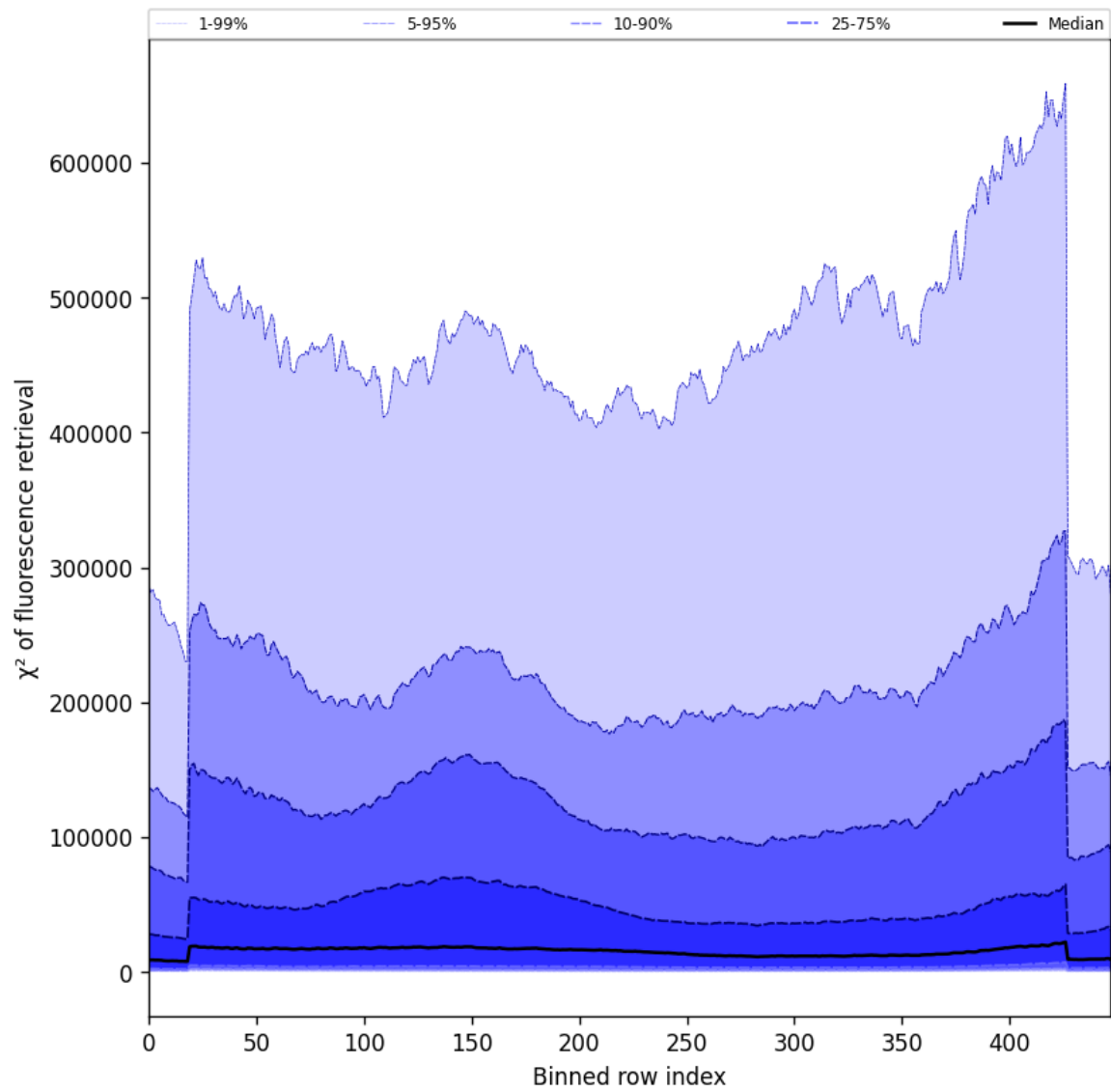
Figure 59: Along track statistics of “ \chi^2 of fluorescence retrieval” for 2025-01-30 to 2025-02-01
