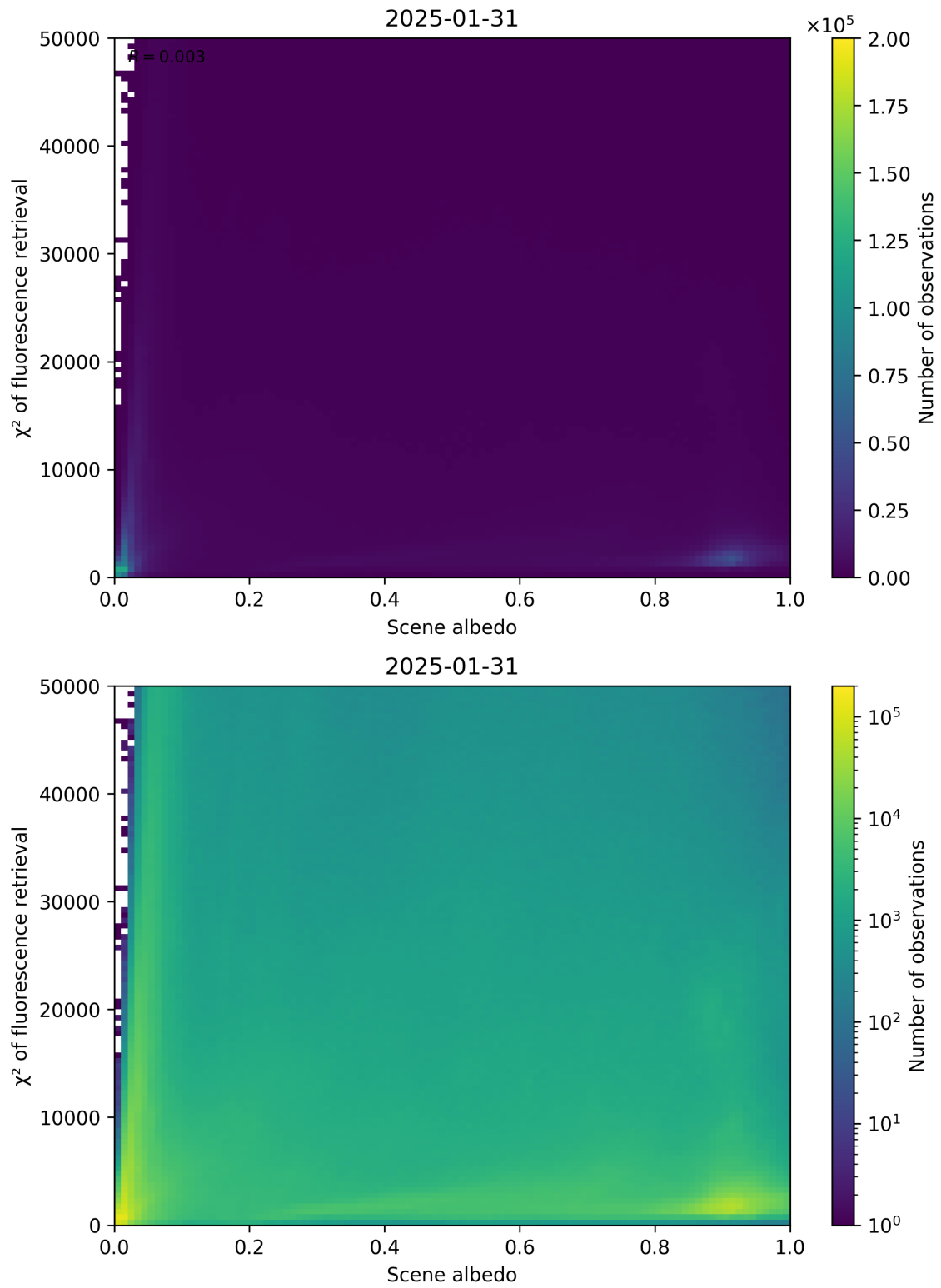
Figure 103: Scatter density plot of “Scene albedo” against “ \chi^2 of fluorescence retrieval” for 2025-01-30 to 2025-02-01.
