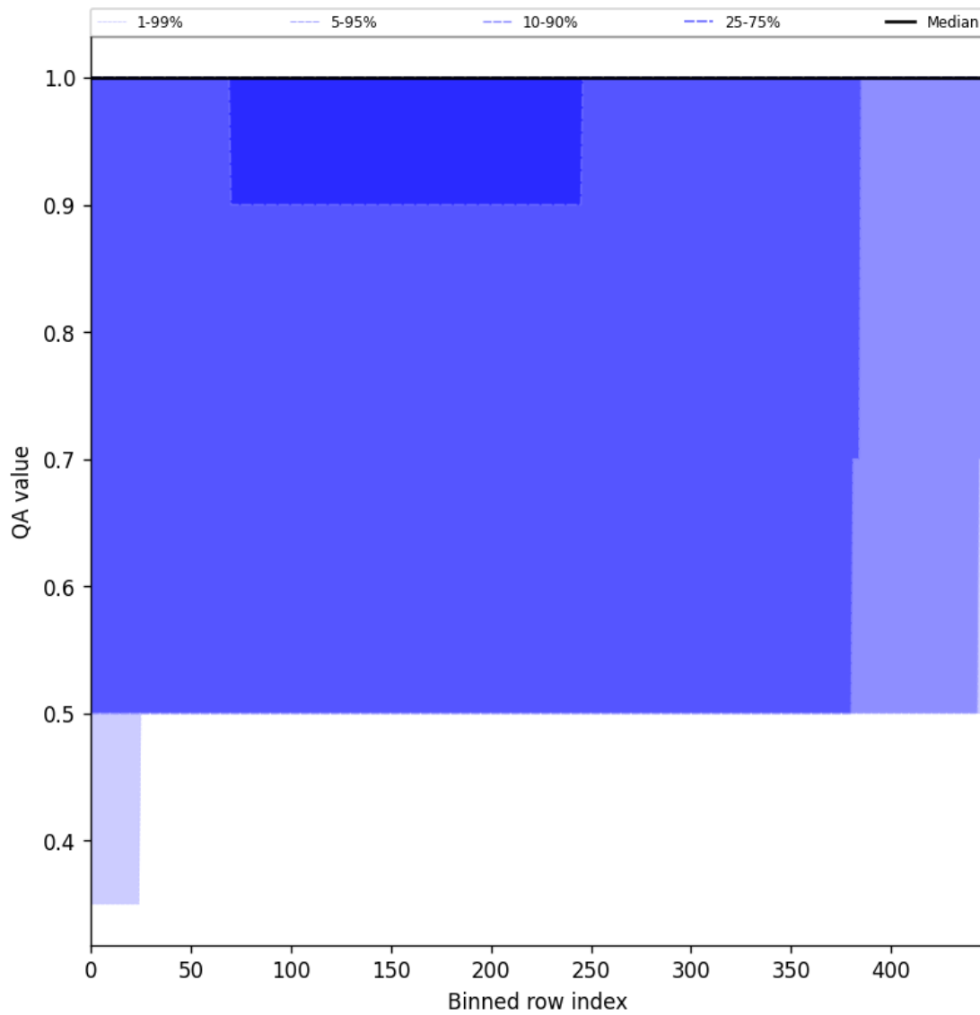
Figure 46: Along track statistics of “QA value” for 2025-01-30 to 2025-02-01
