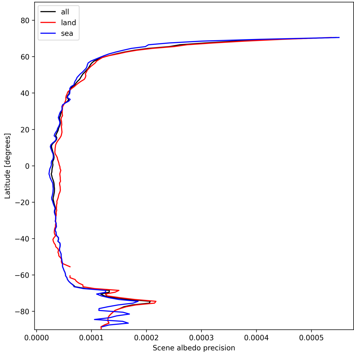
Figure 18: Zonal average of “Scene albedo precision” for 2025-01-30 to 2025-02-01.
