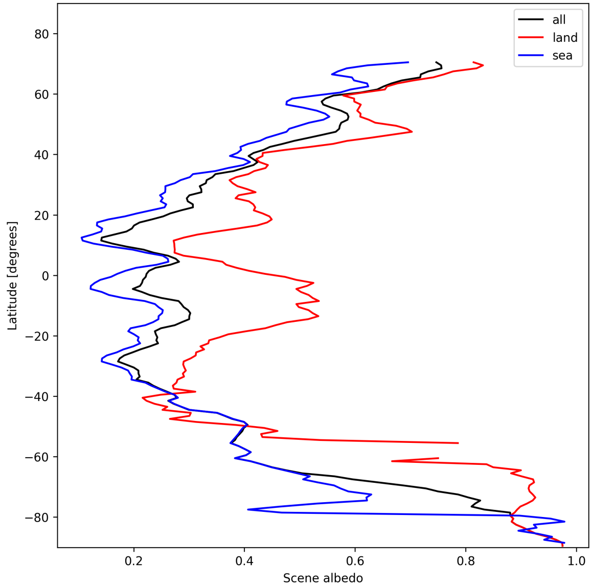
Figure 17: Zonal average of “Scene albedo” for 2025-01-30 to 2025-02-01.
