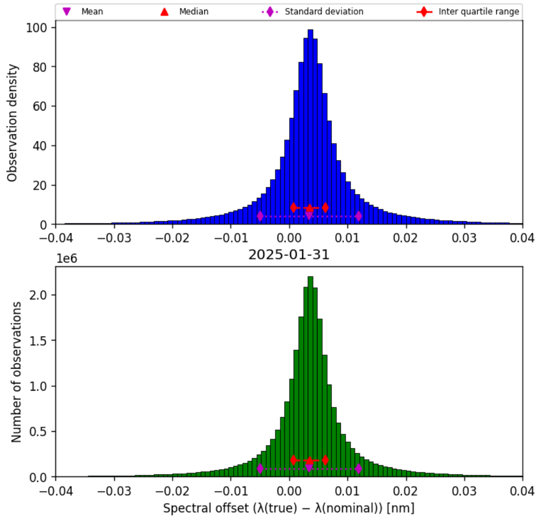
Figure 45: Histogram of “Spectral offset ( \lambda_{\text{true}} - \lambda_{\text{nominal}} )” for 2025-01-30 to 2025-02-01
