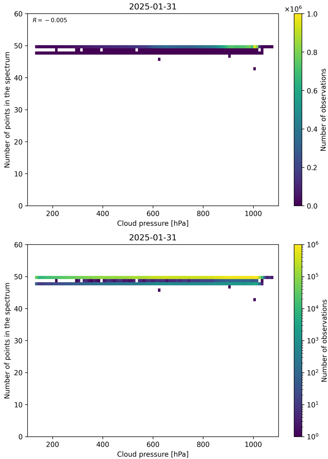
Figure 82: Scatter density plot of “Cloud pressure” against “Number of points in the spectrum” for 2025-01-30 to 2025-02-01.
