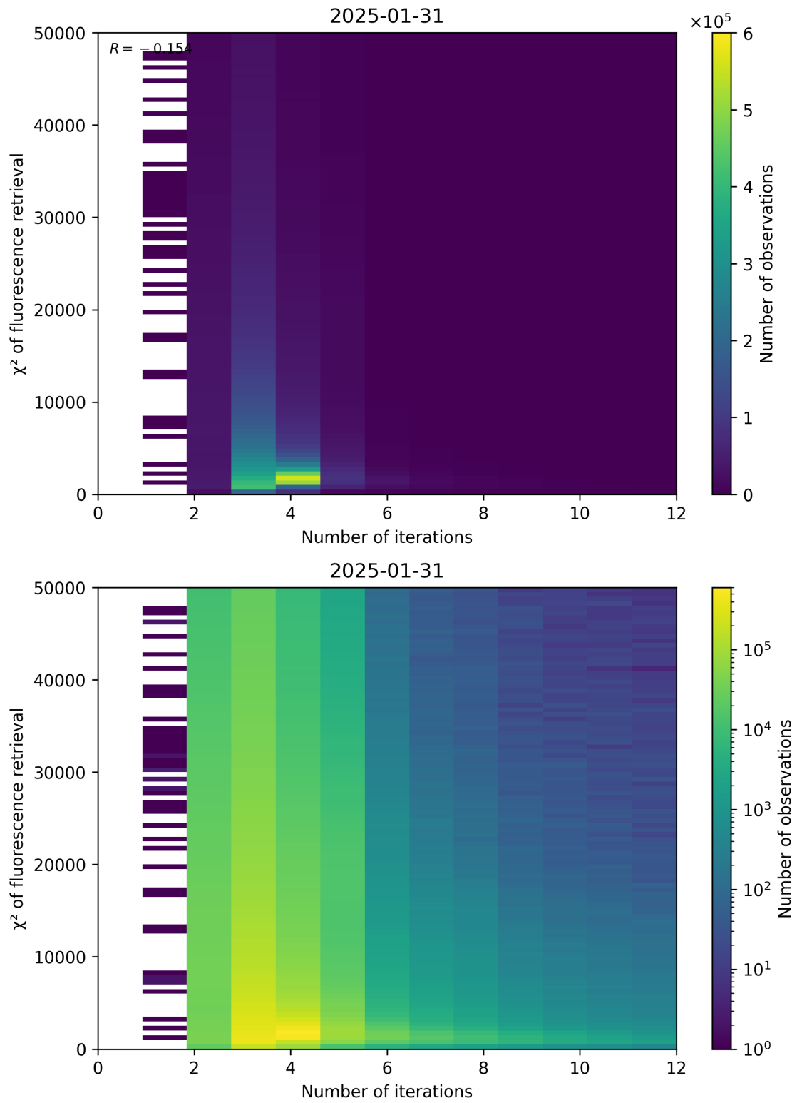
Figure 97: Scatter density plot of “Number of iterations” against “ \chi^2 of fluorescence retrieval” for 2025-01-30 to 2025-02-01.
