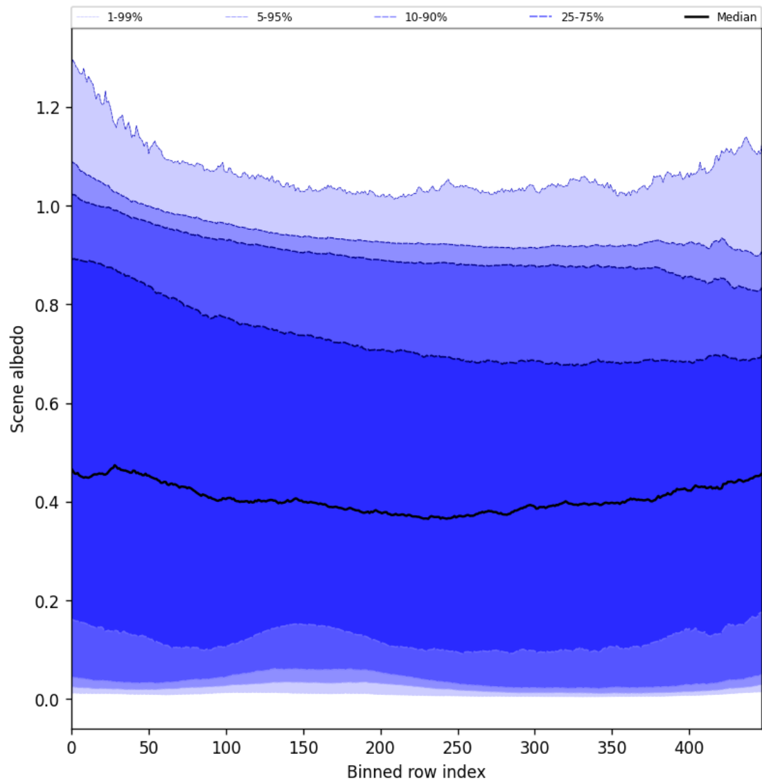
Figure 51: Along track statistics of “Scene albedo” for 2025-01-30 to 2025-02-01
