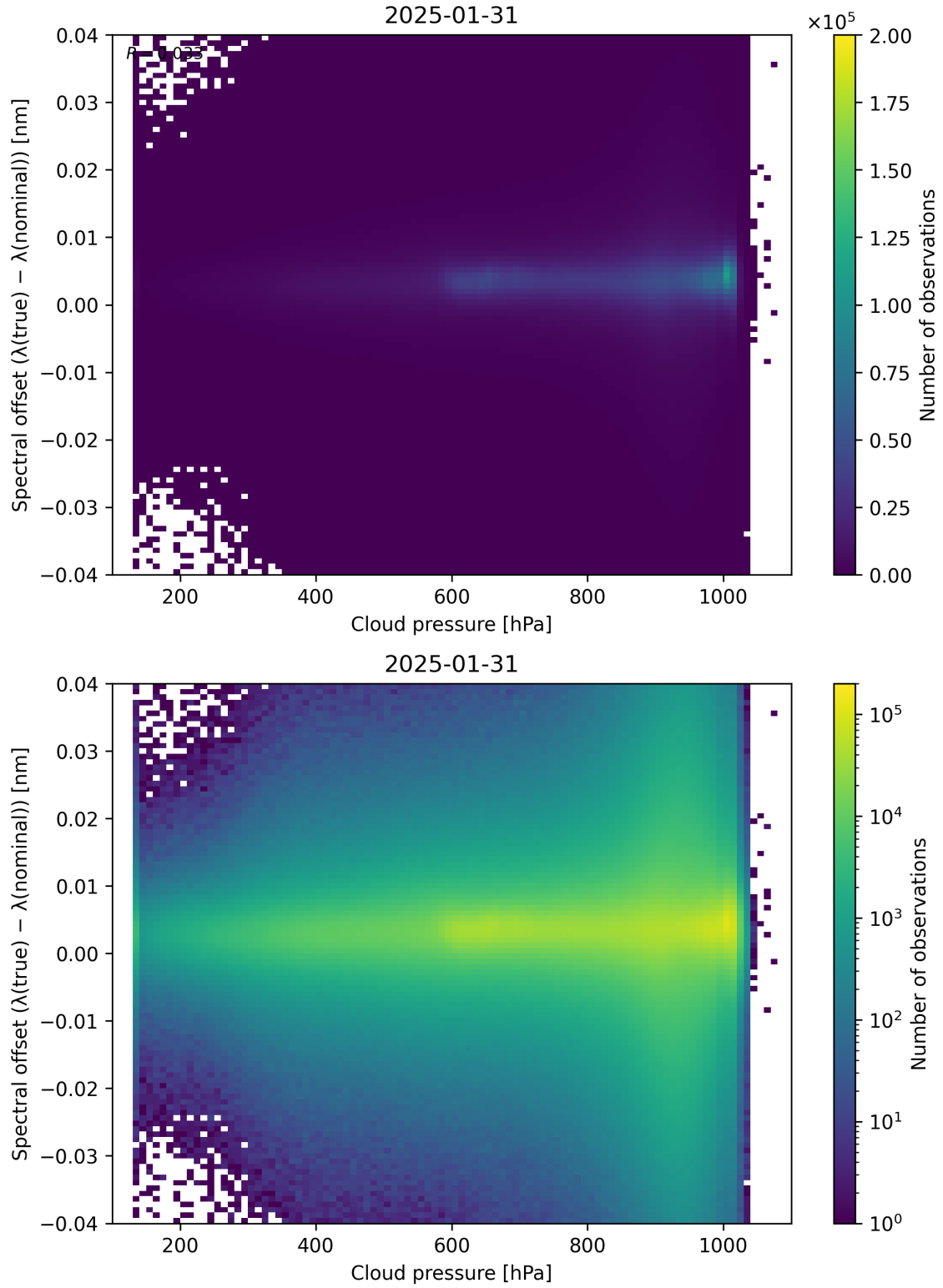
Figure 84: Scatter density plot of “Cloud pressure” against “Spectral offset ( \lambda_{\text{true}} - \lambda_{\text{nominal}} )” for 2025-01-30 to 2025-02-01.
