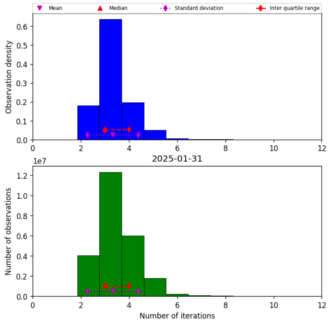
Figure 39: Histogram of “Number of iterations” for 2025-01-30 to 2025-02-01
