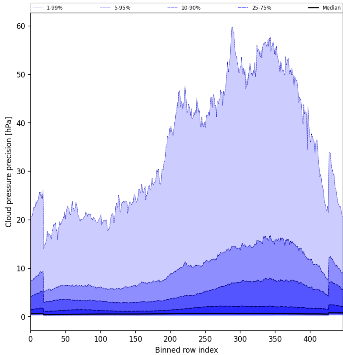
Figure 48: Along track statistics of “Cloud pressure precision” for 2025-01-30 to 2025-02-01
