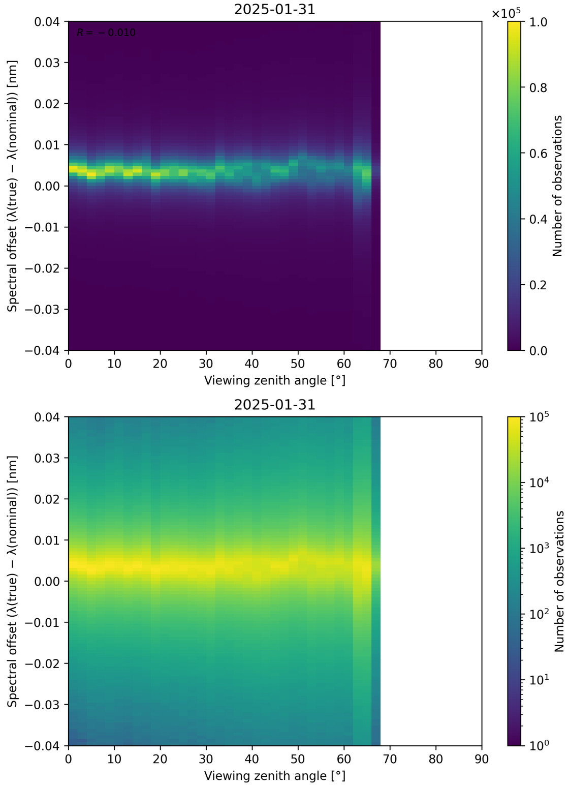
Figure 128: Scatter density plot of “Viewing zenith angle” against “Spectral offset ( \lambda_{\text{true}} - \lambda_{\text{nominal}} )” for 2025-01-30 to 2025-02-01.
