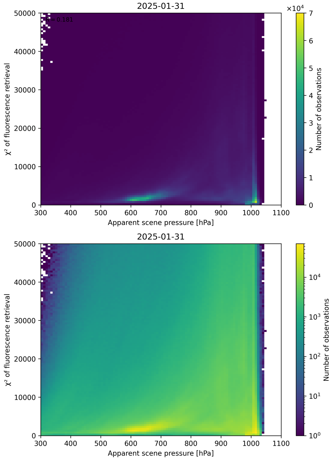
Figure 63: Scatter density plot of “Apparent scene pressure” against “ \chi^2 of fluorescence retrieval” for 2025-01-30 to 2025-02-01.
