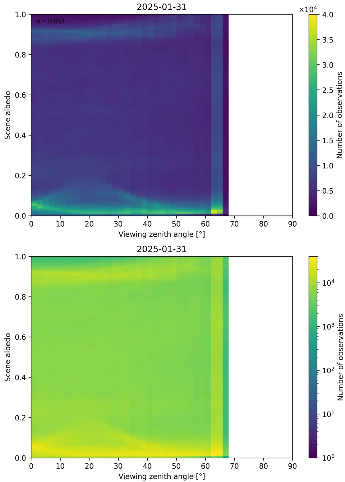
Figure 126: Scatter density plot of “Viewing zenith angle” against “Scene albedo” for 2025-01-30 to 2025-02-01.
