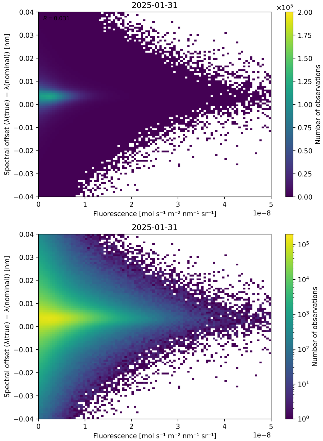
Figure 87: Scatter density plot of “Fluorescence” against “Spectral offset ( \lambda_{\text{true}} - \lambda_{\text{nominal}} )” for 2025-01-30 to 2025-02-01.
