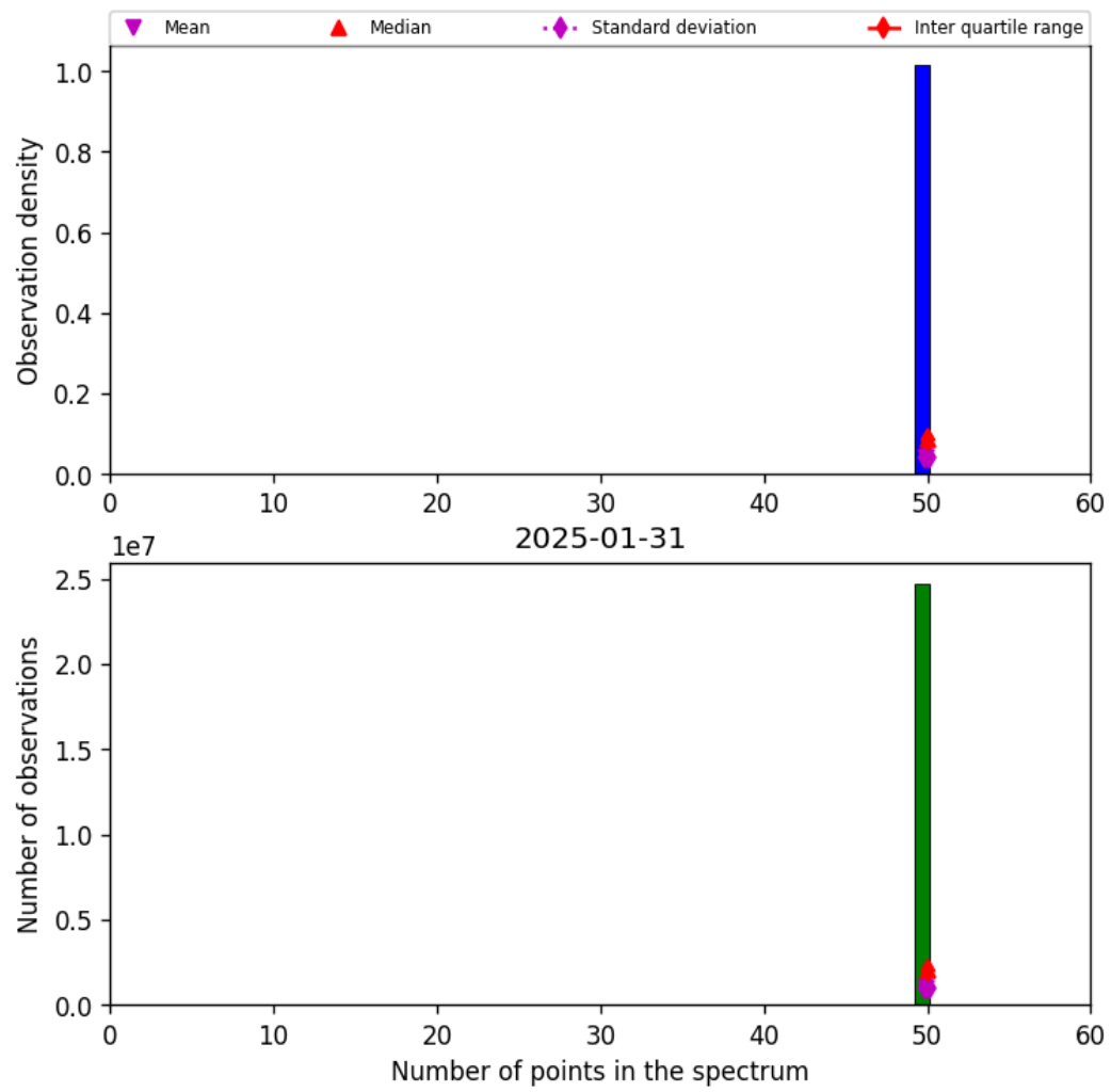
Figure 44: Histogram of "Number of points in the spectrum" for 2025-01-30 to 2025-02-01
