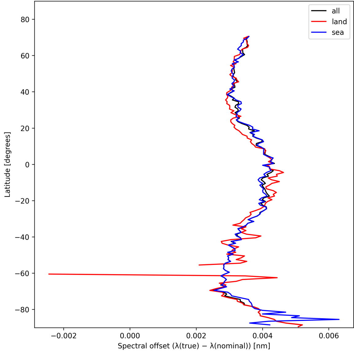
Figure 28: Zonal average of “Spectral offset ( \lambda_{\text{true}} - \lambda_{\text{nominal}} )” for 2025-01-30 to 2025-02-01.
