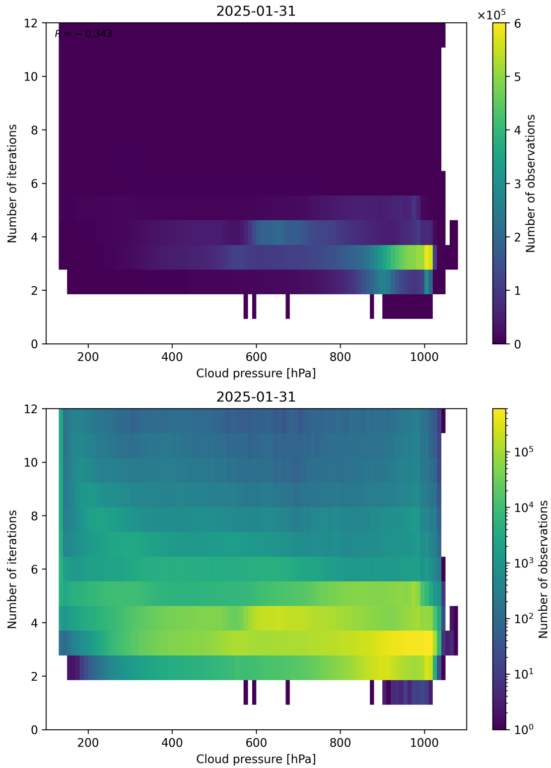
Figure 81: Scatter density plot of “Cloud pressure” against “Number of iterations” for 2025-01-30 to 2025-02-01.
