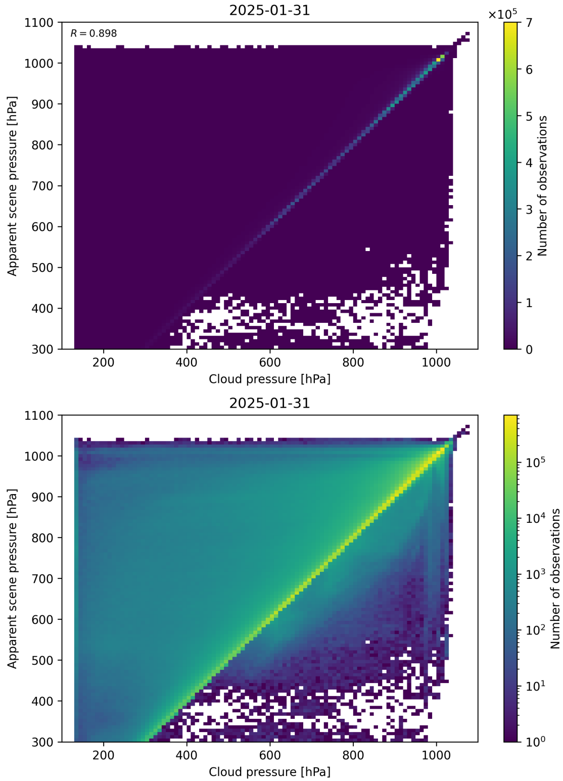
Figure 77: Scatter density plot of “Cloud pressure” against “Apparent scene pressure” for 2025-01-30 to 2025-02-01.
