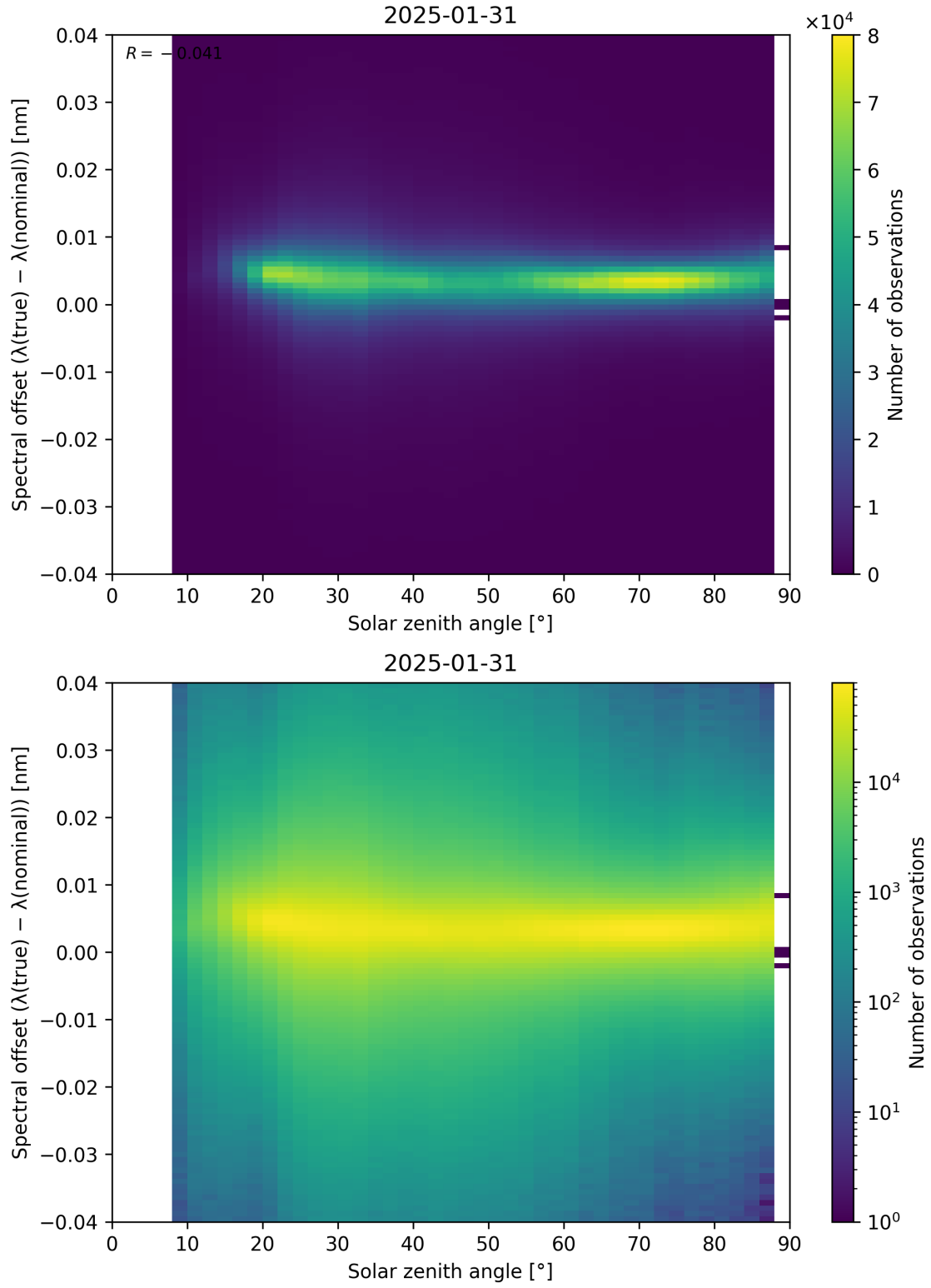
Figure 117: Scatter density plot of “Solar zenith angle” against “Spectral offset ( \lambda_{\text{true}} - \lambda_{\text{nominal}} )” for 2025-01-30 to 2025-02-01.
