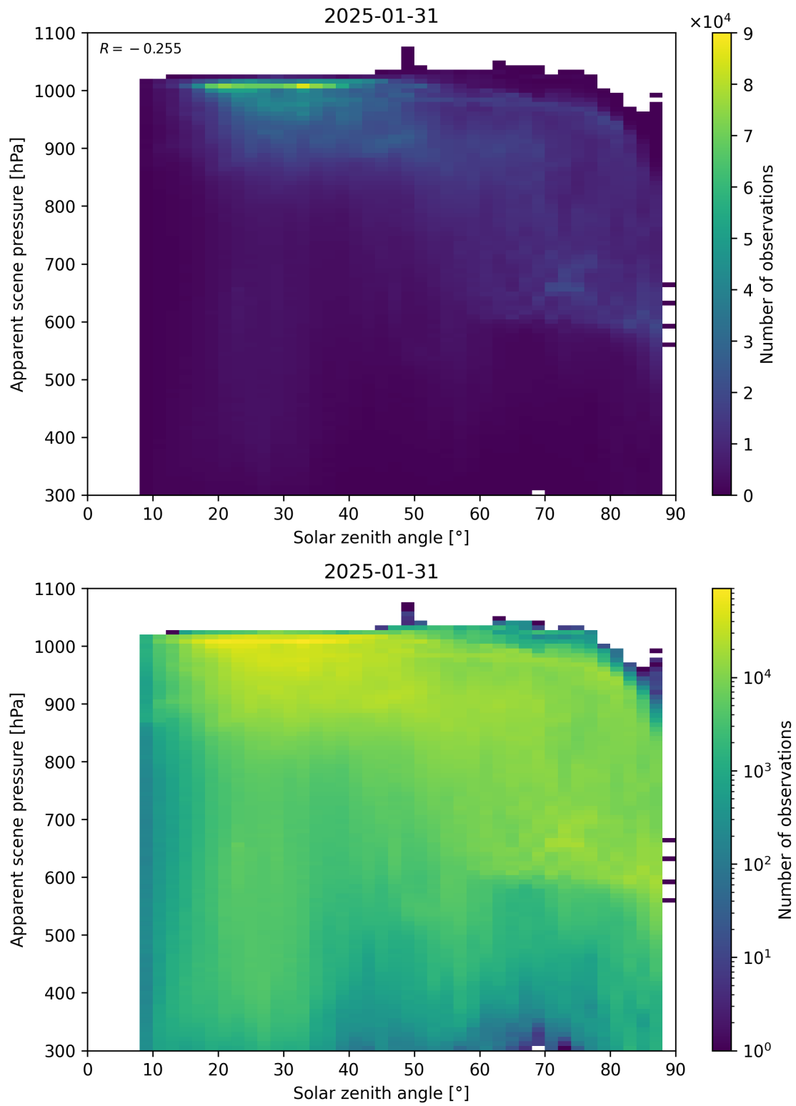
Figure 108: Scatter density plot of “Solar zenith angle” against “Apparent scene pressure” for 2025-01-30 to 2025-02-01.
