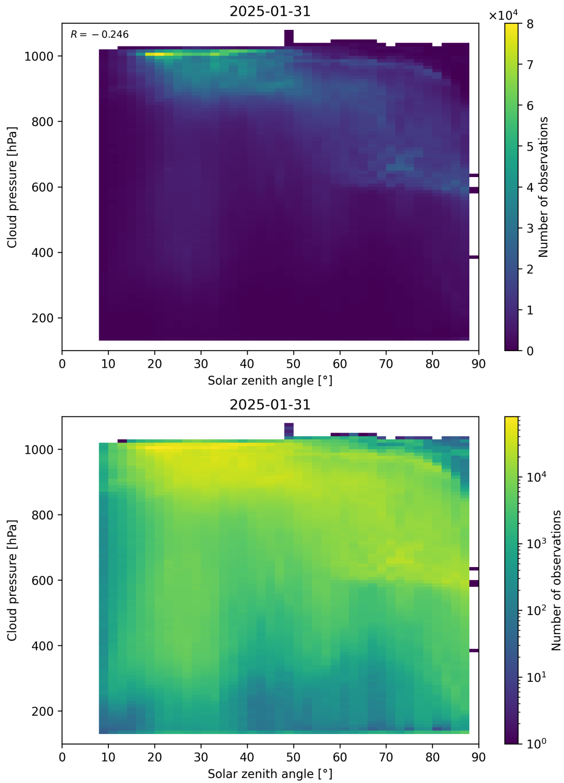
Figure 111: Scatter density plot of “Solar zenith angle” against “Cloud pressure” for 2025-01-30 to 2025-02-01.
