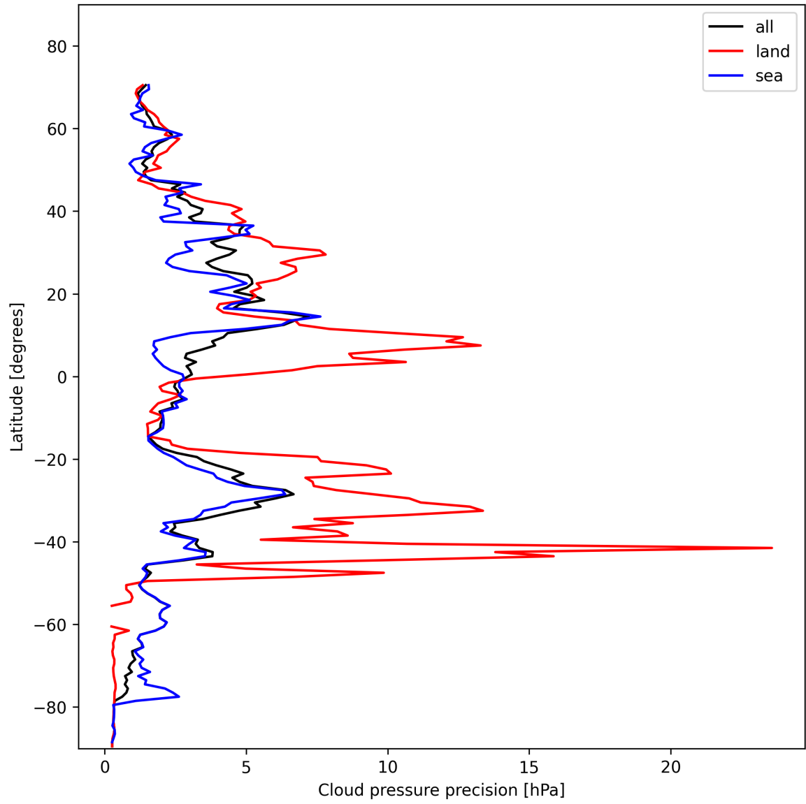
Figure 14: Zonal average of "Cloud pressure precision" for 2025-01-30 to 2025-02-01.
