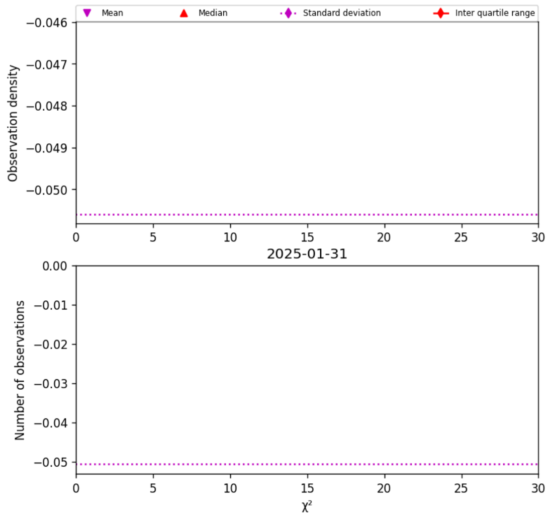
Figure 38: Histogram of “ \chi^2 ” for 2025-01-30 to 2025-02-01
