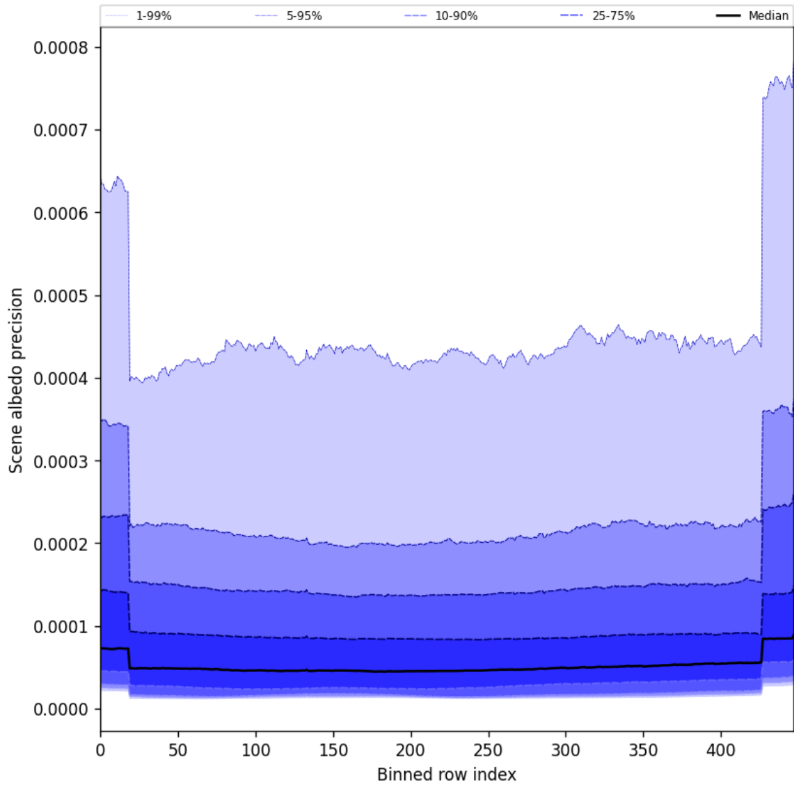
Figure 52: Along track statistics of “Scene albedo precision” for 2025-01-30 to 2025-02-01
