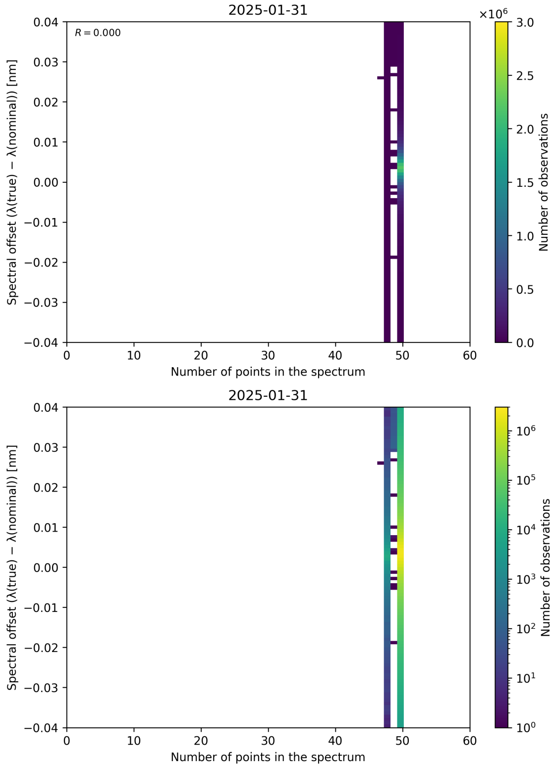
Figure 101: Scatter density plot of “Number of points in the spectrum” against “Spectral offset ( \lambda_{\text{true}} - \lambda_{\text{nominal}} )” for 2025-01-30 to 2025-02-01.
