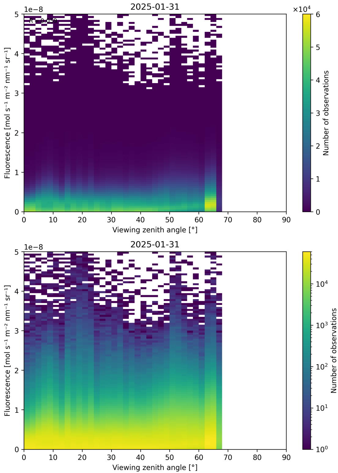
Figure 122: Scatter density plot of “Viewing zenith angle” against “Fluorescence” for 2025-01-30 to 2025-02-01.
