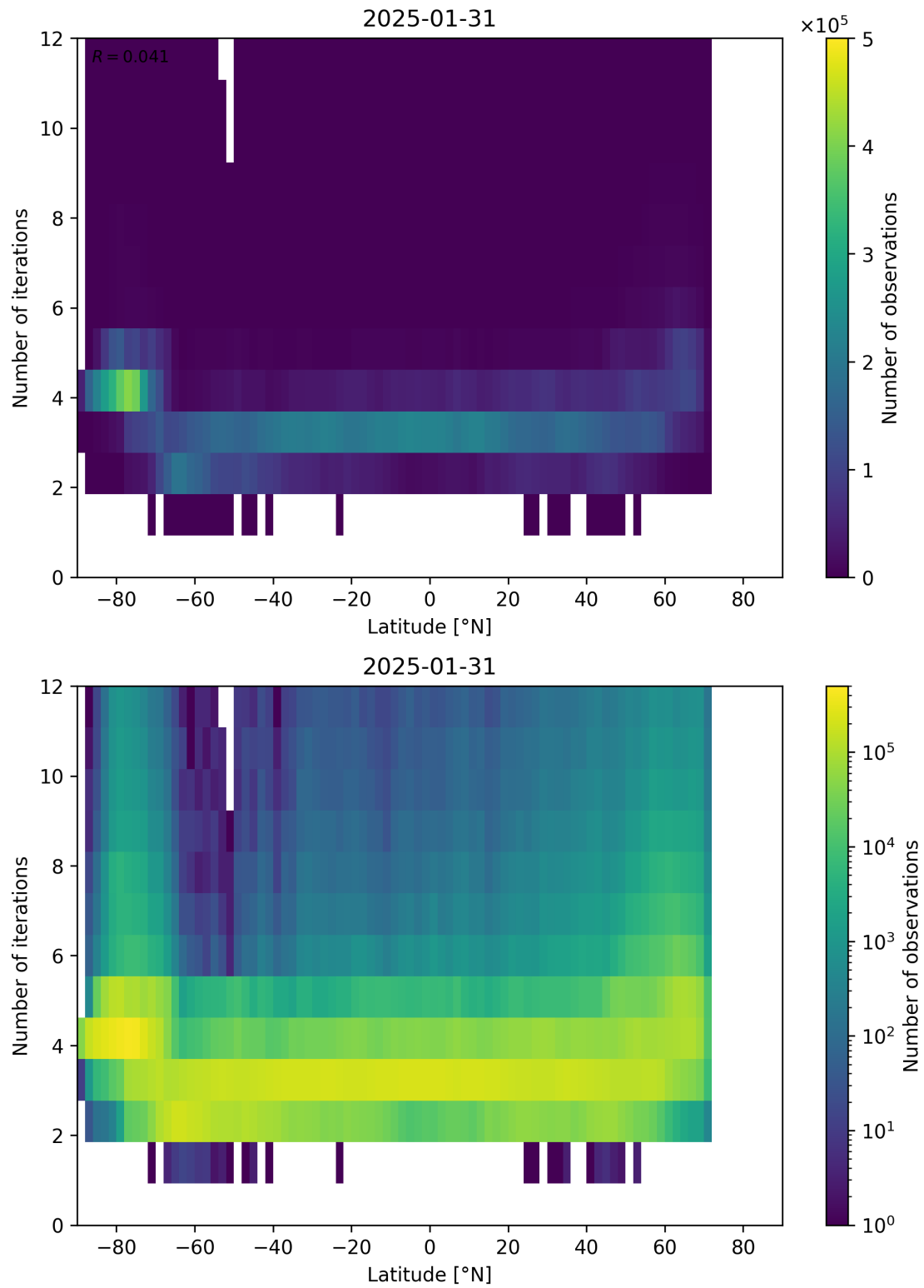
Figure 93: Scatter density plot of “Latitude” against “Number of iterations” for 2025-01-30 to 2025-02-01.
