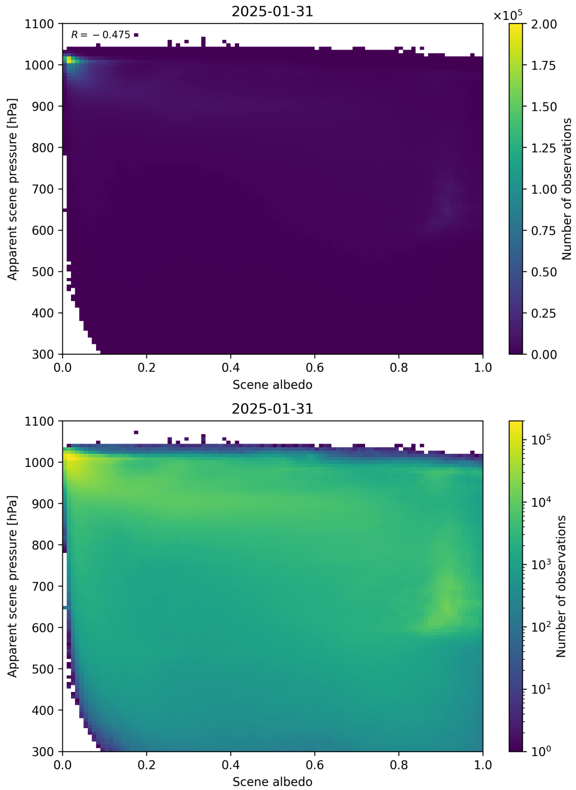
Figure 102: Scatter density plot of “Scene albedo” against “Apparent scene pressure” for 2025-01-30 to 2025-02-01.
