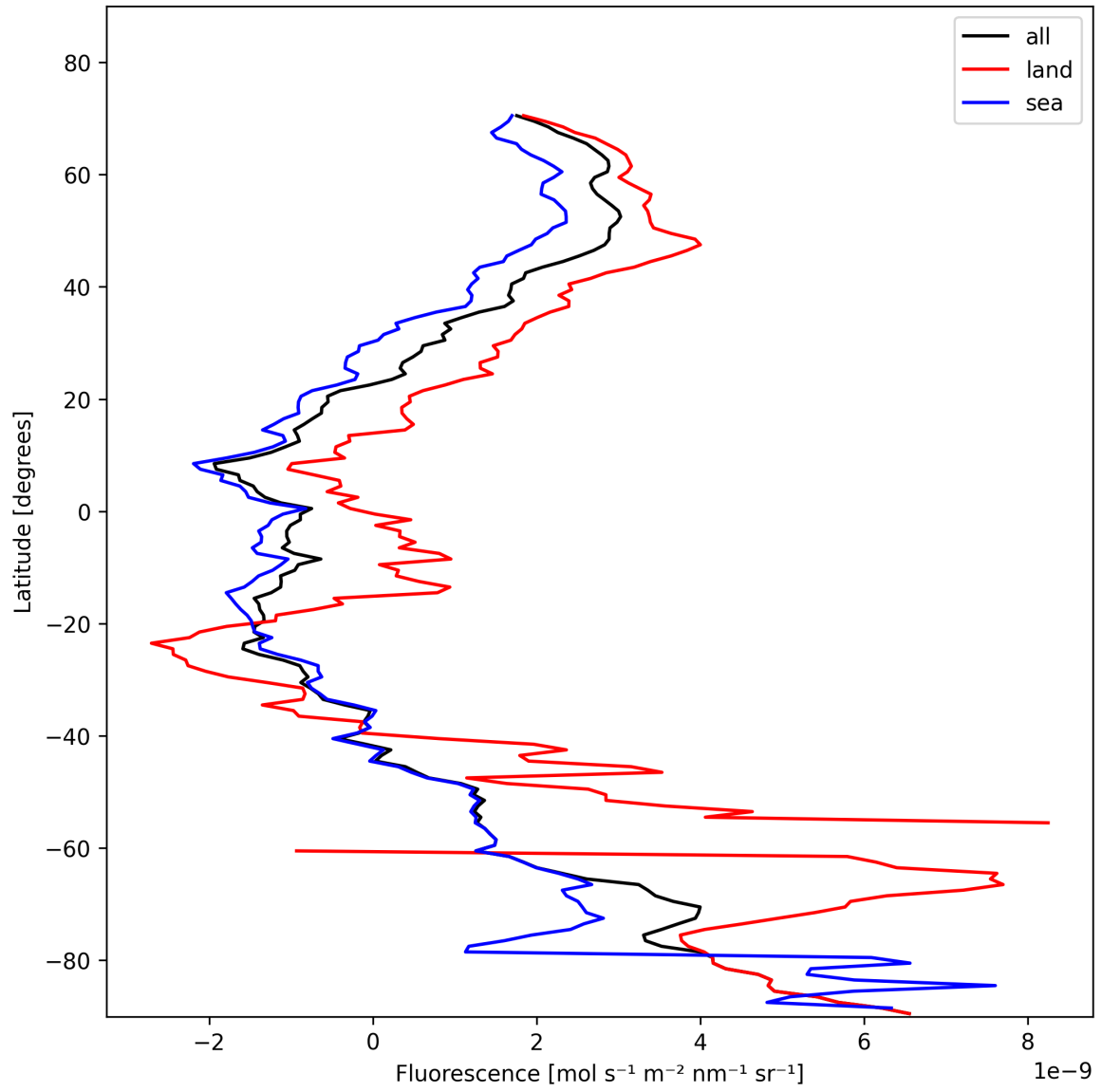
Figure 23: Zonal average of “Fluorescence” for 2025-01-30 to 2025-02-01.
