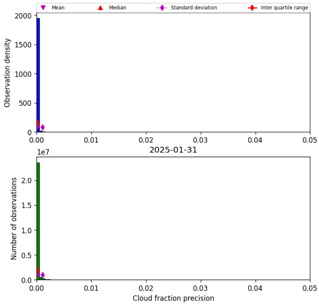
Figure 33: Histogram of “Cloud fraction precision” for 2025-01-30 to 2025-02-01
