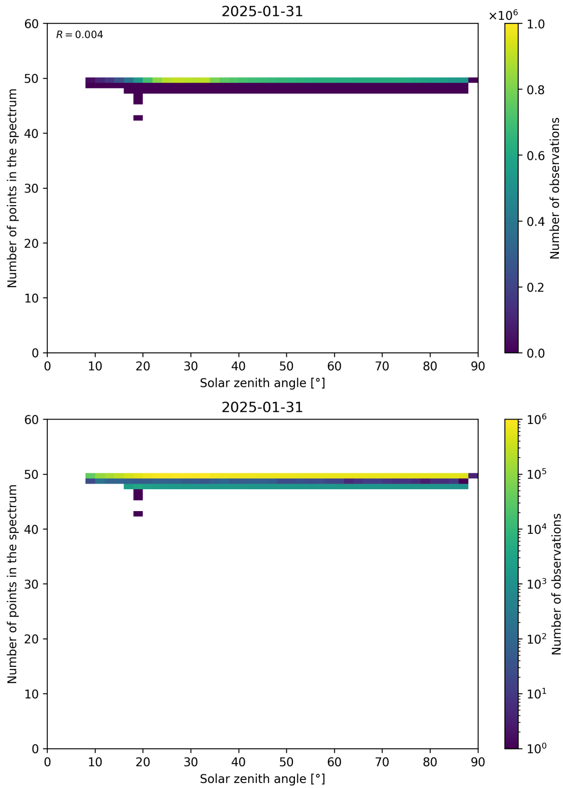
Figure 115: Scatter density plot of “Solar zenith angle” against “Number of points in the spectrum” for 2025-01-30 to 2025-02-01.
