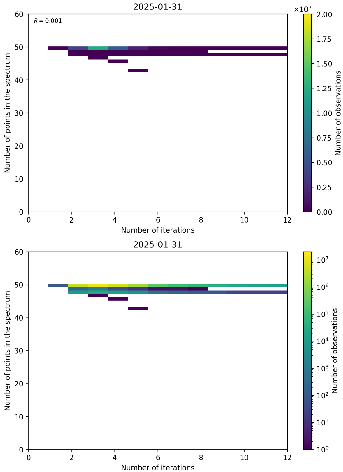
Figure 99: Scatter density plot of “Number of iterations” against “Number of points in the spectrum” for 2025-01-30 to 2025-02-01.
