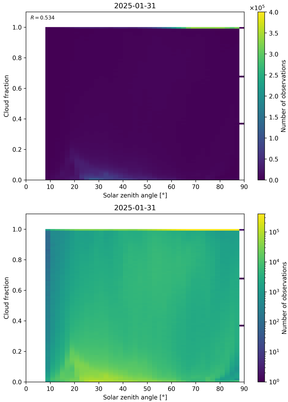
Figure 110: Scatter density plot of “Solar zenith angle” against “Cloud fraction” for 2025-01-30 to 2025-02-01.
