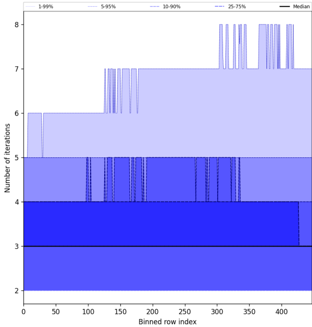
Figure 56: Along track statistics of “Number of iterations” for 2025-01-30 to 2025-02-01
