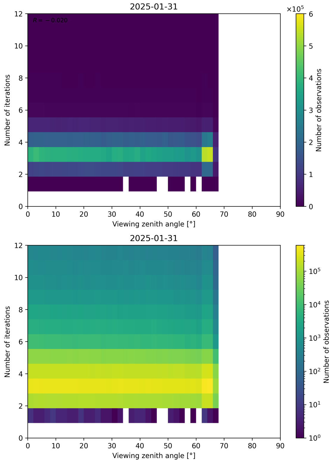
Figure 124: Scatter density plot of “Viewing zenith angle” against “Number of iterations” for 2025-01-30 to 2025-02-01.
