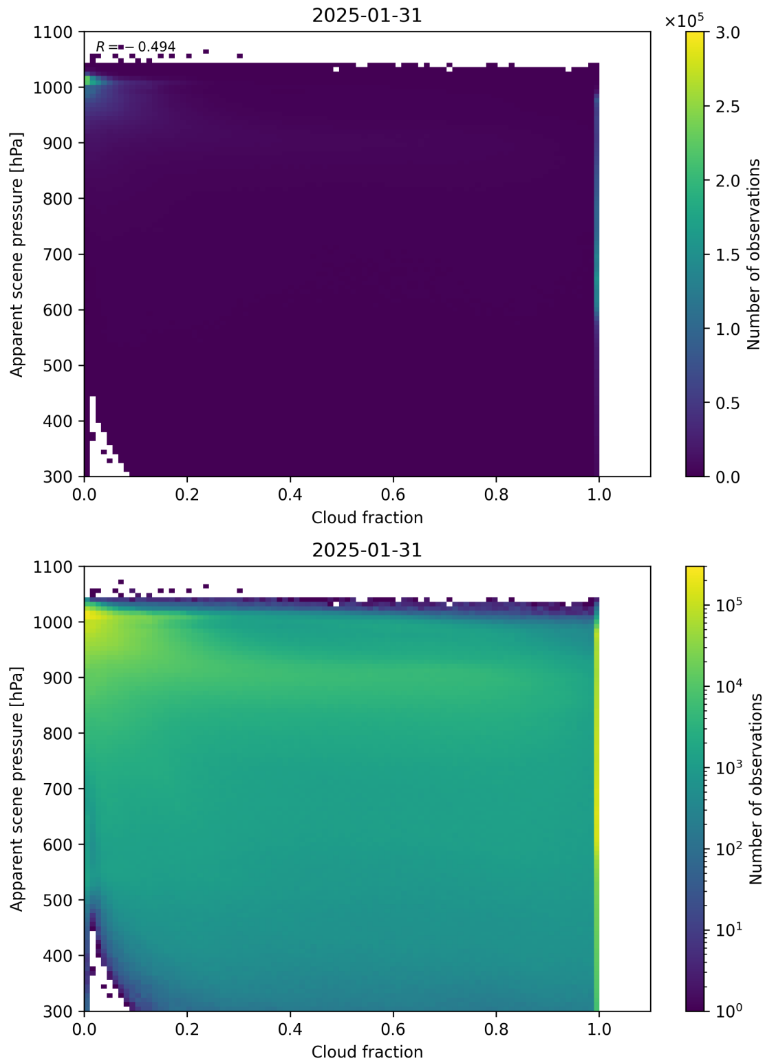
Figure 70: Scatter density plot of “Cloud fraction” against “Apparent scene pressure” for 2025-01-30 to 2025-02-01.
