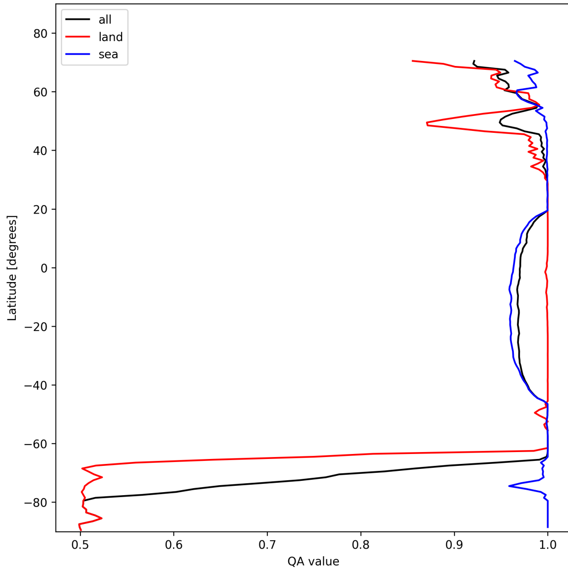
Figure 12: Zonal average of “QA value” for 2025-01-30 to 2025-02-01.
