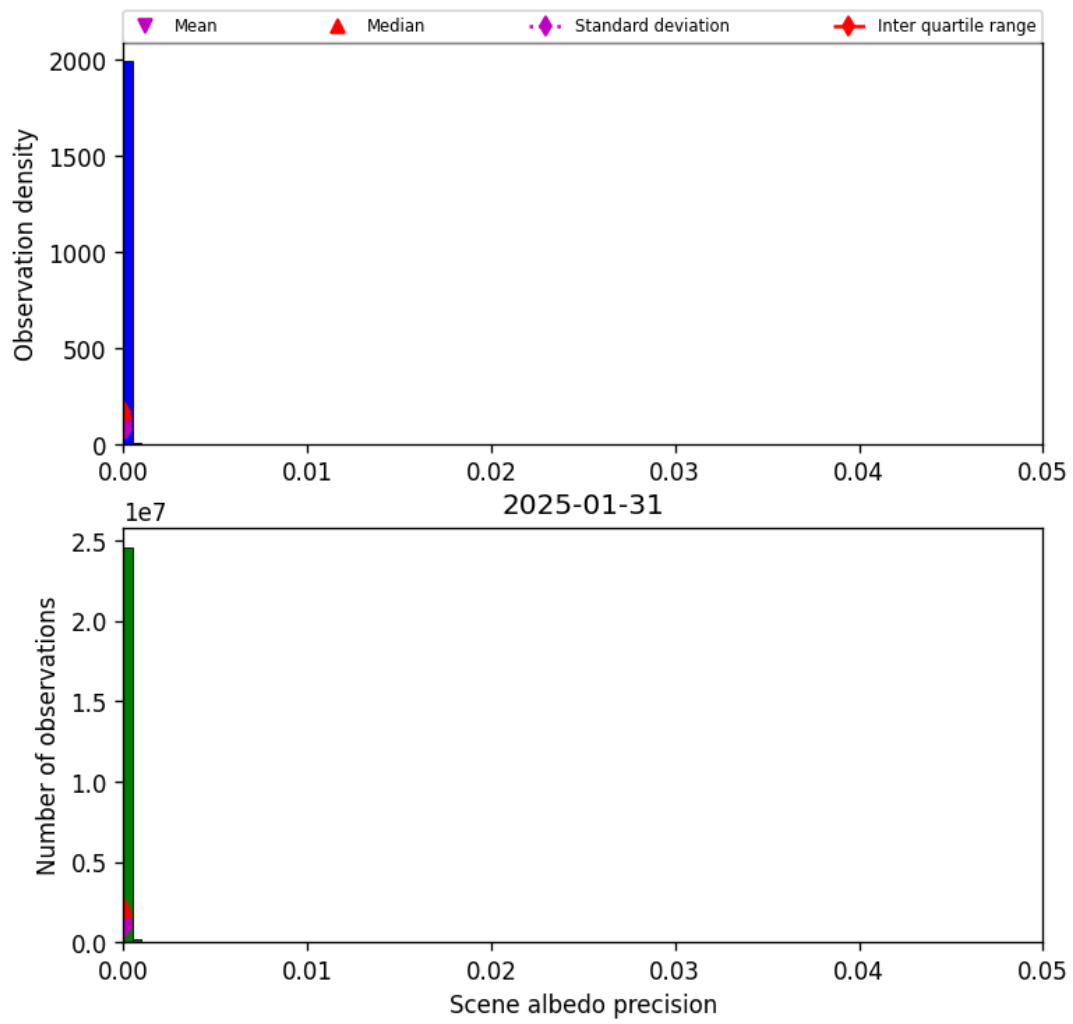
Figure 35: Histogram of “Scene albedo precision” for 2025-01-30 to 2025-02-01
