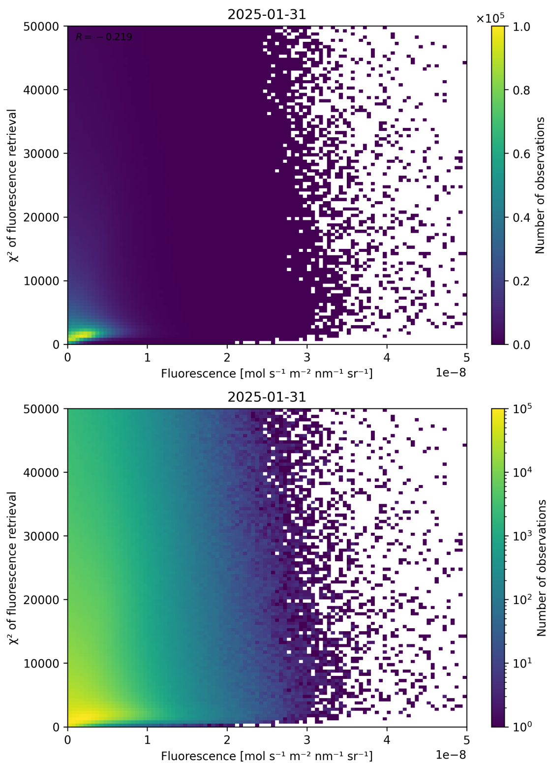
Figure 85: Scatter density plot of “Fluorescence” against “ \chi^2 of fluorescence retrieval” for 2025-01-30 to 2025-02-01.
