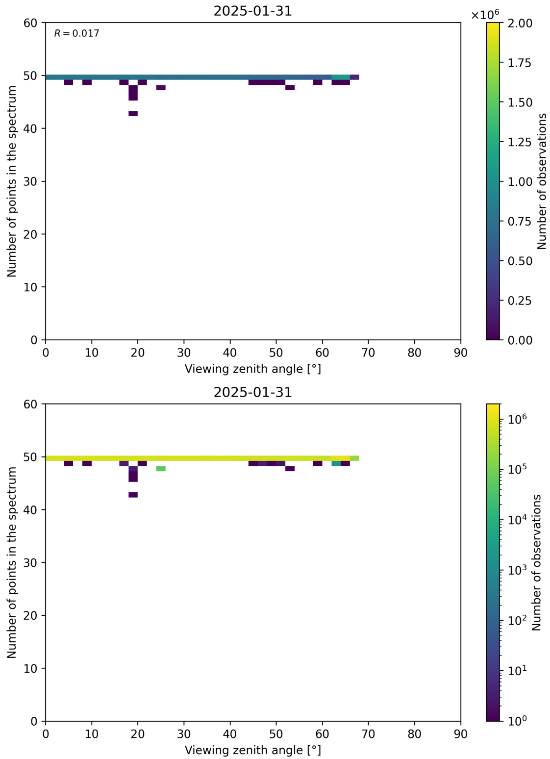
Figure 125: Scatter density plot of “Viewing zenith angle” against “Number of points in the spectrum” for 2025-01-30 to 2025-02-01.
