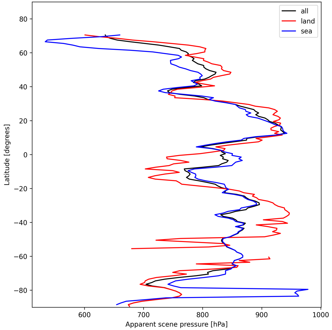
Figure 19: Zonal average of “Apparent scene pressure” for 2025-01-30 to 2025-02-01.
