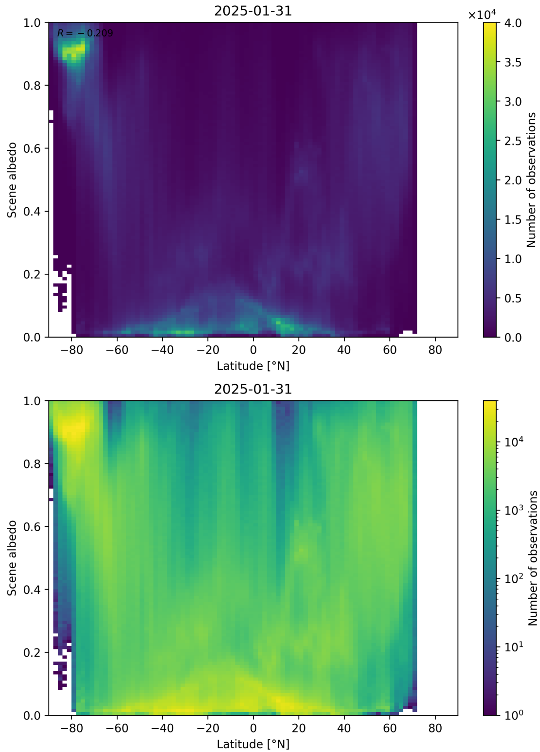
Figure 95: Scatter density plot of “Latitude” against “Scene albedo” for 2025-01-30 to 2025-02-01.
