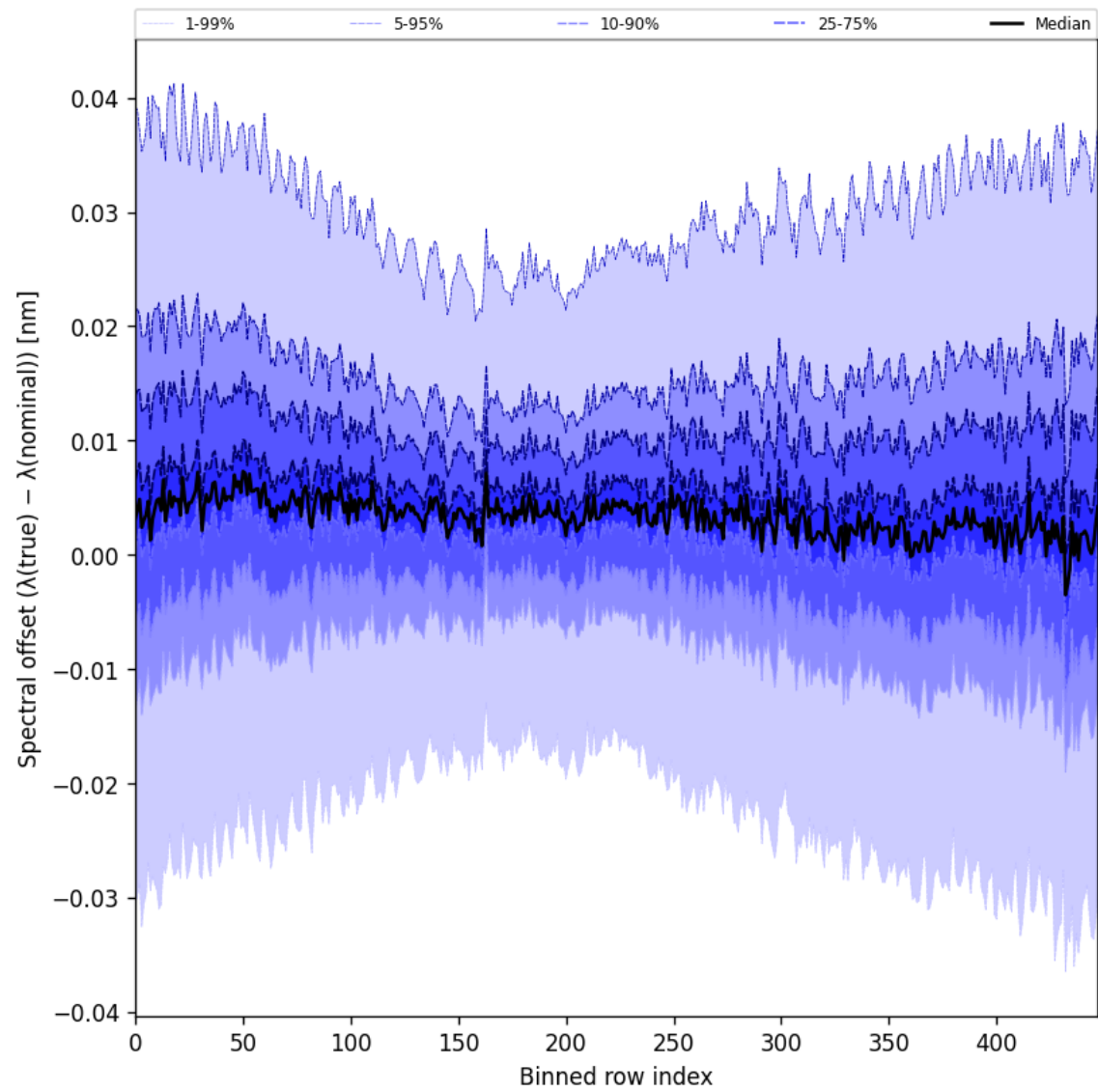
Figure 62: Along track statistics of “Spectral offset ( \lambda_{\text{true}} - \lambda_{\text{nominal}} )” for 2025-01-30 to 2025-02-01
