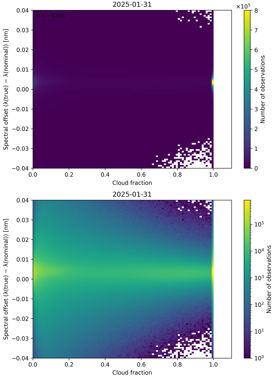
Figure 76: Scatter density plot of “Cloud fraction” against “Spectral offset ( \lambda_{\text{true}} - \lambda_{\text{nominal}} )” for 2025-01-30 to 2025-02-01.
