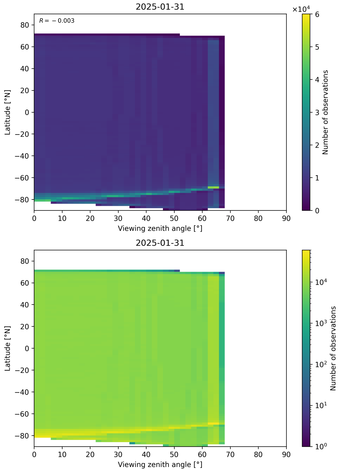
Figure 123: Scatter density plot of “Viewing zenith angle” against “Latitude” for 2025-01-30 to 2025-02-01.
