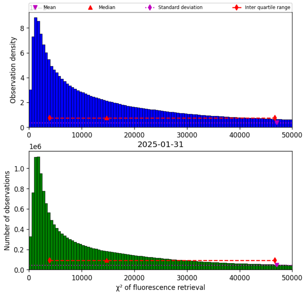
Figure 42: Histogram of “ \chi^2 of fluorescence retrieval” for 2025-01-30 to 2025-02-01
