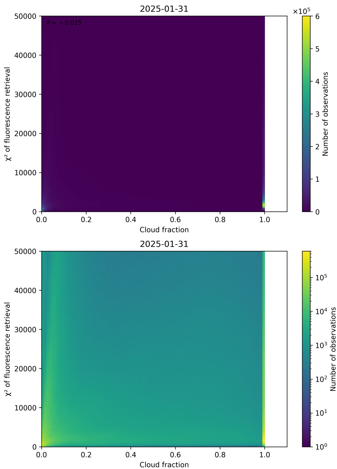
Figure 71: Scatter density plot of “Cloud fraction” against “ \chi^2 of fluorescence retrieval” for 2025-01-30 to 2025-02-01.
