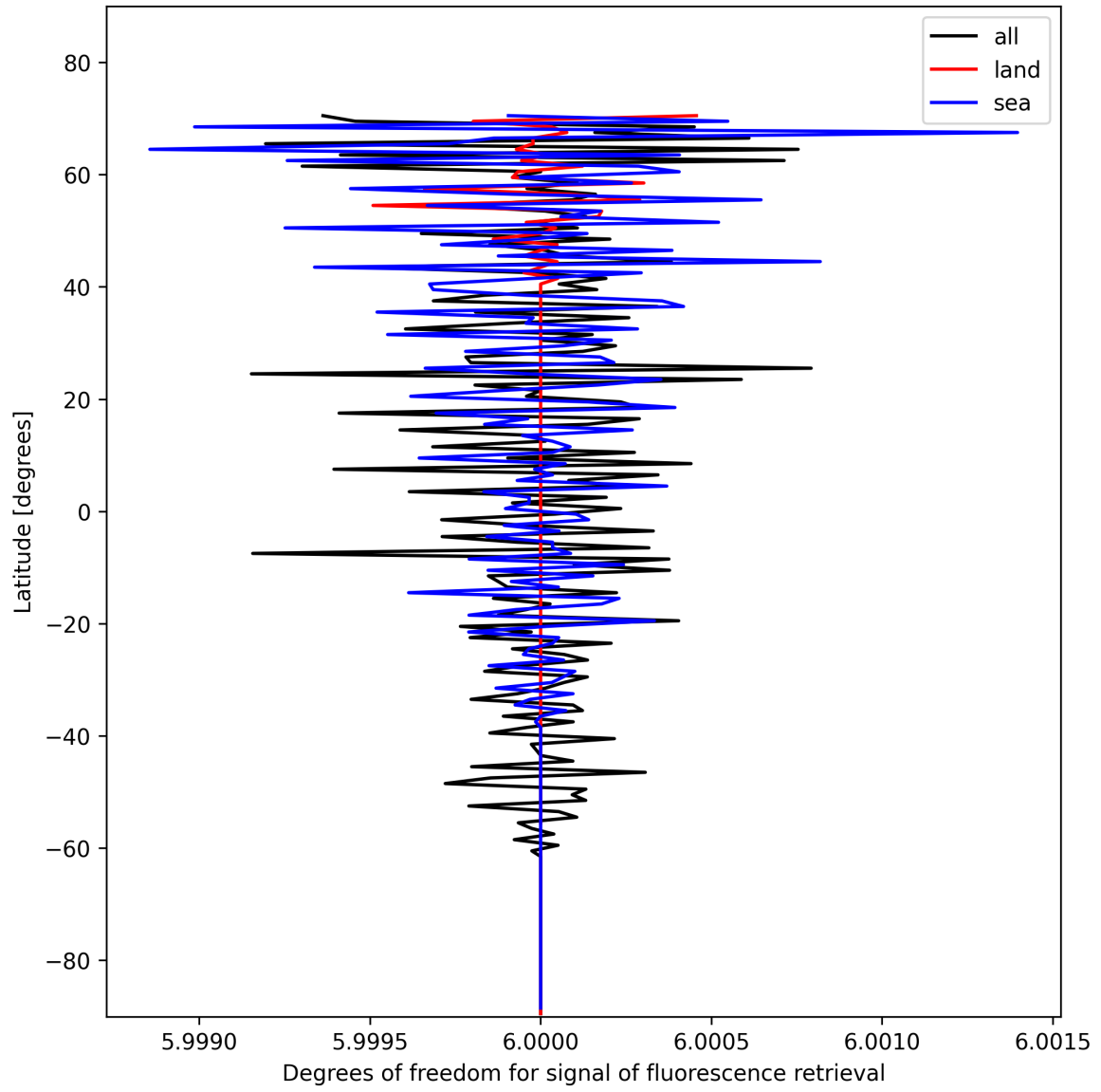
Figure 26: Zonal average of “Degrees of freedom for signal of fluorescence retrieval” for 2025-01-30 to 2025-02-01.
