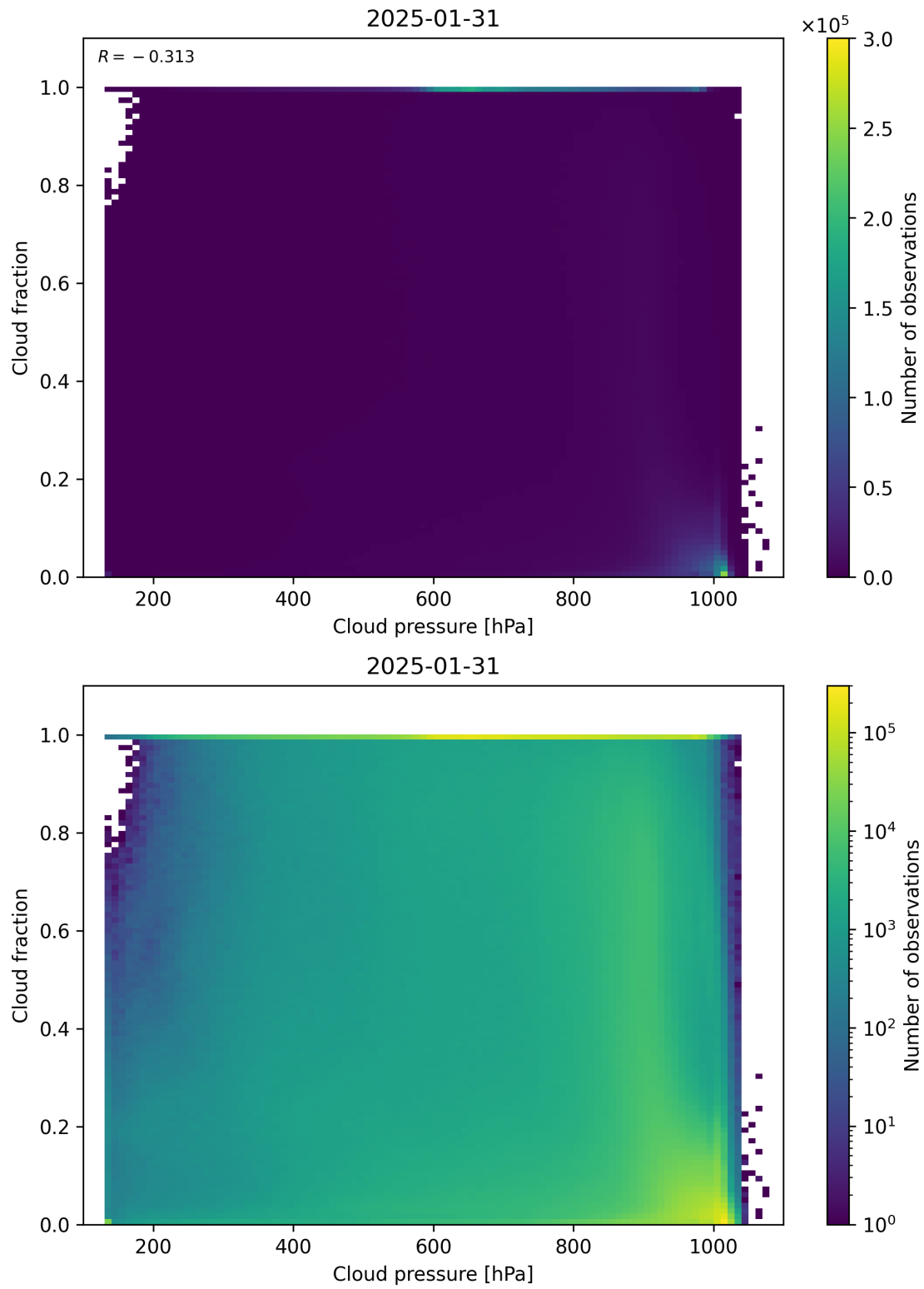
Figure 79: Scatter density plot of “Cloud pressure” against “Cloud fraction” for 2025-01-30 to 2025-02-01.
