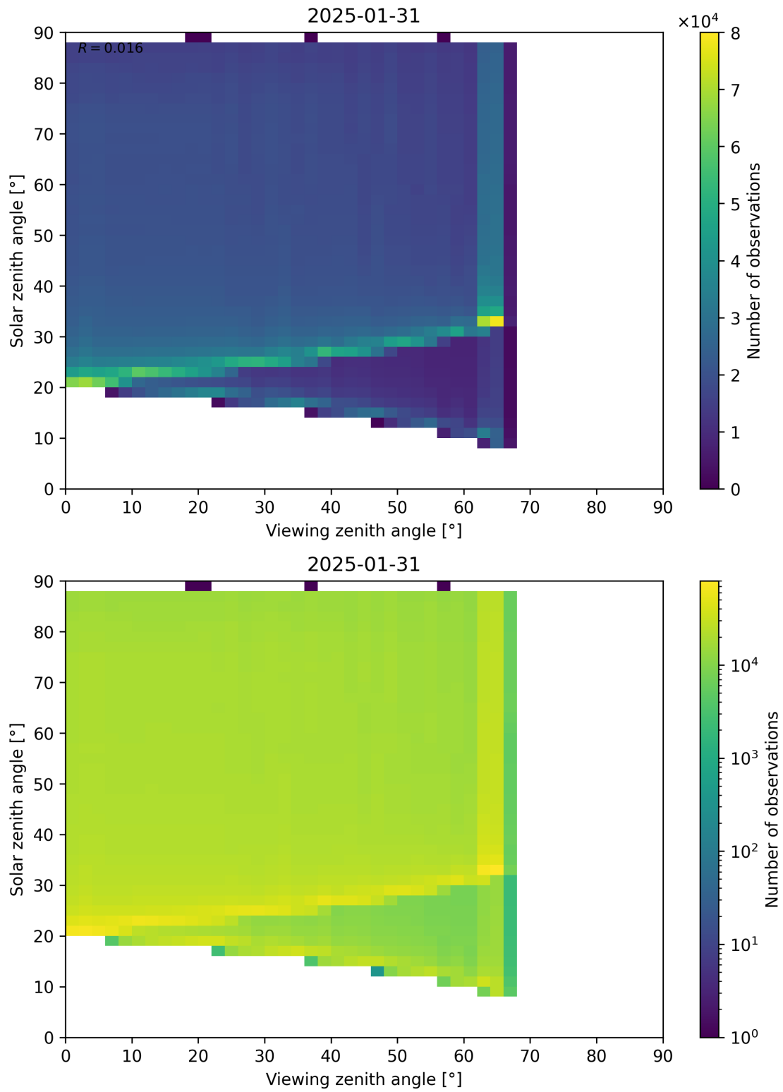
Figure 127: Scatter density plot of “Viewing zenith angle” against “Solar zenith angle” for 2025-01-30 to 2025-02-01.
