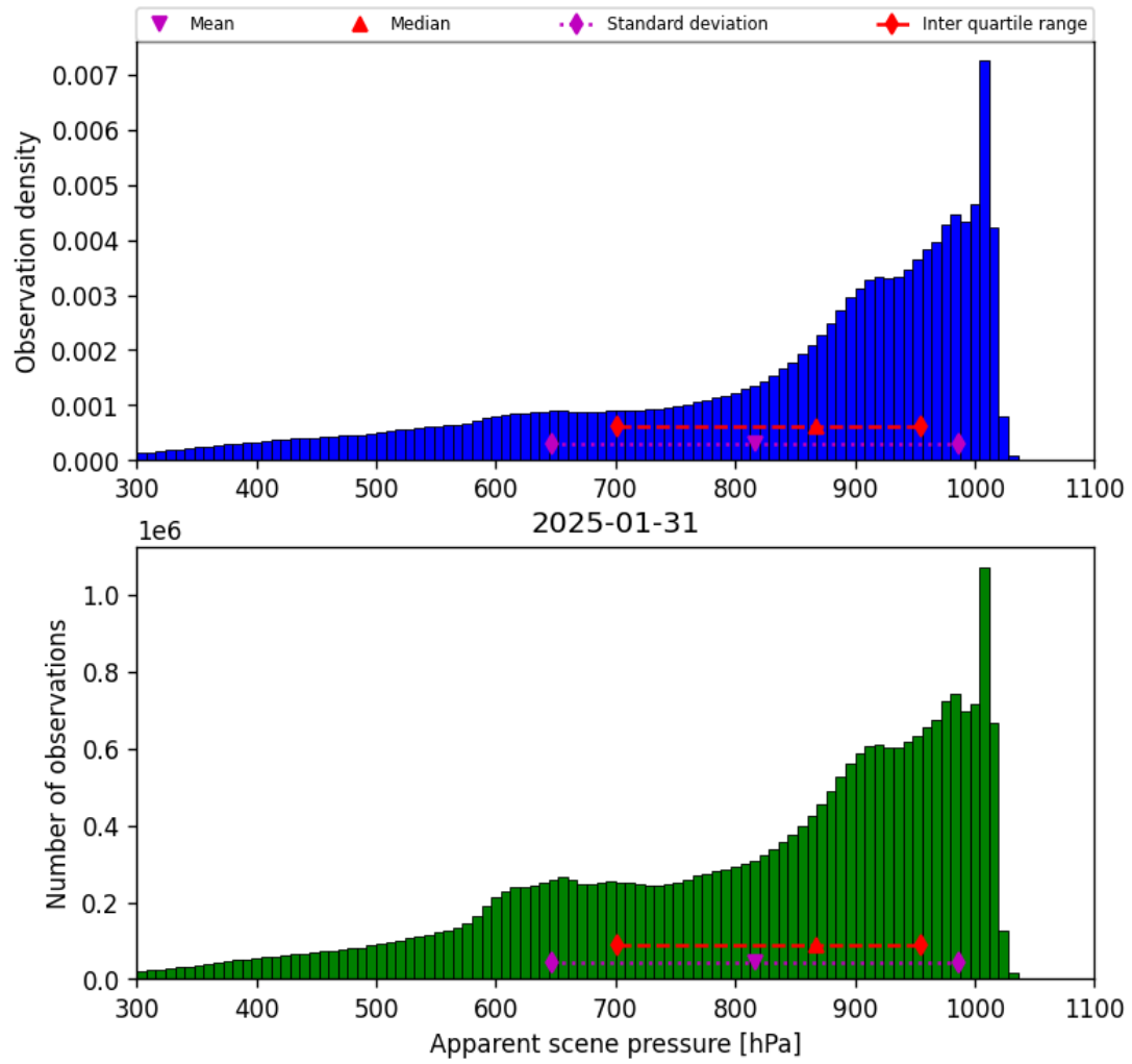
Figure 36: Histogram of “Apparent scene pressure” for 2025-01-30 to 2025-02-01
