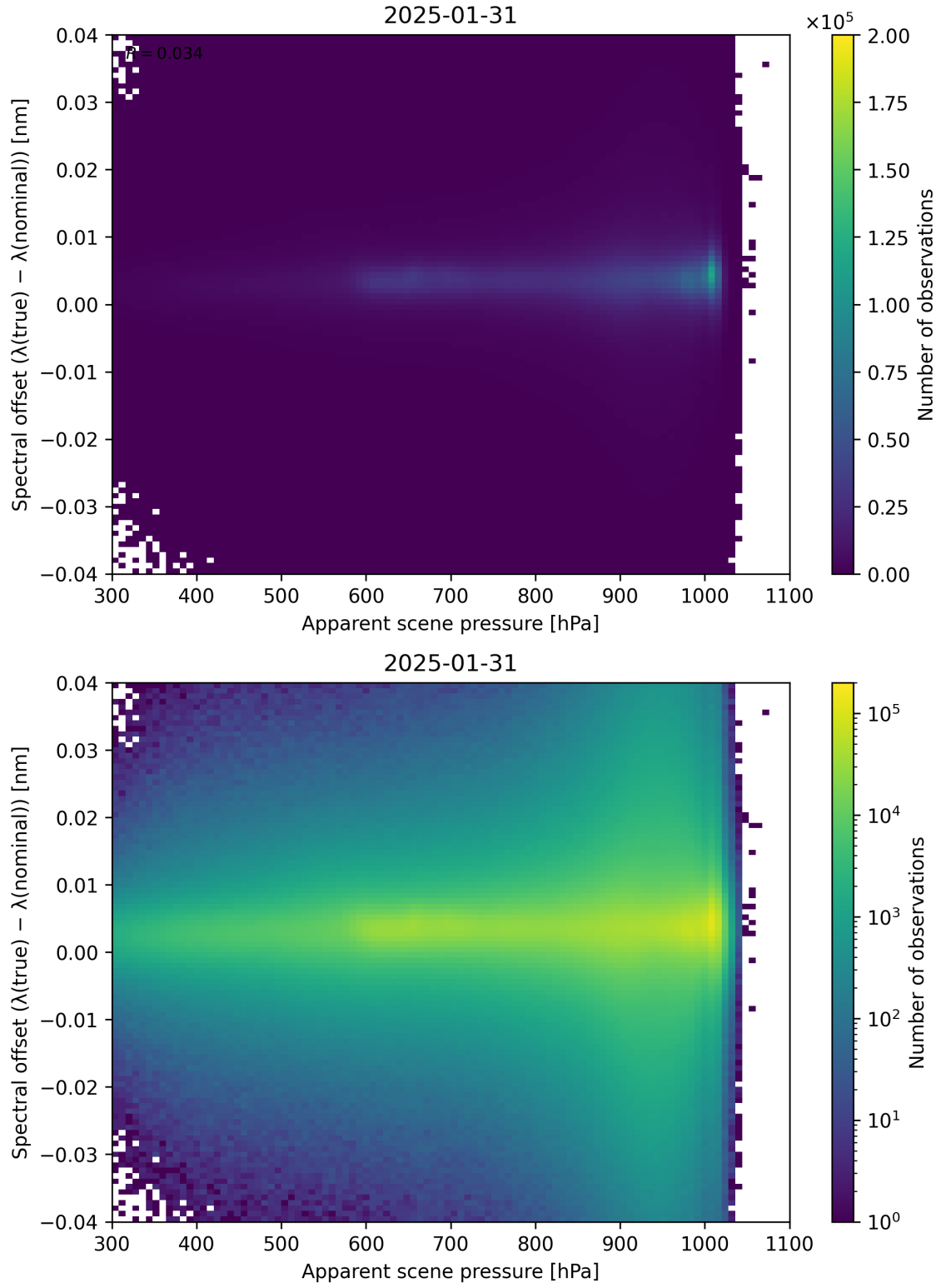
Figure 67: Scatter density plot of “Apparent scene pressure” against “Spectral offset ( \lambda_{\text{true}} - \lambda_{\text{nominal}} )” for 2025-01-30 to 2025-02-01.
