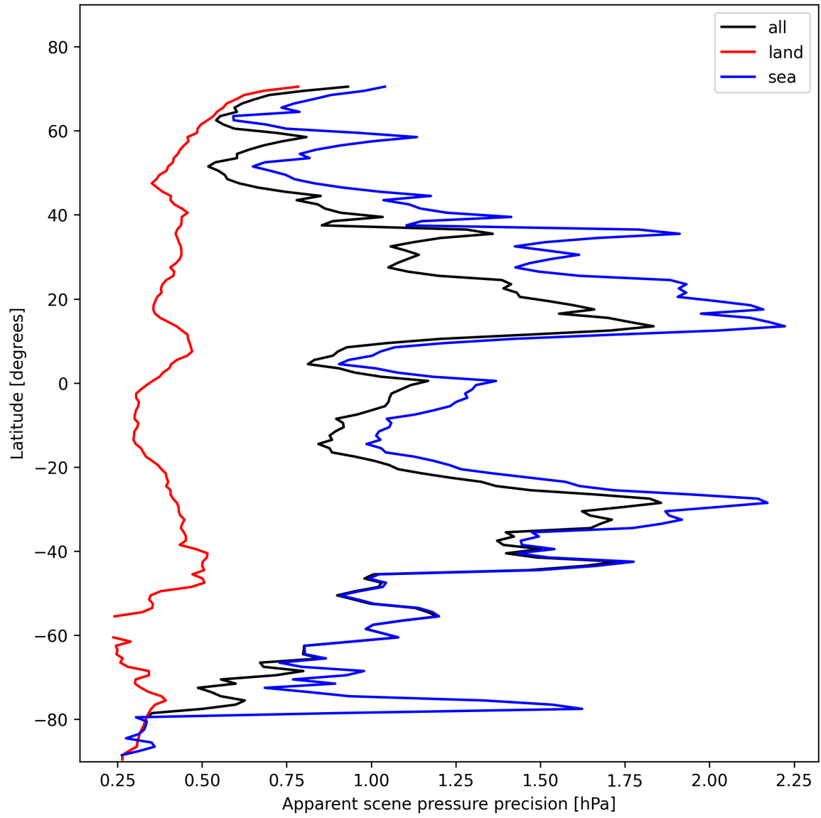
Figure 20: Zonal average of “Apparent scene pressure precision” for 2025-01-30 to 2025-02-01.
