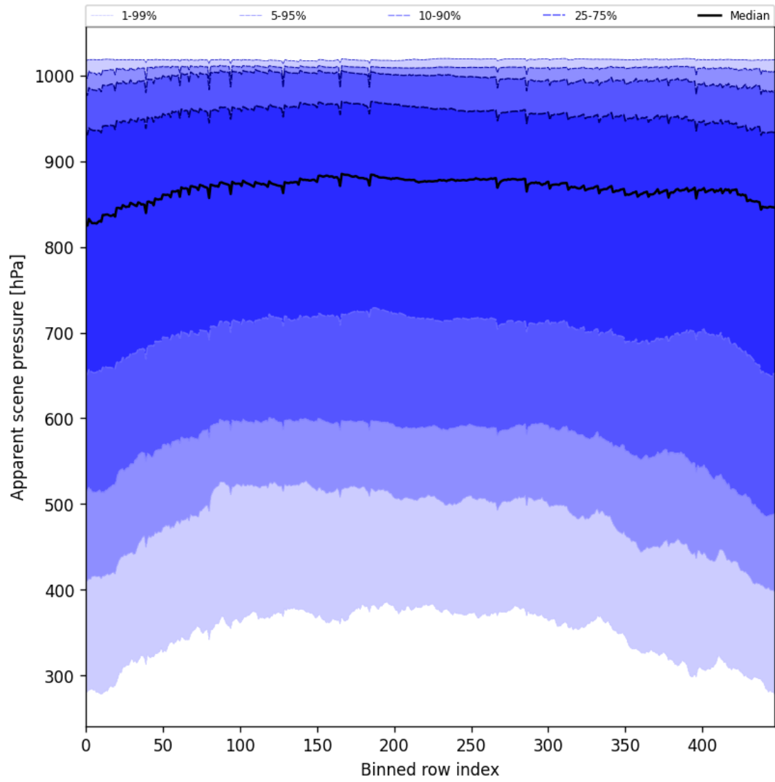
Figure 53: Along track statistics of “Apparent scene pressure” for 2025-01-30 to 2025-02-01
