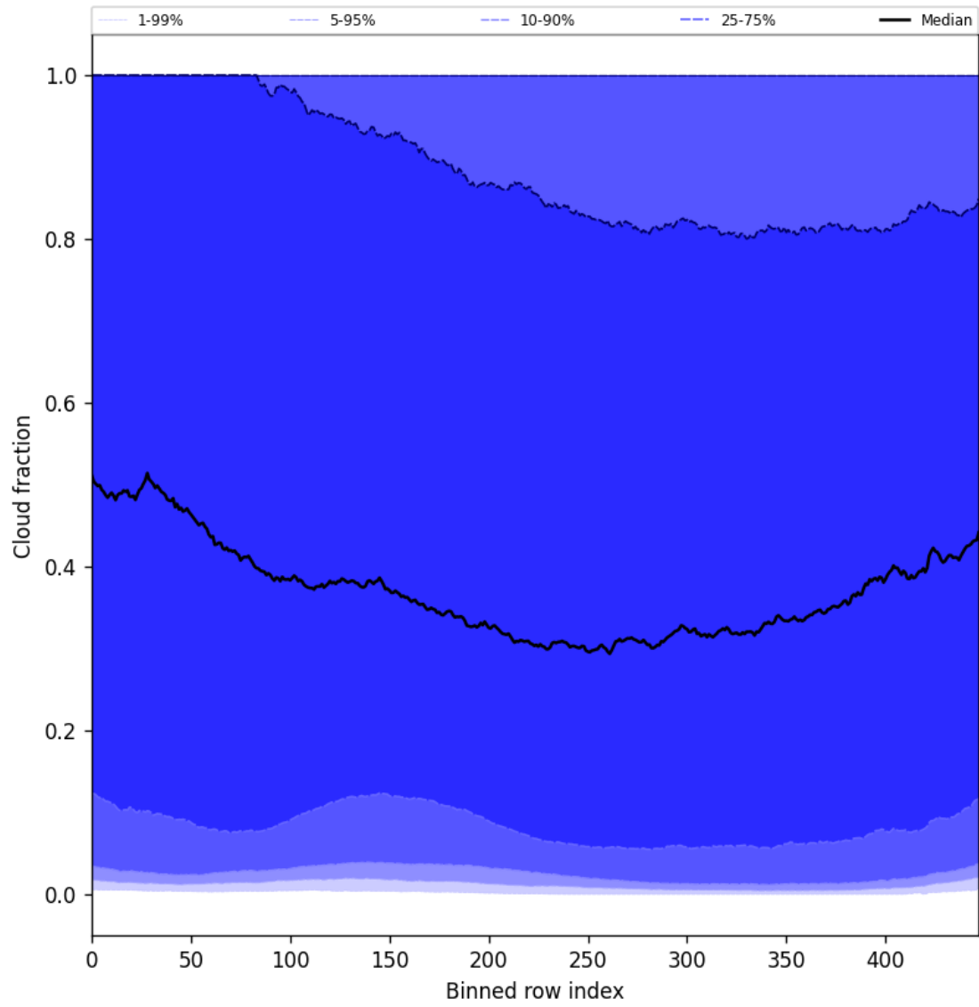
Figure 49: Along track statistics of “Cloud fraction” for 2025-01-30 to 2025-02-01
