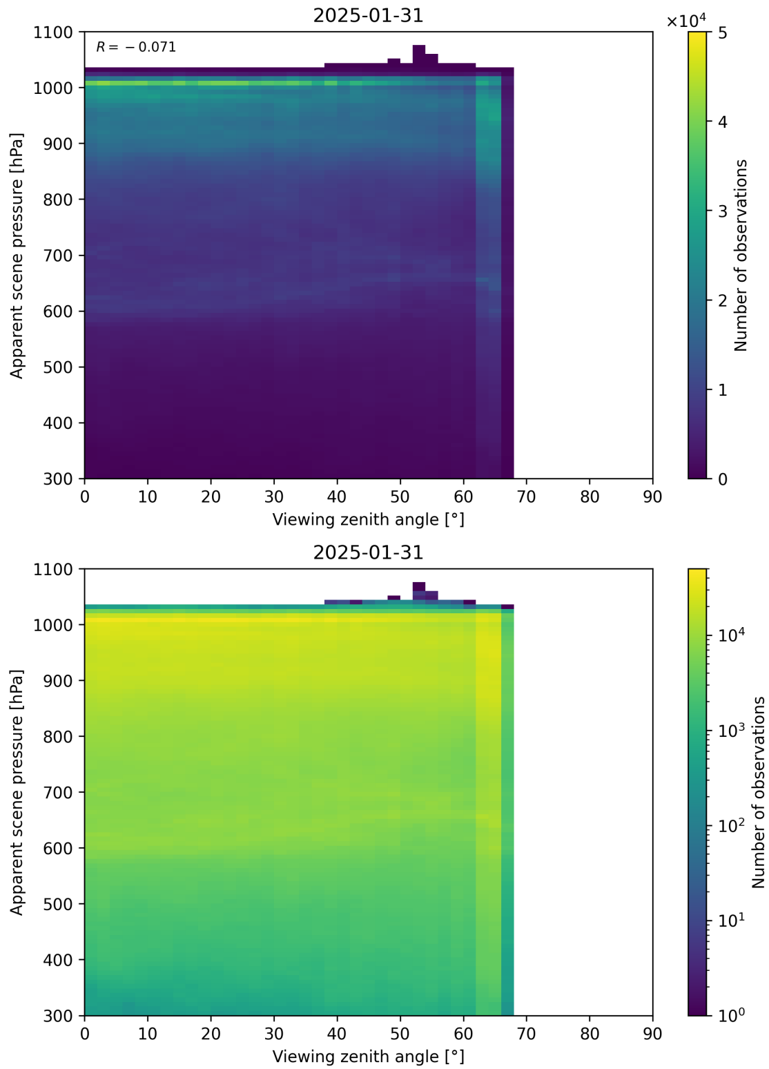
Figure 118: Scatter density plot of “Viewing zenith angle” against “Apparent scene pressure” for 2025-01-30 to 2025-02-01.
