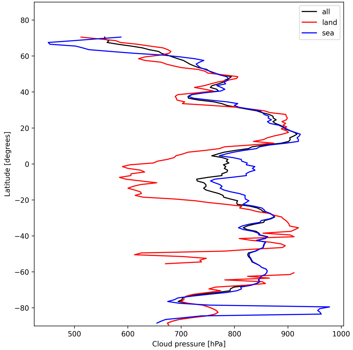
Figure 13: Zonal average of “Cloud pressure” for 2025-01-30 to 2025-02-01.
