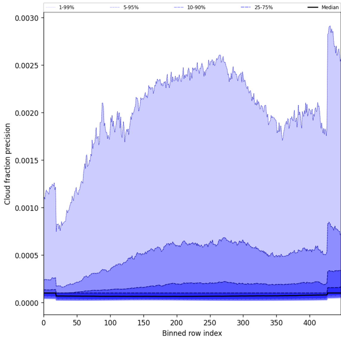
Figure 50: Along track statistics of “Cloud fraction precision” for 2025-01-30 to 2025-02-01
