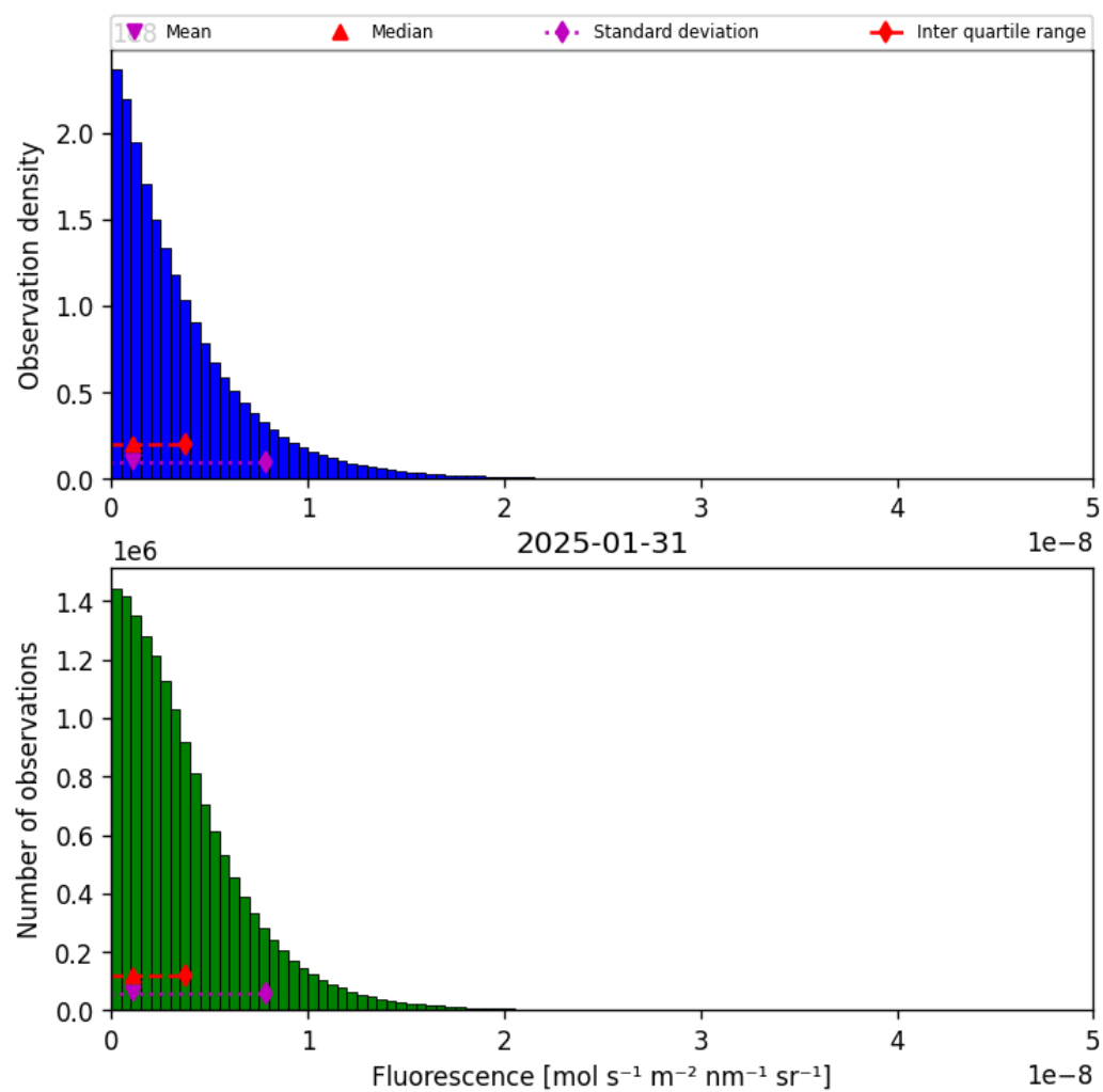
Figure 40: Histogram of “Fluorescence” for 2025-01-30 to 2025-02-01
