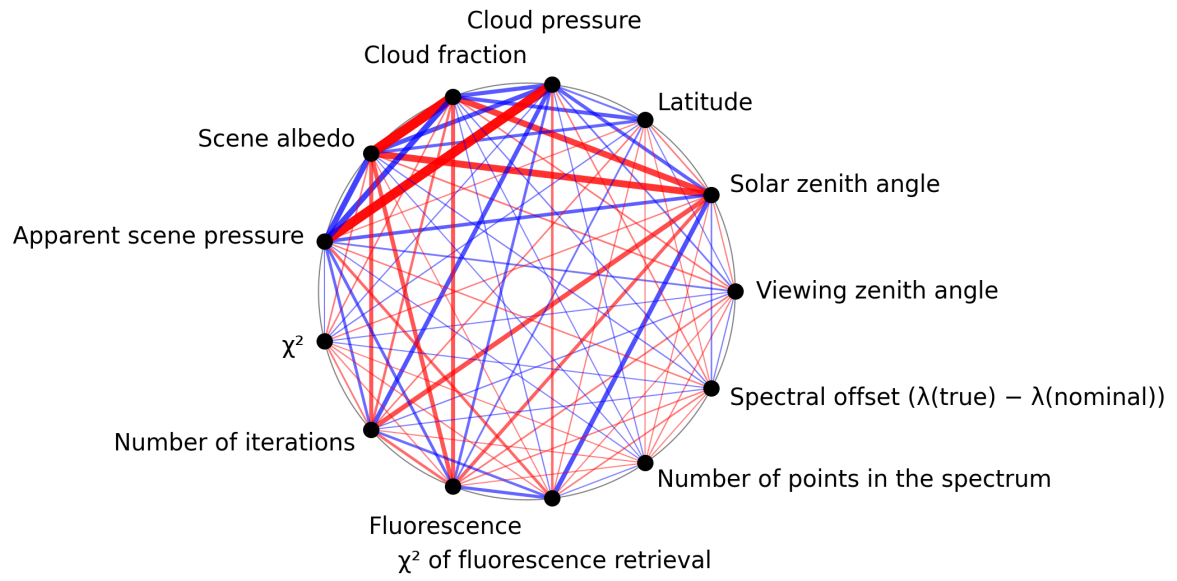
Figure 1: Map of correlation graph for 2025-01-30 to 2025-02-01.
