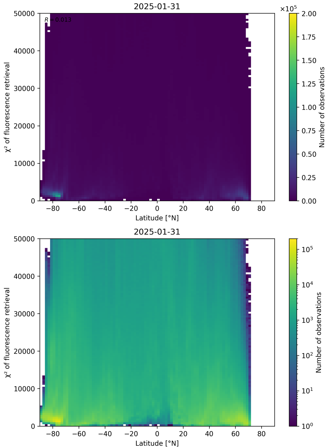
Figure 89: Scatter density plot of “Latitude” against “ \chi^2 of fluorescence retrieval” for 2025-01-30 to 2025-02-01.
