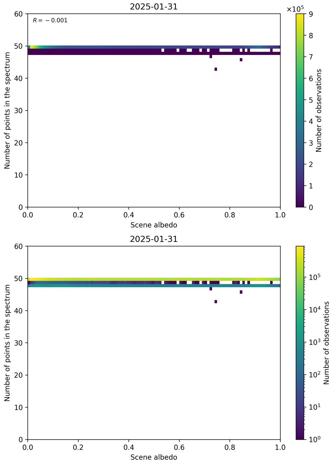
Figure 106: Scatter density plot of “Scene albedo” against “Number of points in the spectrum” for 2025-01-30 to 2025-02-01.
