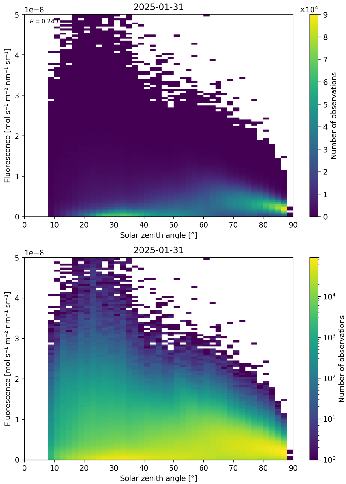
Figure 112: Scatter density plot of “Solar zenith angle” against “Fluorescence” for 2025-01-30 to 2025-02-01.
