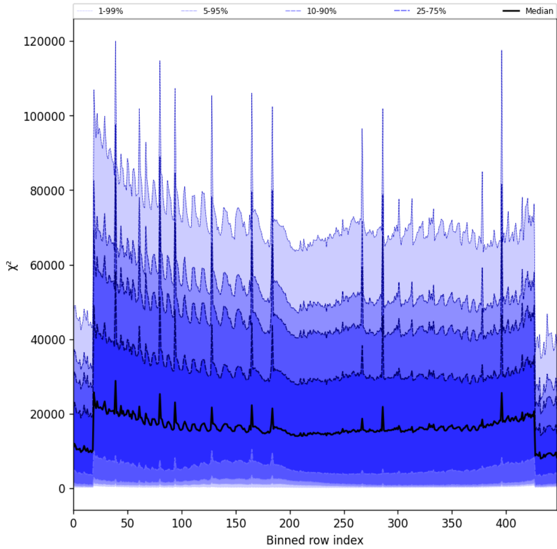
Figure 55: Along track statistics of “ \chi^2 ” for 2025-01-30 to 2025-02-01
