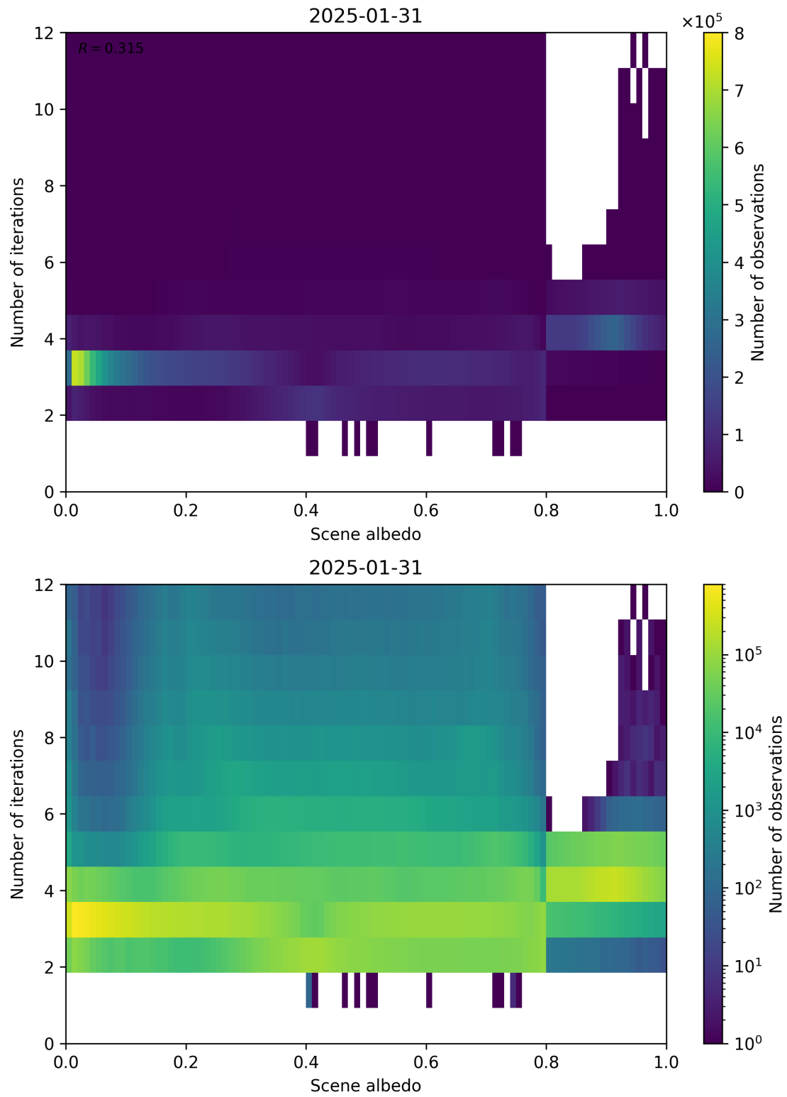
Figure 105: Scatter density plot of “Scene albedo” against “Number of iterations” for 2025-01-30 to 2025-02-01.
