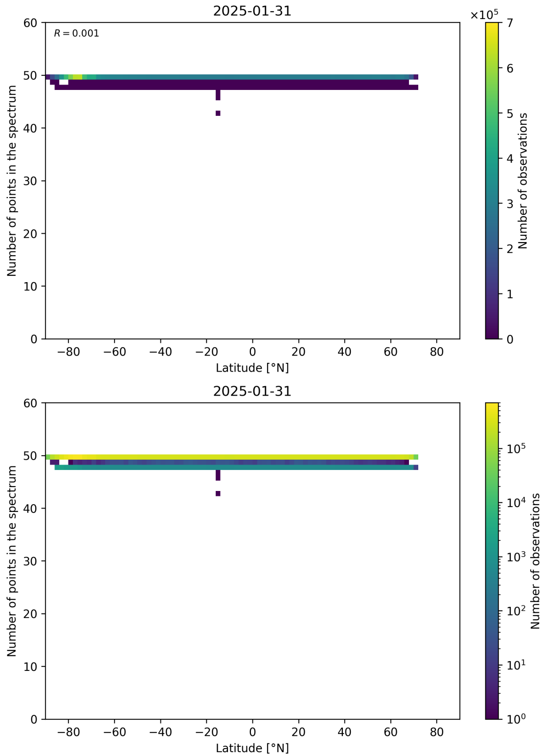
Figure 94: Scatter density plot of “Latitude” against “Number of points in the spectrum” for 2025-01-30 to 2025-02-01.
