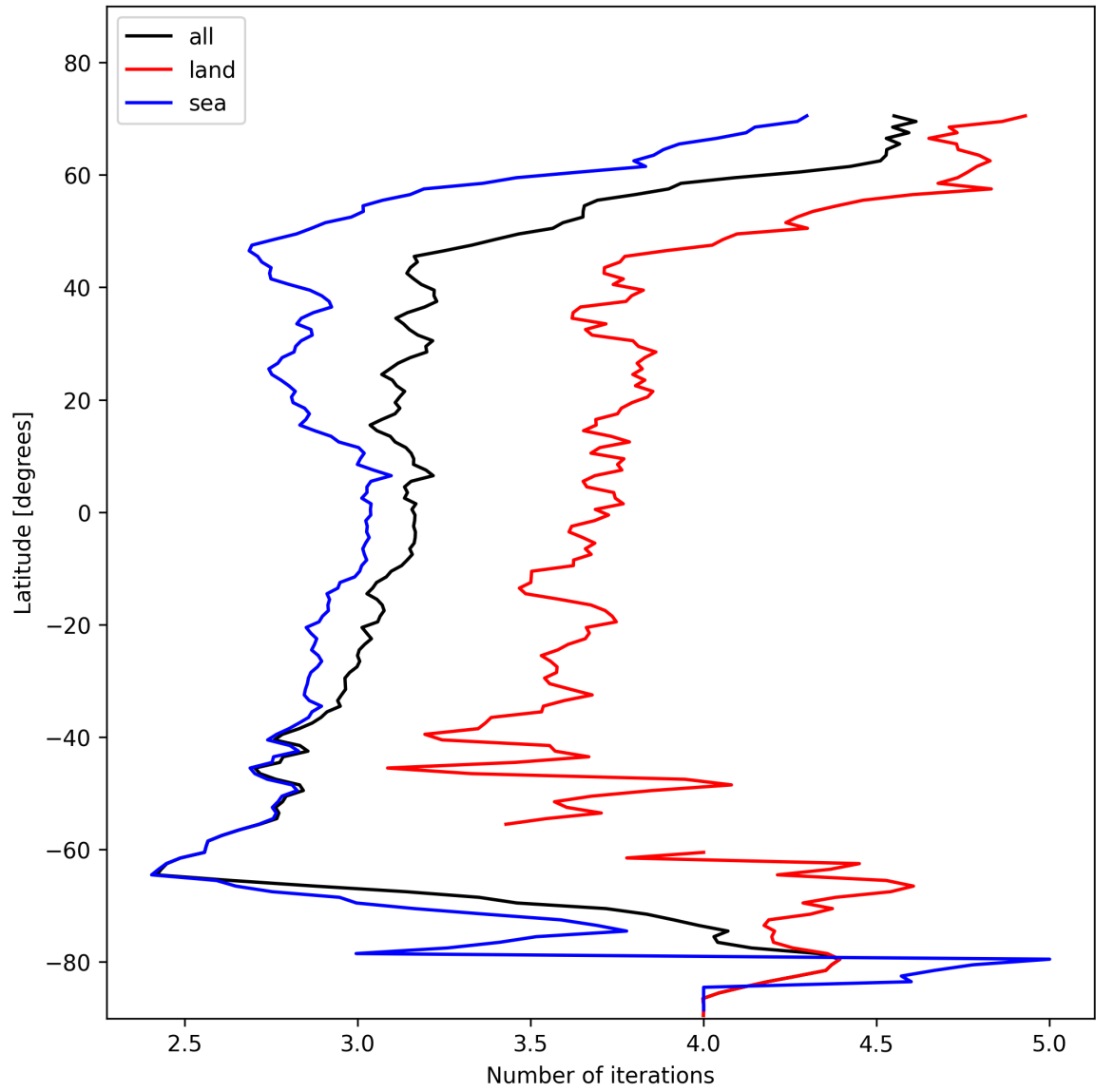
Figure 22: Zonal average of “Number of iterations” for 2025-01-30 to 2025-02-01.
