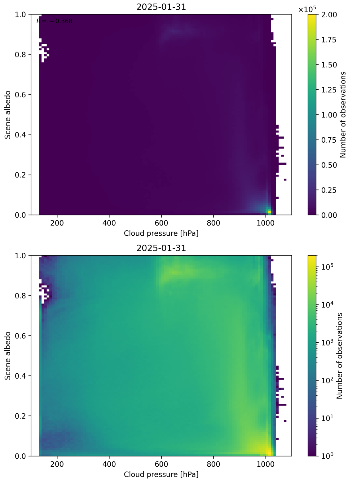
Figure 83: Scatter density plot of “Cloud pressure” against “Scene albedo” for 2025-01-30 to 2025-02-01.
