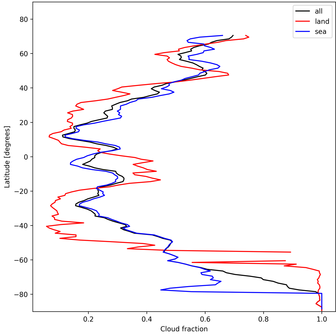
Figure 15: Zonal average of “Cloud fraction” for 2025-01-30 to 2025-02-01.
