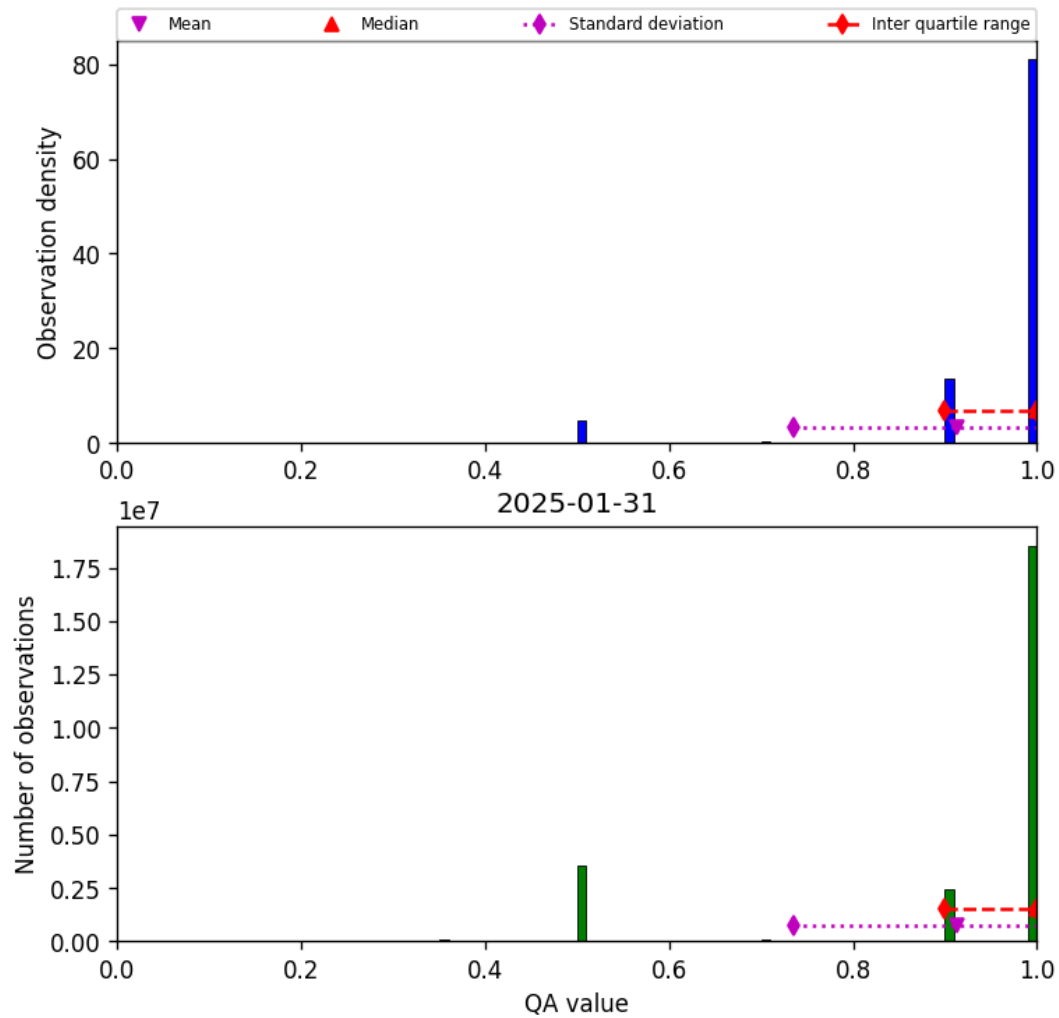
Figure 29: Histogram of “QA value” for 2025-01-30 to 2025-02-01
