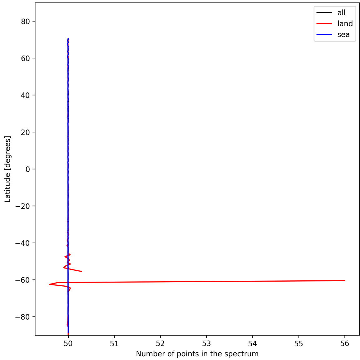
Figure 27: Zonal average of “Number of points in the spectrum” for 2025-01-30 to 2025-02-01.
