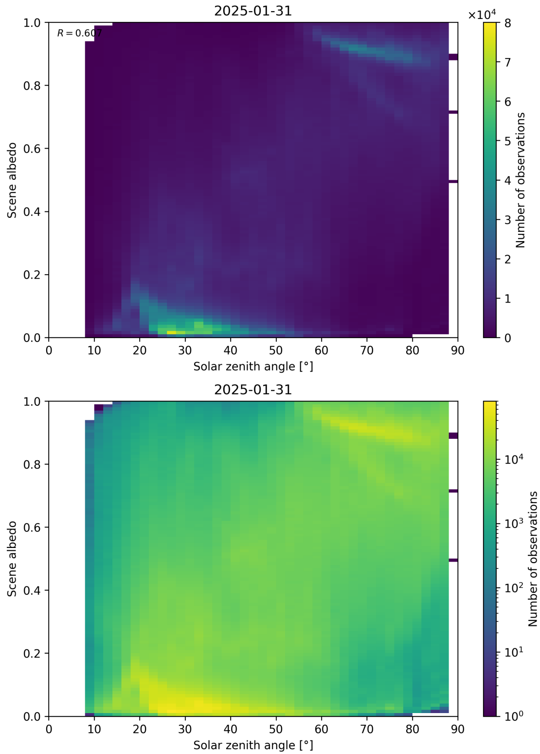
Figure 116: Scatter density plot of “Solar zenith angle” against “Scene albedo” for 2025-01-30 to 2025-02-01.
