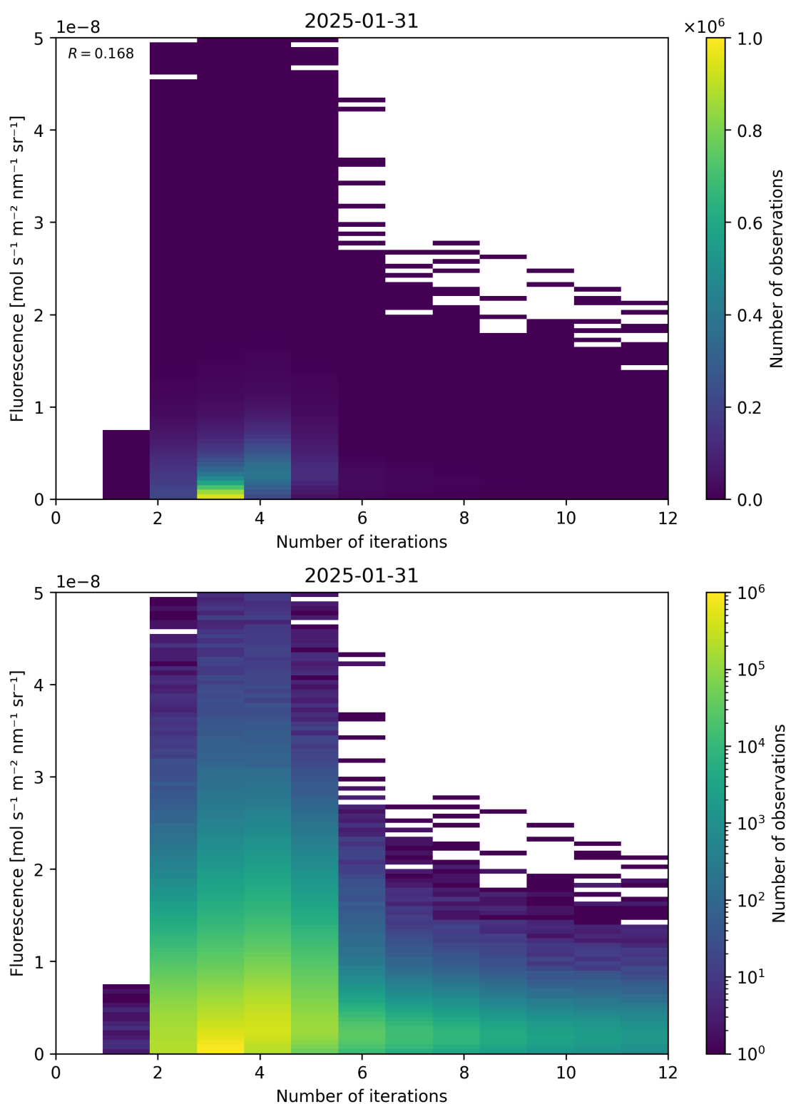
Figure 98: Scatter density plot of “Number of iterations” against “Fluorescence” for 2025-01-30 to 2025-02-01.
