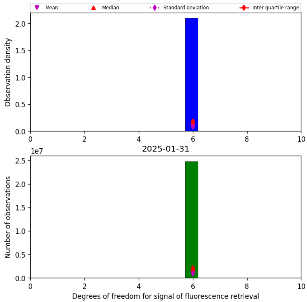
Figure 43: Histogram of “Degrees of freedom for signal of fluorescence retrieval” for 2025-01-30 to 2025-02-01
