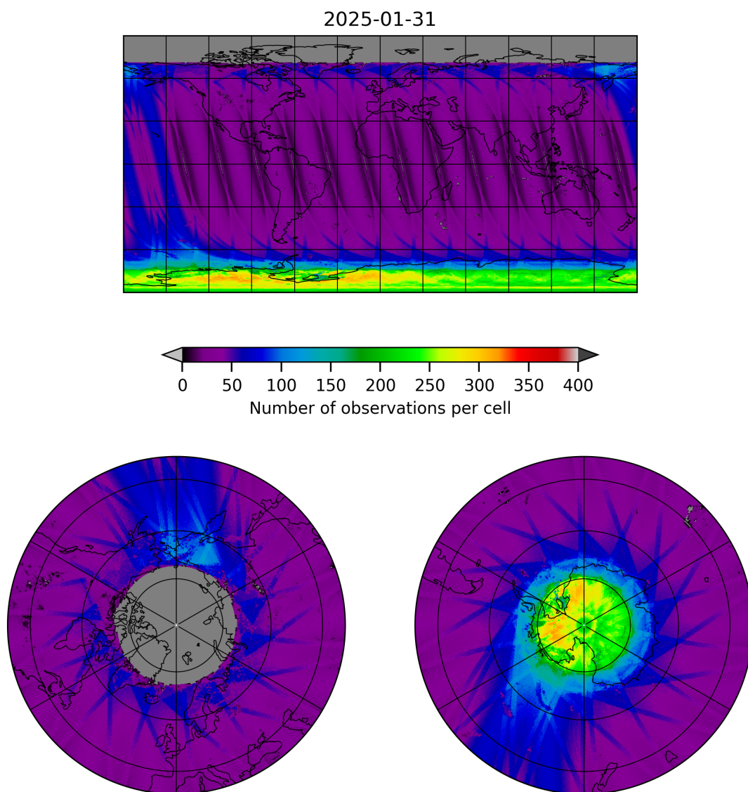
Figure 11: Map of the number of observations for 2025-01-30 to 2025-02-01
