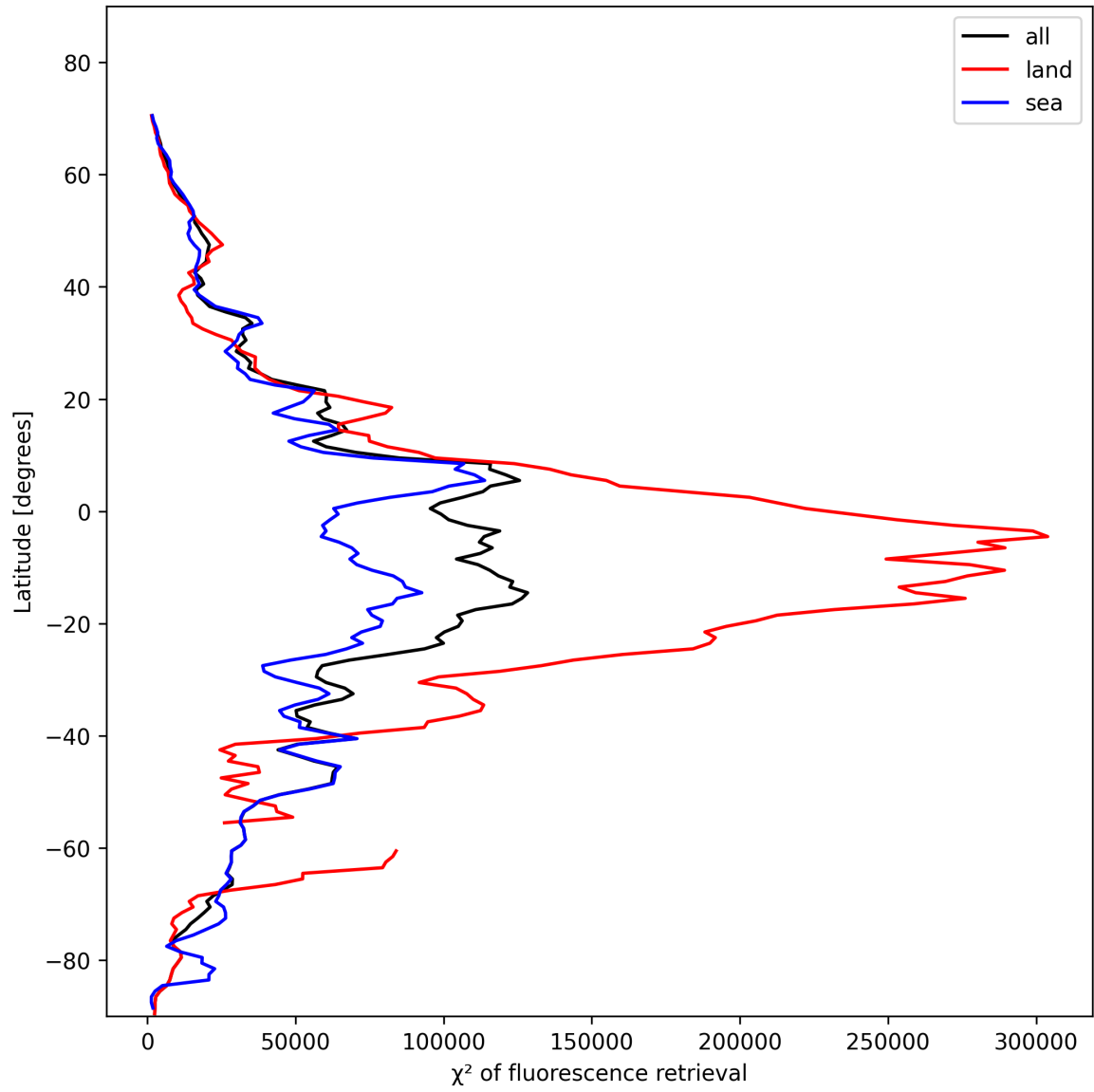
Figure 25: Zonal average of “ \chi^2 of fluorescence retrieval” for 2025-01-30 to 2025-02-01.
