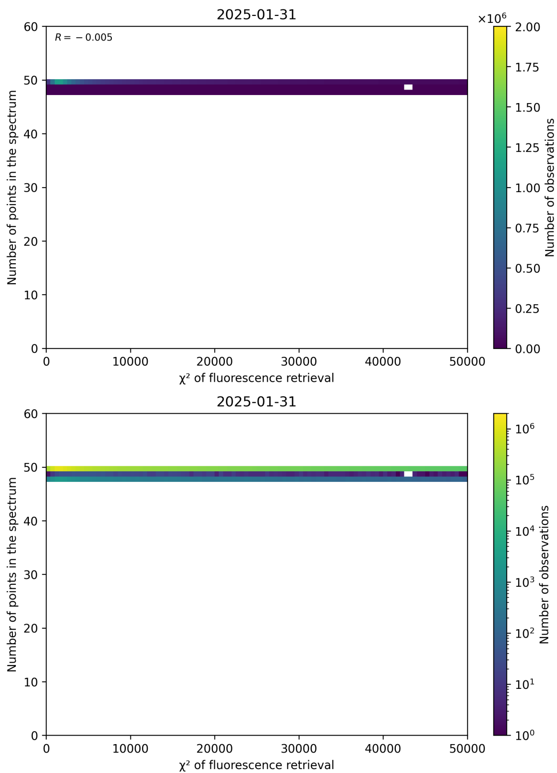
Figure 68: Scatter density plot of “ \chi^2 of fluorescence retrieval” against “Number of points in the spectrum” for 2025-01-30 to 2025-02-01.
