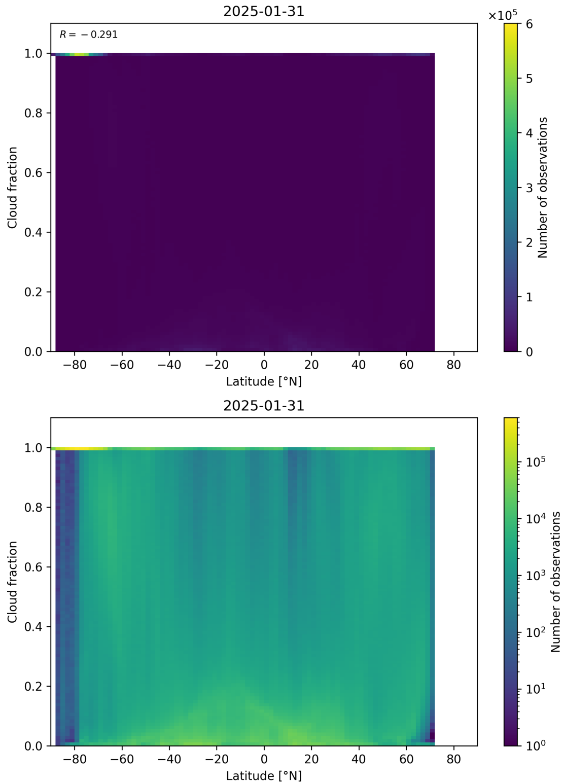
Figure 90: Scatter density plot of “Latitude” against “Cloud fraction” for 2025-01-30 to 2025-02-01.
