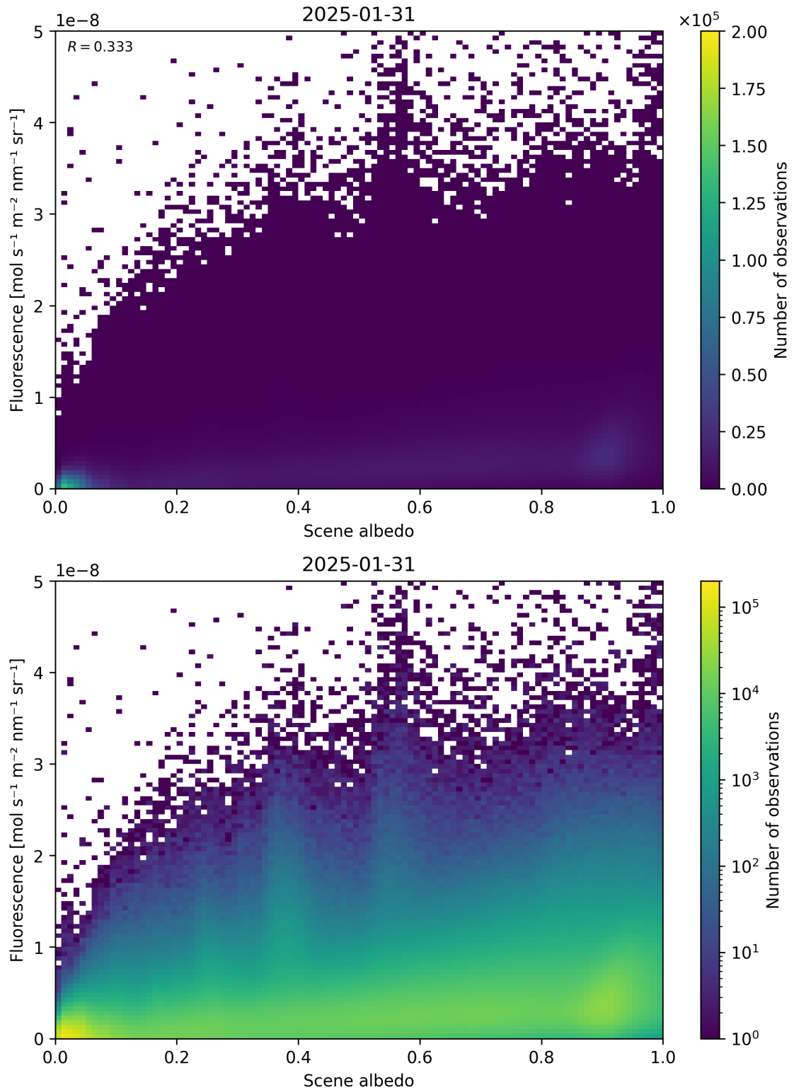
Figure 104: Scatter density plot of “Scene albedo” against “Fluorescence” for 2025-01-30 to 2025-02-01.
