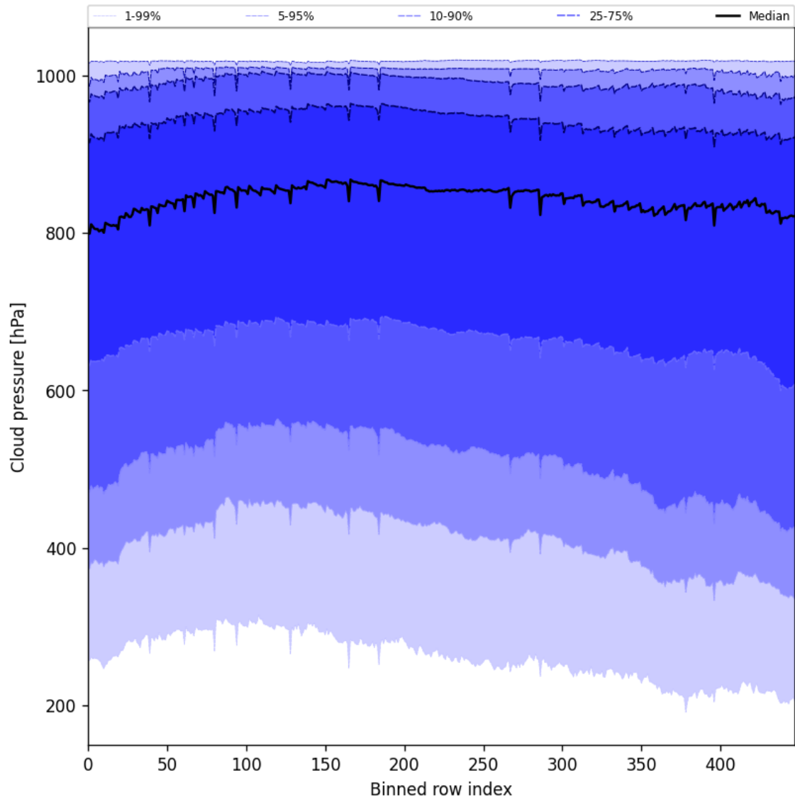
Figure 47: Along track statistics of “Cloud pressure” for 2025-01-30 to 2025-02-01
