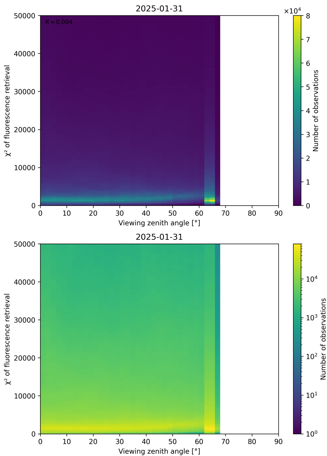
Figure 119: Scatter density plot of “Viewing zenith angle” against “ \chi^2 of fluorescence retrieval” for 2025-01-30 to 2025-02-01.
