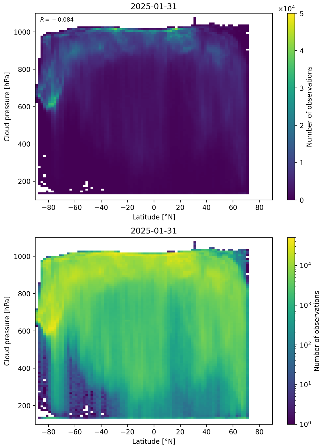
Figure 91: Scatter density plot of “Latitude” against “Cloud pressure” for 2025-01-30 to 2025-02-01.
