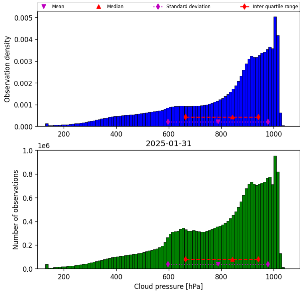
Figure 30: Histogram of “Cloud pressure” for 2025-01-30 to 2025-02-01
