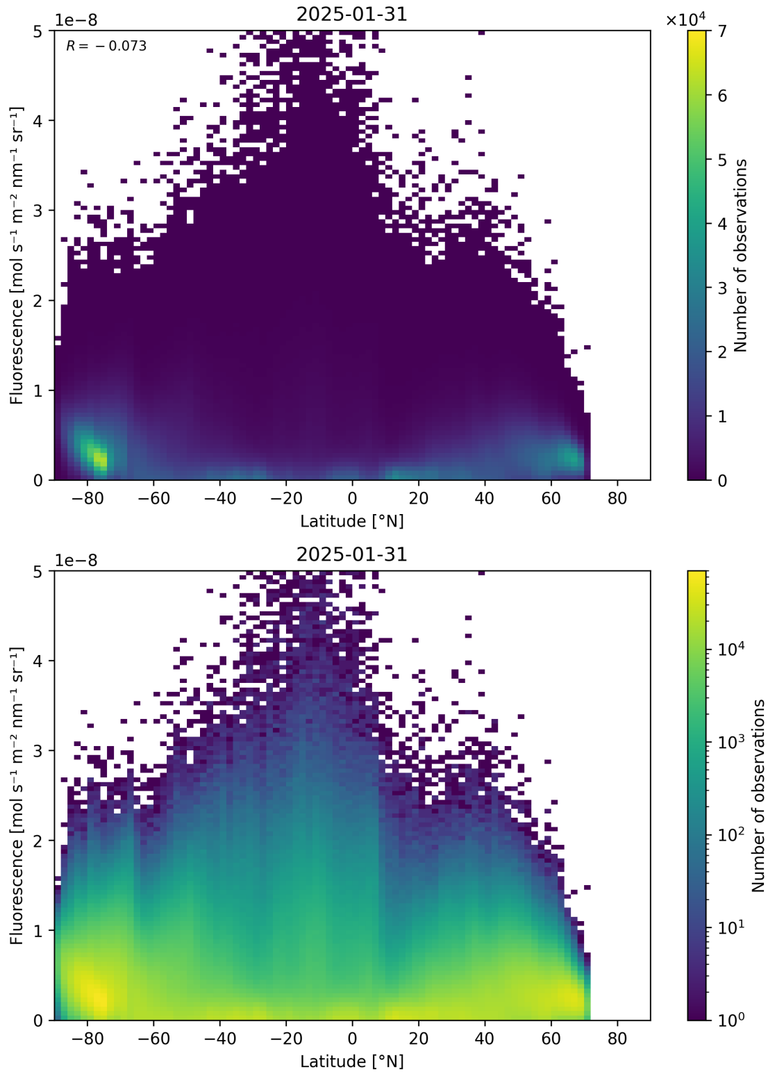
Figure 92: Scatter density plot of “Latitude” against “Fluorescence” for 2025-01-30 to 2025-02-01.
