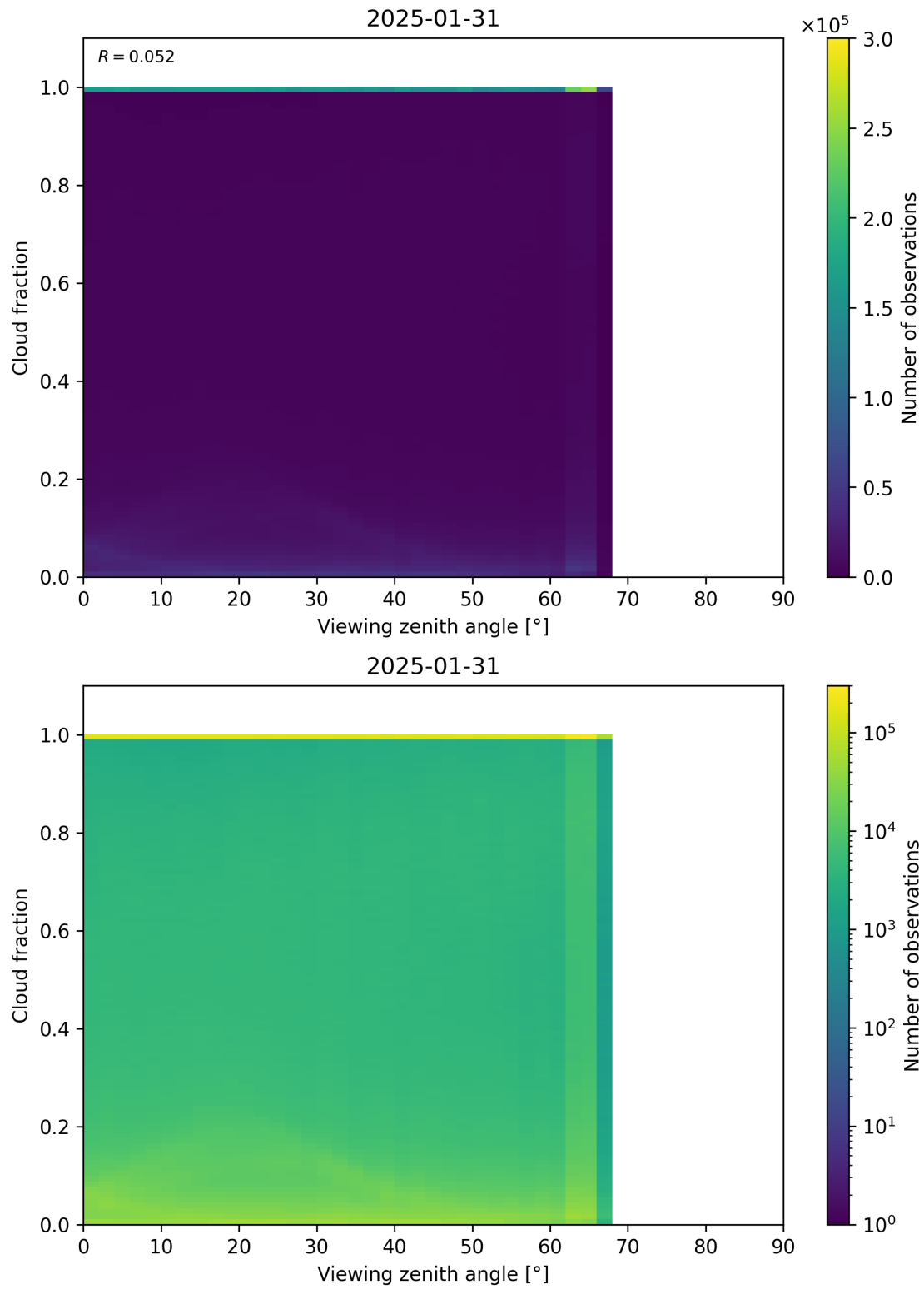
Figure 120: Scatter density plot of “Viewing zenith angle” against “Cloud fraction” for 2025-01-30 to 2025-02-01.
