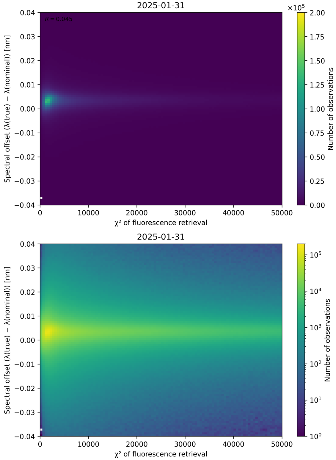
Figure 69: Scatter density plot of “ \chi^2 of fluorescence retrieval” against “Spectral offset ( \lambda_{\text{true}} - \lambda_{\text{nominal}} )” for 2025-01-30 to 2025-02-01.
