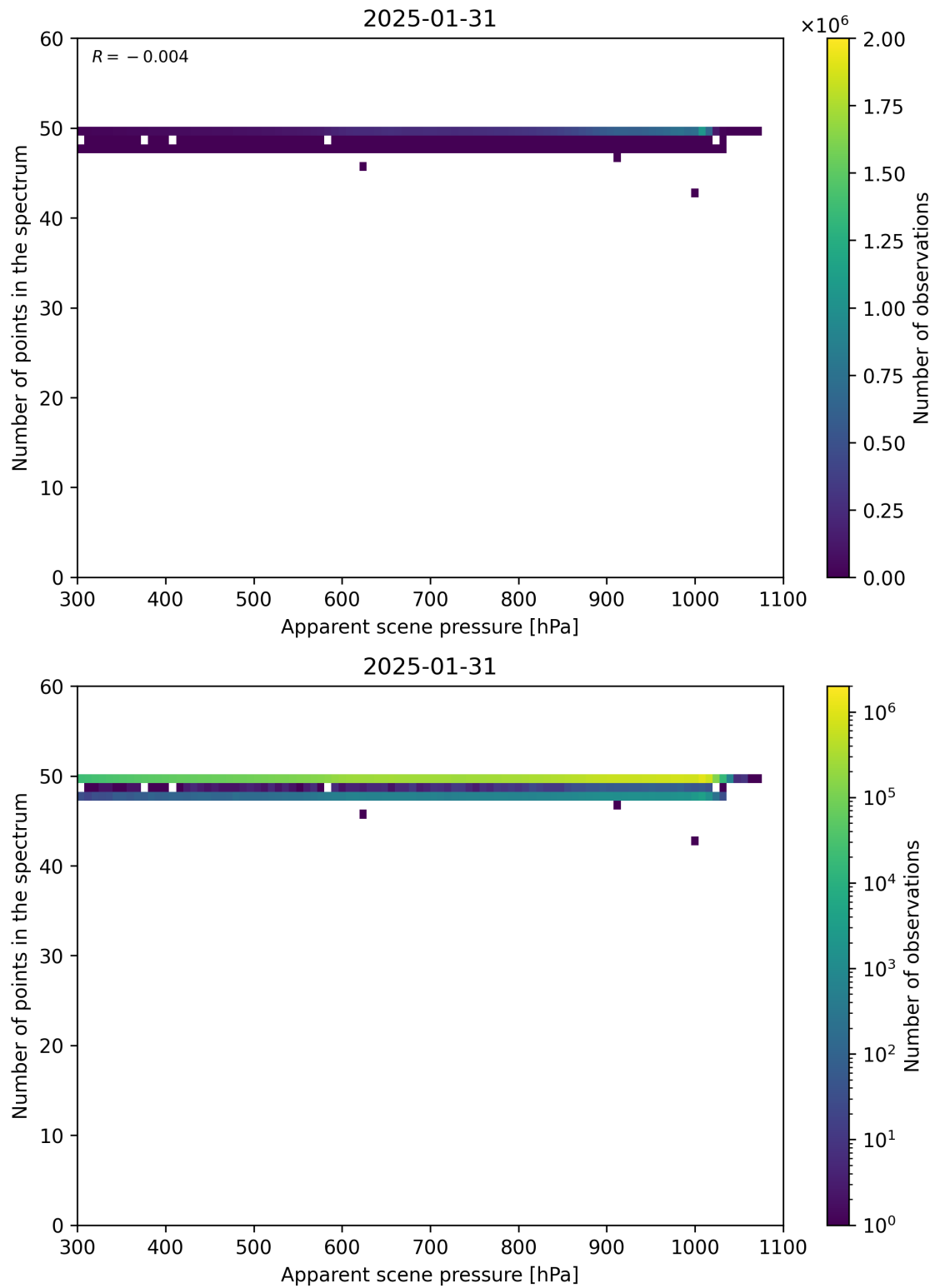
Figure 66: Scatter density plot of “Apparent scene pressure” against “Number of points in the spectrum” for 2025-01-30 to 2025-02-01.
