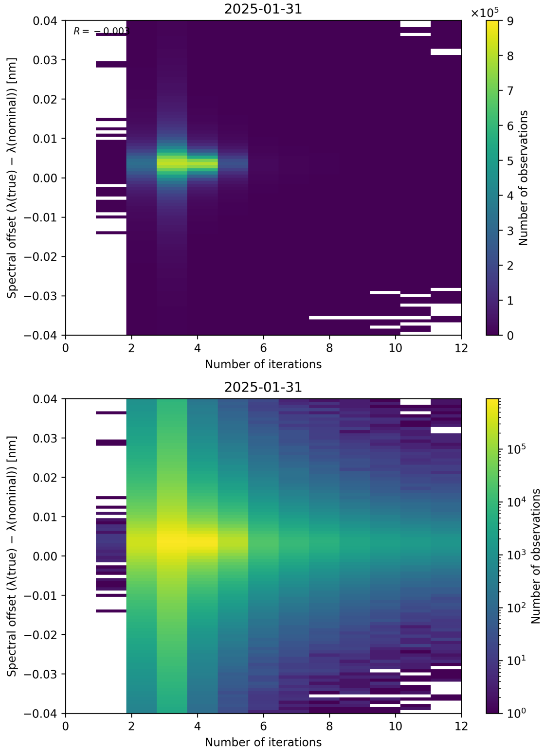
Figure 100: Scatter density plot of “Number of iterations” against “Spectral offset ( \lambda_{\text{true}} - \lambda_{\text{nominal}} )” for 2025-01-30 to 2025-02-01.
