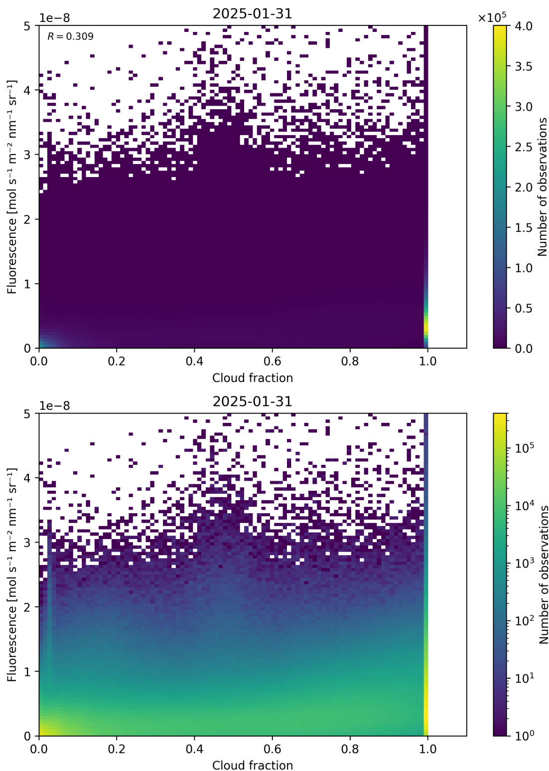
Figure 72: Scatter density plot of “Cloud fraction” against “Fluorescence” for 2025-01-30 to 2025-02-01.
