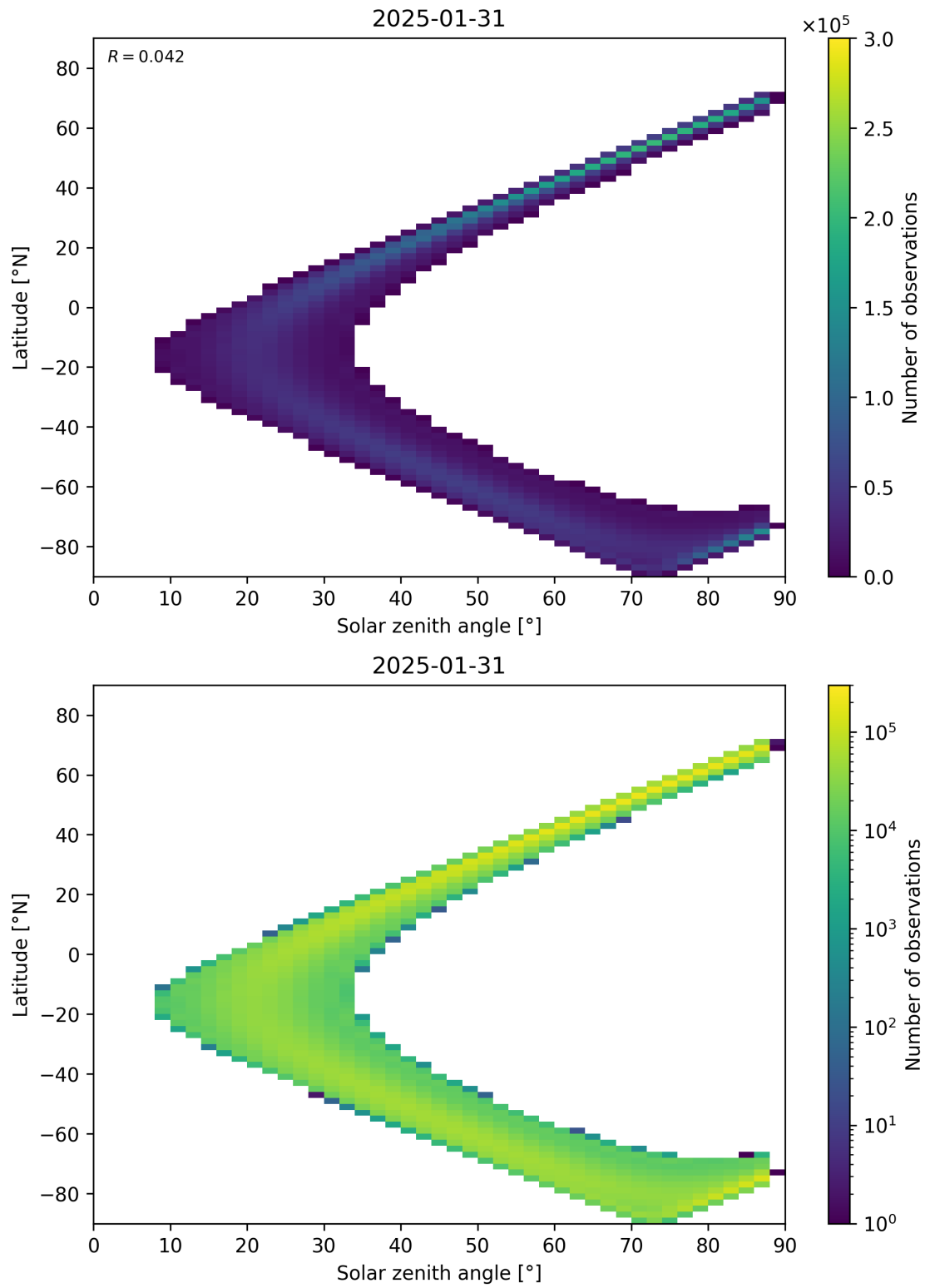
Figure 113: Scatter density plot of “Solar zenith angle” against “Latitude” for 2025-01-30 to 2025-02-01.
