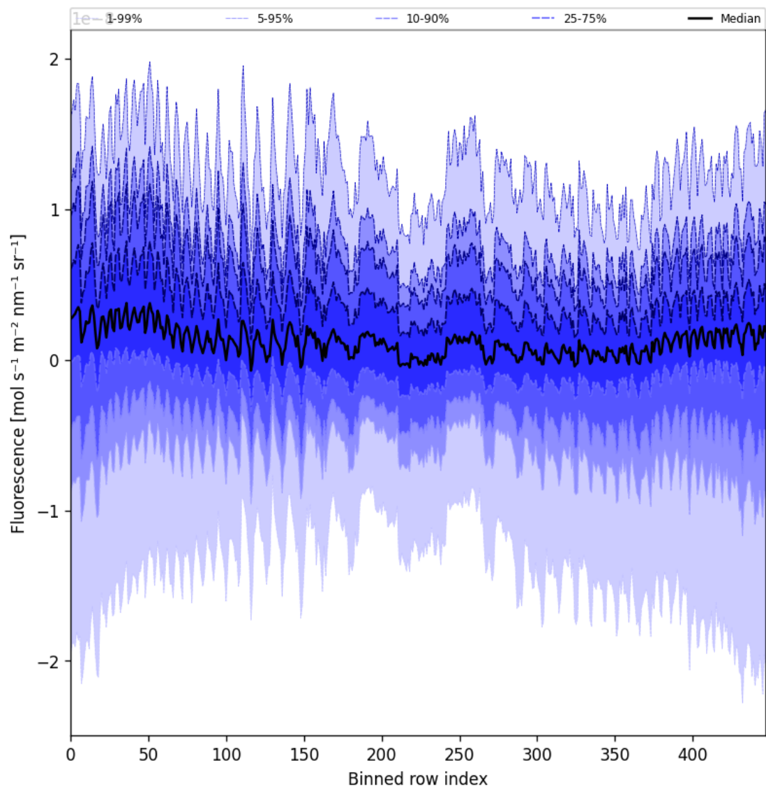
Figure 57: Along track statistics of “Fluorescence” for 2025-01-30 to 2025-02-01
