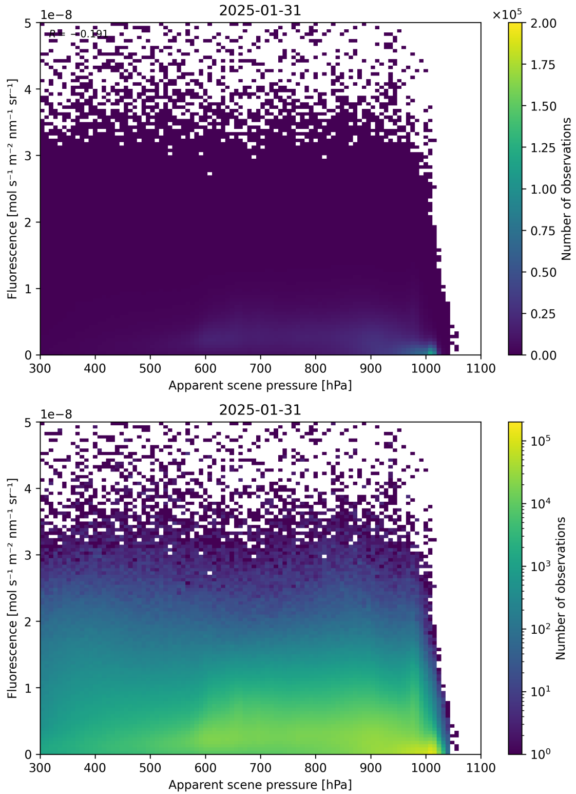
Figure 64: Scatter density plot of “Apparent scene pressure” against “Fluorescence” for 2025-01-30 to 2025-02-01.
