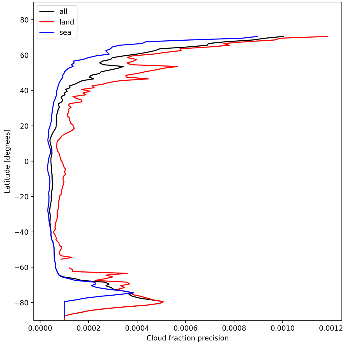
Figure 16: Zonal average of “Cloud fraction precision” for 2025-01-30 to 2025-02-01.
