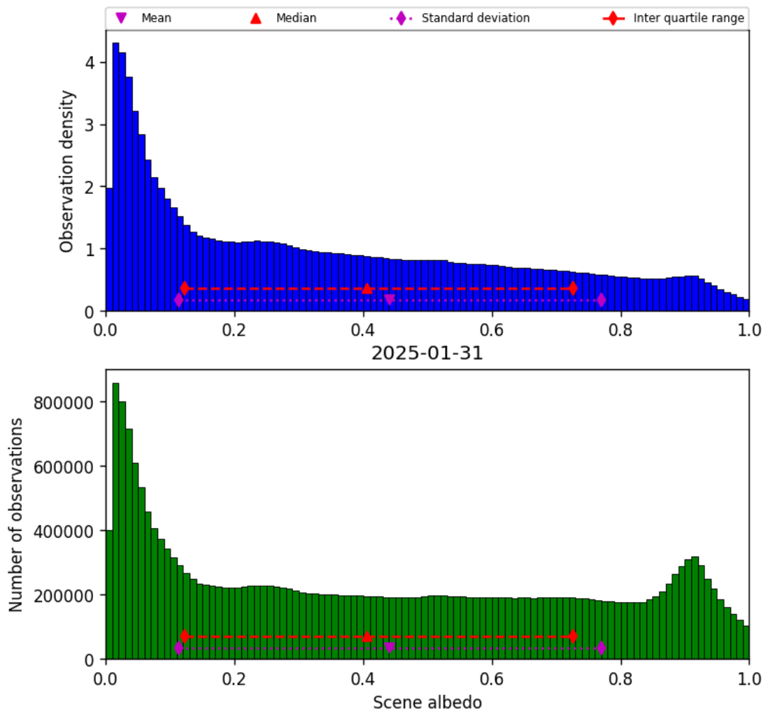
Figure 34: Histogram of “Scene albedo” for 2025-01-30 to 2025-02-01
