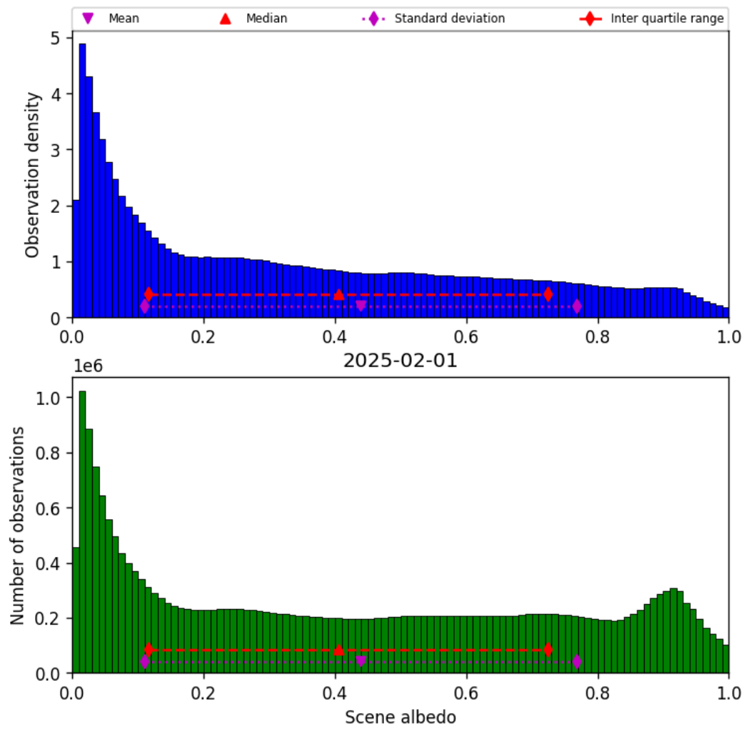
Figure 34: Histogram of “Scene albedo” for 2025-01-31 to 2025-02-02
