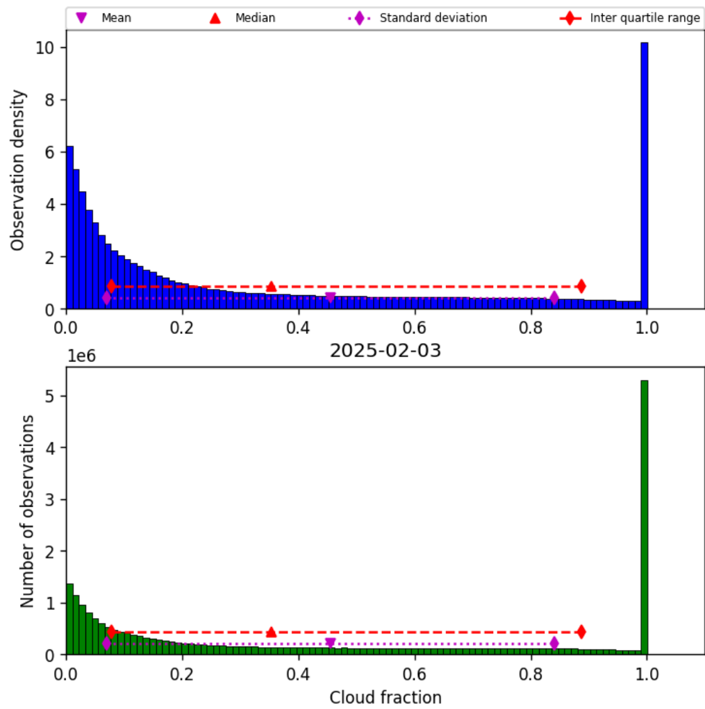
Figure 32: Histogram of “Cloud fraction” for 2025-02-03 to 2025-02-04
