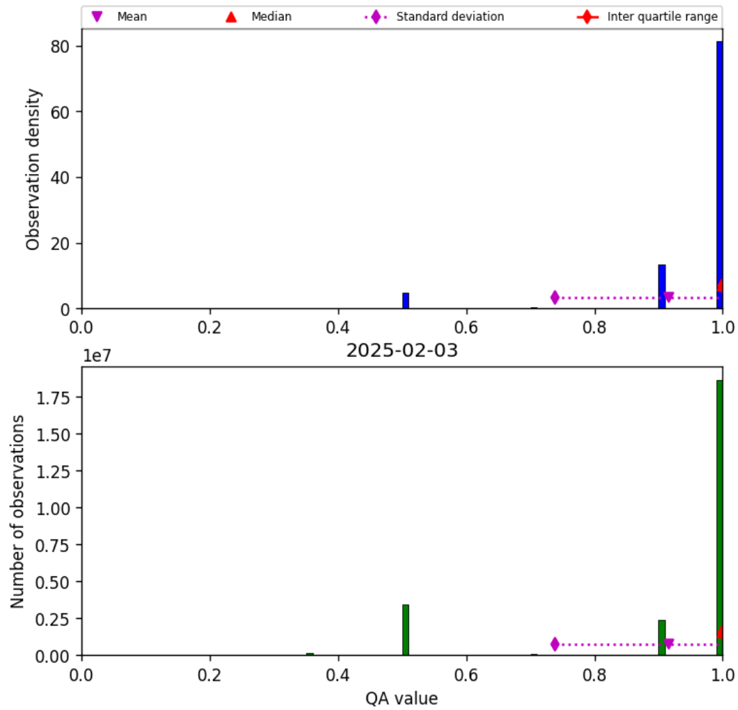
Figure 29: Histogram of “QA value” for 2025-02-03 to 2025-02-04
