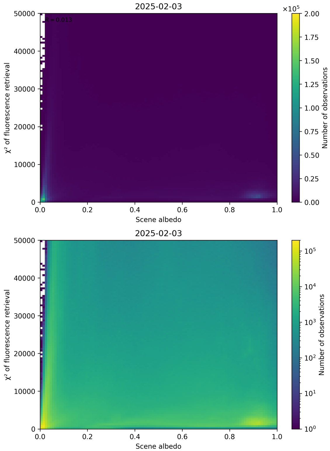
Figure 103: Scatter density plot of “Scene albedo” against “ \chi^2 of fluorescence retrieval” for 2025-02-03 to 2025-02-04.
