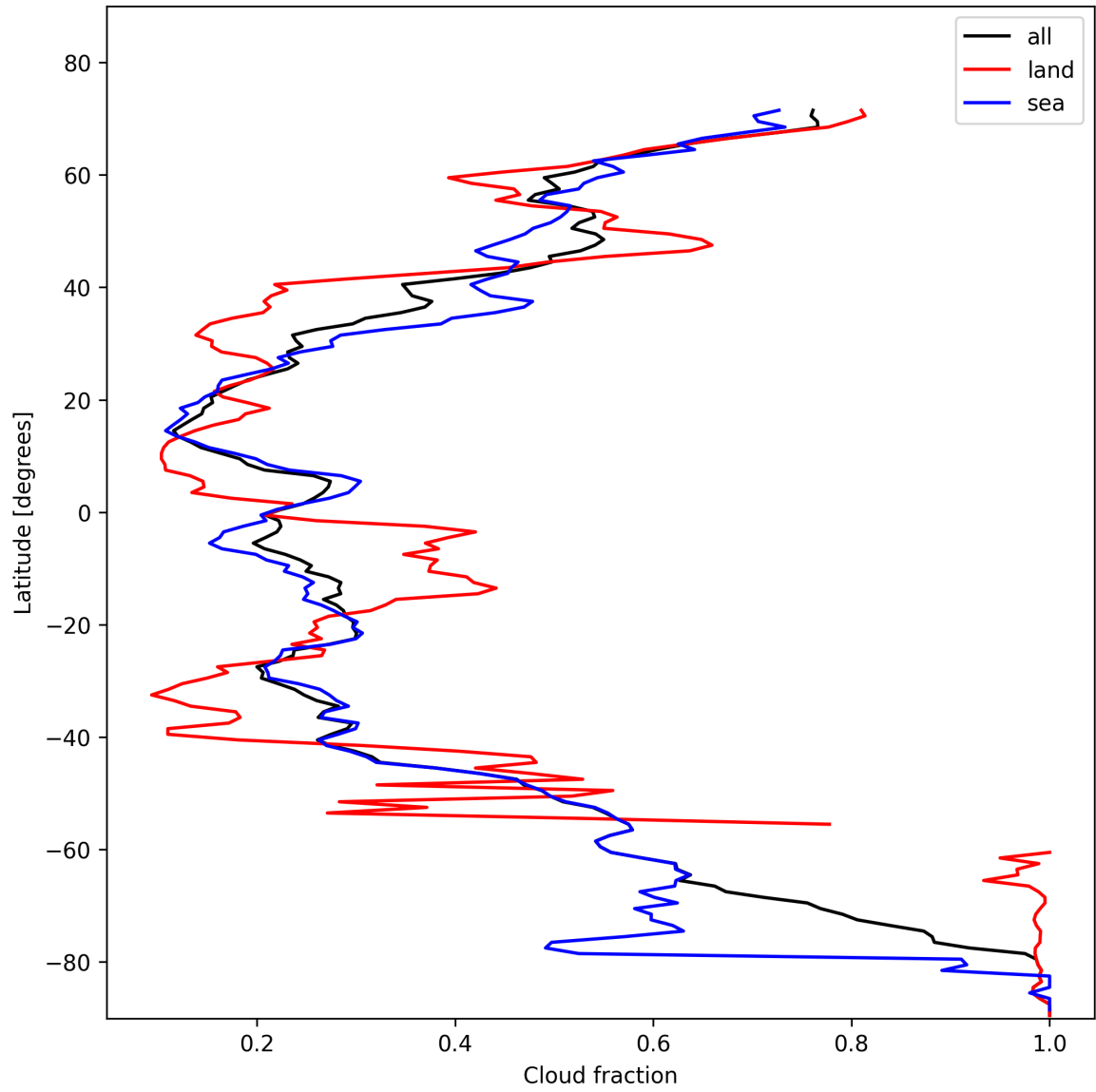
Figure 15: Zonal average of “Cloud fraction” for 2025-02-03 to 2025-02-04.
