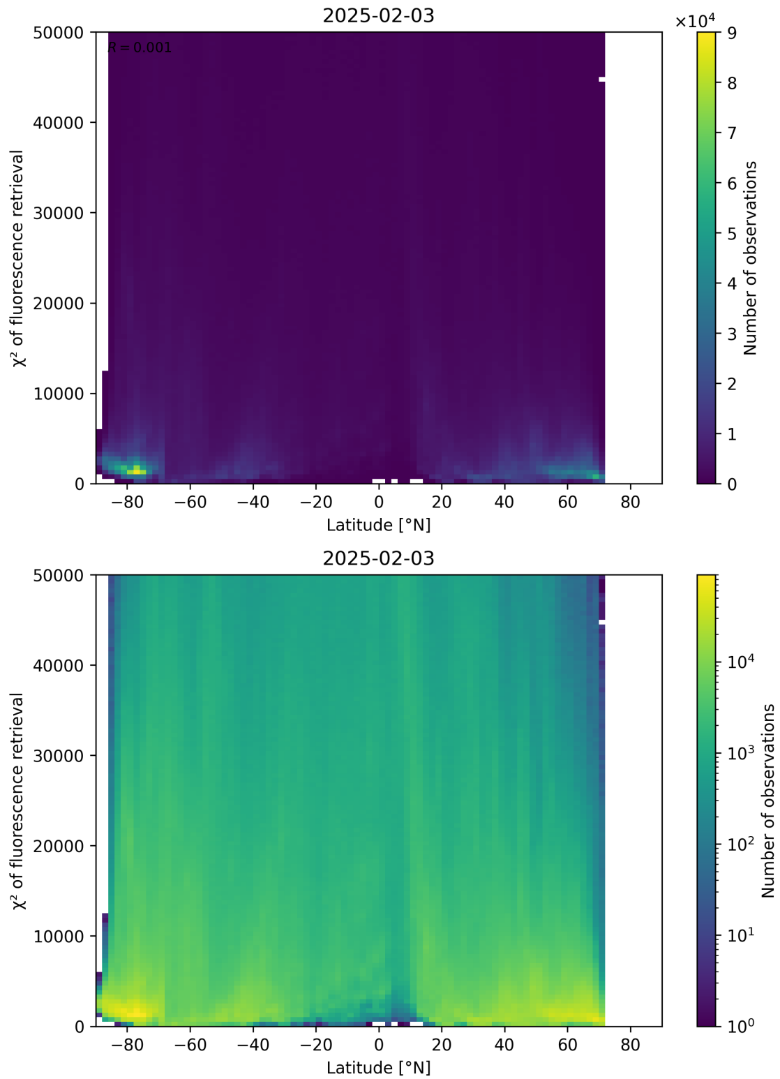
Figure 89: Scatter density plot of “Latitude” against “ \chi^2 of fluorescence retrieval” for 2025-02-03 to 2025-02-04.
