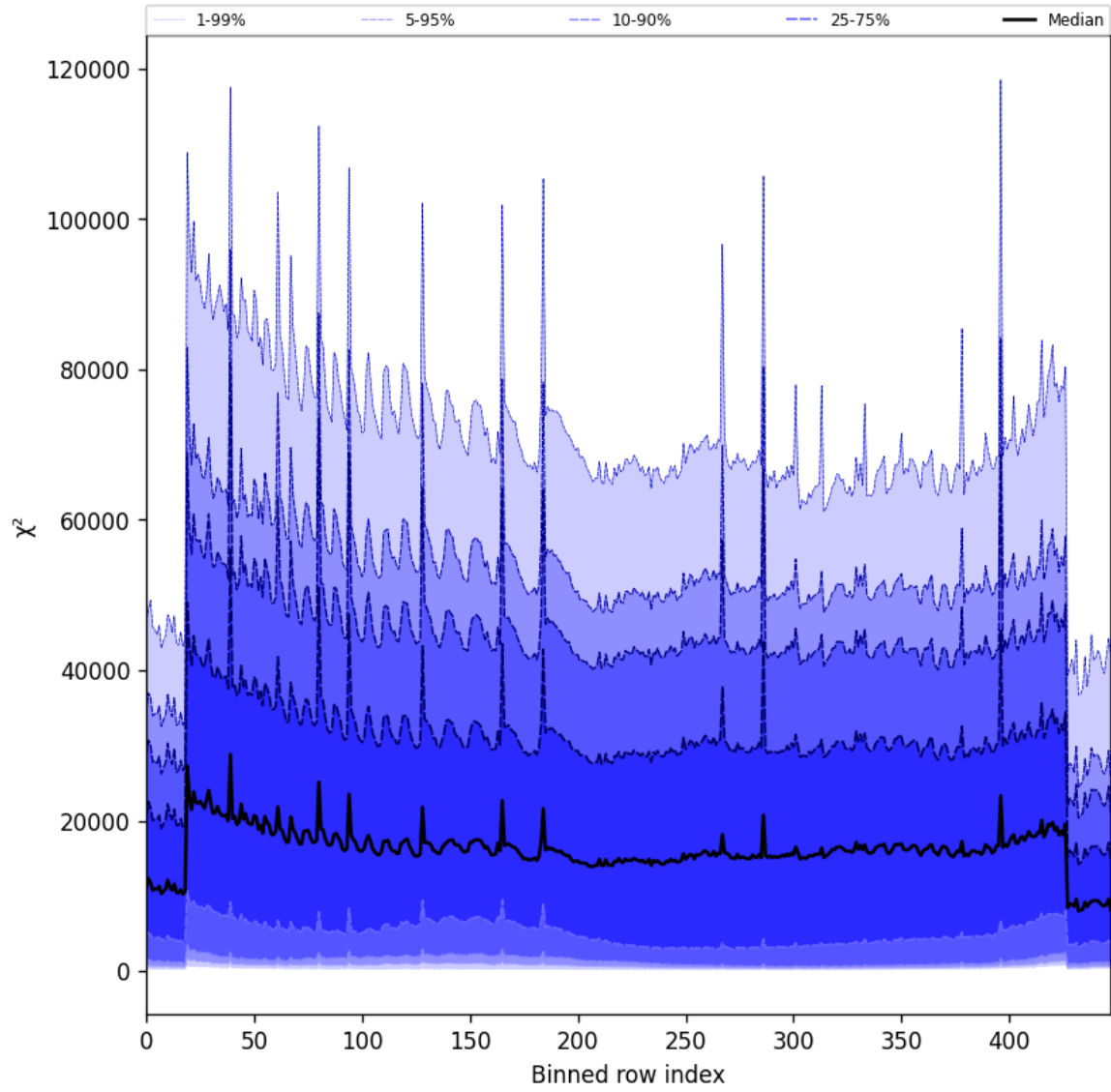
Figure 55: Along track statistics of “ \chi^2 ” for 2025-02-03 to 2025-02-04
