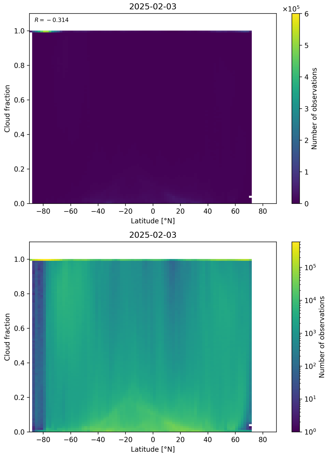
Figure 90: Scatter density plot of “Latitude” against “Cloud fraction” for 2025-02-03 to 2025-02-04.
