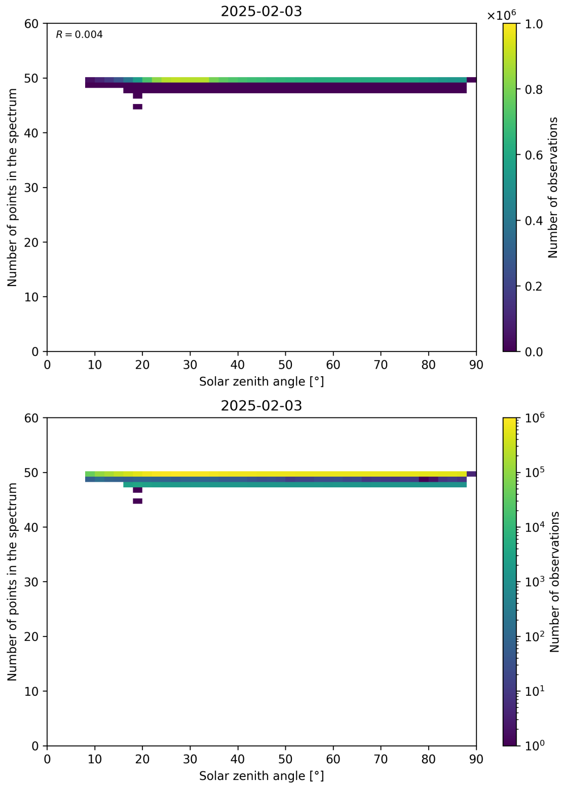
Figure 115: Scatter density plot of “Solar zenith angle” against “Number of points in the spectrum” for 2025-02-03 to 2025-02-04.
