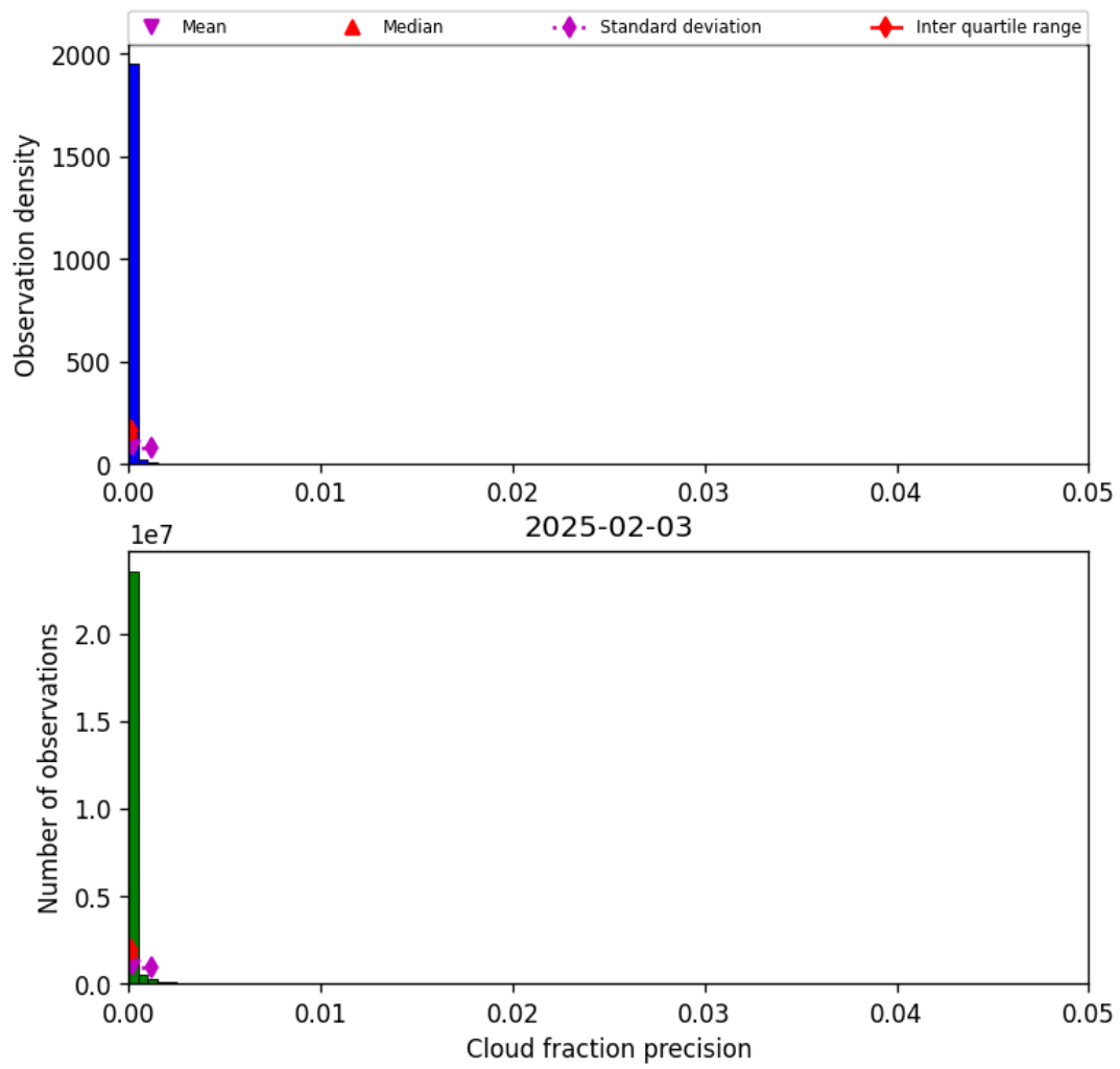
Figure 33: Histogram of “Cloud fraction precision” for 2025-02-03 to 2025-02-04
