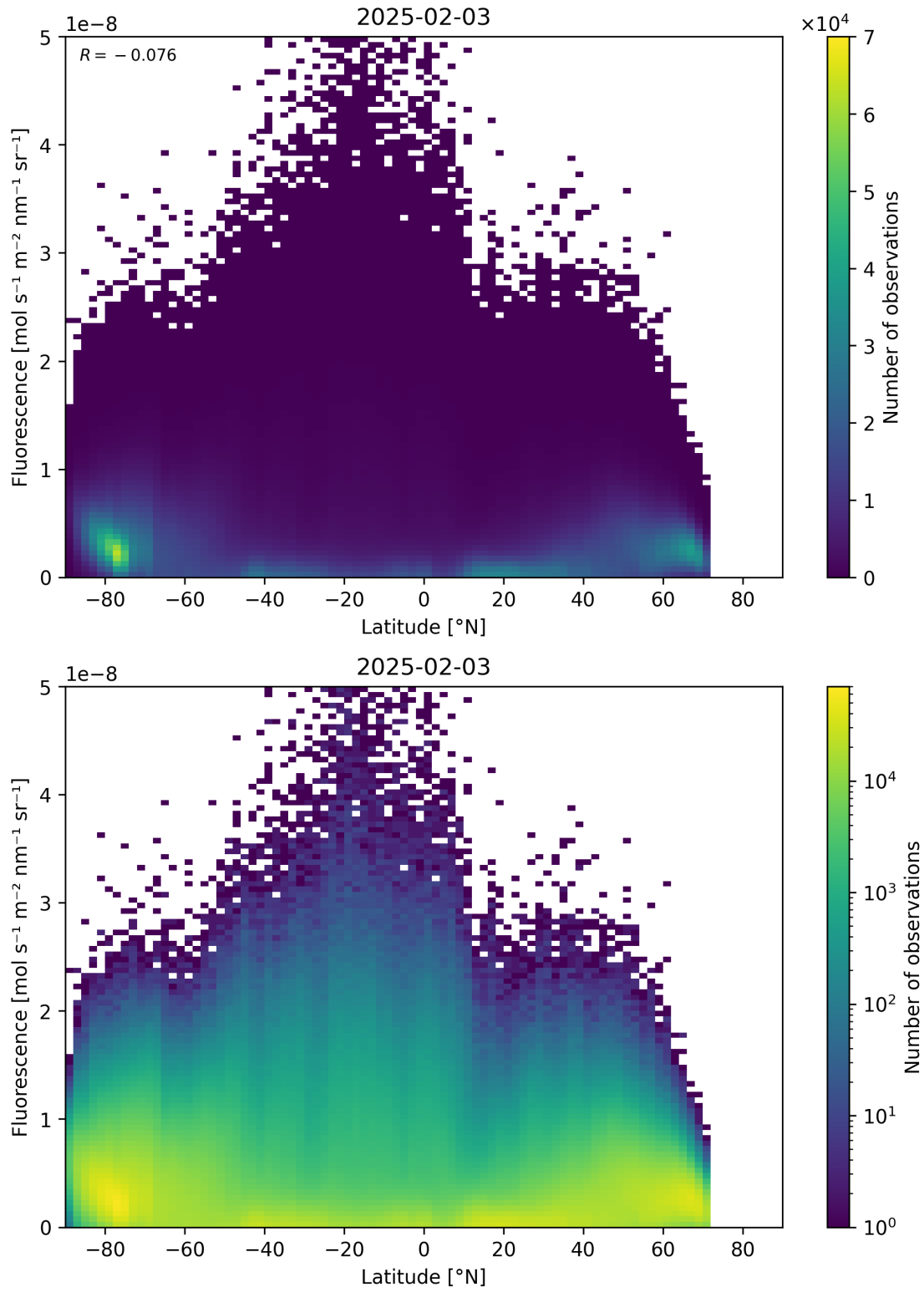
Figure 92: Scatter density plot of “Latitude” against “Fluorescence” for 2025-02-03 to 2025-02-04.
