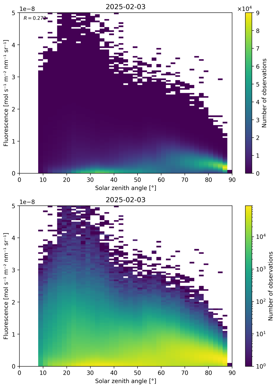
Figure 112: Scatter density plot of “Solar zenith angle” against “Fluorescence” for 2025-02-03 to 2025-02-04.
