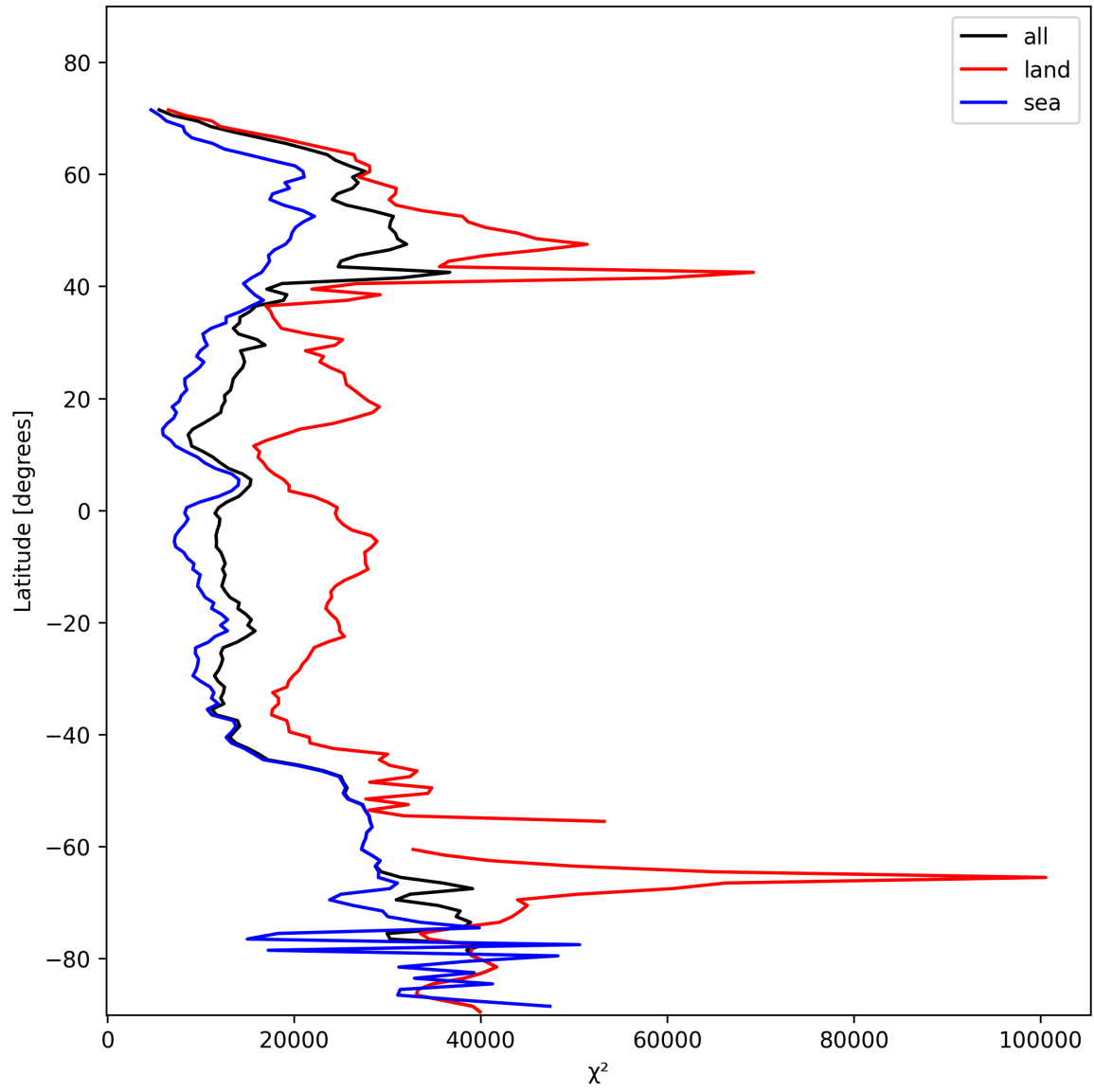
Figure 21: Zonal average of “ \chi^2 ” for 2025-02-03 to 2025-02-04.
