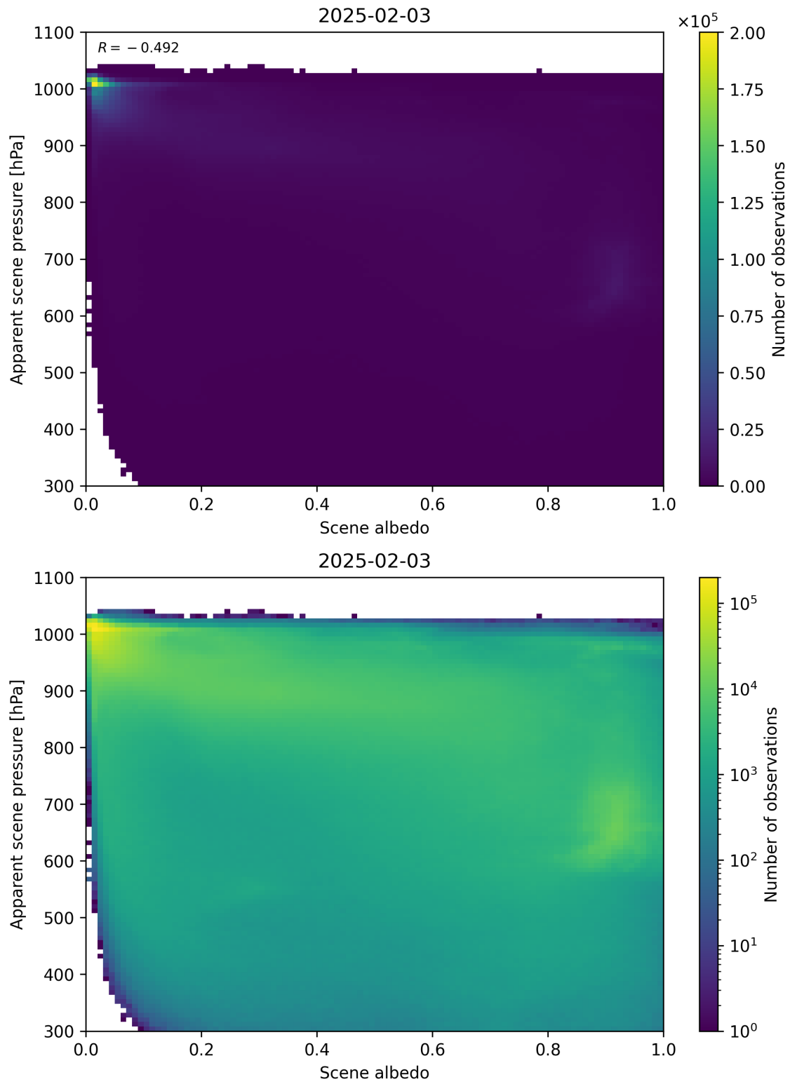
Figure 102: Scatter density plot of “Scene albedo” against “Apparent scene pressure” for 2025-02-03 to 2025-02-04.
