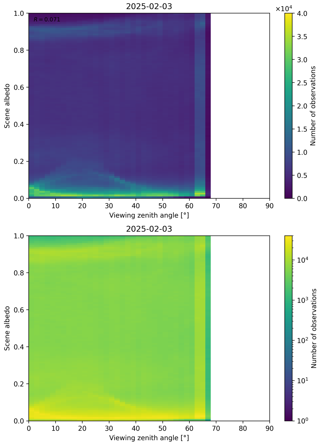
Figure 126: Scatter density plot of “Viewing zenith angle” against “Scene albedo” for 2025-02-03 to 2025-02-04.
