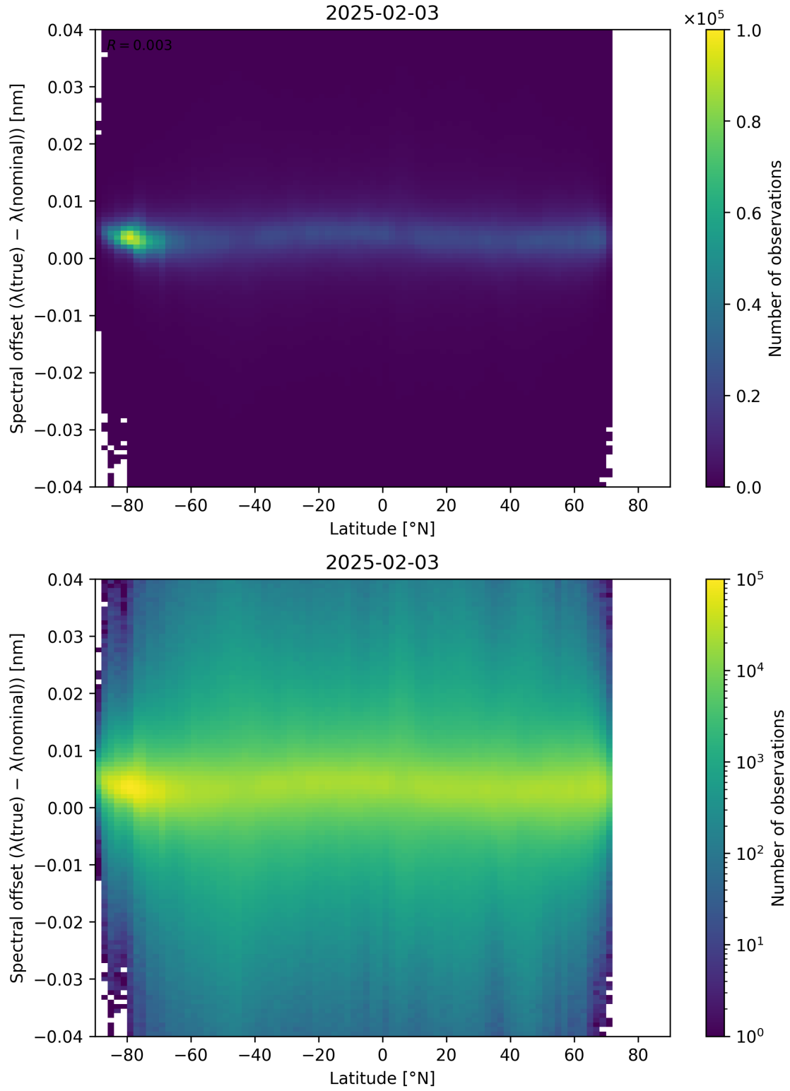
Figure 96: Scatter density plot of “Latitude” against “Spectral offset ( \lambda_{\text{true}} - \lambda_{\text{nominal}} )” for 2025-02-03 to 2025-02-04.
