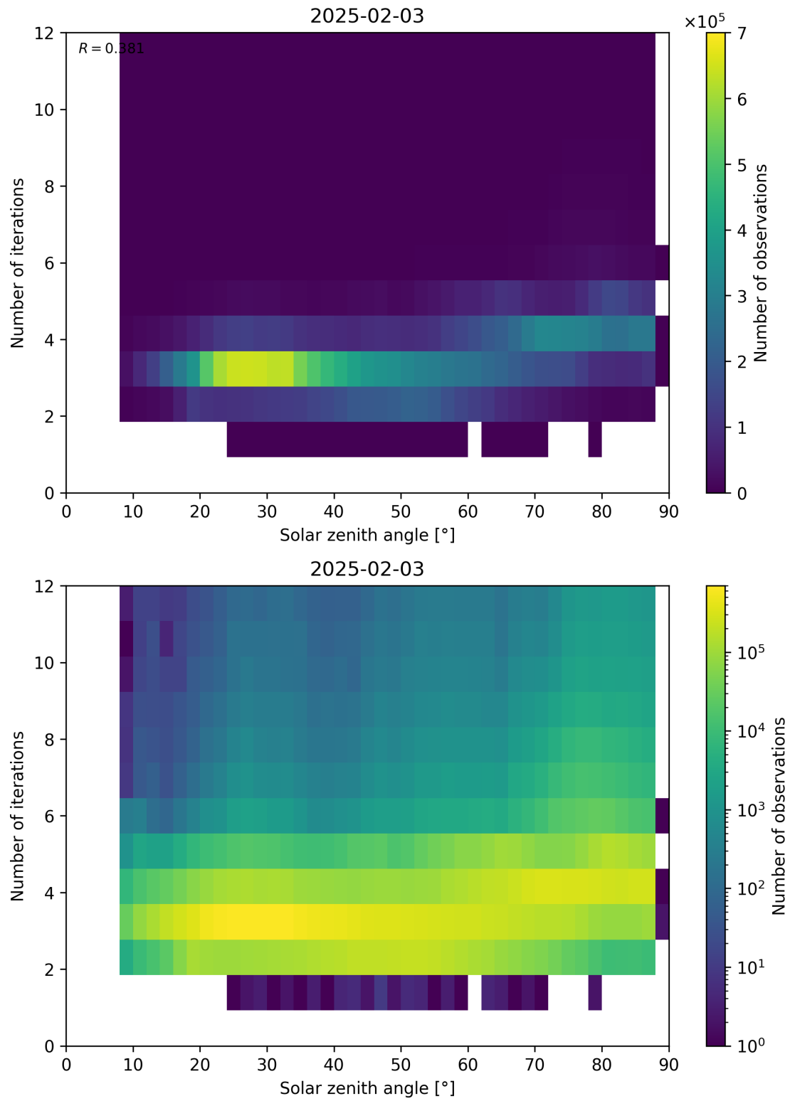
Figure 114: Scatter density plot of “Solar zenith angle” against “Number of iterations” for 2025-02-03 to 2025-02-04.
