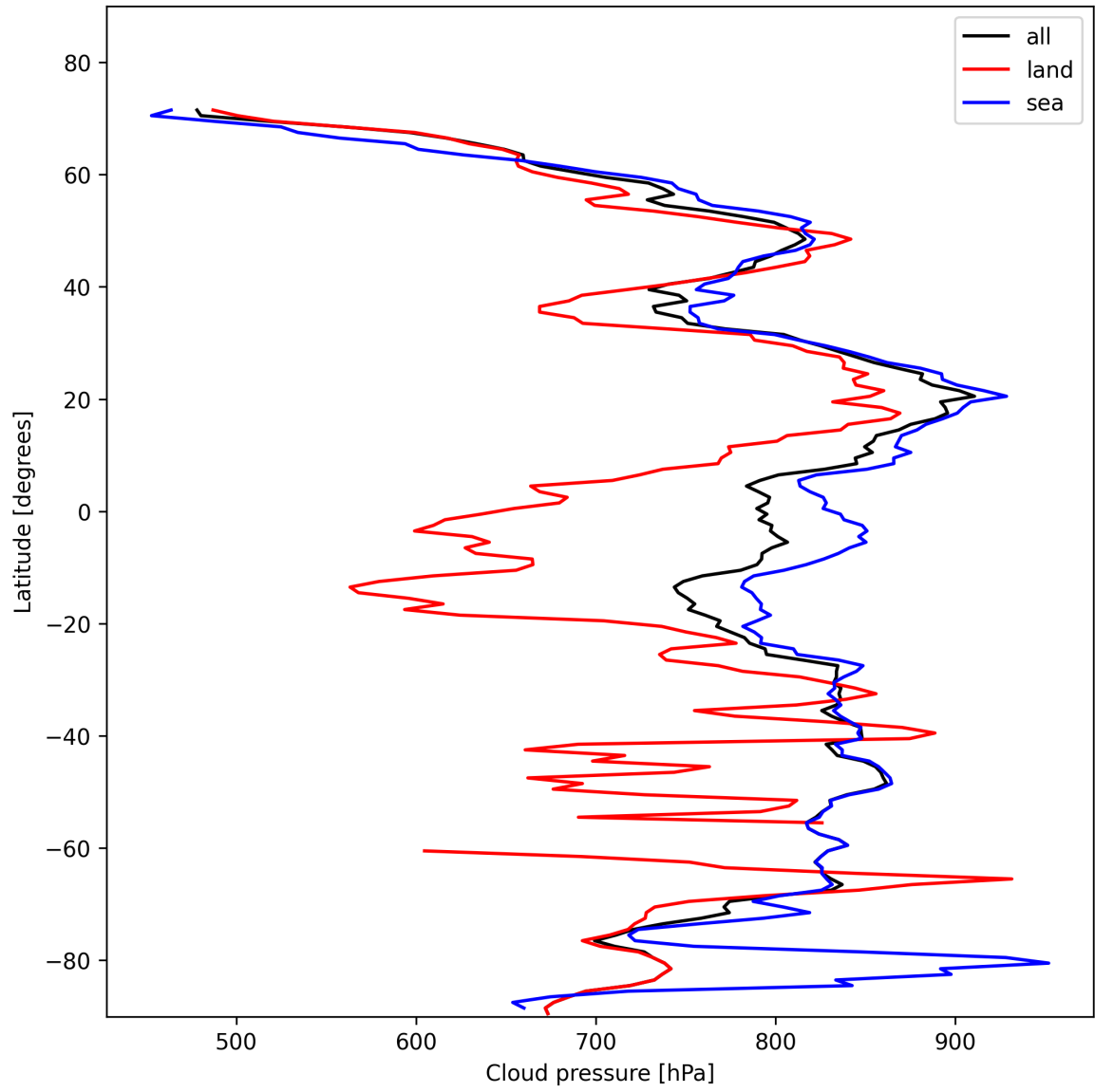
Figure 13: Zonal average of “Cloud pressure” for 2025-02-03 to 2025-02-04.
