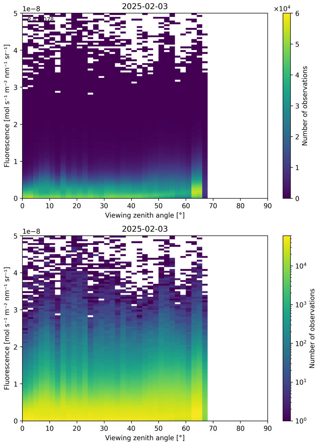
Figure 122: Scatter density plot of “Viewing zenith angle” against “Fluorescence” for 2025-02-03 to 2025-02-04.
