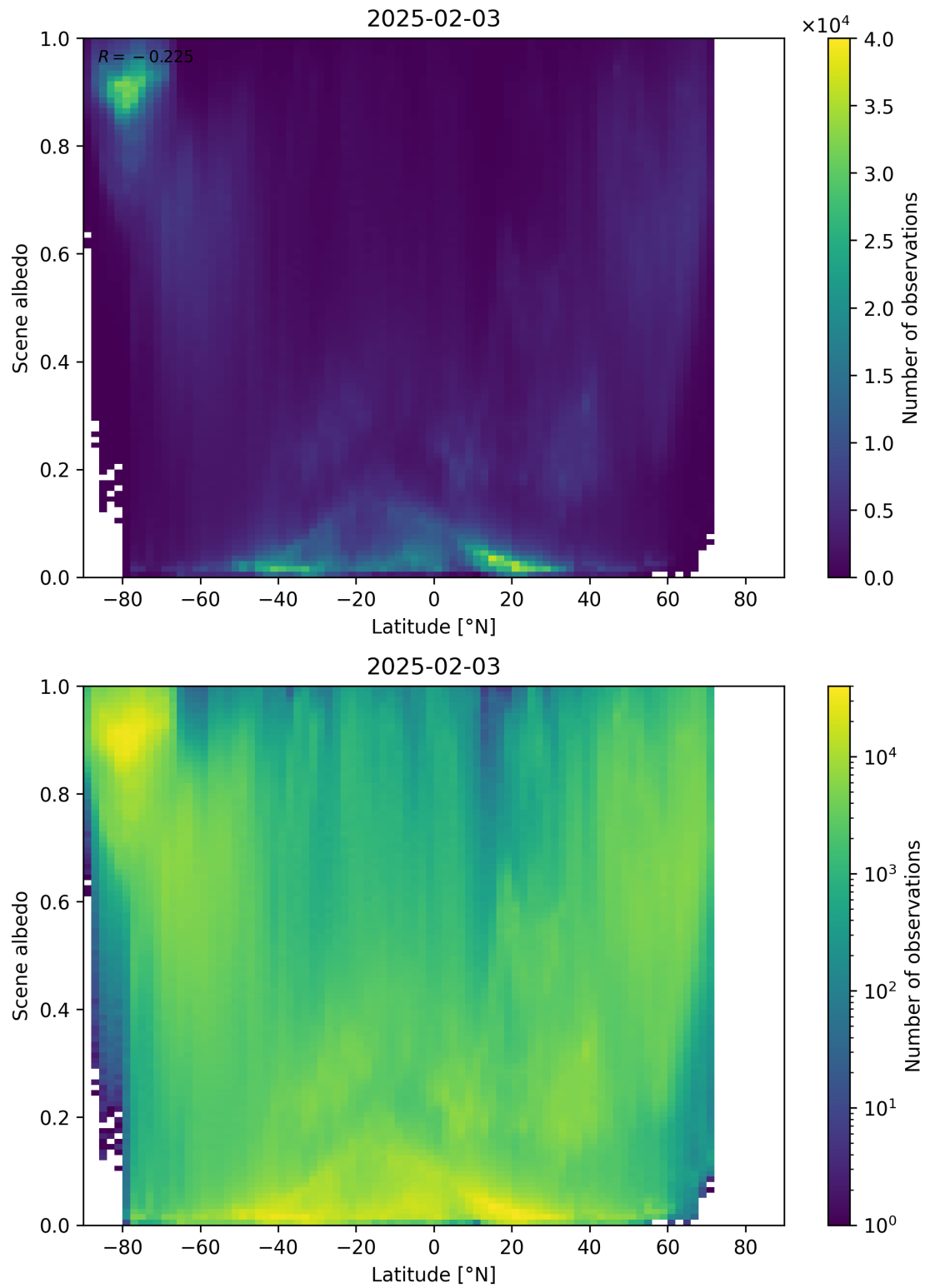
Figure 95: Scatter density plot of “Latitude” against “Scene albedo” for 2025-02-03 to 2025-02-04.
