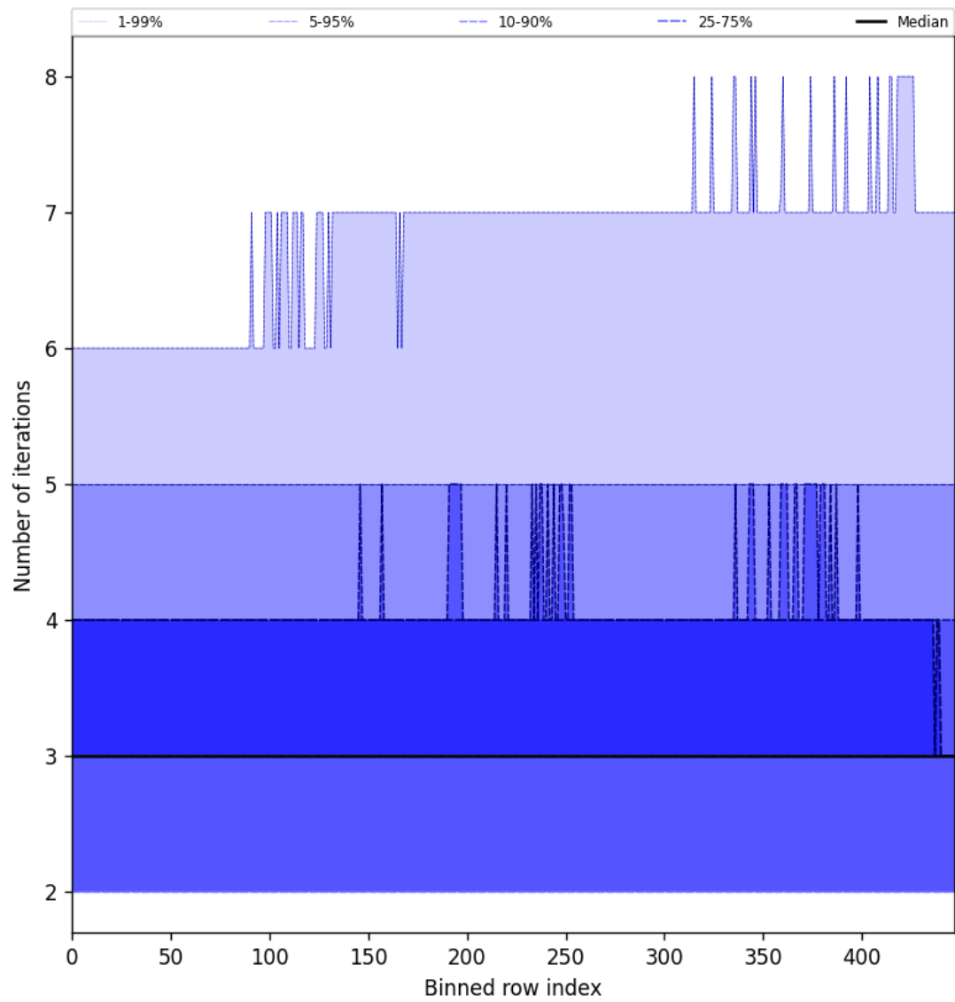
Figure 56: Along track statistics of “Number of iterations” for 2025-02-03 to 2025-02-04
