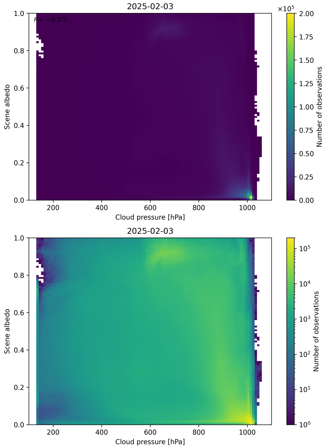
Figure 83: Scatter density plot of “Cloud pressure” against “Scene albedo” for 2025-02-03 to 2025-02-04.
