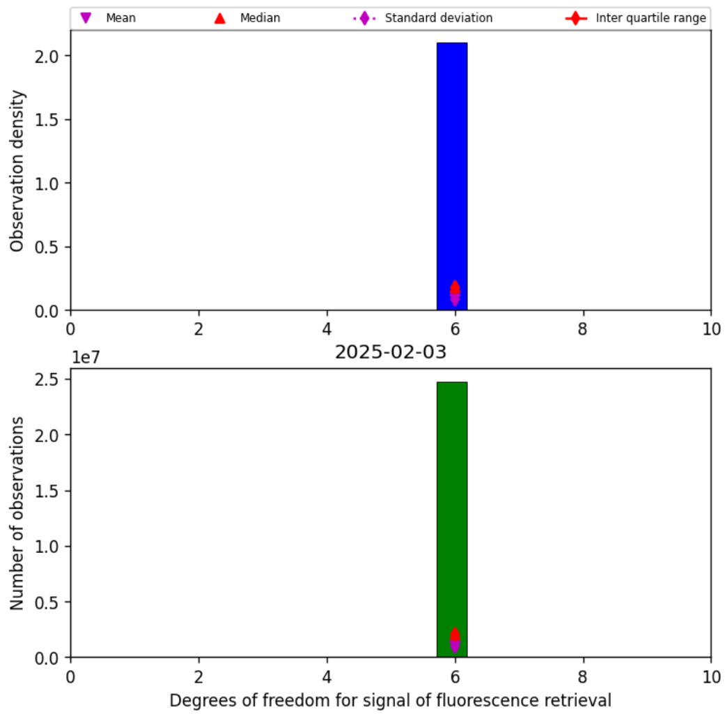
Figure 43: Histogram of “Degrees of freedom for signal of fluorescence retrieval” for 2025-02-03 to 2025-02-04
