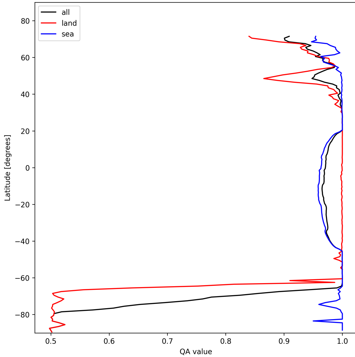
Figure 12: Zonal average of “QA value” for 2025-02-03 to 2025-02-04.
