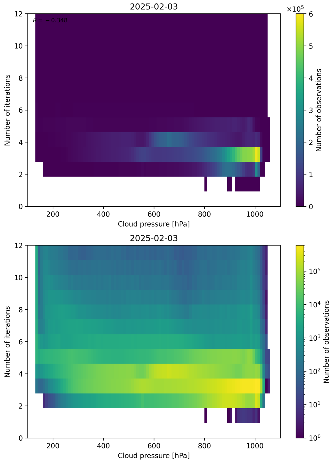
Figure 81: Scatter density plot of “Cloud pressure” against “Number of iterations” for 2025-02-03 to 2025-02-04.
