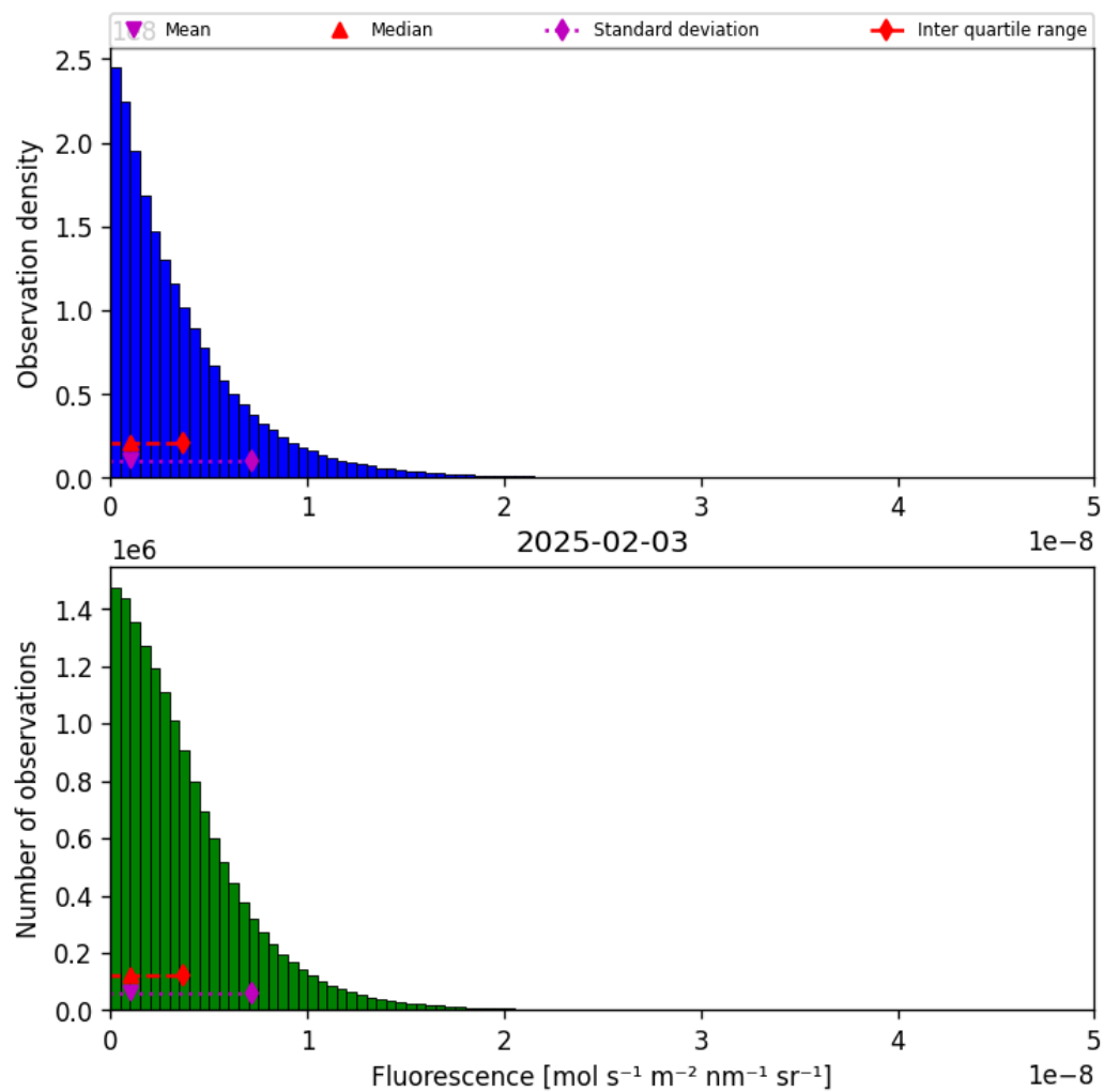
Figure 40: Histogram of “Fluorescence” for 2025-02-03 to 2025-02-04
