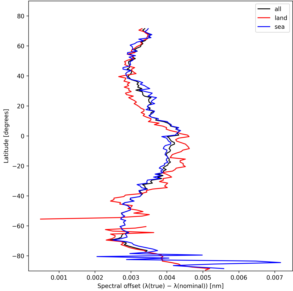
Figure 28: Zonal average of “Spectral offset ( \lambda_{\text{true}} - \lambda_{\text{nominal}} )” for 2025-02-03 to 2025-02-04.
