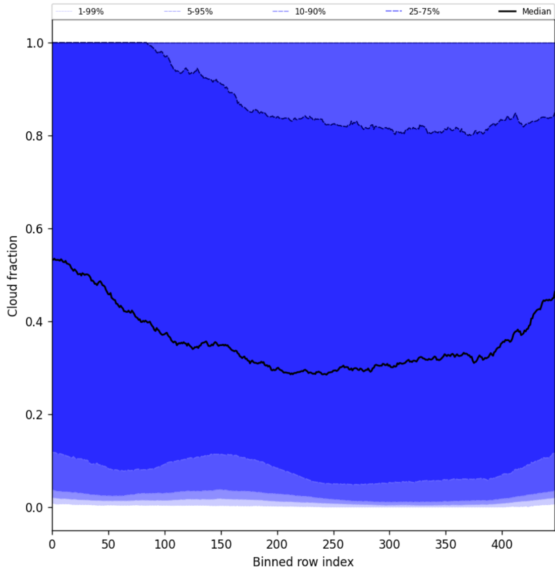
Figure 49: Along track statistics of “Cloud fraction” for 2025-02-03 to 2025-02-04
