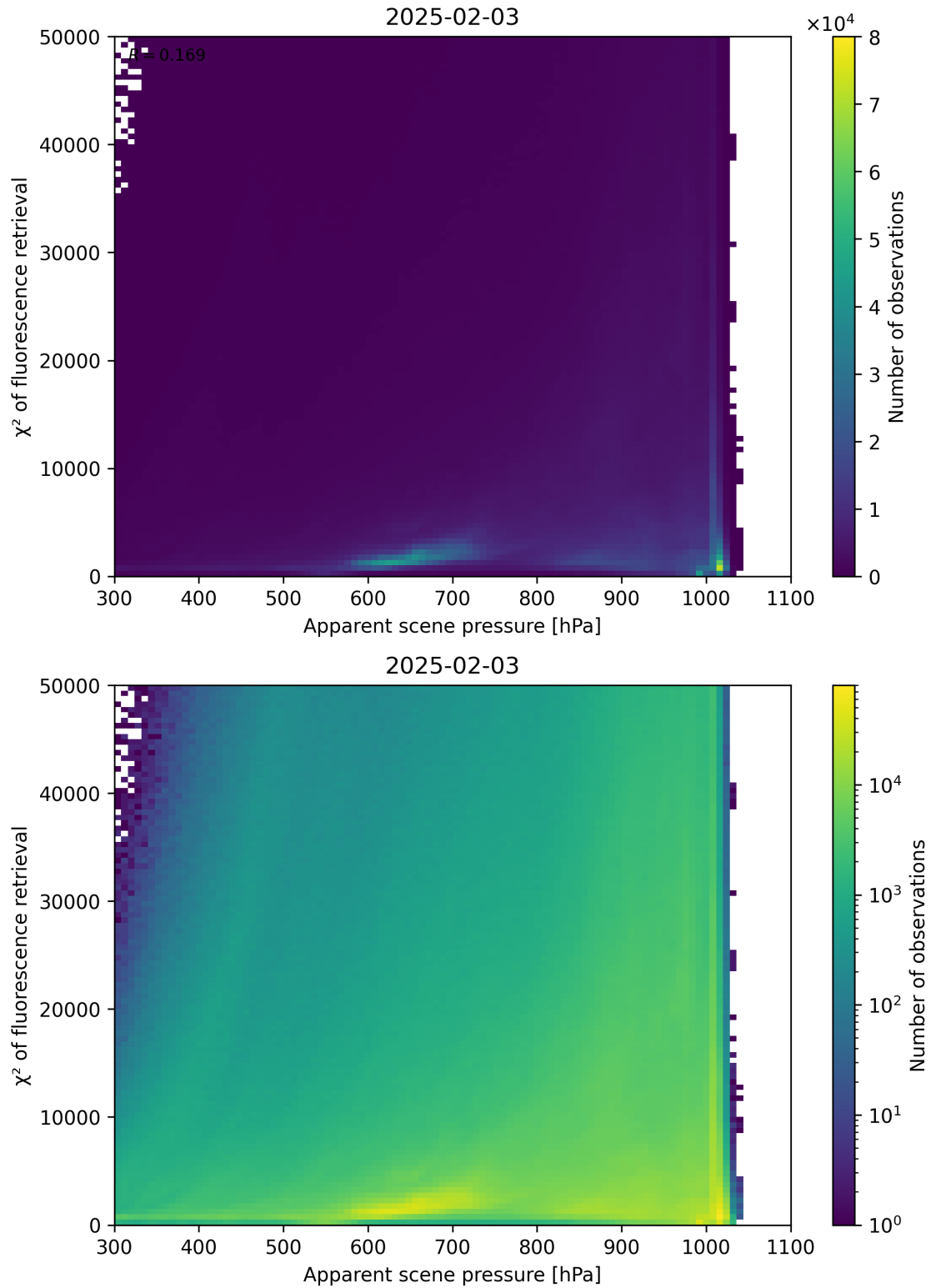
Figure 63: Scatter density plot of “Apparent scene pressure” against “ \chi^2 of fluorescence retrieval” for 2025-02-03 to 2025-02-04.
