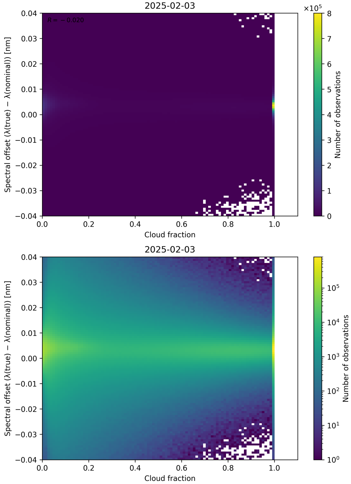
Figure 76: Scatter density plot of “Cloud fraction” against “Spectral offset ( \lambda_{\text{true}} - \lambda_{\text{nominal}} )” for 2025-02-03 to 2025-02-04.
