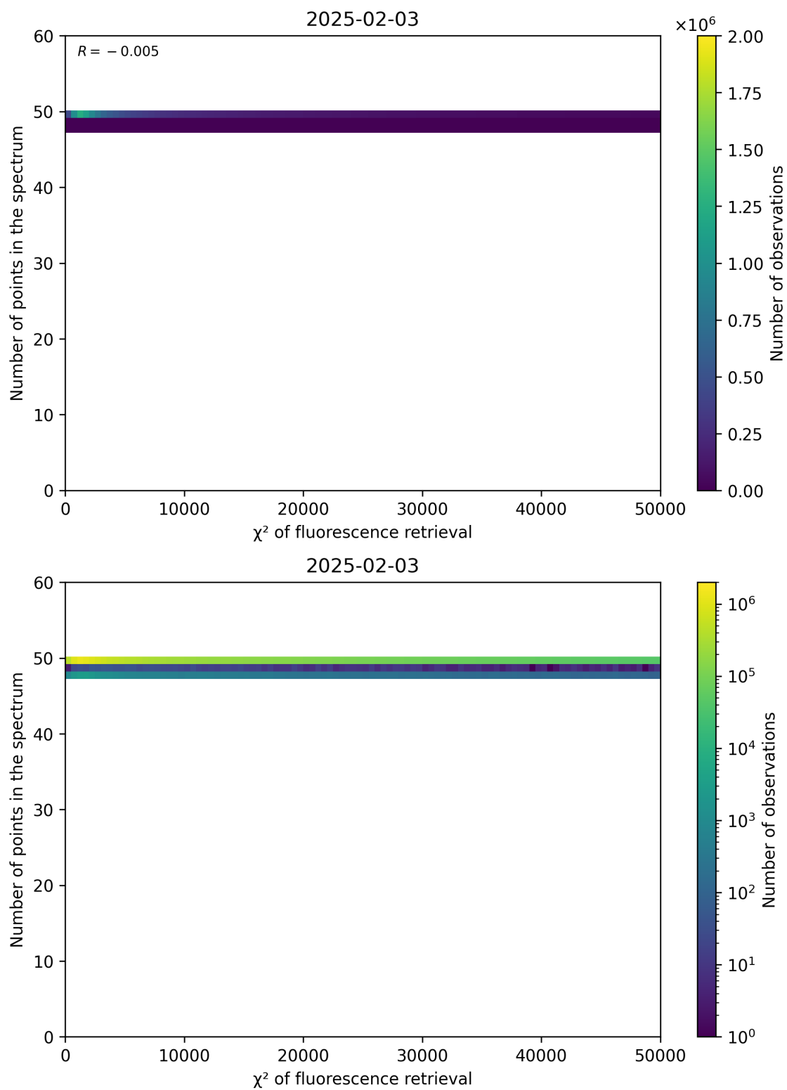
Figure 68: Scatter density plot of " \chi^2 of fluorescence retrieval" against "Number of points in the spectrum" for 2025-02-03 to 2025-02-04.
