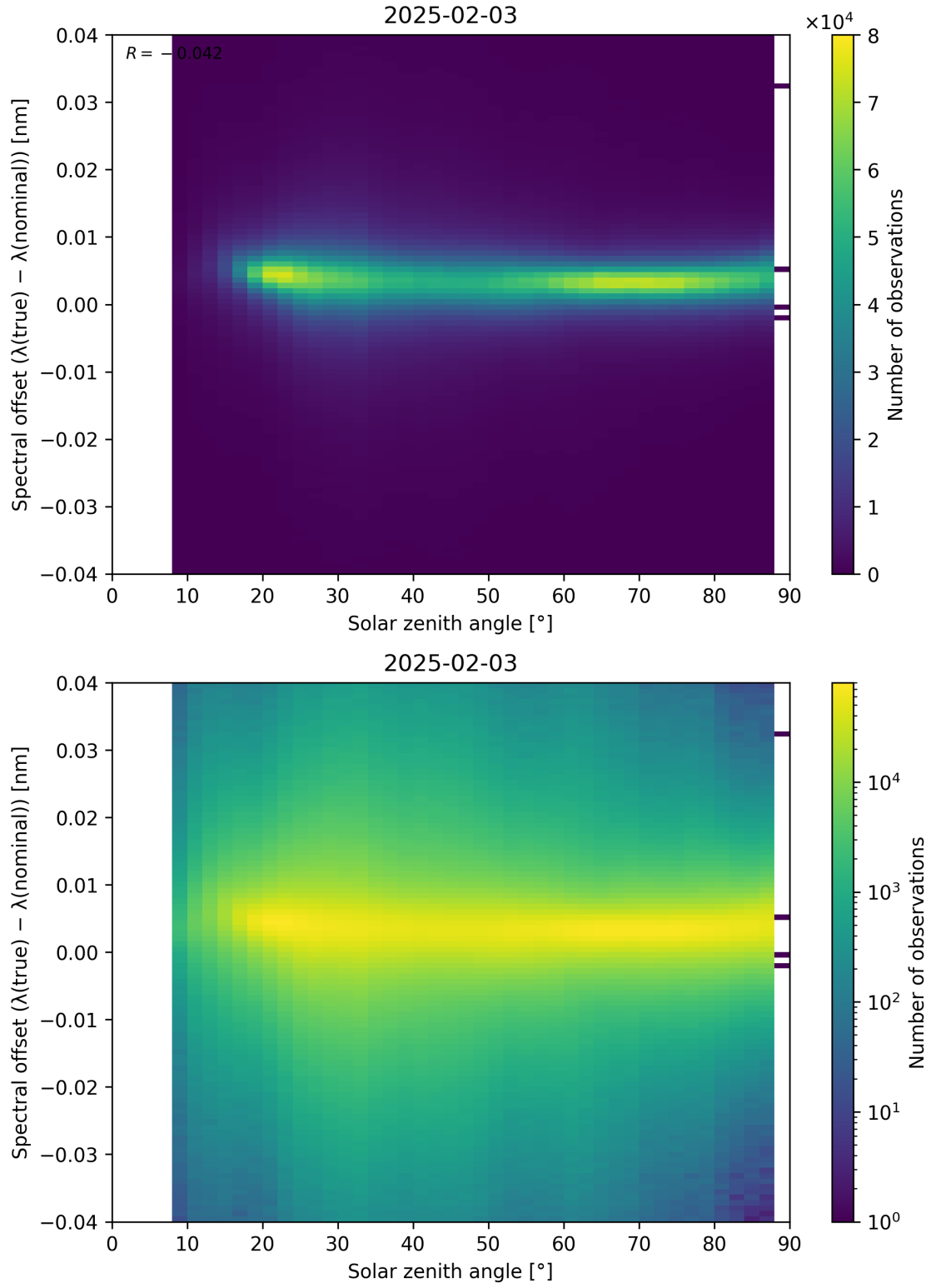
Figure 117: Scatter density plot of “Solar zenith angle” against “Spectral offset ( \lambda_{\text{true}} - \lambda_{\text{nominal}} )” for 2025-02-03 to 2025-02-04.
