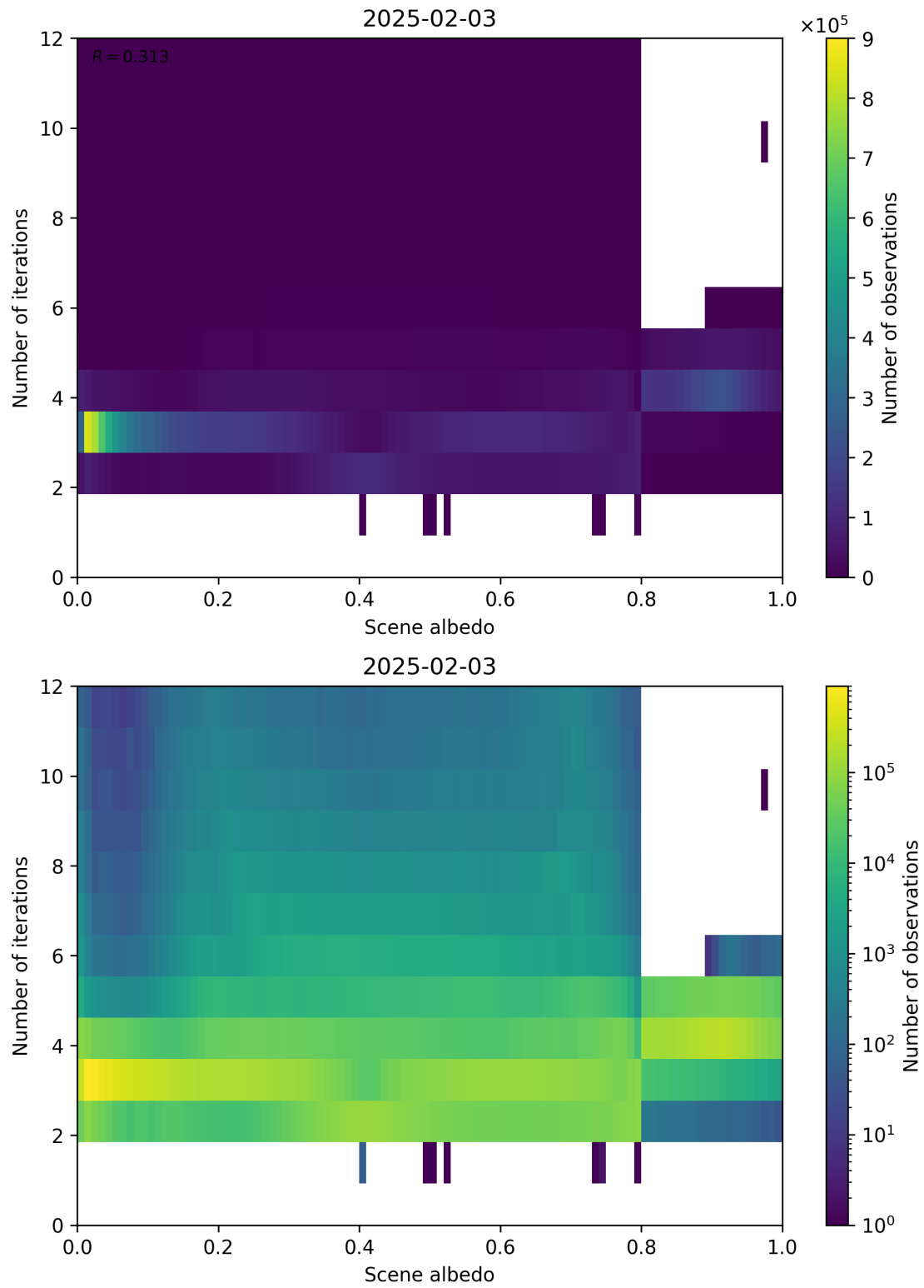
Figure 105: Scatter density plot of “Scene albedo” against “Number of iterations” for 2025-02-03 to 2025-02-04.
