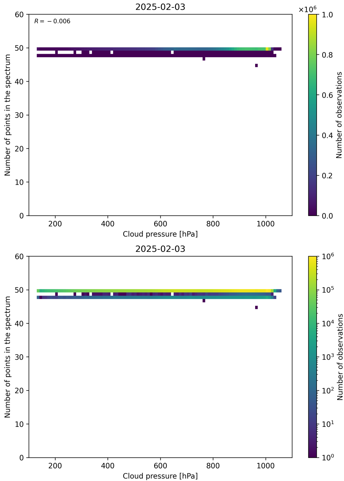
Figure 82: Scatter density plot of “Cloud pressure” against “Number of points in the spectrum” for 2025-02-03 to 2025-02-04.
