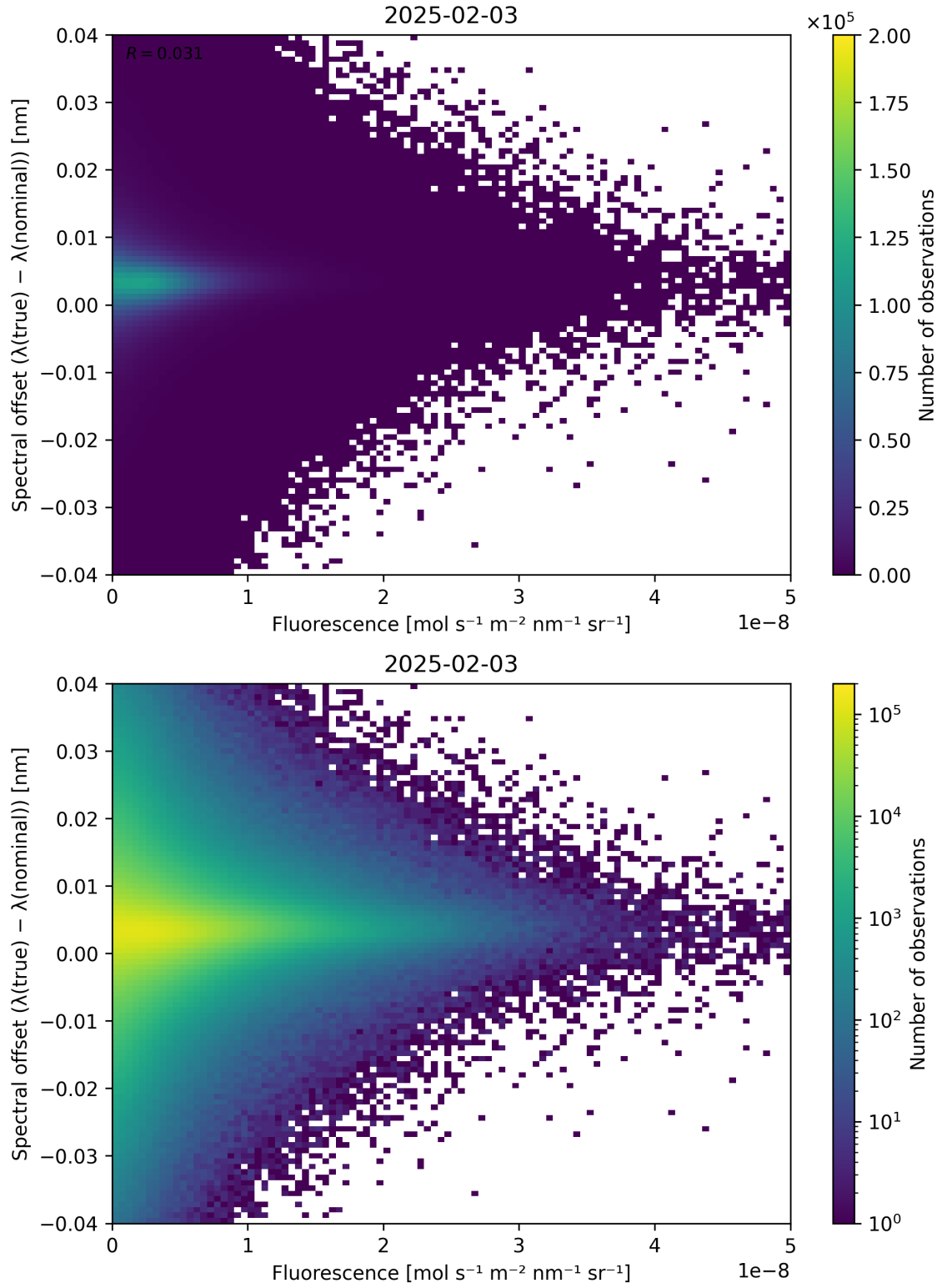
Figure 87: Scatter density plot of “Fluorescence” against “Spectral offset ( \lambda_{\text{true}} - \lambda_{\text{nominal}} )” for 2025-02-03 to 2025-02-04.
