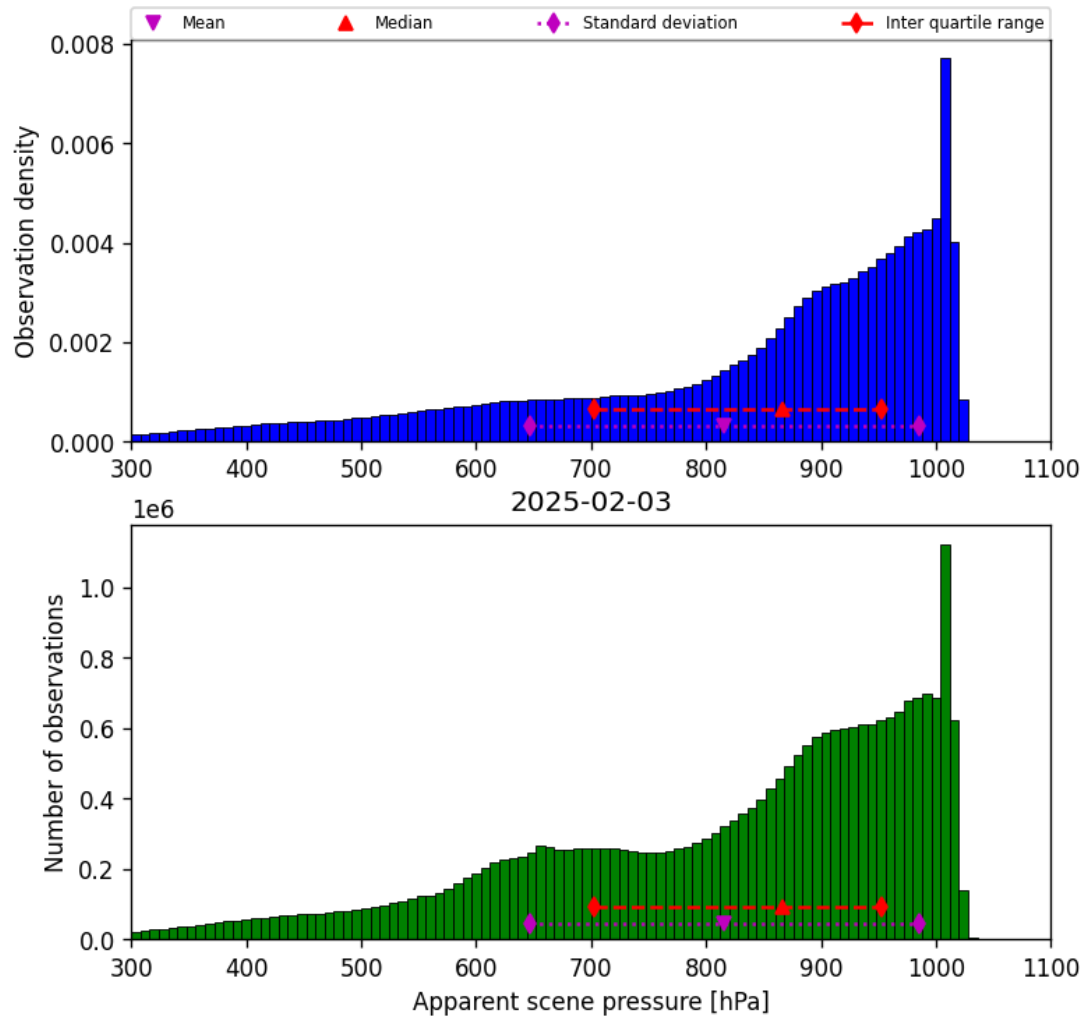
Figure 36: Histogram of “Apparent scene pressure” for 2025-02-03 to 2025-02-04
