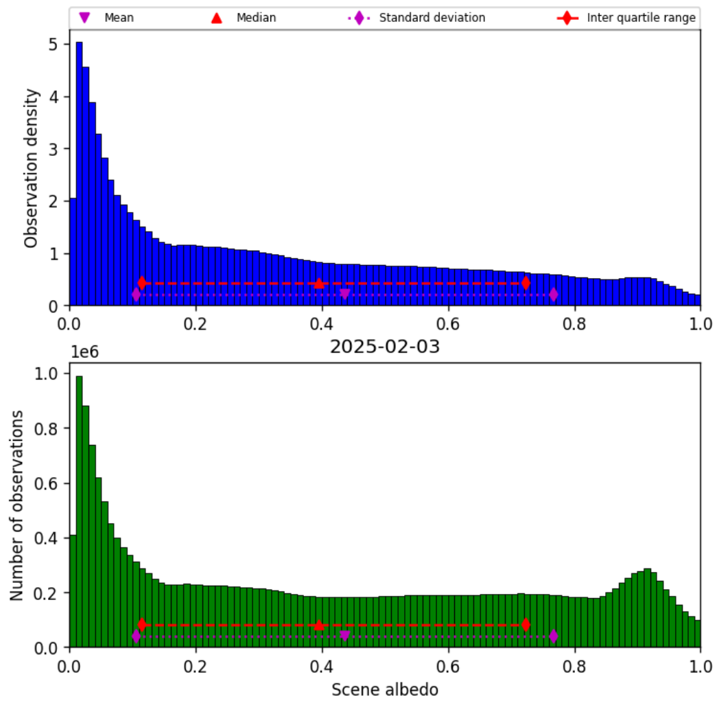
Figure 34: Histogram of “Scene albedo” for 2025-02-03 to 2025-02-04
