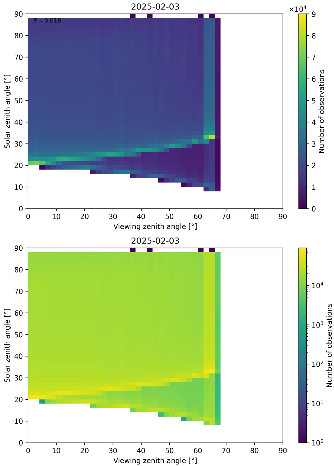
Figure 127: Scatter density plot of “Viewing zenith angle” against “Solar zenith angle” for 2025-02-03 to 2025-02-04.
