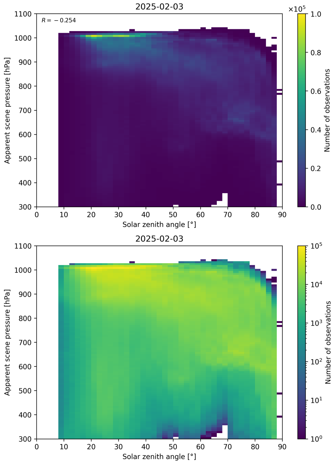
Figure 108: Scatter density plot of “Solar zenith angle” against “Apparent scene pressure” for 2025-02-03 to 2025-02-04.
