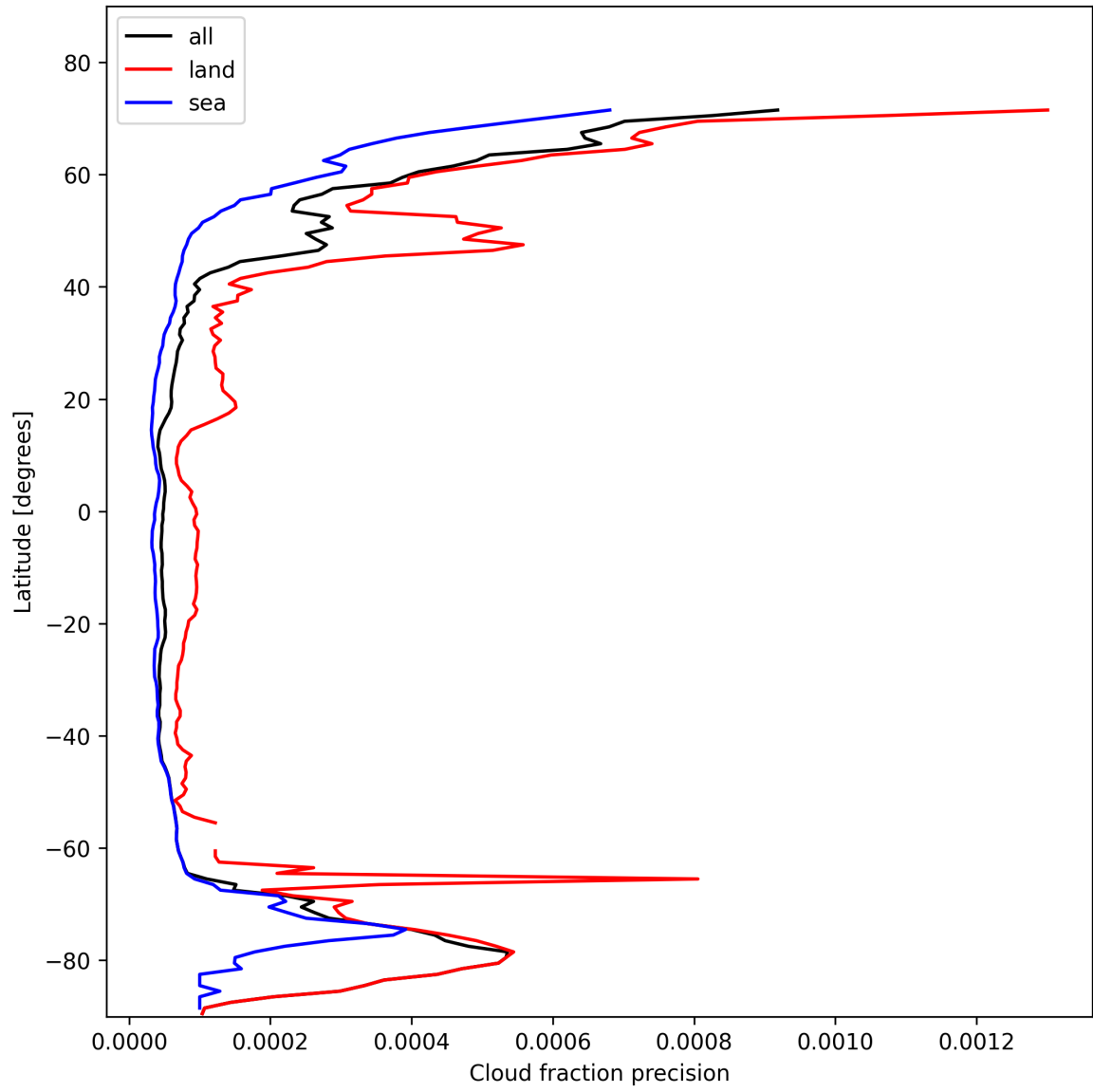
Figure 16: Zonal average of “Cloud fraction precision” for 2025-02-03 to 2025-02-04.
