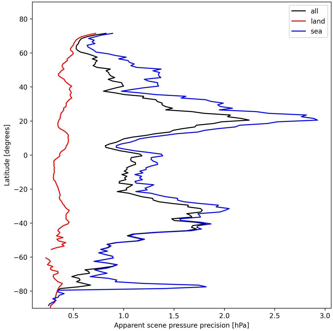
Figure 20: Zonal average of “Apparent scene pressure precision” for 2025-02-03 to 2025-02-04.
