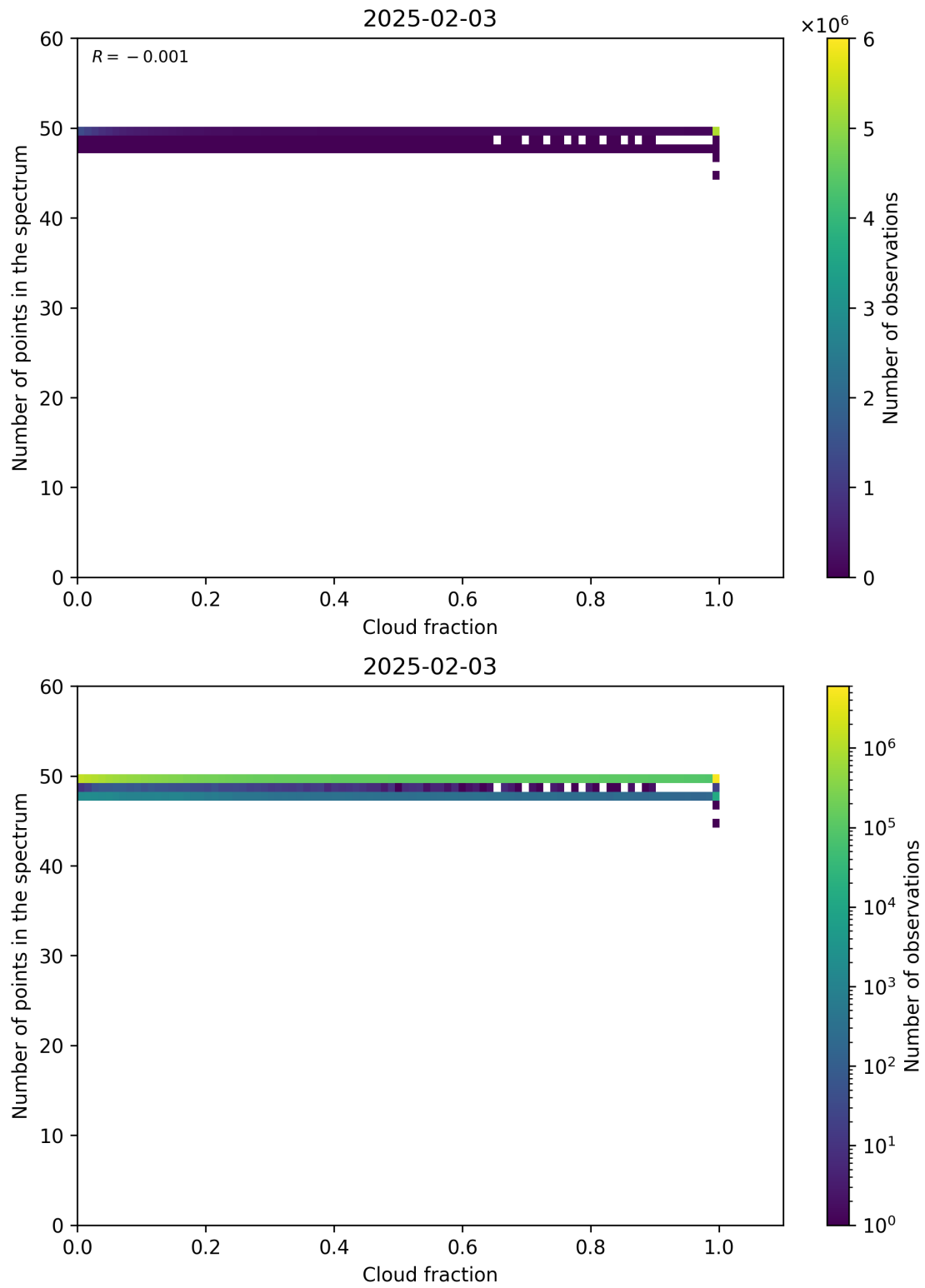
Figure 74: Scatter density plot of “Cloud fraction” against “Number of points in the spectrum” for 2025-02-03 to 2025-02-04.
