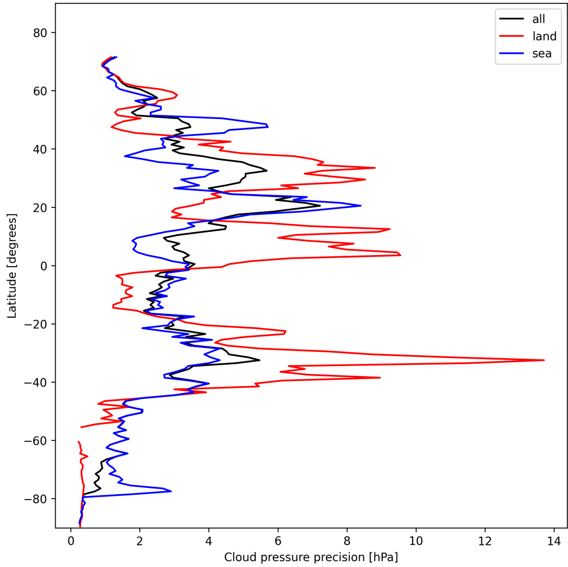
Figure 14: Zonal average of "Cloud pressure precision" for 2025-02-03 to 2025-02-04.
