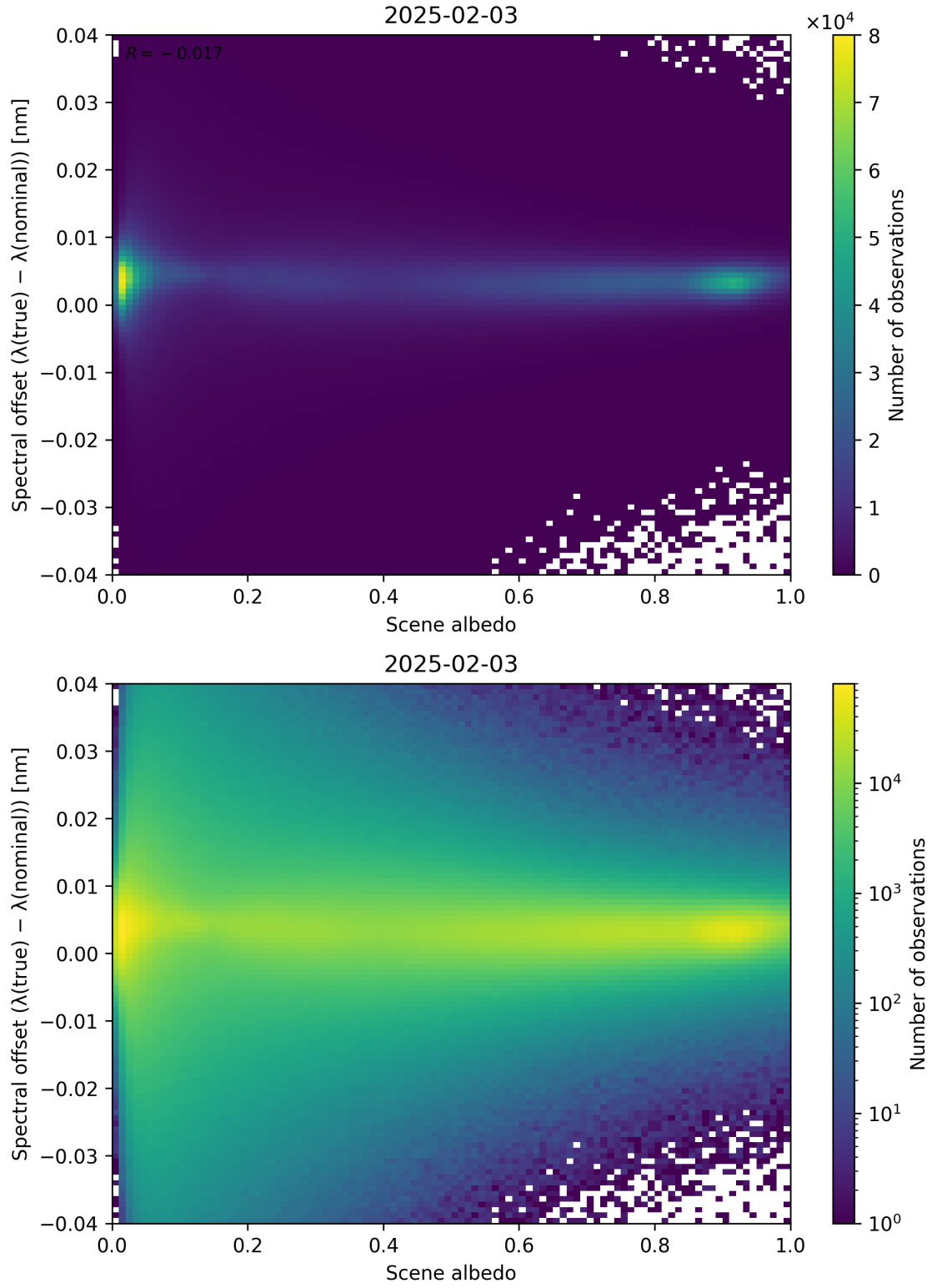
Figure 107: Scatter density plot of “Scene albedo” against “Spectral offset ( \lambda_{\text{true}} - \lambda_{\text{nominal}} )” for 2025-02-03 to 2025-02-04.
