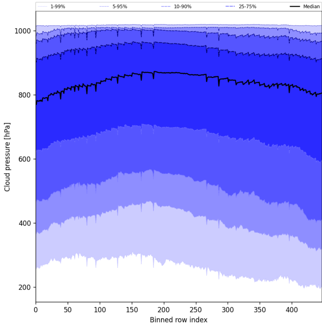
Figure 47: Along track statistics of “Cloud pressure” for 2025-02-03 to 2025-02-04
