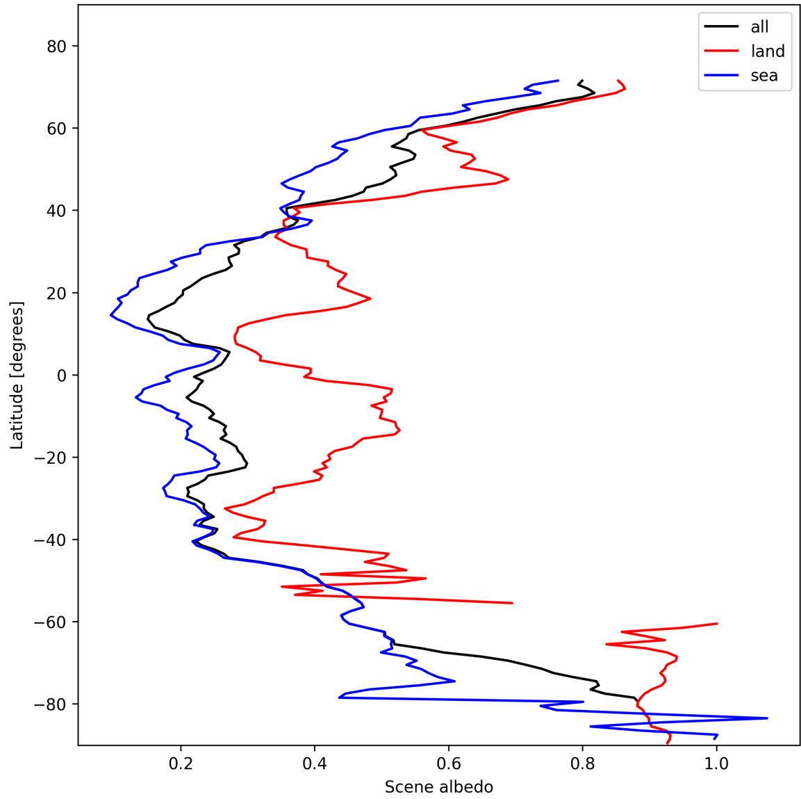
Figure 17: Zonal average of “Scene albedo” for 2025-02-03 to 2025-02-04.
