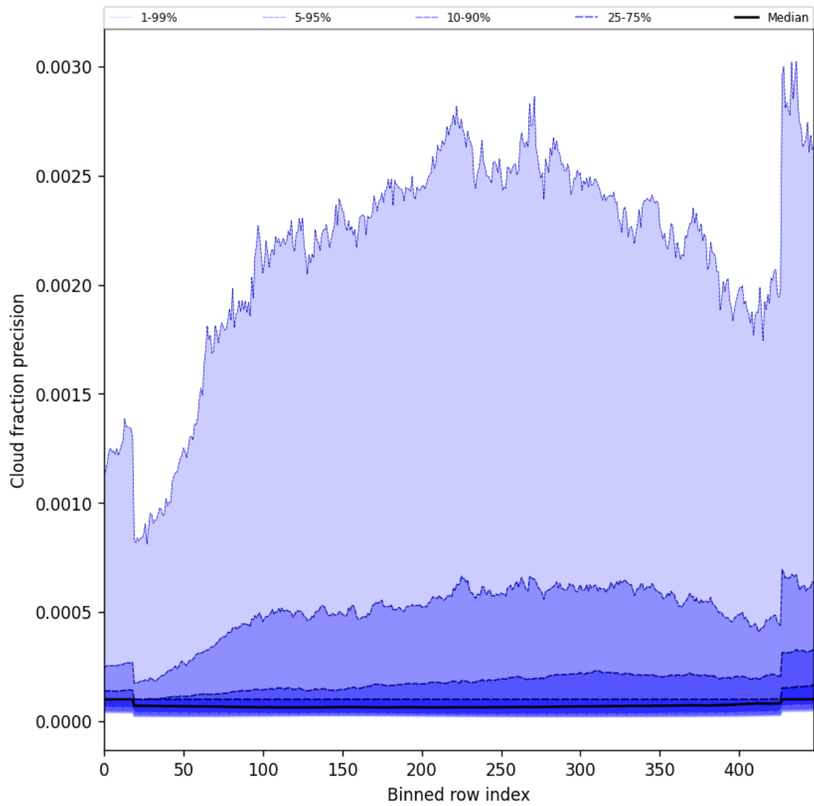
Figure 50: Along track statistics of “Cloud fraction precision” for 2025-02-03 to 2025-02-04
