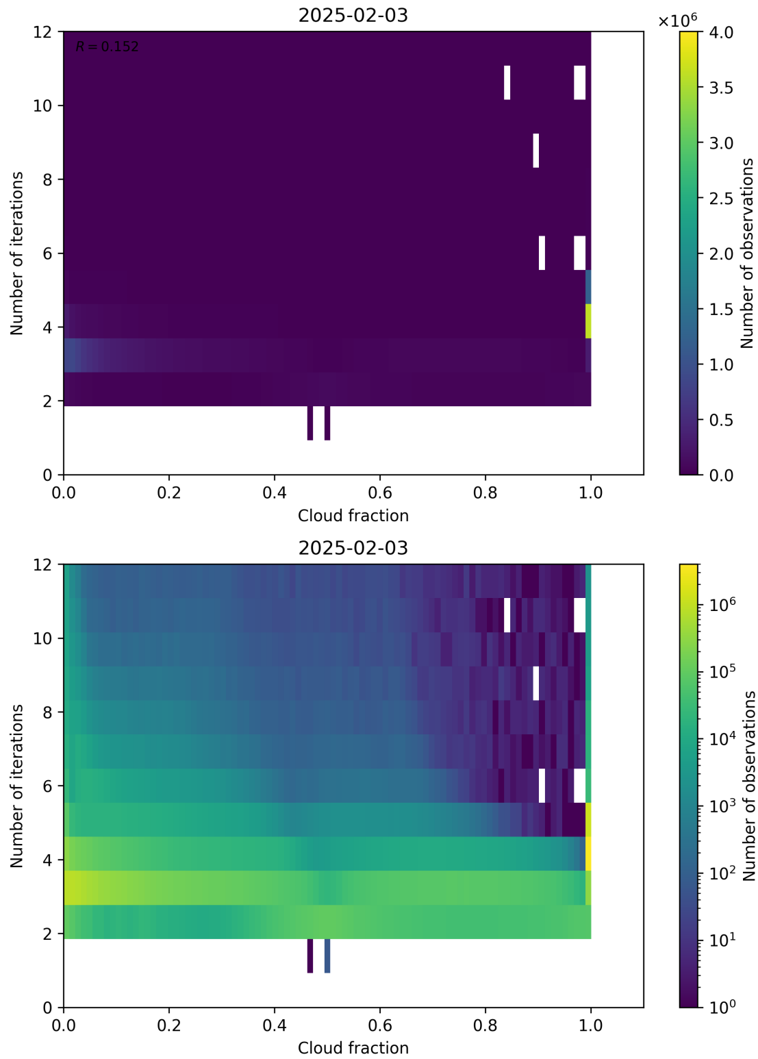
Figure 73: Scatter density plot of “Cloud fraction” against “Number of iterations” for 2025-02-03 to 2025-02-04.
