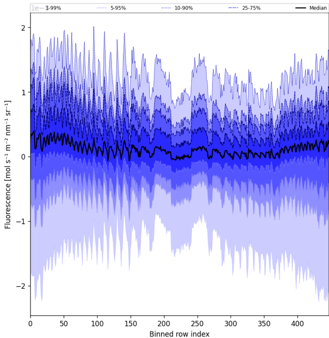
Figure 57: Along track statistics of “Fluorescence” for 2025-02-03 to 2025-02-04
