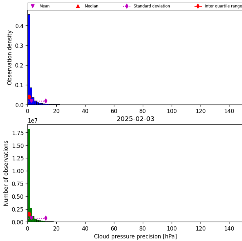
Figure 31: Histogram of “Cloud pressure precision” for 2025-02-03 to 2025-02-04
