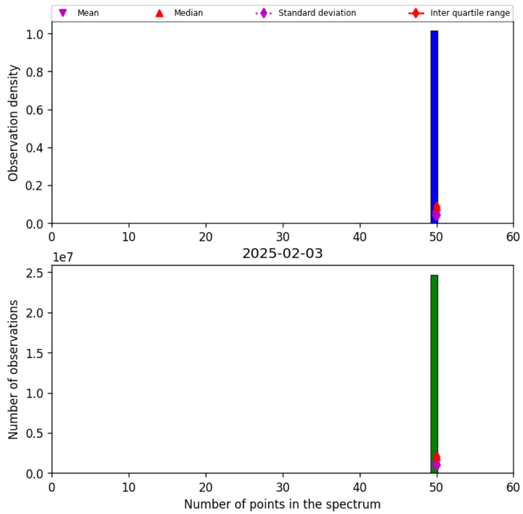
Figure 44: Histogram of “Number of points in the spectrum” for 2025-02-03 to 2025-02-04
