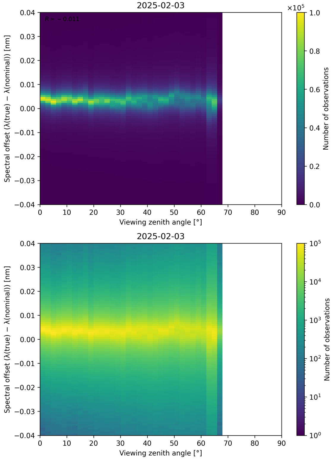
Figure 128: Scatter density plot of “Viewing zenith angle” against “Spectral offset ( \lambda_{\text{true}} - \lambda_{\text{nominal}} )” for 2025-02-03 to 2025-02-04.
