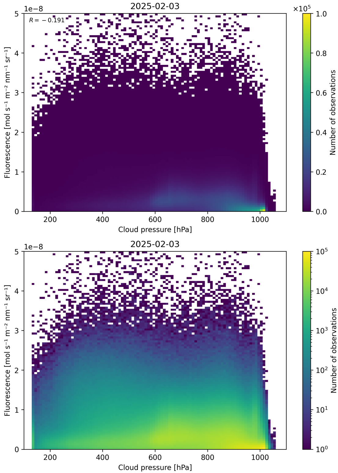
Figure 80: Scatter density plot of “Cloud pressure” against “Fluorescence” for 2025-02-03 to 2025-02-04.
