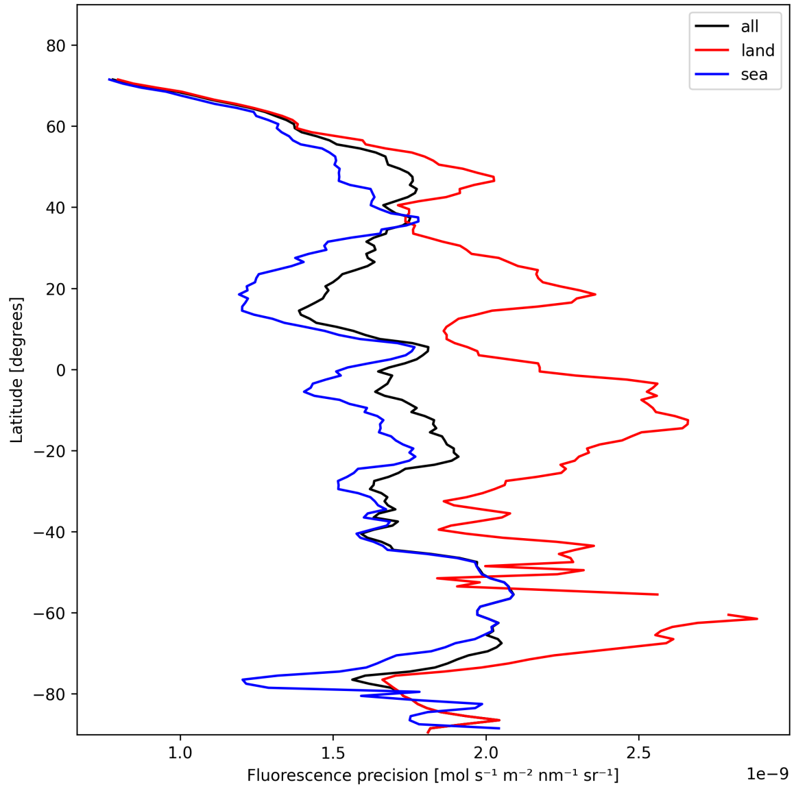
Figure 24: Zonal average of “Fluorescence precision” for 2025-02-03 to 2025-02-04.
