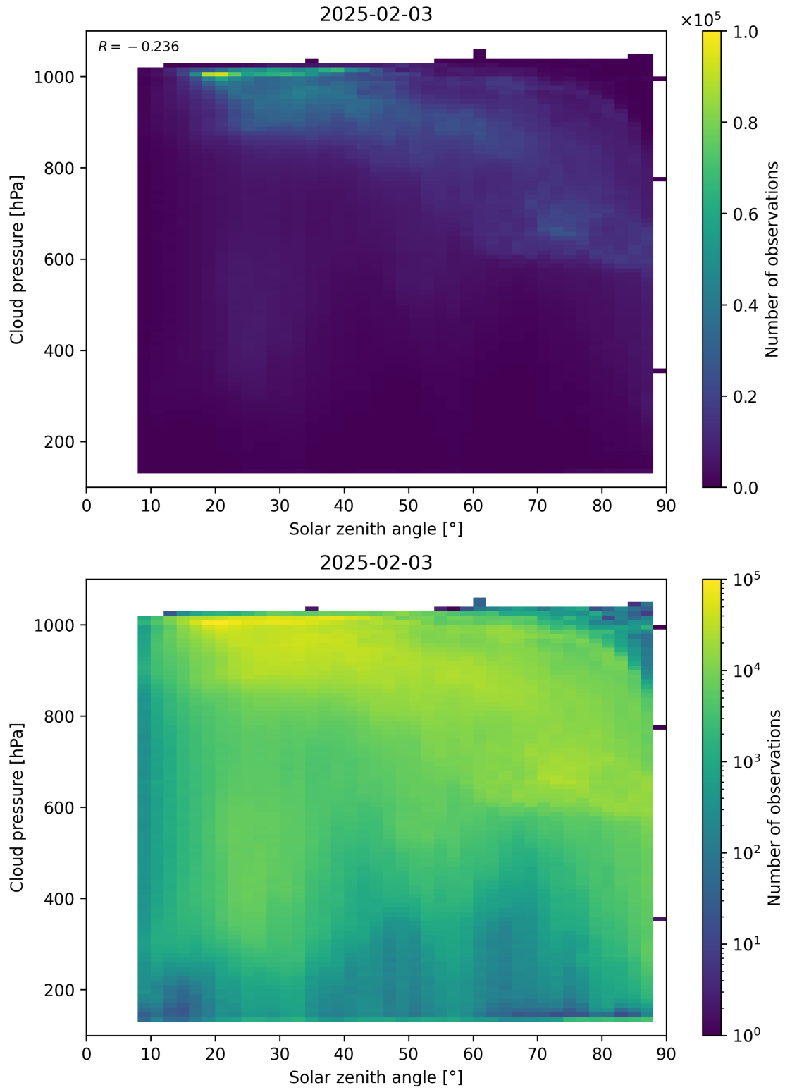
Figure 111: Scatter density plot of “Solar zenith angle” against “Cloud pressure” for 2025-02-03 to 2025-02-04.
