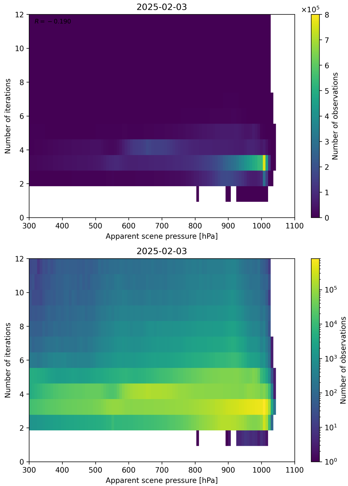
Figure 65: Scatter density plot of “Apparent scene pressure” against “Number of iterations” for 2025-02-03 to 2025-02-04.
