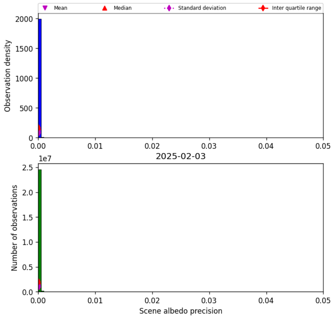
Figure 35: Histogram of “Scene albedo precision” for 2025-02-03 to 2025-02-04
