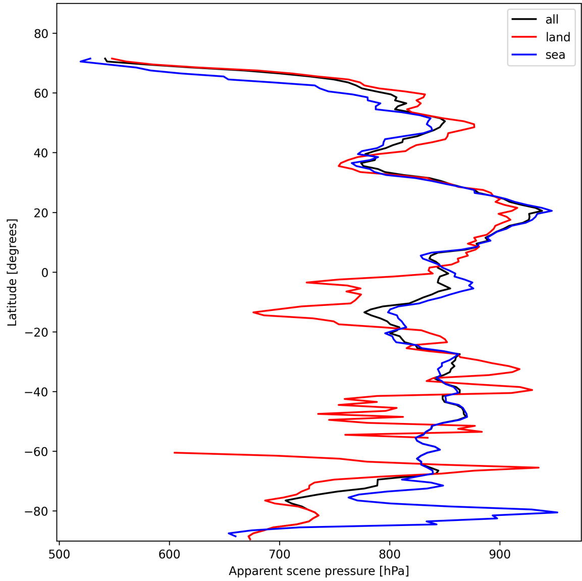
Figure 19: Zonal average of “Apparent scene pressure” for 2025-02-03 to 2025-02-04.
