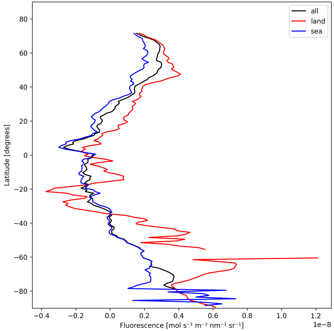
Figure 23: Zonal average of “Fluorescence” for 2025-02-03 to 2025-02-04.
