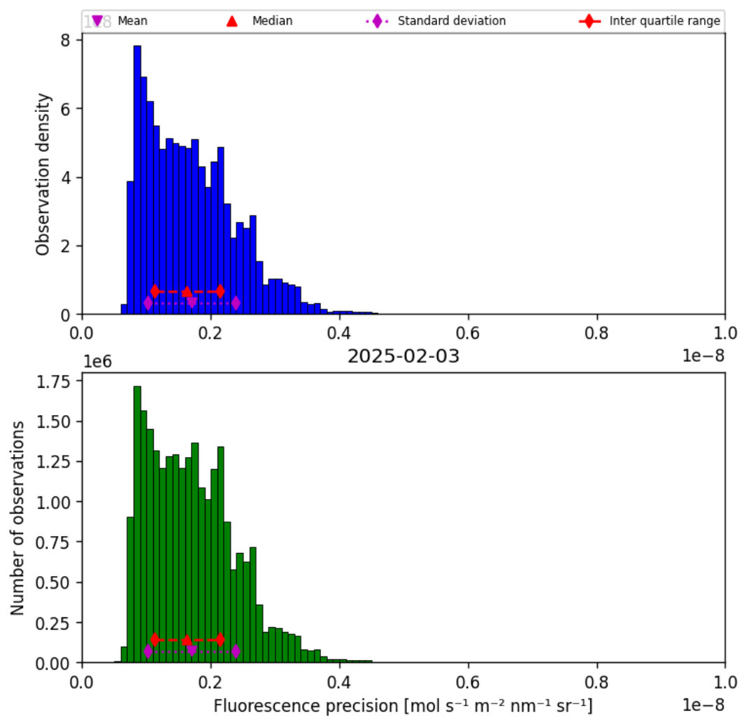
Figure 41: Histogram of “Fluorescence precision” for 2025-02-03 to 2025-02-04
