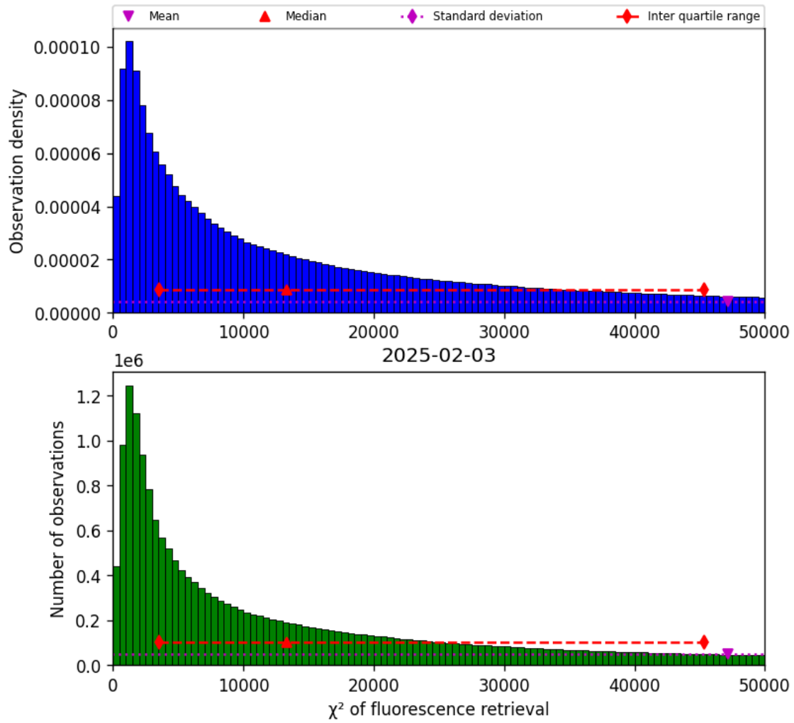
Figure 42: Histogram of “ \chi^2 of fluorescence retrieval” for 2025-02-03 to 2025-02-04
