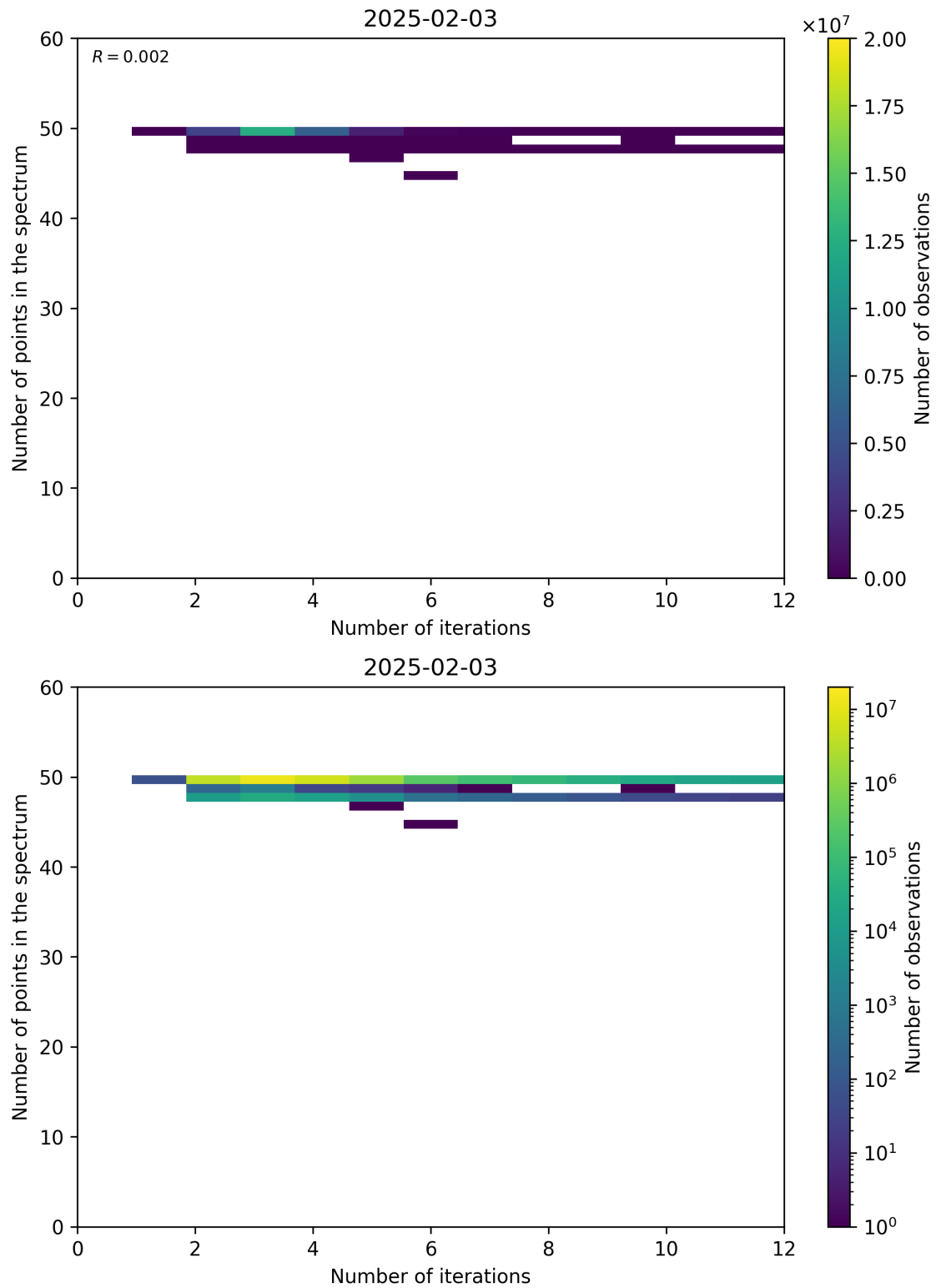
Figure 99: Scatter density plot of “Number of iterations” against “Number of points in the spectrum” for 2025-02-03 to 2025-02-04.
