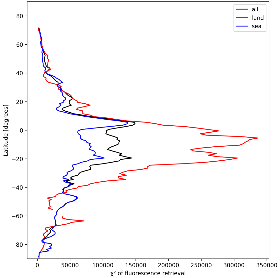
Figure 25: Zonal average of “ \chi^2 of fluorescence retrieval” for 2025-02-03 to 2025-02-04.
