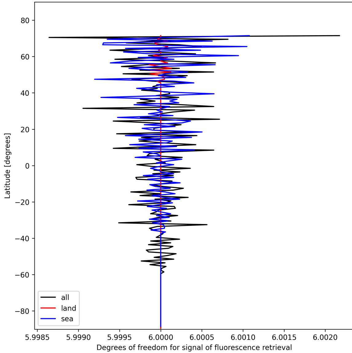
Figure 26: Zonal average of “Degrees of freedom for signal of fluorescence retrieval” for 2025-02-03 to 2025-02-04.
