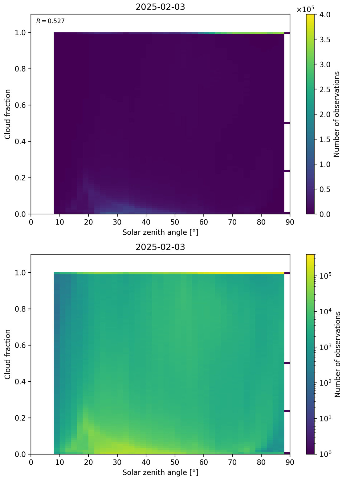
Figure 110: Scatter density plot of “Solar zenith angle” against “Cloud fraction” for 2025-02-03 to 2025-02-04.
