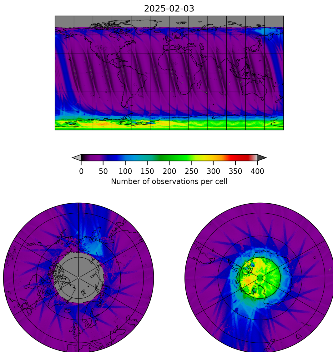
Figure 11: Map of the number of observations for 2025-02-03 to 2025-02-04
