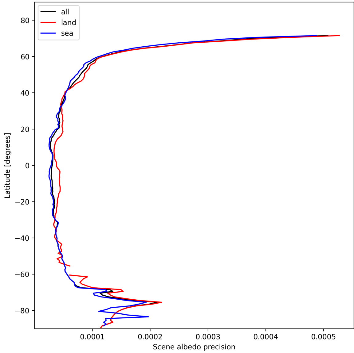
Figure 18: Zonal average of “Scene albedo precision” for 2025-02-03 to 2025-02-04.
