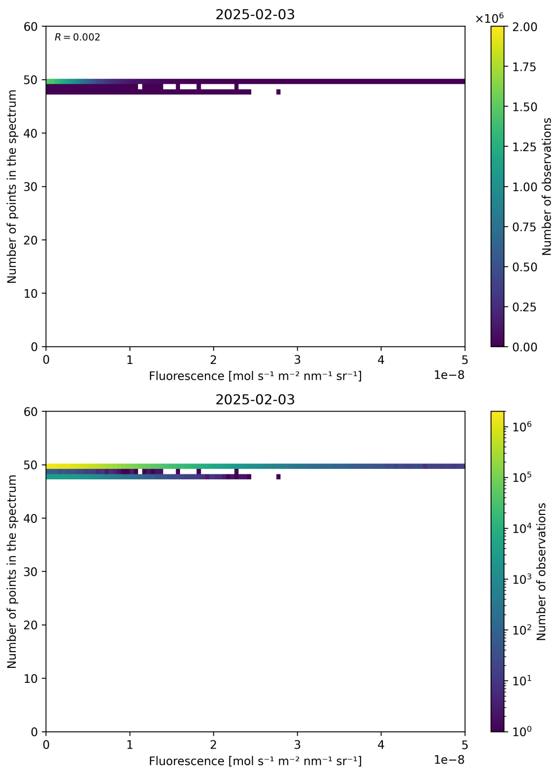
Figure 86: Scatter density plot of “Fluorescence” against “Number of points in the spectrum” for 2025-02-03 to 2025-02-04.
