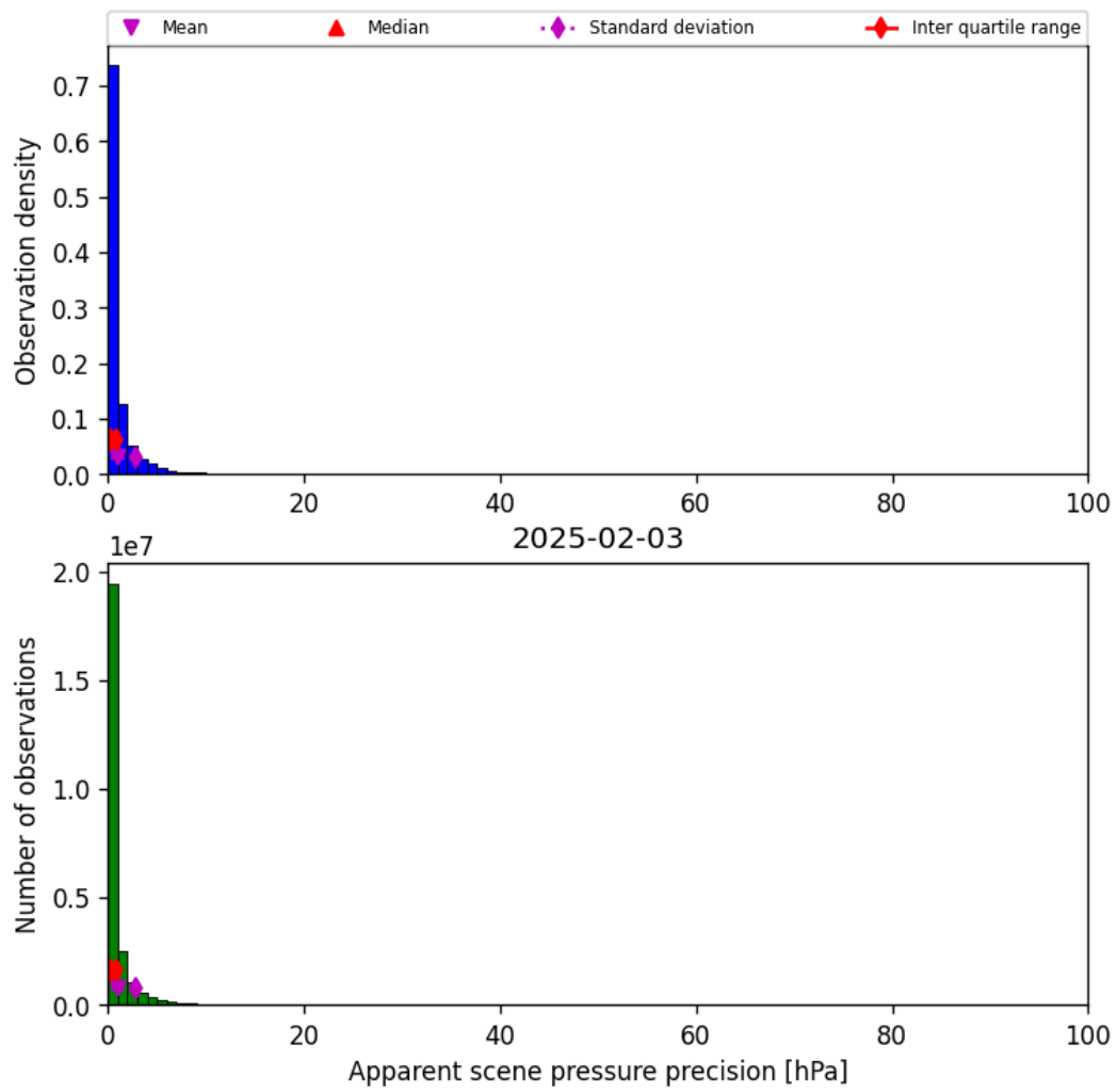
Figure 37: Histogram of “Apparent scene pressure precision” for 2025-02-03 to 2025-02-04
