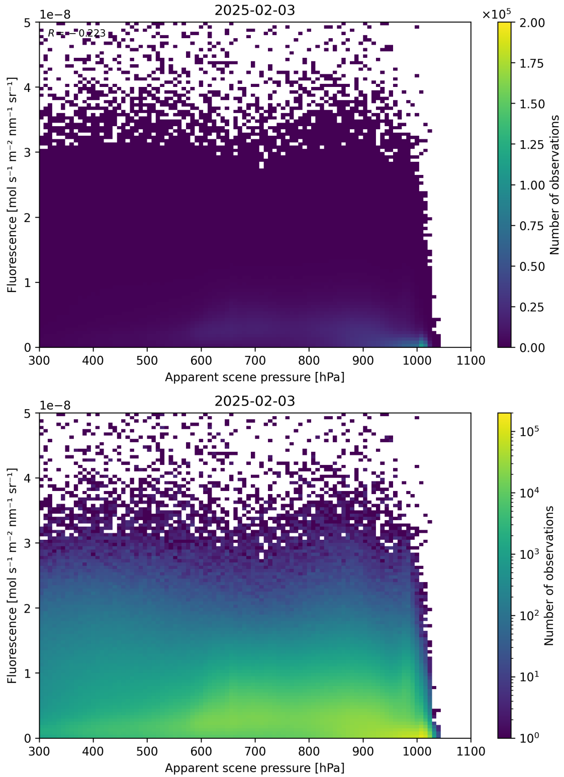
Figure 64: Scatter density plot of “Apparent scene pressure” against “Fluorescence” for 2025-02-03 to 2025-02-04.
