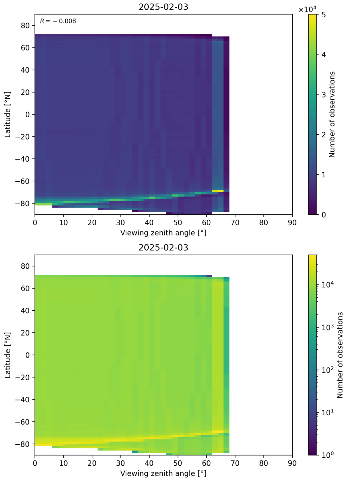
Figure 123: Scatter density plot of “Viewing zenith angle” against “Latitude” for 2025-02-03 to 2025-02-04.
