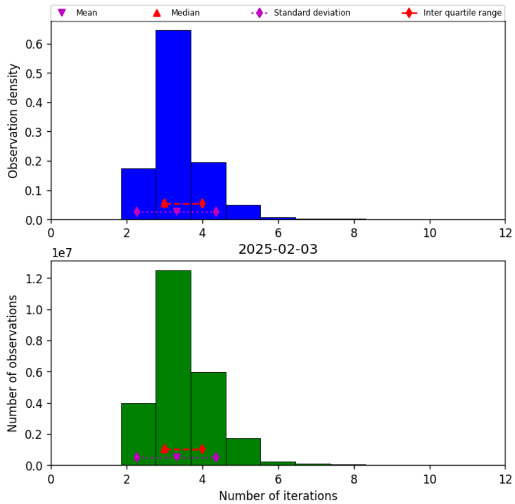
Figure 39: Histogram of “Number of iterations” for 2025-02-03 to 2025-02-04
