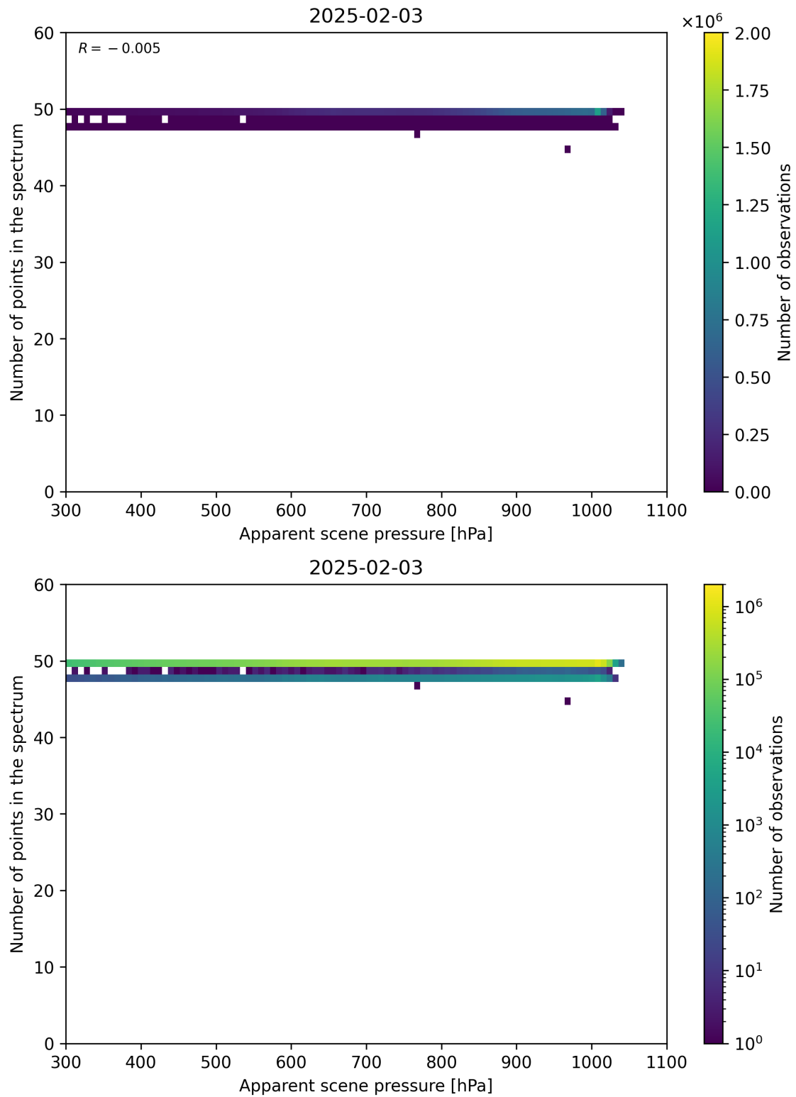
Figure 66: Scatter density plot of “Apparent scene pressure” against “Number of points in the spectrum” for 2025-02-03 to 2025-02-04.
