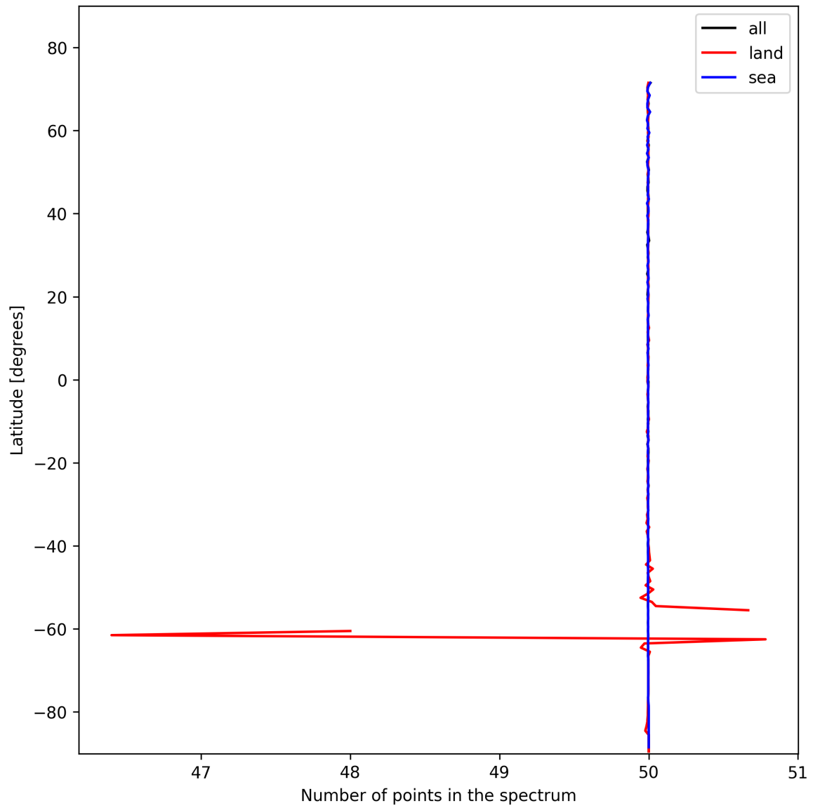
Figure 27: Zonal average of “Number of points in the spectrum” for 2025-02-03 to 2025-02-04.
