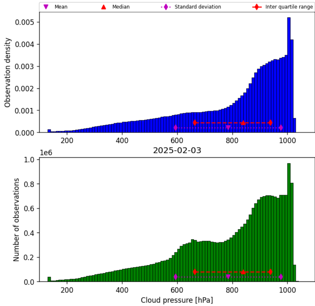
Figure 30: Histogram of “Cloud pressure” for 2025-02-03 to 2025-02-04
