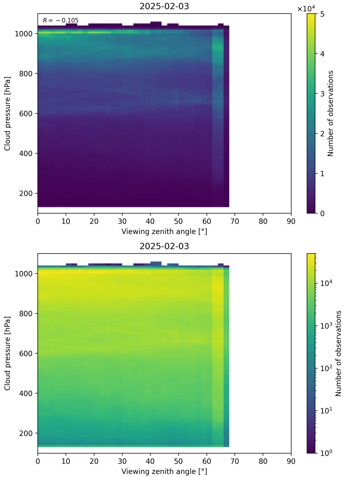
Figure 121: Scatter density plot of “Viewing zenith angle” against “Cloud pressure” for 2025-02-03 to 2025-02-04.
