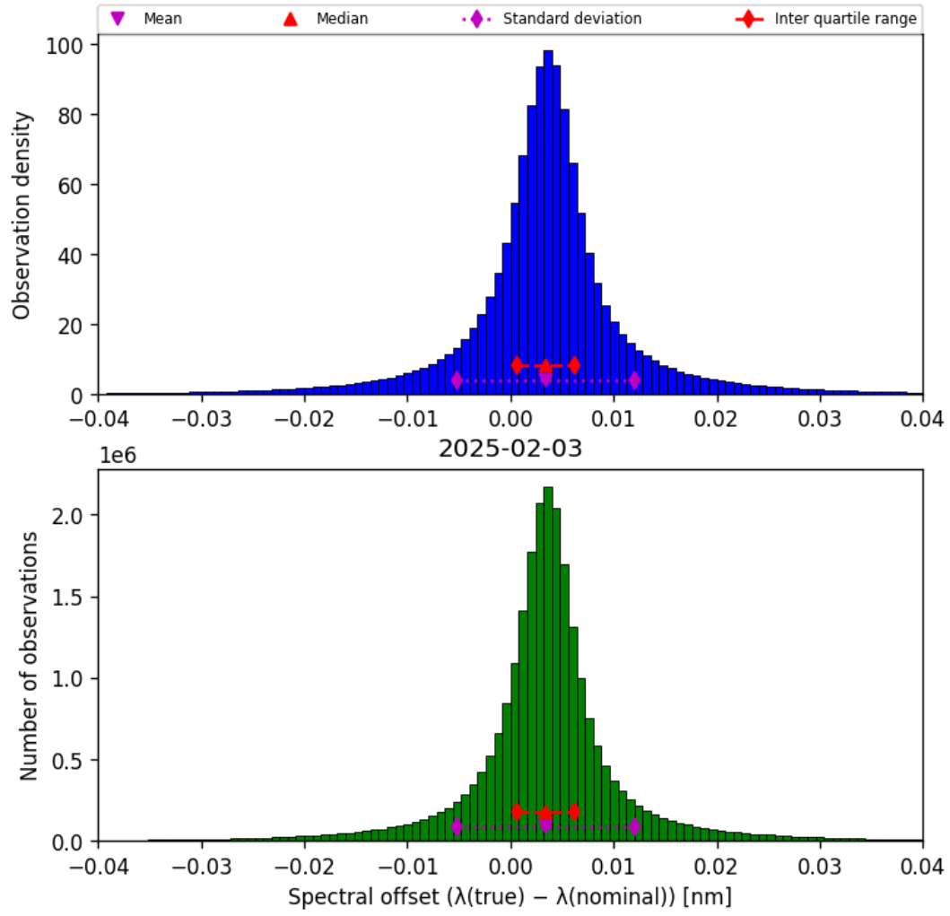
Figure 45: Histogram of “Spectral offset ( \lambda_{\text{true}} - \lambda_{\text{nominal}} )” for 2025-02-03 to 2025-02-04
