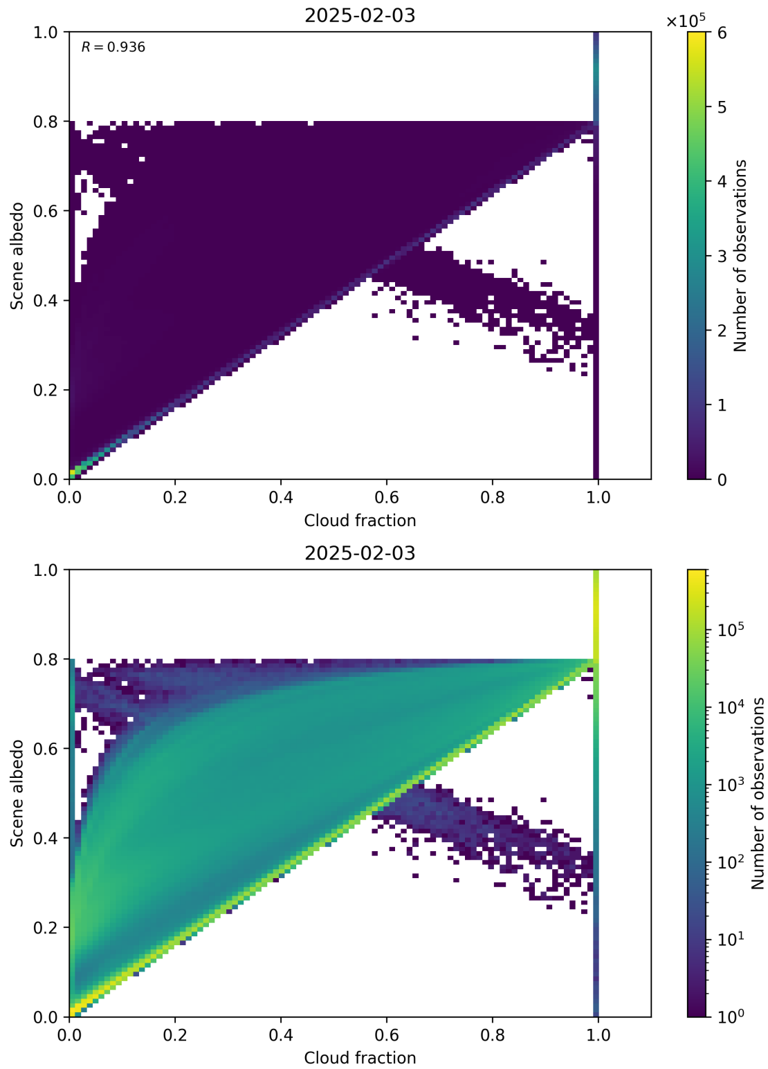
Figure 75: Scatter density plot of “Cloud fraction” against “Scene albedo” for 2025-02-03 to 2025-02-04.
