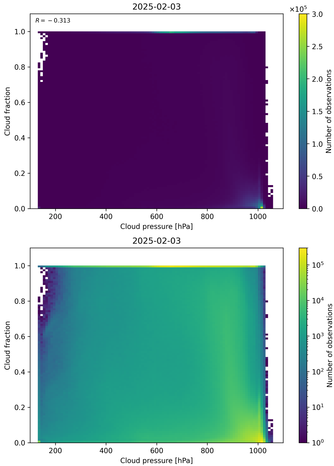
Figure 79: Scatter density plot of “Cloud pressure” against “Cloud fraction” for 2025-02-03 to 2025-02-04.
