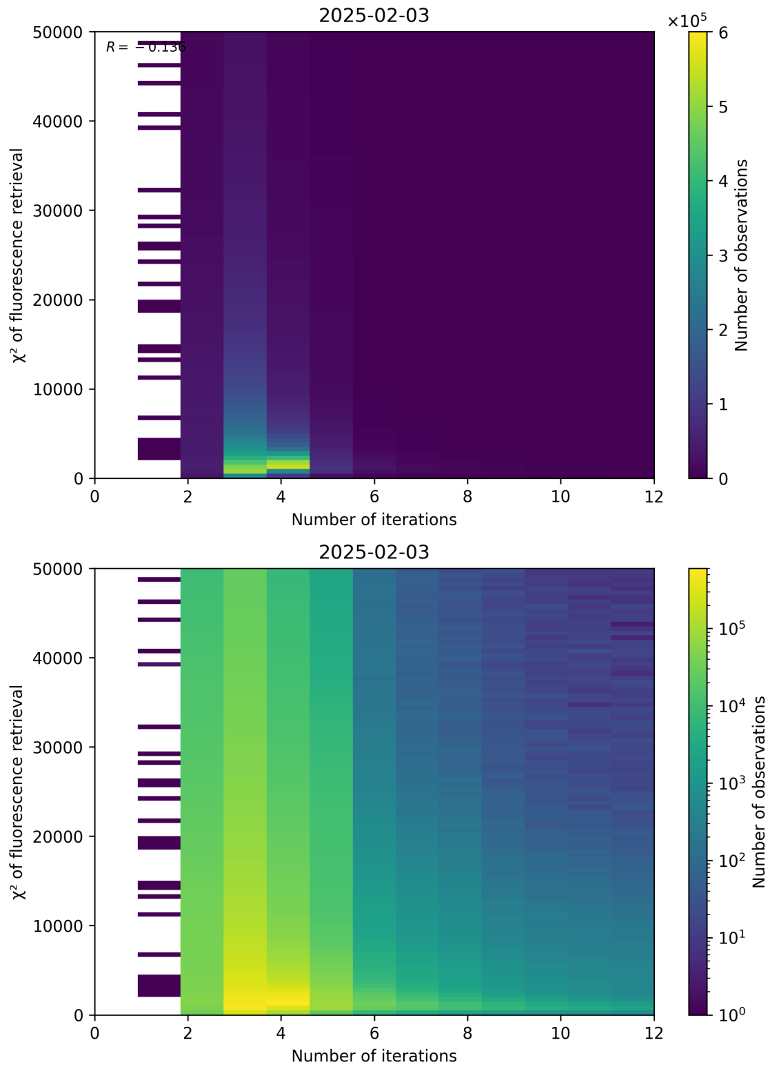
Figure 97: Scatter density plot of “Number of iterations” against “ \chi^2 of fluorescence retrieval” for 2025-02-03 to 2025-02-04.
