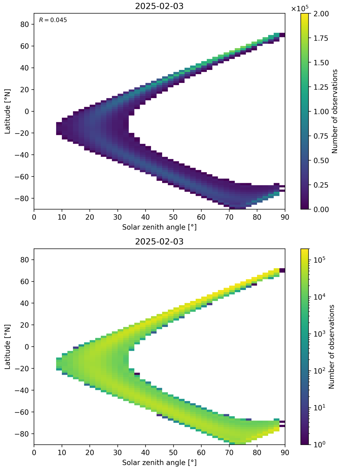
Figure 113: Scatter density plot of “Solar zenith angle” against “Latitude” for 2025-02-03 to 2025-02-04.
