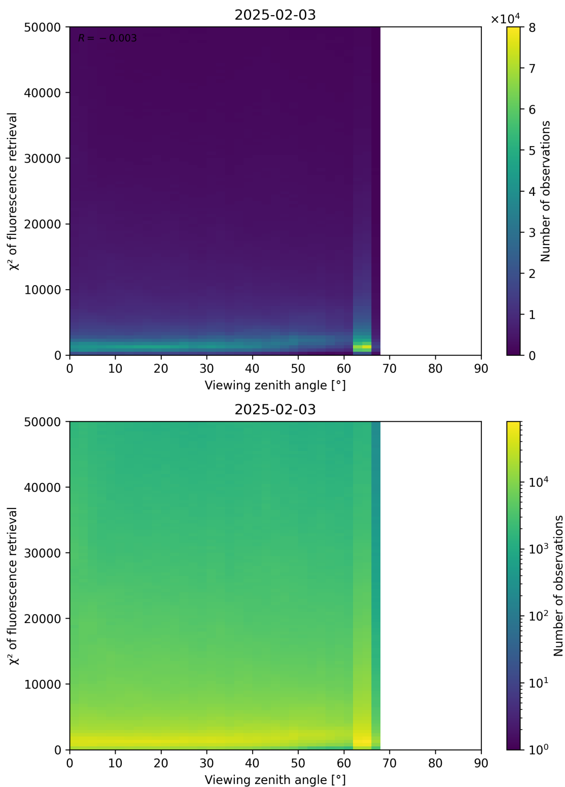
Figure 119: Scatter density plot of “Viewing zenith angle” against “ \chi^2 of fluorescence retrieval” for 2025-02-03 to 2025-02-04.
