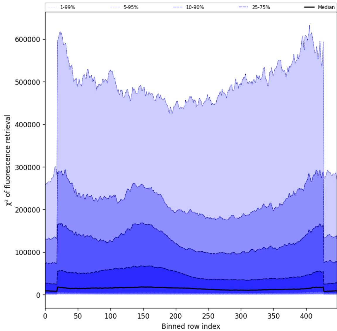
Figure 59: Along track statistics of “ \chi^2 of fluorescence retrieval” for 2025-02-03 to 2025-02-04
