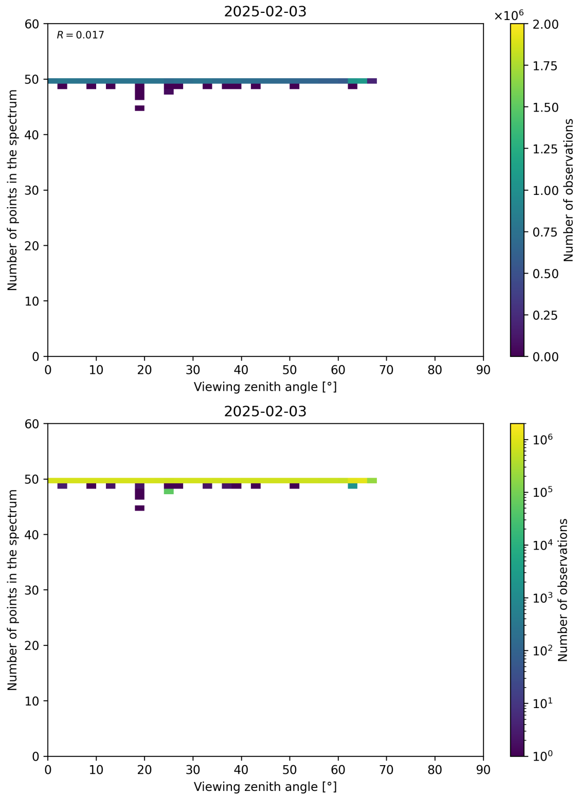
Figure 125: Scatter density plot of “Viewing zenith angle” against “Number of points in the spectrum” for 2025-02-03 to 2025-02-04.
