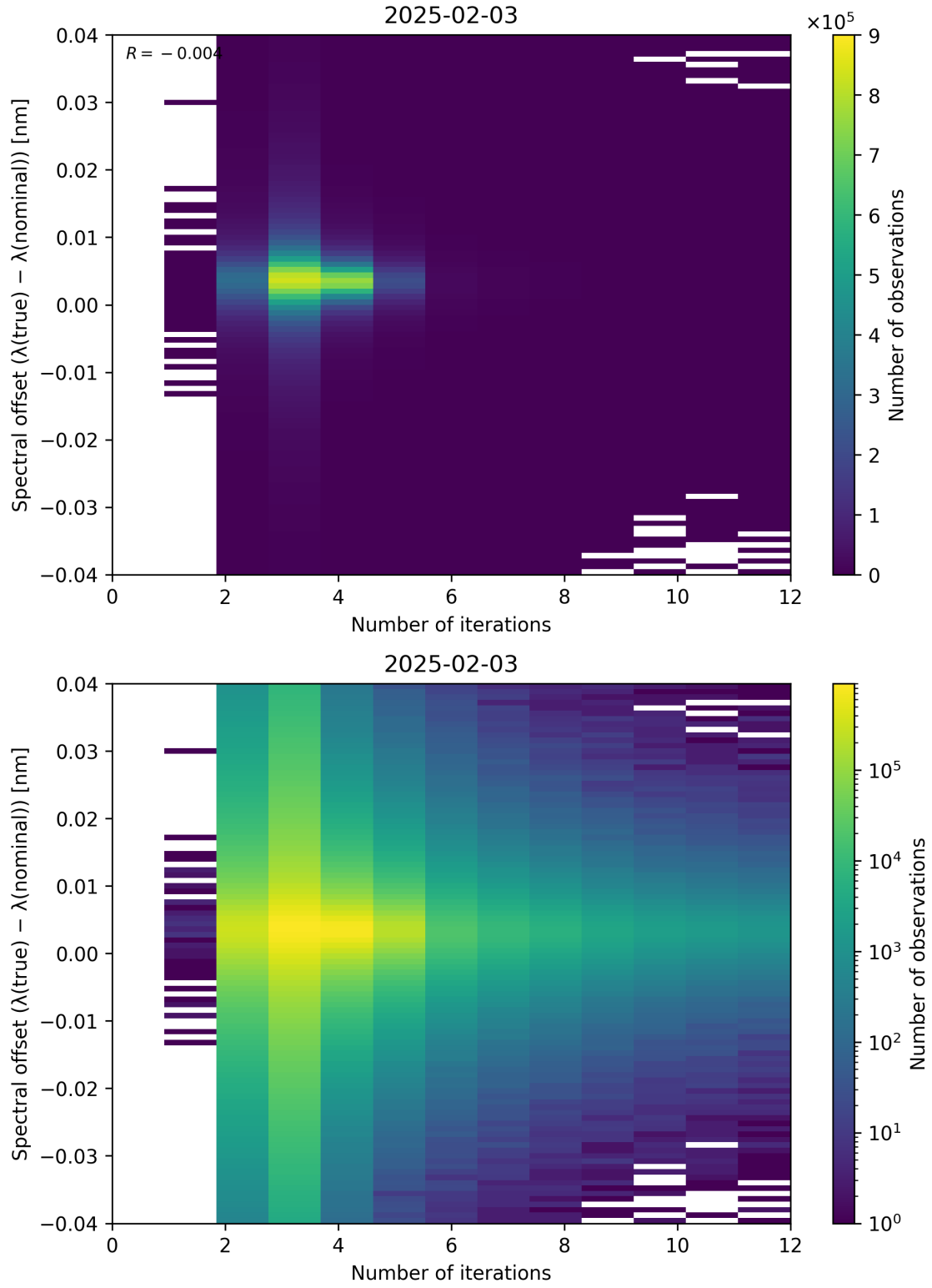
Figure 100: Scatter density plot of “Number of iterations” against “Spectral offset ( \lambda_{\text{true}} - \lambda_{\text{nominal}} )” for 2025-02-03 to 2025-02-04.
