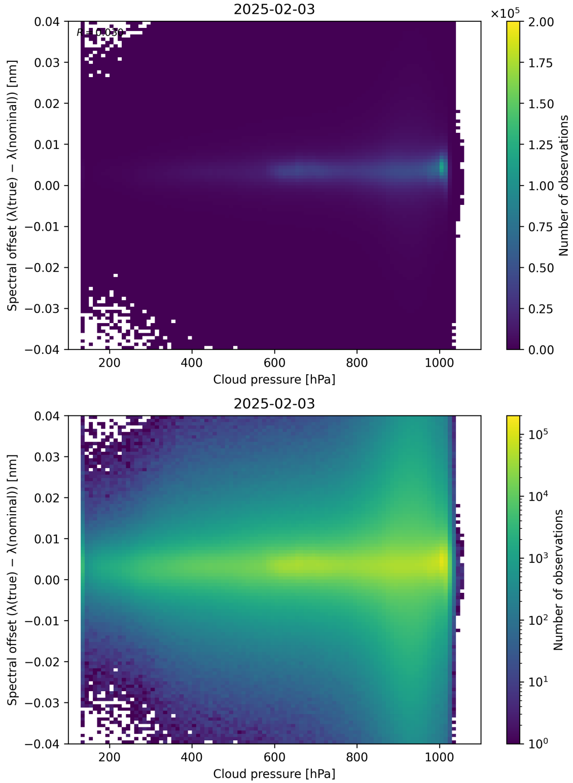
Figure 84: Scatter density plot of “Cloud pressure” against “Spectral offset ( \lambda_{\text{true}} - \lambda_{\text{nominal}} )” for 2025-02-03 to 2025-02-04.
