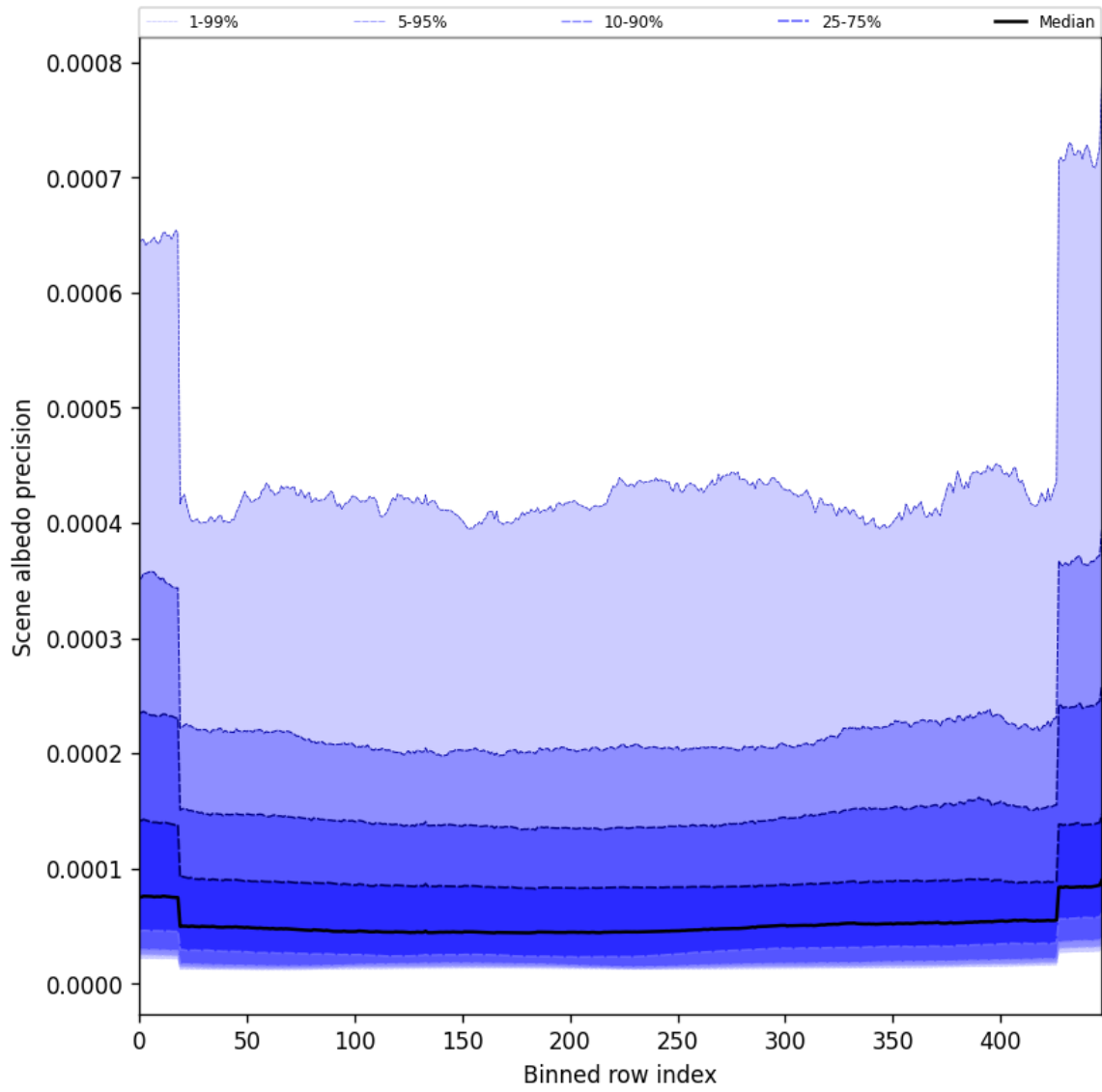
Figure 52: Along track statistics of “Scene albedo precision” for 2025-02-03 to 2025-02-04
