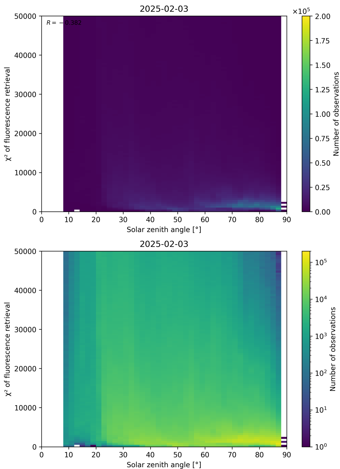
Figure 109: Scatter density plot of “Solar zenith angle” against “ \chi^2 of fluorescence retrieval” for 2025-02-03 to 2025-02-04.
