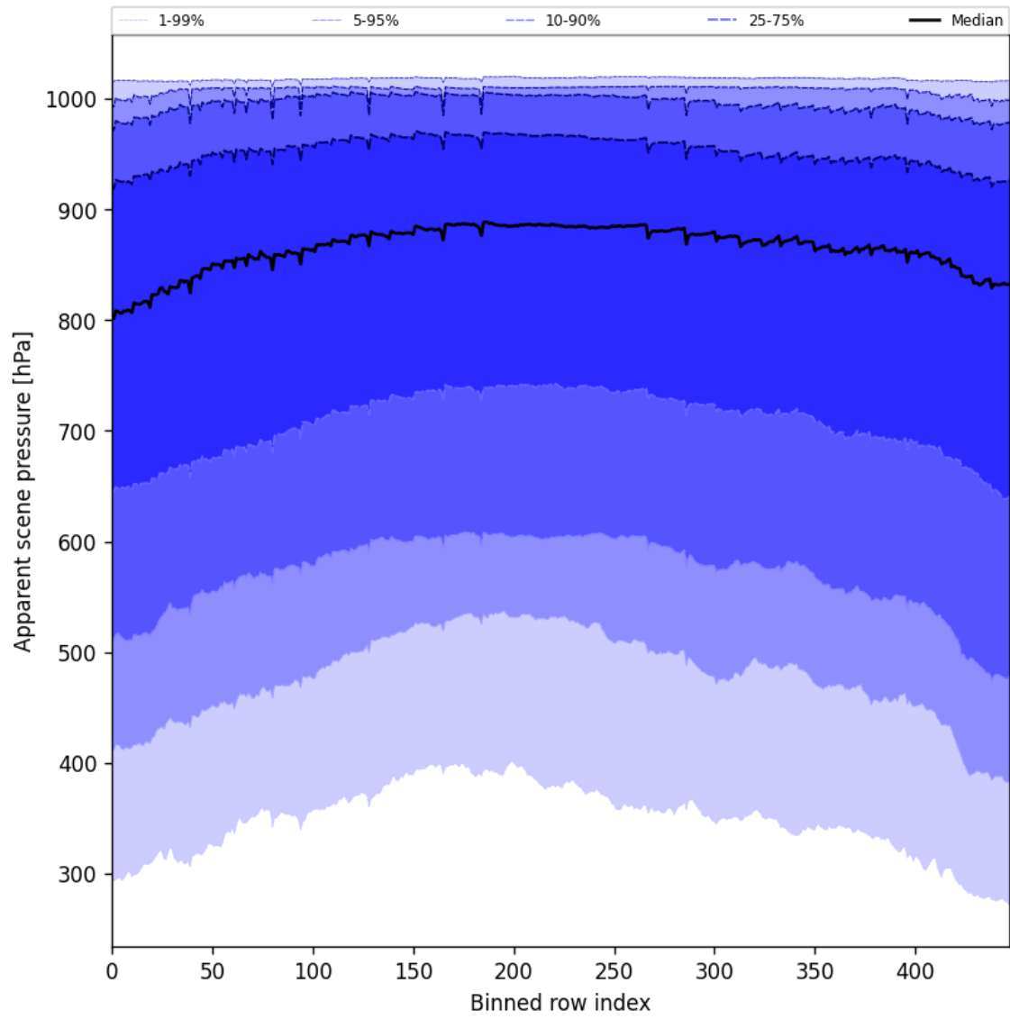
Figure 53: Along track statistics of “Apparent scene pressure” for 2025-02-03 to 2025-02-04
