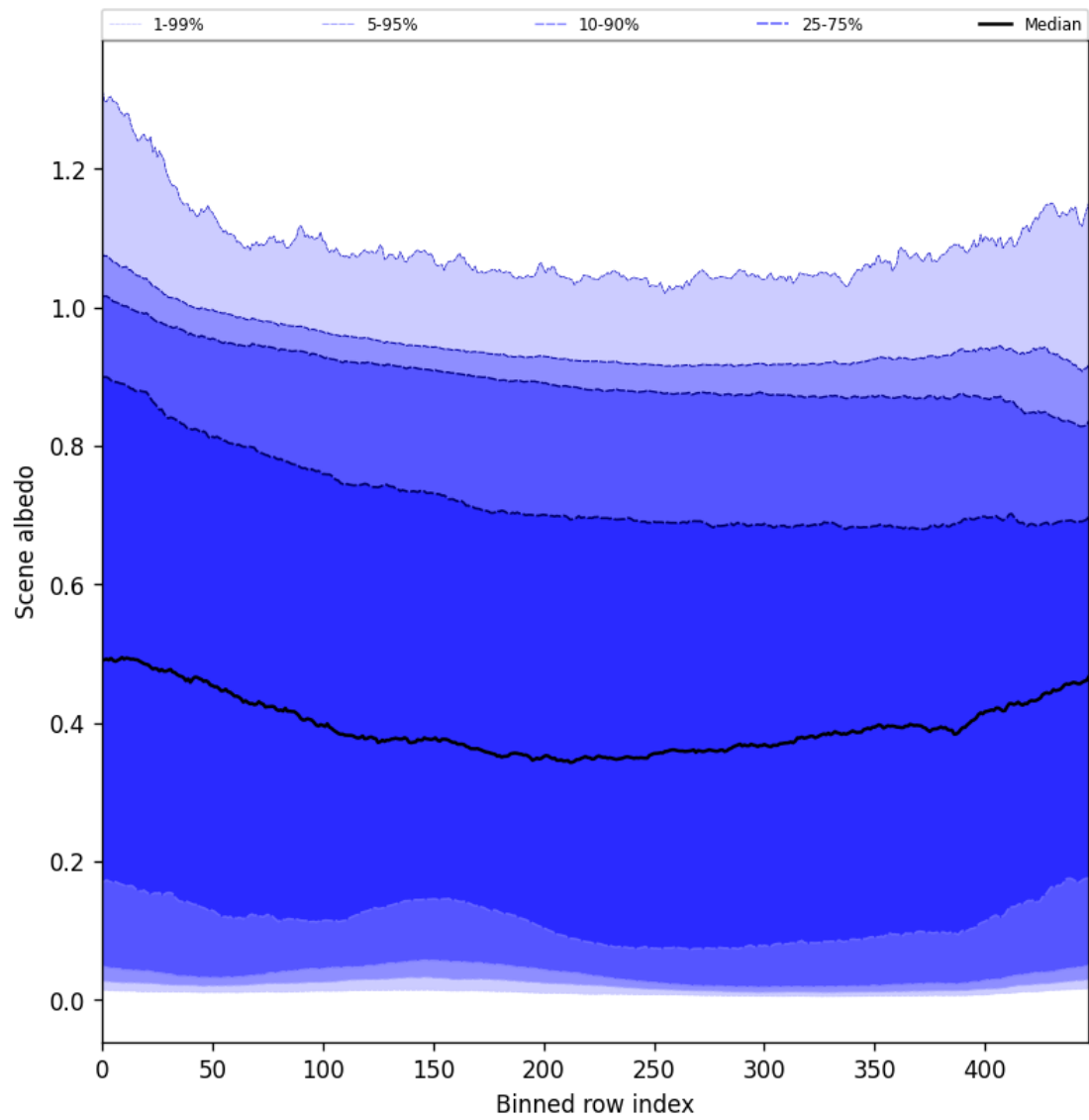
Figure 51: Along track statistics of "Scene albedo" for 2025-02-03 to 2025-02-04
