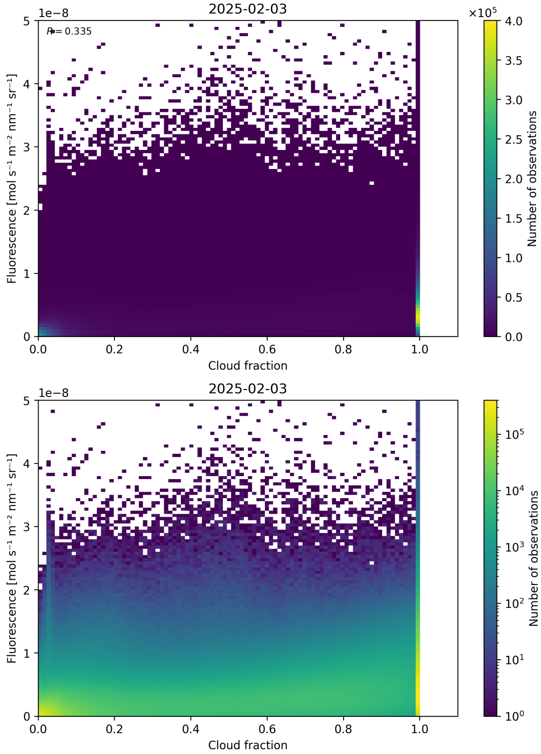
Figure 72: Scatter density plot of “Cloud fraction” against “Fluorescence” for 2025-02-03 to 2025-02-04.
