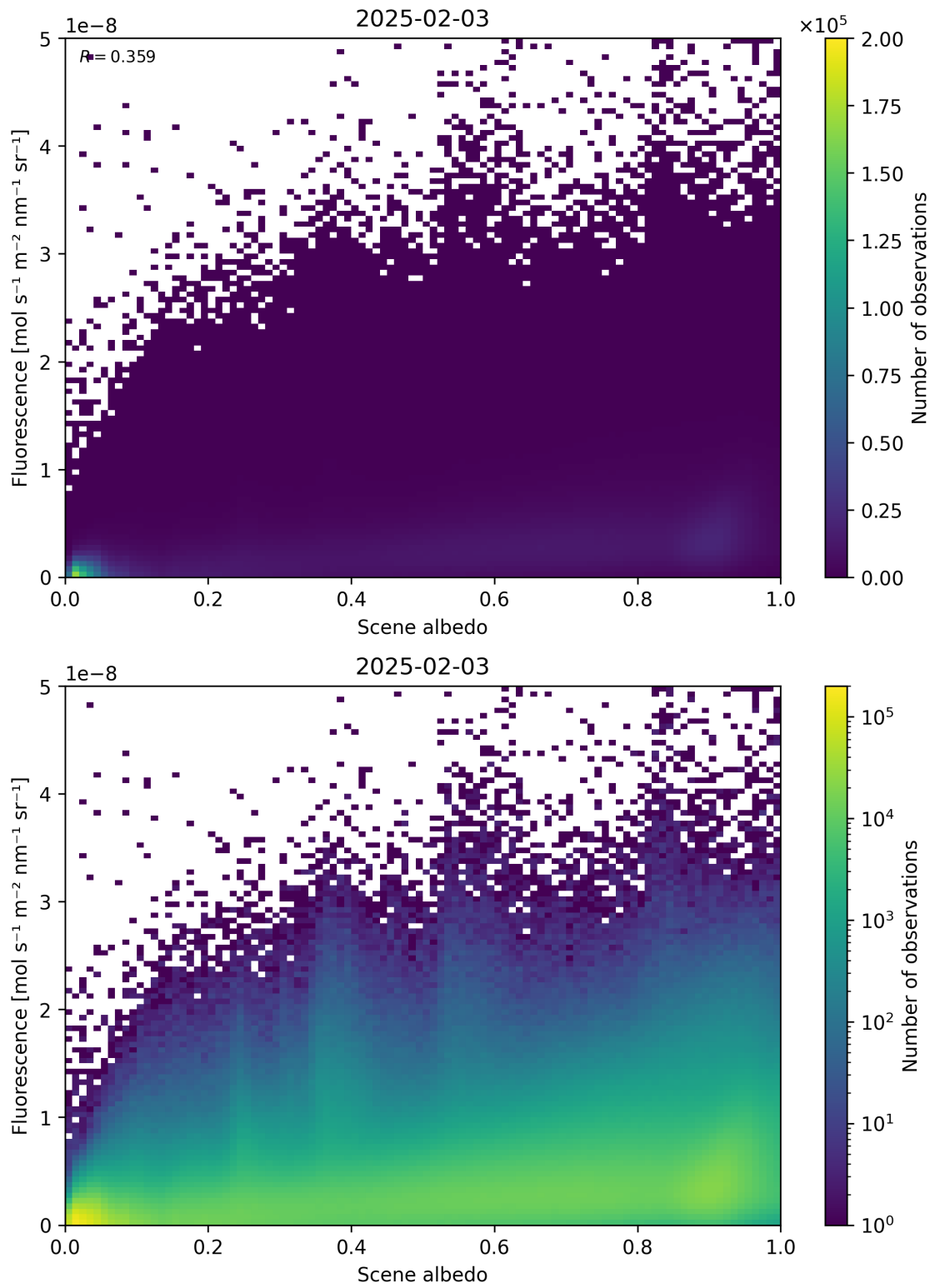
Figure 104: Scatter density plot of “Scene albedo” against “Fluorescence” for 2025-02-03 to 2025-02-04.
