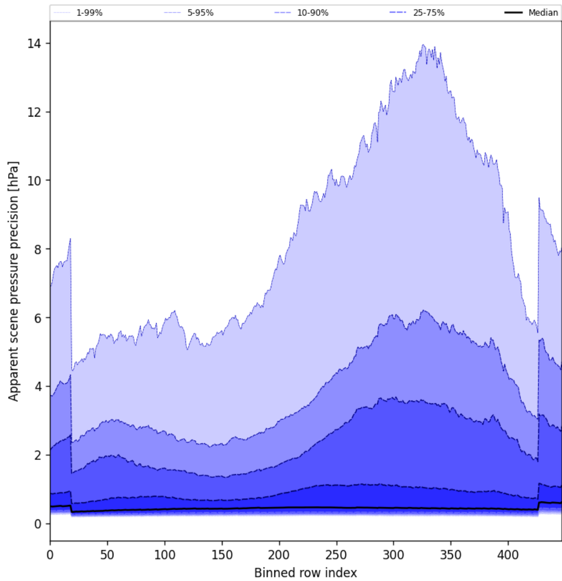
Figure 54: Along track statistics of “Apparent scene pressure precision” for 2025-02-03 to 2025-02-04
