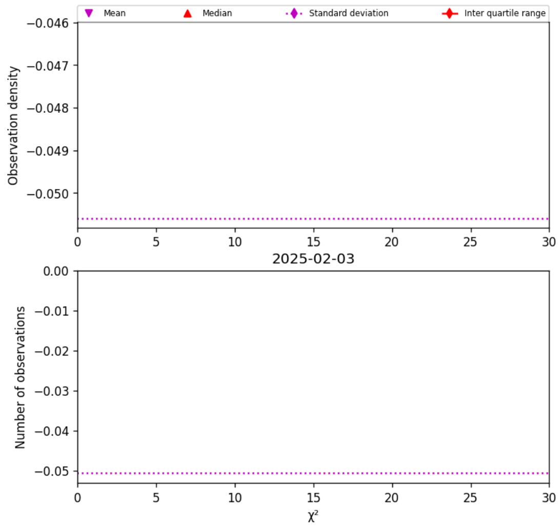
Figure 38: Histogram of " \chi^2 " for 2025-02-03 to 2025-02-04
