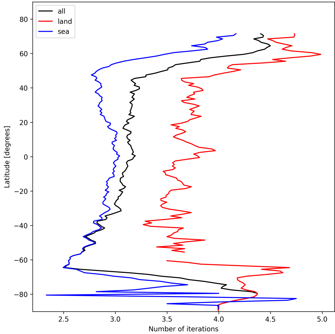
Figure 22: Zonal average of “Number of iterations” for 2025-02-03 to 2025-02-04.
