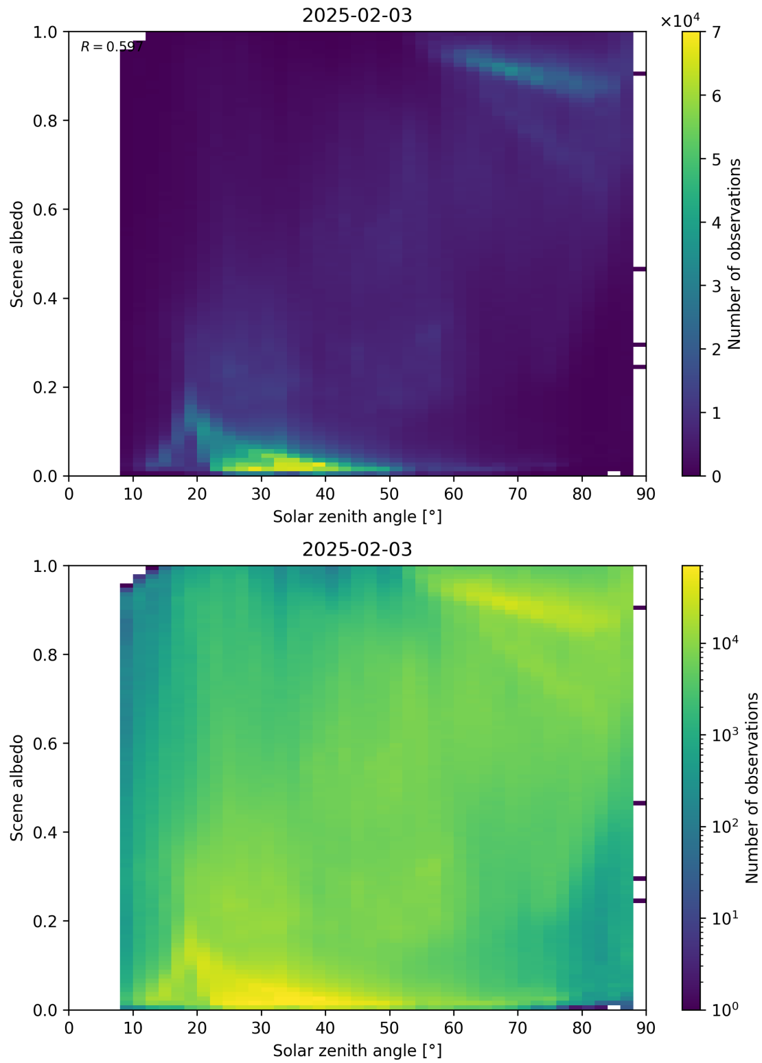
Figure 116: Scatter density plot of “Solar zenith angle” against “Scene albedo” for 2025-02-03 to 2025-02-04.
