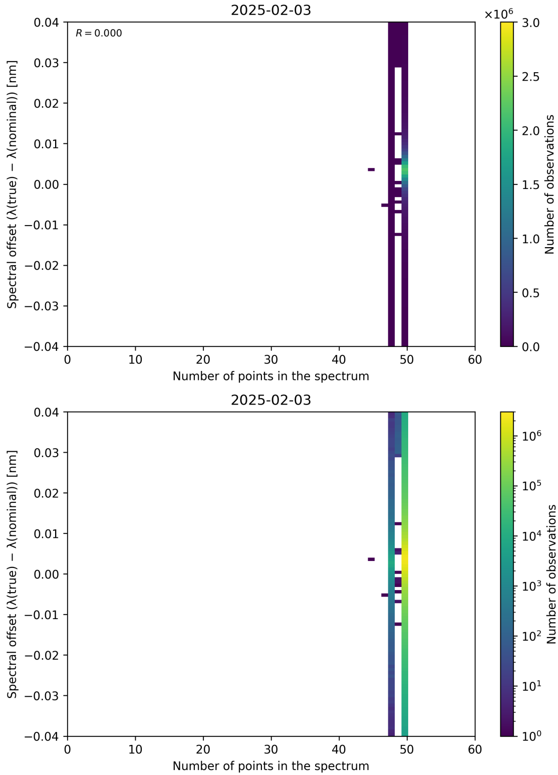
Figure 101: Scatter density plot of “Number of points in the spectrum” against “Spectral offset ( \lambda_{\text{true}} - \lambda_{\text{nominal}} )” for 2025-02-03 to 2025-02-04.
