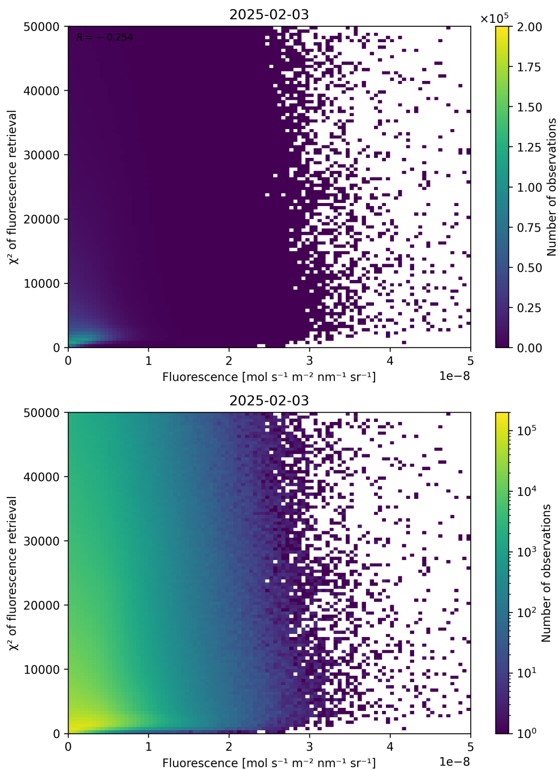
Figure 85: Scatter density plot of “Fluorescence” against “ \chi^2 of fluorescence retrieval” for 2025-02-03 to 2025-02-04.
