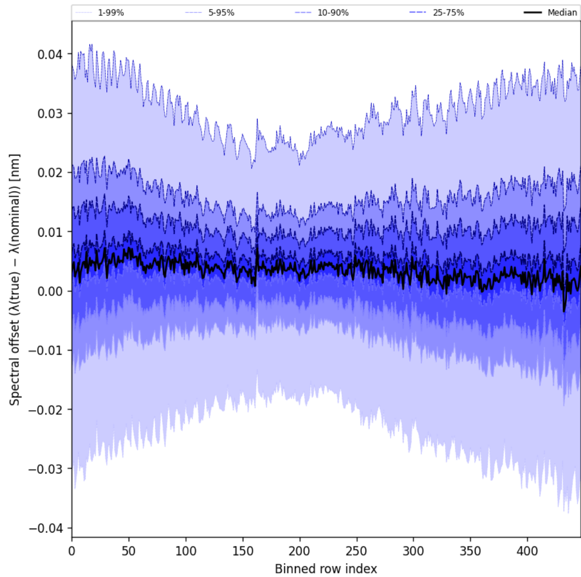
Figure 62: Along track statistics of “Spectral offset ( \lambda_{\text{true}} - \lambda_{\text{nominal}} )” for 2025-02-03 to 2025-02-04
