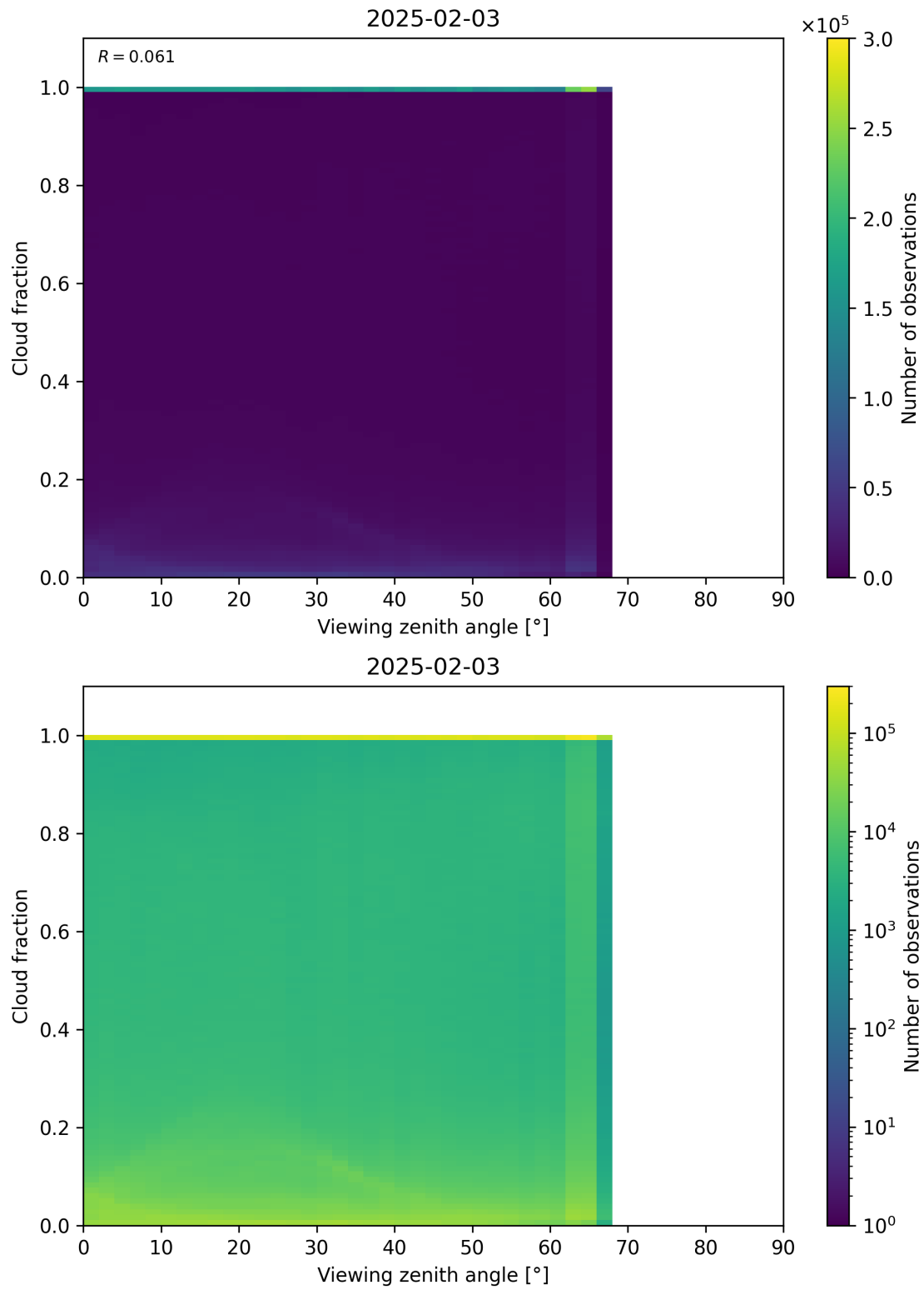
Figure 120: Scatter density plot of “Viewing zenith angle” against “Cloud fraction” for 2025-02-03 to 2025-02-04.
