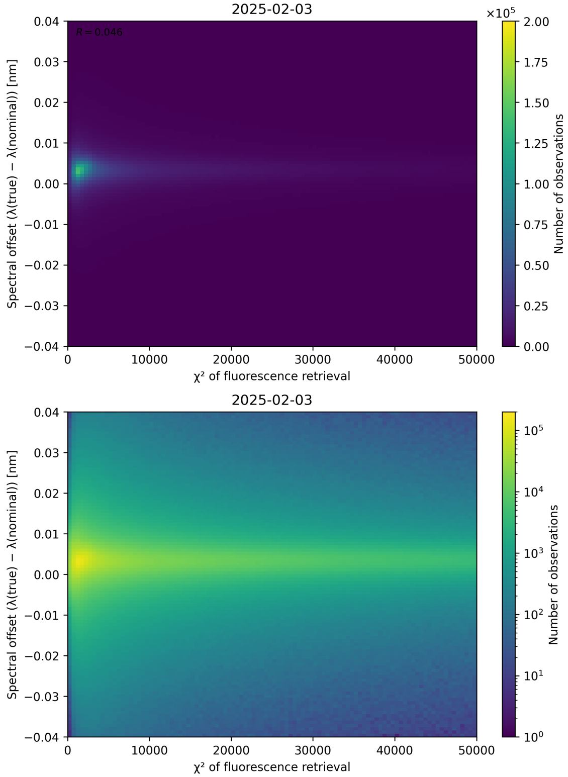
Figure 69: Scatter density plot of “ \chi^2 of fluorescence retrieval” against “Spectral offset ( \lambda_{\text{true}} - \lambda_{\text{nominal}} )” for 2025-02-03 to 2025-02-04.
