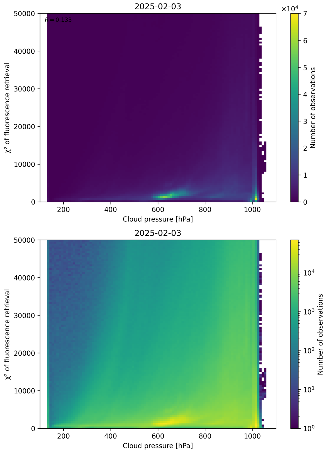
Figure 78: Scatter density plot of “Cloud pressure” against “ \chi^2 of fluorescence retrieval” for 2025-02-03 to 2025-02-04.
