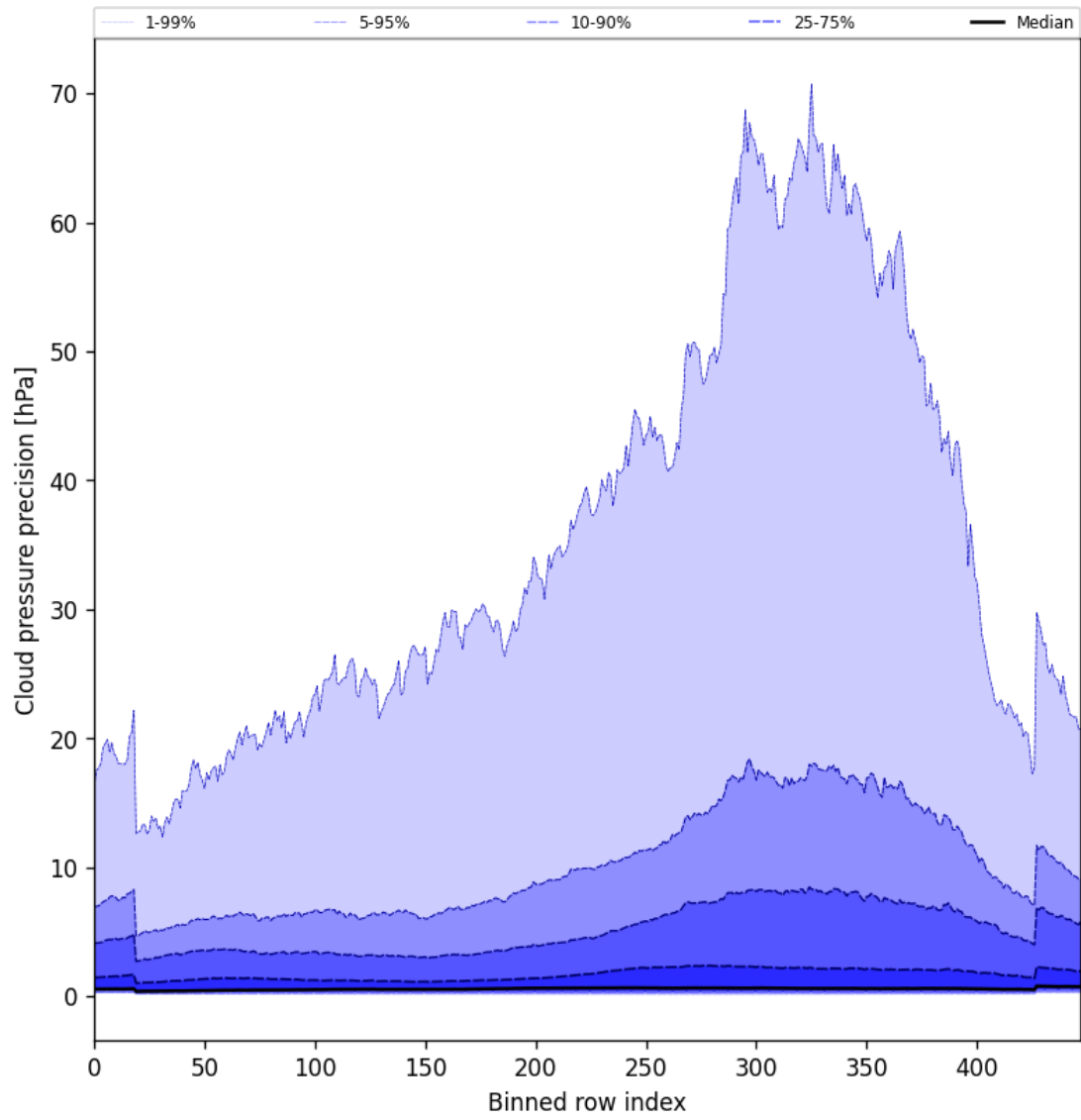
Figure 48: Along track statistics of “Cloud pressure precision” for 2025-02-03 to 2025-02-04
