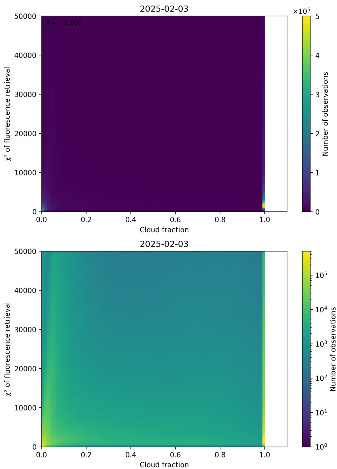
Figure 71: Scatter density plot of “Cloud fraction” against “ \chi^2 of fluorescence retrieval” for 2025-02-03 to 2025-02-04.
