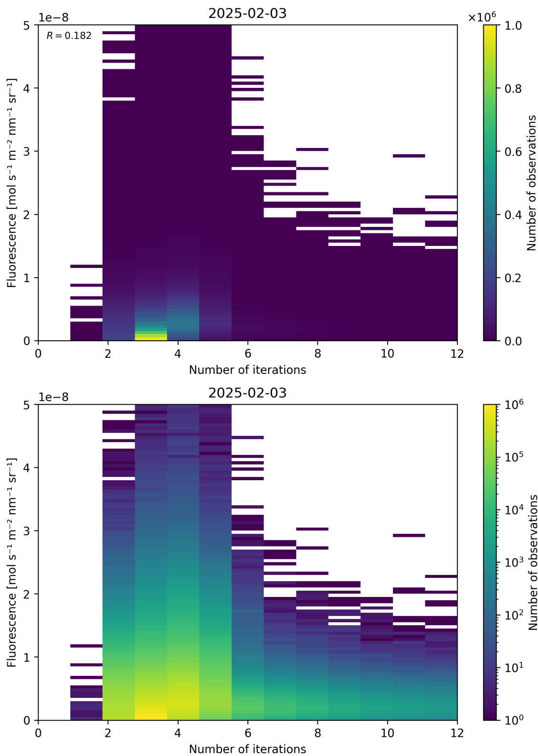
Figure 98: Scatter density plot of “Number of iterations” against “Fluorescence” for 2025-02-03 to 2025-02-04.
