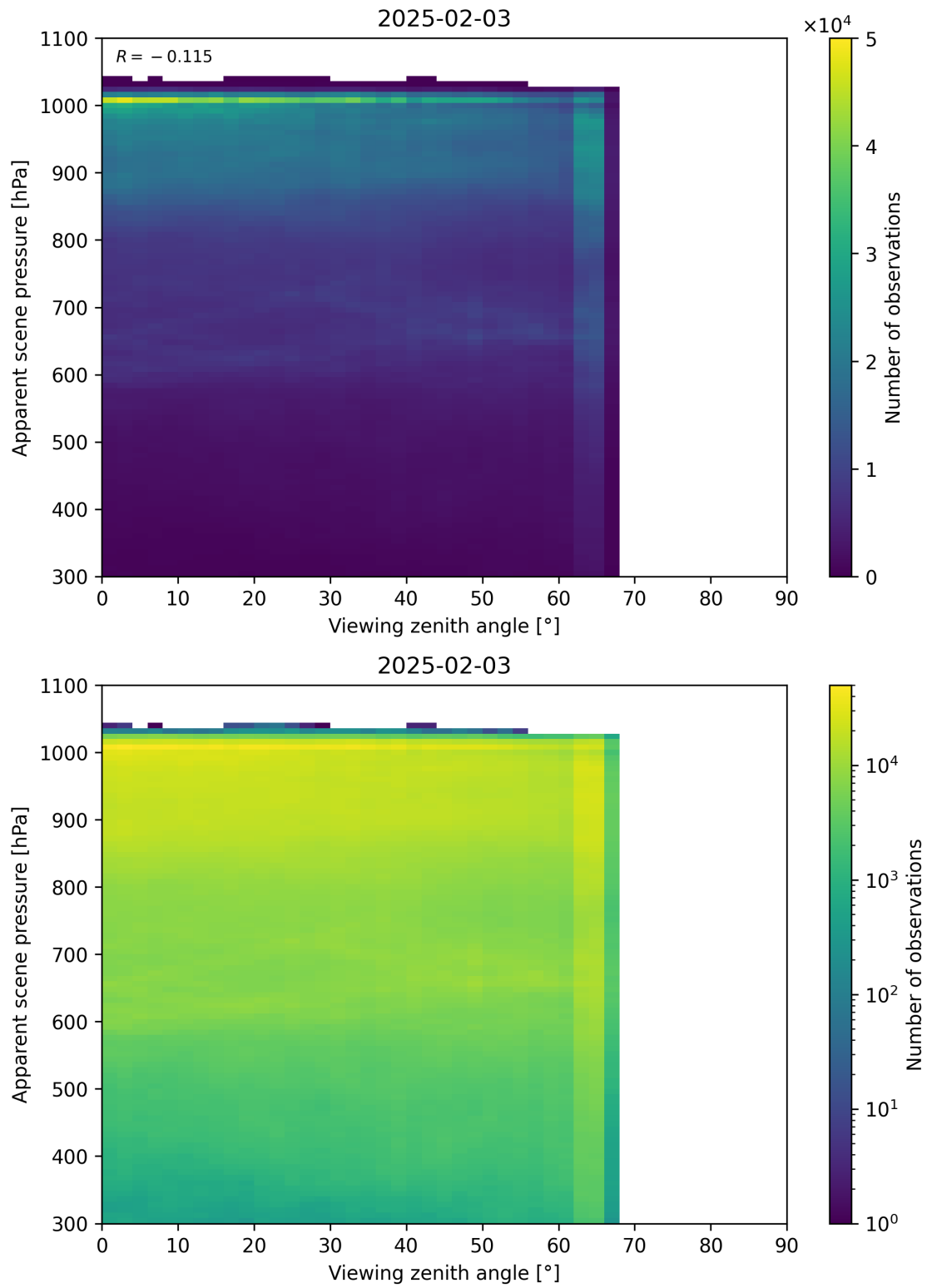
Figure 118: Scatter density plot of “Viewing zenith angle” against “Apparent scene pressure” for 2025-02-03 to 2025-02-04.
