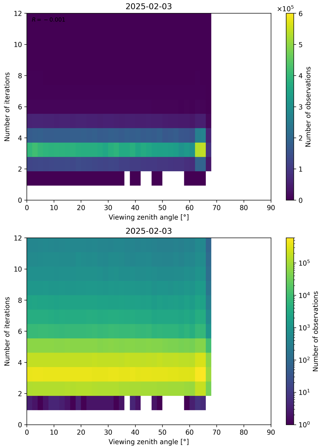
Figure 124: Scatter density plot of “Viewing zenith angle” against “Number of iterations” for 2025-02-03 to 2025-02-04.
