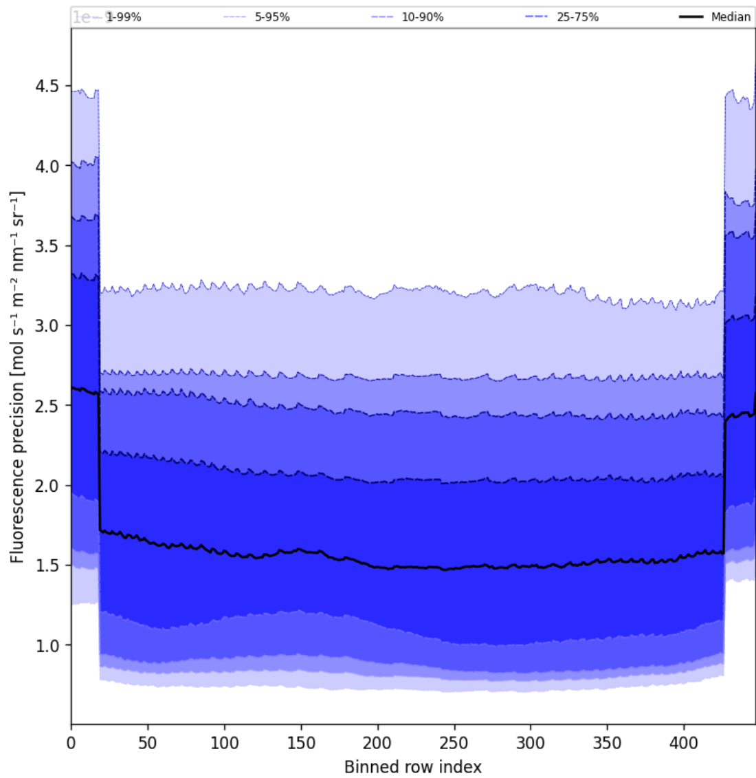
Figure 58: Along track statistics of “Fluorescence precision” for 2025-02-03 to 2025-02-04
