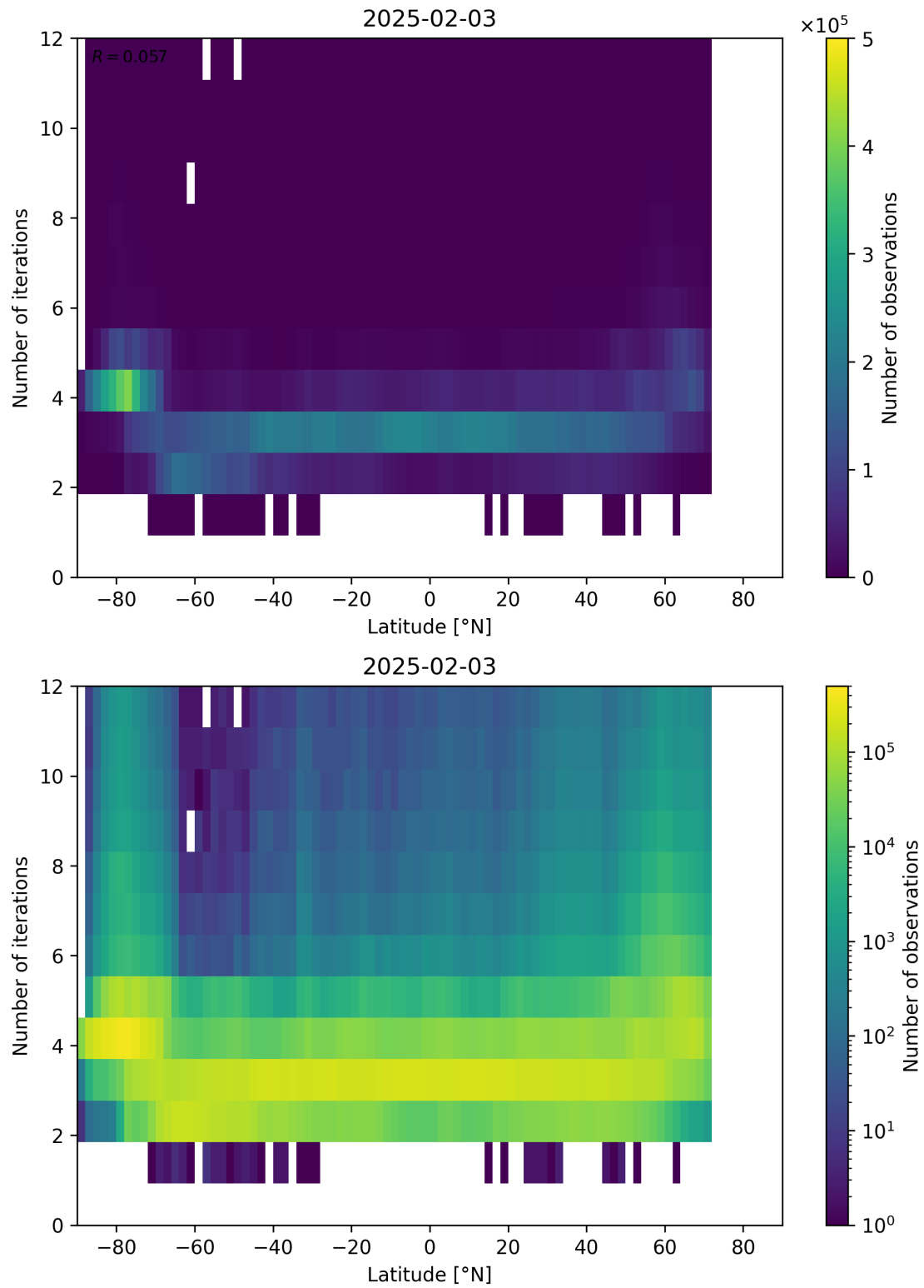
Figure 93: Scatter density plot of “Latitude” against “Number of iterations” for 2025-02-03 to 2025-02-04.
