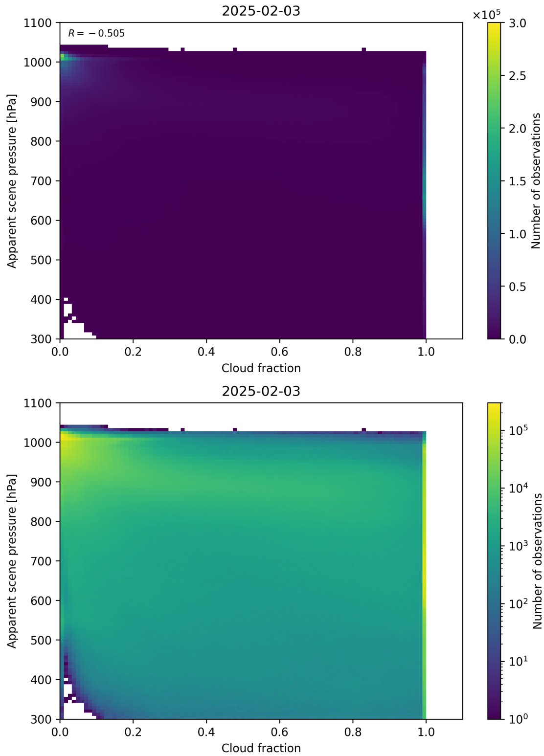
Figure 70: Scatter density plot of “Cloud fraction” against “Apparent scene pressure” for 2025-02-03 to 2025-02-04.
