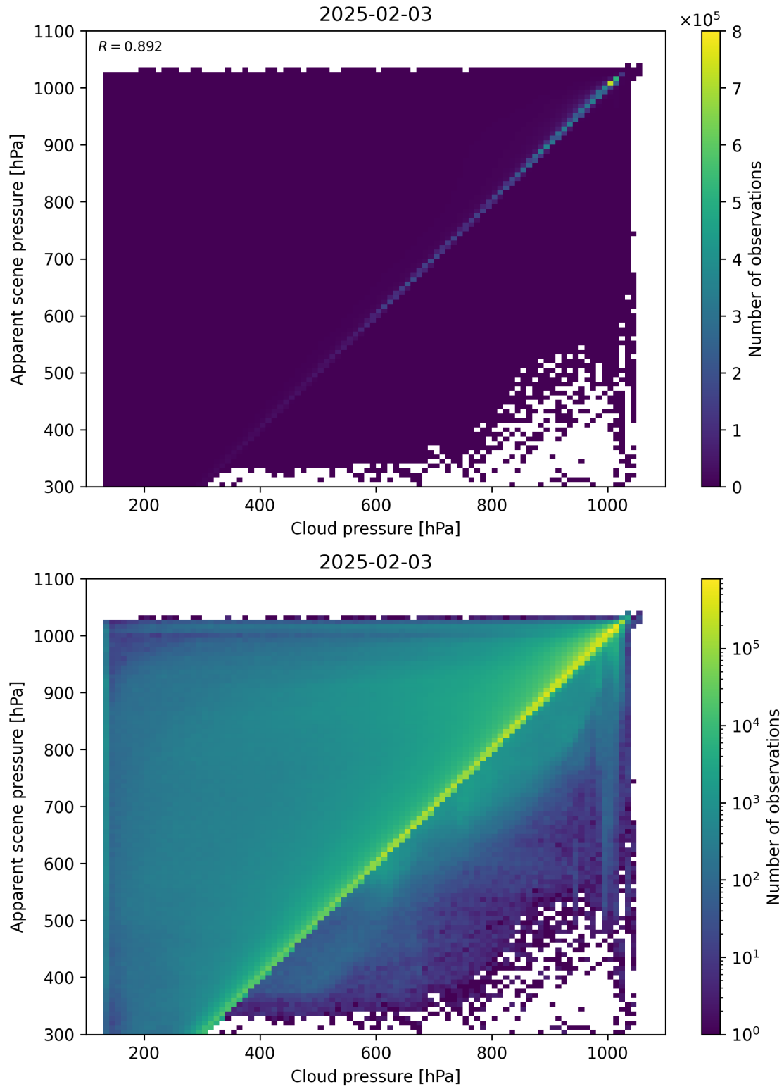
Figure 77: Scatter density plot of “Cloud pressure” against “Apparent scene pressure” for 2025-02-03 to 2025-02-04.
