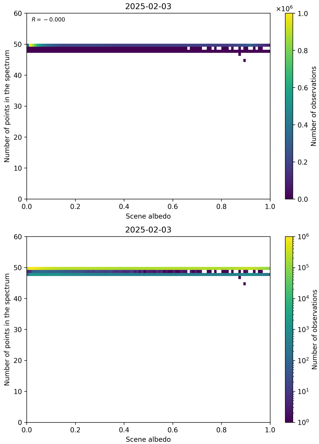
Figure 106: Scatter density plot of “Scene albedo” against “Number of points in the spectrum” for 2025-02-03 to 2025-02-04.
