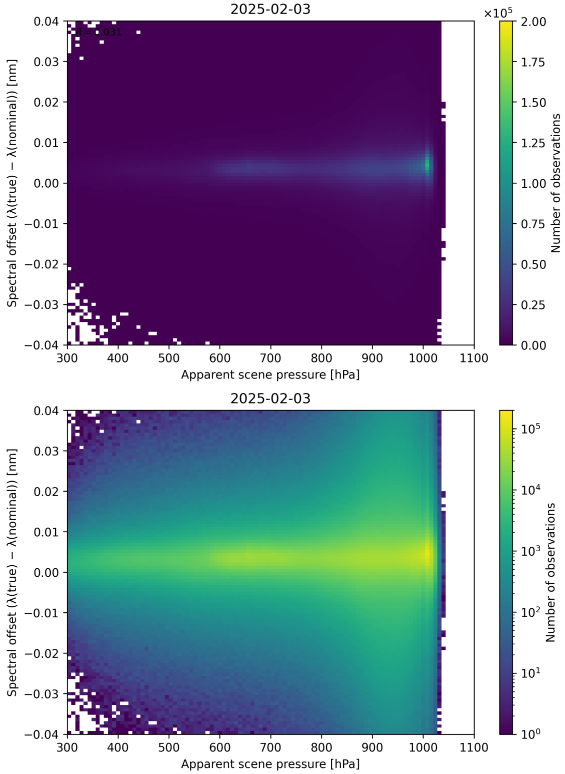
Figure 67: Scatter density plot of “Apparent scene pressure” against “Spectral offset ( \lambda_{\text{true}} - \lambda_{\text{nominal}} )” for 2025-02-03 to 2025-02-04.
