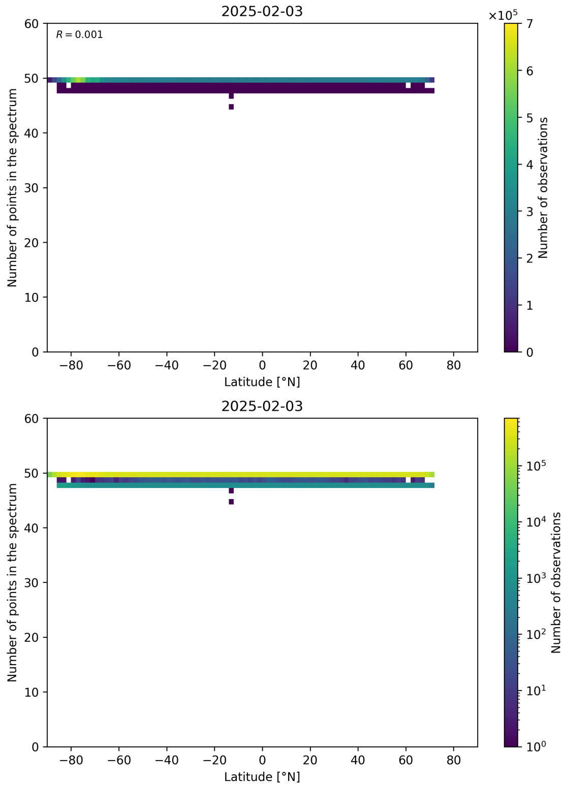
Figure 94: Scatter density plot of “Latitude” against “Number of points in the spectrum” for 2025-02-03 to 2025-02-04.
