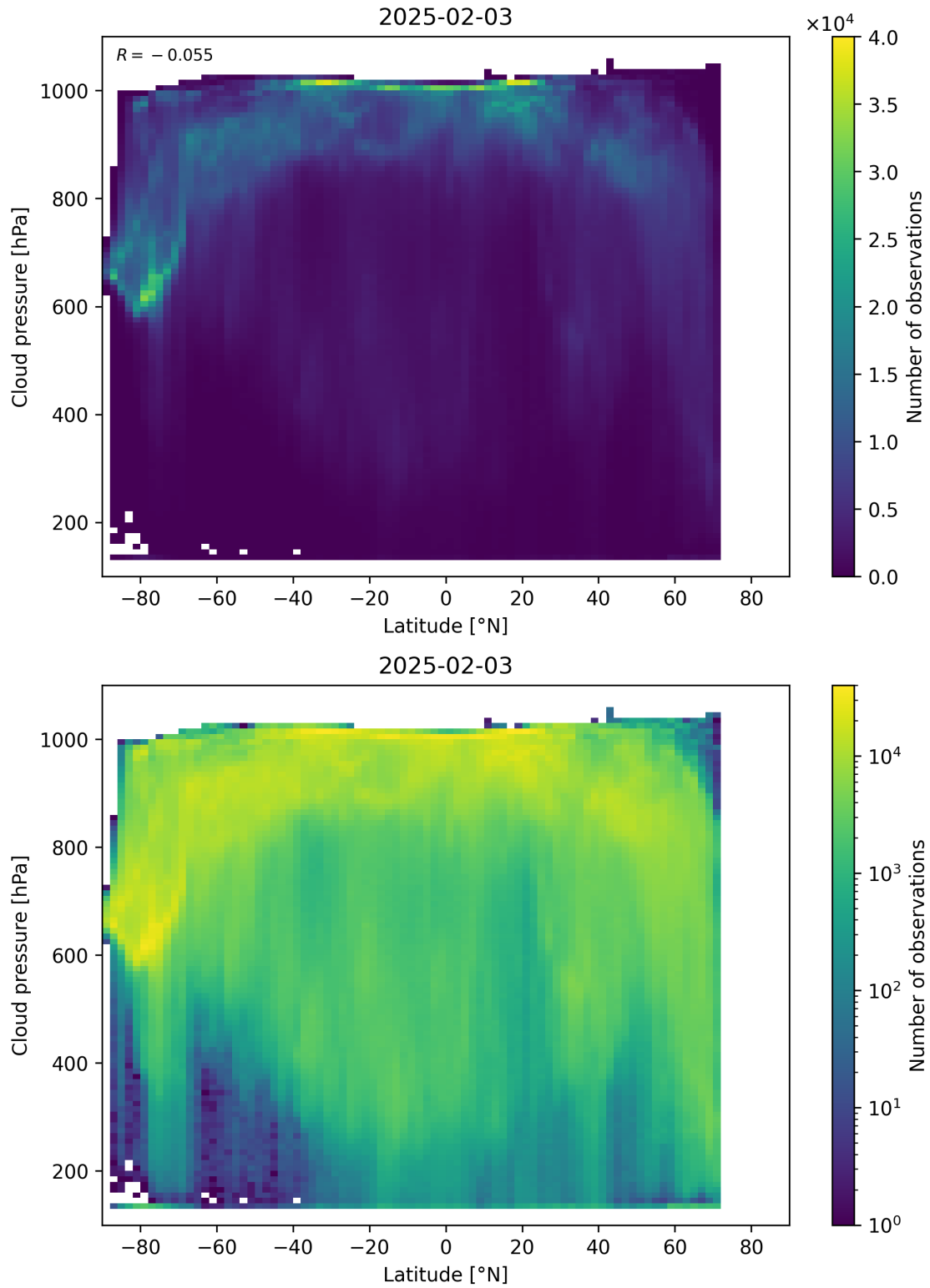
Figure 91: Scatter density plot of “Latitude” against “Cloud pressure” for 2025-02-03 to 2025-02-04.
