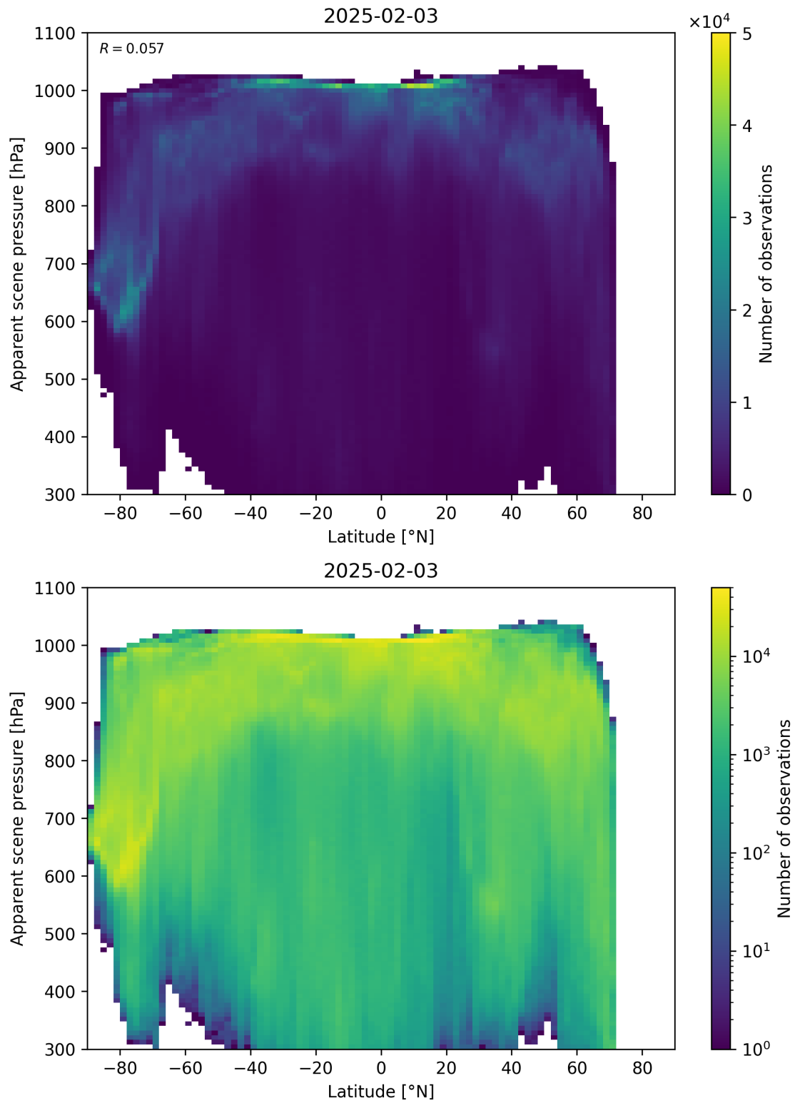
Figure 88: Scatter density plot of “Latitude” against “Apparent scene pressure” for 2025-02-03 to 2025-02-04.
