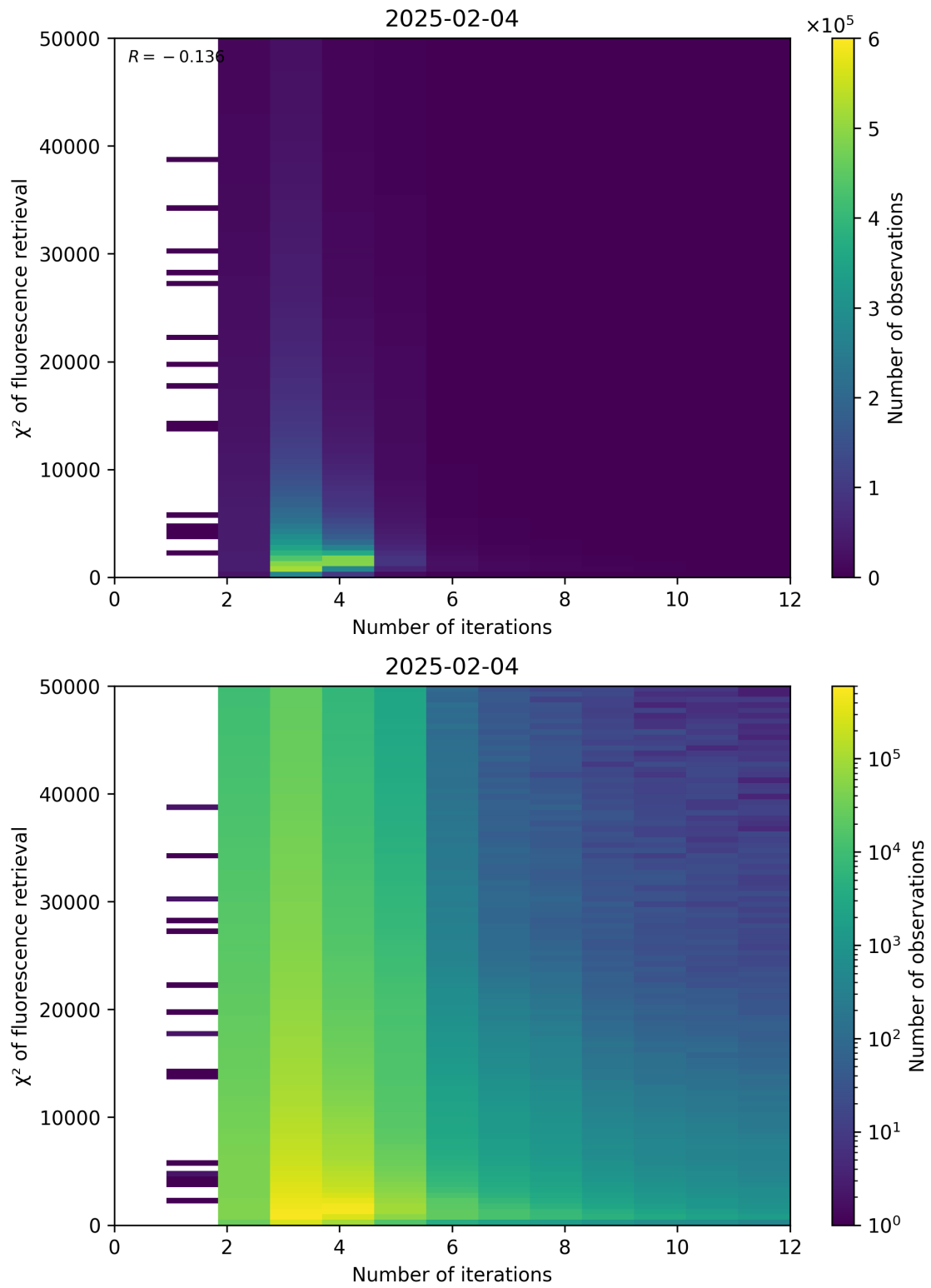
Figure 97: Scatter density plot of “Number of iterations” against “ \chi^2 of fluorescence retrieval” for 2025-02-03 to 2025-02-05.
