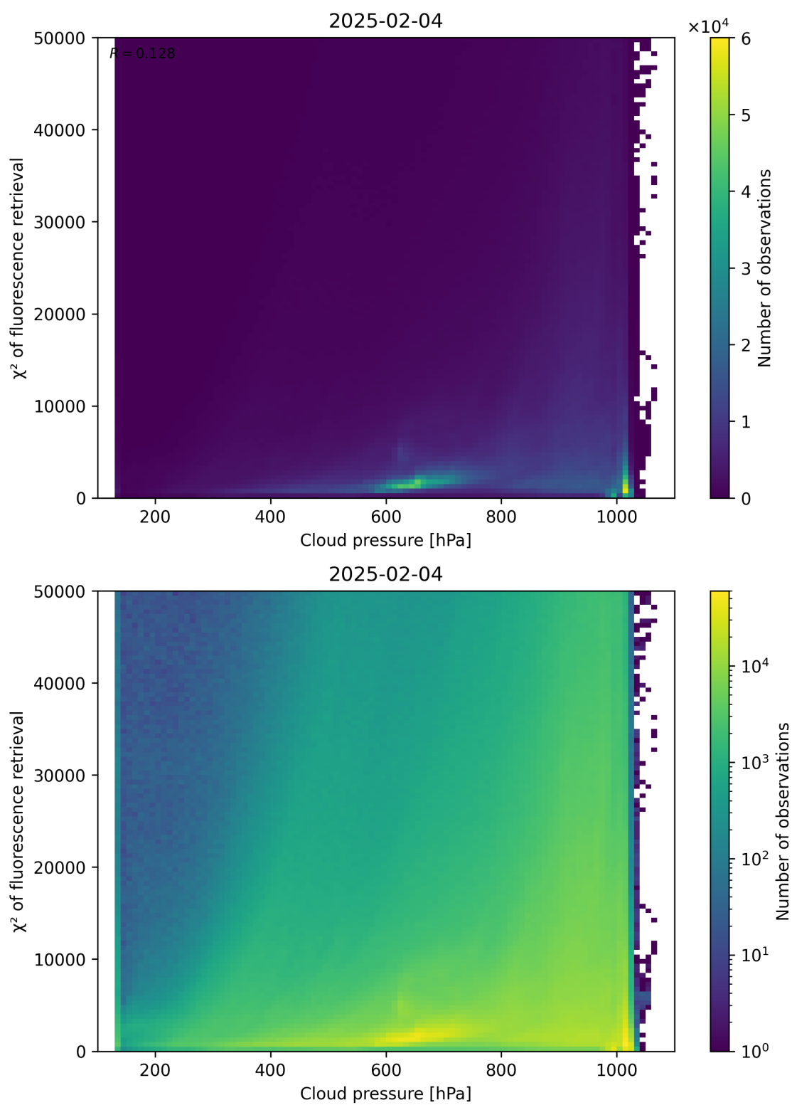
Figure 78: Scatter density plot of “Cloud pressure” against “ \chi^2 of fluorescence retrieval” for 2025-02-03 to 2025-02-05.
