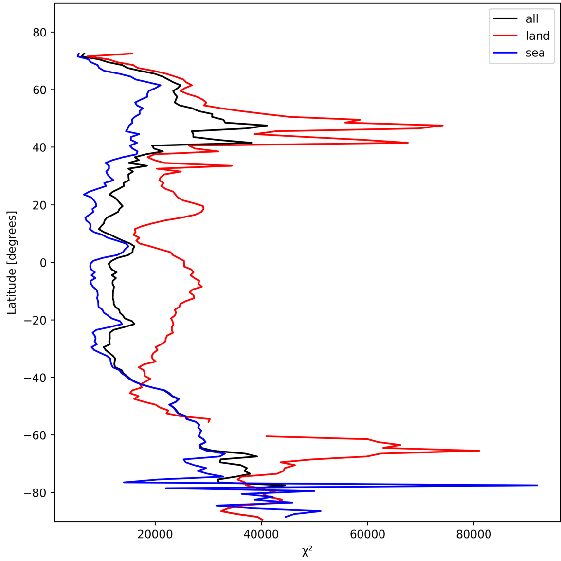
Figure 21: Zonal average of “ \chi^2 ” for 2025-02-03 to 2025-02-05.
