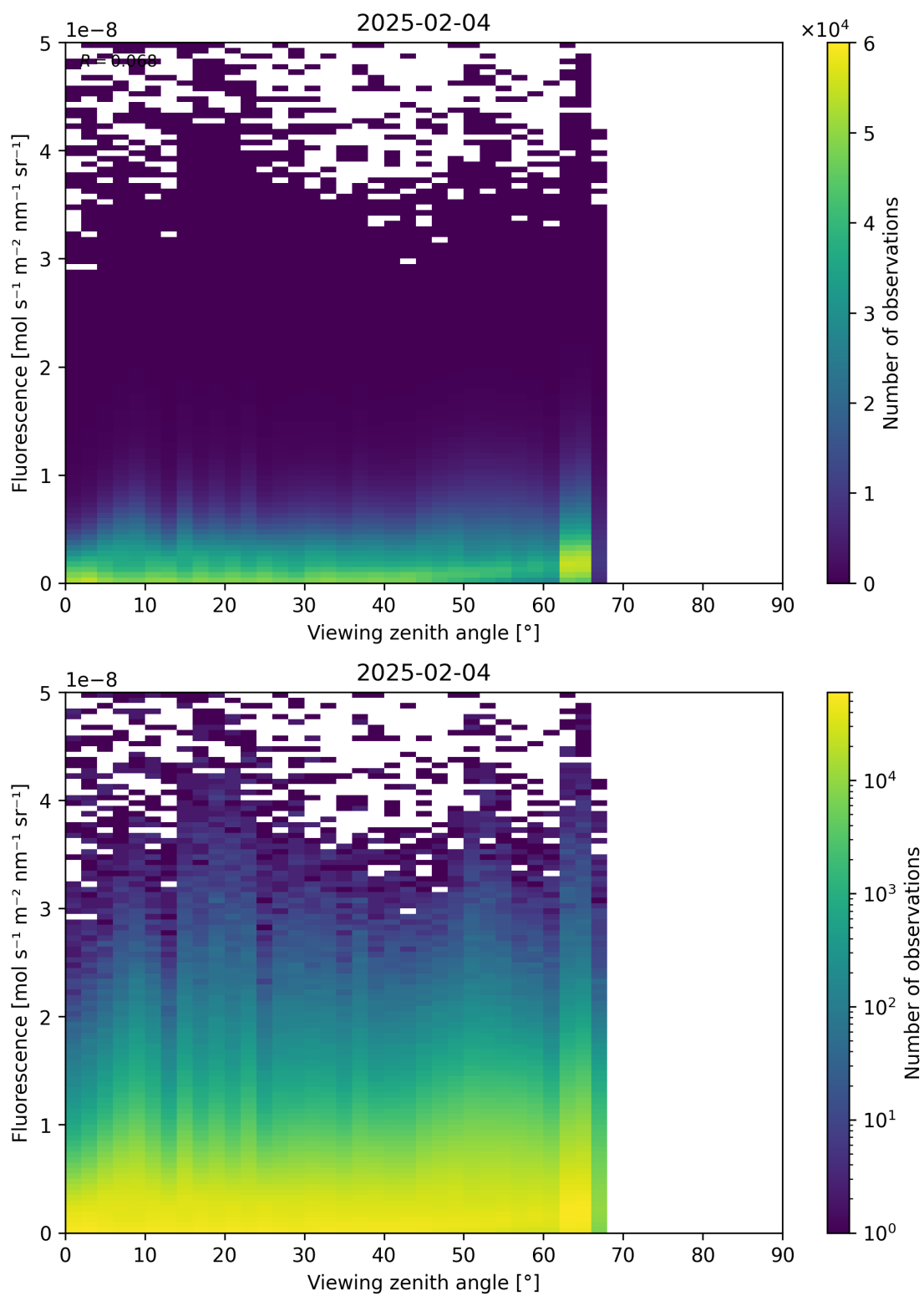
Figure 122: Scatter density plot of “Viewing zenith angle” against “Fluorescence” for 2025-02-03 to 2025-02-05.
