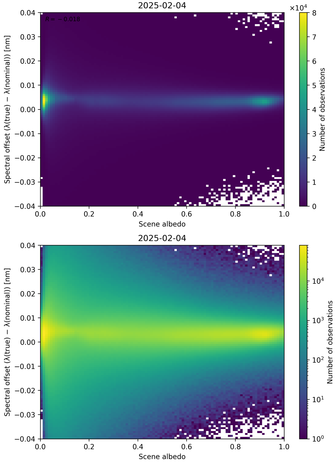
Figure 107: Scatter density plot of “Scene albedo” against “Spectral offset ( \lambda_{\text{true}} - \lambda_{\text{nominal}} )” for 2025-02-03 to 2025-02-05.
