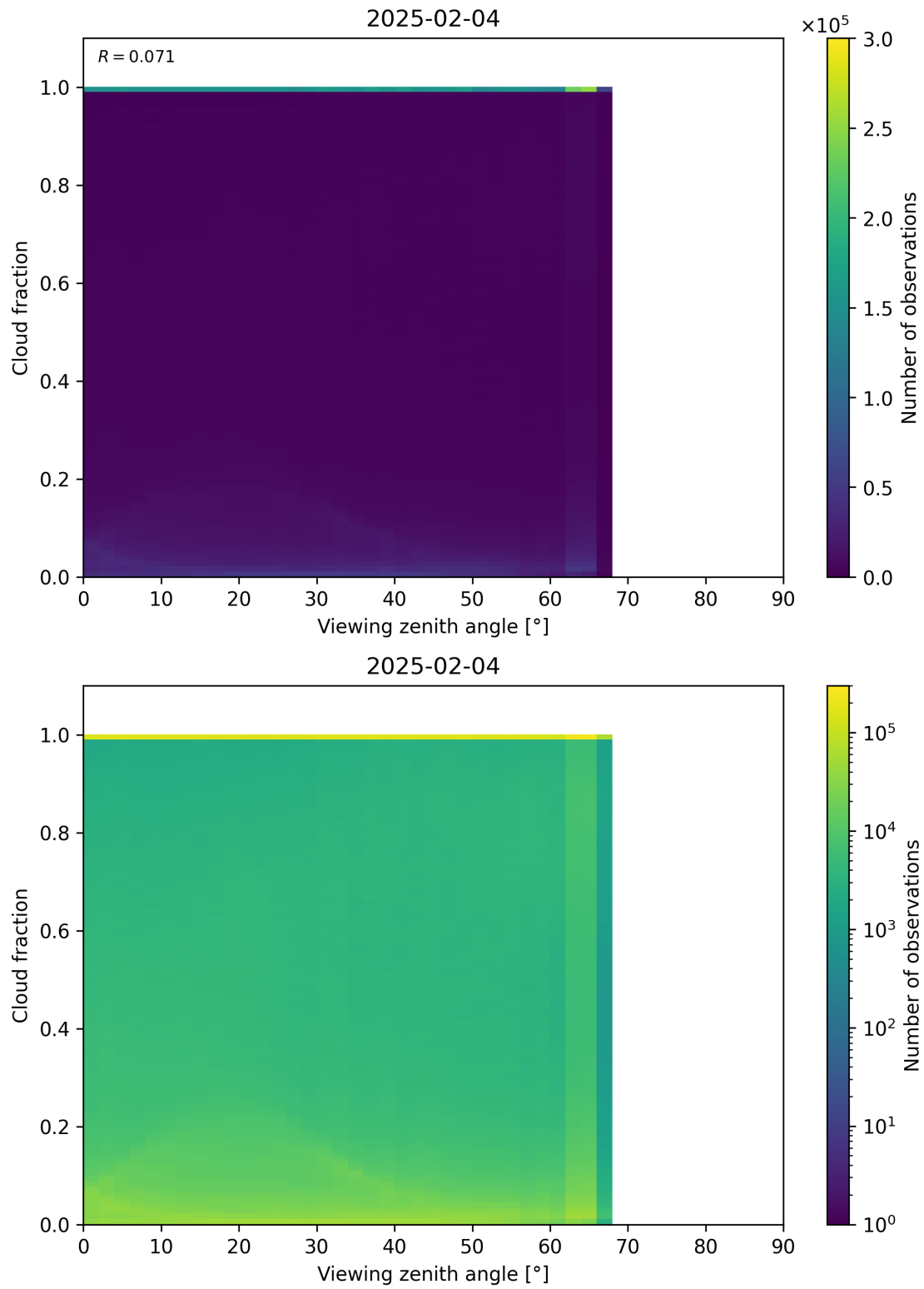
Figure 120: Scatter density plot of “Viewing zenith angle” against “Cloud fraction” for 2025-02-03 to 2025-02-05.
