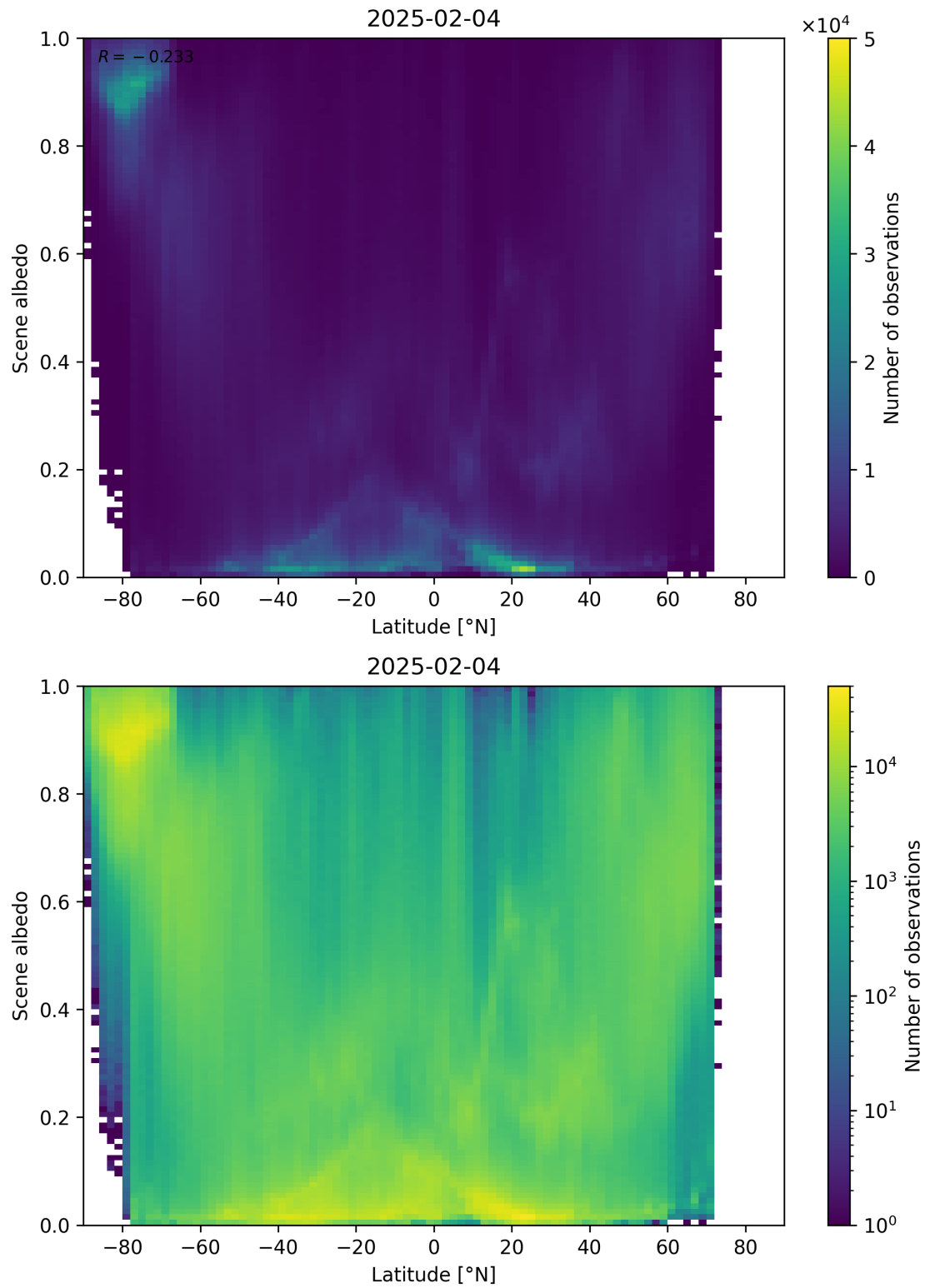
Figure 95: Scatter density plot of “Latitude” against “Scene albedo” for 2025-02-03 to 2025-02-05.
