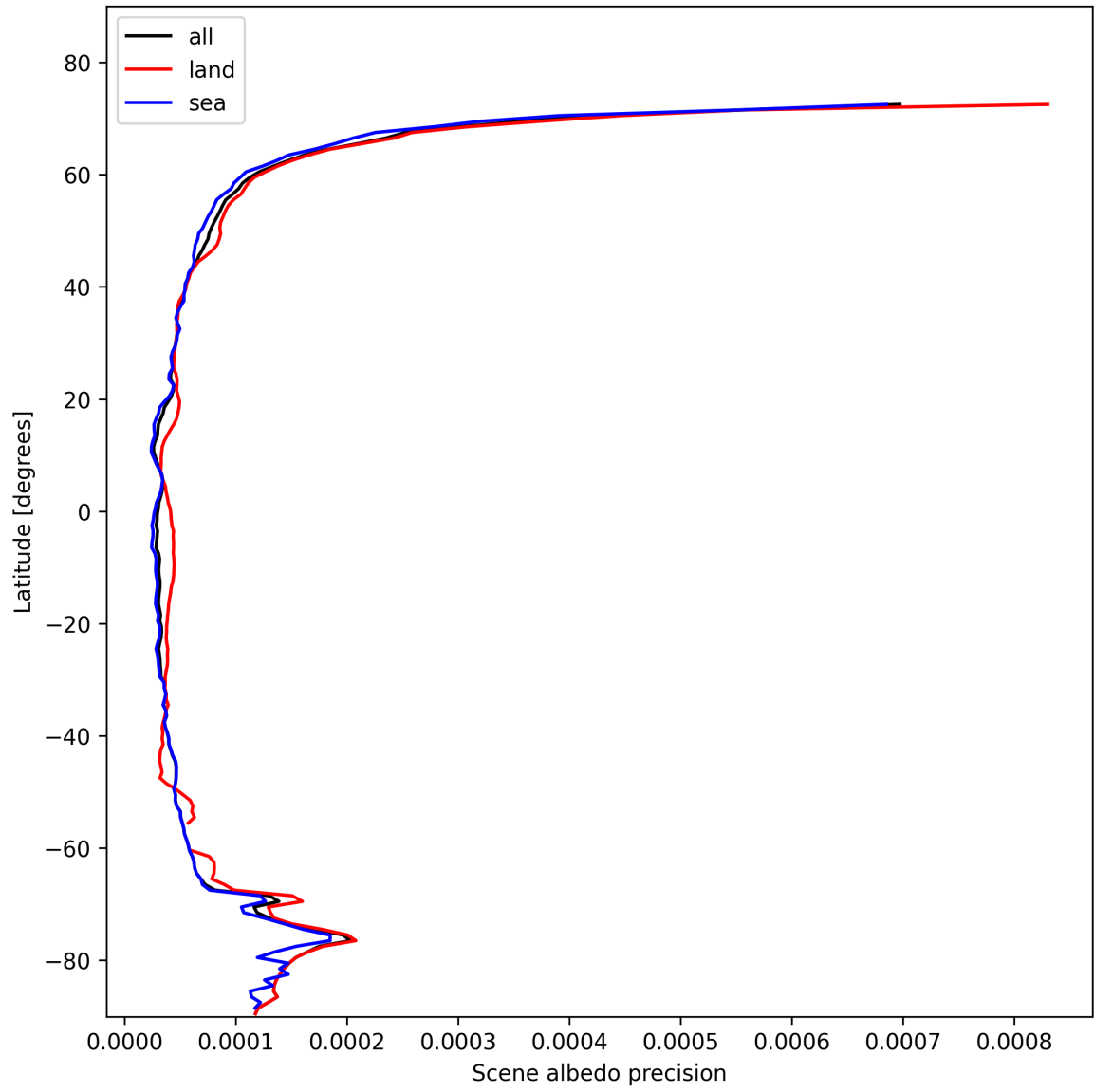
Figure 18: Zonal average of “Scene albedo precision” for 2025-02-03 to 2025-02-05.
