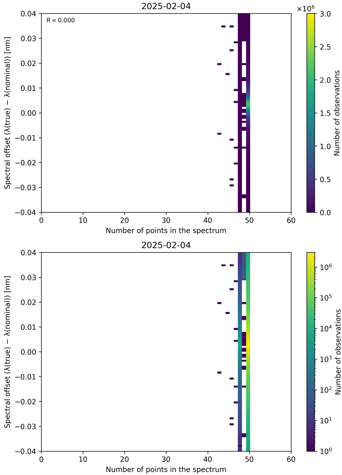
Figure 101: Scatter density plot of “Number of points in the spectrum” against “Spectral offset ( \lambda_{\text{true}} - \lambda_{\text{nominal}} )” for 2025-02-03 to 2025-02-05.
