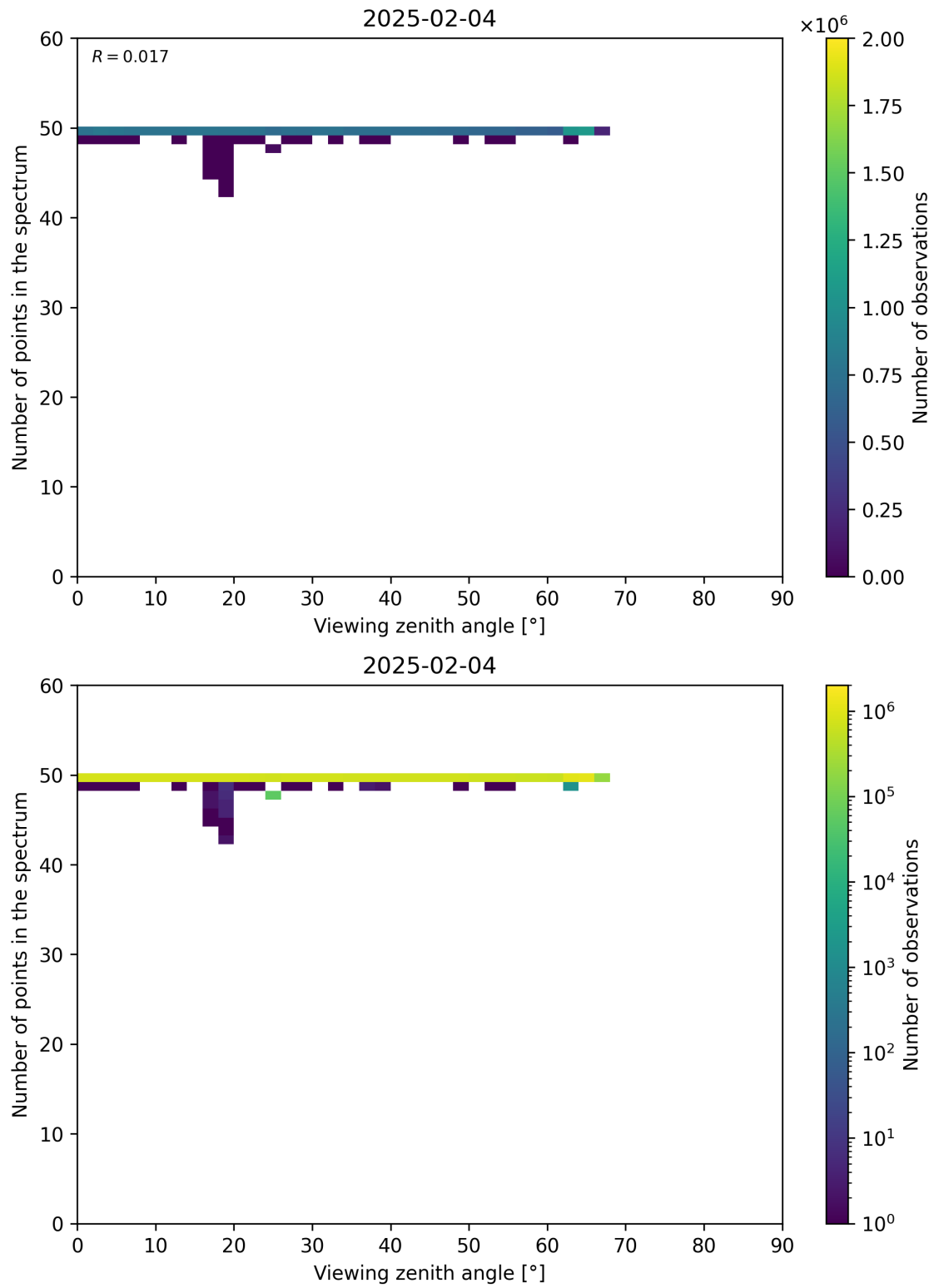
Figure 125: Scatter density plot of “Viewing zenith angle” against “Number of points in the spectrum” for 2025-02-03 to 2025-02-05.
