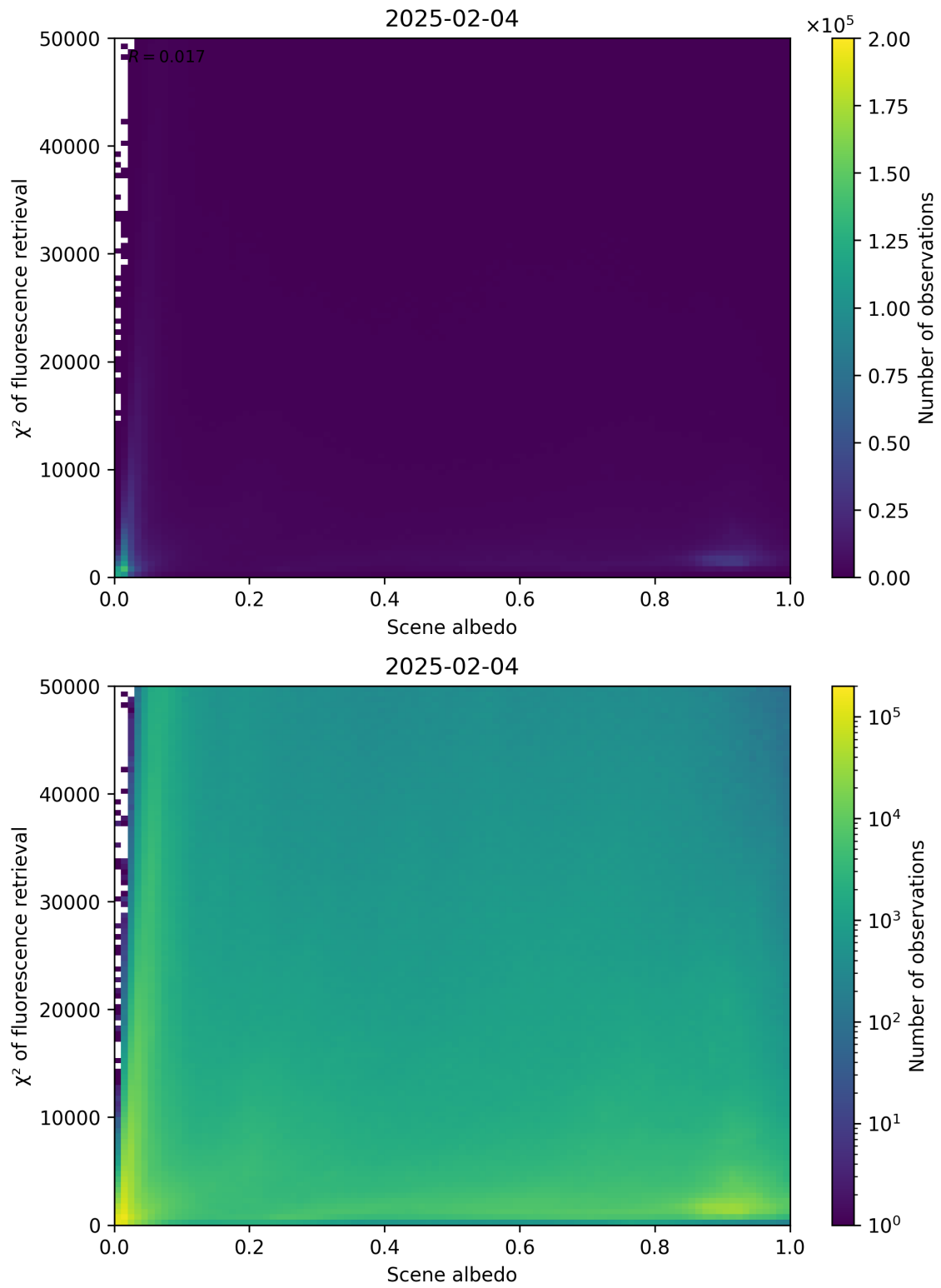
Figure 103: Scatter density plot of “Scene albedo” against “ \chi^2 of fluorescence retrieval” for 2025-02-03 to 2025-02-05.
