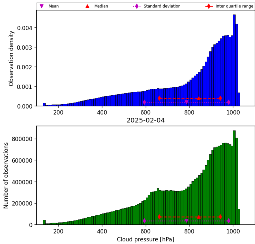
Figure 30: Histogram of “Cloud pressure” for 2025-02-03 to 2025-02-05
