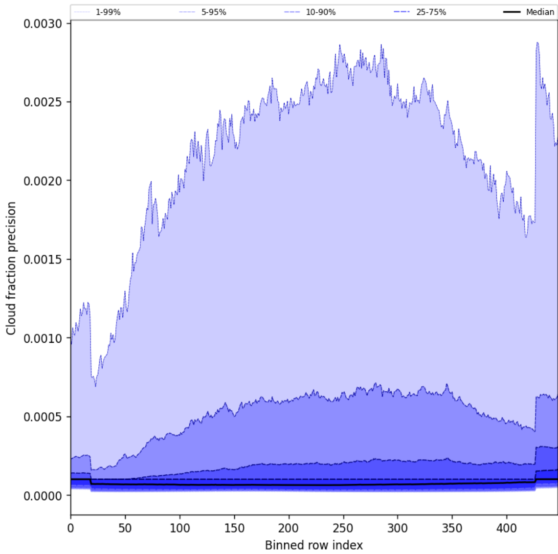
Figure 50: Along track statistics of “Cloud fraction precision” for 2025-02-03 to 2025-02-05
