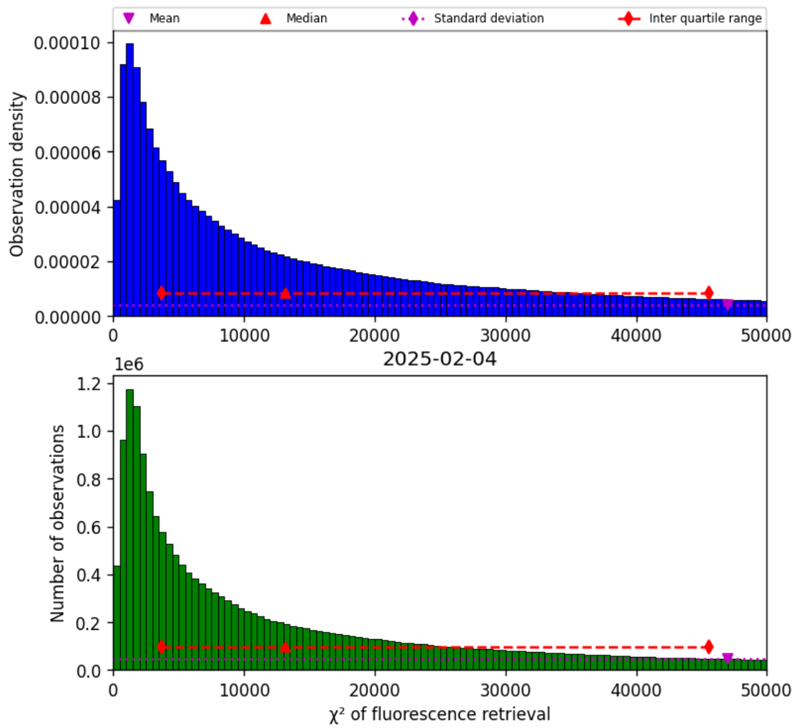
Figure 42: Histogram of “ \chi^2 of fluorescence retrieval” for 2025-02-03 to 2025-02-05
