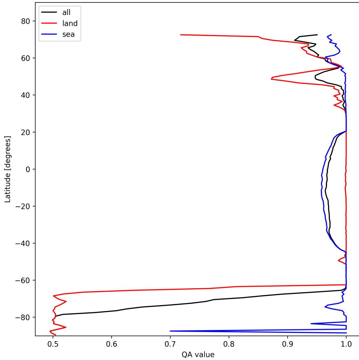
Figure 12: Zonal average of “QA value” for 2025-02-03 to 2025-02-05.
