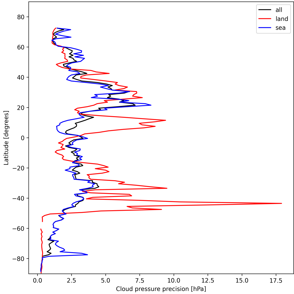
Figure 14: Zonal average of “Cloud pressure precision” for 2025-02-03 to 2025-02-05.
