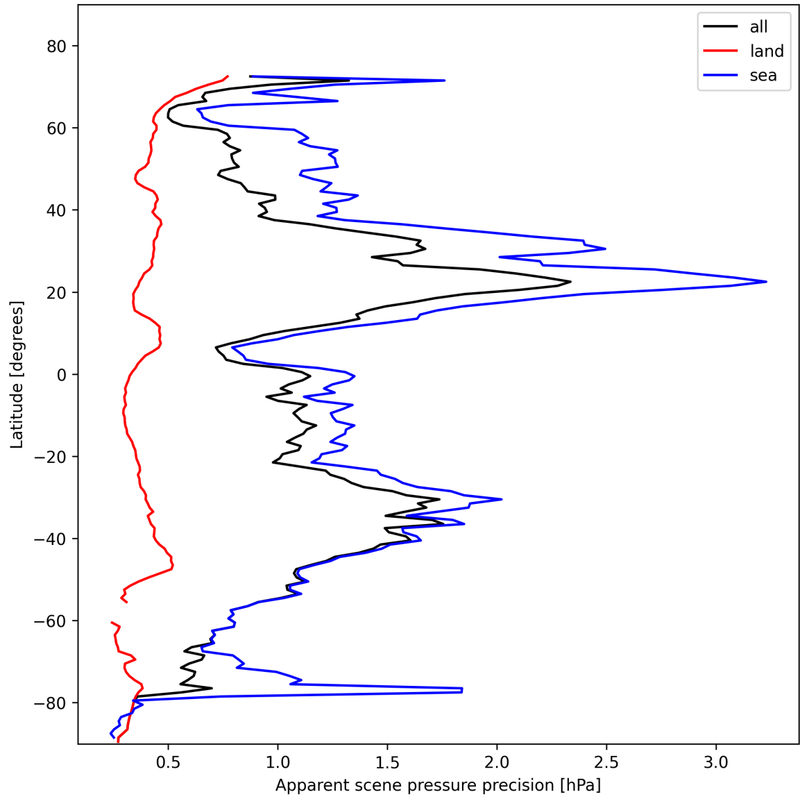
Figure 20: Zonal average of “Apparent scene pressure precision” for 2025-02-03 to 2025-02-05.
