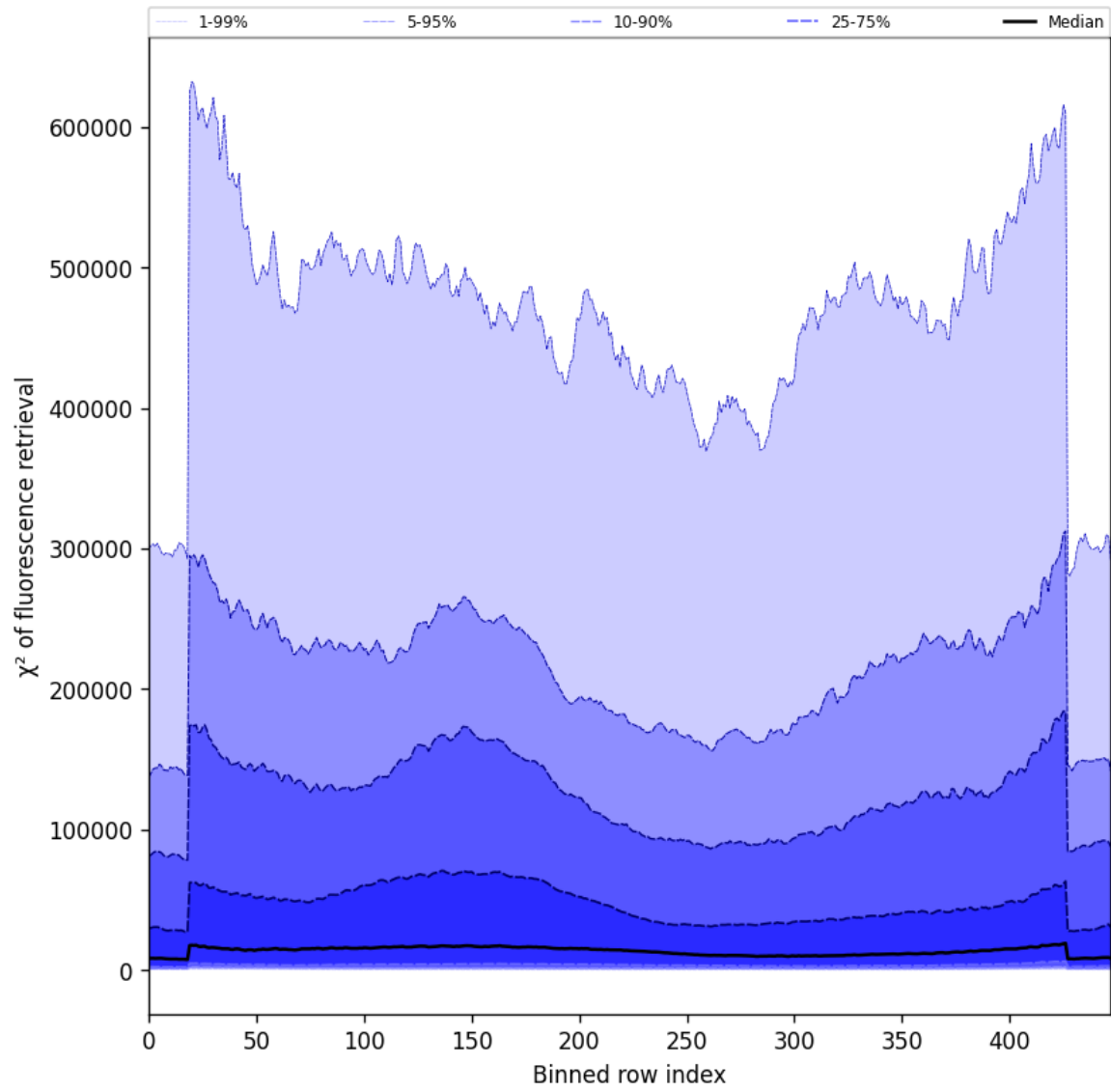
Figure 59: Along track statistics of “ \chi^2 of fluorescence retrieval” for 2025-02-03 to 2025-02-05
