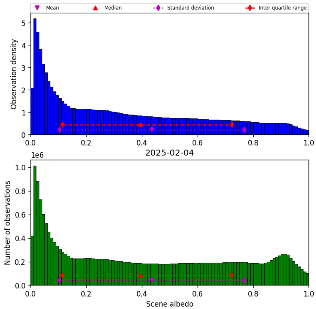
Figure 34: Histogram of “Scene albedo” for 2025-02-03 to 2025-02-05
