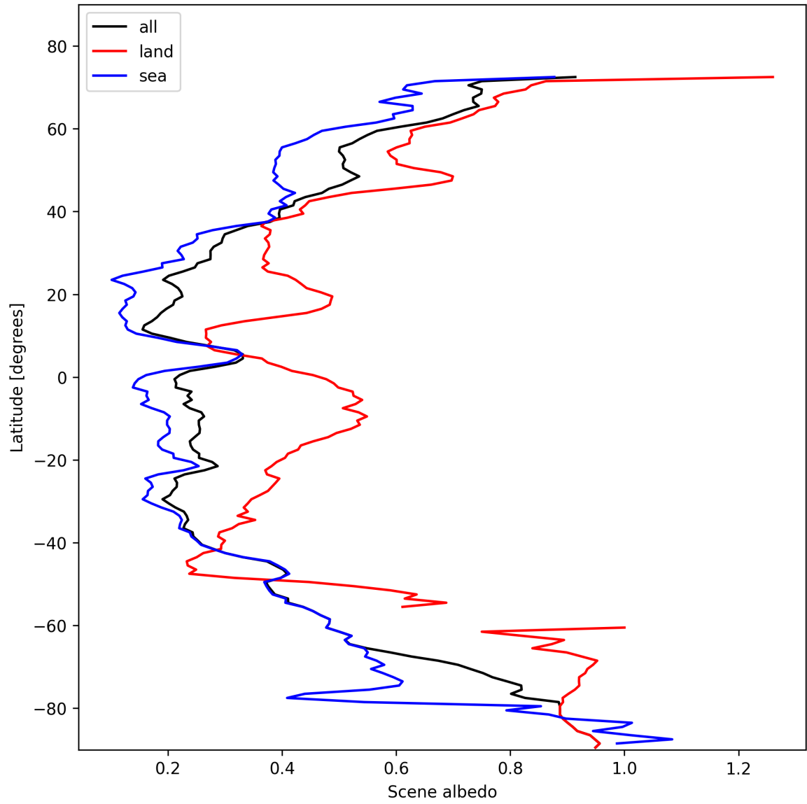
Figure 17: Zonal average of “Scene albedo” for 2025-02-03 to 2025-02-05.
