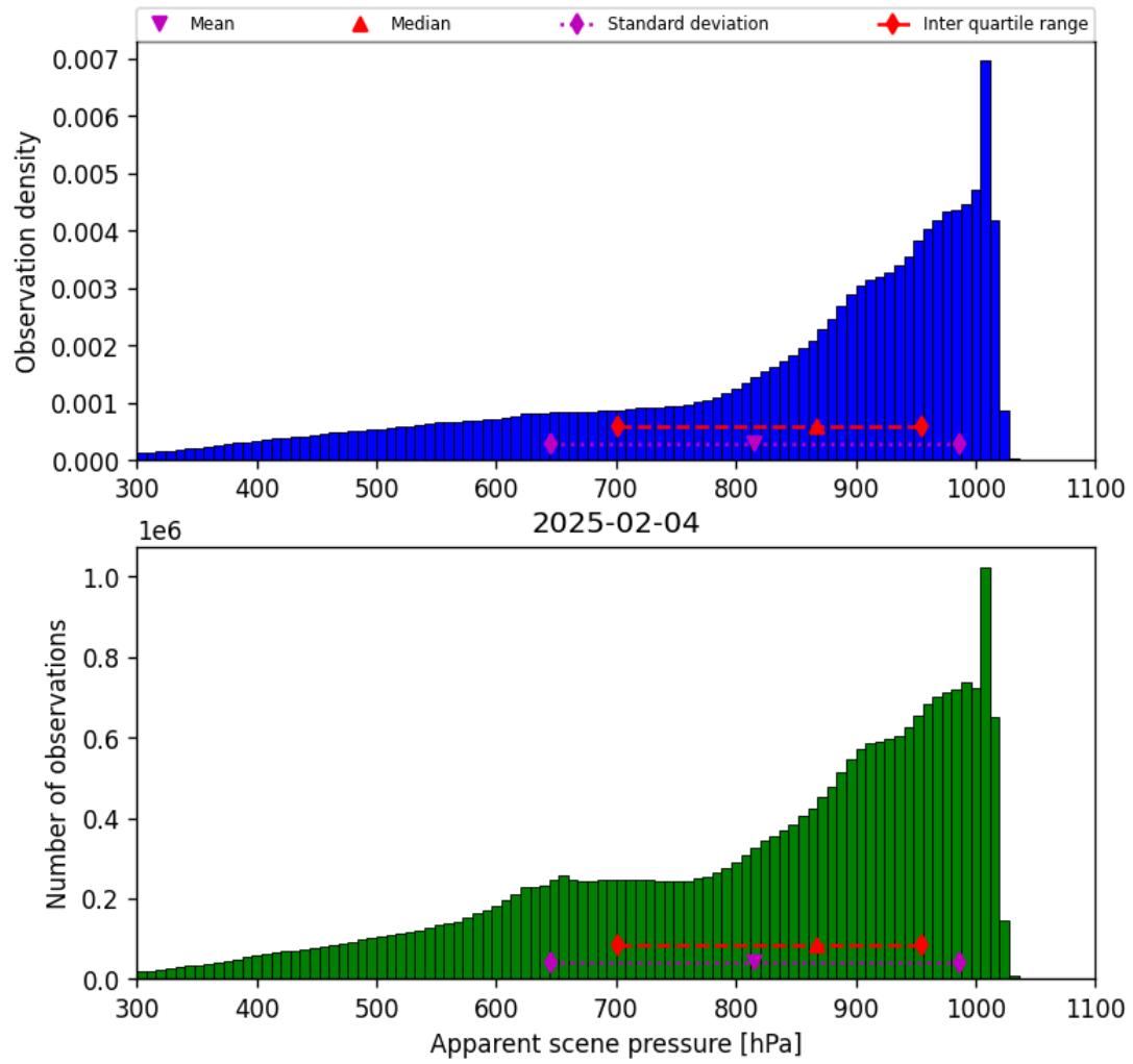
Figure 36: Histogram of “Apparent scene pressure” for 2025-02-03 to 2025-02-05
