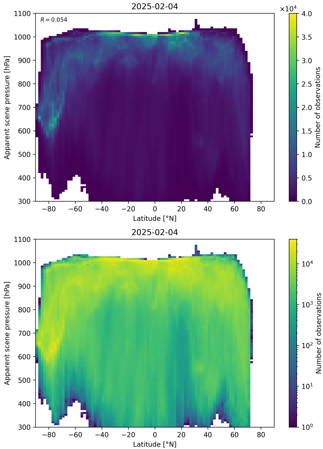
Figure 88: Scatter density plot of “Latitude” against “Apparent scene pressure” for 2025-02-03 to 2025-02-05.
