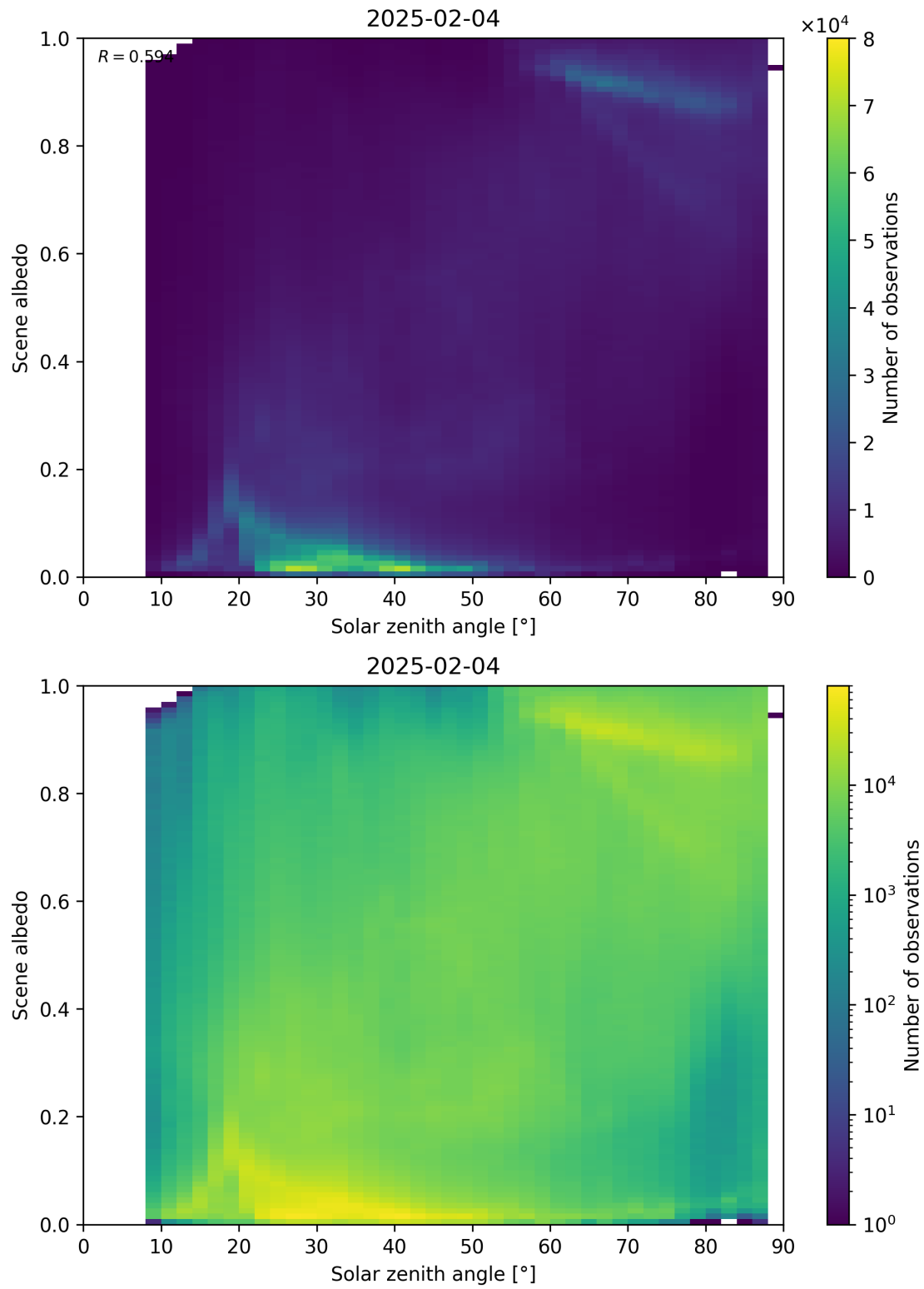
Figure 116: Scatter density plot of “Solar zenith angle” against “Scene albedo” for 2025-02-03 to 2025-02-05.
