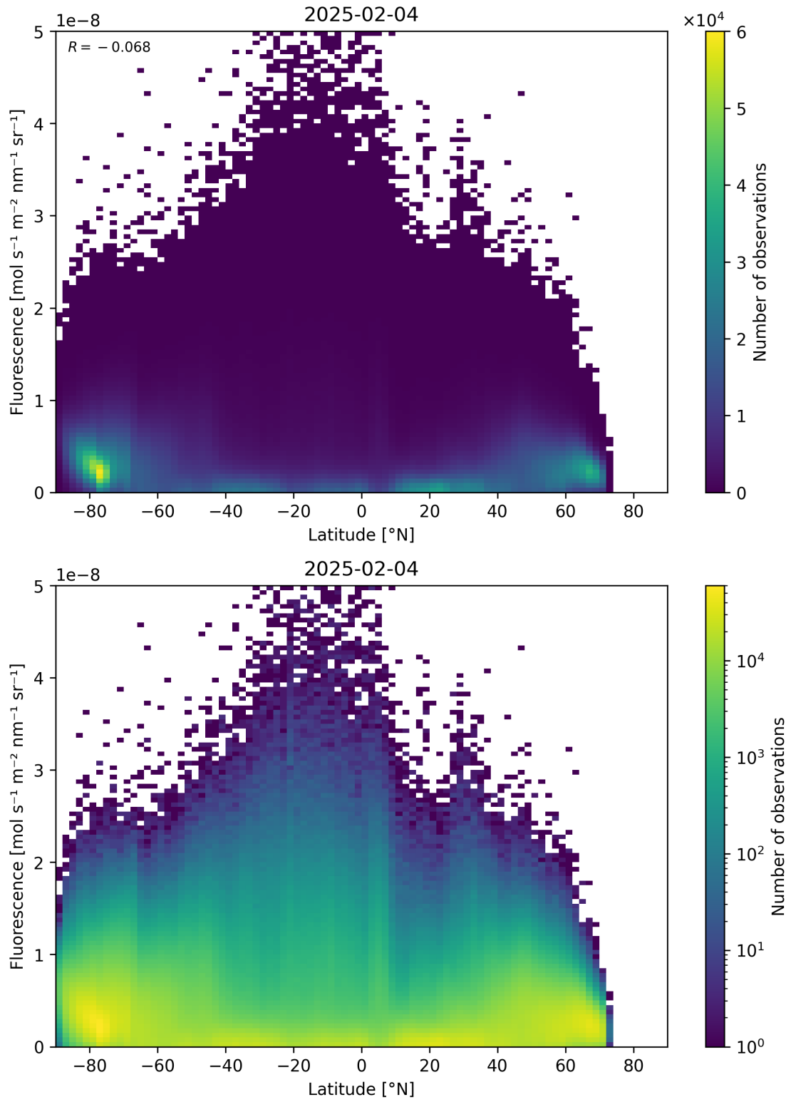
Figure 92: Scatter density plot of “Latitude” against “Fluorescence” for 2025-02-03 to 2025-02-05.
