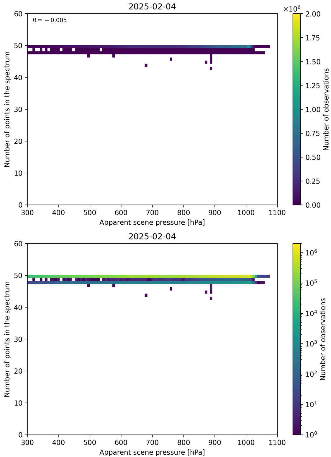
Figure 66: Scatter density plot of “Apparent scene pressure” against “Number of points in the spectrum” for 2025-02-03 to 2025-02-05.
