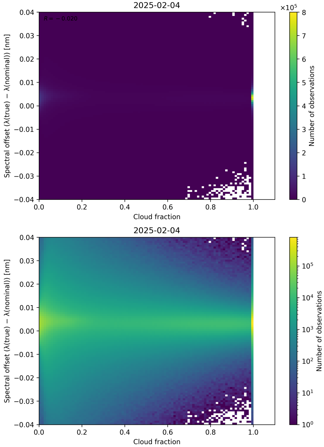
Figure 76: Scatter density plot of “Cloud fraction” against “Spectral offset ( \lambda_{\text{true}} - \lambda_{\text{nominal}} )” for 2025-02-03 to 2025-02-05.
