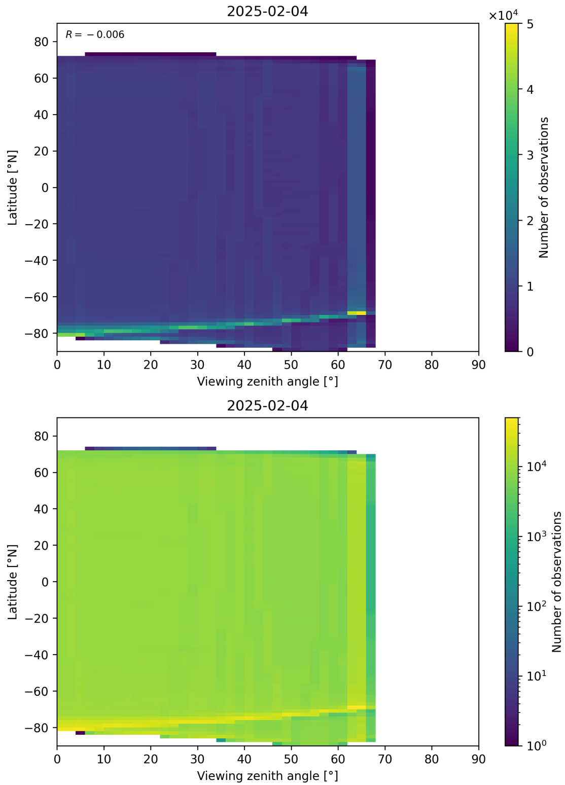
Figure 123: Scatter density plot of “Viewing zenith angle” against “Latitude” for 2025-02-03 to 2025-02-05.
