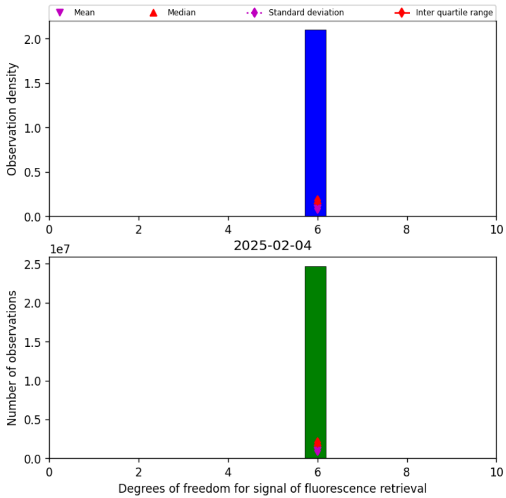
Figure 43: Histogram of “Degrees of freedom for signal of fluorescence retrieval” for 2025-02-03 to 2025-02-05
