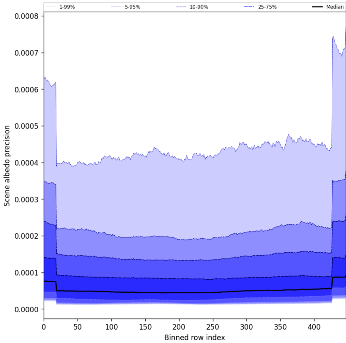
Figure 52: Along track statistics of “Scene albedo precision” for 2025-02-03 to 2025-02-05
