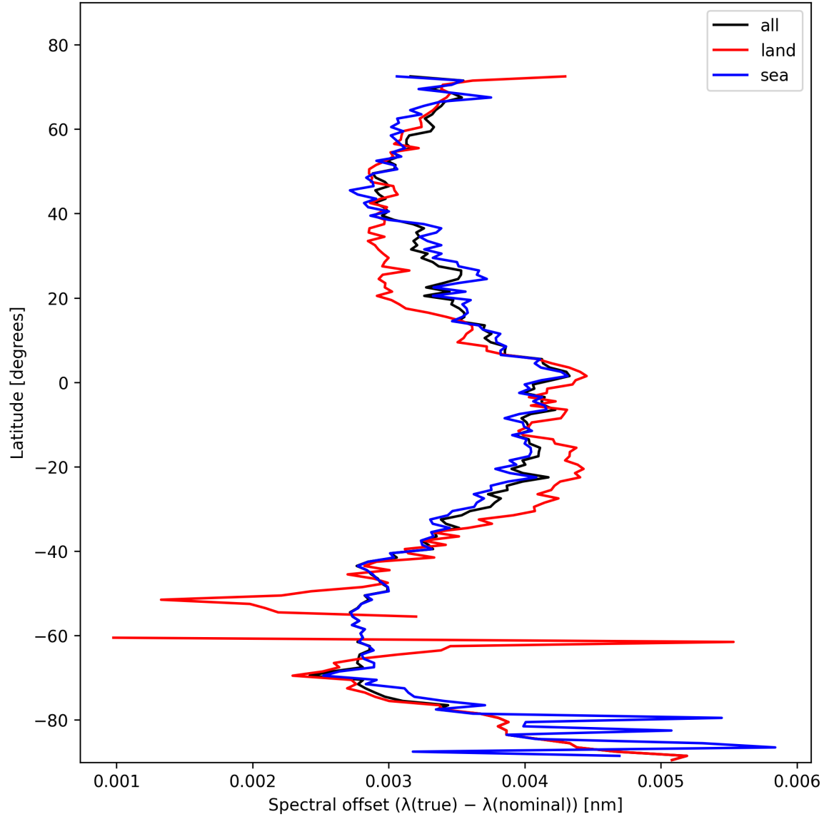
Figure 28: Zonal average of “Spectral offset ( \lambda_{\text{true}} - \lambda_{\text{nominal}} )” for 2025-02-03 to 2025-02-05.
