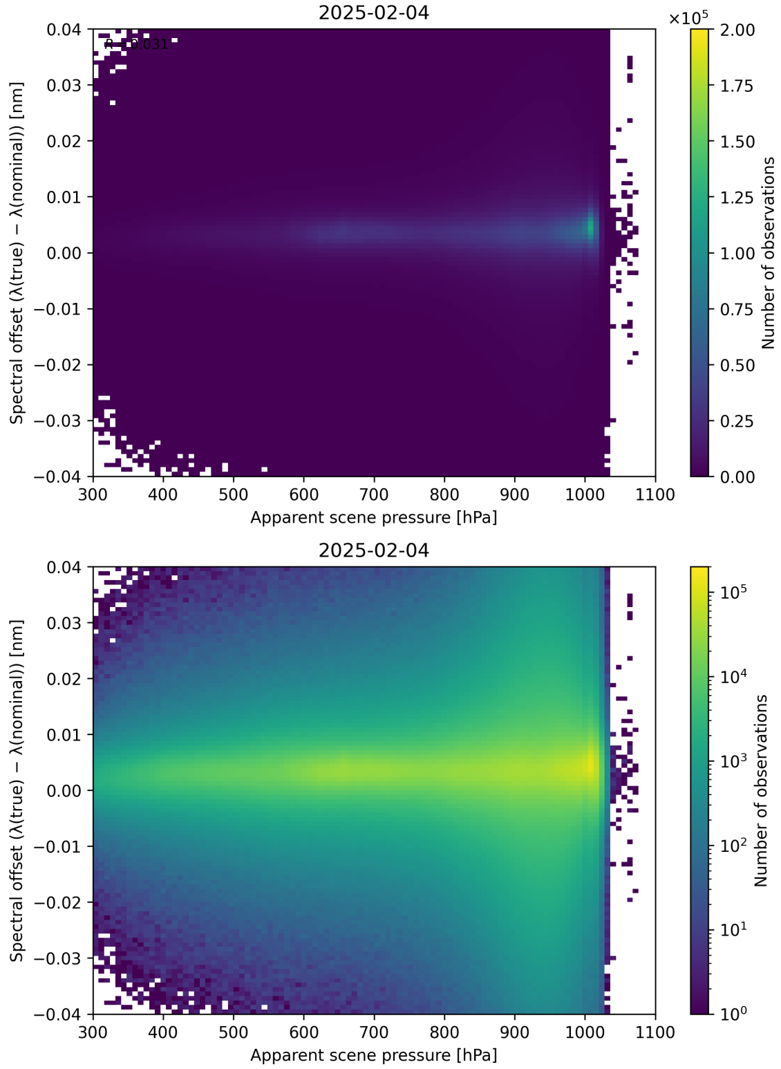
Figure 67: Scatter density plot of “Apparent scene pressure” against “Spectral offset ( \lambda_{\text{true}} - \lambda_{\text{nominal}} )” for 2025-02-03 to 2025-02-05.
