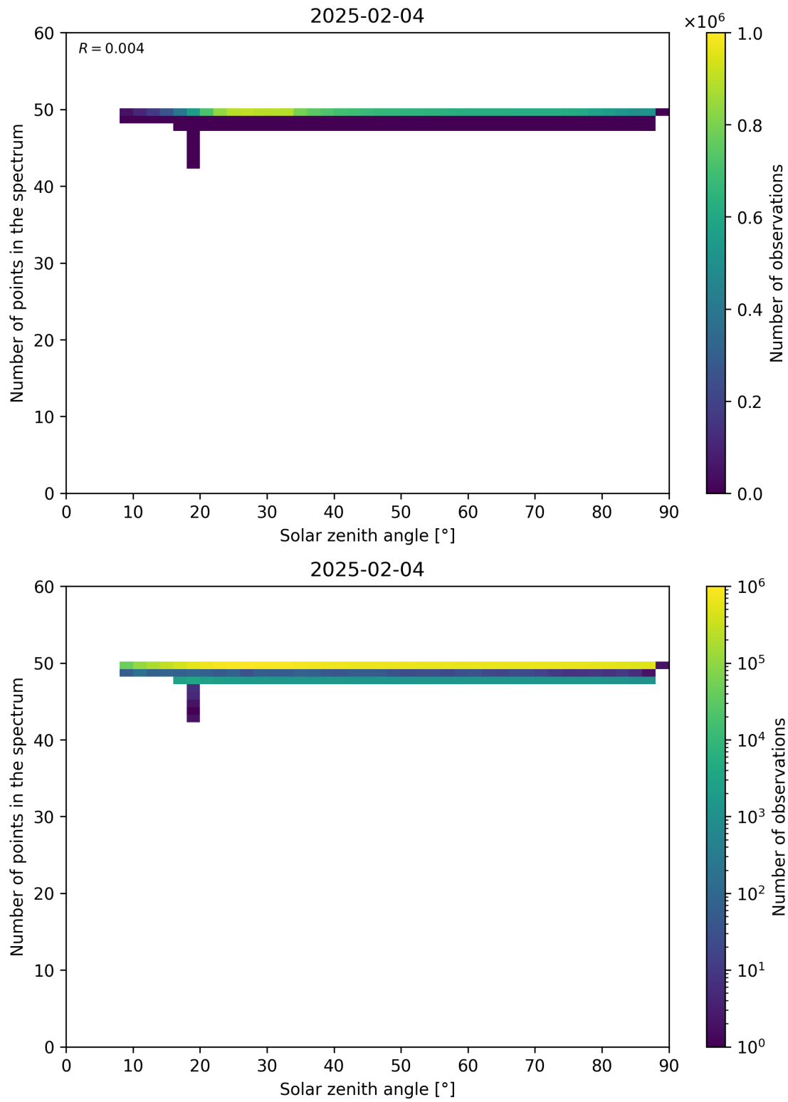
Figure 115: Scatter density plot of “Solar zenith angle” against “Number of points in the spectrum” for 2025-02-03 to 2025-02-05.
