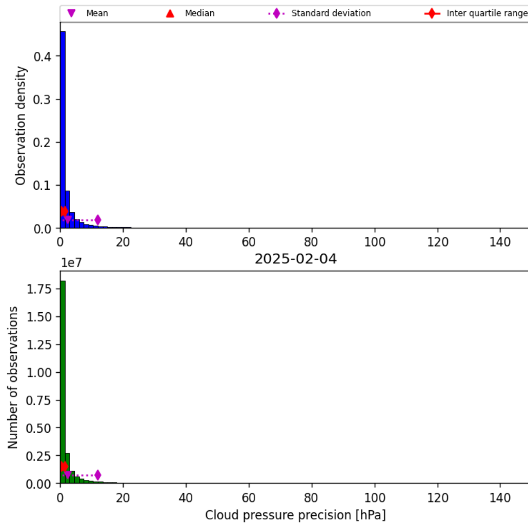
Figure 31: Histogram of “Cloud pressure precision” for 2025-02-03 to 2025-02-05
