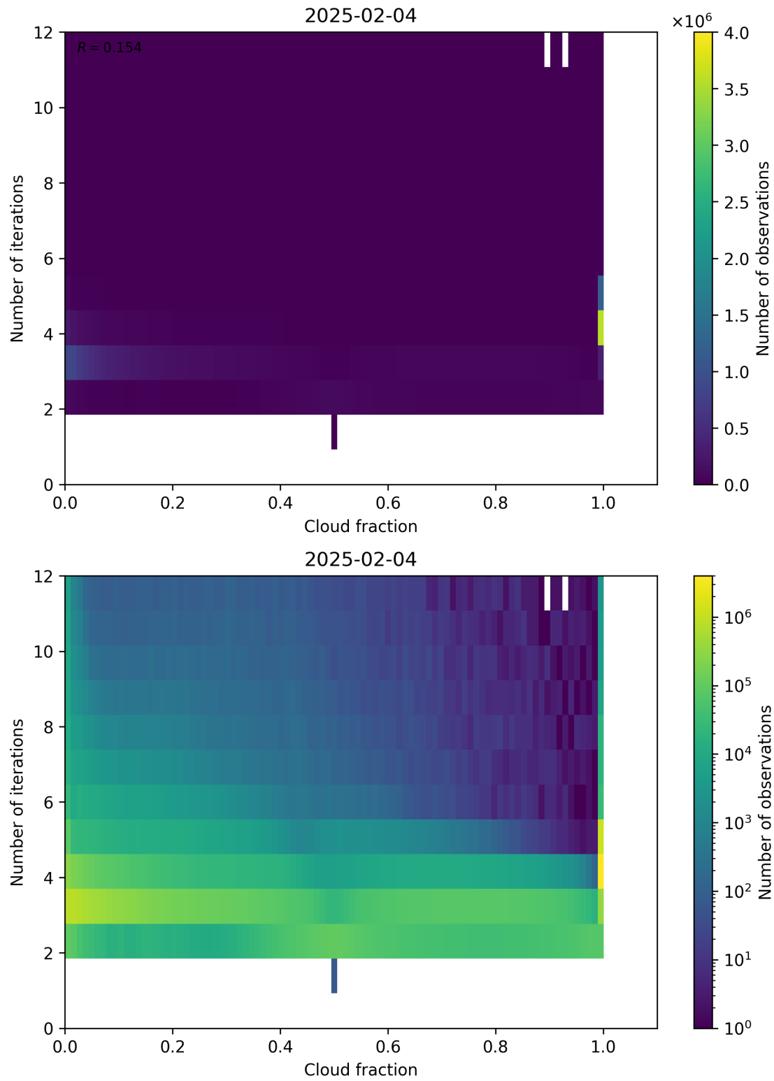
Figure 73: Scatter density plot of “Cloud fraction” against “Number of iterations” for 2025-02-03 to 2025-02-05.
