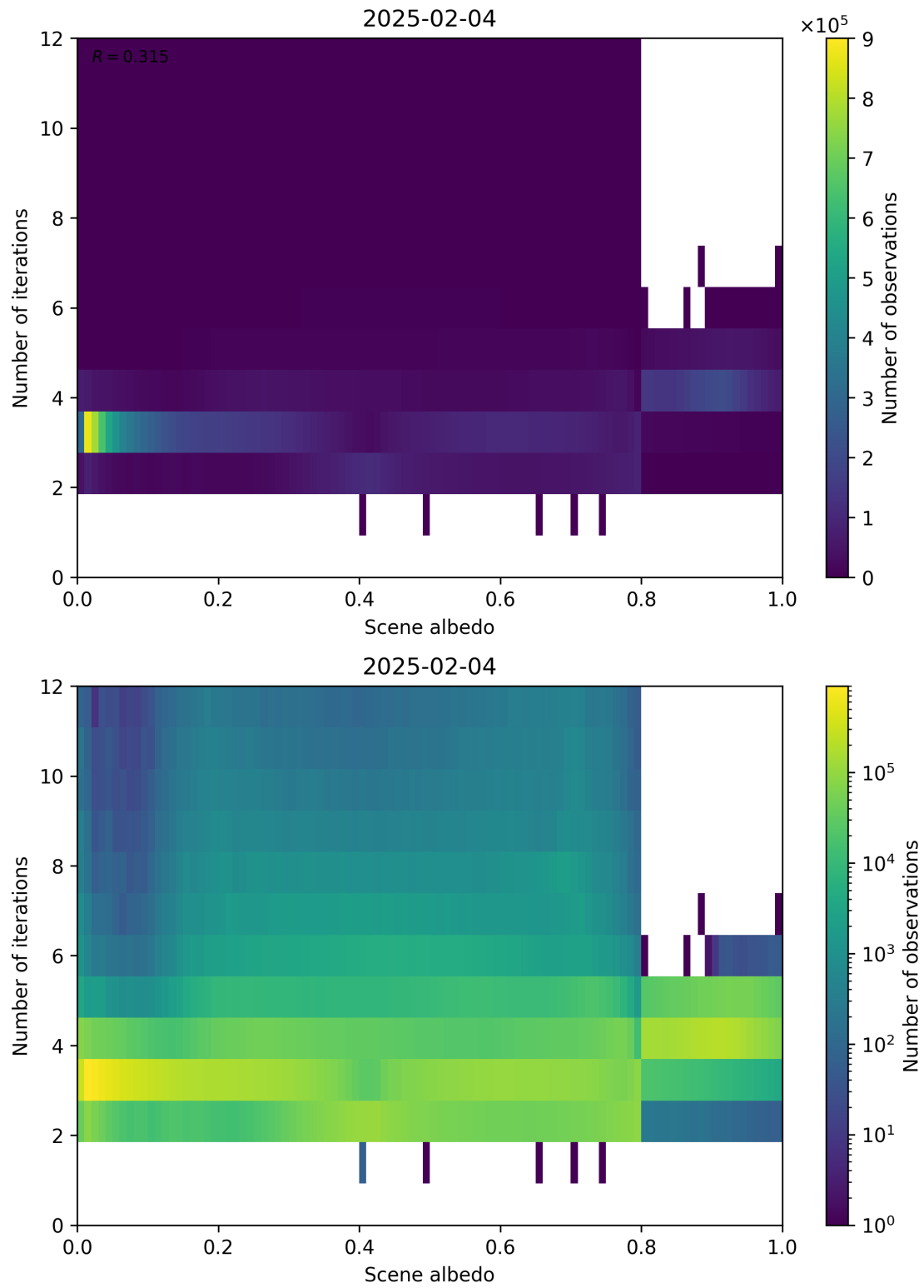
Figure 105: Scatter density plot of “Scene albedo” against “Number of iterations” for 2025-02-03 to 2025-02-05.
