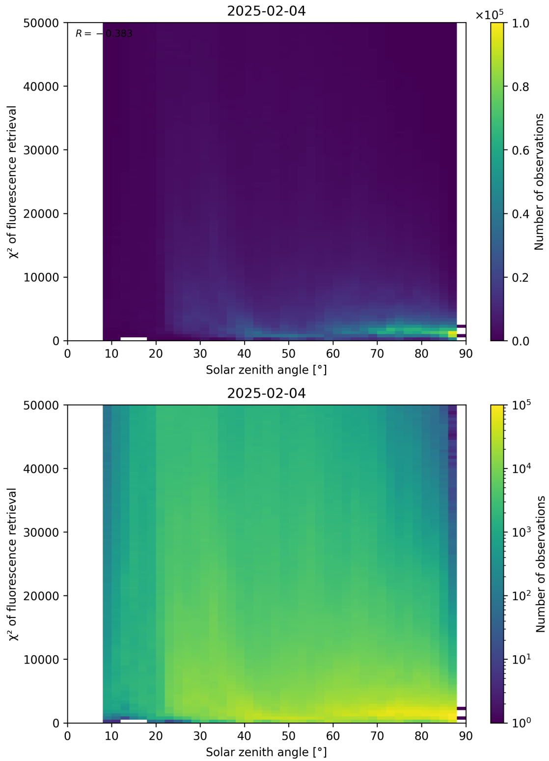
Figure 109: Scatter density plot of “Solar zenith angle” against “ \chi^2 of fluorescence retrieval” for 2025-02-03 to 2025-02-05.
