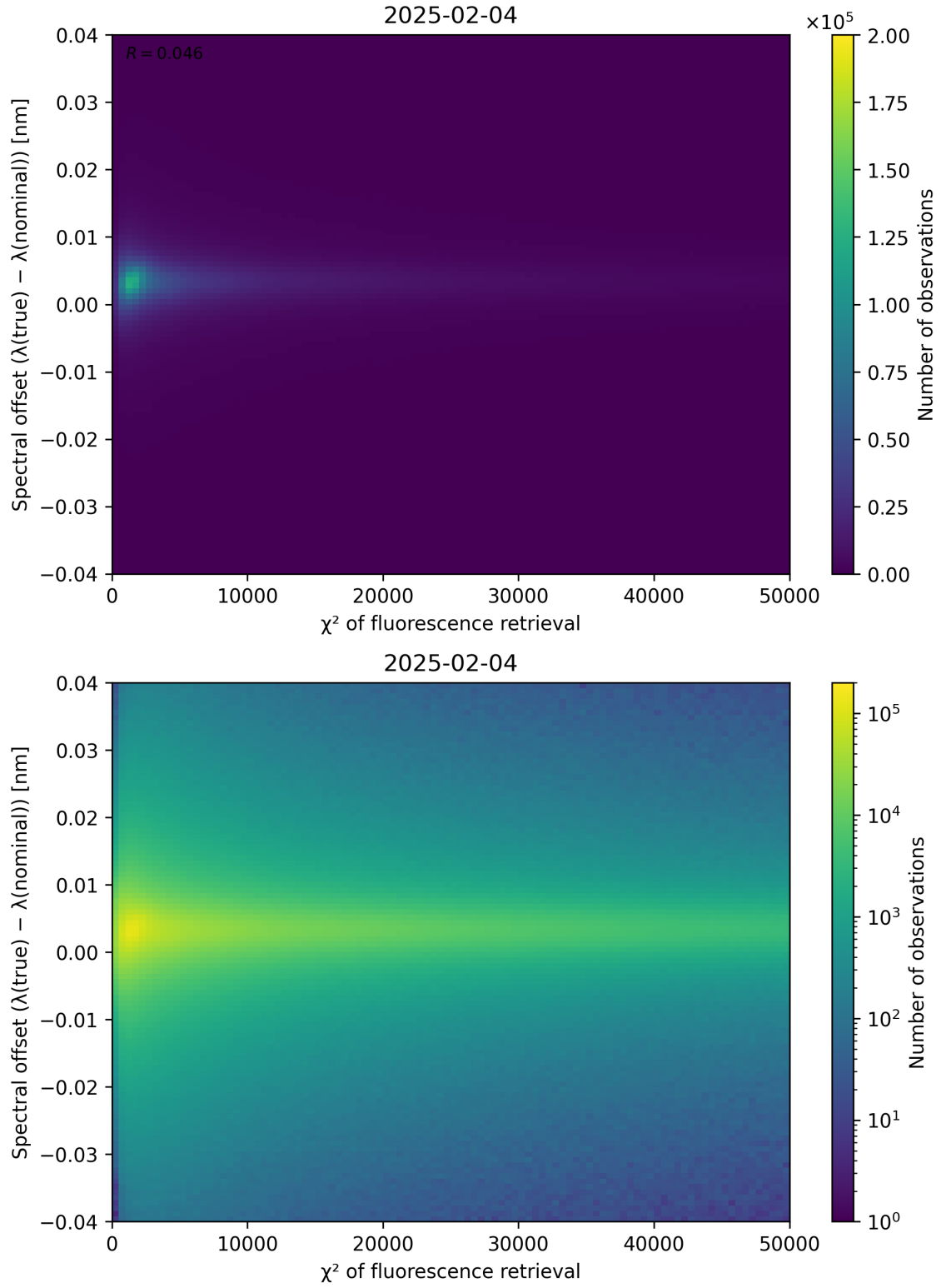
Figure 69: Scatter density plot of “ \chi^2 of fluorescence retrieval” against “Spectral offset ( \lambda_{\text{true}} - \lambda_{\text{nominal}} )” for 2025-02-03 to 2025-02-05.
