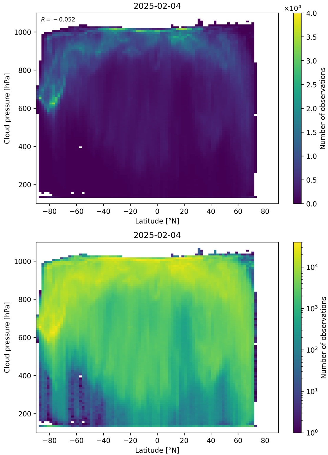
Figure 91: Scatter density plot of “Latitude” against “Cloud pressure” for 2025-02-03 to 2025-02-05.
