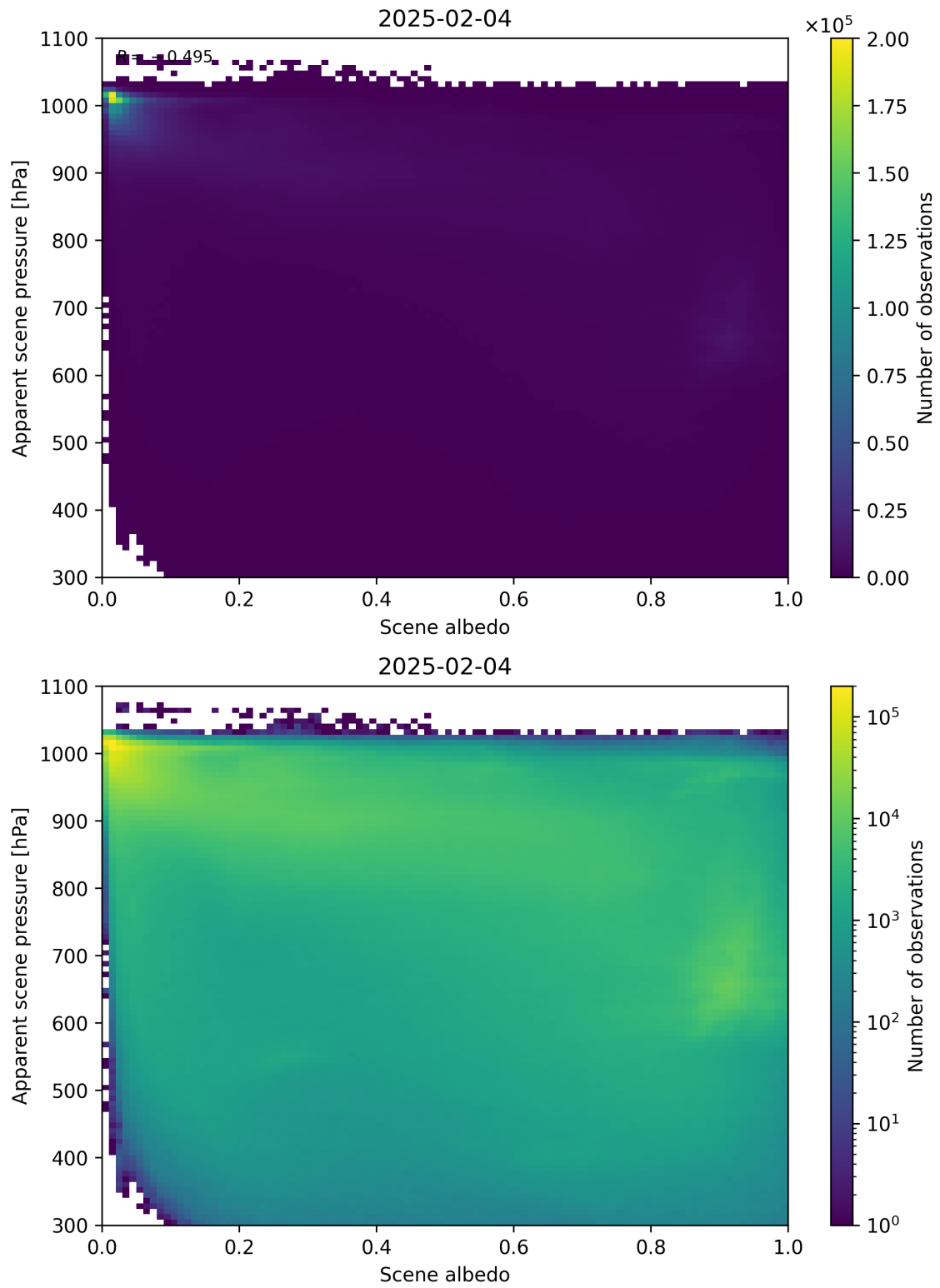
Figure 102: Scatter density plot of “Scene albedo” against “Apparent scene pressure” for 2025-02-03 to 2025-02-05.
