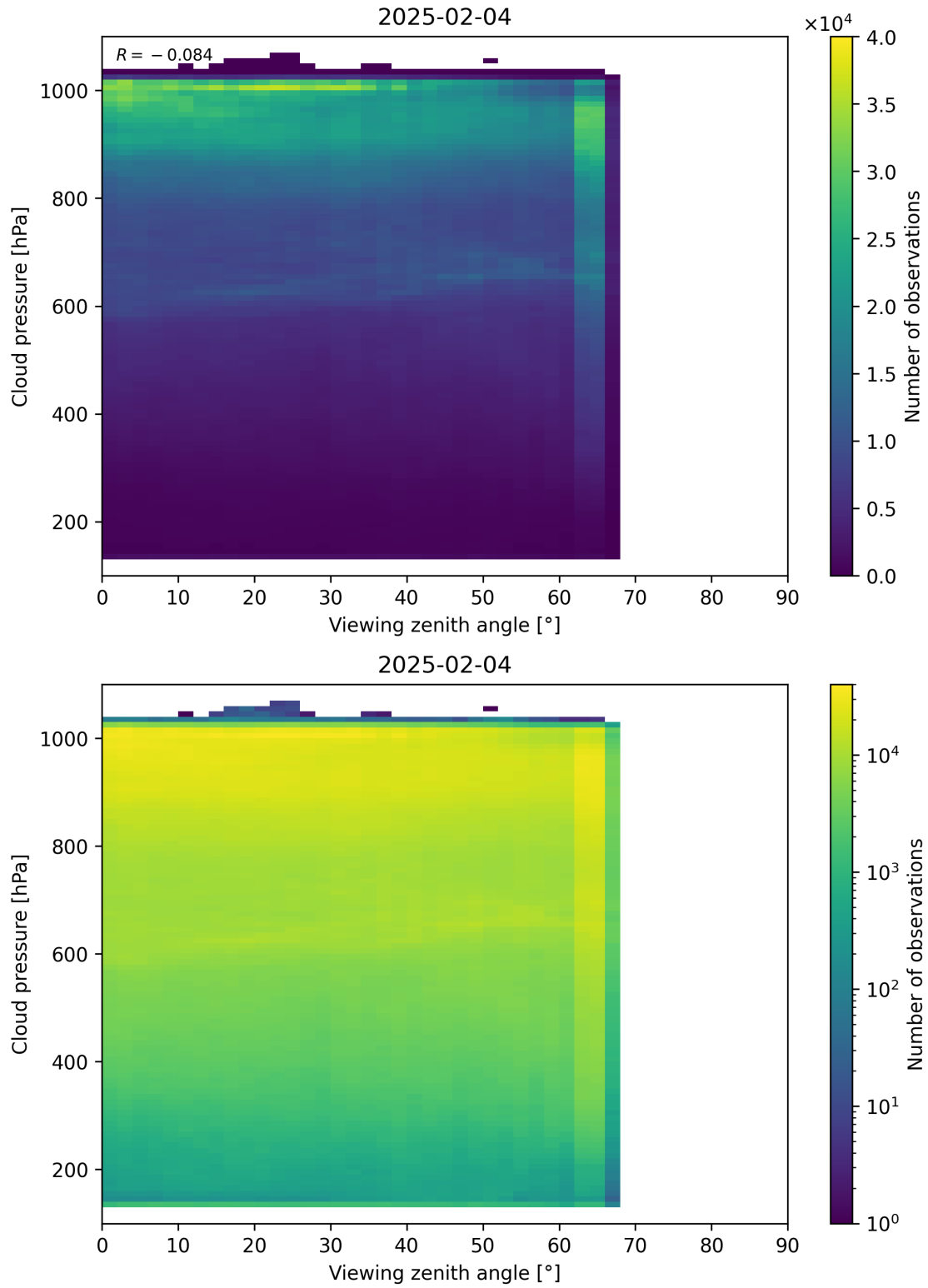
Figure 121: Scatter density plot of “Viewing zenith angle” against “Cloud pressure” for 2025-02-03 to 2025-02-05.
