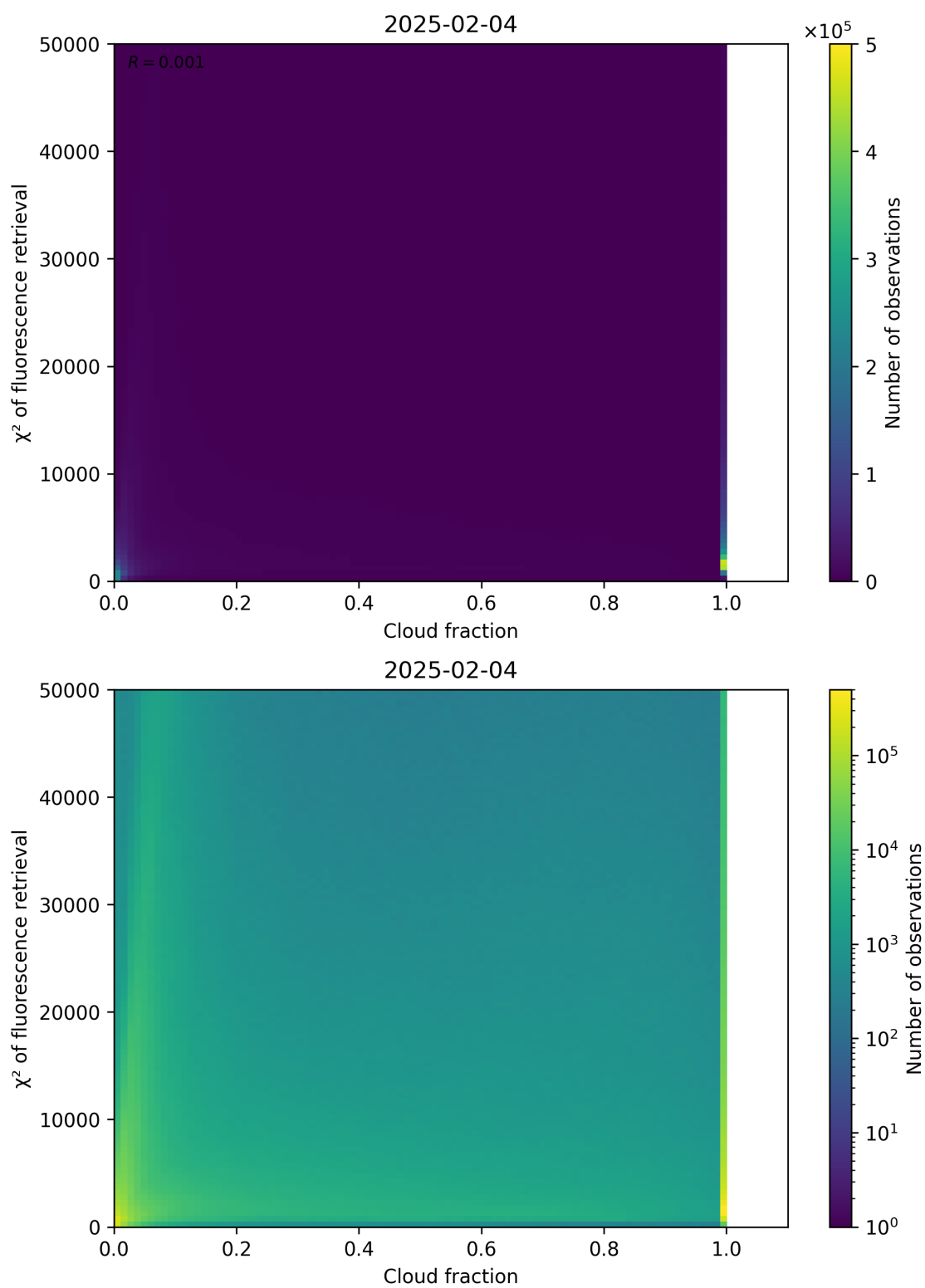
Figure 71: Scatter density plot of “Cloud fraction” against “ \chi^2 of fluorescence retrieval” for 2025-02-03 to 2025-02-05.
