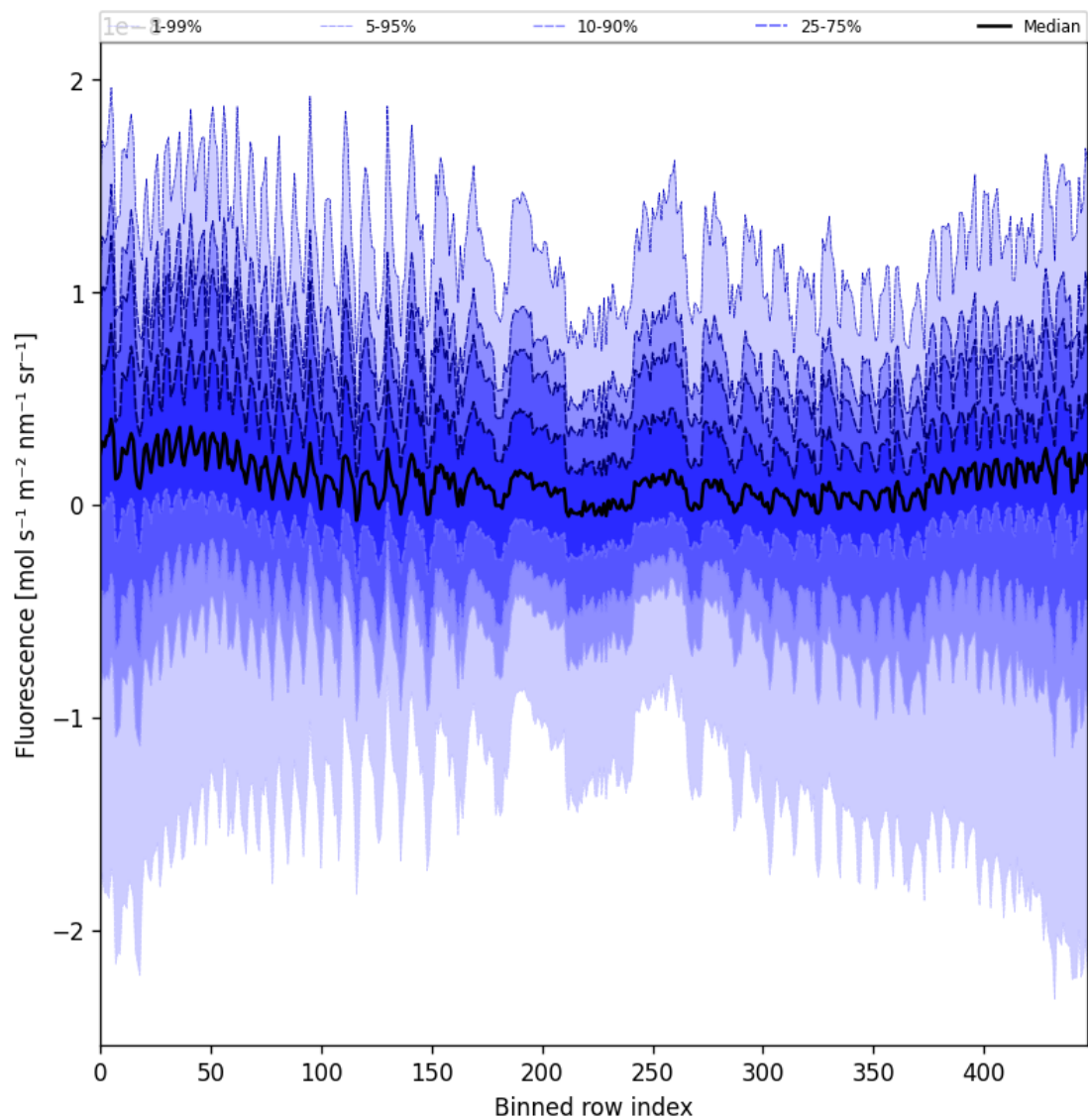
Figure 57: Along track statistics of “Fluorescence” for 2025-02-03 to 2025-02-05
