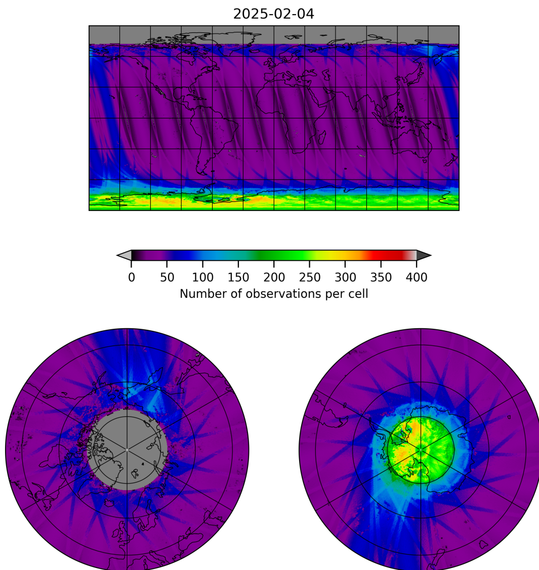
Figure 11: Map of the number of observations for 2025-02-03 to 2025-02-05
