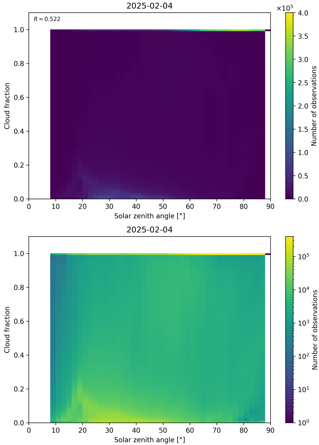
Figure 110: Scatter density plot of “Solar zenith angle” against “Cloud fraction” for 2025-02-03 to 2025-02-05.
