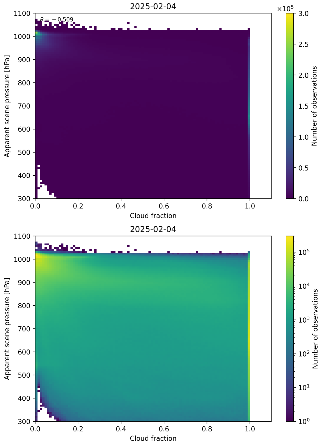
Figure 70: Scatter density plot of “Cloud fraction” against “Apparent scene pressure” for 2025-02-03 to 2025-02-05.
