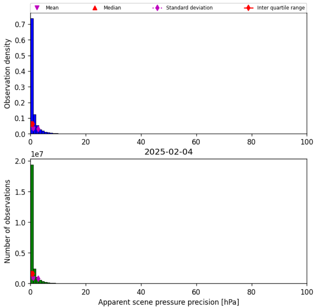
Figure 37: Histogram of “Apparent scene pressure precision” for 2025-02-03 to 2025-02-05
