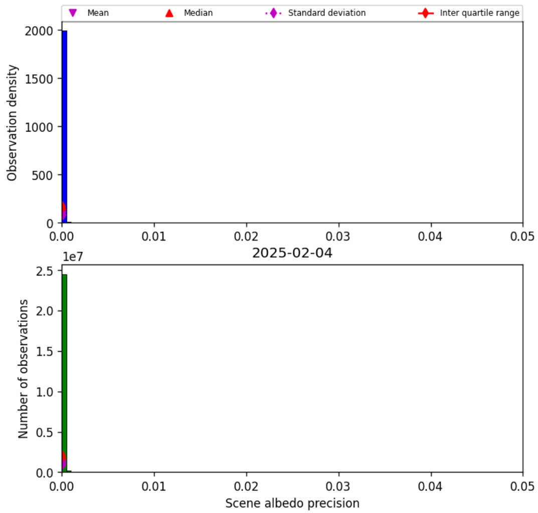
Figure 35: Histogram of “Scene albedo precision” for 2025-02-03 to 2025-02-05
