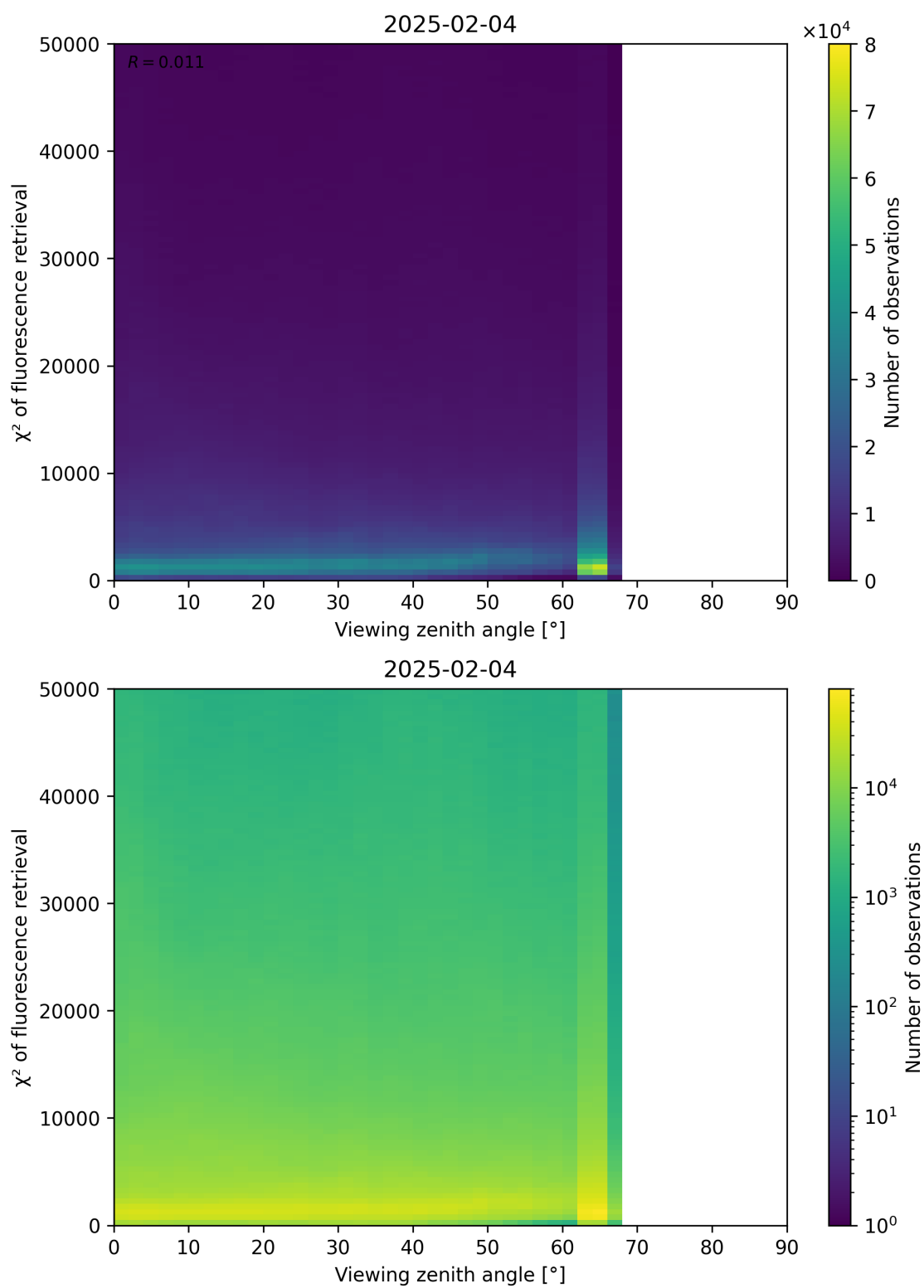
Figure 119: Scatter density plot of “Viewing zenith angle” against “ \chi^2 of fluorescence retrieval” for 2025-02-03 to 2025-02-05.
