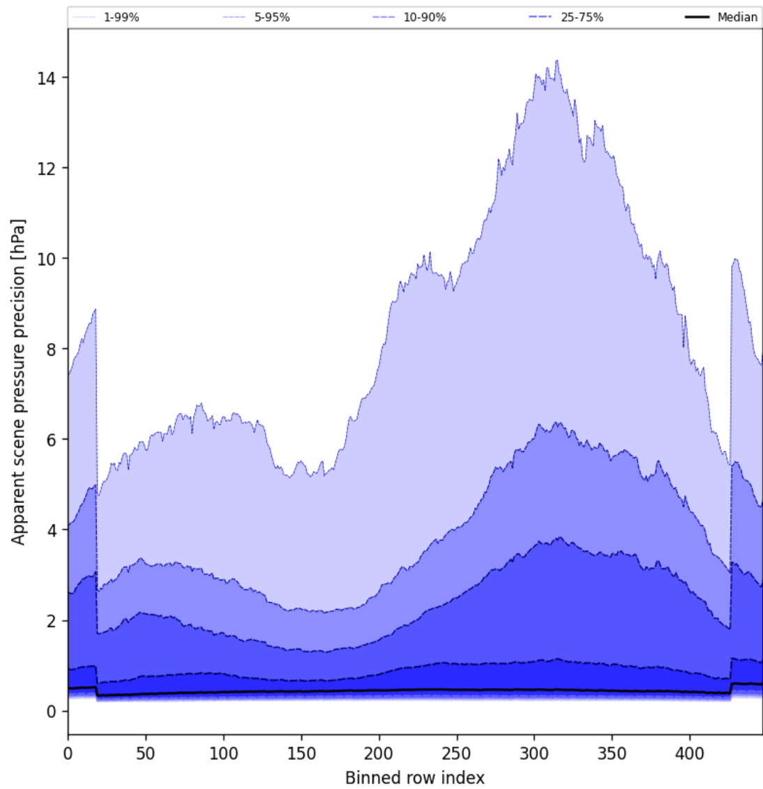
Figure 54: Along track statistics of “Apparent scene pressure precision” for 2025-02-03 to 2025-02-05
