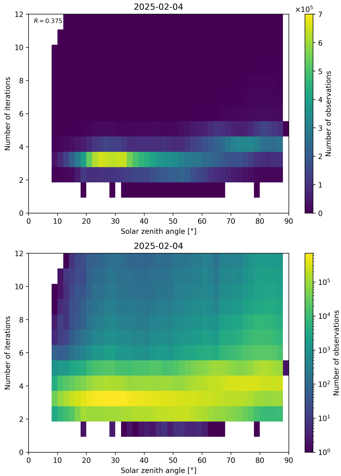
Figure 114: Scatter density plot of “Solar zenith angle” against “Number of iterations” for 2025-02-03 to 2025-02-05.
