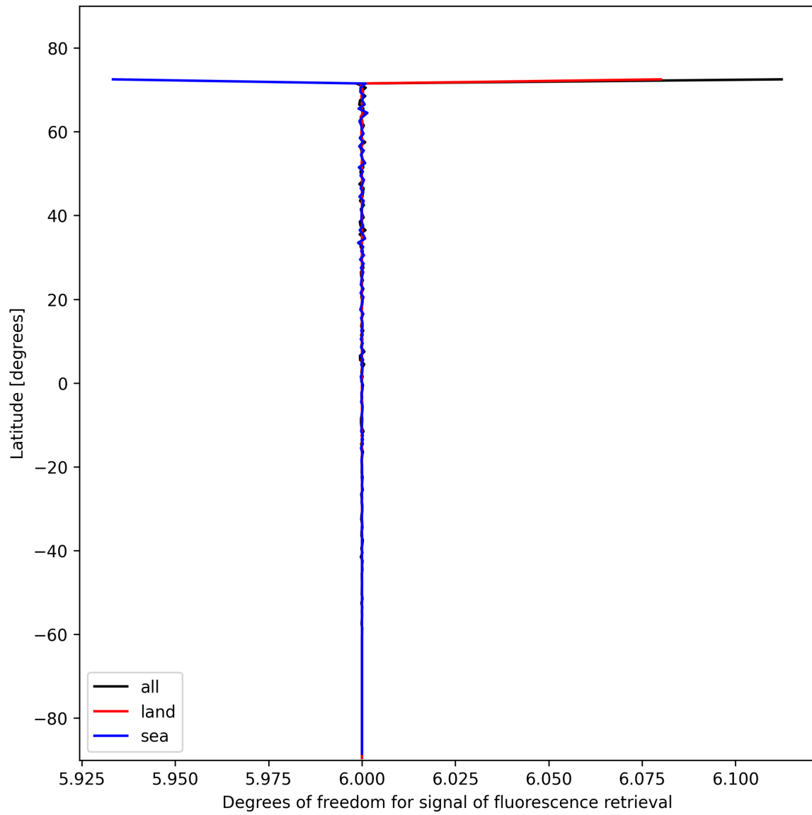
Figure 26: Zonal average of “Degrees of freedom for signal of fluorescence retrieval” for 2025-02-03 to 2025-02-05.
