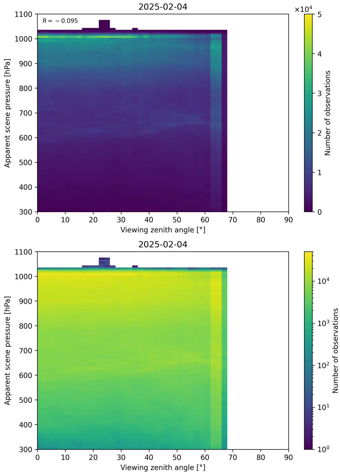
Figure 118: Scatter density plot of “Viewing zenith angle” against “Apparent scene pressure” for 2025-02-03 to 2025-02-05.
