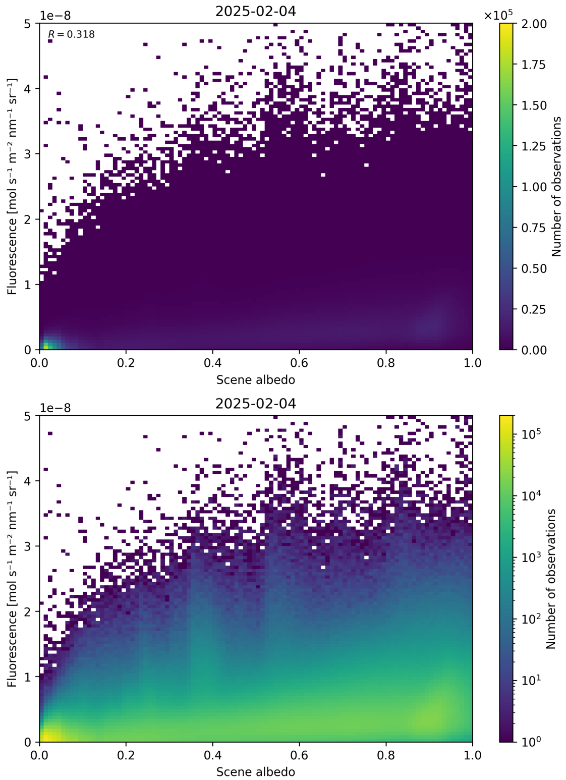
Figure 104: Scatter density plot of “Scene albedo” against “Fluorescence” for 2025-02-03 to 2025-02-05.
