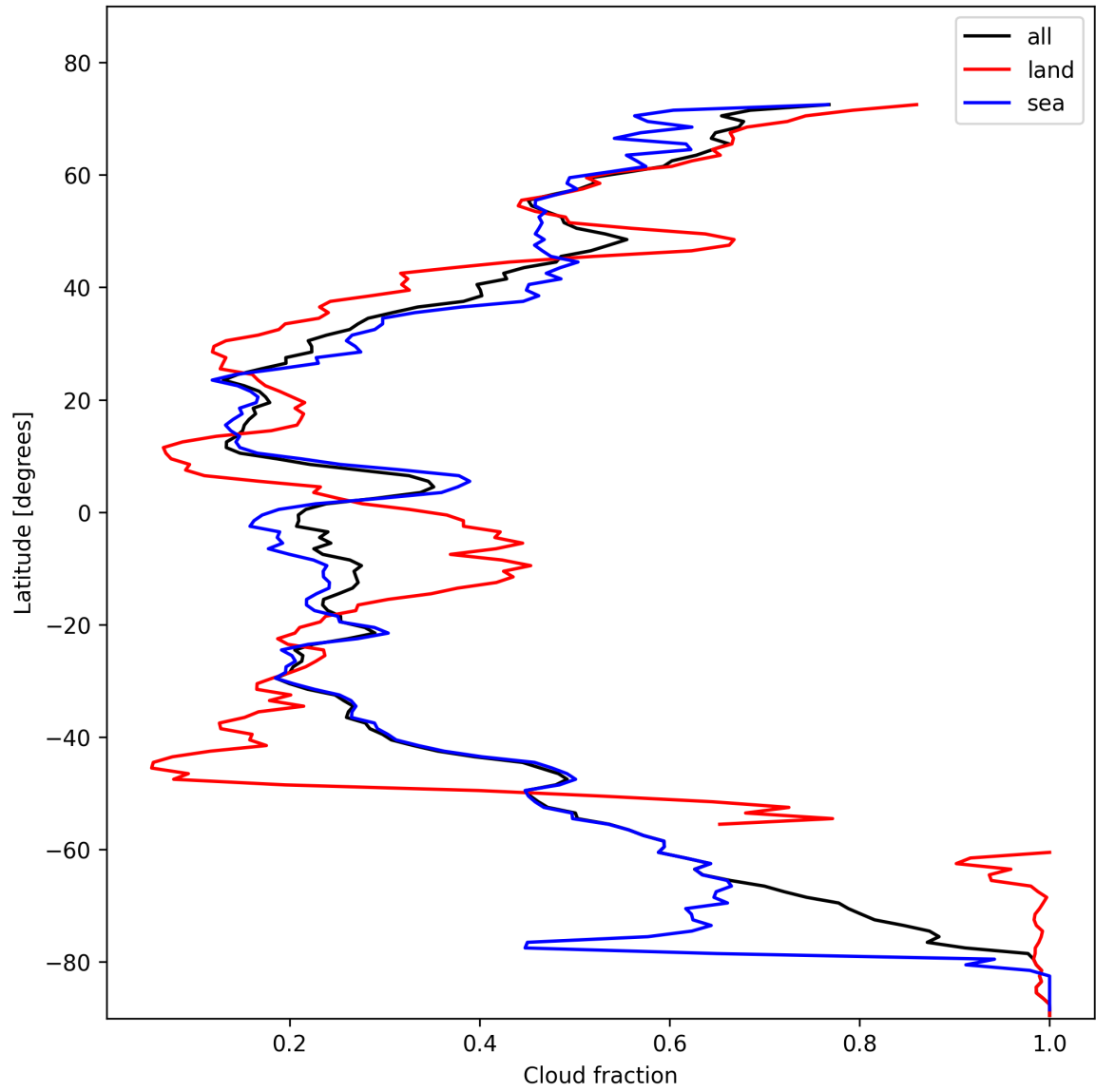
Figure 15: Zonal average of “Cloud fraction” for 2025-02-03 to 2025-02-05.
