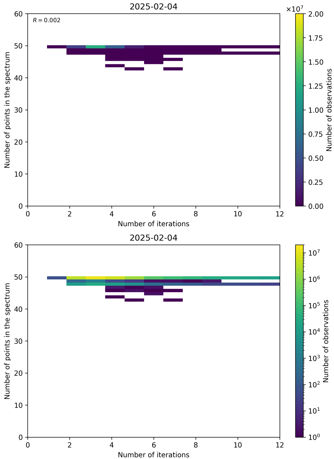
Figure 99: Scatter density plot of “Number of iterations” against “Number of points in the spectrum” for 2025-02-03 to 2025-02-05.
