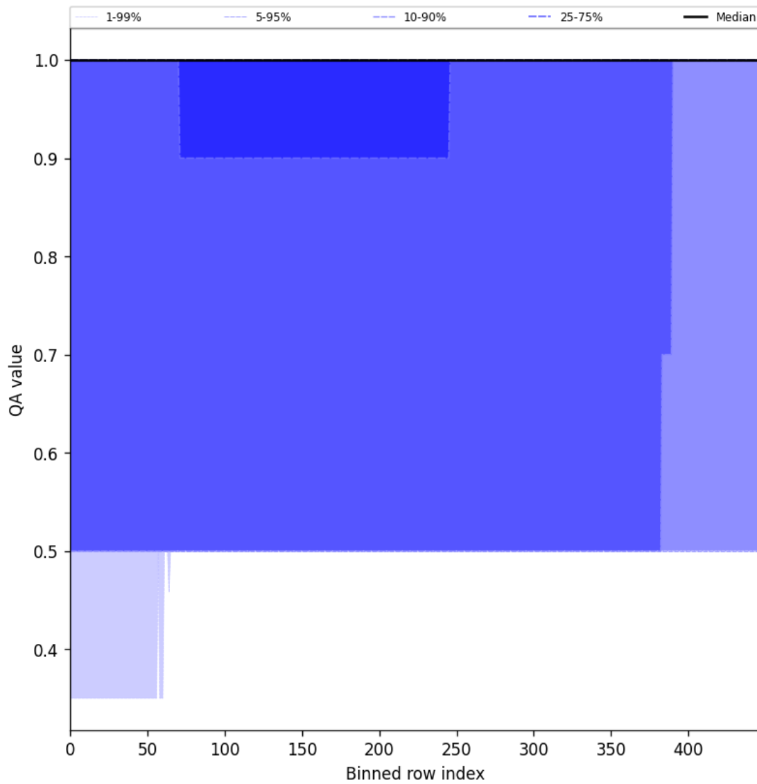
Figure 46: Along track statistics of “QA value” for 2025-02-03 to 2025-02-05
