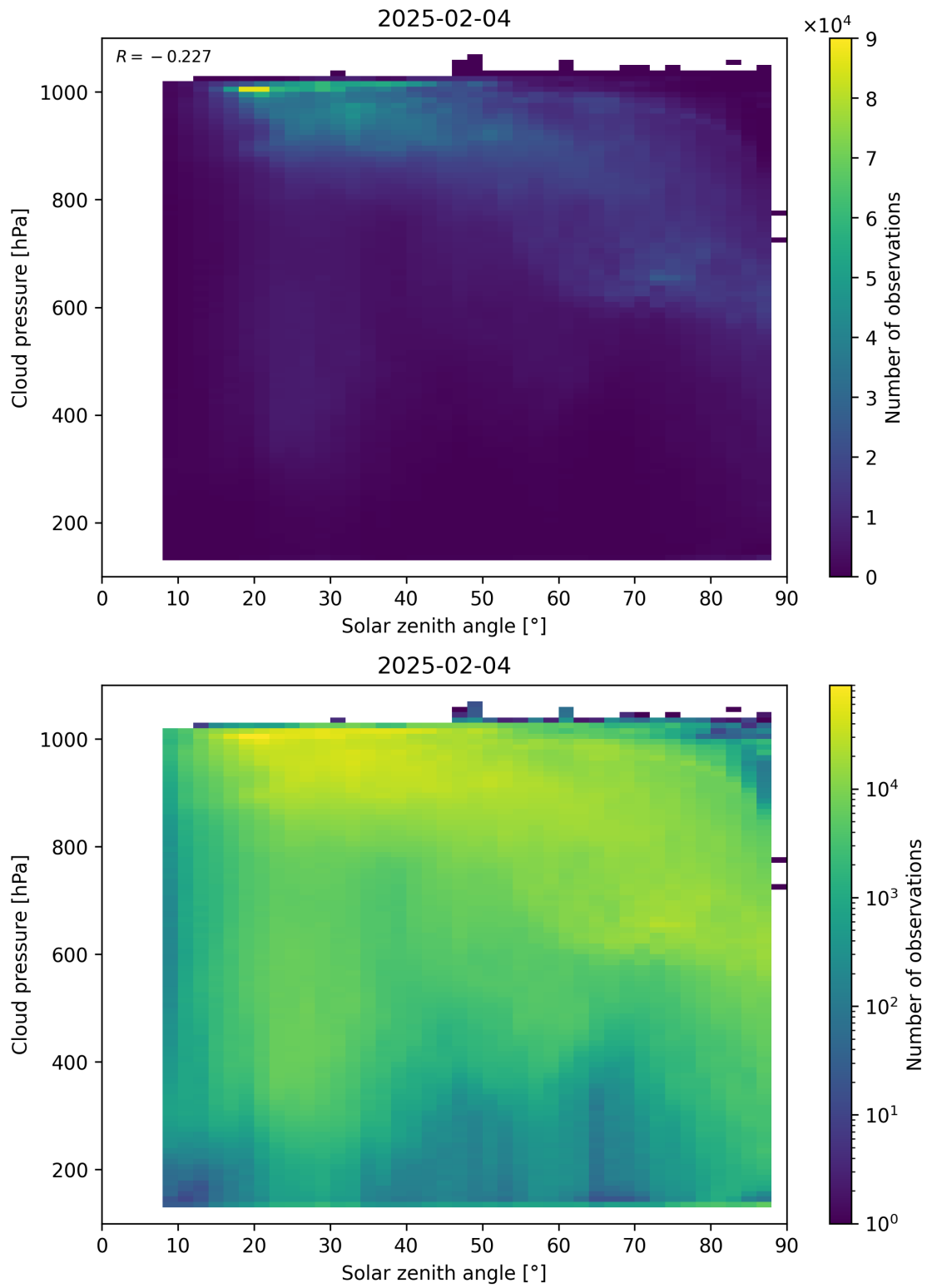
Figure 111: Scatter density plot of “Solar zenith angle” against “Cloud pressure” for 2025-02-03 to 2025-02-05.
