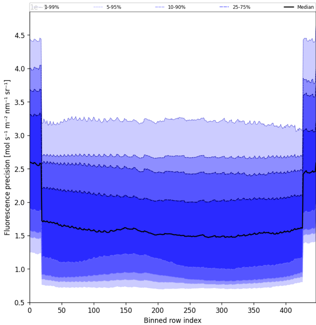
Figure 58: Along track statistics of “Fluorescence precision” for 2025-02-03 to 2025-02-05
