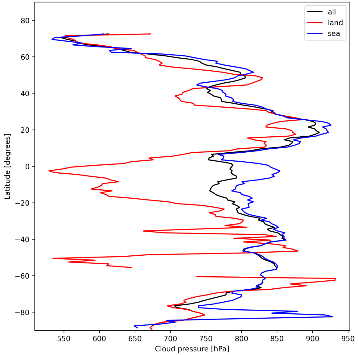
Figure 13: Zonal average of “Cloud pressure” for 2025-02-03 to 2025-02-05.
