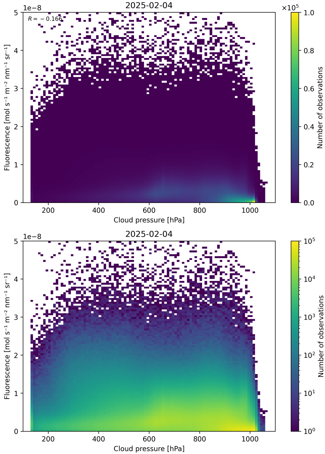
Figure 80: Scatter density plot of “Cloud pressure” against “Fluorescence” for 2025-02-03 to 2025-02-05.
