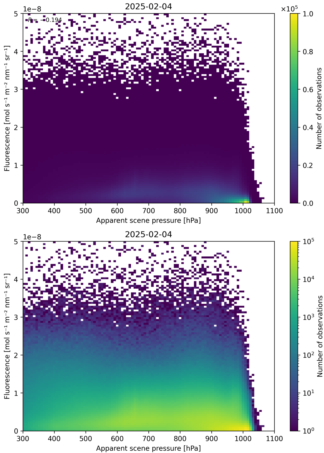
Figure 64: Scatter density plot of “Apparent scene pressure” against “Fluorescence” for 2025-02-03 to 2025-02-05.
