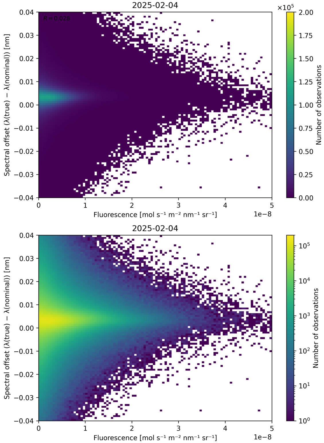
Figure 87: Scatter density plot of “Fluorescence” against “Spectral offset ( \lambda_{\text{true}} - \lambda_{\text{nominal}} )” for 2025-02-03 to 2025-02-05.
