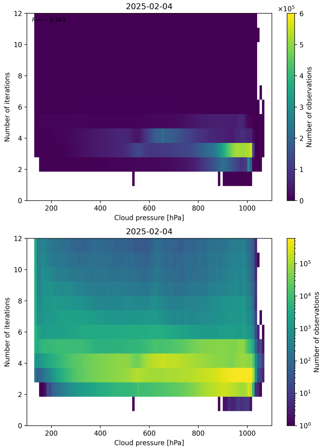
Figure 81: Scatter density plot of “Cloud pressure” against “Number of iterations” for 2025-02-03 to 2025-02-05.
