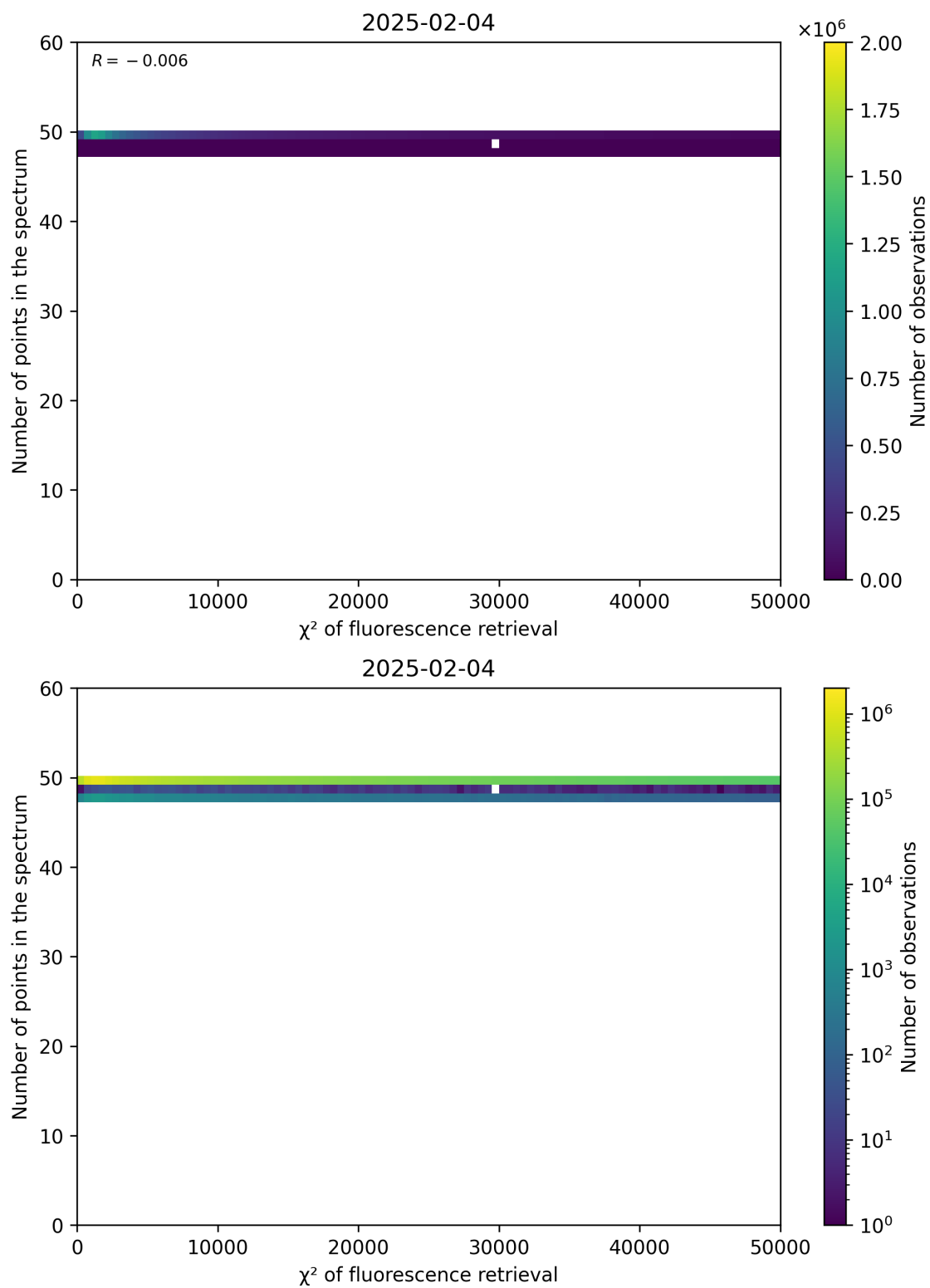
Figure 68: Scatter density plot of " \chi^2 of fluorescence retrieval" against "Number of points in the spectrum" for 2025-02-03 to 2025-02-05.
