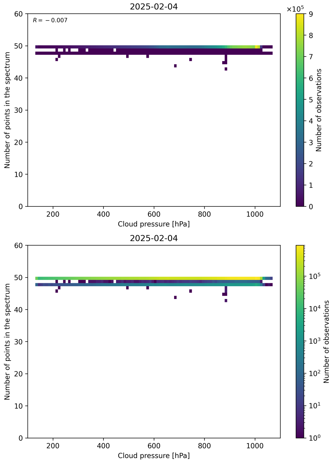
Figure 82: Scatter density plot of “Cloud pressure” against “Number of points in the spectrum” for 2025-02-03 to 2025-02-05.
