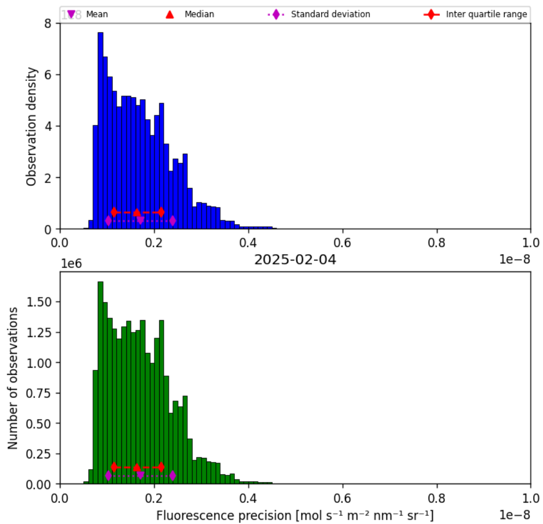
Figure 41: Histogram of “Fluorescence precision” for 2025-02-03 to 2025-02-05
