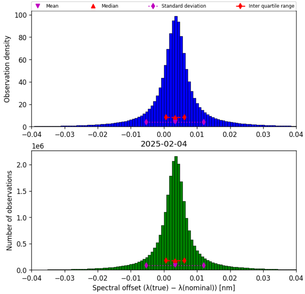
Figure 45: Histogram of “Spectral offset ( \lambda_{\text{true}} - \lambda_{\text{nominal}} )” for 2025-02-03 to 2025-02-05
