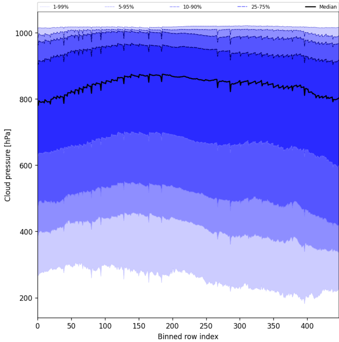
Figure 47: Along track statistics of “Cloud pressure” for 2025-02-03 to 2025-02-05
