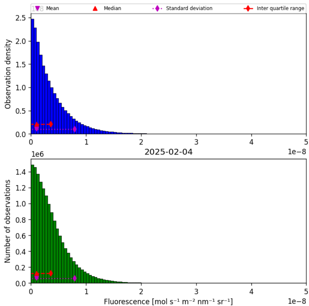
Figure 40: Histogram of “Fluorescence” for 2025-02-03 to 2025-02-05
