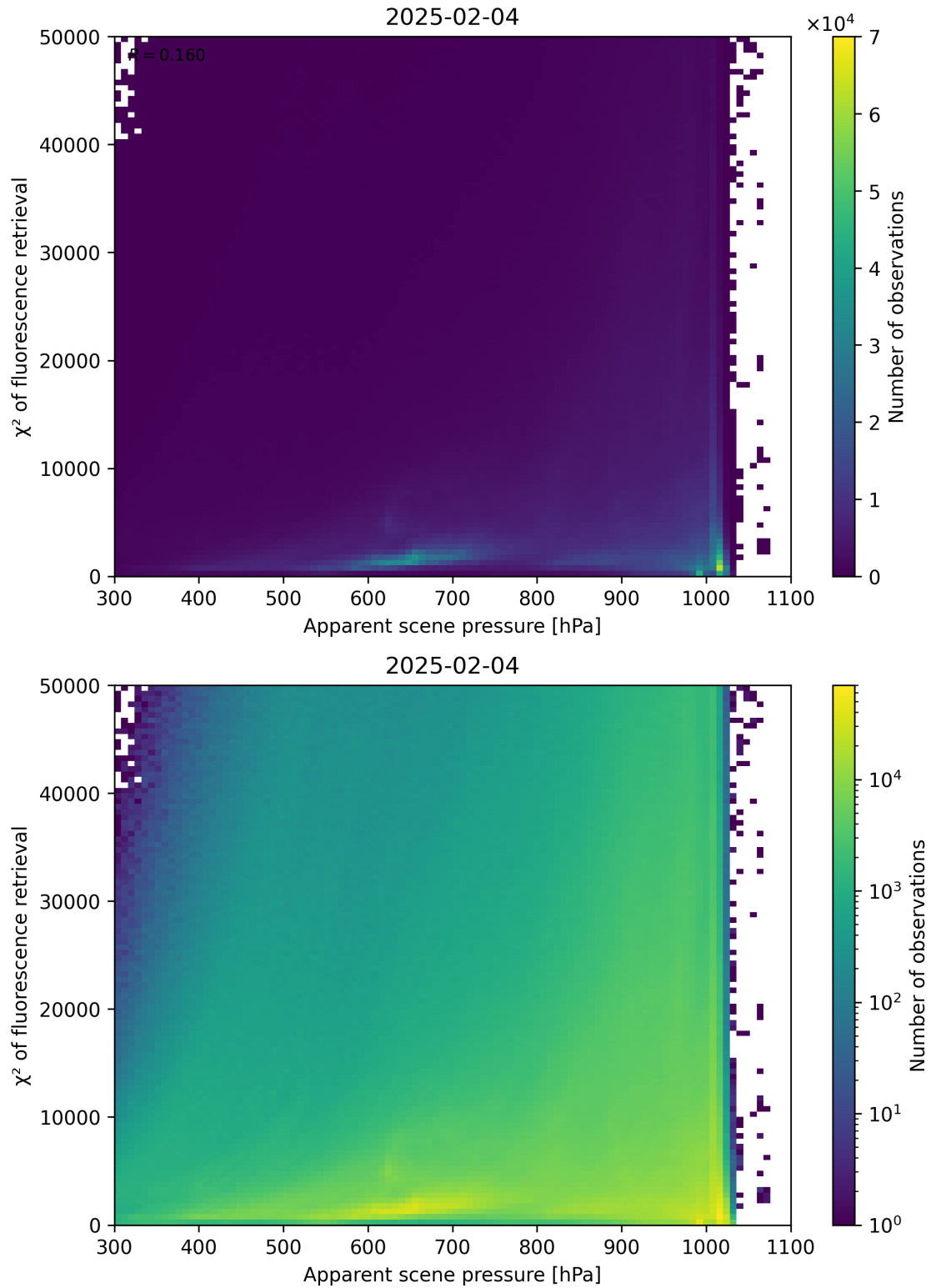
Figure 63: Scatter density plot of “Apparent scene pressure” against “ \chi^2 of fluorescence retrieval” for 2025-02-03 to 2025-02-05.
