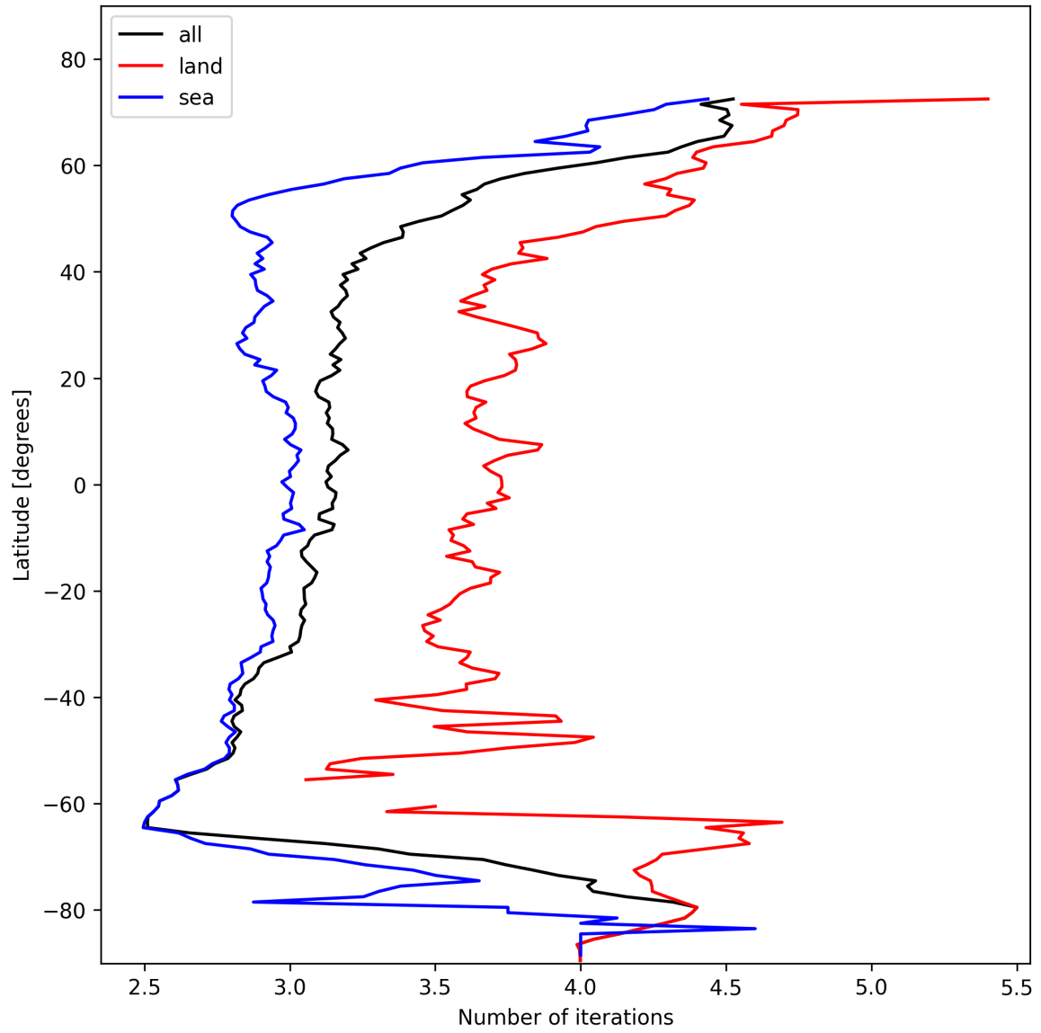
Figure 22: Zonal average of “Number of iterations” for 2025-02-03 to 2025-02-05.
