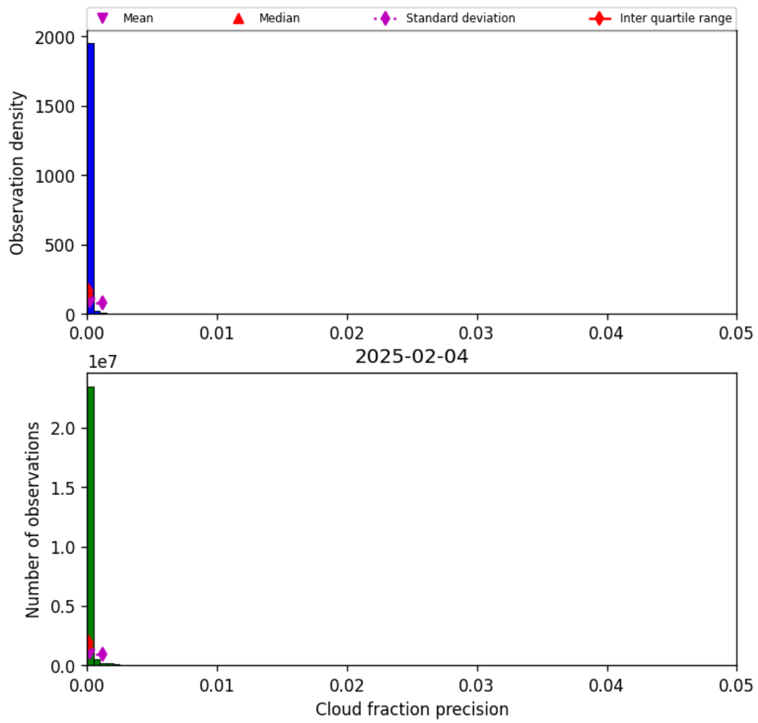
Figure 33: Histogram of “Cloud fraction precision” for 2025-02-03 to 2025-02-05
