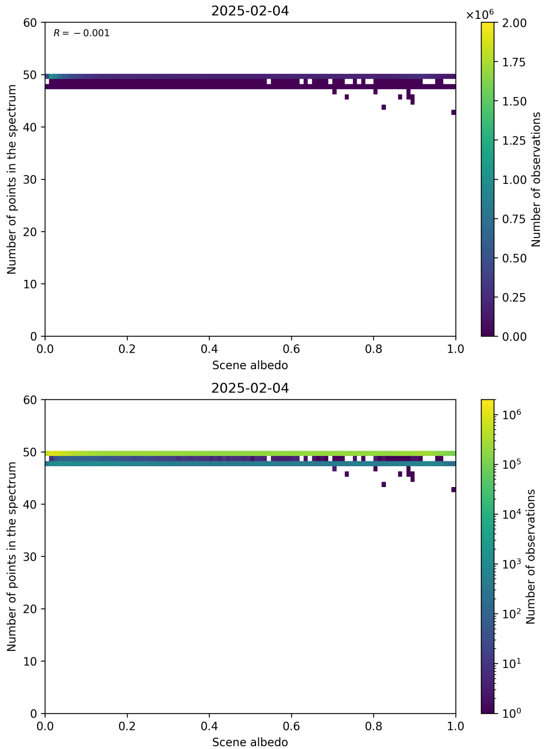
Figure 106: Scatter density plot of “Scene albedo” against “Number of points in the spectrum” for 2025-02-03 to 2025-02-05.
