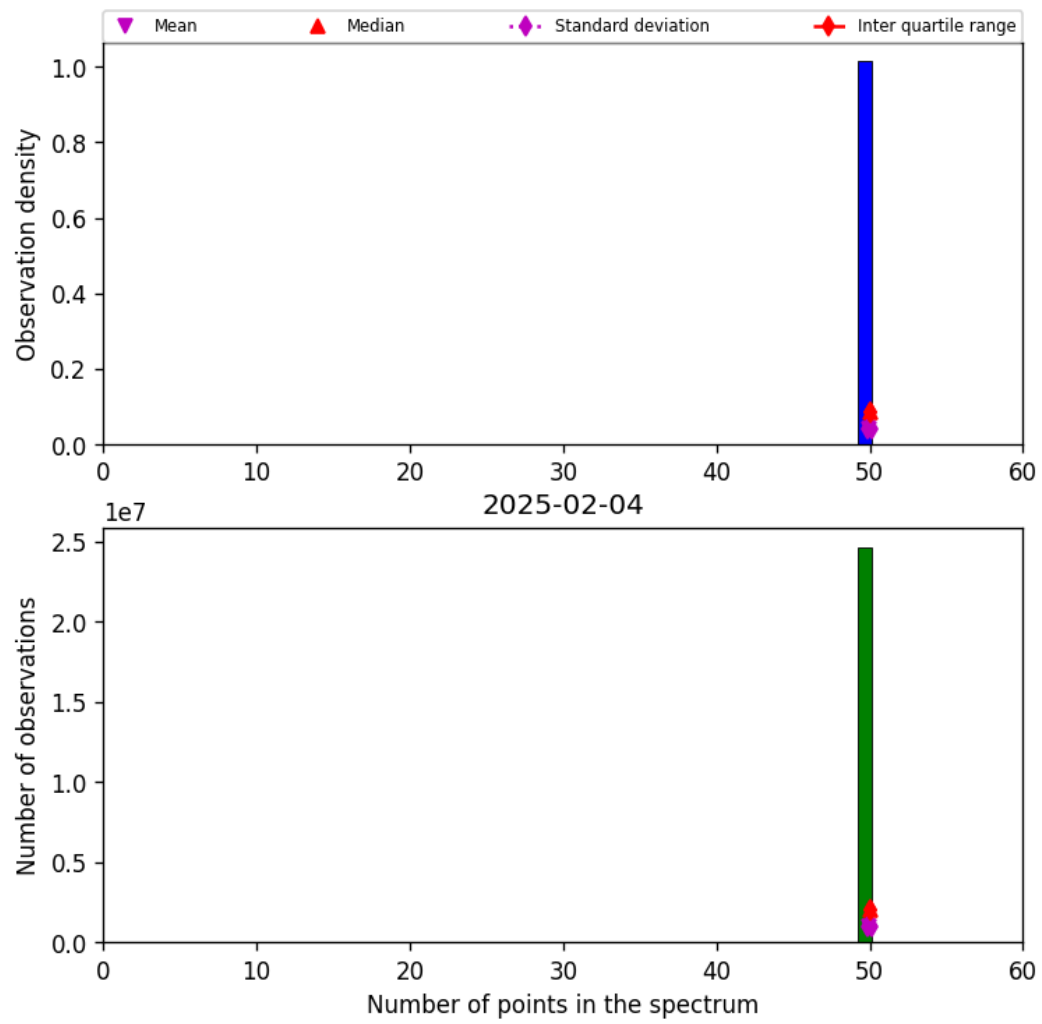
Figure 44: Histogram of “Number of points in the spectrum” for 2025-02-03 to 2025-02-05
