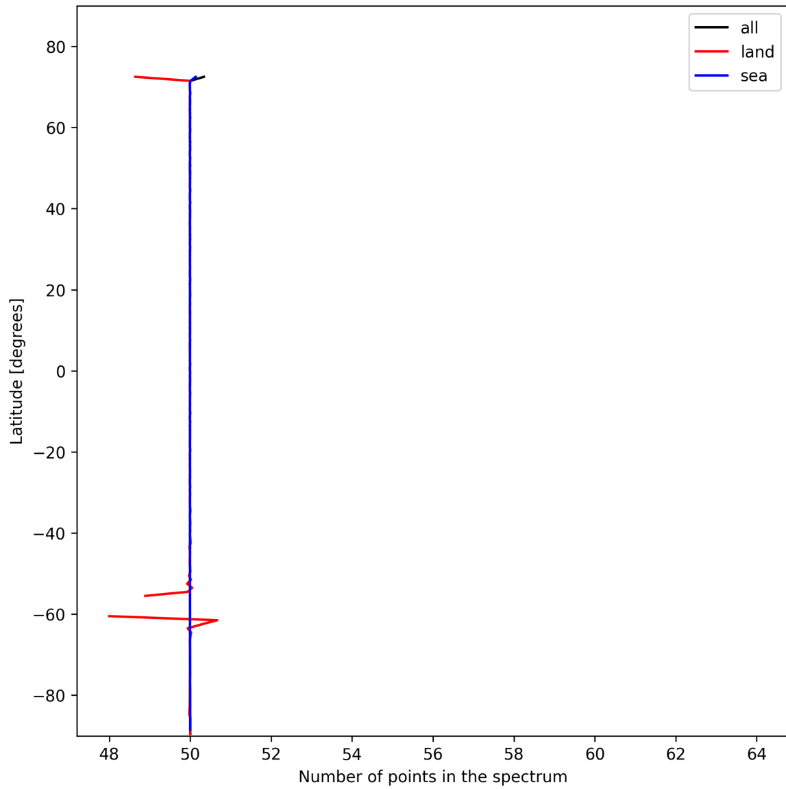
Figure 27: Zonal average of “Number of points in the spectrum” for 2025-02-03 to 2025-02-05.
