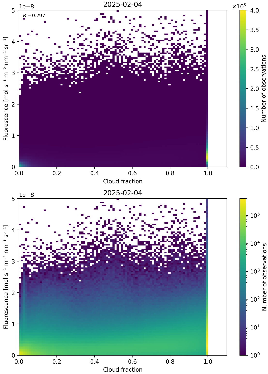
Figure 72: Scatter density plot of “Cloud fraction” against “Fluorescence” for 2025-02-03 to 2025-02-05.
