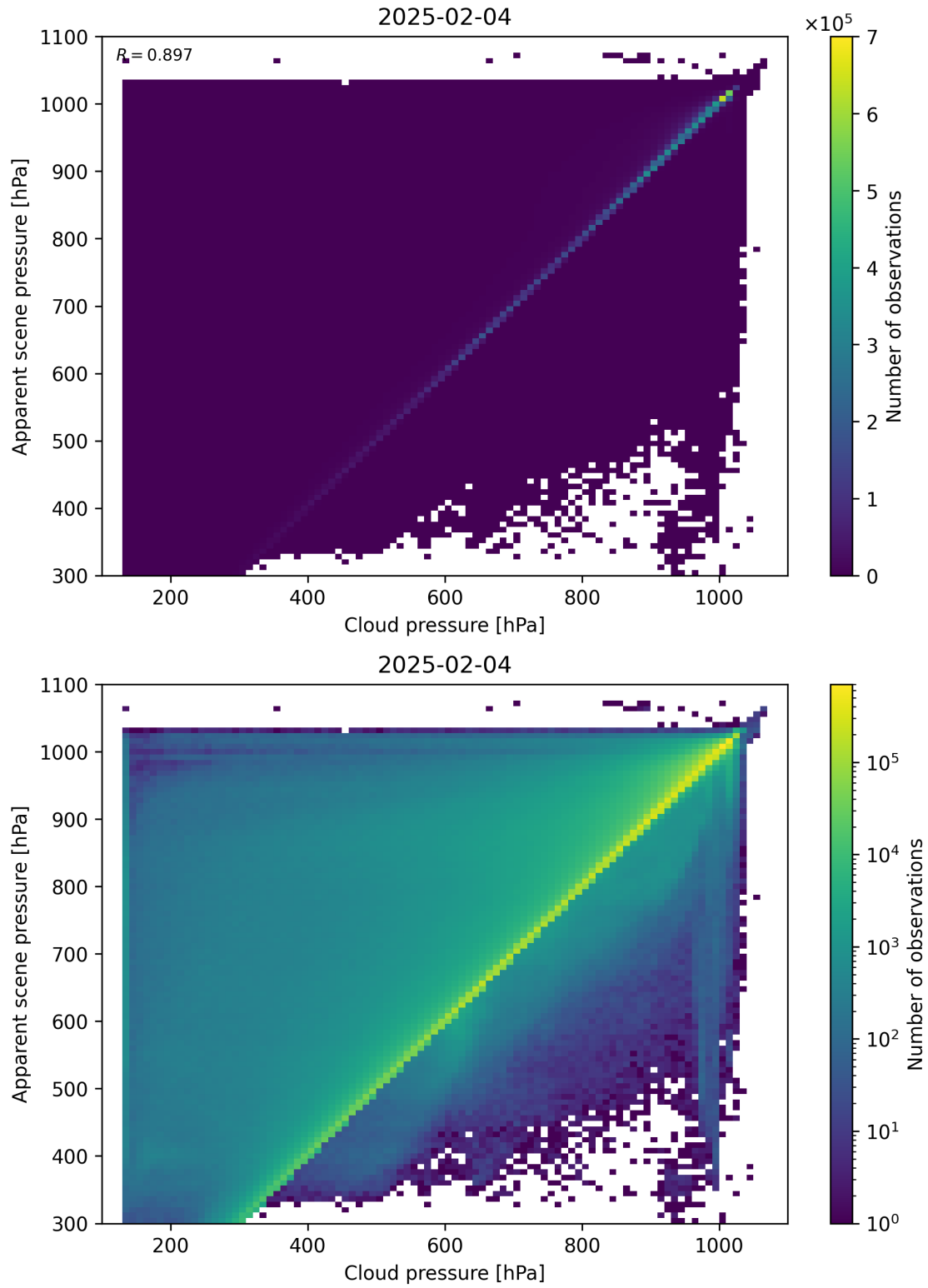
Figure 77: Scatter density plot of “Cloud pressure” against “Apparent scene pressure” for 2025-02-03 to 2025-02-05.
