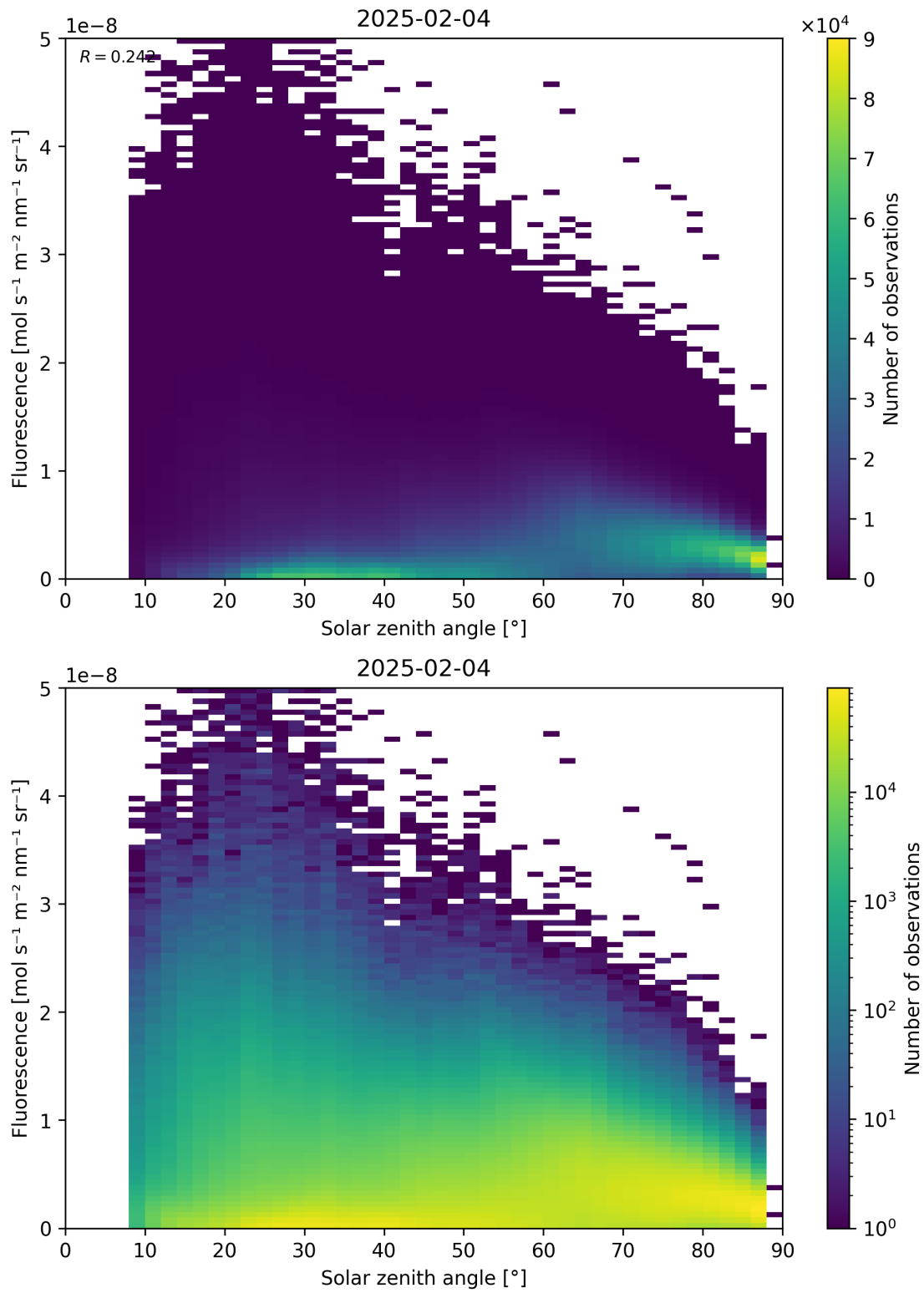
Figure 112: Scatter density plot of “Solar zenith angle” against “Fluorescence” for 2025-02-03 to 2025-02-05.
