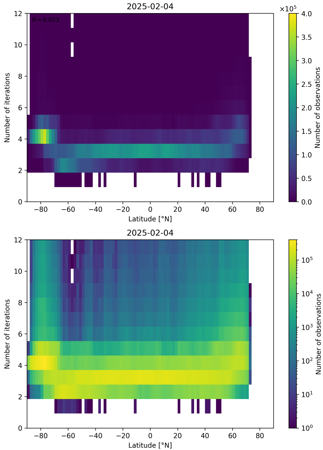
Figure 93: Scatter density plot of “Latitude” against “Number of iterations” for 2025-02-03 to 2025-02-05.
