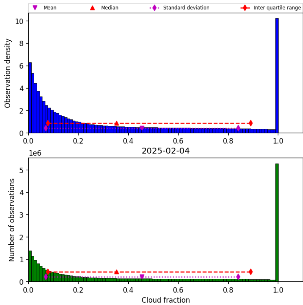
Figure 32: Histogram of “Cloud fraction” for 2025-02-03 to 2025-02-05
