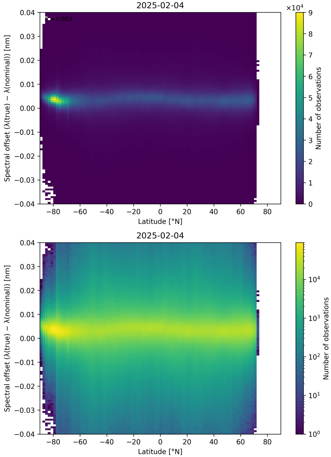
Figure 96: Scatter density plot of “Latitude” against “Spectral offset ( \lambda_{\text{true}} - \lambda_{\text{nominal}} )” for 2025-02-03 to 2025-02-05.
