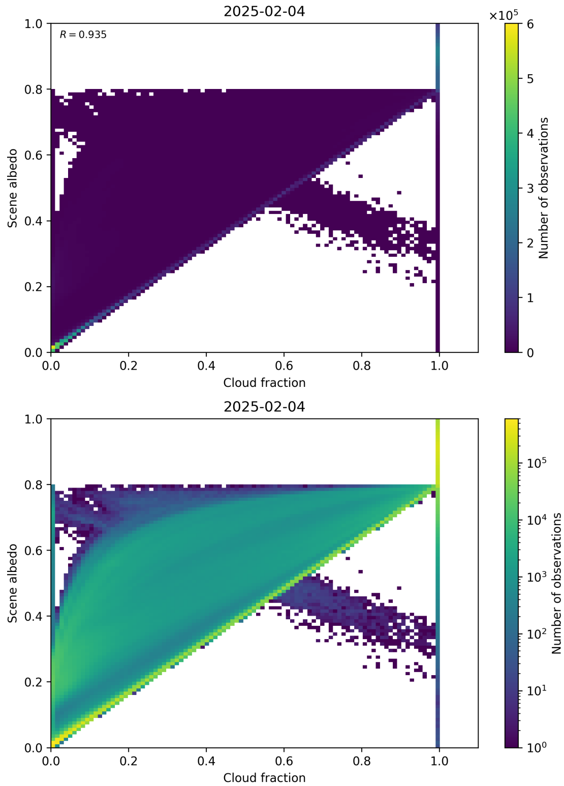
Figure 75: Scatter density plot of “Cloud fraction” against “Scene albedo” for 2025-02-03 to 2025-02-05.
