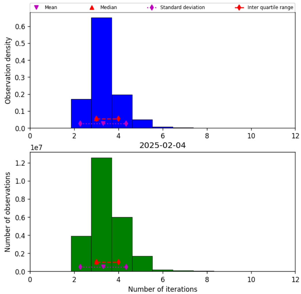
Figure 39: Histogram of “Number of iterations” for 2025-02-03 to 2025-02-05
