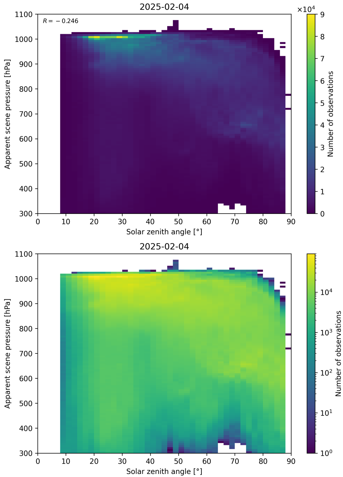
Figure 108: Scatter density plot of “Solar zenith angle” against “Apparent scene pressure” for 2025-02-03 to 2025-02-05.
