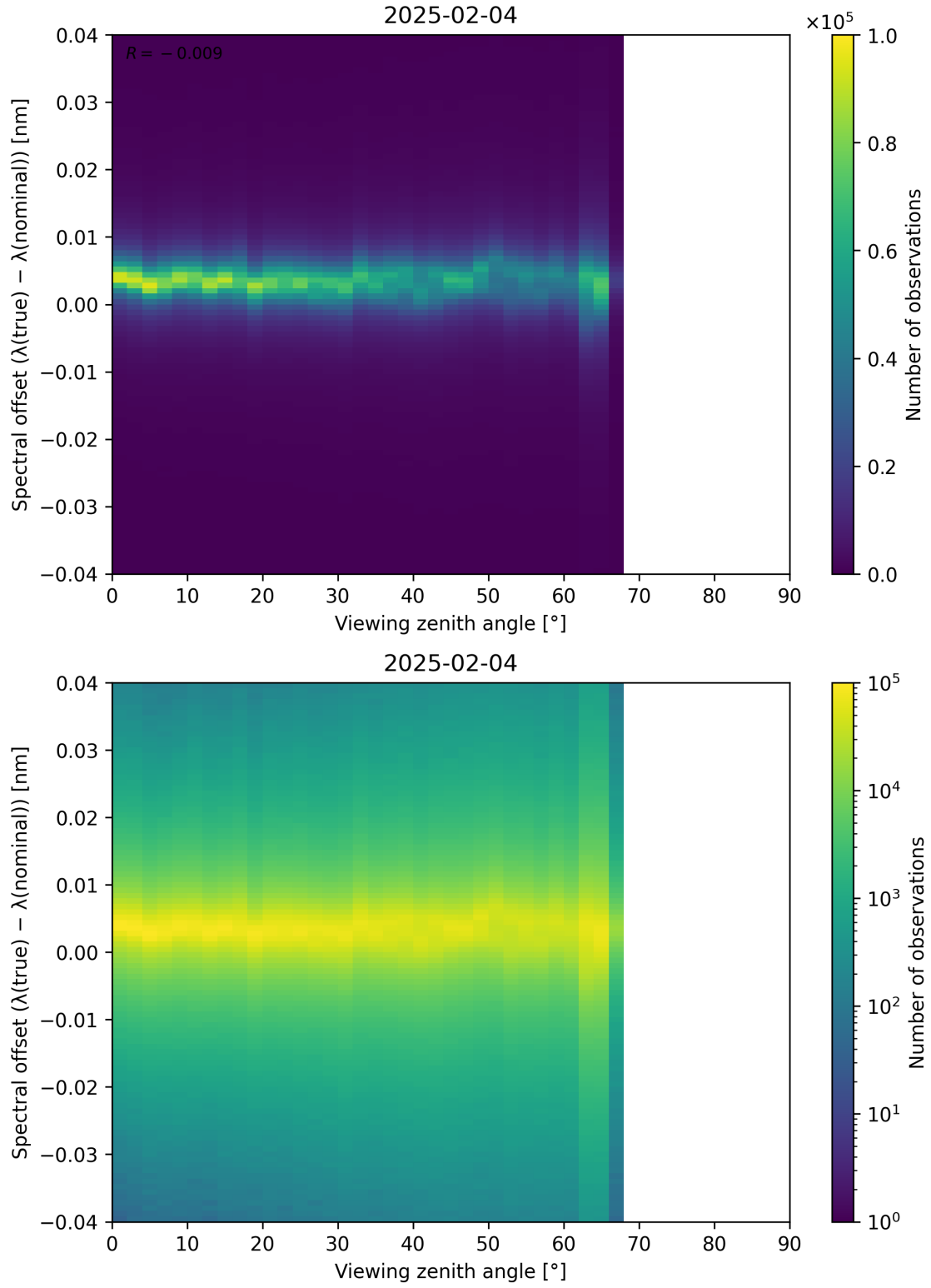
Figure 128: Scatter density plot of “Viewing zenith angle” against “Spectral offset ( \lambda_{\text{true}} - \lambda_{\text{nominal}} )” for 2025-02-03 to 2025-02-05.
