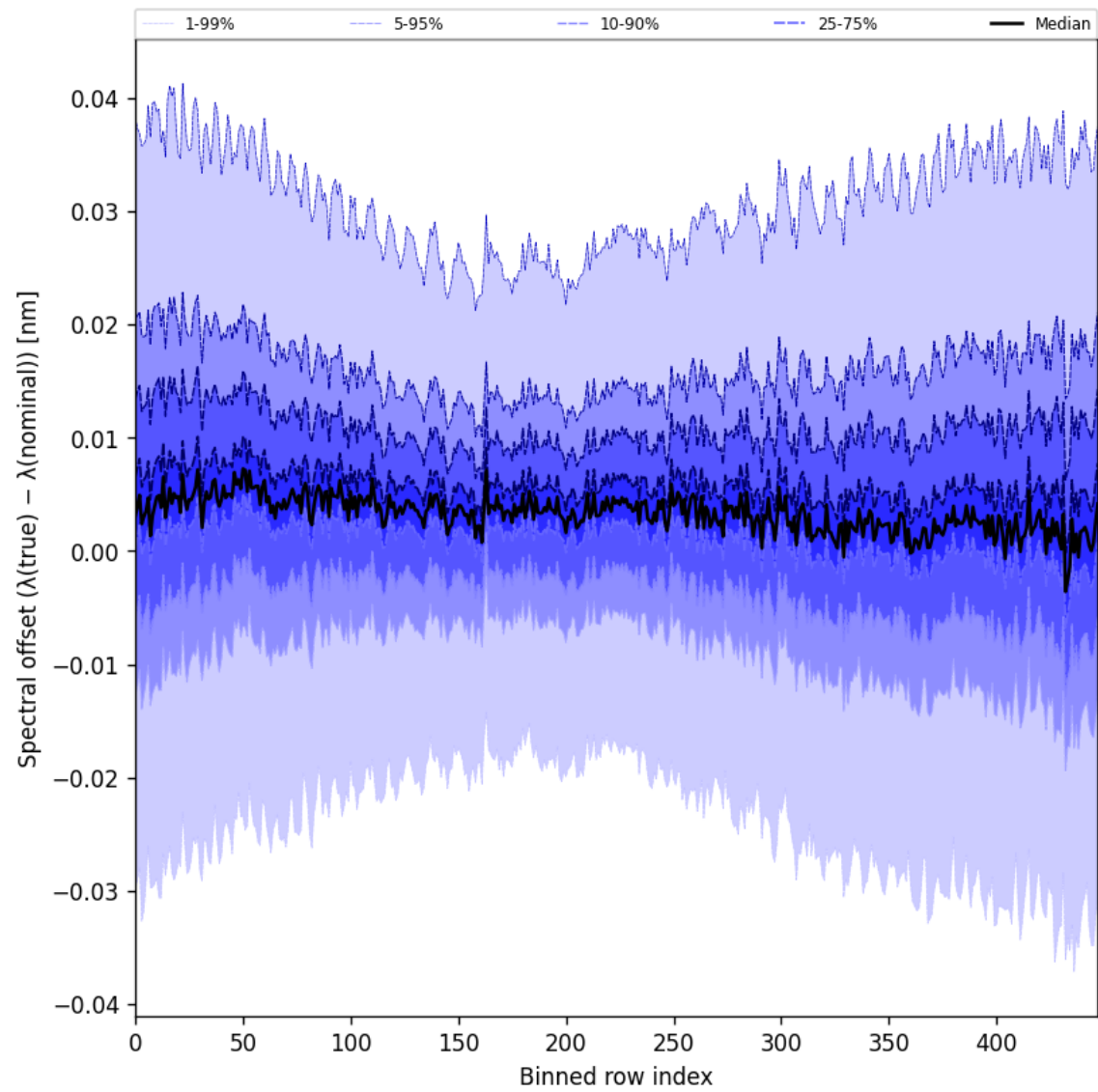
Figure 62: Along track statistics of “Spectral offset ( \lambda_{\text{true}} - \lambda_{\text{nominal}} )” for 2025-02-03 to 2025-02-05
