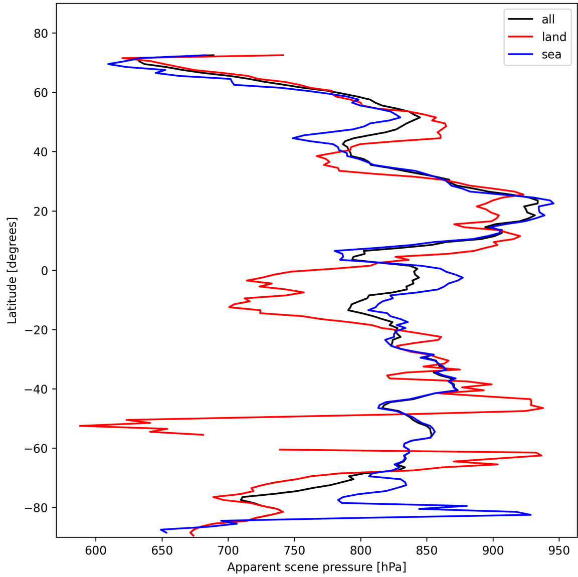
Figure 19: Zonal average of “Apparent scene pressure” for 2025-02-03 to 2025-02-05.
