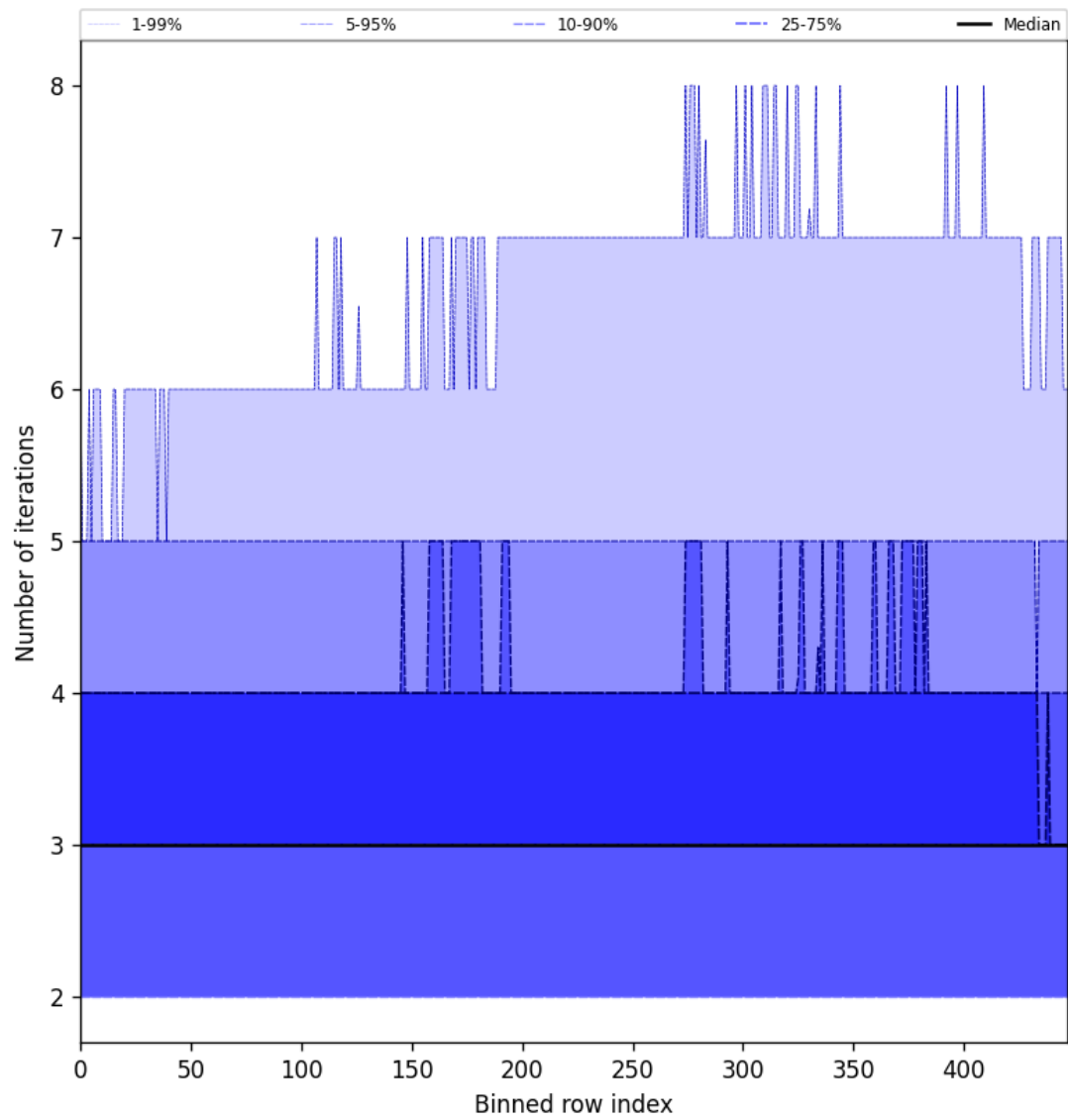
Figure 56: Along track statistics of “Number of iterations” for 2025-02-03 to 2025-02-05
