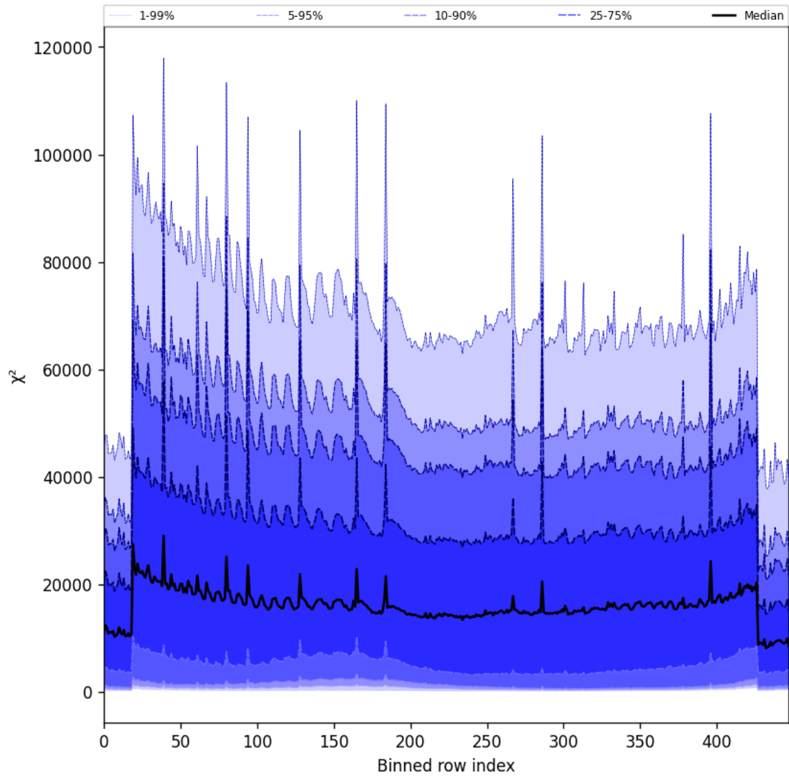
Figure 55: Along track statistics of “ \chi^2 ” for 2025-02-03 to 2025-02-05
