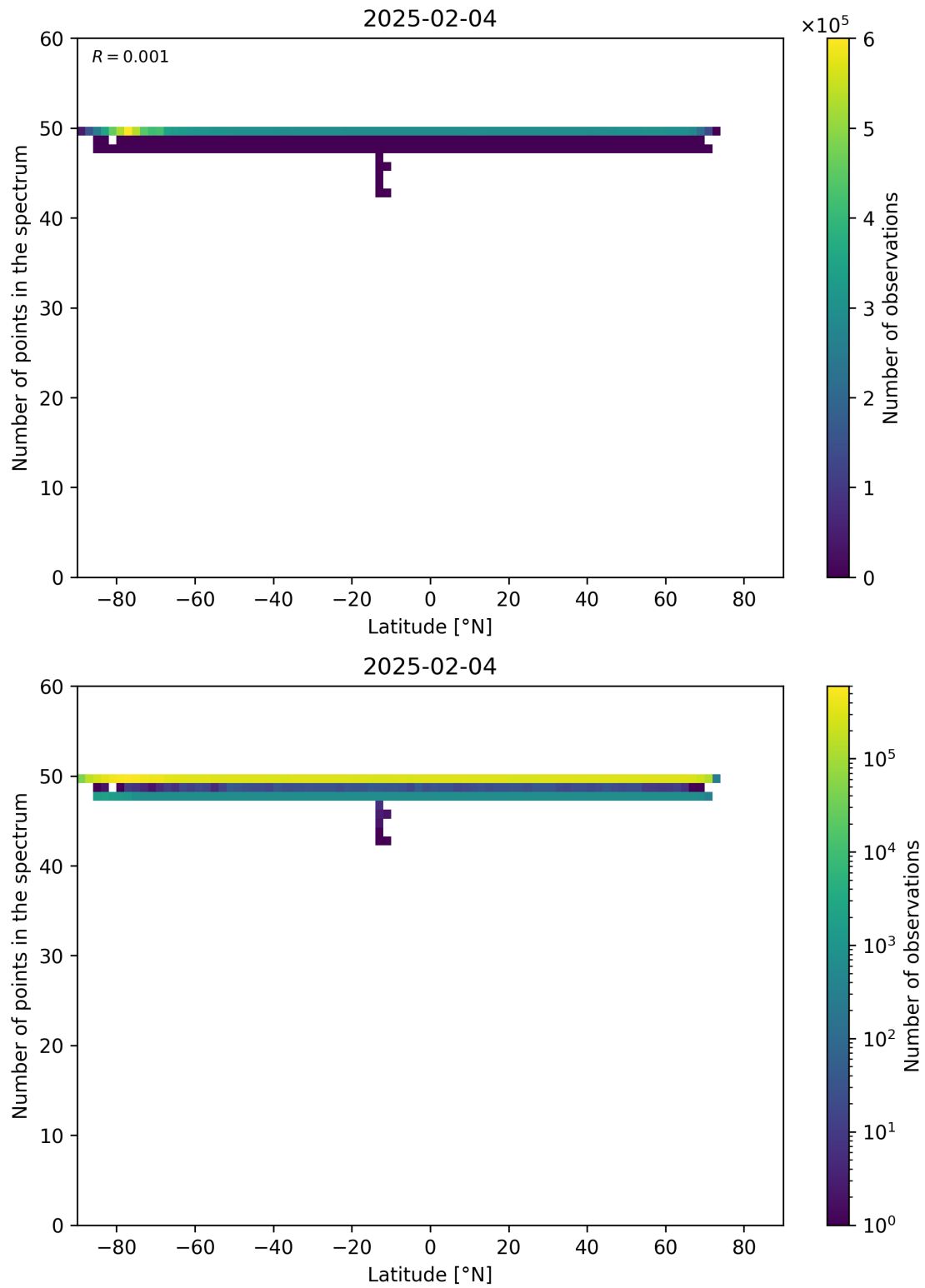
Figure 94: Scatter density plot of “Latitude” against “Number of points in the spectrum” for 2025-02-03 to 2025-02-05.
