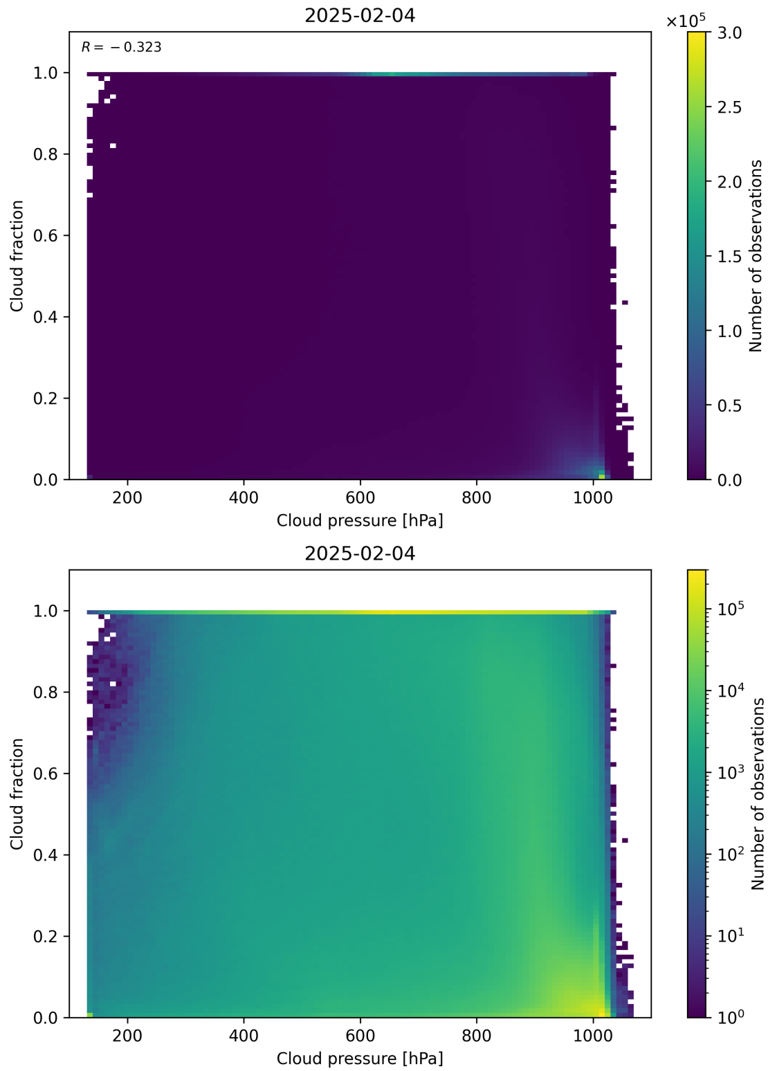
Figure 79: Scatter density plot of “Cloud pressure” against “Cloud fraction” for 2025-02-03 to 2025-02-05.
