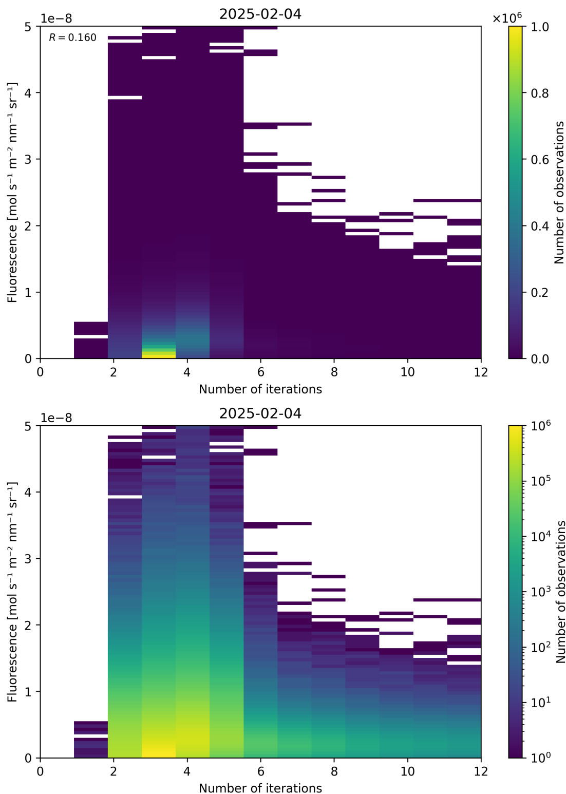
Figure 98: Scatter density plot of “Number of iterations” against “Fluorescence” for 2025-02-03 to 2025-02-05.
