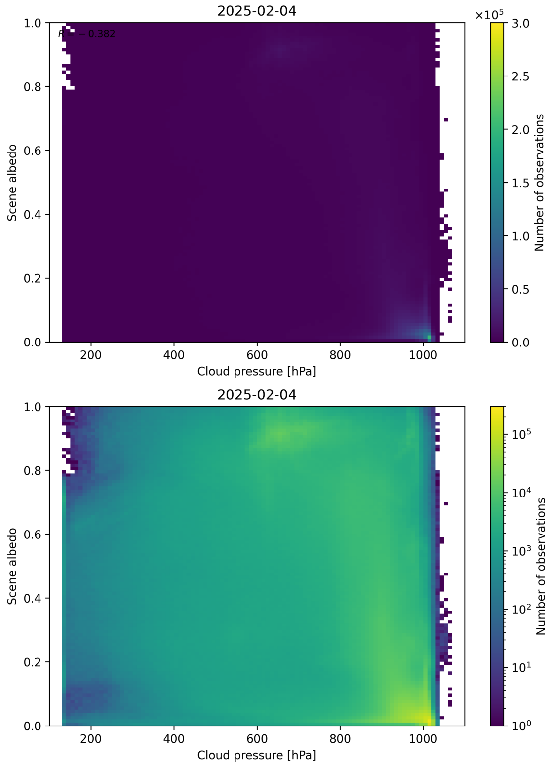
Figure 83: Scatter density plot of “Cloud pressure” against “Scene albedo” for 2025-02-03 to 2025-02-05.
