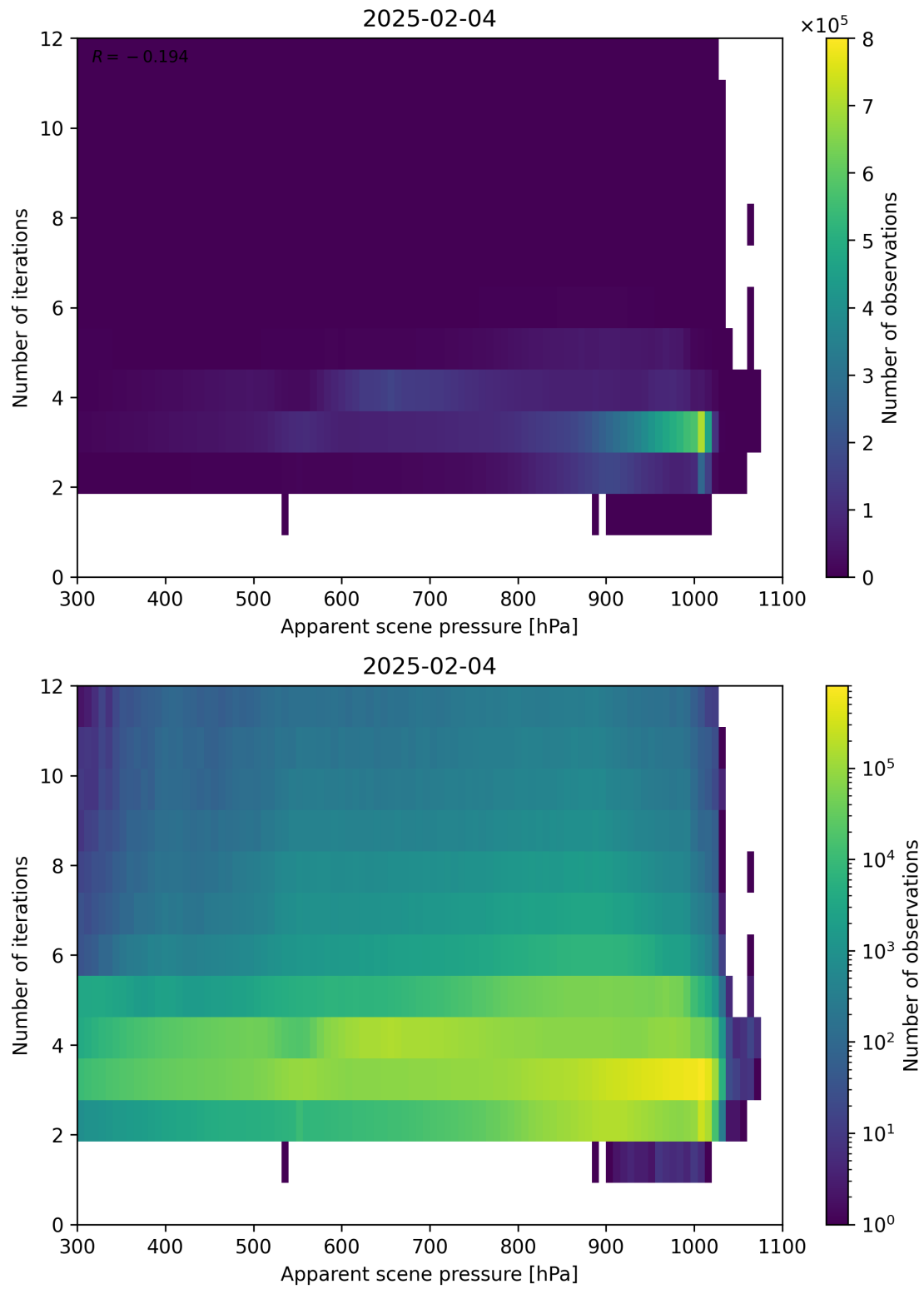
Figure 65: Scatter density plot of “Apparent scene pressure” against “Number of iterations” for 2025-02-03 to 2025-02-05.
