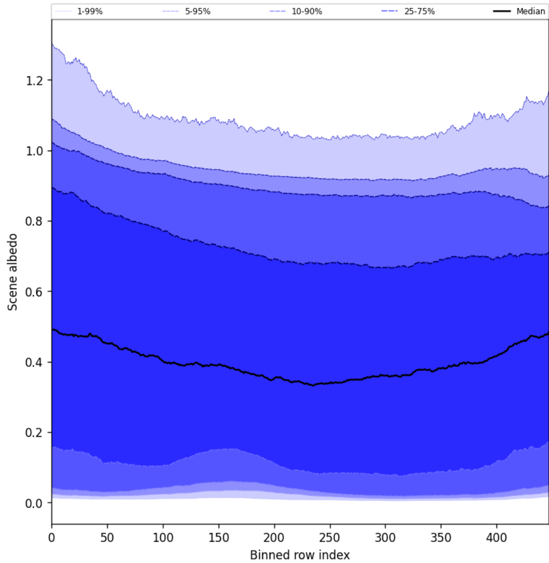
Figure 51: Along track statistics of “Scene albedo” for 2025-02-03 to 2025-02-05
