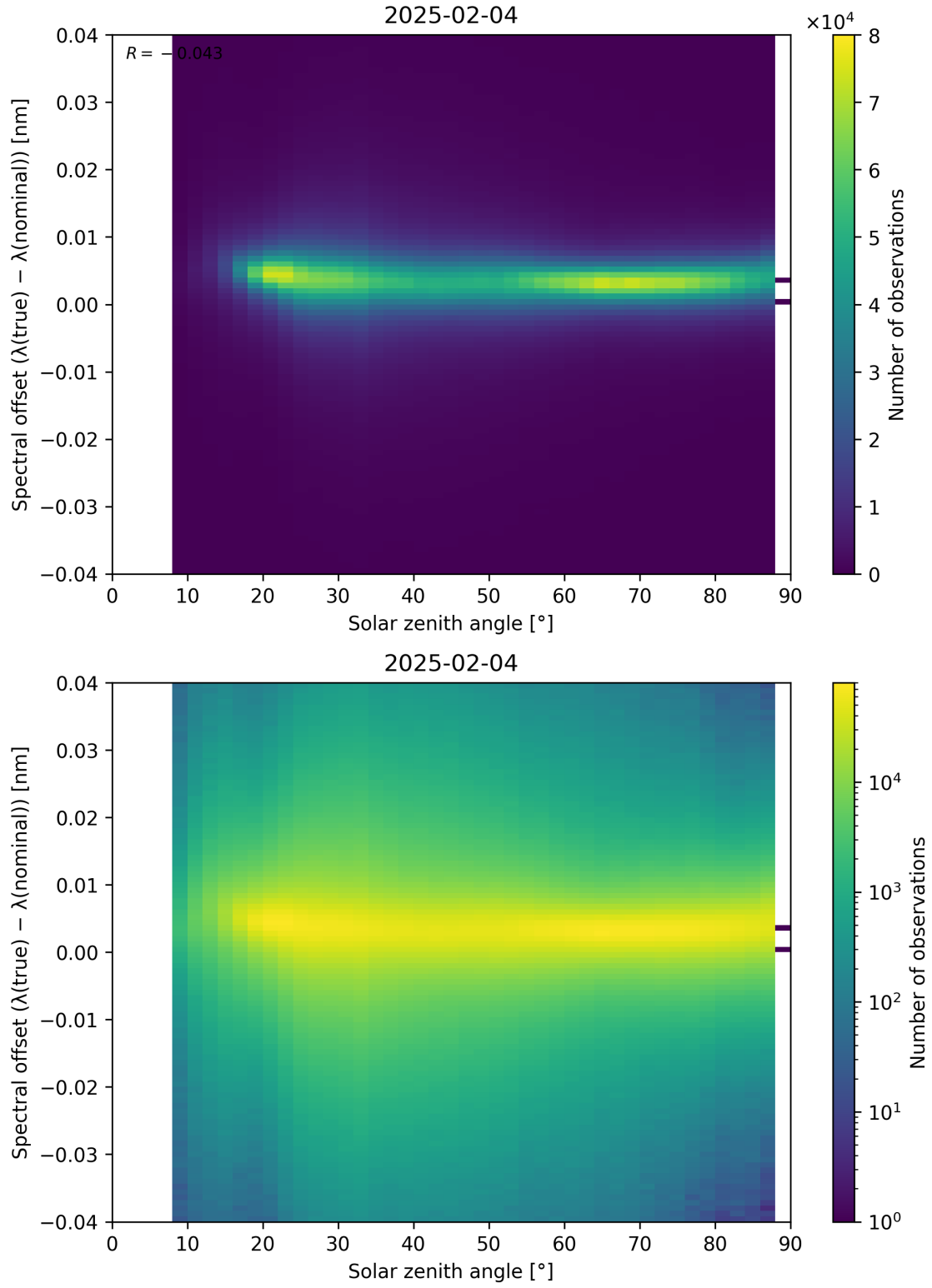
Figure 117: Scatter density plot of “Solar zenith angle” against “Spectral offset ( \lambda_{\text{true}} - \lambda_{\text{nominal}} )” for 2025-02-03 to 2025-02-05.
