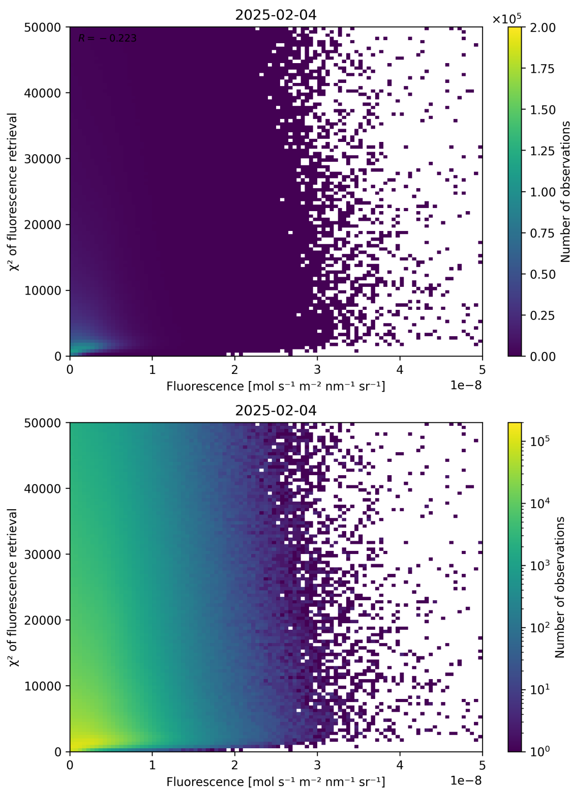
Figure 85: Scatter density plot of “Fluorescence” against “ \chi^2 of fluorescence retrieval” for 2025-02-03 to 2025-02-05.
