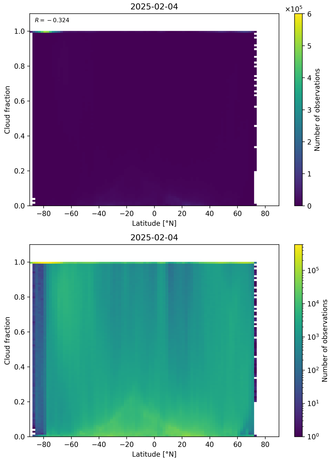
Figure 90: Scatter density plot of “Latitude” against “Cloud fraction” for 2025-02-03 to 2025-02-05.
