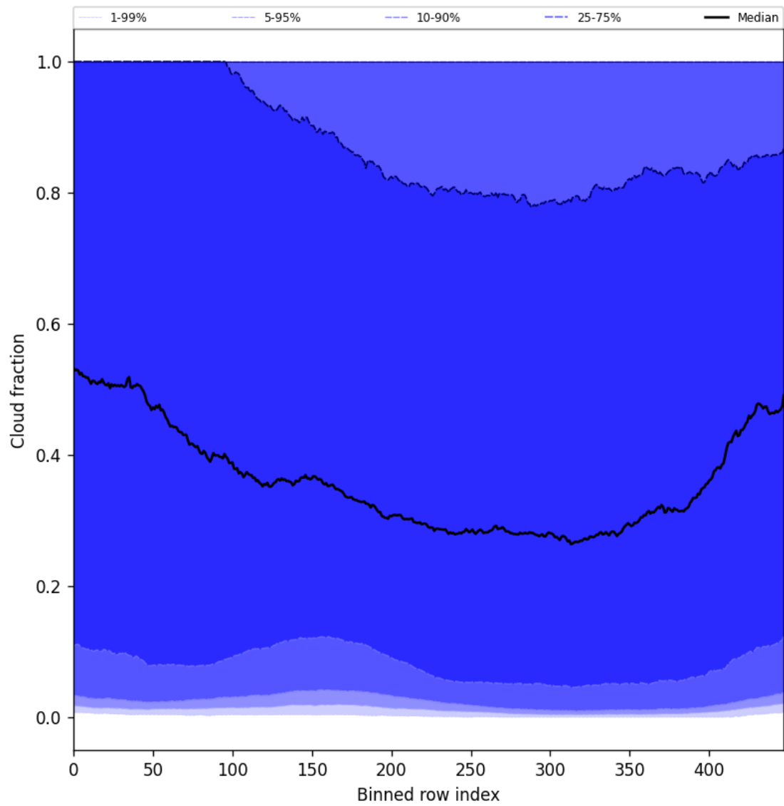
Figure 49: Along track statistics of “Cloud fraction” for 2025-02-03 to 2025-02-05
