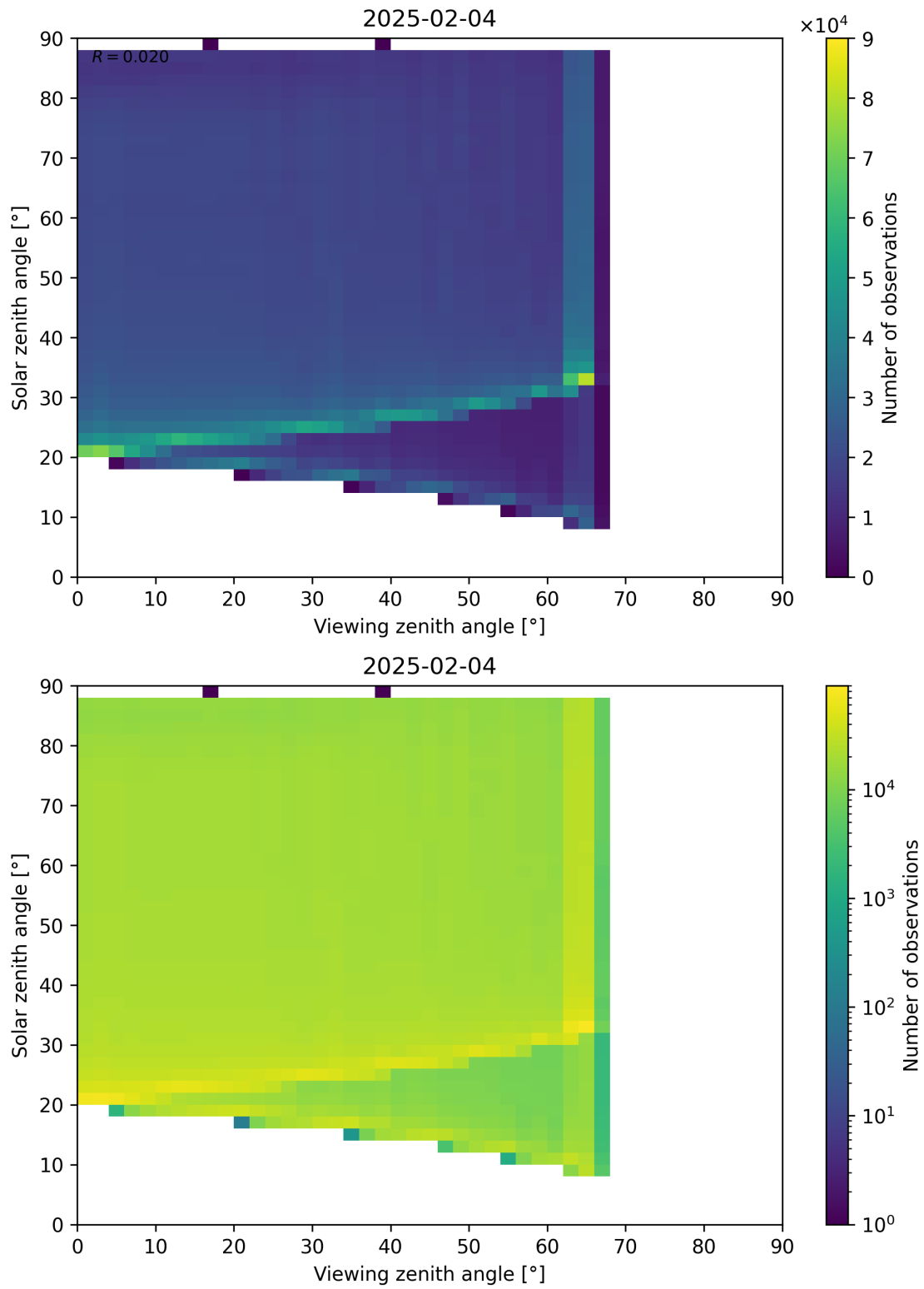
Figure 127: Scatter density plot of “Viewing zenith angle” against “Solar zenith angle” for 2025-02-03 to 2025-02-05.
