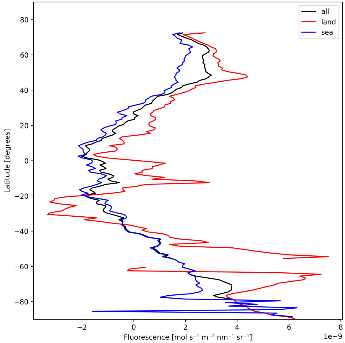
Figure 23: Zonal average of “Fluorescence” for 2025-02-03 to 2025-02-05.
