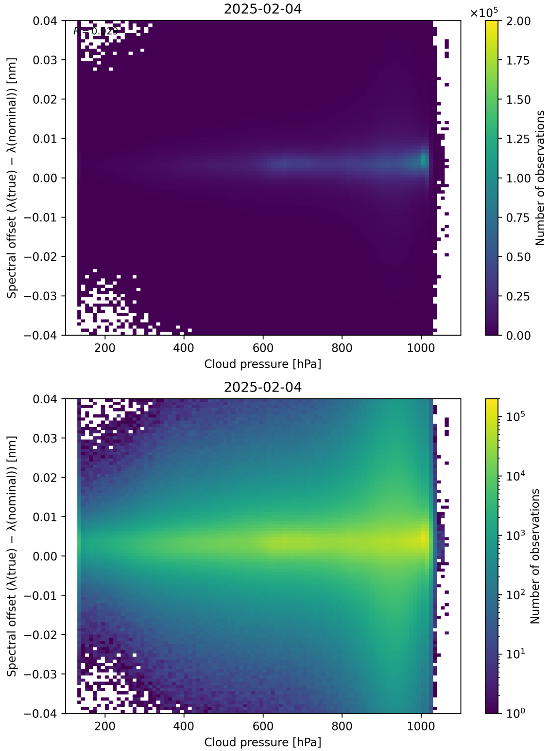
Figure 84: Scatter density plot of “Cloud pressure” against “Spectral offset ( \lambda_{\text{true}} - \lambda_{\text{nominal}} )” for 2025-02-03 to 2025-02-05.
