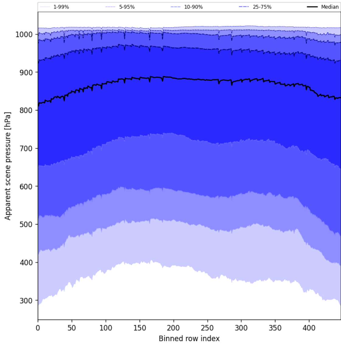
Figure 53: Along track statistics of “Apparent scene pressure” for 2025-02-03 to 2025-02-05
