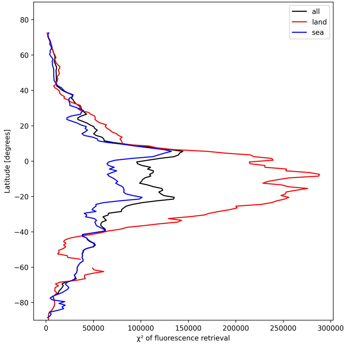
Figure 25: Zonal average of “ \chi^2 of fluorescence retrieval” for 2025-02-03 to 2025-02-05.
