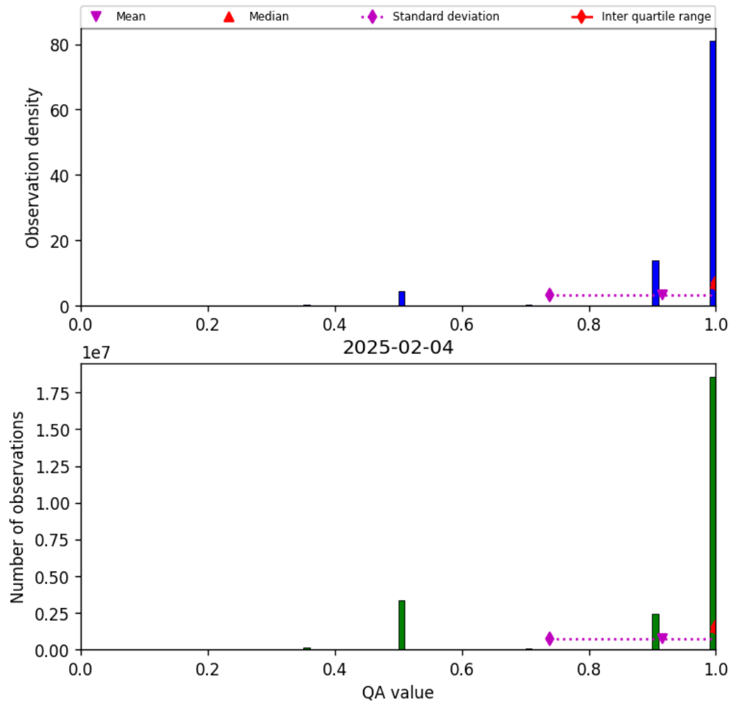
Figure 29: Histogram of “QA value” for 2025-02-03 to 2025-02-05
