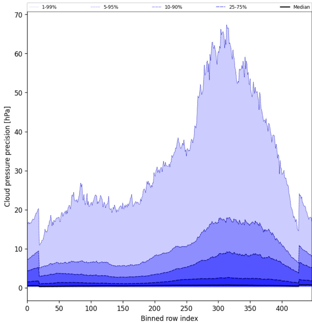
Figure 48: Along track statistics of “Cloud pressure precision” for 2025-02-03 to 2025-02-05
