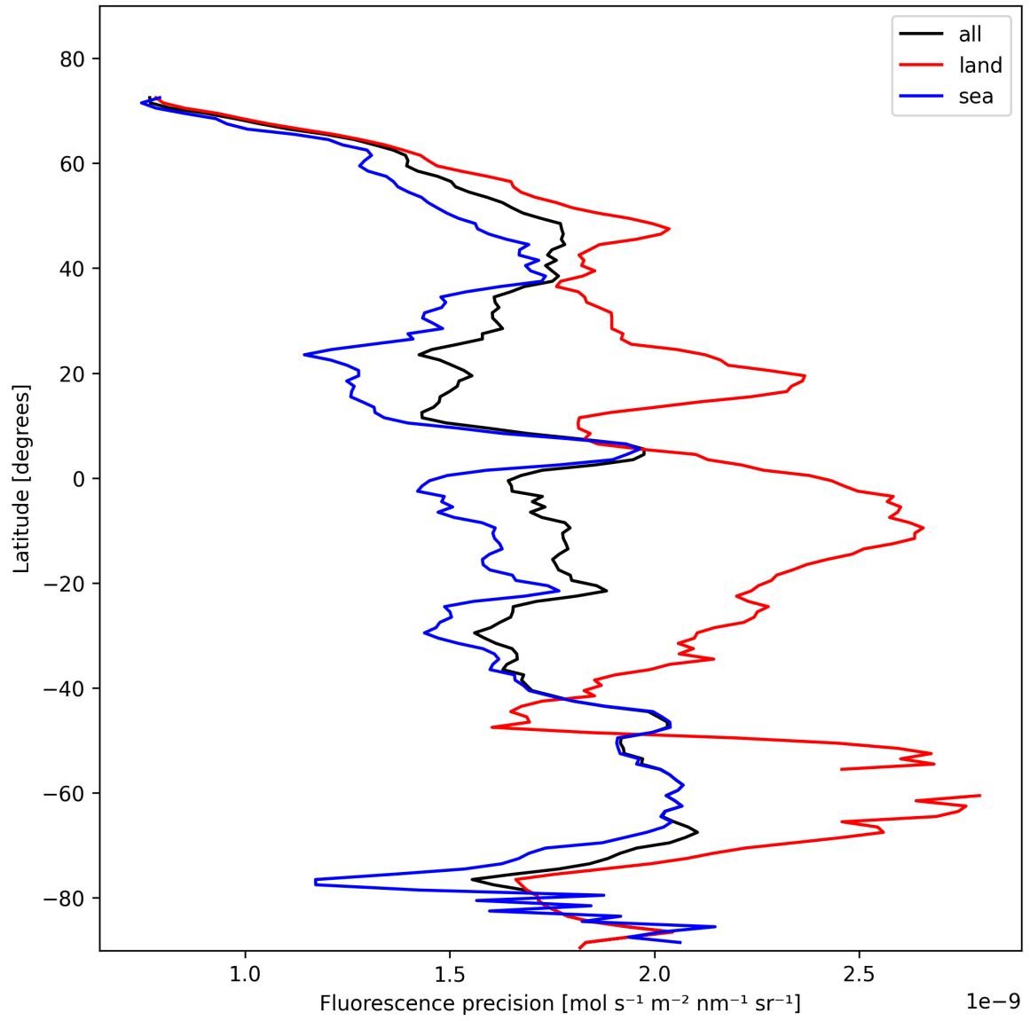
Figure 24: Zonal average of “Fluorescence precision” for 2025-02-03 to 2025-02-05.
