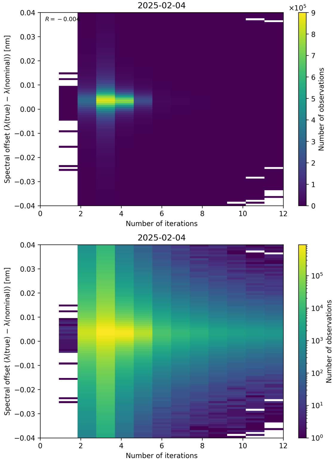
Figure 100: Scatter density plot of “Number of iterations” against “Spectral offset ( \lambda_{\text{true}} - \lambda_{\text{nominal}} )” for 2025-02-03 to 2025-02-05.
