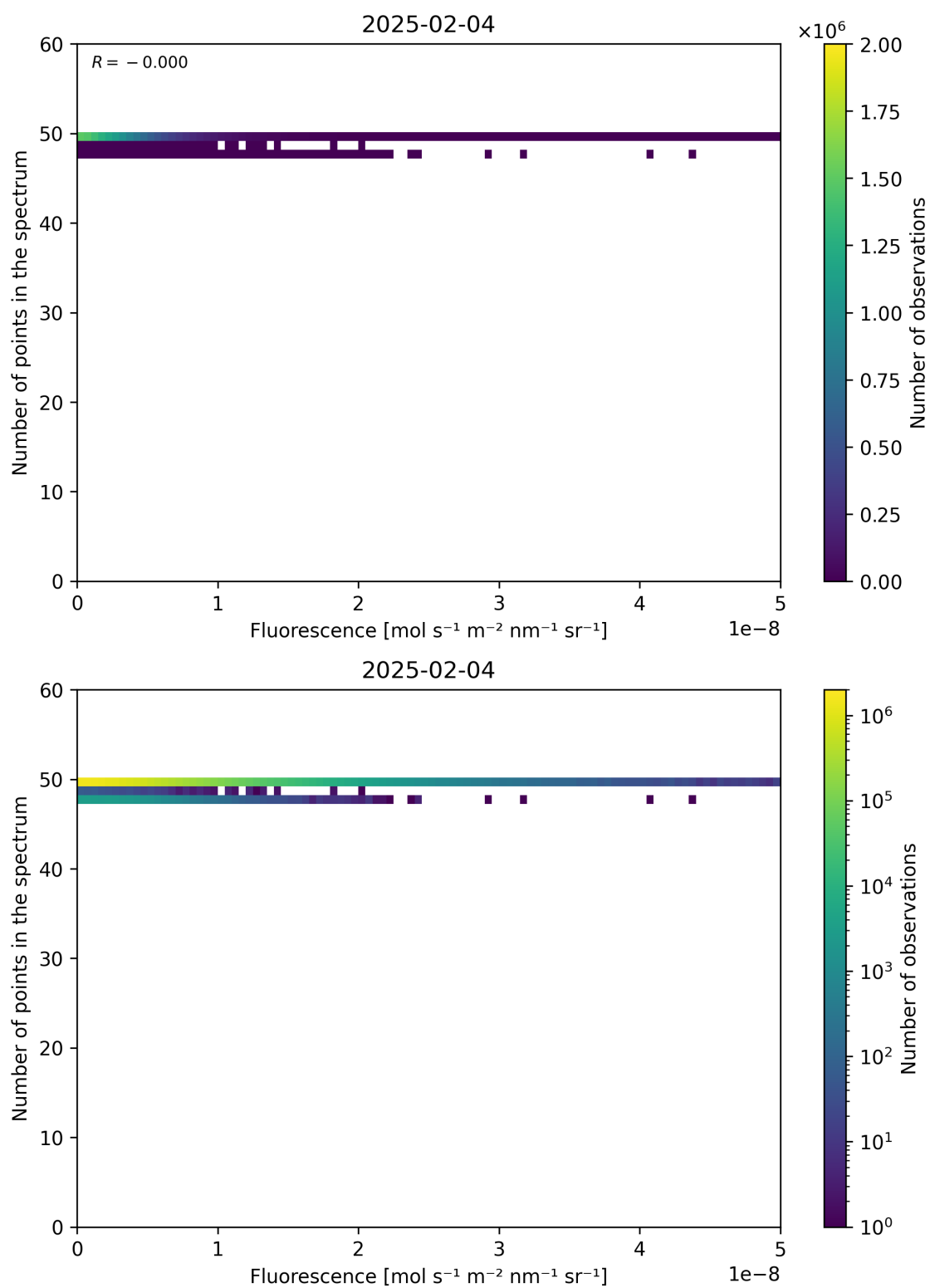
Figure 86: Scatter density plot of “Fluorescence” against “Number of points in the spectrum” for 2025-02-03 to 2025-02-05.
