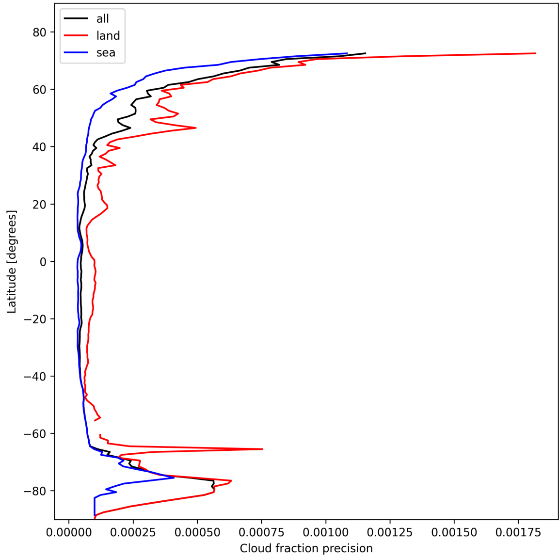
Figure 16: Zonal average of “Cloud fraction precision” for 2025-02-03 to 2025-02-05.
