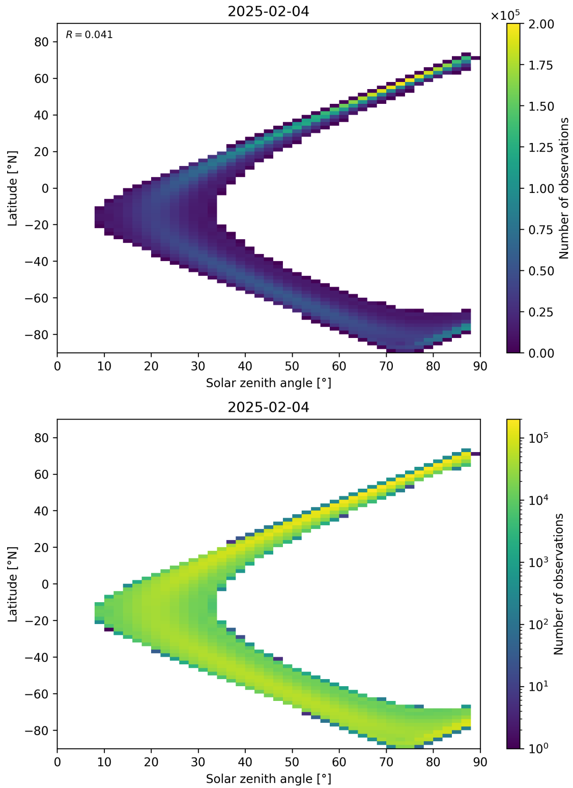
Figure 113: Scatter density plot of “Solar zenith angle” against “Latitude” for 2025-02-03 to 2025-02-05.
