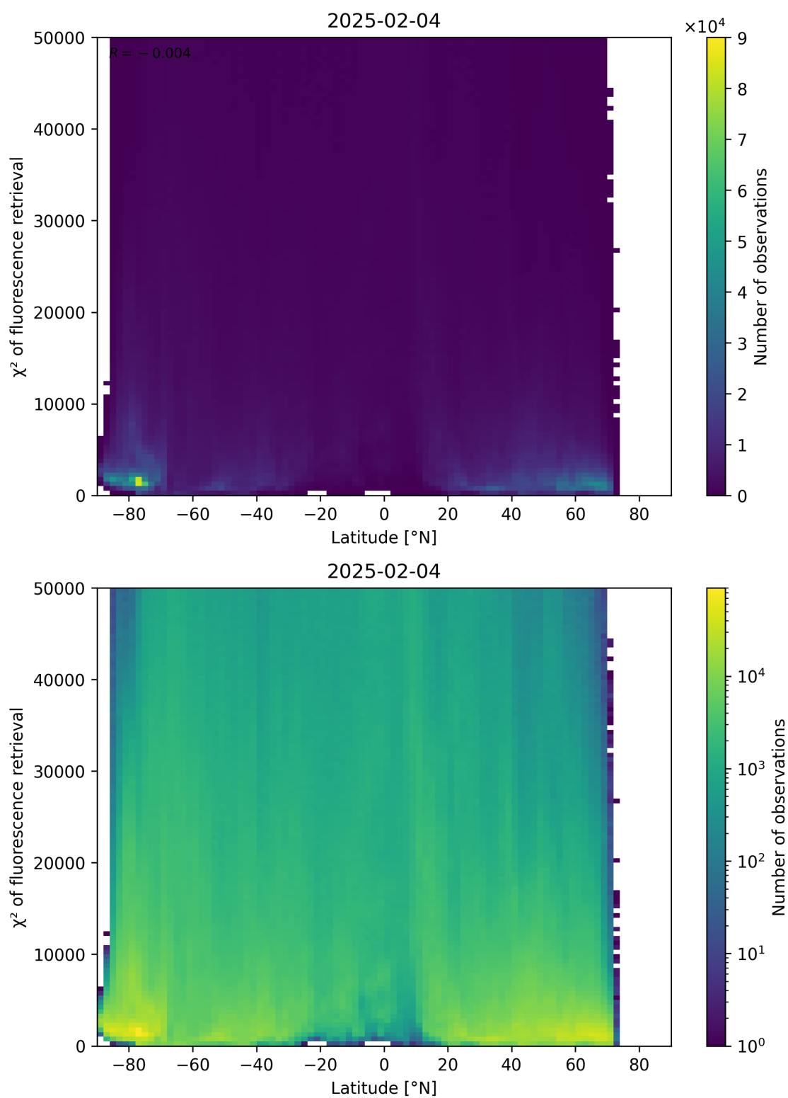
Figure 89: Scatter density plot of “Latitude” against “ \chi^2 of fluorescence retrieval” for 2025-02-03 to 2025-02-05.
