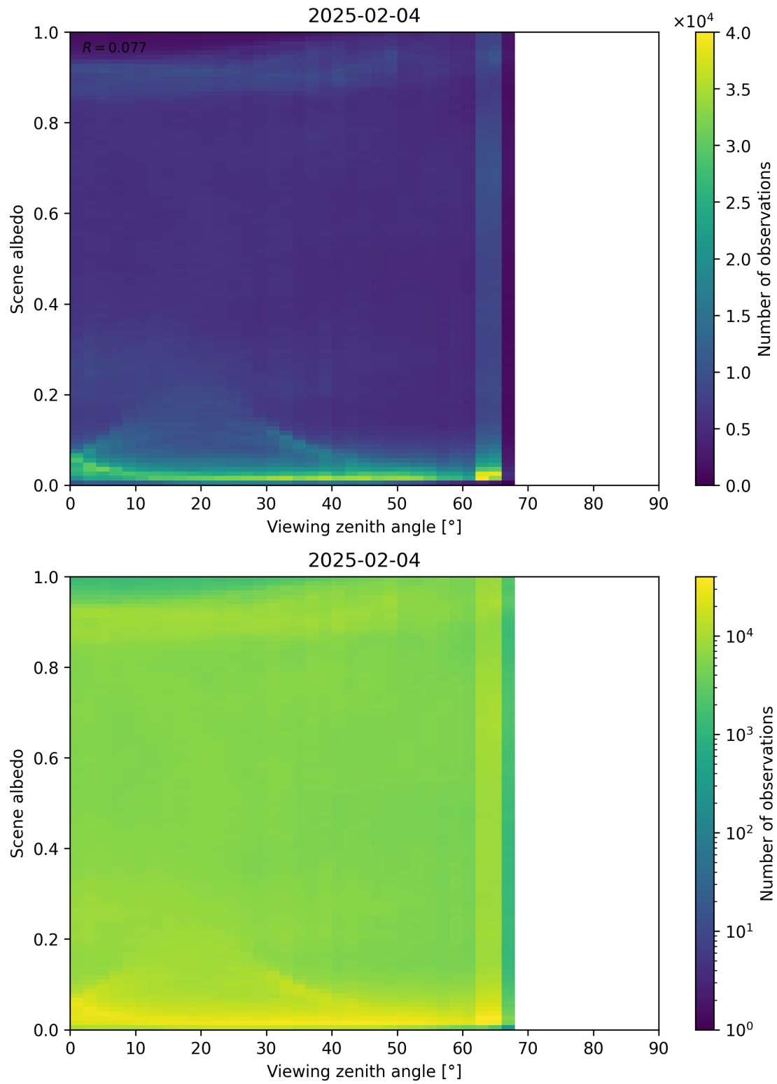
Figure 126: Scatter density plot of “Viewing zenith angle” against “Scene albedo” for 2025-02-03 to 2025-02-05.
