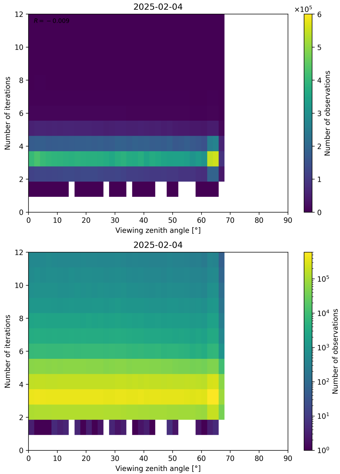
Figure 124: Scatter density plot of “Viewing zenith angle” against “Number of iterations” for 2025-02-03 to 2025-02-05.
