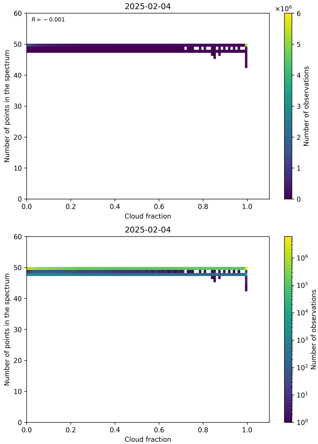
Figure 74: Scatter density plot of “Cloud fraction” against “Number of points in the spectrum” for 2025-02-03 to 2025-02-05.
