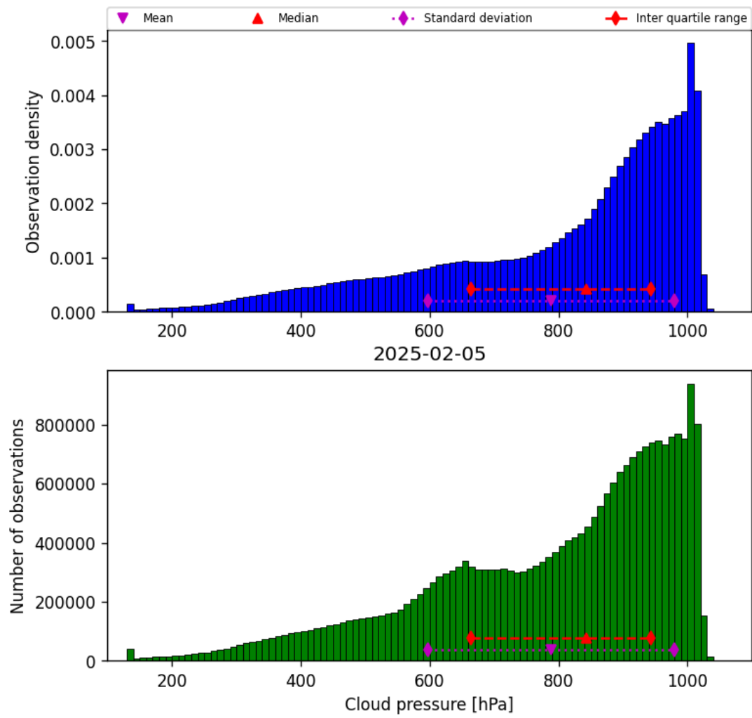
Figure 30: Histogram of “Cloud pressure” for 2025-02-04 to 2025-02-06
