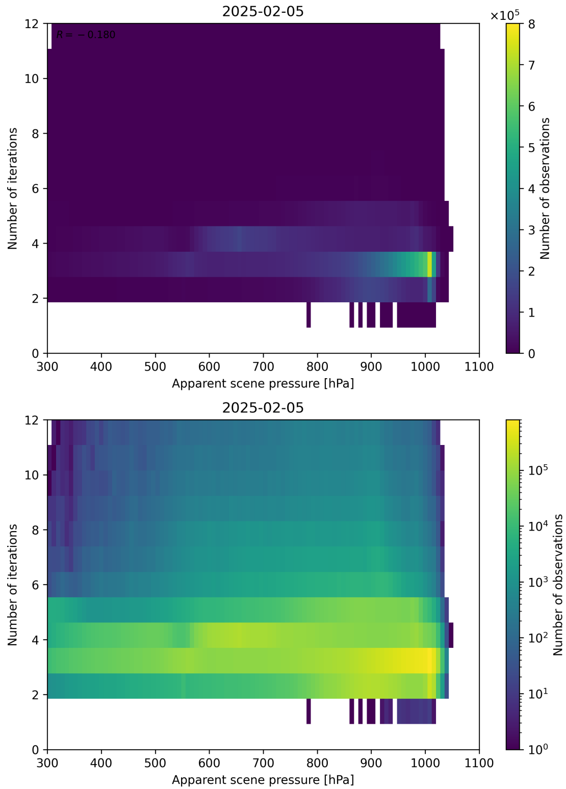
Figure 65: Scatter density plot of “Apparent scene pressure” against “Number of iterations” for 2025-02-04 to 2025-02-06.
