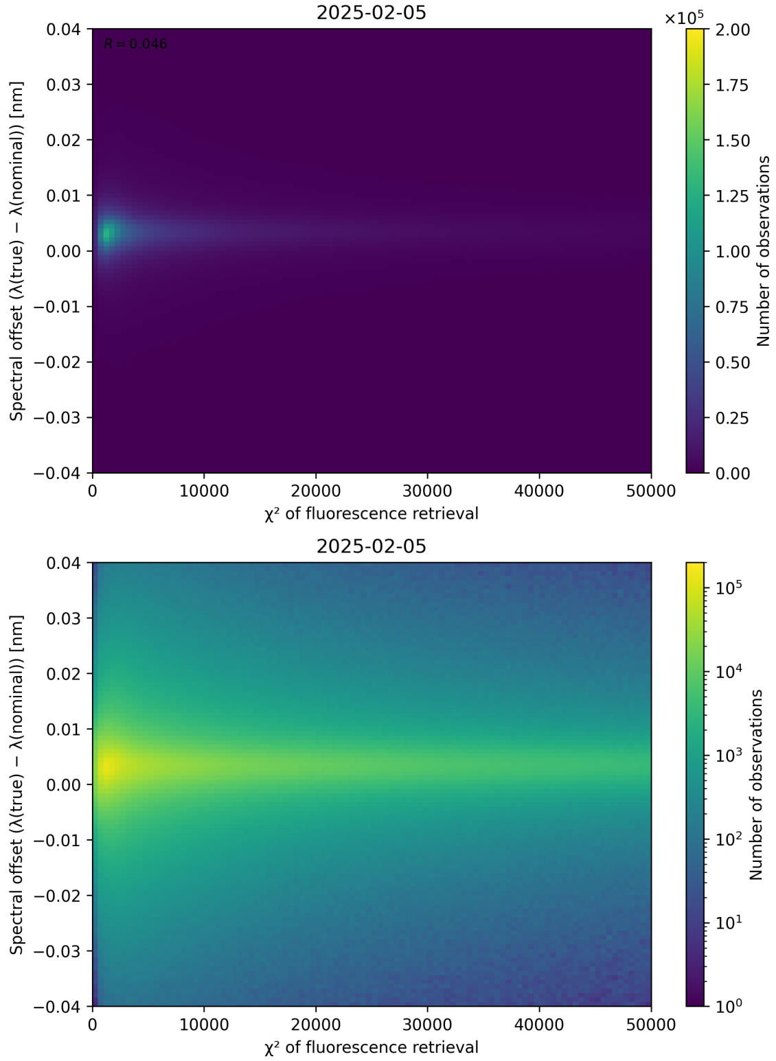
Figure 69: Scatter density plot of “ \chi^2 of fluorescence retrieval” against “Spectral offset ( \lambda_{\text{true}} - \lambda_{\text{nominal}} )” for 2025-02-04 to 2025-02-06.
