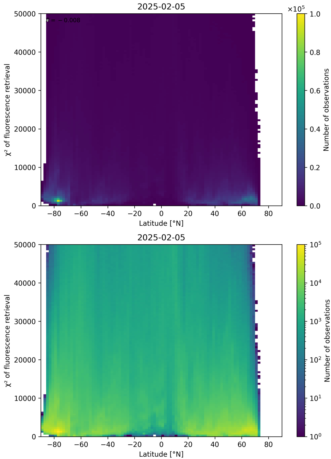
Figure 89: Scatter density plot of “Latitude” against “ \chi^2 of fluorescence retrieval” for 2025-02-04 to 2025-02-06.
