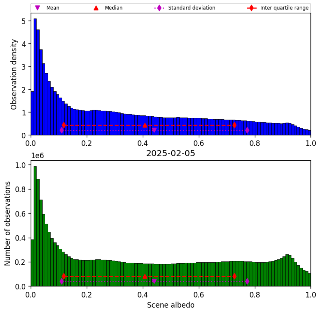
Figure 34: Histogram of “Scene albedo” for 2025-02-04 to 2025-02-06
