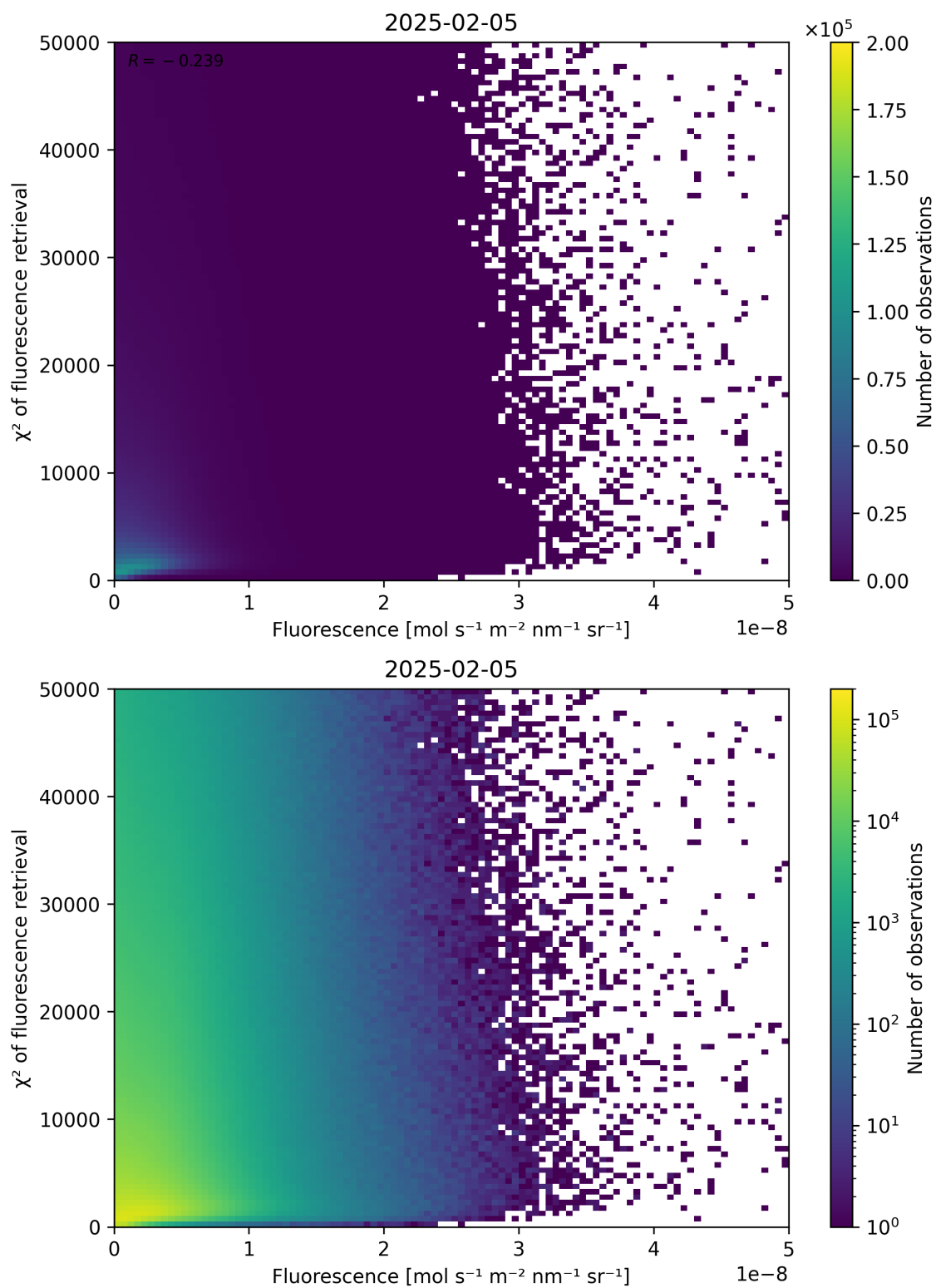
Figure 85: Scatter density plot of “Fluorescence” against “ \chi^2 of fluorescence retrieval” for 2025-02-04 to 2025-02-06.
