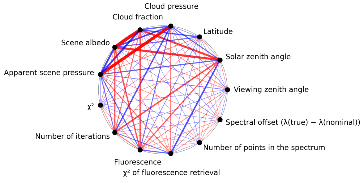
Figure 1: Map of correlation graph for 2025-02-04 to 2025-02-06.
