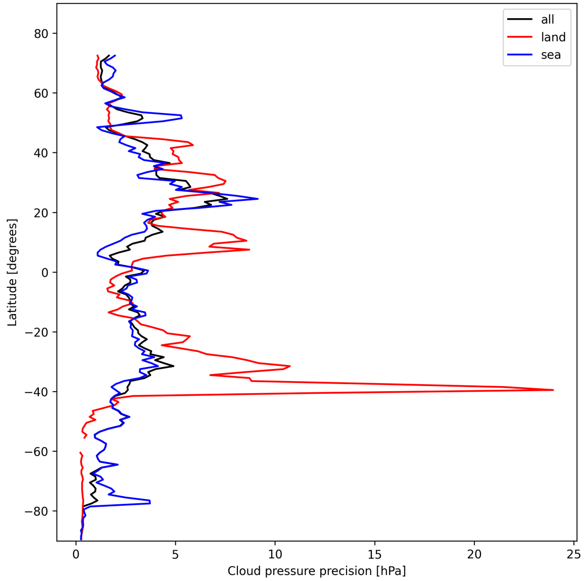
Figure 14: Zonal average of “Cloud pressure precision” for 2025-02-04 to 2025-02-06.
