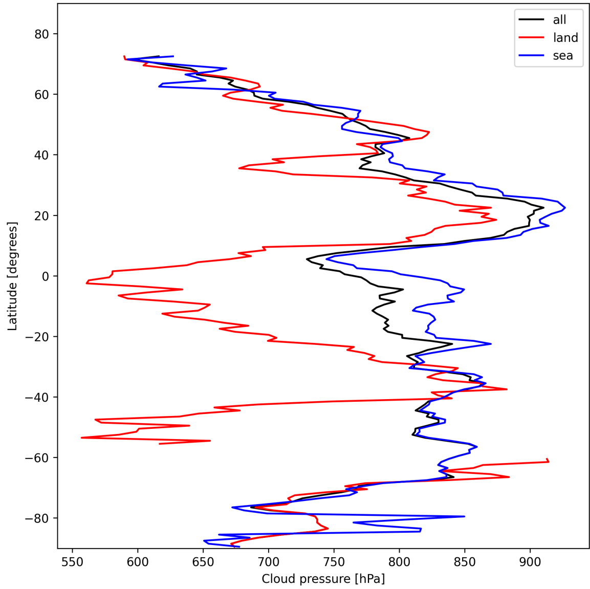
Figure 13: Zonal average of “Cloud pressure” for 2025-02-04 to 2025-02-06.
