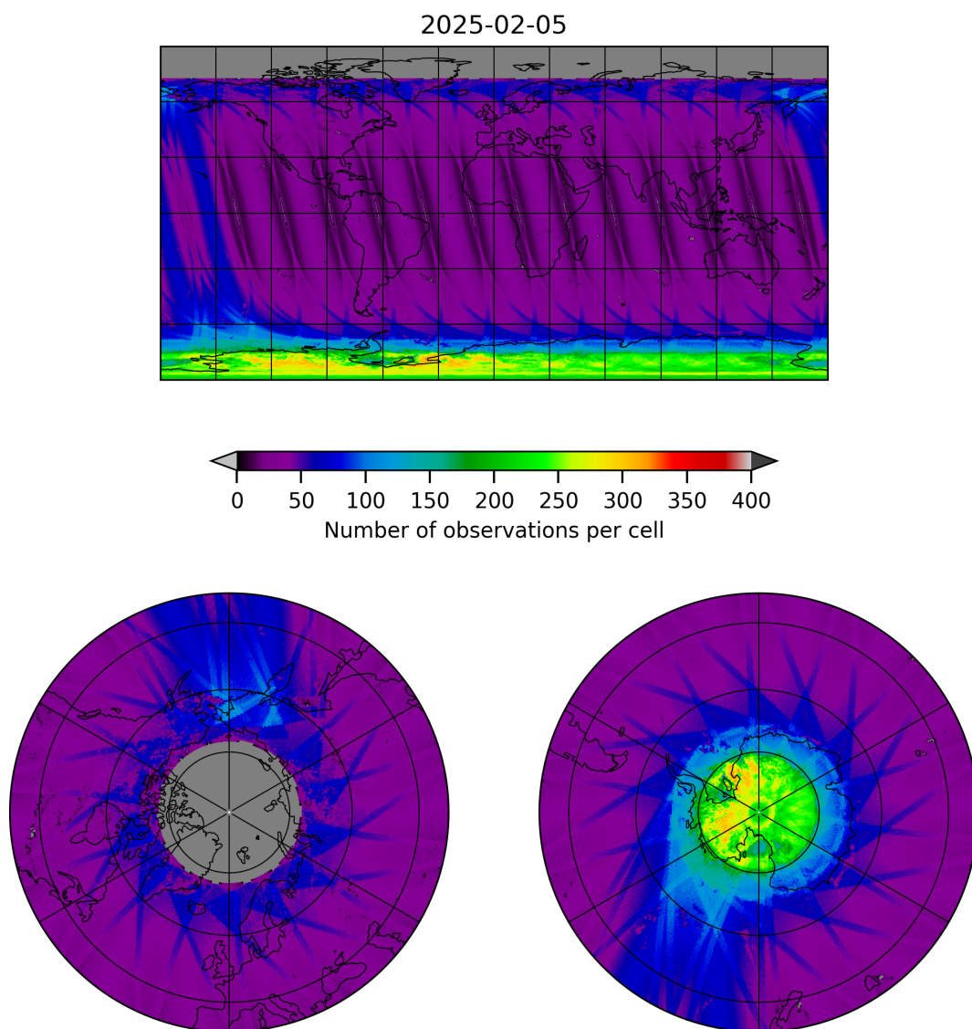
Figure 11: Map of the number of observations for 2025-02-04 to 2025-02-06
