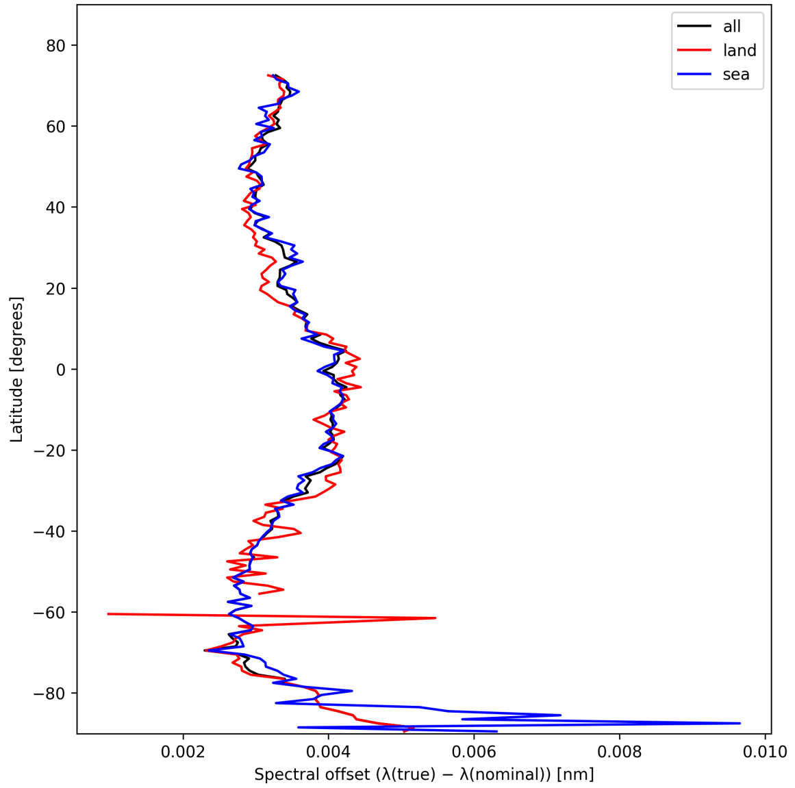
Figure 28: Zonal average of “Spectral offset ( \lambda_{\text{true}} - \lambda_{\text{nominal}} )” for 2025-02-04 to 2025-02-06.
