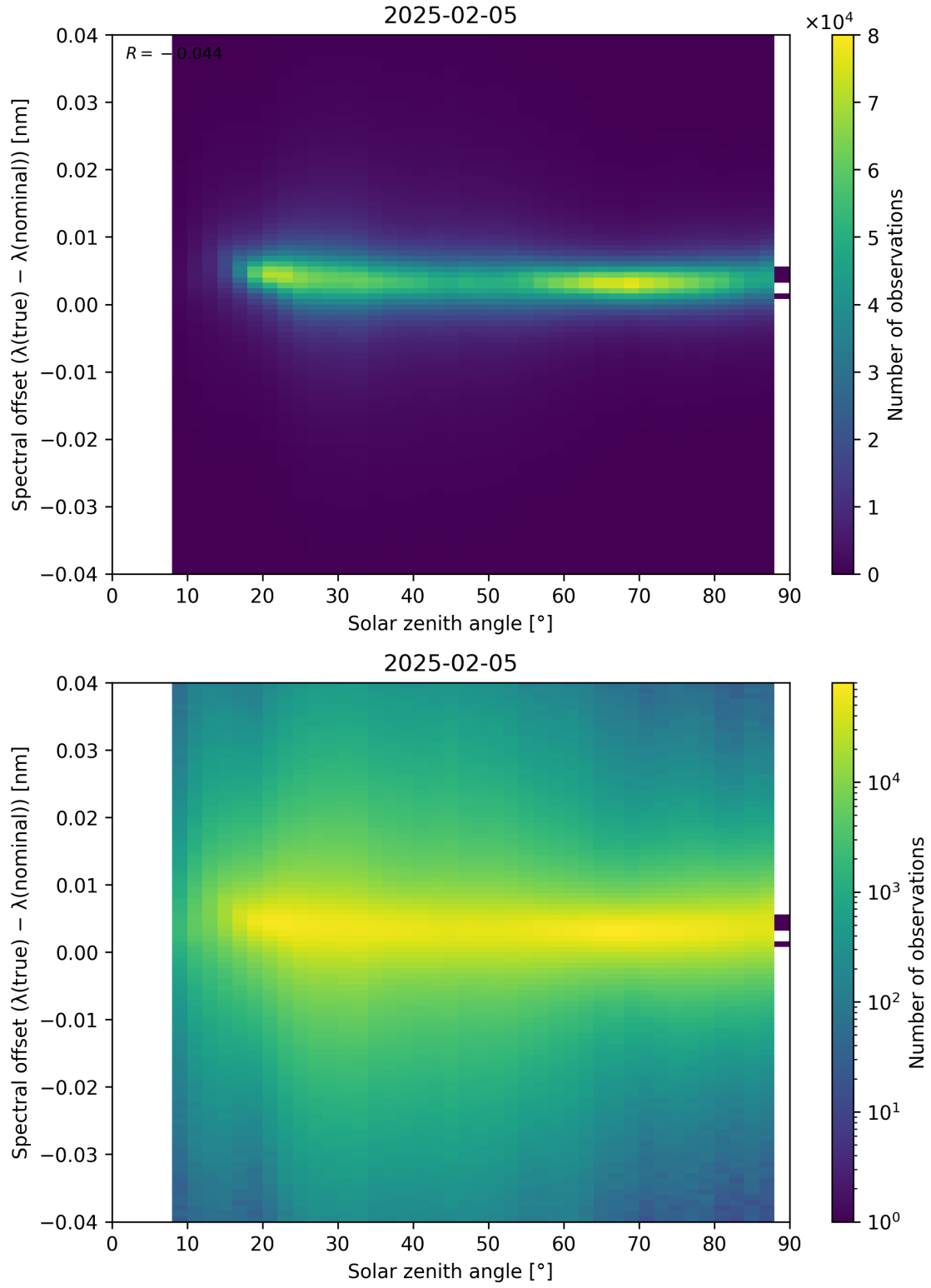
Figure 117: Scatter density plot of “Solar zenith angle” against “Spectral offset ( \lambda_{\text{true}} - \lambda_{\text{nominal}} )” for 2025-02-04 to 2025-02-06.
