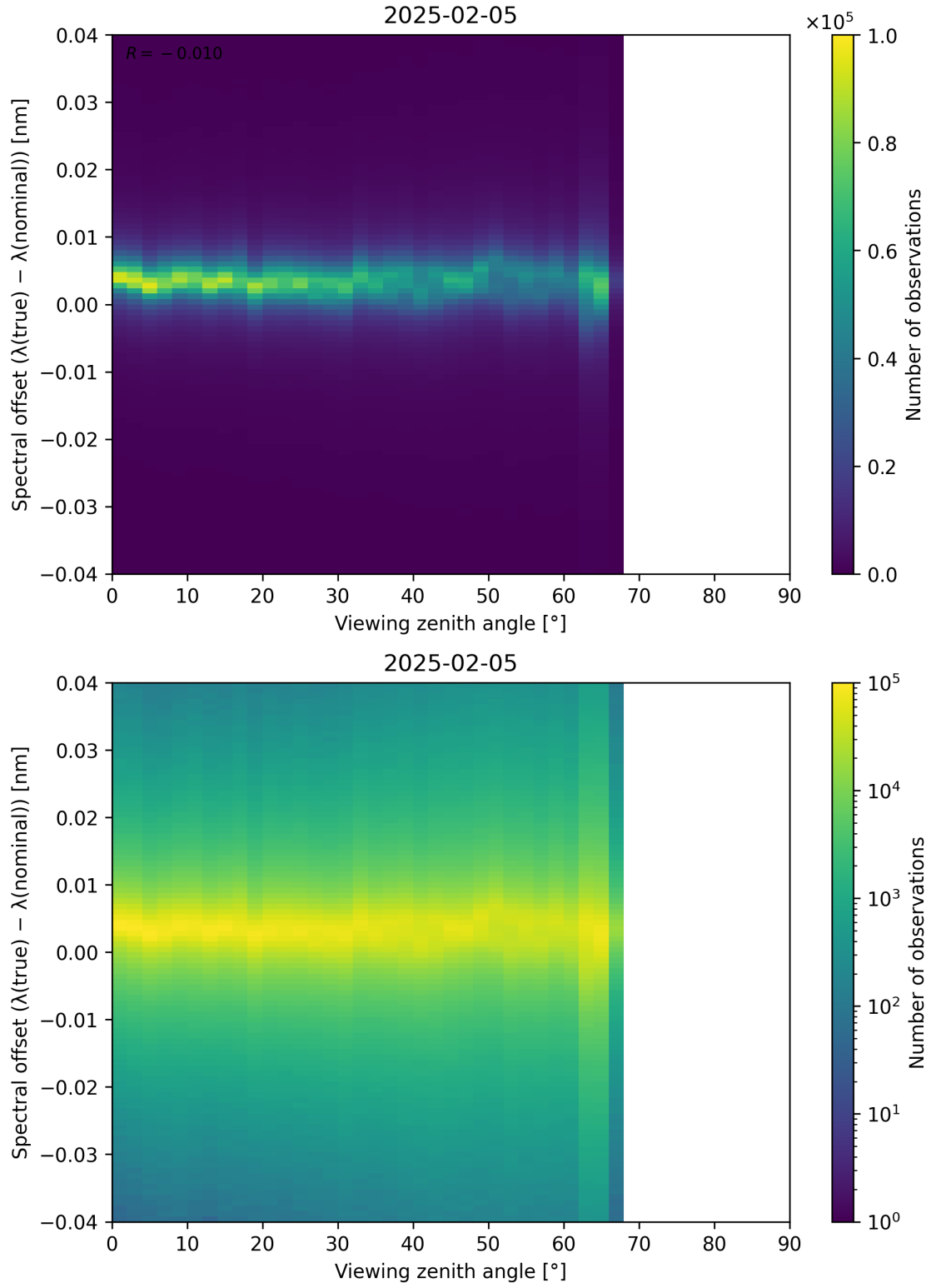
Figure 128: Scatter density plot of “Viewing zenith angle” against “Spectral offset ( \lambda_{\text{true}} - \lambda_{\text{nominal}} )” for 2025-02-04 to 2025-02-06.
