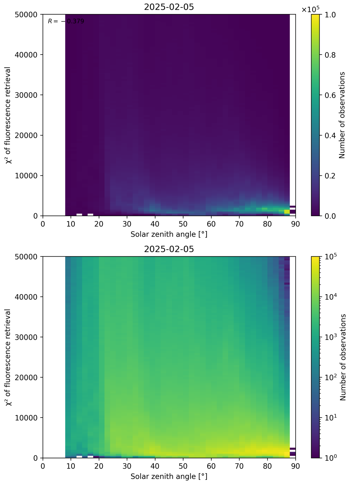
Figure 109: Scatter density plot of “Solar zenith angle” against “ \chi^2 of fluorescence retrieval” for 2025-02-04 to 2025-02-06.
