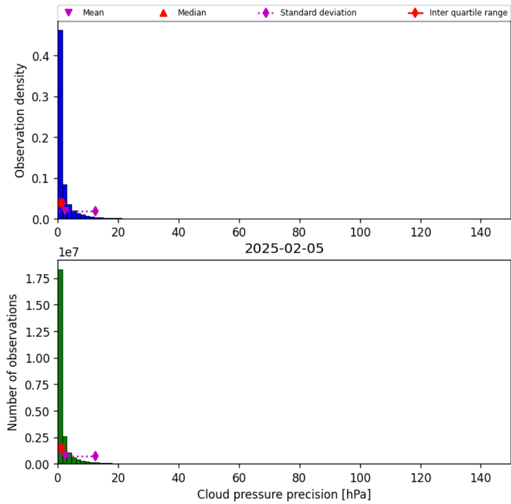
Figure 31: Histogram of “Cloud pressure precision” for 2025-02-04 to 2025-02-06
