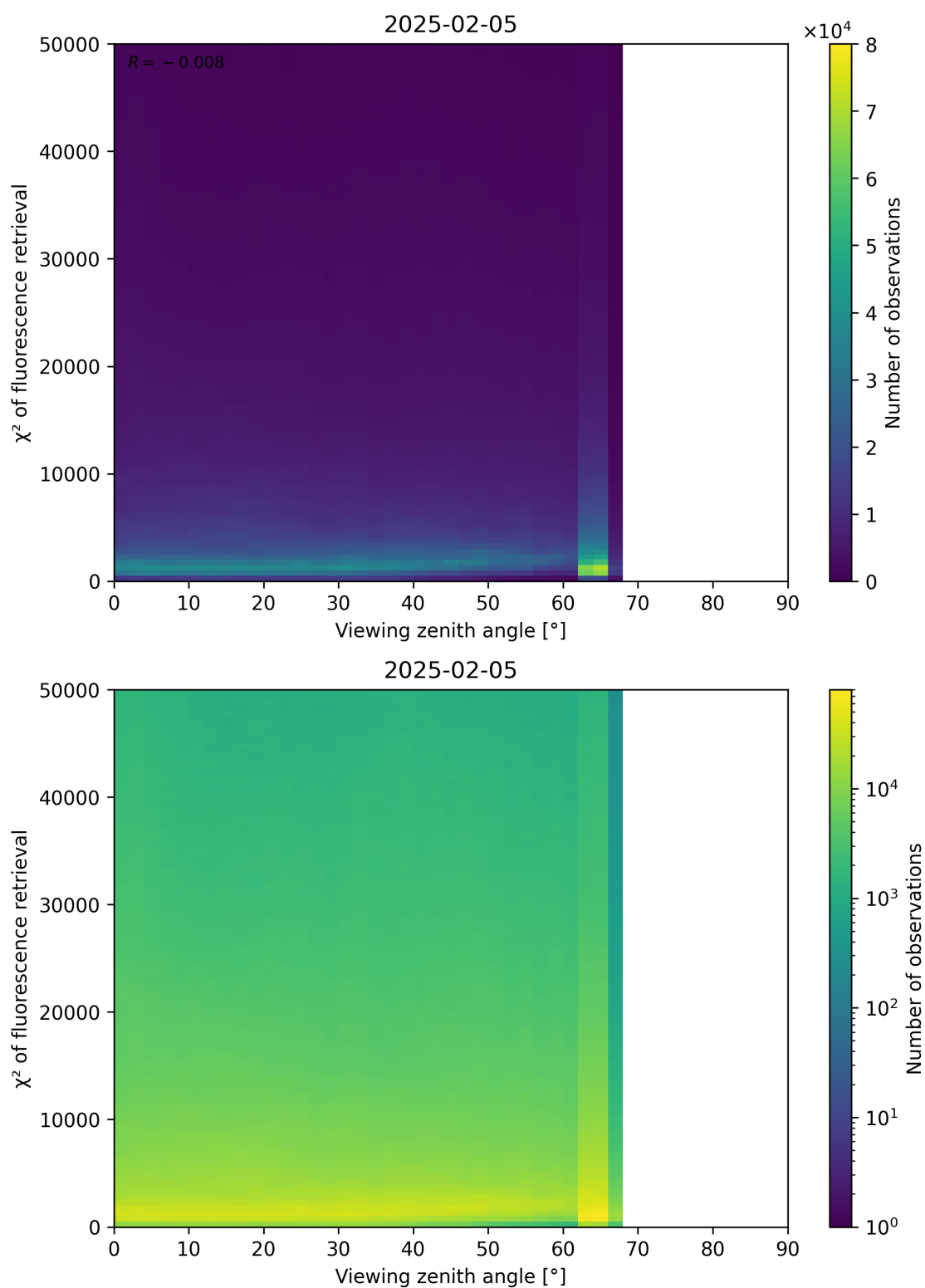
Figure 119: Scatter density plot of “Viewing zenith angle” against “ \chi^2 of fluorescence retrieval” for 2025-02-04 to 2025-02-06.
