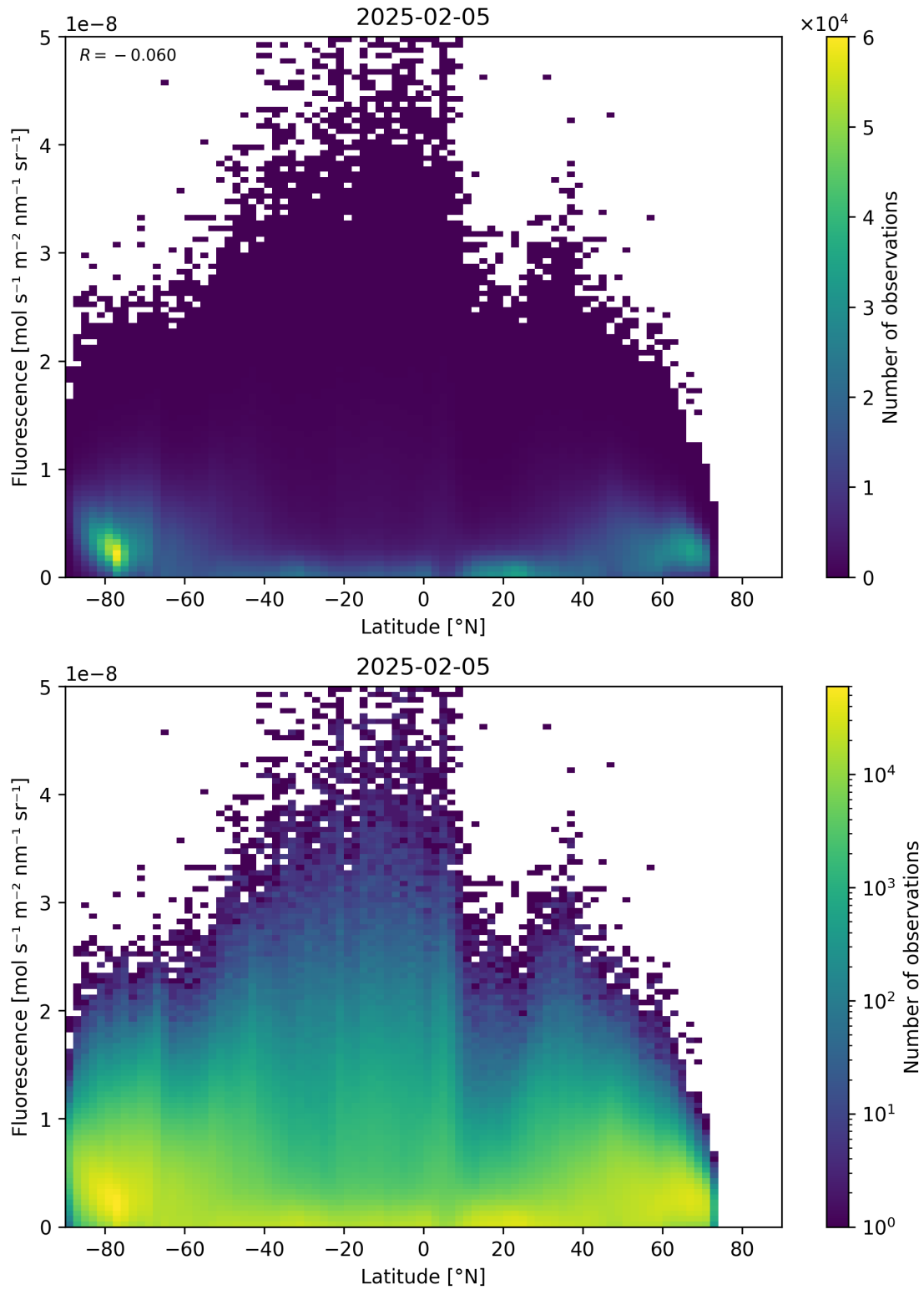
Figure 92: Scatter density plot of “Latitude” against “Fluorescence” for 2025-02-04 to 2025-02-06.
