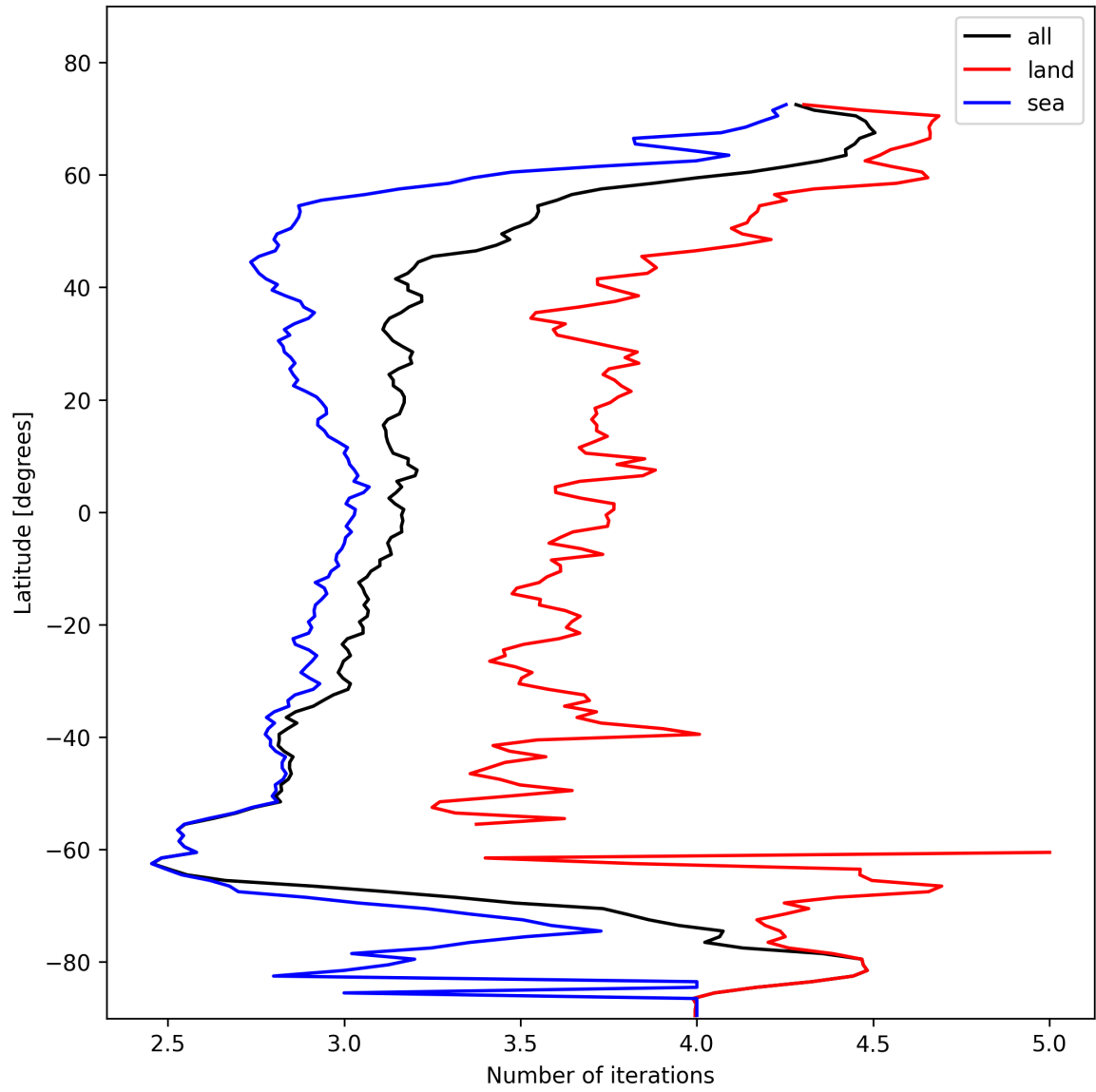
Figure 22: Zonal average of “Number of iterations” for 2025-02-04 to 2025-02-06.
