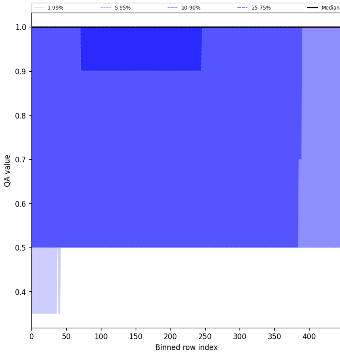
Figure 46: Along track statistics of “QA value” for 2025-02-04 to 2025-02-06
