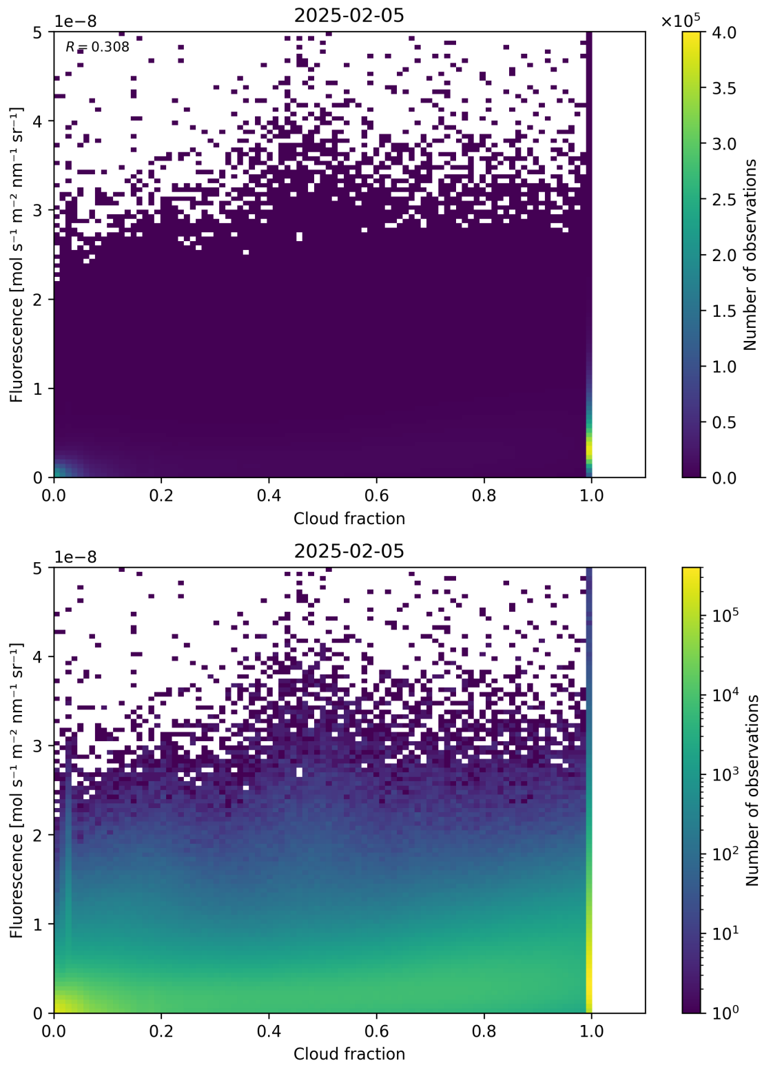
Figure 72: Scatter density plot of “Cloud fraction” against “Fluorescence” for 2025-02-04 to 2025-02-06.
