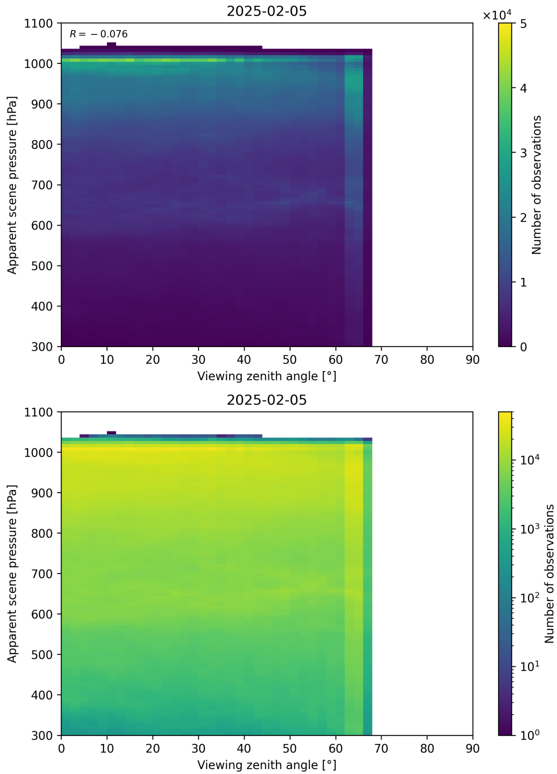
Figure 118: Scatter density plot of “Viewing zenith angle” against “Apparent scene pressure” for 2025-02-04 to 2025-02-06.
