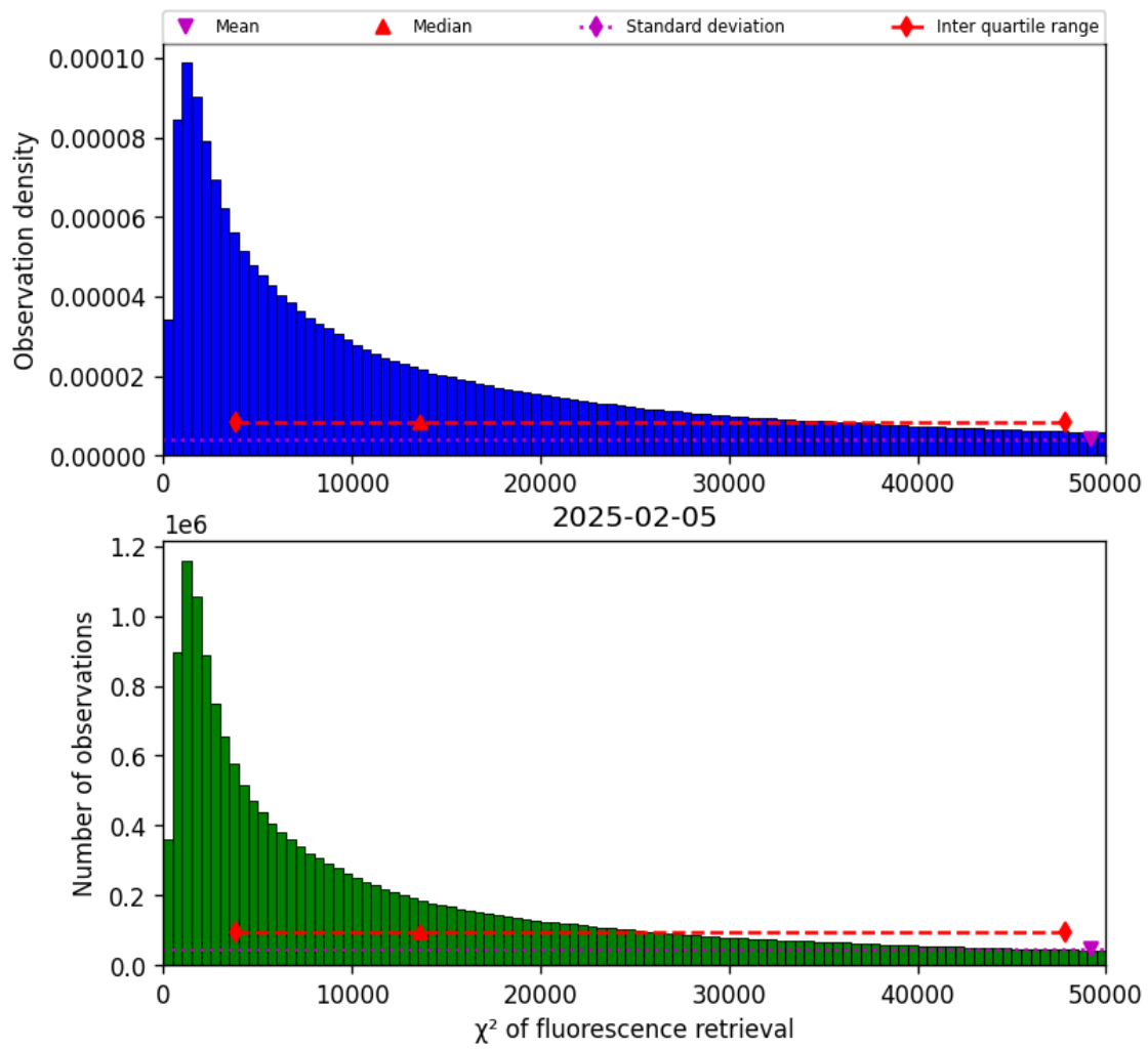
Figure 42: Histogram of “ \chi^2 of fluorescence retrieval” for 2025-02-04 to 2025-02-06
