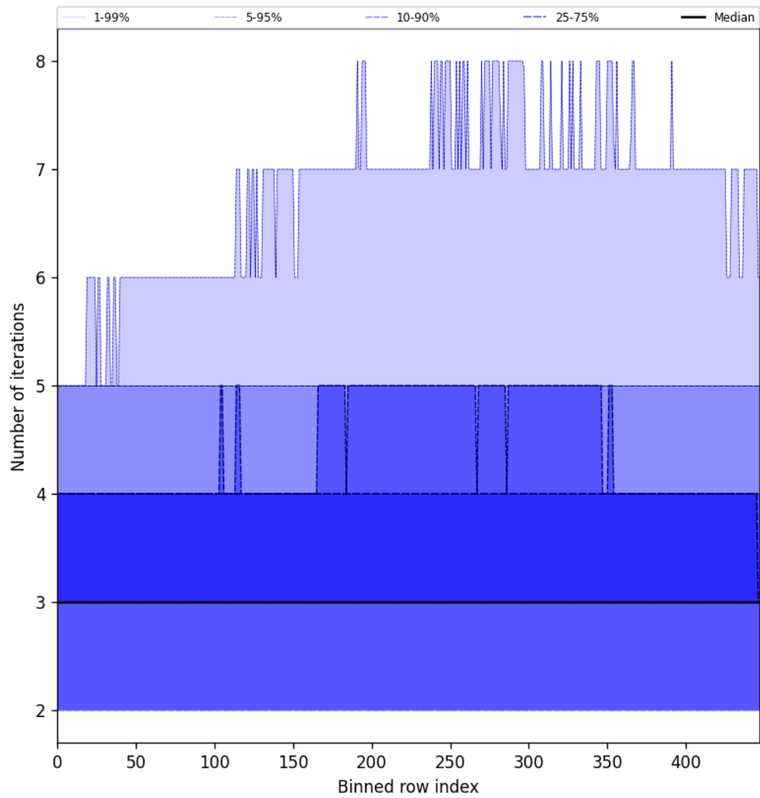
Figure 56: Along track statistics of “Number of iterations” for 2025-02-04 to 2025-02-06
