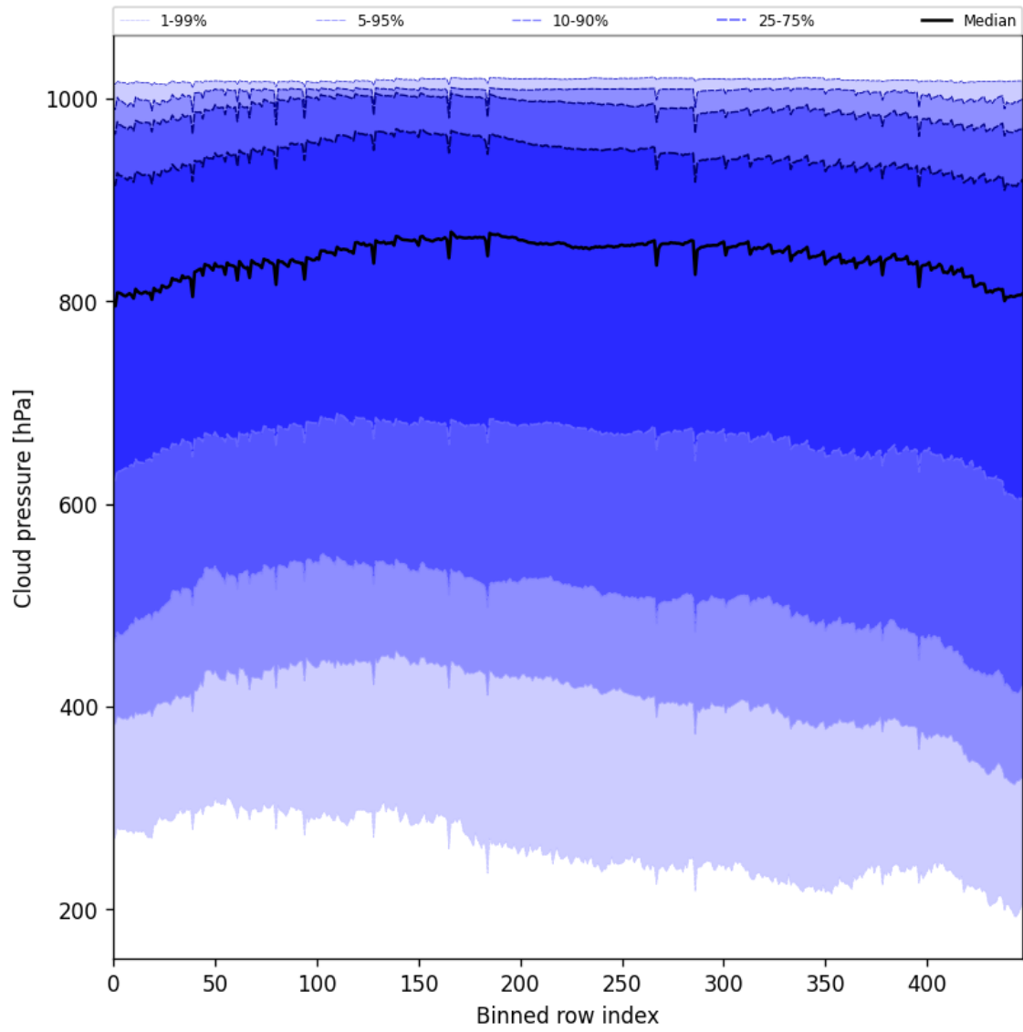
Figure 47: Along track statistics of “Cloud pressure” for 2025-02-04 to 2025-02-06
