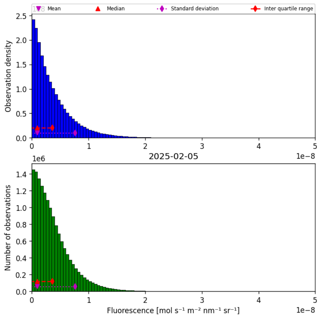
Figure 40: Histogram of “Fluorescence” for 2025-02-04 to 2025-02-06
