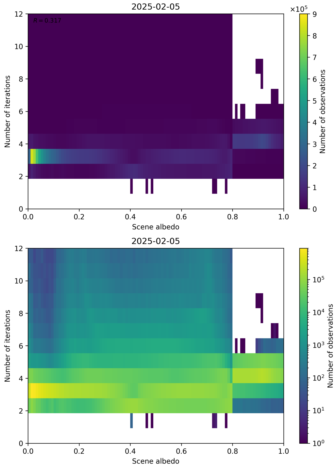
Figure 105: Scatter density plot of “Scene albedo” against “Number of iterations” for 2025-02-04 to 2025-02-06.
