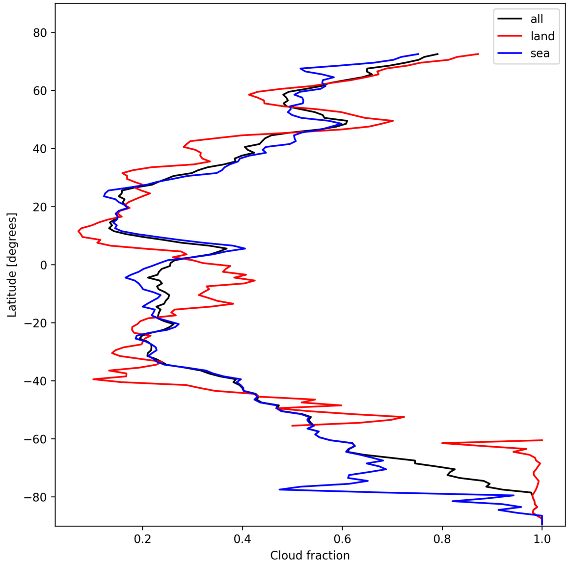
Figure 15: Zonal average of “Cloud fraction” for 2025-02-04 to 2025-02-06.
