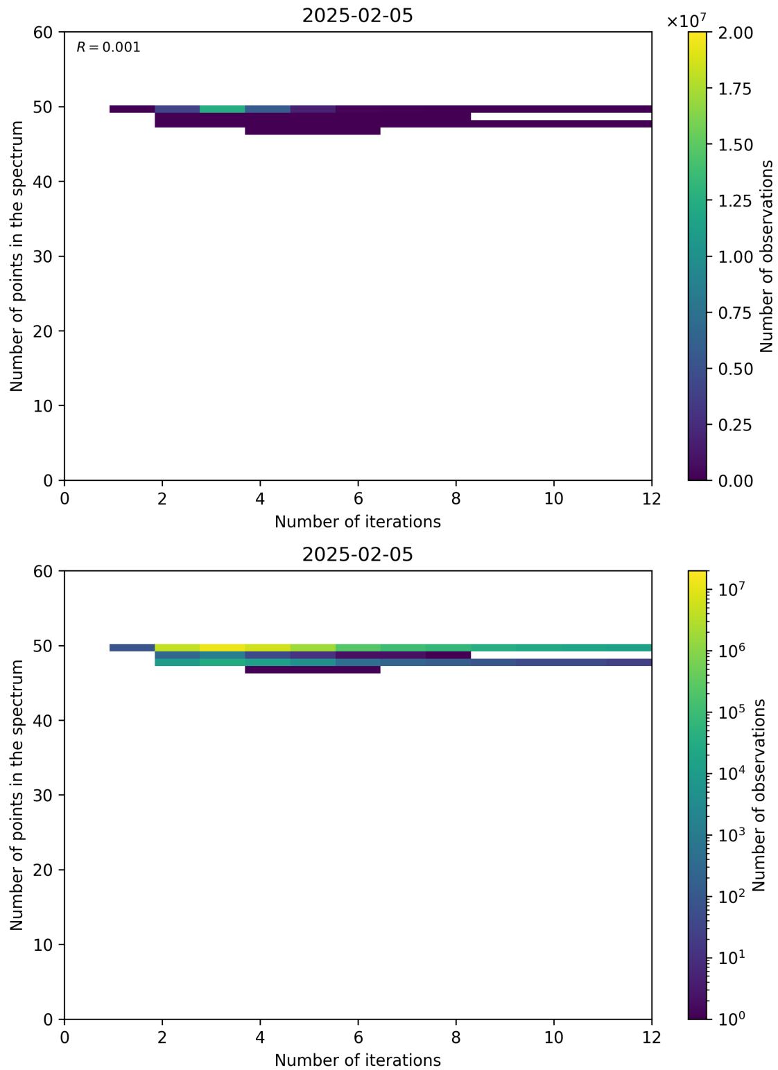
Figure 99: Scatter density plot of “Number of iterations” against “Number of points in the spectrum” for 2025-02-04 to 2025-02-06.
