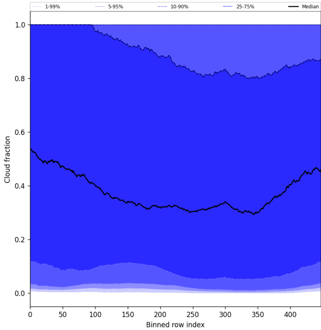
Figure 49: Along track statistics of “Cloud fraction” for 2025-02-04 to 2025-02-06
