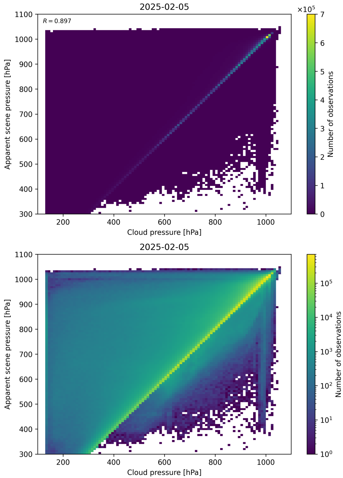
Figure 77: Scatter density plot of “Cloud pressure” against “Apparent scene pressure” for 2025-02-04 to 2025-02-06.
