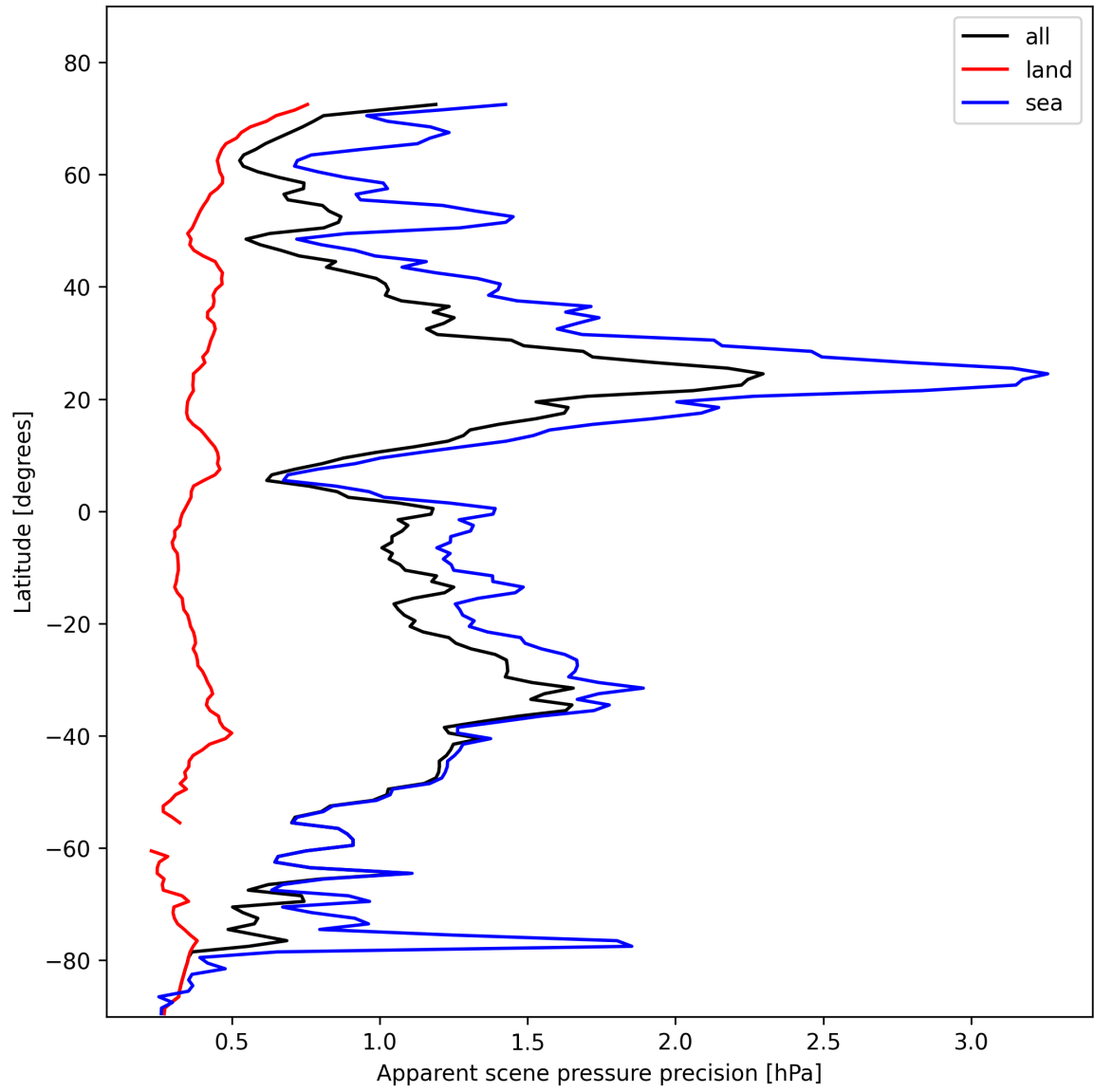
Figure 20: Zonal average of “Apparent scene pressure precision” for 2025-02-04 to 2025-02-06.
