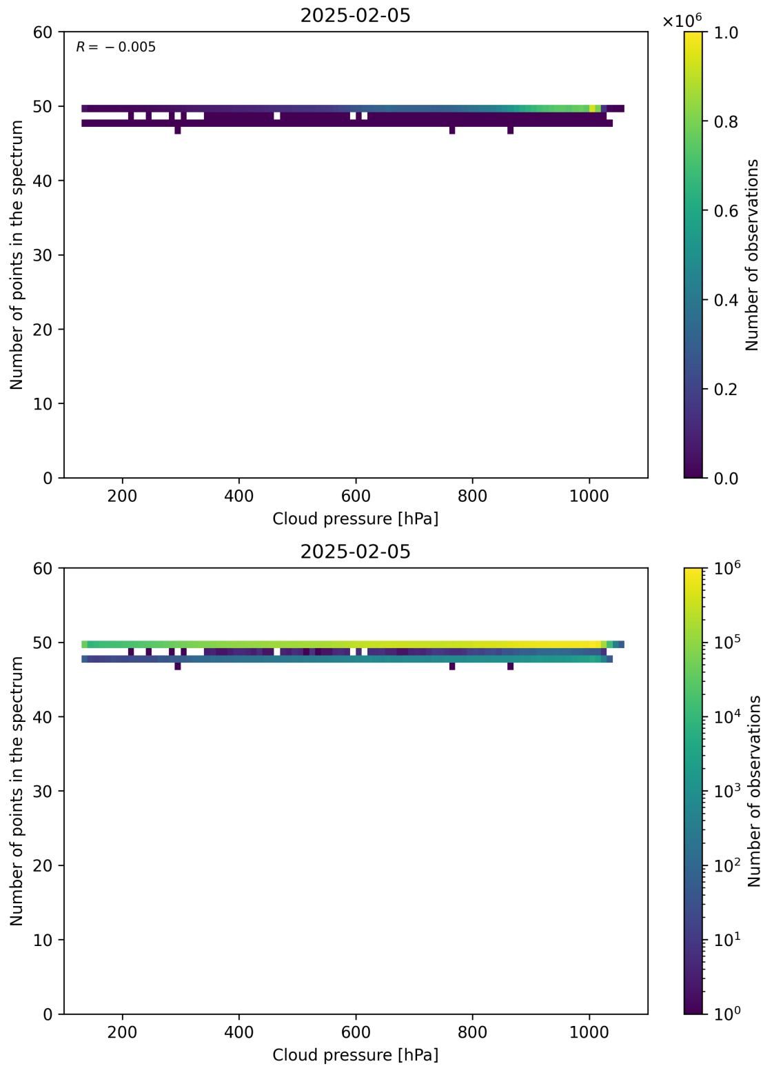
Figure 82: Scatter density plot of “Cloud pressure” against “Number of points in the spectrum” for 2025-02-04 to 2025-02-06.
