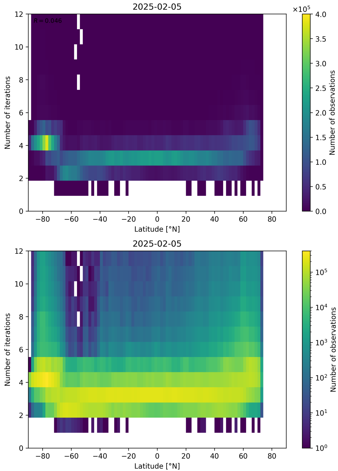
Figure 93: Scatter density plot of “Latitude” against “Number of iterations” for 2025-02-04 to 2025-02-06.
