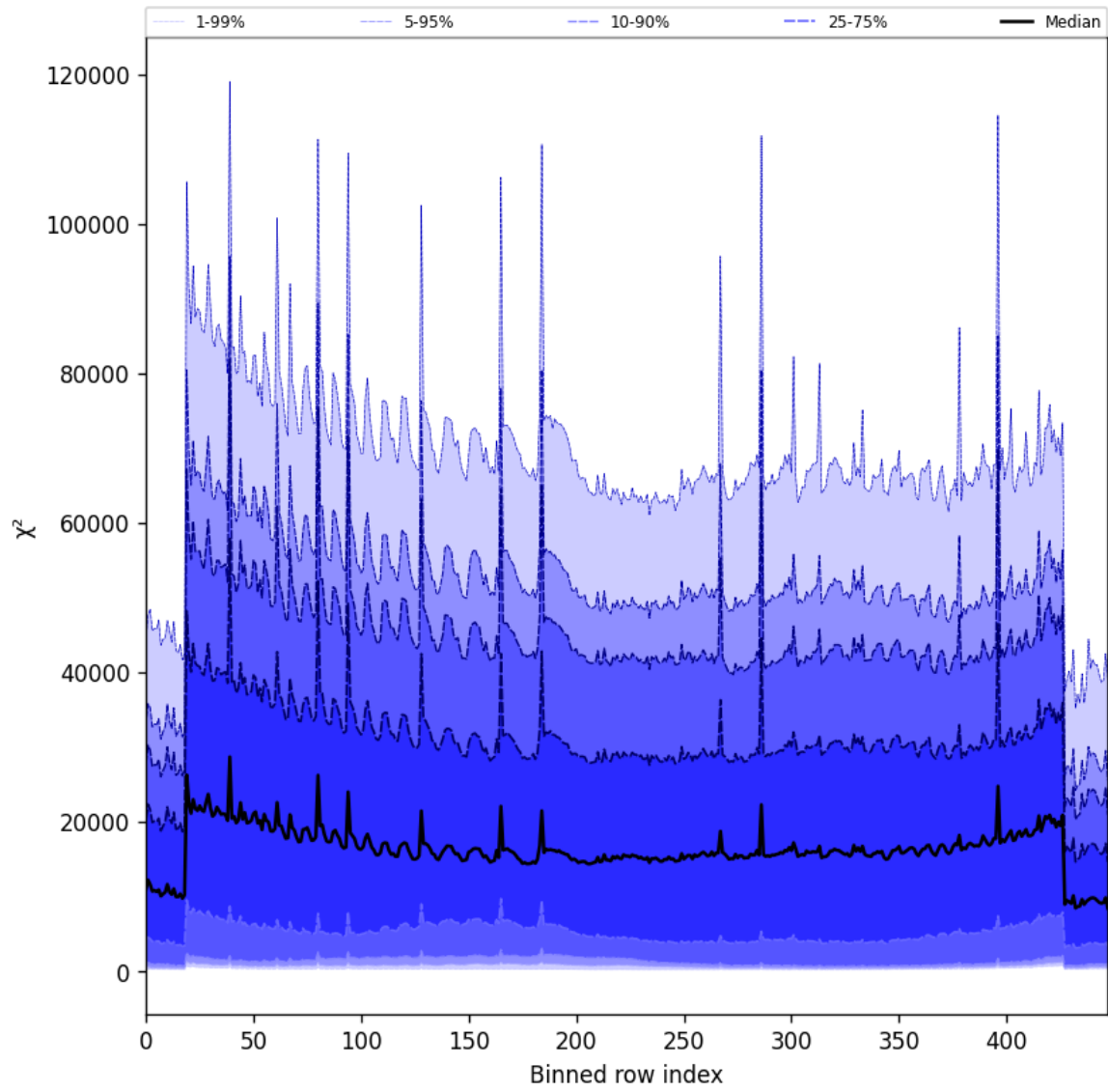
Figure 55: Along track statistics of “ \chi^2 ” for 2025-02-04 to 2025-02-06
