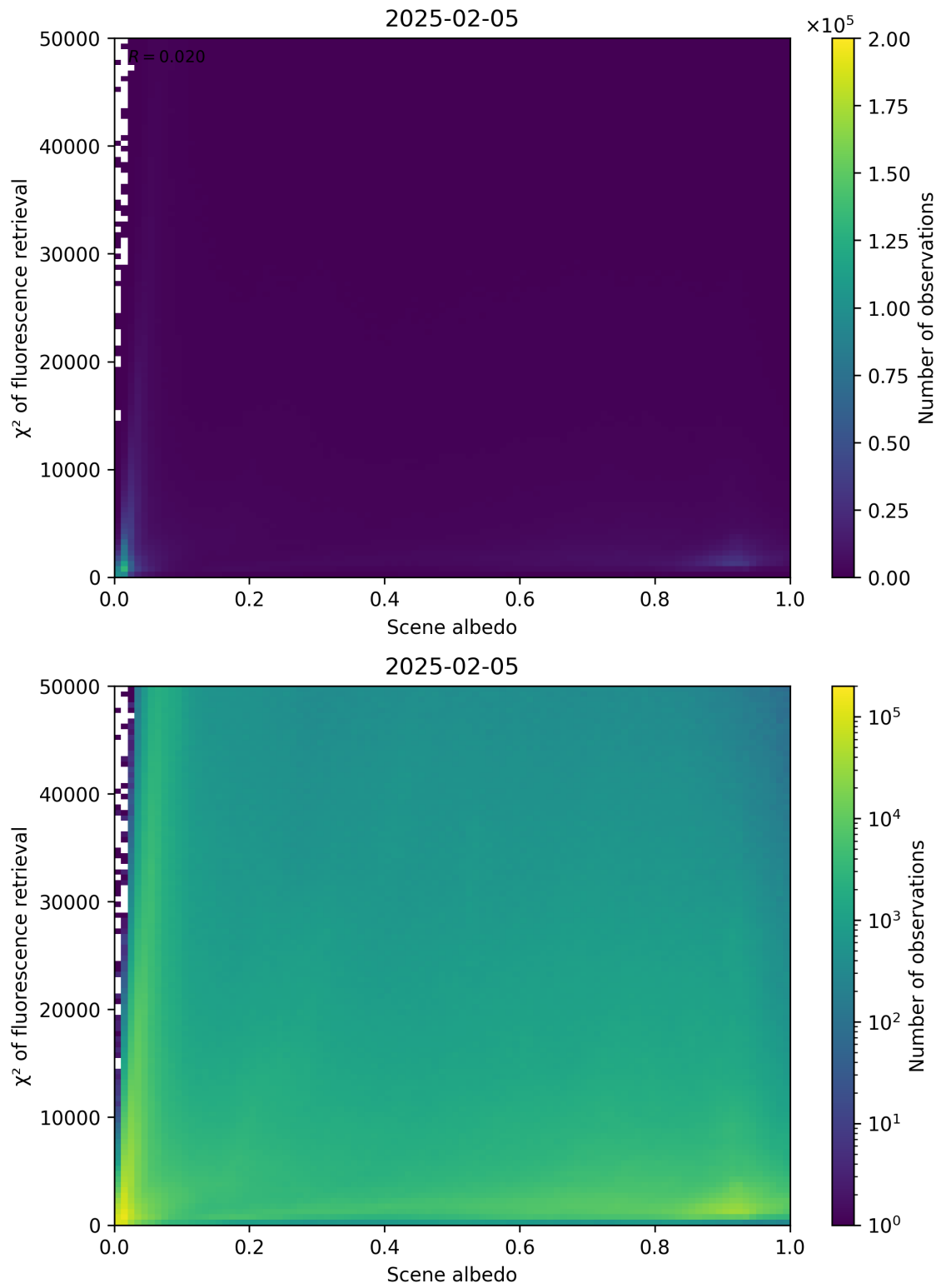
Figure 103: Scatter density plot of “Scene albedo” against “ \chi^2 of fluorescence retrieval” for 2025-02-04 to 2025-02-06.
