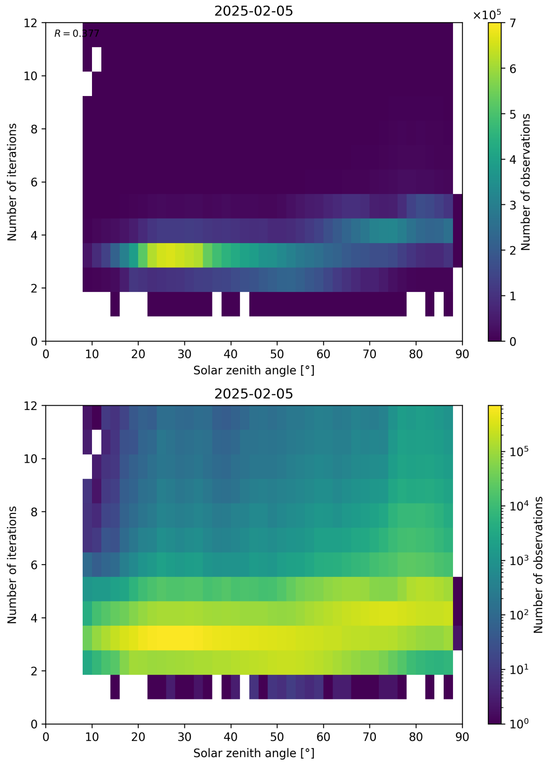
Figure 114: Scatter density plot of “Solar zenith angle” against “Number of iterations” for 2025-02-04 to 2025-02-06.
