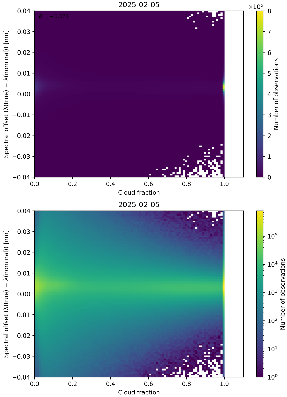
Figure 76: Scatter density plot of “Cloud fraction” against “Spectral offset ( \lambda_{\text{true}} - \lambda_{\text{nominal}} )” for 2025-02-04 to 2025-02-06.
