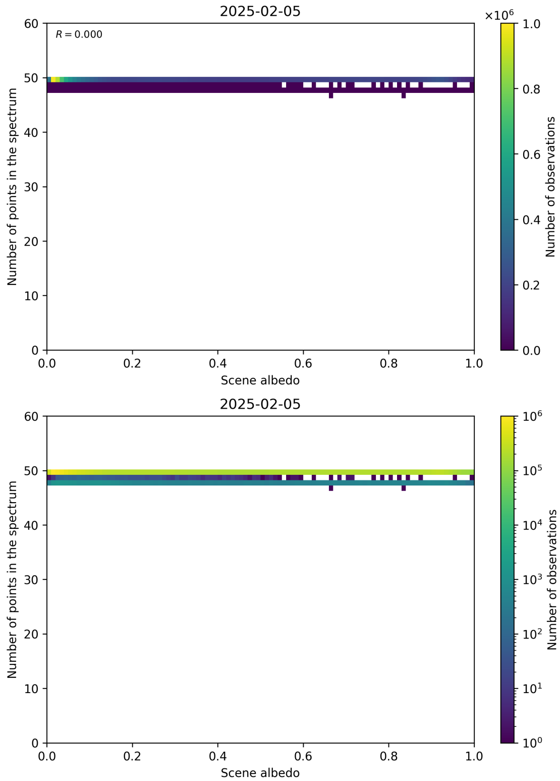
Figure 106: Scatter density plot of “Scene albedo” against “Number of points in the spectrum” for 2025-02-04 to 2025-02-06.
