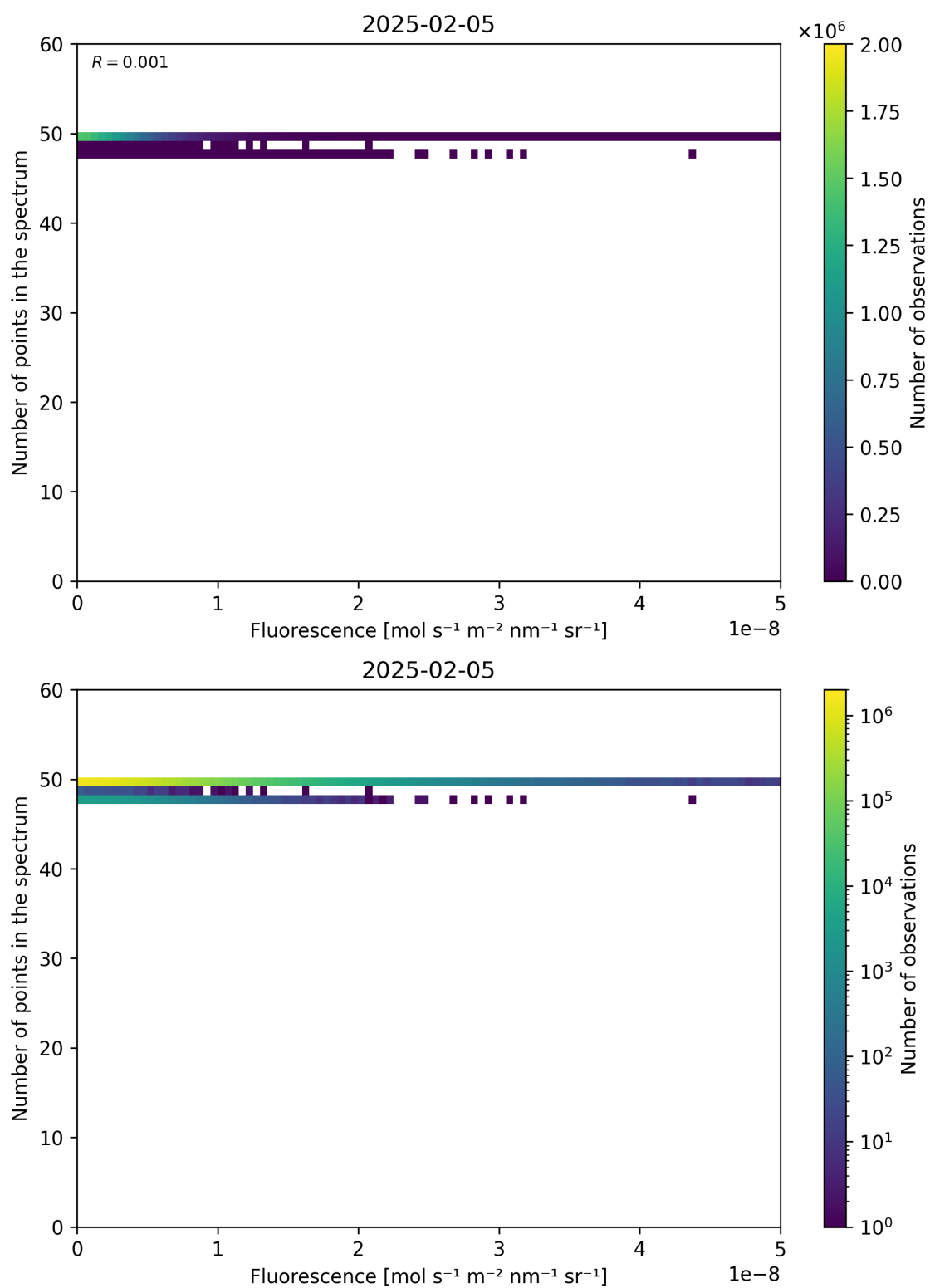
Figure 86: Scatter density plot of “Fluorescence” against “Number of points in the spectrum” for 2025-02-04 to 2025-02-06.
