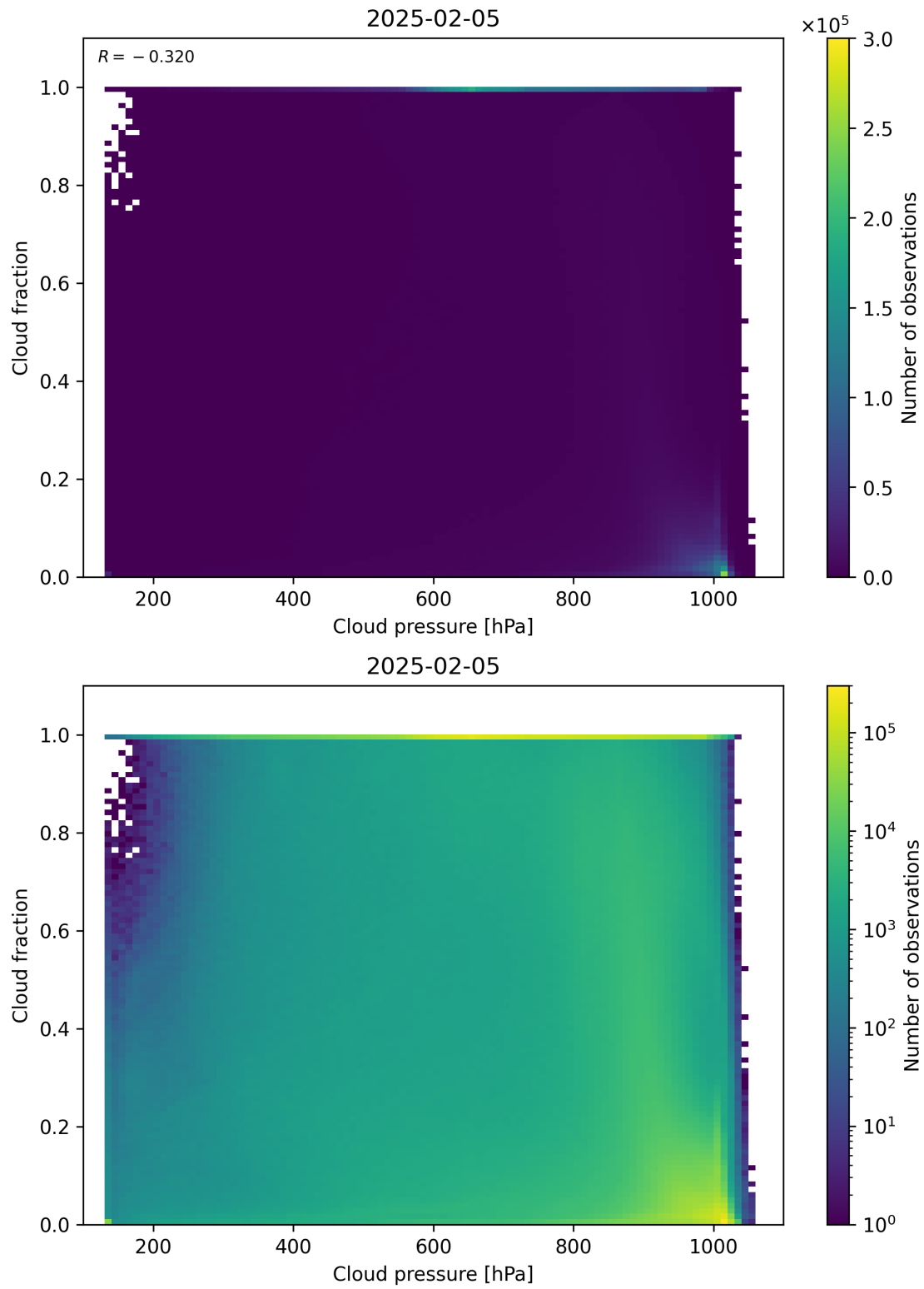
Figure 79: Scatter density plot of “Cloud pressure” against “Cloud fraction” for 2025-02-04 to 2025-02-06.
