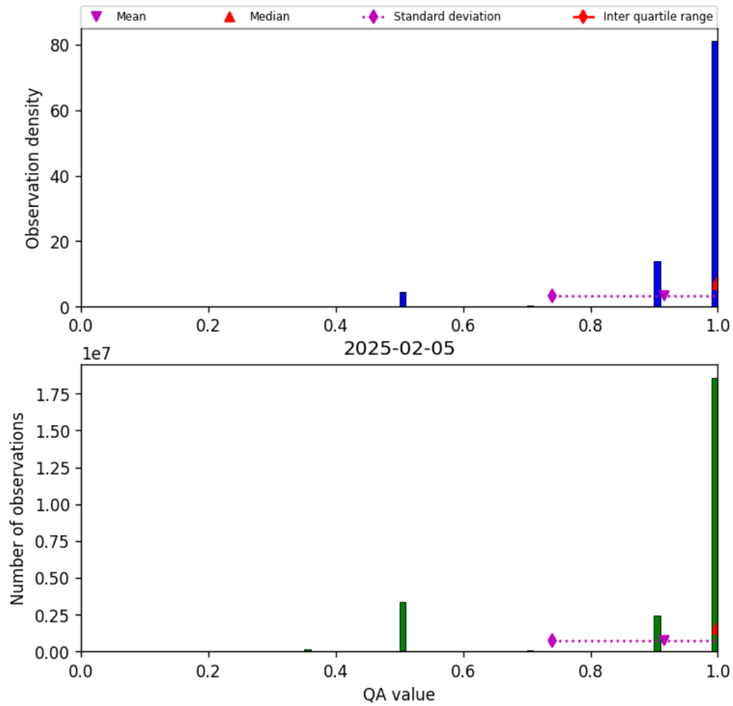
Figure 29: Histogram of “QA value” for 2025-02-04 to 2025-02-06
