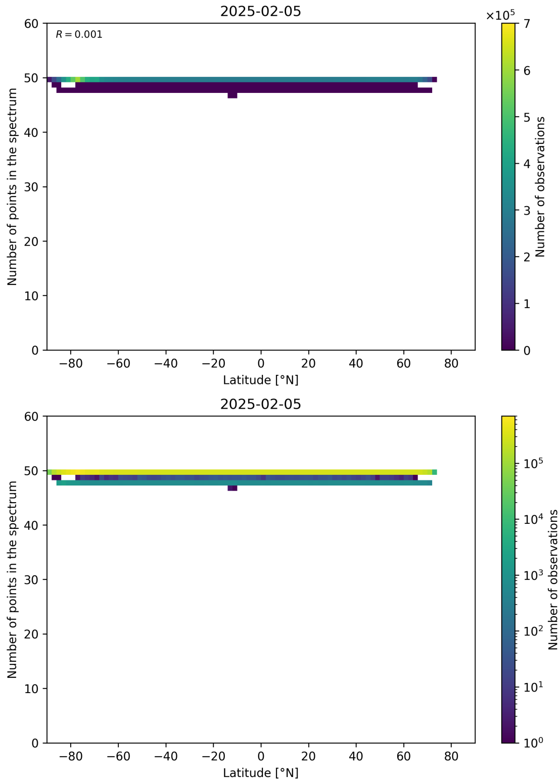
Figure 94: Scatter density plot of “Latitude” against “Number of points in the spectrum” for 2025-02-04 to 2025-02-06.
