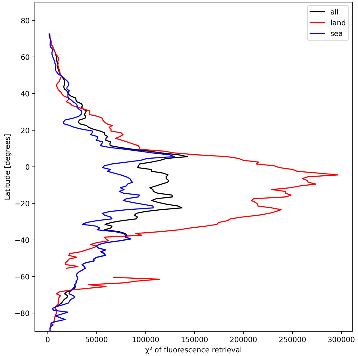
Figure 25: Zonal average of “ \chi^2 of fluorescence retrieval” for 2025-02-04 to 2025-02-06.
