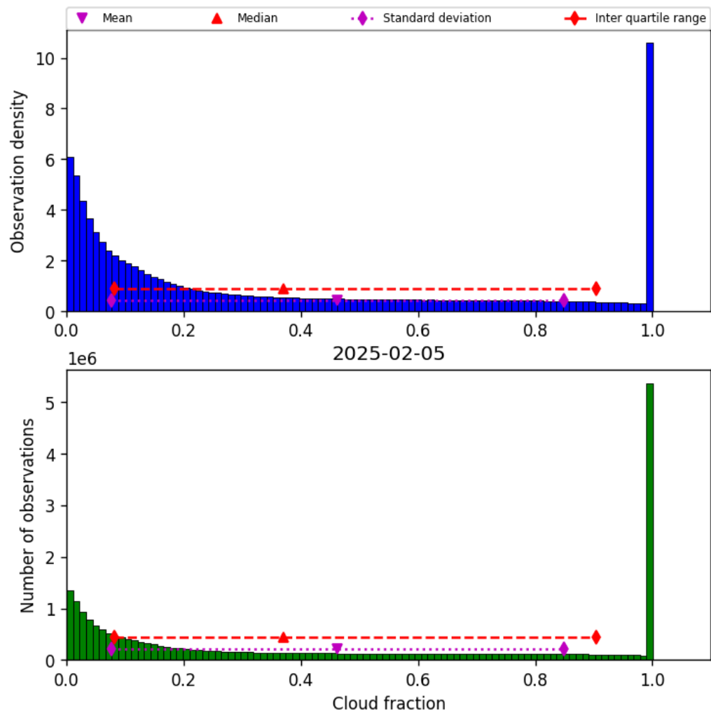
Figure 32: Histogram of “Cloud fraction” for 2025-02-04 to 2025-02-06
