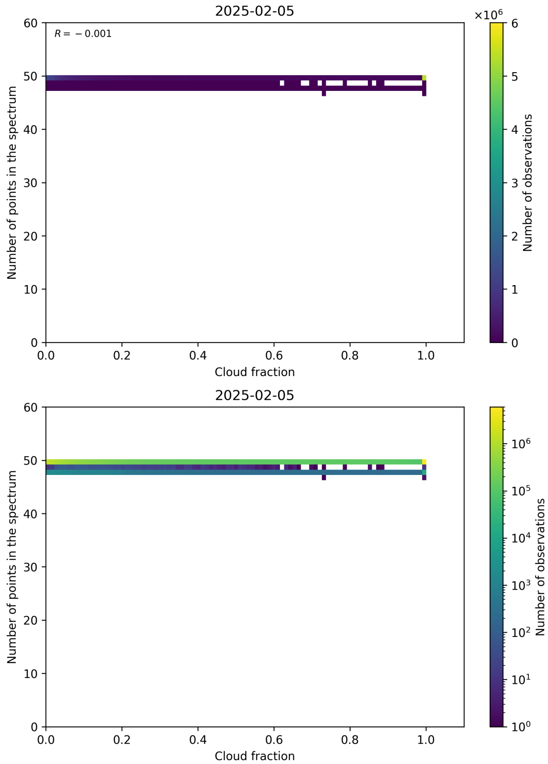
Figure 74: Scatter density plot of “Cloud fraction” against “Number of points in the spectrum” for 2025-02-04 to 2025-02-06.
