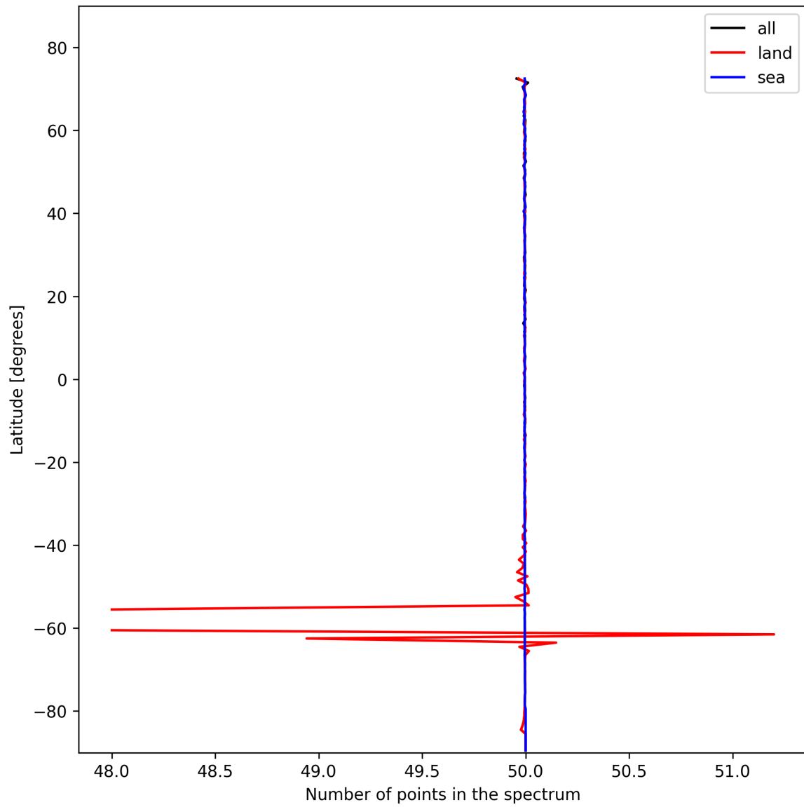
Figure 27: Zonal average of “Number of points in the spectrum” for 2025-02-04 to 2025-02-06.
