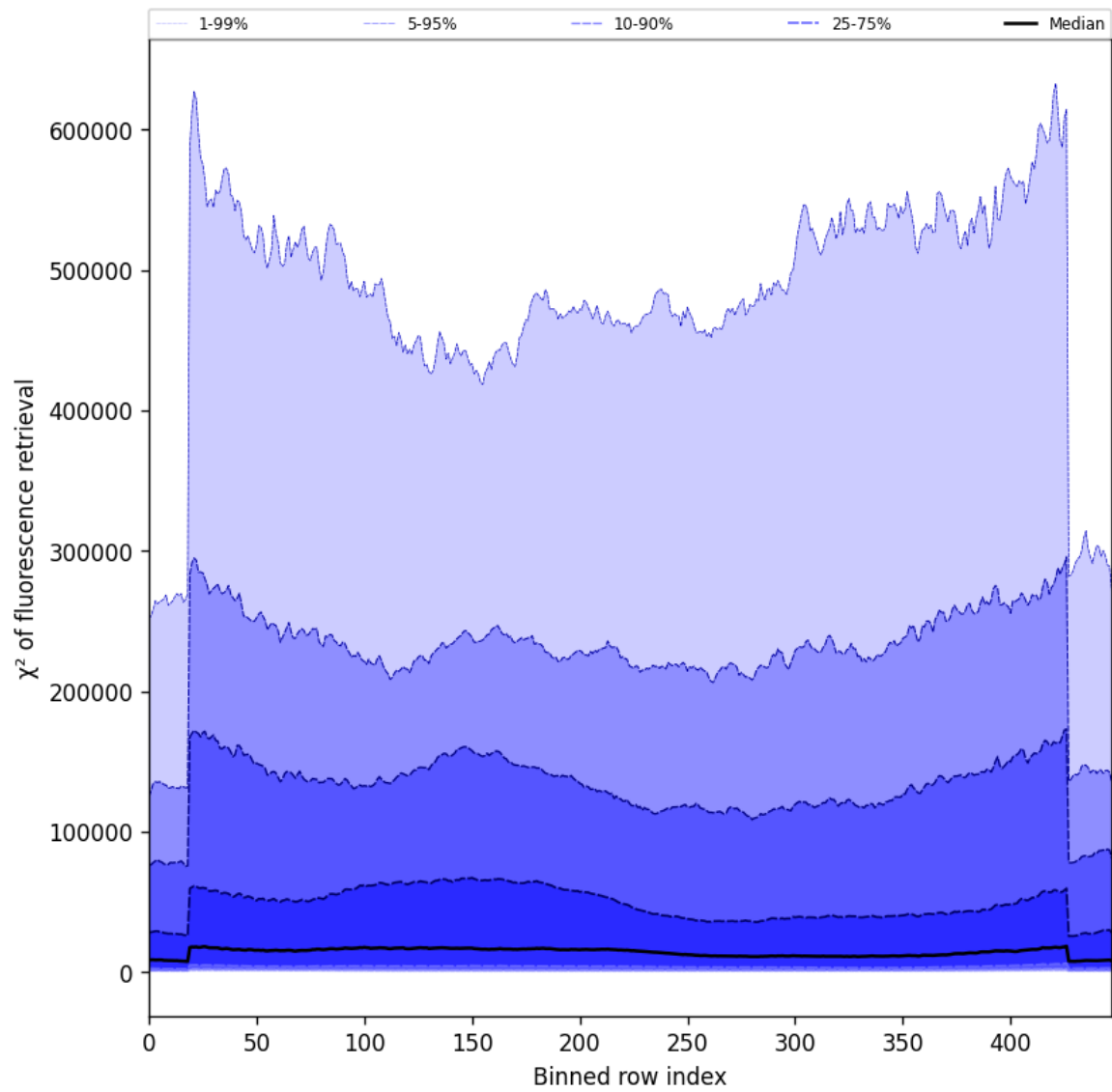
Figure 59: Along track statistics of “ \chi^2 of fluorescence retrieval” for 2025-02-04 to 2025-02-06
