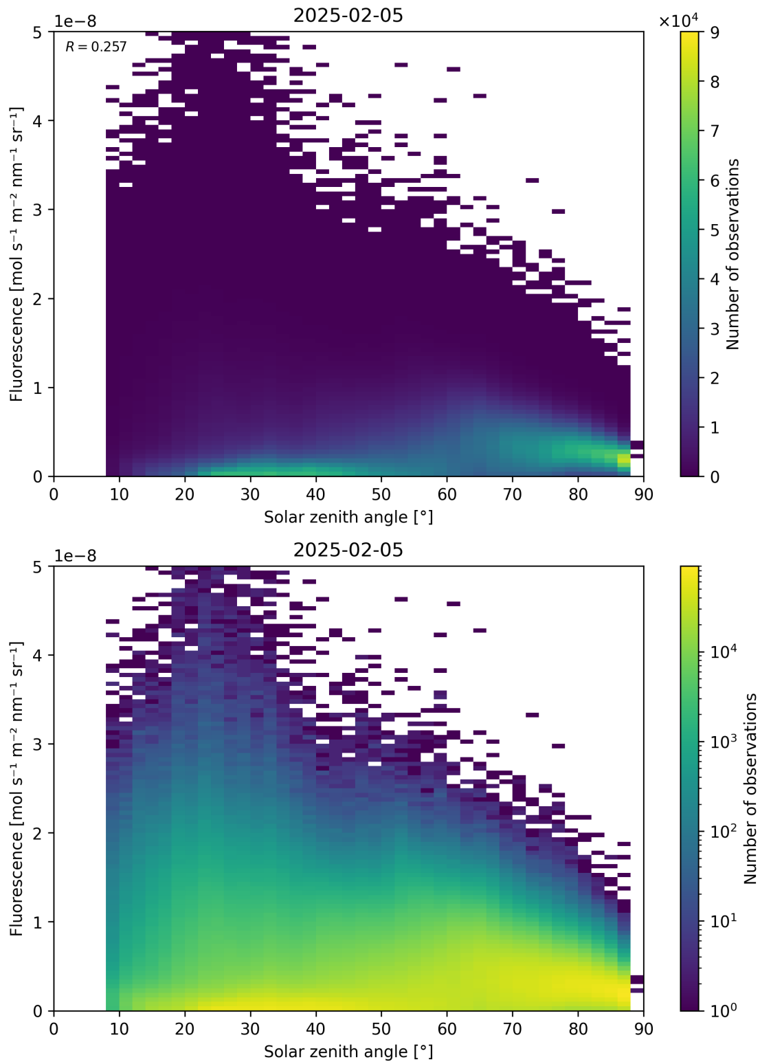
Figure 112: Scatter density plot of “Solar zenith angle” against “Fluorescence” for 2025-02-04 to 2025-02-06.
