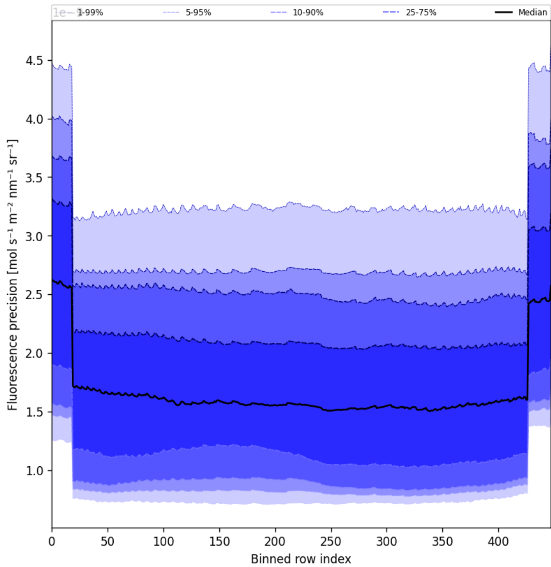
Figure 58: Along track statistics of “Fluorescence precision” for 2025-02-04 to 2025-02-06
