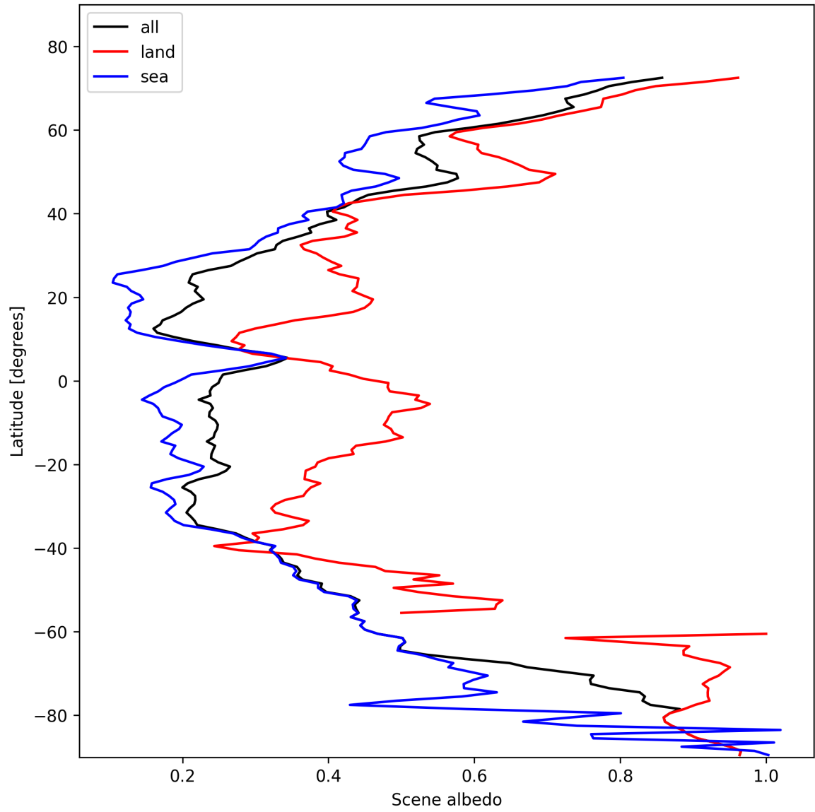
Figure 17: Zonal average of “Scene albedo” for 2025-02-04 to 2025-02-06.
