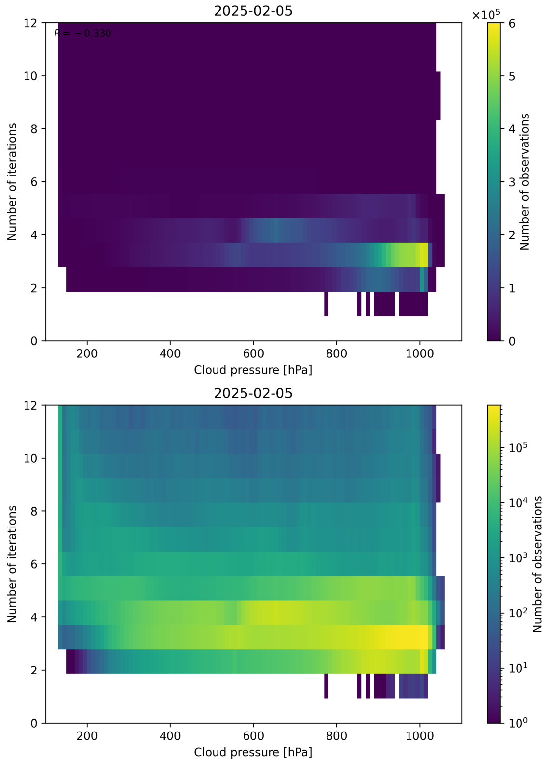
Figure 81: Scatter density plot of “Cloud pressure” against “Number of iterations” for 2025-02-04 to 2025-02-06.
