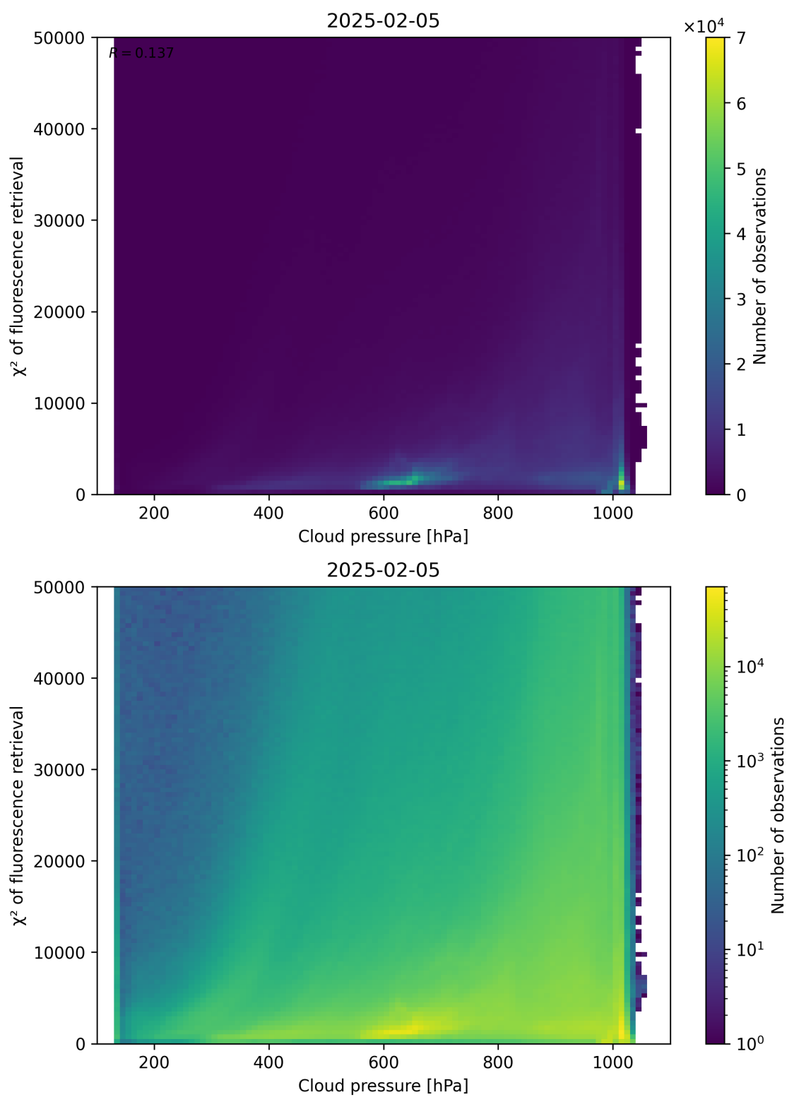
Figure 78: Scatter density plot of “Cloud pressure” against “ \chi^2 of fluorescence retrieval” for 2025-02-04 to 2025-02-06.
