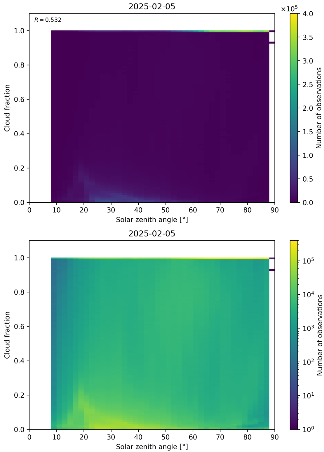
Figure 110: Scatter density plot of “Solar zenith angle” against “Cloud fraction” for 2025-02-04 to 2025-02-06.
