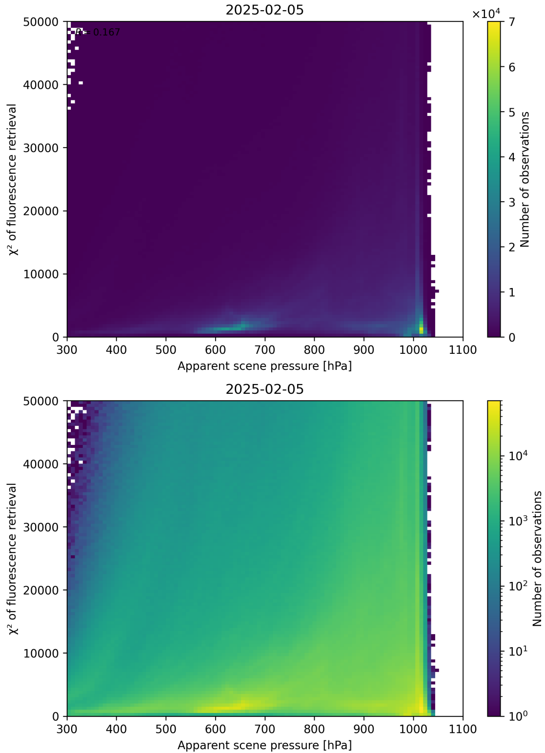
Figure 63: Scatter density plot of “Apparent scene pressure” against “ \chi^2 of fluorescence retrieval” for 2025-02-04 to 2025-02-06.
