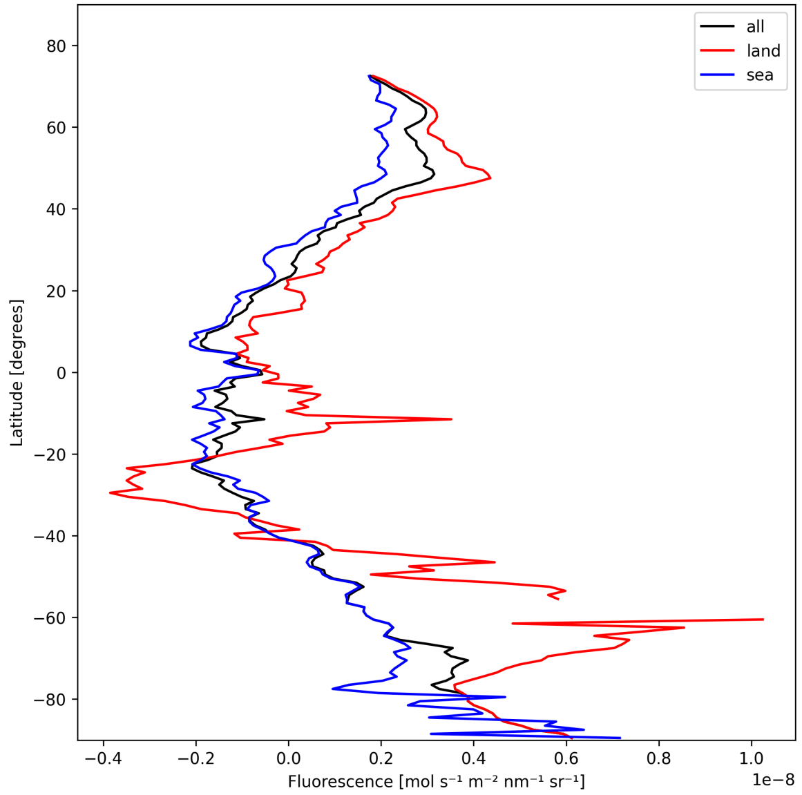
Figure 23: Zonal average of “Fluorescence” for 2025-02-04 to 2025-02-06.
