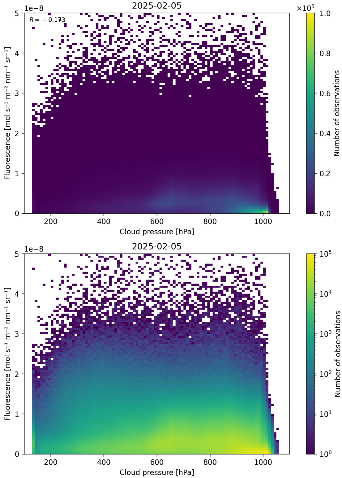
Figure 80: Scatter density plot of “Cloud pressure” against “Fluorescence” for 2025-02-04 to 2025-02-06.
