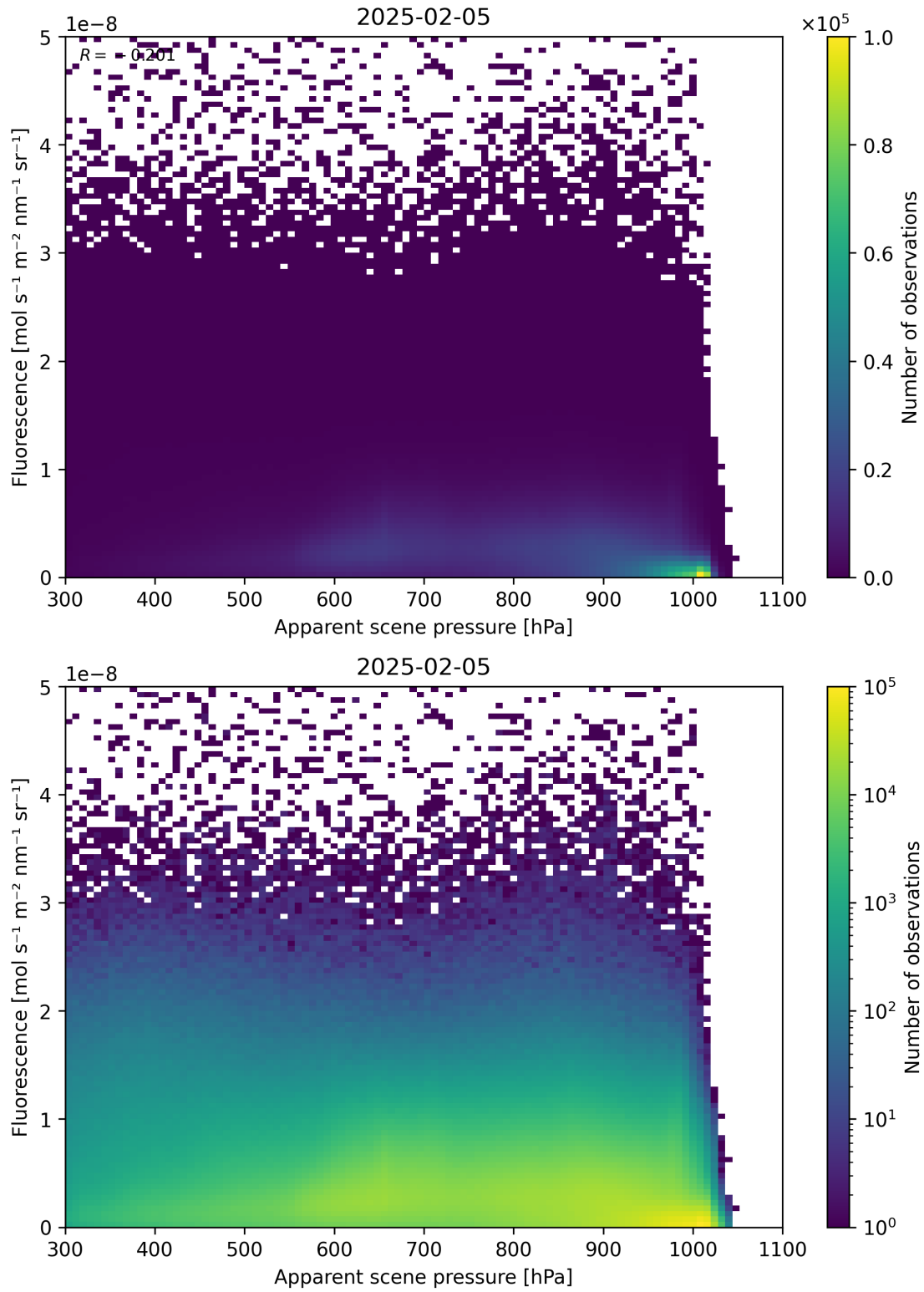
Figure 64: Scatter density plot of “Apparent scene pressure” against “Fluorescence” for 2025-02-04 to 2025-02-06.
