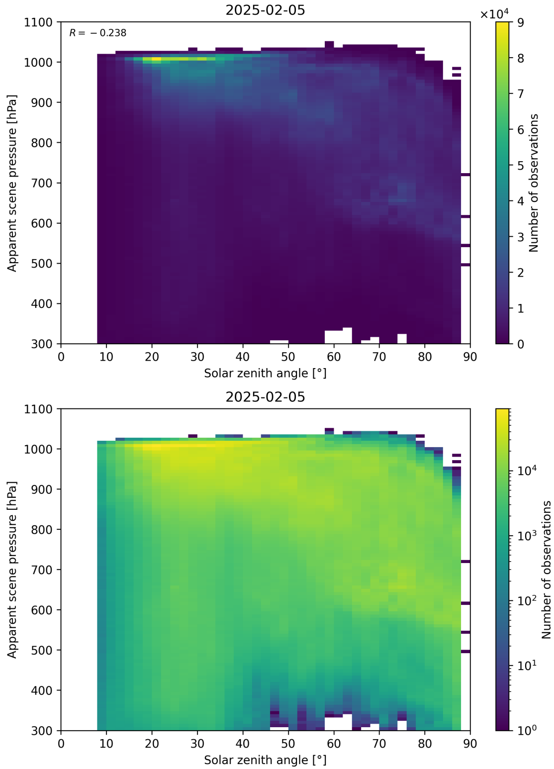
Figure 108: Scatter density plot of “Solar zenith angle” against “Apparent scene pressure” for 2025-02-04 to 2025-02-06.
