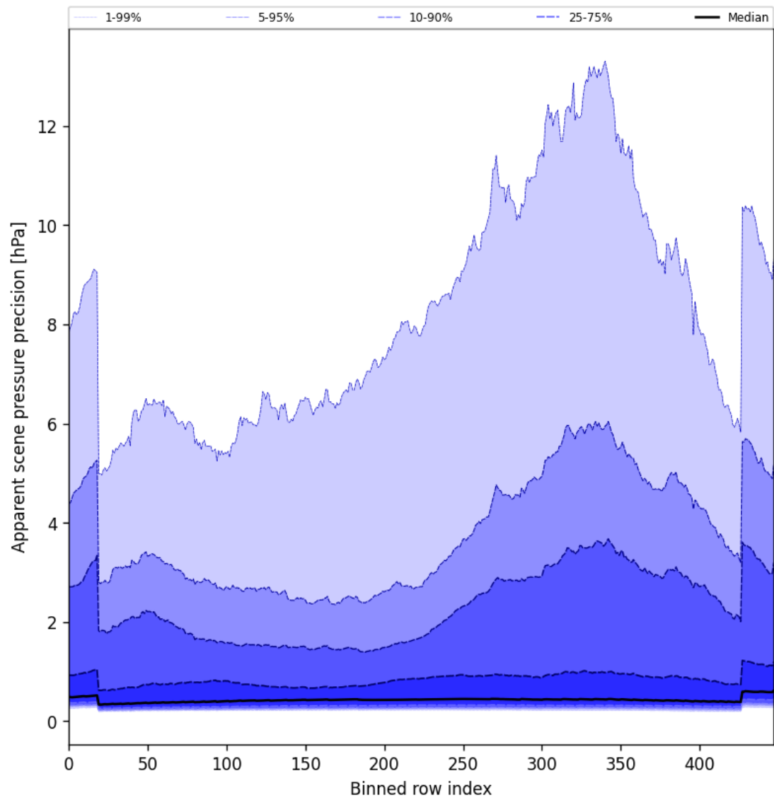
Figure 54: Along track statistics of “Apparent scene pressure precision” for 2025-02-04 to 2025-02-06
