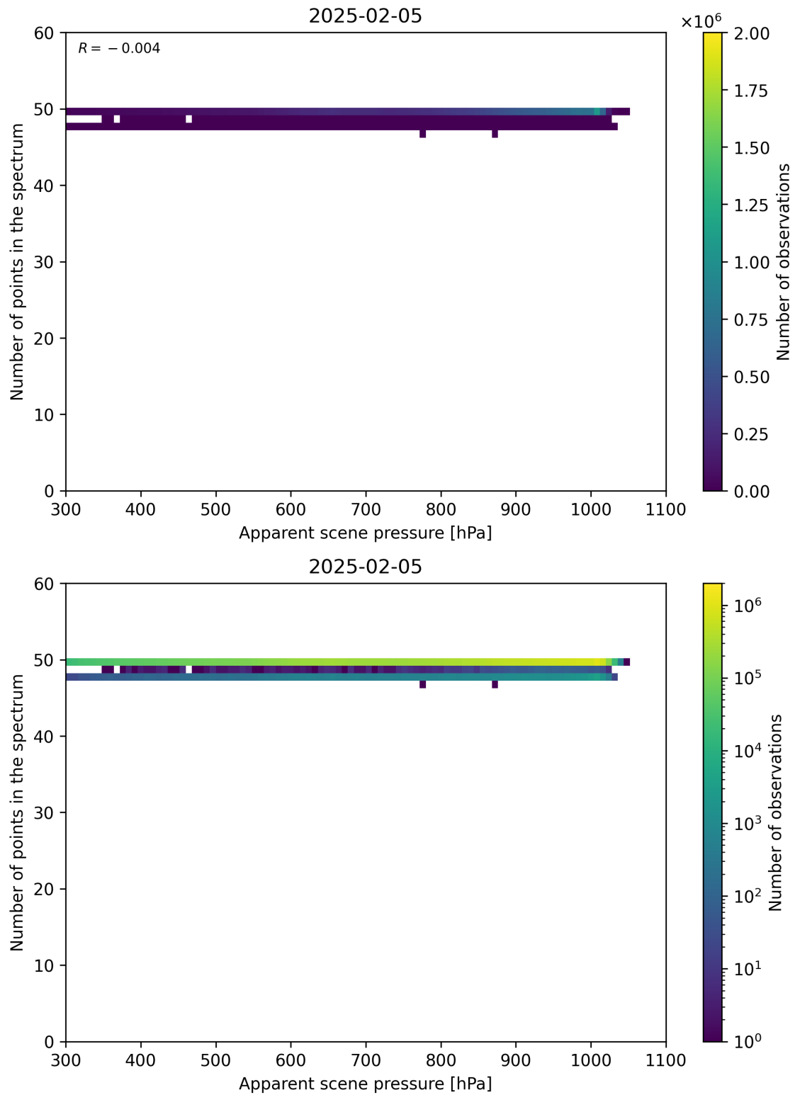
Figure 66: Scatter density plot of “Apparent scene pressure” against “Number of points in the spectrum” for 2025-02-04 to 2025-02-06.
