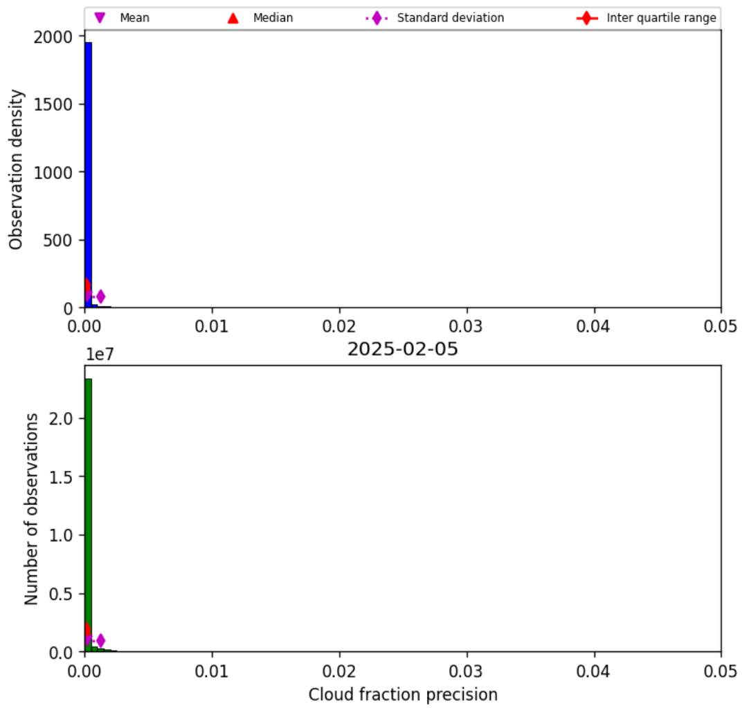
Figure 33: Histogram of “Cloud fraction precision” for 2025-02-04 to 2025-02-06
