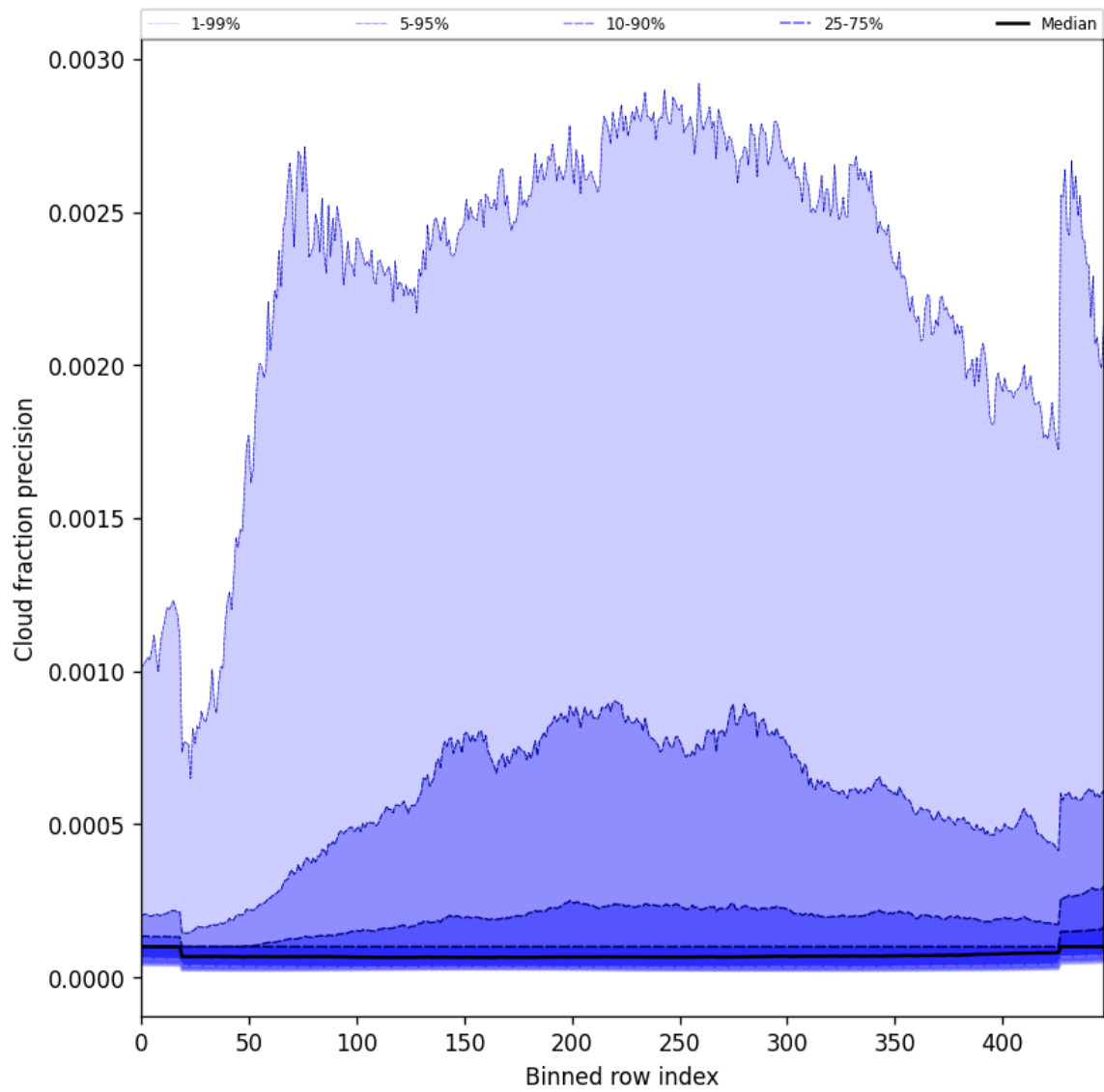
Figure 50: Along track statistics of “Cloud fraction precision” for 2025-02-04 to 2025-02-06
