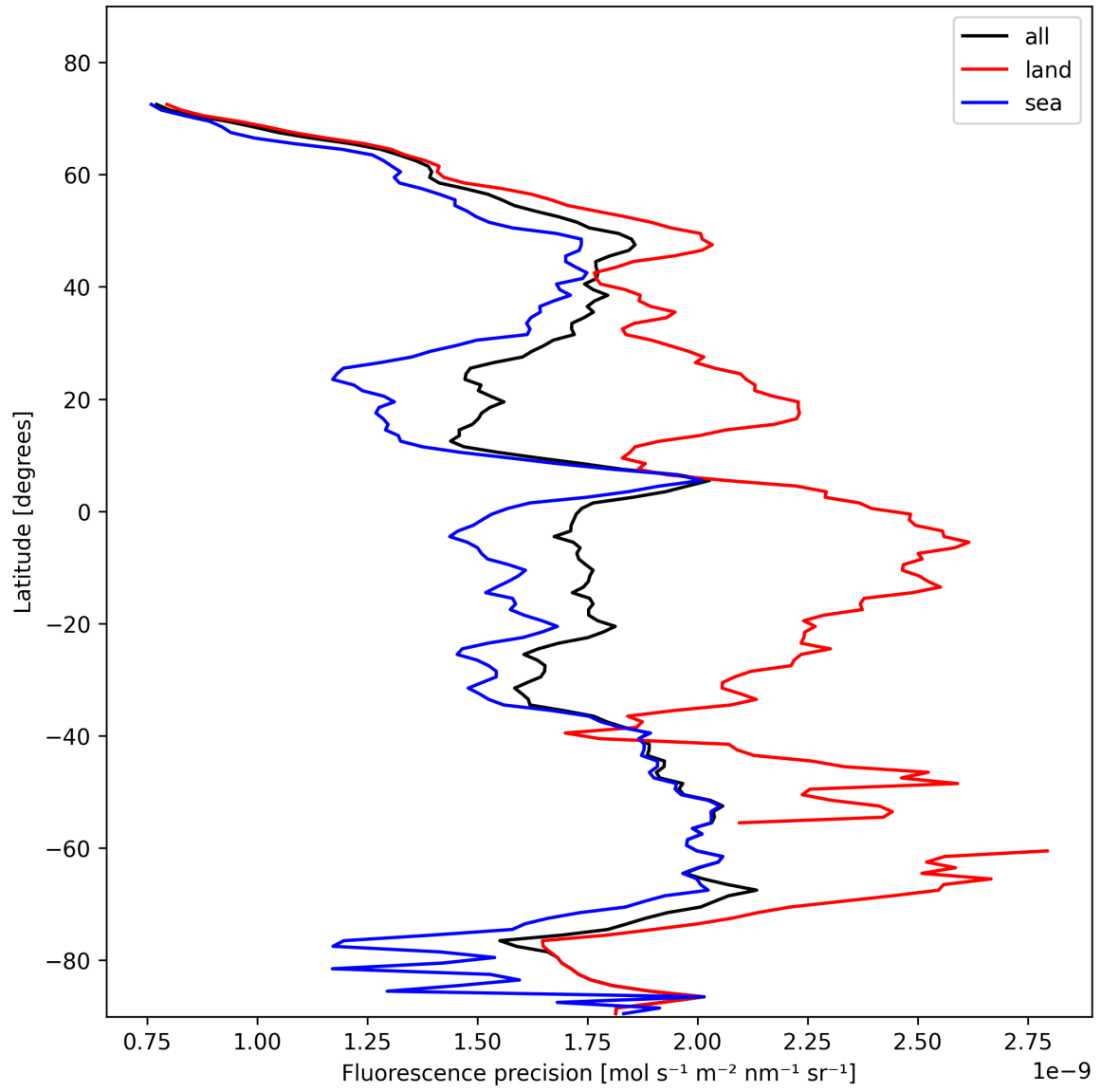
Figure 24: Zonal average of “Fluorescence precision” for 2025-02-04 to 2025-02-06.
