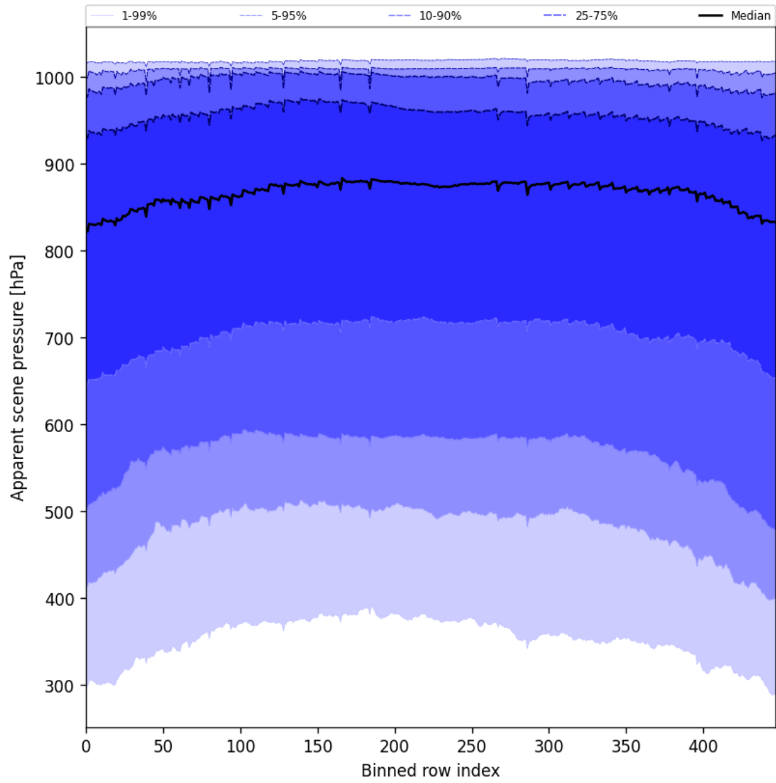
Figure 53: Along track statistics of “Apparent scene pressure” for 2025-02-04 to 2025-02-06
