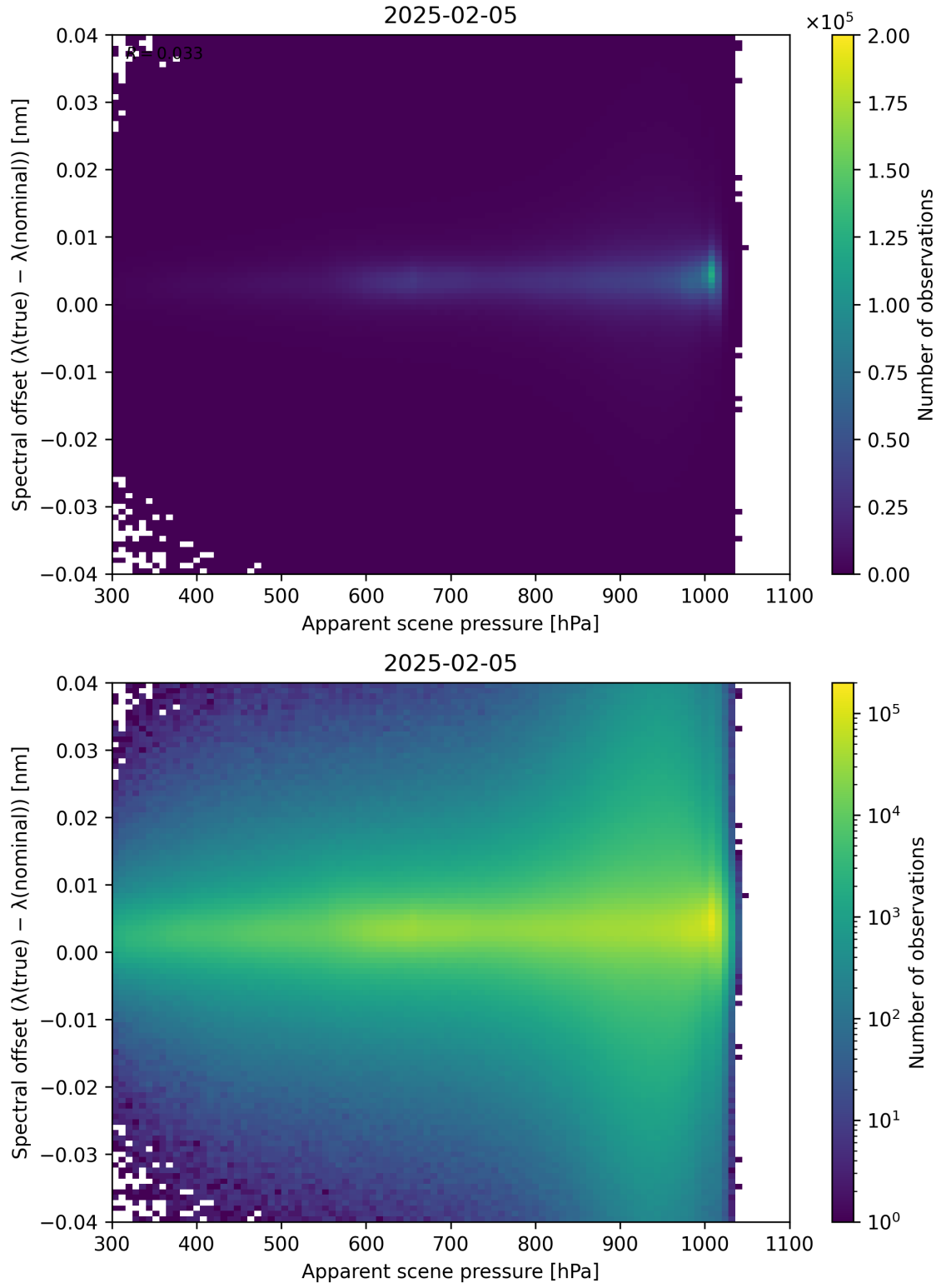
Figure 67: Scatter density plot of “Apparent scene pressure” against “Spectral offset ( \lambda_{\text{true}} - \lambda_{\text{nominal}} )” for 2025-02-04 to 2025-02-06.
