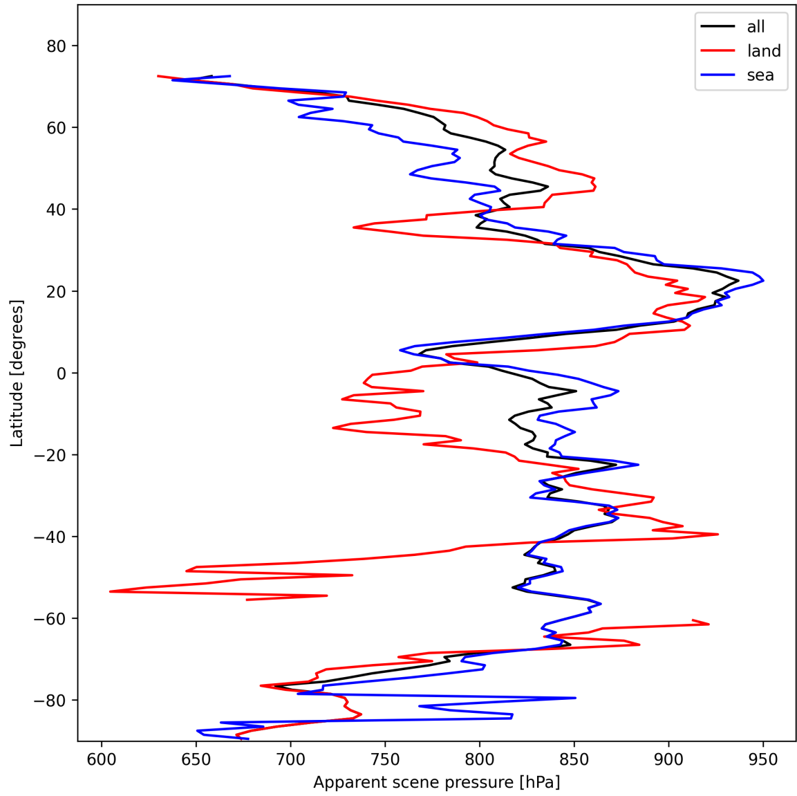
Figure 19: Zonal average of “Apparent scene pressure” for 2025-02-04 to 2025-02-06.
