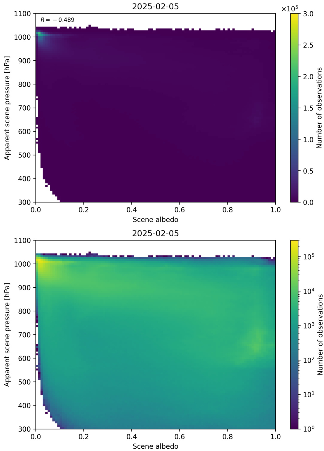
Figure 102: Scatter density plot of “Scene albedo” against “Apparent scene pressure” for 2025-02-04 to 2025-02-06.
