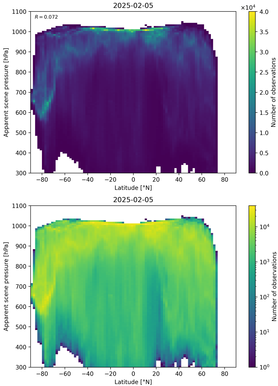
Figure 88: Scatter density plot of “Latitude” against “Apparent scene pressure” for 2025-02-04 to 2025-02-06.
