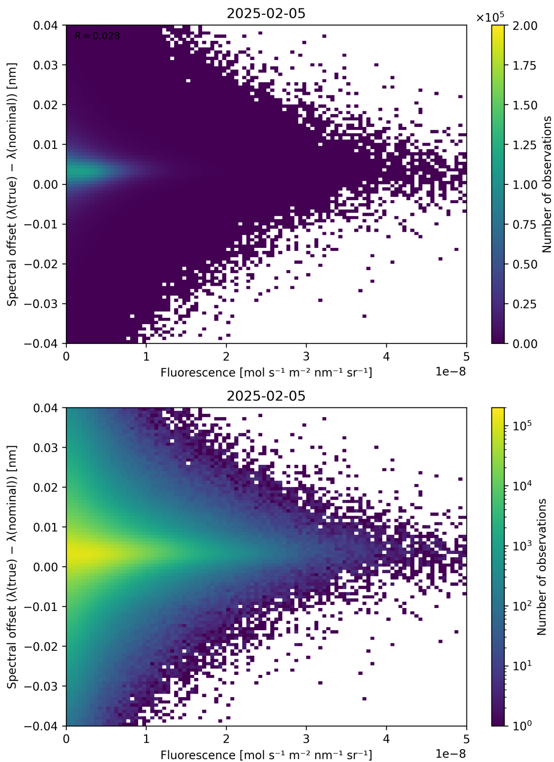
Figure 87: Scatter density plot of “Fluorescence” against “Spectral offset ( \lambda_{\text{true}} - \lambda_{\text{nominal}} )” for 2025-02-04 to 2025-02-06.
