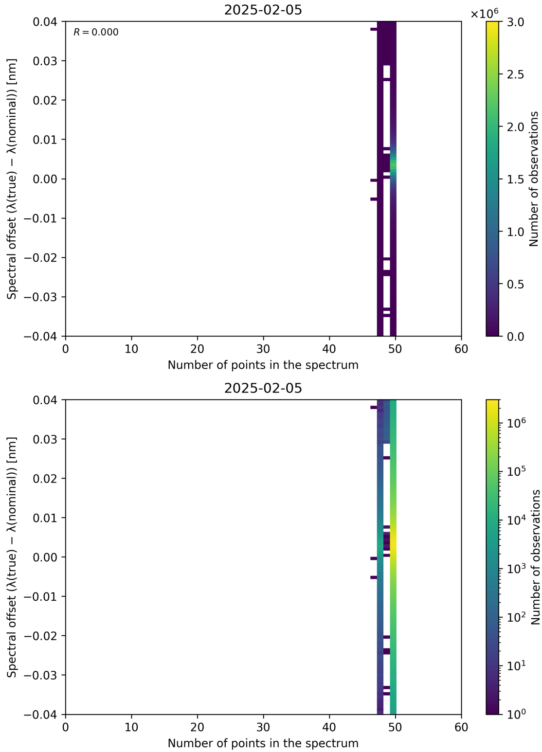
Figure 101: Scatter density plot of “Number of points in the spectrum” against “Spectral offset ( \lambda_{\text{true}} - \lambda_{\text{nominal}} )” for 2025-02-04 to 2025-02-06.
