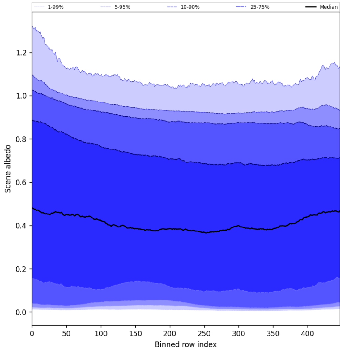
Figure 51: Along track statistics of “Scene albedo” for 2025-02-04 to 2025-02-06
