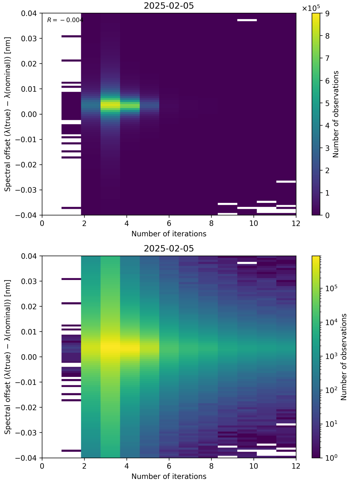
Figure 100: Scatter density plot of “Number of iterations” against “Spectral offset ( \lambda_{\text{true}} - \lambda_{\text{nominal}} )” for 2025-02-04 to 2025-02-06.
