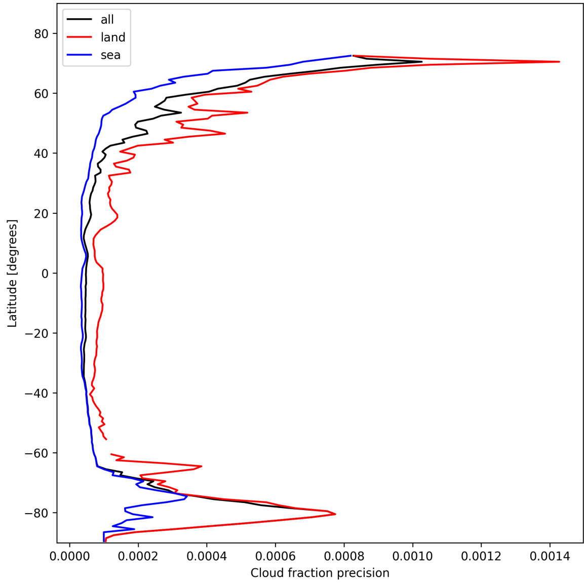
Figure 16: Zonal average of “Cloud fraction precision” for 2025-02-04 to 2025-02-06.
