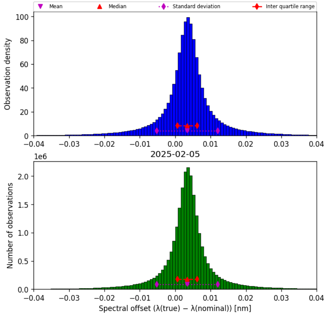
Figure 45: Histogram of “Spectral offset ( \lambda_{\text{true}} - \lambda_{\text{nominal}} )” for 2025-02-04 to 2025-02-06
