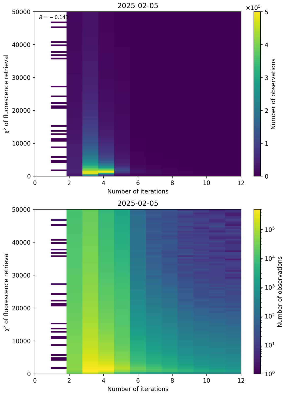
Figure 97: Scatter density plot of “Number of iterations” against “ \chi^2 of fluorescence retrieval” for 2025-02-04 to 2025-02-06.
