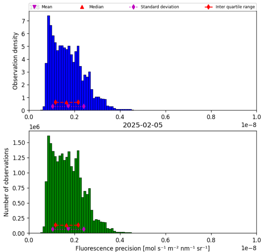
Figure 41: Histogram of “Fluorescence precision” for 2025-02-04 to 2025-02-06
