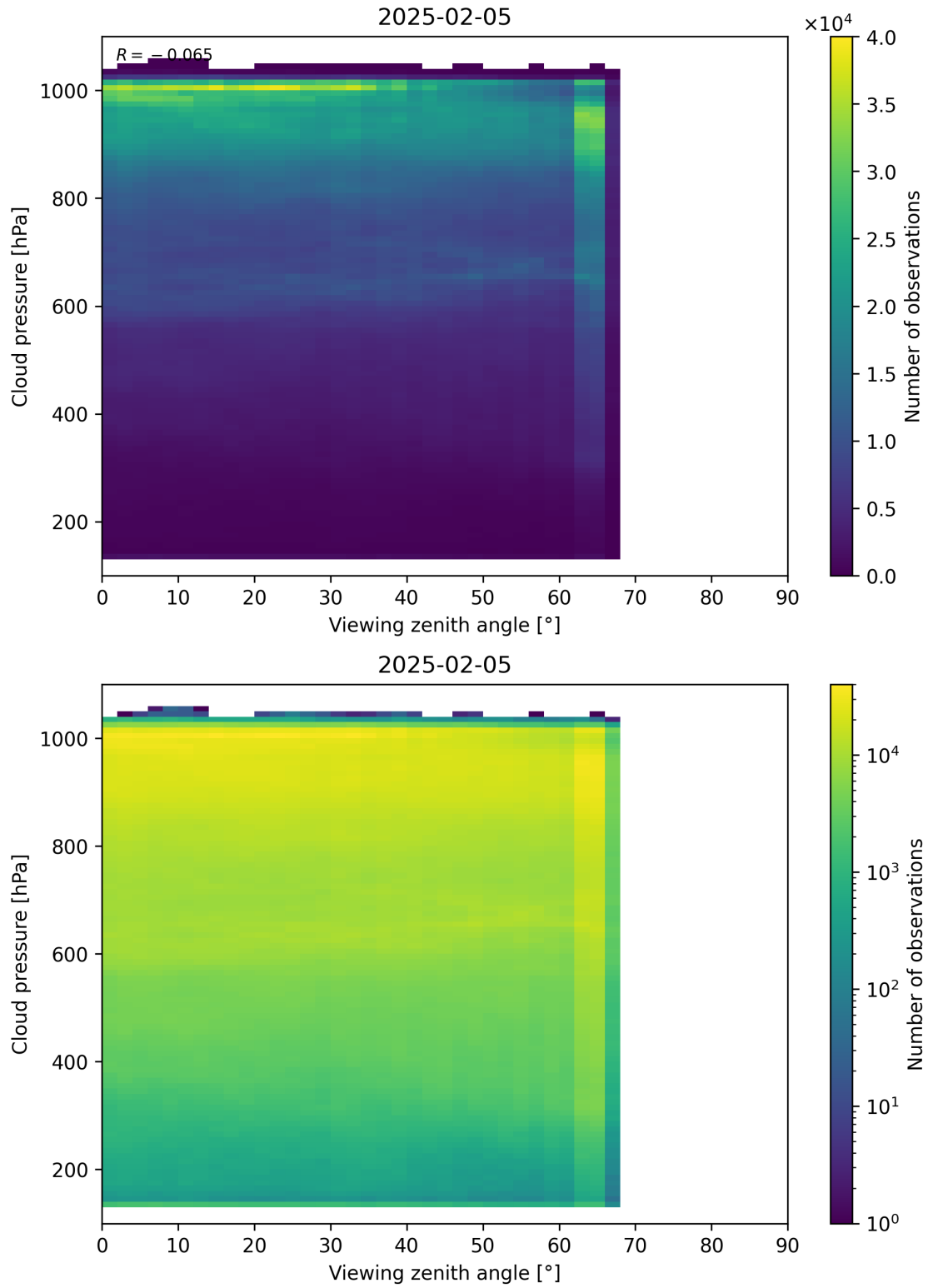
Figure 121: Scatter density plot of “Viewing zenith angle” against “Cloud pressure” for 2025-02-04 to 2025-02-06.
