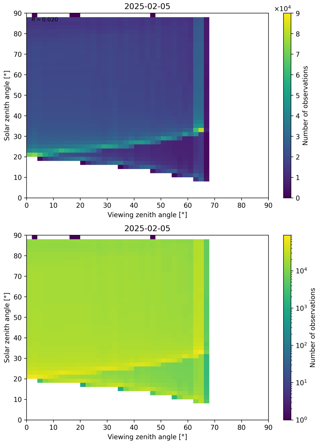
Figure 127: Scatter density plot of “Viewing zenith angle” against “Solar zenith angle” for 2025-02-04 to 2025-02-06.
