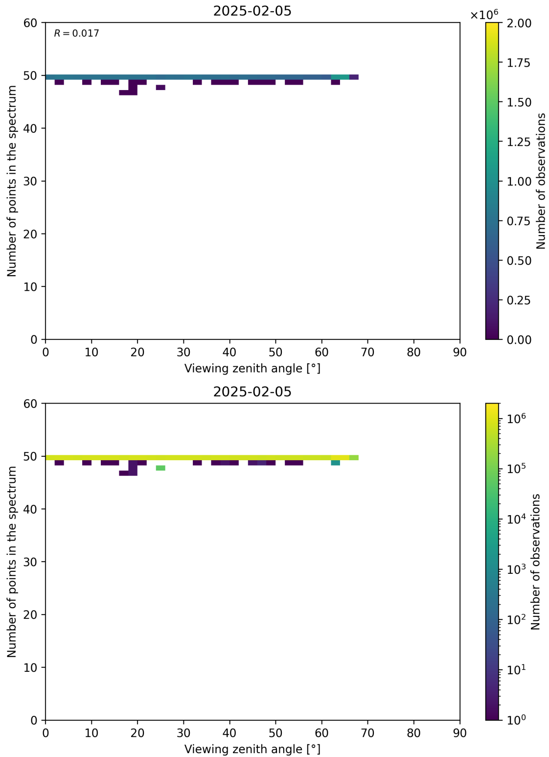
Figure 125: Scatter density plot of “Viewing zenith angle” against “Number of points in the spectrum” for 2025-02-04 to 2025-02-06.
