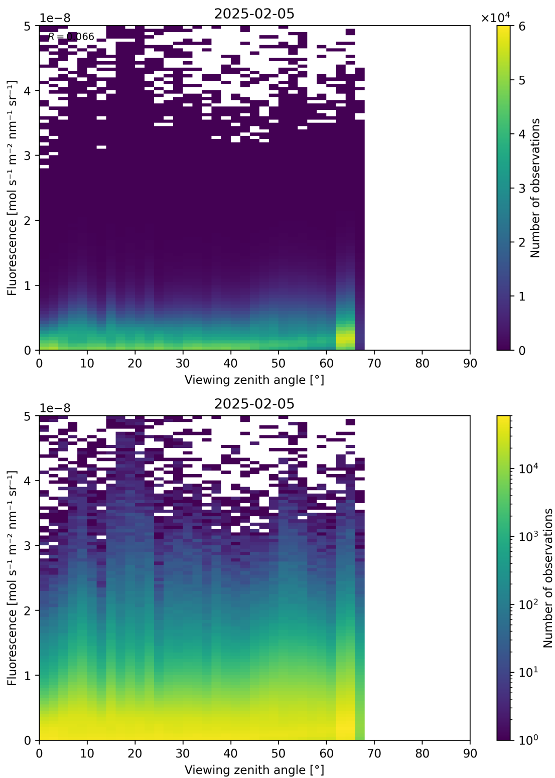
Figure 122: Scatter density plot of "Viewing zenith angle" against "Fluorescence" for 2025-02-04 to 2025-02-06.
