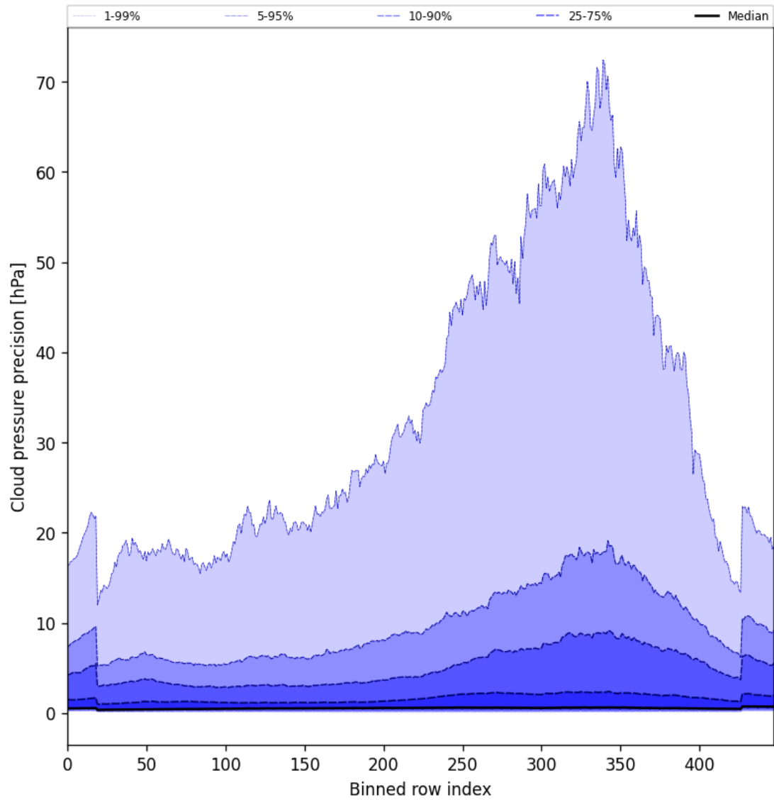
Figure 48: Along track statistics of “Cloud pressure precision” for 2025-02-04 to 2025-02-06
