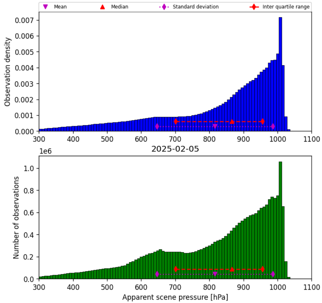
Figure 36: Histogram of “Apparent scene pressure” for 2025-02-04 to 2025-02-06
