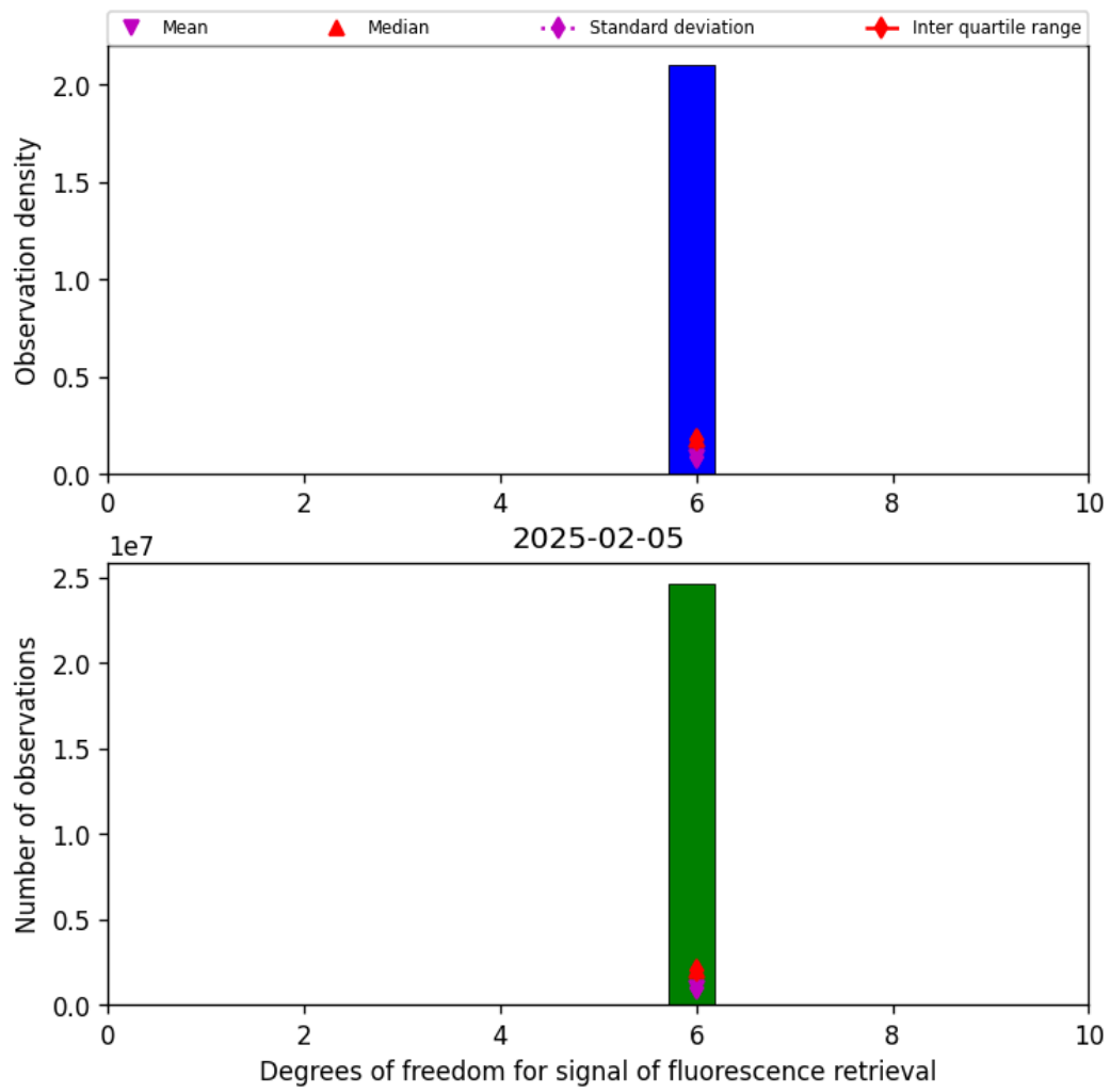
Figure 43: Histogram of "Degrees of freedom for signal of fluorescence retrieval" for 2025-02-04 to 2025-02-06
