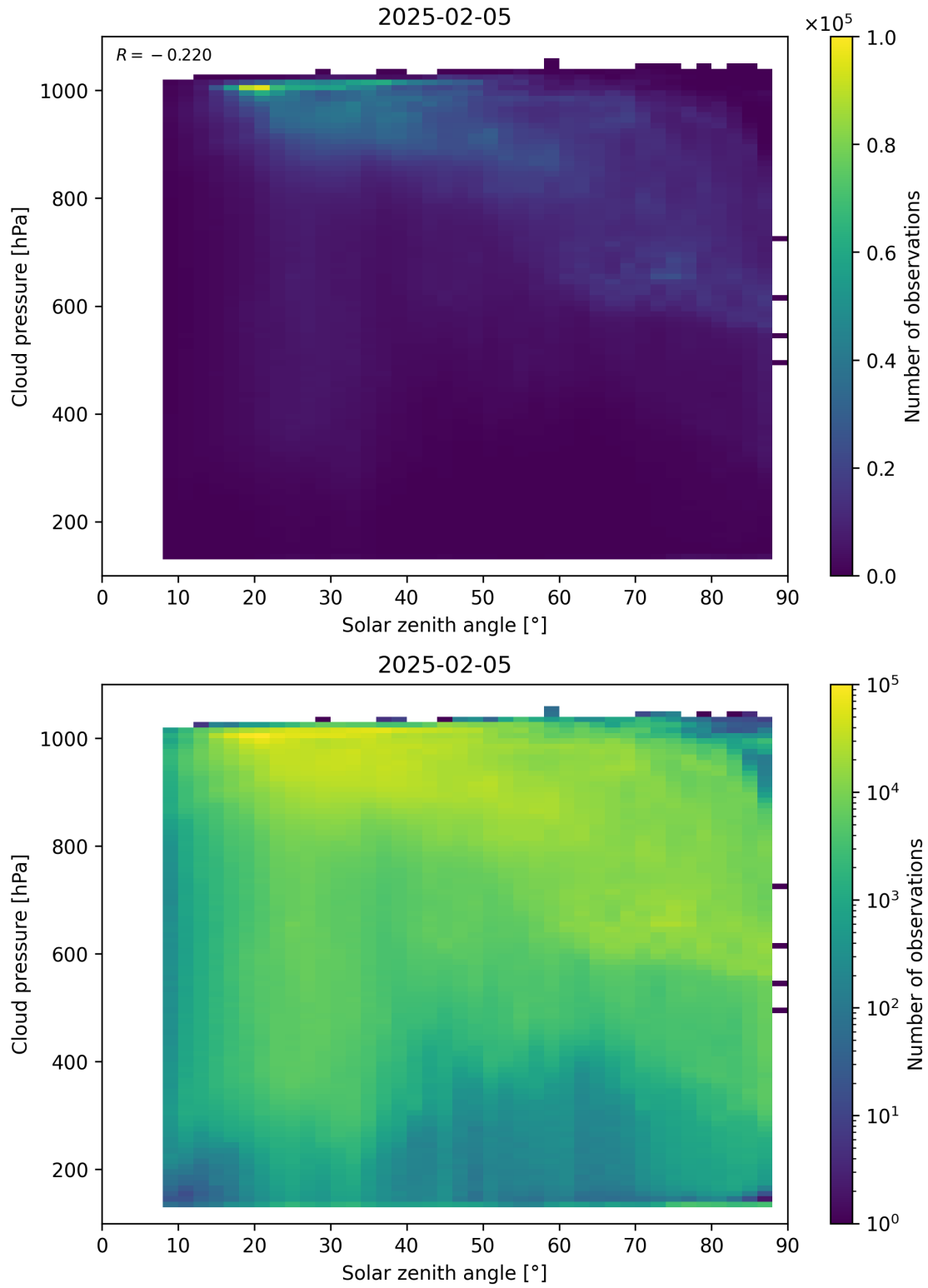
Figure 111: Scatter density plot of “Solar zenith angle” against “Cloud pressure” for 2025-02-04 to 2025-02-06.
