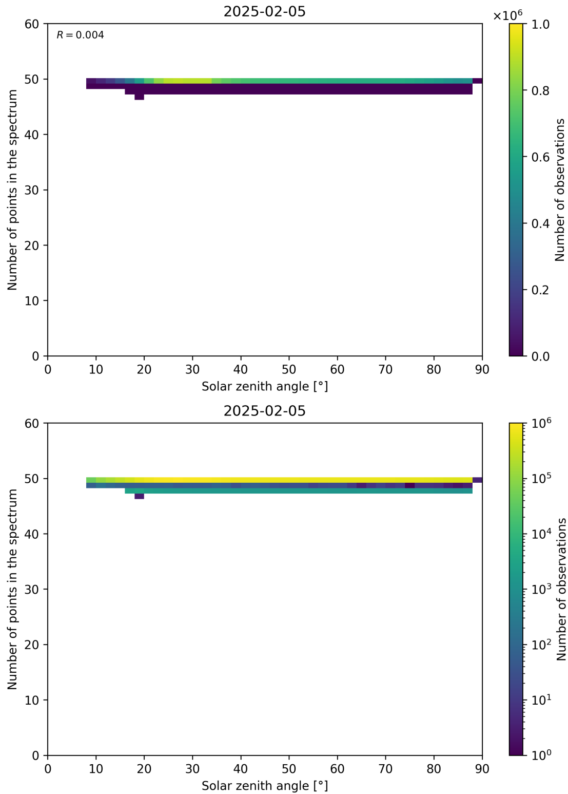
Figure 115: Scatter density plot of “Solar zenith angle” against “Number of points in the spectrum” for 2025-02-04 to 2025-02-06.
