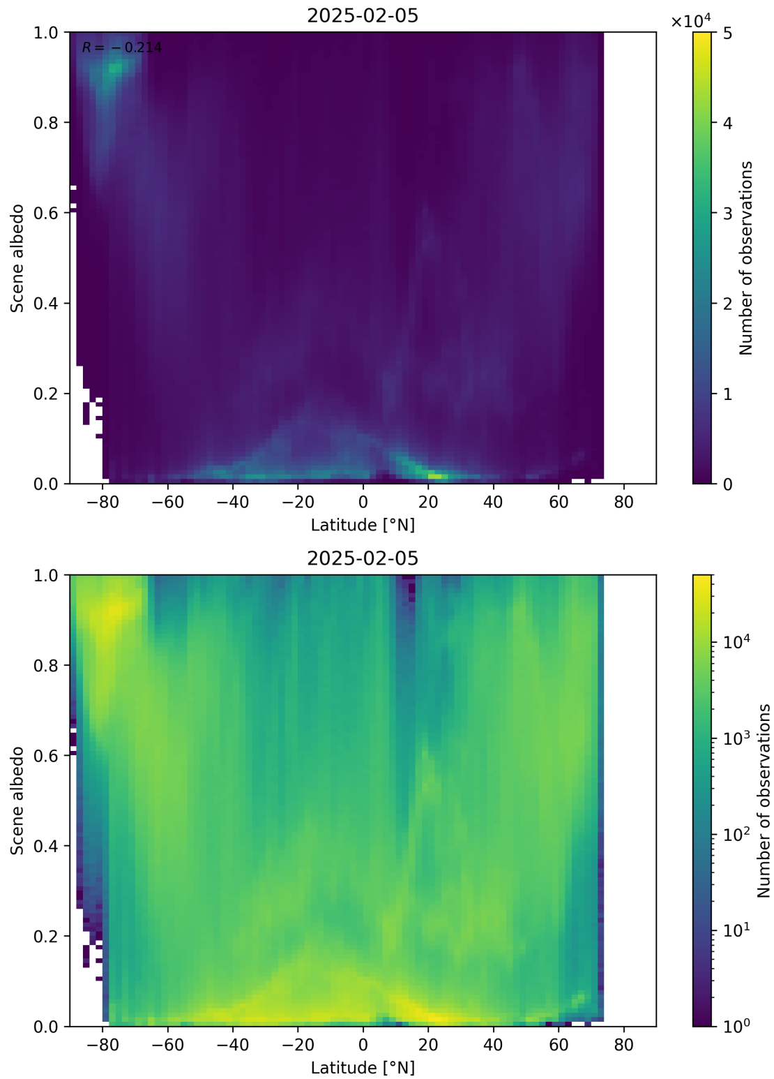
Figure 95: Scatter density plot of “Latitude” against “Scene albedo” for 2025-02-04 to 2025-02-06.
