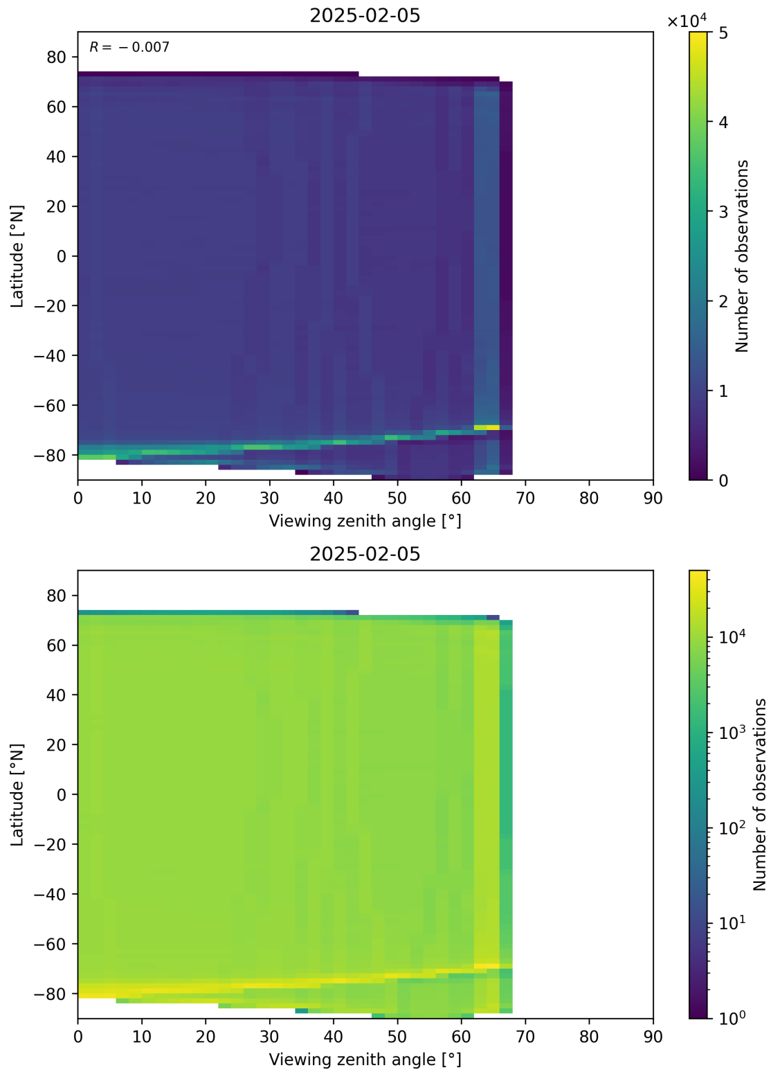
Figure 123: Scatter density plot of “Viewing zenith angle” against “Latitude” for 2025-02-04 to 2025-02-06.
