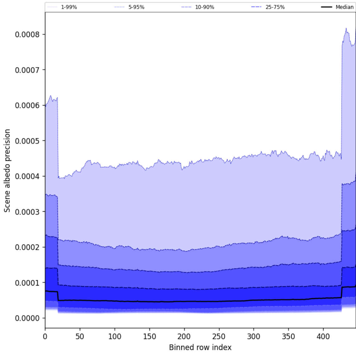
Figure 52: Along track statistics of “Scene albedo precision” for 2025-02-04 to 2025-02-06
