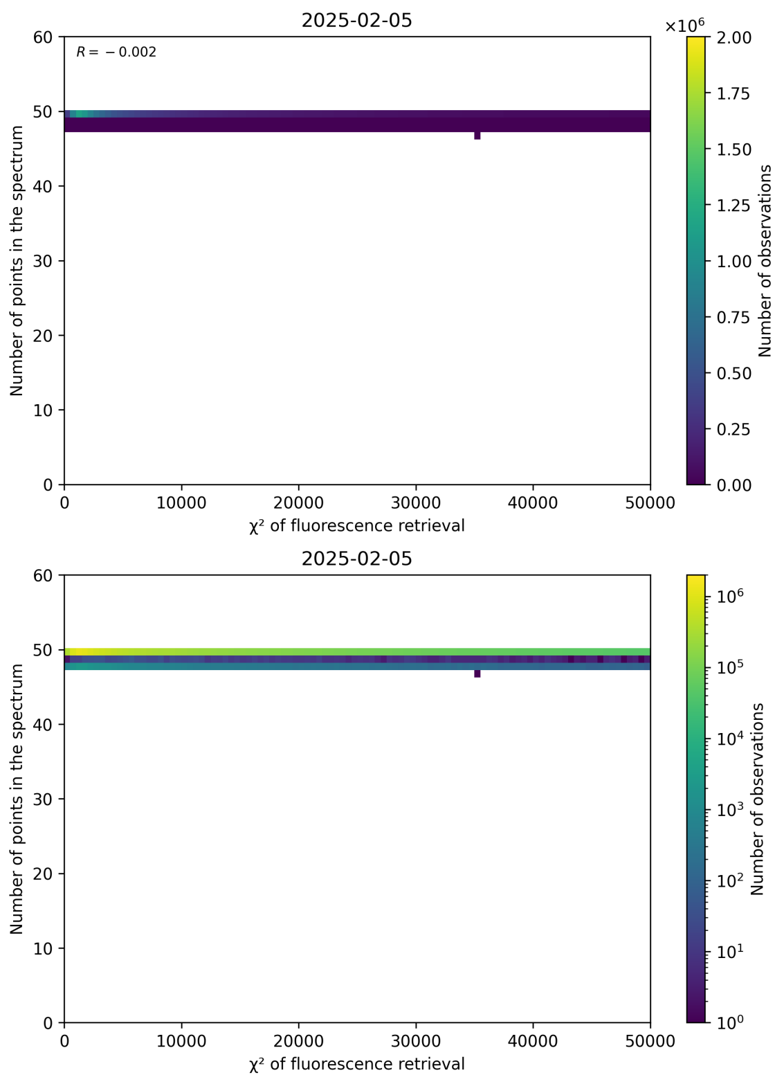
Figure 68: Scatter density plot of " \chi^2 of fluorescence retrieval" against "Number of points in the spectrum" for 2025-02-04 to 2025-02-06.
