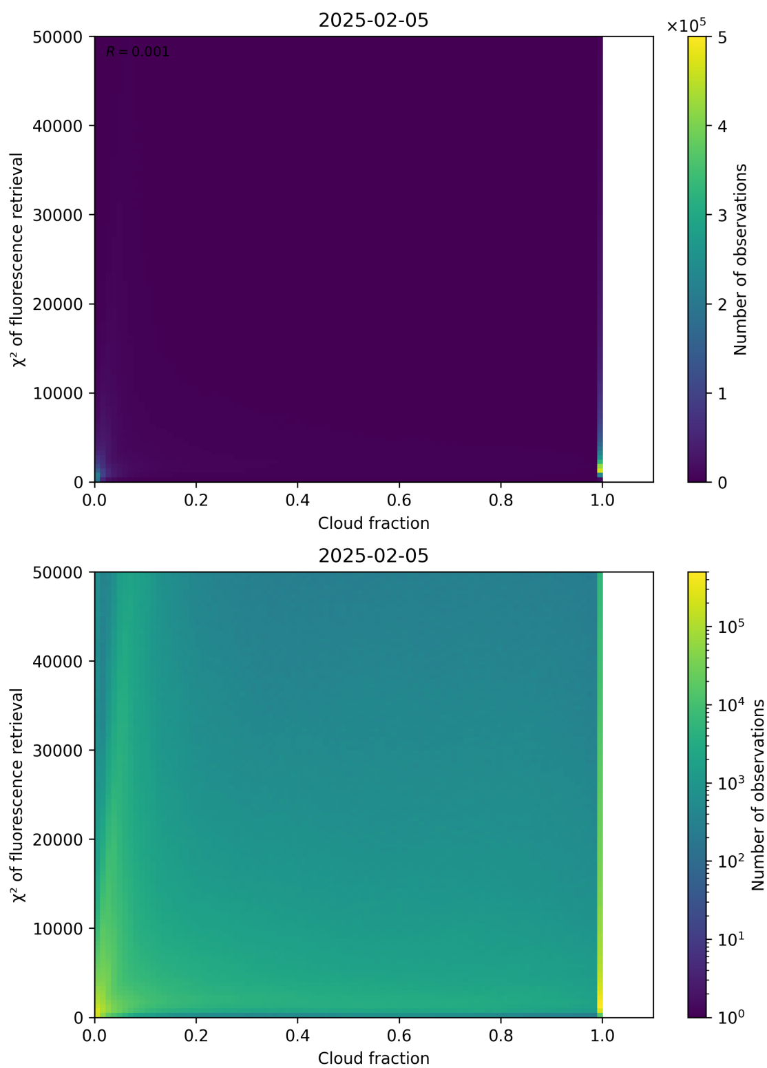
Figure 71: Scatter density plot of “Cloud fraction” against “ \chi^2 of fluorescence retrieval” for 2025-02-04 to 2025-02-06.
