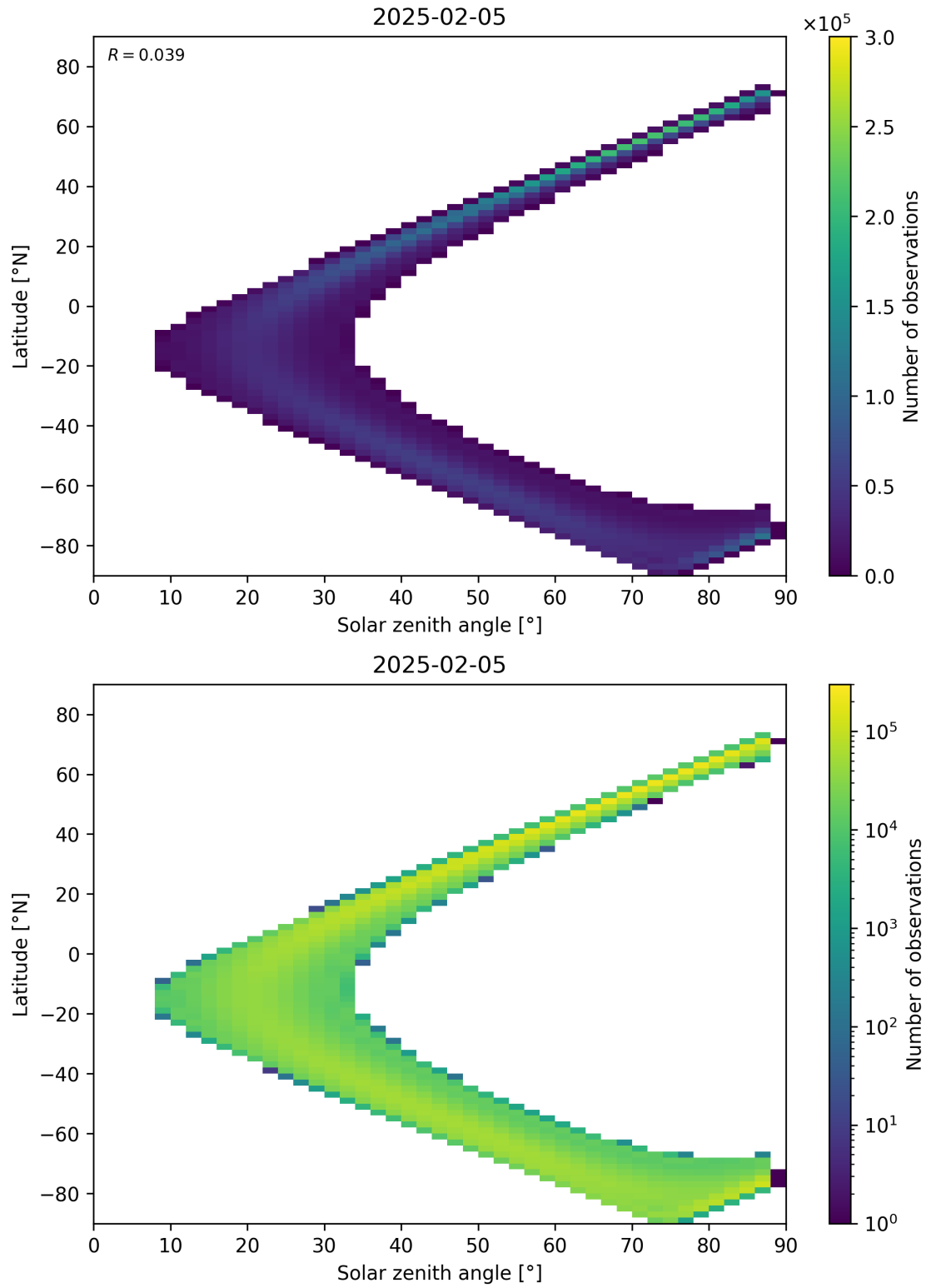
Figure 113: Scatter density plot of “Solar zenith angle” against “Latitude” for 2025-02-04 to 2025-02-06.
