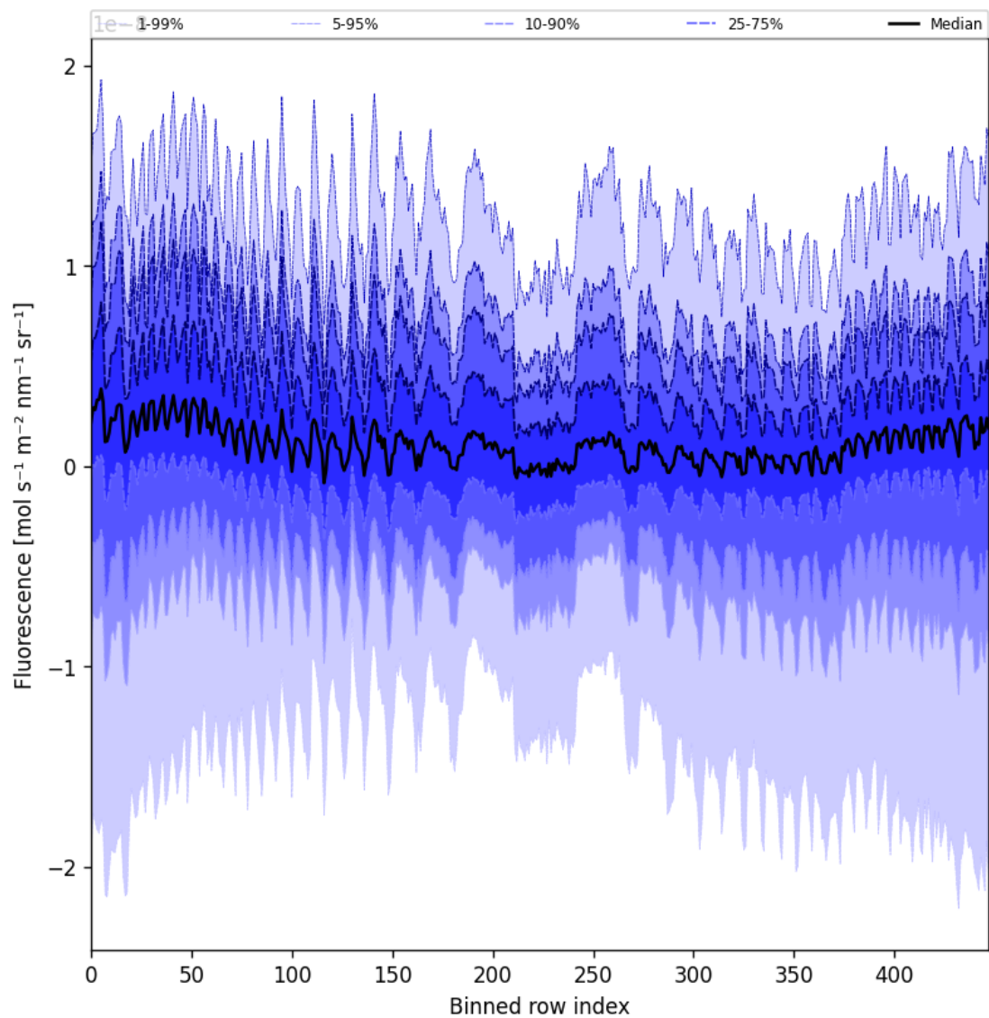
Figure 57: Along track statistics of “Fluorescence” for 2025-02-04 to 2025-02-06
