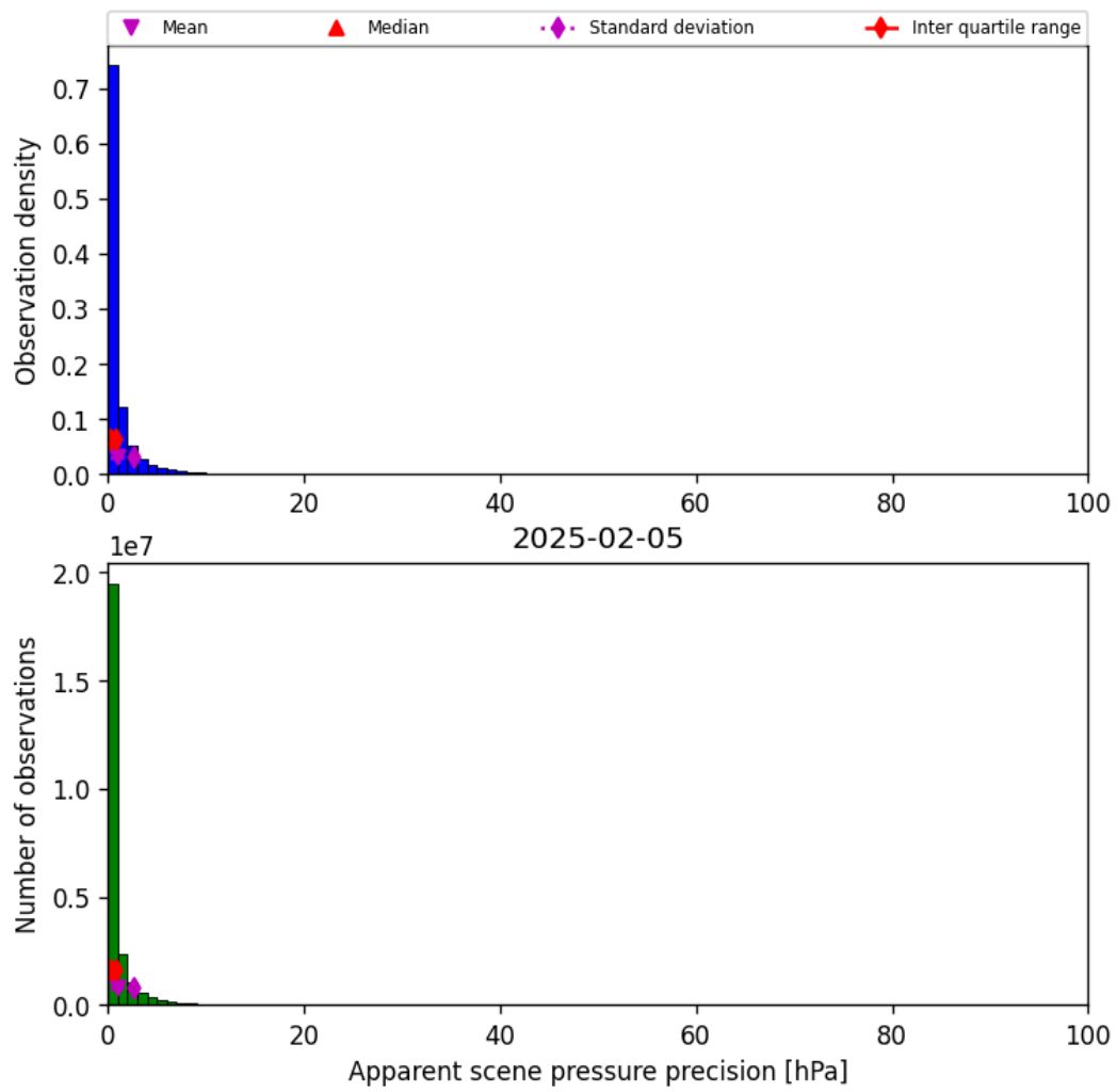
Figure 37: Histogram of “Apparent scene pressure precision” for 2025-02-04 to 2025-02-06
