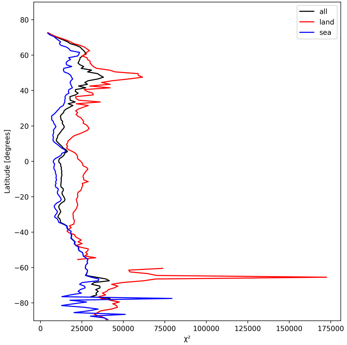
Figure 21: Zonal average of “ \chi^2 ” for 2025-02-04 to 2025-02-06.
