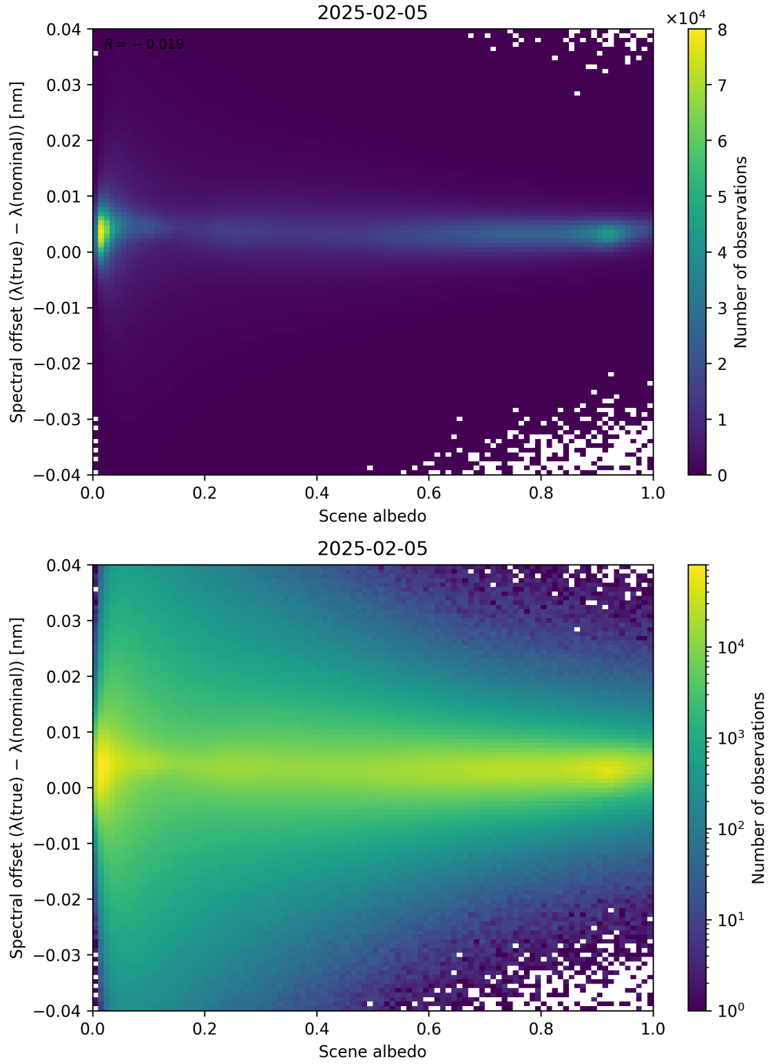
Figure 107: Scatter density plot of “Scene albedo” against “Spectral offset ( \lambda_{\text{true}} - \lambda_{\text{nominal}} )” for 2025-02-04 to 2025-02-06.
