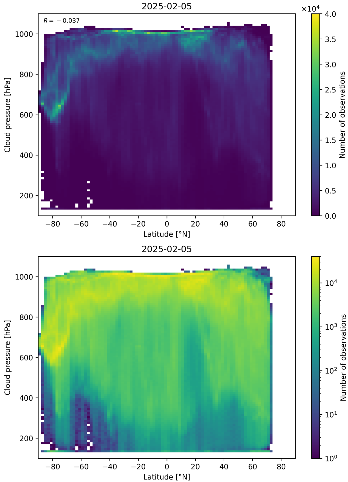
Figure 91: Scatter density plot of “Latitude” against “Cloud pressure” for 2025-02-04 to 2025-02-06.
