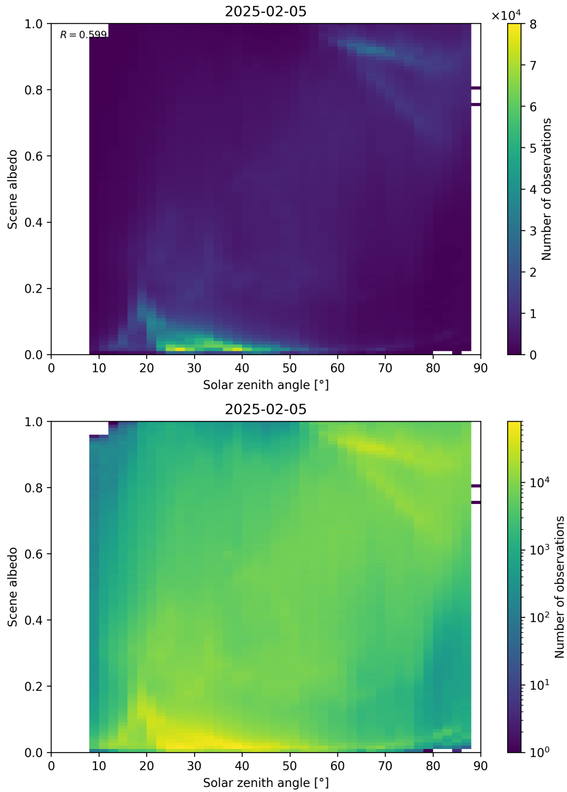
Figure 116: Scatter density plot of “Solar zenith angle” against “Scene albedo” for 2025-02-04 to 2025-02-06.
