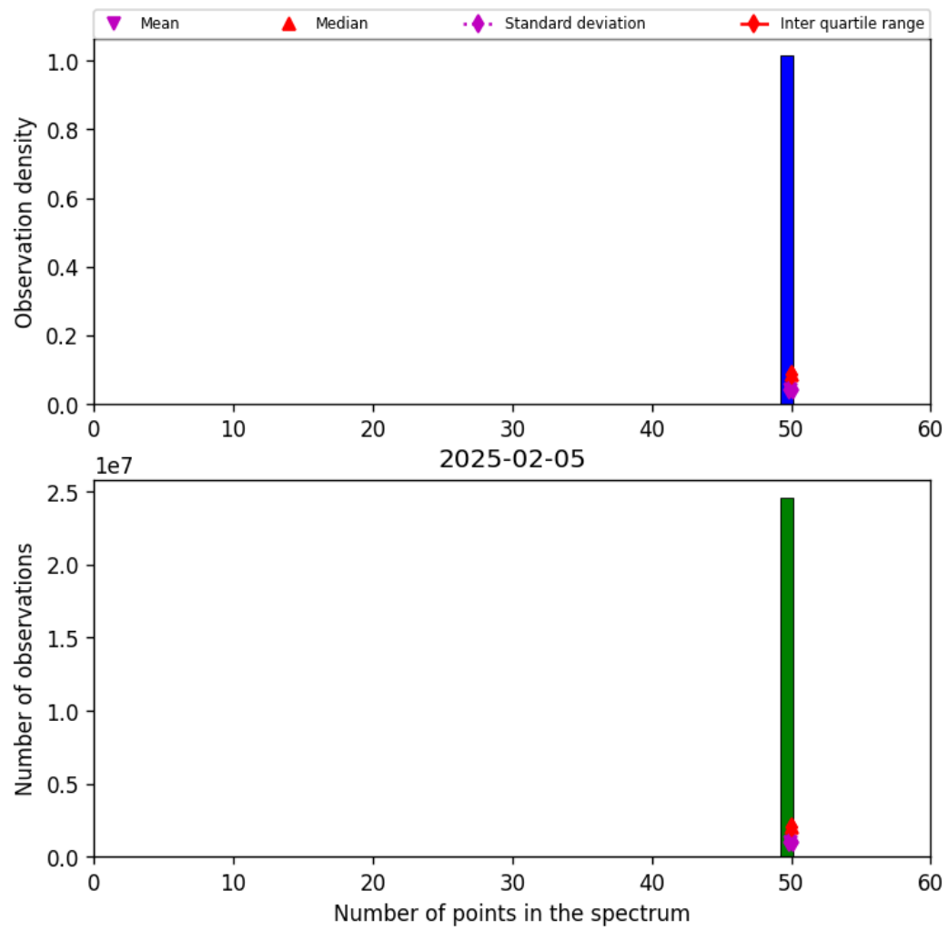
Figure 44: Histogram of “Number of points in the spectrum” for 2025-02-04 to 2025-02-06
