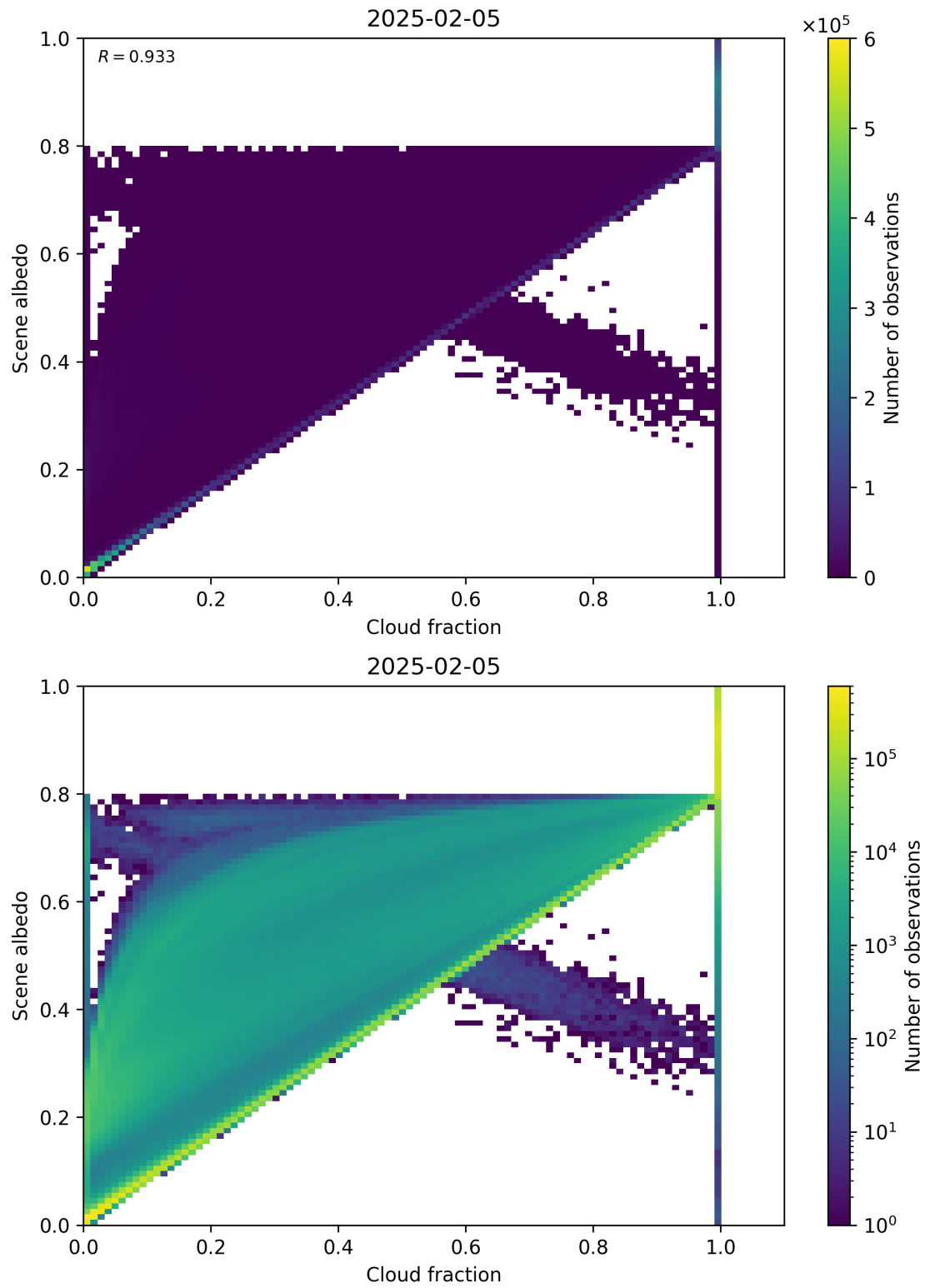
Figure 75: Scatter density plot of “Cloud fraction” against “Scene albedo” for 2025-02-04 to 2025-02-06.
