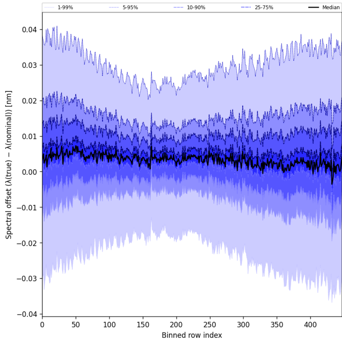
Figure 62: Along track statistics of “Spectral offset ( \lambda_{\text{true}} - \lambda_{\text{nominal}} )” for 2025-02-04 to 2025-02-06
