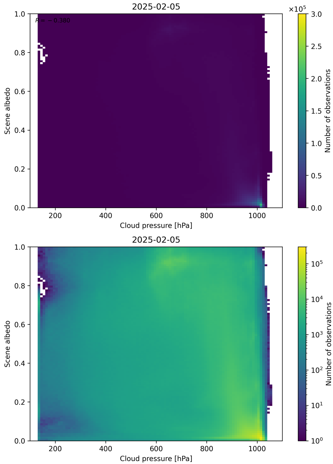
Figure 83: Scatter density plot of “Cloud pressure” against “Scene albedo” for 2025-02-04 to 2025-02-06.
