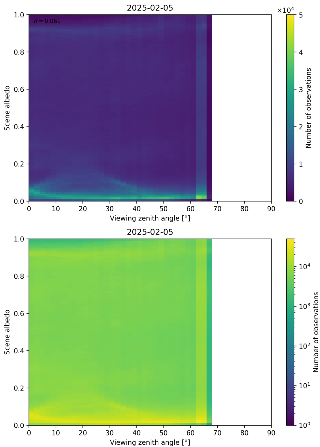
Figure 126: Scatter density plot of “Viewing zenith angle” against “Scene albedo” for 2025-02-04 to 2025-02-06.
