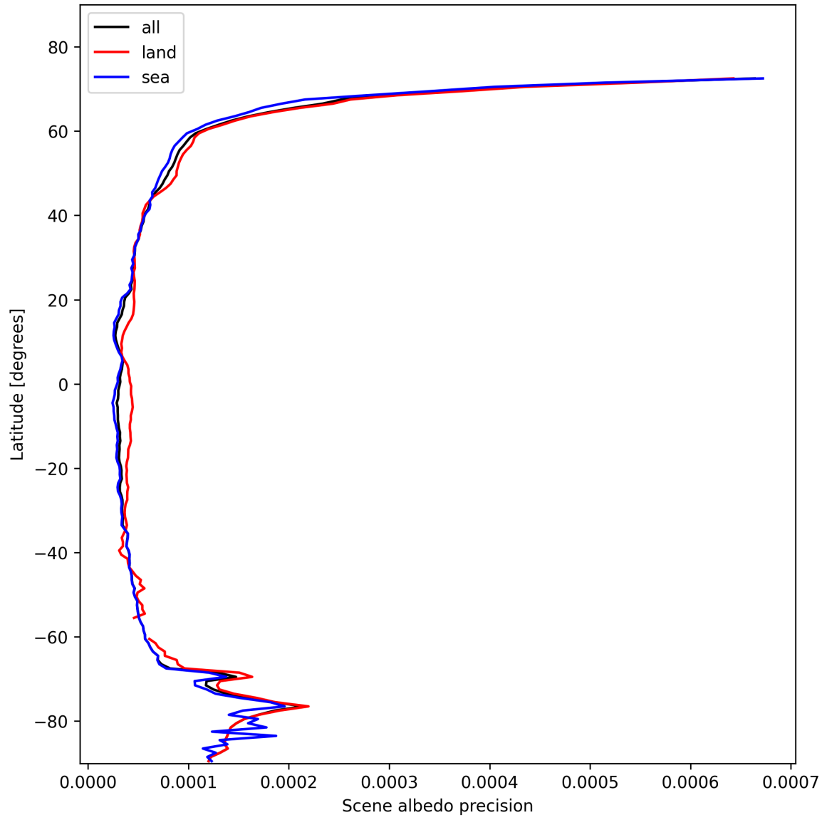
Figure 18: Zonal average of “Scene albedo precision” for 2025-02-04 to 2025-02-06.
