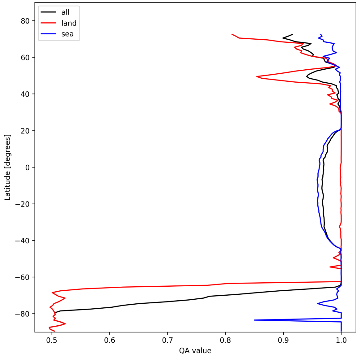
Figure 12: Zonal average of “QA value” for 2025-02-04 to 2025-02-06.
