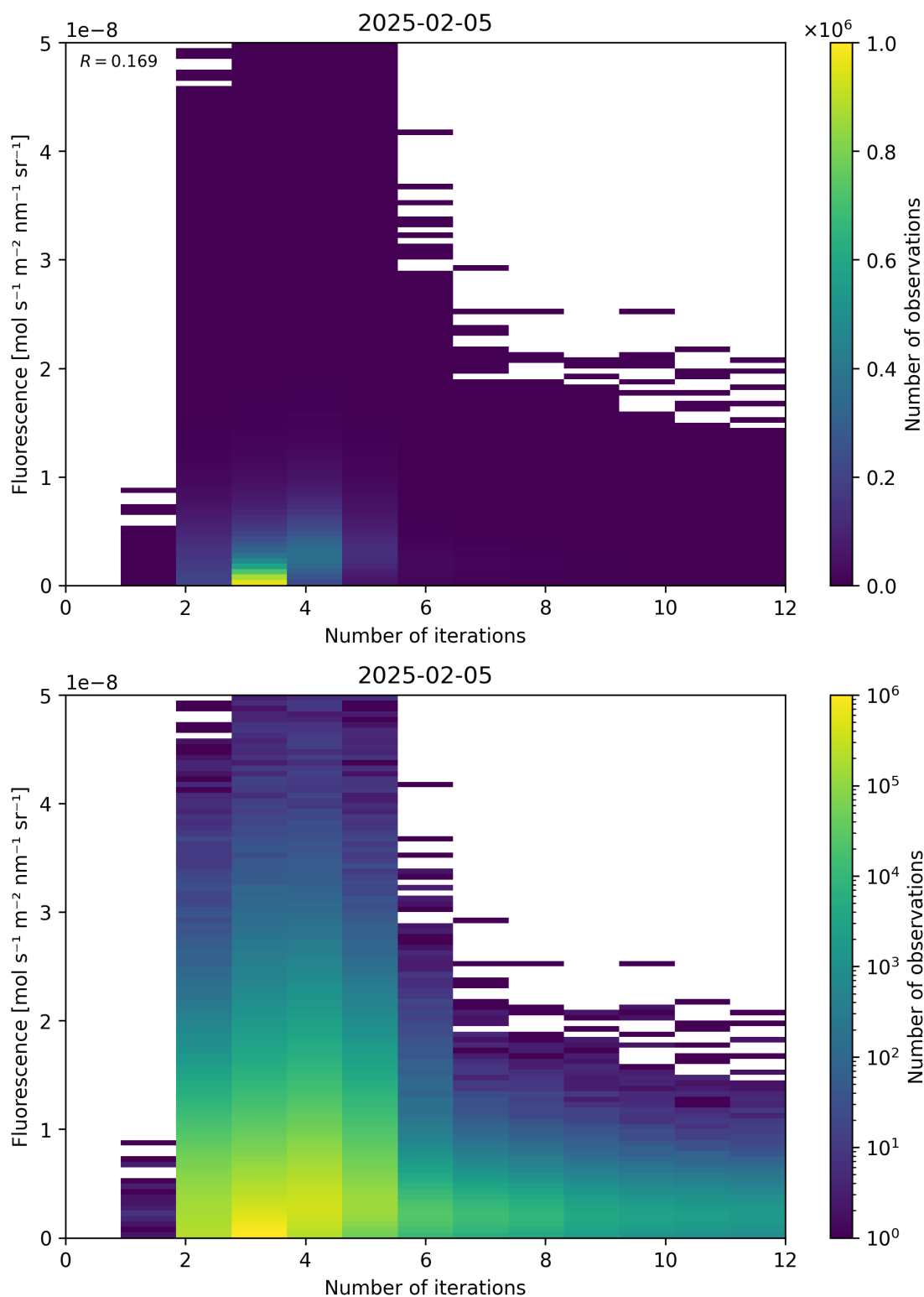
Figure 98: Scatter density plot of “Number of iterations” against “Fluorescence” for 2025-02-04 to 2025-02-06.
