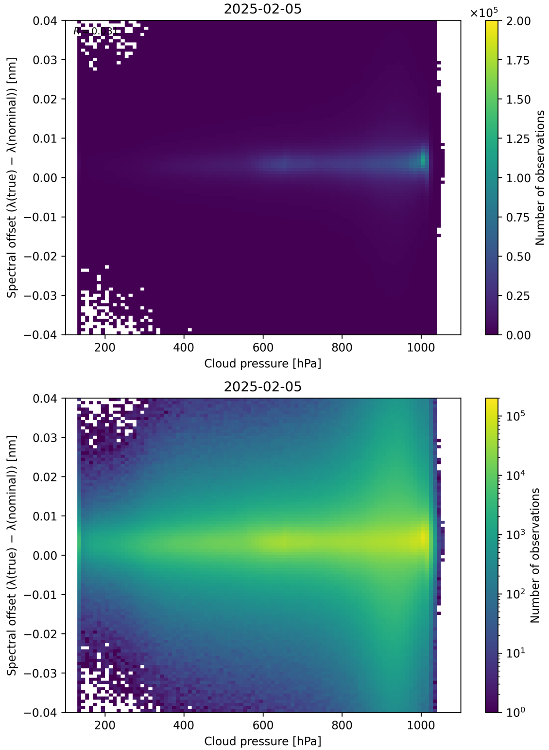
Figure 84: Scatter density plot of “Cloud pressure” against “Spectral offset ( \lambda_{\text{true}} - \lambda_{\text{nominal}} )” for 2025-02-04 to 2025-02-06.
