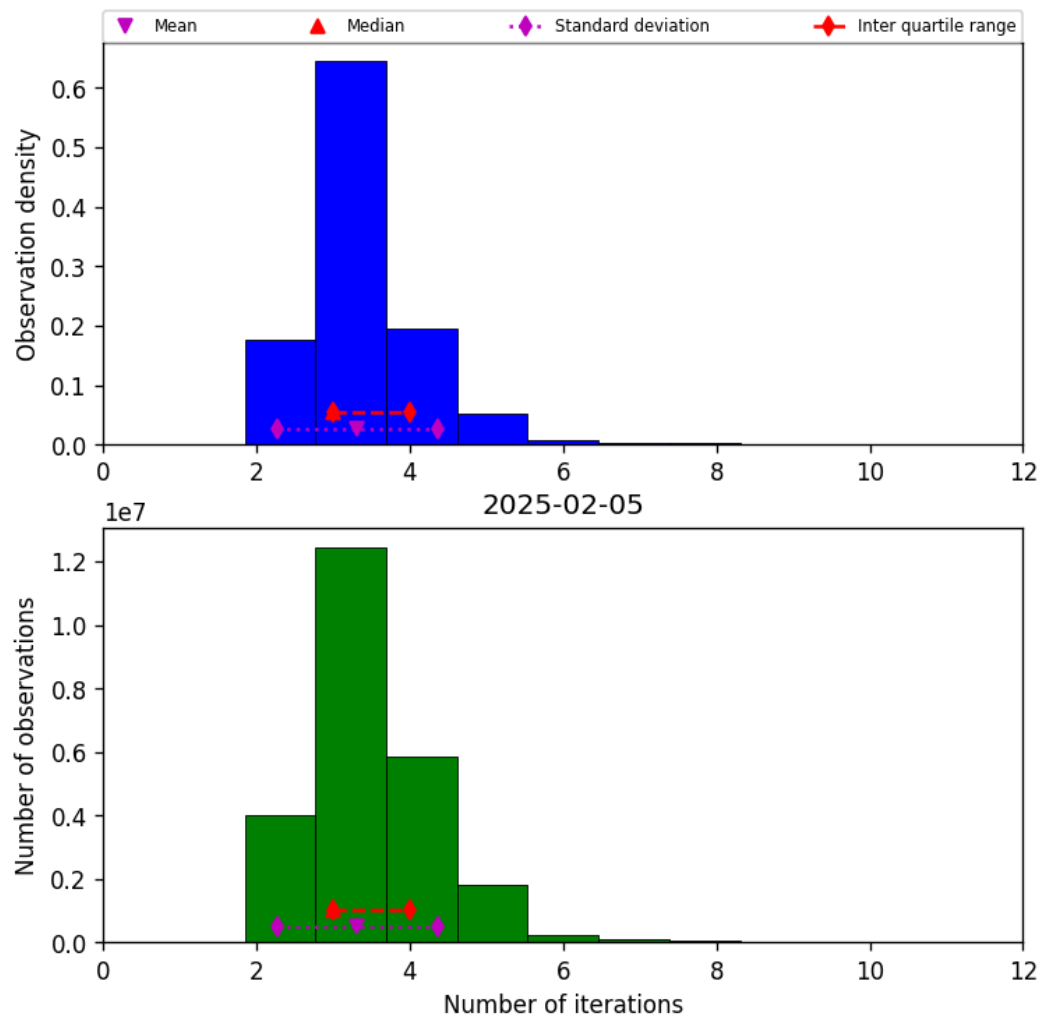
Figure 39: Histogram of “Number of iterations” for 2025-02-04 to 2025-02-06
