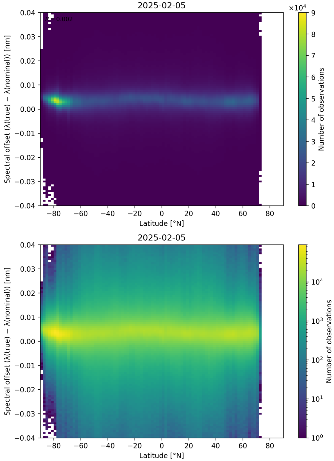
Figure 96: Scatter density plot of “Latitude” against “Spectral offset ( \lambda_{\text{true}} - \lambda_{\text{nominal}} )” for 2025-02-04 to 2025-02-06.
