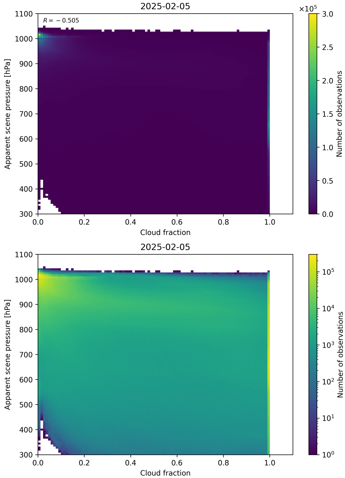
Figure 70: Scatter density plot of “Cloud fraction” against “Apparent scene pressure” for 2025-02-04 to 2025-02-06.
