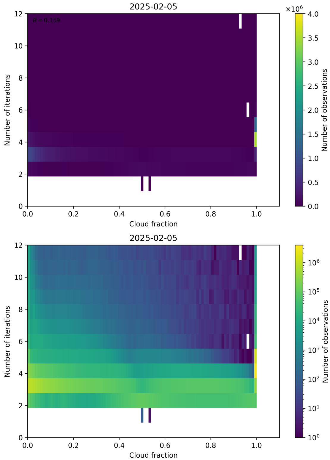
Figure 73: Scatter density plot of “Cloud fraction” against “Number of iterations” for 2025-02-04 to 2025-02-06.
