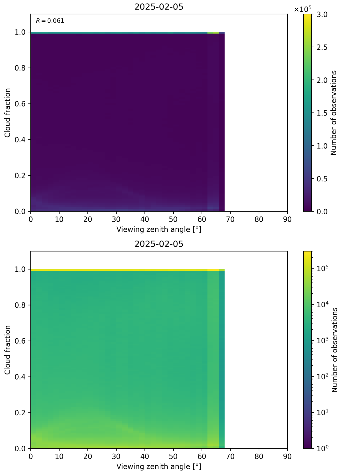
Figure 120: Scatter density plot of “Viewing zenith angle” against “Cloud fraction” for 2025-02-04 to 2025-02-06.
