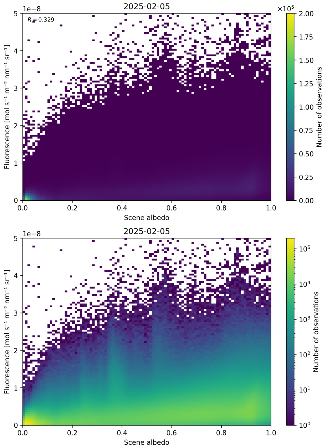
Figure 104: Scatter density plot of “Scene albedo” against “Fluorescence” for 2025-02-04 to 2025-02-06.
