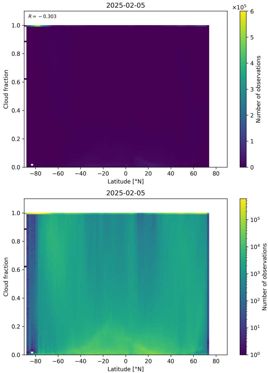
Figure 90: Scatter density plot of “Latitude” against “Cloud fraction” for 2025-02-04 to 2025-02-06.
