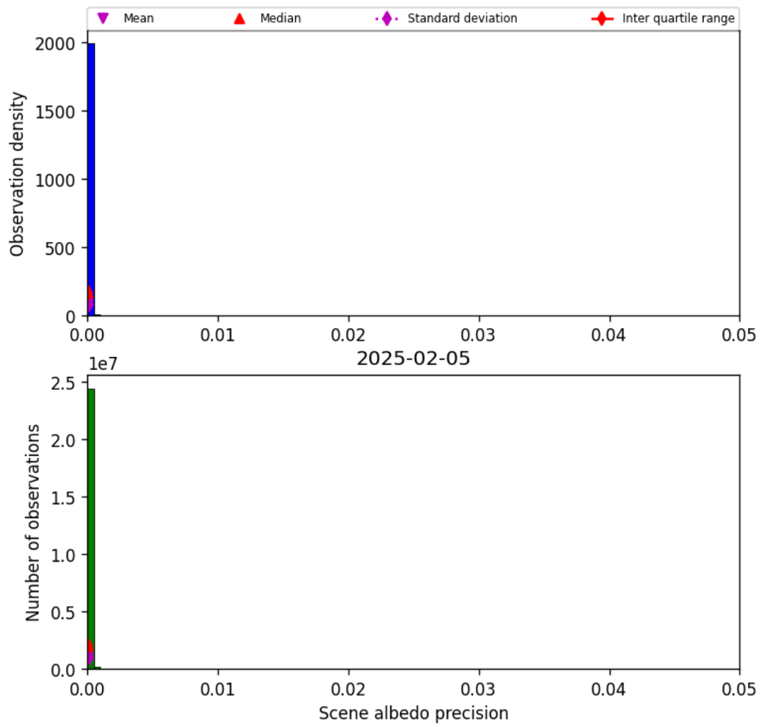
Figure 35: Histogram of “Scene albedo precision” for 2025-02-04 to 2025-02-06
