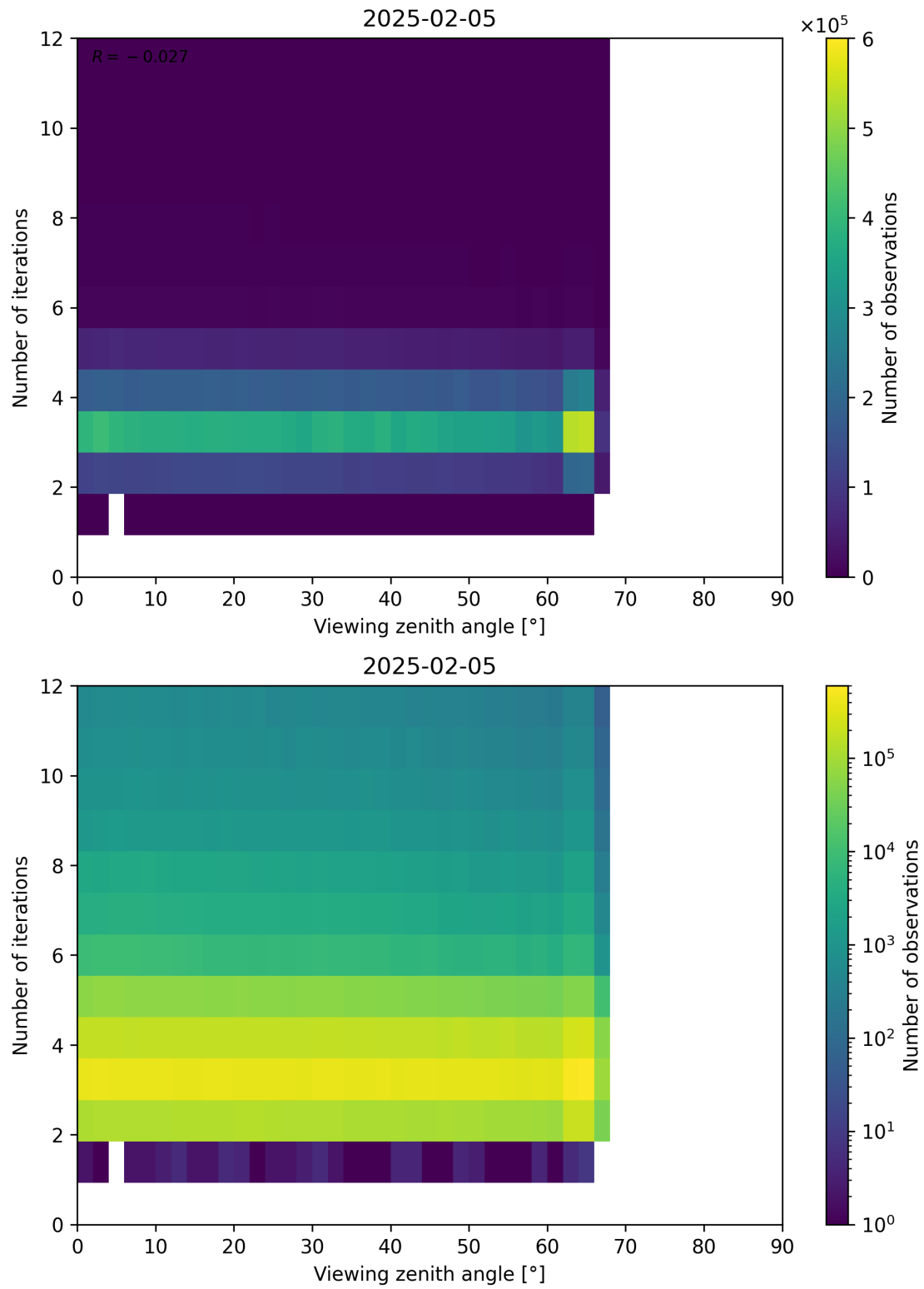
Figure 124: Scatter density plot of “Viewing zenith angle” against “Number of iterations” for 2025-02-04 to 2025-02-06.
