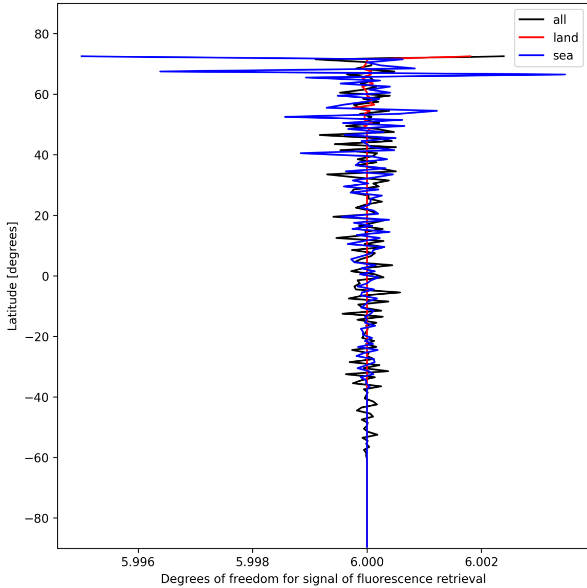
Figure 26: Zonal average of “Degrees of freedom for signal of fluorescence retrieval” for 2025-02-04 to 2025-02-06.
