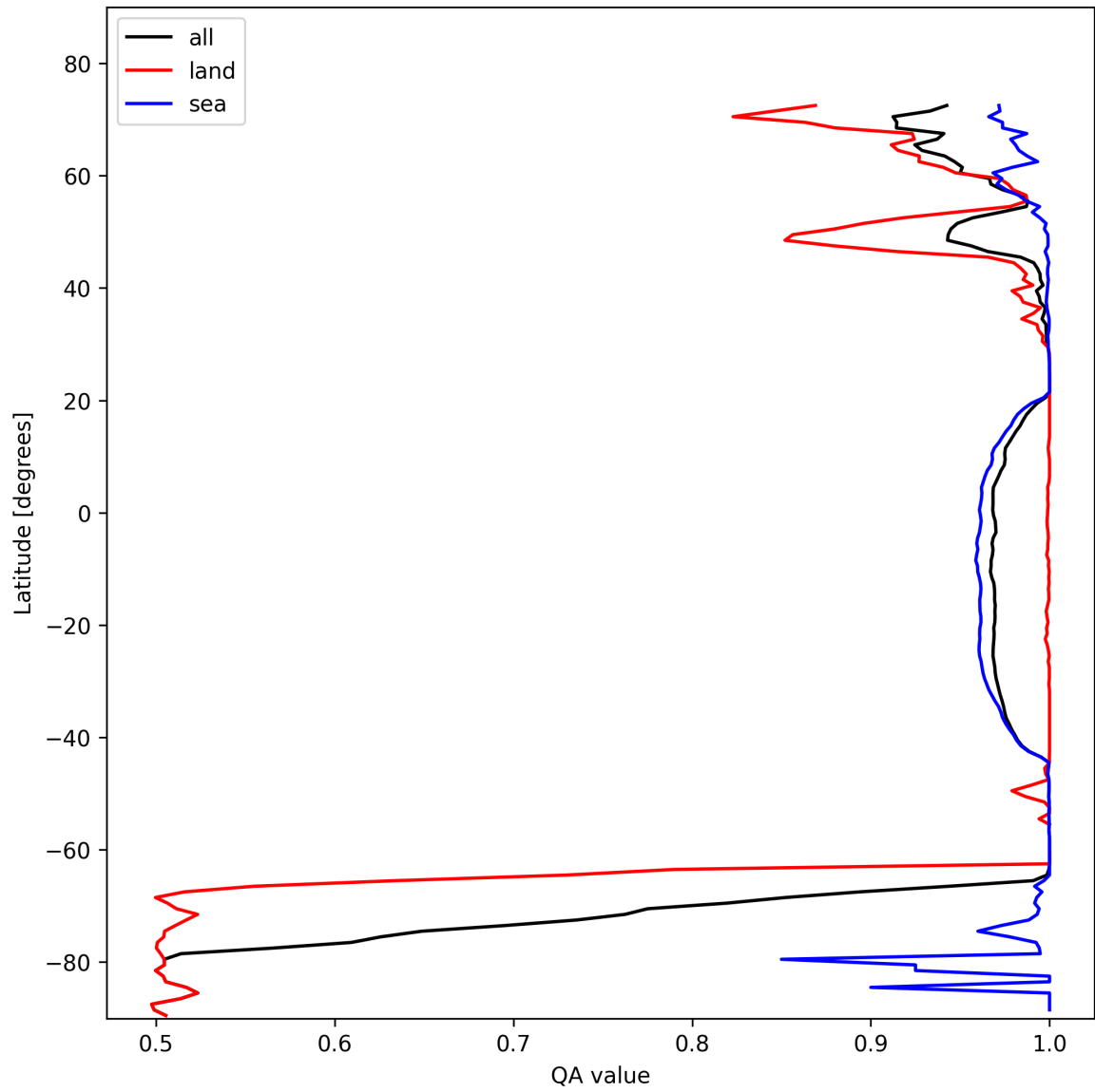
Figure 12: Zonal average of “QA value” for 2025-02-05 to 2025-02-07.
