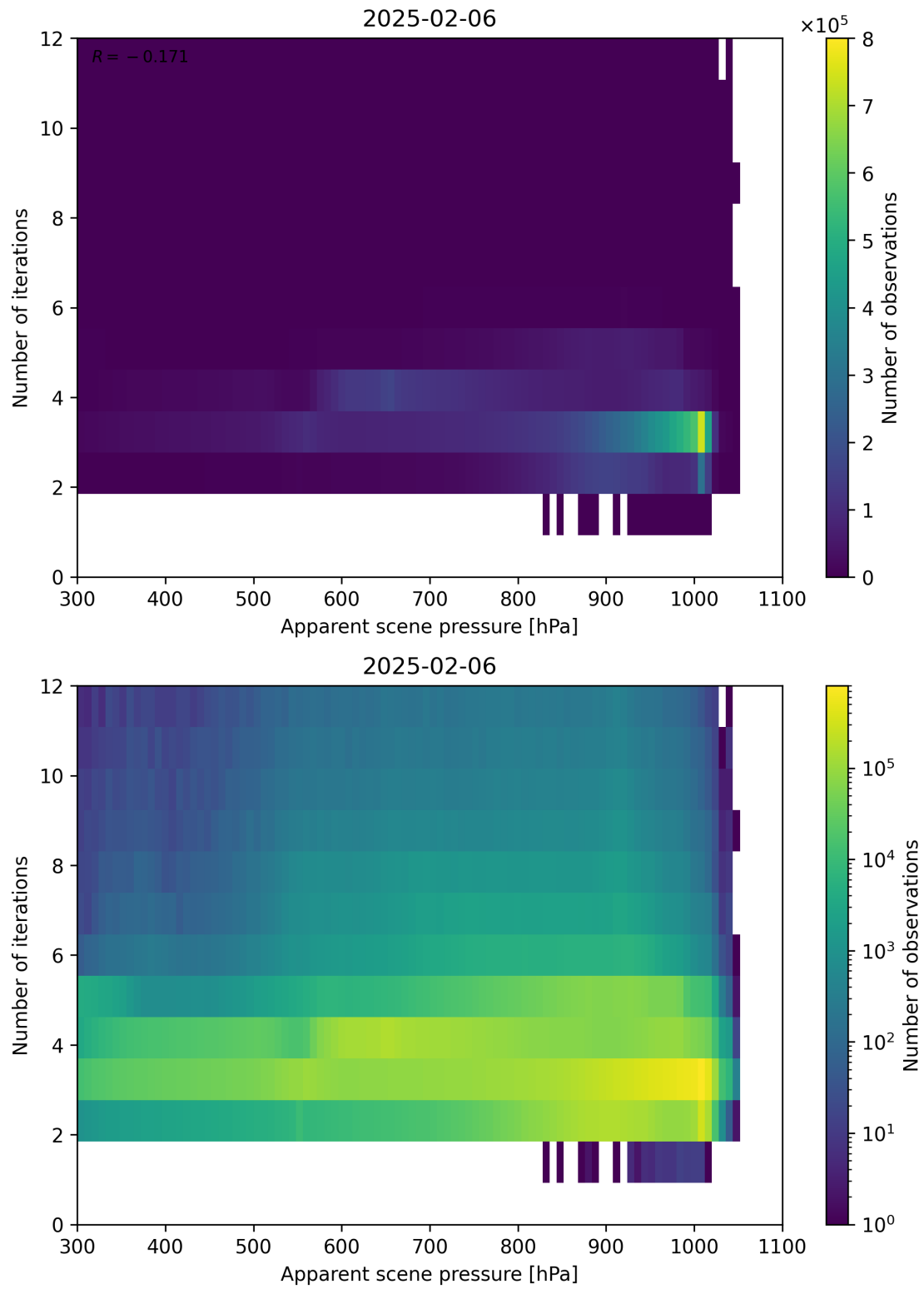
Figure 65: Scatter density plot of “Apparent scene pressure” against “Number of iterations” for 2025-02-05 to 2025-02-07.
