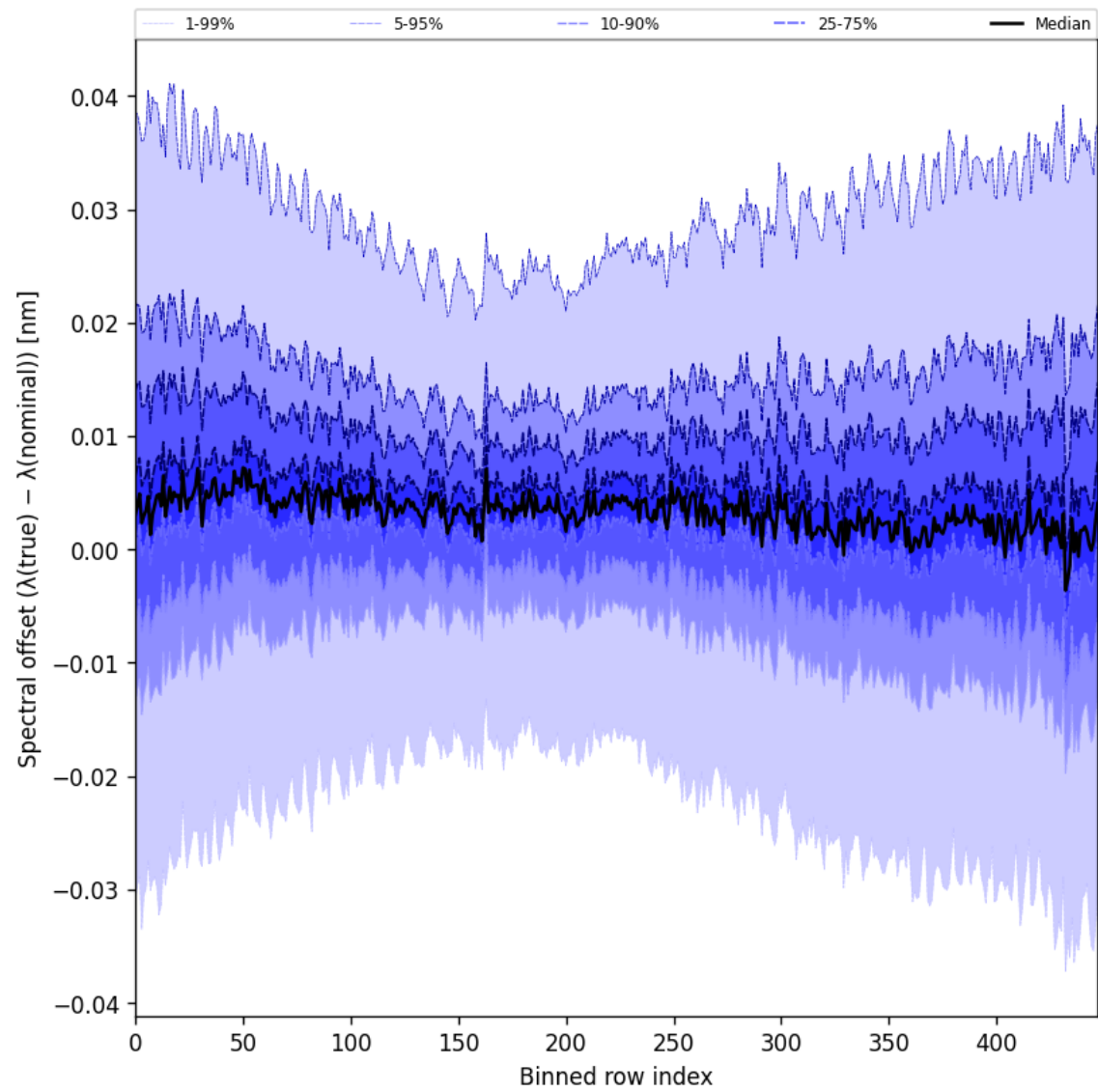
Figure 62: Along track statistics of “Spectral offset ( \lambda_{\text{true}} - \lambda_{\text{nominal}} )” for 2025-02-05 to 2025-02-07
