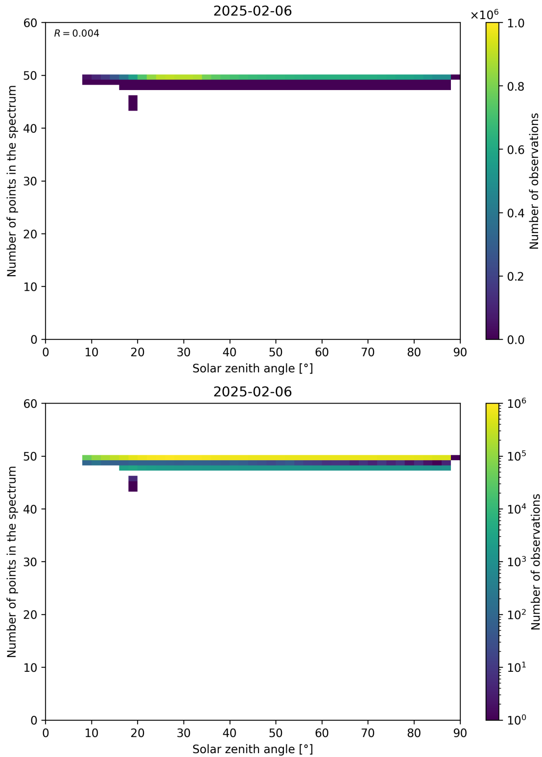
Figure 115: Scatter density plot of “Solar zenith angle” against “Number of points in the spectrum” for 2025-02-05 to 2025-02-07.
