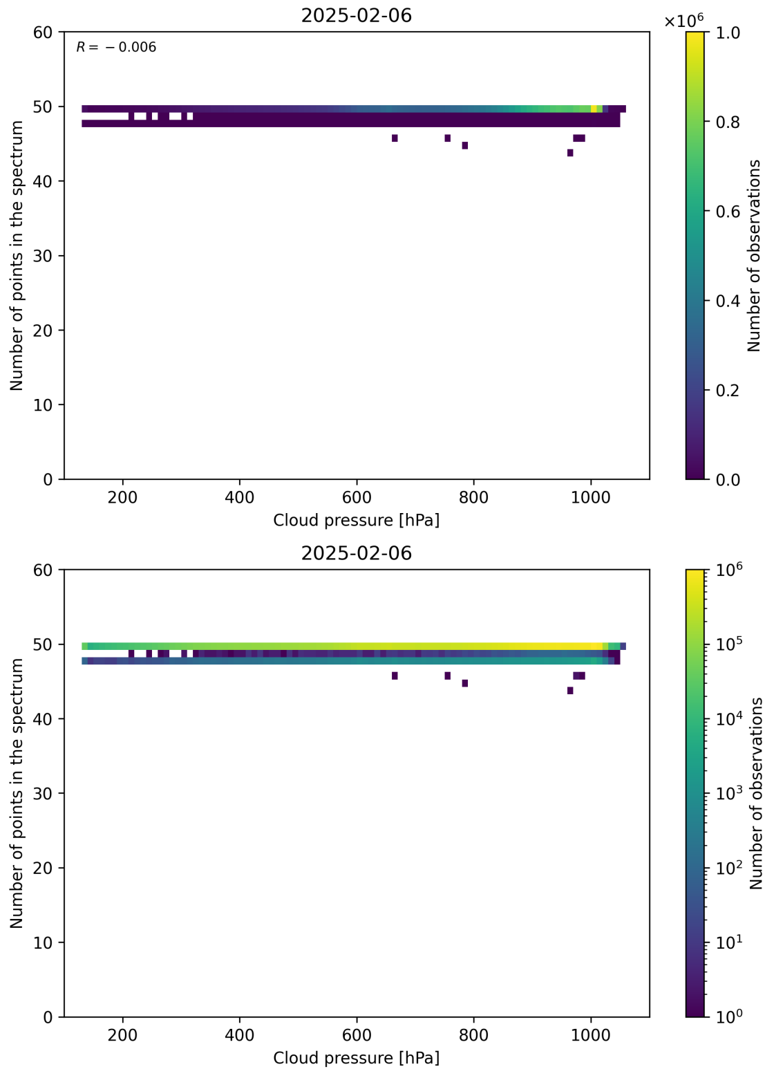
Figure 82: Scatter density plot of “Cloud pressure” against “Number of points in the spectrum” for 2025-02-05 to 2025-02-07.
