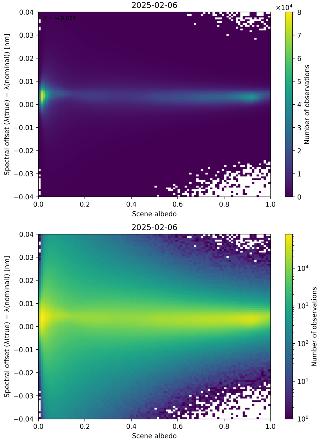
Figure 107: Scatter density plot of “Scene albedo” against “Spectral offset ( \lambda_{\text{true}} - \lambda_{\text{nominal}} )” for 2025-02-05 to 2025-02-07.
