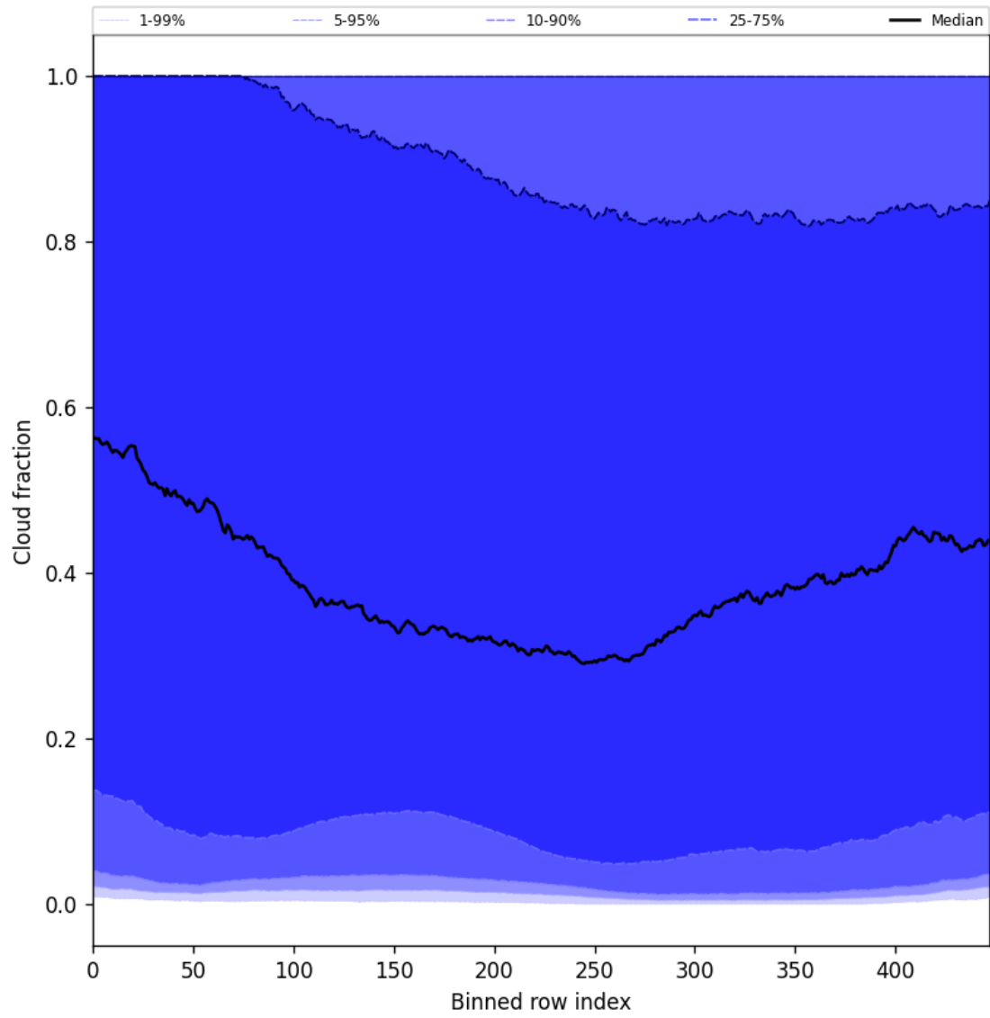
Figure 49: Along track statistics of “Cloud fraction” for 2025-02-05 to 2025-02-07
