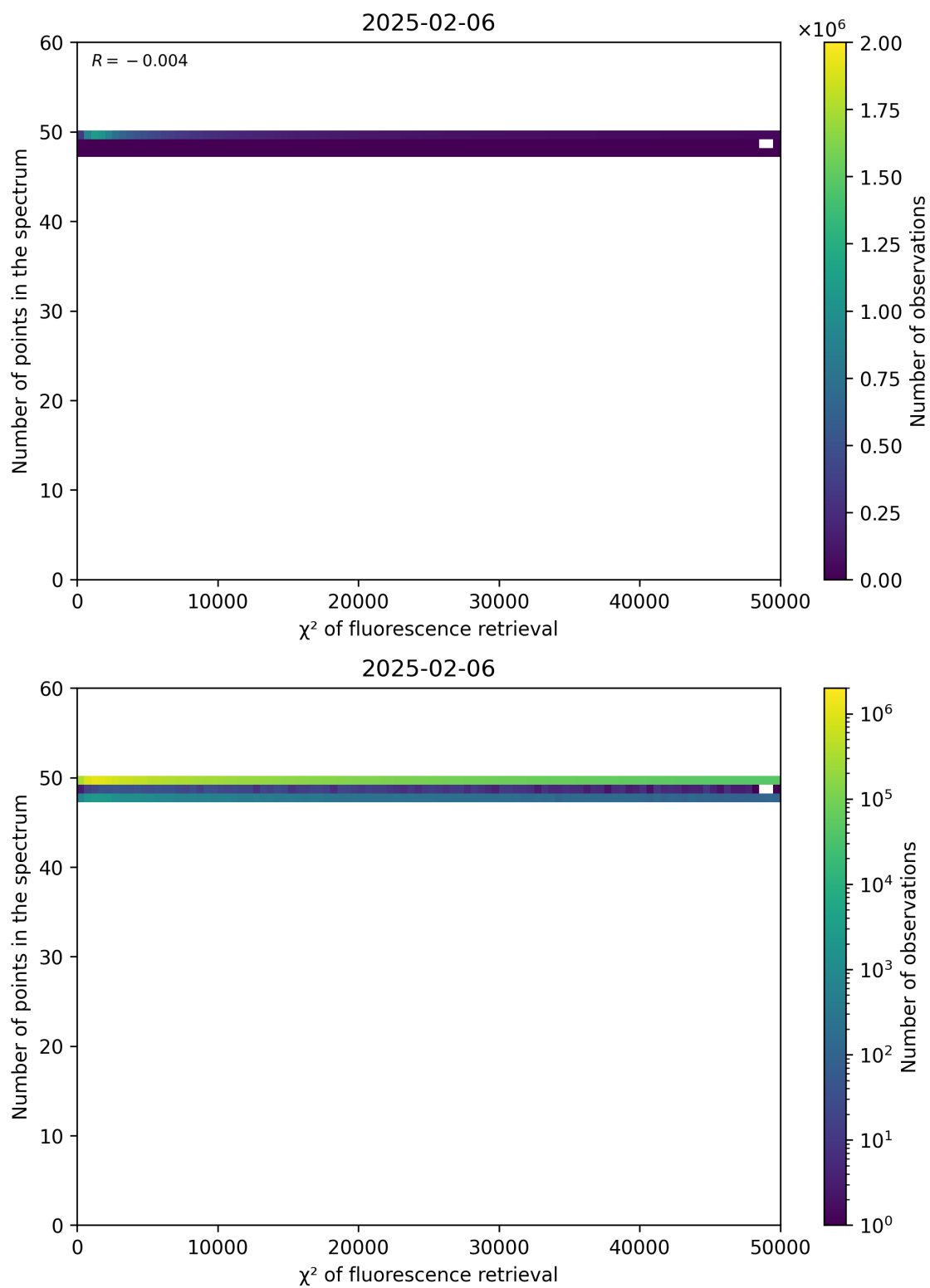
Figure 68: Scatter density plot of " \chi^2 of fluorescence retrieval" against "Number of points in the spectrum" for 2025-02-05 to 2025-02-07.
