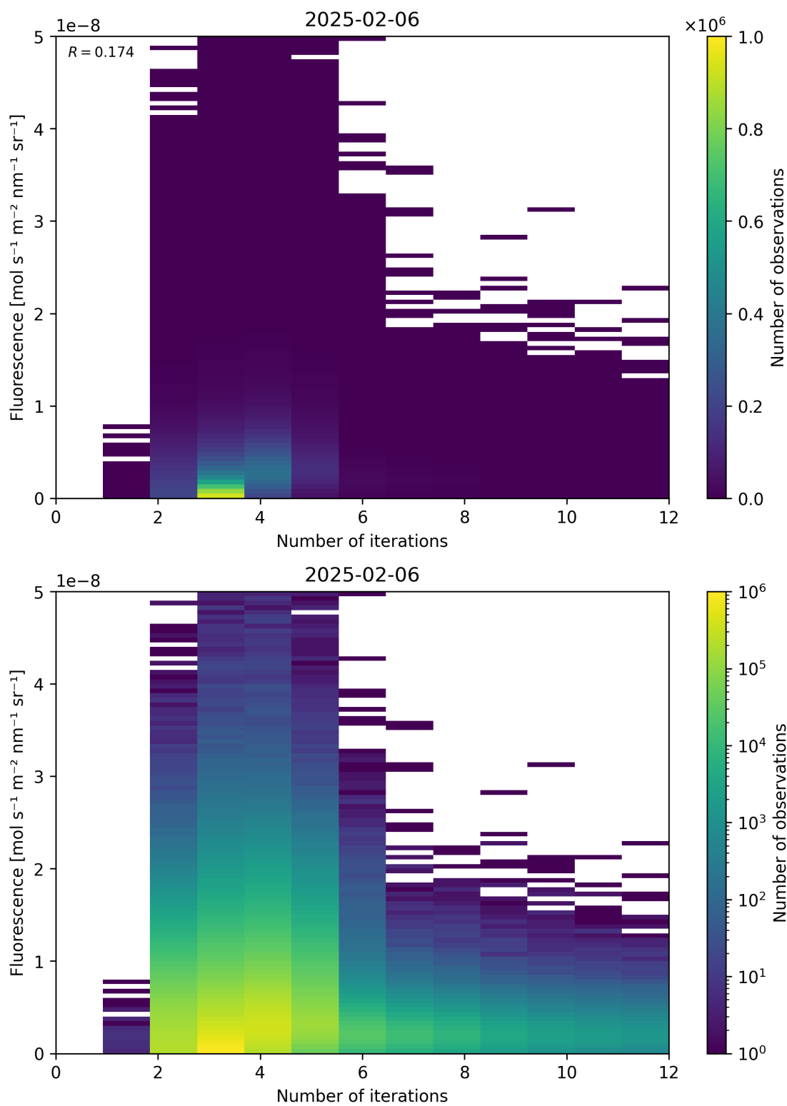
Figure 98: Scatter density plot of “Number of iterations” against “Fluorescence” for 2025-02-05 to 2025-02-07.
