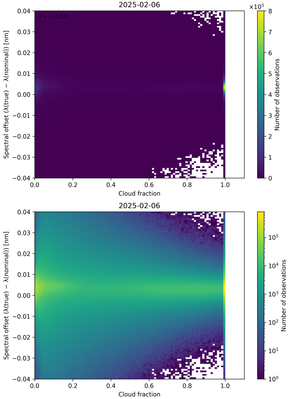
Figure 76: Scatter density plot of “Cloud fraction” against “Spectral offset ( \lambda_{\text{true}} - \lambda_{\text{nominal}} )” for 2025-02-05 to 2025-02-07.
