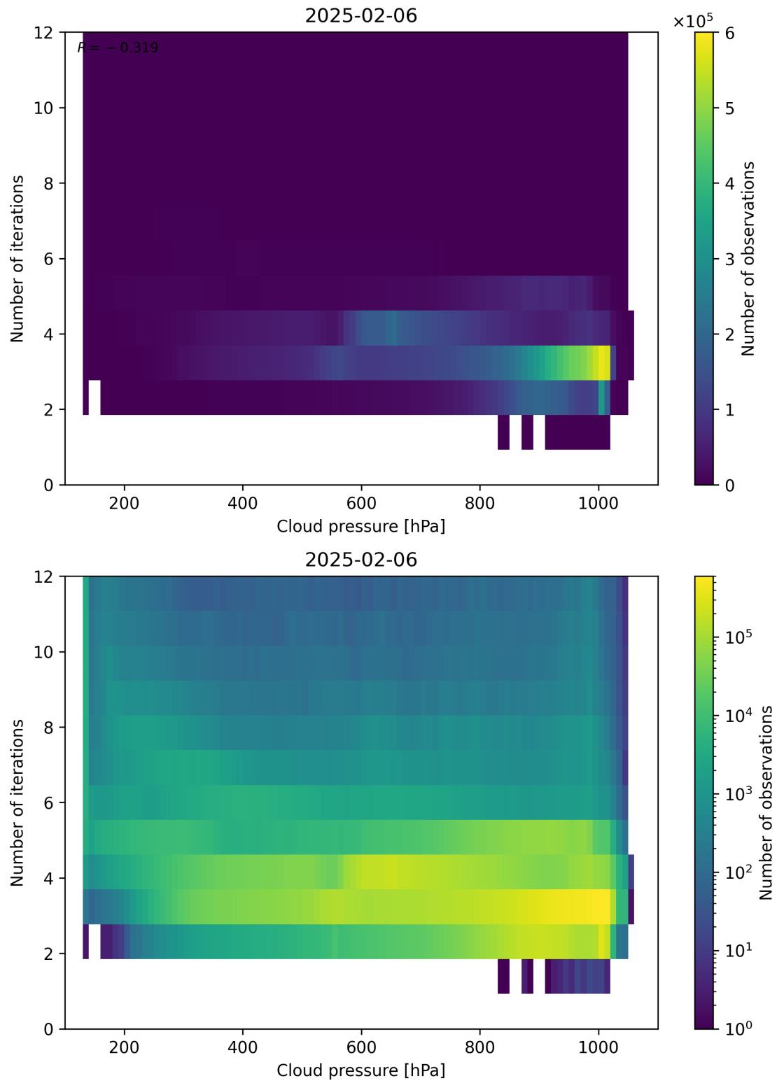
Figure 81: Scatter density plot of “Cloud pressure” against “Number of iterations” for 2025-02-05 to 2025-02-07.
