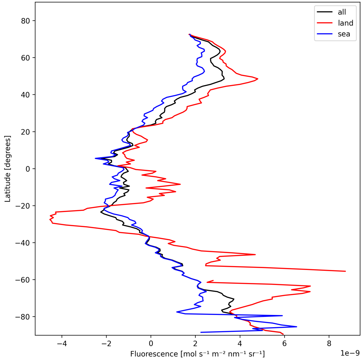
Figure 23: Zonal average of “Fluorescence” for 2025-02-05 to 2025-02-07.
