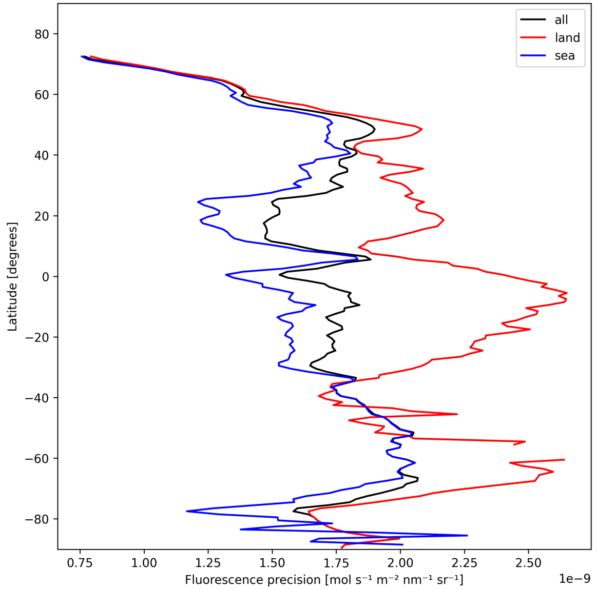
Figure 24: Zonal average of “Fluorescence precision” for 2025-02-05 to 2025-02-07.
