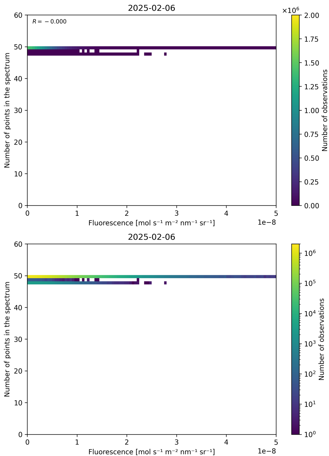
Figure 86: Scatter density plot of “Fluorescence” against “Number of points in the spectrum” for 2025-02-05 to 2025-02-07.
