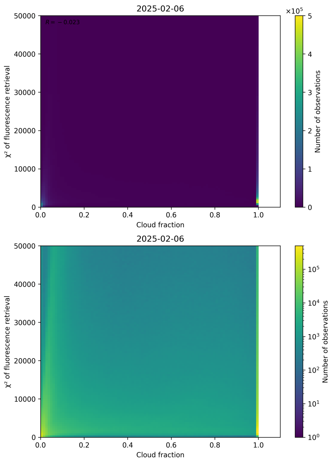
Figure 71: Scatter density plot of “Cloud fraction” against “ \chi^2 of fluorescence retrieval” for 2025-02-05 to 2025-02-07.
