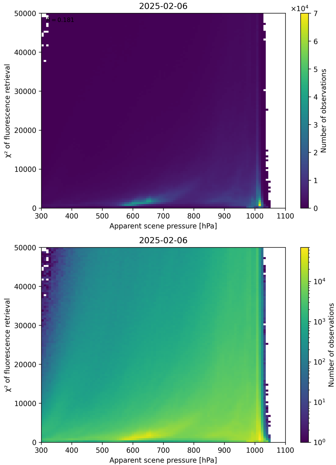
Figure 63: Scatter density plot of “Apparent scene pressure” against “ \chi^2 of fluorescence retrieval” for 2025-02-05 to 2025-02-07.
