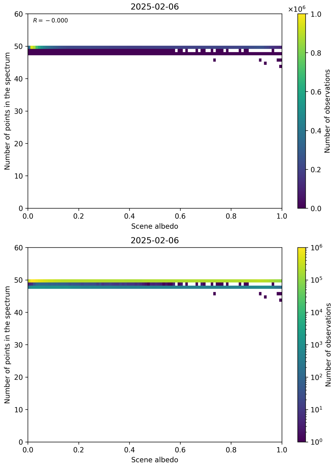
Figure 106: Scatter density plot of “Scene albedo” against “Number of points in the spectrum” for 2025-02-05 to 2025-02-07.
