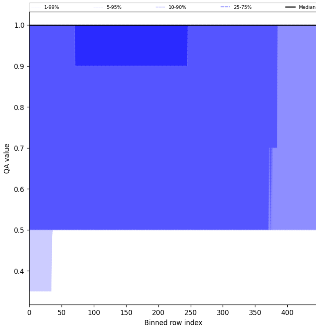
Figure 46: Along track statistics of “QA value” for 2025-02-05 to 2025-02-07
