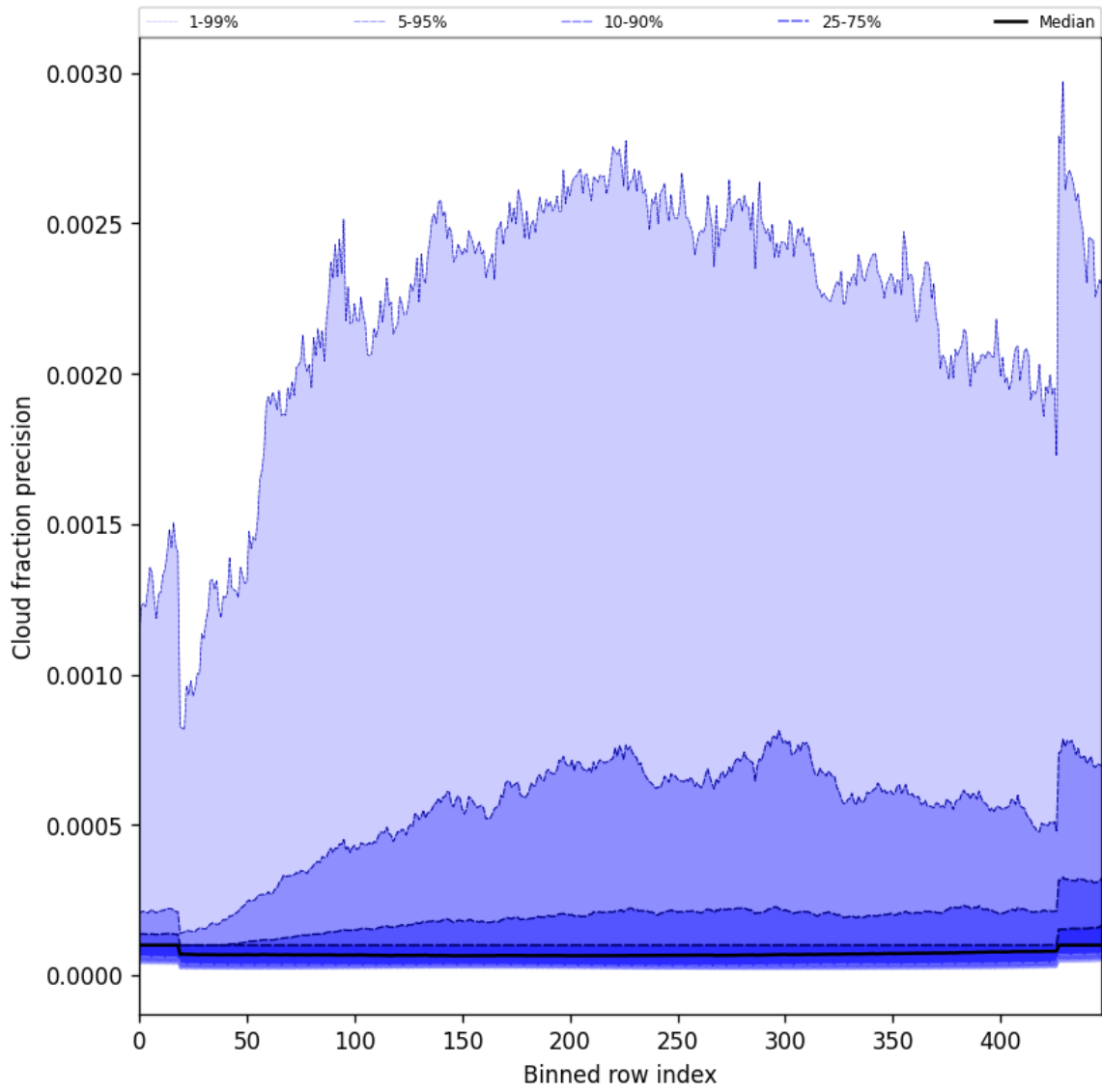
Figure 50: Along track statistics of “Cloud fraction precision” for 2025-02-05 to 2025-02-07
