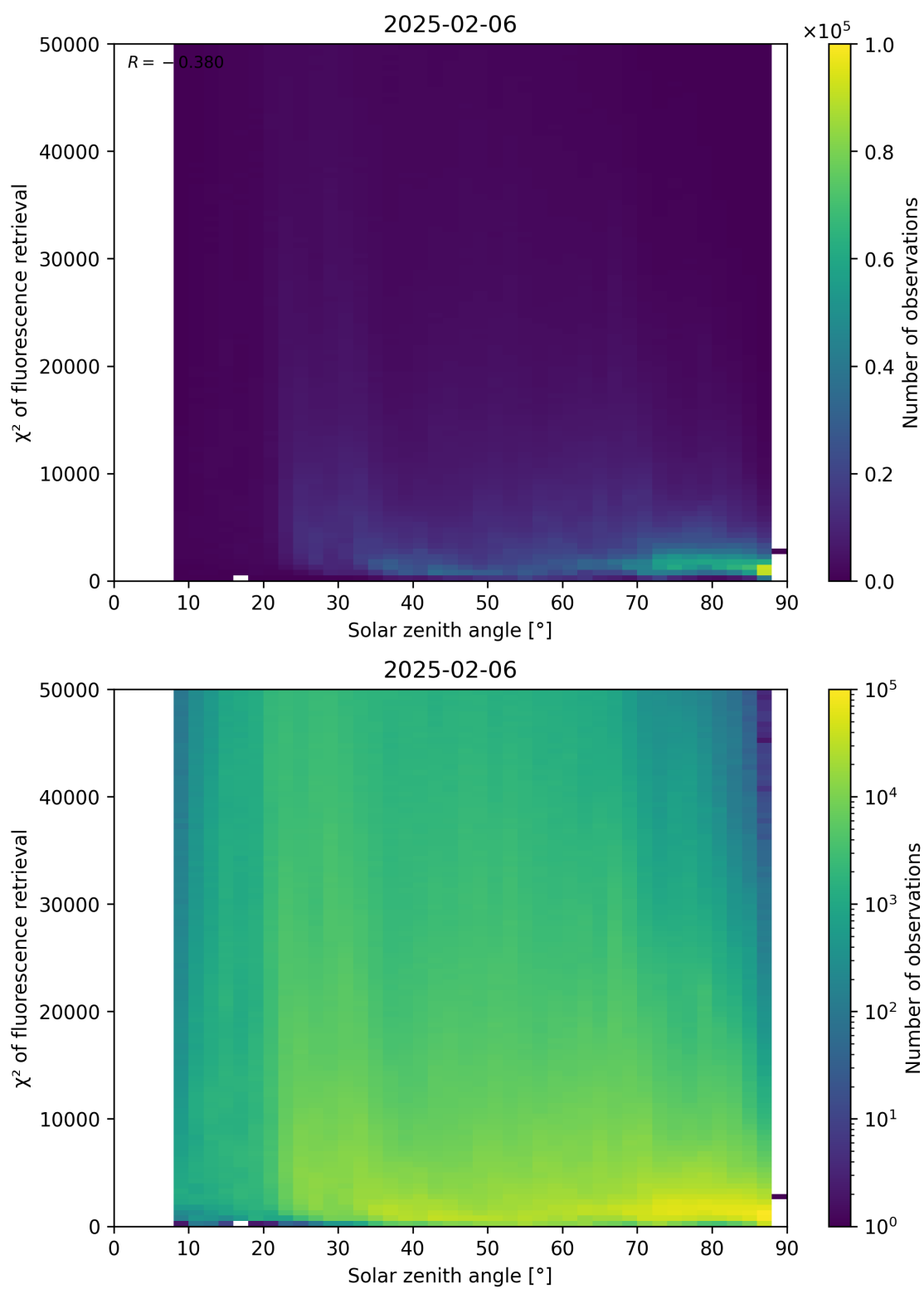
Figure 109: Scatter density plot of “Solar zenith angle” against “ \chi^2 of fluorescence retrieval” for 2025-02-05 to 2025-02-07.
