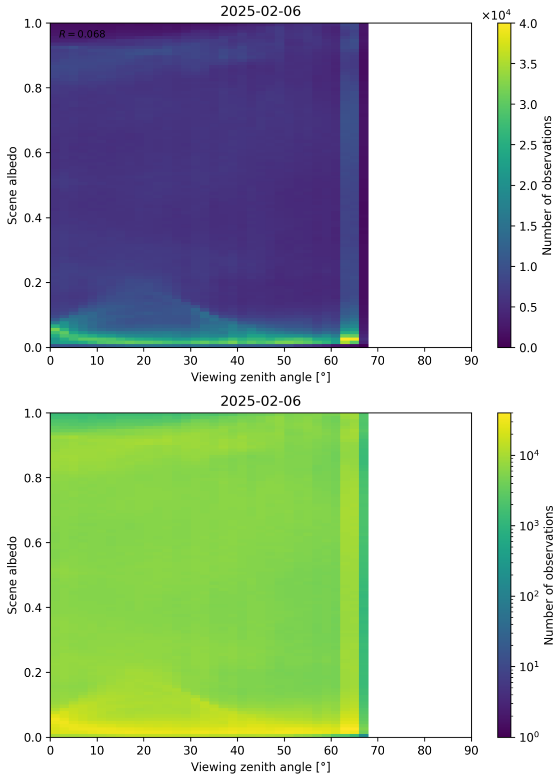
Figure 126: Scatter density plot of “Viewing zenith angle” against “Scene albedo” for 2025-02-05 to 2025-02-07.
