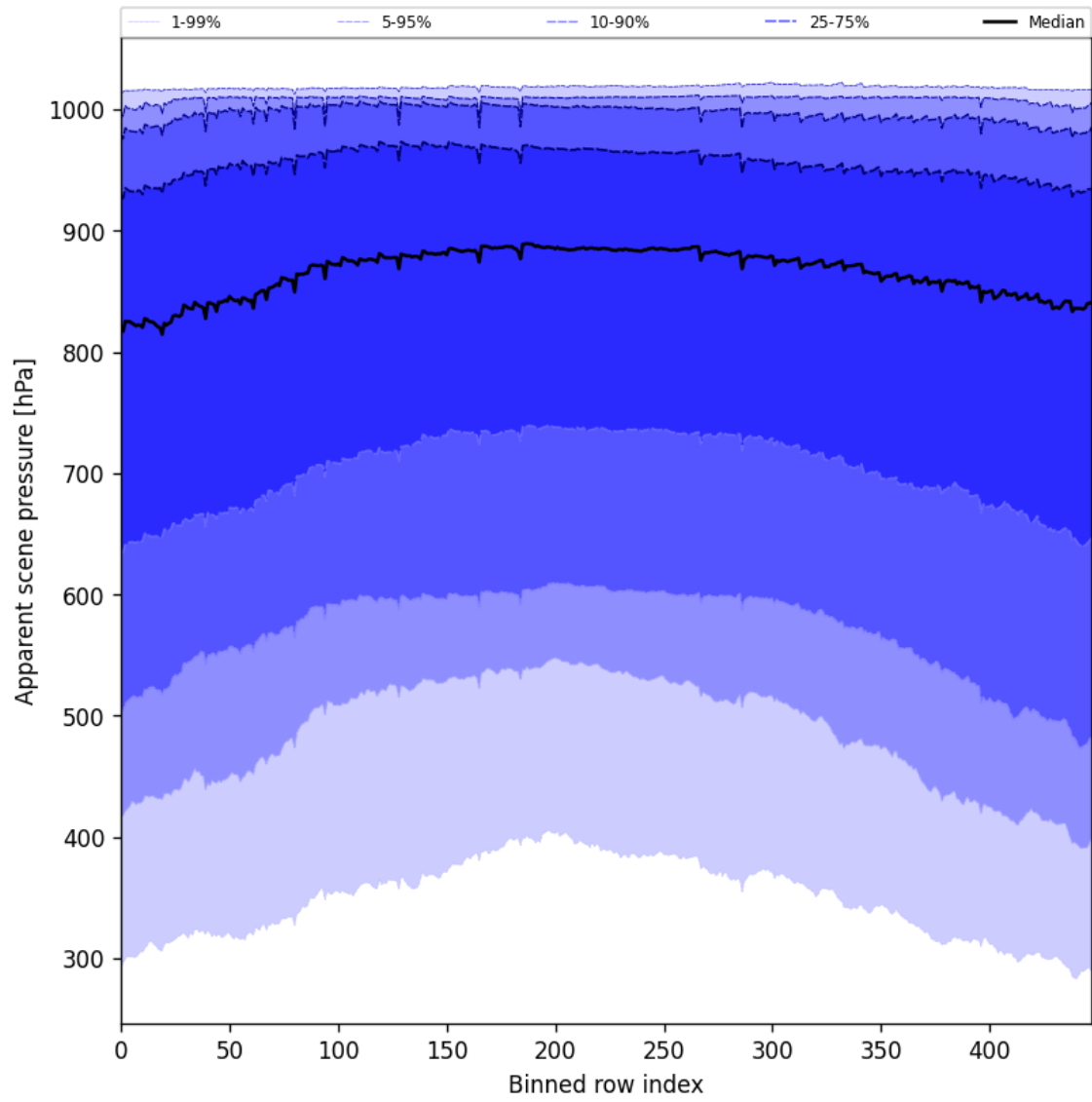
Figure 53: Along track statistics of “Apparent scene pressure” for 2025-02-05 to 2025-02-07
