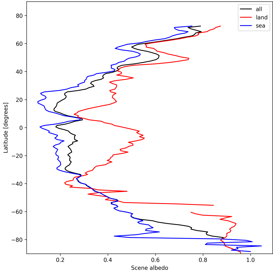
Figure 17: Zonal average of “Scene albedo” for 2025-02-05 to 2025-02-07.
