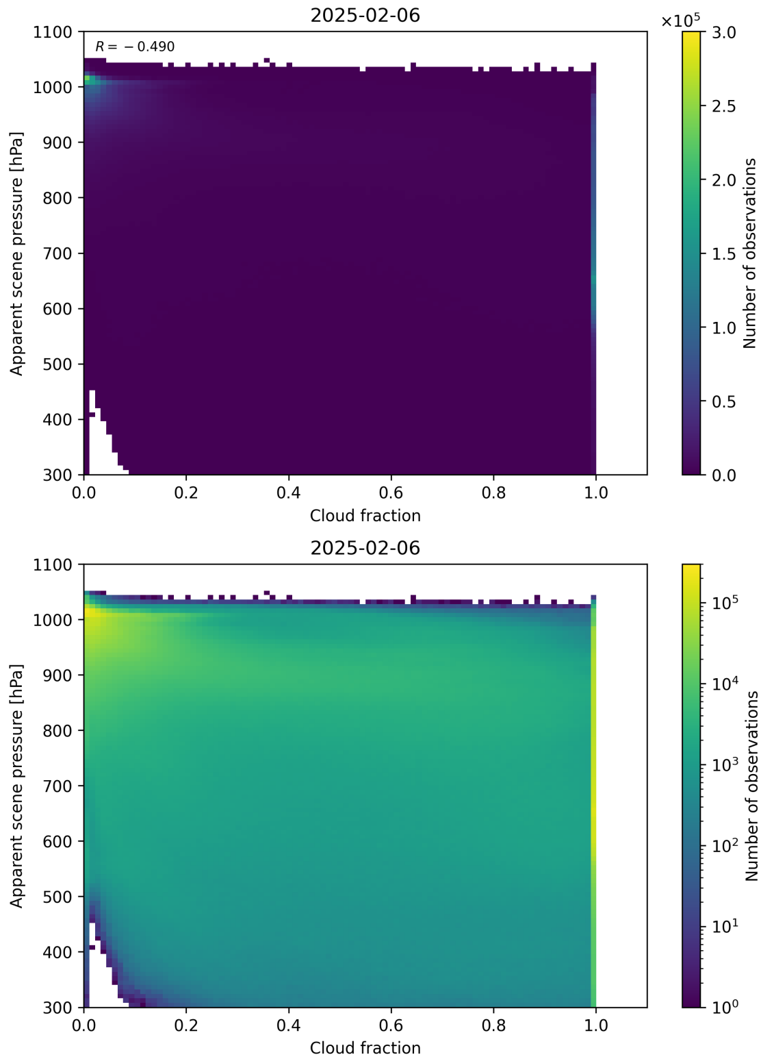
Figure 70: Scatter density plot of “Cloud fraction” against “Apparent scene pressure” for 2025-02-05 to 2025-02-07.
