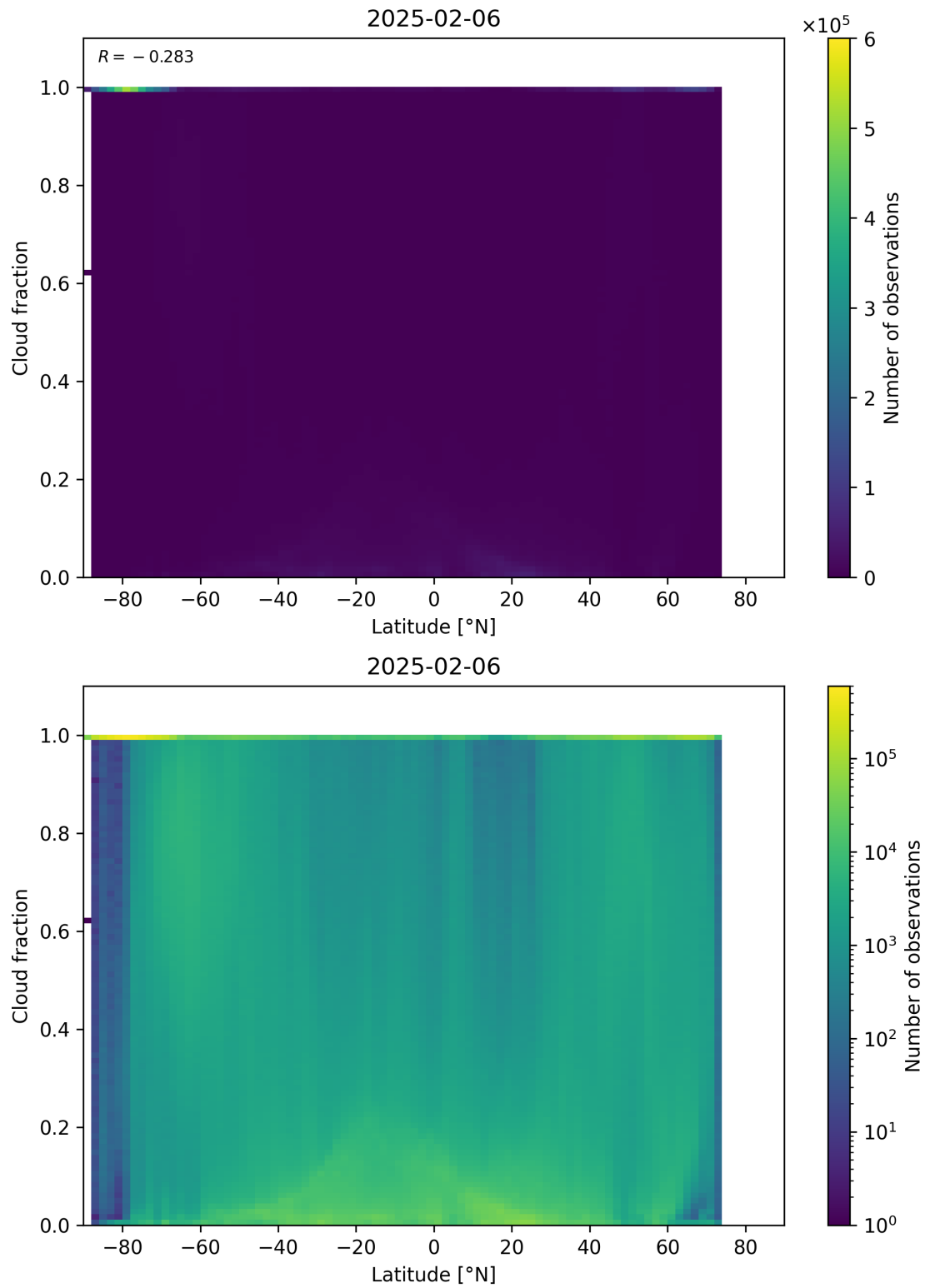
Figure 90: Scatter density plot of “Latitude” against “Cloud fraction” for 2025-02-05 to 2025-02-07.
