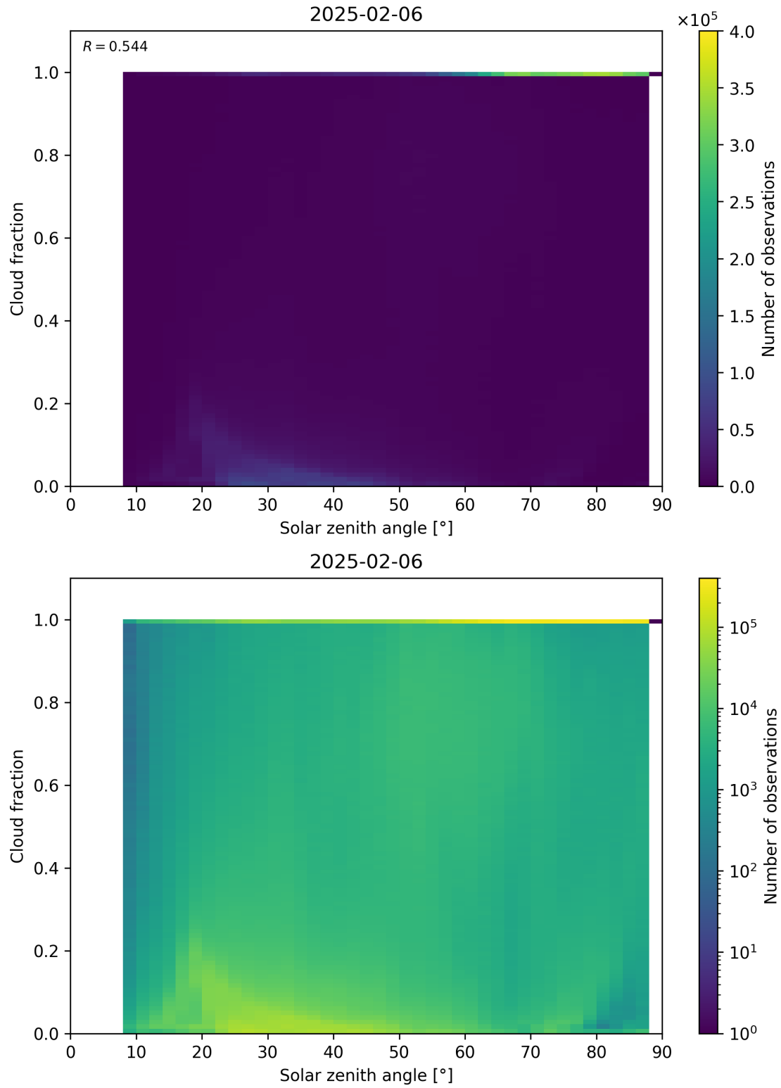
Figure 110: Scatter density plot of “Solar zenith angle” against “Cloud fraction” for 2025-02-05 to 2025-02-07.
