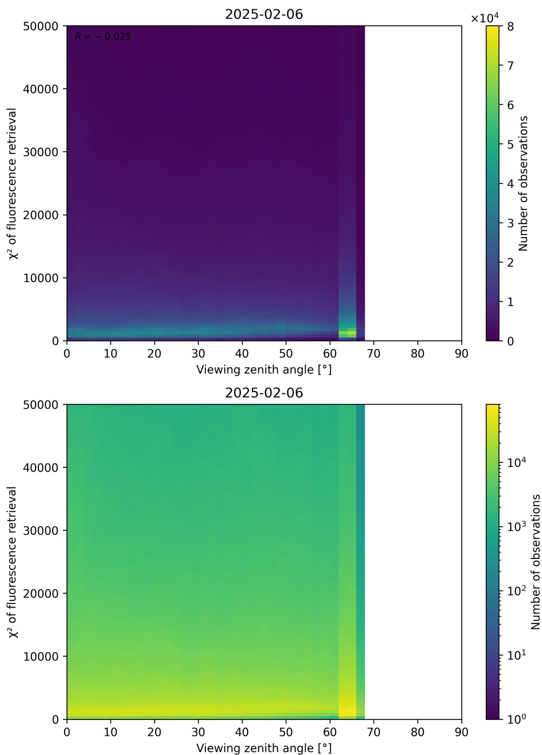
Figure 119: Scatter density plot of “Viewing zenith angle” against “ \chi^2 of fluorescence retrieval” for 2025-02-05 to 2025-02-07.
