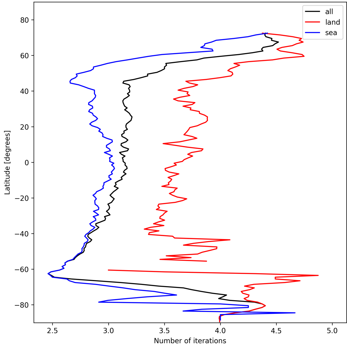
Figure 22: Zonal average of “Number of iterations” for 2025-02-05 to 2025-02-07.
