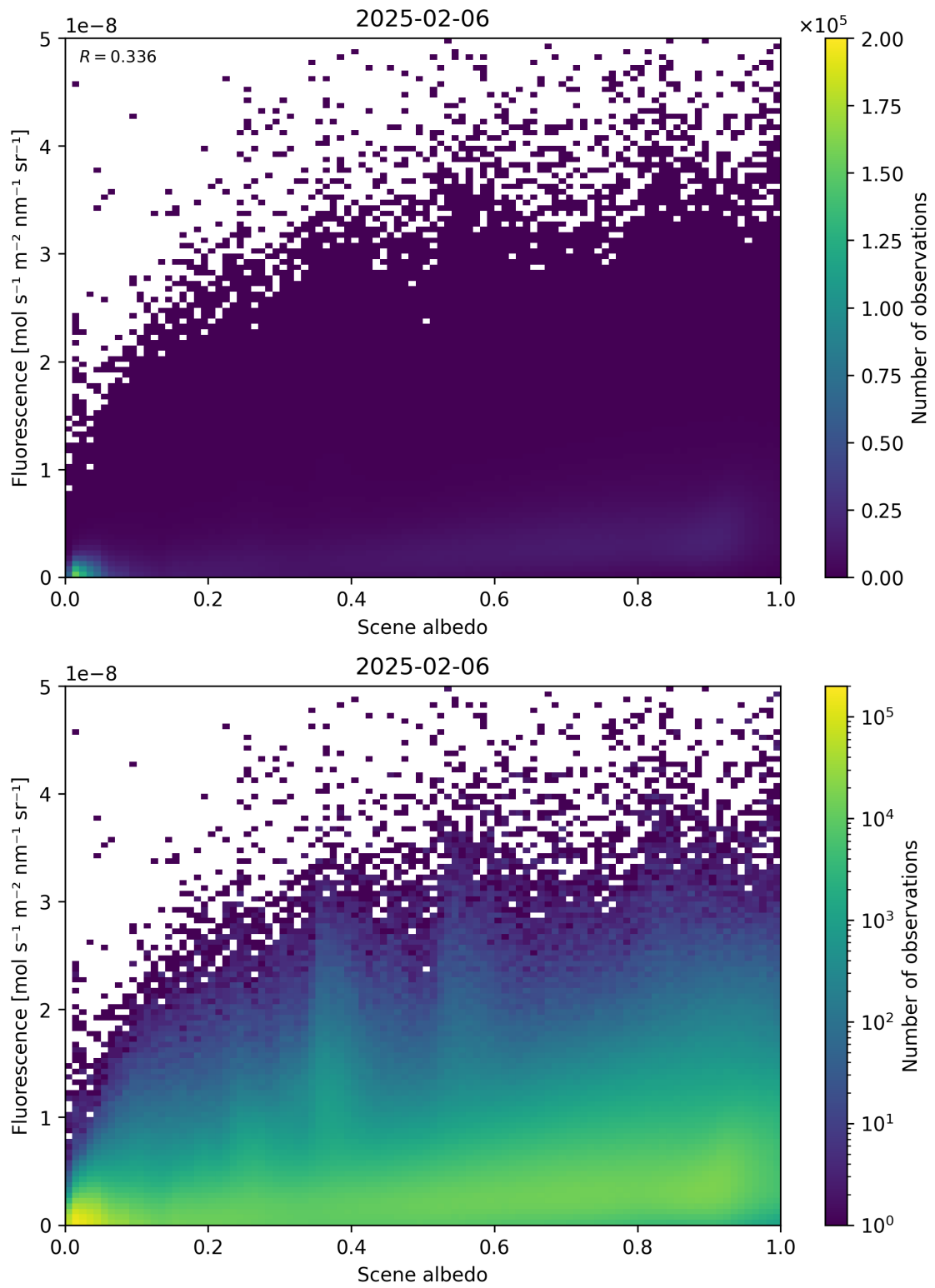
Figure 104: Scatter density plot of “Scene albedo” against “Fluorescence” for 2025-02-05 to 2025-02-07.
