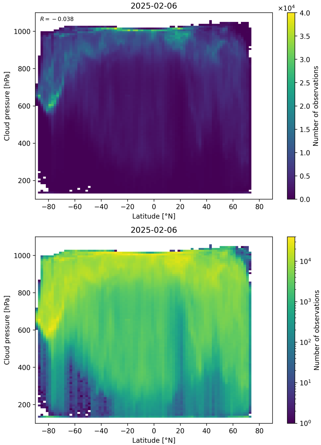
Figure 91: Scatter density plot of “Latitude” against “Cloud pressure” for 2025-02-05 to 2025-02-07.
