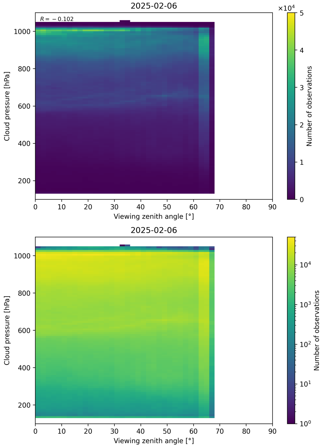
Figure 121: Scatter density plot of “Viewing zenith angle” against “Cloud pressure” for 2025-02-05 to 2025-02-07.
