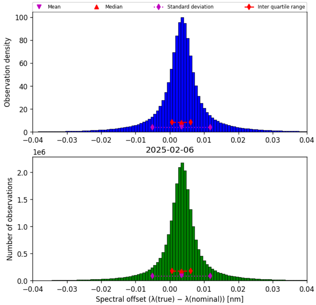
Figure 45: Histogram of “Spectral offset ( \lambda_{\text{true}} - \lambda_{\text{nominal}} )” for 2025-02-05 to 2025-02-07
