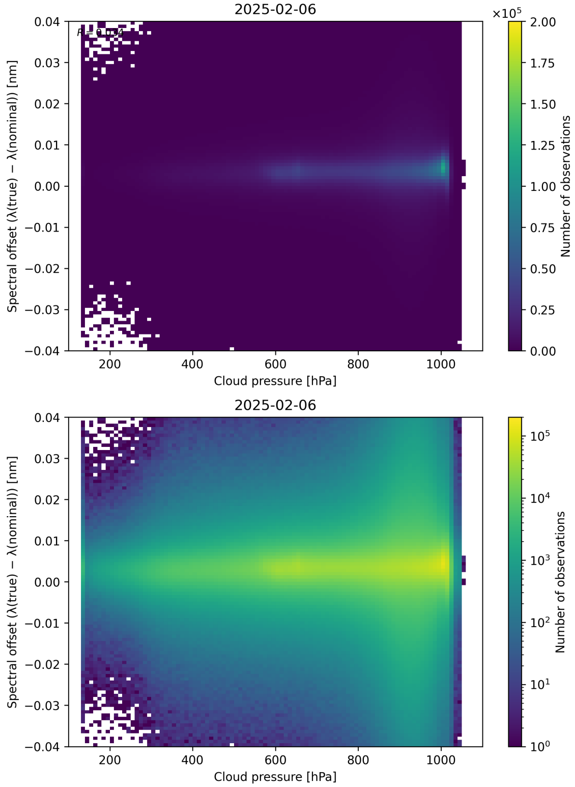
Figure 84: Scatter density plot of “Cloud pressure” against “Spectral offset ( \lambda_{\text{true}} - \lambda_{\text{nominal}} )” for 2025-02-05 to 2025-02-07.
