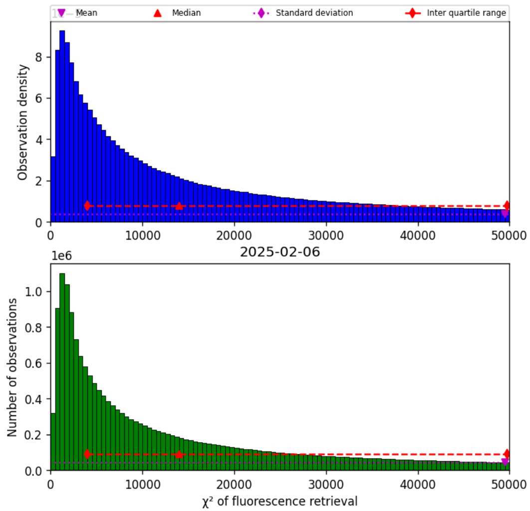
Figure 42: Histogram of “ \chi^2 of fluorescence retrieval” for 2025-02-05 to 2025-02-07
