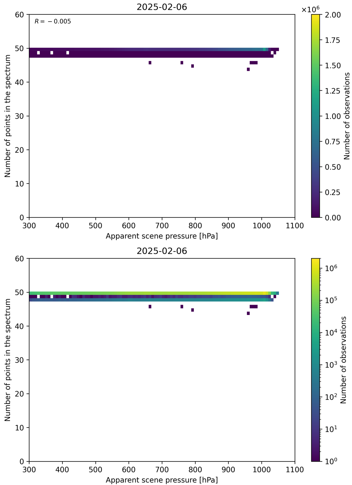
Figure 66: Scatter density plot of “Apparent scene pressure” against “Number of points in the spectrum” for 2025-02-05 to 2025-02-07.
