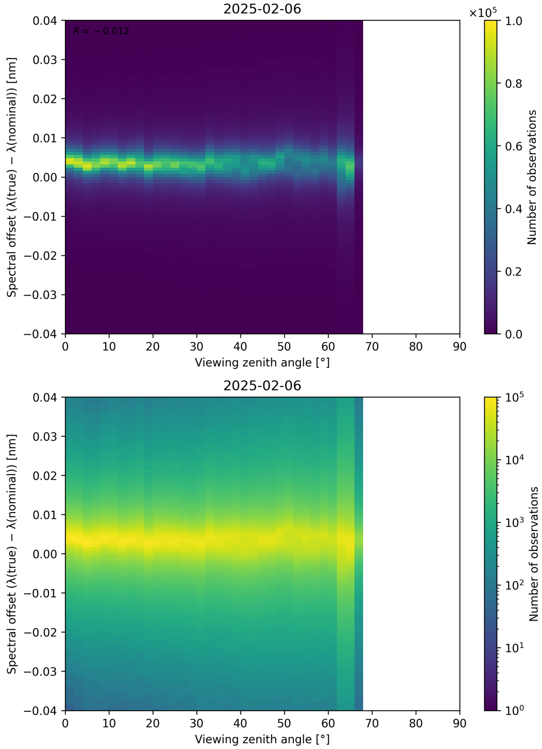
Figure 128: Scatter density plot of “Viewing zenith angle” against “Spectral offset ( \lambda_{\text{true}} - \lambda_{\text{nominal}} )” for 2025-02-05 to 2025-02-07.
