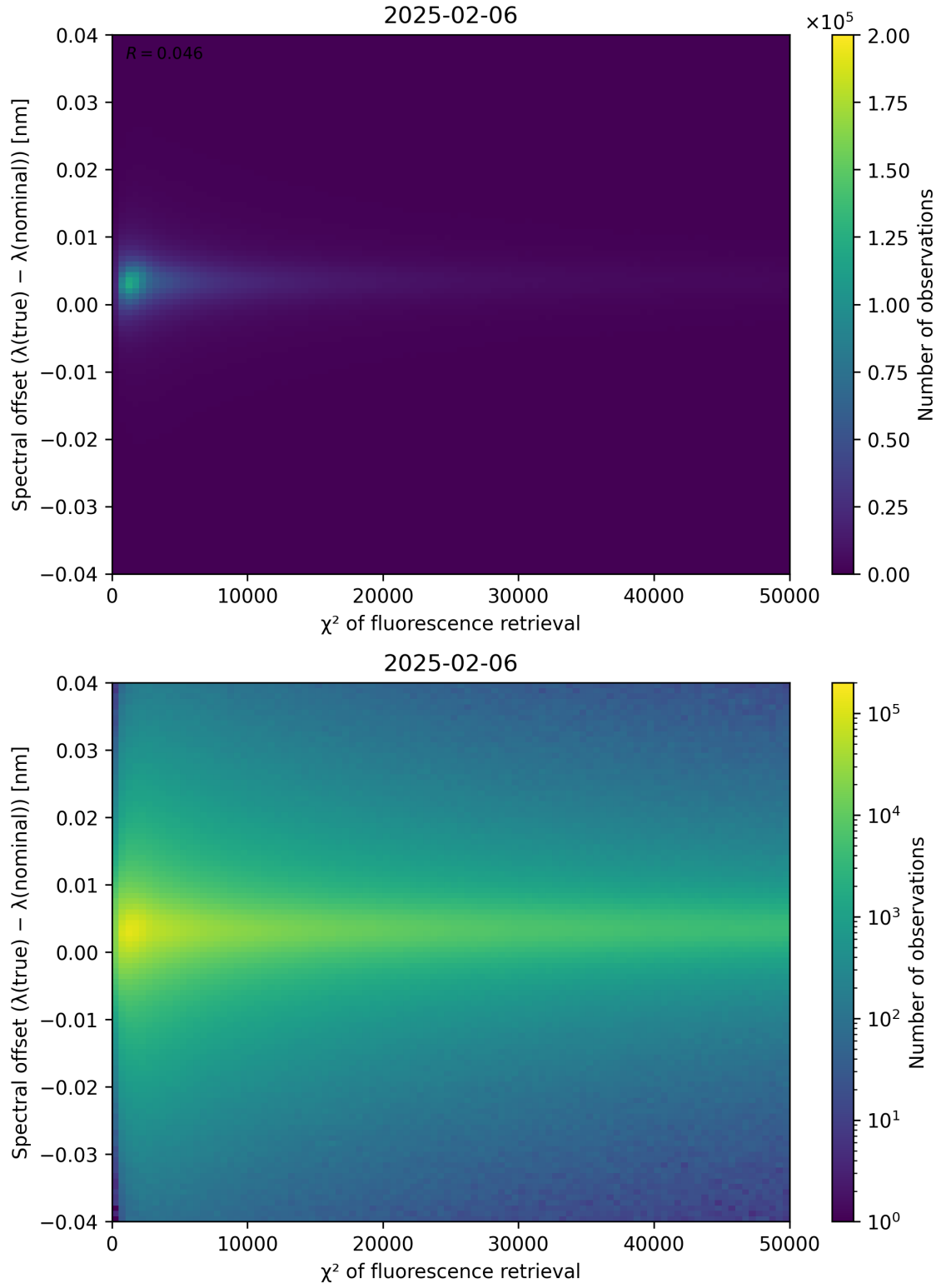
Figure 69: Scatter density plot of “ \chi^2 of fluorescence retrieval” against “Spectral offset ( \lambda_{\text{true}} - \lambda_{\text{nominal}} )” for 2025-02-05 to 2025-02-07.
