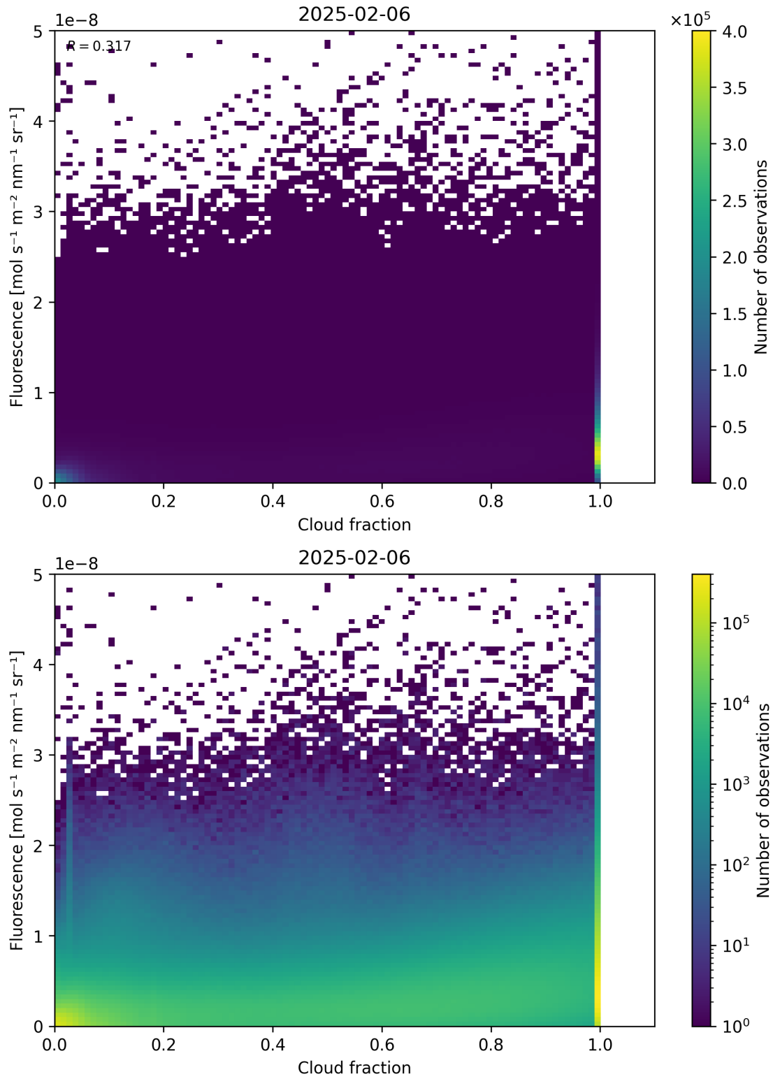
Figure 72: Scatter density plot of “Cloud fraction” against “Fluorescence” for 2025-02-05 to 2025-02-07.
