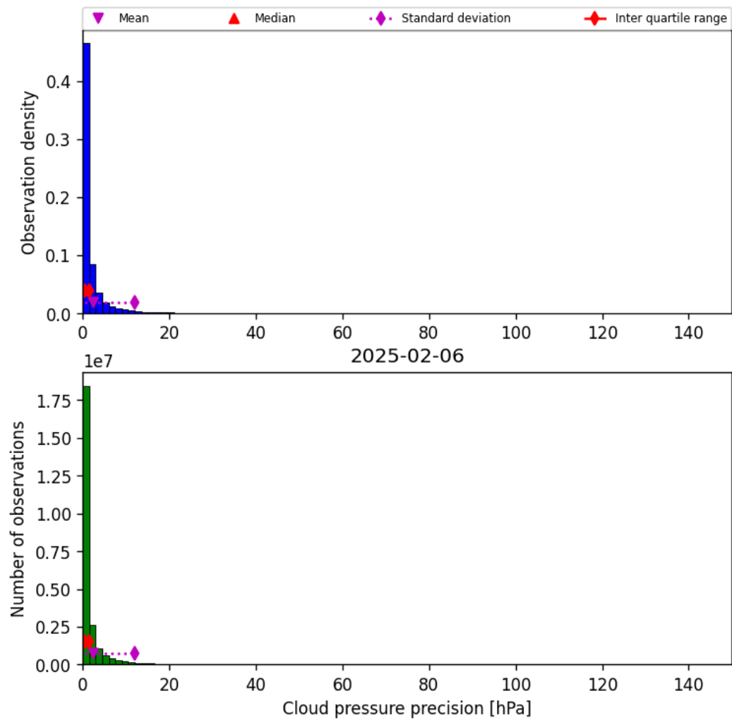
Figure 31: Histogram of “Cloud pressure precision” for 2025-02-05 to 2025-02-07
