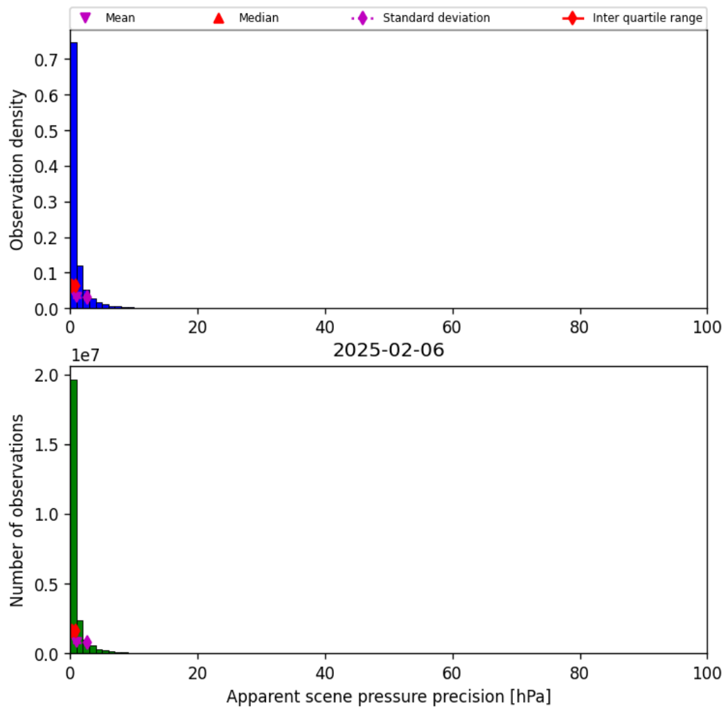
Figure 37: Histogram of “Apparent scene pressure precision” for 2025-02-05 to 2025-02-07
