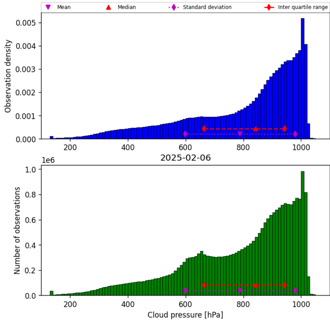
Figure 30: Histogram of “Cloud pressure” for 2025-02-05 to 2025-02-07
