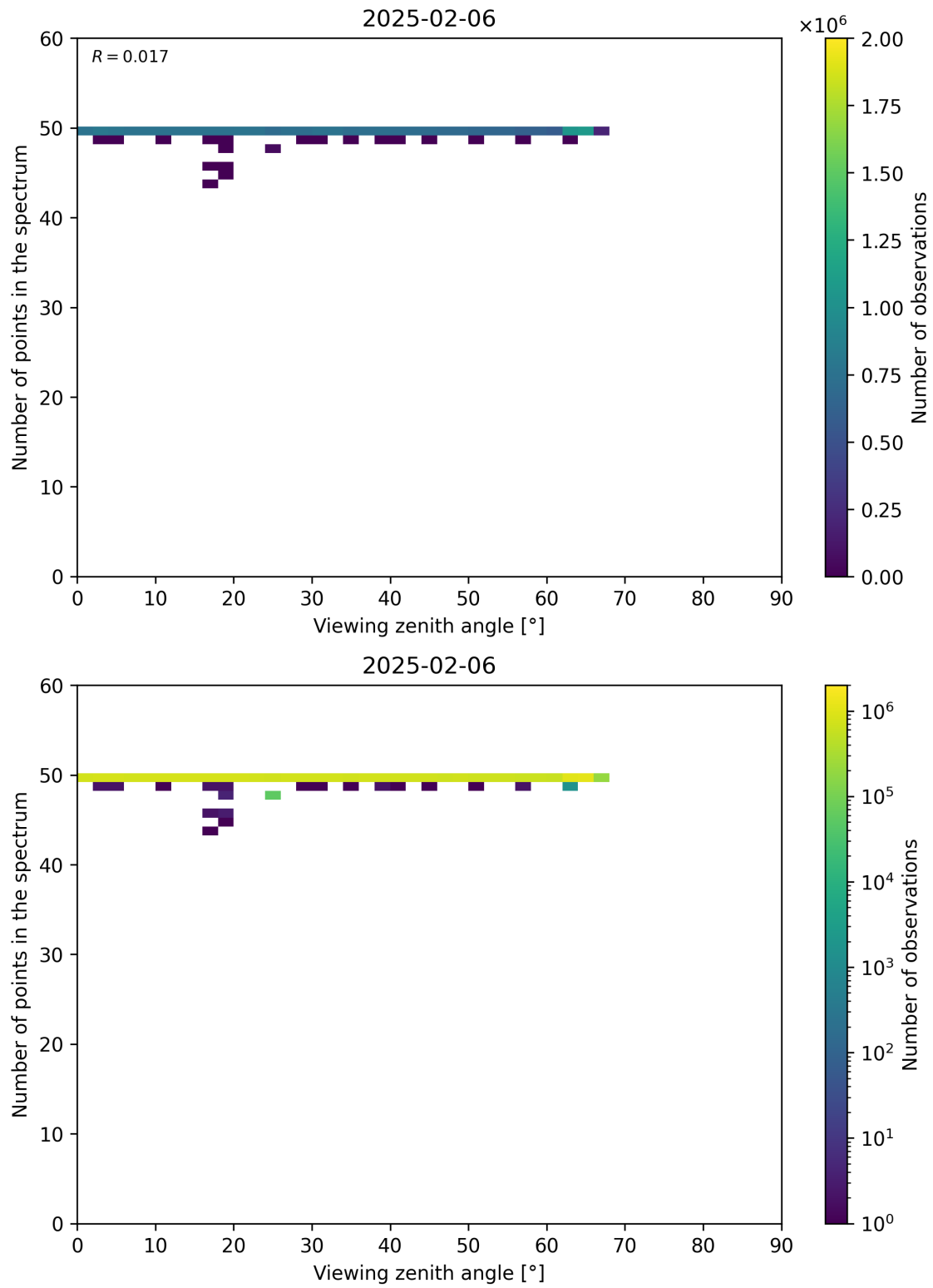
Figure 125: Scatter density plot of “Viewing zenith angle” against “Number of points in the spectrum” for 2025-02-05 to 2025-02-07.
