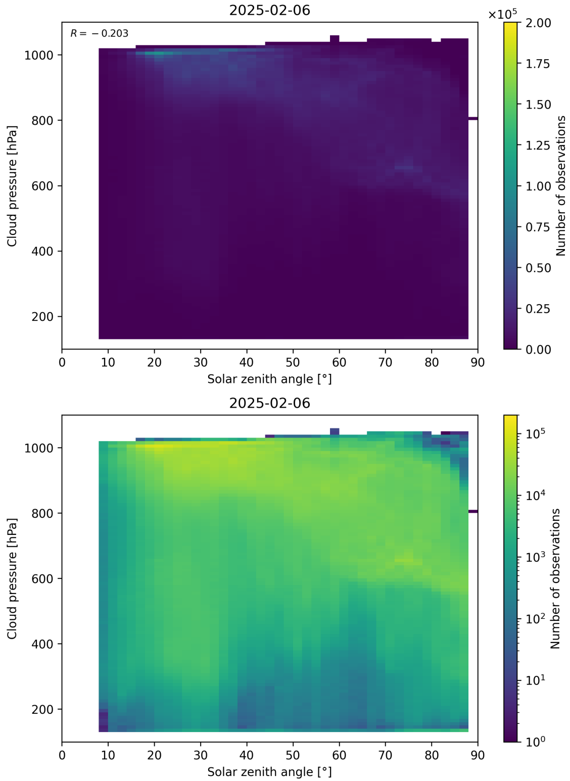
Figure 111: Scatter density plot of “Solar zenith angle” against “Cloud pressure” for 2025-02-05 to 2025-02-07.
