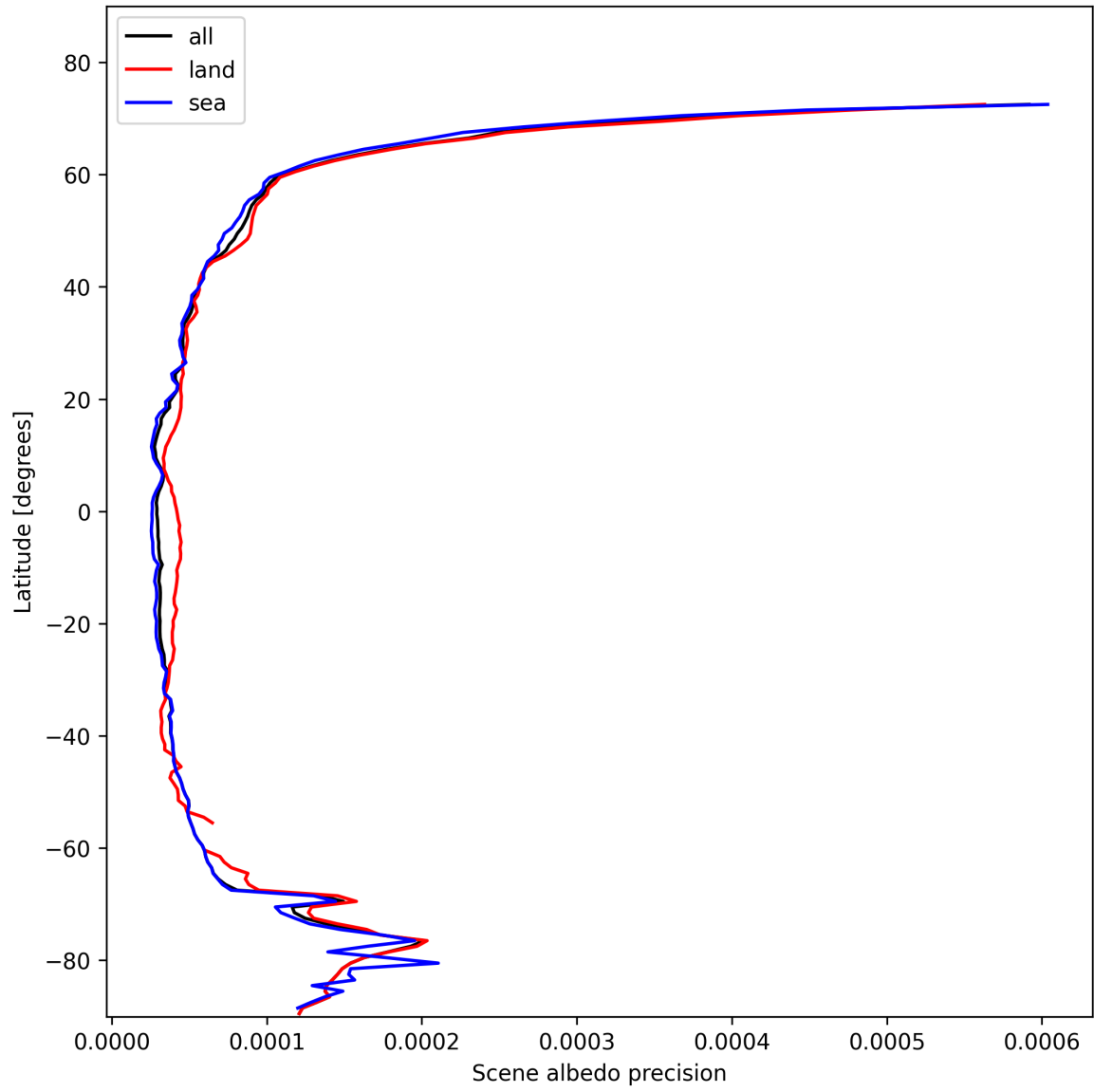
Figure 18: Zonal average of “Scene albedo precision” for 2025-02-05 to 2025-02-07.
