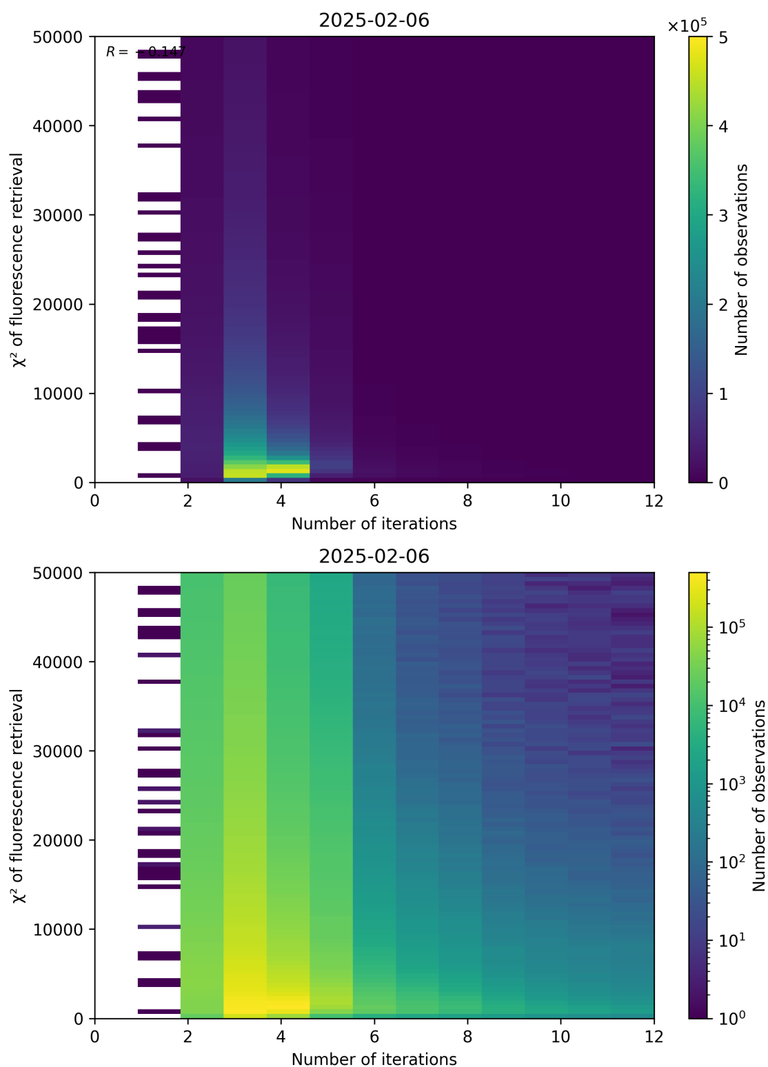
Figure 97: Scatter density plot of “Number of iterations” against “ \chi^2 of fluorescence retrieval” for 2025-02-05 to 2025-02-07.
