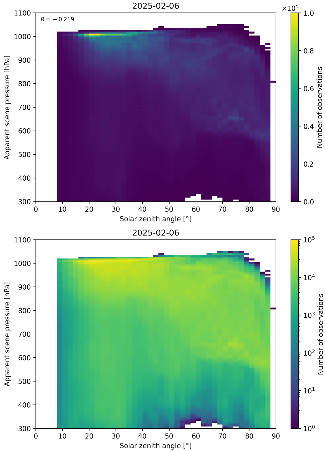
Figure 108: Scatter density plot of “Solar zenith angle” against “Apparent scene pressure” for 2025-02-05 to 2025-02-07.
