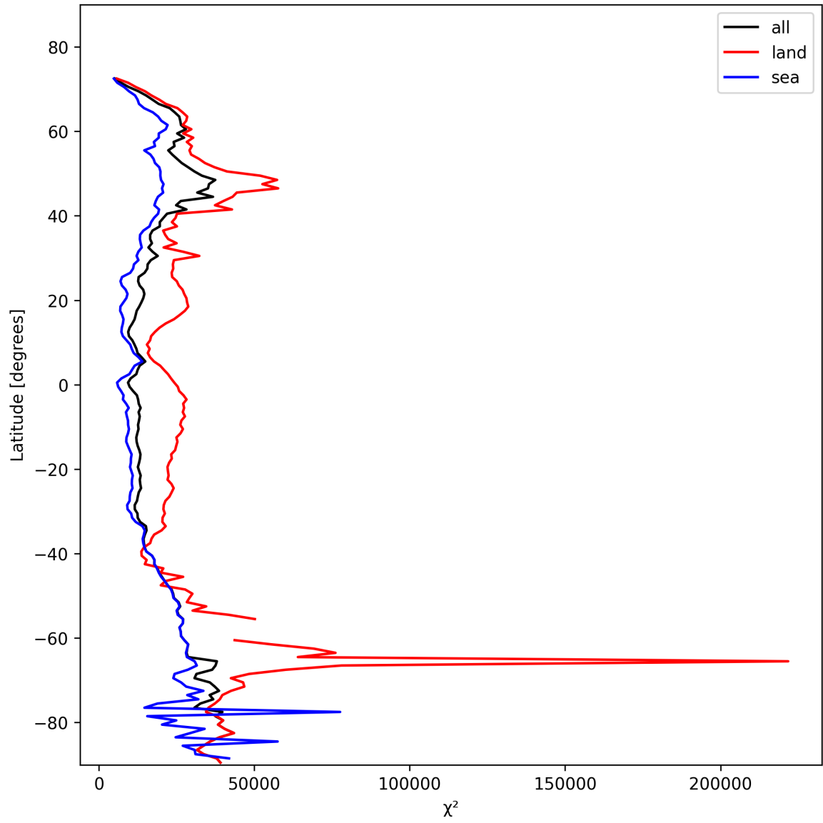
Figure 21: Zonal average of “ \chi^2 ” for 2025-02-05 to 2025-02-07.
