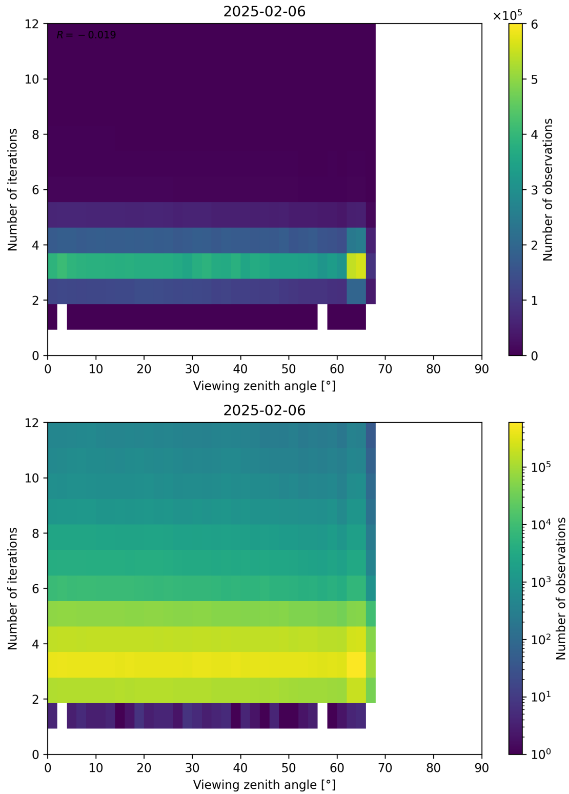
Figure 124: Scatter density plot of “Viewing zenith angle” against “Number of iterations” for 2025-02-05 to 2025-02-07.
