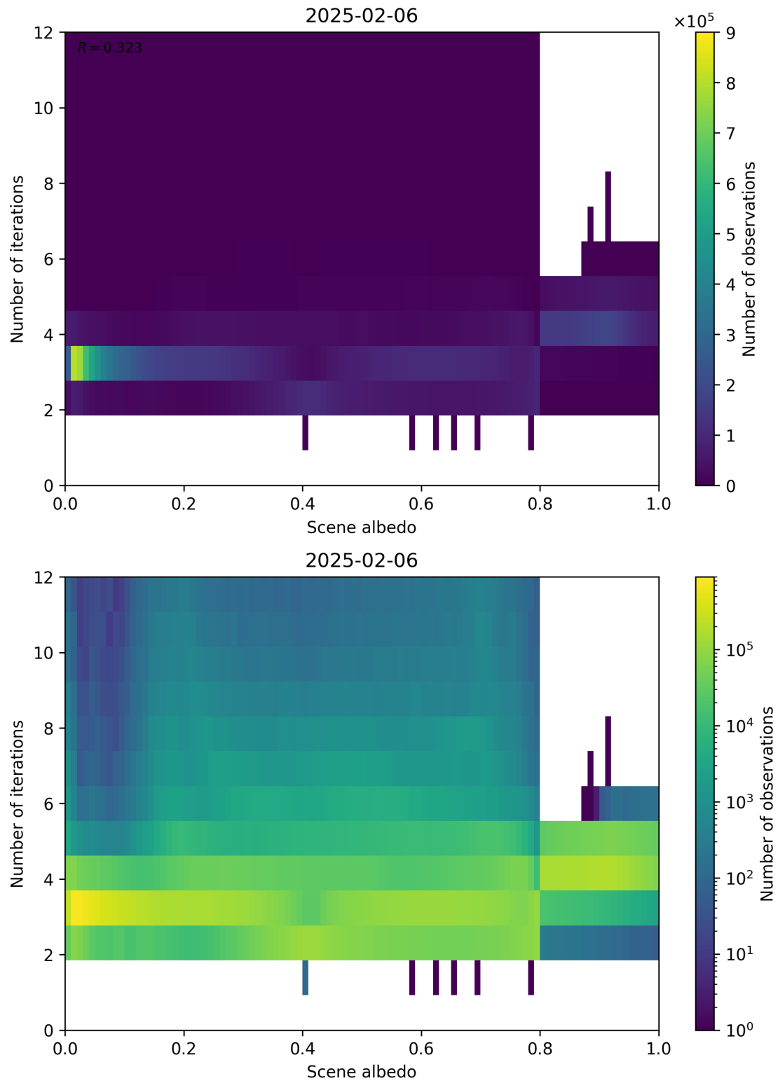
Figure 105: Scatter density plot of “Scene albedo” against “Number of iterations” for 2025-02-05 to 2025-02-07.
