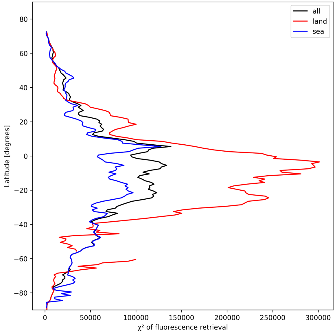
Figure 25: Zonal average of “ \chi^2 of fluorescence retrieval” for 2025-02-05 to 2025-02-07.
