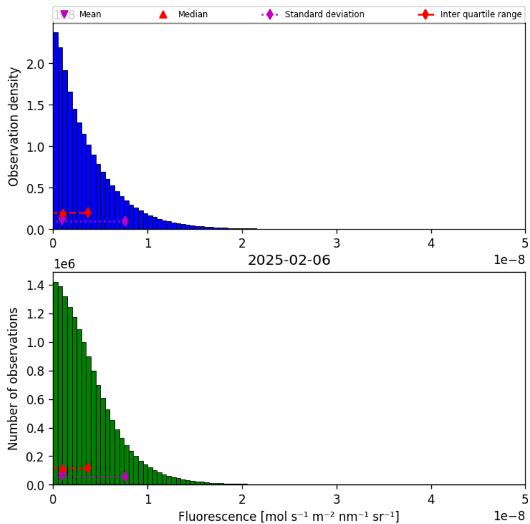
Figure 40: Histogram of “Fluorescence” for 2025-02-05 to 2025-02-07
