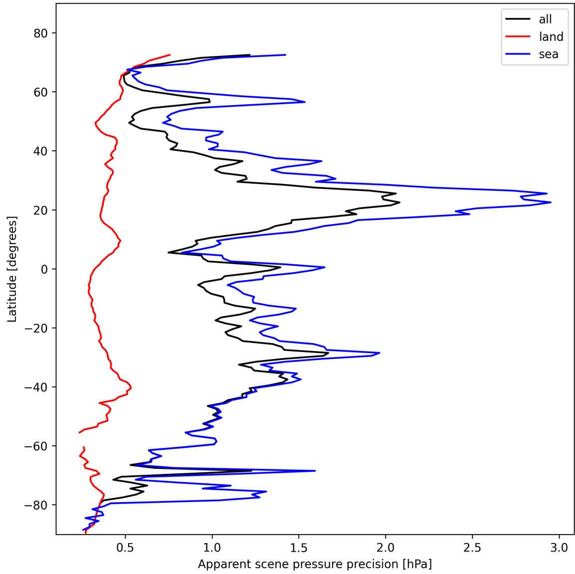
Figure 20: Zonal average of “Apparent scene pressure precision” for 2025-02-05 to 2025-02-07.
