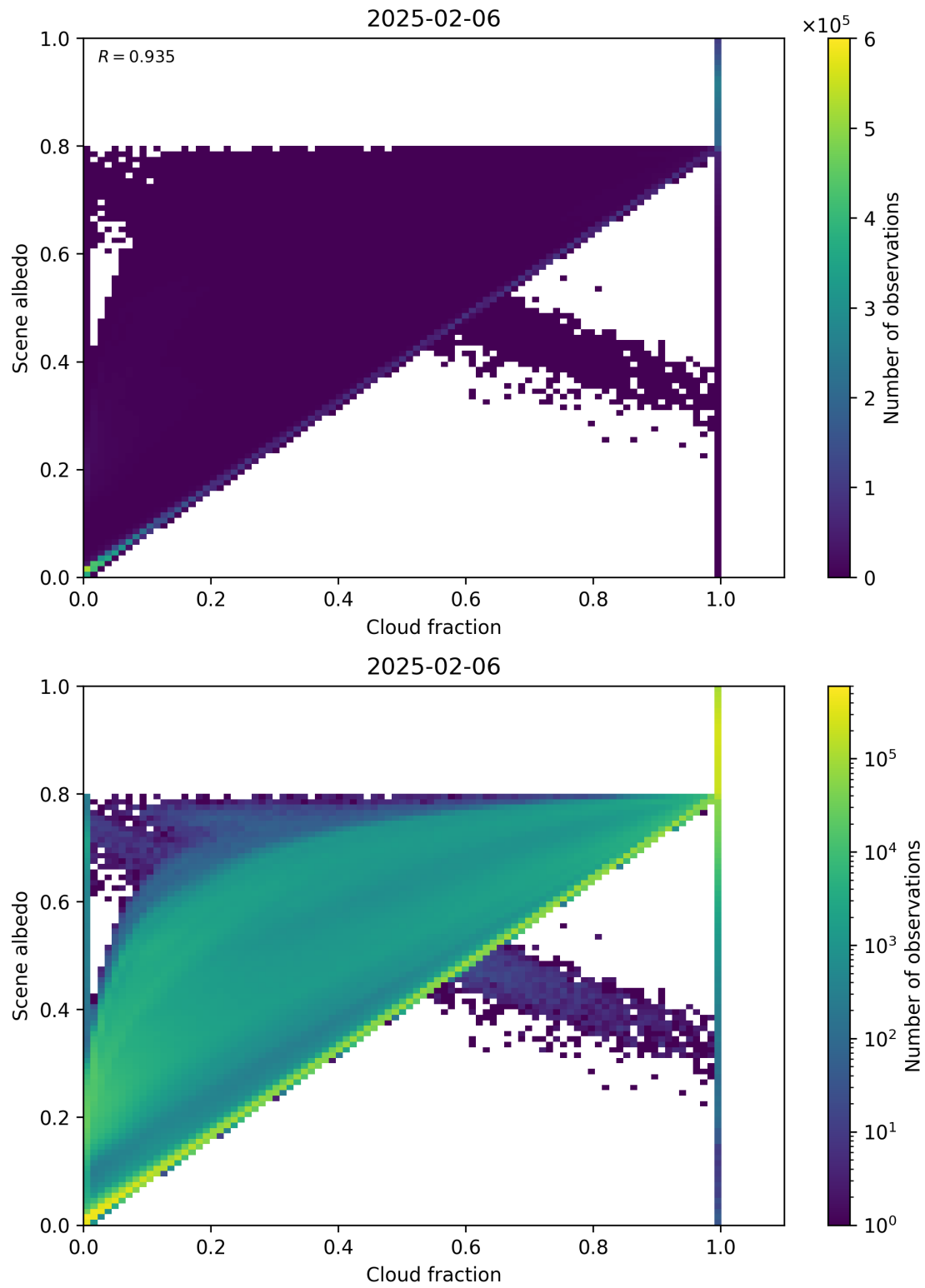
Figure 75: Scatter density plot of “Cloud fraction” against “Scene albedo” for 2025-02-05 to 2025-02-07.
