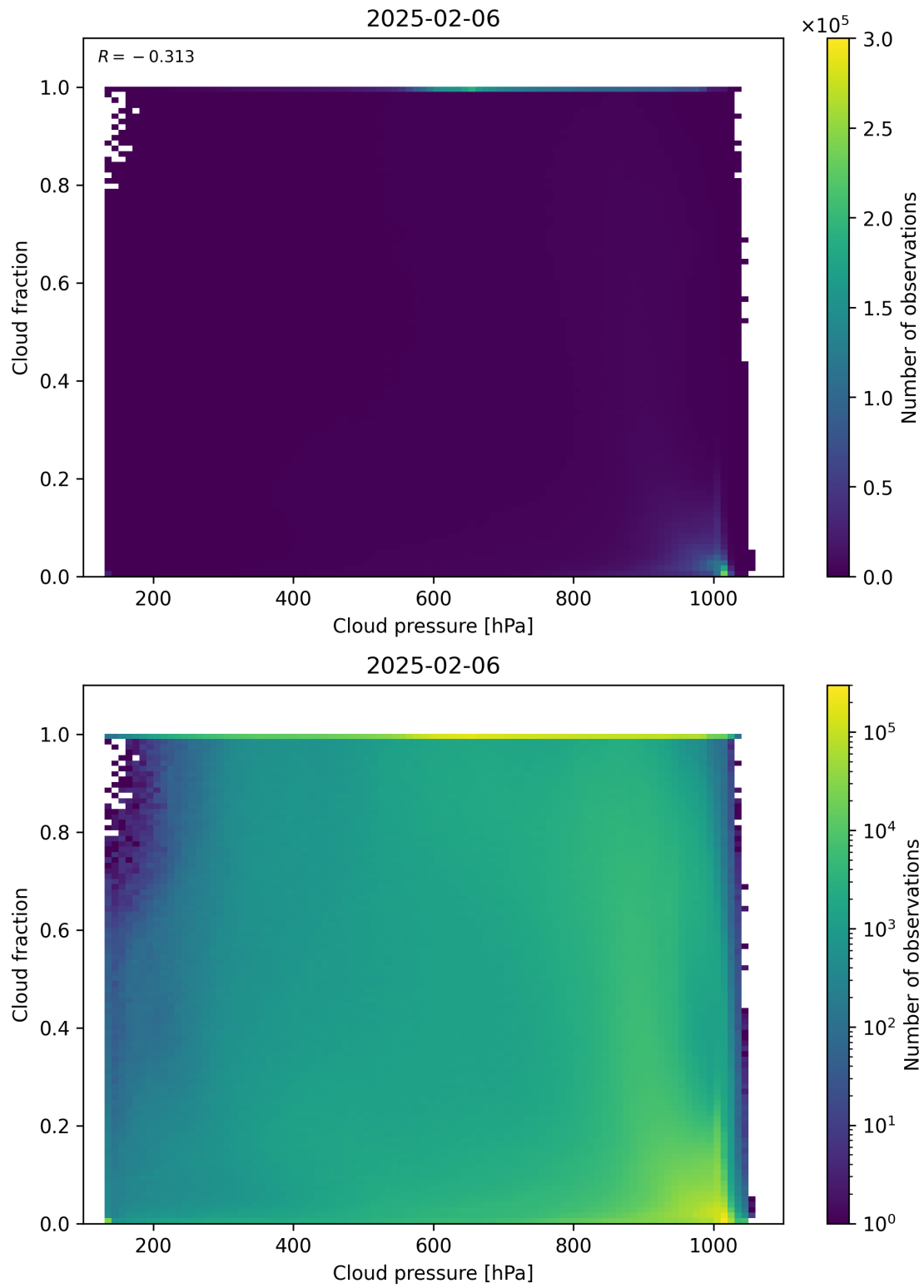
Figure 79: Scatter density plot of “Cloud pressure” against “Cloud fraction” for 2025-02-05 to 2025-02-07.
