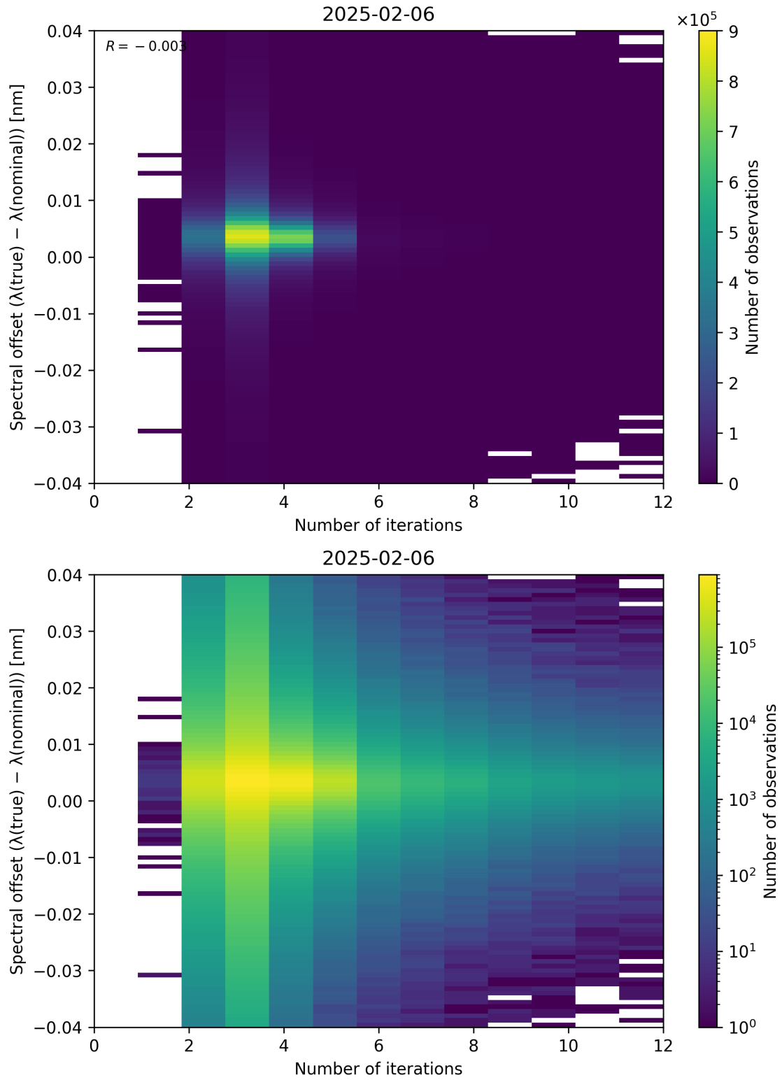
Figure 100: Scatter density plot of “Number of iterations” against “Spectral offset ( \lambda_{\text{true}} - \lambda_{\text{nominal}} )” for 2025-02-05 to 2025-02-07.
