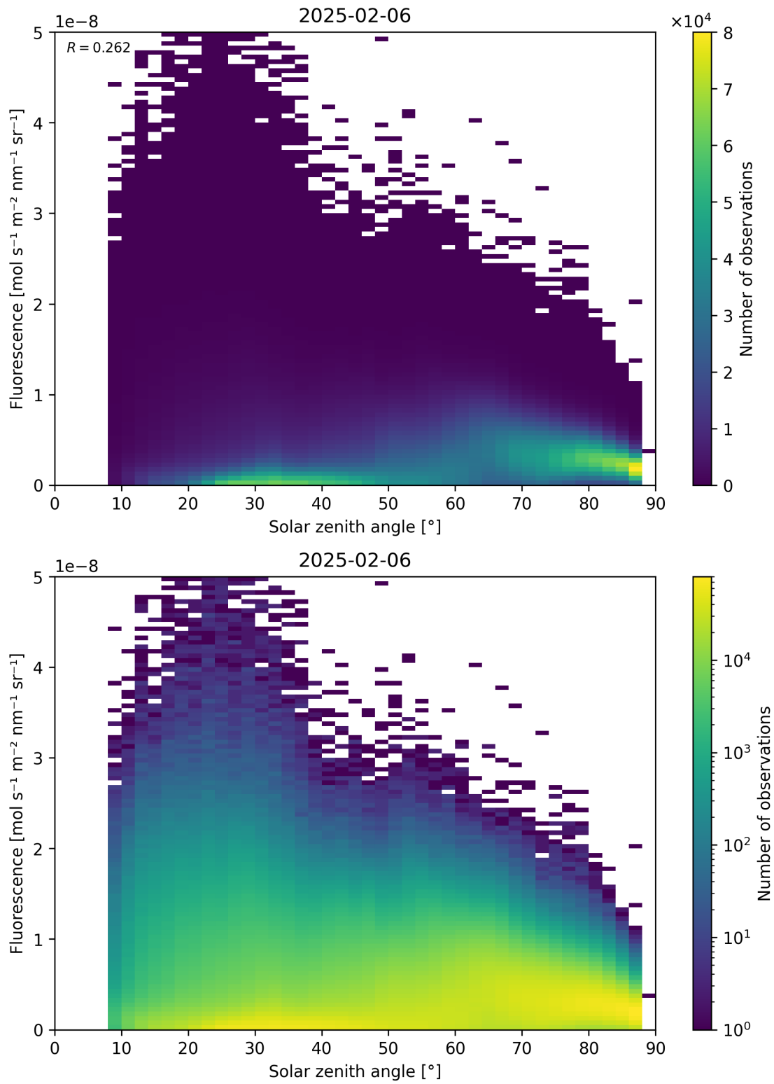
Figure 112: Scatter density plot of “Solar zenith angle” against “Fluorescence” for 2025-02-05 to 2025-02-07.
