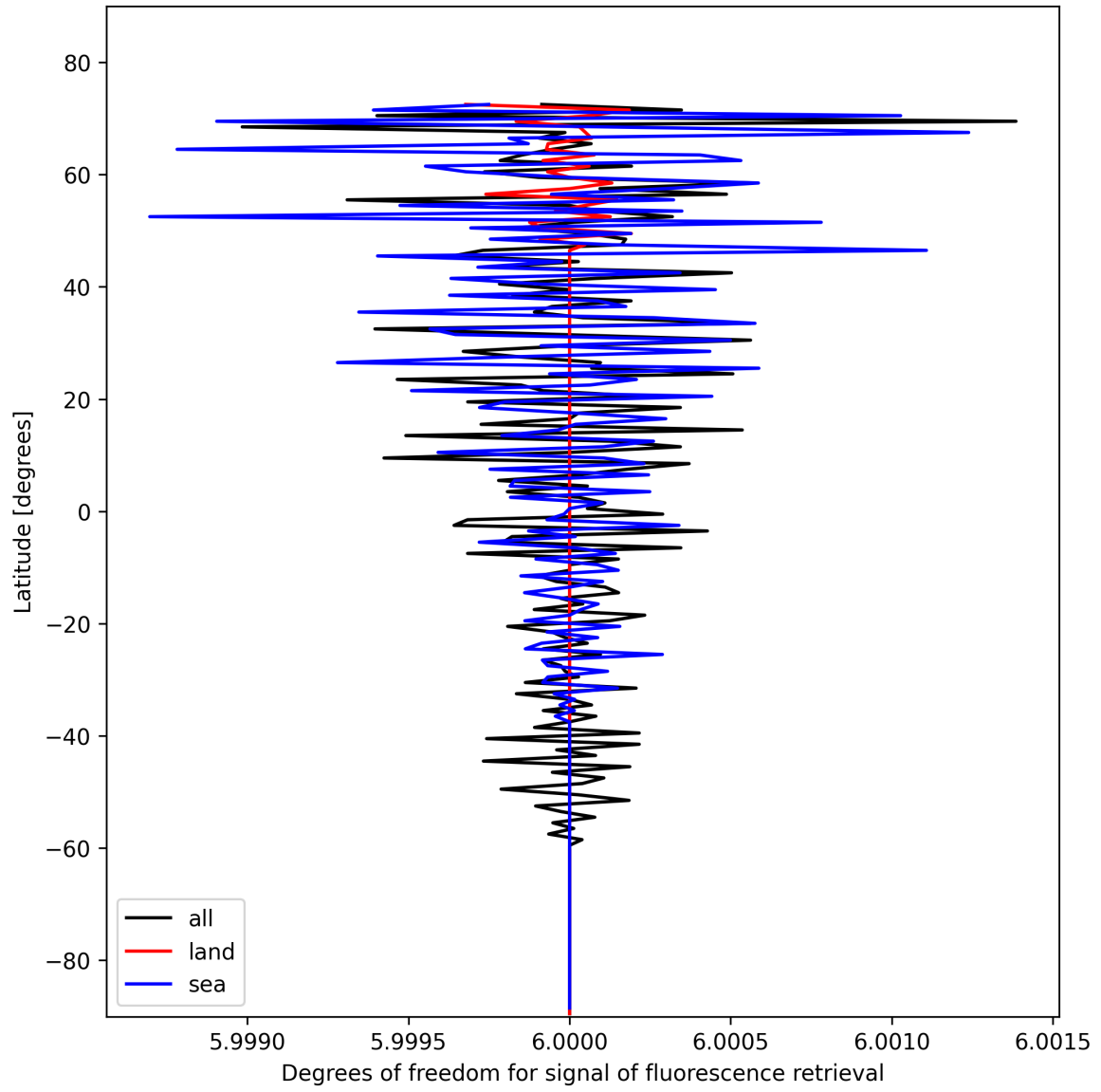
Figure 26: Zonal average of “Degrees of freedom for signal of fluorescence retrieval” for 2025-02-05 to 2025-02-07.
