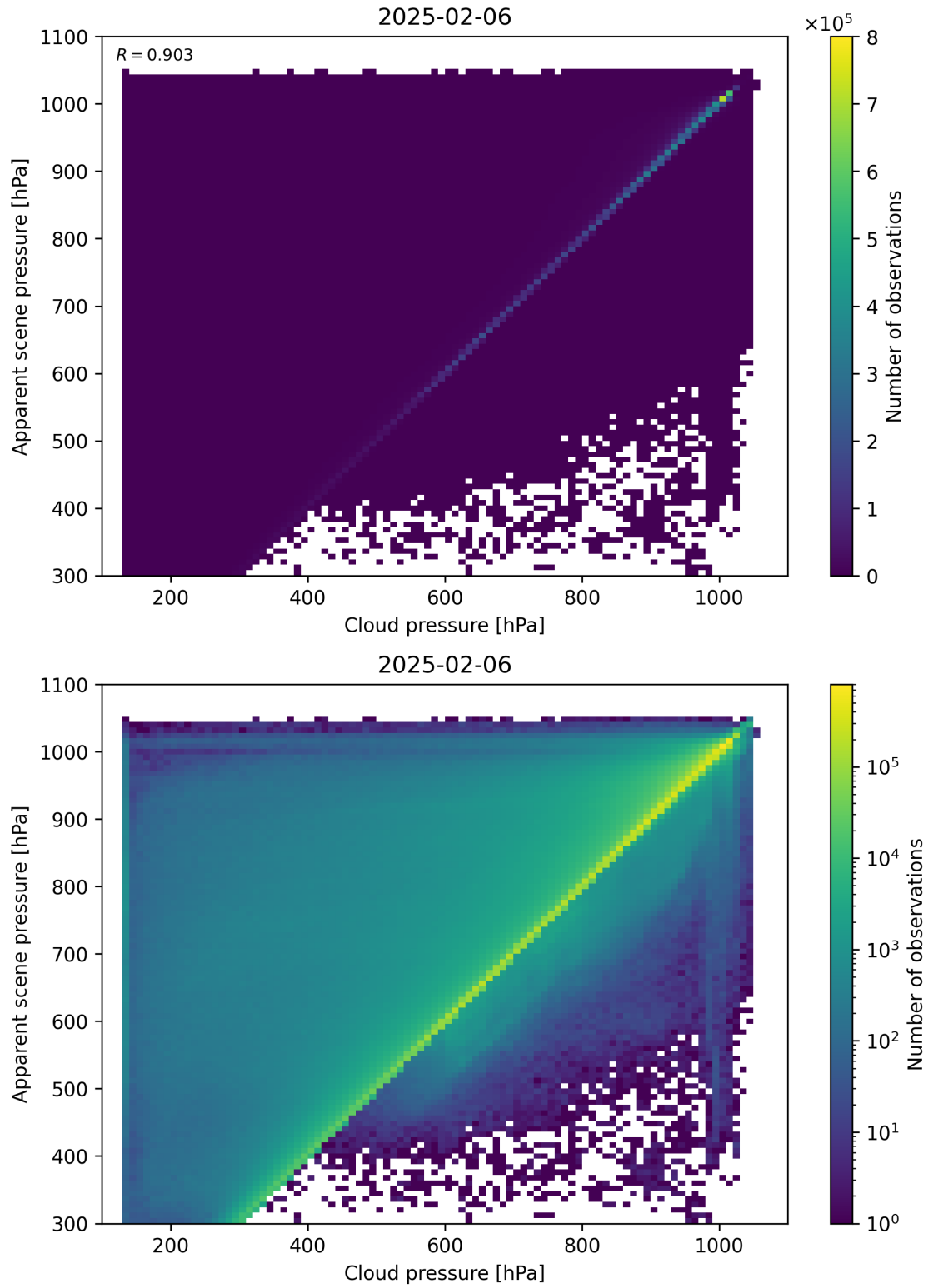
Figure 77: Scatter density plot of “Cloud pressure” against “Apparent scene pressure” for 2025-02-05 to 2025-02-07.
