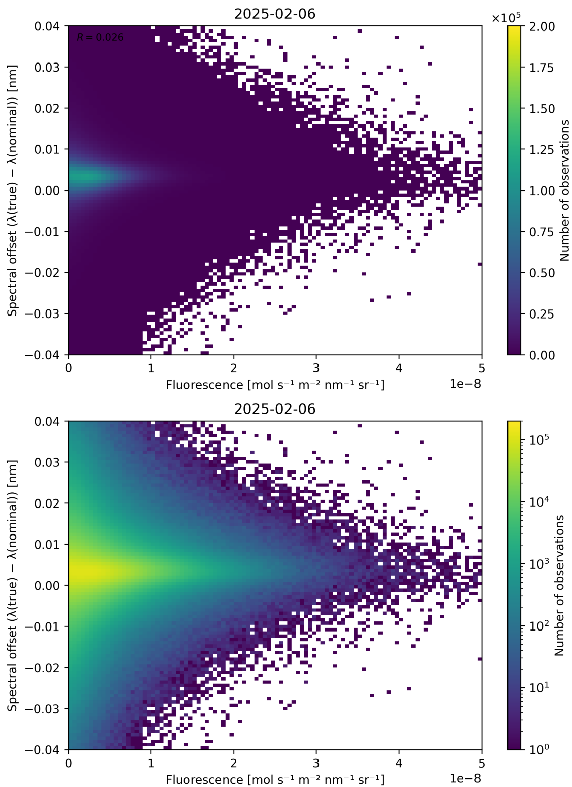
Figure 87: Scatter density plot of “Fluorescence” against “Spectral offset ( \lambda_{\text{true}} - \lambda_{\text{nominal}} )” for 2025-02-05 to 2025-02-07.
