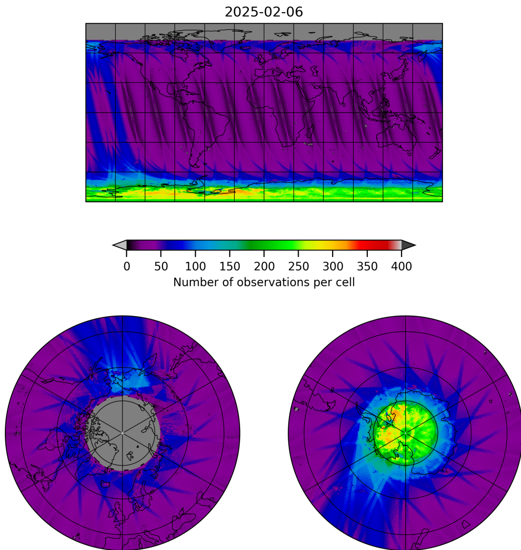
Figure 11: Map of the number of observations for 2025-02-05 to 2025-02-07
