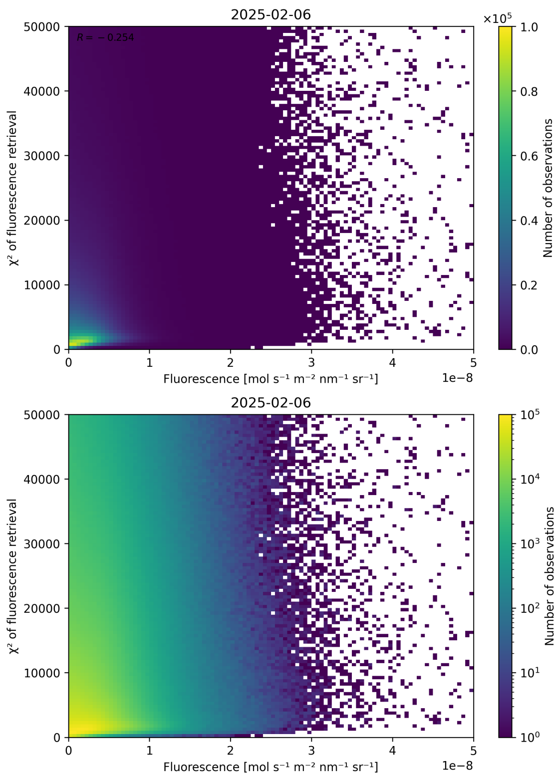
Figure 85: Scatter density plot of “Fluorescence” against “ \chi^2 of fluorescence retrieval” for 2025-02-05 to 2025-02-07.
