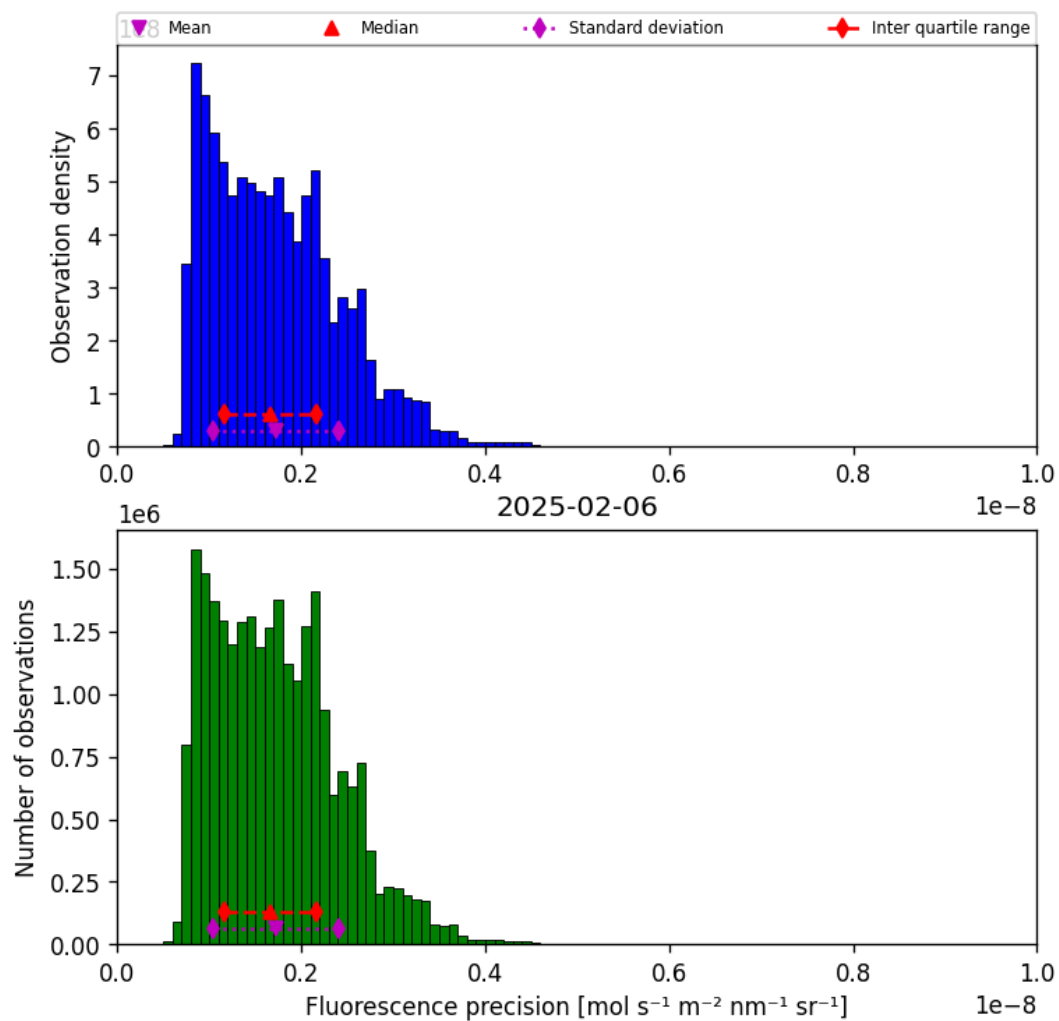
Figure 41: Histogram of “Fluorescence precision” for 2025-02-05 to 2025-02-07
