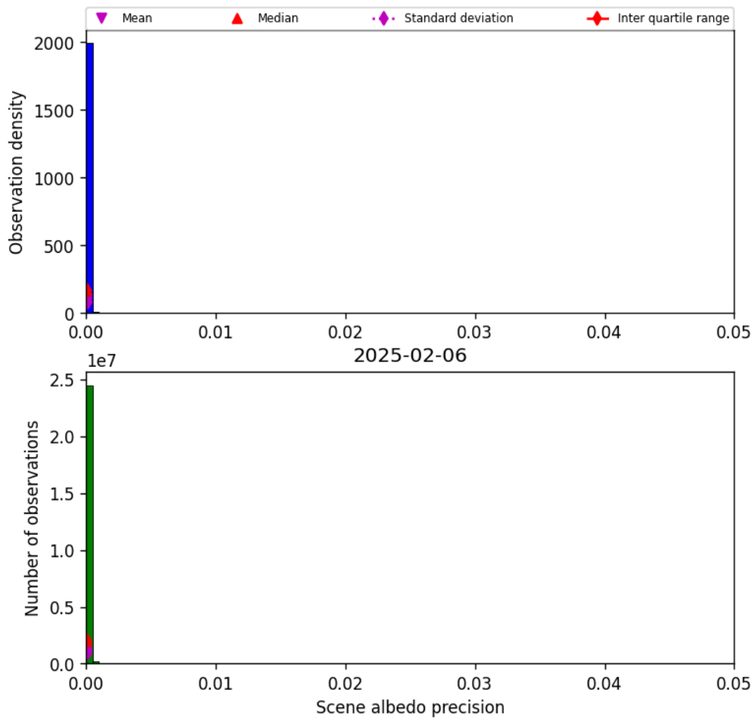
Figure 35: Histogram of “Scene albedo precision” for 2025-02-05 to 2025-02-07
