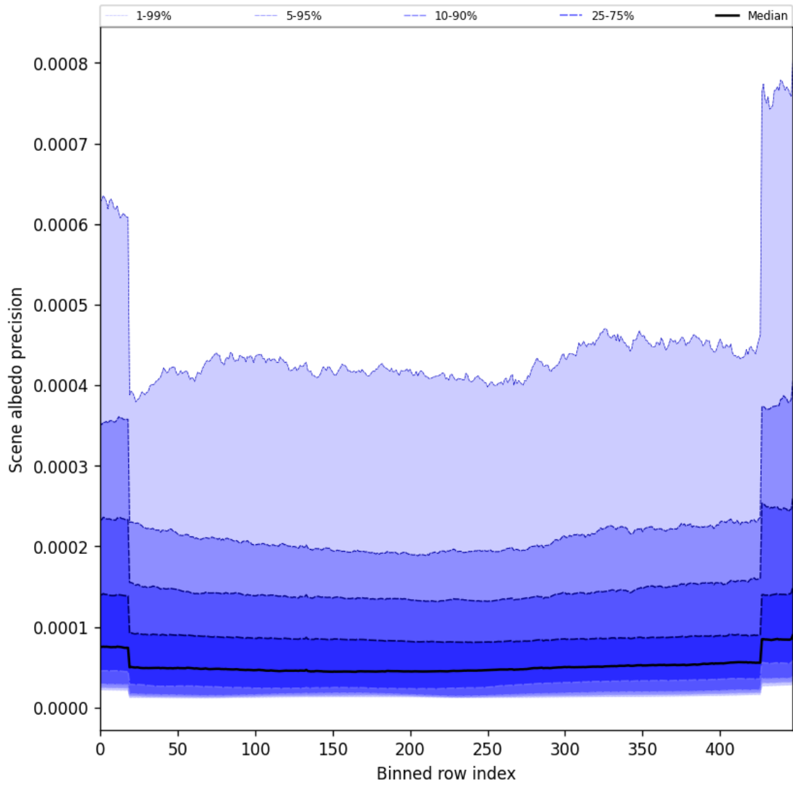
Figure 52: Along track statistics of “Scene albedo precision” for 2025-02-05 to 2025-02-07
