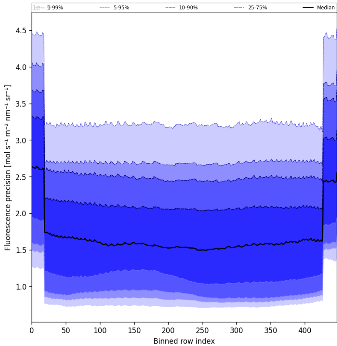
Figure 58: Along track statistics of “Fluorescence precision” for 2025-02-05 to 2025-02-07
