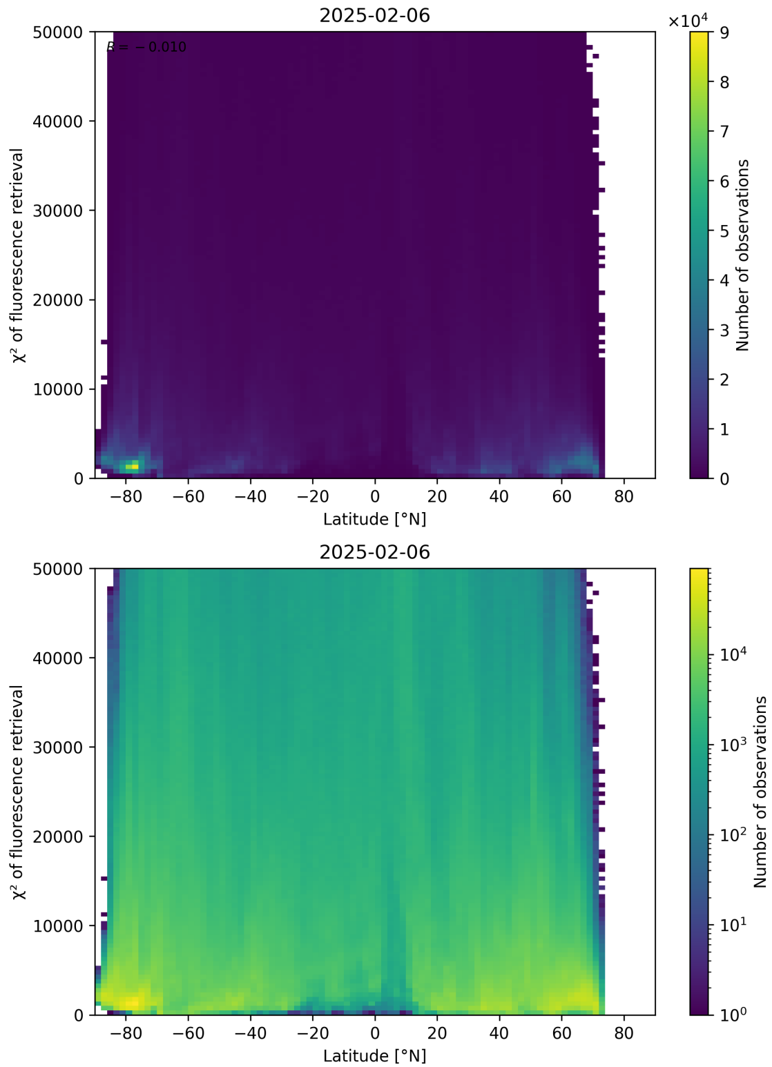
Figure 89: Scatter density plot of “Latitude” against “ \chi^2 of fluorescence retrieval” for 2025-02-05 to 2025-02-07.
