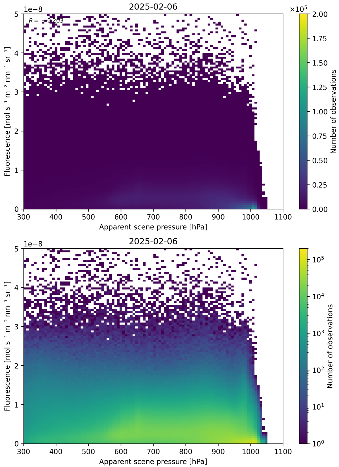
Figure 64: Scatter density plot of “Apparent scene pressure” against “Fluorescence” for 2025-02-05 to 2025-02-07.
