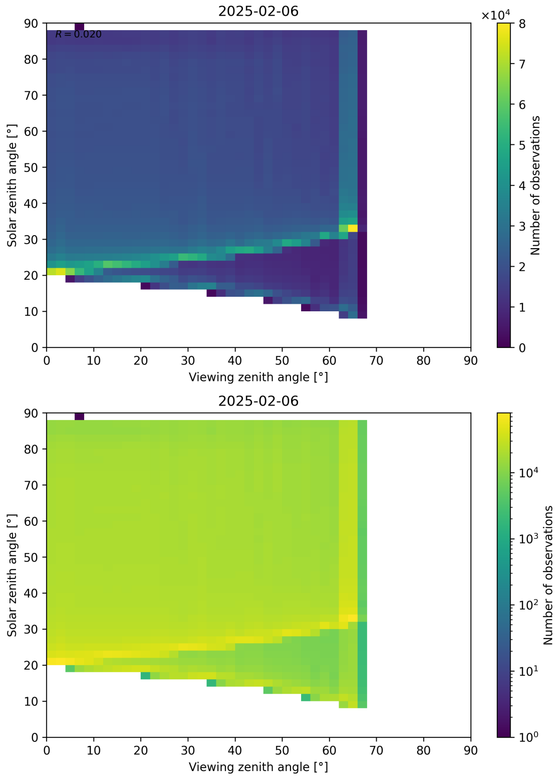
Figure 127: Scatter density plot of “Viewing zenith angle” against “Solar zenith angle” for 2025-02-05 to 2025-02-07.
