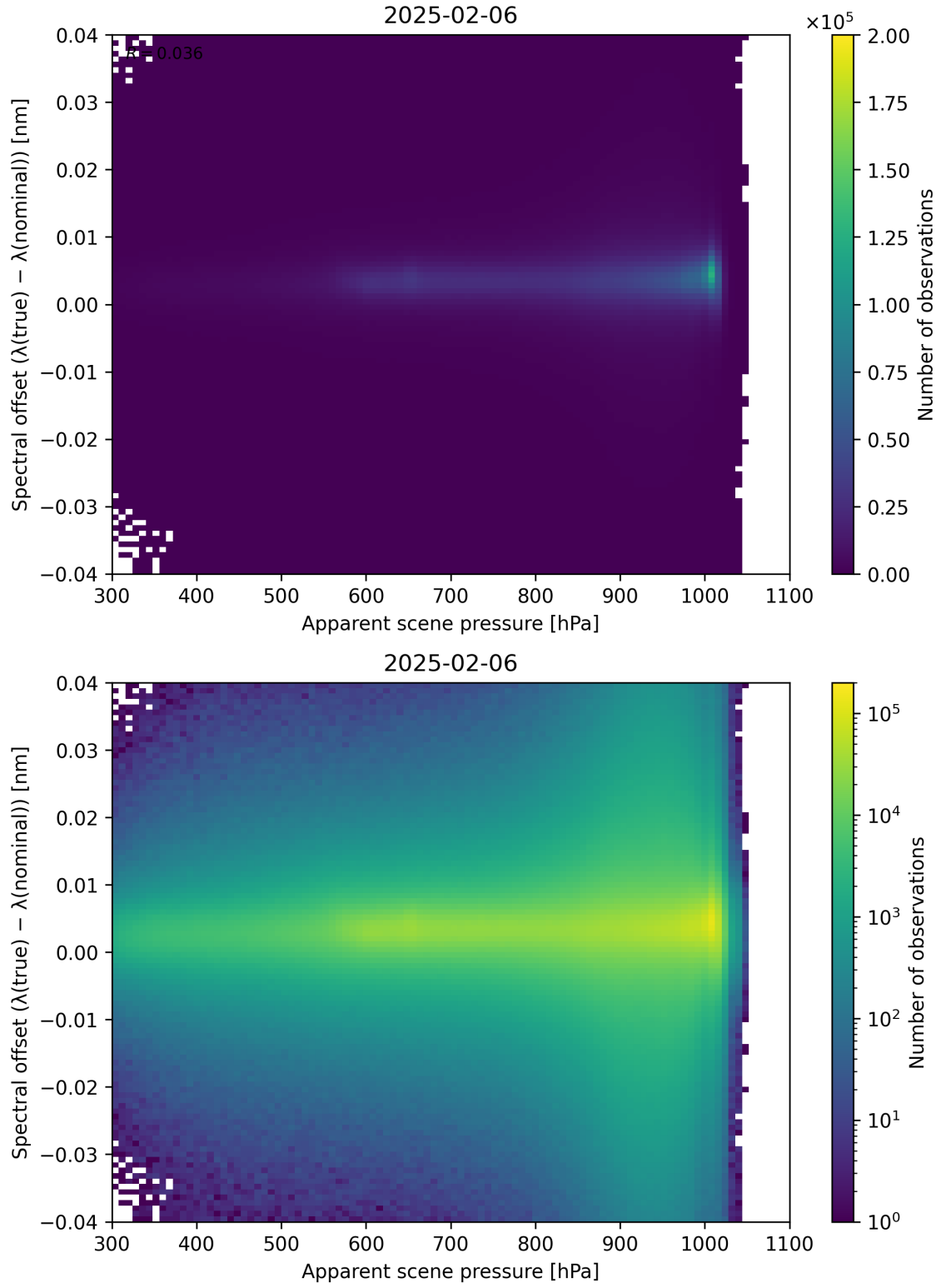
Figure 67: Scatter density plot of “Apparent scene pressure” against “Spectral offset ( \lambda_{\text{true}} - \lambda_{\text{nominal}} )” for 2025-02-05 to 2025-02-07.
