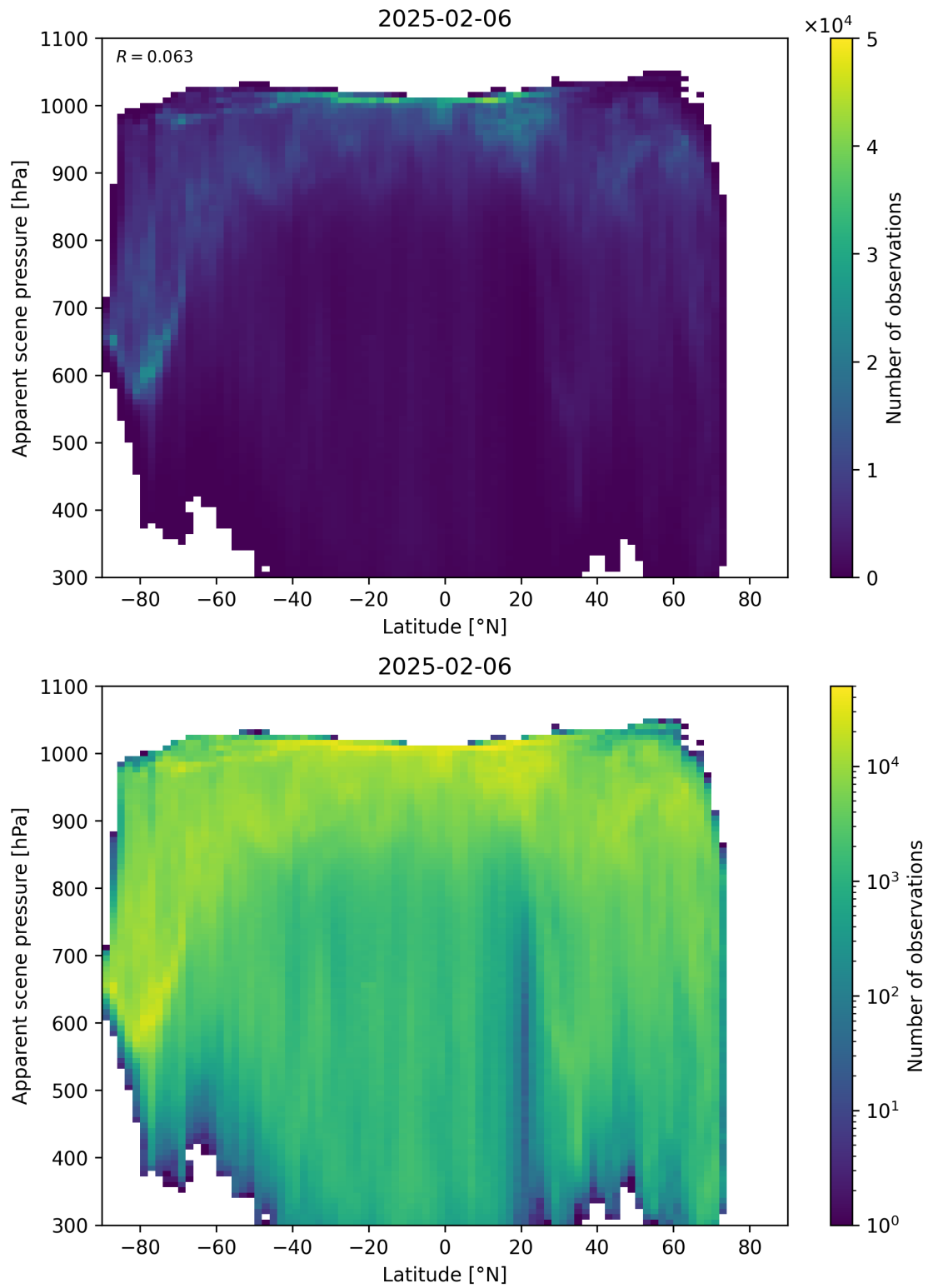
Figure 88: Scatter density plot of “Latitude” against “Apparent scene pressure” for 2025-02-05 to 2025-02-07.
