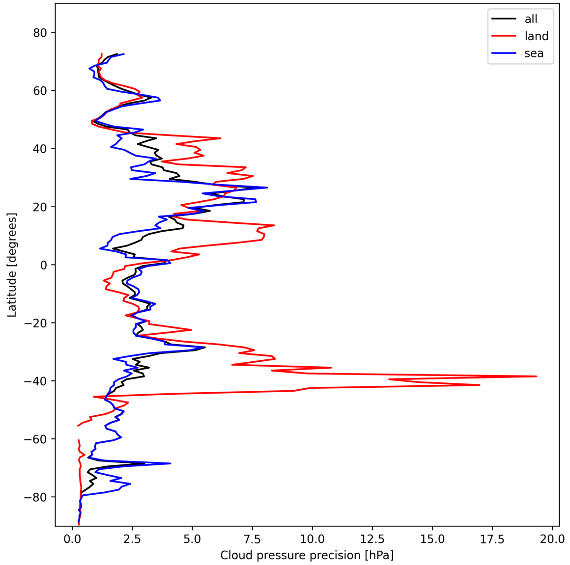
Figure 14: Zonal average of “Cloud pressure precision” for 2025-02-05 to 2025-02-07.
