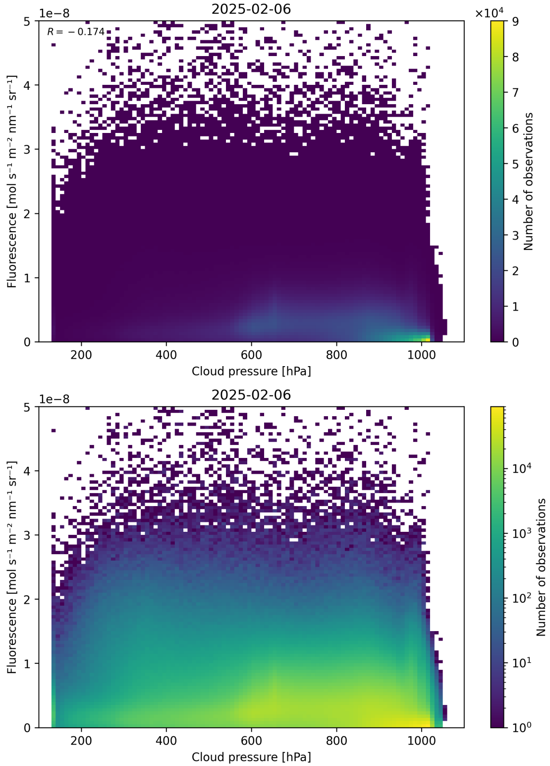
Figure 80: Scatter density plot of “Cloud pressure” against “Fluorescence” for 2025-02-05 to 2025-02-07.
