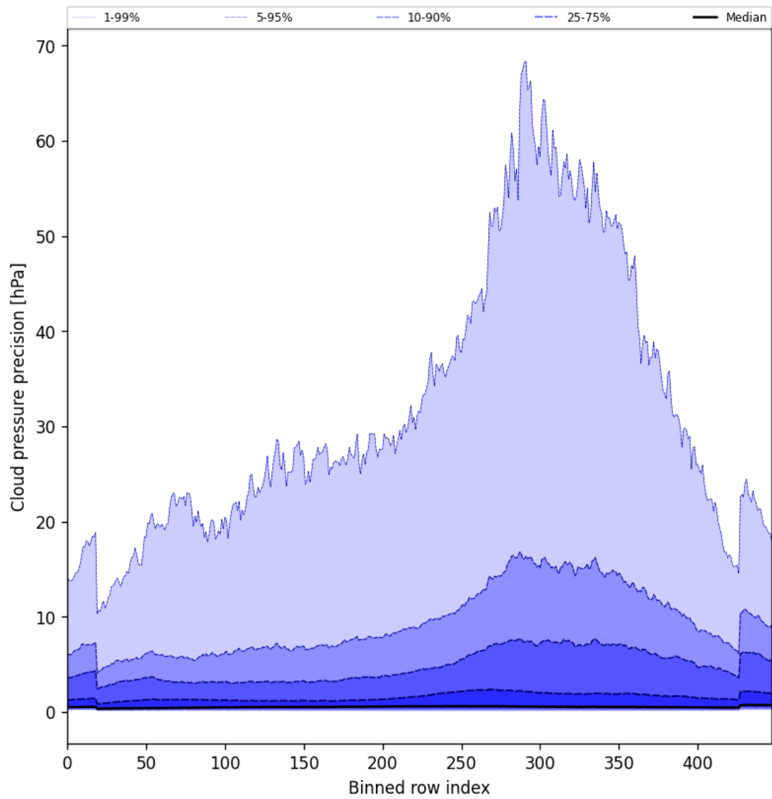
Figure 48: Along track statistics of “Cloud pressure precision” for 2025-02-05 to 2025-02-07
