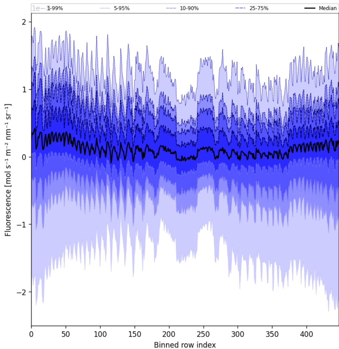
Figure 57: Along track statistics of “Fluorescence” for 2025-02-06 to 2025-02-08
