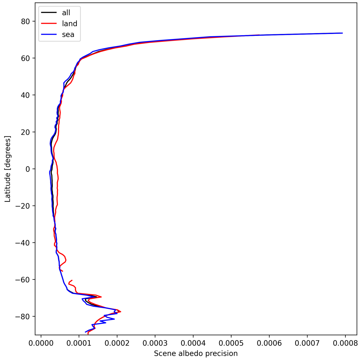
Figure 18: Zonal average of “Scene albedo precision” for 2025-02-06 to 2025-02-08.
