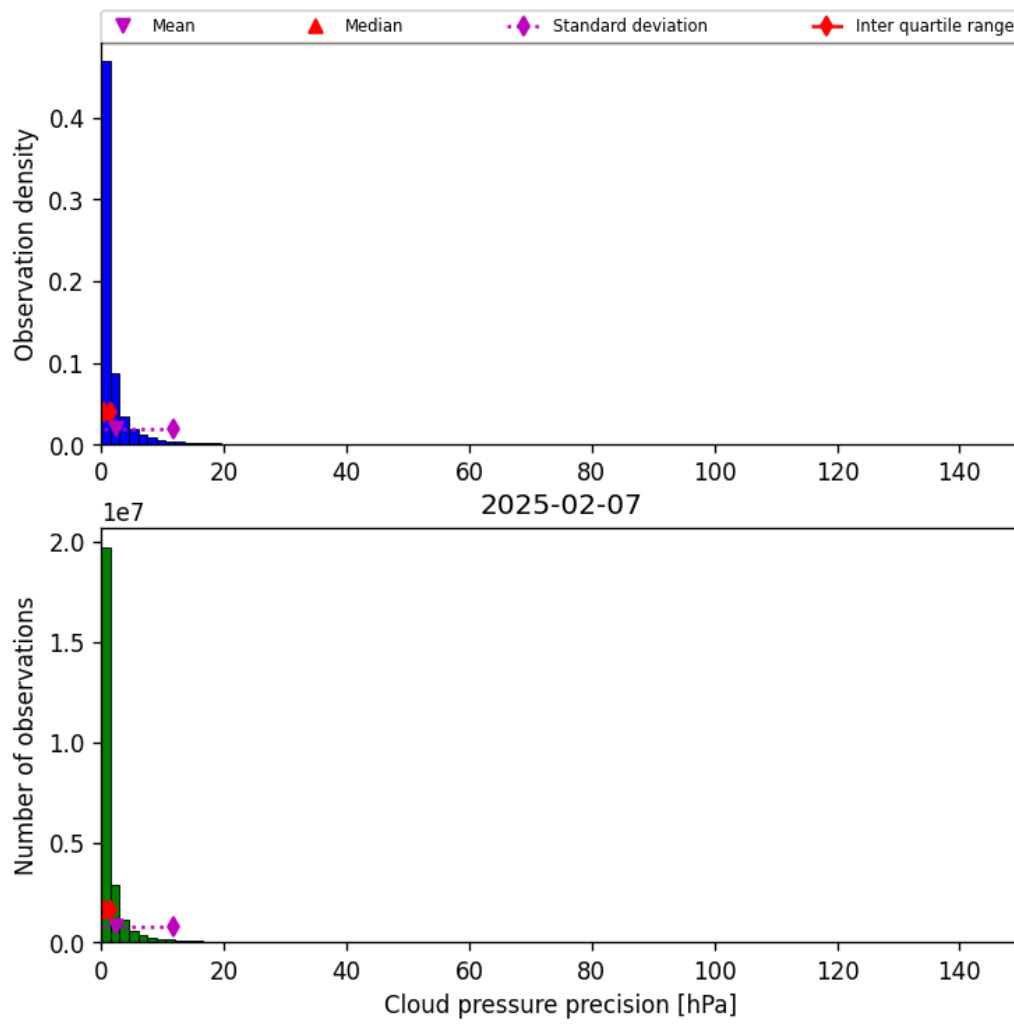
Figure 31: Histogram of “Cloud pressure precision” for 2025-02-06 to 2025-02-08
