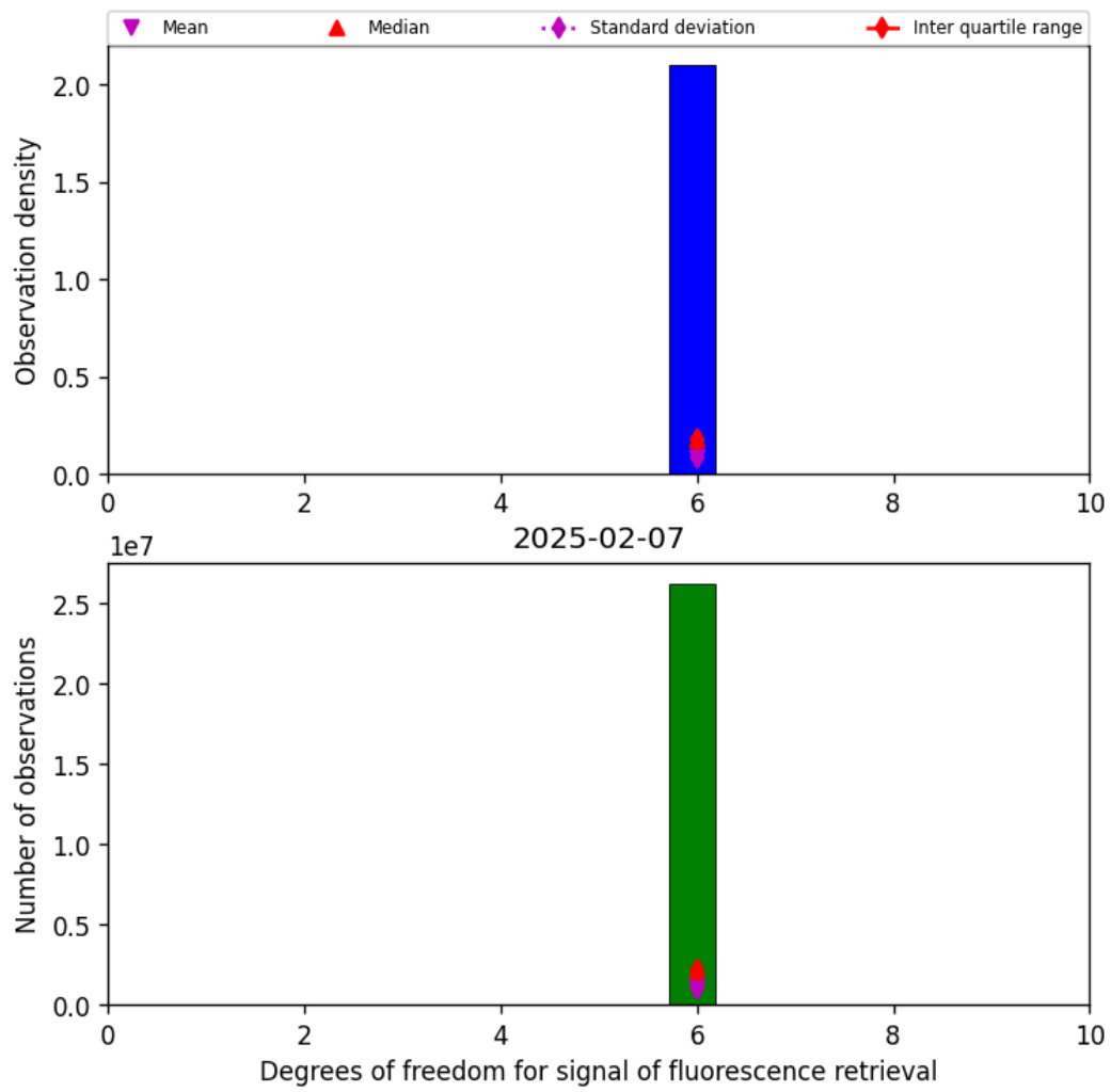
Figure 43: Histogram of "Degrees of freedom for signal of fluorescence retrieval" for 2025-02-06 to 2025-02-08
