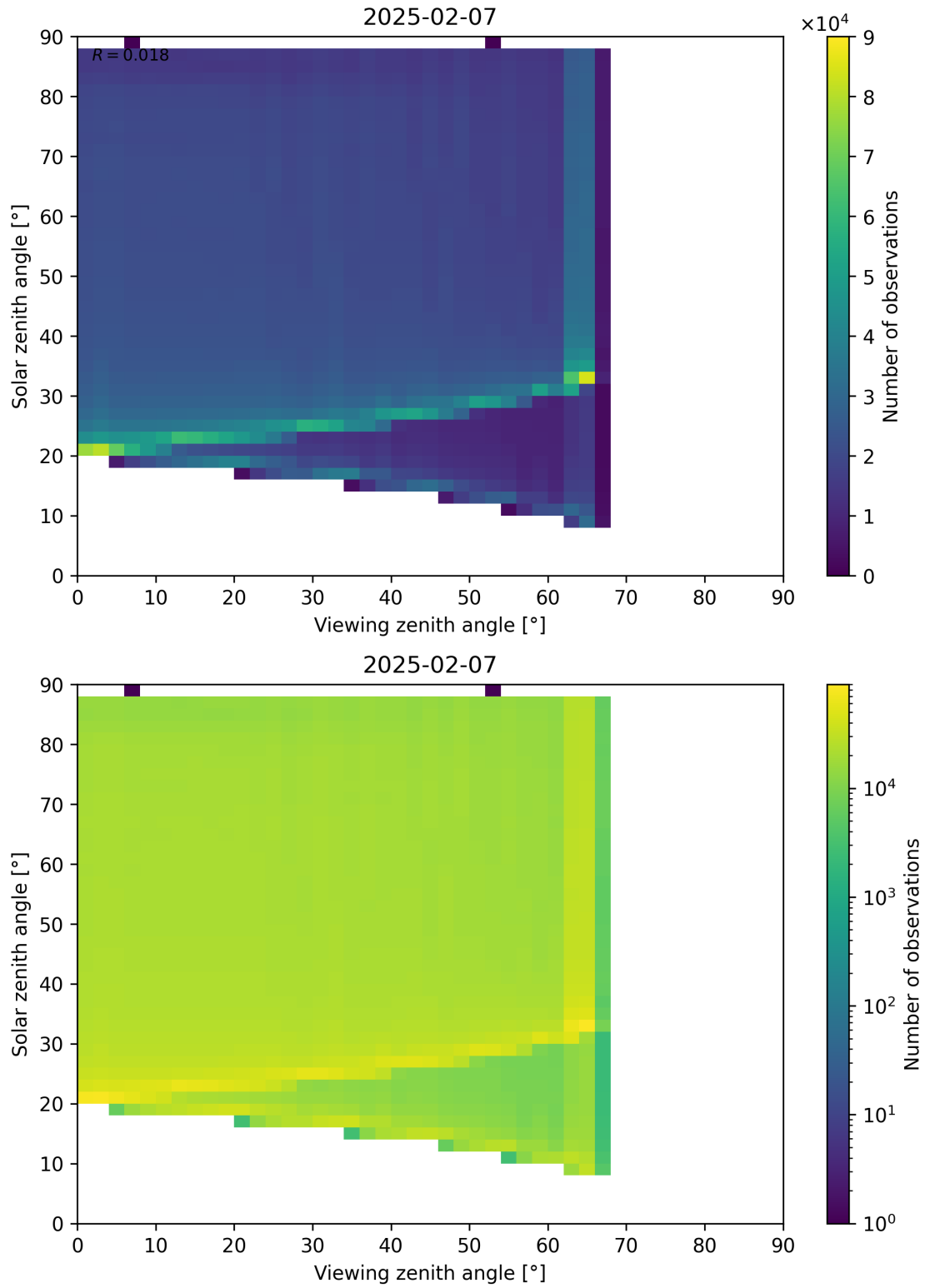
Figure 127: Scatter density plot of “Viewing zenith angle” against “Solar zenith angle” for 2025-02-06 to 2025-02-08.
