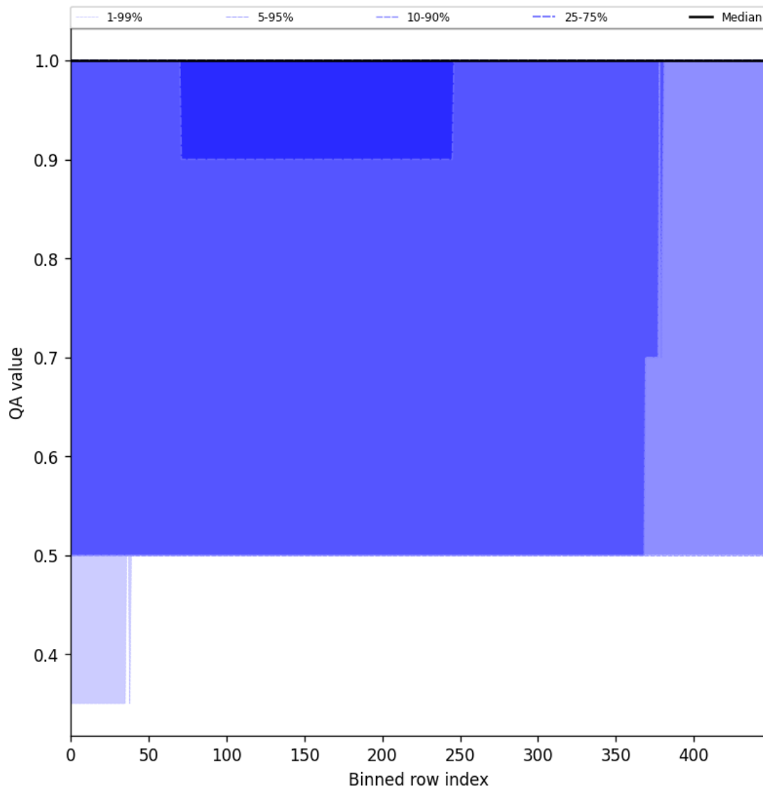
Figure 46: Along track statistics of “QA value” for 2025-02-06 to 2025-02-08
