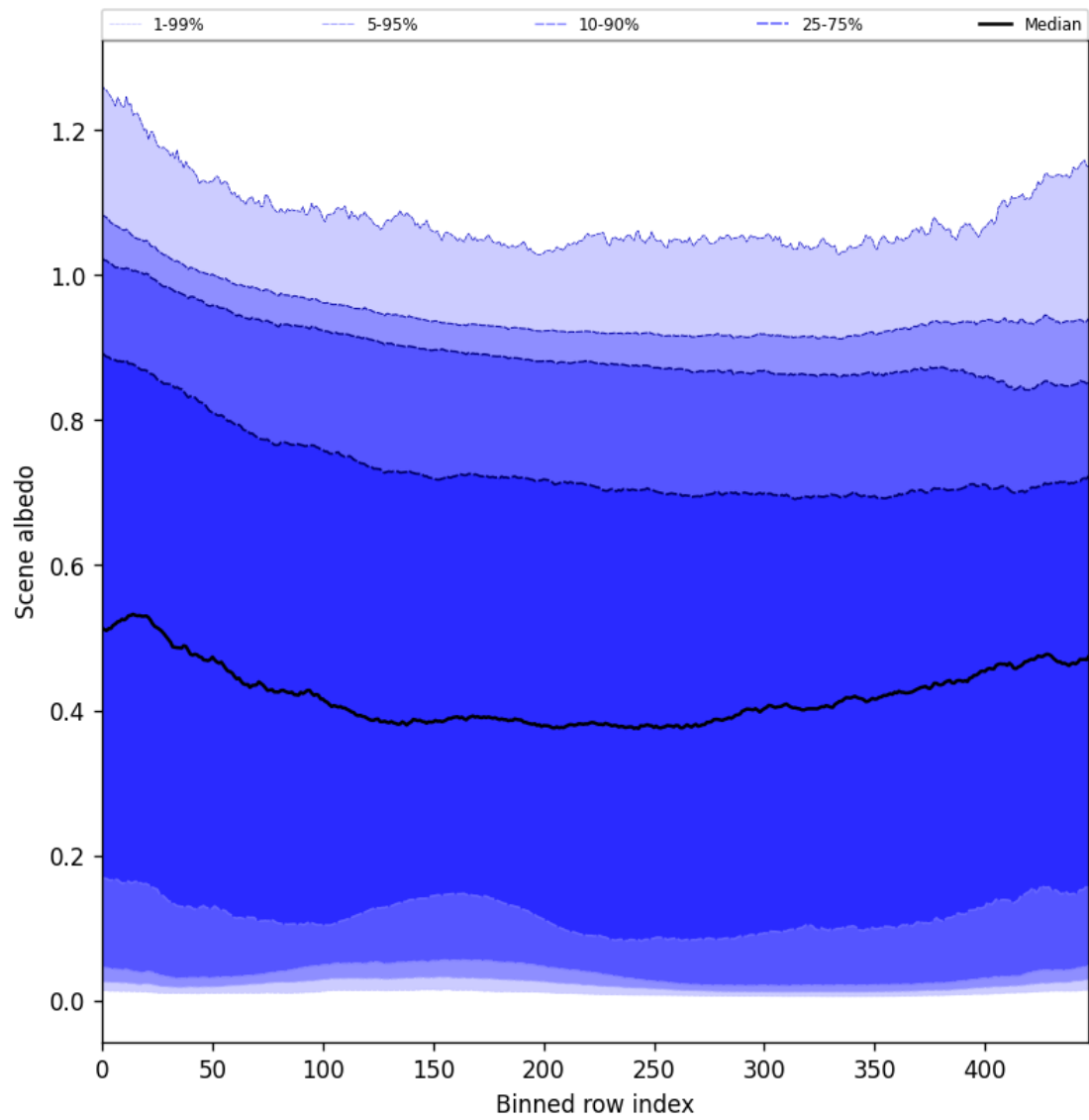
Figure 51: Along track statistics of “Scene albedo” for 2025-02-06 to 2025-02-08
