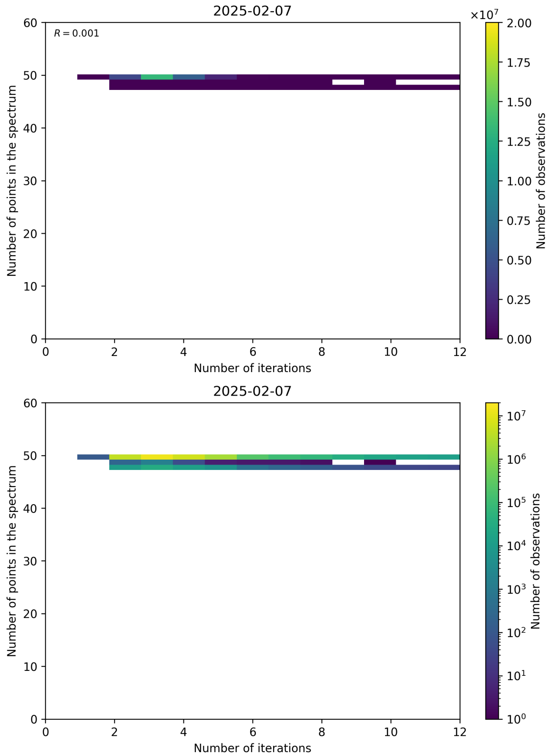
Figure 99: Scatter density plot of “Number of iterations” against “Number of points in the spectrum” for 2025-02-06 to 2025-02-08.
