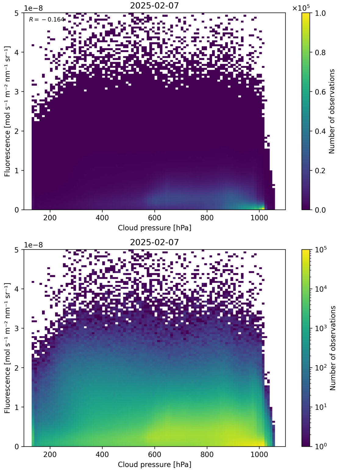
Figure 80: Scatter density plot of “Cloud pressure” against “Fluorescence” for 2025-02-06 to 2025-02-08.
