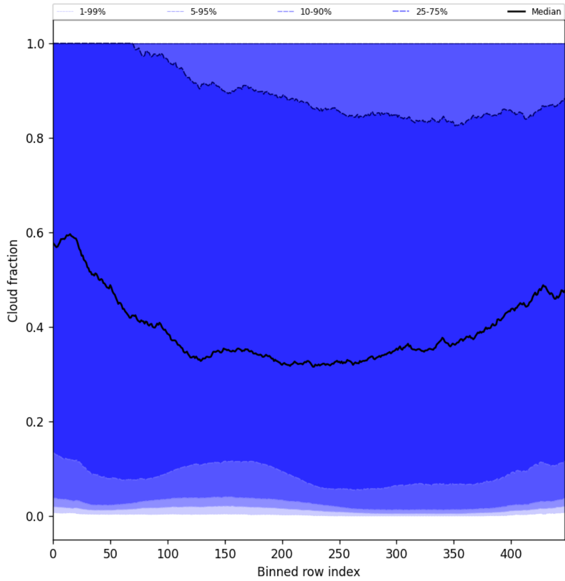
Figure 49: Along track statistics of “Cloud fraction” for 2025-02-06 to 2025-02-08
