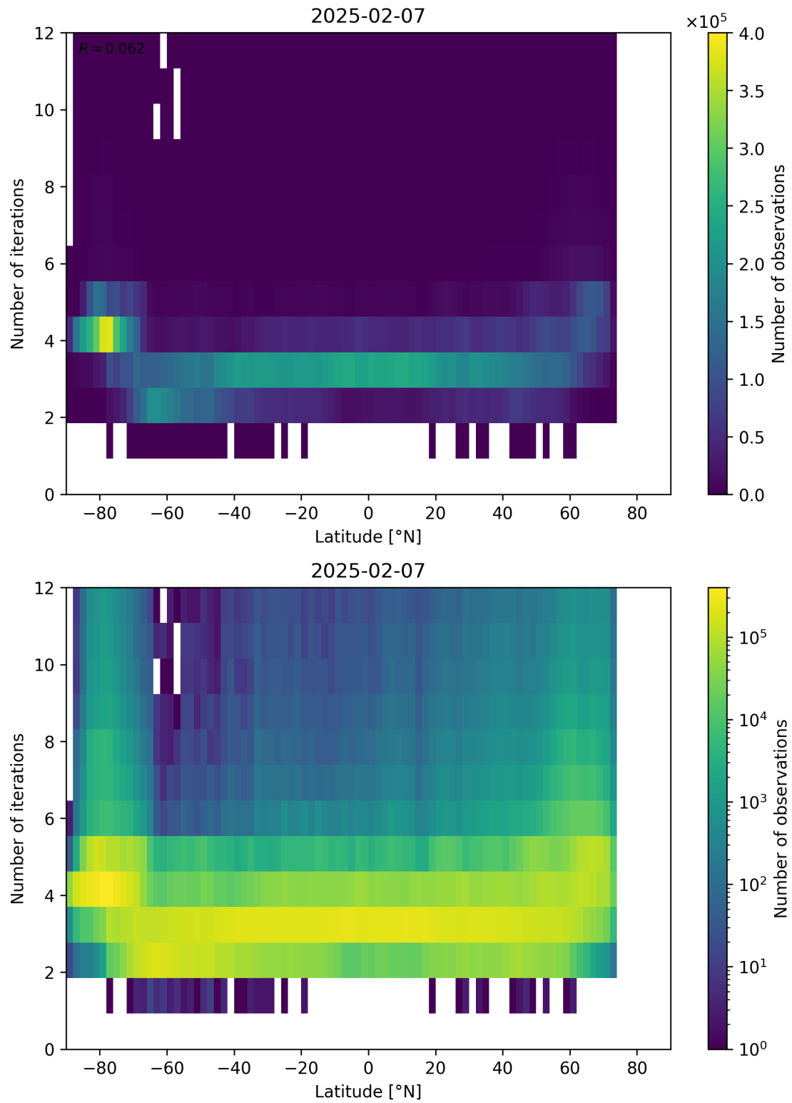
Figure 93: Scatter density plot of “Latitude” against “Number of iterations” for 2025-02-06 to 2025-02-08.
