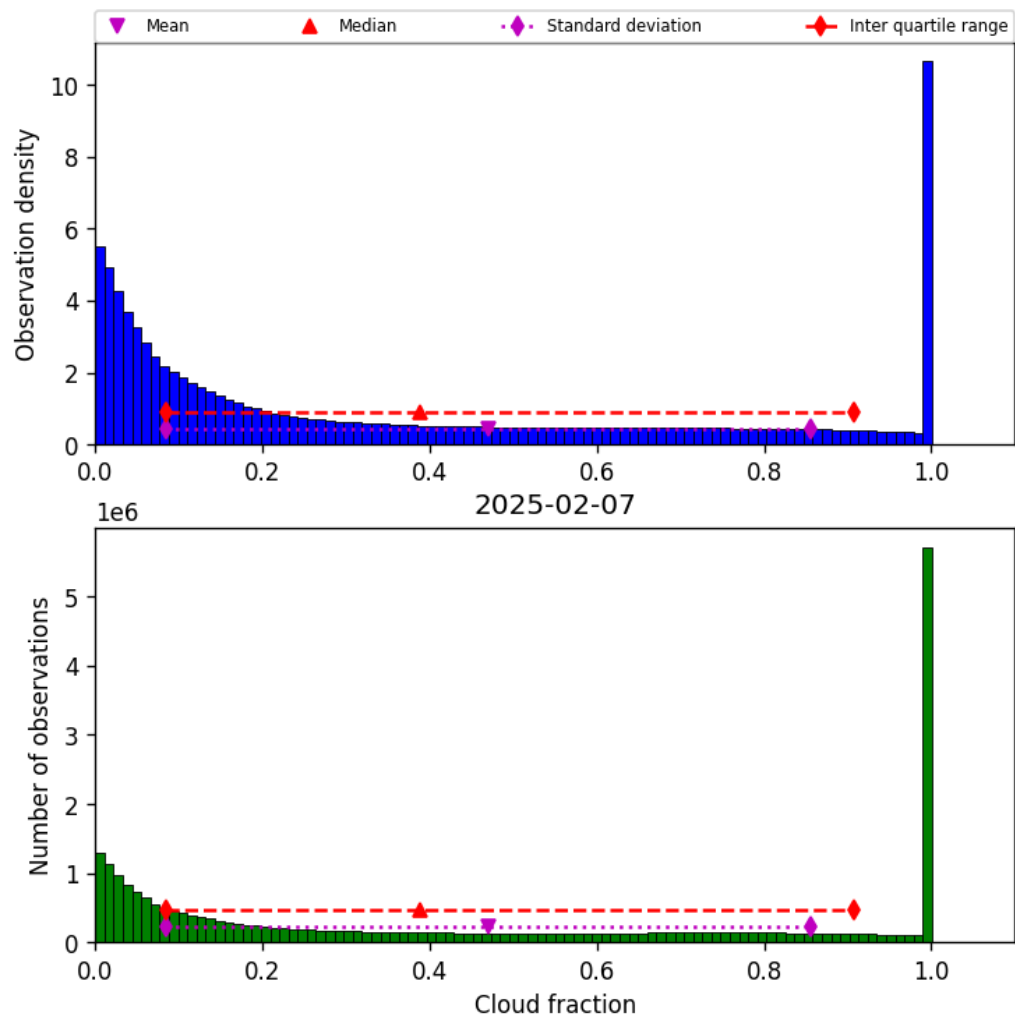
Figure 32: Histogram of “Cloud fraction” for 2025-02-06 to 2025-02-08
