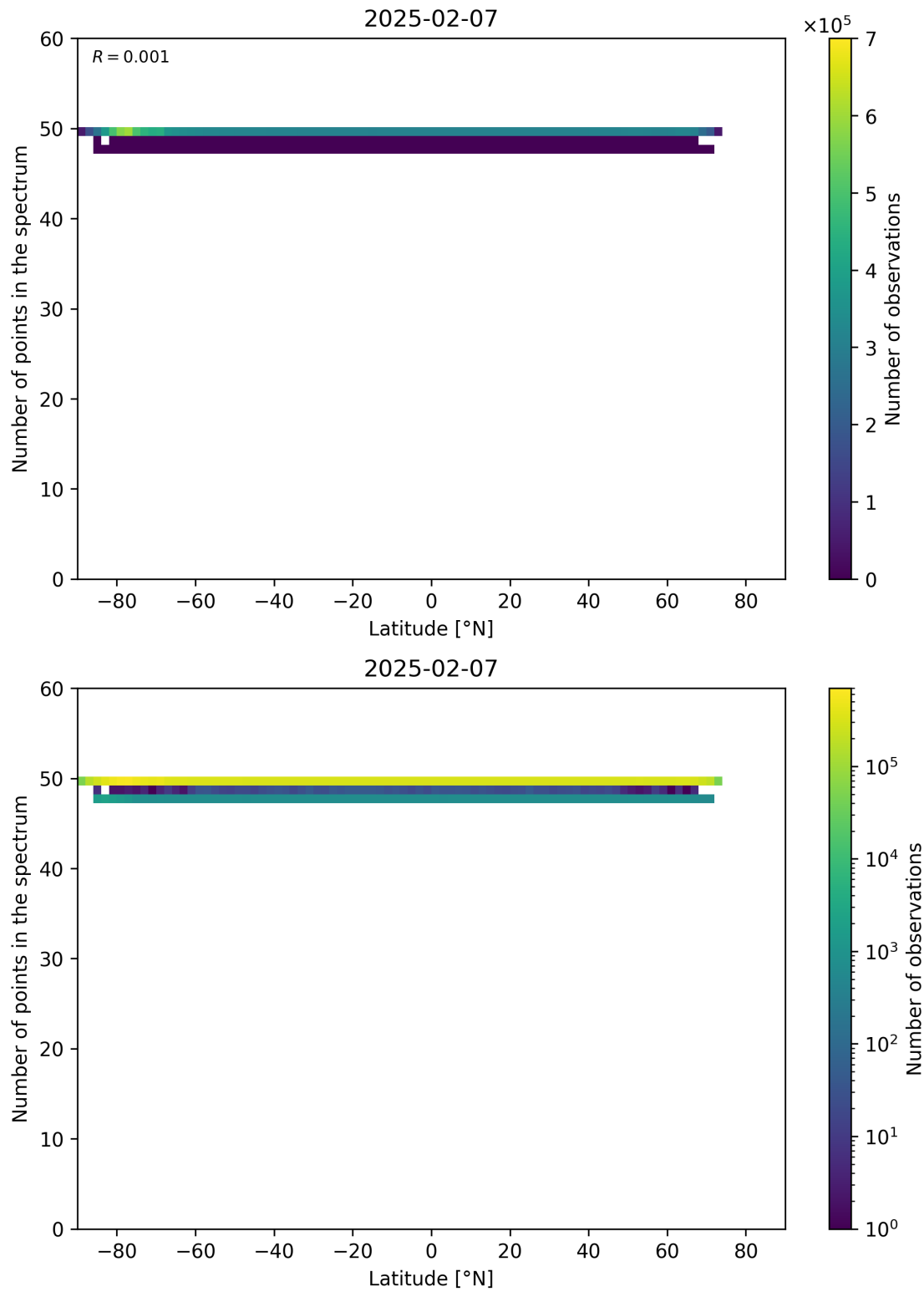
Figure 94: Scatter density plot of “Latitude” against “Number of points in the spectrum” for 2025-02-06 to 2025-02-08.
