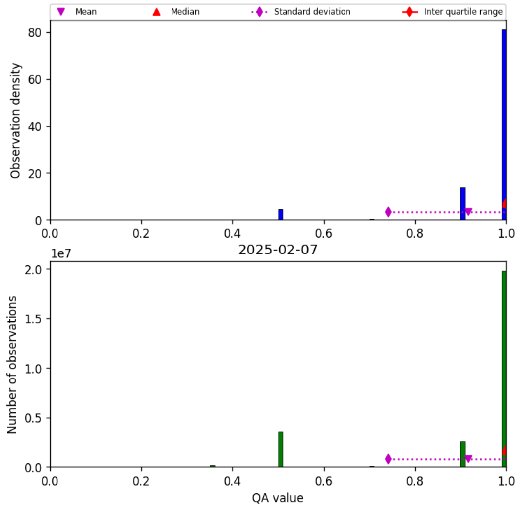
Figure 29: Histogram of “QA value” for 2025-02-06 to 2025-02-08
