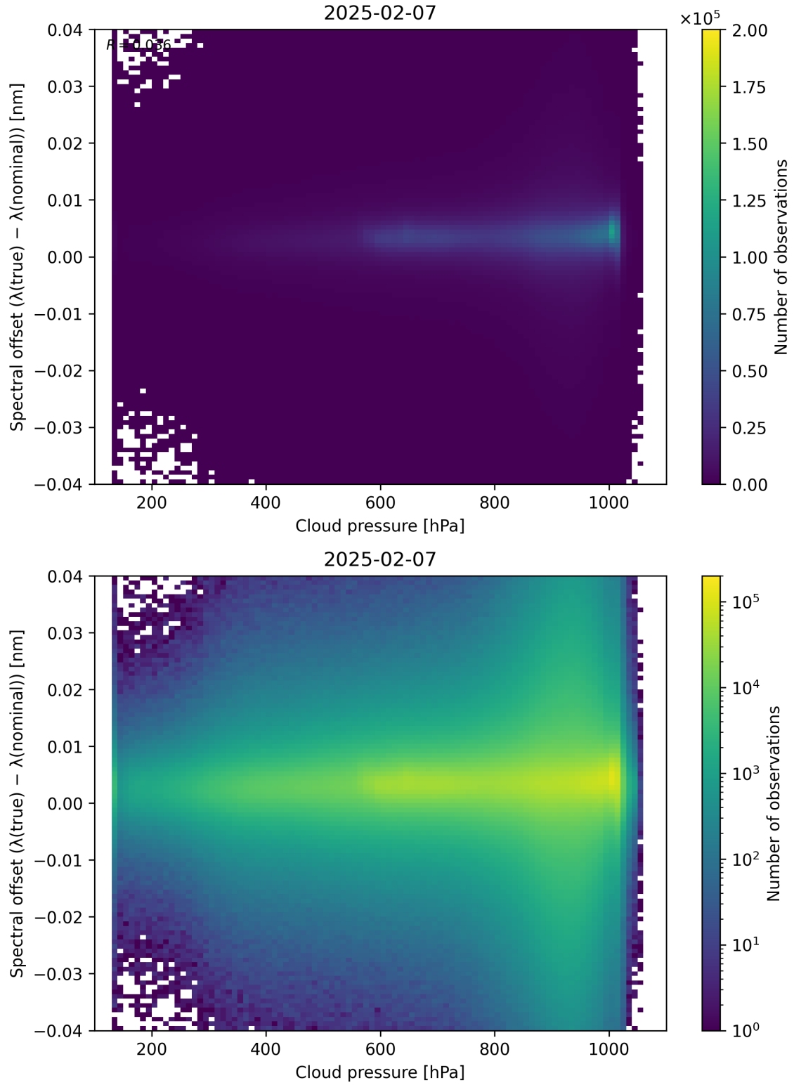
Figure 84: Scatter density plot of “Cloud pressure” against “Spectral offset ( \lambda_{\text{true}} - \lambda_{\text{nominal}} )” for 2025-02-06 to 2025-02-08.
