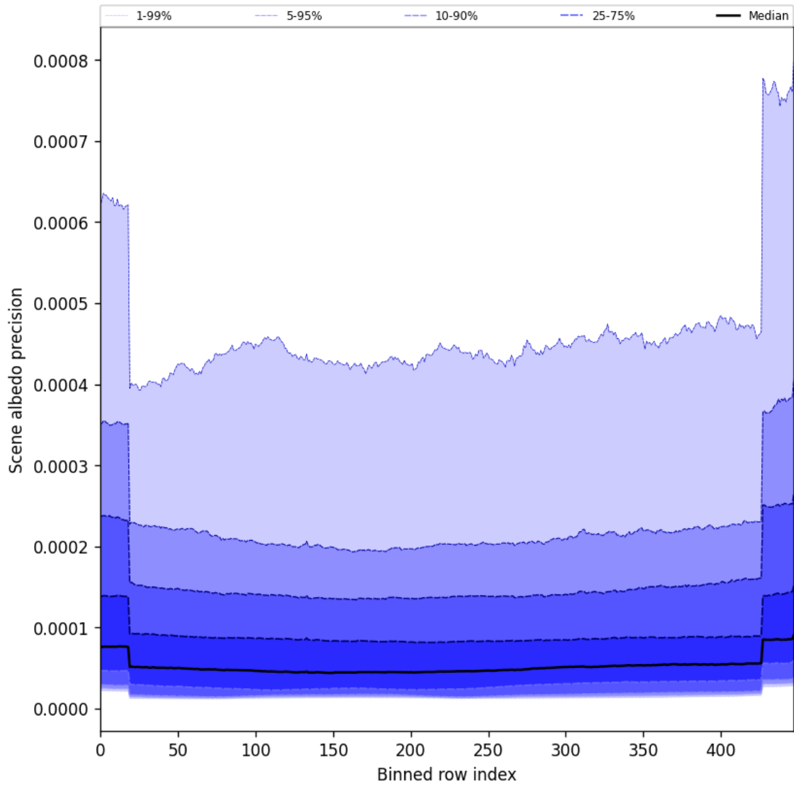
Figure 52: Along track statistics of “Scene albedo precision” for 2025-02-06 to 2025-02-08
