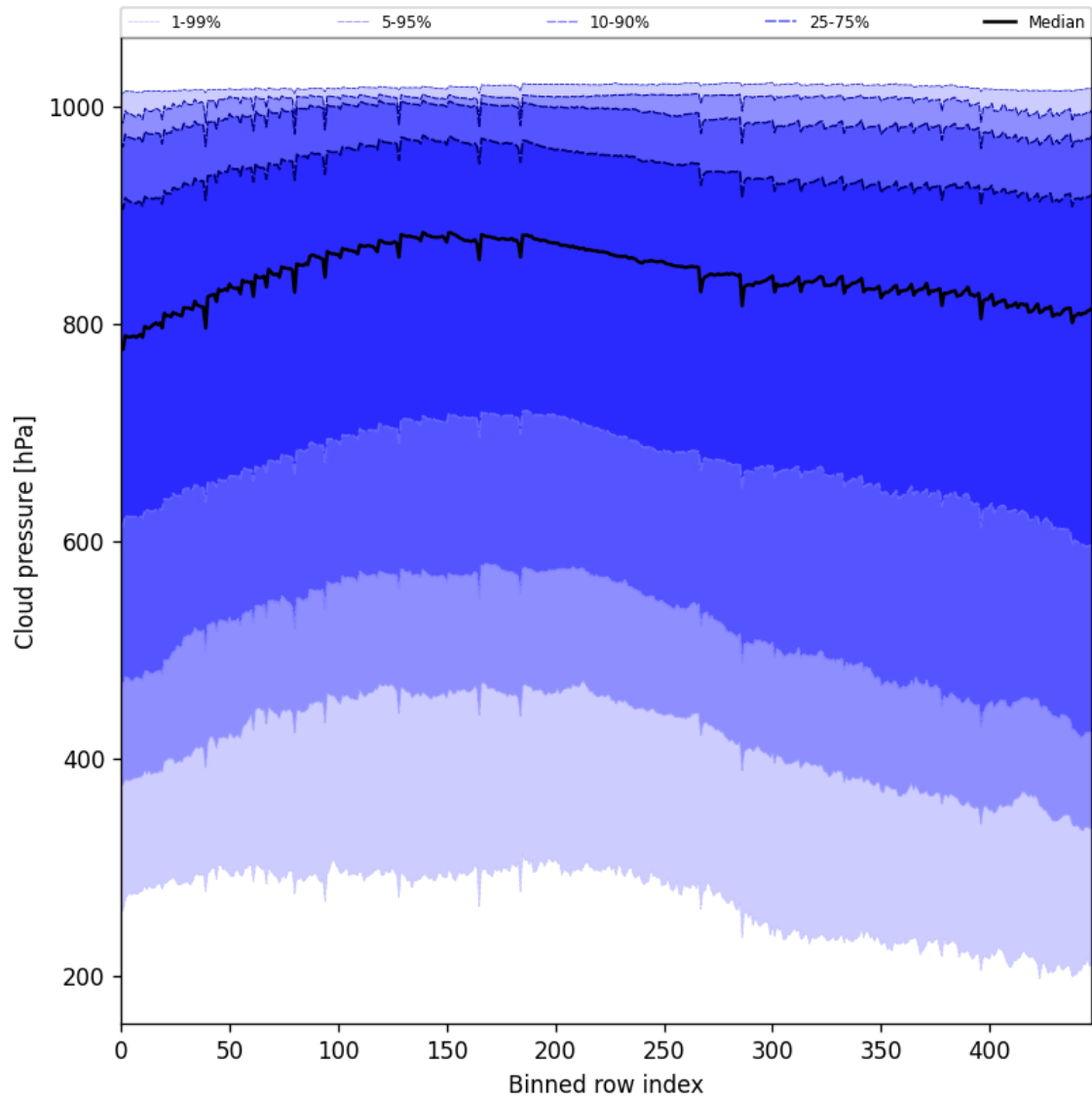
Figure 47: Along track statistics of “Cloud pressure” for 2025-02-06 to 2025-02-08
