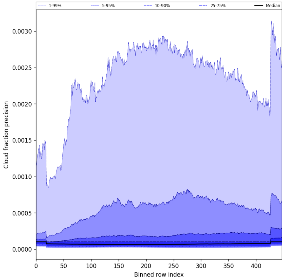
Figure 50: Along track statistics of “Cloud fraction precision” for 2025-02-06 to 2025-02-08
