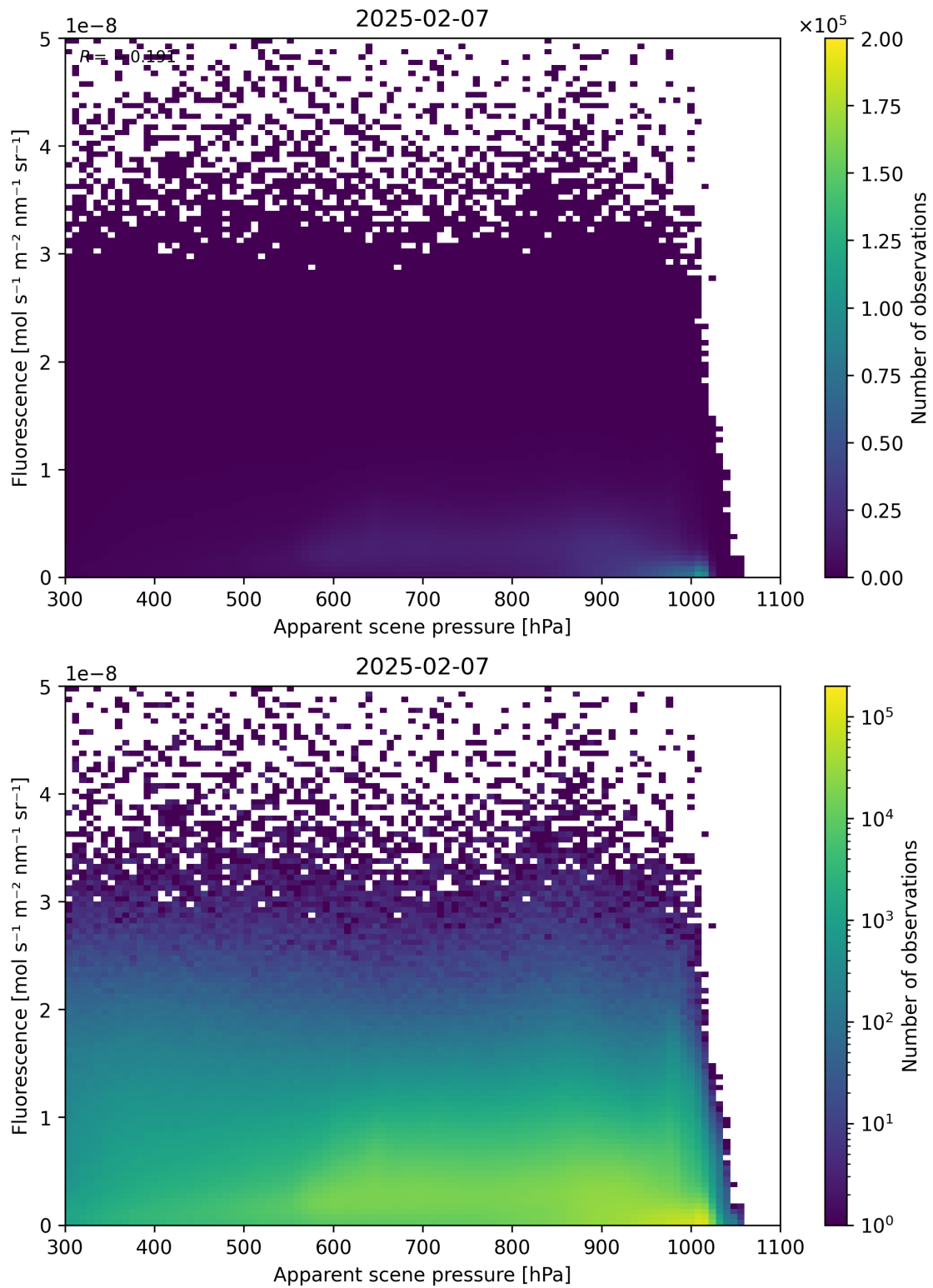
Figure 64: Scatter density plot of “Apparent scene pressure” against “Fluorescence” for 2025-02-06 to 2025-02-08.
