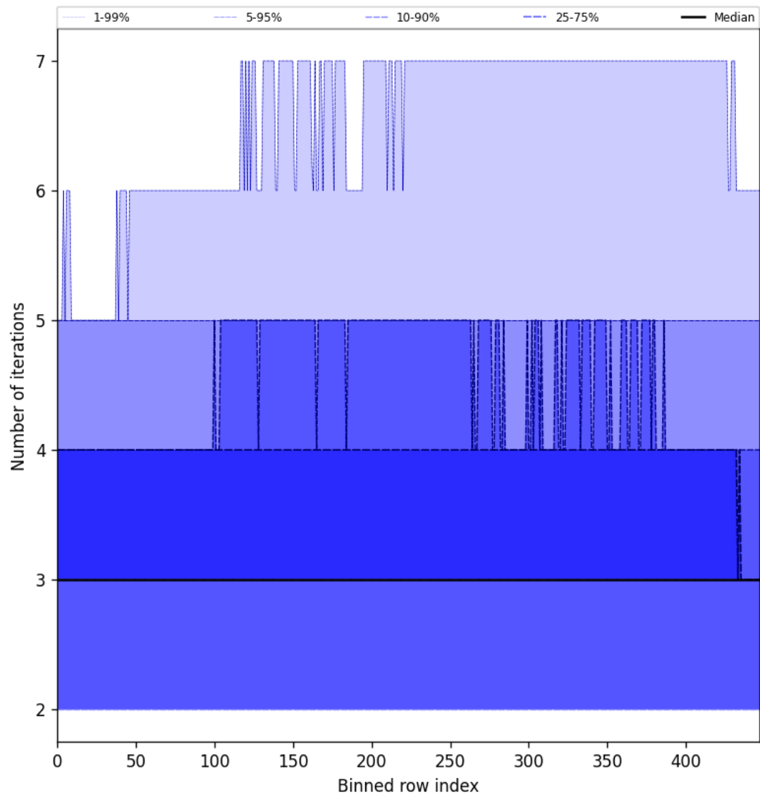
Figure 56: Along track statistics of “Number of iterations” for 2025-02-06 to 2025-02-08
