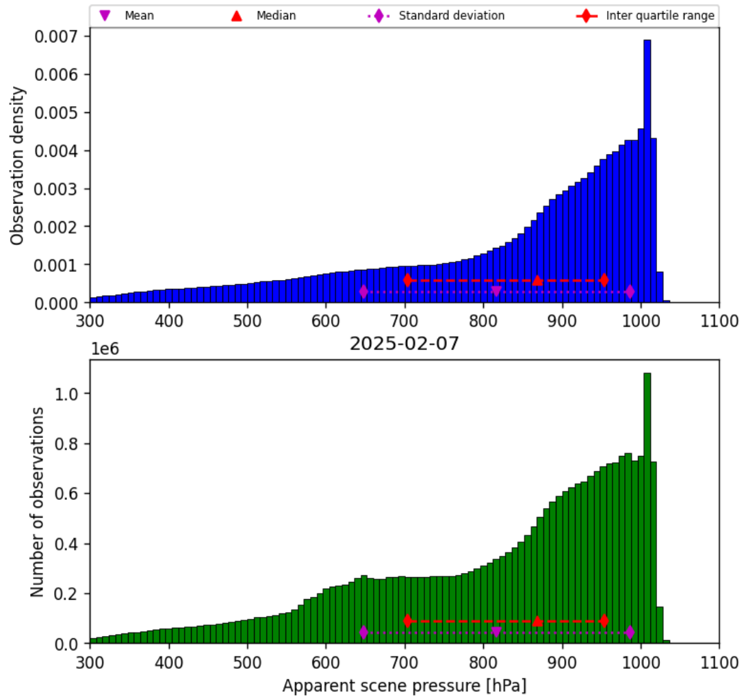
Figure 36: Histogram of “Apparent scene pressure” for 2025-02-06 to 2025-02-08
