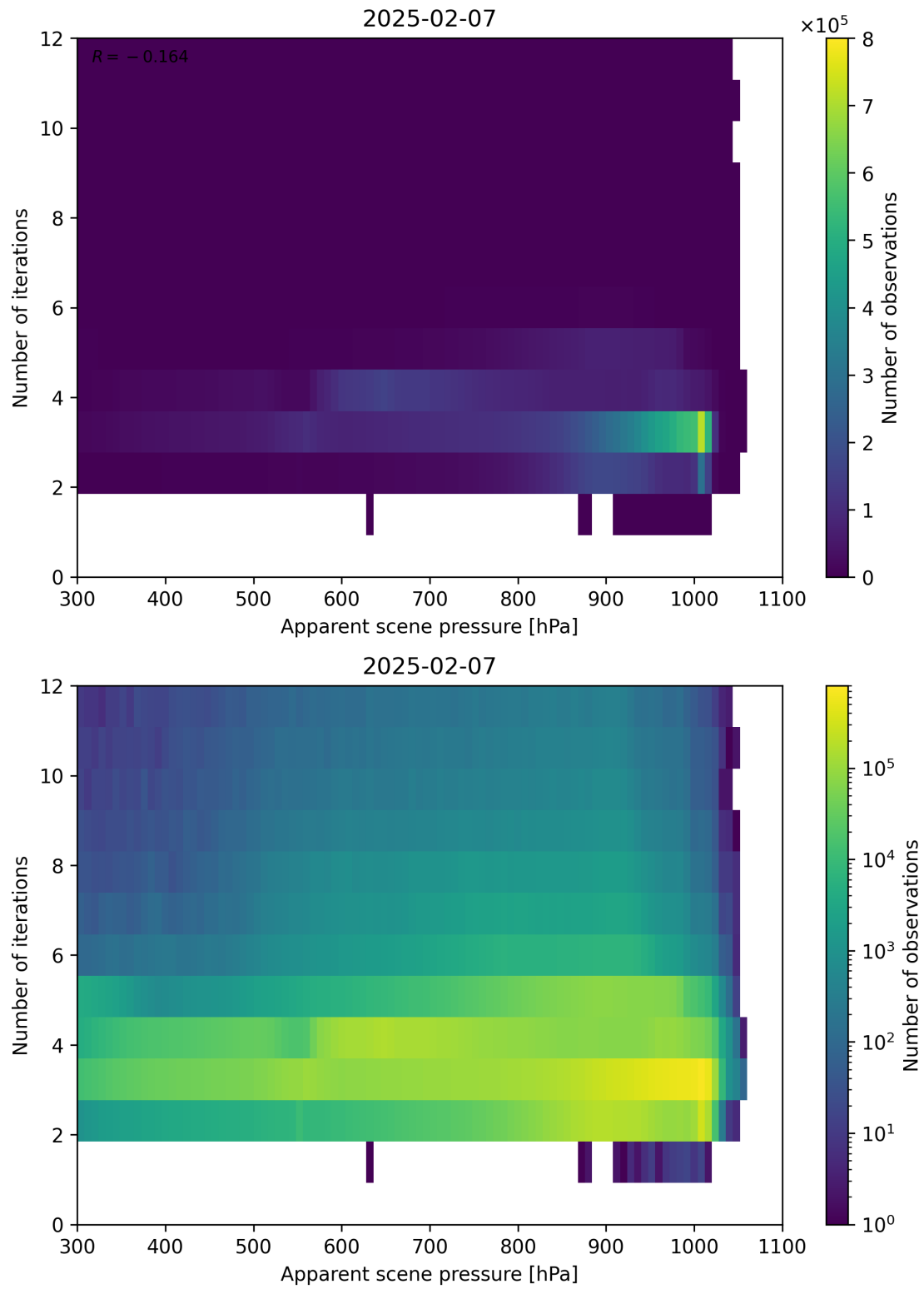
Figure 65: Scatter density plot of “Apparent scene pressure” against “Number of iterations” for 2025-02-06 to 2025-02-08.
