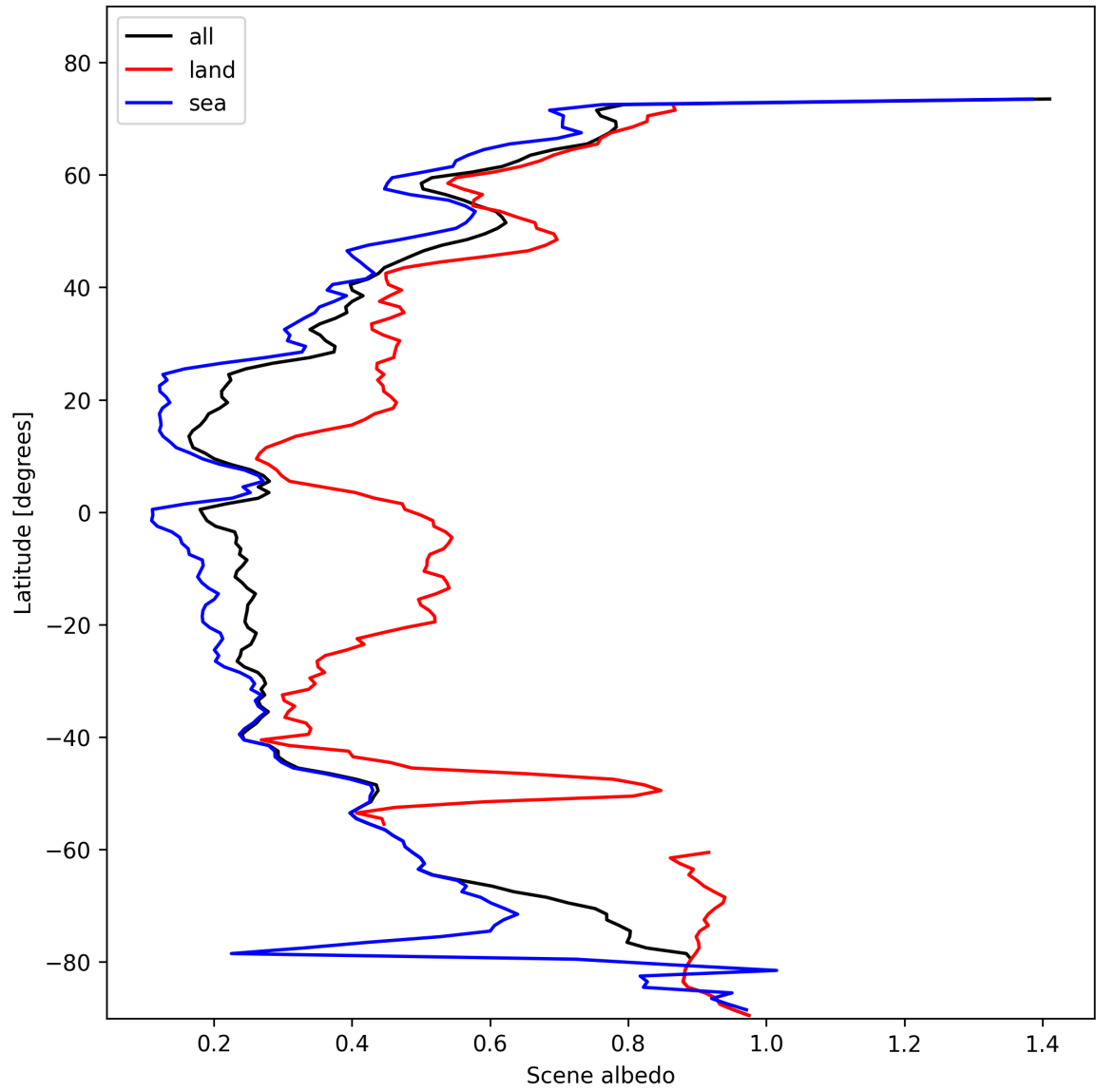
Figure 17: Zonal average of “Scene albedo” for 2025-02-06 to 2025-02-08.
