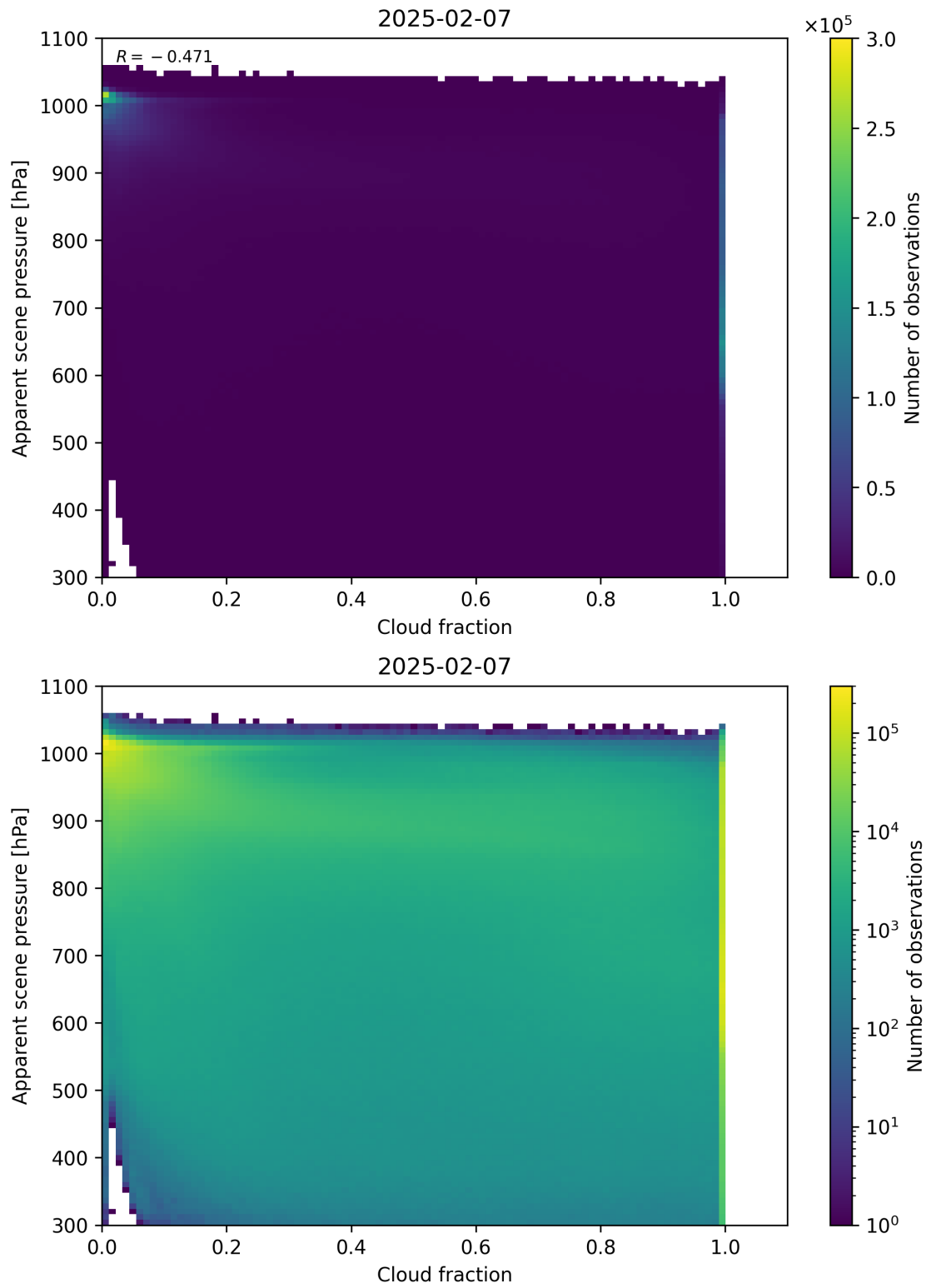
Figure 70: Scatter density plot of “Cloud fraction” against “Apparent scene pressure” for 2025-02-06 to 2025-02-08.
