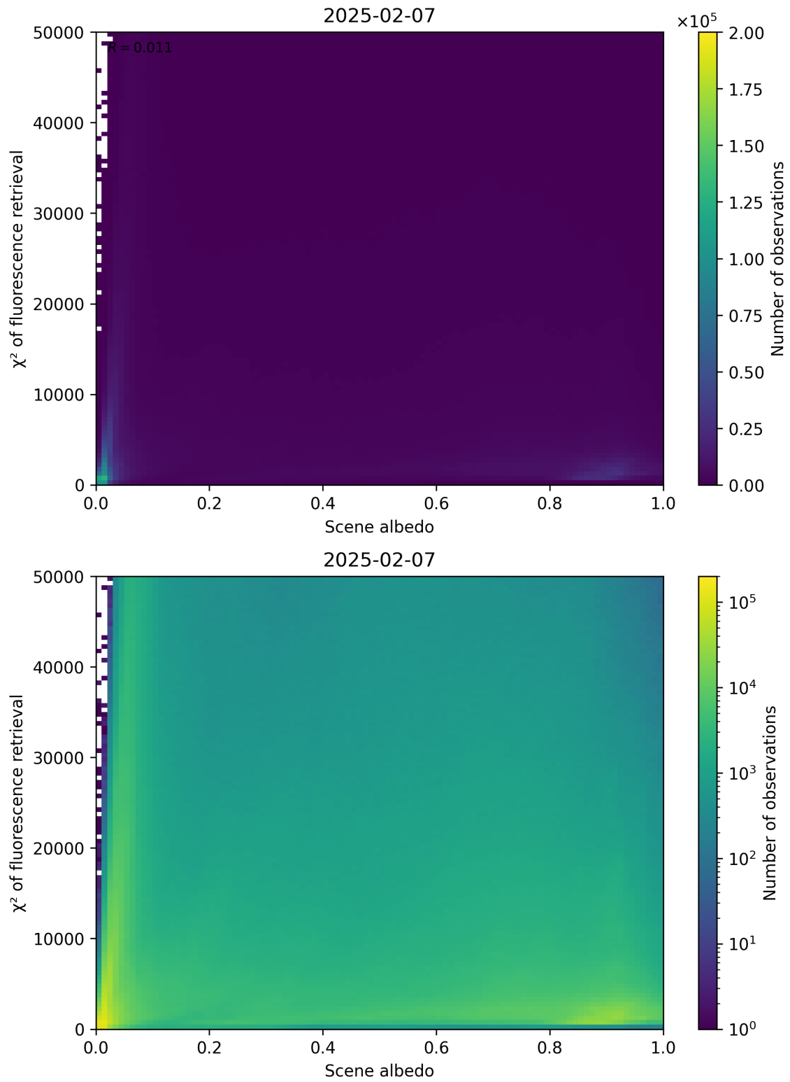
Figure 103: Scatter density plot of “Scene albedo” against “ \chi^2 of fluorescence retrieval” for 2025-02-06 to 2025-02-08.
