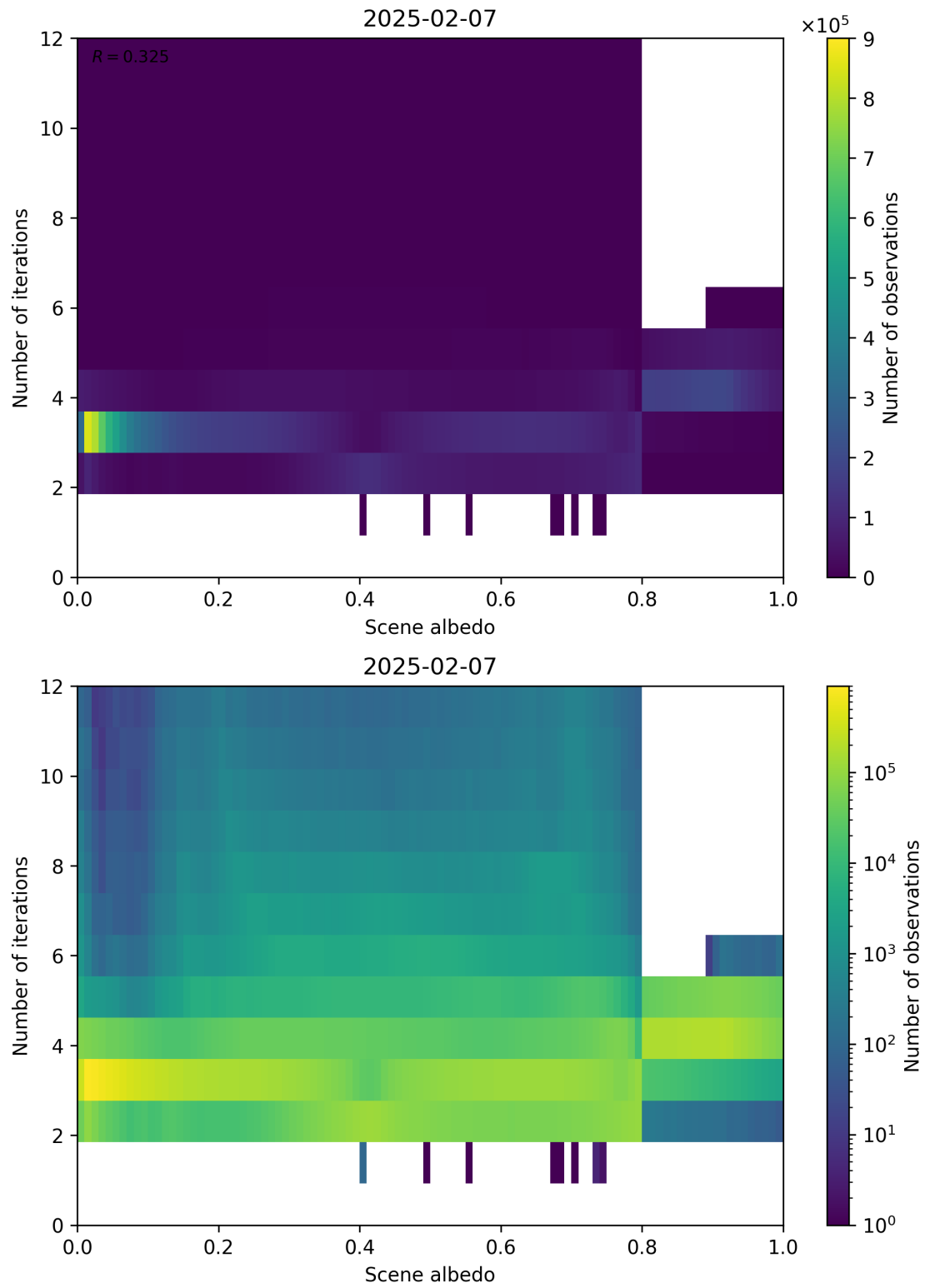
Figure 105: Scatter density plot of “Scene albedo” against “Number of iterations” for 2025-02-06 to 2025-02-08.
