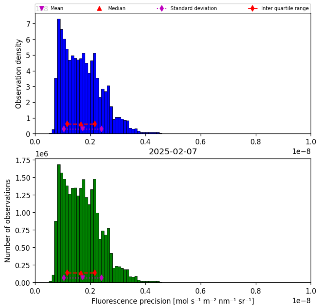
Figure 41: Histogram of “Fluorescence precision” for 2025-02-06 to 2025-02-08
