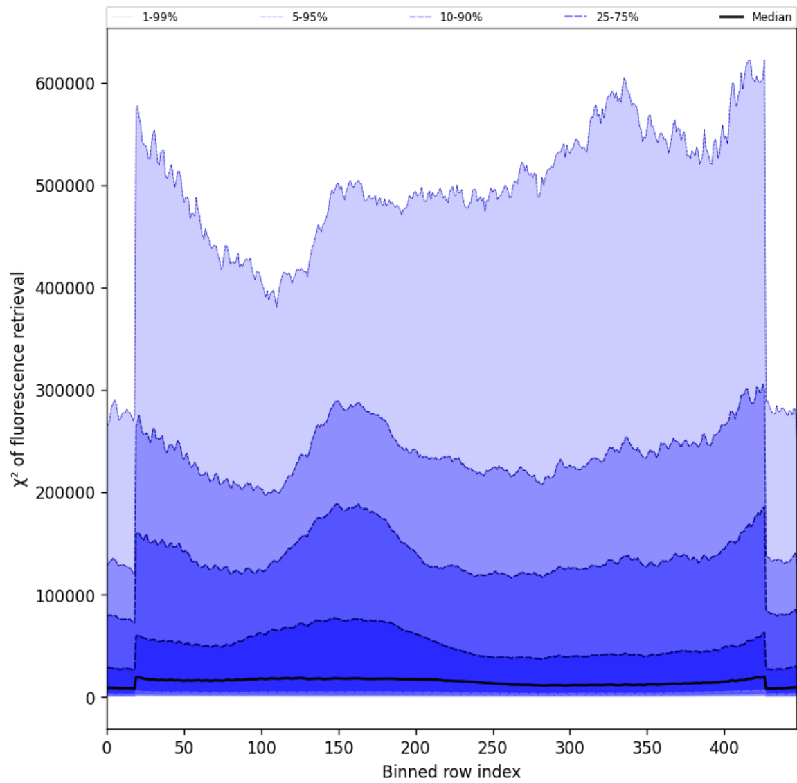
Figure 59: Along track statistics of “ \chi^2 of fluorescence retrieval” for 2025-02-06 to 2025-02-08
