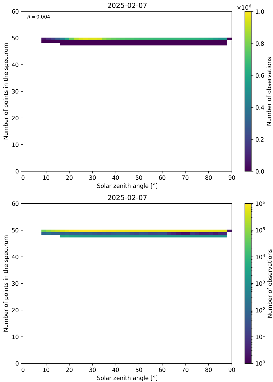
Figure 115: Scatter density plot of “Solar zenith angle” against “Number of points in the spectrum” for 2025-02-06 to 2025-02-08.
