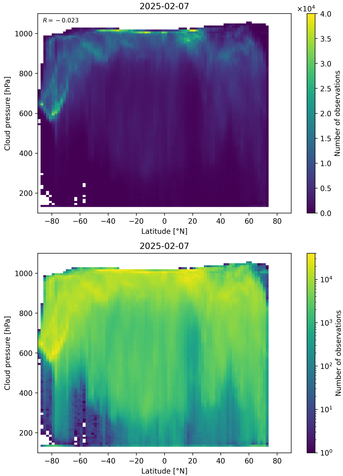
Figure 91: Scatter density plot of “Latitude” against “Cloud pressure” for 2025-02-06 to 2025-02-08.
