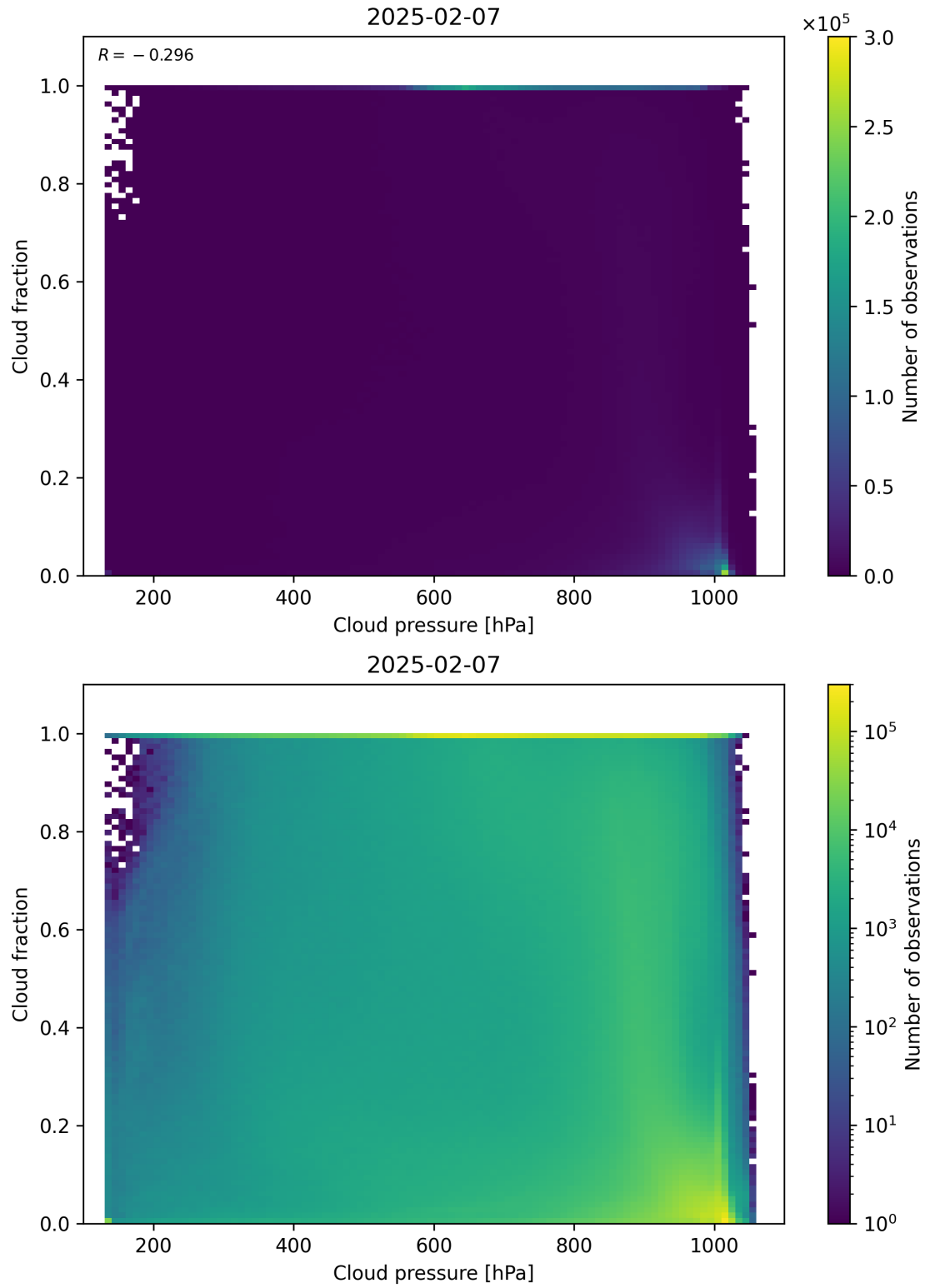
Figure 79: Scatter density plot of “Cloud pressure” against “Cloud fraction” for 2025-02-06 to 2025-02-08.
