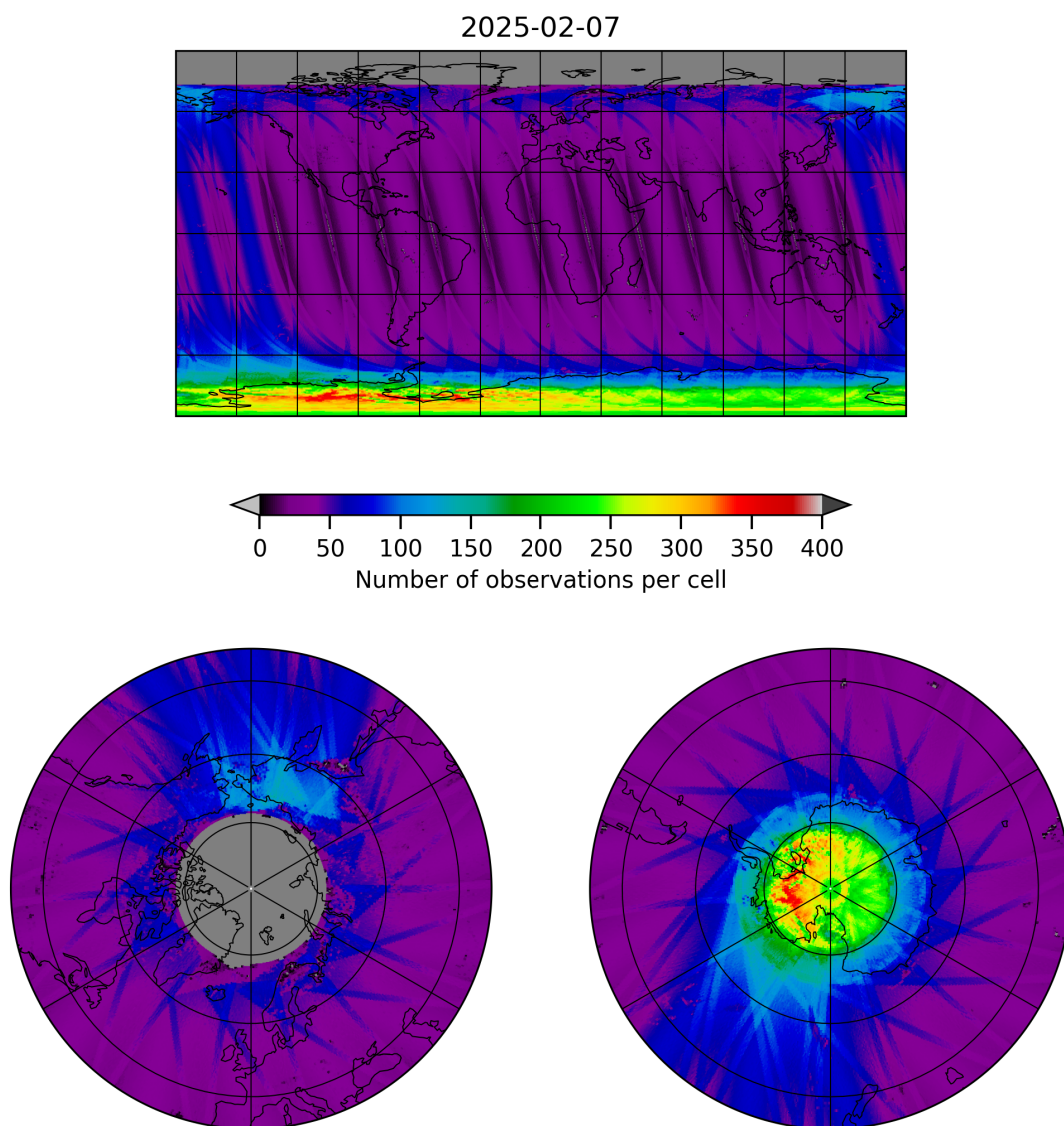
Figure 11: Map of the number of observations for 2025-02-06 to 2025-02-08
