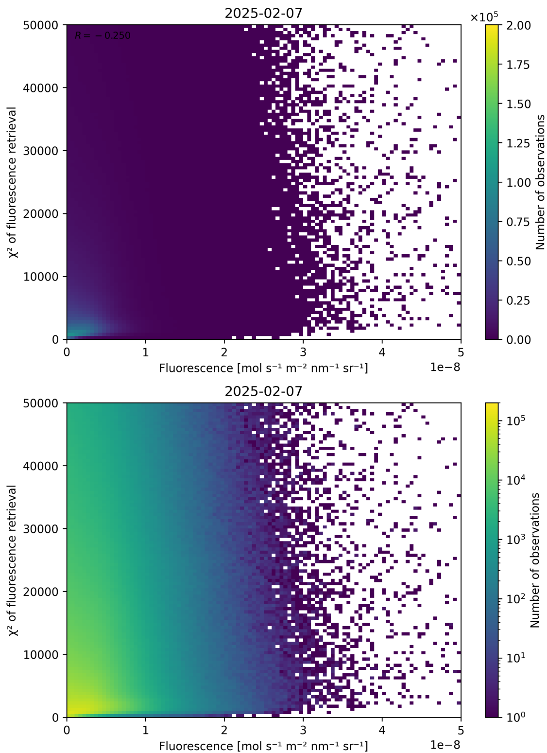
Figure 85: Scatter density plot of “Fluorescence” against “ \chi^2 of fluorescence retrieval” for 2025-02-06 to 2025-02-08.
