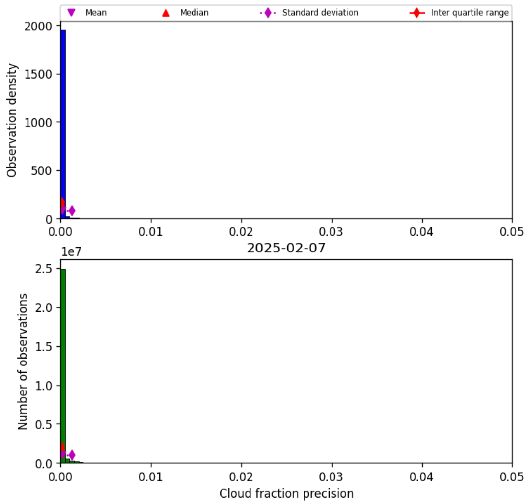
Figure 33: Histogram of “Cloud fraction precision” for 2025-02-06 to 2025-02-08
