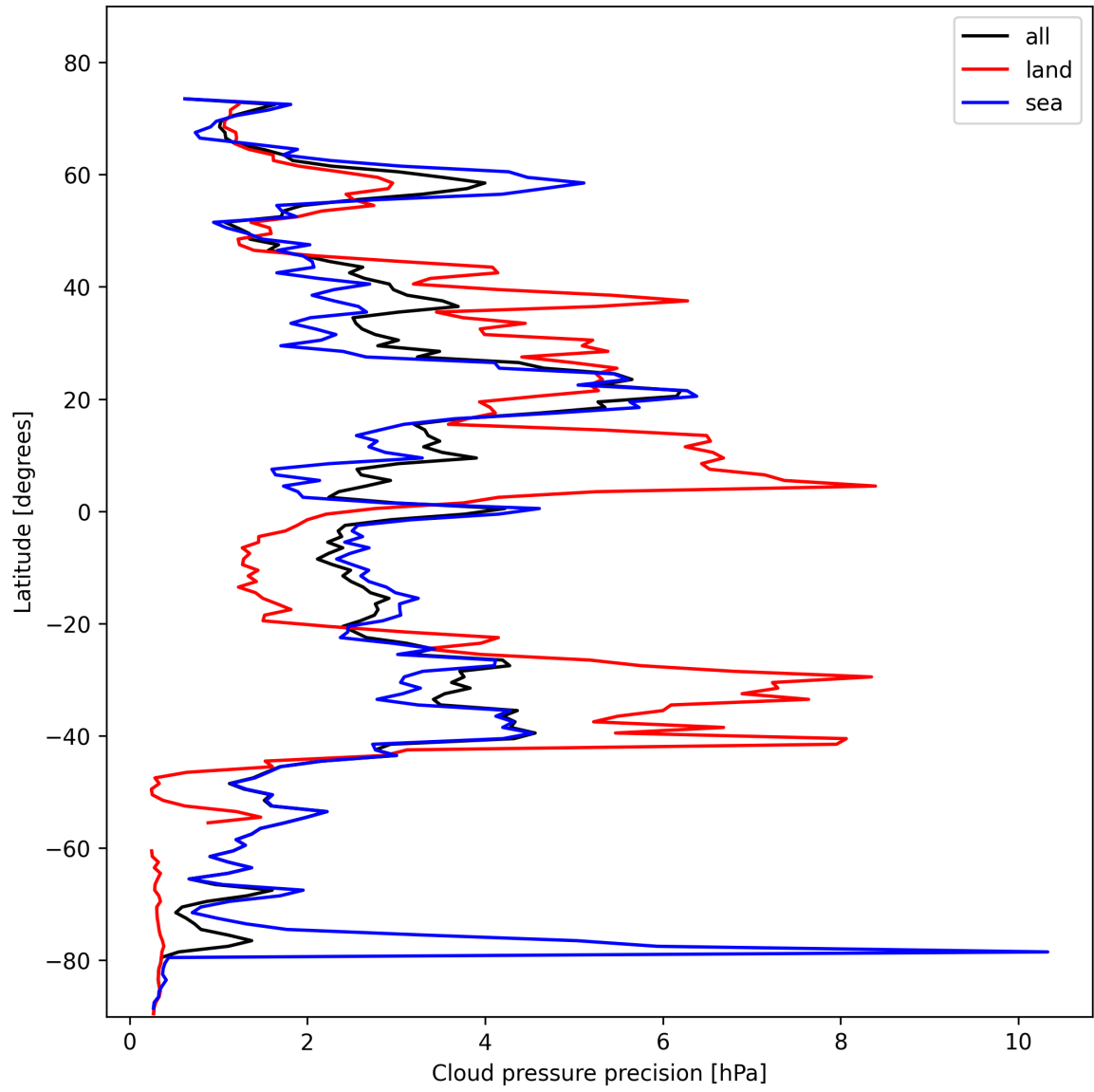
Figure 14: Zonal average of “Cloud pressure precision” for 2025-02-06 to 2025-02-08.
