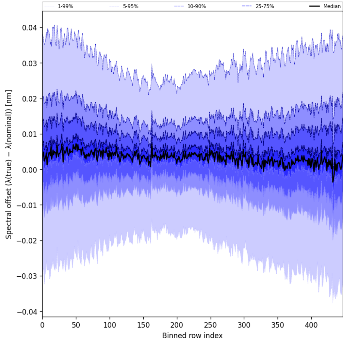
Figure 62: Along track statistics of “Spectral offset ( \lambda_{\text{true}} - \lambda_{\text{nominal}} )” for 2025-02-06 to 2025-02-08
