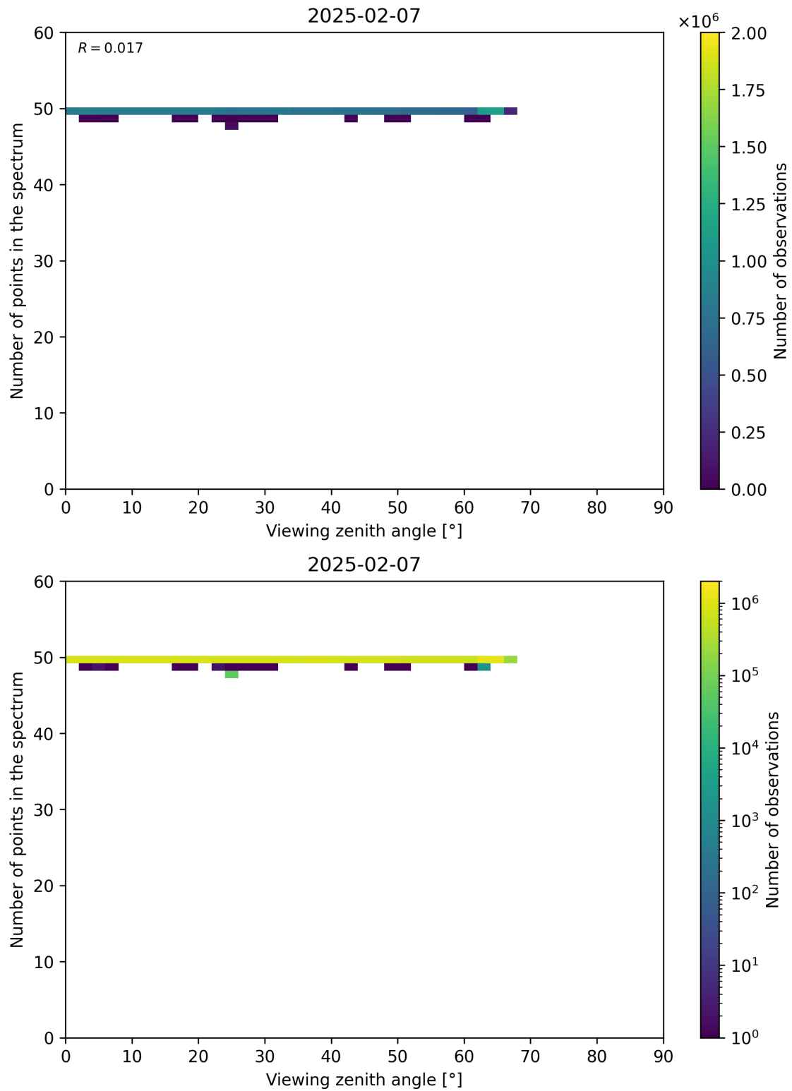
Figure 125: Scatter density plot of “Viewing zenith angle” against “Number of points in the spectrum” for 2025-02-06 to 2025-02-08.
