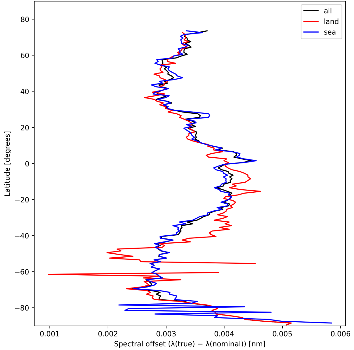
Figure 28: Zonal average of “Spectral offset ( \lambda_{\text{true}} - \lambda_{\text{nominal}} )” for 2025-02-06 to 2025-02-08.
