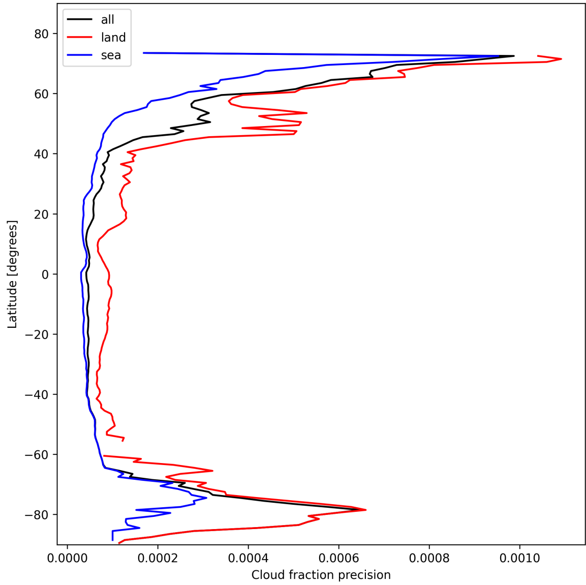
Figure 16: Zonal average of “Cloud fraction precision” for 2025-02-06 to 2025-02-08.
