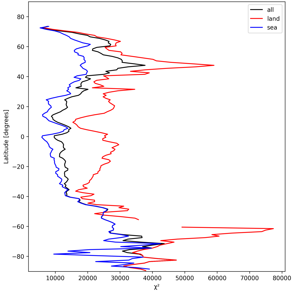
Figure 21: Zonal average of “ \chi^2 ” for 2025-02-06 to 2025-02-08.
