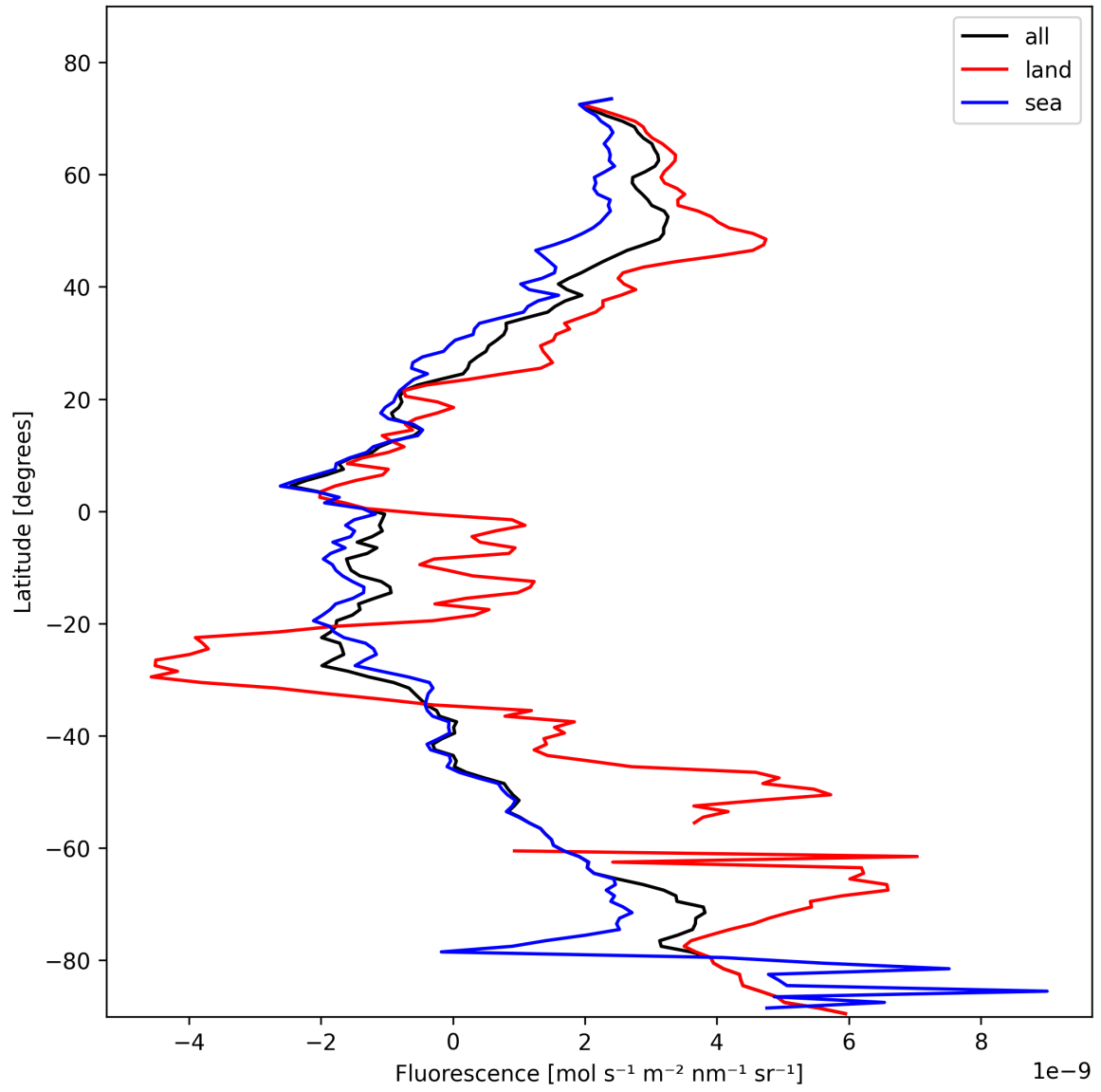
Figure 23: Zonal average of “Fluorescence” for 2025-02-06 to 2025-02-08.
