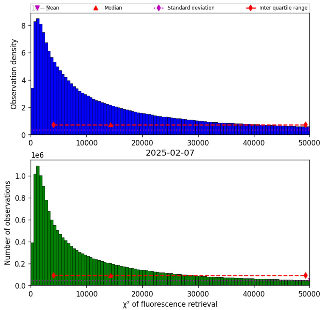
Figure 42: Histogram of “ \chi^2 of fluorescence retrieval” for 2025-02-06 to 2025-02-08
