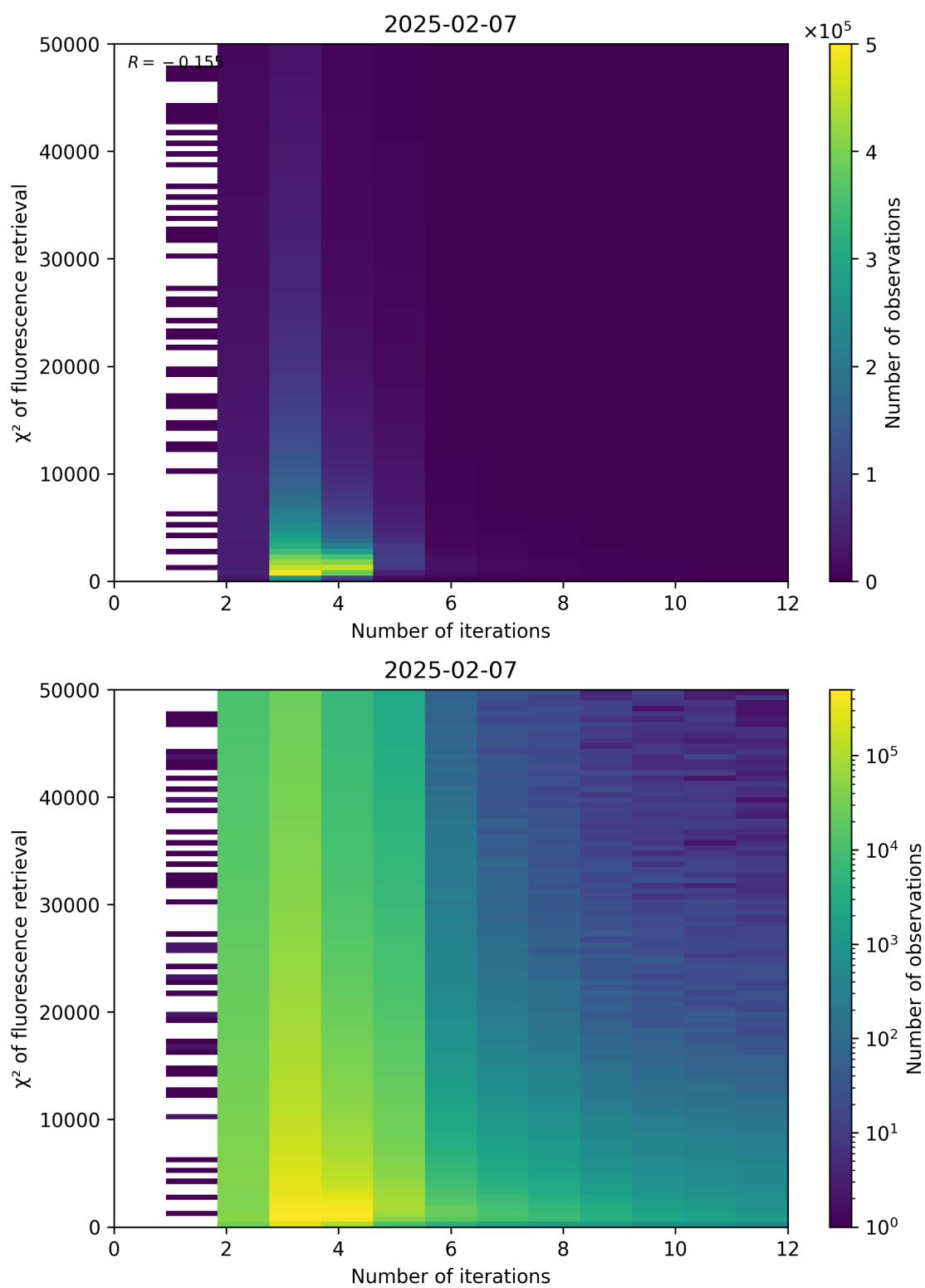
Figure 97: Scatter density plot of “Number of iterations” against “ \chi^2 of fluorescence retrieval” for 2025-02-06 to 2025-02-08.
