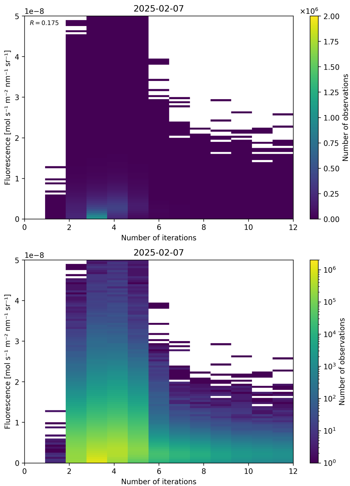
Figure 98: Scatter density plot of “Number of iterations” against “Fluorescence” for 2025-02-06 to 2025-02-08.
