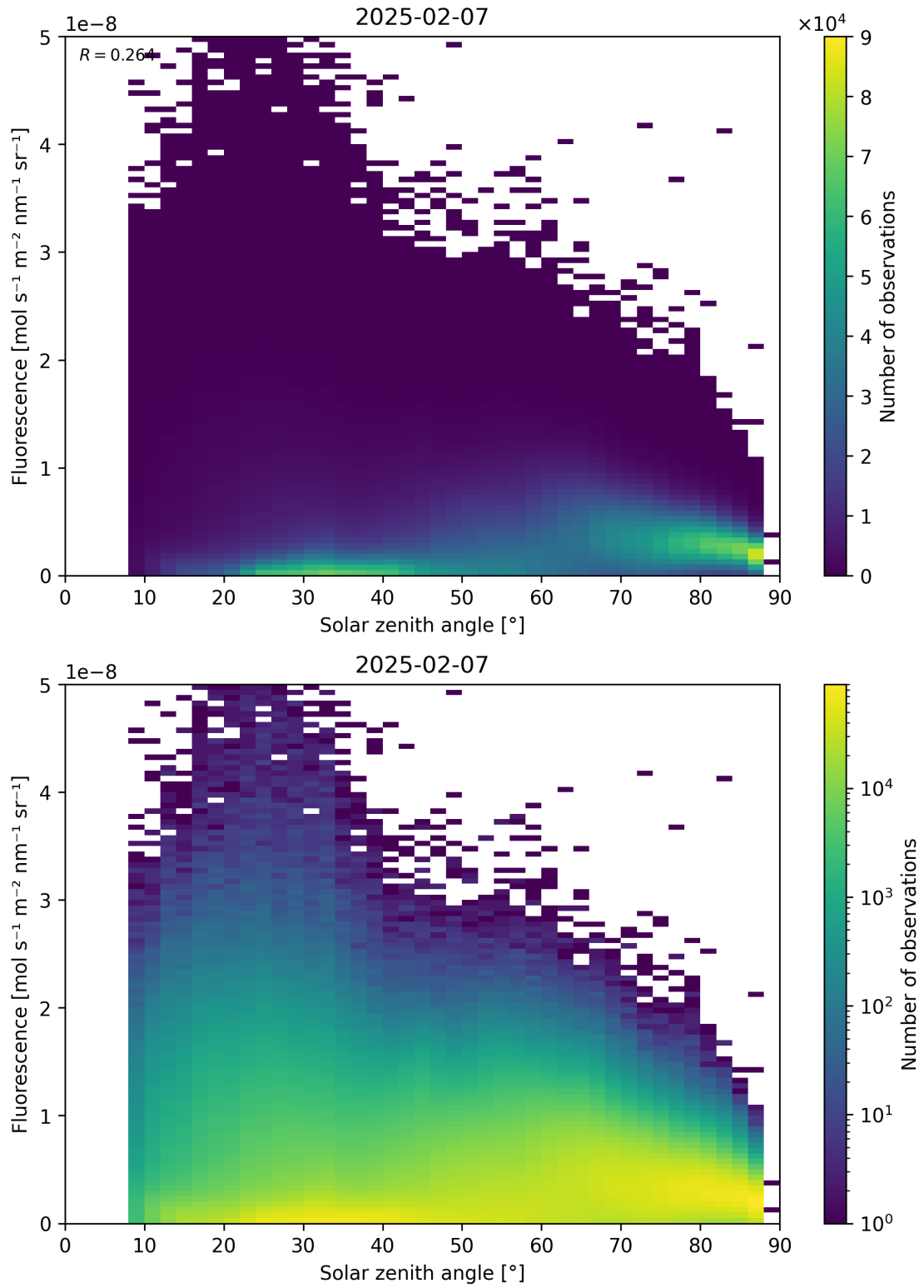
Figure 112: Scatter density plot of “Solar zenith angle” against “Fluorescence” for 2025-02-06 to 2025-02-08.
