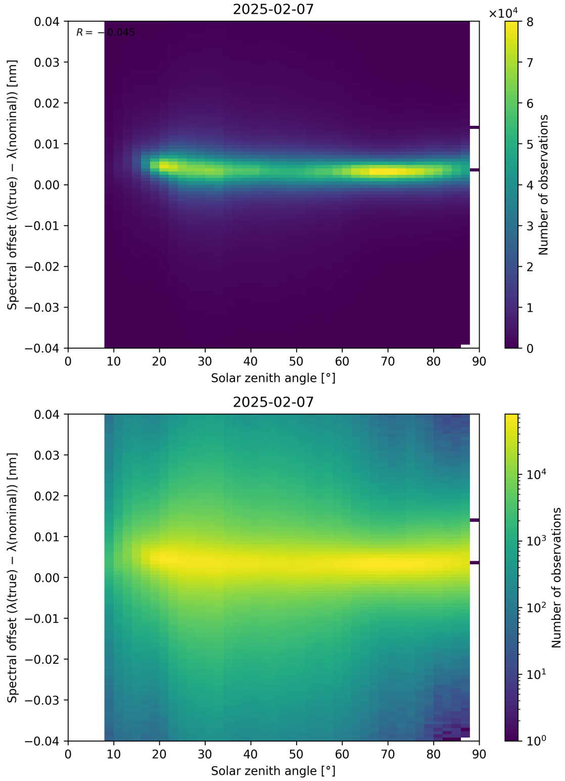
Figure 117: Scatter density plot of “Solar zenith angle” against “Spectral offset ( \lambda_{\text{true}} - \lambda_{\text{nominal}} )” for 2025-02-06 to 2025-02-08.
