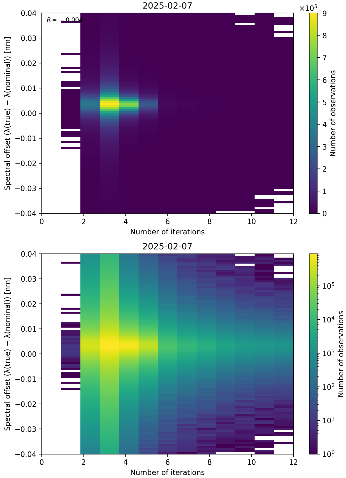
Figure 100: Scatter density plot of “Number of iterations” against “Spectral offset ( \lambda_{\text{true}} - \lambda_{\text{nominal}} )” for 2025-02-06 to 2025-02-08.
