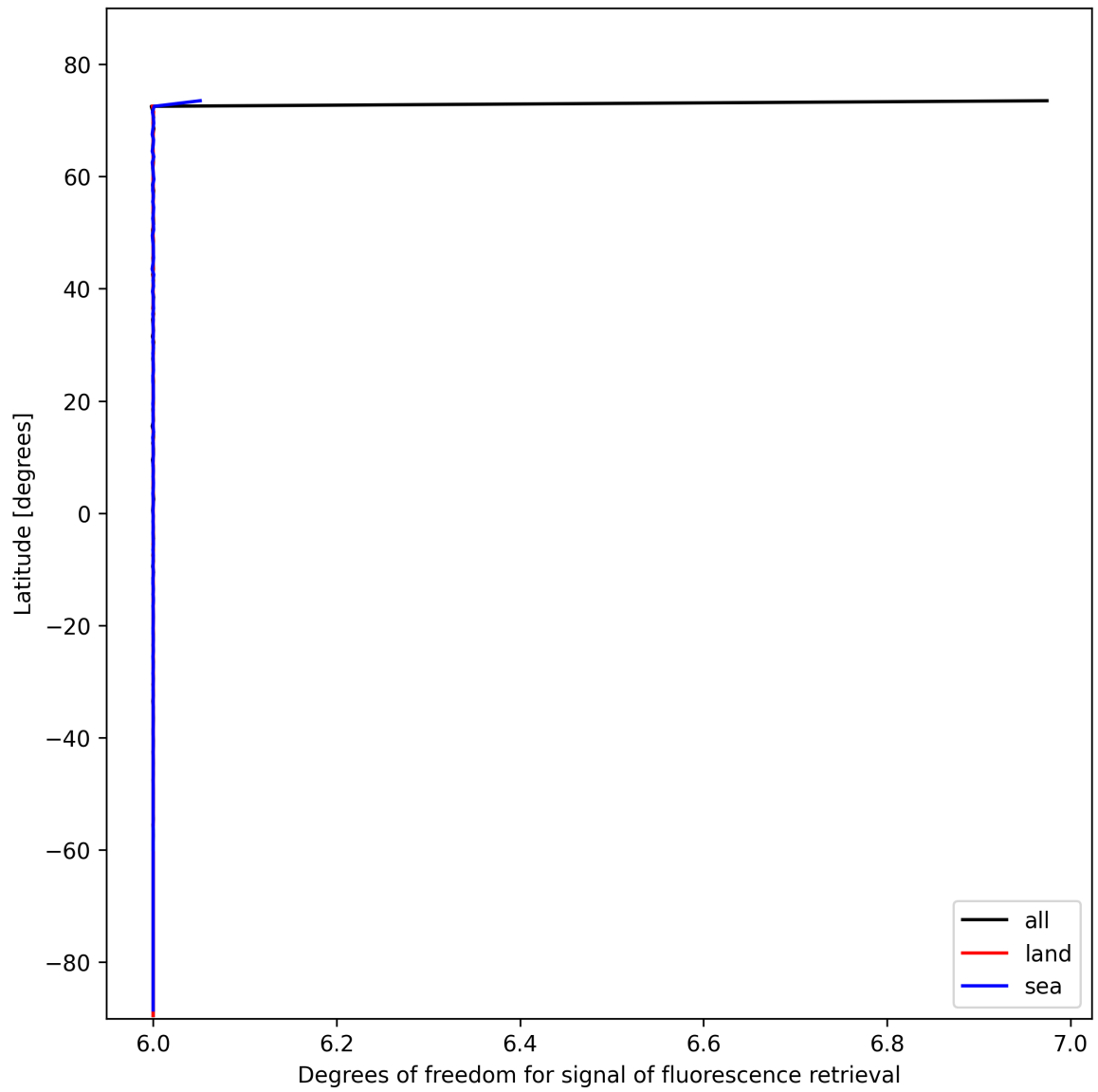
Figure 26: Zonal average of “Degrees of freedom for signal of fluorescence retrieval” for 2025-02-06 to 2025-02-08.
