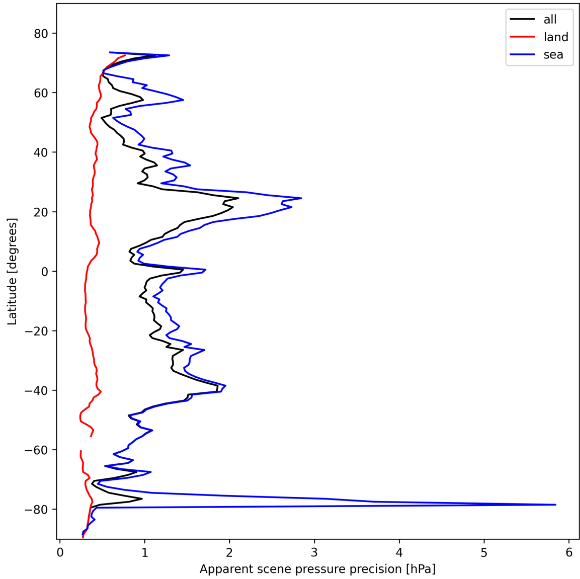
Figure 20: Zonal average of “Apparent scene pressure precision” for 2025-02-06 to 2025-02-08.
