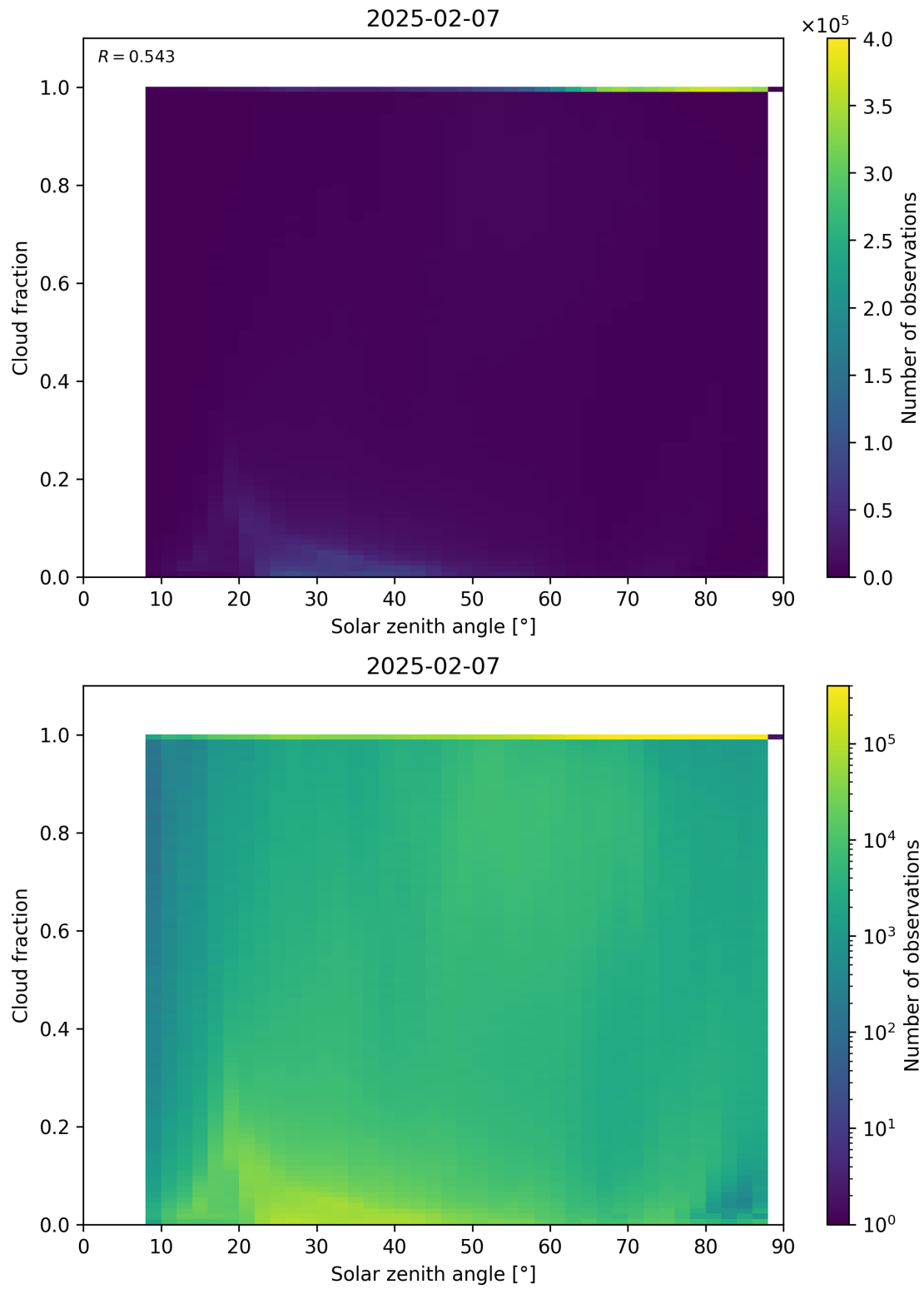
Figure 110: Scatter density plot of “Solar zenith angle” against “Cloud fraction” for 2025-02-06 to 2025-02-08.
