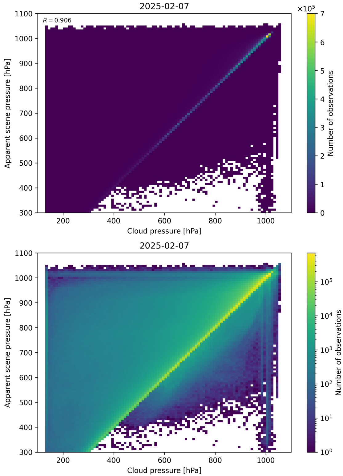
Figure 77: Scatter density plot of “Cloud pressure” against “Apparent scene pressure” for 2025-02-06 to 2025-02-08.
