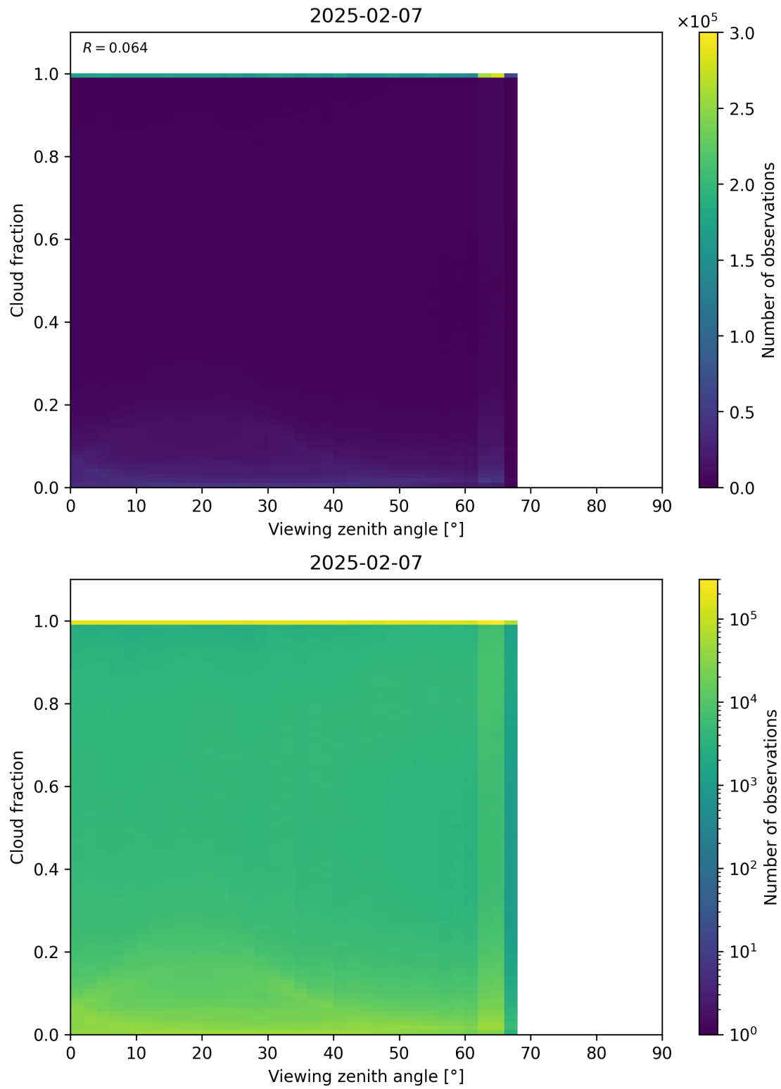
Figure 120: Scatter density plot of “Viewing zenith angle” against “Cloud fraction” for 2025-02-06 to 2025-02-08.
