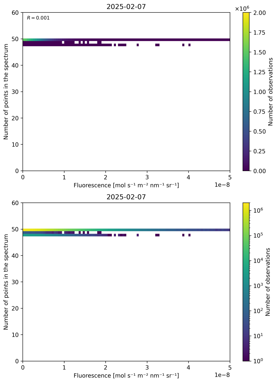
Figure 86: Scatter density plot of “Fluorescence” against “Number of points in the spectrum” for 2025-02-06 to 2025-02-08.
