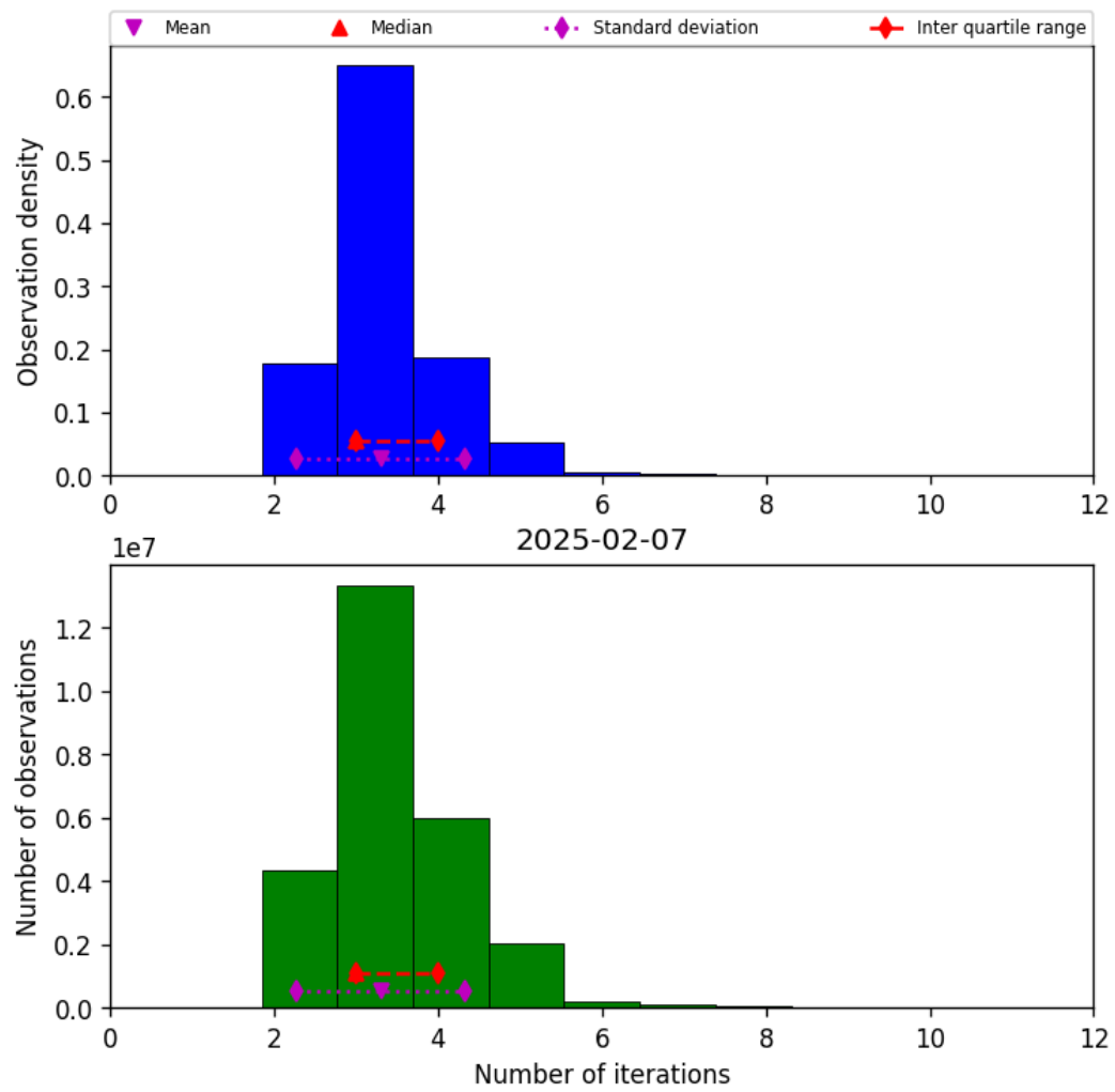
Figure 39: Histogram of “Number of iterations” for 2025-02-06 to 2025-02-08
