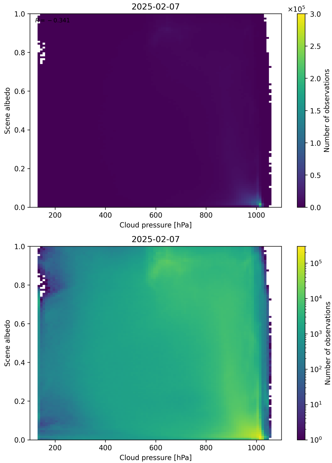
Figure 83: Scatter density plot of “Cloud pressure” against “Scene albedo” for 2025-02-06 to 2025-02-08.
