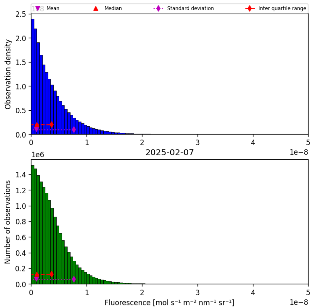
Figure 40: Histogram of “Fluorescence” for 2025-02-06 to 2025-02-08
