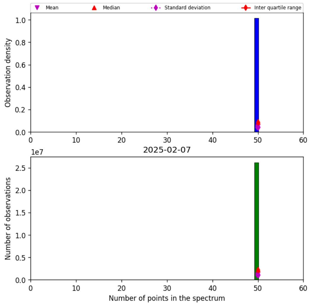
Figure 44: Histogram of “Number of points in the spectrum” for 2025-02-06 to 2025-02-08
