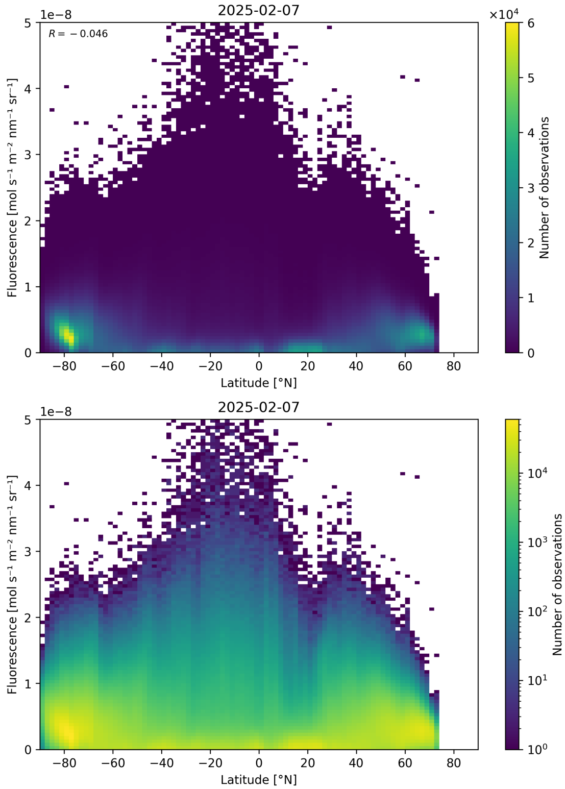
Figure 92: Scatter density plot of “Latitude” against “Fluorescence” for 2025-02-06 to 2025-02-08.
