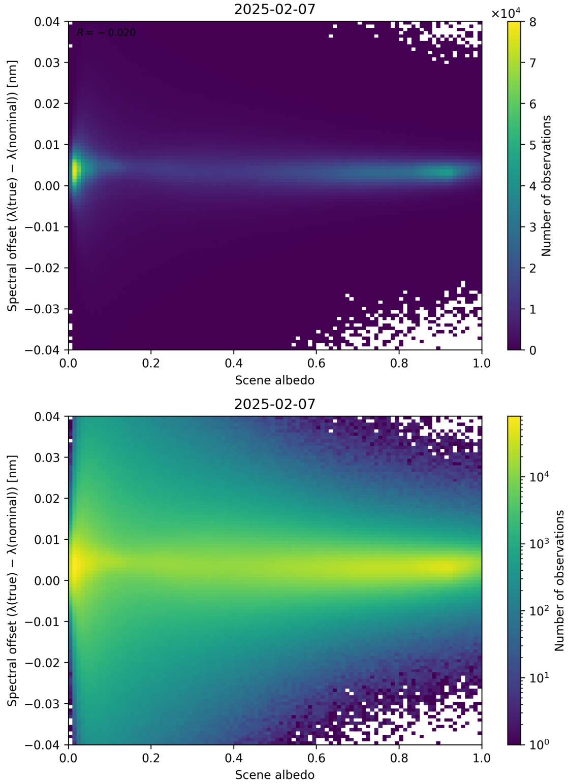
Figure 107: Scatter density plot of “Scene albedo” against “Spectral offset ( \lambda_{\text{true}} - \lambda_{\text{nominal}} )” for 2025-02-06 to 2025-02-08.
