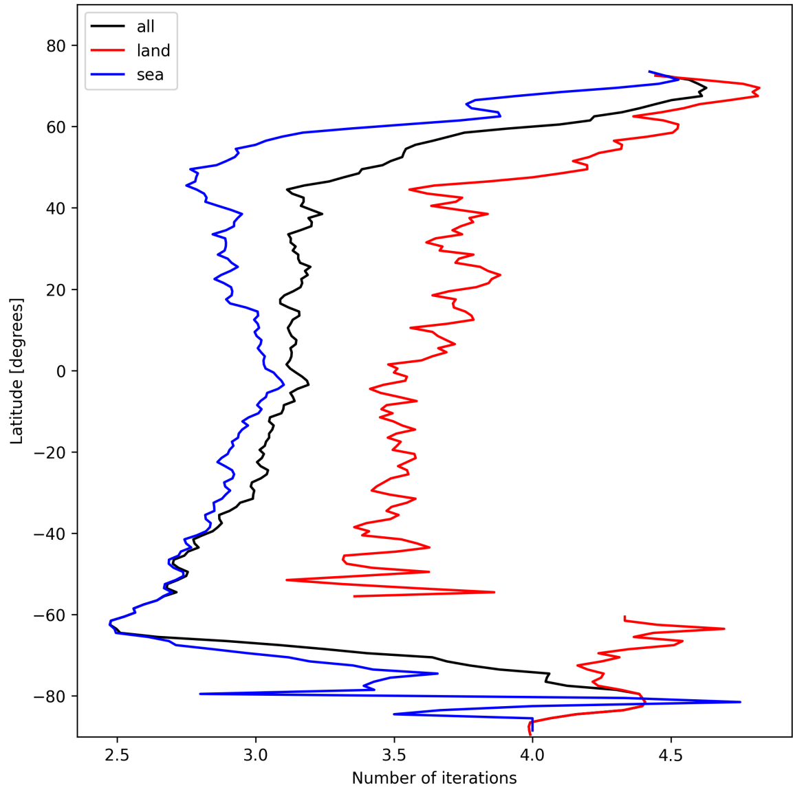
Figure 22: Zonal average of “Number of iterations” for 2025-02-06 to 2025-02-08.
