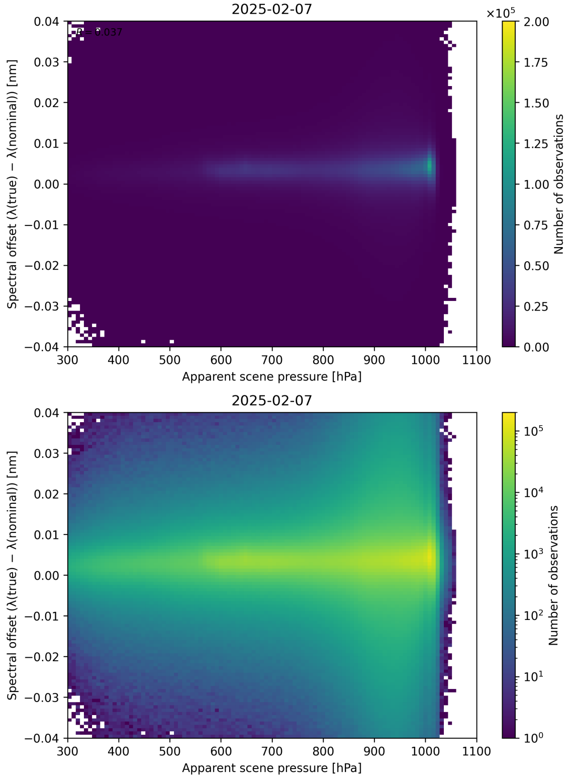
Figure 67: Scatter density plot of “Apparent scene pressure” against “Spectral offset ( \lambda_{\text{true}} - \lambda_{\text{nominal}} )” for 2025-02-06 to 2025-02-08.
