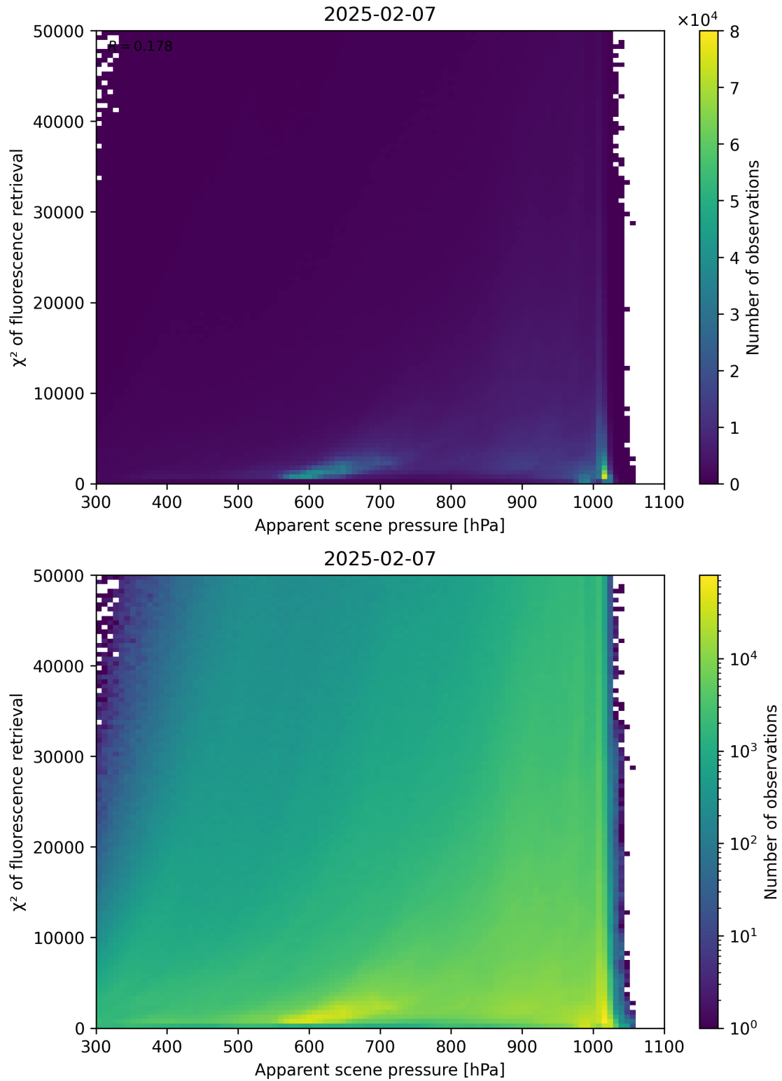
Figure 63: Scatter density plot of “Apparent scene pressure” against “ \chi^2 of fluorescence retrieval” for 2025-02-06 to 2025-02-08.
