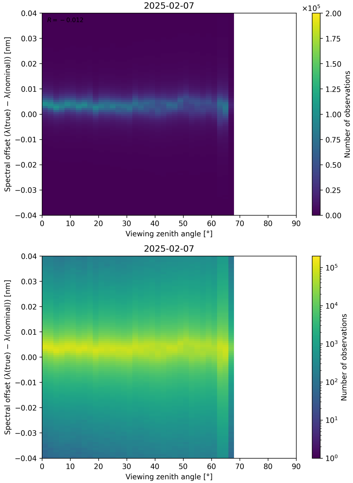
Figure 128: Scatter density plot of “Viewing zenith angle” against “Spectral offset ( \lambda_{\text{true}} - \lambda_{\text{nominal}} )” for 2025-02-06 to 2025-02-08.
