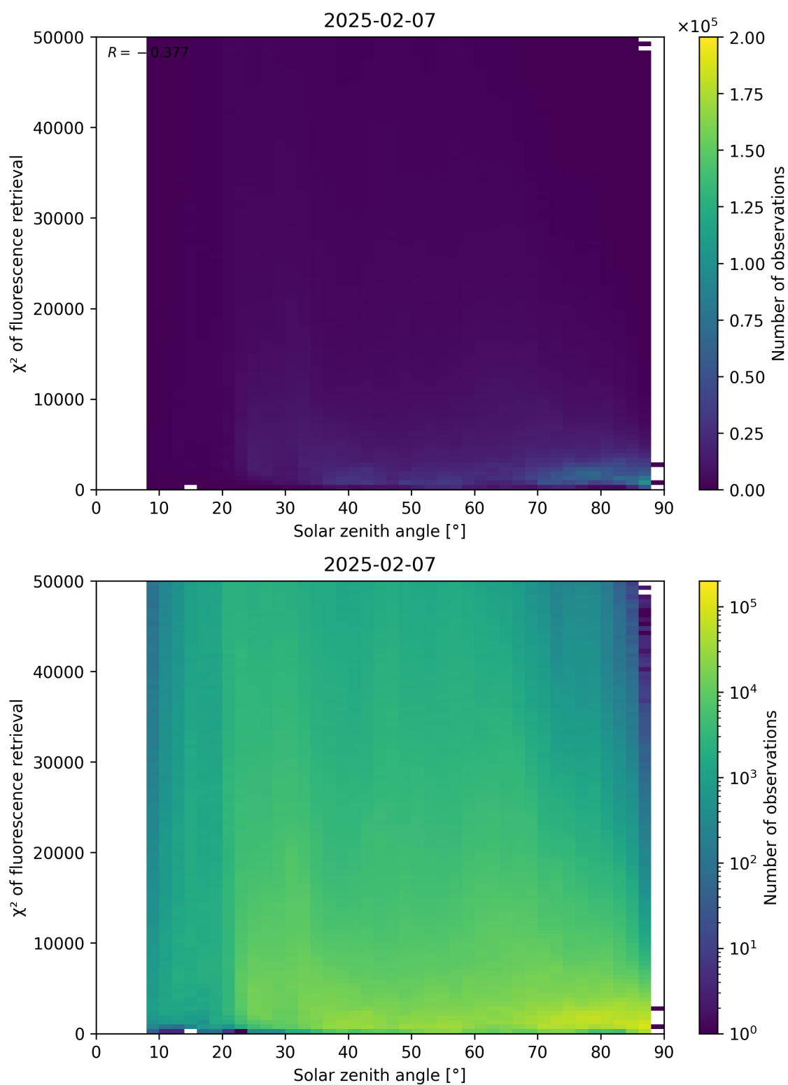
Figure 109: Scatter density plot of “Solar zenith angle” against “ \chi^2 of fluorescence retrieval” for 2025-02-06 to 2025-02-08.
