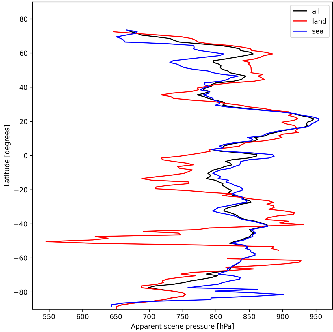
Figure 19: Zonal average of “Apparent scene pressure” for 2025-02-06 to 2025-02-08.
