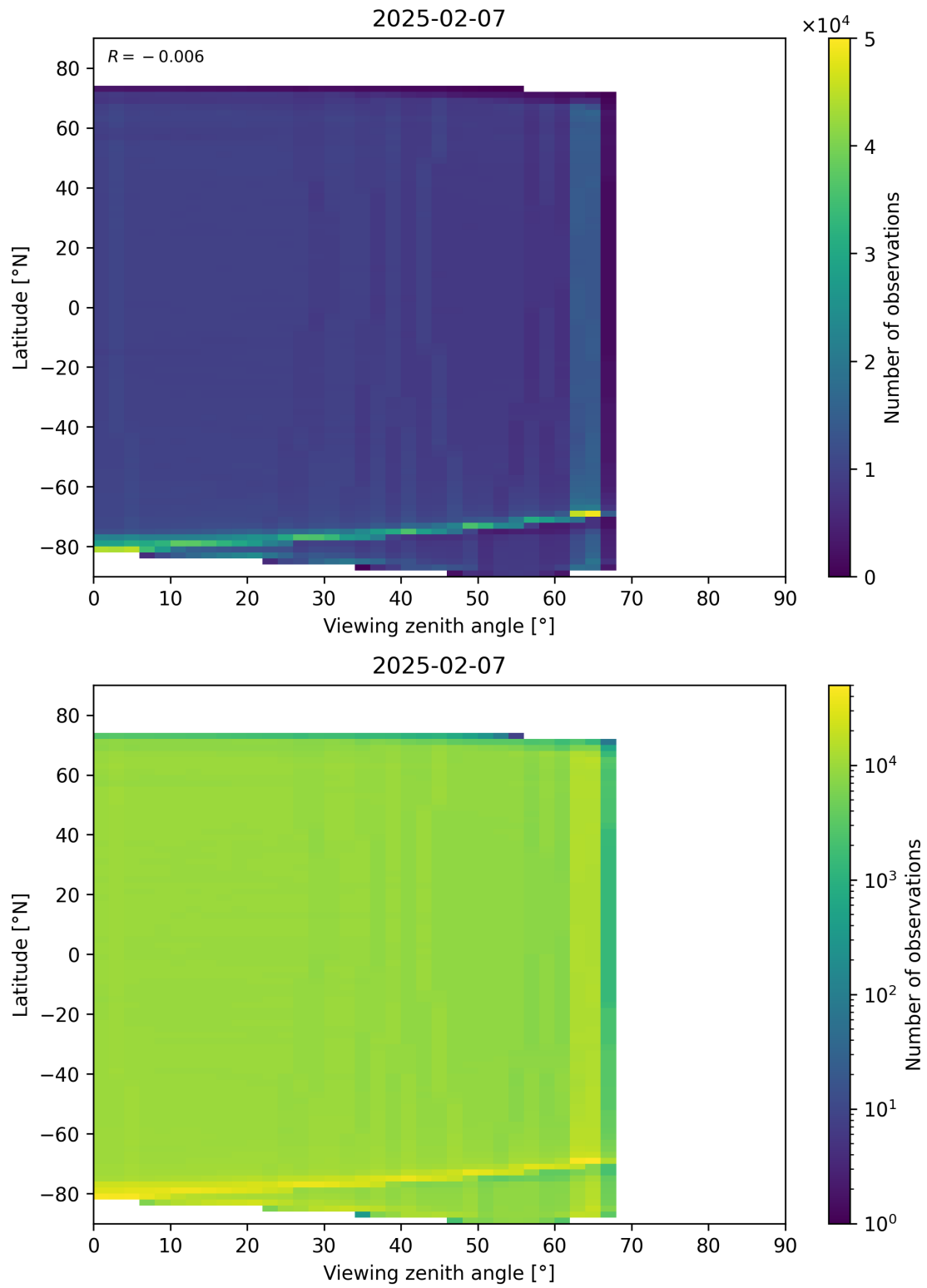
Figure 123: Scatter density plot of “Viewing zenith angle” against “Latitude” for 2025-02-06 to 2025-02-08.
