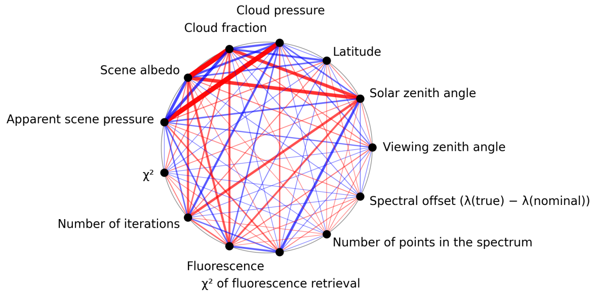
Figure 1: Map of correlation graph for 2025-02-06 to 2025-02-08.
