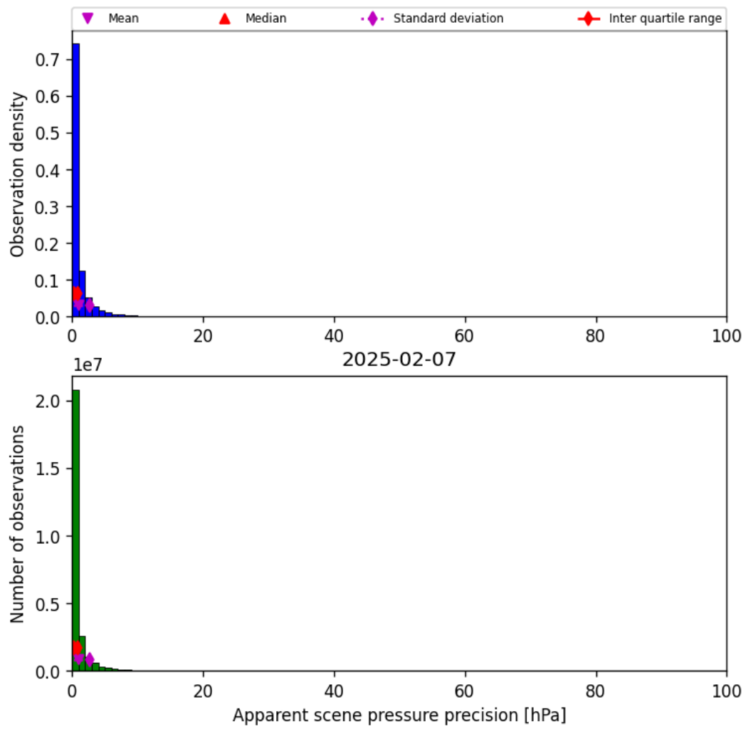
Figure 37: Histogram of “Apparent scene pressure precision” for 2025-02-06 to 2025-02-08
