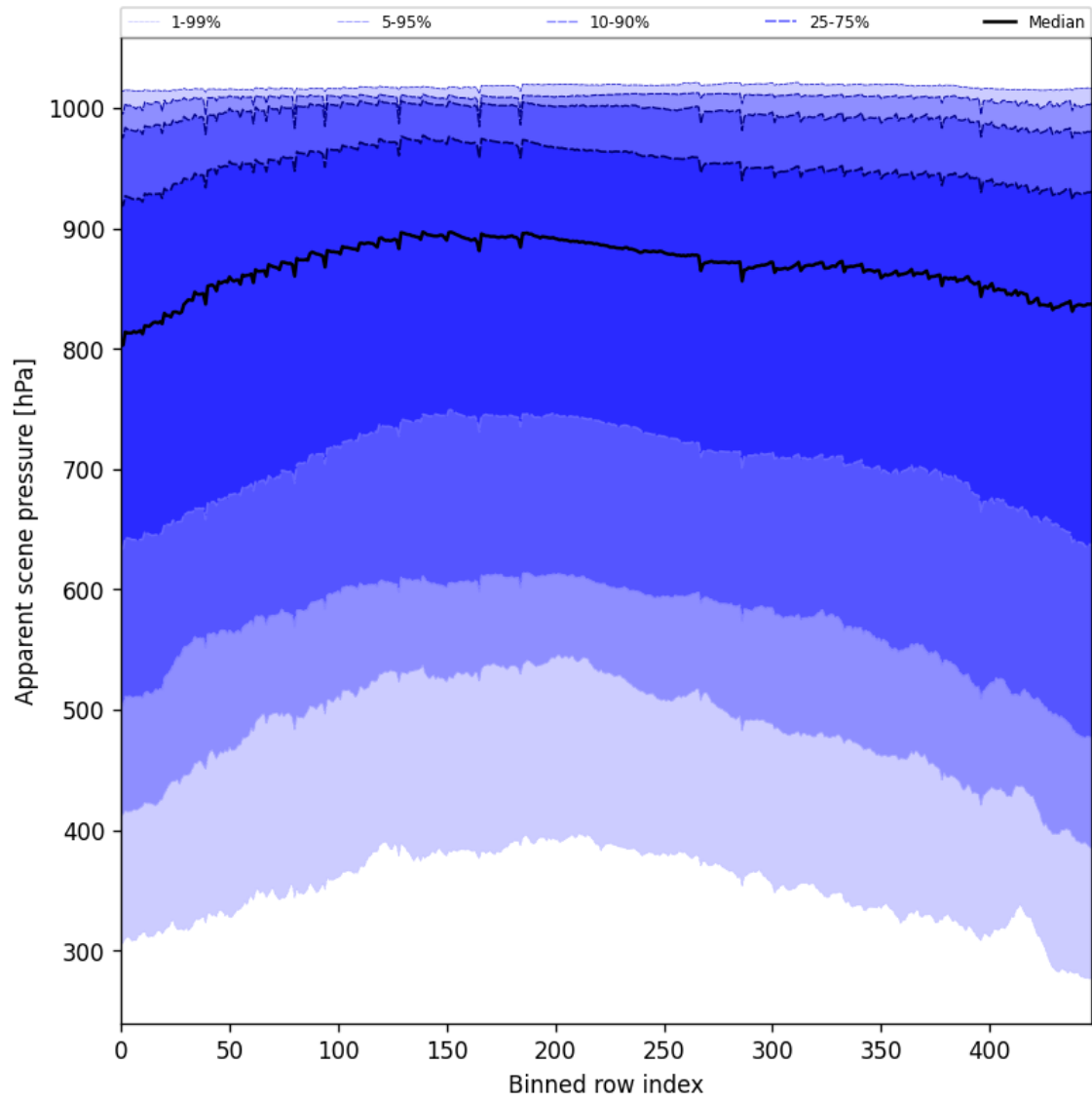
Figure 53: Along track statistics of “Apparent scene pressure” for 2025-02-06 to 2025-02-08
