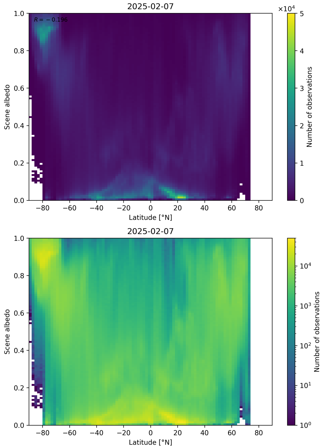
Figure 95: Scatter density plot of “Latitude” against “Scene albedo” for 2025-02-06 to 2025-02-08.
