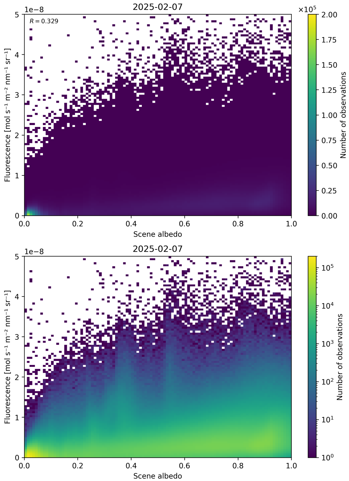
Figure 104: Scatter density plot of “Scene albedo” against “Fluorescence” for 2025-02-06 to 2025-02-08.
