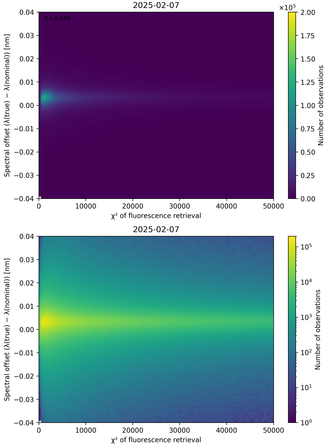
Figure 69: Scatter density plot of “ \chi^2 of fluorescence retrieval” against “Spectral offset ( \lambda_{\text{true}} - \lambda_{\text{nominal}} )” for 2025-02-06 to 2025-02-08.
