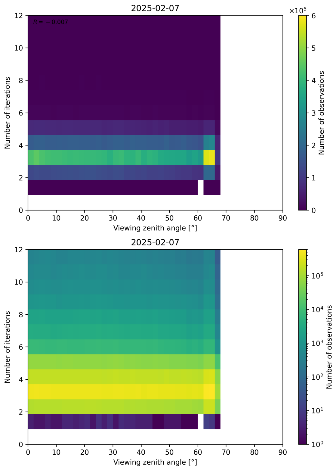
Figure 124: Scatter density plot of “Viewing zenith angle” against “Number of iterations” for 2025-02-06 to 2025-02-08.
