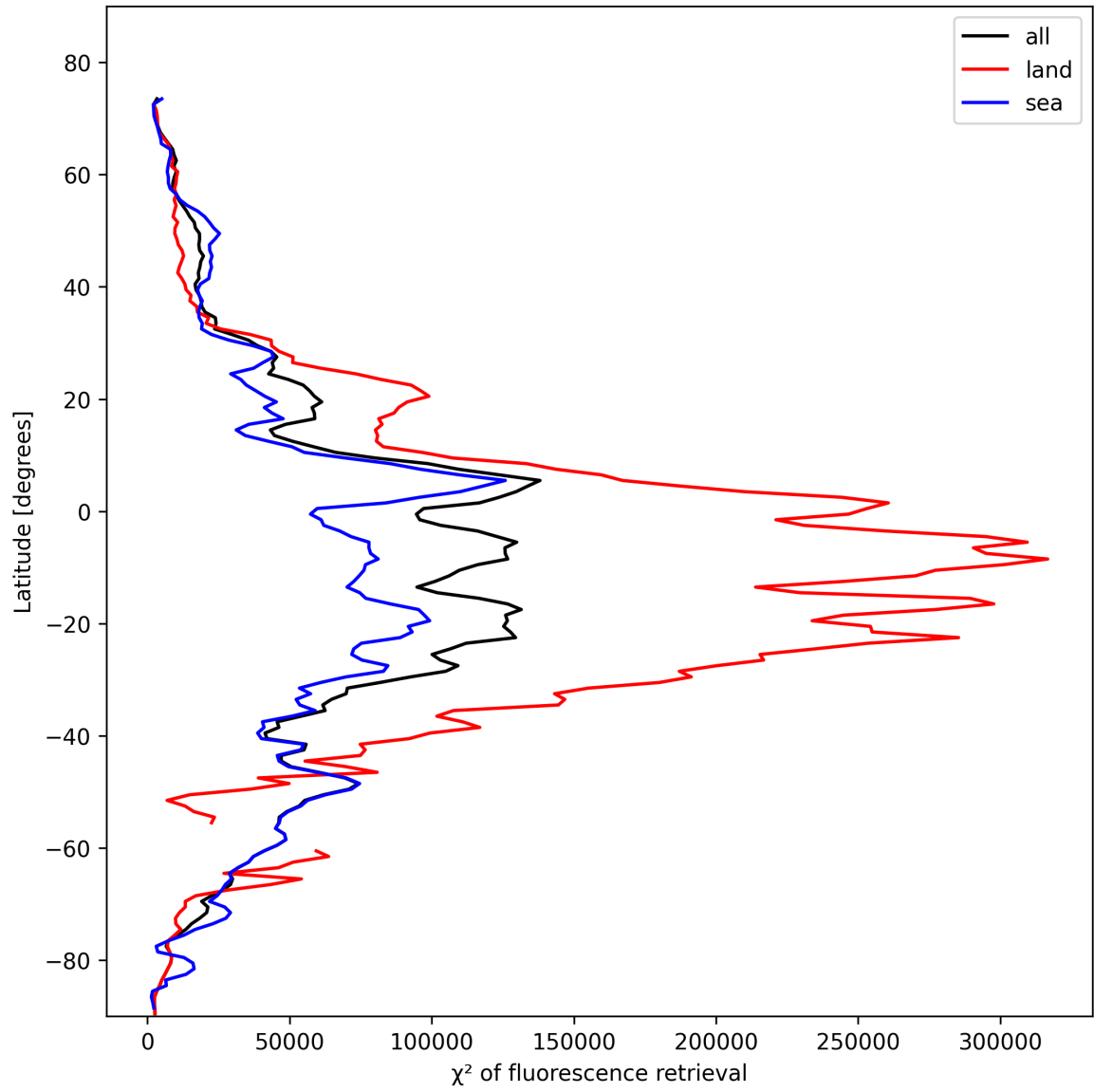
Figure 25: Zonal average of “ \chi^2 of fluorescence retrieval” for 2025-02-06 to 2025-02-08.
