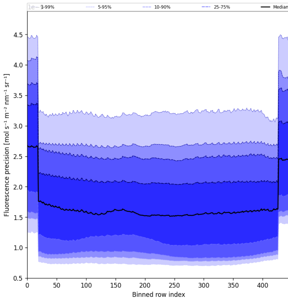
Figure 58: Along track statistics of “Fluorescence precision” for 2025-02-06 to 2025-02-08
