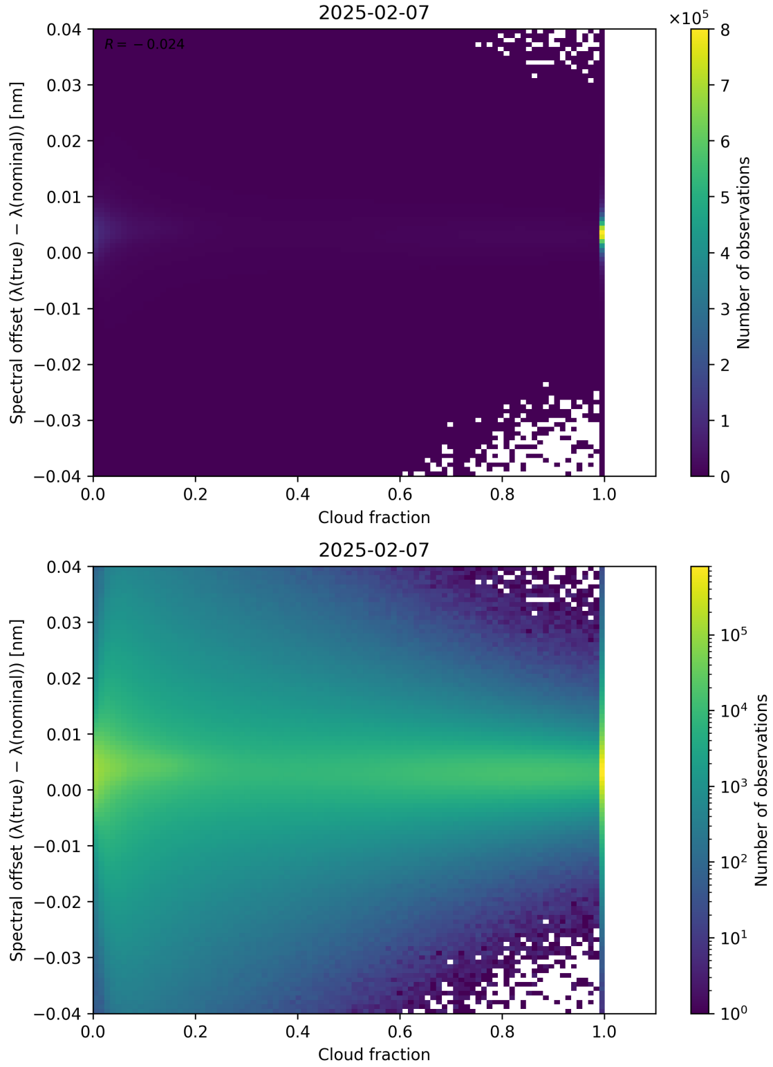
Figure 76: Scatter density plot of “Cloud fraction” against “Spectral offset ( \lambda_{\text{true}} - \lambda_{\text{nominal}} )” for 2025-02-06 to 2025-02-08.
