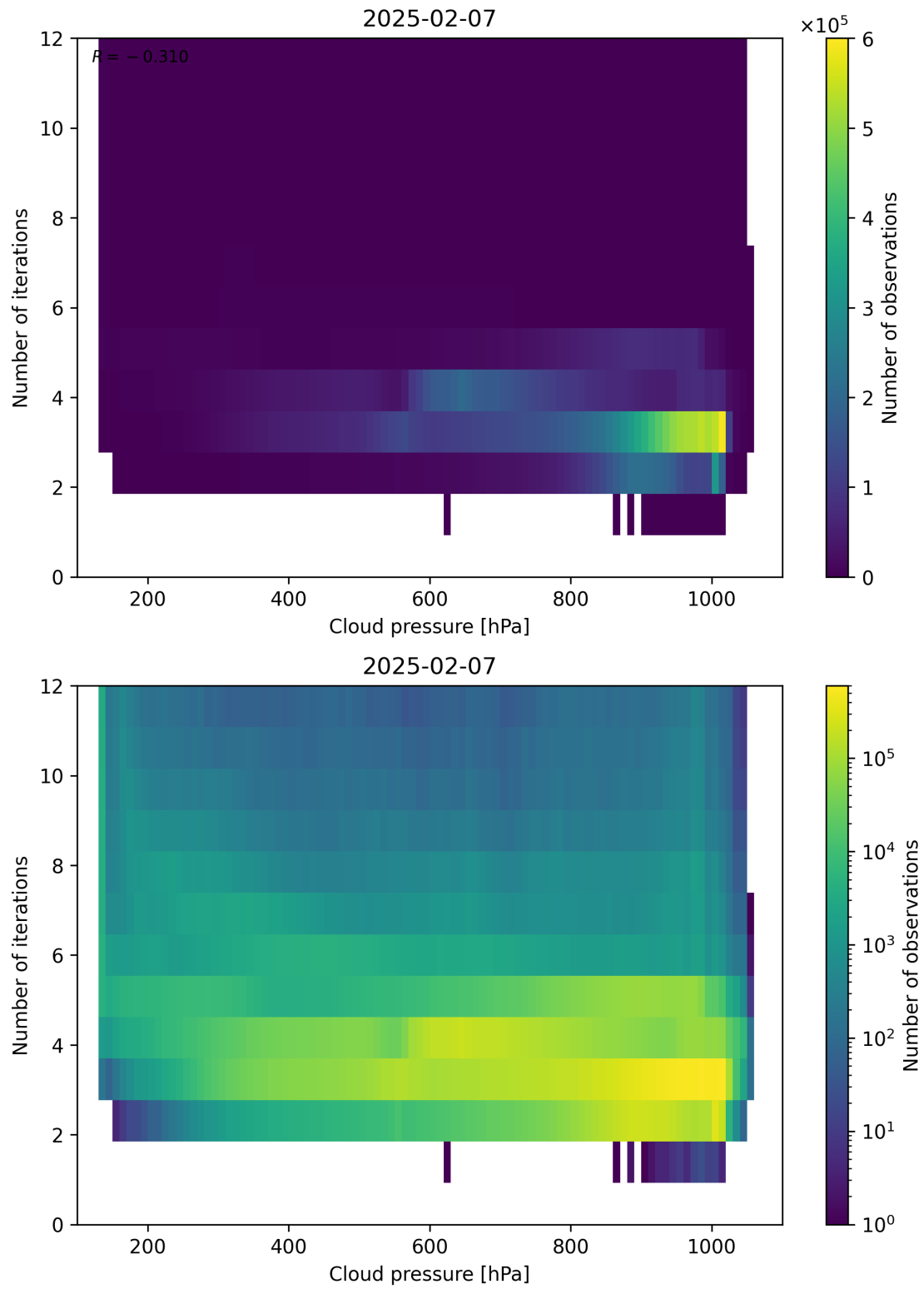
Figure 81: Scatter density plot of “Cloud pressure” against “Number of iterations” for 2025-02-06 to 2025-02-08.
