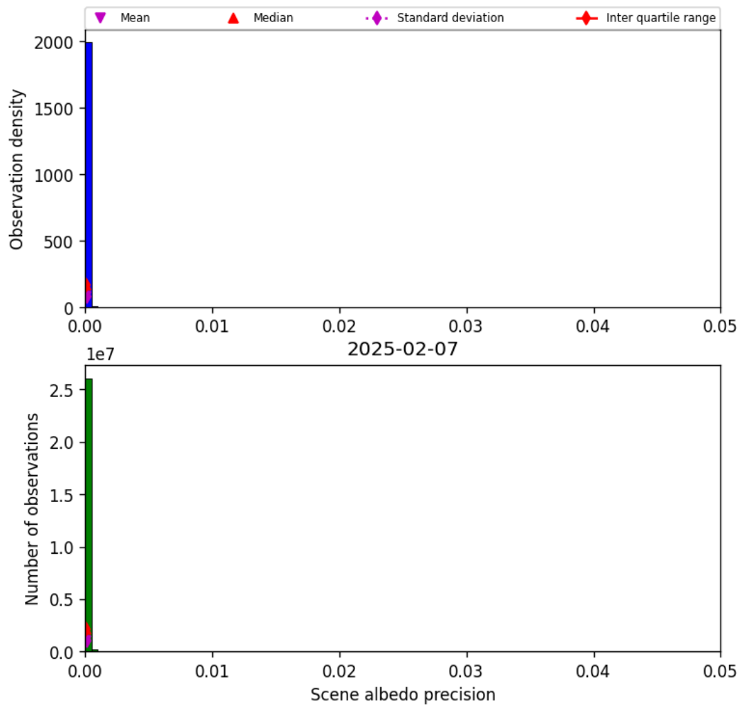
Figure 35: Histogram of “Scene albedo precision” for 2025-02-06 to 2025-02-08
