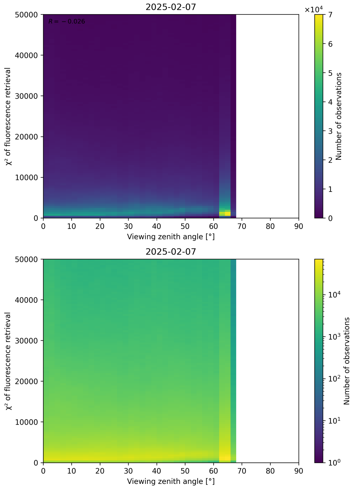
Figure 119: Scatter density plot of “Viewing zenith angle” against “ \chi^2 of fluorescence retrieval” for 2025-02-06 to 2025-02-08.
