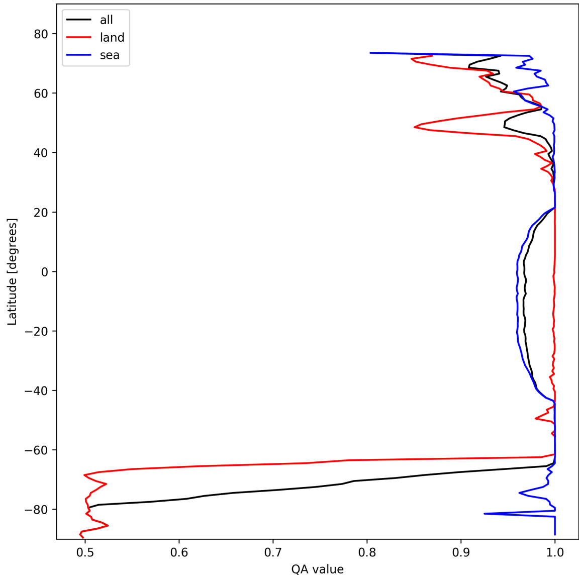
Figure 12: Zonal average of “QA value” for 2025-02-06 to 2025-02-08.
