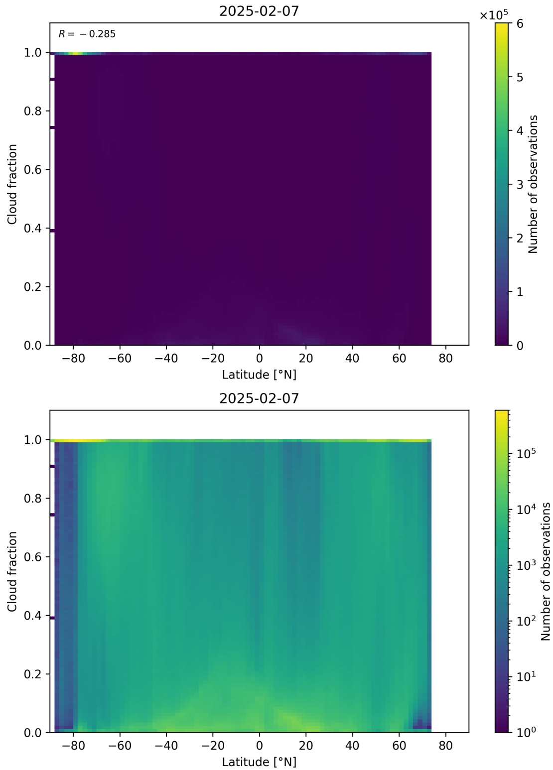
Figure 90: Scatter density plot of “Latitude” against “Cloud fraction” for 2025-02-06 to 2025-02-08.
