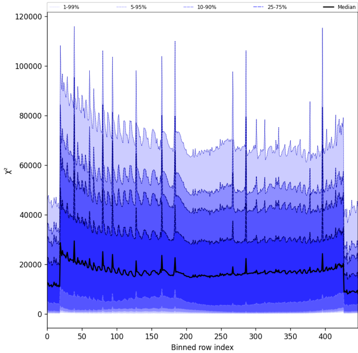
Figure 55: Along track statistics of “ \chi^2 ” for 2025-02-06 to 2025-02-08
