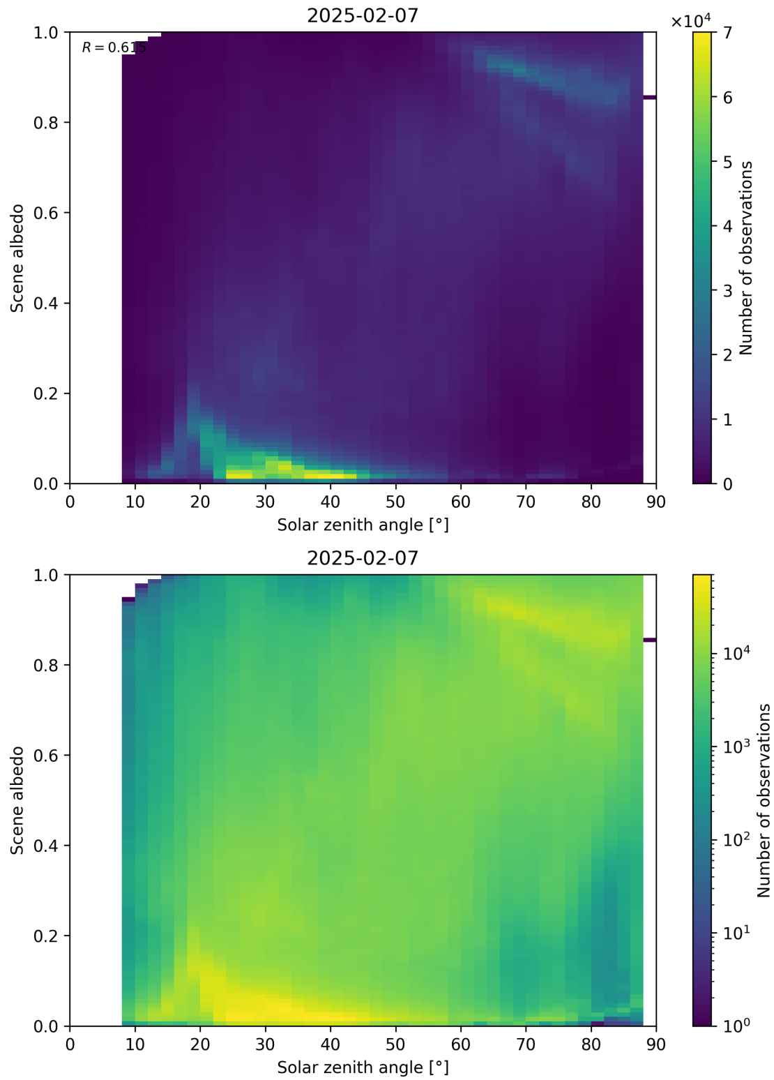
Figure 116: Scatter density plot of “Solar zenith angle” against “Scene albedo” for 2025-02-06 to 2025-02-08.
