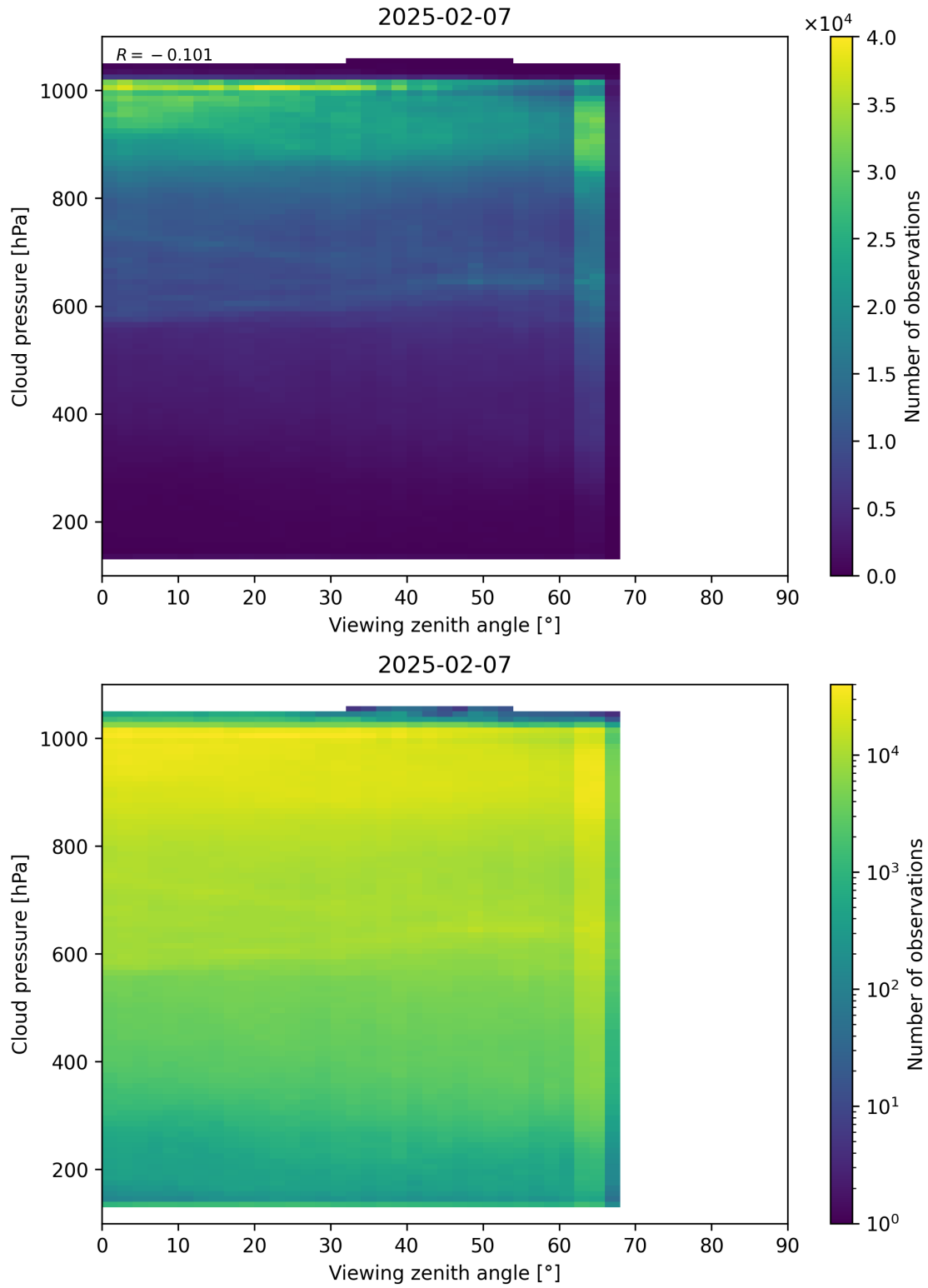
Figure 121: Scatter density plot of “Viewing zenith angle” against “Cloud pressure” for 2025-02-06 to 2025-02-08.
