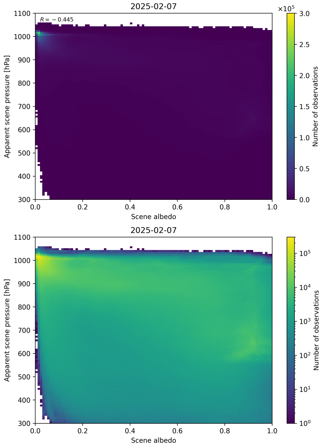
Figure 102: Scatter density plot of “Scene albedo” against “Apparent scene pressure” for 2025-02-06 to 2025-02-08.
