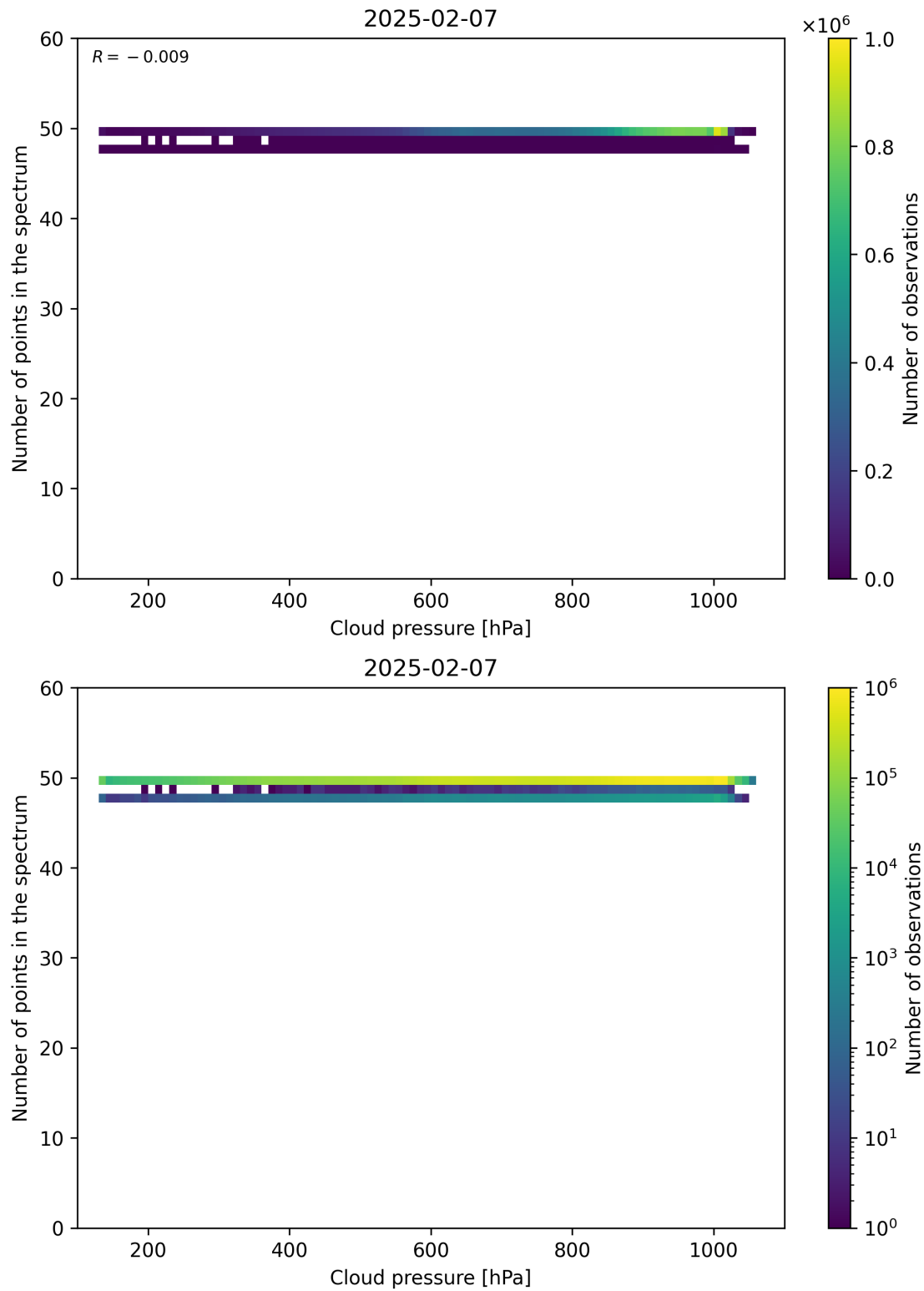
Figure 82: Scatter density plot of “Cloud pressure” against “Number of points in the spectrum” for 2025-02-06 to 2025-02-08.
