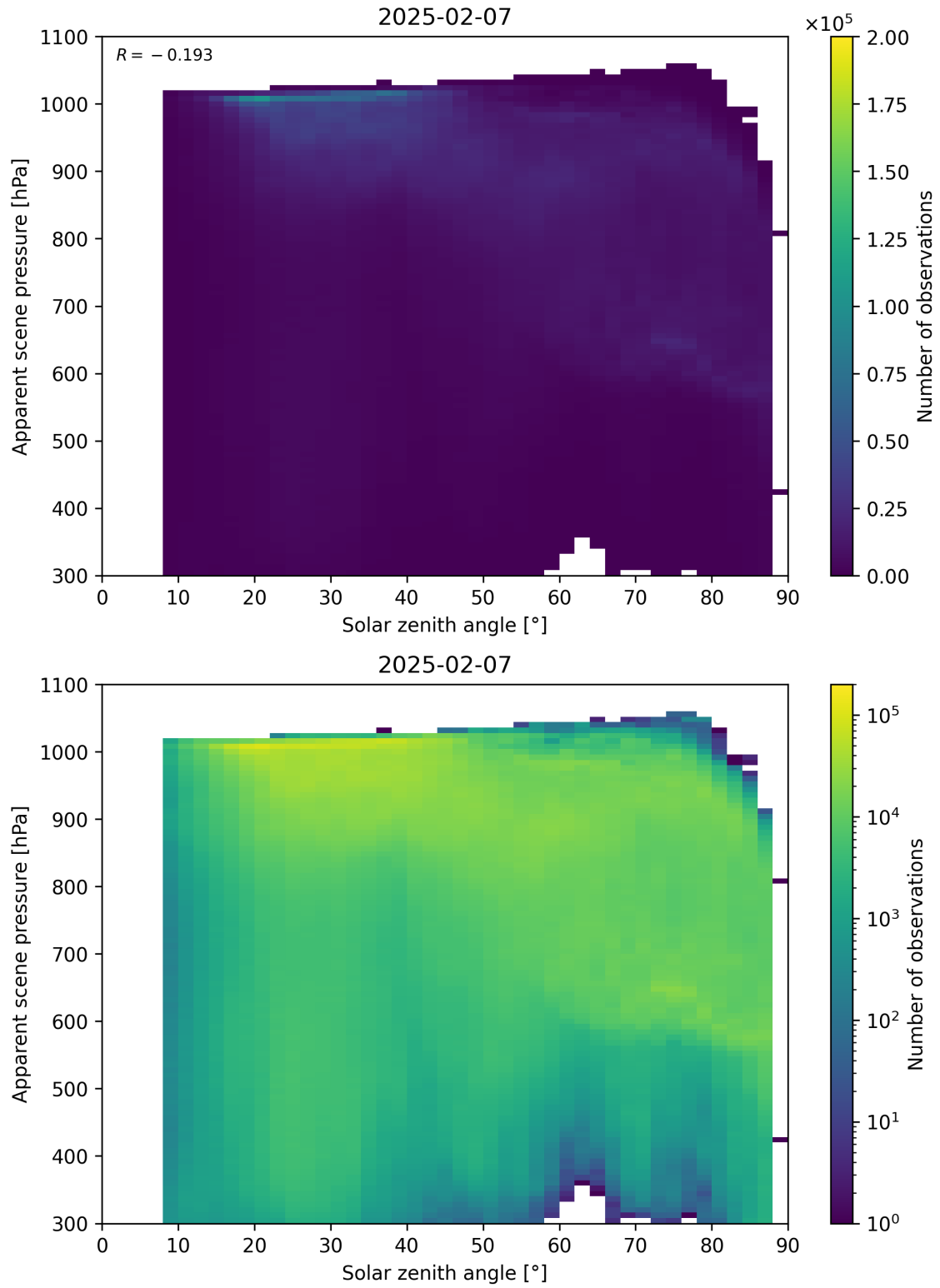
Figure 108: Scatter density plot of “Solar zenith angle” against “Apparent scene pressure” for 2025-02-06 to 2025-02-08.
