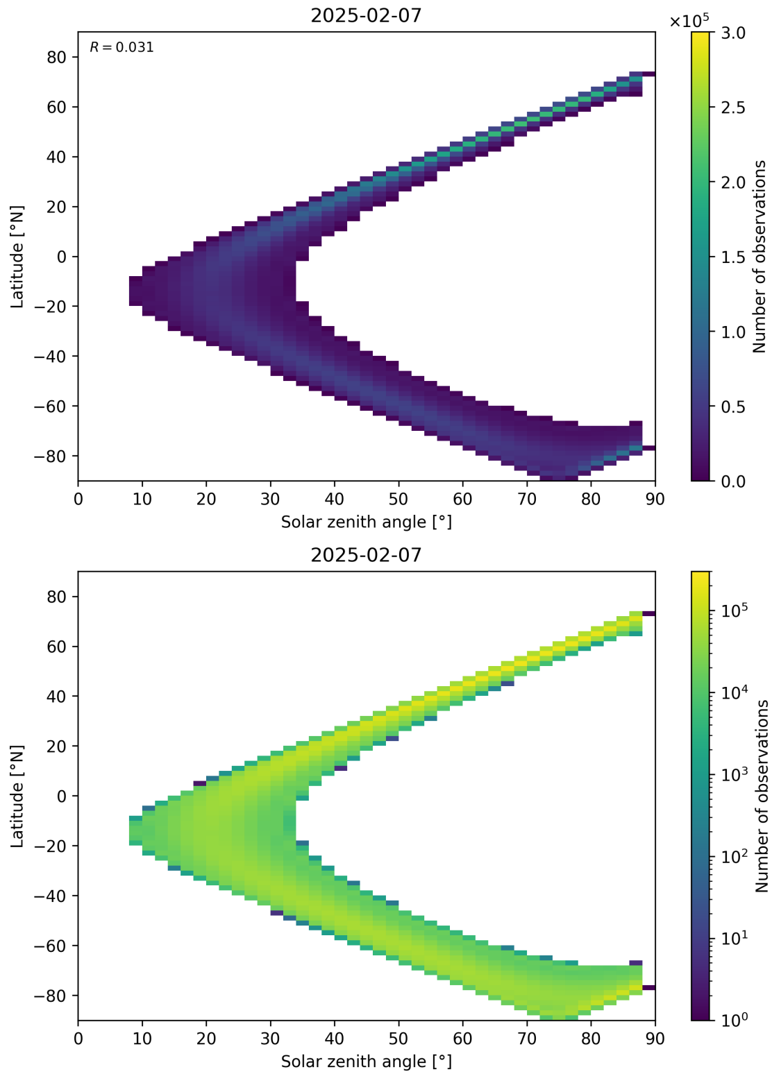
Figure 113: Scatter density plot of “Solar zenith angle” against “Latitude” for 2025-02-06 to 2025-02-08.
