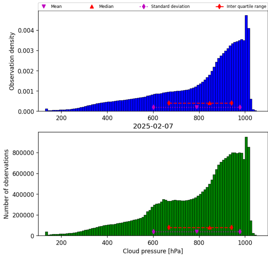
Figure 30: Histogram of “Cloud pressure” for 2025-02-06 to 2025-02-08
