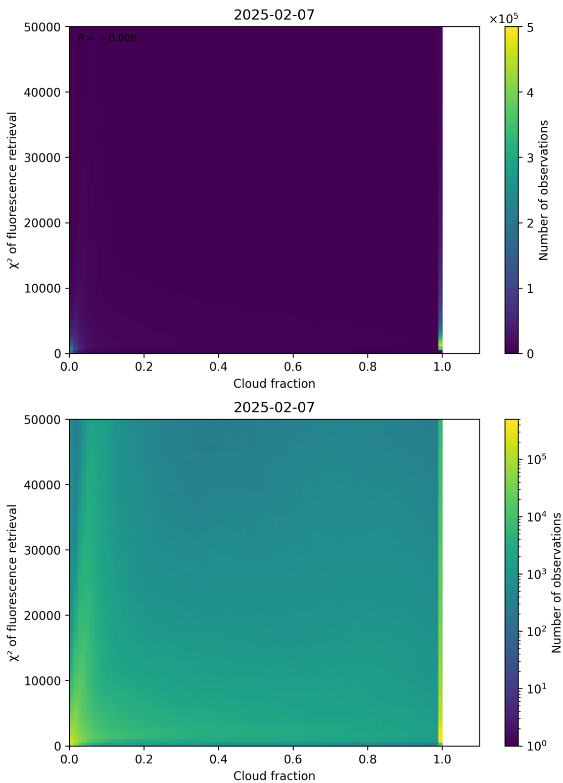
Figure 71: Scatter density plot of “Cloud fraction” against “ \chi^2 of fluorescence retrieval” for 2025-02-06 to 2025-02-08.
