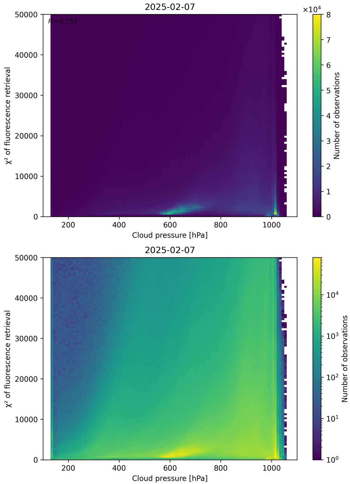
Figure 78: Scatter density plot of “Cloud pressure” against “ \chi^2 of fluorescence retrieval” for 2025-02-06 to 2025-02-08.
