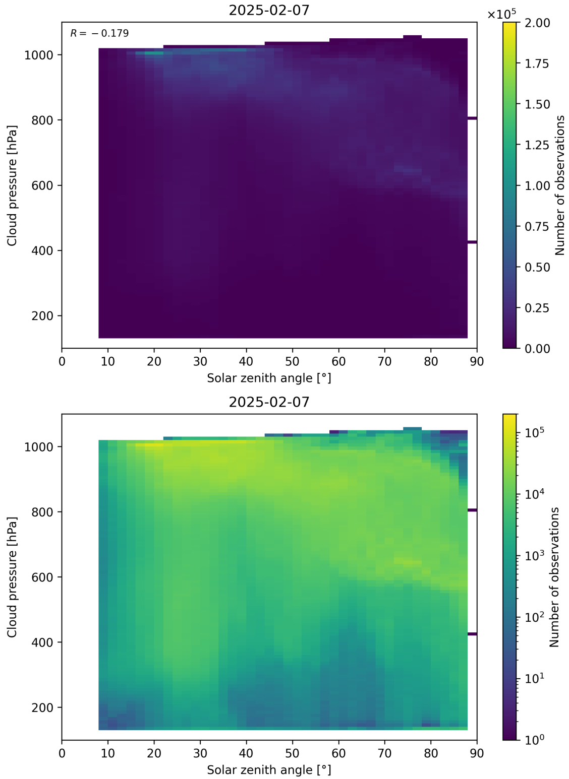
Figure 111: Scatter density plot of “Solar zenith angle” against “Cloud pressure” for 2025-02-06 to 2025-02-08.
