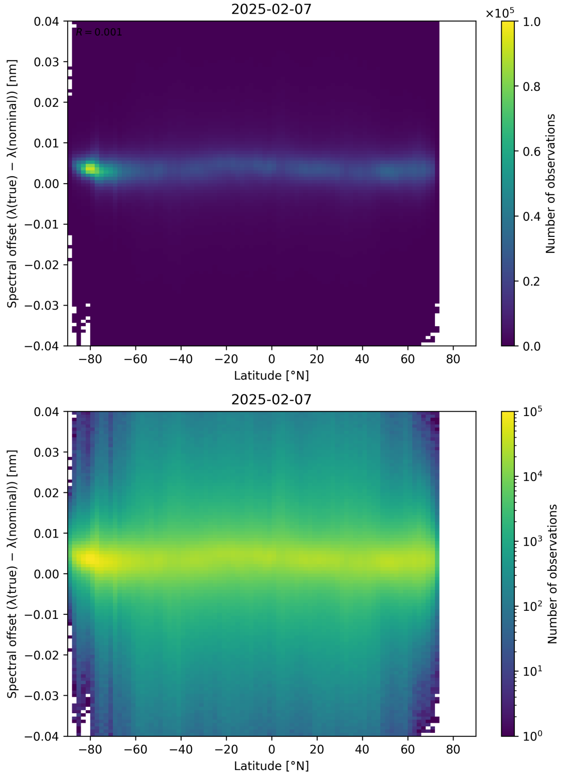
Figure 96: Scatter density plot of “Latitude” against “Spectral offset ( \lambda_{\text{true}} - \lambda_{\text{nominal}} )” for 2025-02-06 to 2025-02-08.
