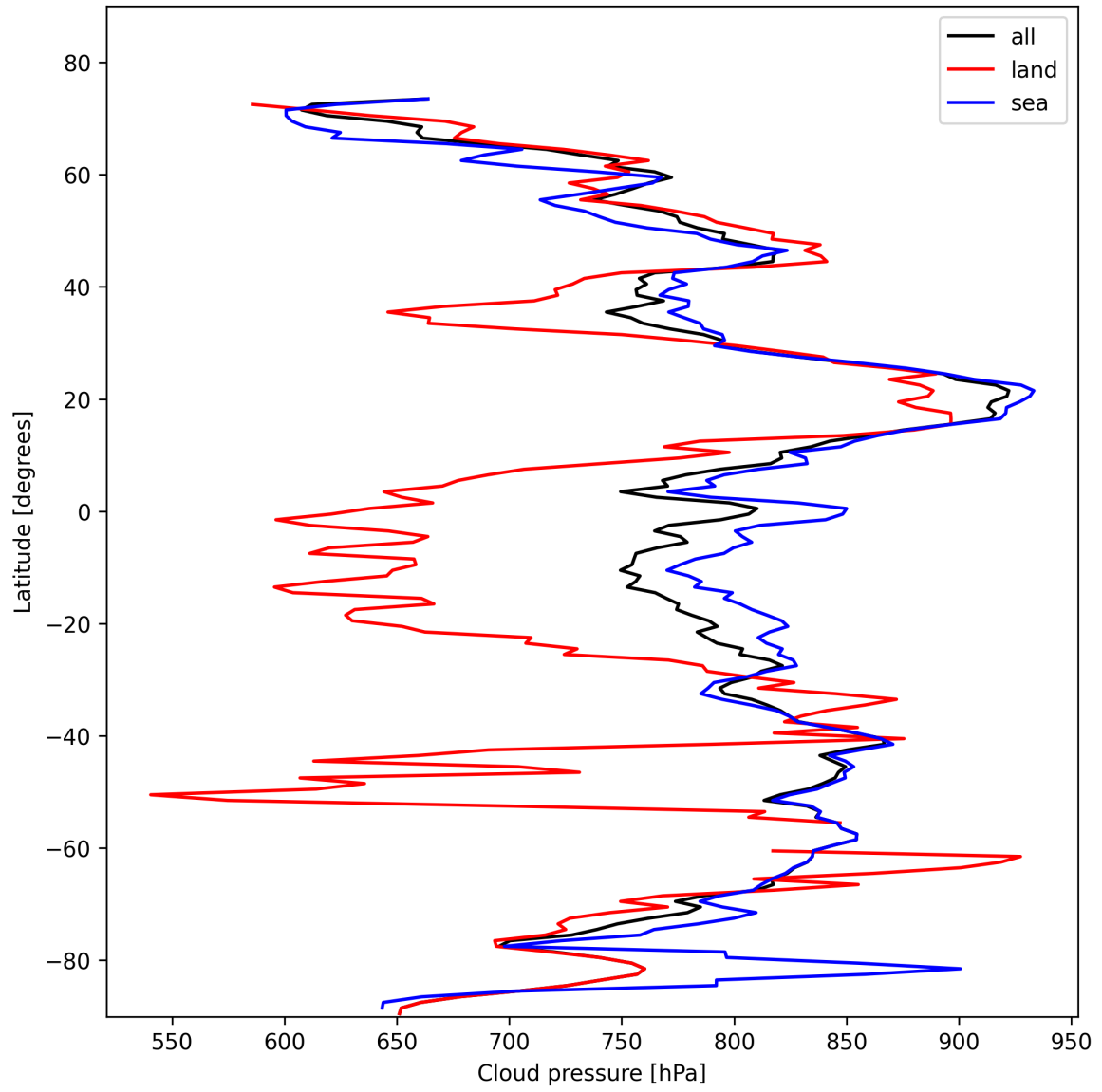
Figure 13: Zonal average of “Cloud pressure” for 2025-02-06 to 2025-02-08.
