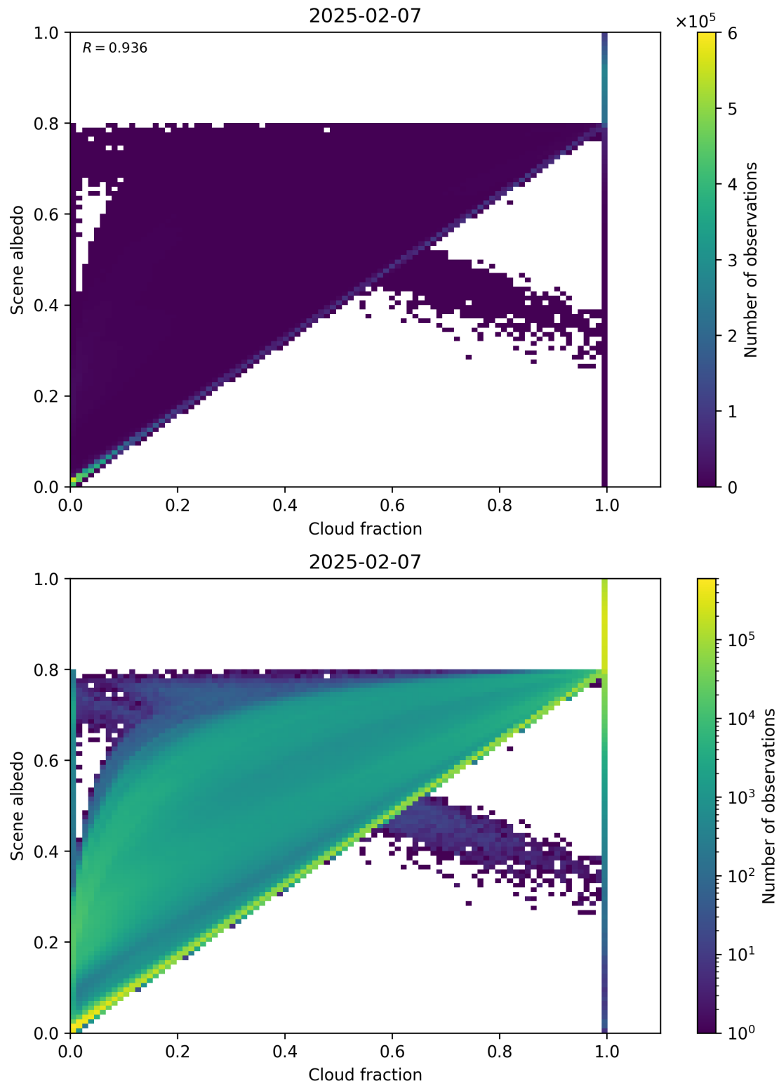
Figure 75: Scatter density plot of “Cloud fraction” against “Scene albedo” for 2025-02-06 to 2025-02-08.
