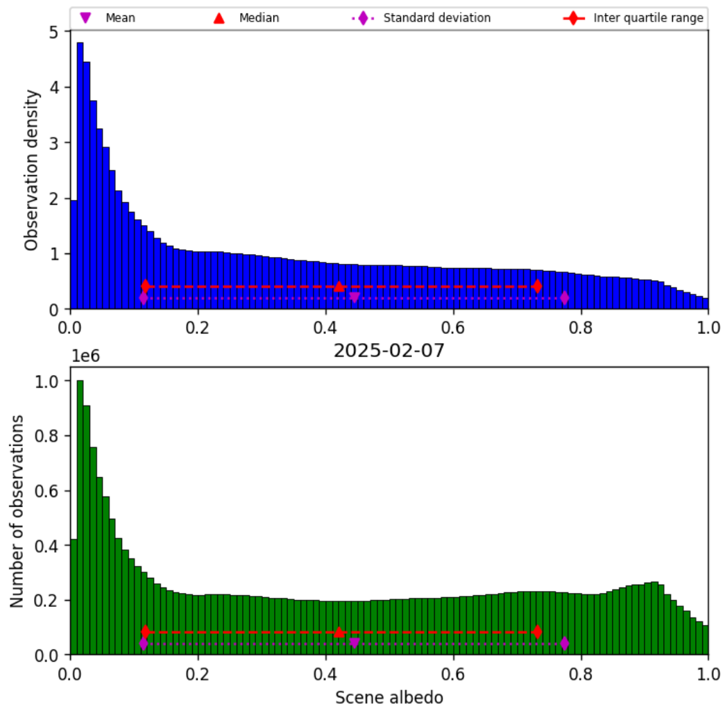
Figure 34: Histogram of “Scene albedo” for 2025-02-06 to 2025-02-08
