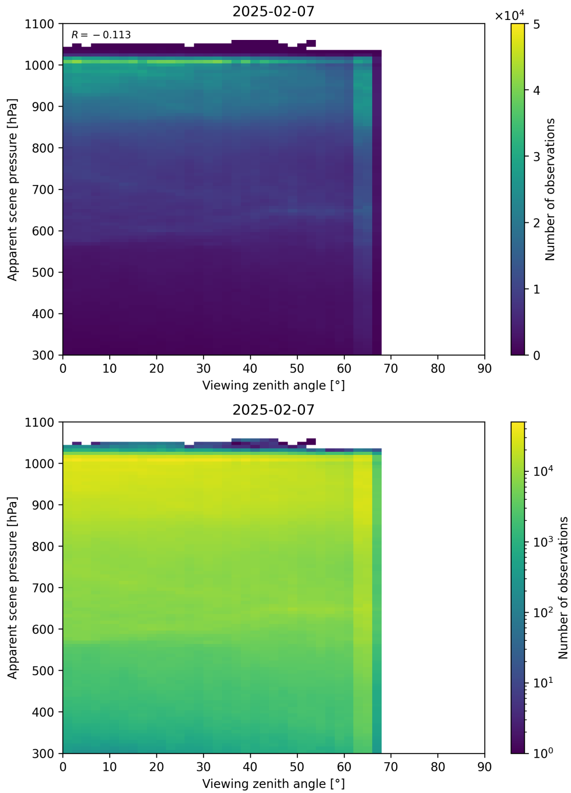
Figure 118: Scatter density plot of “Viewing zenith angle” against “Apparent scene pressure” for 2025-02-06 to 2025-02-08.
