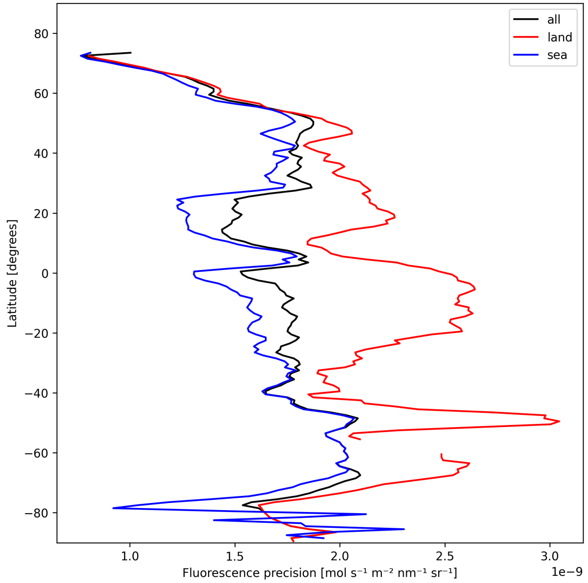
Figure 24: Zonal average of “Fluorescence precision” for 2025-02-06 to 2025-02-08.
