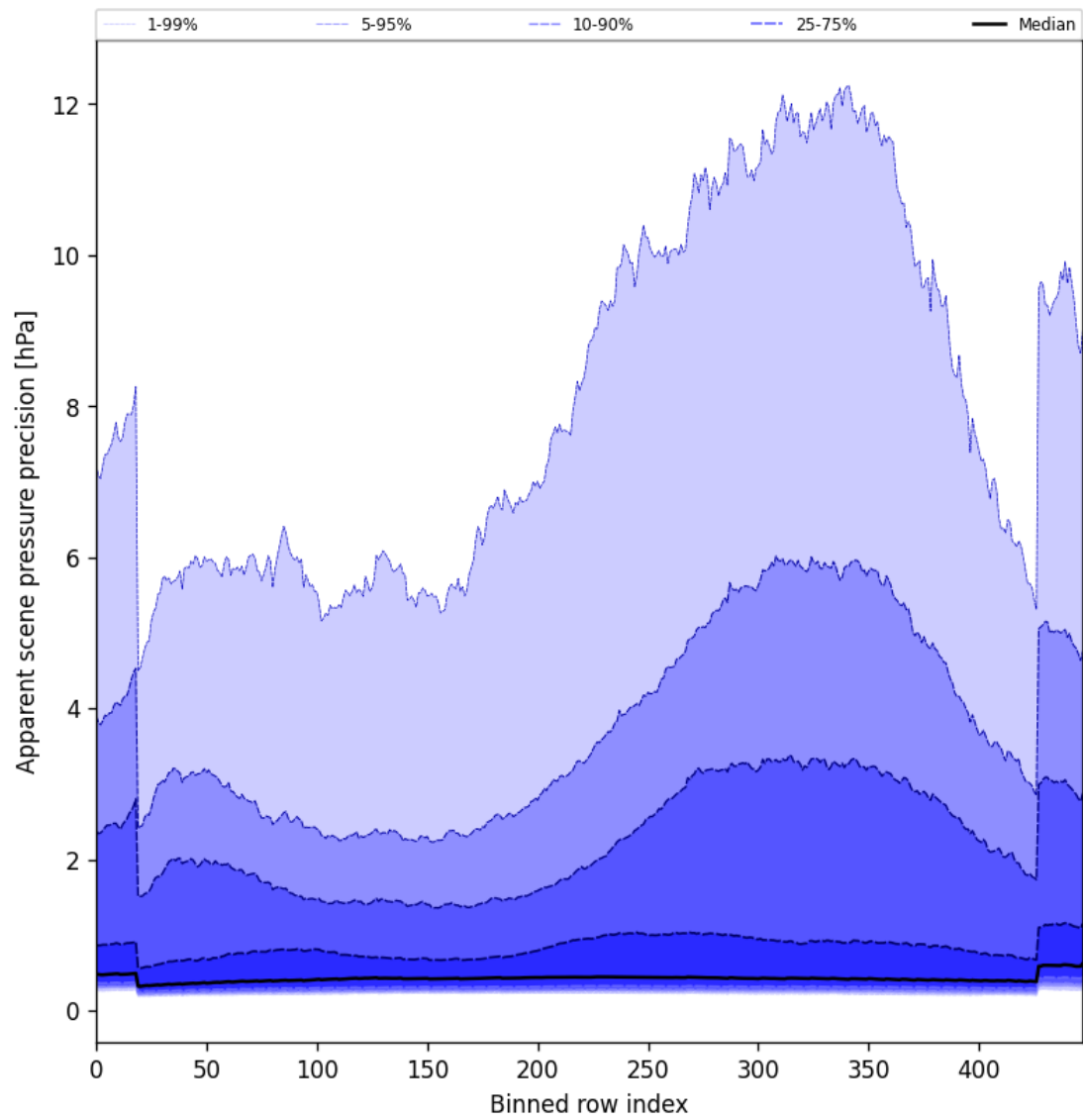
Figure 54: Along track statistics of “Apparent scene pressure precision” for 2025-02-06 to 2025-02-08
