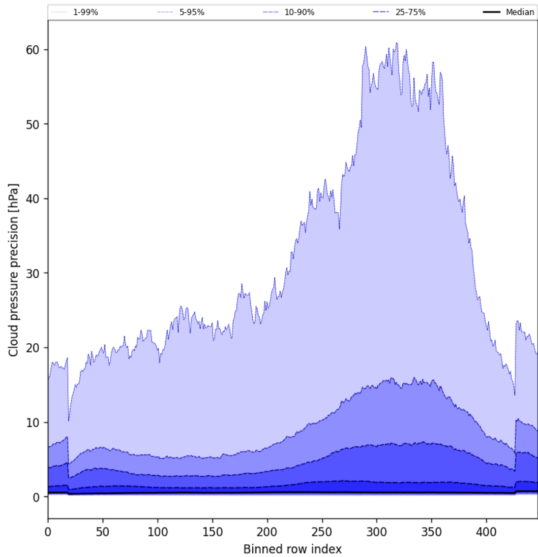
Figure 48: Along track statistics of “Cloud pressure precision” for 2025-02-06 to 2025-02-08
