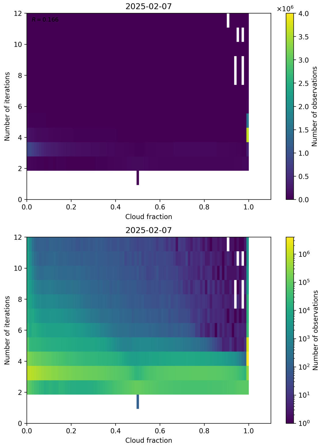
Figure 73: Scatter density plot of “Cloud fraction” against “Number of iterations” for 2025-02-06 to 2025-02-08.
