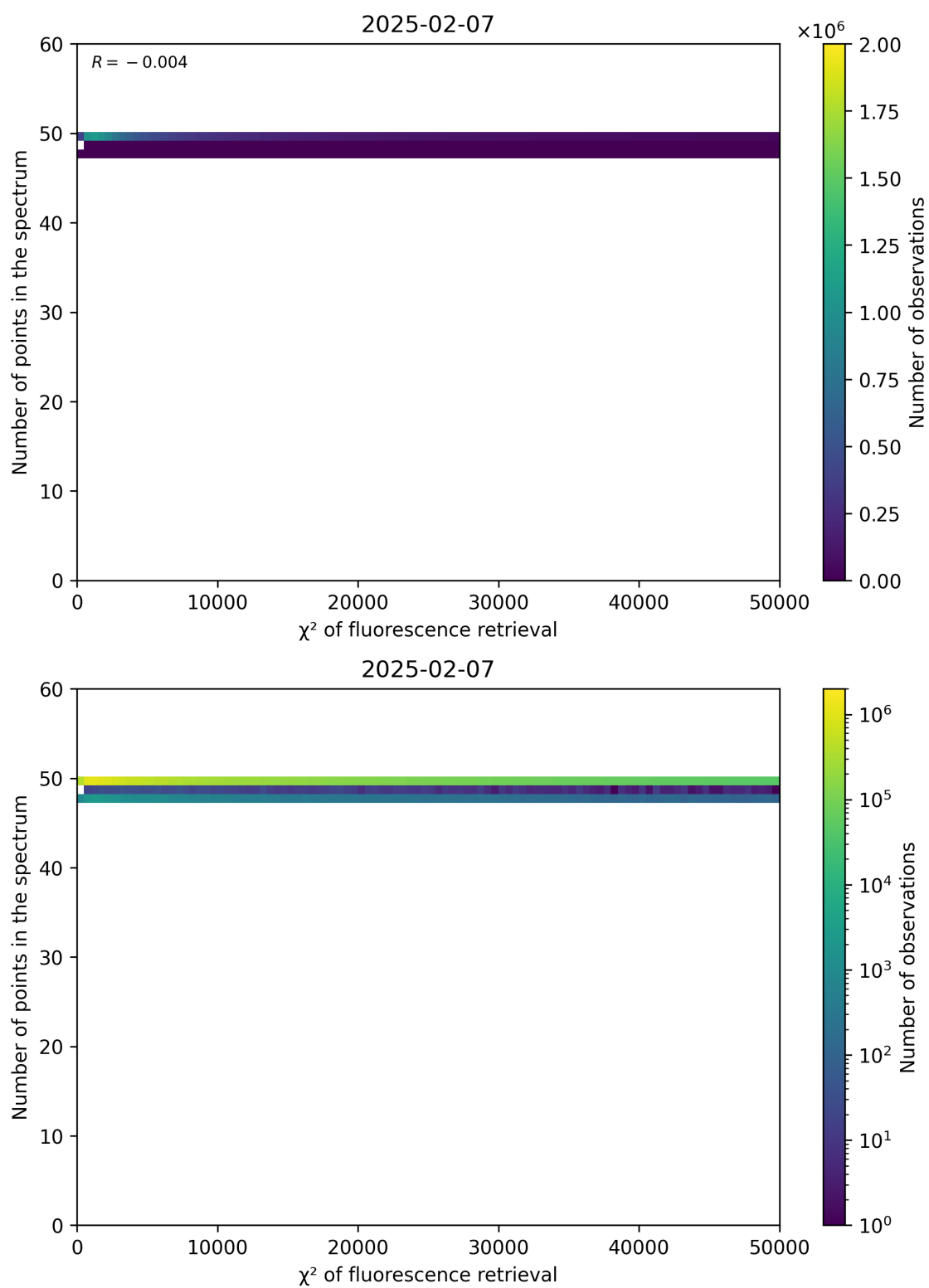
Figure 68: Scatter density plot of “ \chi^2 of fluorescence retrieval” against “Number of points in the spectrum” for 2025-02-06 to 2025-02-08.
