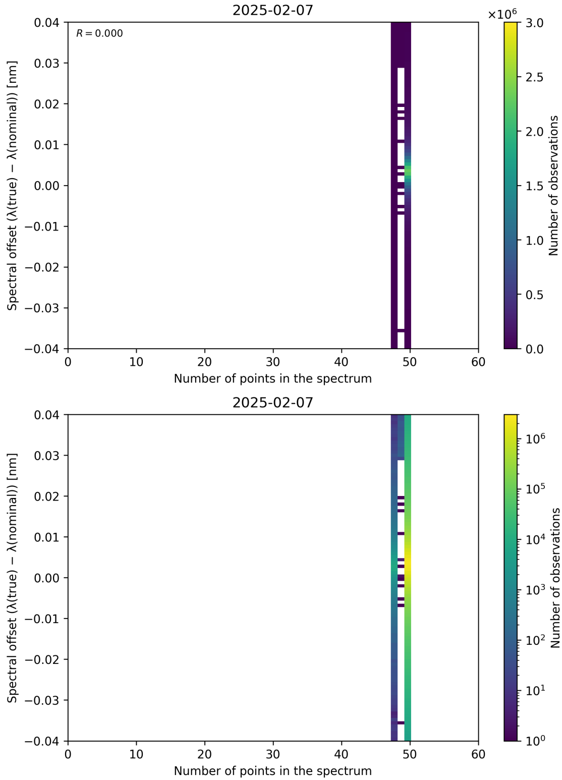
Figure 101: Scatter density plot of “Number of points in the spectrum” against “Spectral offset ( \lambda_{\text{true}} - \lambda_{\text{nominal}} )” for 2025-02-06 to 2025-02-08.
