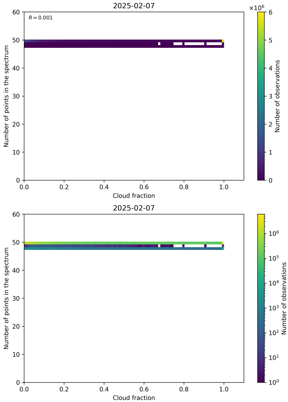
Figure 74: Scatter density plot of “Cloud fraction” against “Number of points in the spectrum” for 2025-02-06 to 2025-02-08.
