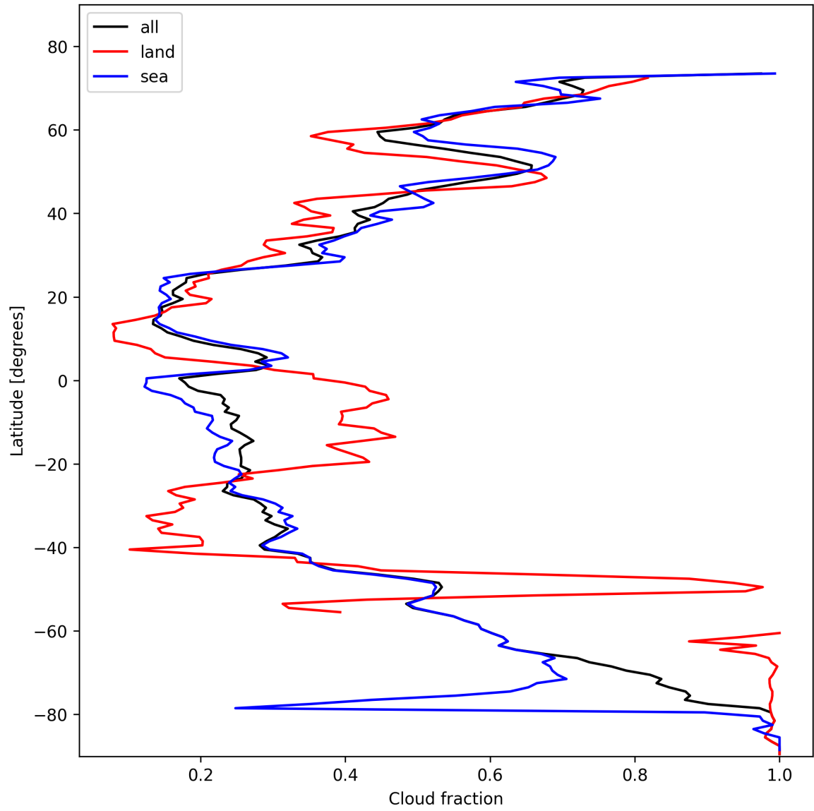
Figure 15: Zonal average of “Cloud fraction” for 2025-02-06 to 2025-02-08.
