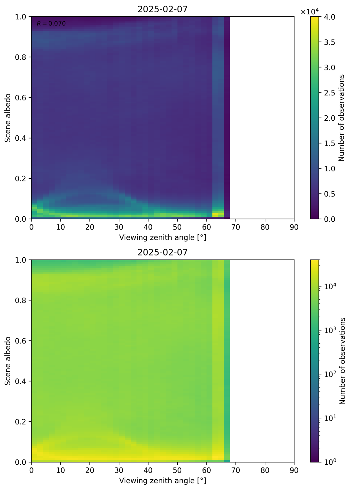
Figure 126: Scatter density plot of “Viewing zenith angle” against “Scene albedo” for 2025-02-06 to 2025-02-08.
