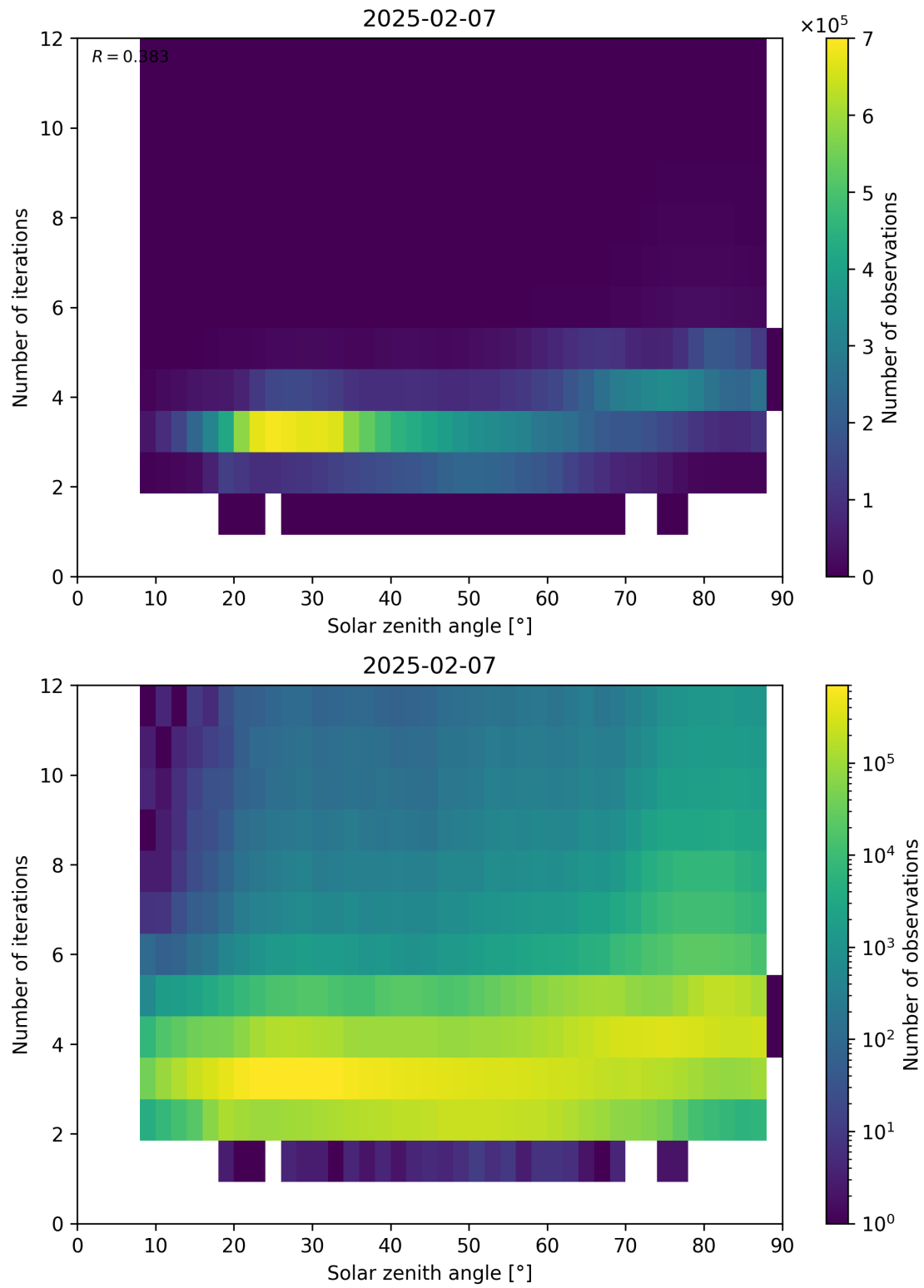
Figure 114: Scatter density plot of “Solar zenith angle” against “Number of iterations” for 2025-02-06 to 2025-02-08.
