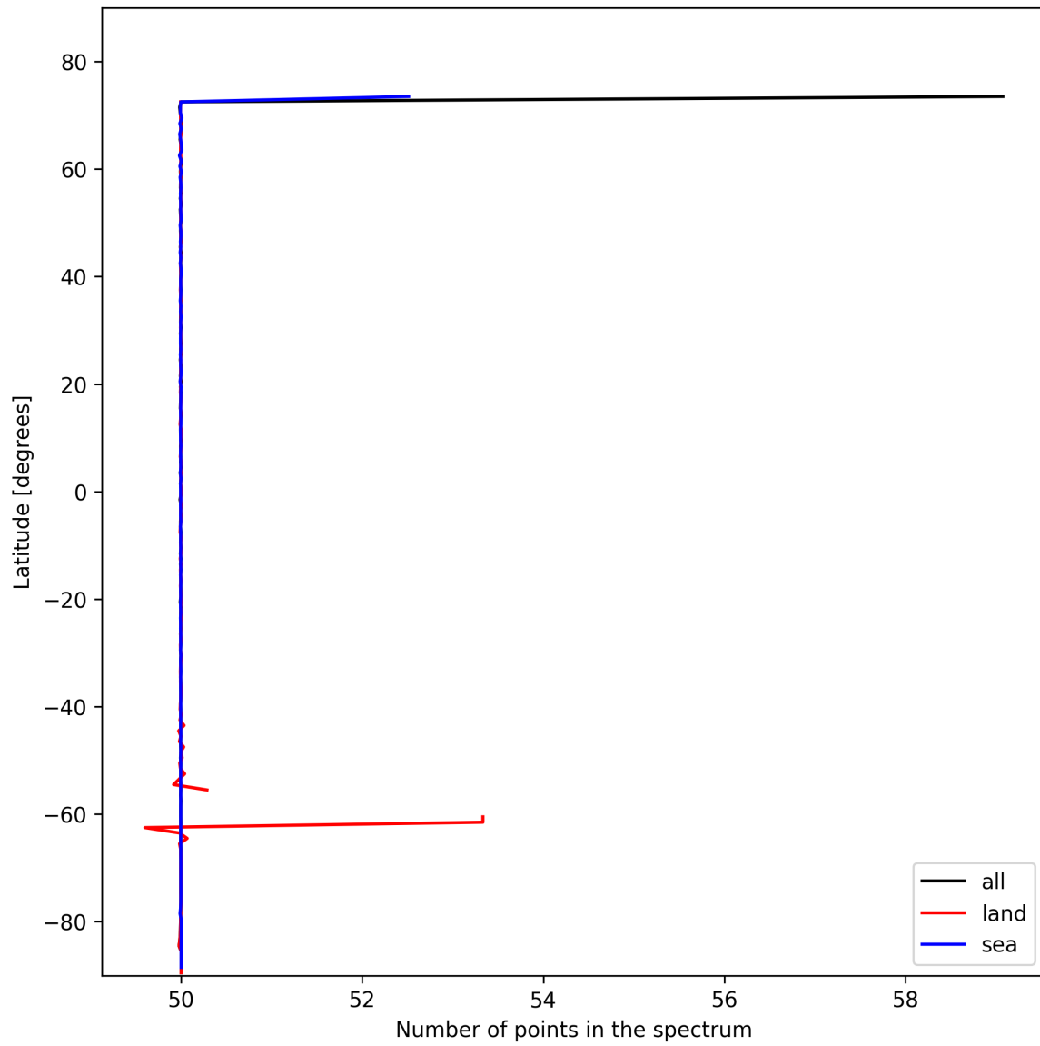
Figure 27: Zonal average of “Number of points in the spectrum” for 2025-02-06 to 2025-02-08.
