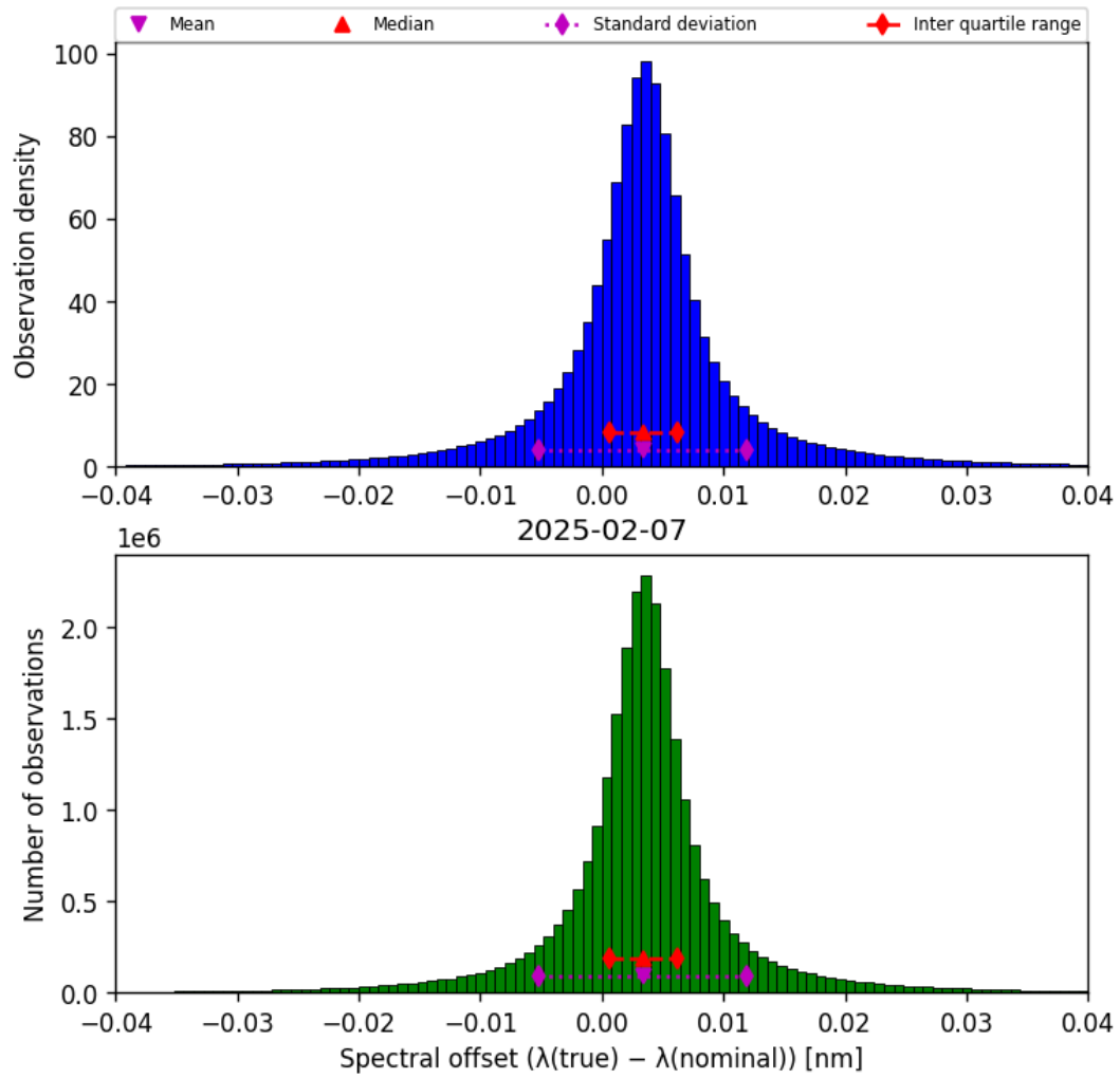
Figure 45: Histogram of “Spectral offset ( \lambda_{\text{true}} - \lambda_{\text{nominal}} )” for 2025-02-06 to 2025-02-08
