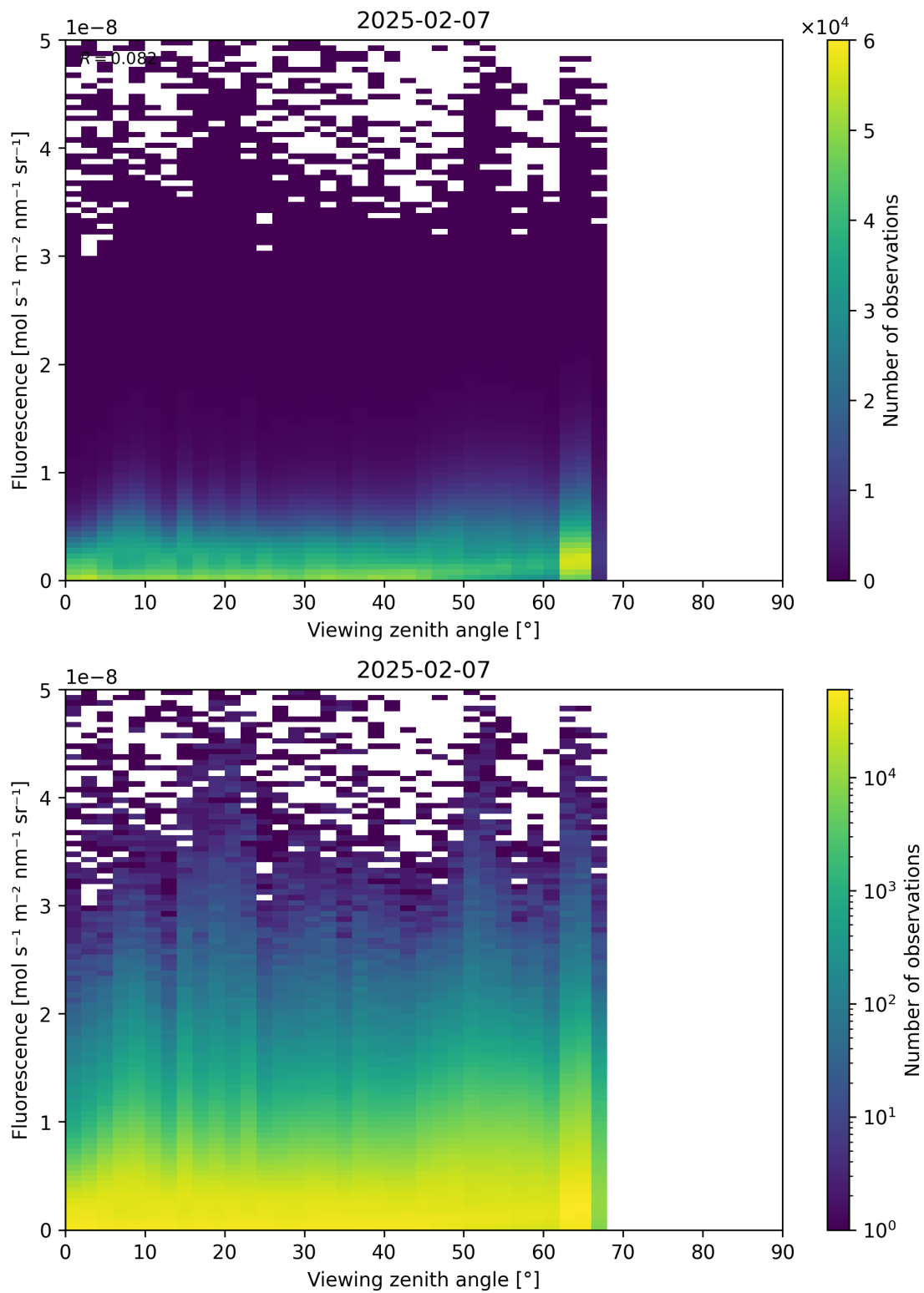
Figure 122: Scatter density plot of “Viewing zenith angle” against “Fluorescence” for 2025-02-06 to 2025-02-08.
