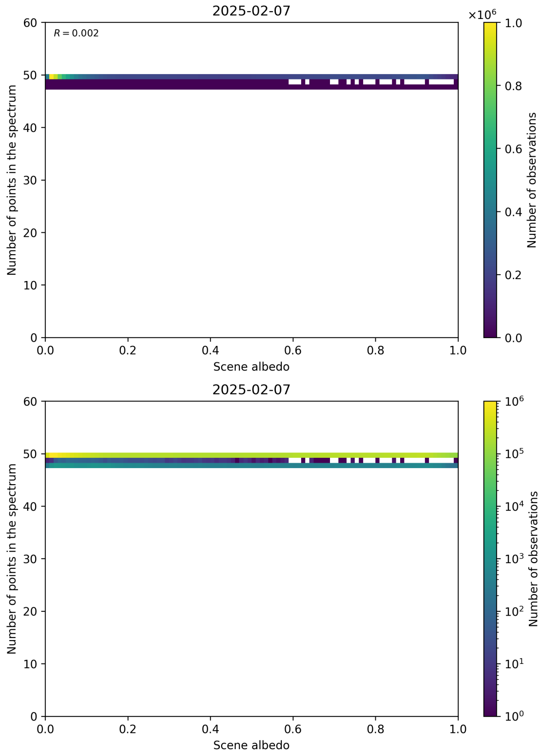
Figure 106: Scatter density plot of “Scene albedo” against “Number of points in the spectrum” for 2025-02-06 to 2025-02-08.
