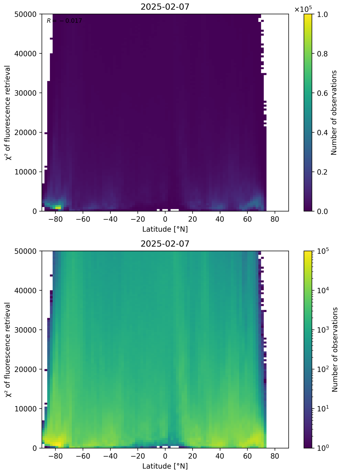
Figure 89: Scatter density plot of “Latitude” against “ \chi^2 of fluorescence retrieval” for 2025-02-06 to 2025-02-08.
