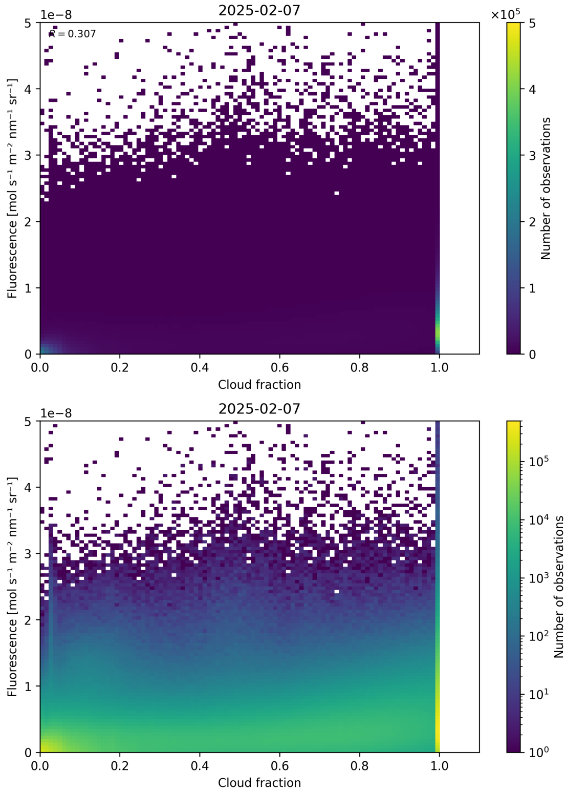
Figure 72: Scatter density plot of “Cloud fraction” against “Fluorescence” for 2025-02-06 to 2025-02-08.
