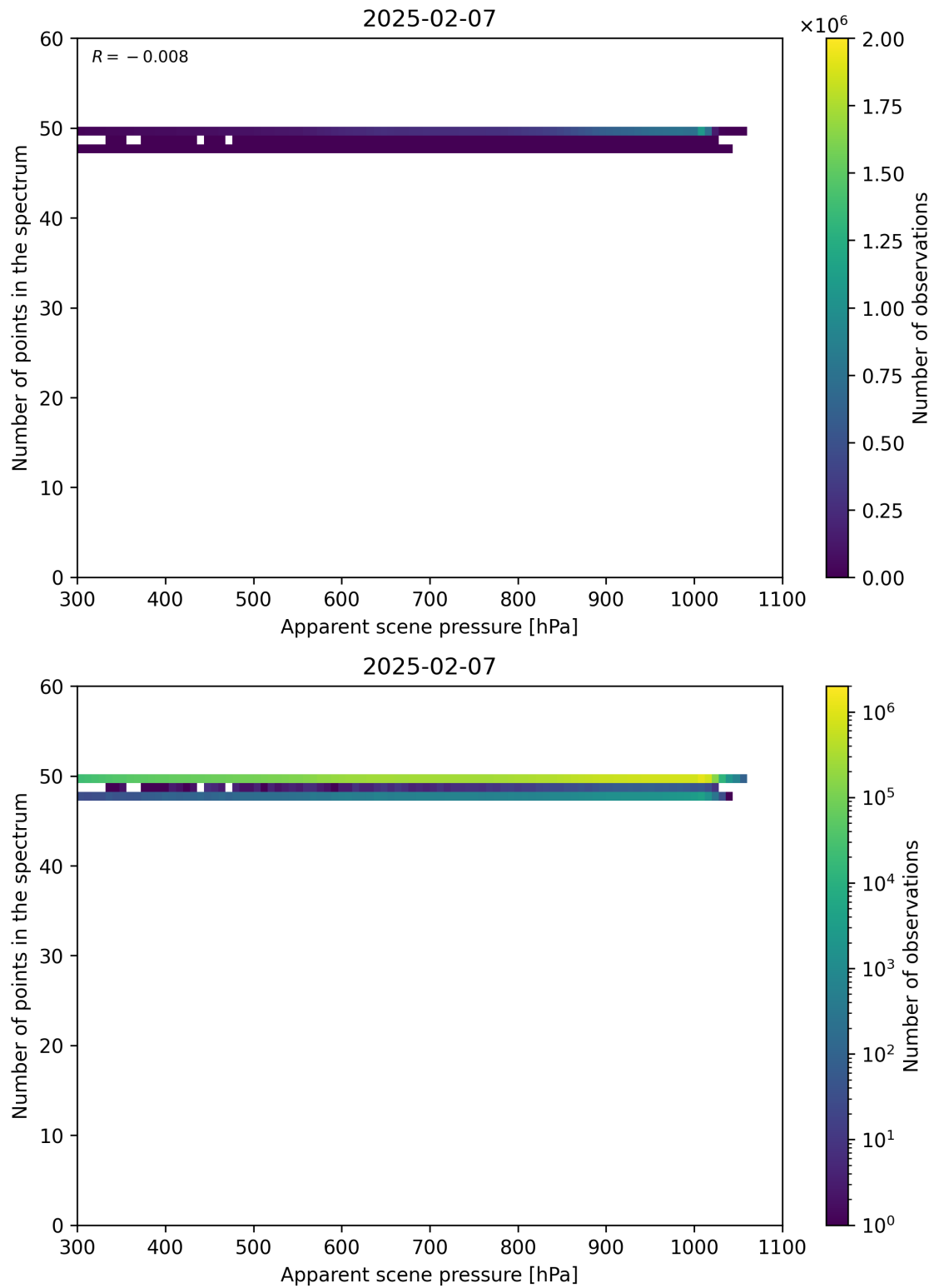
Figure 66: Scatter density plot of “Apparent scene pressure” against “Number of points in the spectrum” for 2025-02-06 to 2025-02-08.
