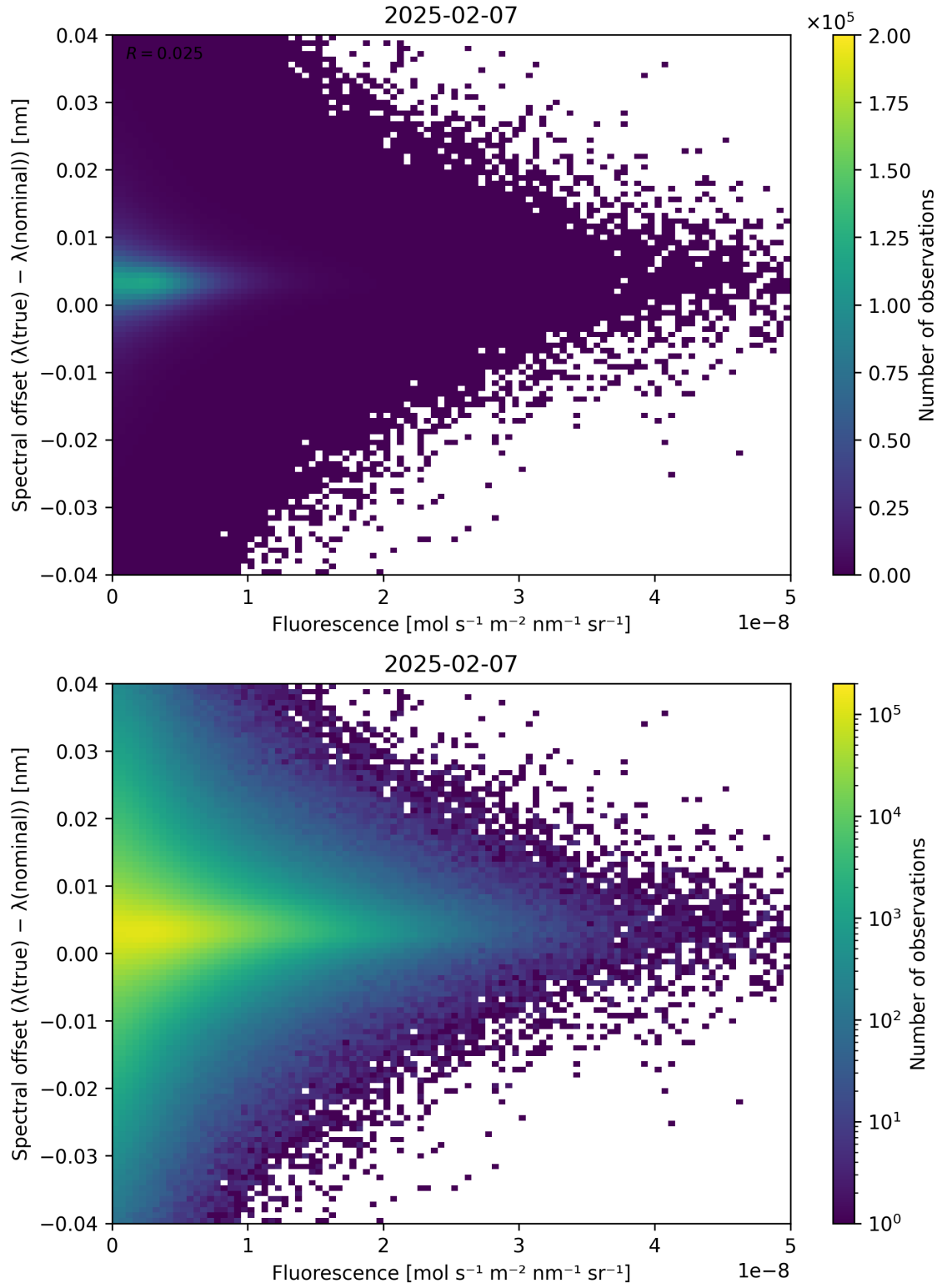
Figure 87: Scatter density plot of “Fluorescence” against “Spectral offset ( \lambda_{\text{true}} - \lambda_{\text{nominal}} )” for 2025-02-06 to 2025-02-08.
