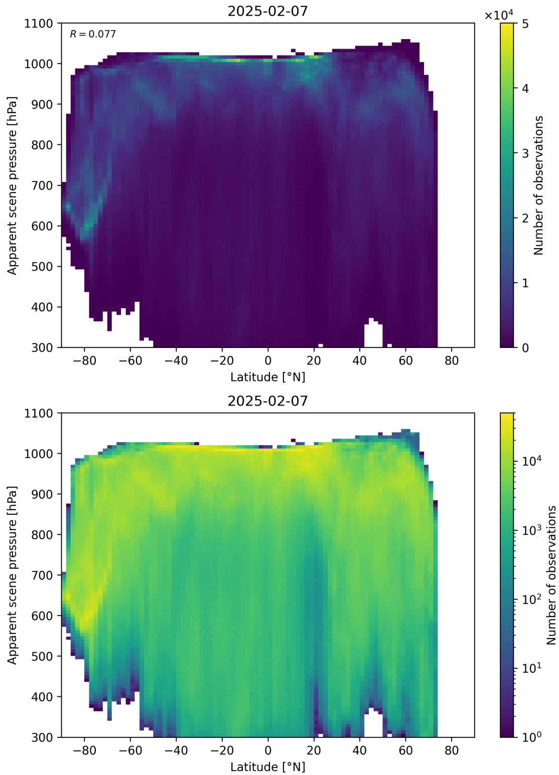
Figure 88: Scatter density plot of “Latitude” against “Apparent scene pressure” for 2025-02-06 to 2025-02-08.
