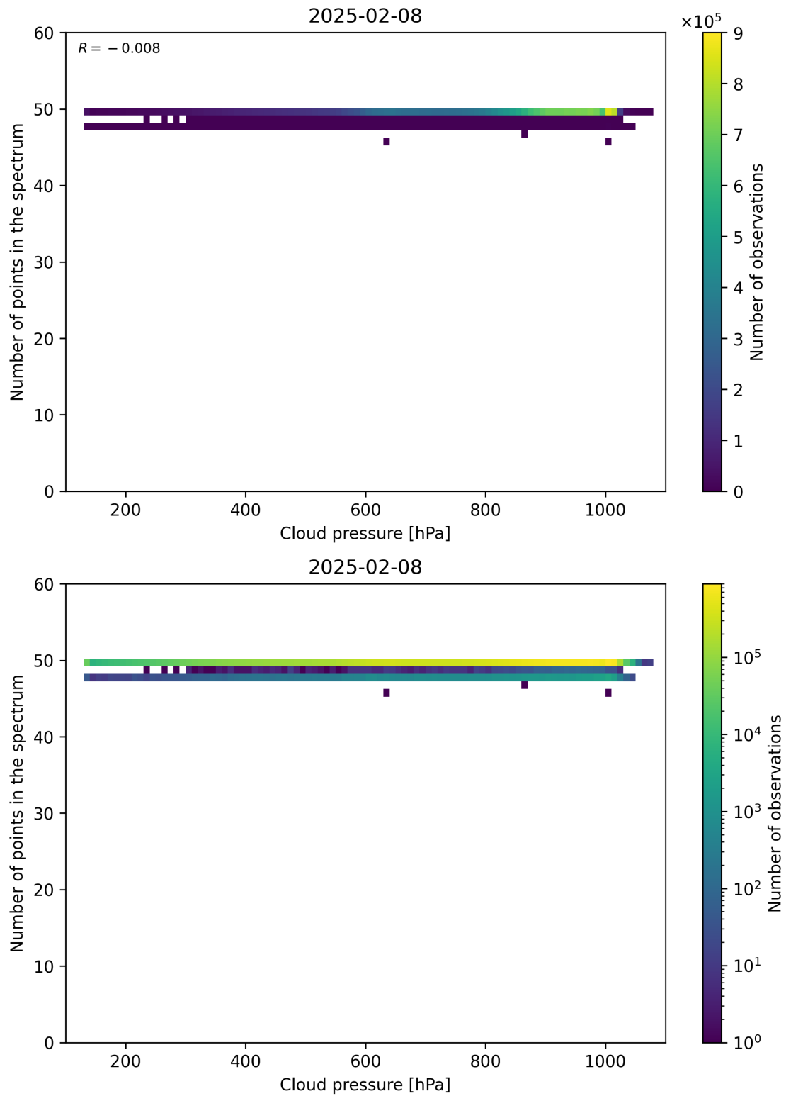
Figure 82: Scatter density plot of “Cloud pressure” against “Number of points in the spectrum” for 2025-02-08 to 2025-02-09.
