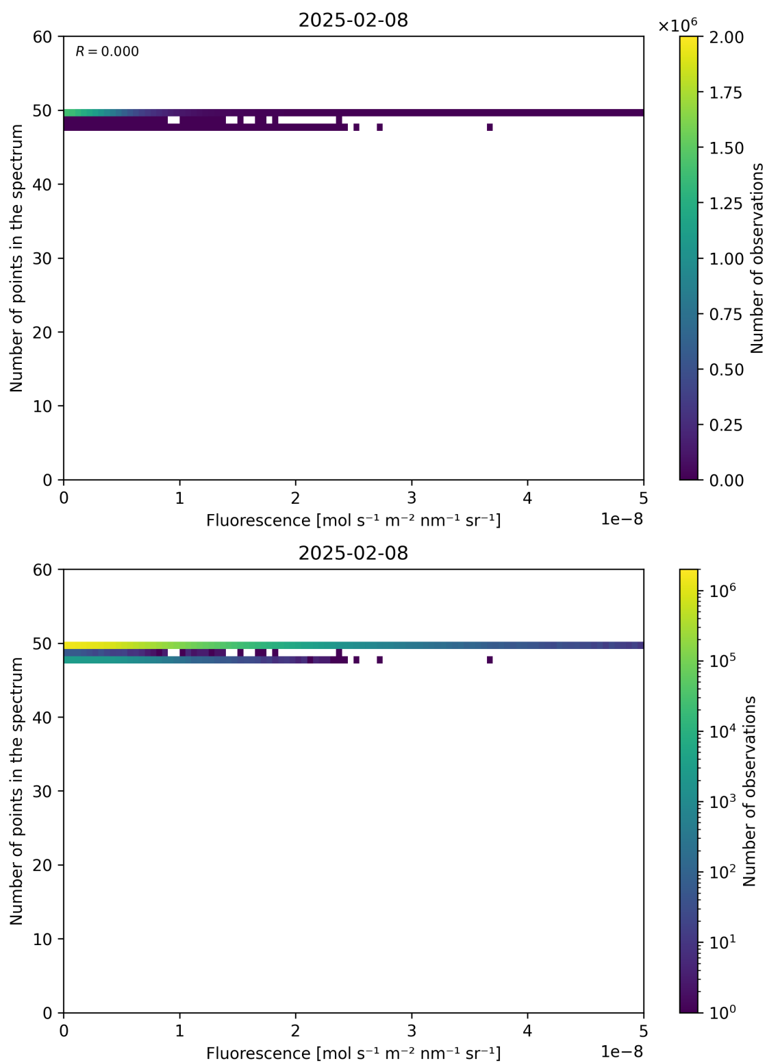
Figure 86: Scatter density plot of “Fluorescence” against “Number of points in the spectrum” for 2025-02-08 to 2025-02-09.
