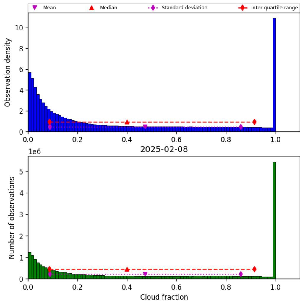
Figure 32: Histogram of “Cloud fraction” for 2025-02-08 to 2025-02-09
