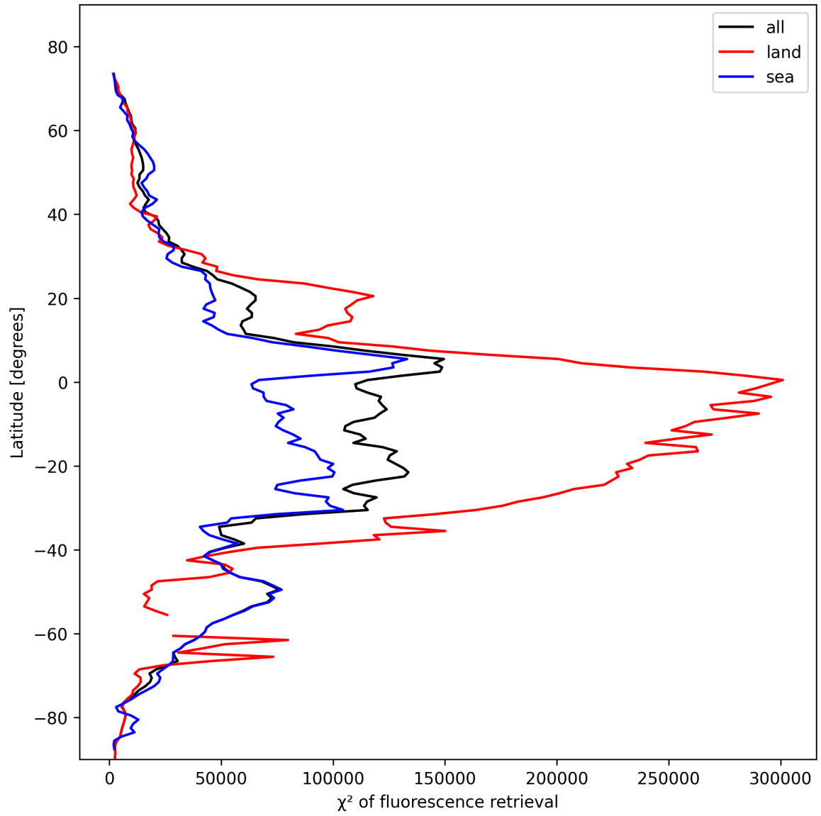
Figure 25: Zonal average of “ \chi^2 of fluorescence retrieval” for 2025-02-08 to 2025-02-09.
