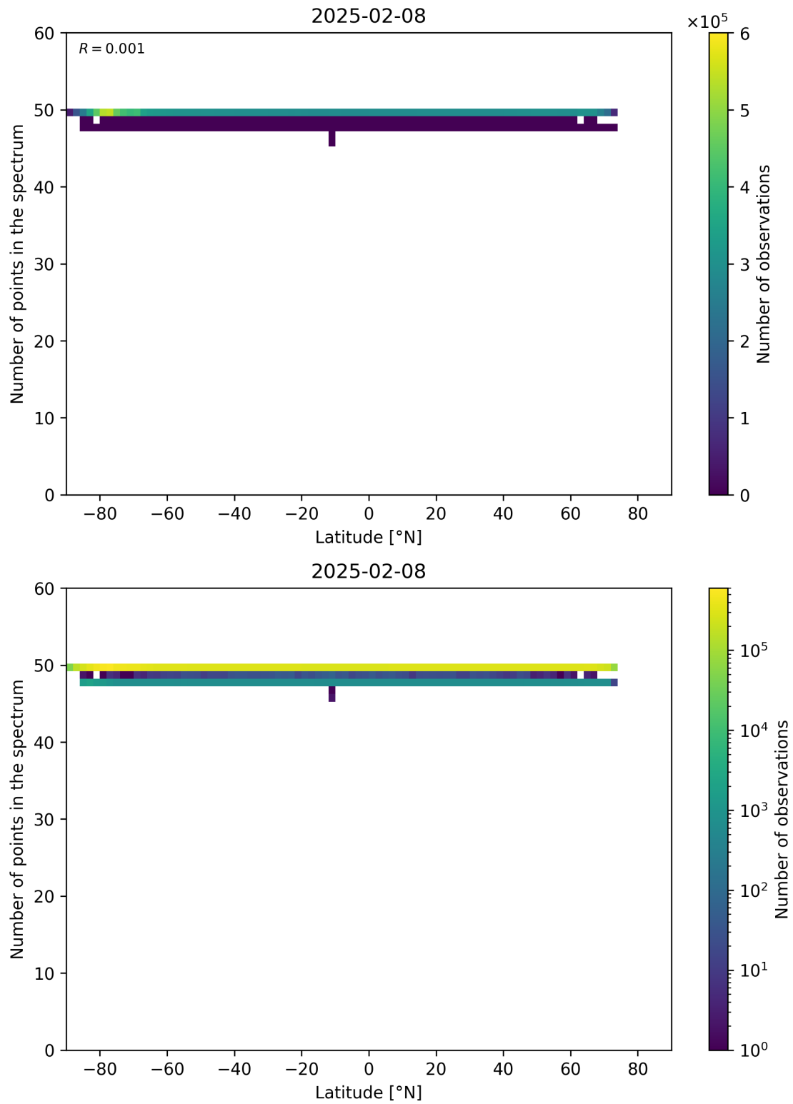
Figure 94: Scatter density plot of “Latitude” against “Number of points in the spectrum” for 2025-02-08 to 2025-02-09.
