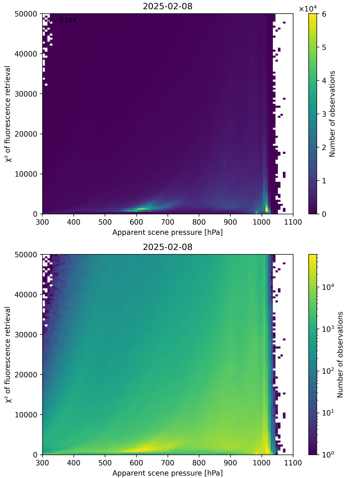
Figure 63: Scatter density plot of “Apparent scene pressure” against “ \chi^2 of fluorescence retrieval” for 2025-02-08 to 2025-02-09.
