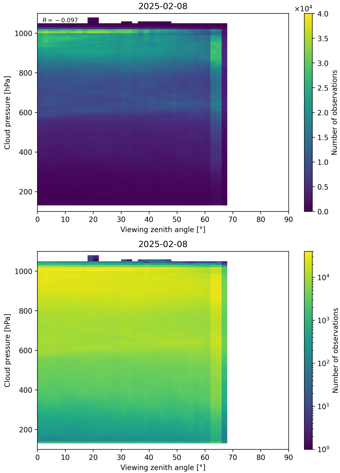
Figure 121: Scatter density plot of “Viewing zenith angle” against “Cloud pressure” for 2025-02-08 to 2025-02-09.
