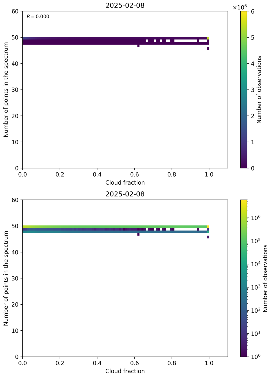
Figure 74: Scatter density plot of “Cloud fraction” against “Number of points in the spectrum” for 2025-02-08 to 2025-02-09.
