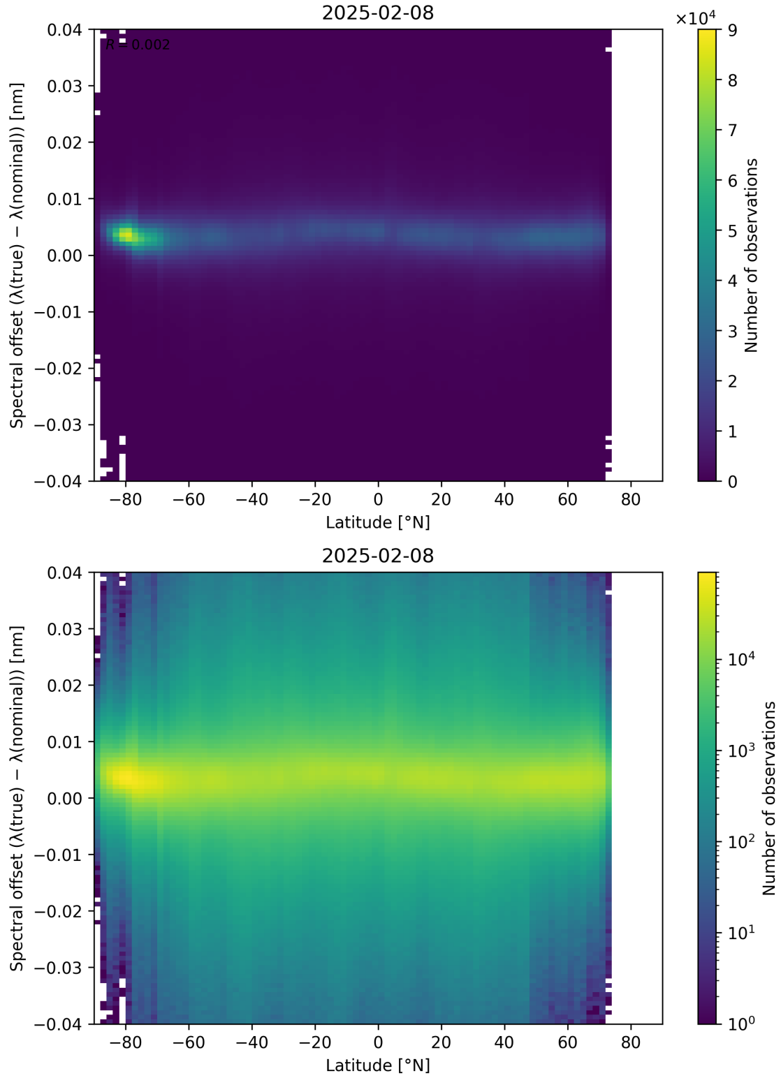
Figure 96: Scatter density plot of “Latitude” against “Spectral offset ( \lambda_{\text{true}} - \lambda_{\text{nominal}} )” for 2025-02-08 to 2025-02-09.
