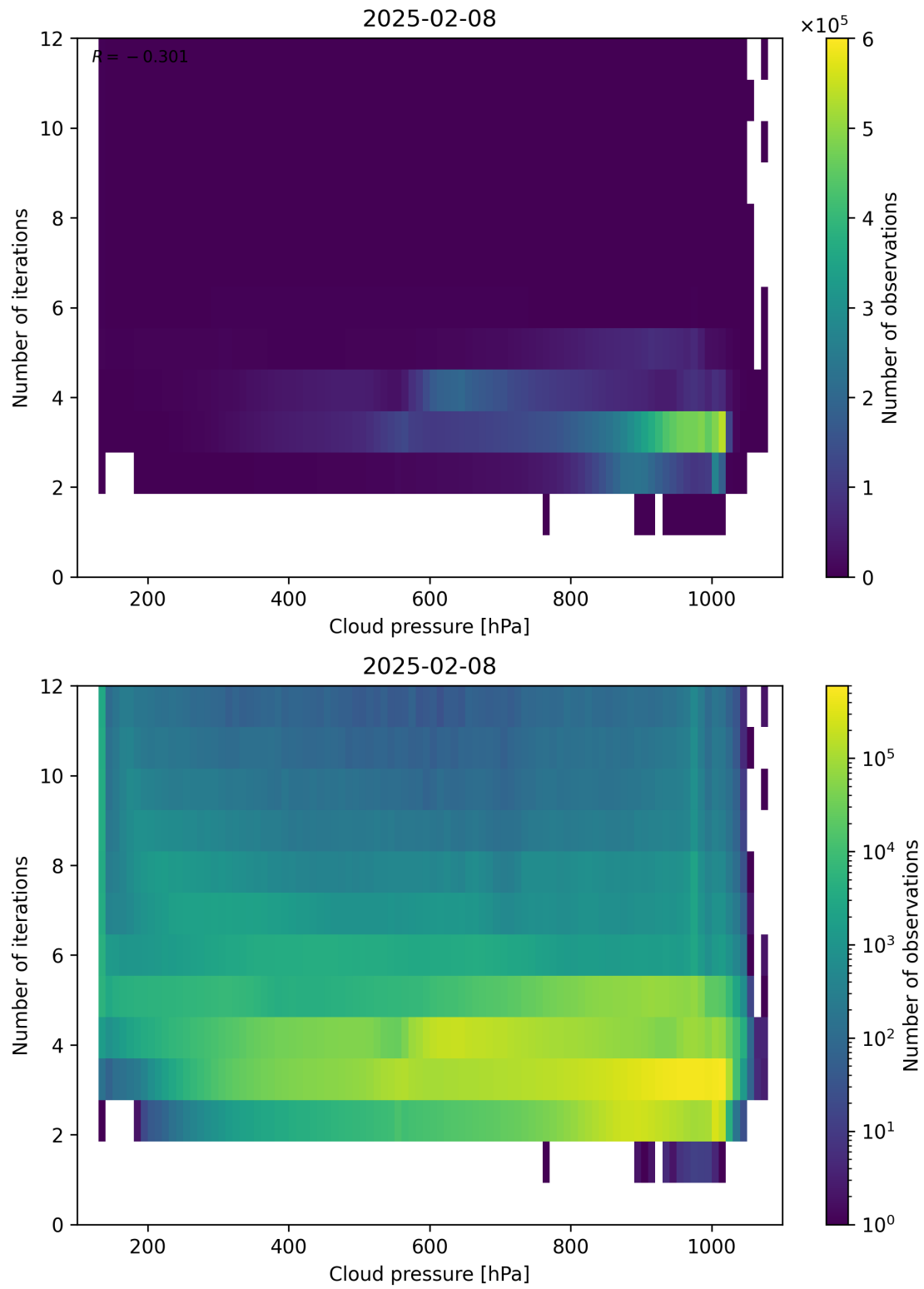
Figure 81: Scatter density plot of “Cloud pressure” against “Number of iterations” for 2025-02-08 to 2025-02-09.
