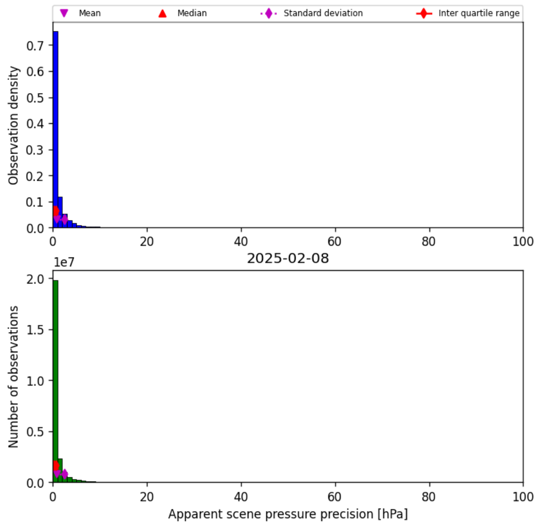
Figure 37: Histogram of “Apparent scene pressure precision” for 2025-02-08 to 2025-02-09
