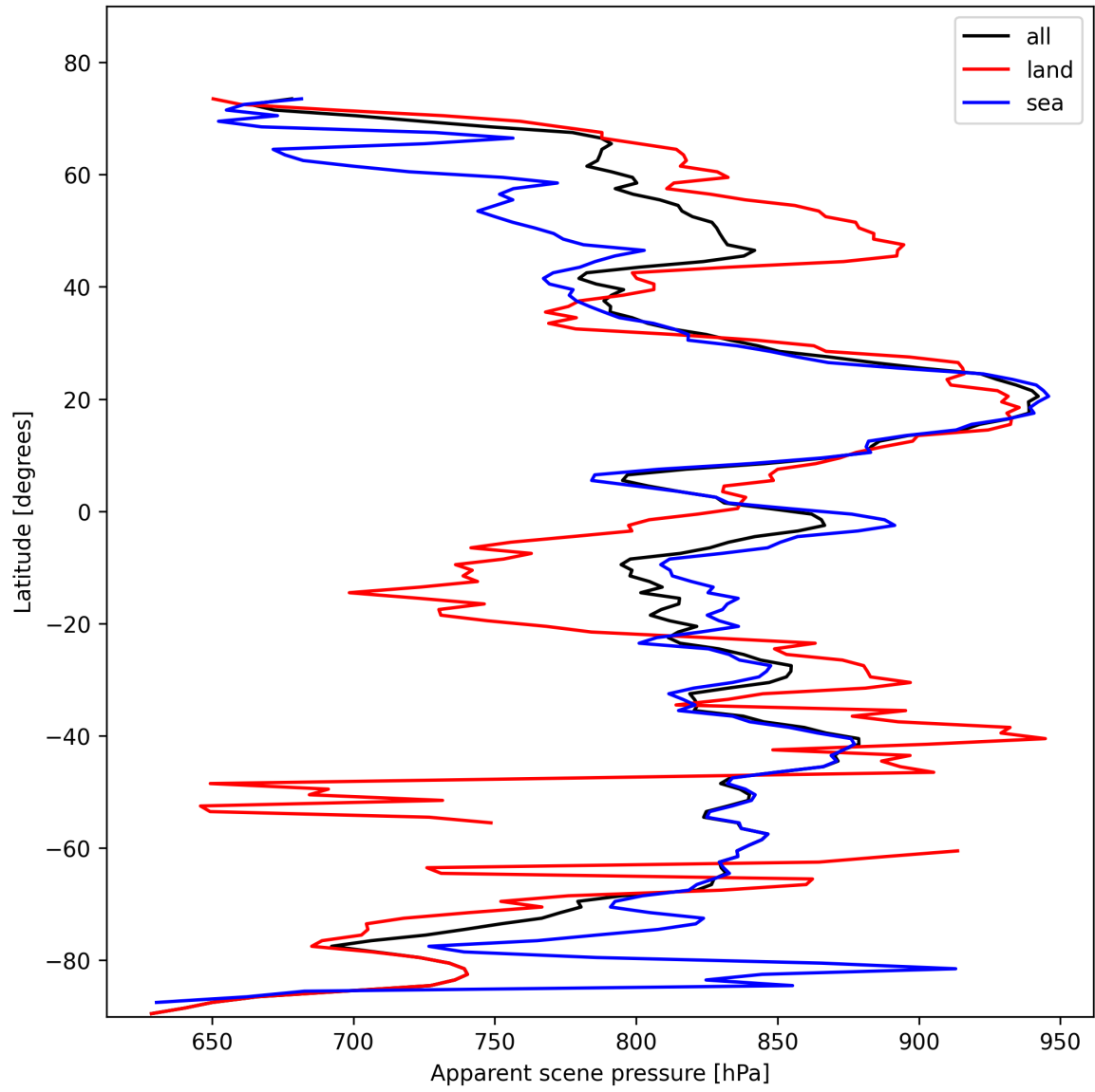
Figure 19: Zonal average of “Apparent scene pressure” for 2025-02-08 to 2025-02-09.
