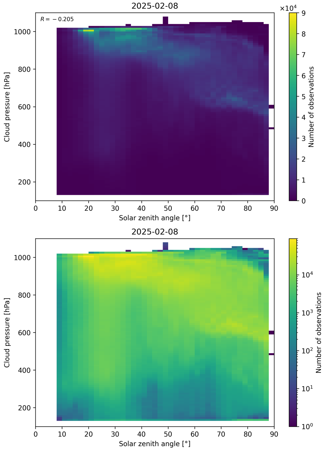
Figure 111: Scatter density plot of “Solar zenith angle” against “Cloud pressure” for 2025-02-08 to 2025-02-09.
