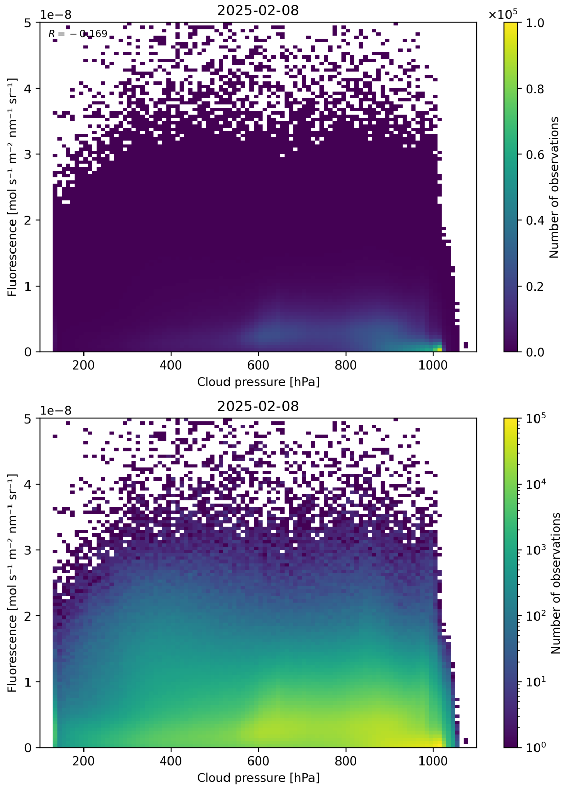
Figure 80: Scatter density plot of “Cloud pressure” against “Fluorescence” for 2025-02-08 to 2025-02-09.
