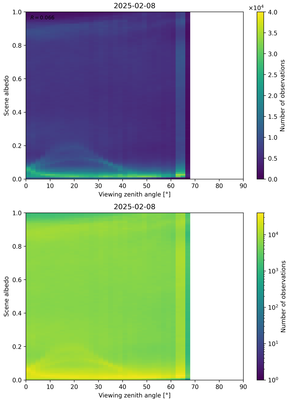
Figure 126: Scatter density plot of “Viewing zenith angle” against “Scene albedo” for 2025-02-08 to 2025-02-09.
