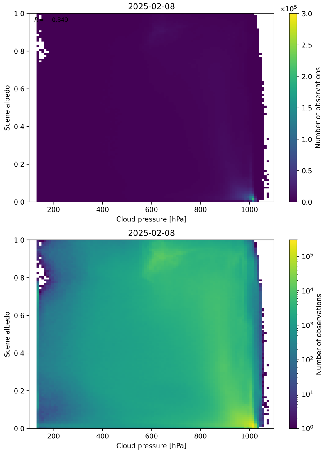
Figure 83: Scatter density plot of “Cloud pressure” against “Scene albedo” for 2025-02-08 to 2025-02-09.
