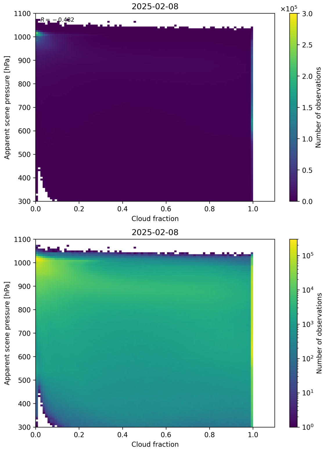
Figure 70: Scatter density plot of “Cloud fraction” against “Apparent scene pressure” for 2025-02-08 to 2025-02-09.
