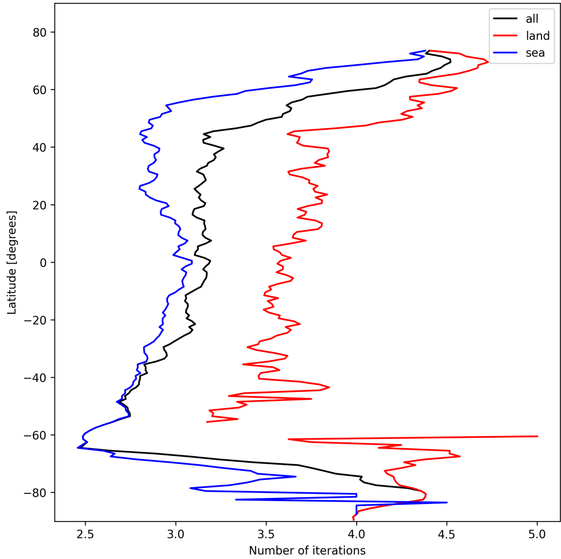
Figure 22: Zonal average of “Number of iterations” for 2025-02-08 to 2025-02-09.
