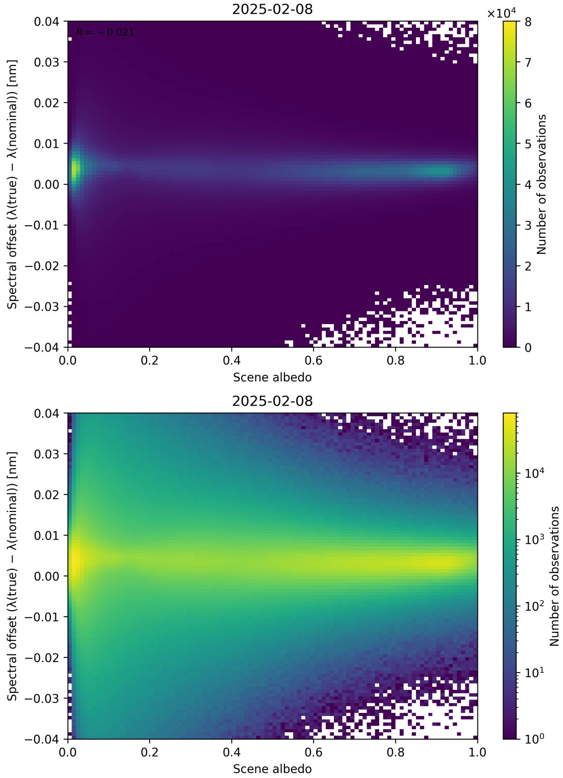
Figure 107: Scatter density plot of “Scene albedo” against “Spectral offset ( \lambda_{\text{true}} - \lambda_{\text{nominal}} )” for 2025-02-08 to 2025-02-09.
