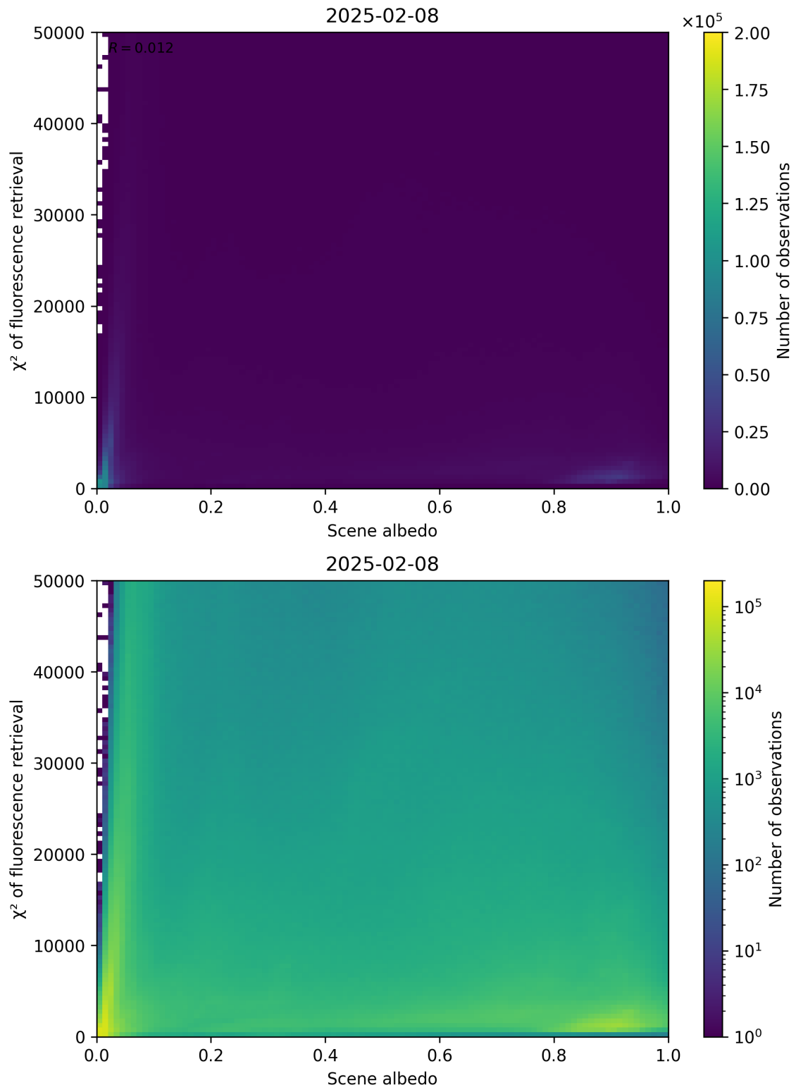
Figure 103: Scatter density plot of “Scene albedo” against “ \chi^2 of fluorescence retrieval” for 2025-02-08 to 2025-02-09.
