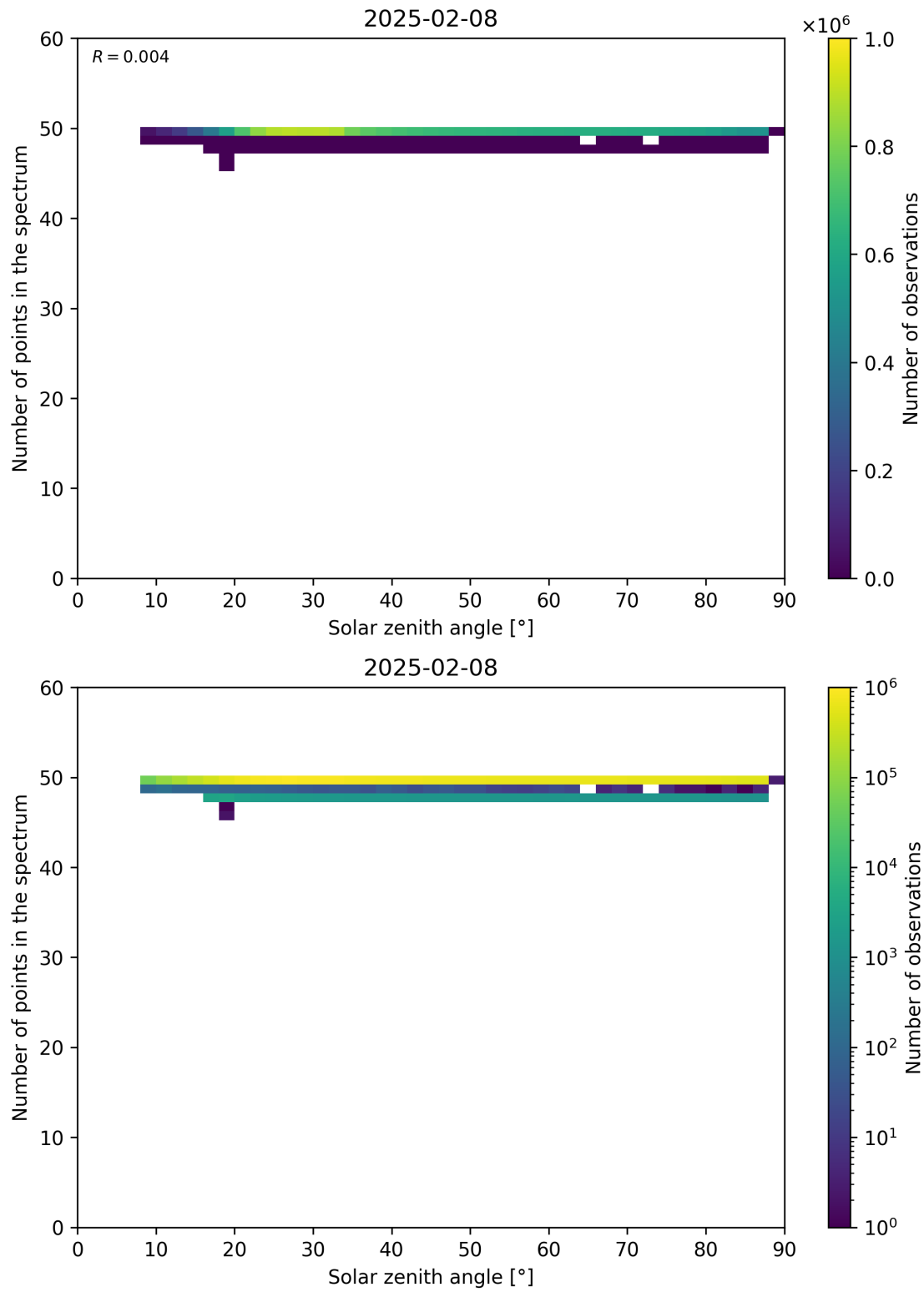
Figure 115: Scatter density plot of “Solar zenith angle” against “Number of points in the spectrum” for 2025-02-08 to 2025-02-09.
