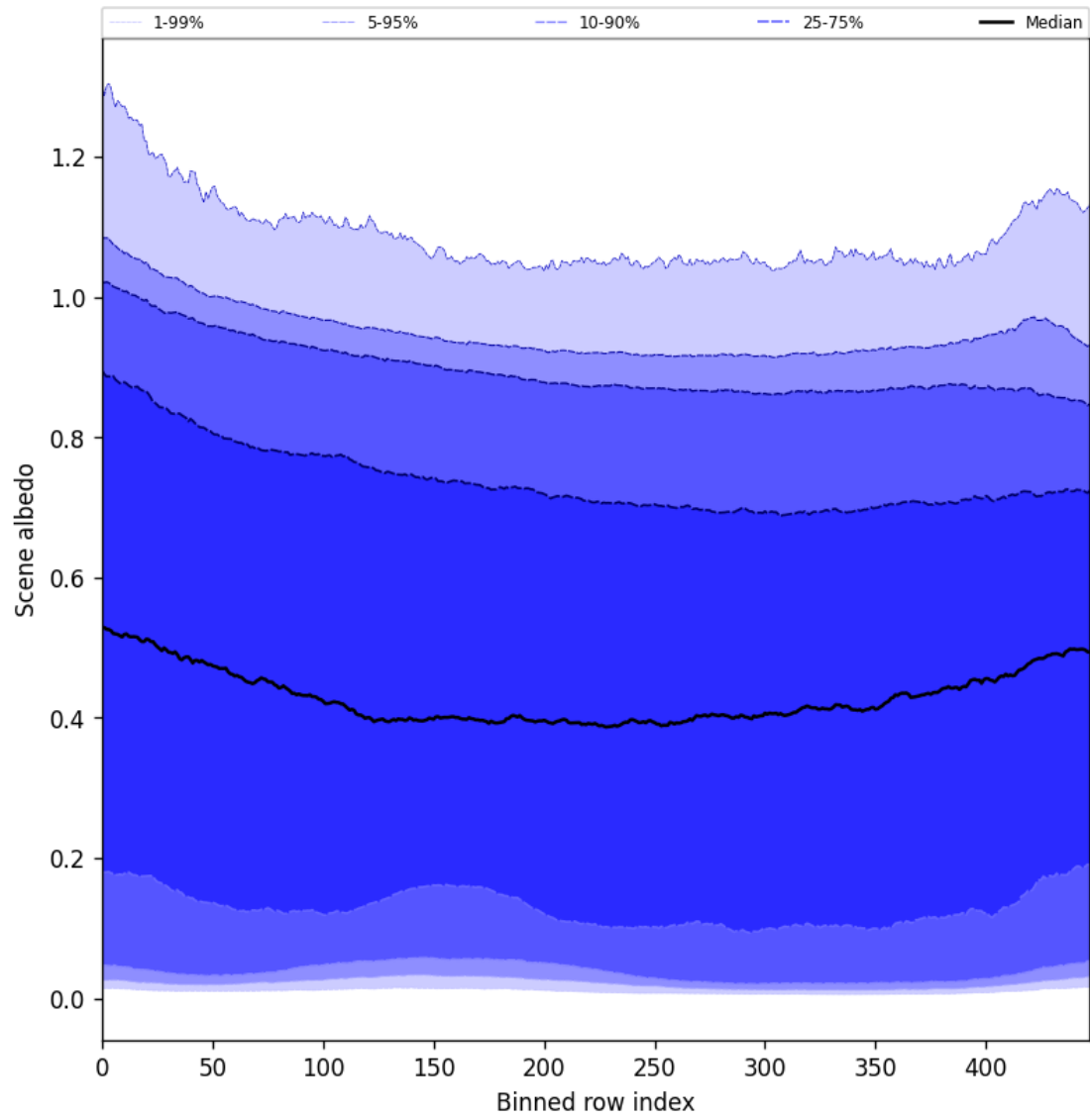
Figure 51: Along track statistics of “Scene albedo” for 2025-02-08 to 2025-02-09
