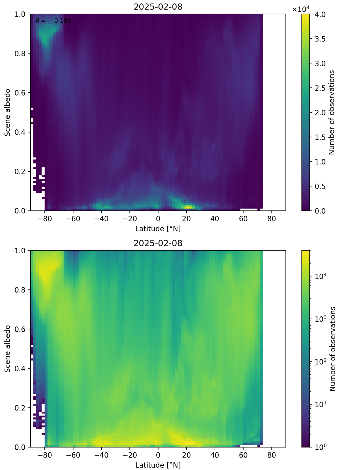
Figure 95: Scatter density plot of “Latitude” against “Scene albedo” for 2025-02-08 to 2025-02-09.
