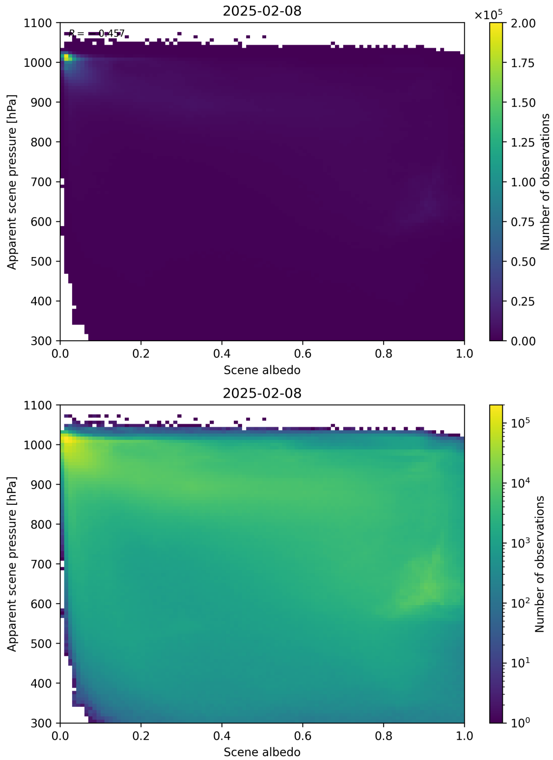
Figure 102: Scatter density plot of “Scene albedo” against “Apparent scene pressure” for 2025-02-08 to 2025-02-09.
