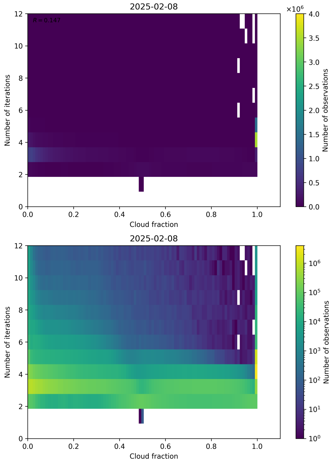
Figure 73: Scatter density plot of “Cloud fraction” against “Number of iterations” for 2025-02-08 to 2025-02-09.
