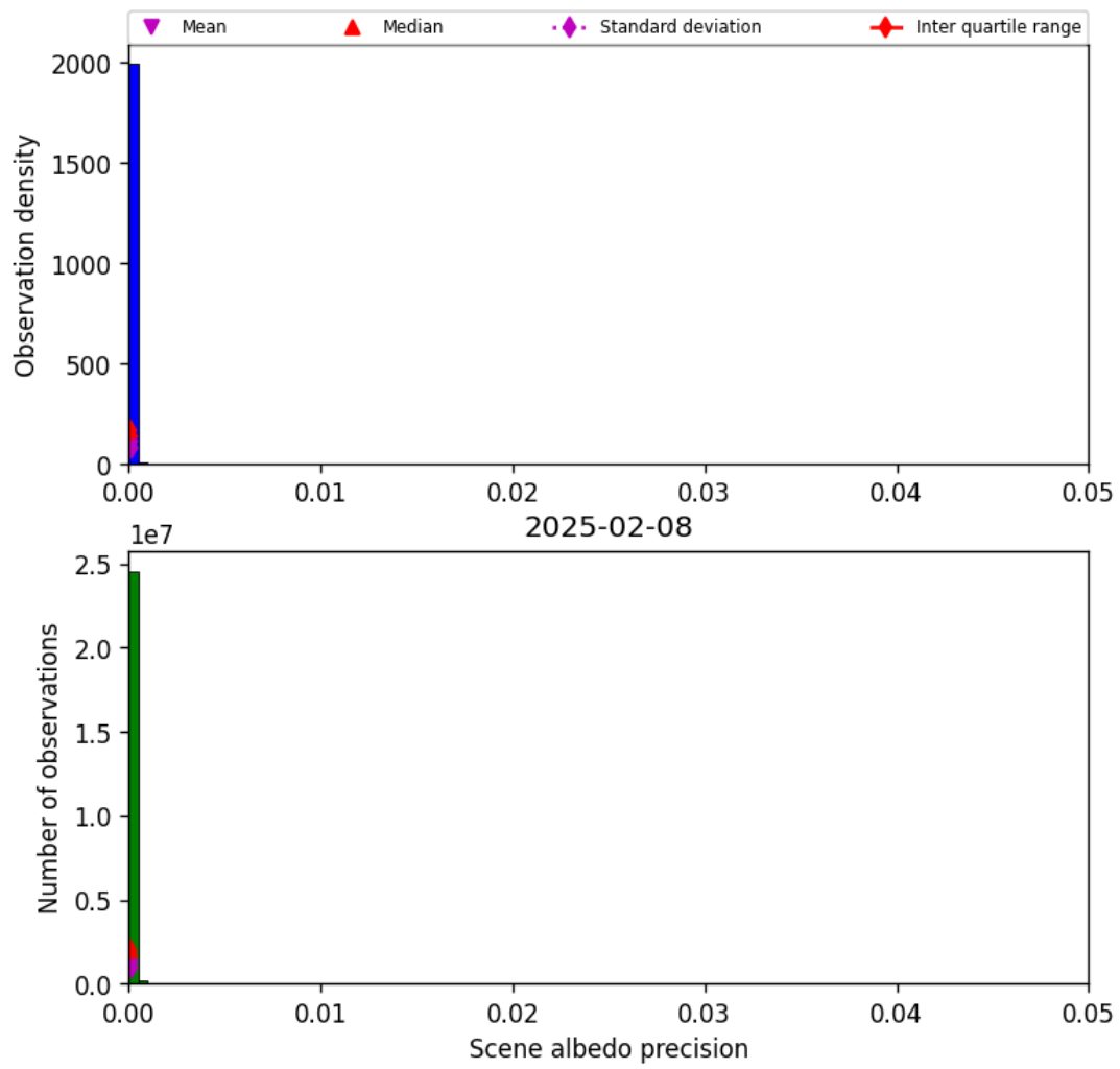
Figure 35: Histogram of “Scene albedo precision” for 2025-02-08 to 2025-02-09
