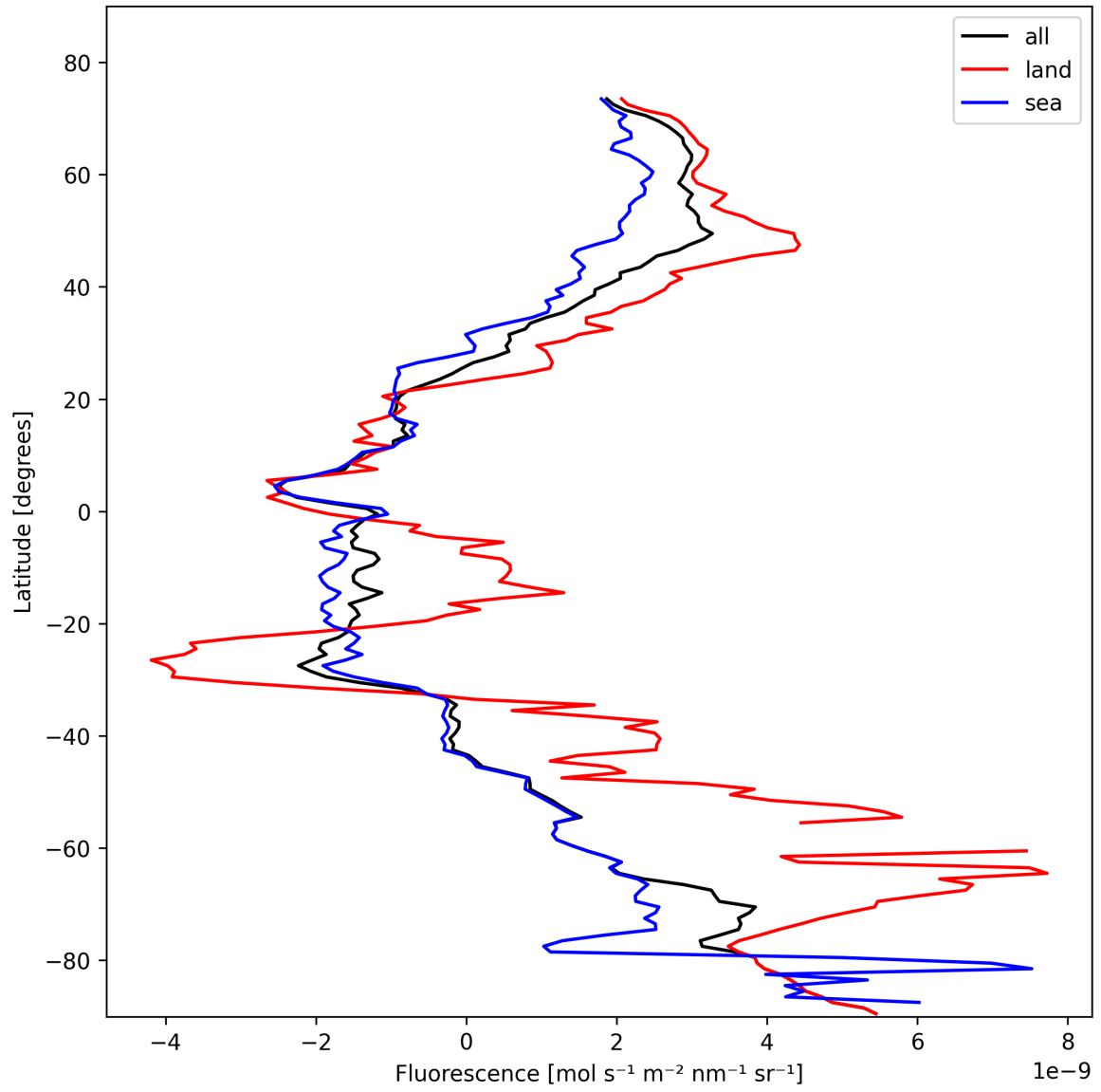
Figure 23: Zonal average of “Fluorescence” for 2025-02-08 to 2025-02-09.
