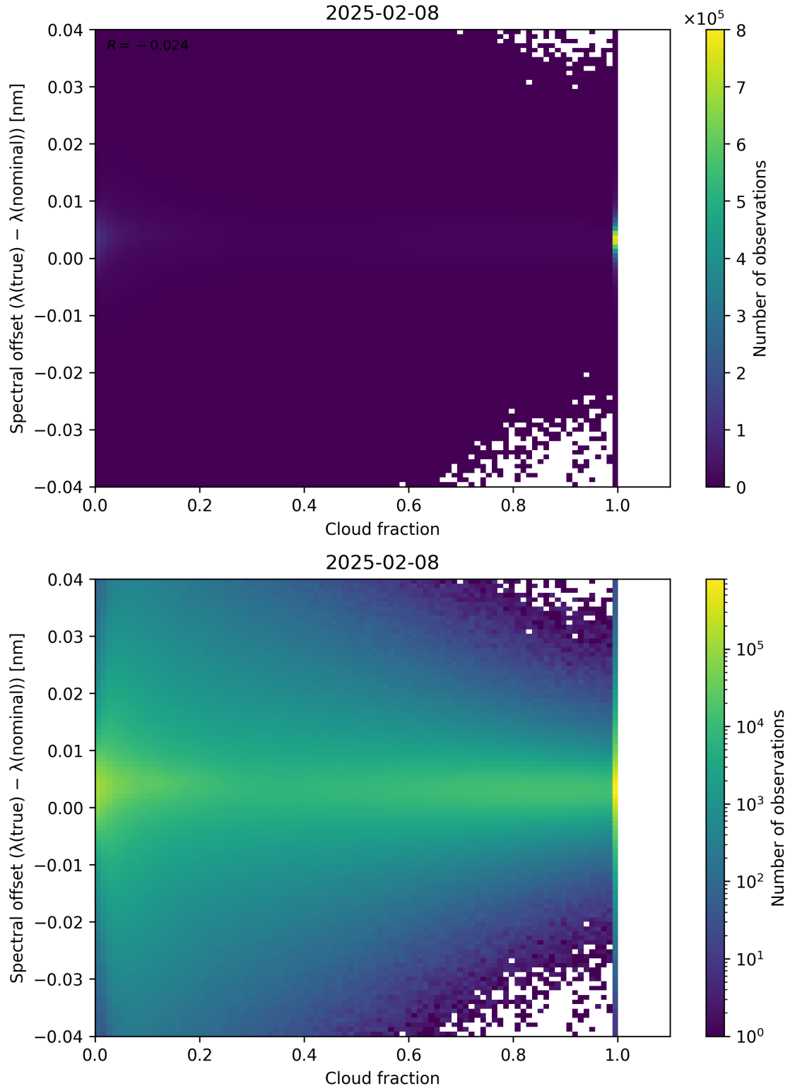
Figure 76: Scatter density plot of “Cloud fraction” against “Spectral offset ( \lambda_{\text{true}} - \lambda_{\text{nominal}} )” for 2025-02-08 to 2025-02-09.
