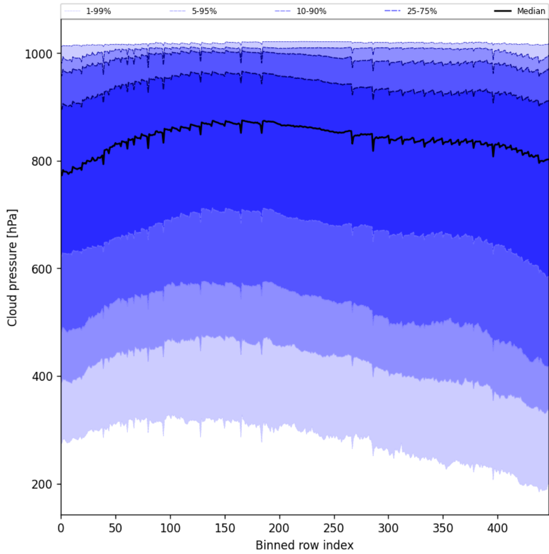
Figure 47: Along track statistics of “Cloud pressure” for 2025-02-08 to 2025-02-09
