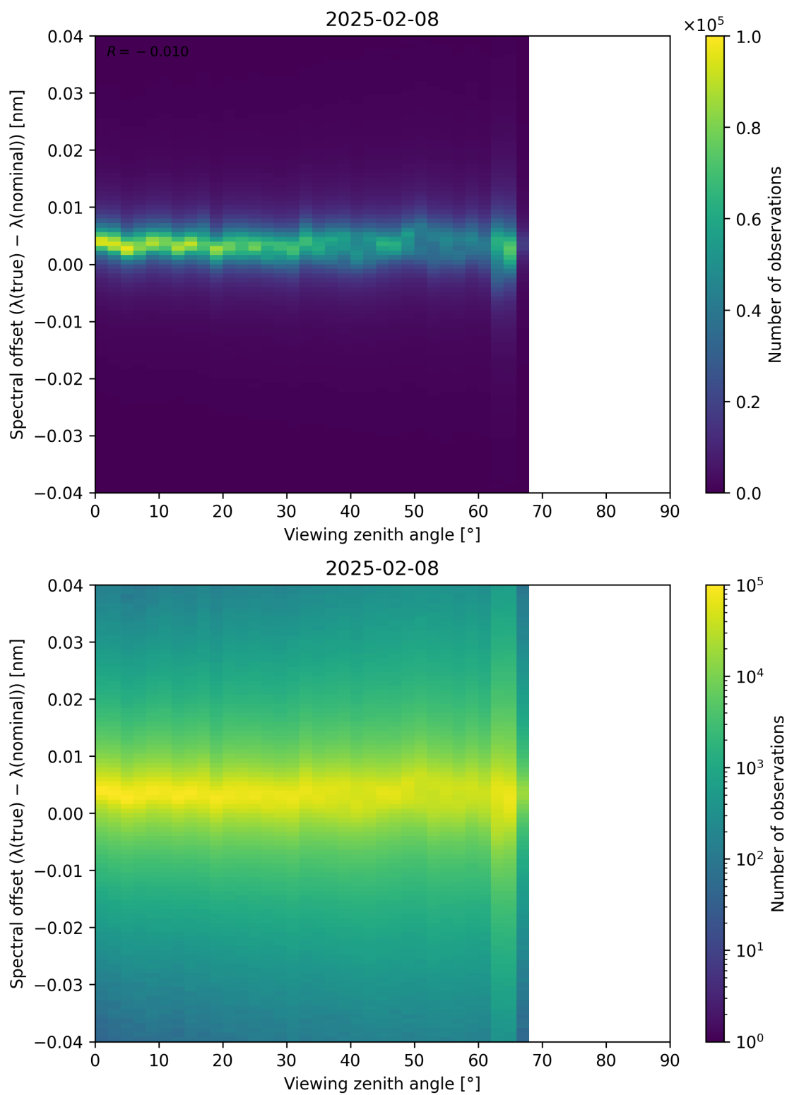
Figure 128: Scatter density plot of “Viewing zenith angle” against “Spectral offset ( \lambda_{\text{true}} - \lambda_{\text{nominal}} )” for 2025-02-08 to 2025-02-09.
