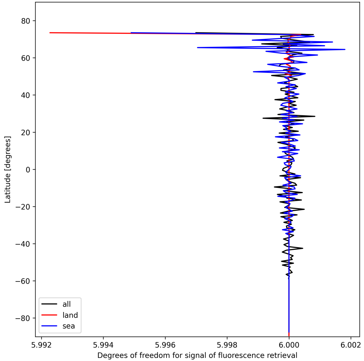
Figure 26: Zonal average of “Degrees of freedom for signal of fluorescence retrieval” for 2025-02-08 to 2025-02-09.
