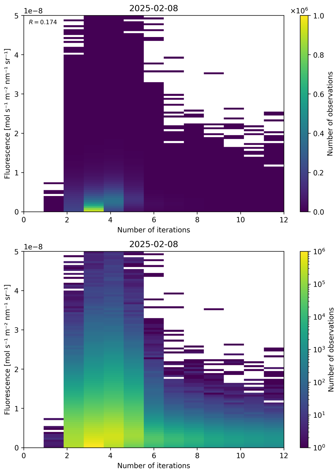
Figure 98: Scatter density plot of “Number of iterations” against “Fluorescence” for 2025-02-08 to 2025-02-09.
