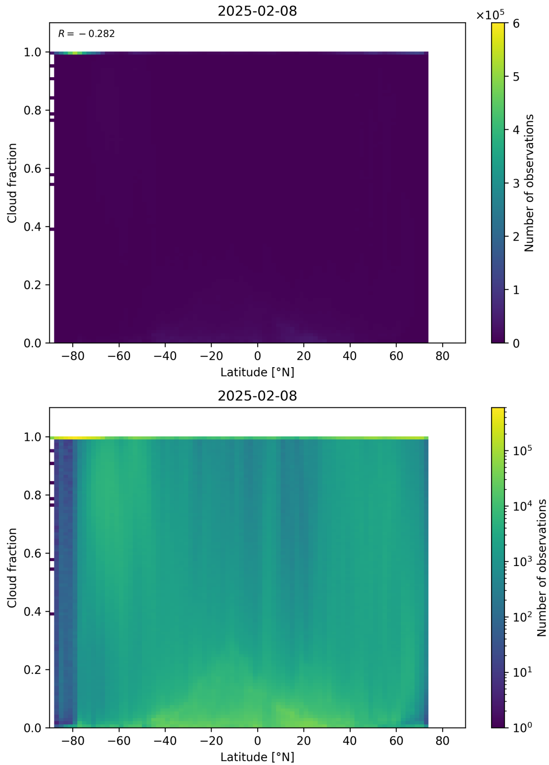
Figure 90: Scatter density plot of “Latitude” against “Cloud fraction” for 2025-02-08 to 2025-02-09.
