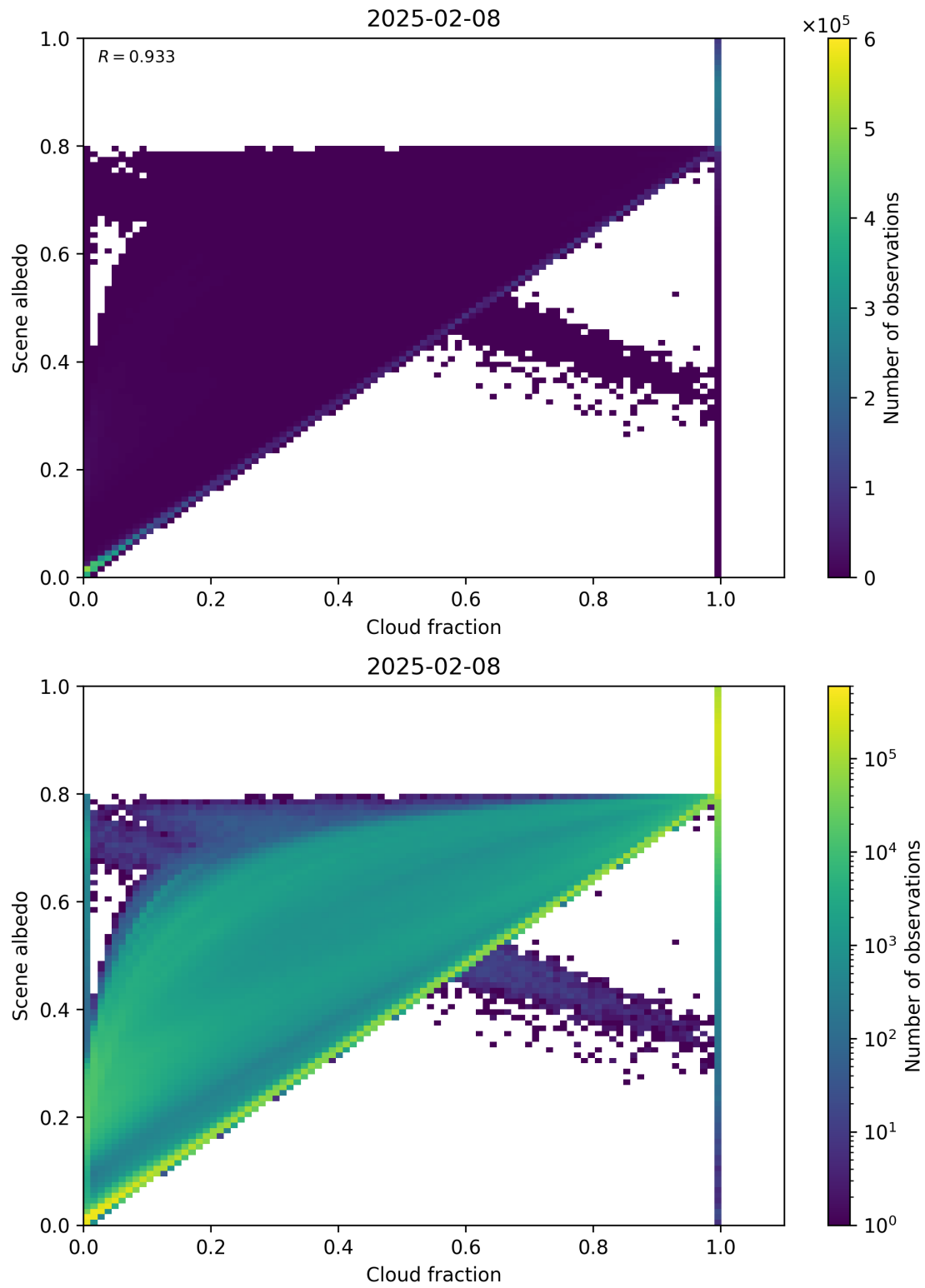
Figure 75: Scatter density plot of “Cloud fraction” against “Scene albedo” for 2025-02-08 to 2025-02-09.
