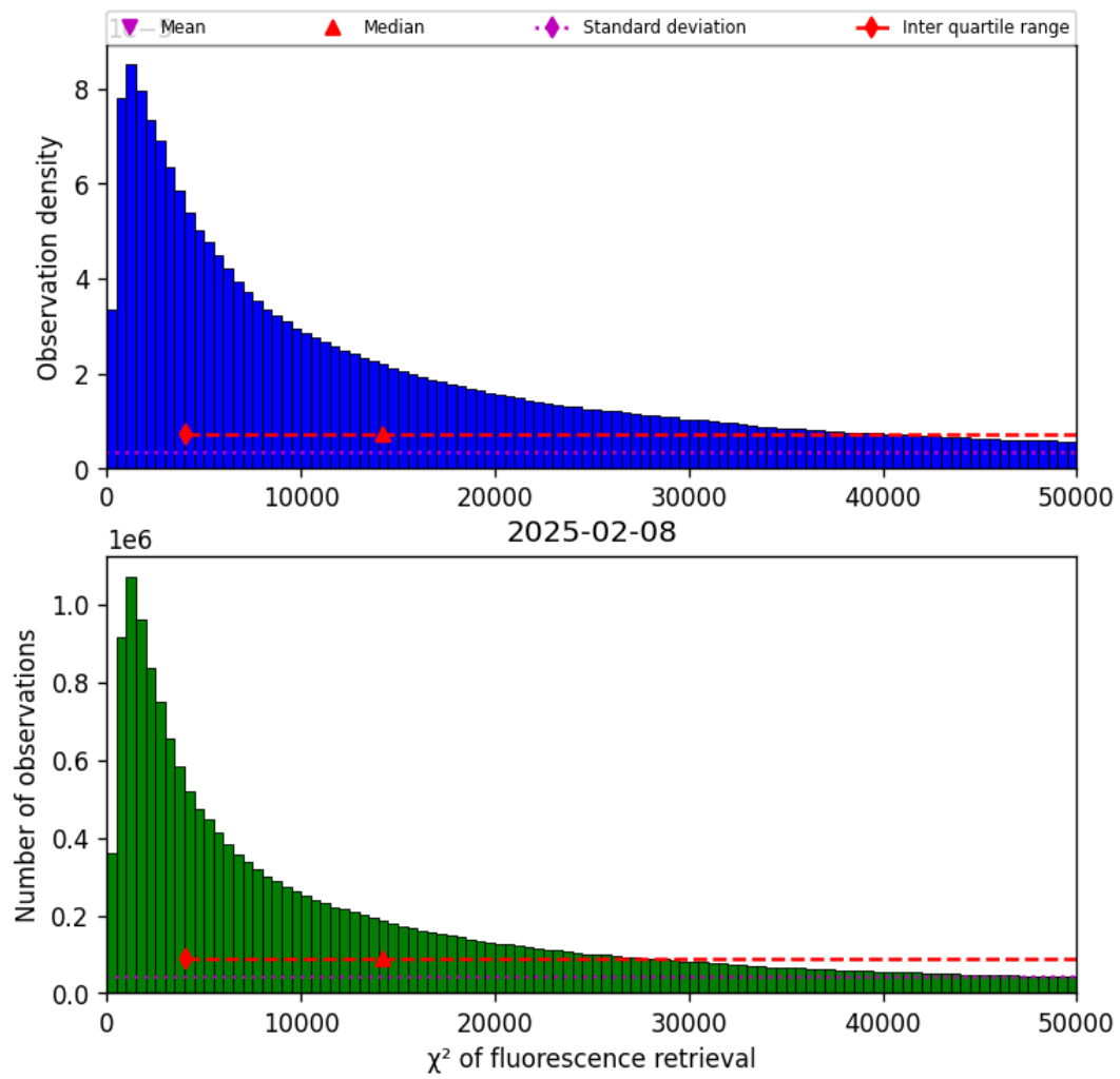
Figure 42: Histogram of “ \chi^2 of fluorescence retrieval” for 2025-02-08 to 2025-02-09
