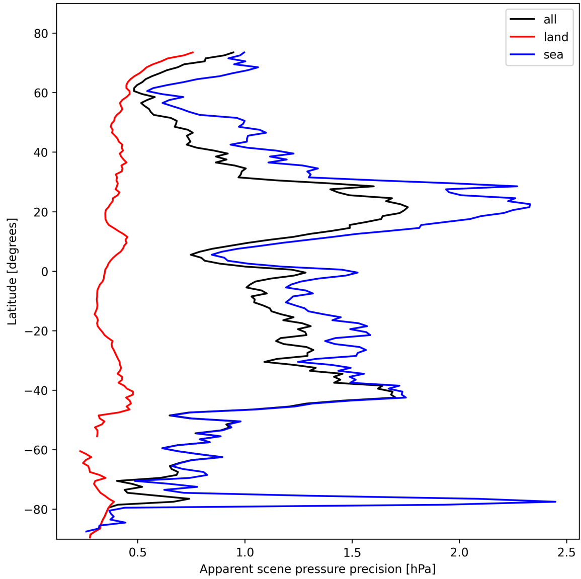
Figure 20: Zonal average of “Apparent scene pressure precision” for 2025-02-08 to 2025-02-09.
