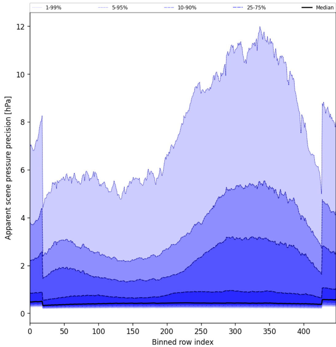
Figure 54: Along track statistics of “Apparent scene pressure precision” for 2025-02-08 to 2025-02-09
