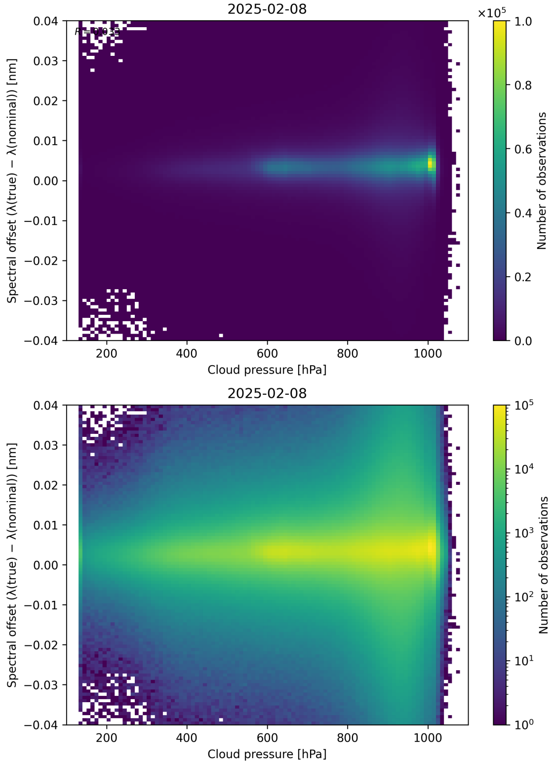
Figure 84: Scatter density plot of “Cloud pressure” against “Spectral offset ( \lambda_{\text{true}} - \lambda_{\text{nominal}} )” for 2025-02-08 to 2025-02-09.
