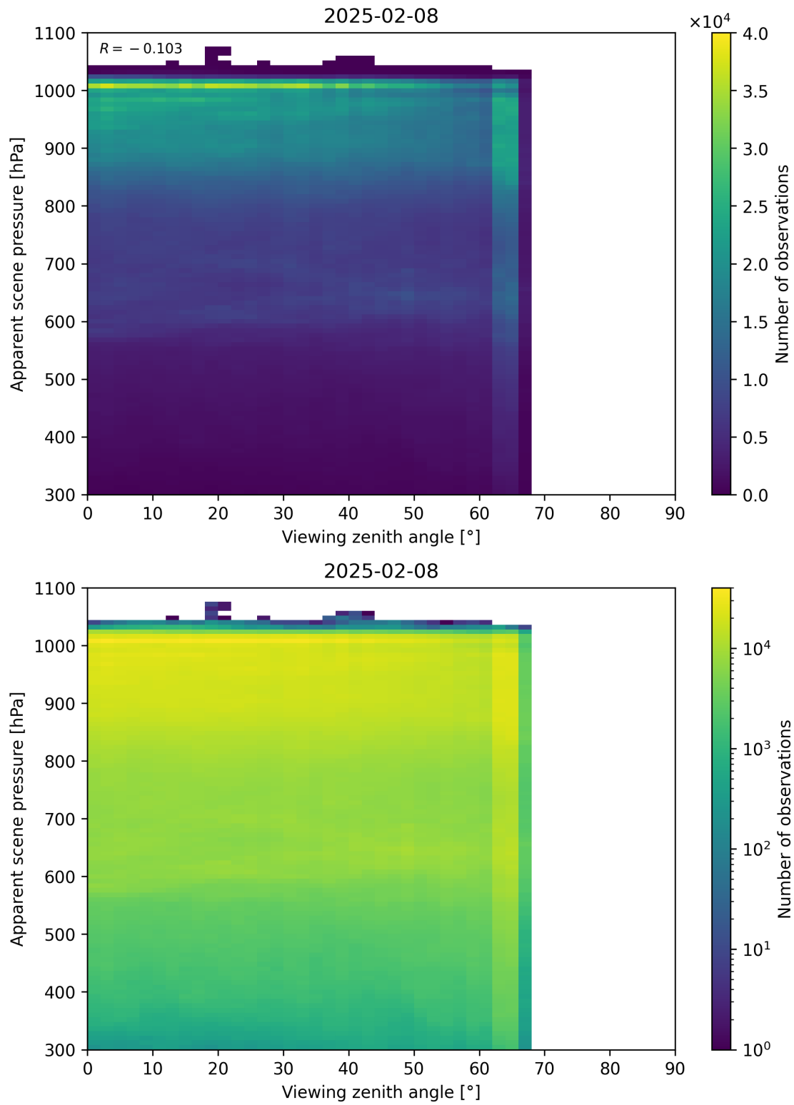
Figure 118: Scatter density plot of “Viewing zenith angle” against “Apparent scene pressure” for 2025-02-08 to 2025-02-09.
