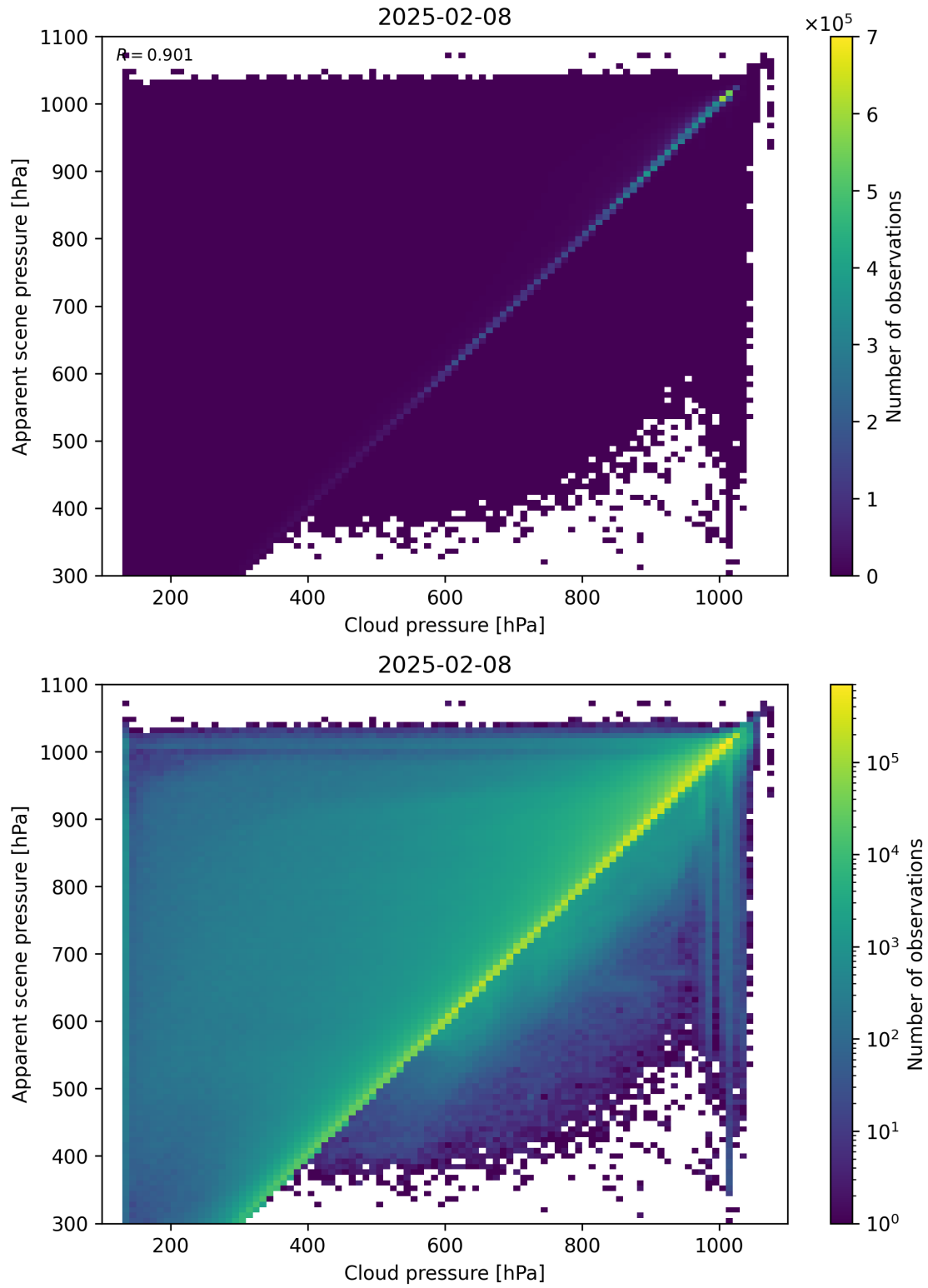
Figure 77: Scatter density plot of “Cloud pressure” against “Apparent scene pressure” for 2025-02-08 to 2025-02-09.
