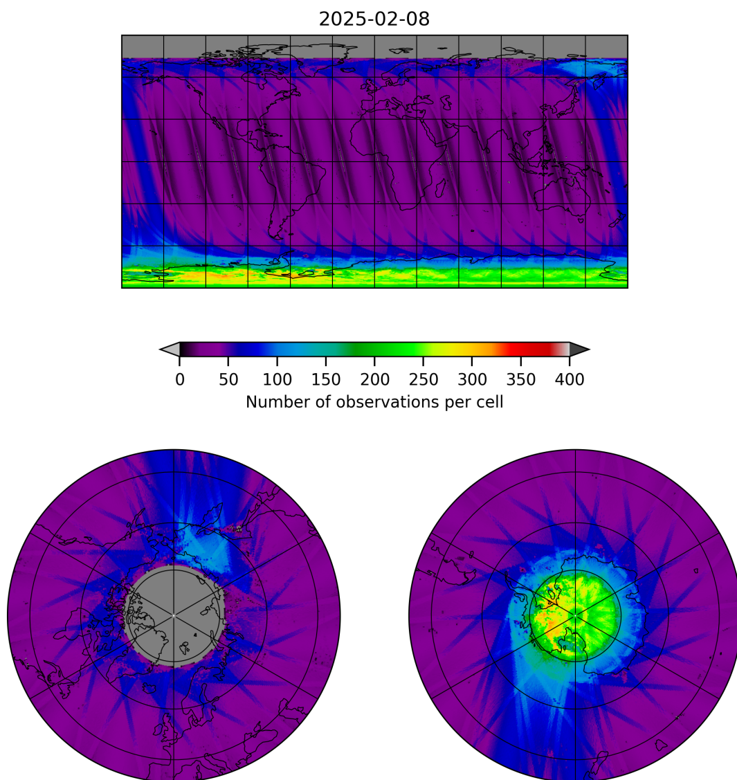
Figure 11: Map of the number of observations for 2025-02-08 to 2025-02-09
