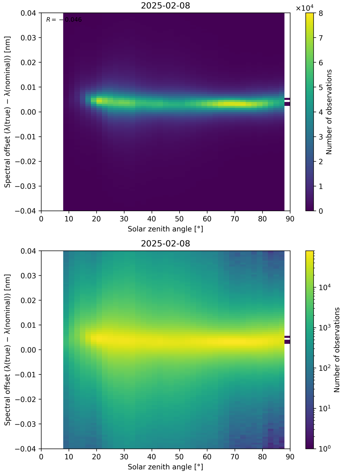
Figure 117: Scatter density plot of “Solar zenith angle” against “Spectral offset ( \lambda_{\text{true}} - \lambda_{\text{nominal}} )” for 2025-02-08 to 2025-02-09.
