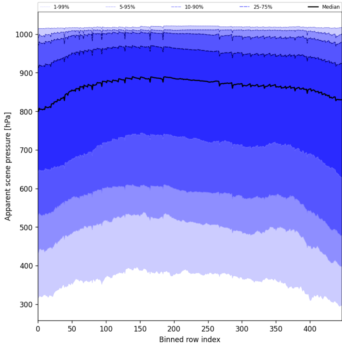
Figure 53: Along track statistics of “Apparent scene pressure” for 2025-02-08 to 2025-02-09
