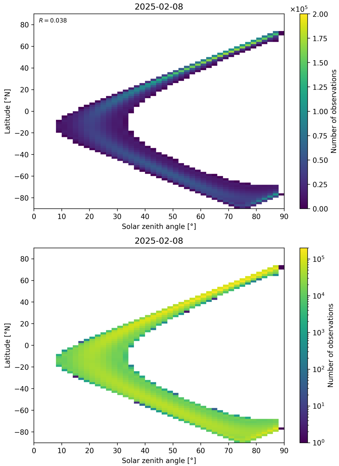
Figure 113: Scatter density plot of “Solar zenith angle” against “Latitude” for 2025-02-08 to 2025-02-09.
