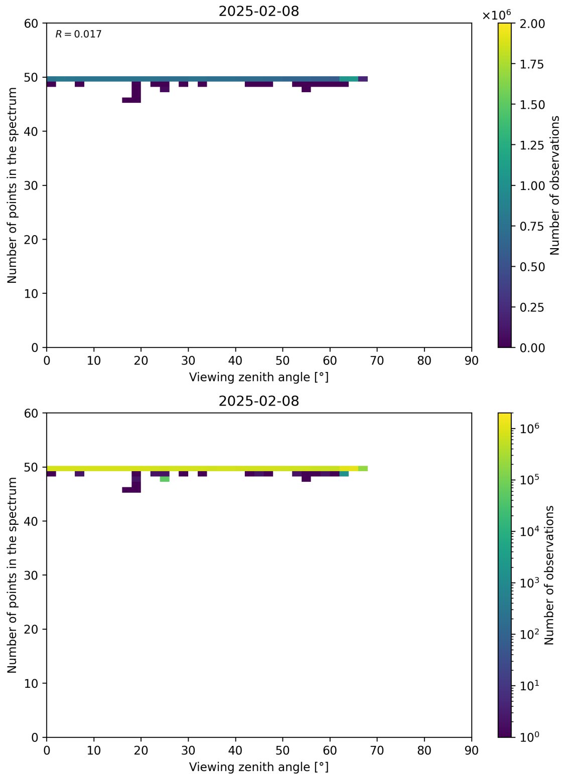
Figure 125: Scatter density plot of “Viewing zenith angle” against “Number of points in the spectrum” for 2025-02-08 to 2025-02-09.
