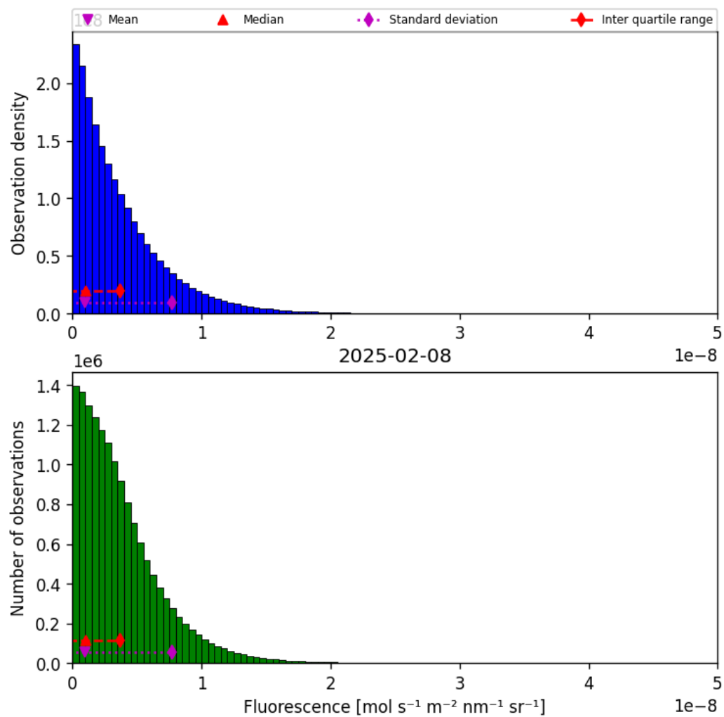
Figure 40: Histogram of “Fluorescence” for 2025-02-08 to 2025-02-09
