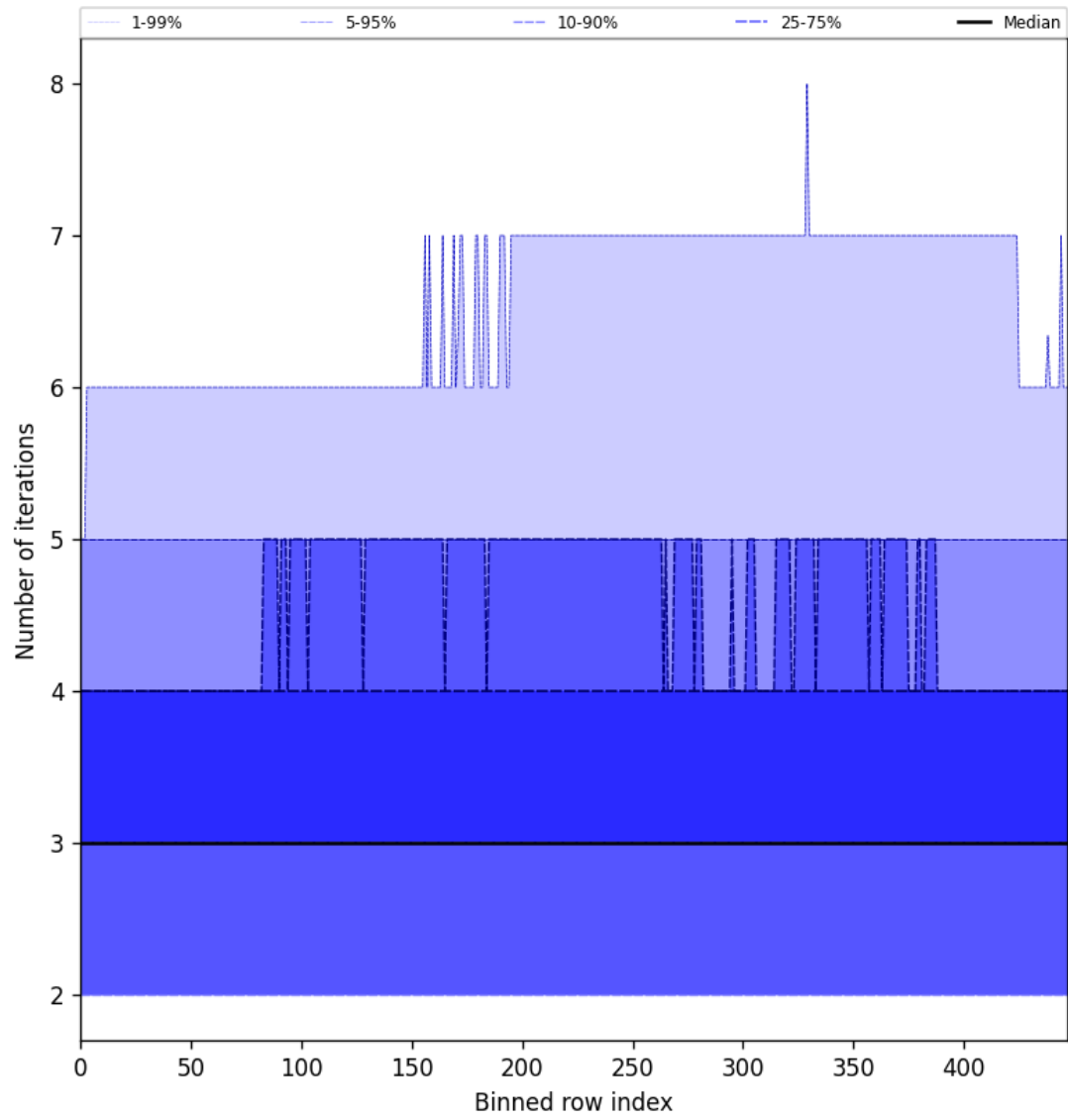
Figure 56: Along track statistics of “Number of iterations” for 2025-02-08 to 2025-02-09
