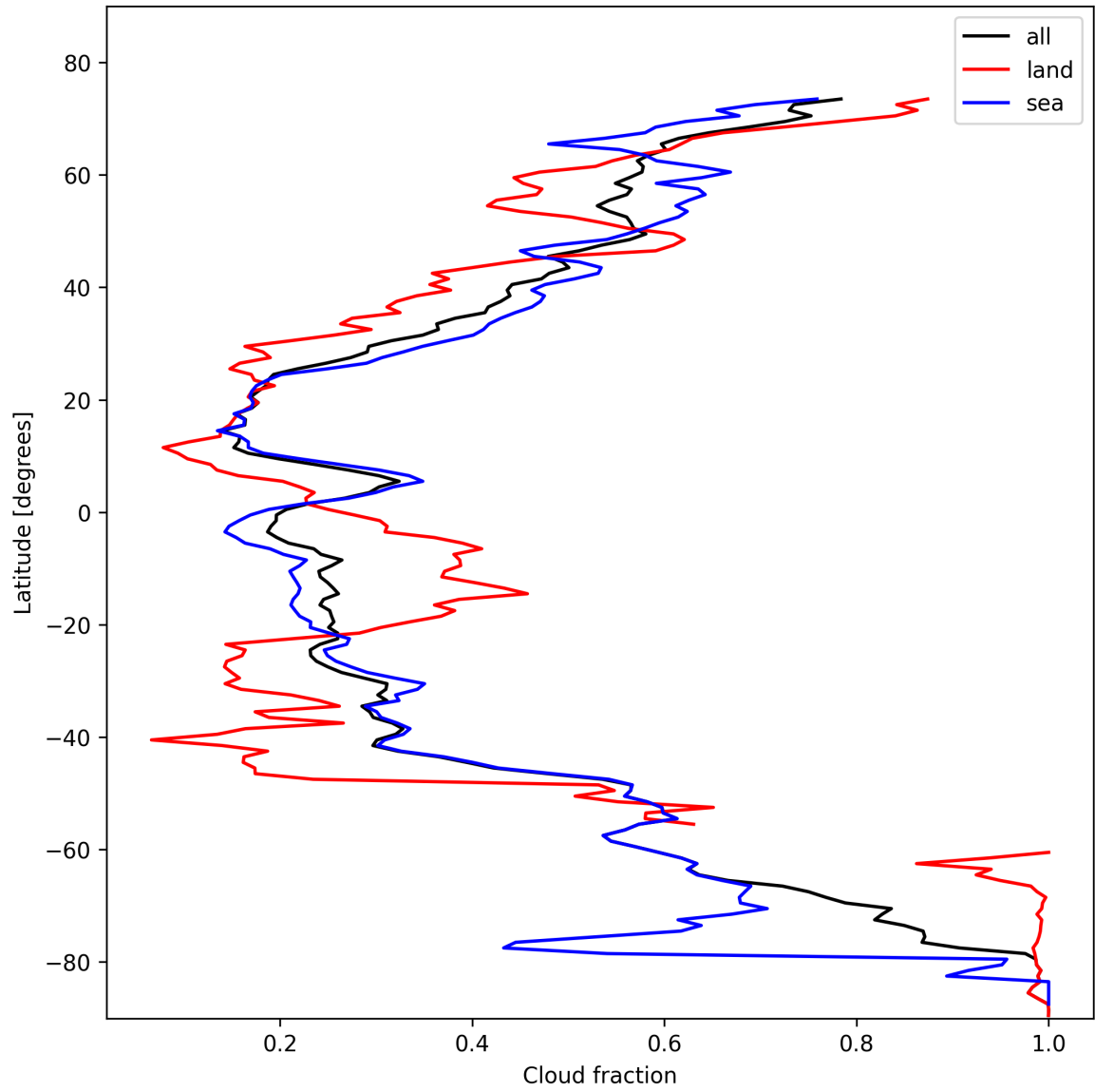
Figure 15: Zonal average of “Cloud fraction” for 2025-02-08 to 2025-02-09.
