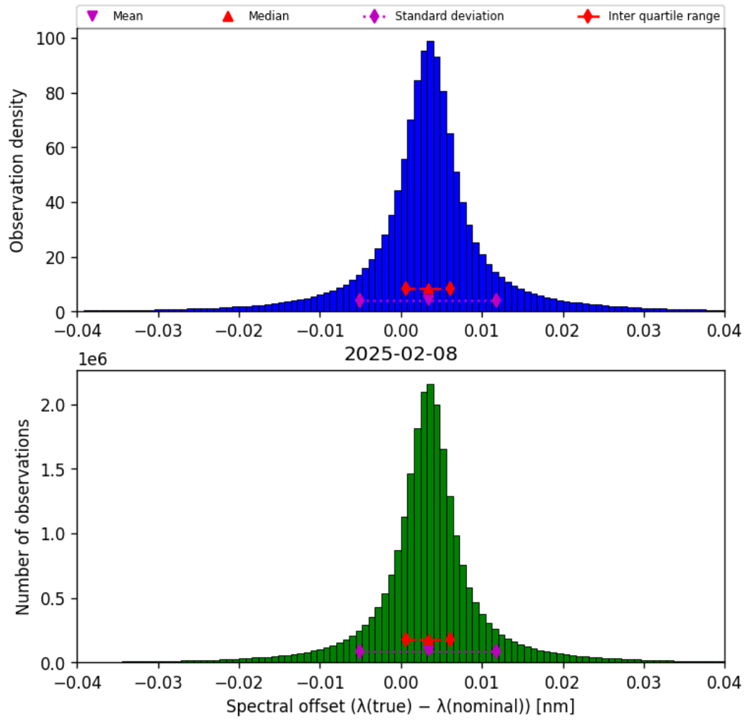
Figure 45: Histogram of “Spectral offset ( \lambda_{\text{true}} - \lambda_{\text{nominal}} )” for 2025-02-08 to 2025-02-09
