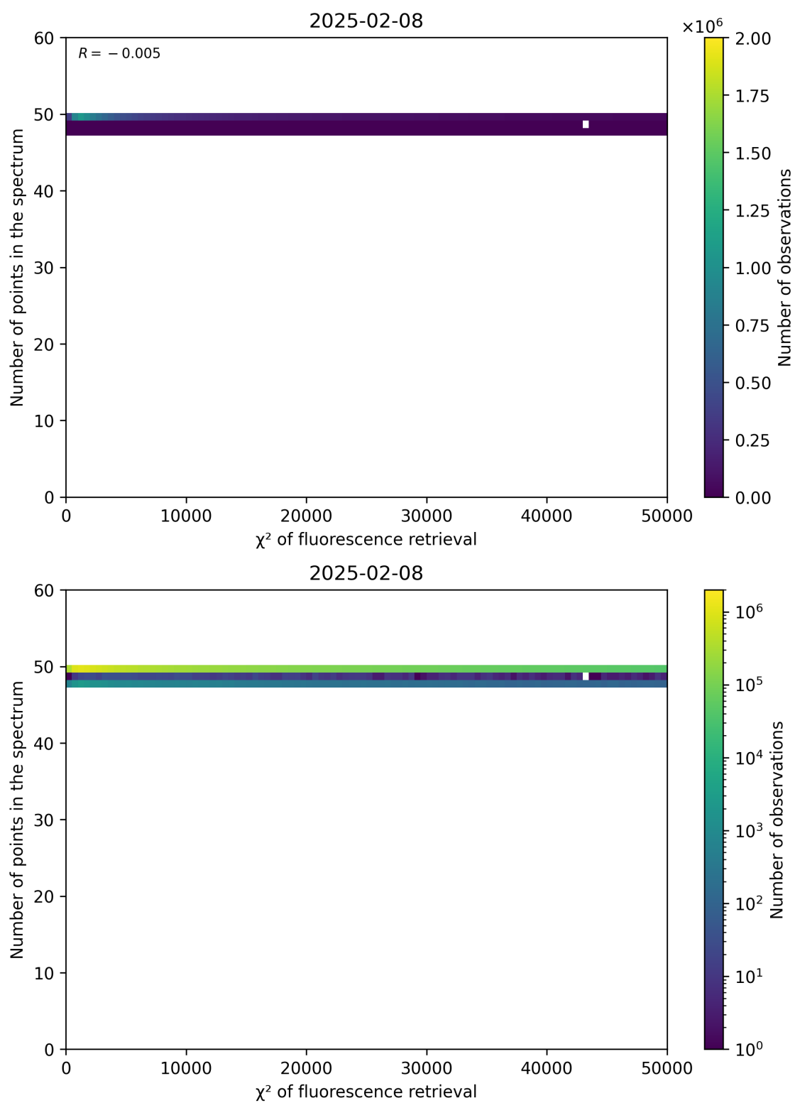
Figure 68: Scatter density plot of " \chi^2 of fluorescence retrieval" against "Number of points in the spectrum" for 2025-02-08 to 2025-02-09.
