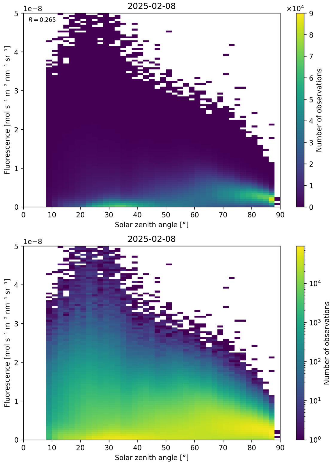
Figure 112: Scatter density plot of “Solar zenith angle” against “Fluorescence” for 2025-02-08 to 2025-02-09.
