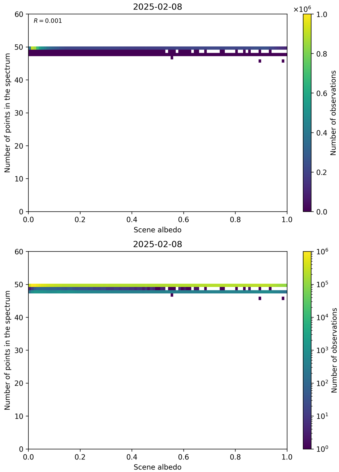
Figure 106: Scatter density plot of “Scene albedo” against “Number of points in the spectrum” for 2025-02-08 to 2025-02-09.
