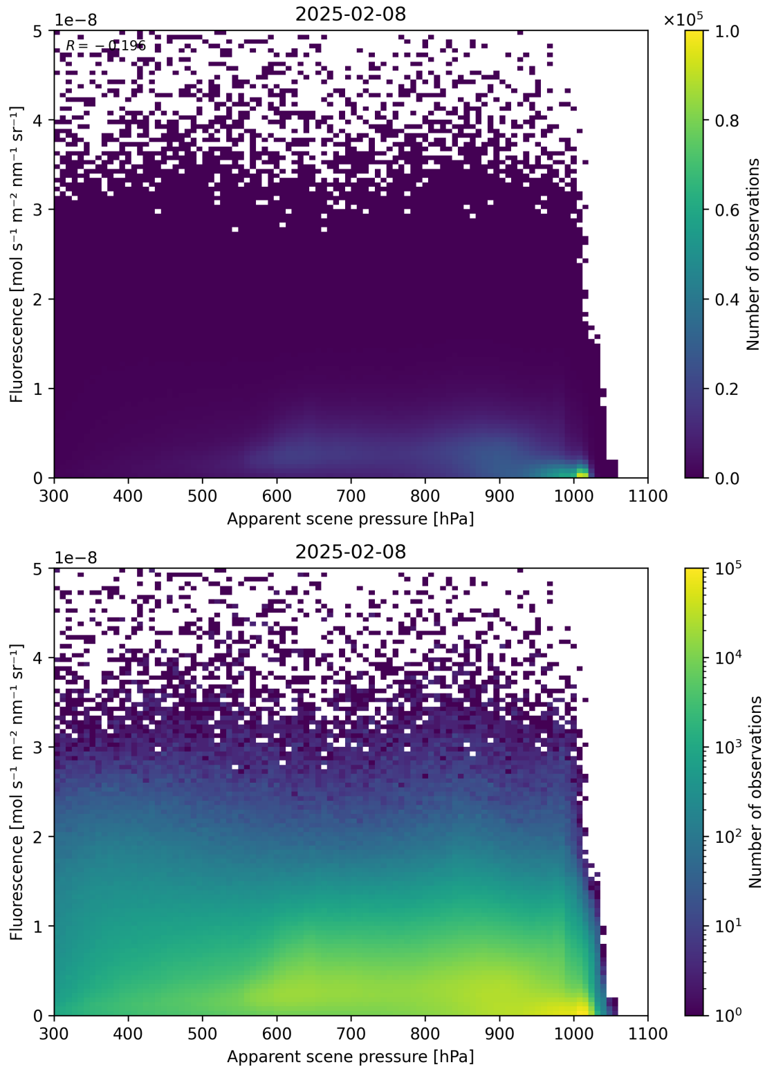
Figure 64: Scatter density plot of “Apparent scene pressure” against “Fluorescence” for 2025-02-08 to 2025-02-09.
