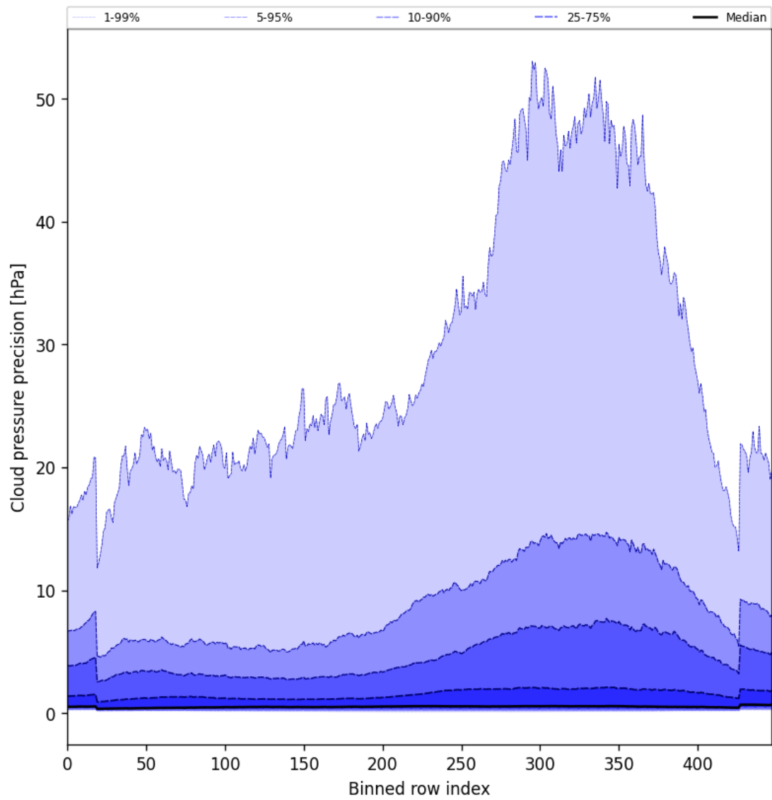
Figure 48: Along track statistics of “Cloud pressure precision” for 2025-02-08 to 2025-02-09
