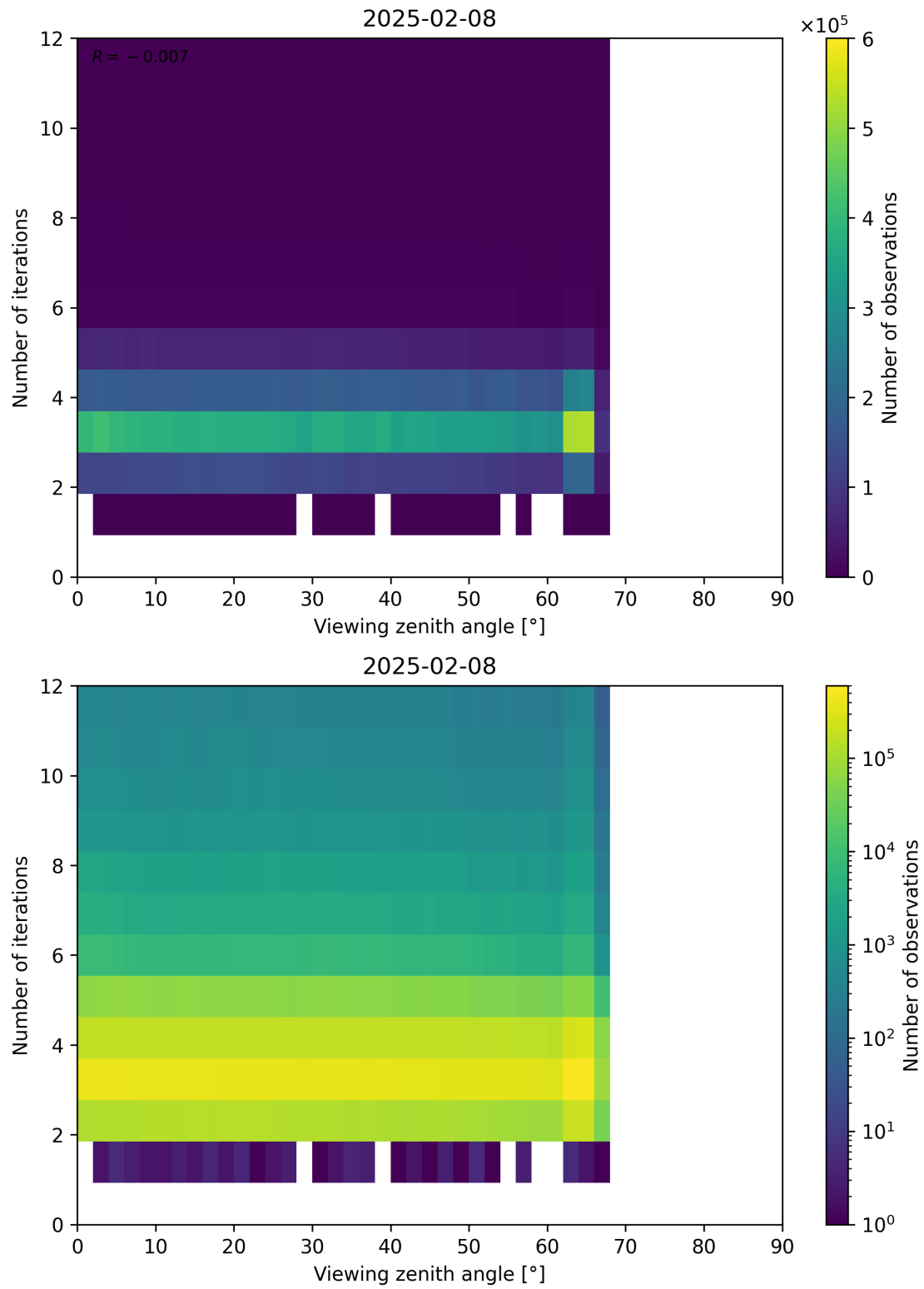
Figure 124: Scatter density plot of “Viewing zenith angle” against “Number of iterations” for 2025-02-08 to 2025-02-09.
