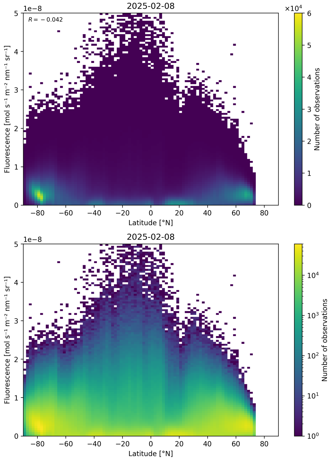
Figure 92: Scatter density plot of “Latitude” against “Fluorescence” for 2025-02-08 to 2025-02-09.
