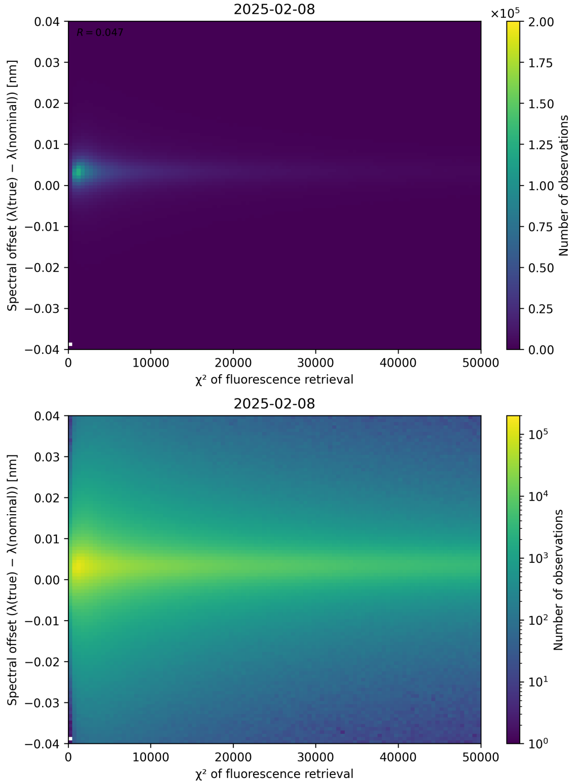
Figure 69: Scatter density plot of “ \chi^2 of fluorescence retrieval” against “Spectral offset ( \lambda_{\text{true}} - \lambda_{\text{nominal}} )” for 2025-02-08 to 2025-02-09.
