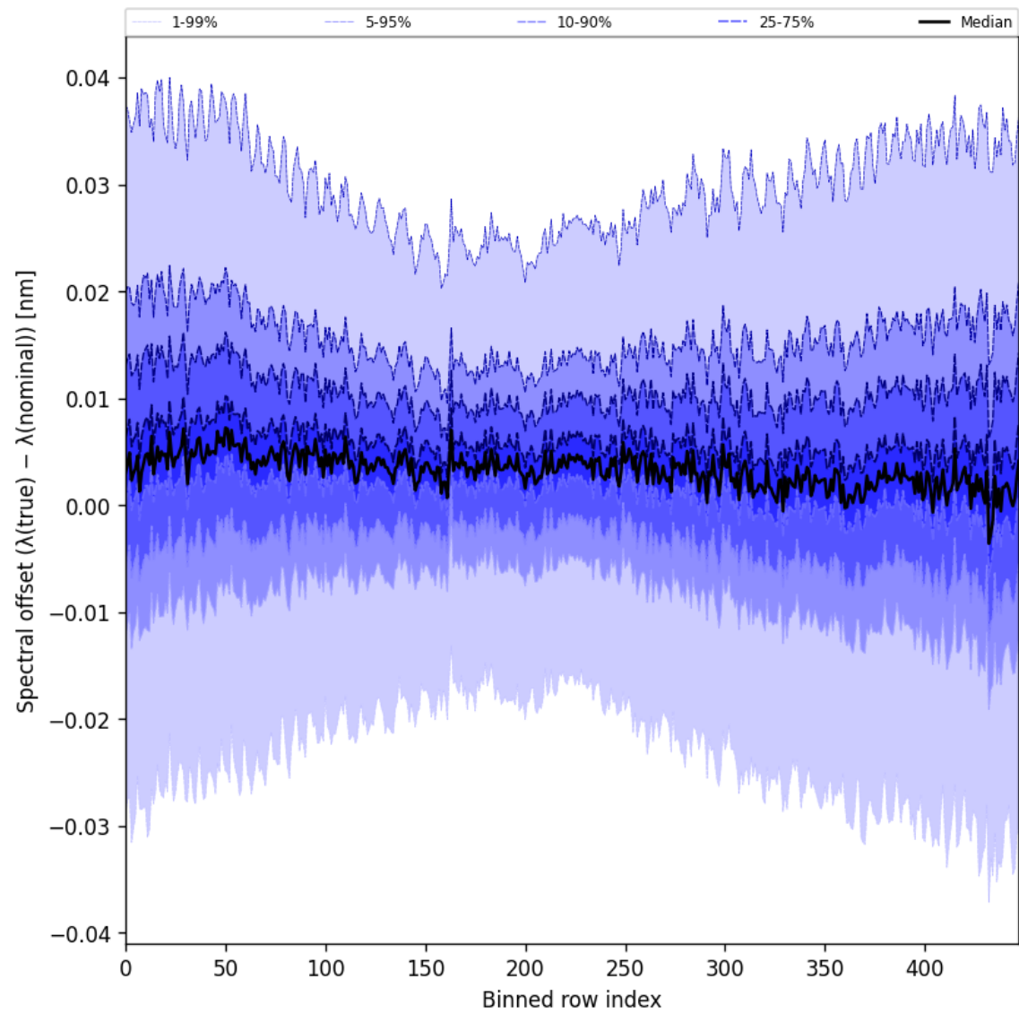
Figure 62: Along track statistics of “Spectral offset ( \lambda_{\text{true}} - \lambda_{\text{nominal}} )” for 2025-02-08 to 2025-02-09
