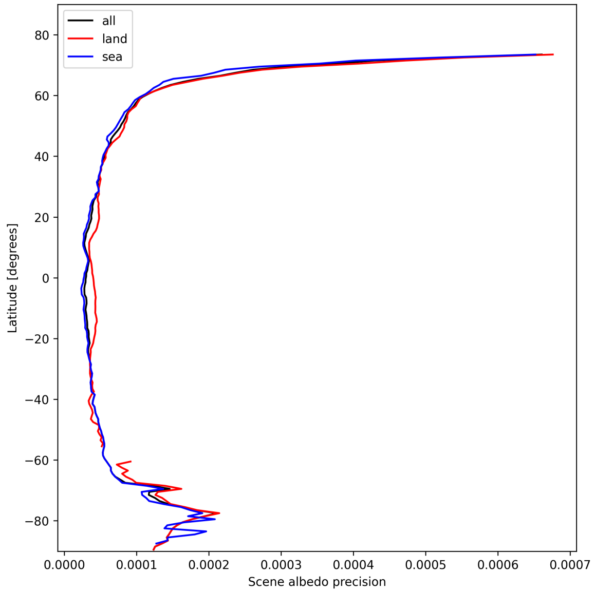
Figure 18: Zonal average of “Scene albedo precision” for 2025-02-08 to 2025-02-09.
