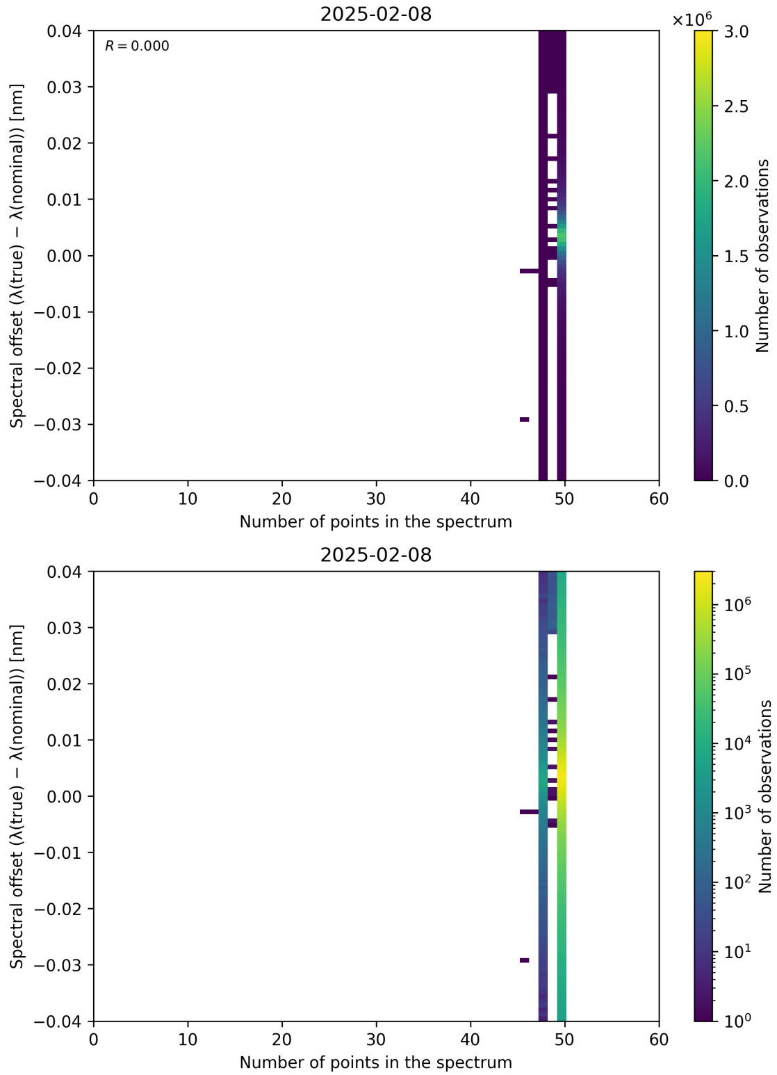
Figure 101: Scatter density plot of “Number of points in the spectrum” against “Spectral offset ( \lambda_{\text{true}} - \lambda_{\text{nominal}} )” for 2025-02-08 to 2025-02-09.
