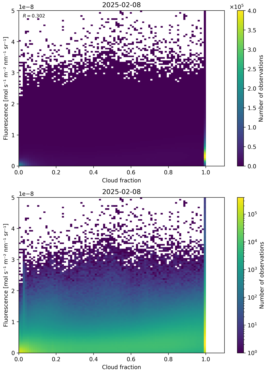
Figure 72: Scatter density plot of “Cloud fraction” against “Fluorescence” for 2025-02-08 to 2025-02-09.
