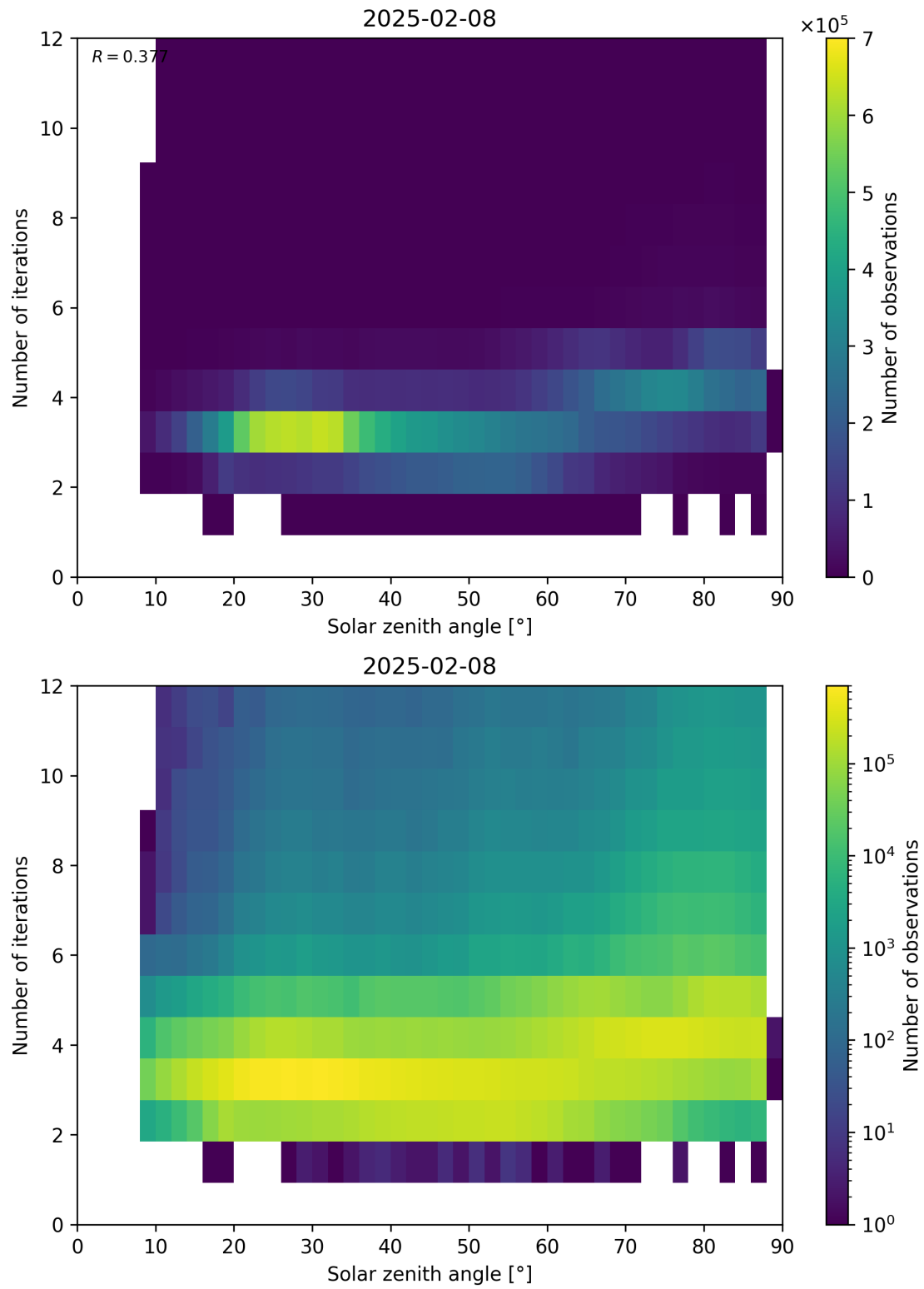
Figure 114: Scatter density plot of “Solar zenith angle” against “Number of iterations” for 2025-02-08 to 2025-02-09.
