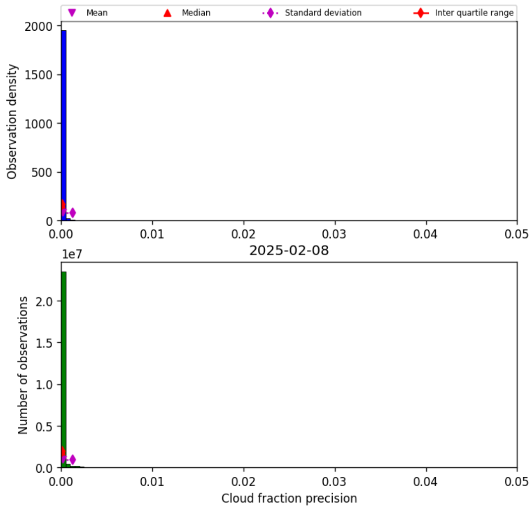
Figure 33: Histogram of “Cloud fraction precision” for 2025-02-08 to 2025-02-09
