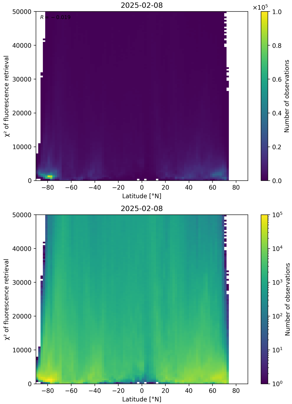
Figure 89: Scatter density plot of “Latitude” against “ \chi^2 of fluorescence retrieval” for 2025-02-08 to 2025-02-09.
