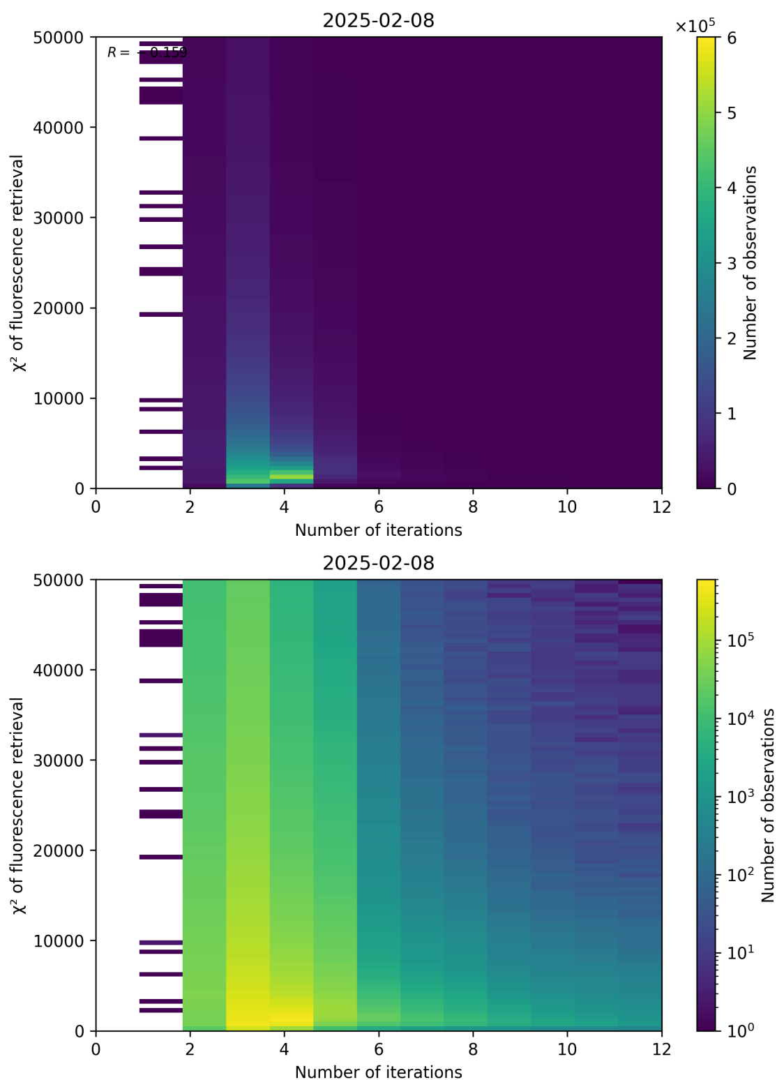
Figure 97: Scatter density plot of “Number of iterations” against “ \chi^2 of fluorescence retrieval” for 2025-02-08 to 2025-02-09.
