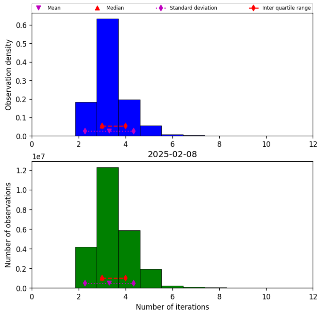
Figure 39: Histogram of “Number of iterations” for 2025-02-08 to 2025-02-09
