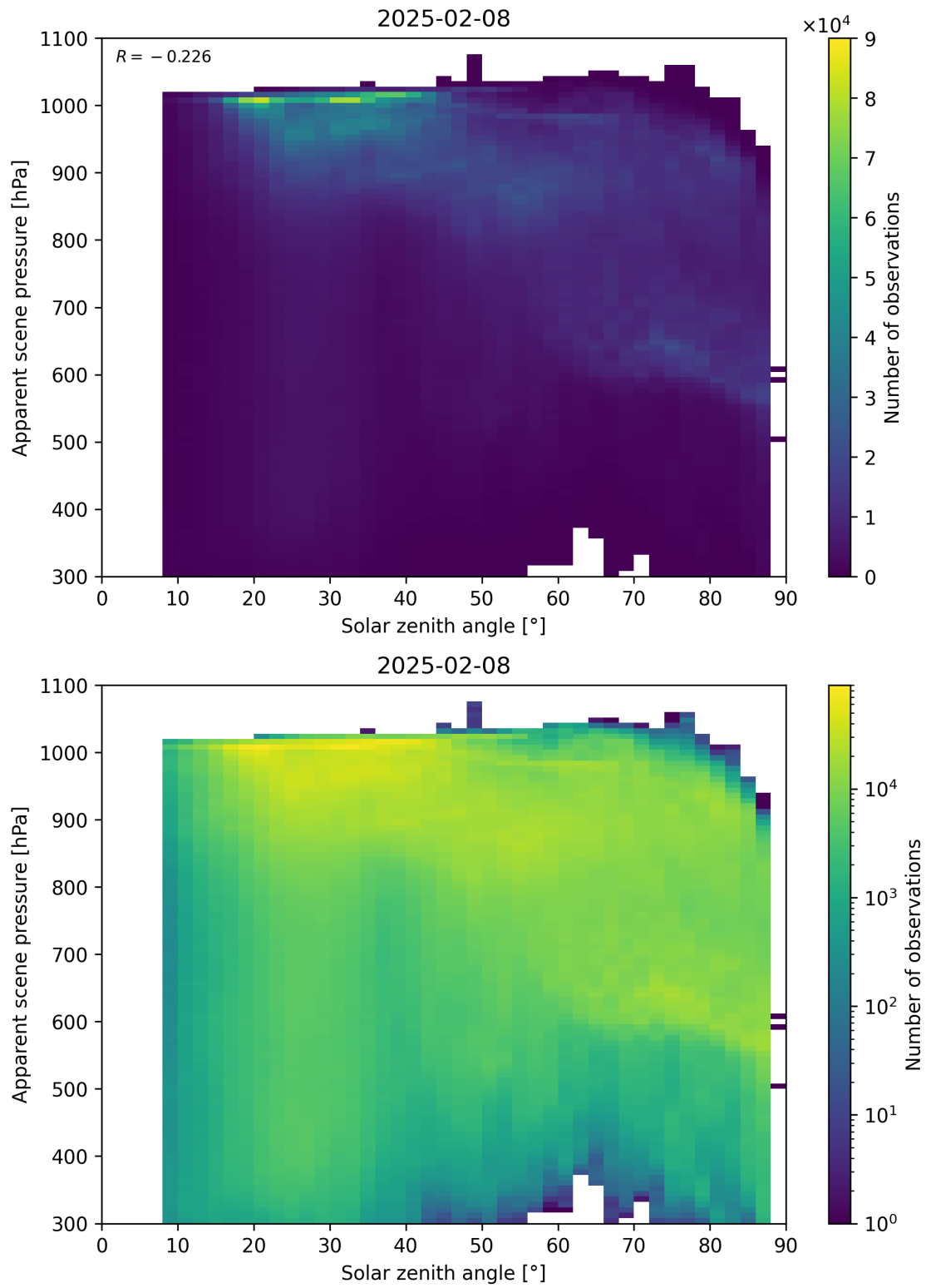
Figure 108: Scatter density plot of “Solar zenith angle” against “Apparent scene pressure” for 2025-02-08 to 2025-02-09.
