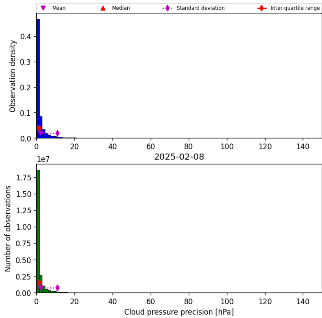
Figure 31: Histogram of “Cloud pressure precision” for 2025-02-08 to 2025-02-09
