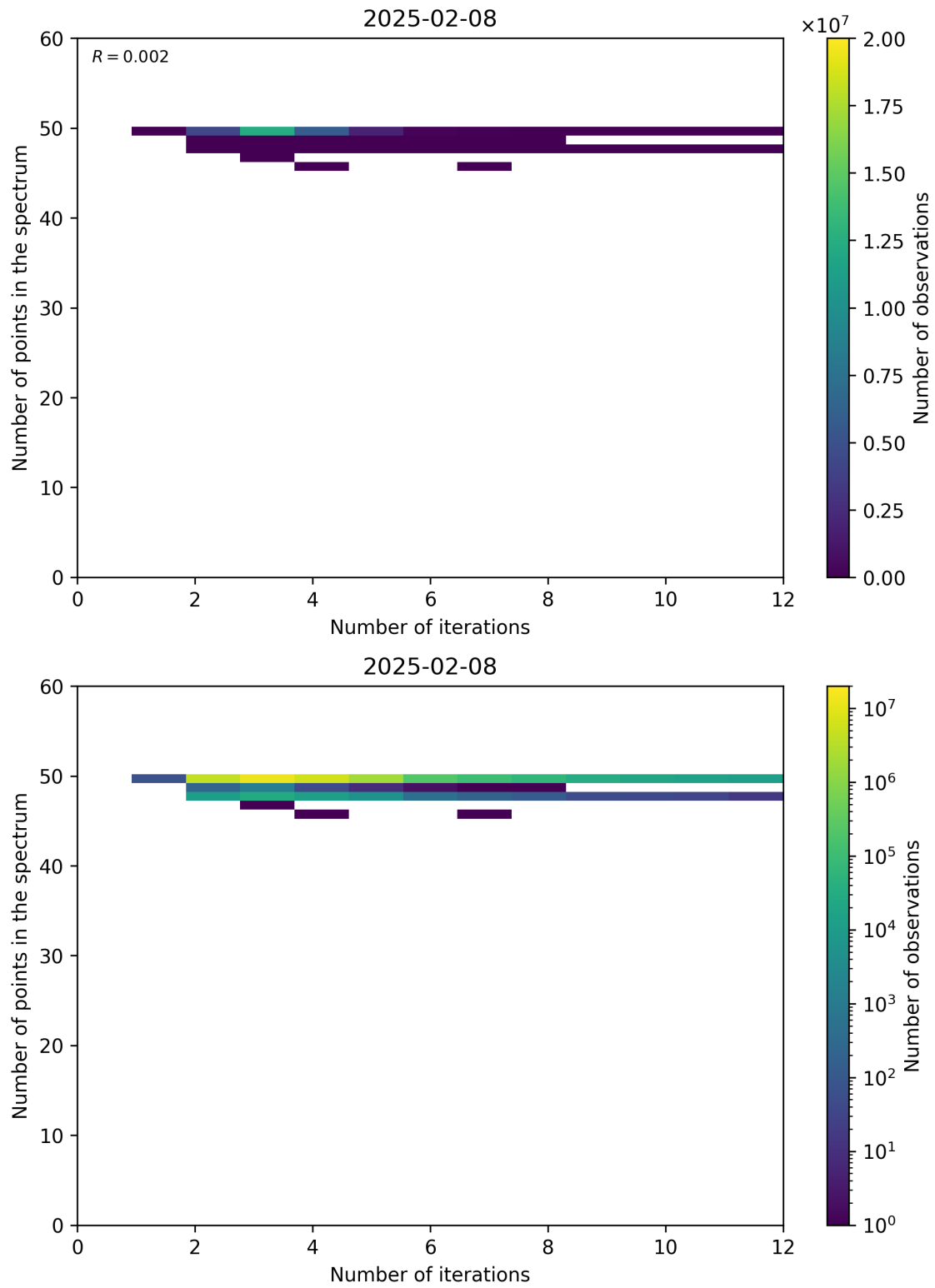
Figure 99: Scatter density plot of “Number of iterations” against “Number of points in the spectrum” for 2025-02-08 to 2025-02-09.
