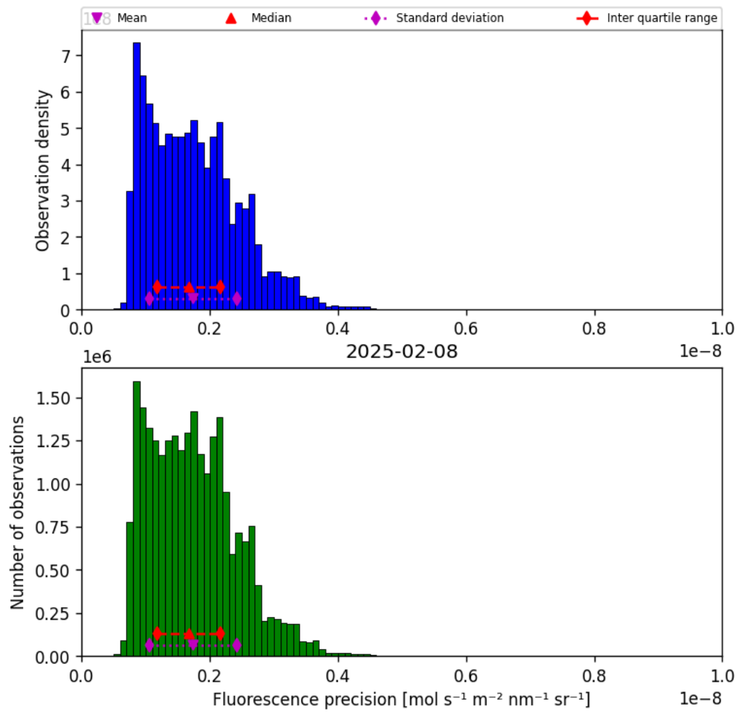
Figure 41: Histogram of “Fluorescence precision” for 2025-02-08 to 2025-02-09
