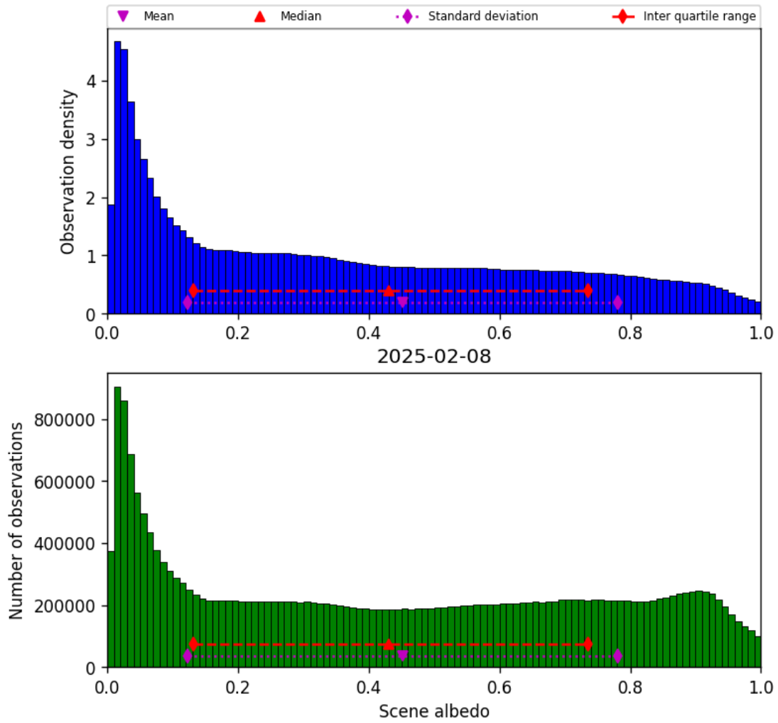
Figure 34: Histogram of “Scene albedo” for 2025-02-08 to 2025-02-09
