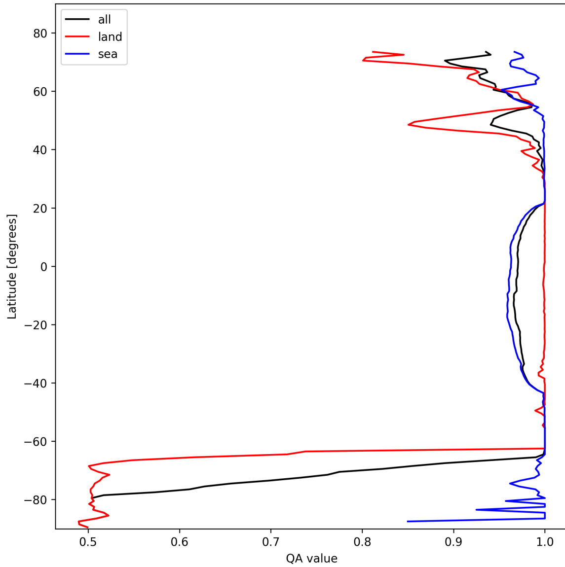
Figure 12: Zonal average of “QA value” for 2025-02-08 to 2025-02-09.
