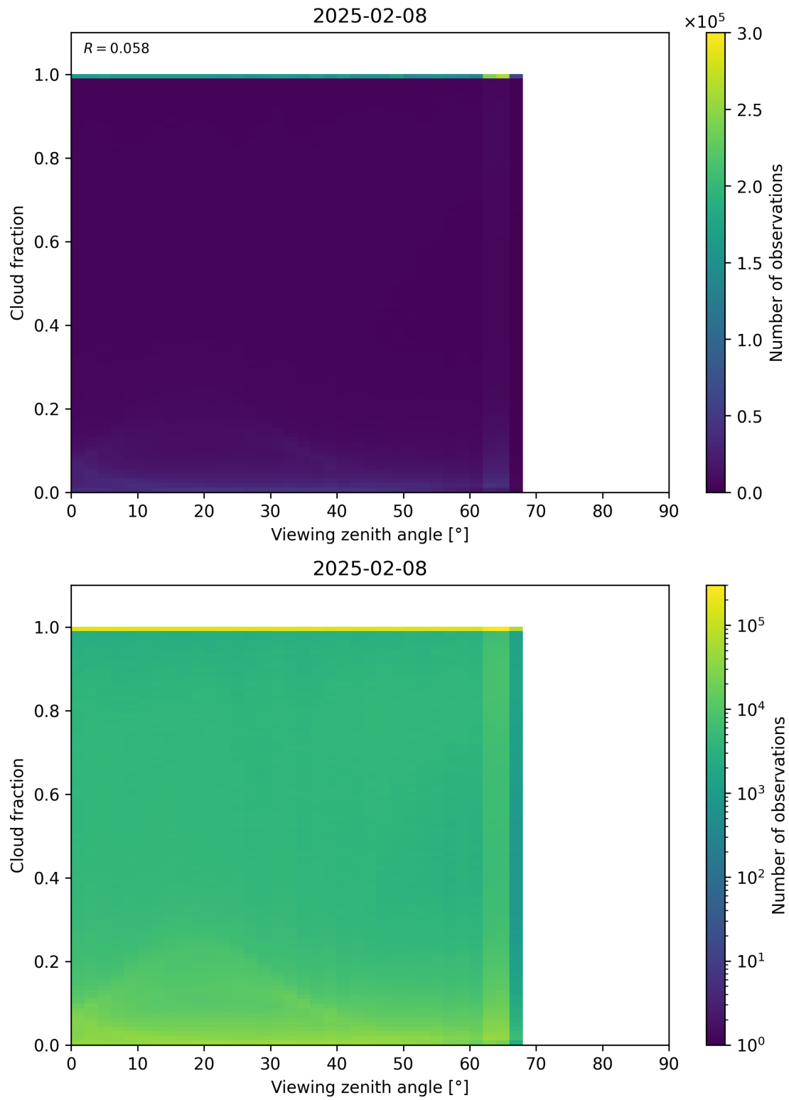
Figure 120: Scatter density plot of “Viewing zenith angle” against “Cloud fraction” for 2025-02-08 to 2025-02-09.
