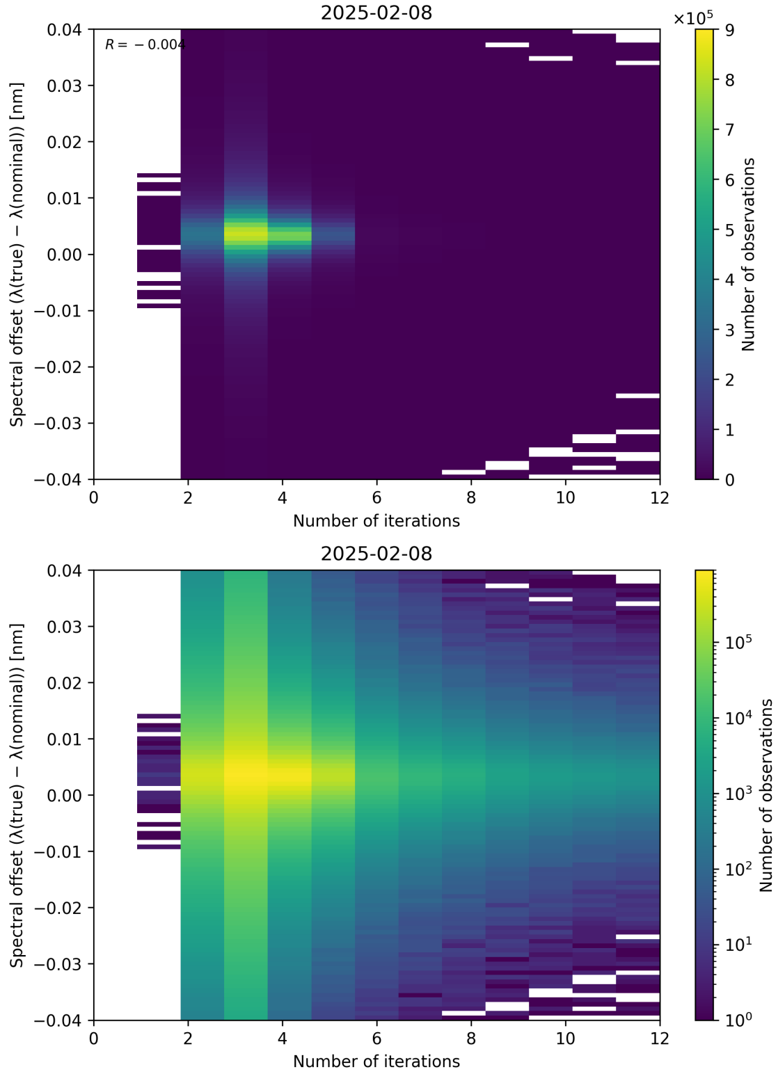
Figure 100: Scatter density plot of “Number of iterations” against “Spectral offset ( \lambda_{\text{true}} - \lambda_{\text{nominal}} )” for 2025-02-08 to 2025-02-09.
