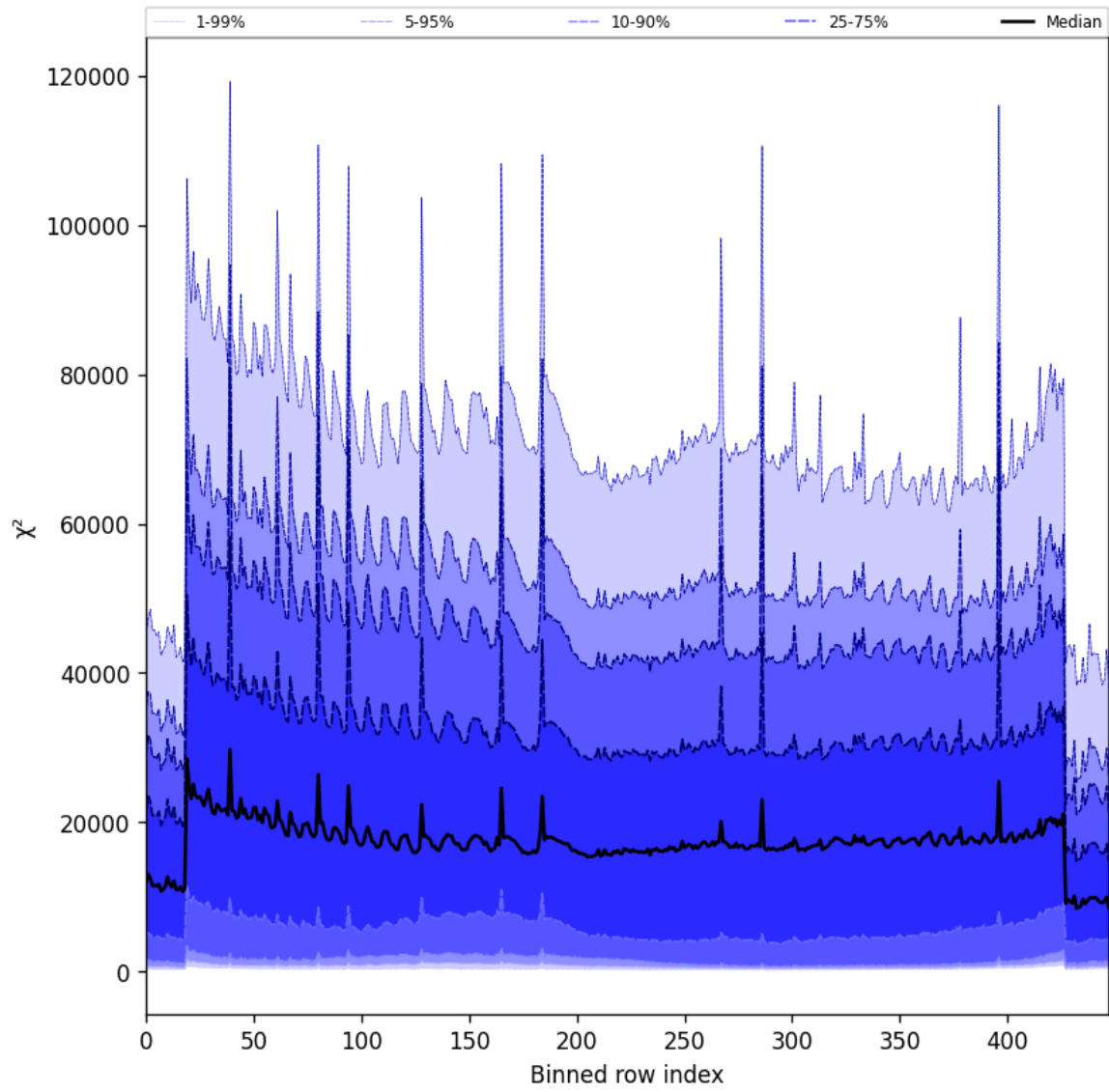
Figure 55: Along track statistics of “ \chi^2 ” for 2025-02-08 to 2025-02-09
