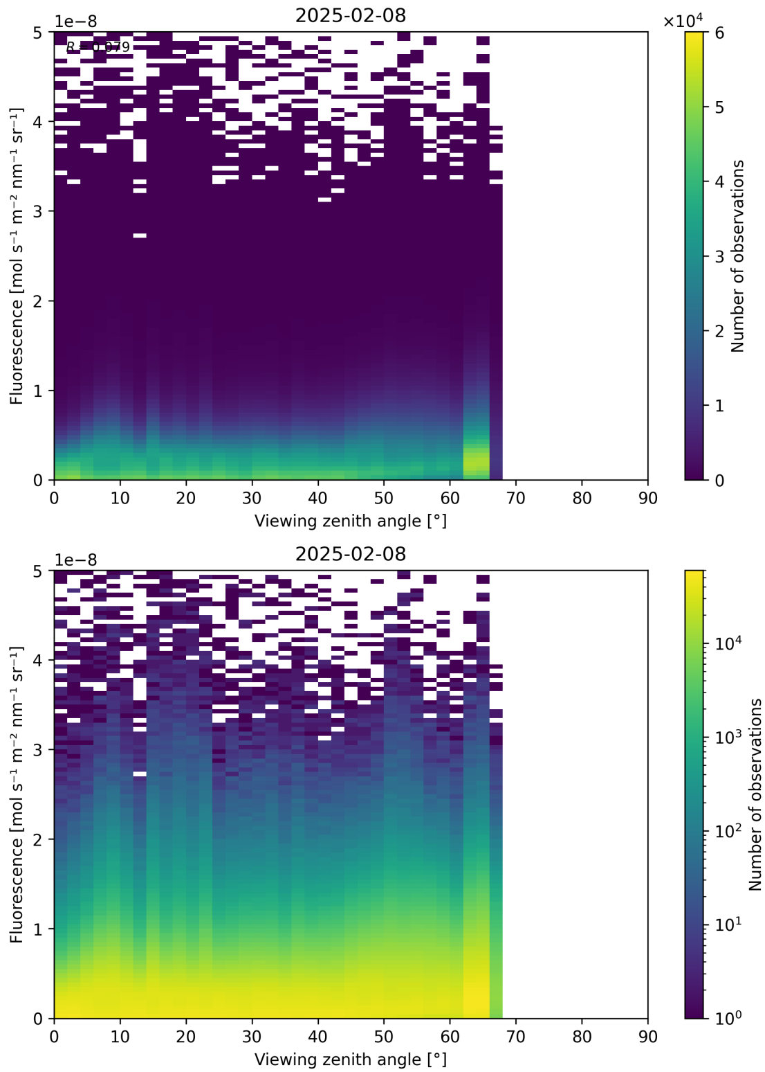
Figure 122: Scatter density plot of “Viewing zenith angle” against “Fluorescence” for 2025-02-08 to 2025-02-09.
