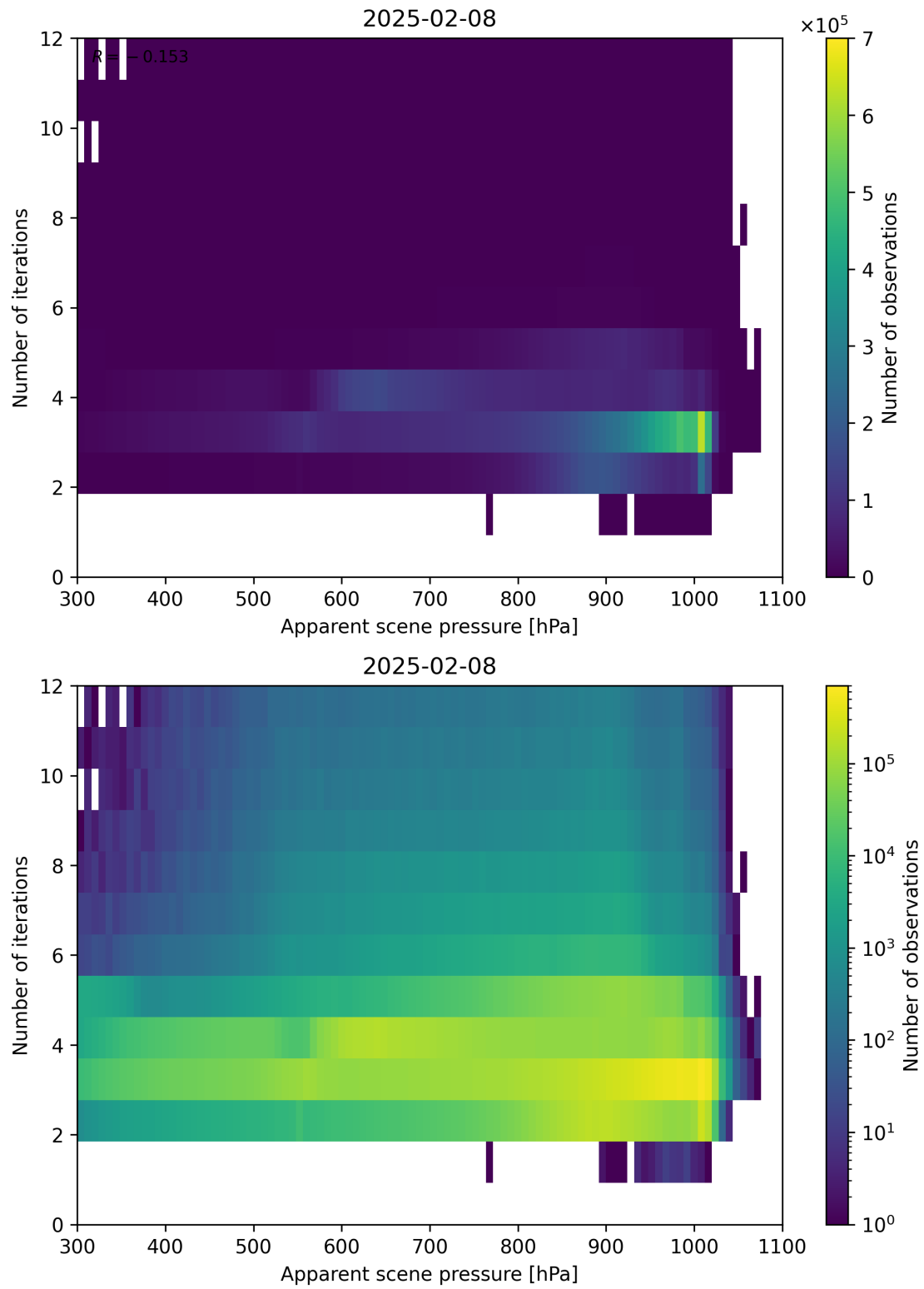
Figure 65: Scatter density plot of “Apparent scene pressure” against “Number of iterations” for 2025-02-08 to 2025-02-09.
