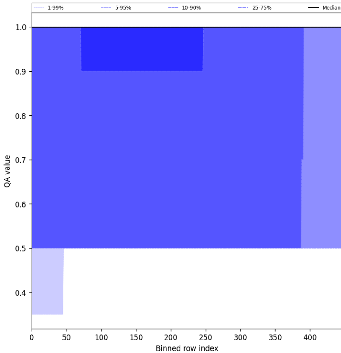
Figure 46: Along track statistics of “QA value” for 2025-02-08 to 2025-02-09
