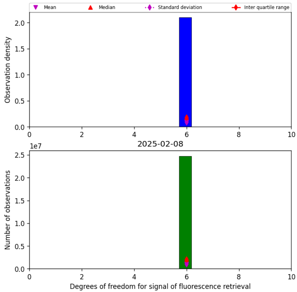
Figure 43: Histogram of “Degrees of freedom for signal of fluorescence retrieval” for 2025-02-08 to 2025-02-09
