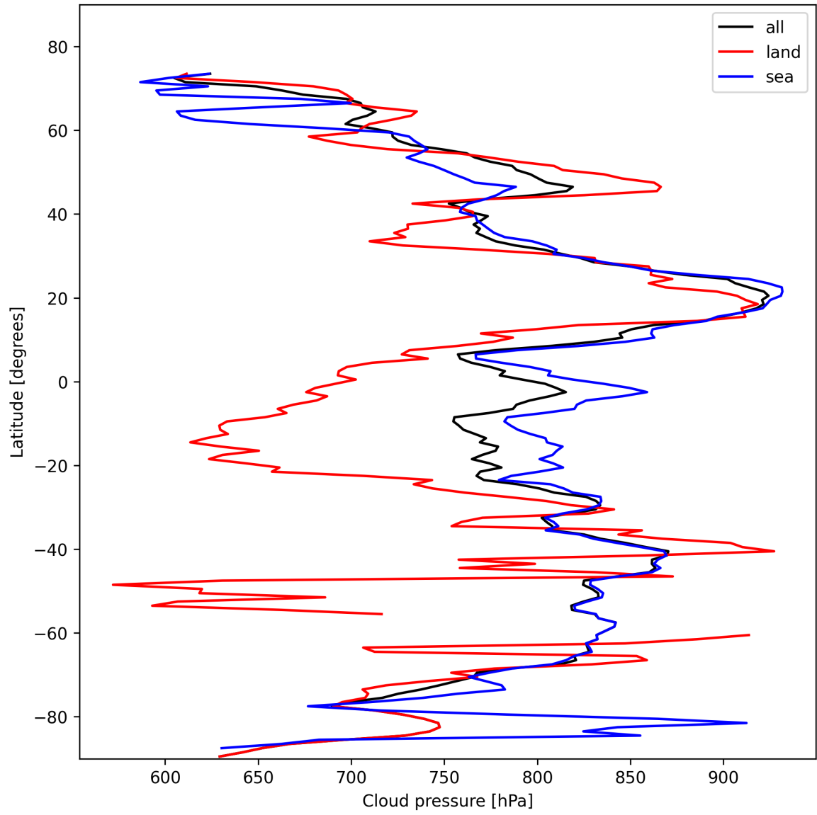
Figure 13: Zonal average of “Cloud pressure” for 2025-02-08 to 2025-02-09.
