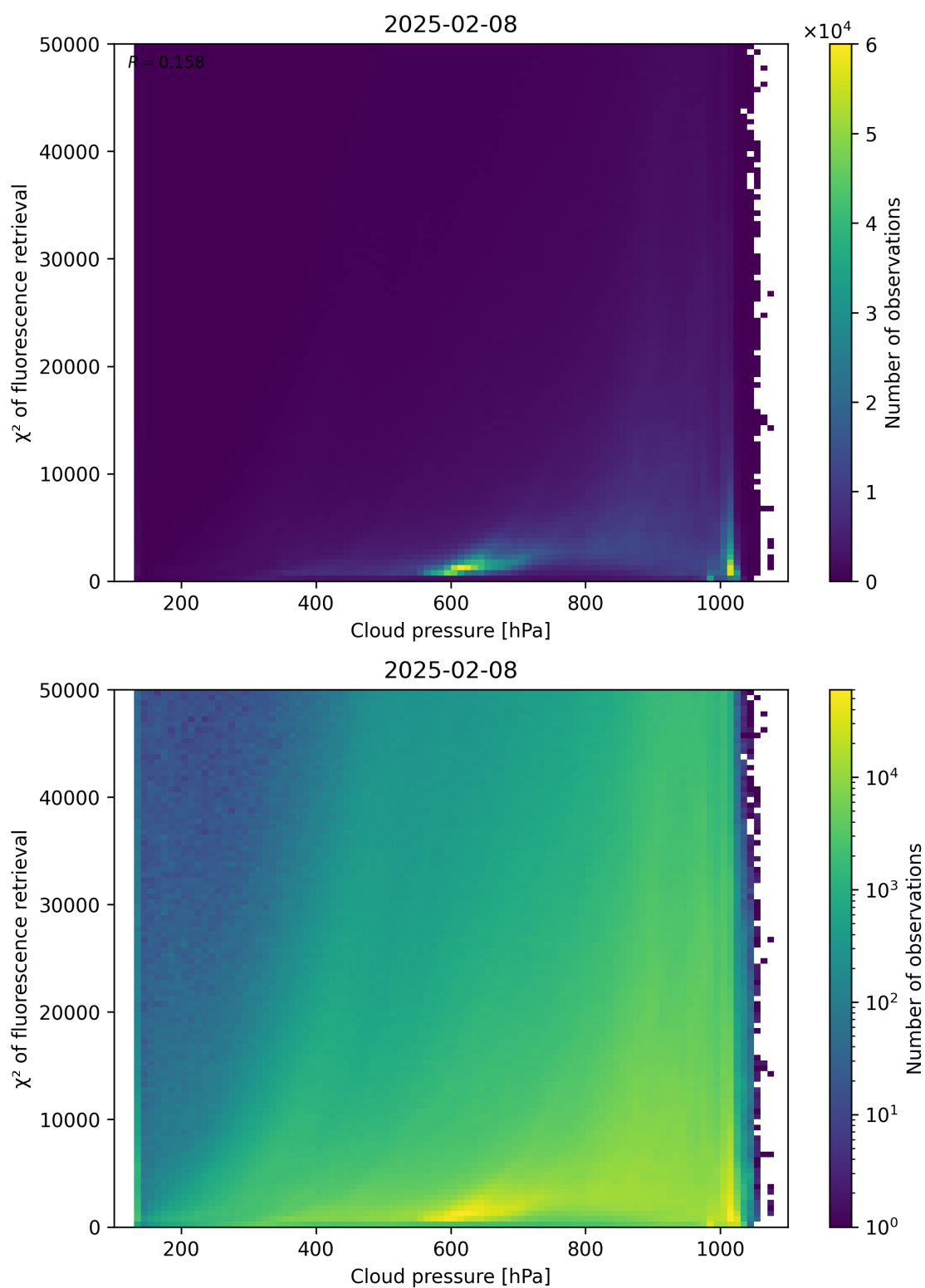
Figure 78: Scatter density plot of “Cloud pressure” against “ \chi^2 of fluorescence retrieval” for 2025-02-08 to 2025-02-09.
