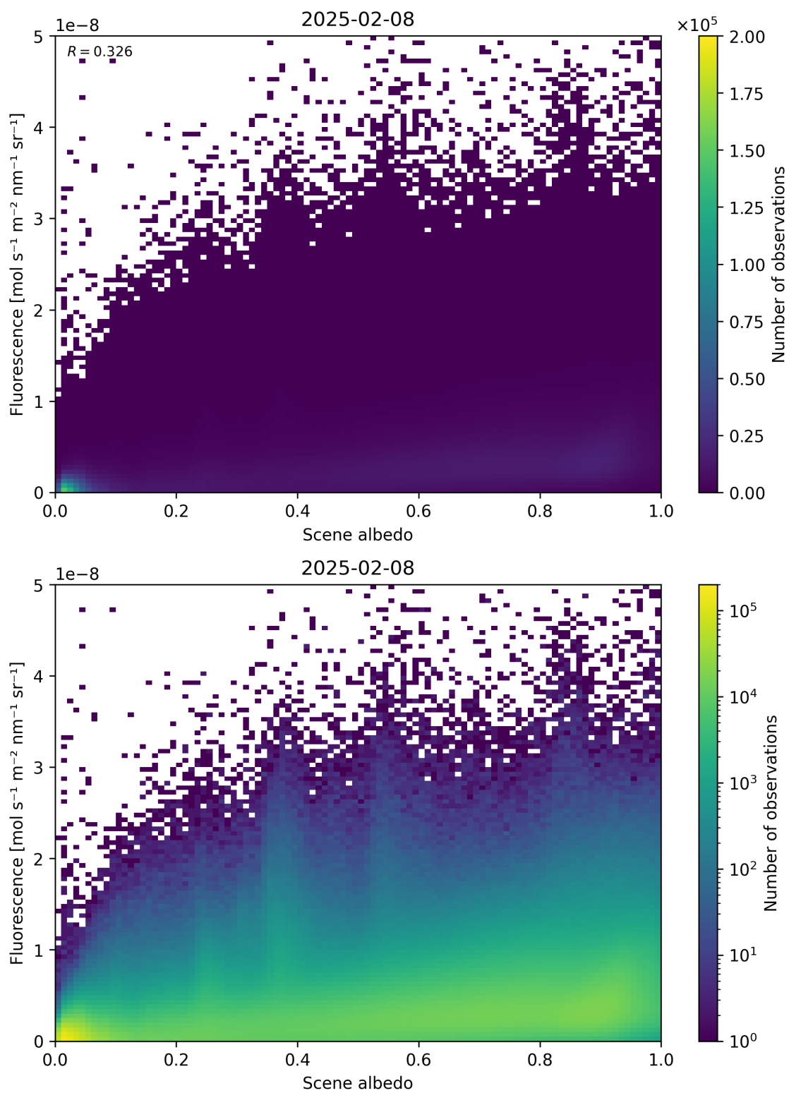
Figure 104: Scatter density plot of “Scene albedo” against “Fluorescence” for 2025-02-08 to 2025-02-09.
