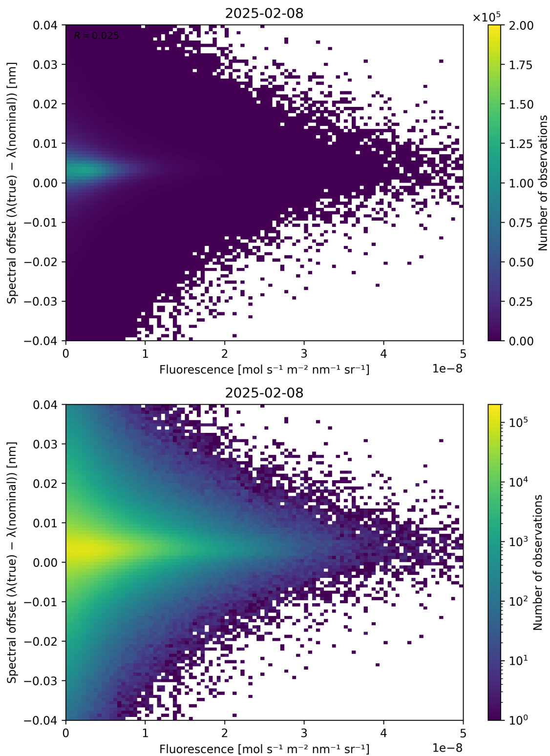
Figure 87: Scatter density plot of “Fluorescence” against “Spectral offset ( \lambda_{\text{true}} - \lambda_{\text{nominal}} )” for 2025-02-08 to 2025-02-09.
