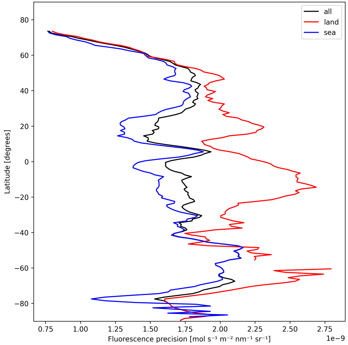
Figure 24: Zonal average of “Fluorescence precision” for 2025-02-08 to 2025-02-09.
