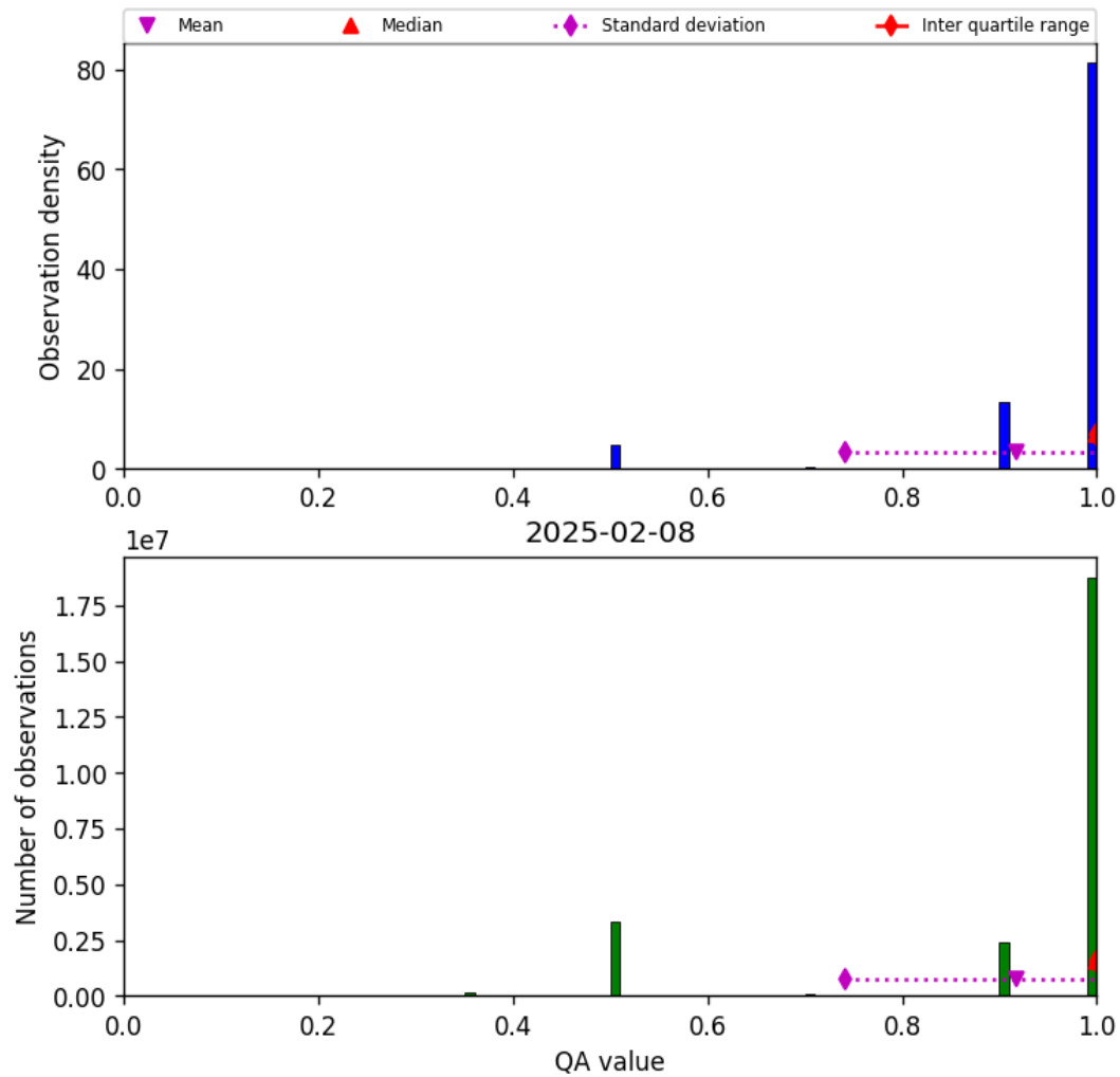
Figure 29: Histogram of “QA value” for 2025-02-08 to 2025-02-09
