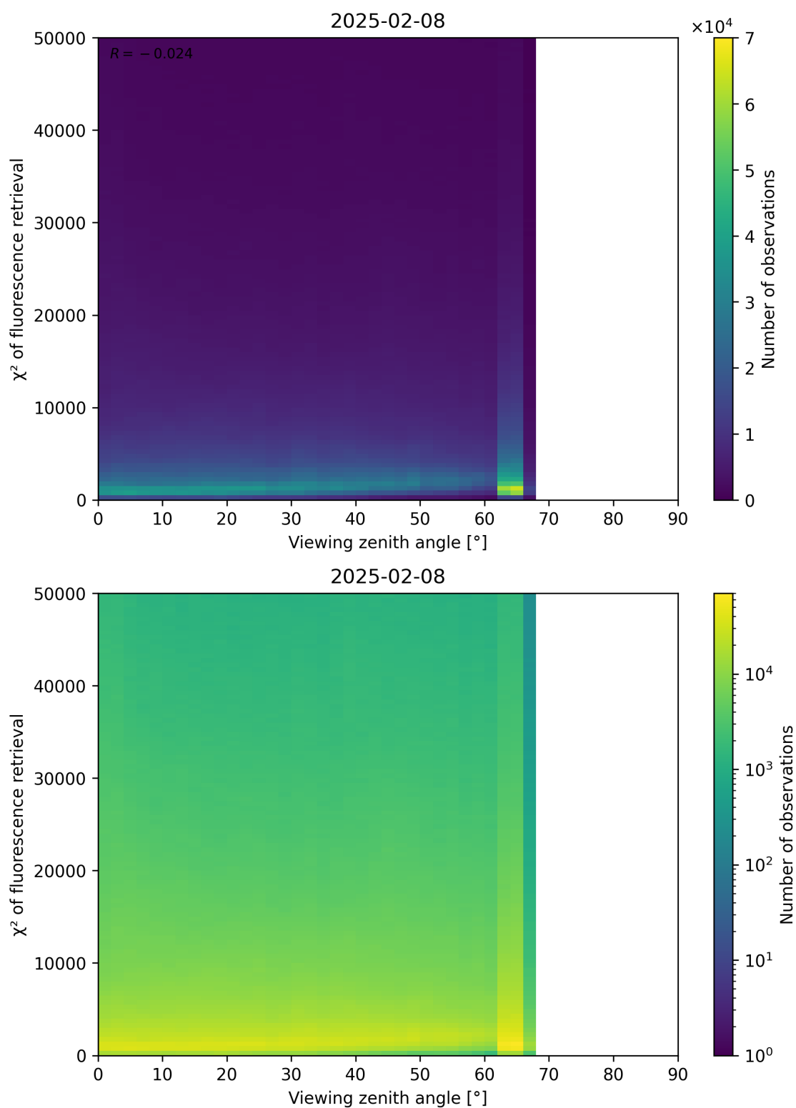
Figure 119: Scatter density plot of “Viewing zenith angle” against “ \chi^2 of fluorescence retrieval” for 2025-02-08 to 2025-02-09.
