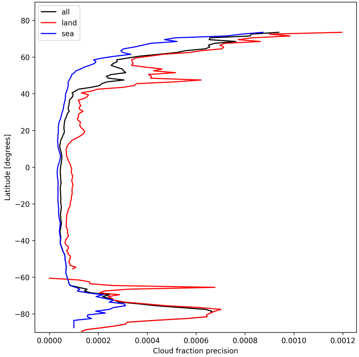
Figure 16: Zonal average of “Cloud fraction precision” for 2025-02-08 to 2025-02-09.
