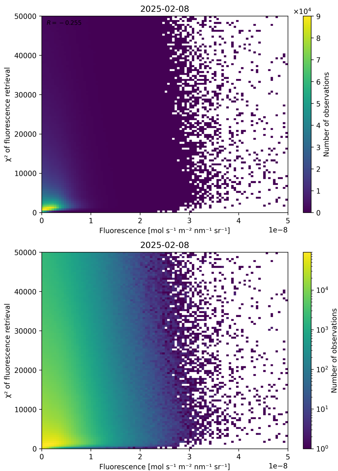
Figure 85: Scatter density plot of “Fluorescence” against “ \chi^2 of fluorescence retrieval” for 2025-02-08 to 2025-02-09.
