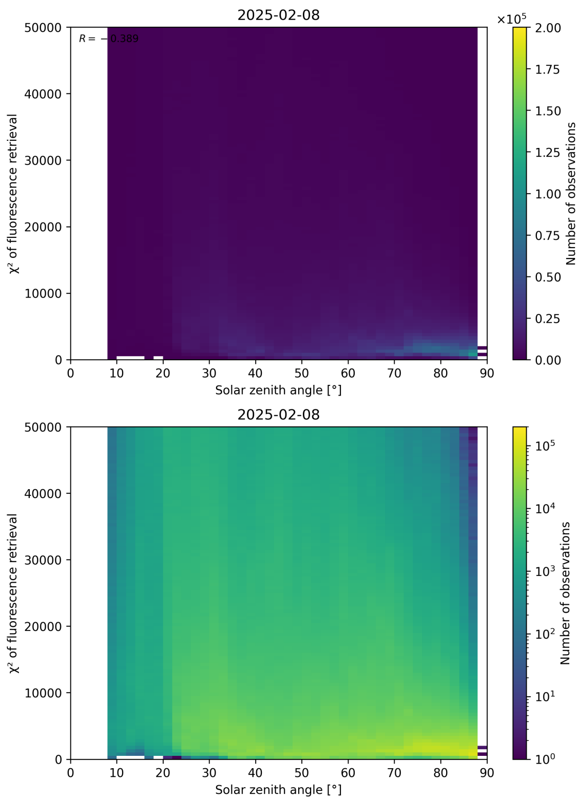
Figure 109: Scatter density plot of “Solar zenith angle” against “ \chi^2 of fluorescence retrieval” for 2025-02-08 to 2025-02-09.
