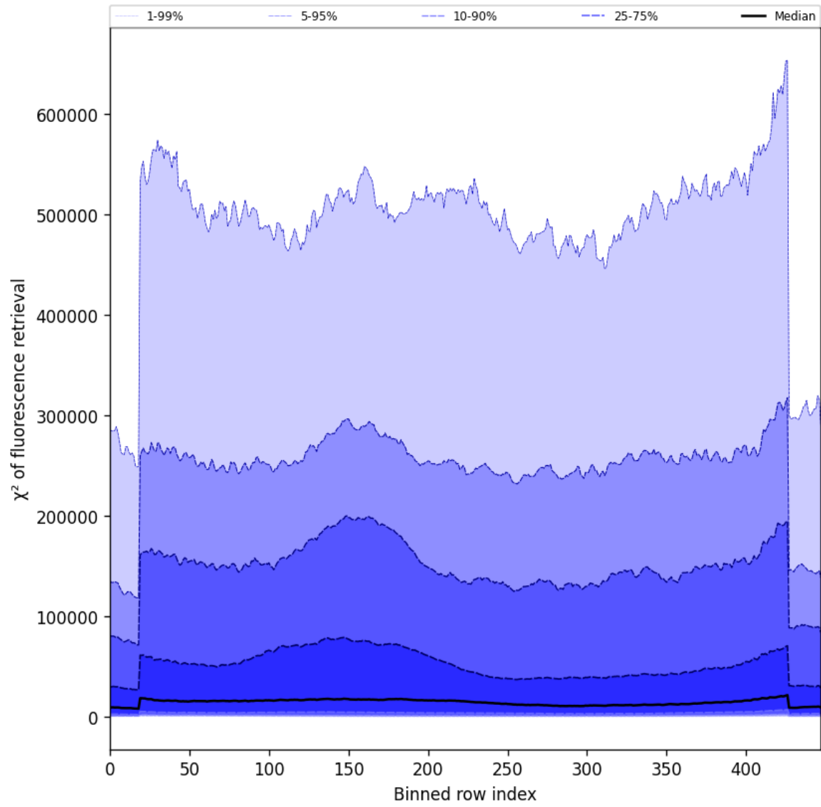
Figure 59: Along track statistics of “ \chi^2 of fluorescence retrieval” for 2025-02-08 to 2025-02-09
