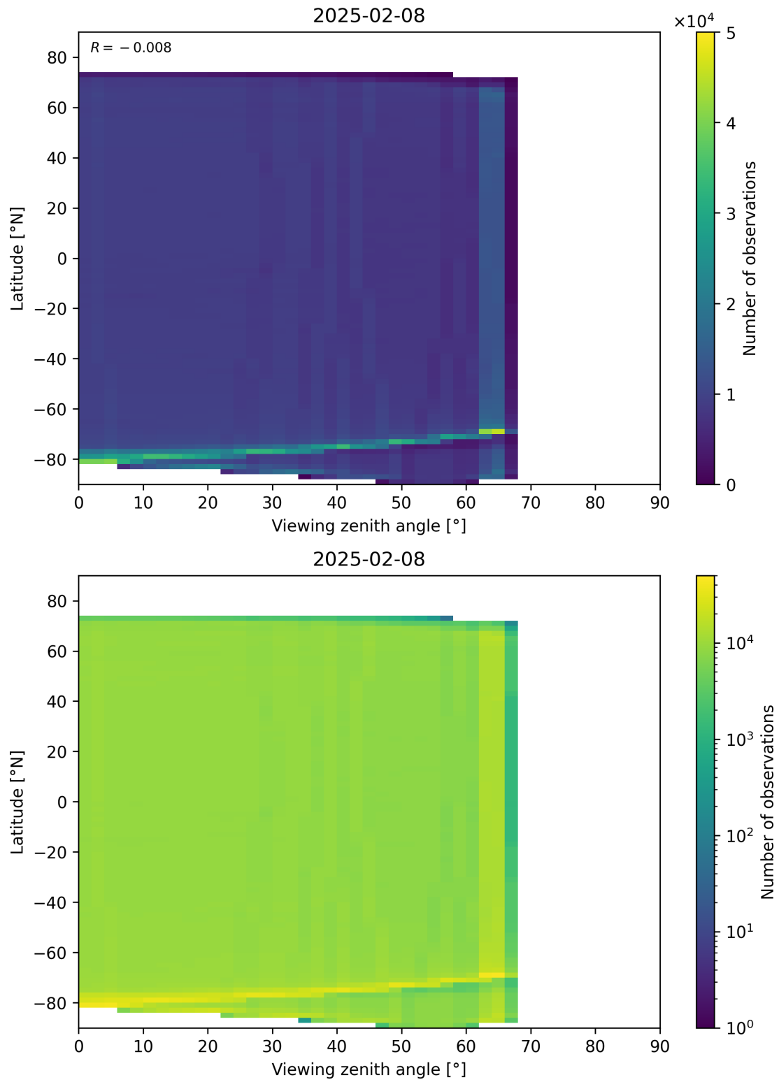
Figure 123: Scatter density plot of “Viewing zenith angle” against “Latitude” for 2025-02-08 to 2025-02-09.
