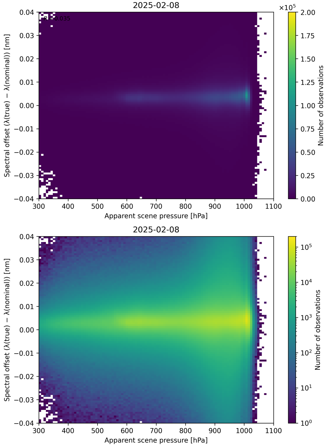
Figure 67: Scatter density plot of “Apparent scene pressure” against “Spectral offset ( \lambda_{\text{true}} - \lambda_{\text{nominal}} )” for 2025-02-08 to 2025-02-09.
