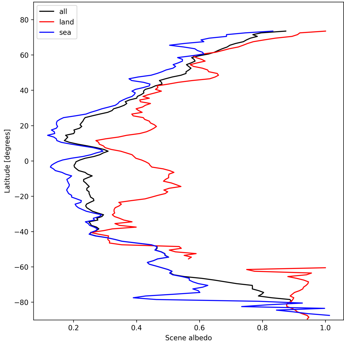
Figure 17: Zonal average of “Scene albedo” for 2025-02-08 to 2025-02-09.
