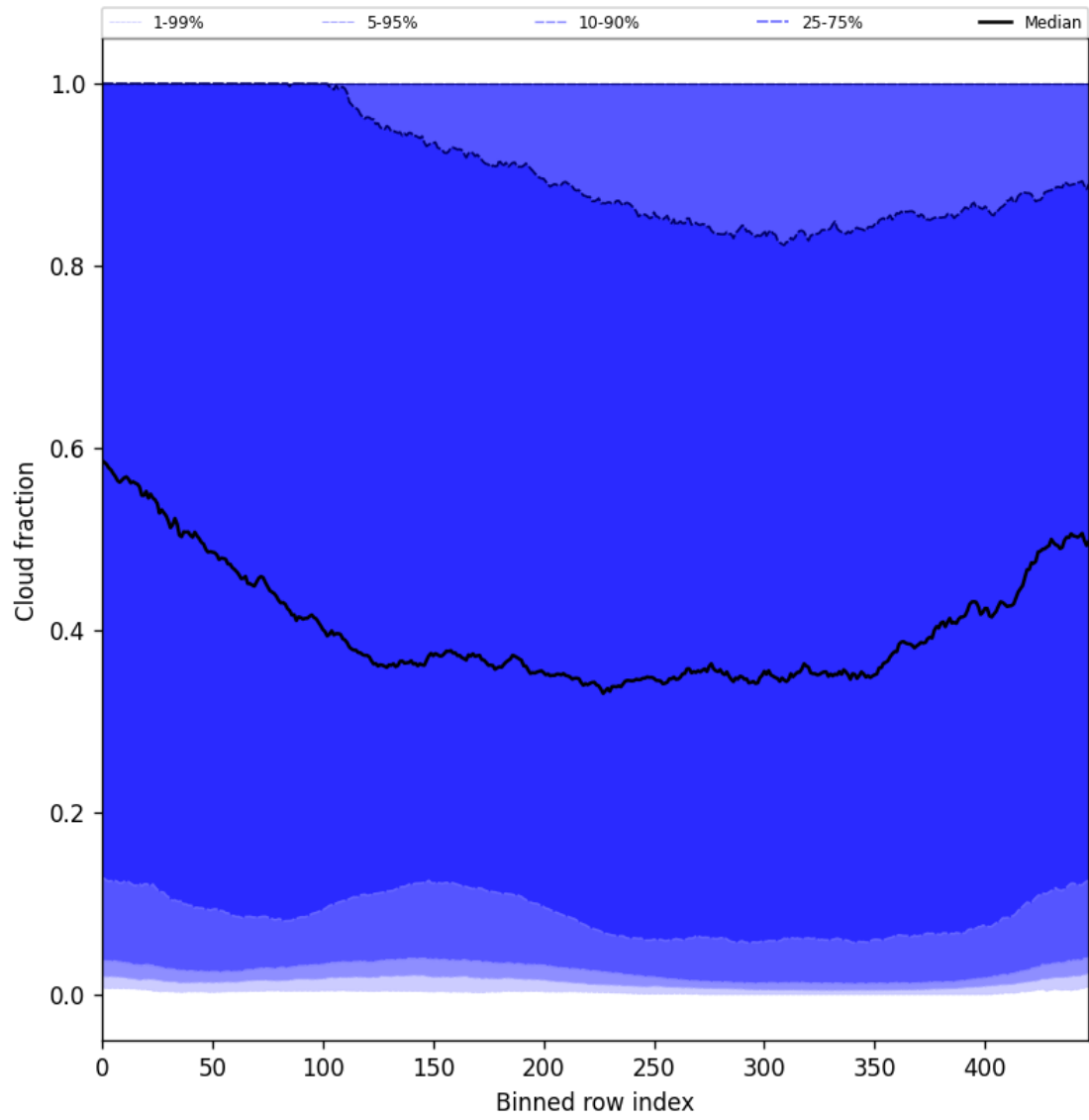
Figure 49: Along track statistics of “Cloud fraction” for 2025-02-08 to 2025-02-09
