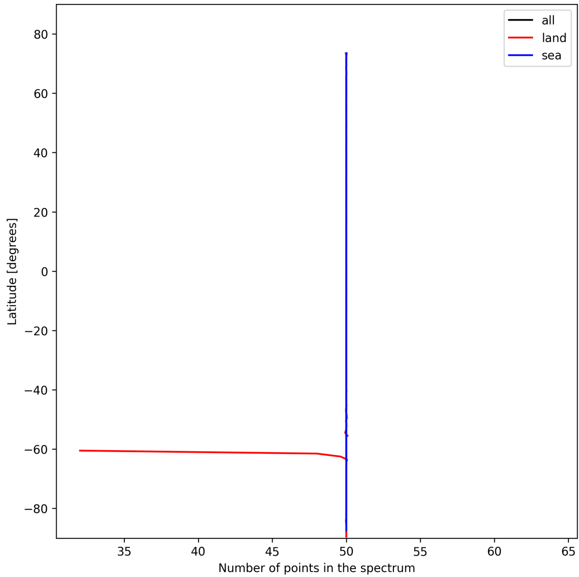
Figure 27: Zonal average of “Number of points in the spectrum” for 2025-02-08 to 2025-02-09.
