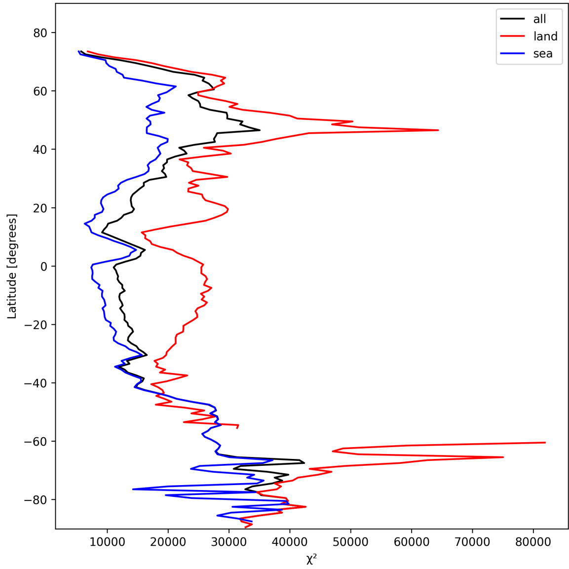
Figure 21: Zonal average of “ \chi^2 ” for 2025-02-08 to 2025-02-09.
