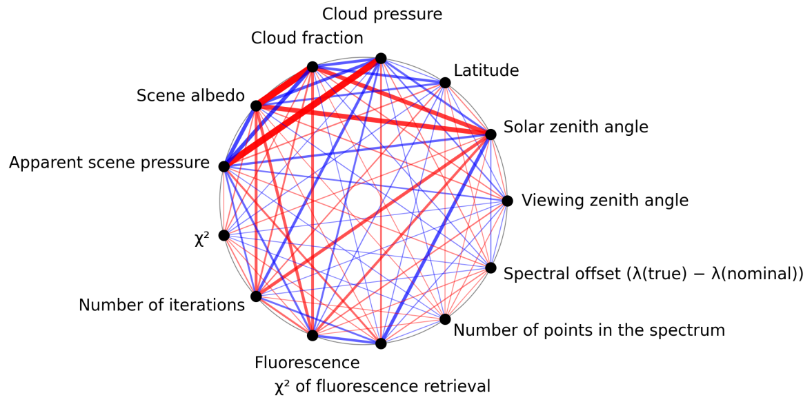
Figure 1: Map of correlation graph for 2025-02-08 to 2025-02-09.
