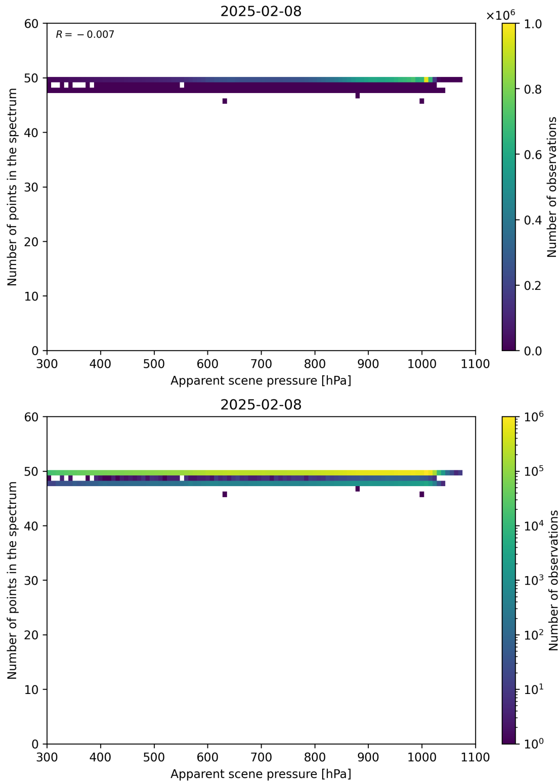
Figure 66: Scatter density plot of “Apparent scene pressure” against “Number of points in the spectrum” for 2025-02-08 to 2025-02-09.
