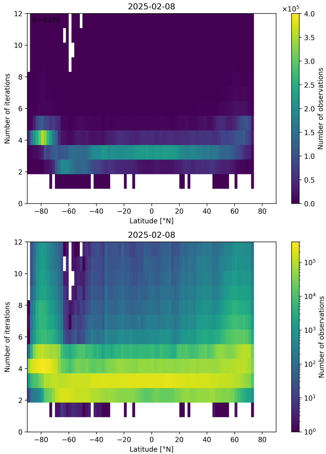
Figure 93: Scatter density plot of “Latitude” against “Number of iterations” for 2025-02-08 to 2025-02-09.
