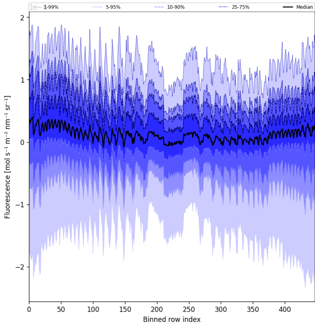
Figure 57: Along track statistics of “Fluorescence” for 2025-02-08 to 2025-02-09
