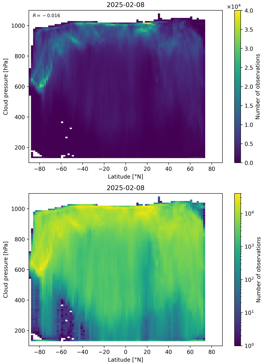
Figure 91: Scatter density plot of “Latitude” against “Cloud pressure” for 2025-02-08 to 2025-02-09.
