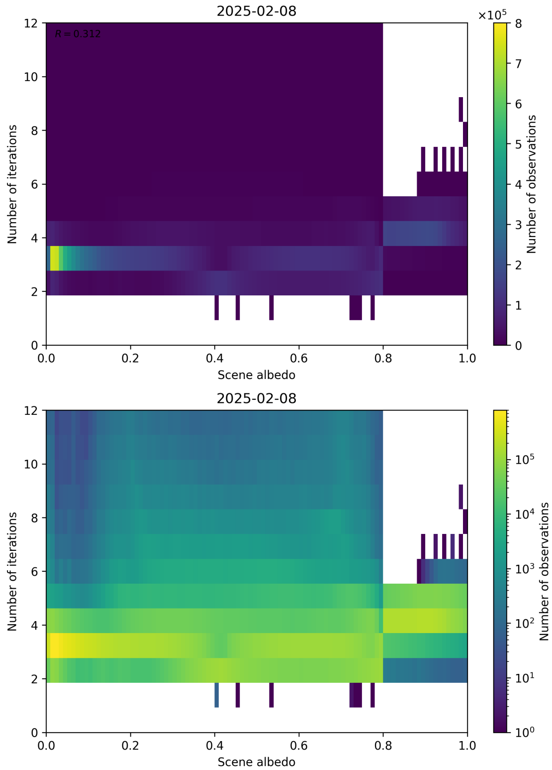
Figure 105: Scatter density plot of “Scene albedo” against “Number of iterations” for 2025-02-08 to 2025-02-09.
