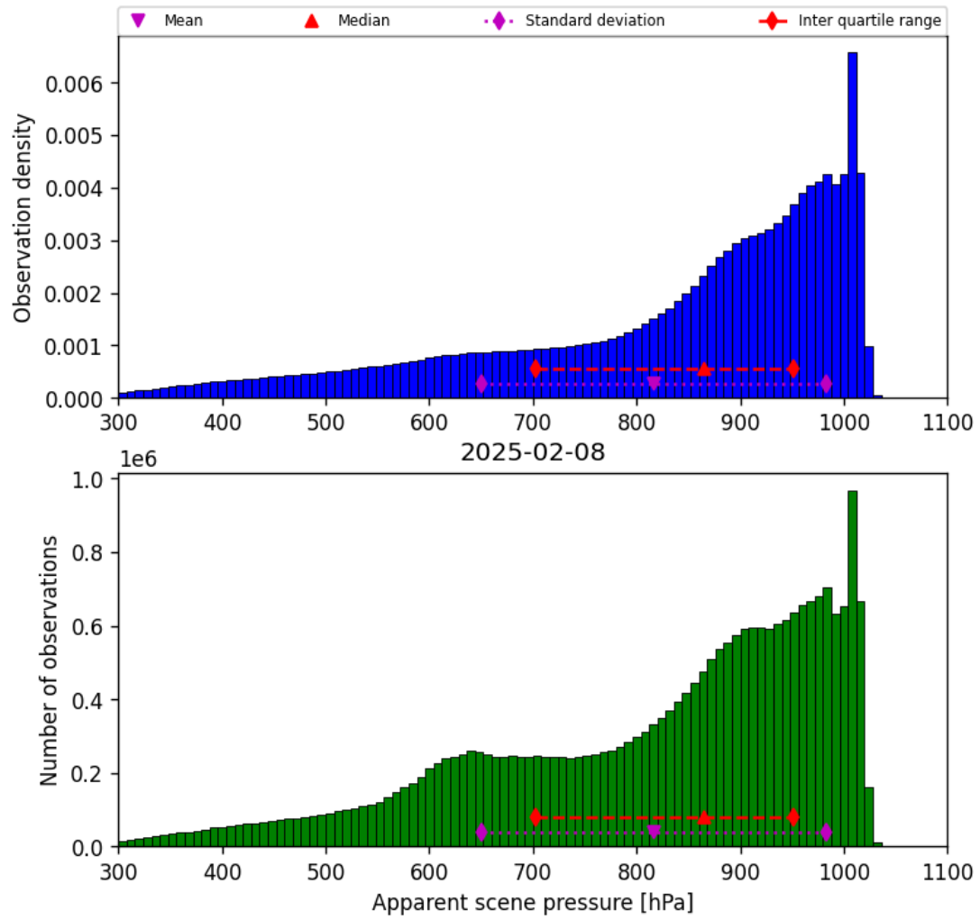
Figure 36: Histogram of “Apparent scene pressure” for 2025-02-08 to 2025-02-09
