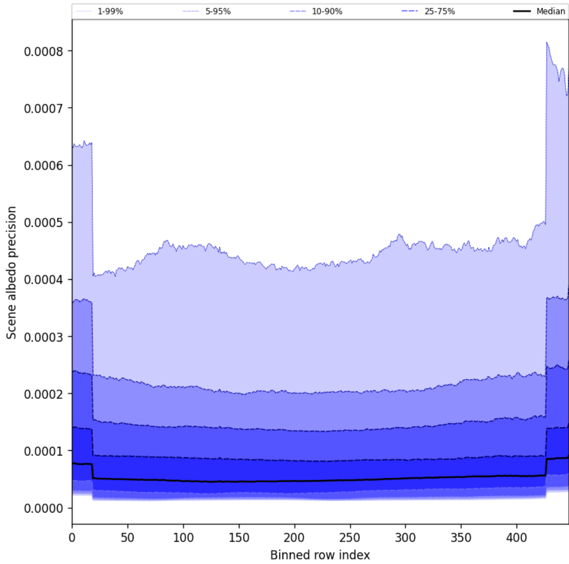
Figure 52: Along track statistics of “Scene albedo precision” for 2025-02-08 to 2025-02-09
