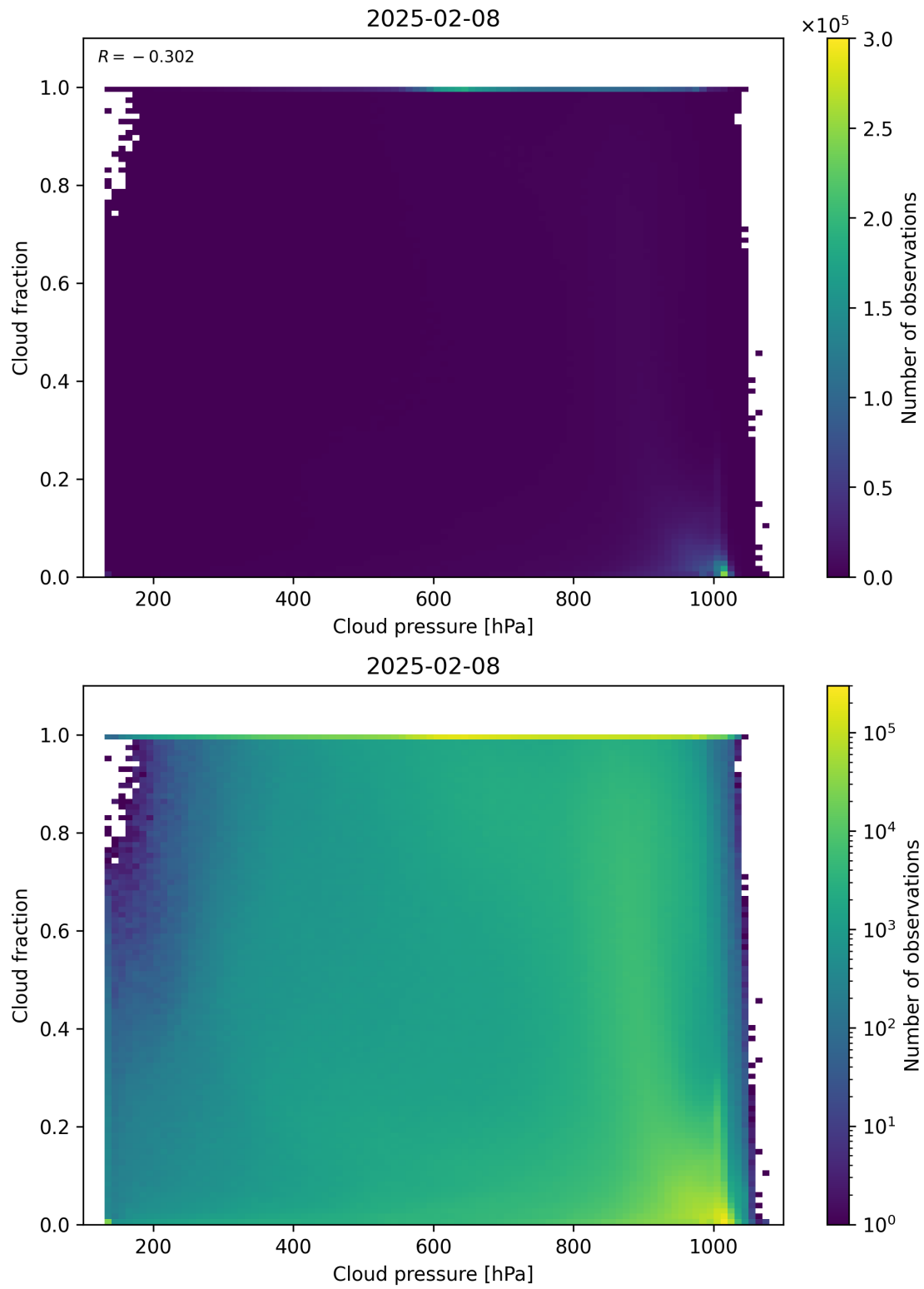
Figure 79: Scatter density plot of “Cloud pressure” against “Cloud fraction” for 2025-02-08 to 2025-02-09.
