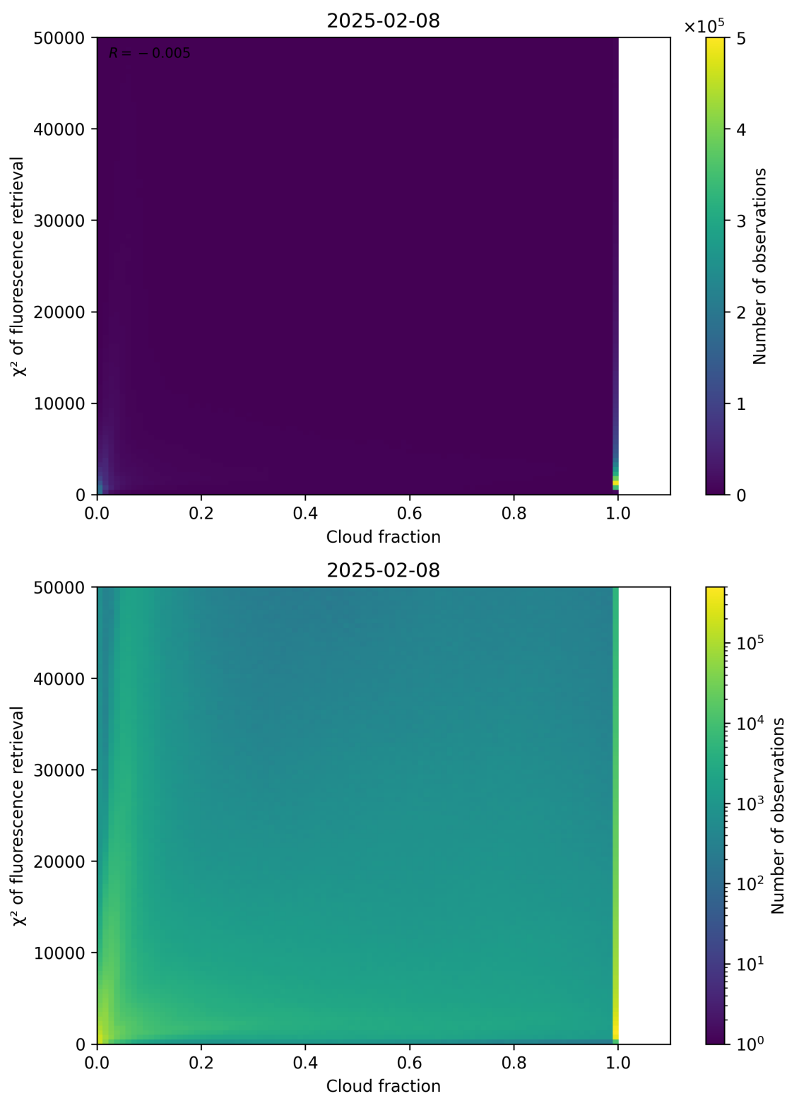
Figure 71: Scatter density plot of “Cloud fraction” against “ \chi^2 of fluorescence retrieval” for 2025-02-08 to 2025-02-09.
