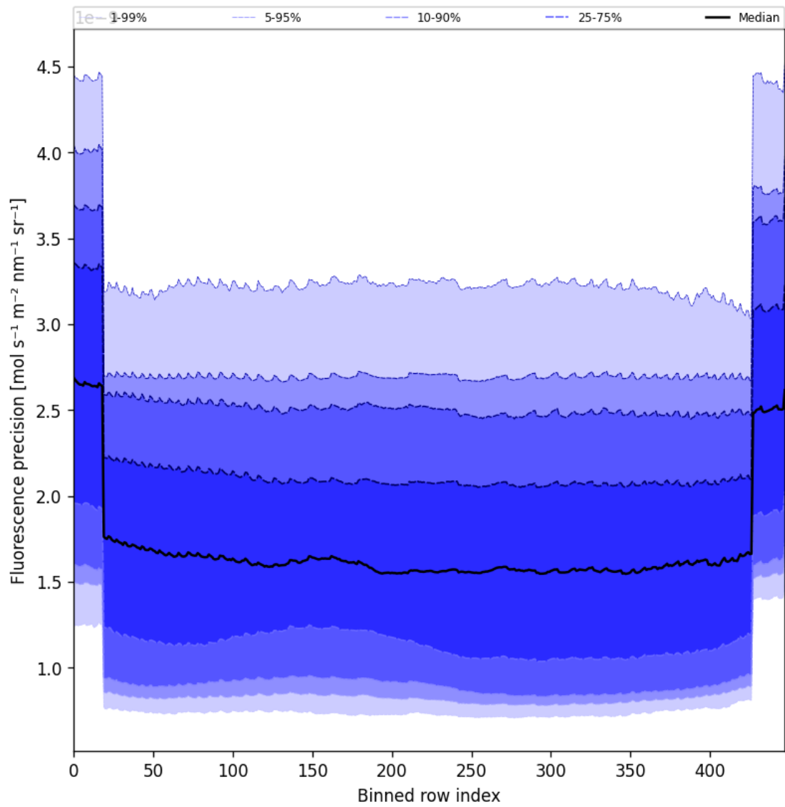
Figure 58: Along track statistics of “Fluorescence precision” for 2025-02-08 to 2025-02-09
