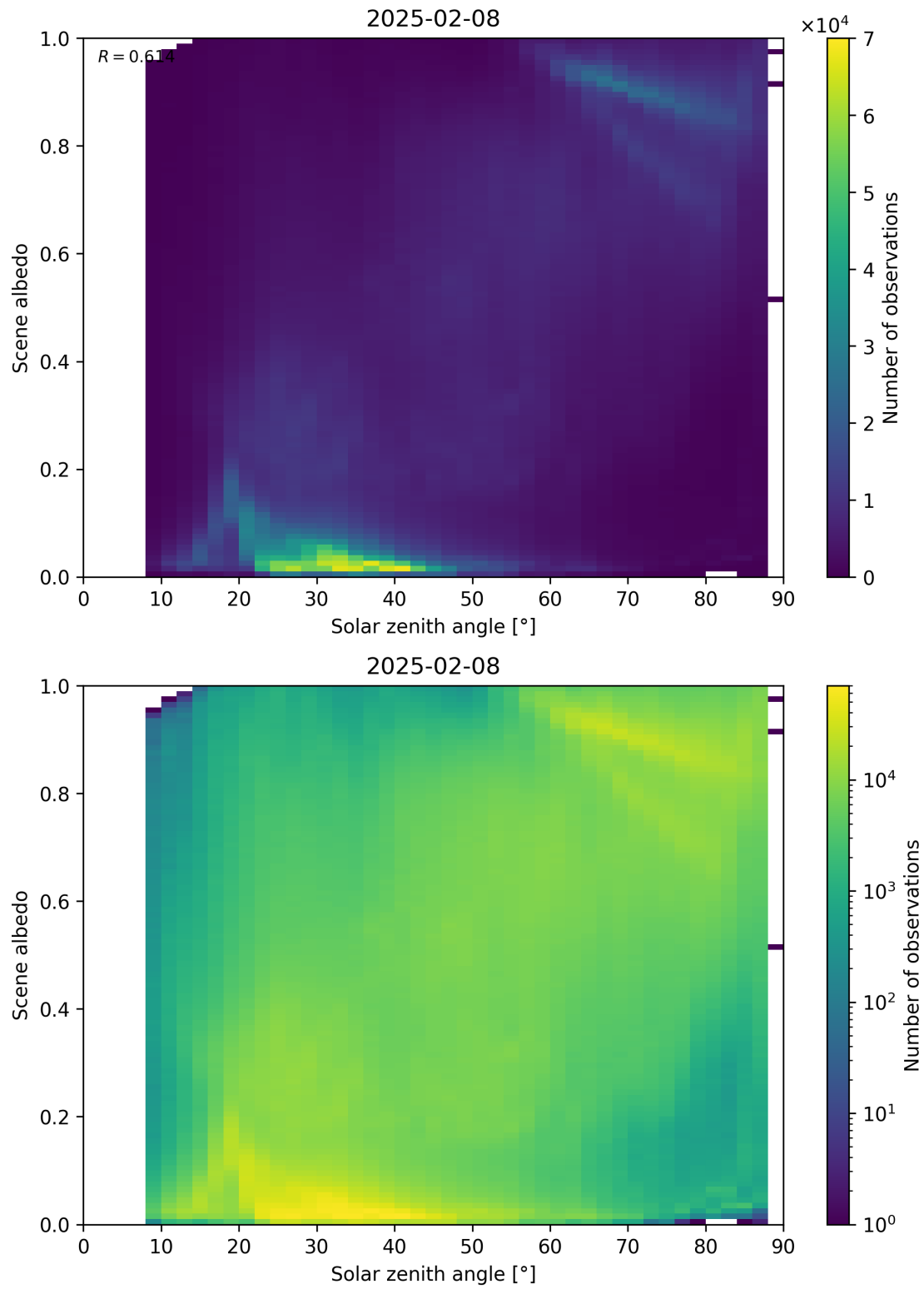
Figure 116: Scatter density plot of “Solar zenith angle” against “Scene albedo” for 2025-02-08 to 2025-02-09.
