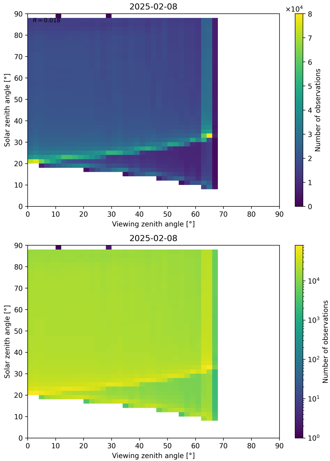
Figure 127: Scatter density plot of “Viewing zenith angle” against “Solar zenith angle” for 2025-02-08 to 2025-02-09.
