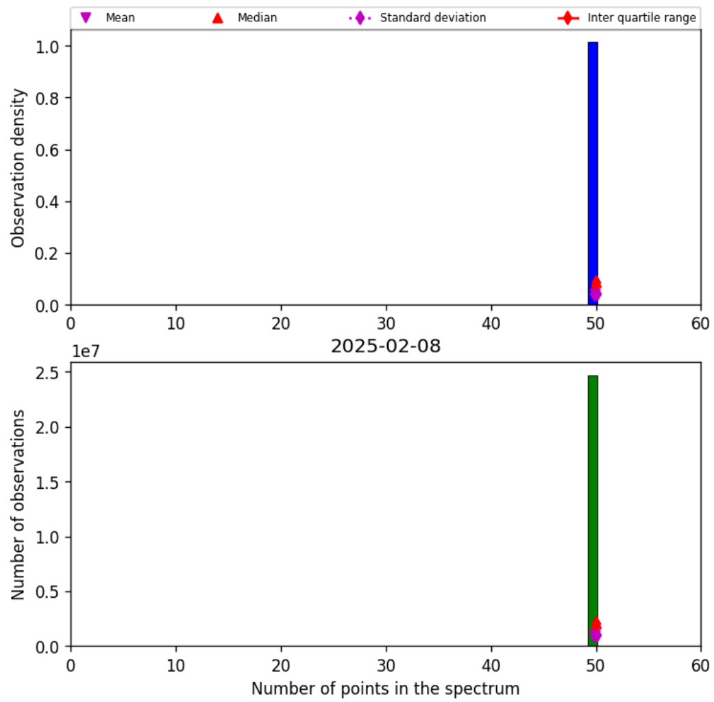
Figure 44: Histogram of “Number of points in the spectrum” for 2025-02-08 to 2025-02-09
