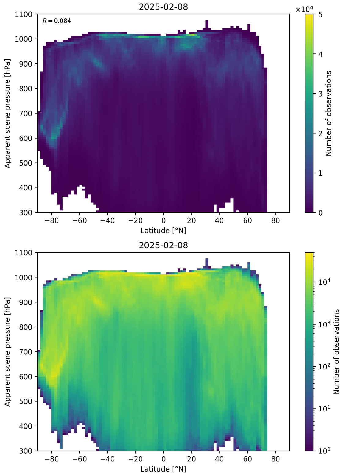
Figure 88: Scatter density plot of “Latitude” against “Apparent scene pressure” for 2025-02-08 to 2025-02-09.
