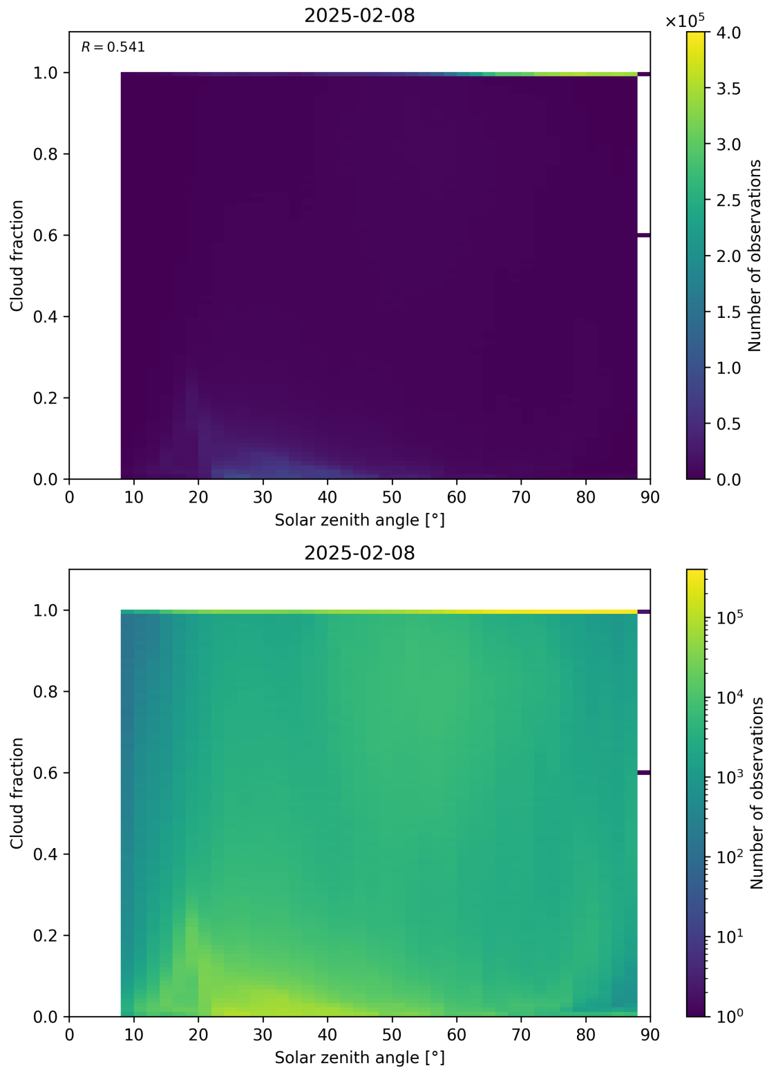
Figure 110: Scatter density plot of “Solar zenith angle” against “Cloud fraction” for 2025-02-08 to 2025-02-09.
