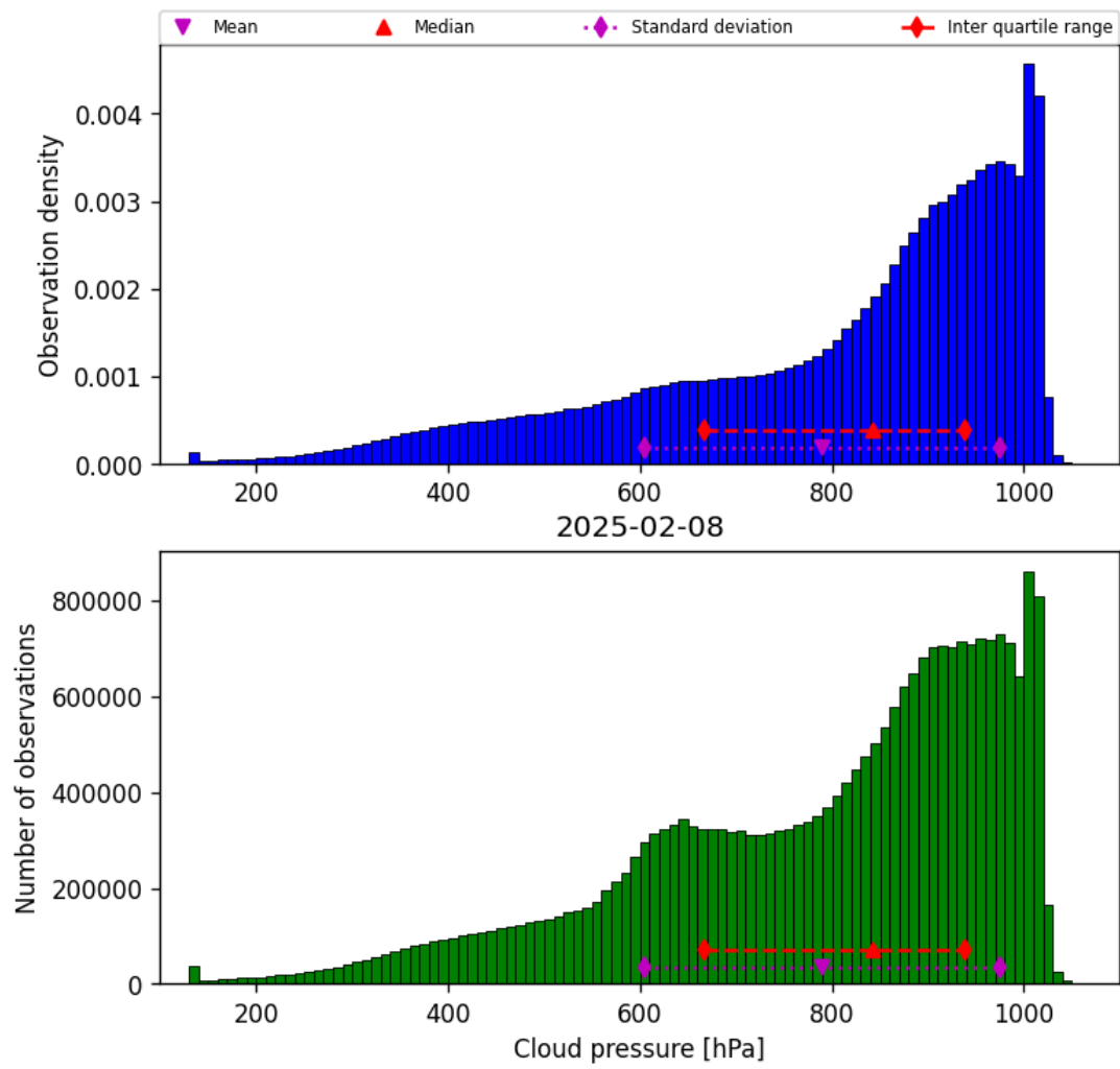
Figure 30: Histogram of “Cloud pressure” for 2025-02-08 to 2025-02-09
