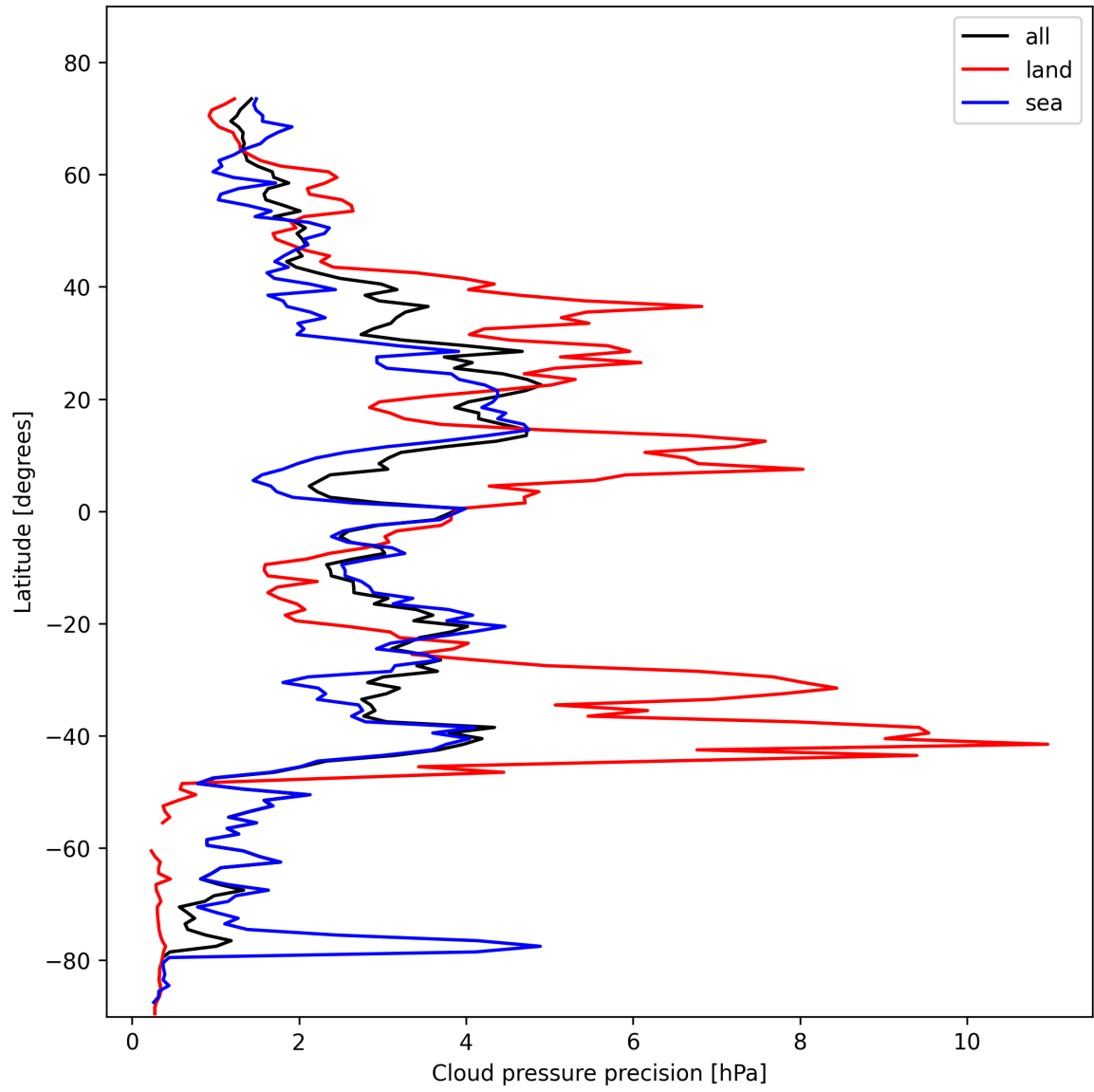
Figure 14: Zonal average of "Cloud pressure precision" for 2025-02-08 to 2025-02-09.
