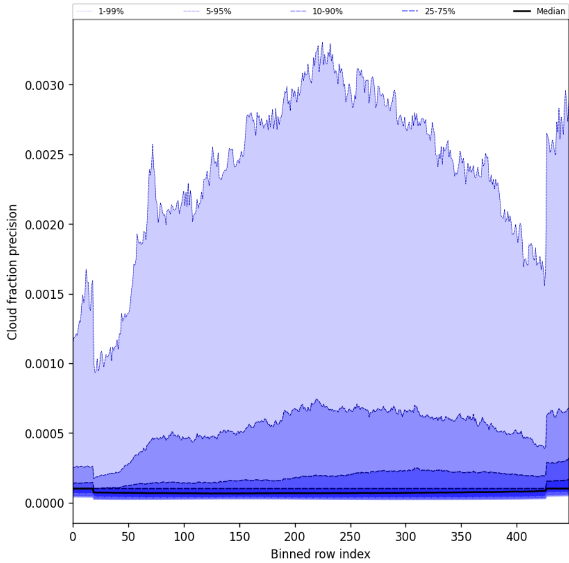
Figure 50: Along track statistics of “Cloud fraction precision” for 2025-02-08 to 2025-02-09
