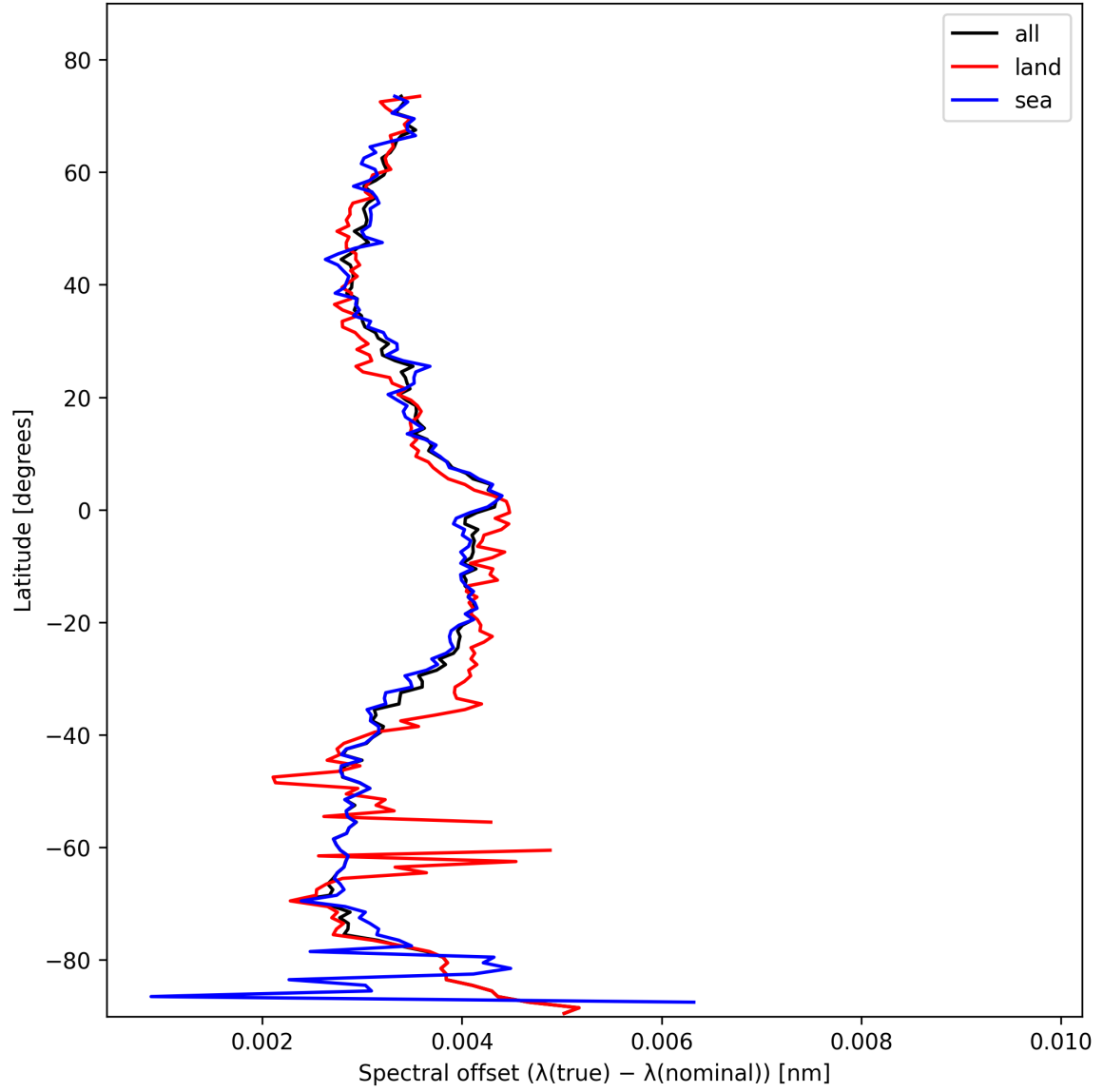
Figure 28: Zonal average of “Spectral offset ( \lambda_{\text{true}} - \lambda_{\text{nominal}} )” for 2025-02-08 to 2025-02-09.
