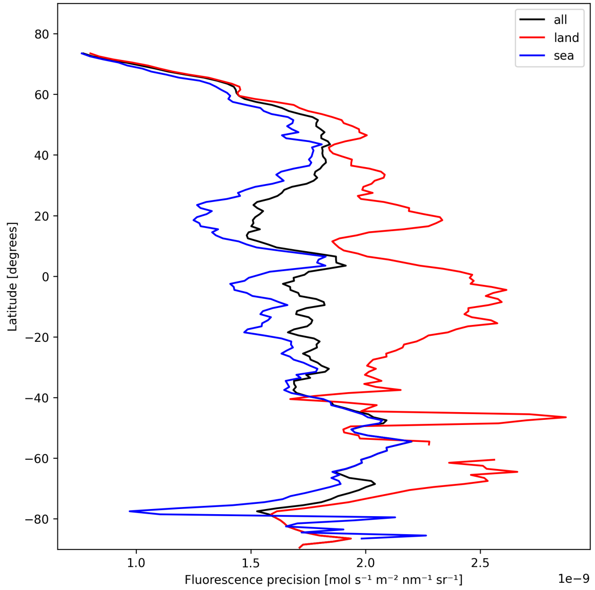
Figure 24: Zonal average of “Fluorescence precision” for 2025-02-08 to 2025-02-10.
