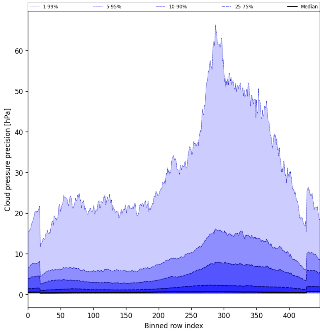
Figure 48: Along track statistics of “Cloud pressure precision” for 2025-02-08 to 2025-02-10
