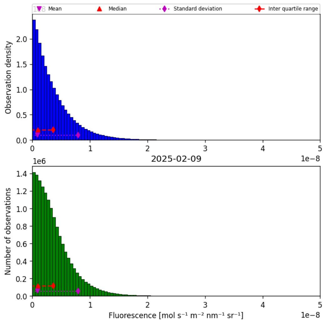
Figure 40: Histogram of “Fluorescence” for 2025-02-08 to 2025-02-10
