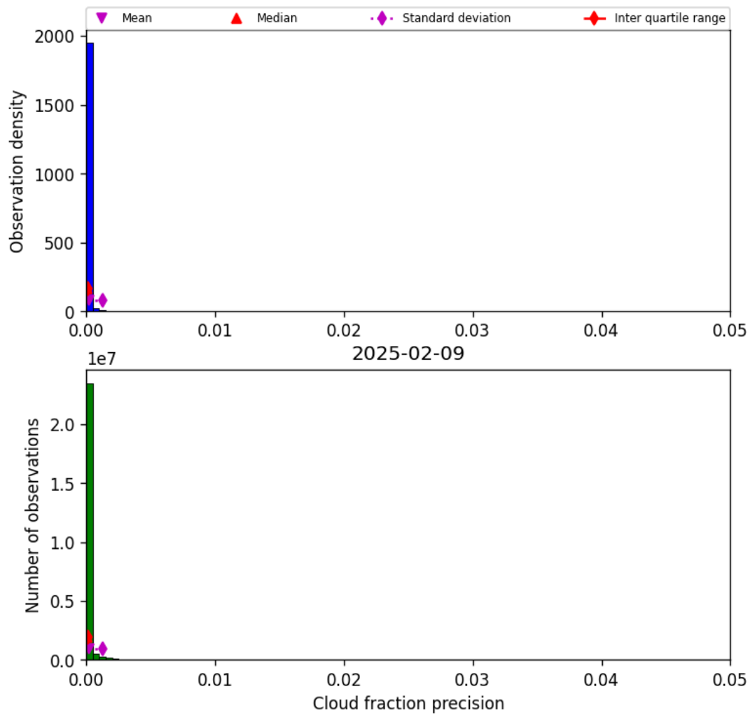
Figure 33: Histogram of “Cloud fraction precision” for 2025-02-08 to 2025-02-10
