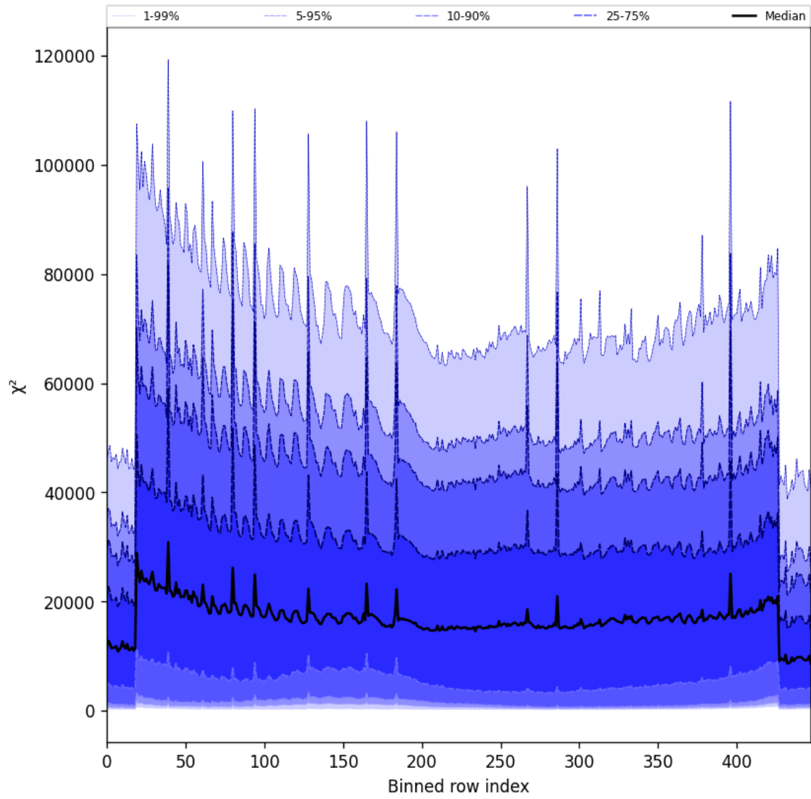
Figure 55: Along track statistics of “ \chi^2 ” for 2025-02-08 to 2025-02-10
