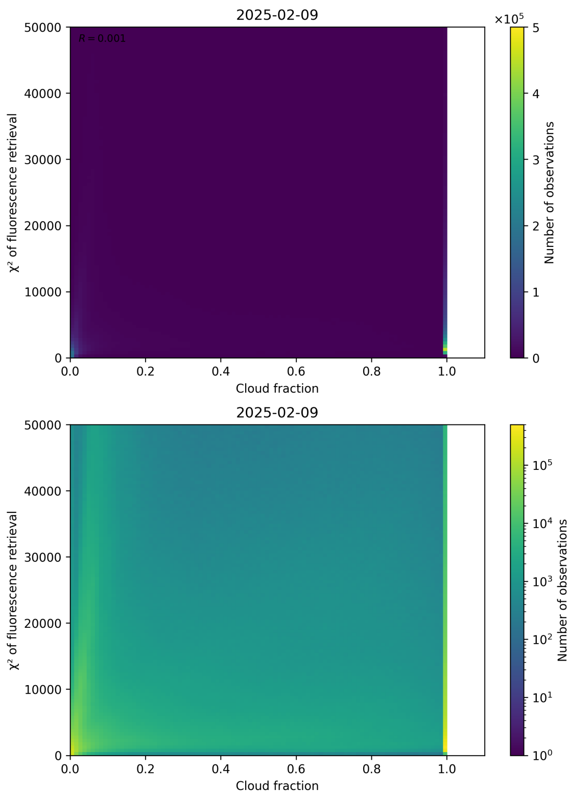
Figure 71: Scatter density plot of “Cloud fraction” against “ \chi^2 of fluorescence retrieval” for 2025-02-08 to 2025-02-10.
