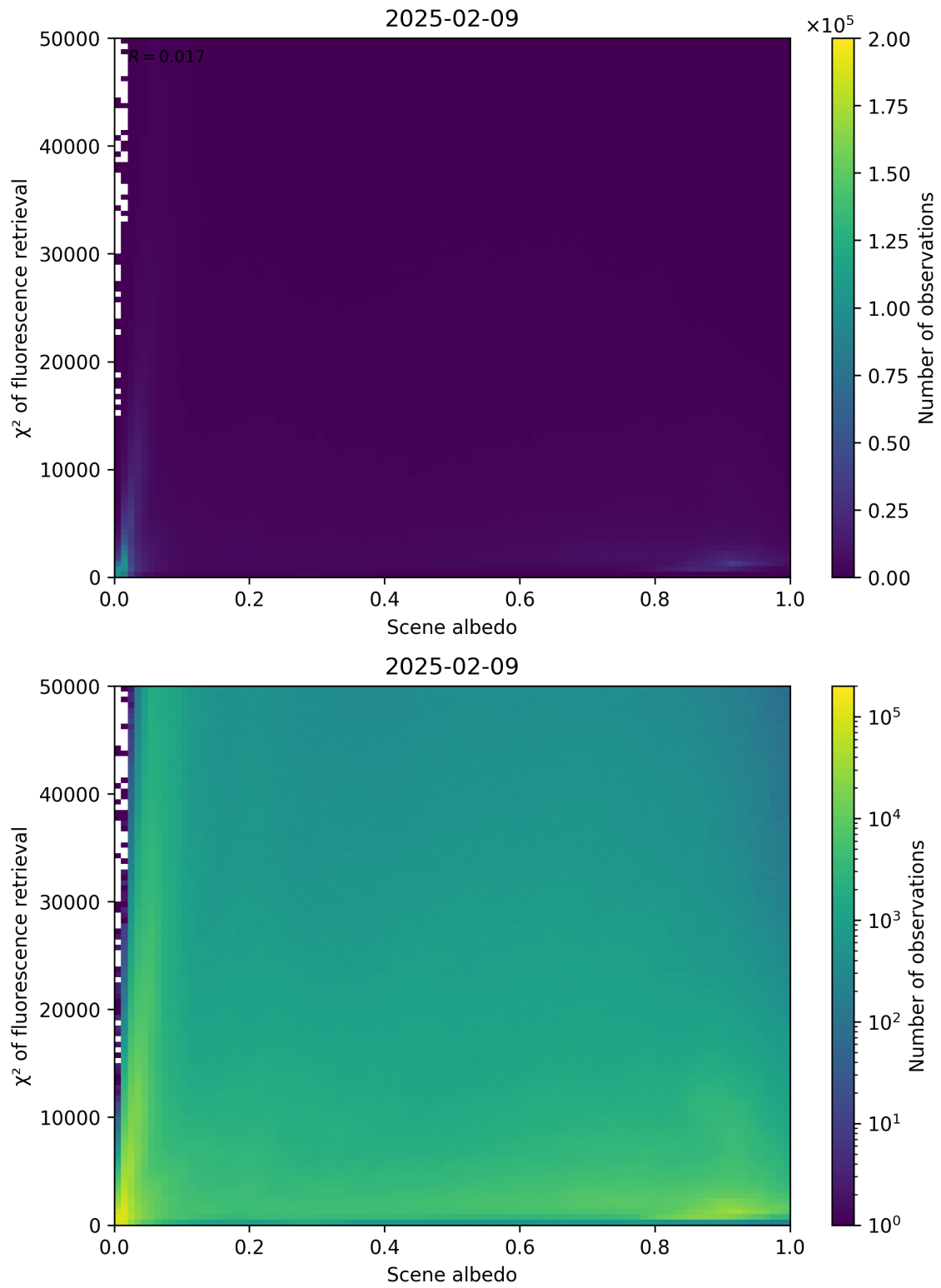
Figure 103: Scatter density plot of “Scene albedo” against “ \chi^2 of fluorescence retrieval” for 2025-02-08 to 2025-02-10.
