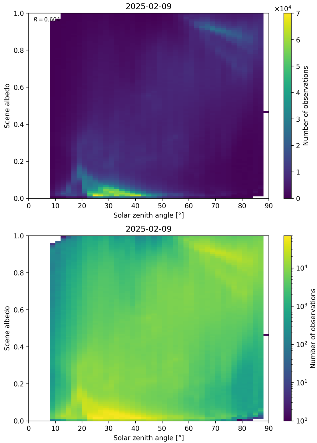
Figure 116: Scatter density plot of “Solar zenith angle” against “Scene albedo” for 2025-02-08 to 2025-02-10.
