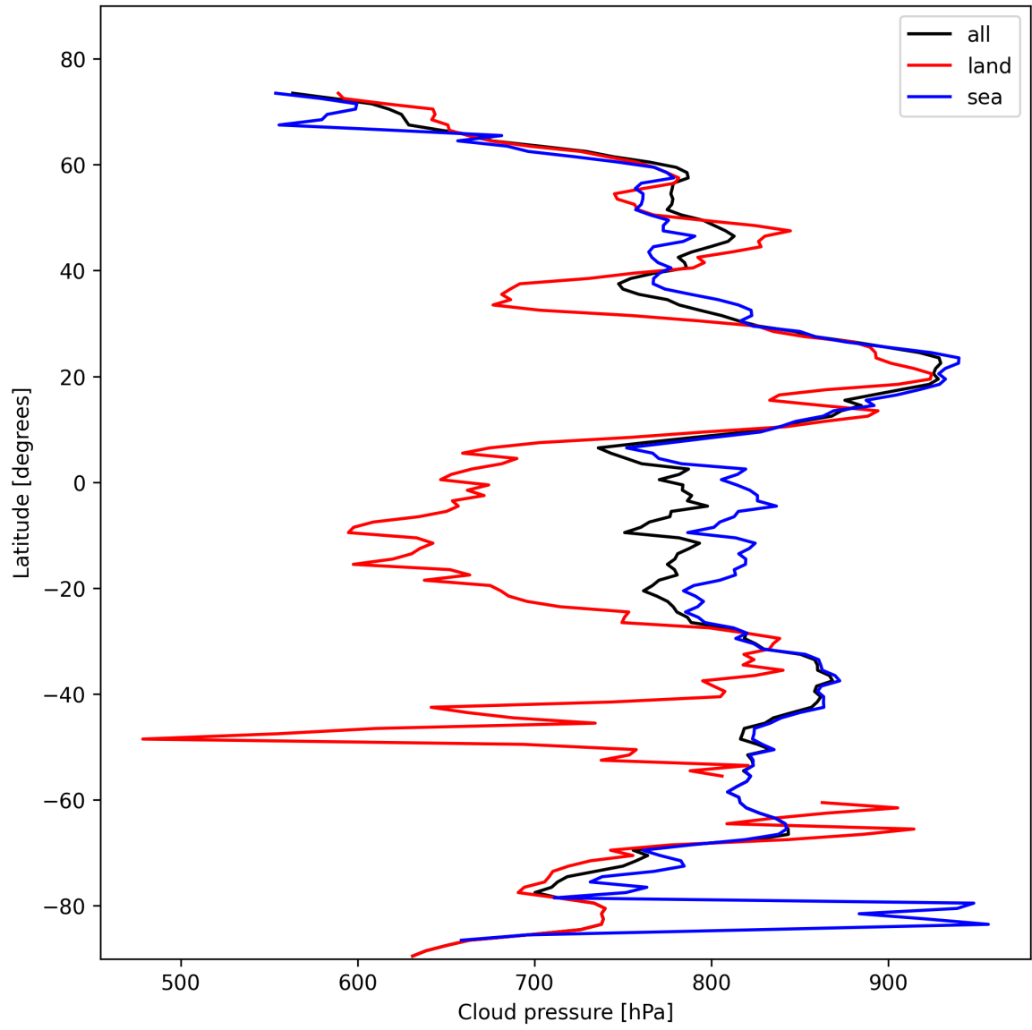
Figure 13: Zonal average of “Cloud pressure” for 2025-02-08 to 2025-02-10.
