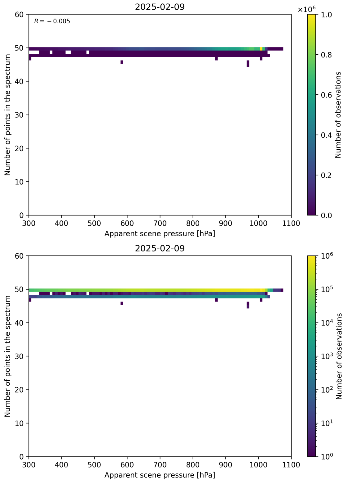
Figure 66: Scatter density plot of “Apparent scene pressure” against “Number of points in the spectrum” for 2025-02-08 to 2025-02-10.
