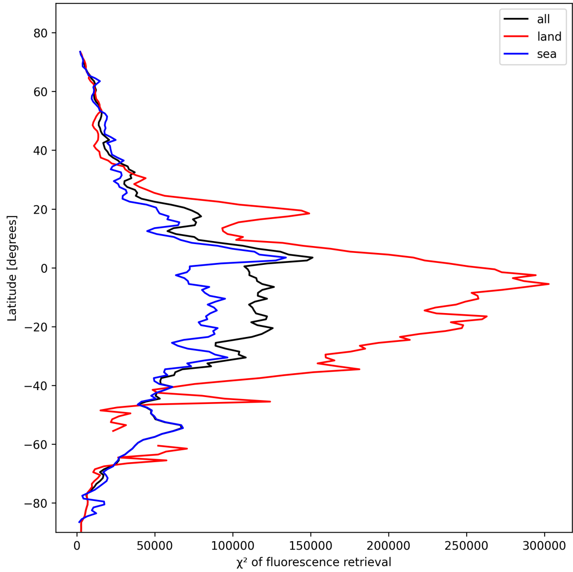
Figure 25: Zonal average of “ \chi^2 of fluorescence retrieval” for 2025-02-08 to 2025-02-10.
