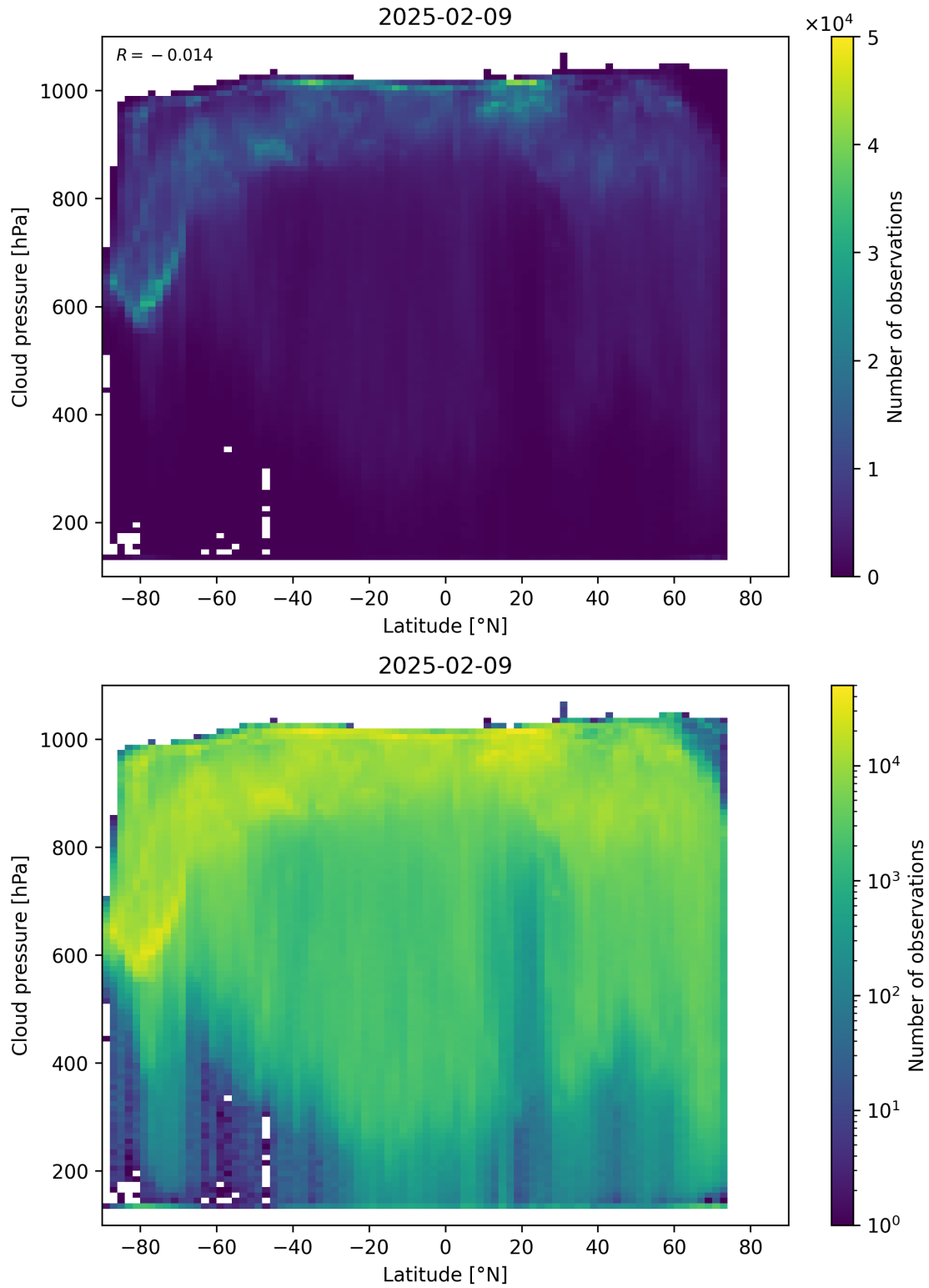
Figure 91: Scatter density plot of “Latitude” against “Cloud pressure” for 2025-02-08 to 2025-02-10.
