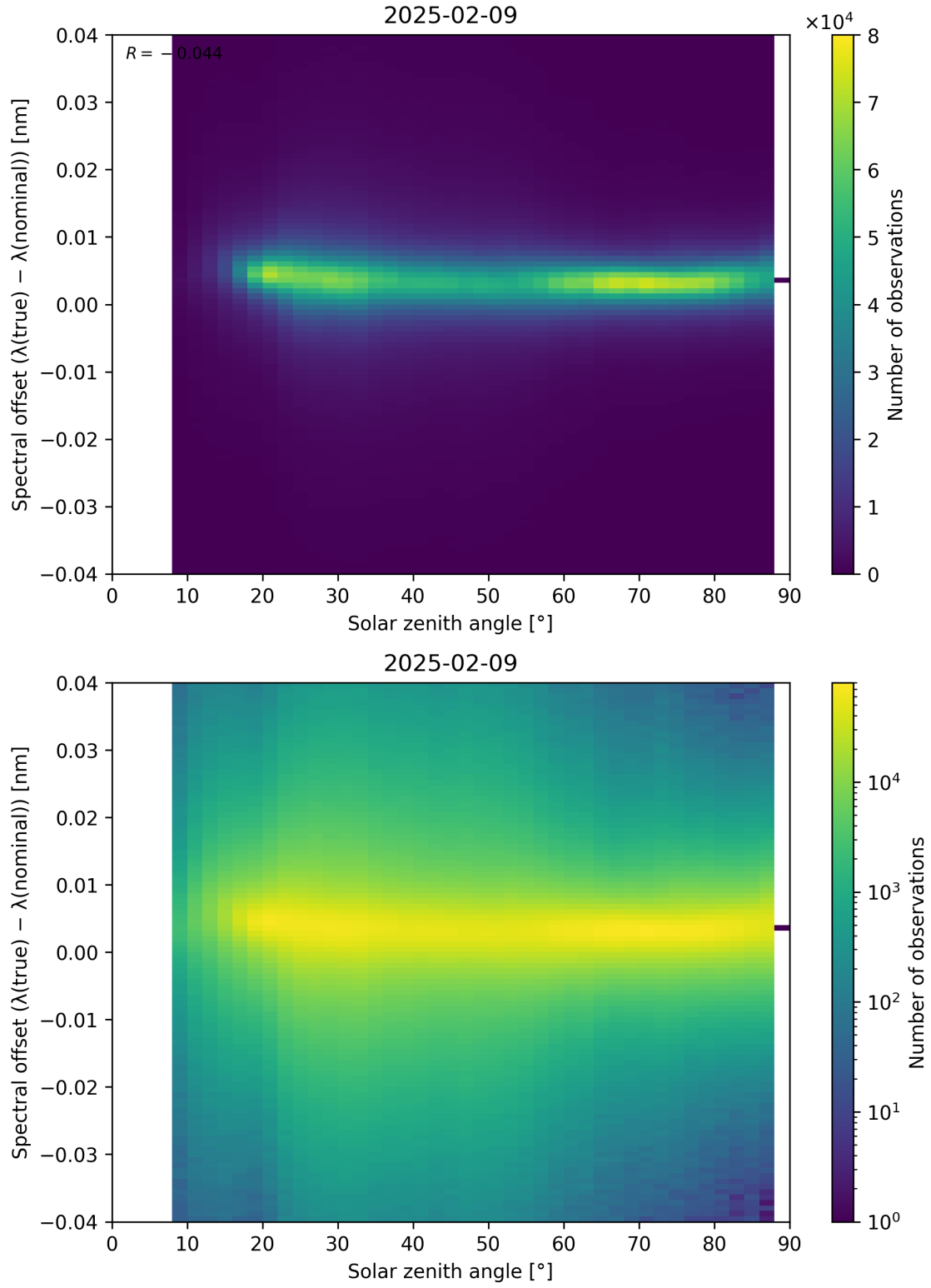
Figure 117: Scatter density plot of “Solar zenith angle” against “Spectral offset ( \lambda_{\text{true}} - \lambda_{\text{nominal}} )” for 2025-02-08 to 2025-02-10.
