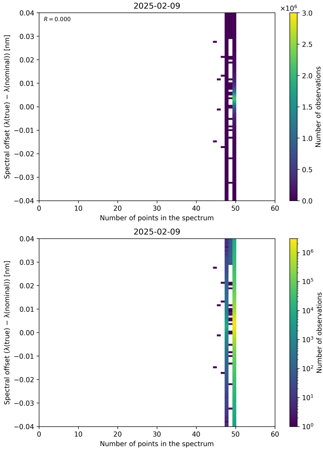
Figure 101: Scatter density plot of “Number of points in the spectrum” against “Spectral offset ( \lambda_{\text{true}} - \lambda_{\text{nominal}} )” for 2025-02-08 to 2025-02-10.
