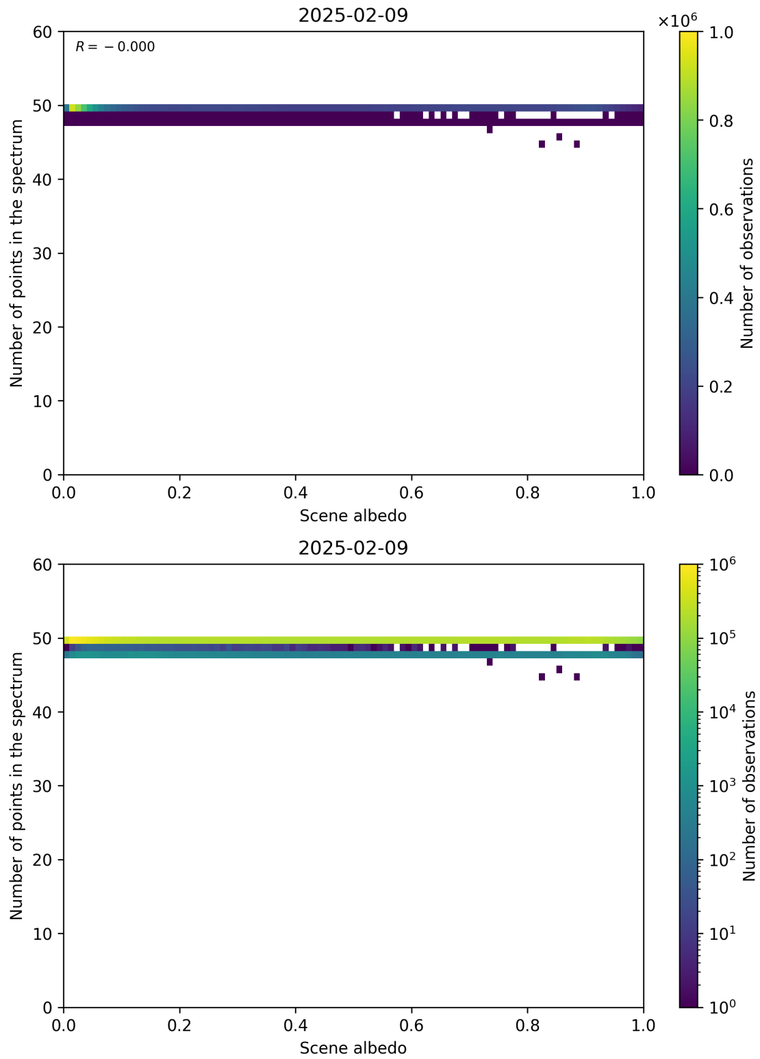
Figure 106: Scatter density plot of “Scene albedo” against “Number of points in the spectrum” for 2025-02-08 to 2025-02-10.
