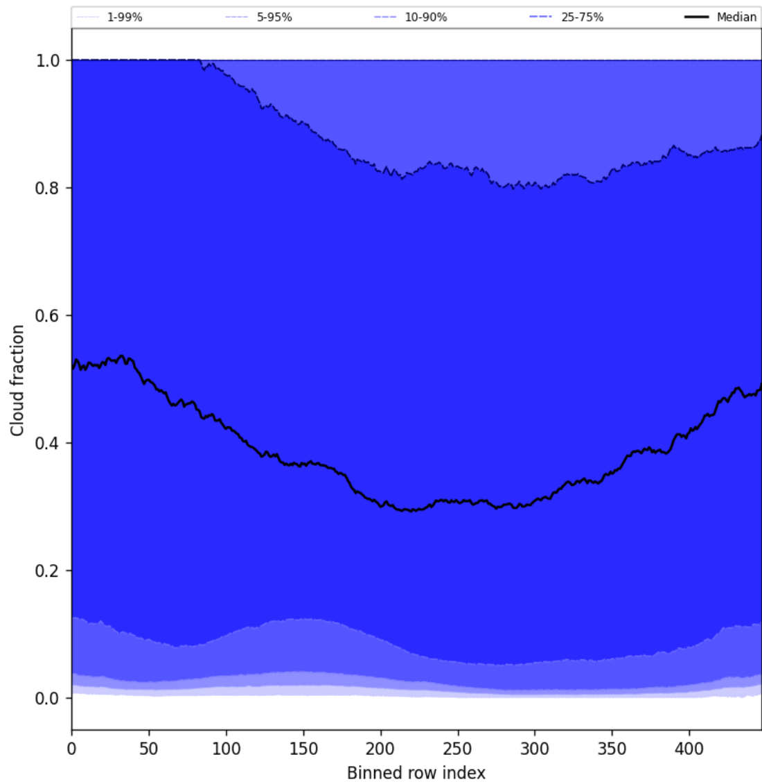
Figure 49: Along track statistics of “Cloud fraction” for 2025-02-08 to 2025-02-10
