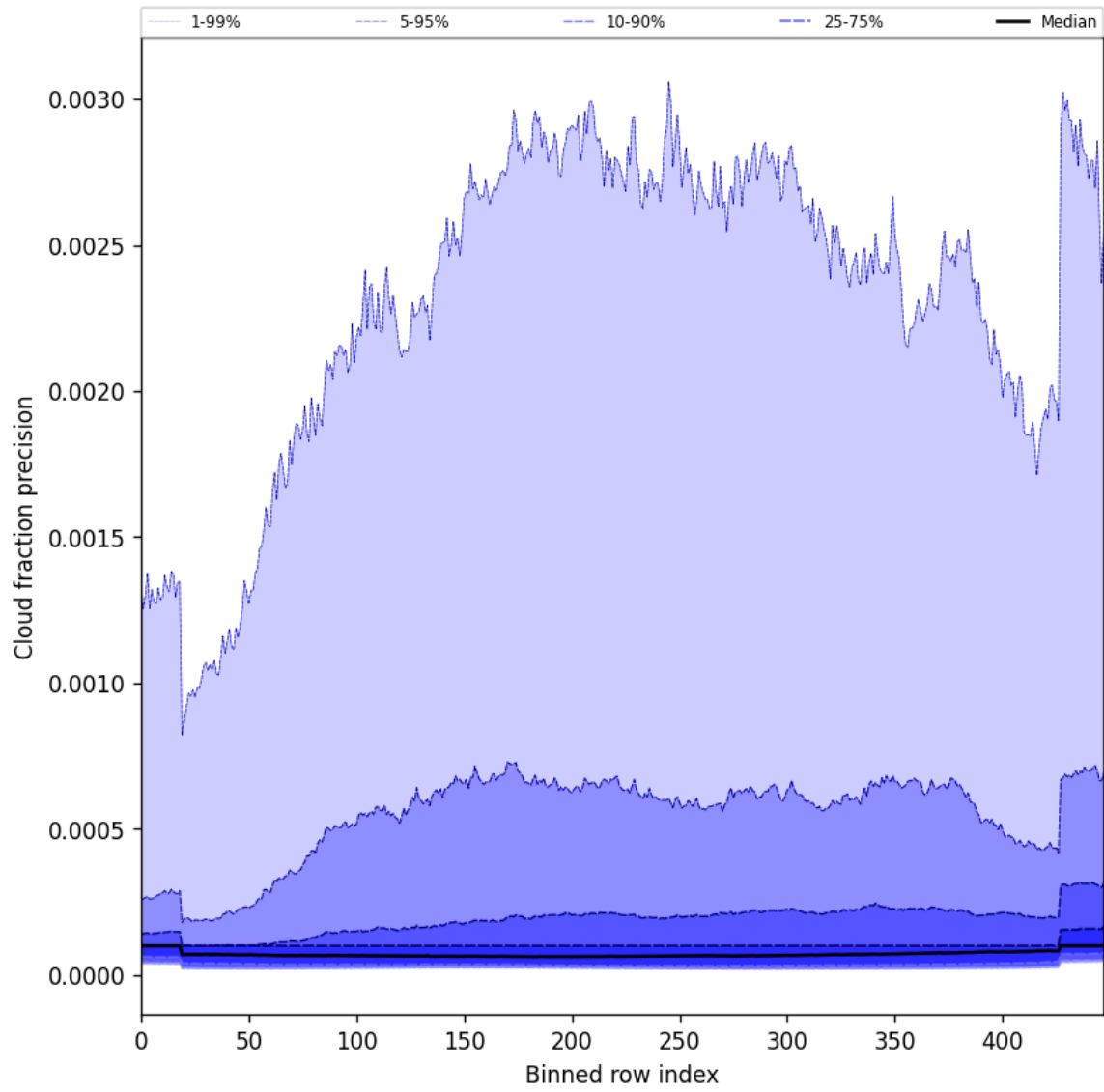
Figure 50: Along track statistics of “Cloud fraction precision” for 2025-02-08 to 2025-02-10
