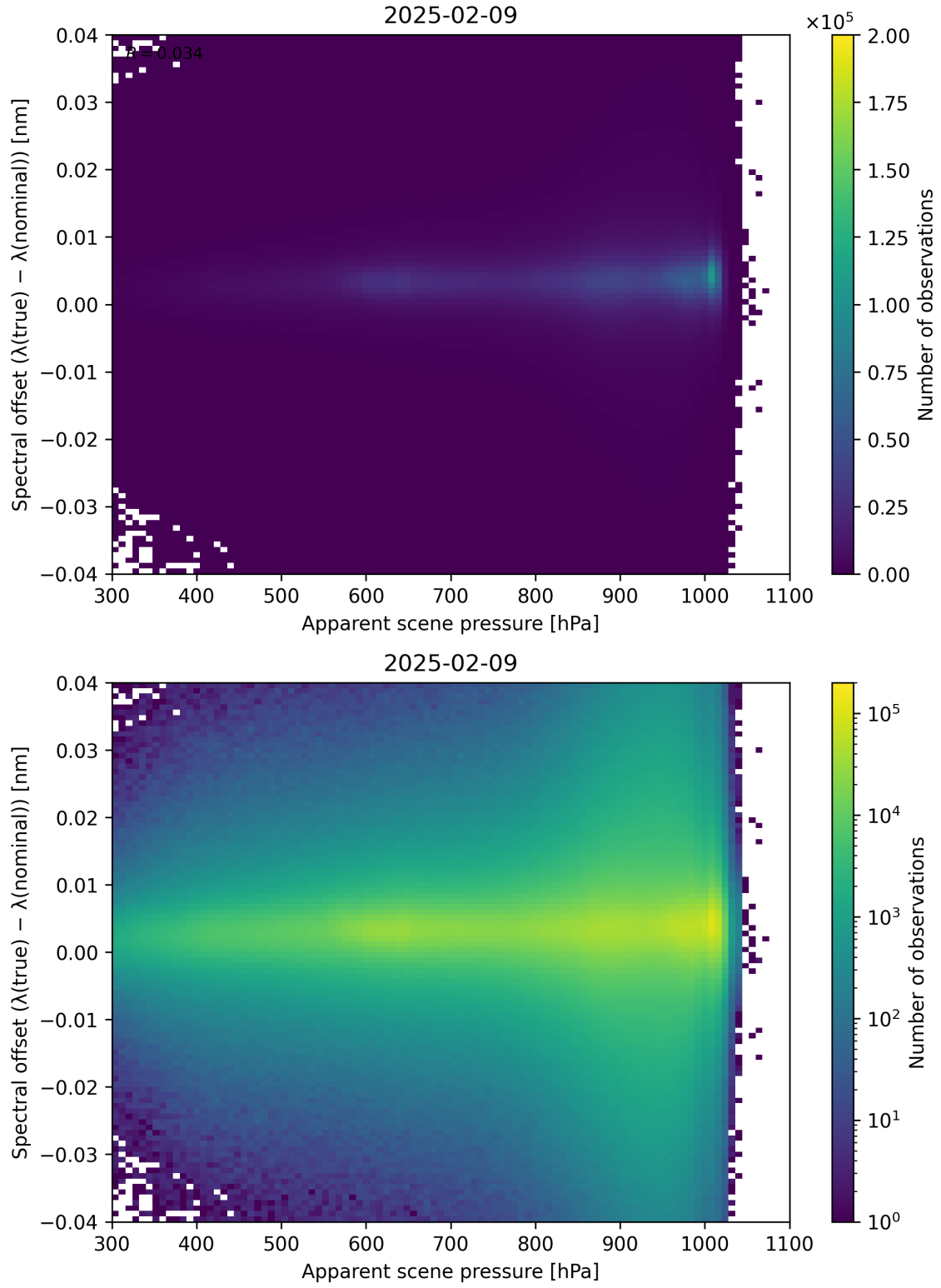
Figure 67: Scatter density plot of “Apparent scene pressure” against “Spectral offset ( \lambda_{\text{true}} - \lambda_{\text{nominal}} )” for 2025-02-08 to 2025-02-10.
