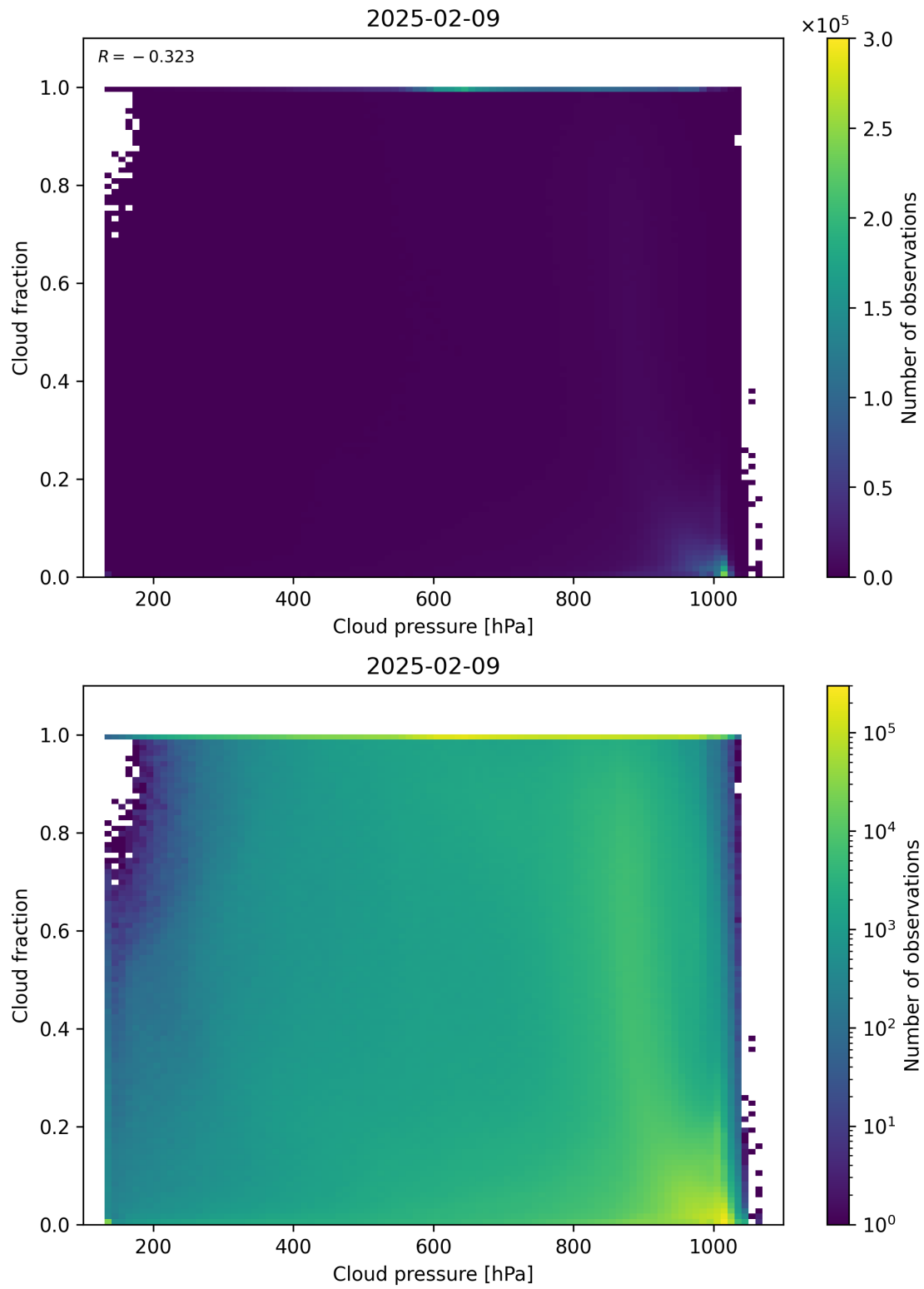
Figure 79: Scatter density plot of “Cloud pressure” against “Cloud fraction” for 2025-02-08 to 2025-02-10.
