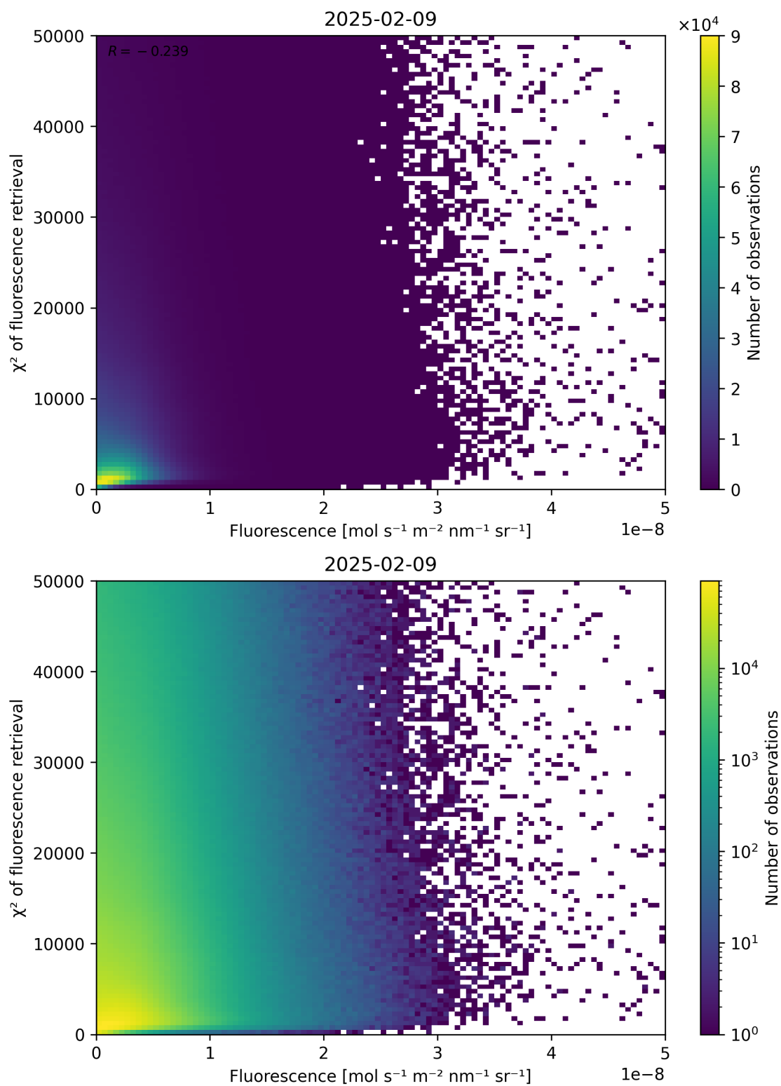
Figure 85: Scatter density plot of “Fluorescence” against “ \chi^2 of fluorescence retrieval” for 2025-02-08 to 2025-02-10.
