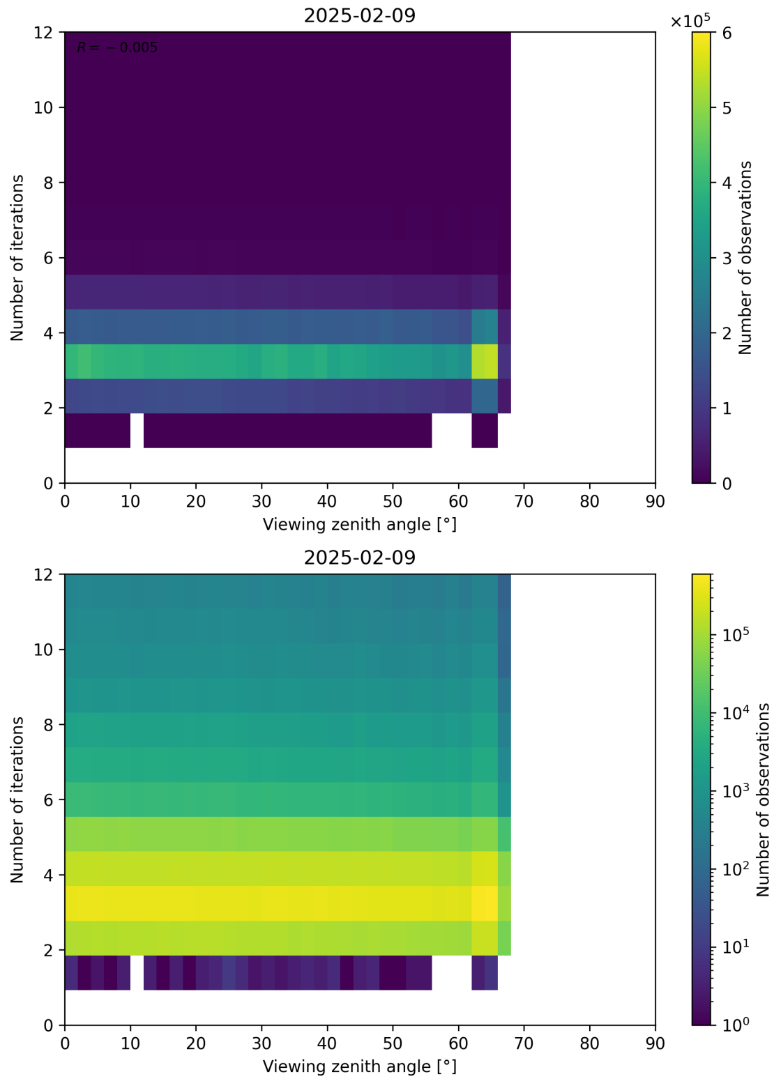
Figure 124: Scatter density plot of “Viewing zenith angle” against “Number of iterations” for 2025-02-08 to 2025-02-10.
