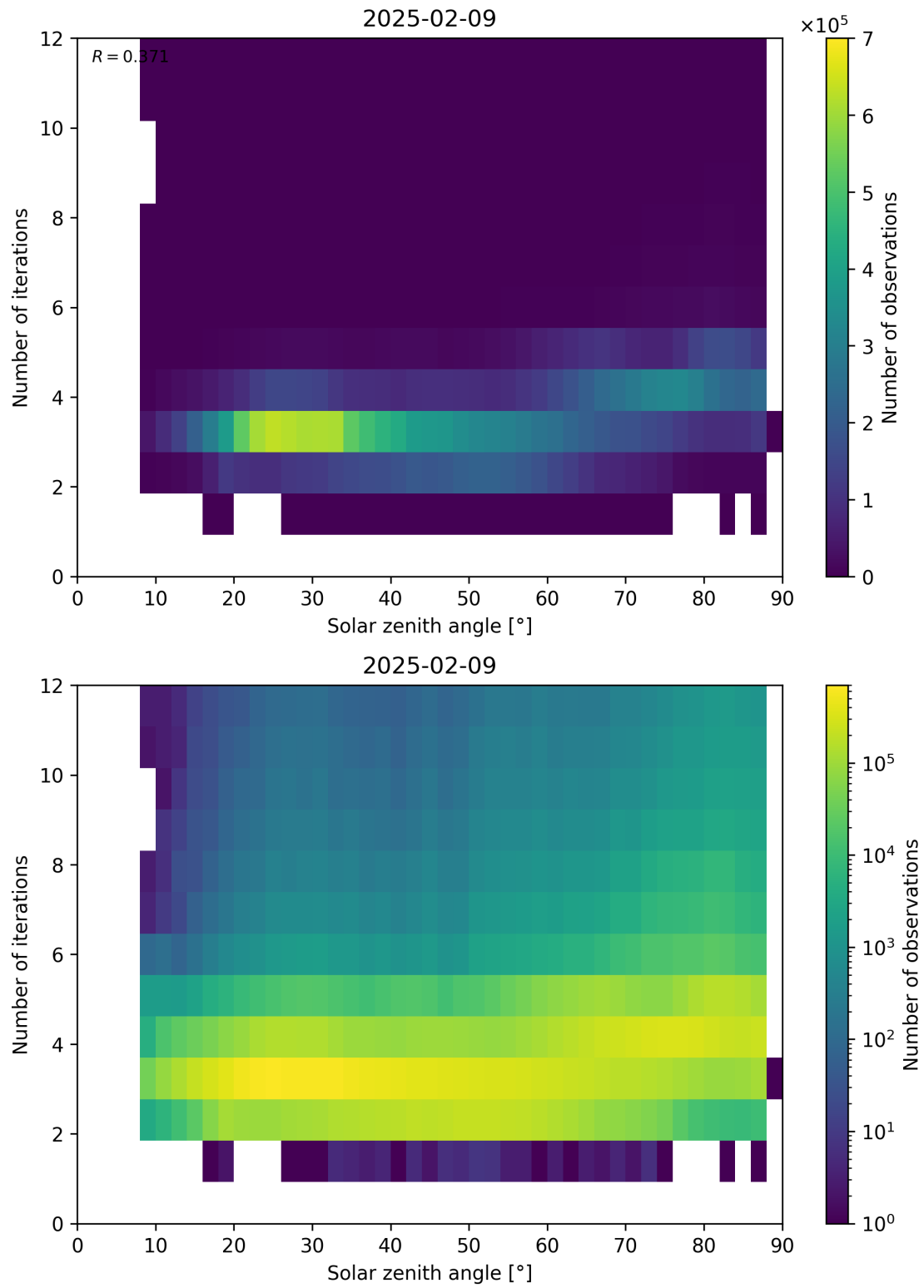
Figure 114: Scatter density plot of “Solar zenith angle” against “Number of iterations” for 2025-02-08 to 2025-02-10.
