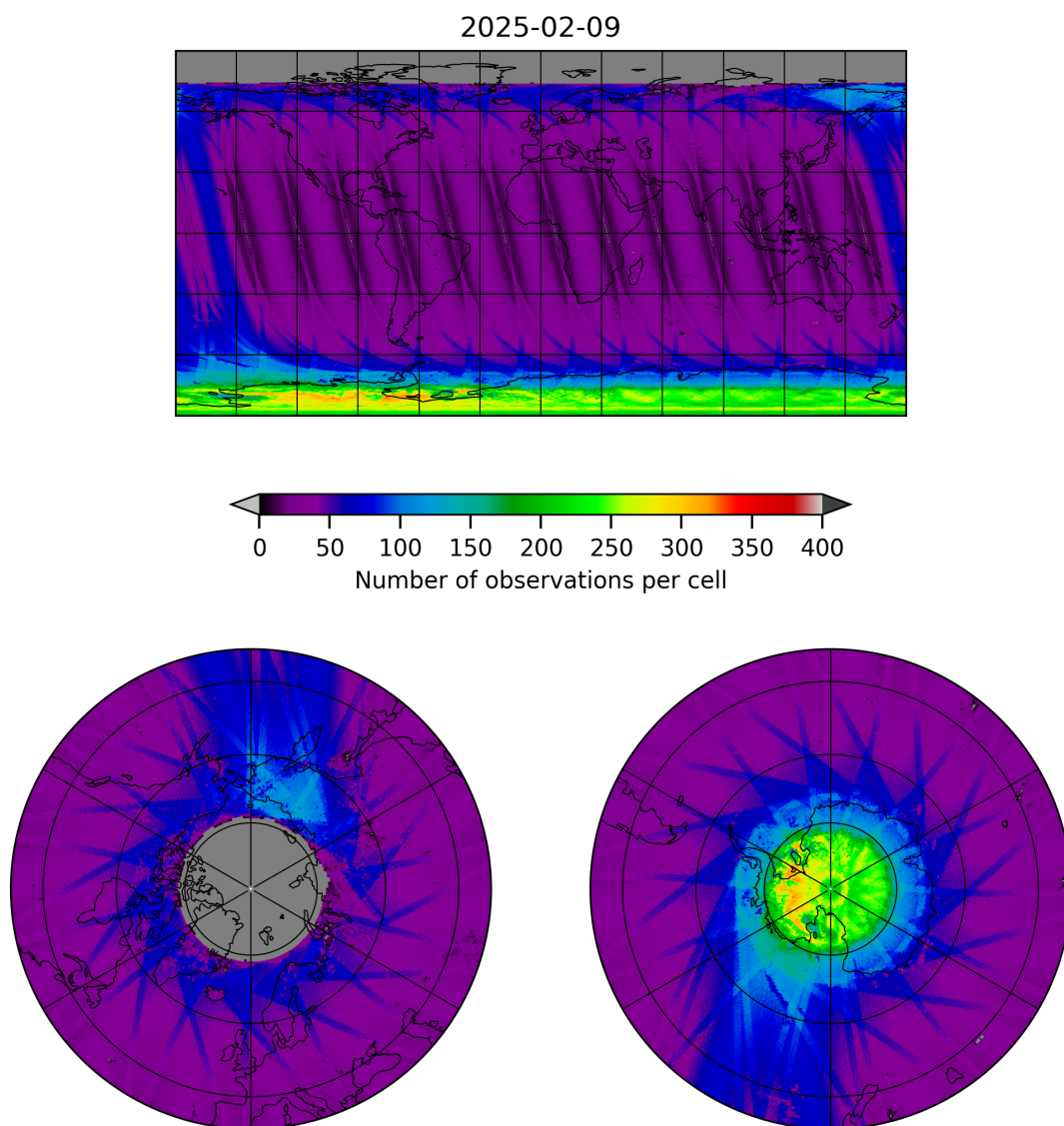
Figure 11: Map of the number of observations for 2025-02-08 to 2025-02-10
