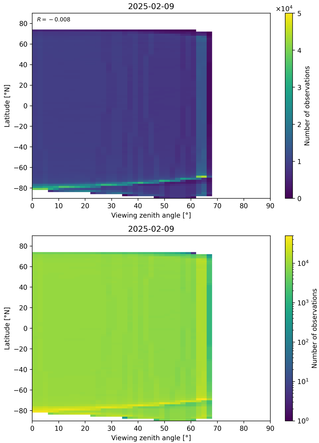
Figure 123: Scatter density plot of “Viewing zenith angle” against “Latitude” for 2025-02-08 to 2025-02-10.
