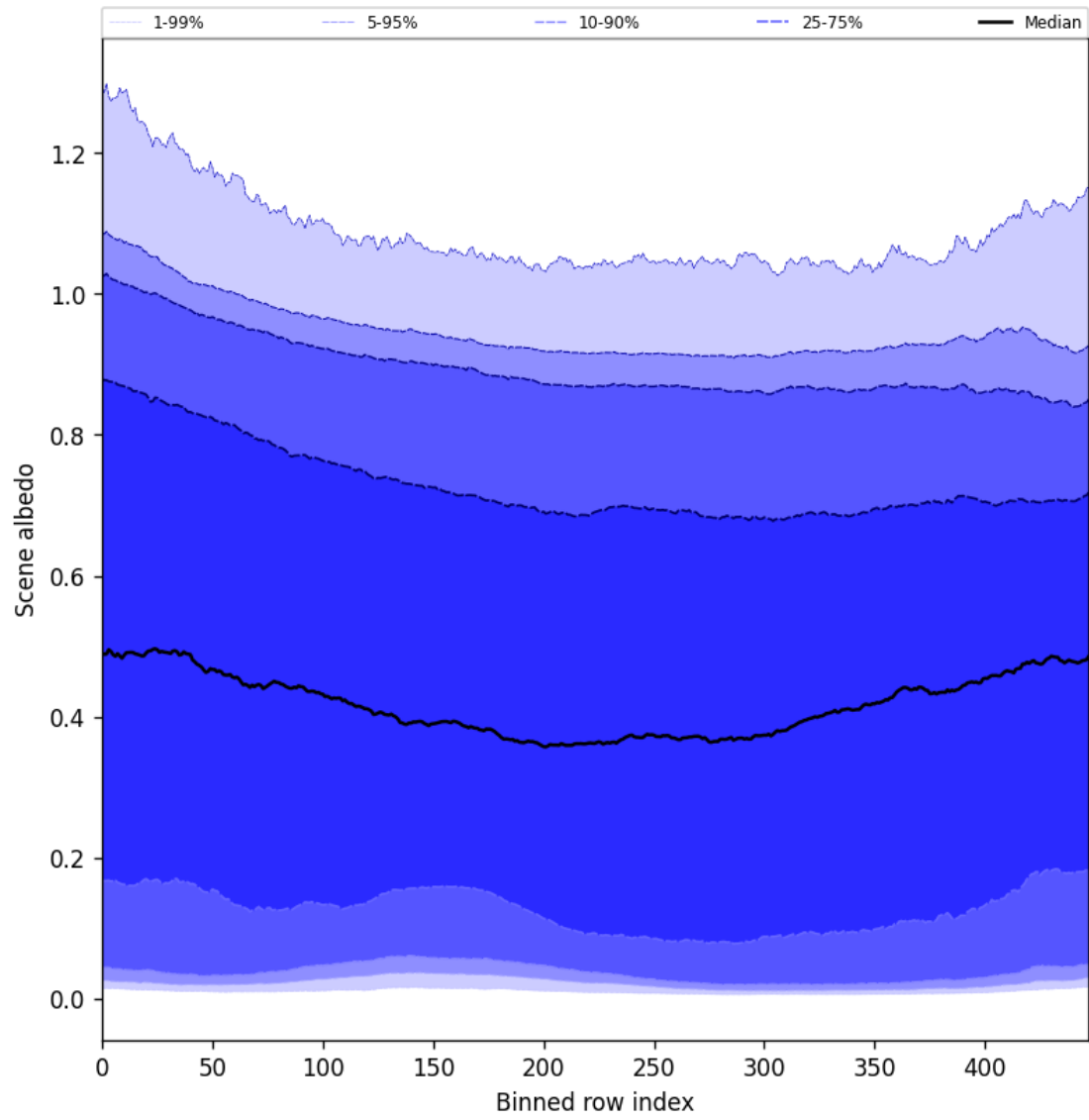
Figure 51: Along track statistics of “Scene albedo” for 2025-02-08 to 2025-02-10
