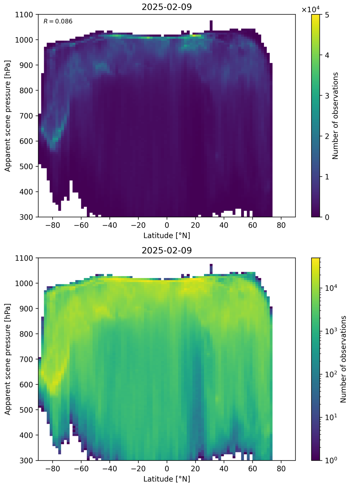
Figure 88: Scatter density plot of “Latitude” against “Apparent scene pressure” for 2025-02-08 to 2025-02-10.
