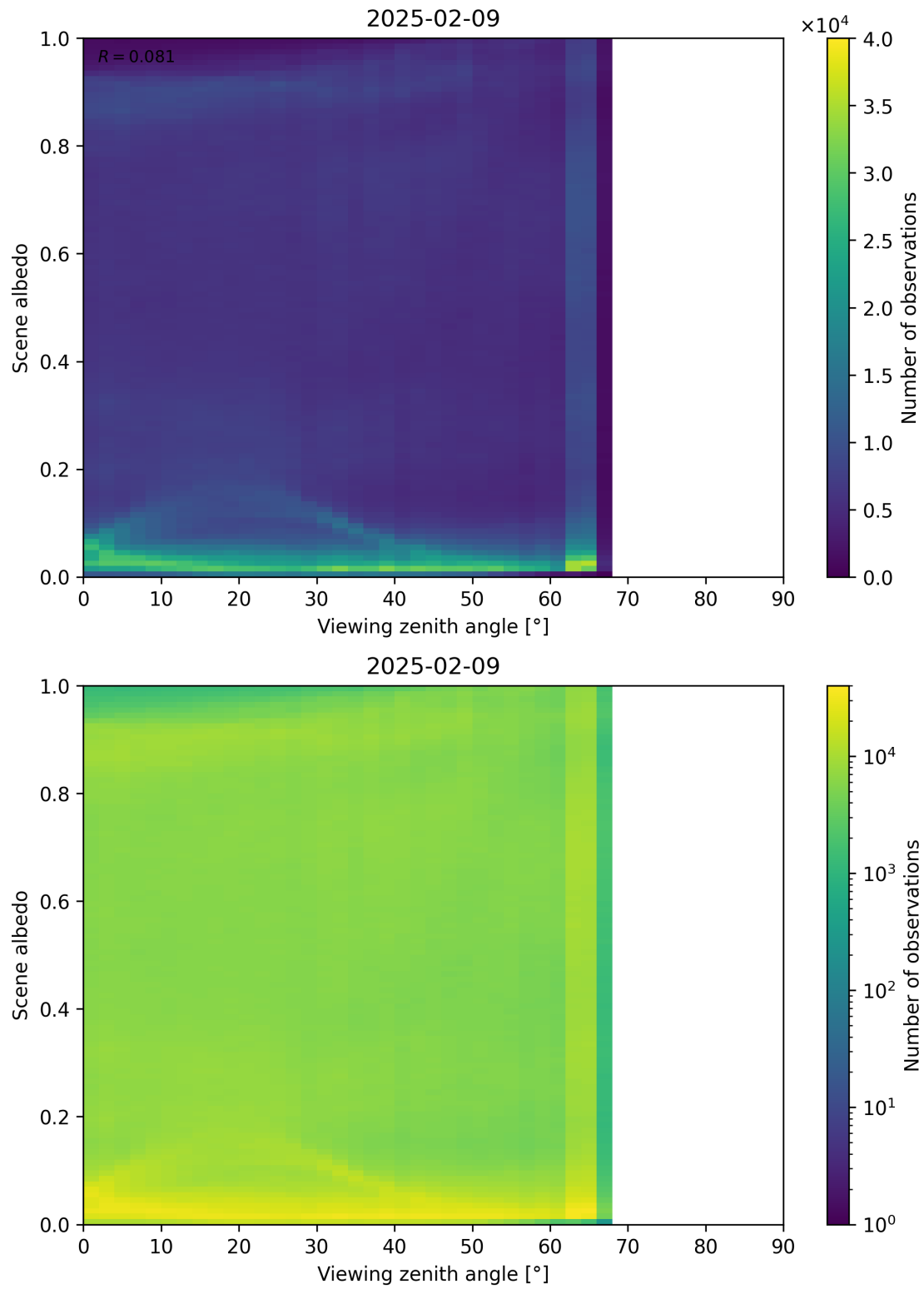
Figure 126: Scatter density plot of “Viewing zenith angle” against “Scene albedo” for 2025-02-08 to 2025-02-10.
