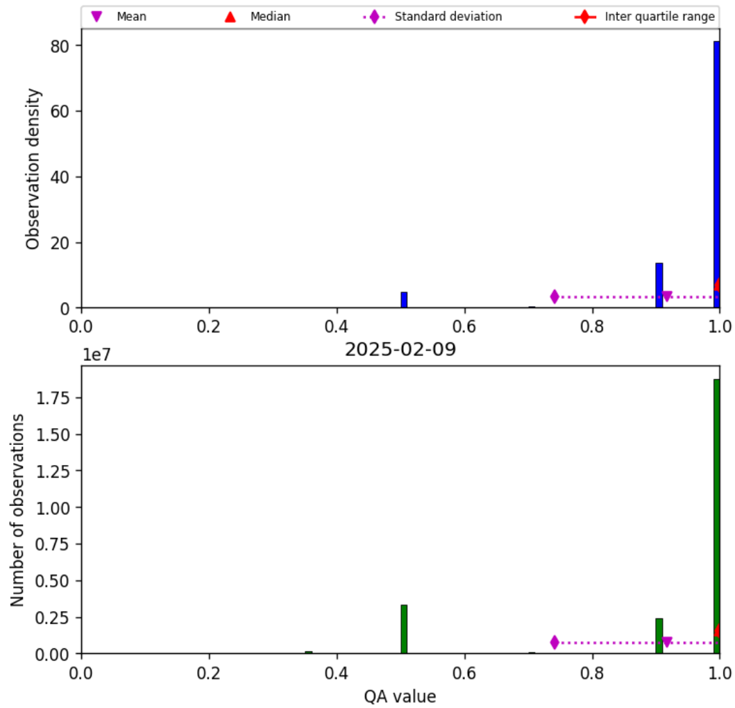
Figure 29: Histogram of “QA value” for 2025-02-08 to 2025-02-10
