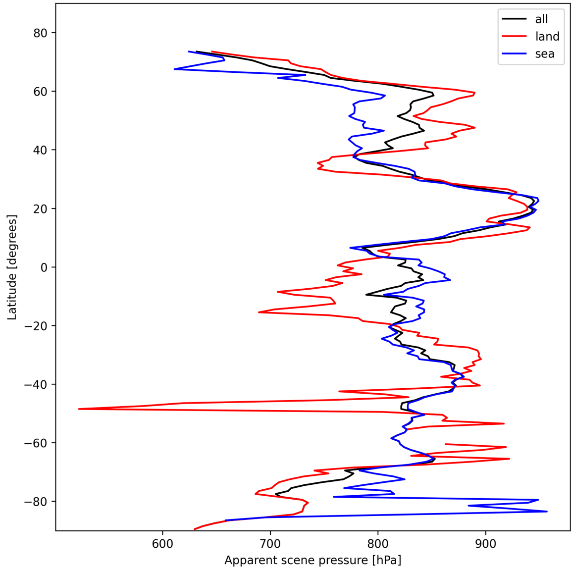
Figure 19: Zonal average of “Apparent scene pressure” for 2025-02-08 to 2025-02-10.
