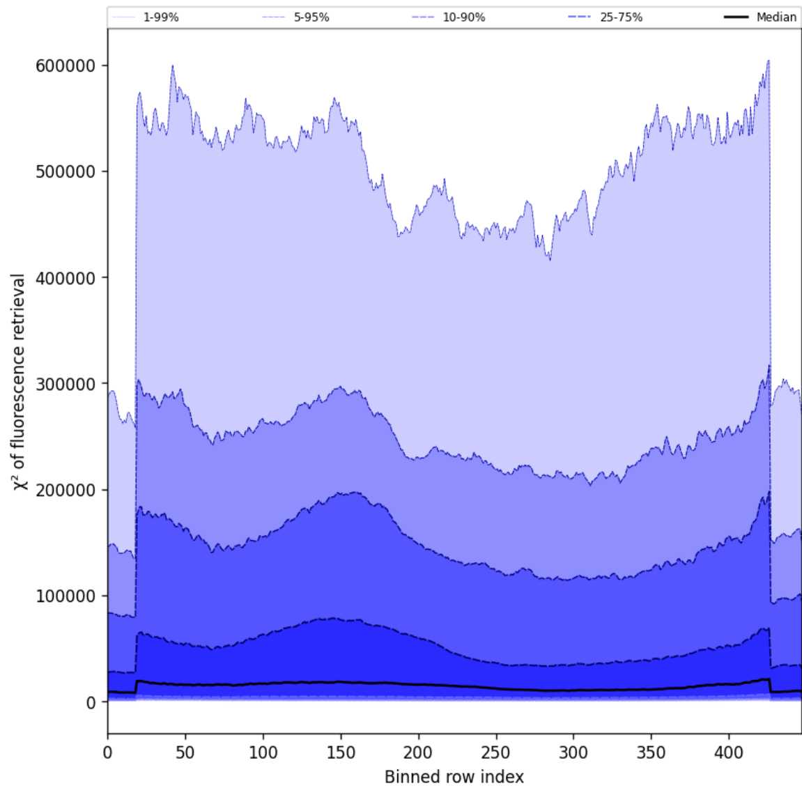
Figure 59: Along track statistics of “ \chi^2 of fluorescence retrieval” for 2025-02-08 to 2025-02-10
