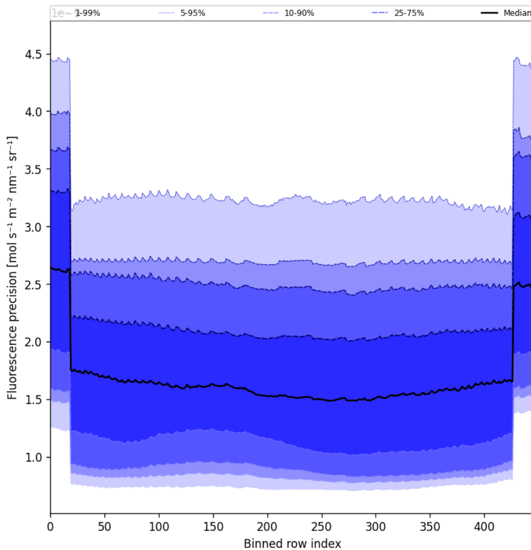
Figure 58: Along track statistics of “Fluorescence precision” for 2025-02-08 to 2025-02-10
