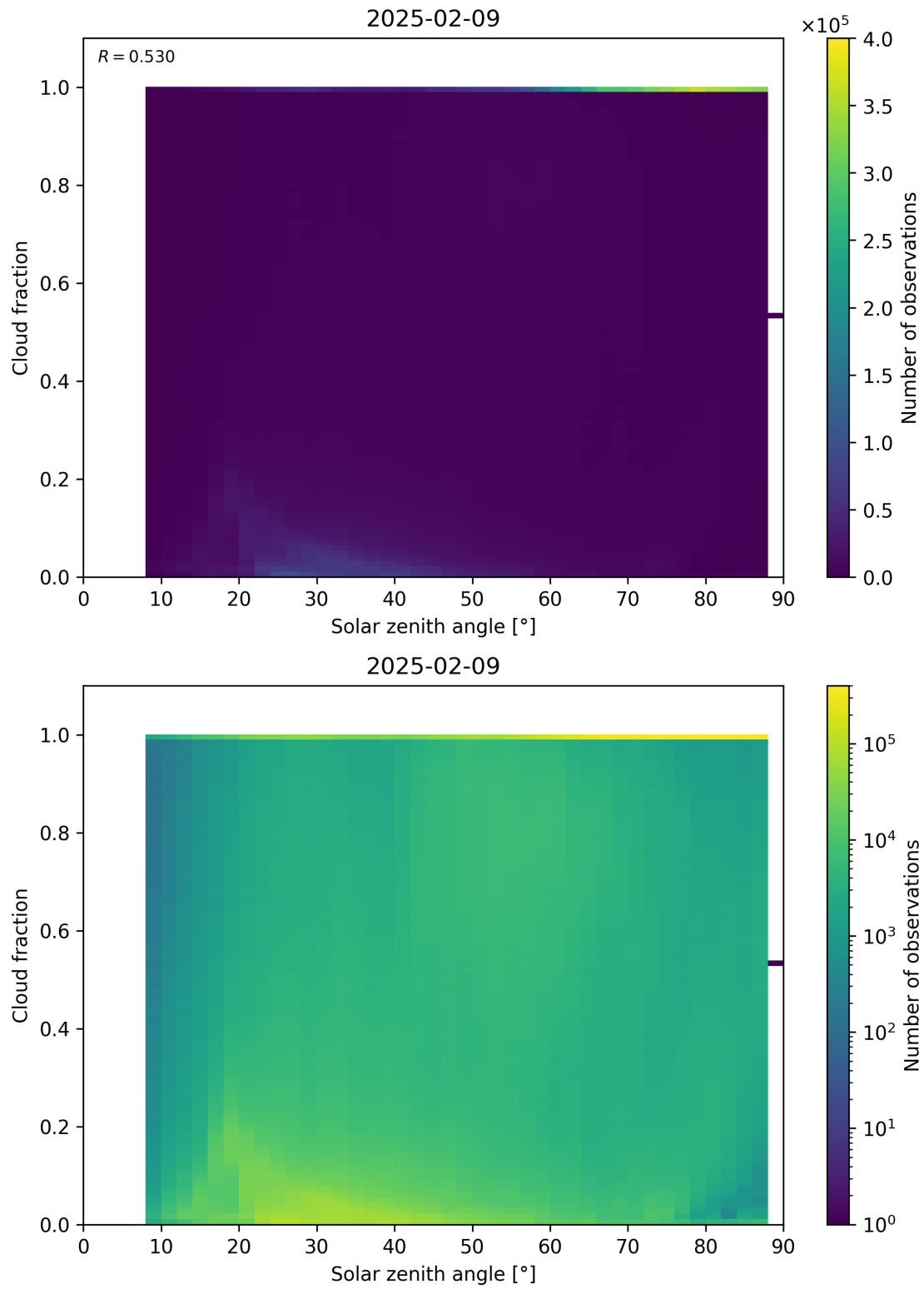
Figure 110: Scatter density plot of “Solar zenith angle” against “Cloud fraction” for 2025-02-08 to 2025-02-10.
