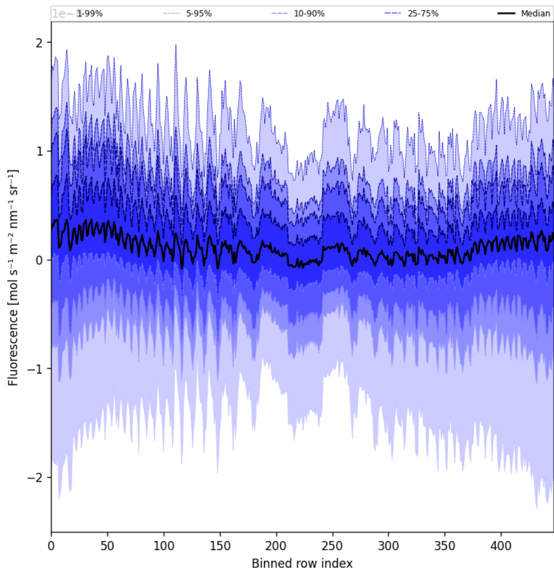
Figure 57: Along track statistics of “Fluorescence” for 2025-02-08 to 2025-02-10
