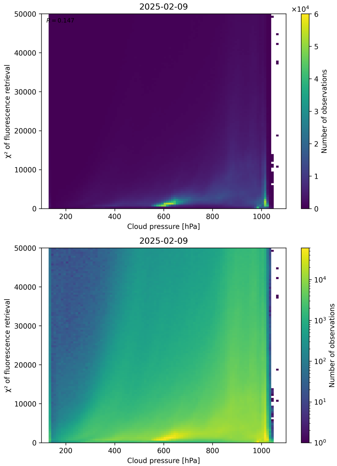
Figure 78: Scatter density plot of “Cloud pressure” against “ \chi^2 of fluorescence retrieval” for 2025-02-08 to 2025-02-10.
