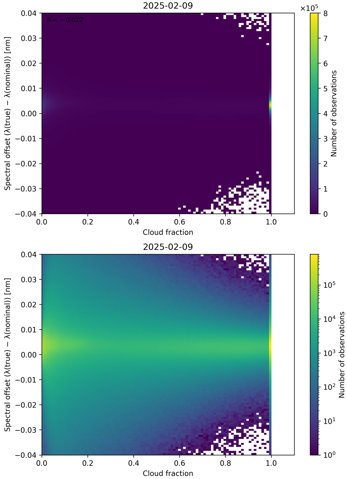
Figure 76: Scatter density plot of “Cloud fraction” against “Spectral offset ( \lambda_{\text{true}} - \lambda_{\text{nominal}} )” for 2025-02-08 to 2025-02-10.
