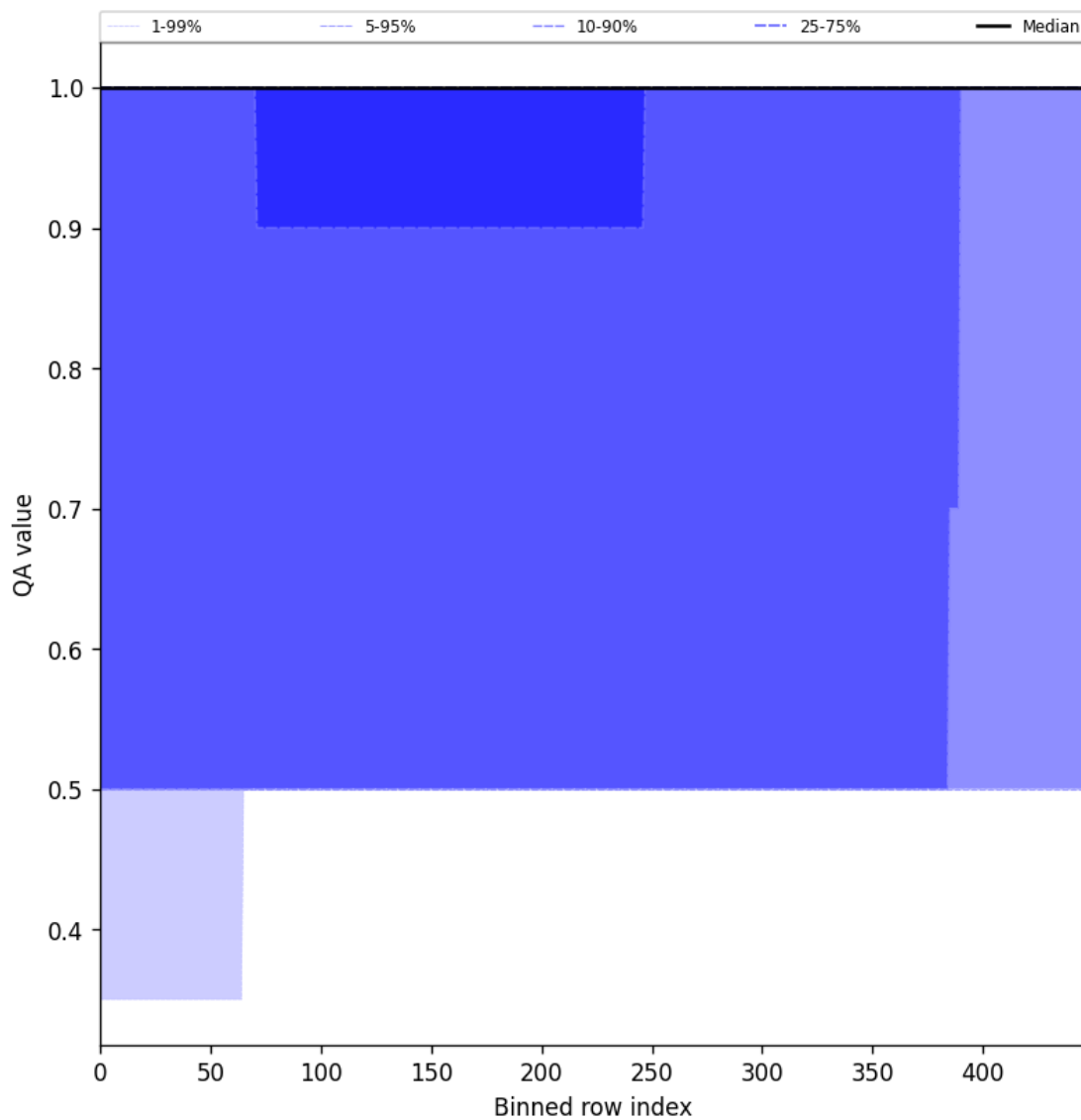
Figure 46: Along track statistics of “QA value” for 2025-02-08 to 2025-02-10
