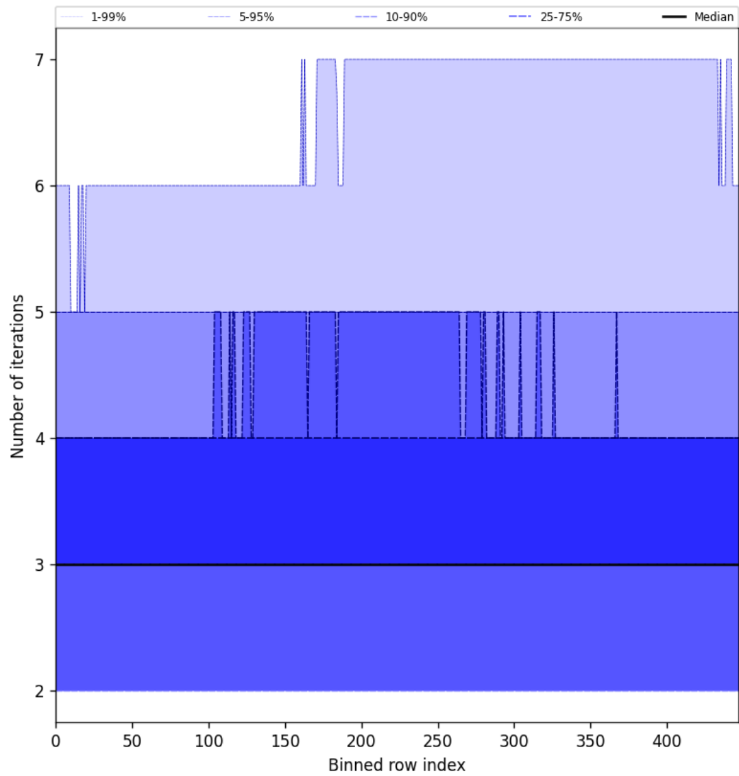
Figure 56: Along track statistics of “Number of iterations” for 2025-02-08 to 2025-02-10
