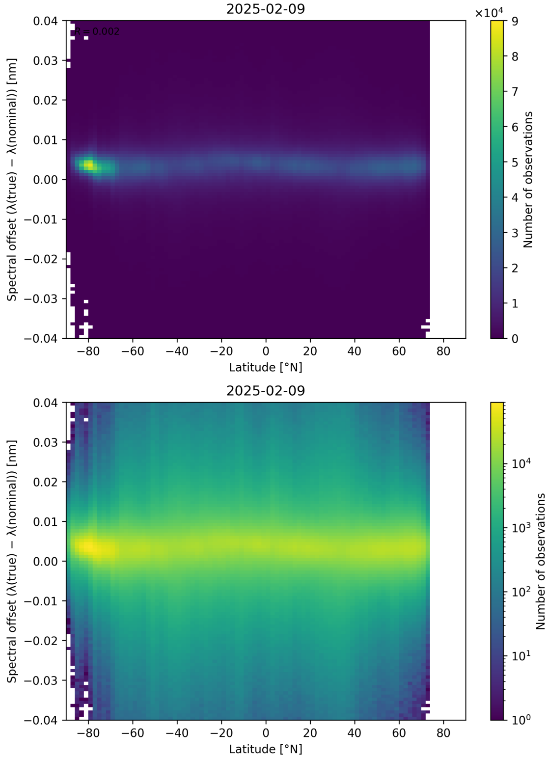
Figure 96: Scatter density plot of “Latitude” against “Spectral offset ( \lambda_{\text{true}} - \lambda_{\text{nominal}} )” for 2025-02-08 to 2025-02-10.
