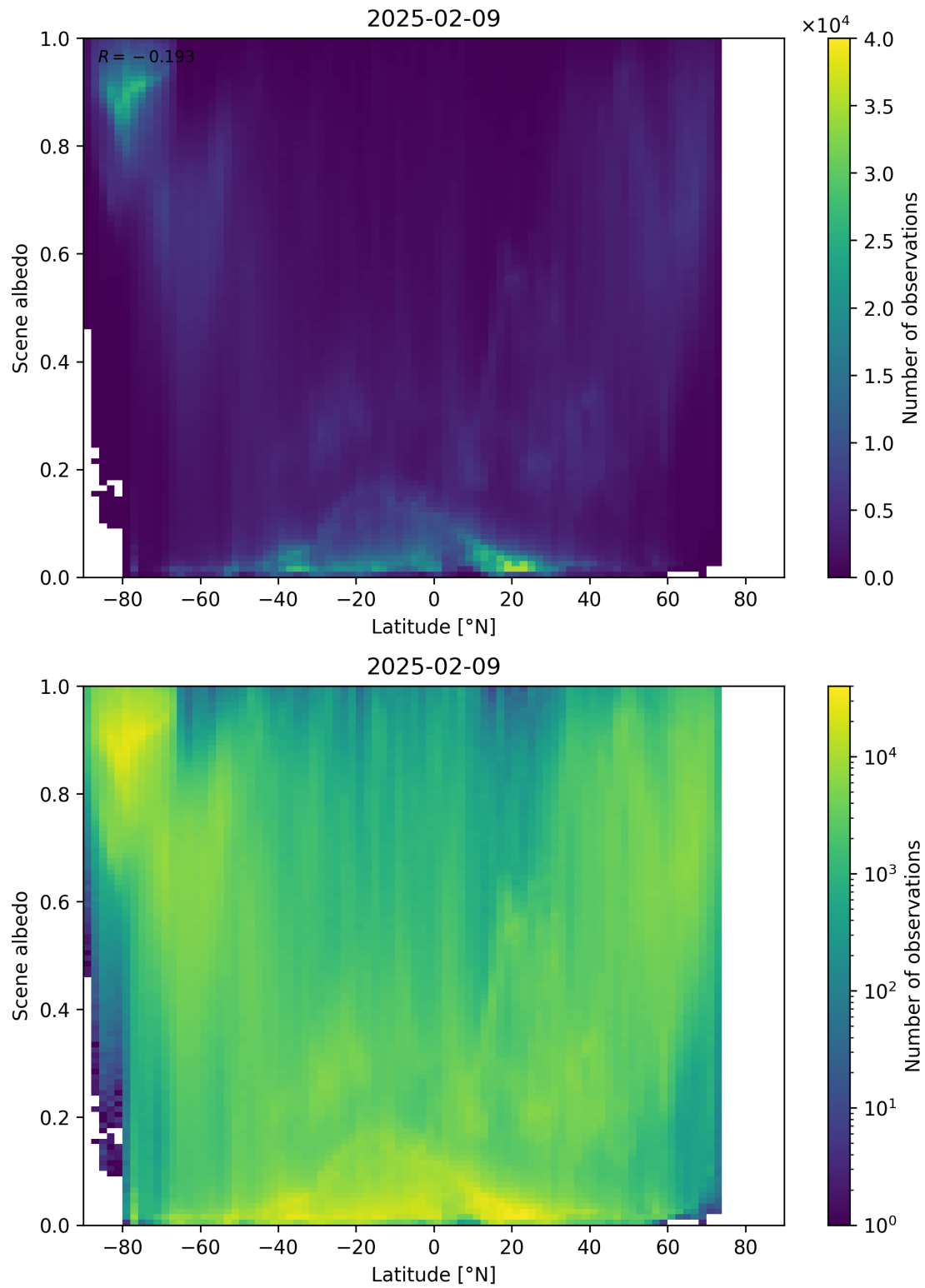
Figure 95: Scatter density plot of “Latitude” against “Scene albedo” for 2025-02-08 to 2025-02-10.
