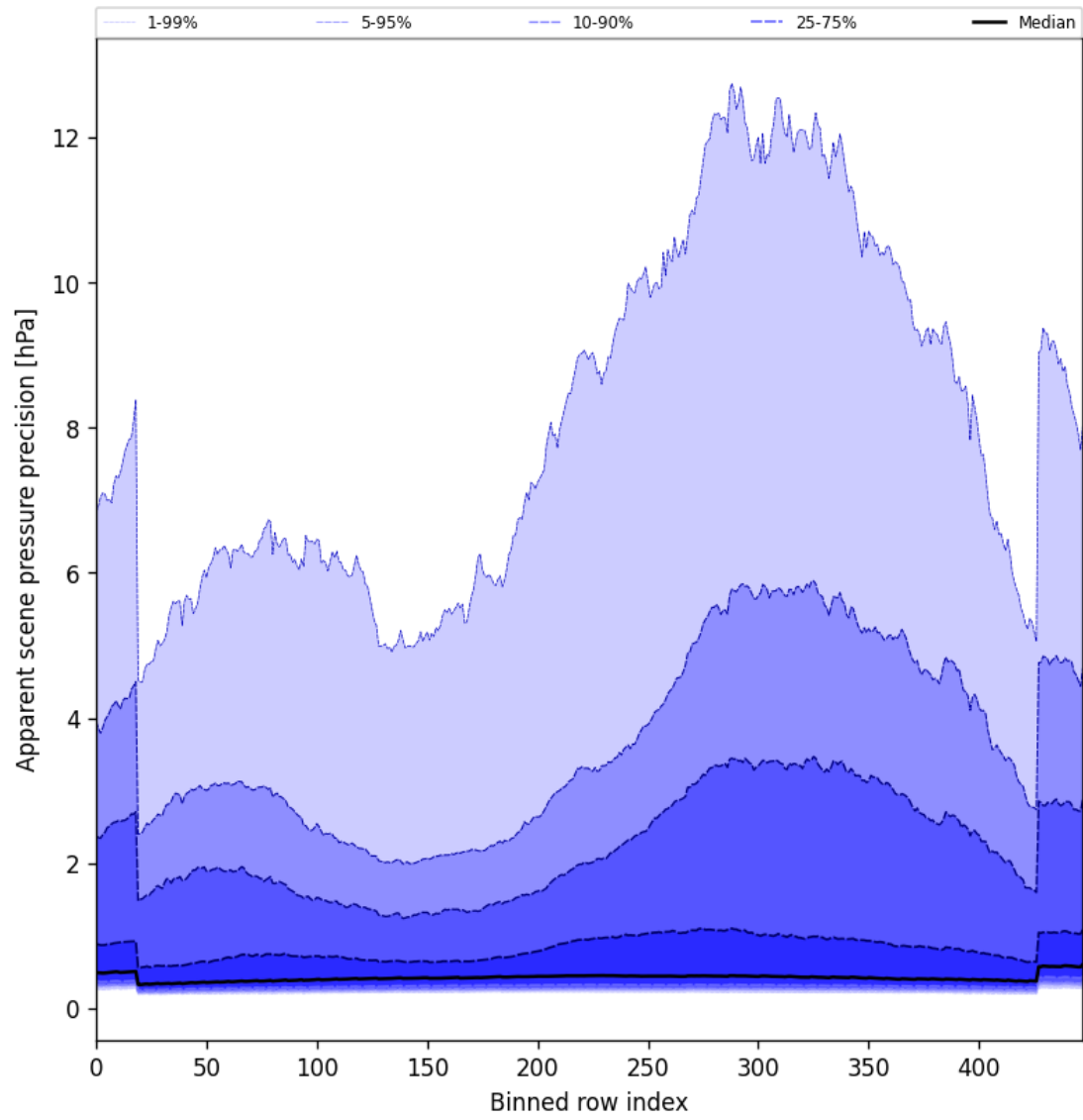
Figure 54: Along track statistics of “Apparent scene pressure precision” for 2025-02-08 to 2025-02-10
