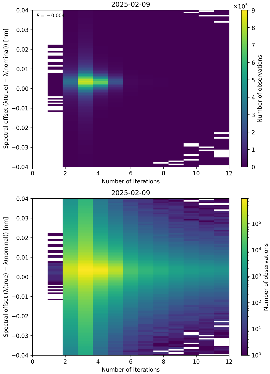
Figure 100: Scatter density plot of “Number of iterations” against “Spectral offset ( \lambda_{\text{true}} - \lambda_{\text{nominal}} )” for 2025-02-08 to 2025-02-10.
