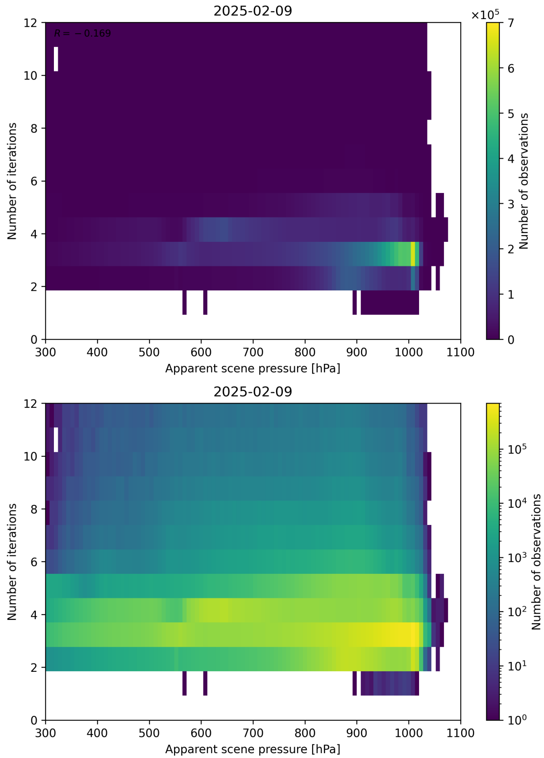
Figure 65: Scatter density plot of “Apparent scene pressure” against “Number of iterations” for 2025-02-08 to 2025-02-10.
