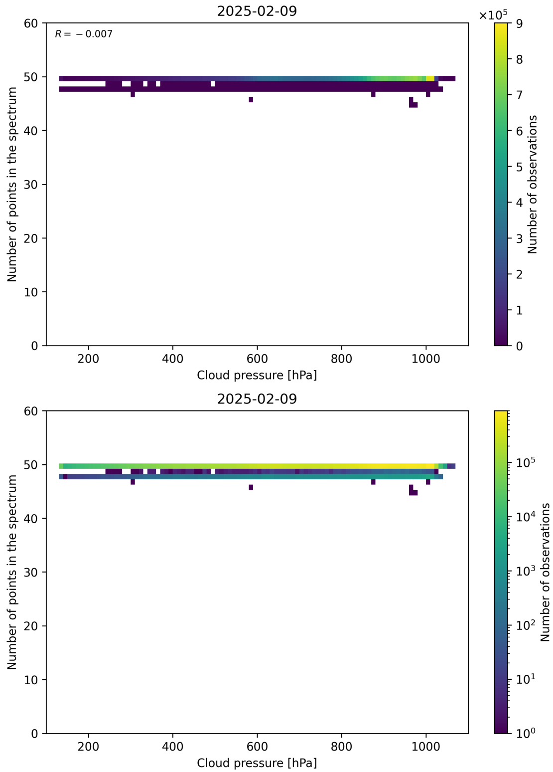
Figure 82: Scatter density plot of “Cloud pressure” against “Number of points in the spectrum” for 2025-02-08 to 2025-02-10.
