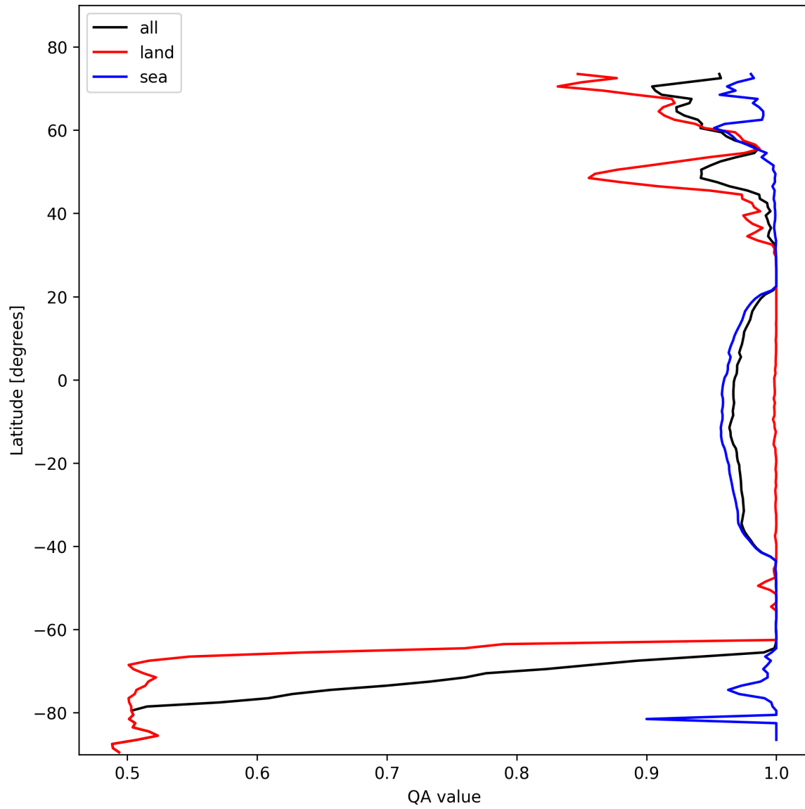
Figure 12: Zonal average of “QA value” for 2025-02-08 to 2025-02-10.
