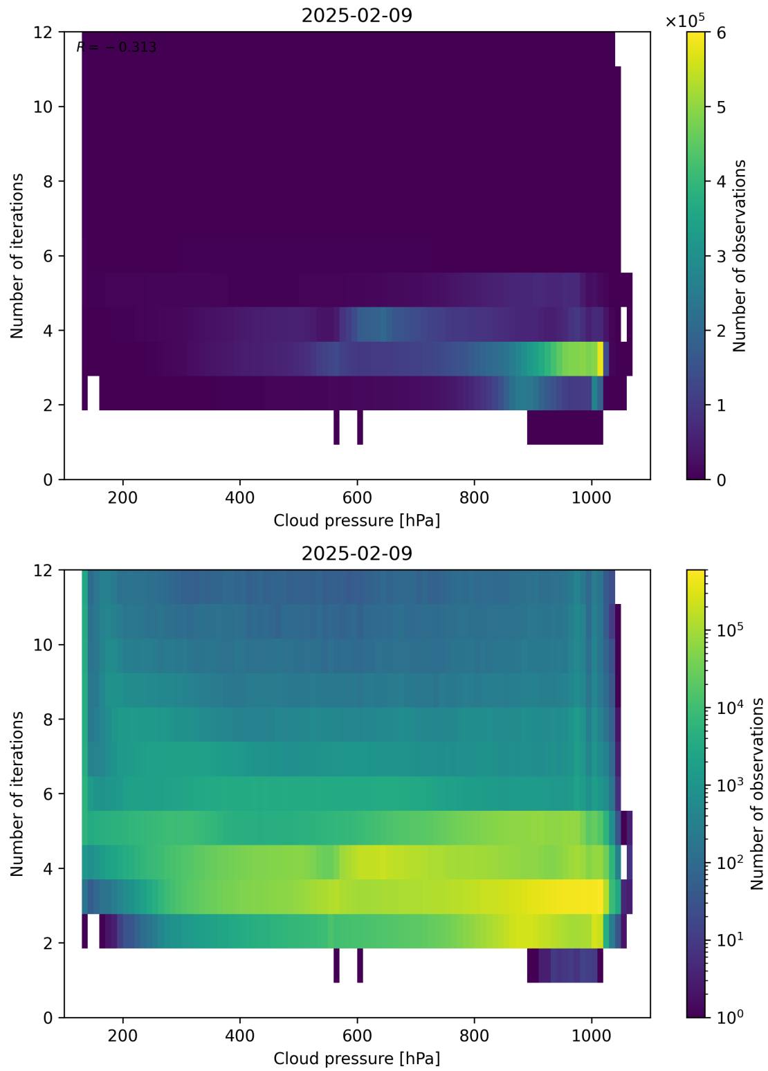
Figure 81: Scatter density plot of “Cloud pressure” against “Number of iterations” for 2025-02-08 to 2025-02-10.
