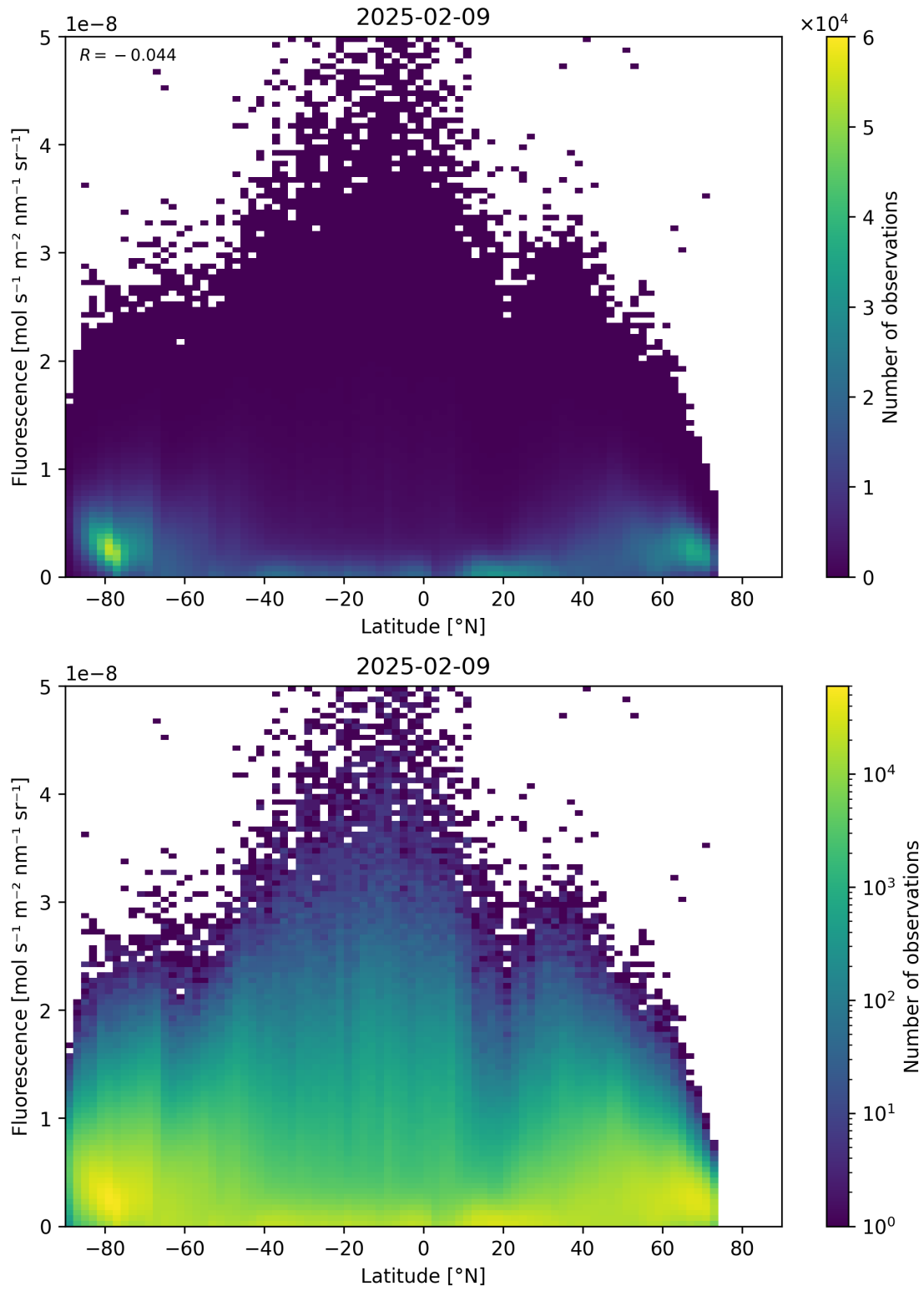
Figure 92: Scatter density plot of “Latitude” against “Fluorescence” for 2025-02-08 to 2025-02-10.
