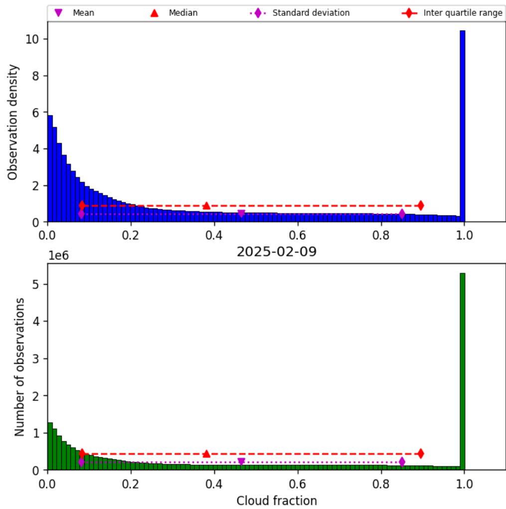
Figure 32: Histogram of “Cloud fraction” for 2025-02-08 to 2025-02-10
