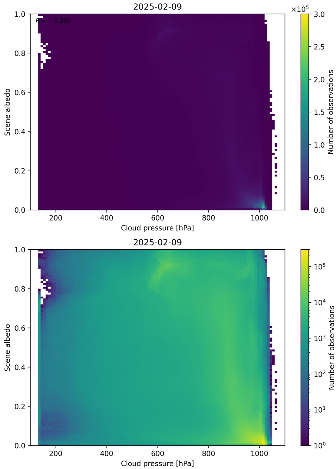
Figure 83: Scatter density plot of “Cloud pressure” against “Scene albedo” for 2025-02-08 to 2025-02-10.
