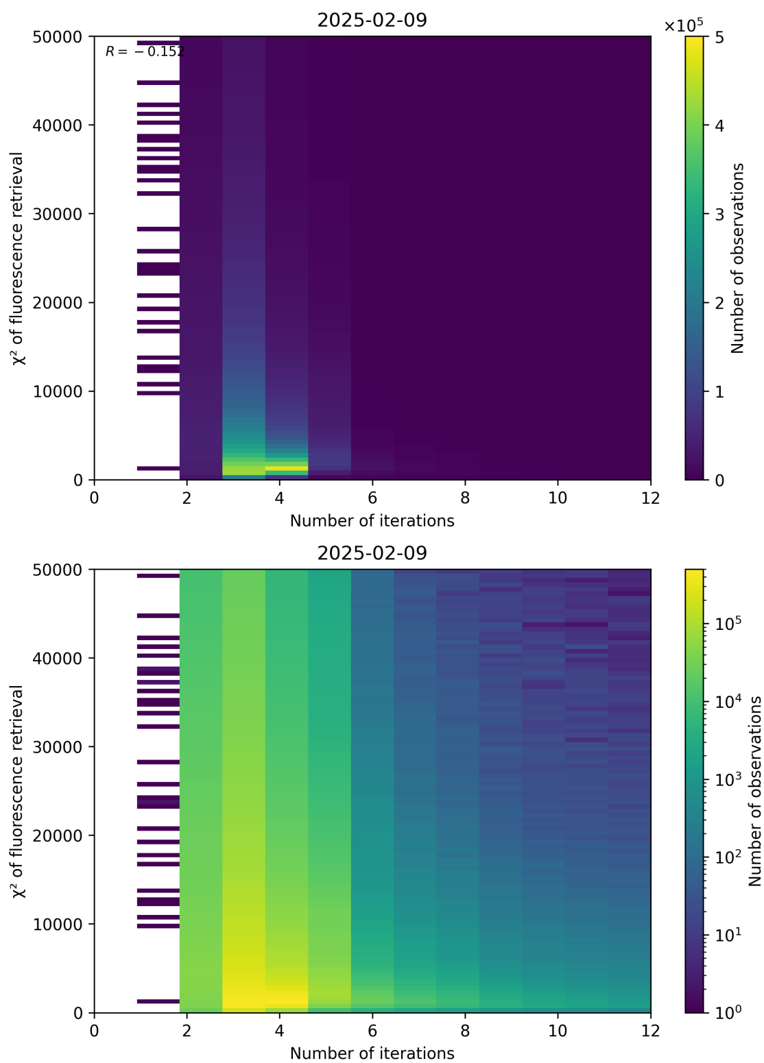
Figure 97: Scatter density plot of “Number of iterations” against “ \chi^2 of fluorescence retrieval” for 2025-02-08 to 2025-02-10.
