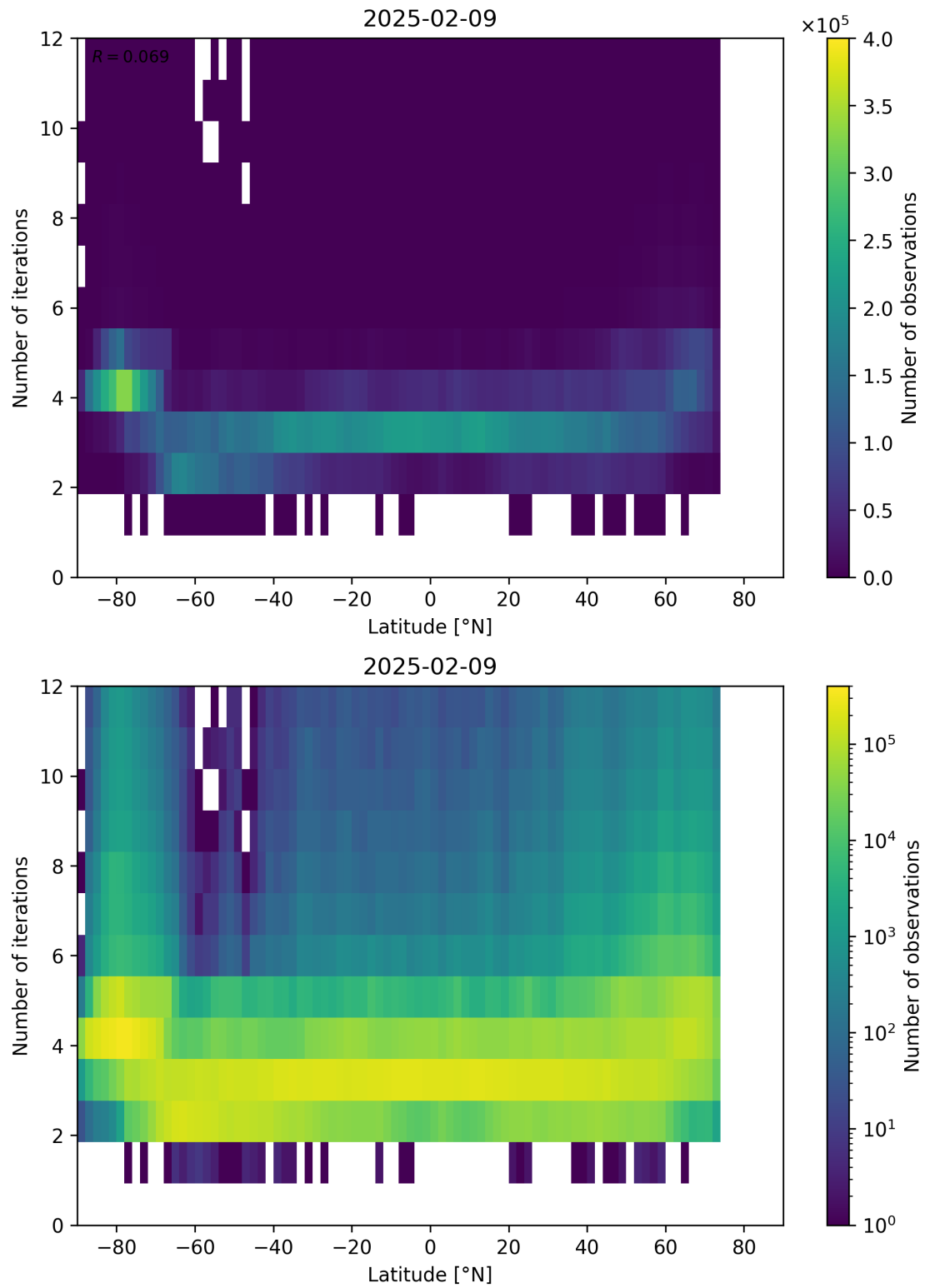
Figure 93: Scatter density plot of “Latitude” against “Number of iterations” for 2025-02-08 to 2025-02-10.
