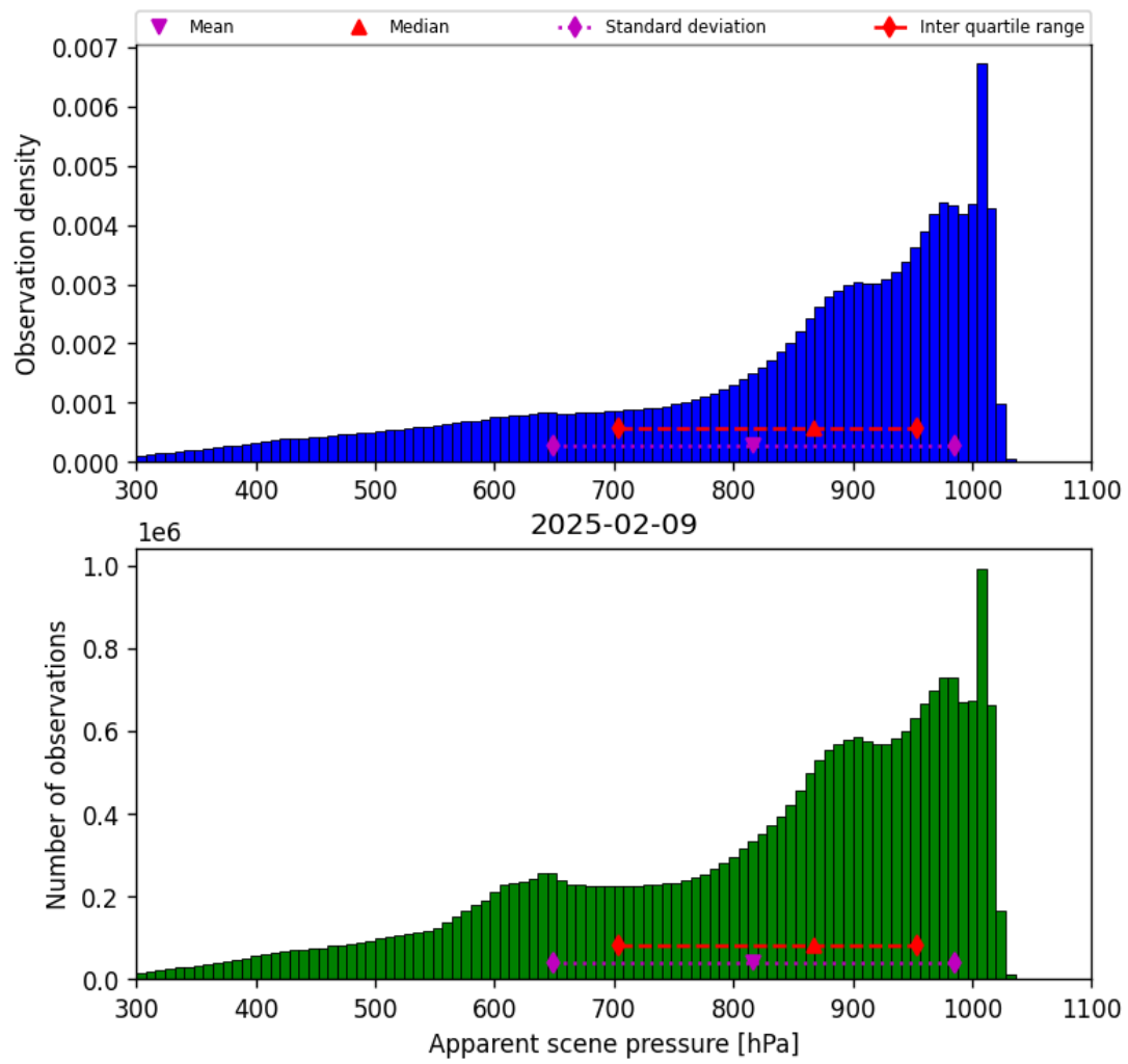
Figure 36: Histogram of “Apparent scene pressure” for 2025-02-08 to 2025-02-10
