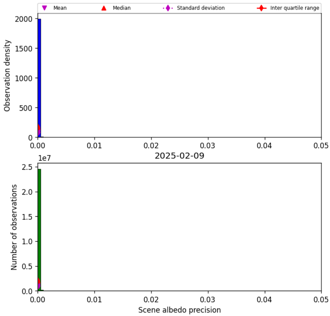
Figure 35: Histogram of “Scene albedo precision” for 2025-02-08 to 2025-02-10
