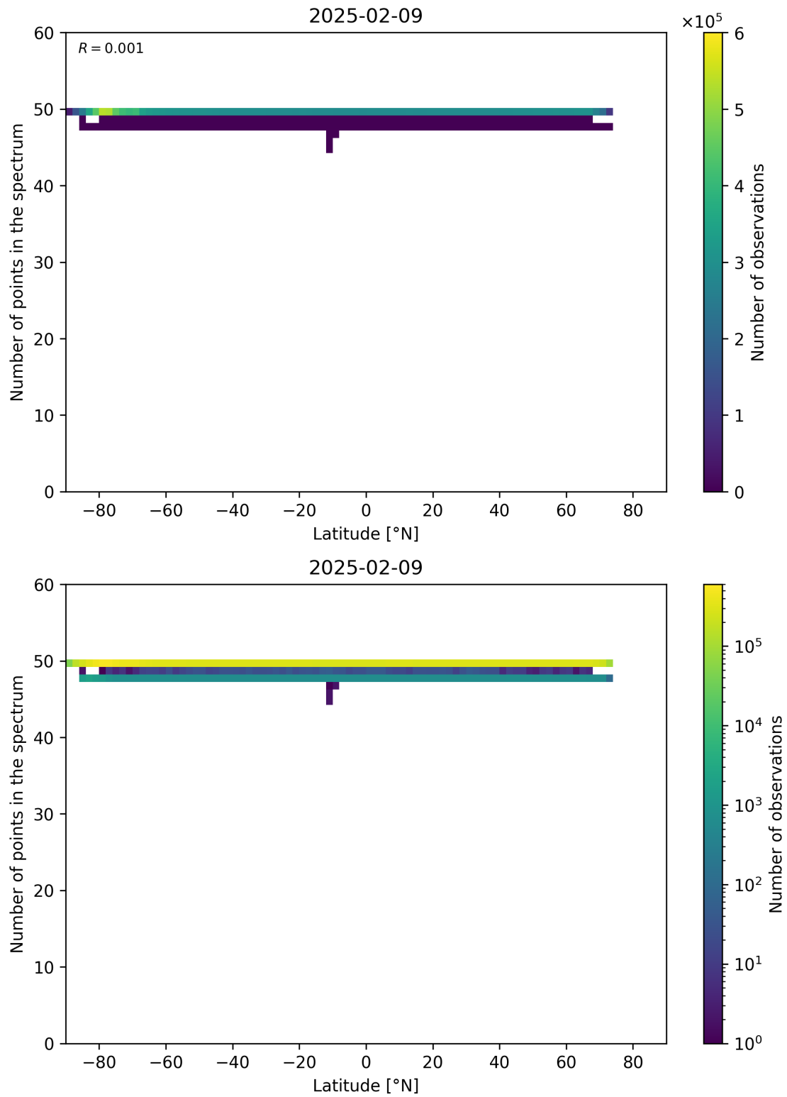
Figure 94: Scatter density plot of “Latitude” against “Number of points in the spectrum” for 2025-02-08 to 2025-02-10.
