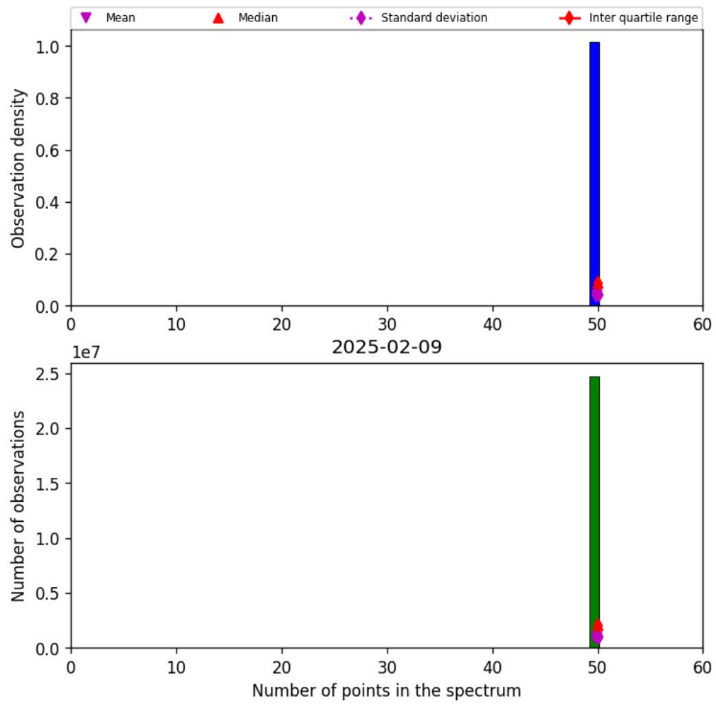
Figure 44: Histogram of “Number of points in the spectrum” for 2025-02-08 to 2025-02-10
