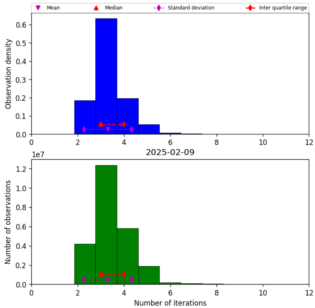
Figure 39: Histogram of “Number of iterations” for 2025-02-08 to 2025-02-10
