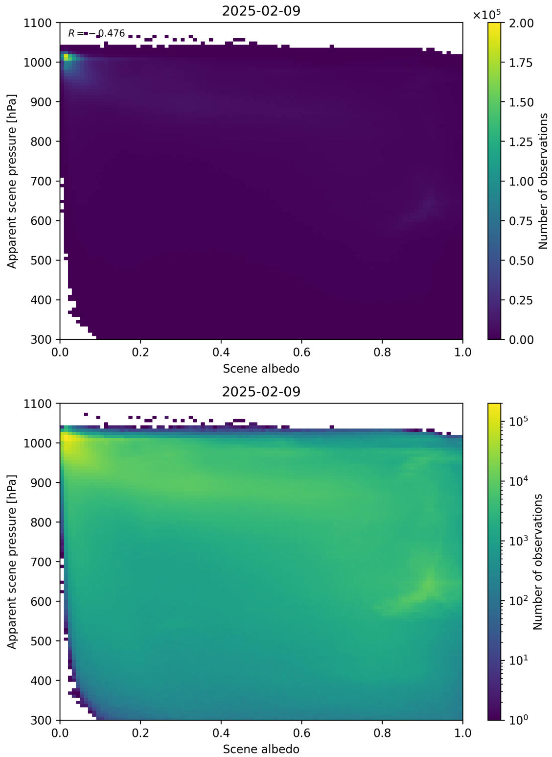
Figure 102: Scatter density plot of “Scene albedo” against “Apparent scene pressure” for 2025-02-08 to 2025-02-10.
