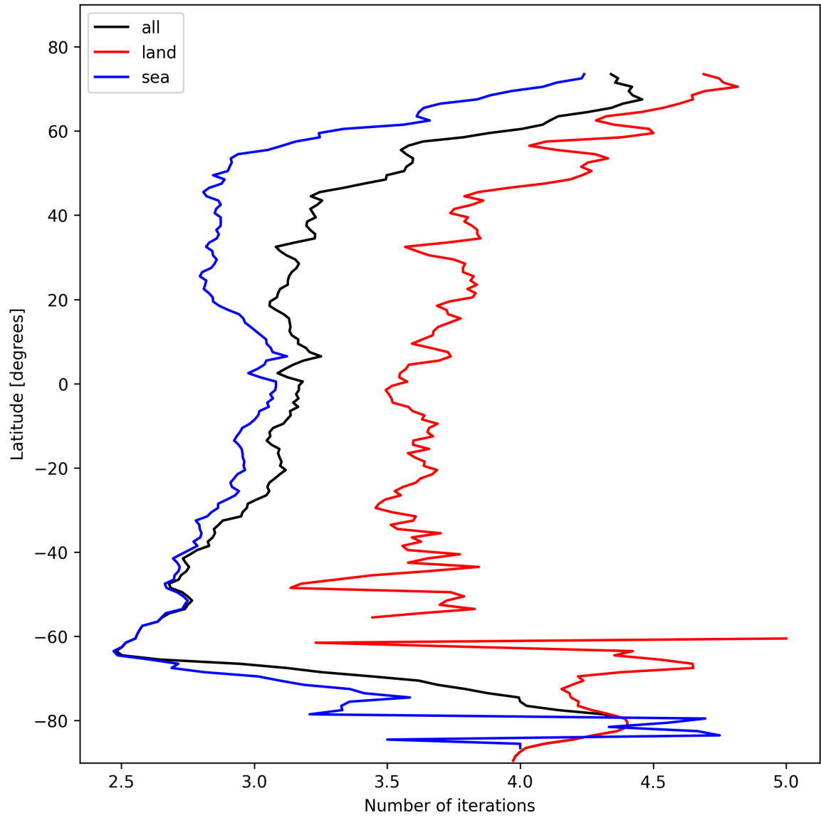
Figure 22: Zonal average of “Number of iterations” for 2025-02-08 to 2025-02-10.
