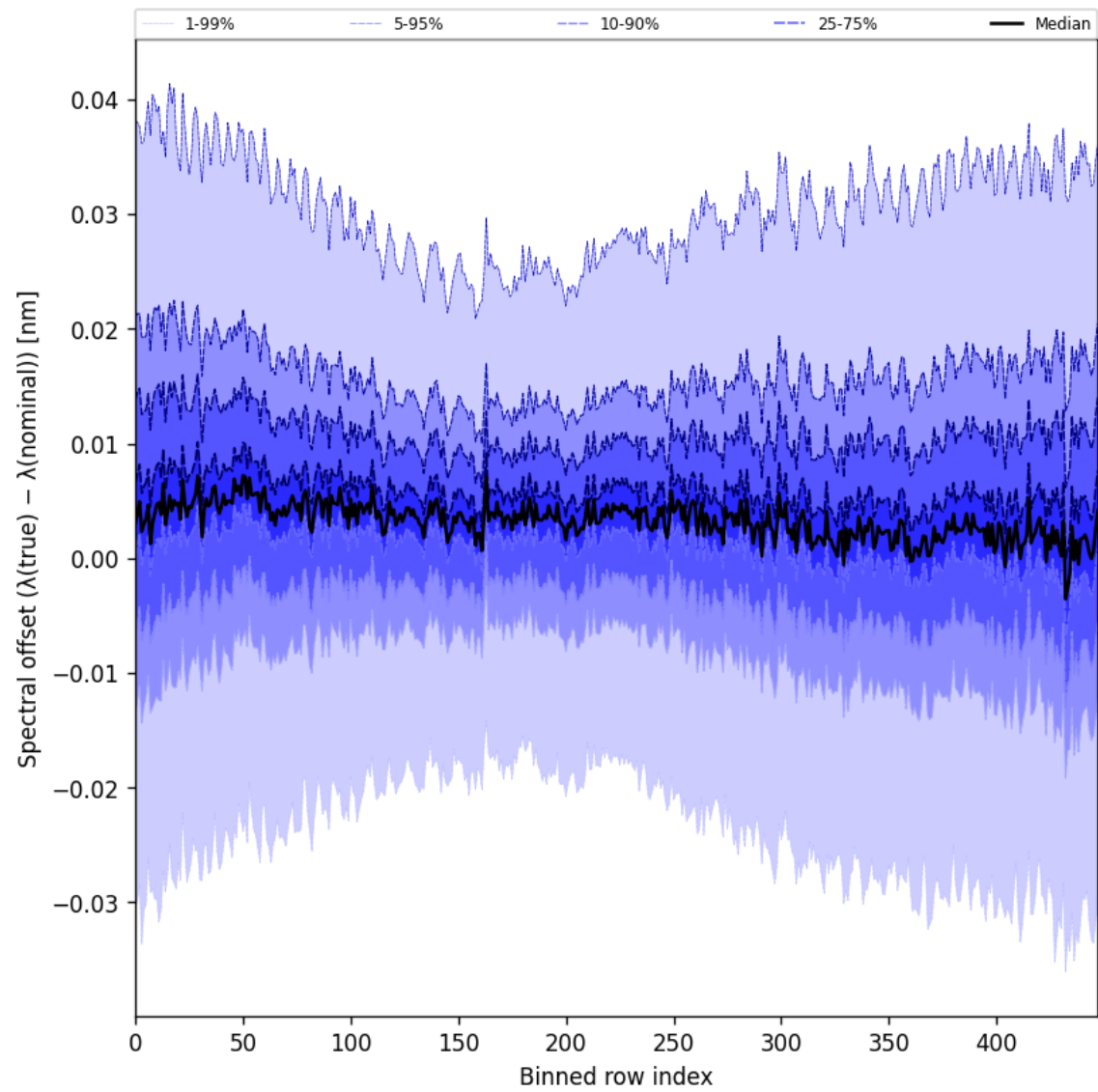
Figure 62: Along track statistics of “Spectral offset ( \lambda_{\text{true}} - \lambda_{\text{nominal}} )” for 2025-02-08 to 2025-02-10
