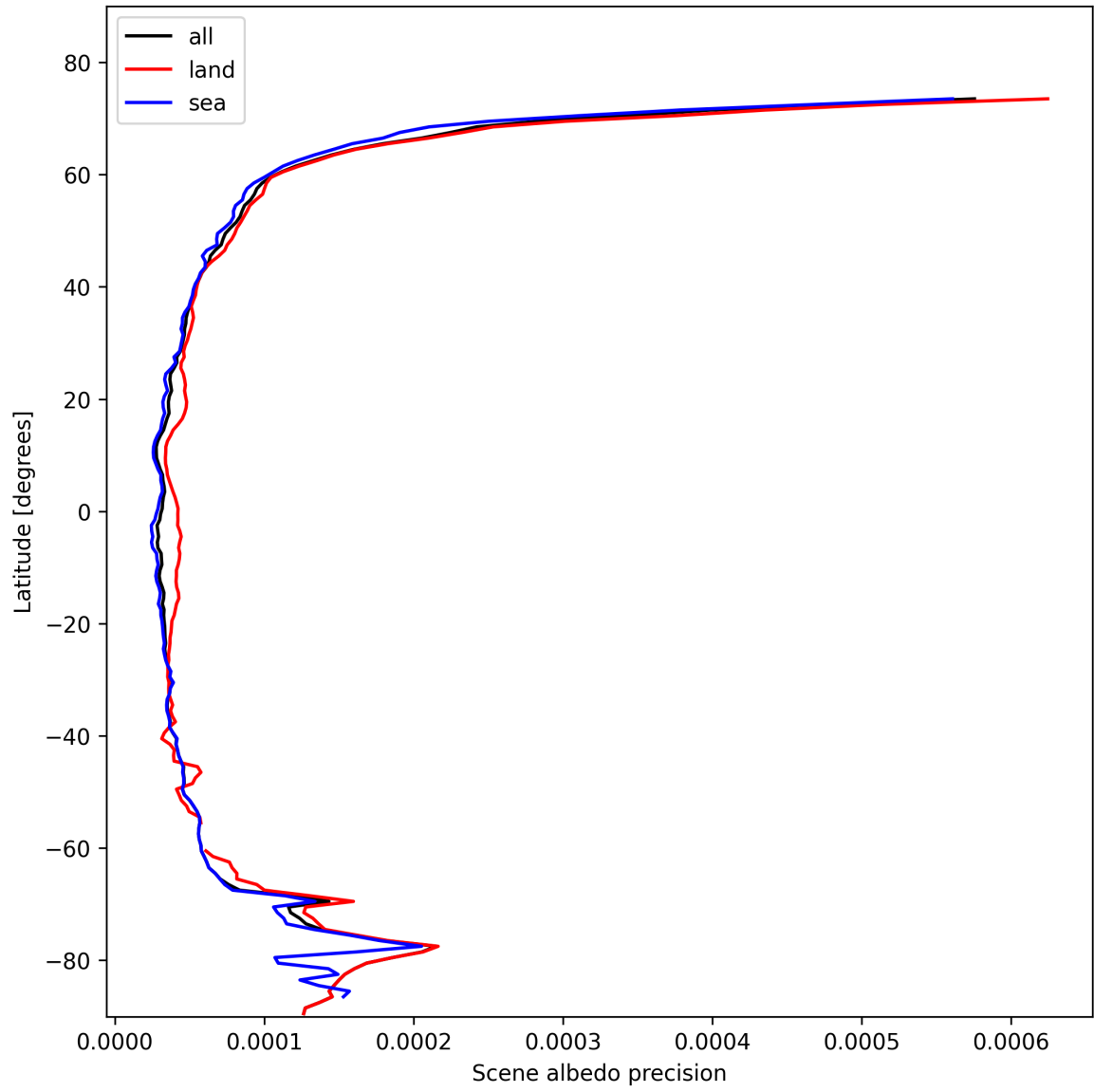
Figure 18: Zonal average of “Scene albedo precision” for 2025-02-08 to 2025-02-10.
