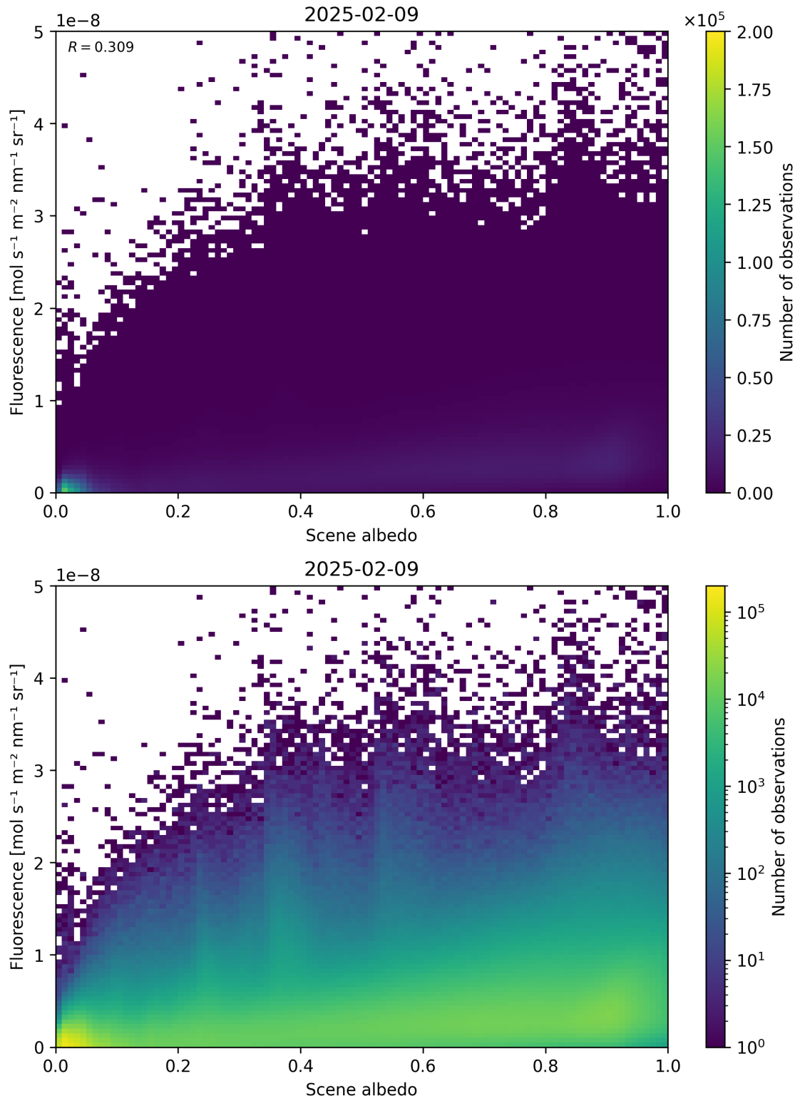
Figure 104: Scatter density plot of “Scene albedo” against “Fluorescence” for 2025-02-08 to 2025-02-10.
