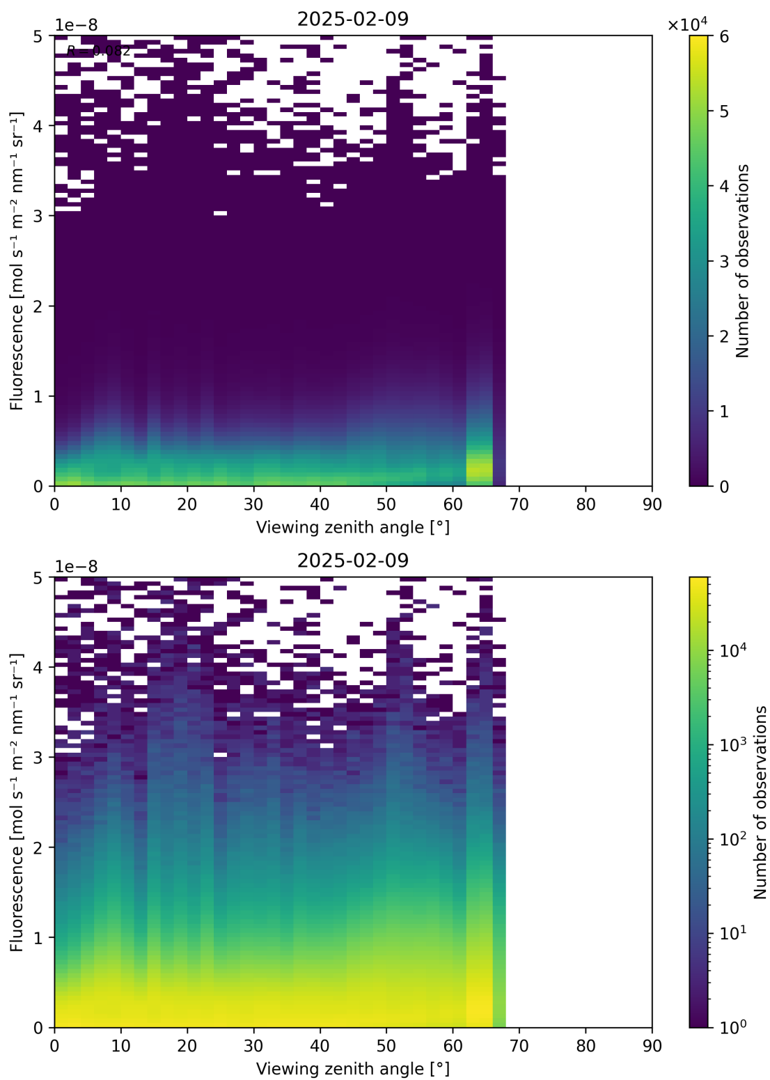
Figure 122: Scatter density plot of “Viewing zenith angle” against “Fluorescence” for 2025-02-08 to 2025-02-10.
