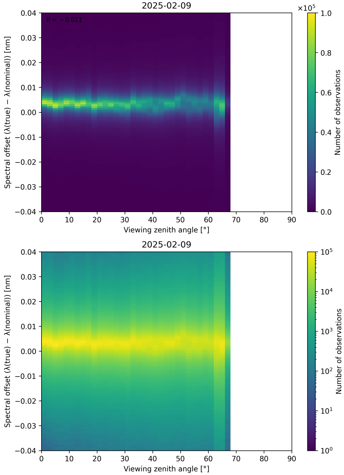
Figure 128: Scatter density plot of “Viewing zenith angle” against “Spectral offset ( \lambda_{\text{true}} - \lambda_{\text{nominal}} )” for 2025-02-08 to 2025-02-10.
