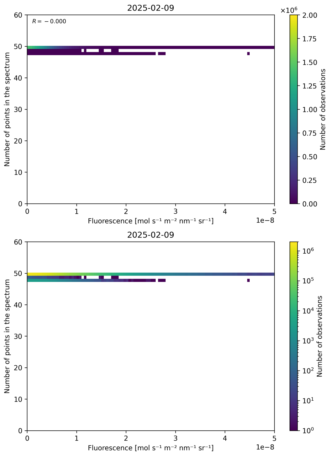
Figure 86: Scatter density plot of “Fluorescence” against “Number of points in the spectrum” for 2025-02-08 to 2025-02-10.
