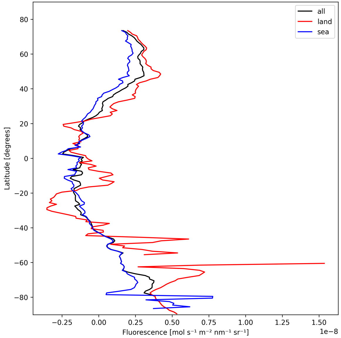
Figure 23: Zonal average of “Fluorescence” for 2025-02-08 to 2025-02-10.
