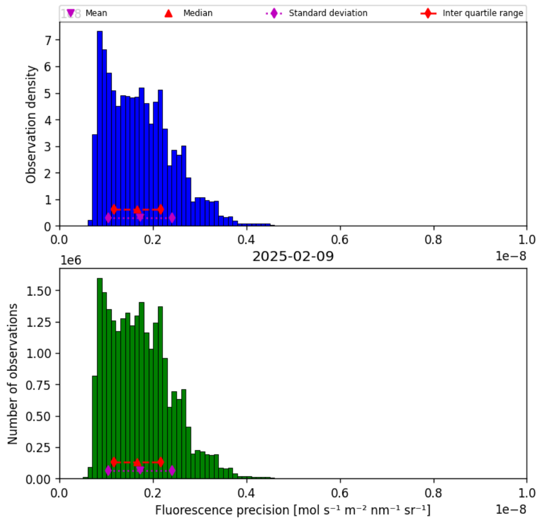
Figure 41: Histogram of “Fluorescence precision” for 2025-02-08 to 2025-02-10
