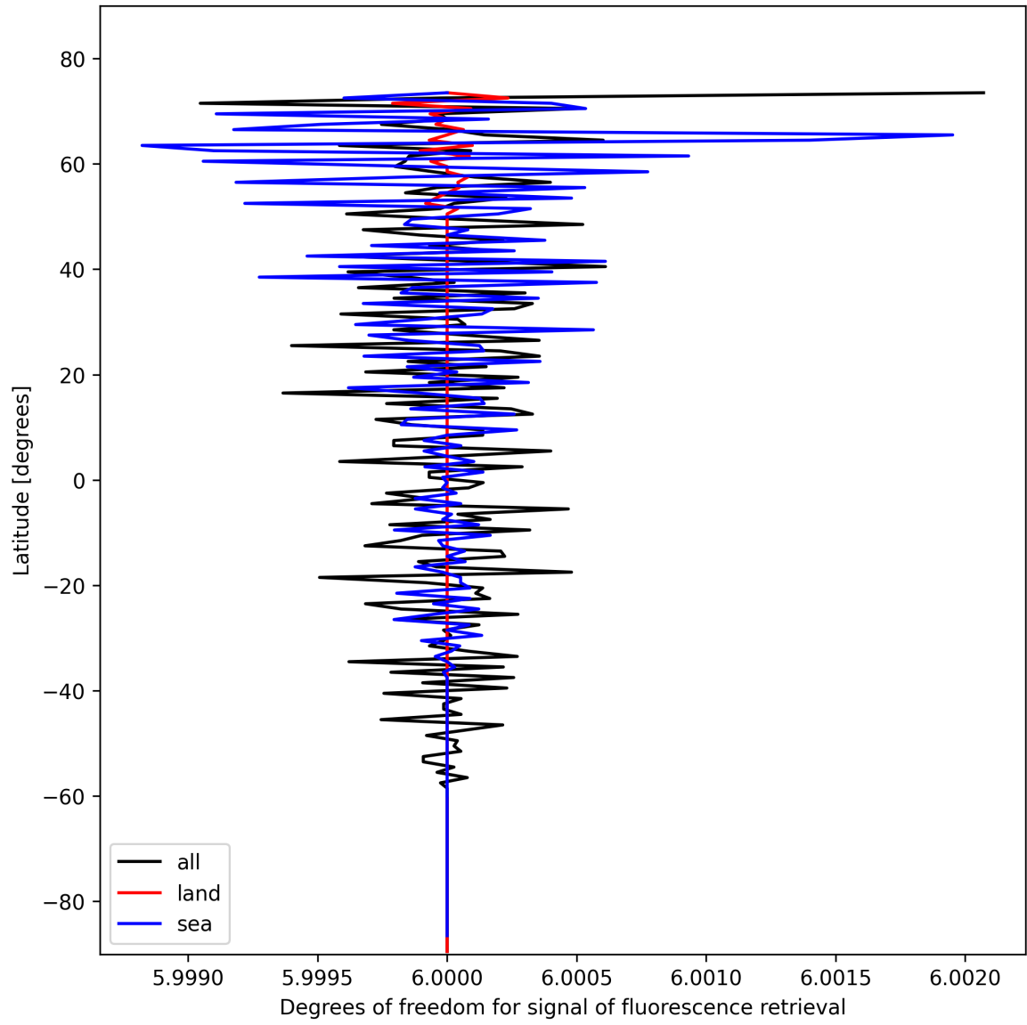
Figure 26: Zonal average of “Degrees of freedom for signal of fluorescence retrieval” for 2025-02-08 to 2025-02-10.
