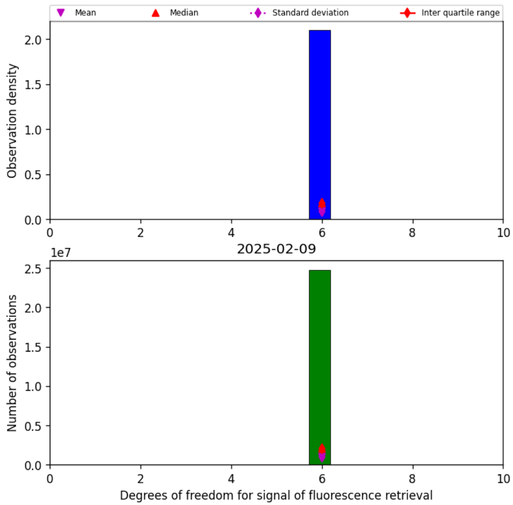
Figure 43: Histogram of “Degrees of freedom for signal of fluorescence retrieval” for 2025-02-08 to 2025-02-10
