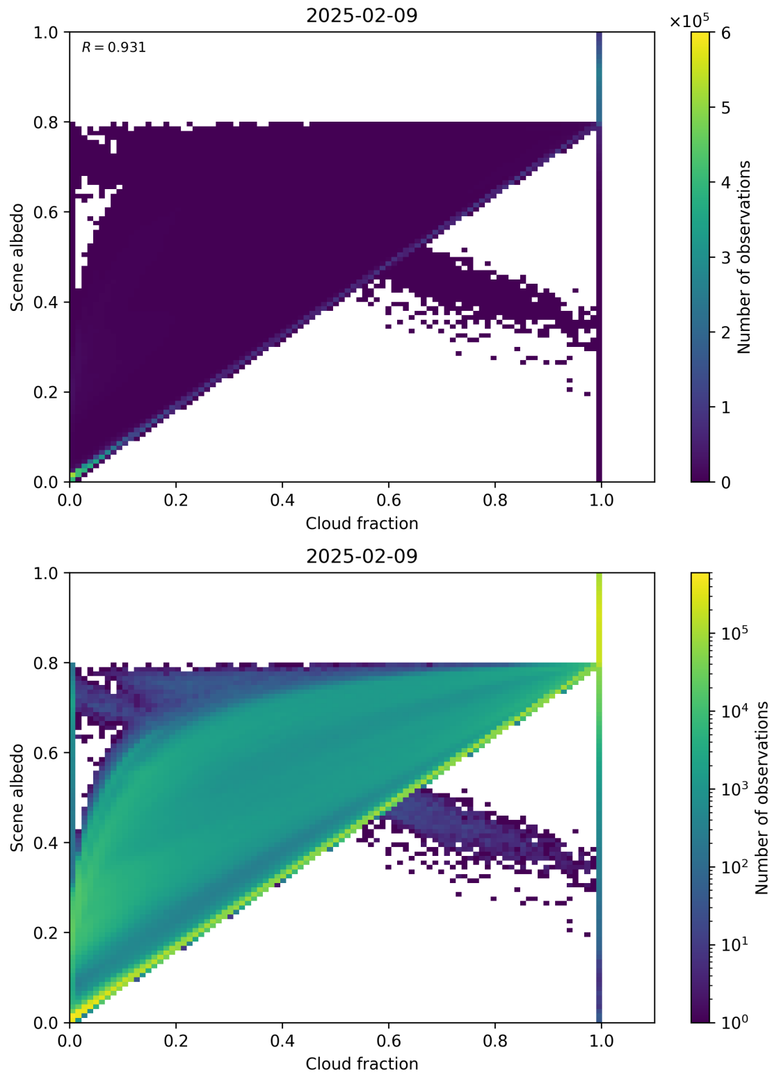
Figure 75: Scatter density plot of “Cloud fraction” against “Scene albedo” for 2025-02-08 to 2025-02-10.
