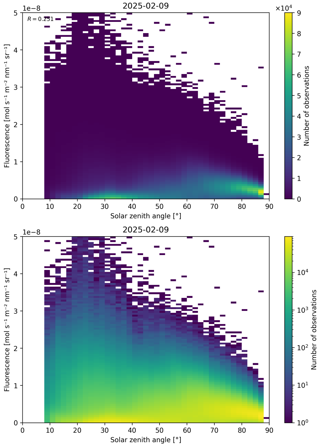
Figure 112: Scatter density plot of “Solar zenith angle” against “Fluorescence” for 2025-02-08 to 2025-02-10.
