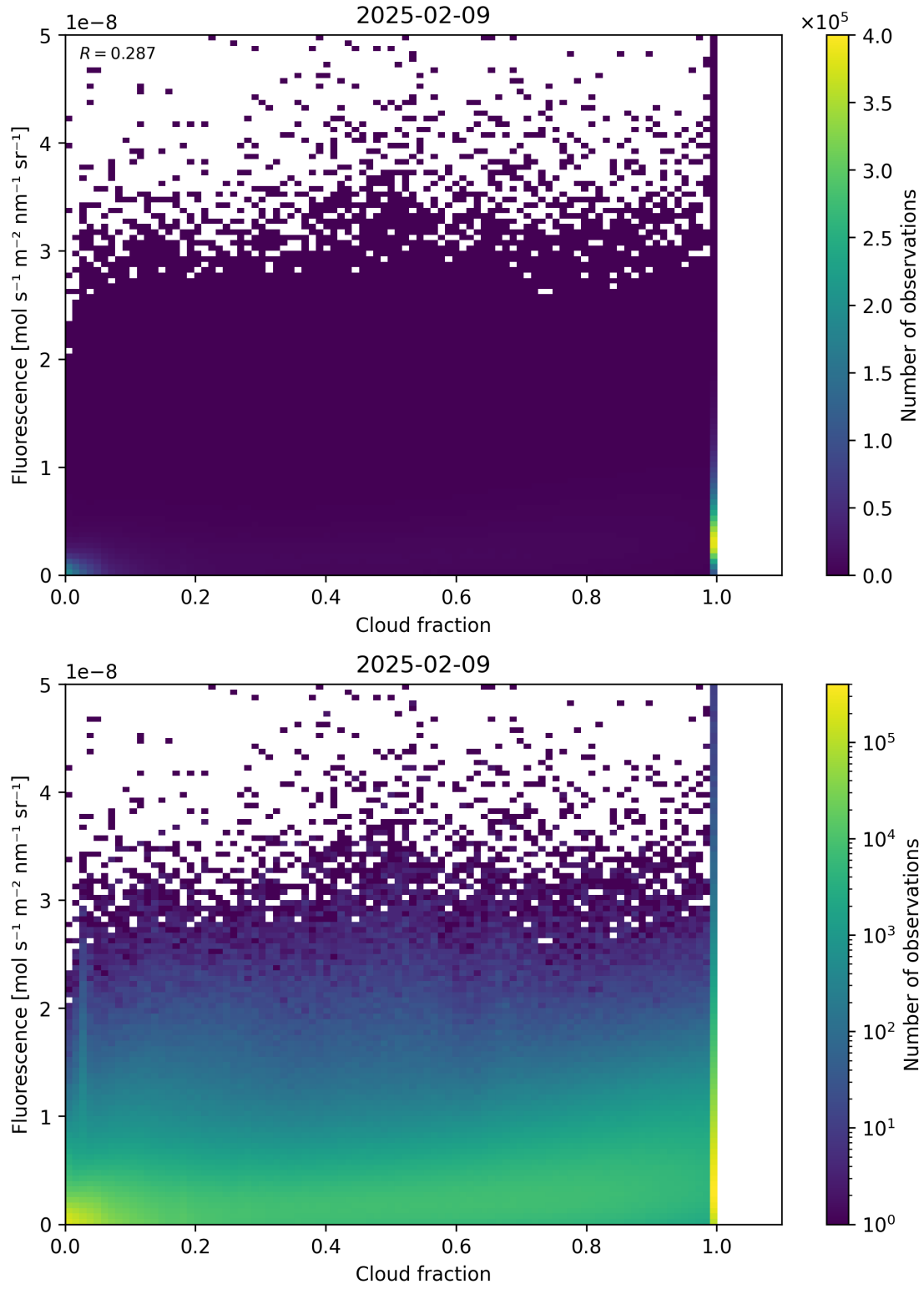
Figure 72: Scatter density plot of “Cloud fraction” against “Fluorescence” for 2025-02-08 to 2025-02-10.
