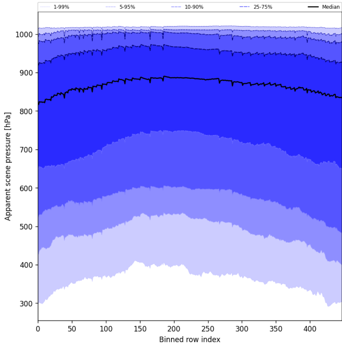
Figure 53: Along track statistics of “Apparent scene pressure” for 2025-02-08 to 2025-02-10
