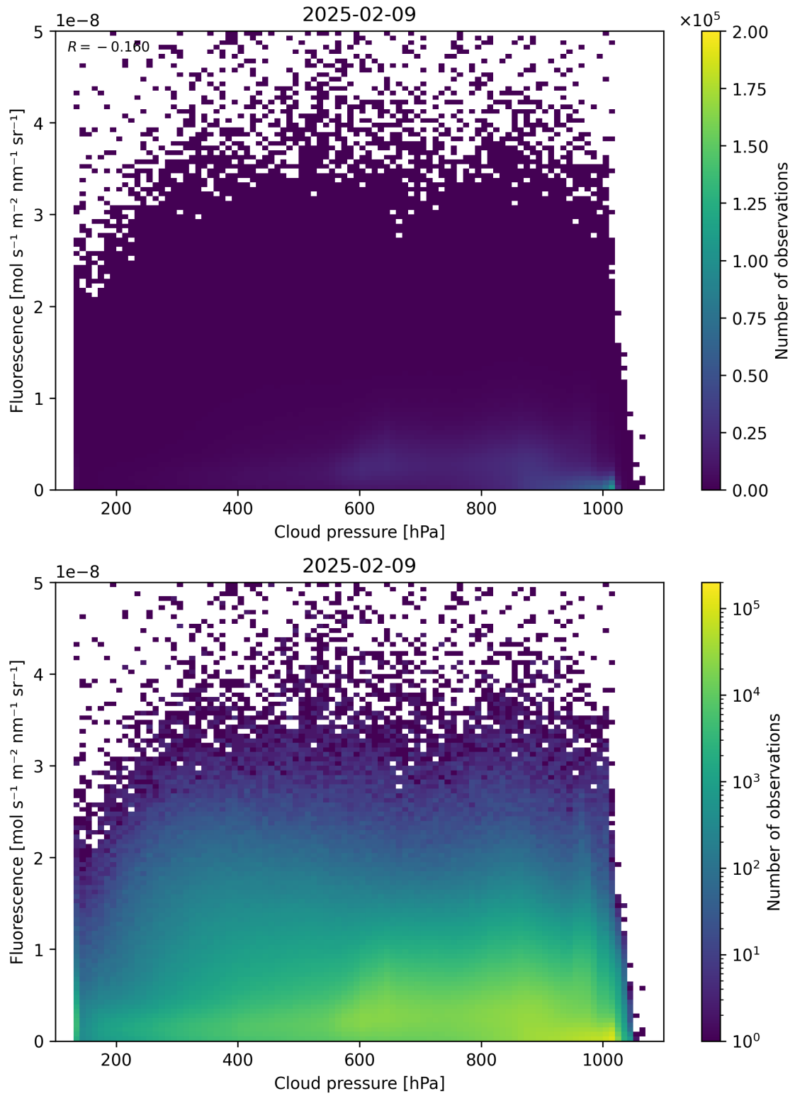
Figure 80: Scatter density plot of “Cloud pressure” against “Fluorescence” for 2025-02-08 to 2025-02-10.
