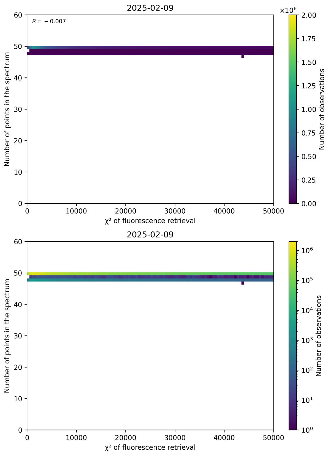
Figure 68: Scatter density plot of “ \chi^2 of fluorescence retrieval” against “Number of points in the spectrum” for 2025-02-08 to 2025-02-10.
