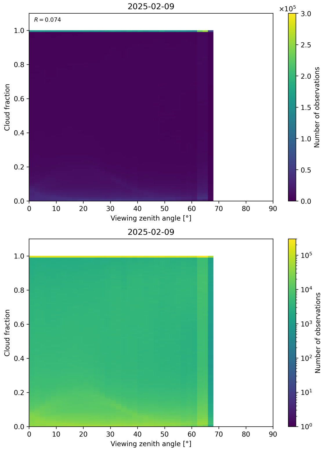
Figure 120: Scatter density plot of “Viewing zenith angle” against “Cloud fraction” for 2025-02-08 to 2025-02-10.
