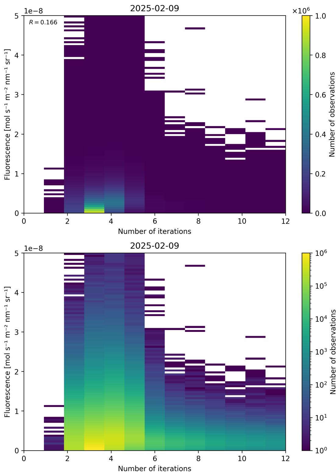
Figure 98: Scatter density plot of “Number of iterations” against “Fluorescence” for 2025-02-08 to 2025-02-10.
