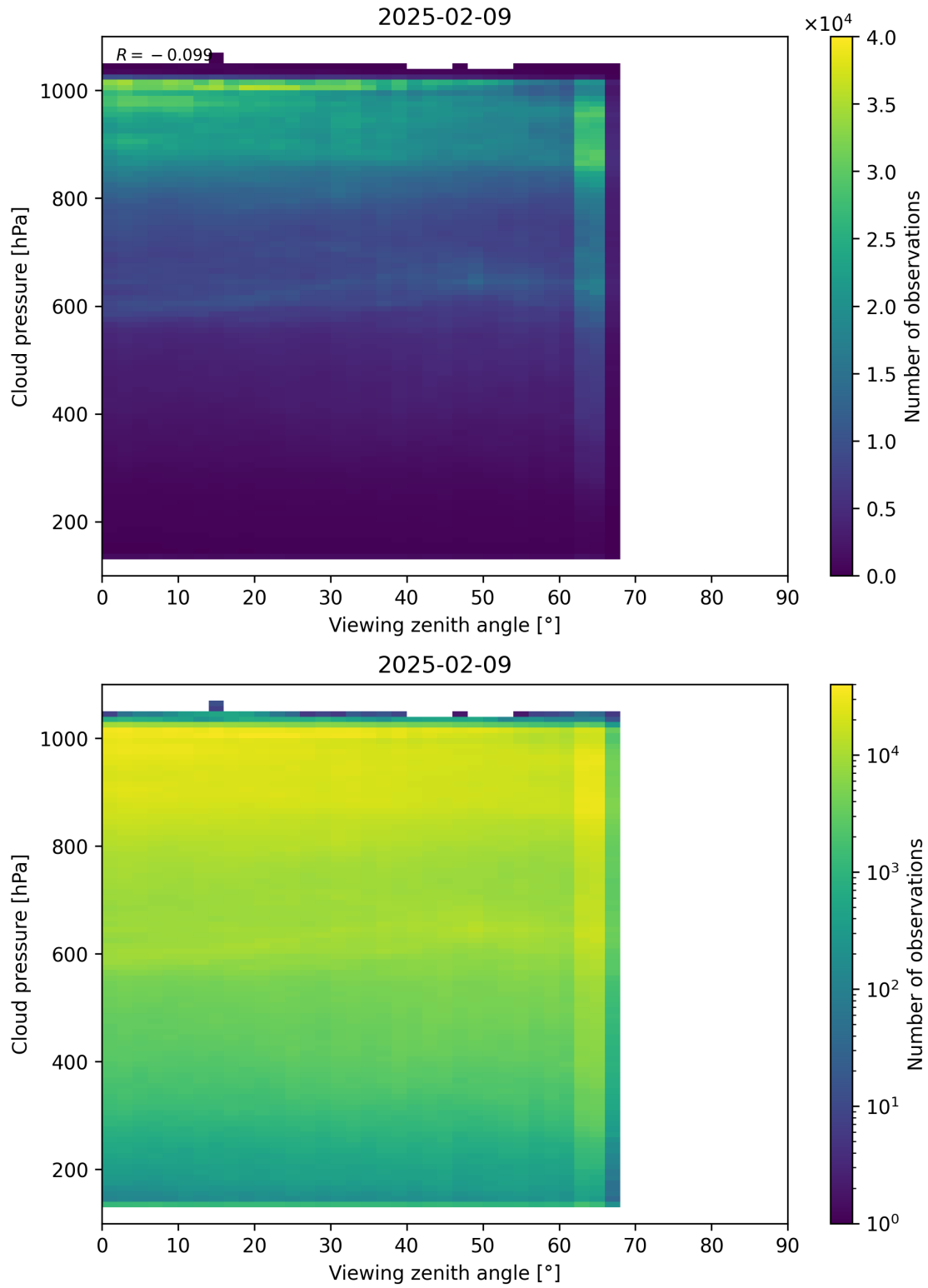
Figure 121: Scatter density plot of “Viewing zenith angle” against “Cloud pressure” for 2025-02-08 to 2025-02-10.
