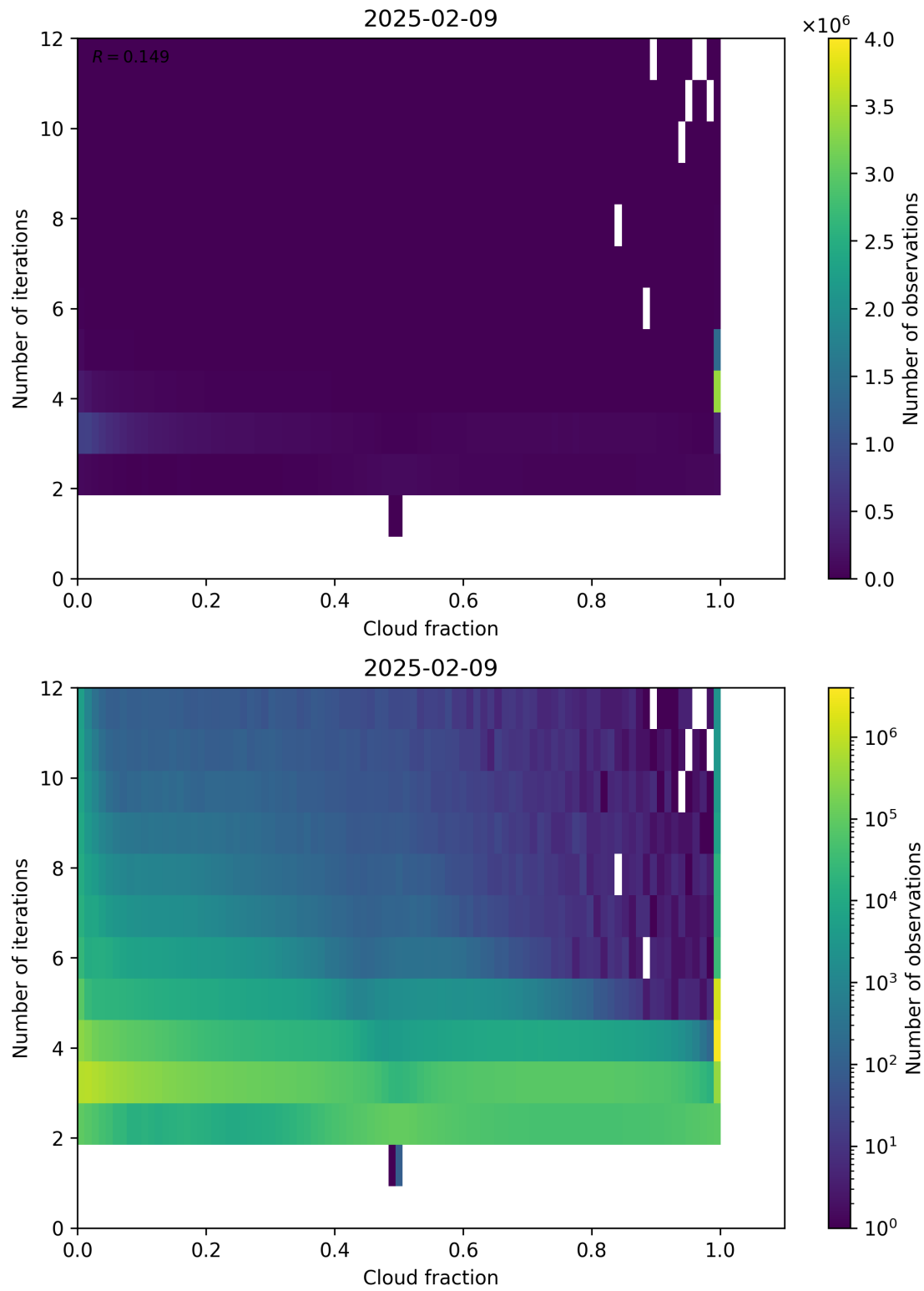
Figure 73: Scatter density plot of “Cloud fraction” against “Number of iterations” for 2025-02-08 to 2025-02-10.
