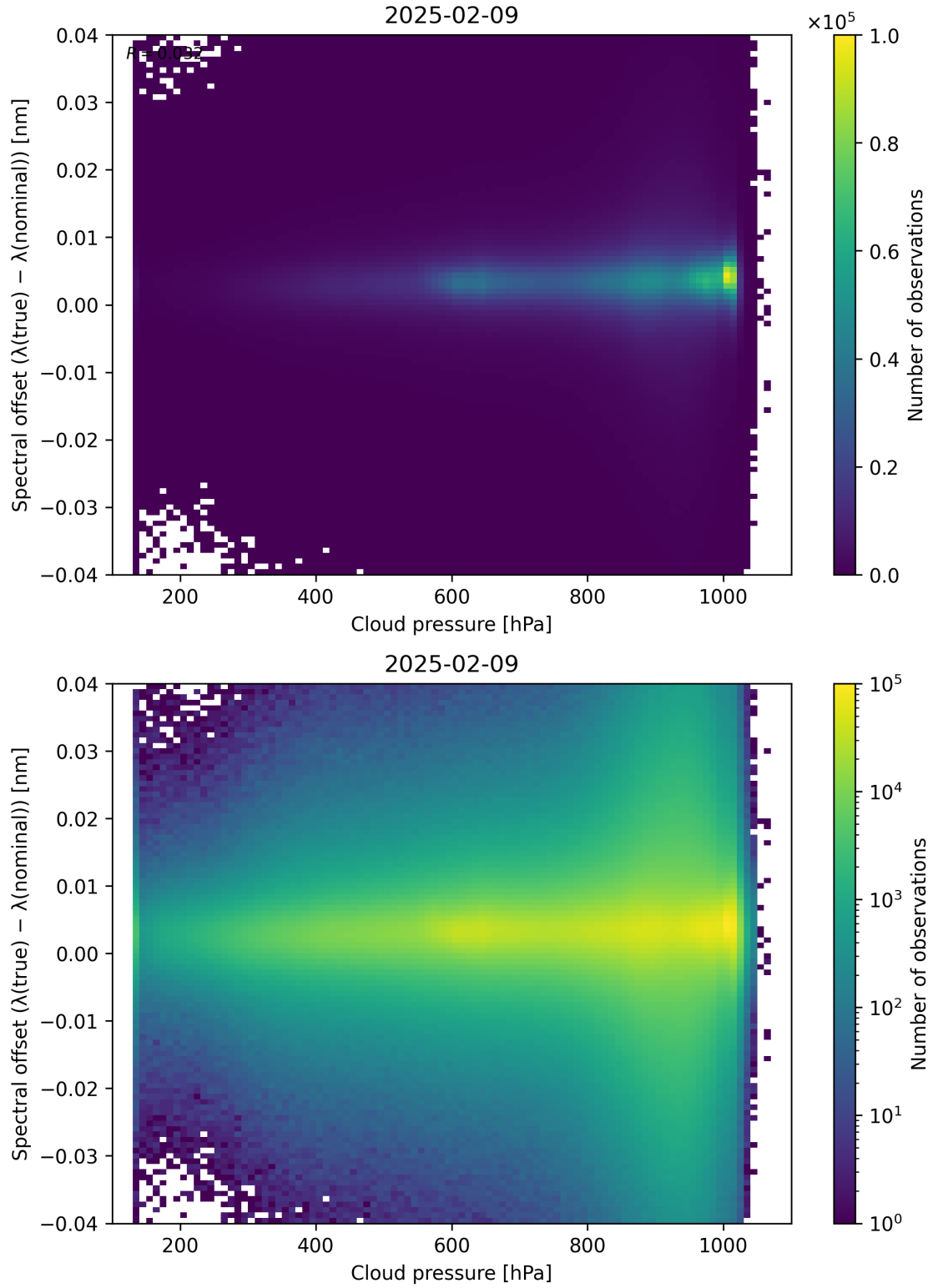
Figure 84: Scatter density plot of “Cloud pressure” against “Spectral offset ( \lambda_{\text{true}} - \lambda_{\text{nominal}} )” for 2025-02-08 to 2025-02-10.
