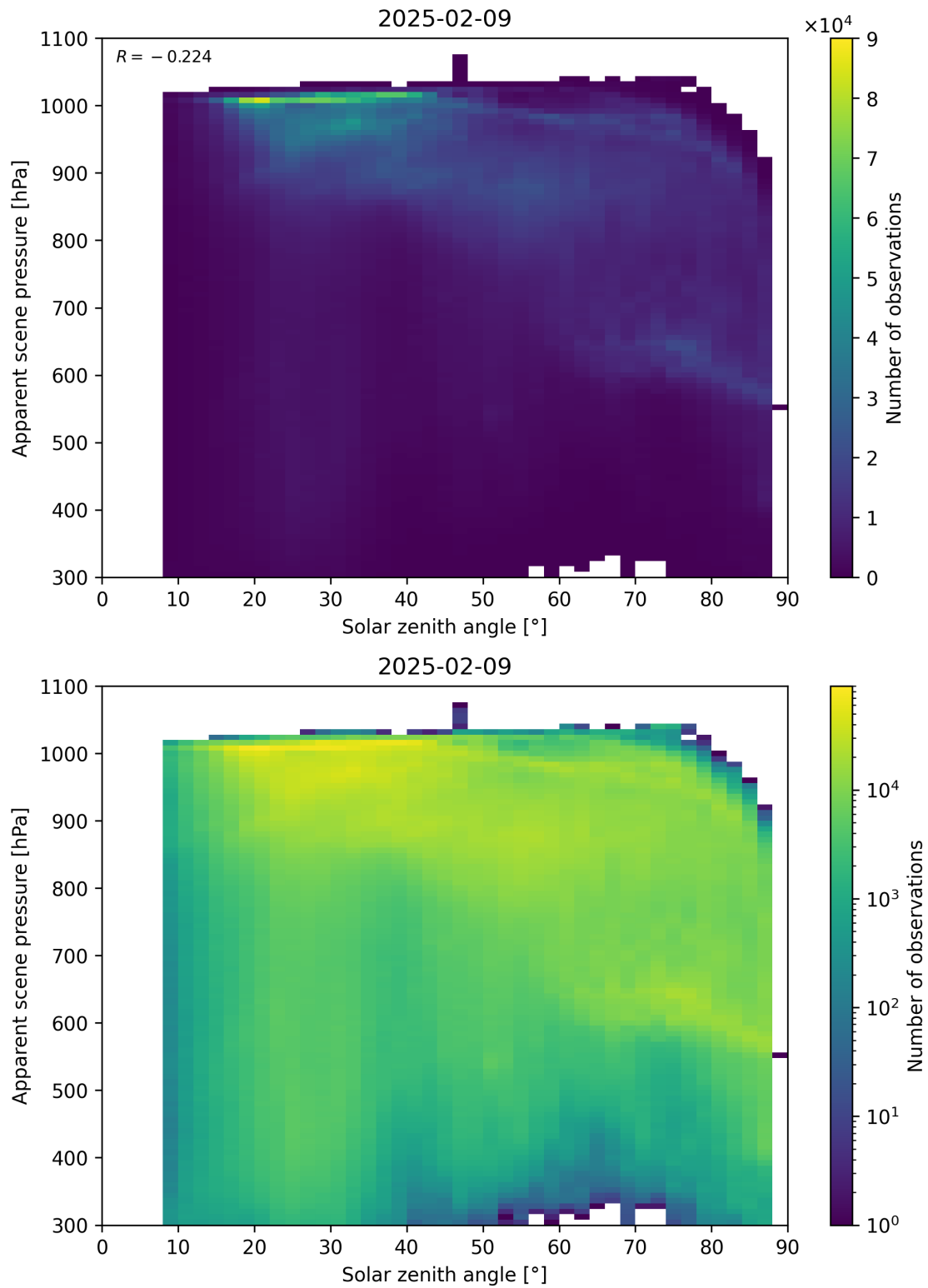
Figure 108: Scatter density plot of “Solar zenith angle” against “Apparent scene pressure” for 2025-02-08 to 2025-02-10.
