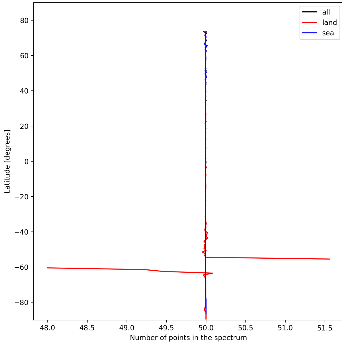
Figure 27: Zonal average of “Number of points in the spectrum” for 2025-02-08 to 2025-02-10.
