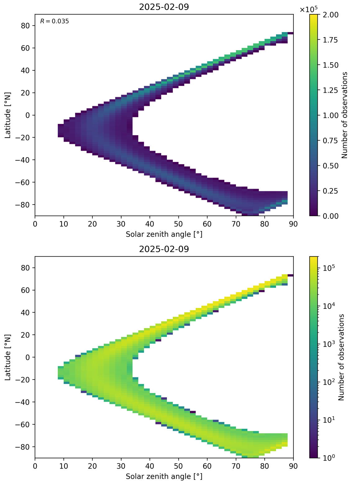
Figure 113: Scatter density plot of “Solar zenith angle” against “Latitude” for 2025-02-08 to 2025-02-10.
