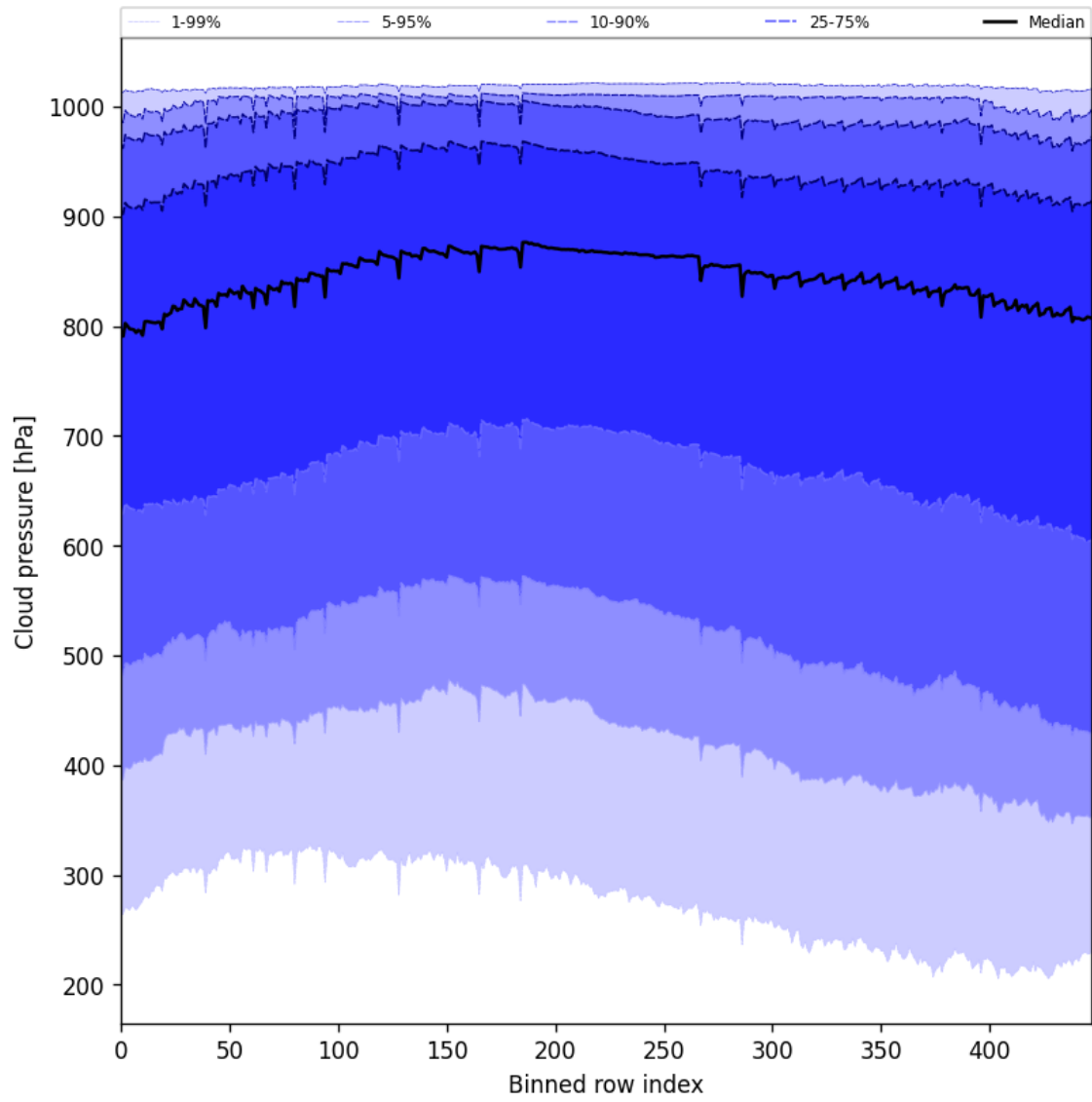
Figure 47: Along track statistics of "Cloud pressure" for 2025-02-08 to 2025-02-10
