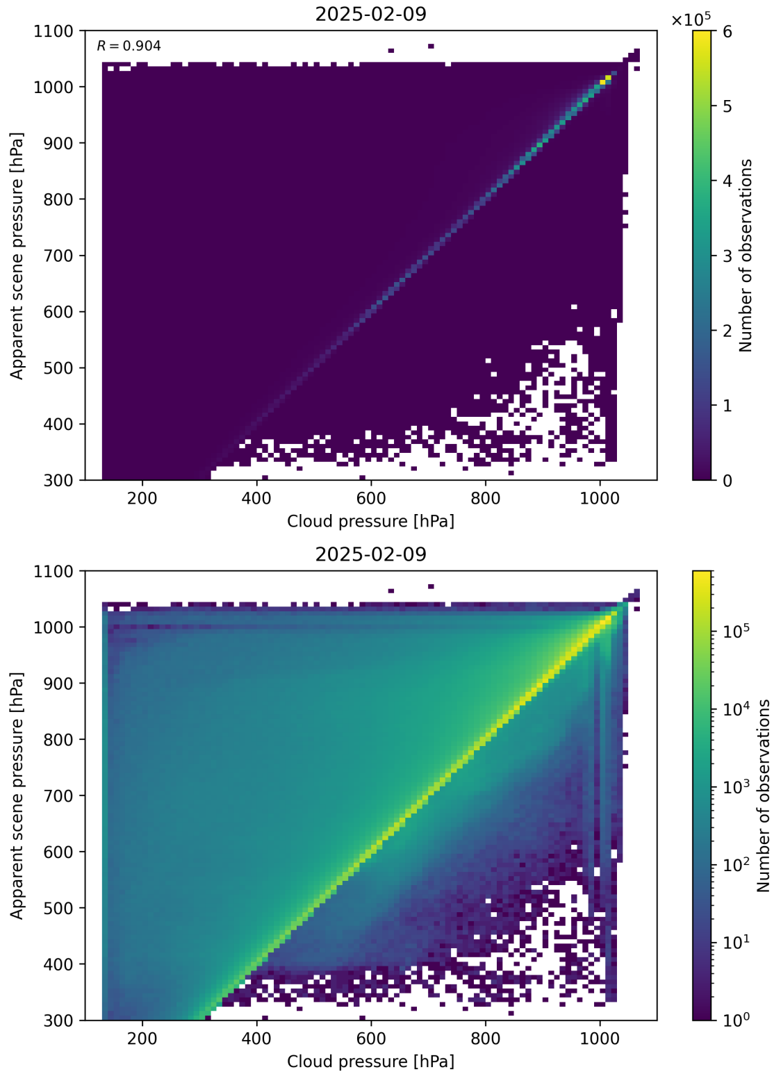
Figure 77: Scatter density plot of “Cloud pressure” against “Apparent scene pressure” for 2025-02-08 to 2025-02-10.
