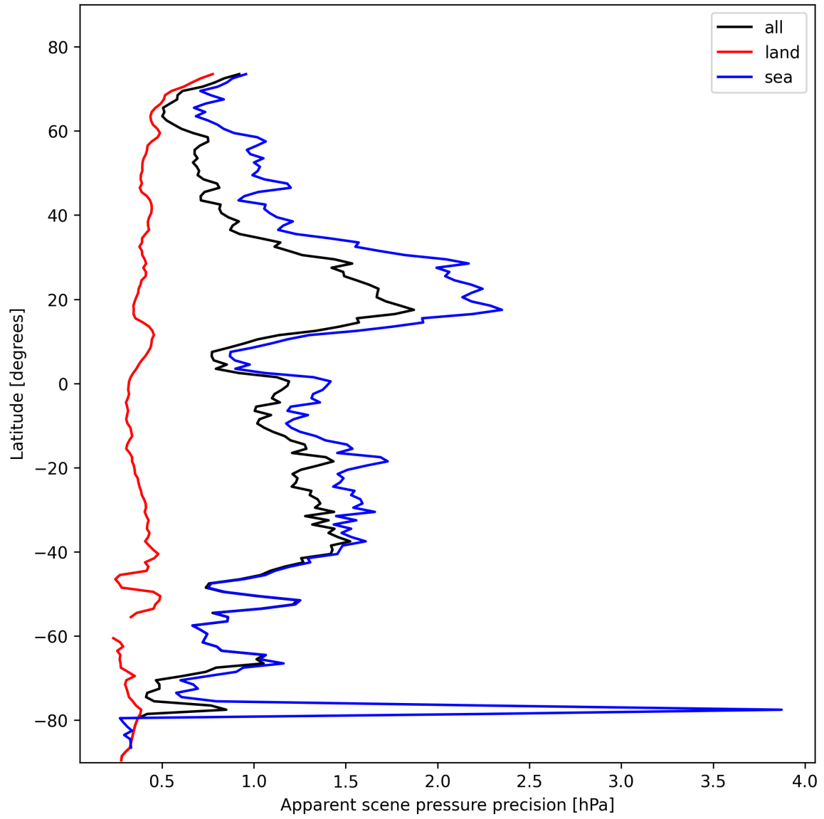
Figure 20: Zonal average of “Apparent scene pressure precision” for 2025-02-08 to 2025-02-10.
