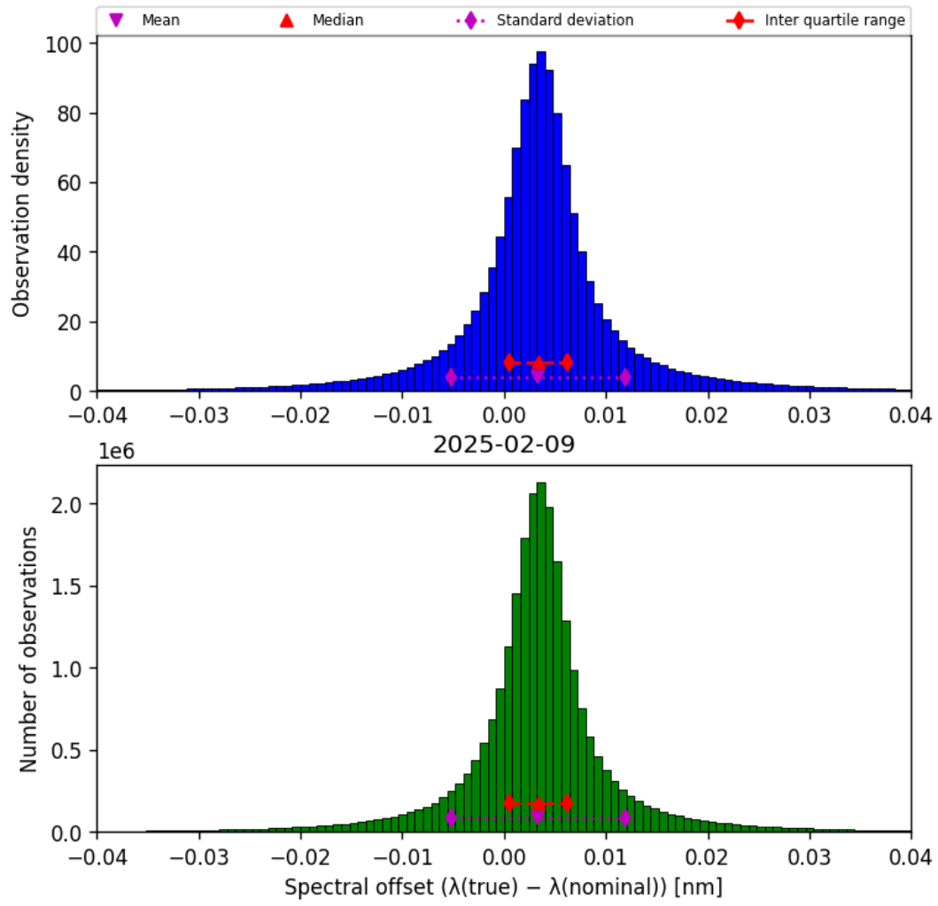
Figure 45: Histogram of “Spectral offset ( \lambda_{\text{true}} - \lambda_{\text{nominal}} )” for 2025-02-08 to 2025-02-10
