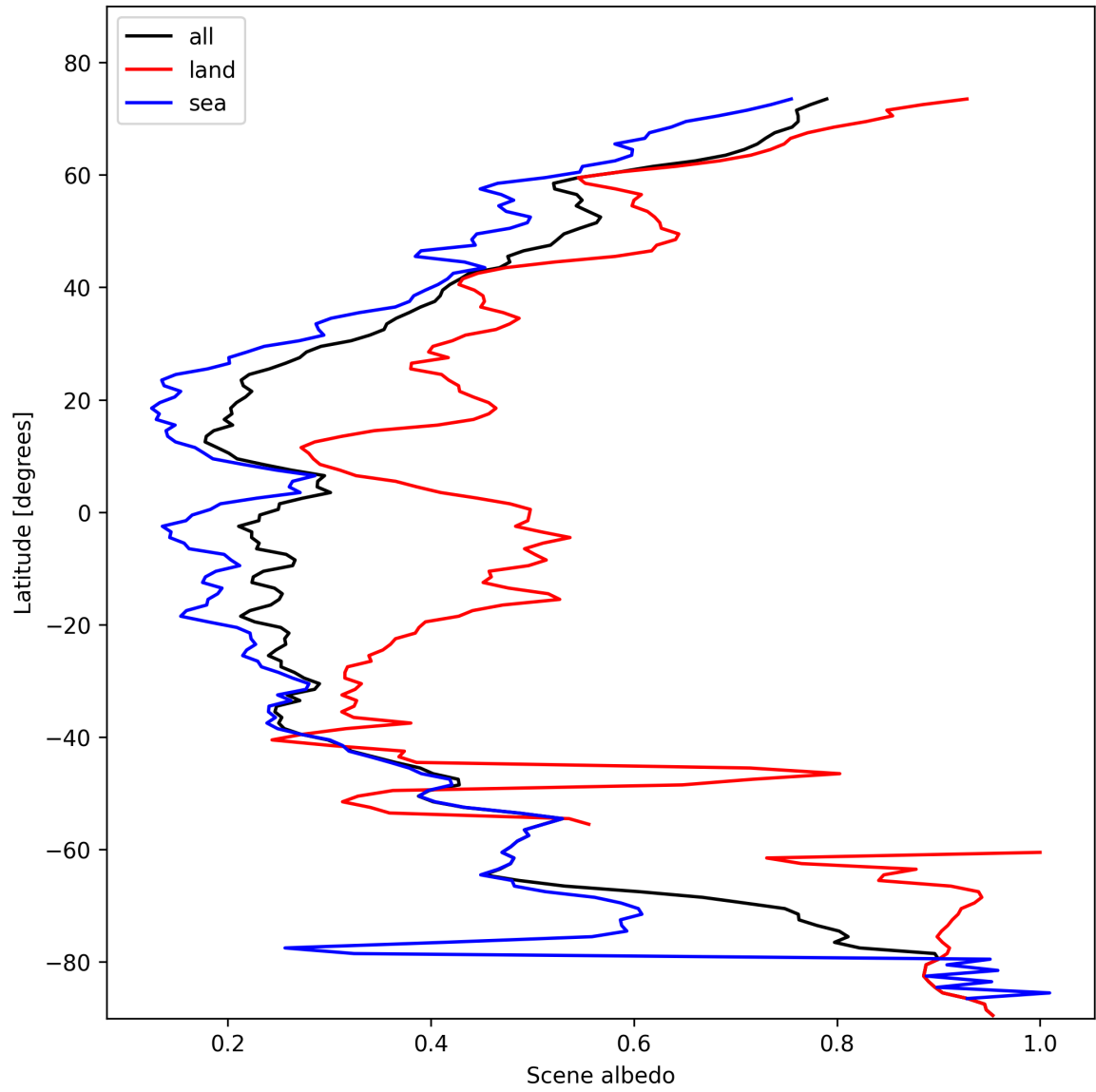
Figure 17: Zonal average of “Scene albedo” for 2025-02-08 to 2025-02-10.
