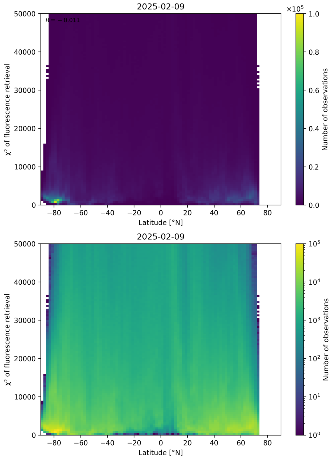
Figure 89: Scatter density plot of “Latitude” against “ \chi^2 of fluorescence retrieval” for 2025-02-08 to 2025-02-10.
