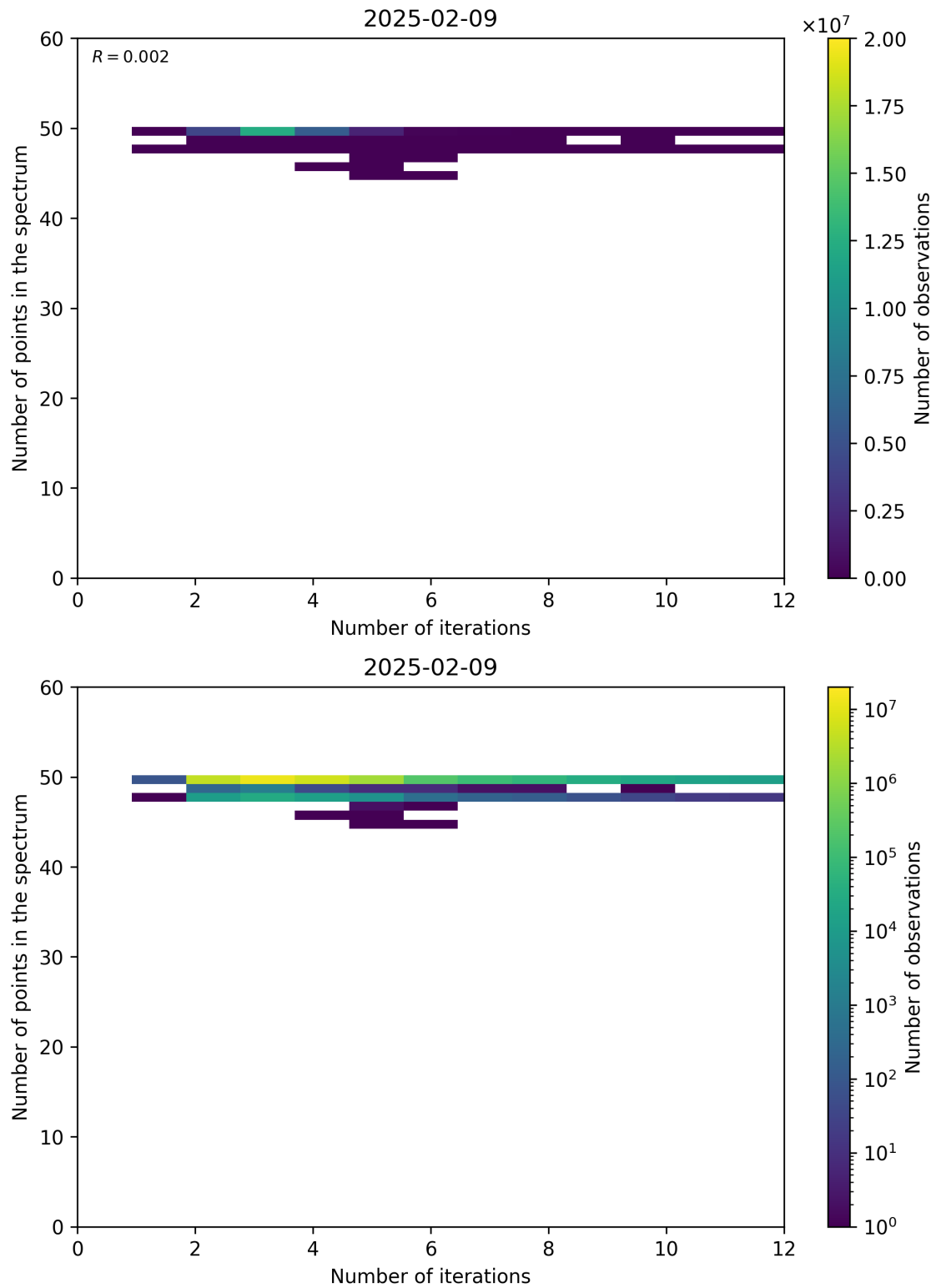
Figure 99: Scatter density plot of “Number of iterations” against “Number of points in the spectrum” for 2025-02-08 to 2025-02-10.
