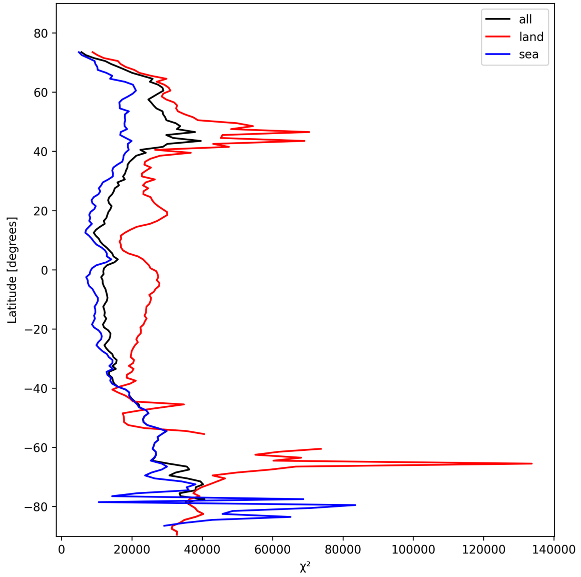
Figure 21: Zonal average of “ \chi^2 ” for 2025-02-08 to 2025-02-10.
