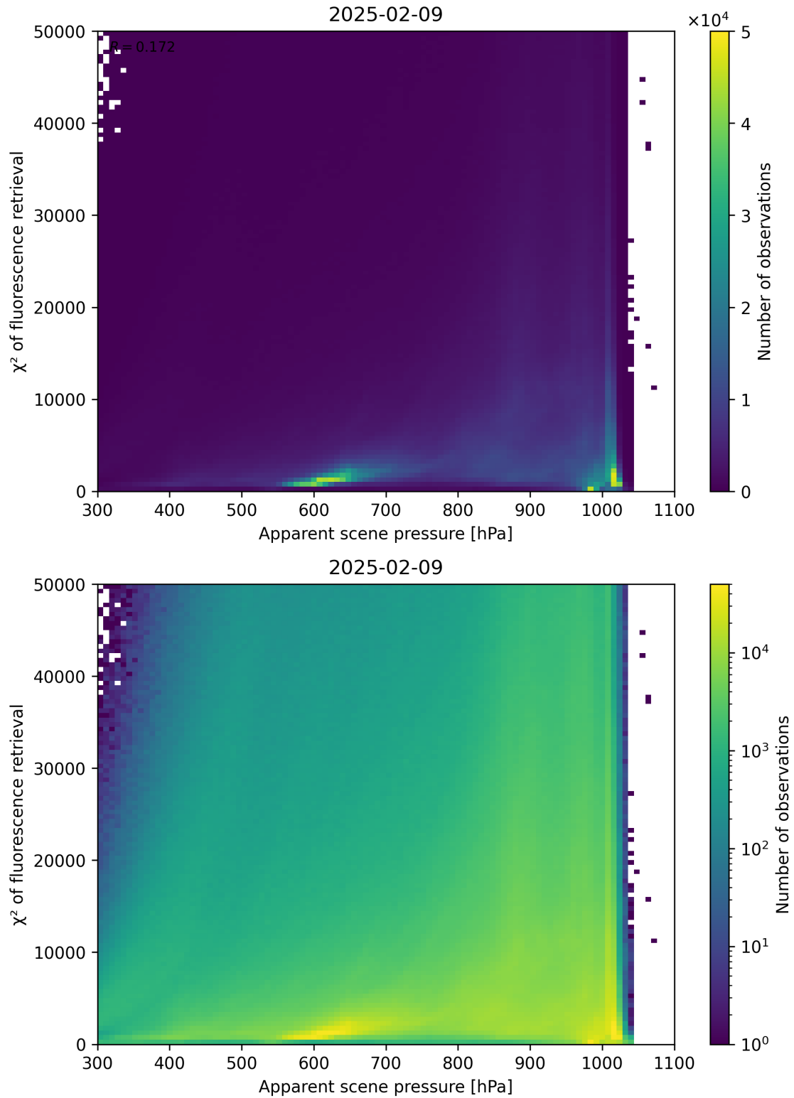
Figure 63: Scatter density plot of “Apparent scene pressure” against “ \chi^2 of fluorescence retrieval” for 2025-02-08 to 2025-02-10.
