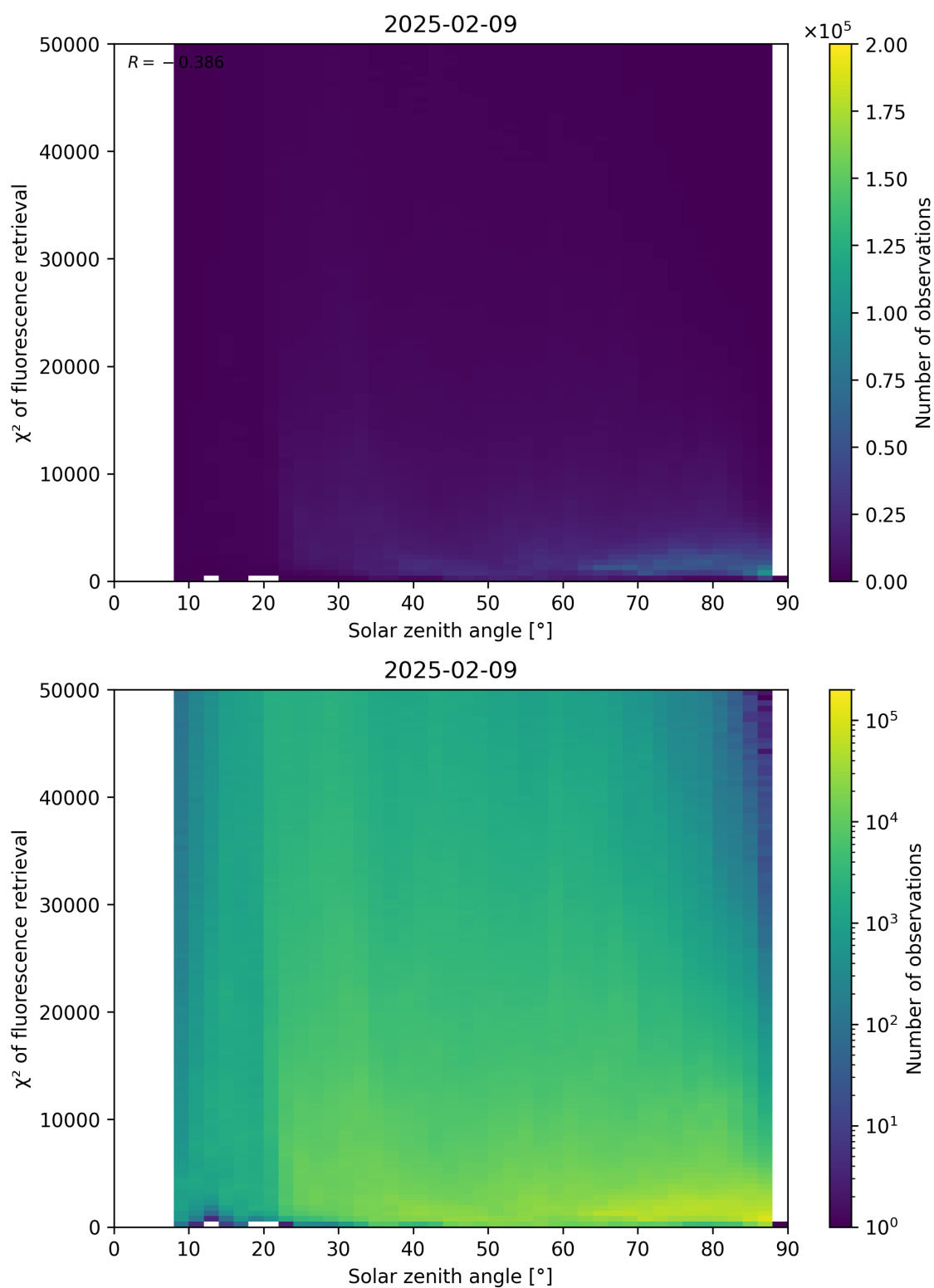
Figure 109: Scatter density plot of “Solar zenith angle” against “ \chi^2 of fluorescence retrieval” for 2025-02-08 to 2025-02-10.
