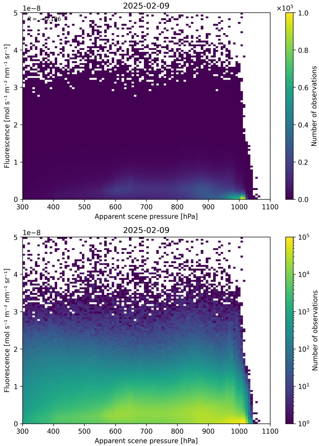
Figure 64: Scatter density plot of “Apparent scene pressure” against “Fluorescence” for 2025-02-08 to 2025-02-10.
