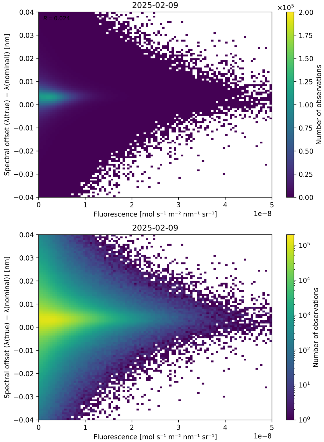
Figure 87: Scatter density plot of “Fluorescence” against “Spectral offset ( \lambda_{\text{true}} - \lambda_{\text{nominal}} )” for 2025-02-08 to 2025-02-10.
