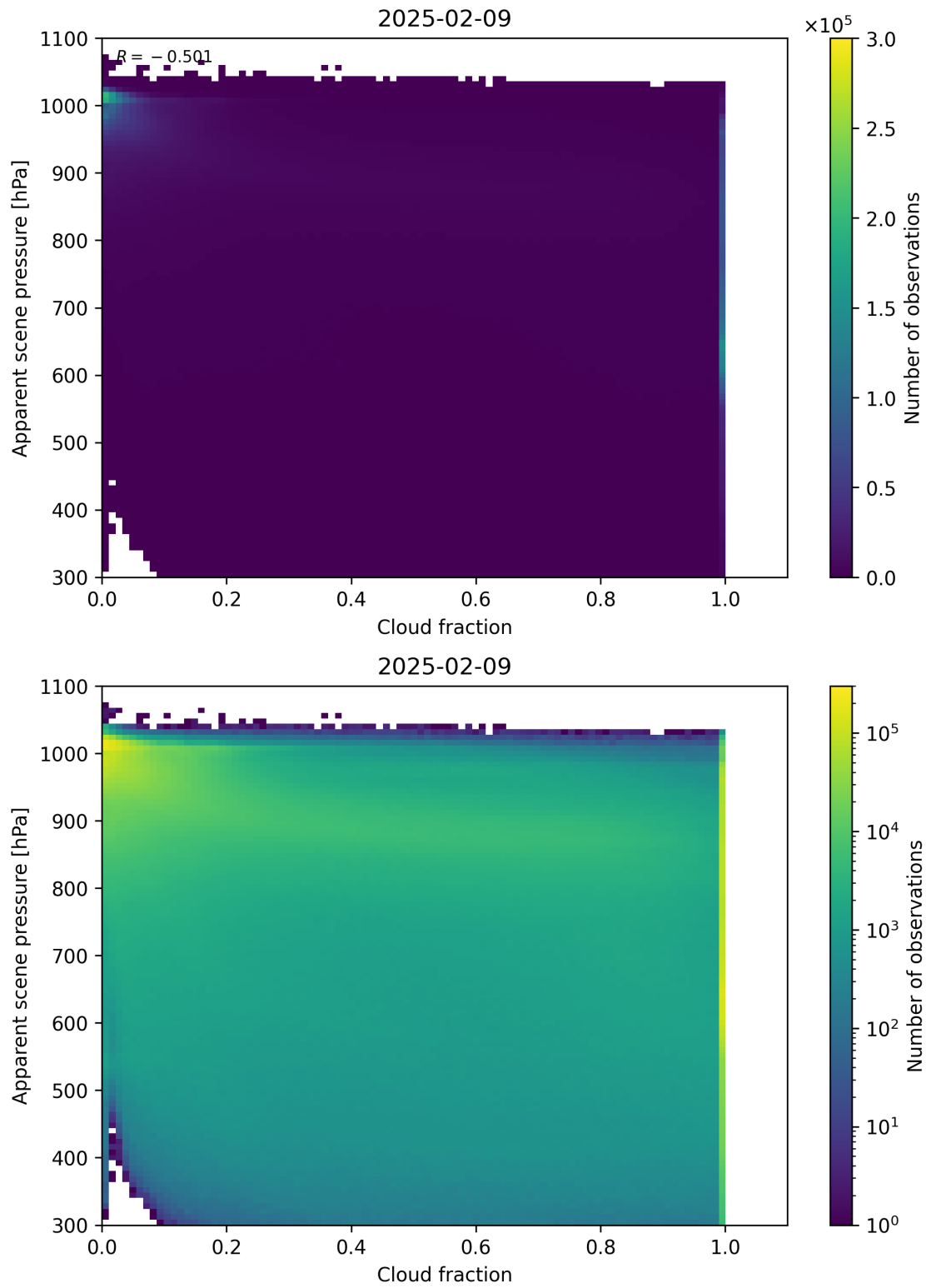
Figure 70: Scatter density plot of “Cloud fraction” against “Apparent scene pressure” for 2025-02-08 to 2025-02-10.
