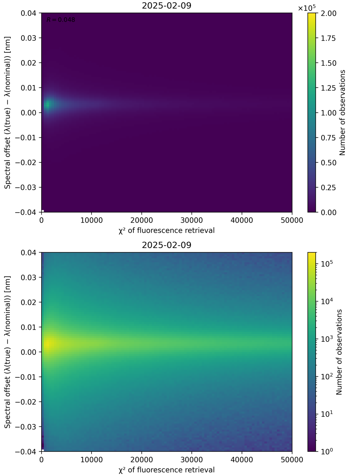
Figure 69: Scatter density plot of “ \chi^2 of fluorescence retrieval” against “Spectral offset ( \lambda_{\text{true}} - \lambda_{\text{nominal}} )” for 2025-02-08 to 2025-02-10.
