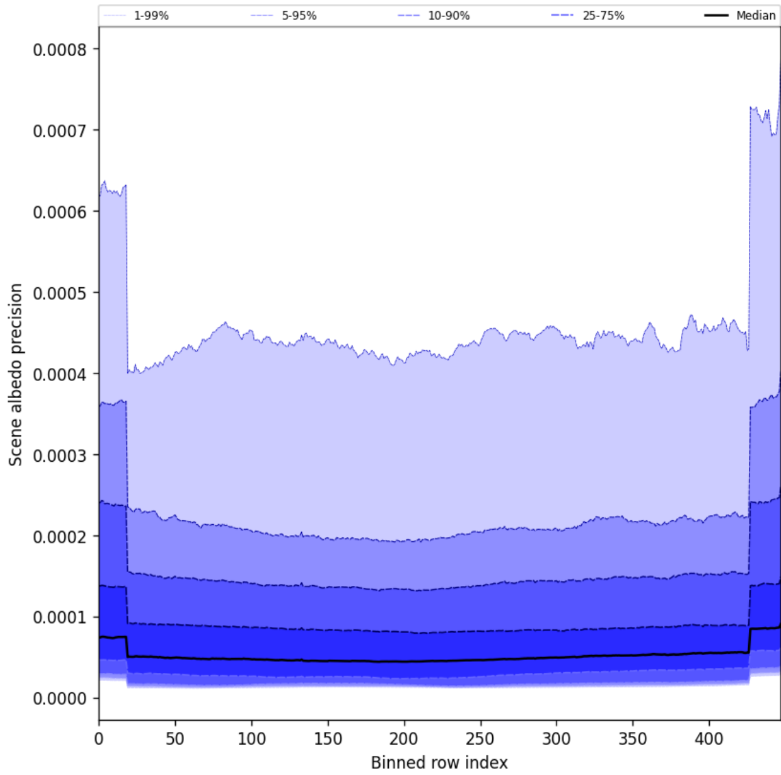
Figure 52: Along track statistics of “Scene albedo precision” for 2025-02-08 to 2025-02-10
