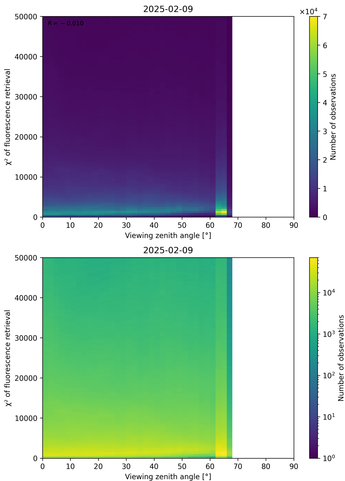
Figure 119: Scatter density plot of “Viewing zenith angle” against “ \chi^2 of fluorescence retrieval” for 2025-02-08 to 2025-02-10.
