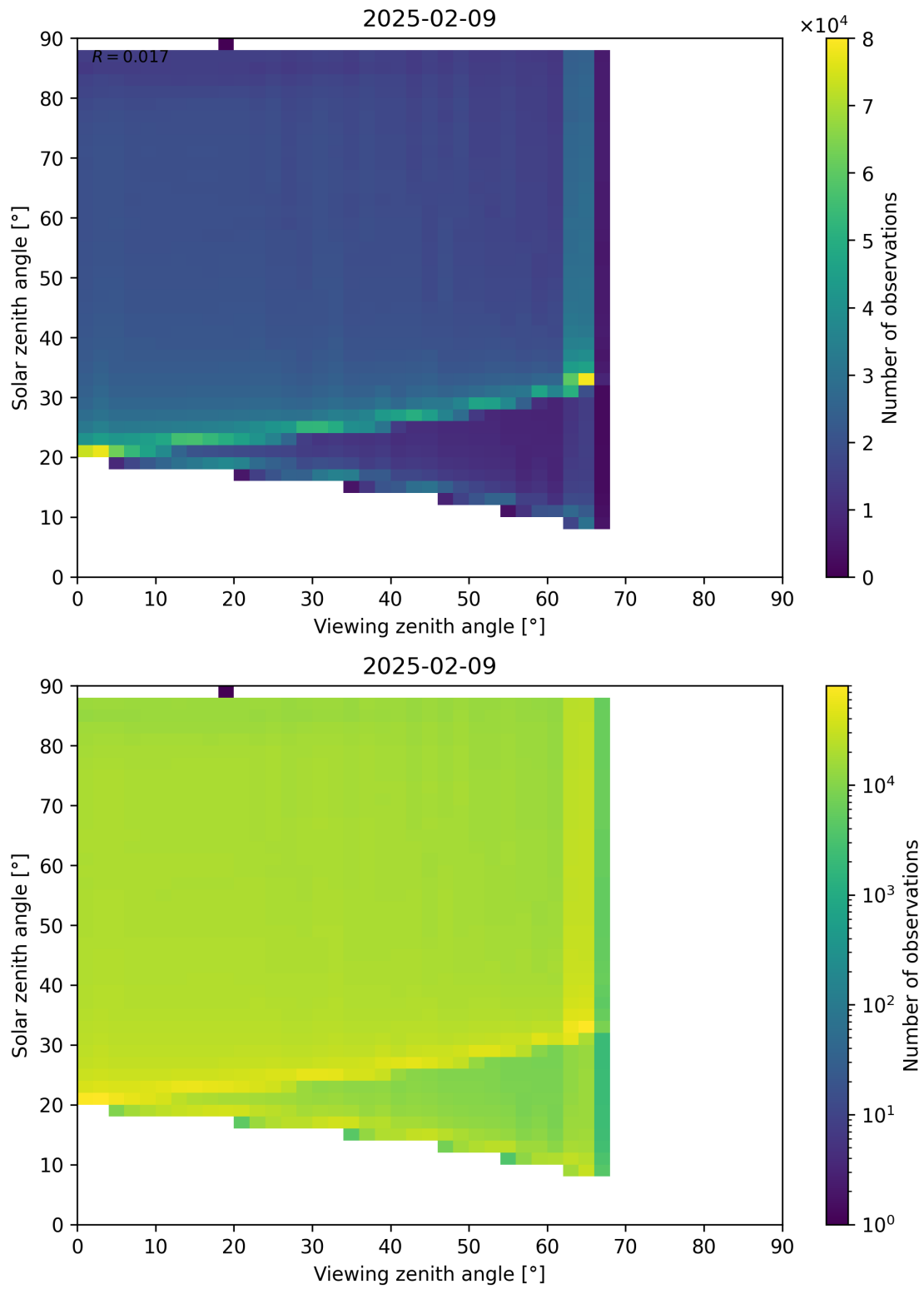
Figure 127: Scatter density plot of “Viewing zenith angle” against “Solar zenith angle” for 2025-02-08 to 2025-02-10.
