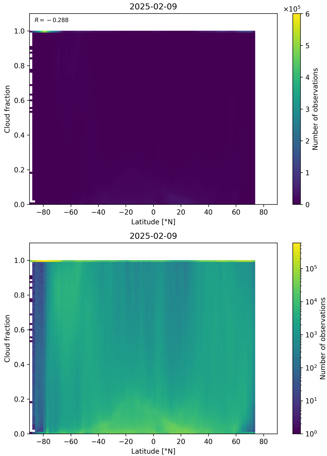
Figure 90: Scatter density plot of “Latitude” against “Cloud fraction” for 2025-02-08 to 2025-02-10.
