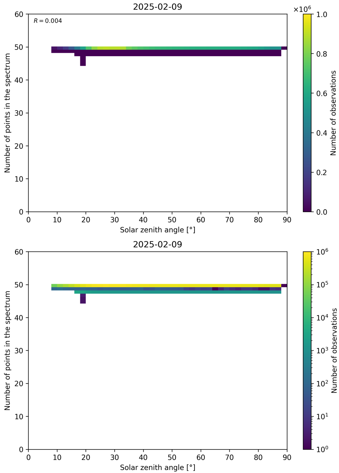
Figure 115: Scatter density plot of “Solar zenith angle” against “Number of points in the spectrum” for 2025-02-08 to 2025-02-10.
