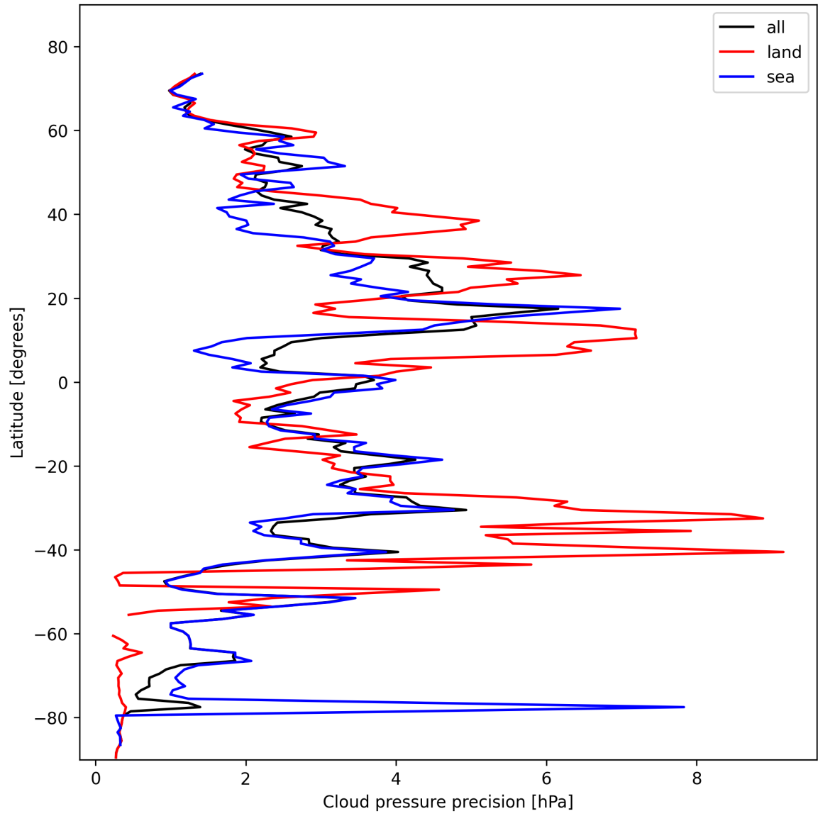
Figure 14: Zonal average of “Cloud pressure precision” for 2025-02-08 to 2025-02-10.
