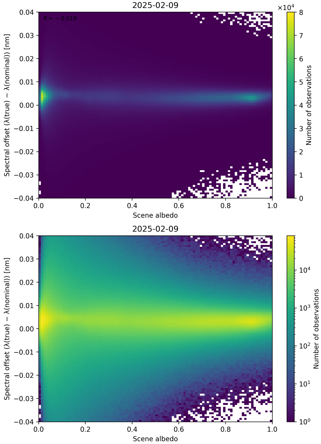
Figure 107: Scatter density plot of “Scene albedo” against “Spectral offset ( \lambda_{\text{true}} - \lambda_{\text{nominal}} )” for 2025-02-08 to 2025-02-10.
