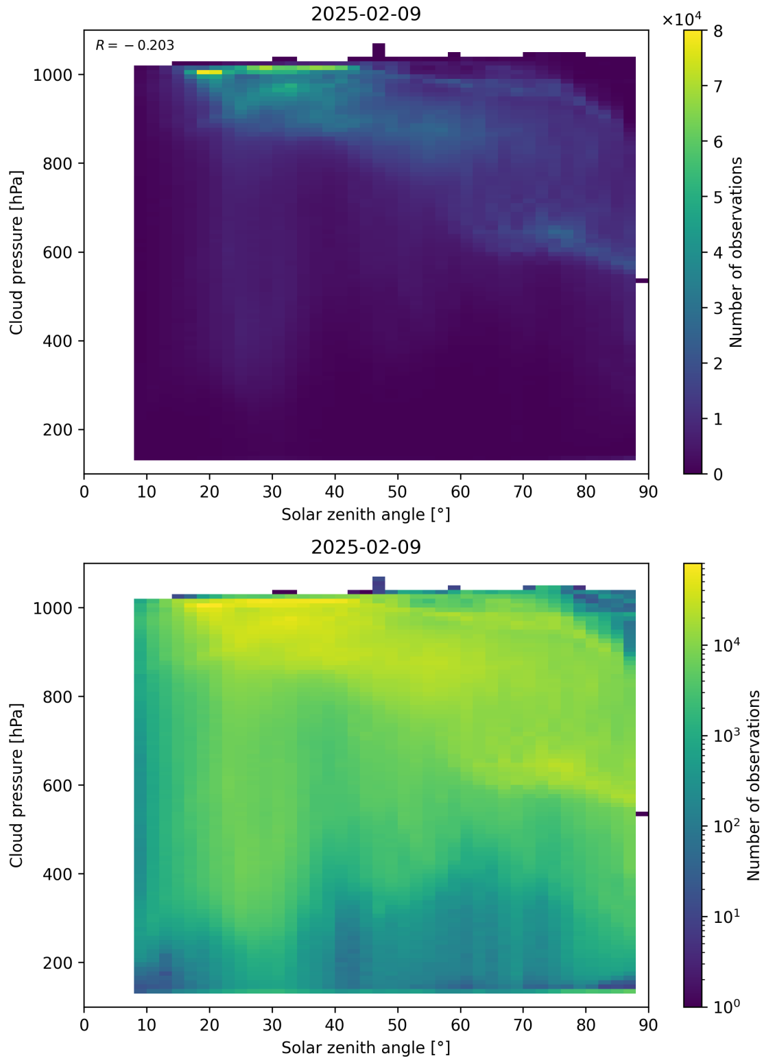
Figure 111: Scatter density plot of “Solar zenith angle” against “Cloud pressure” for 2025-02-08 to 2025-02-10.
