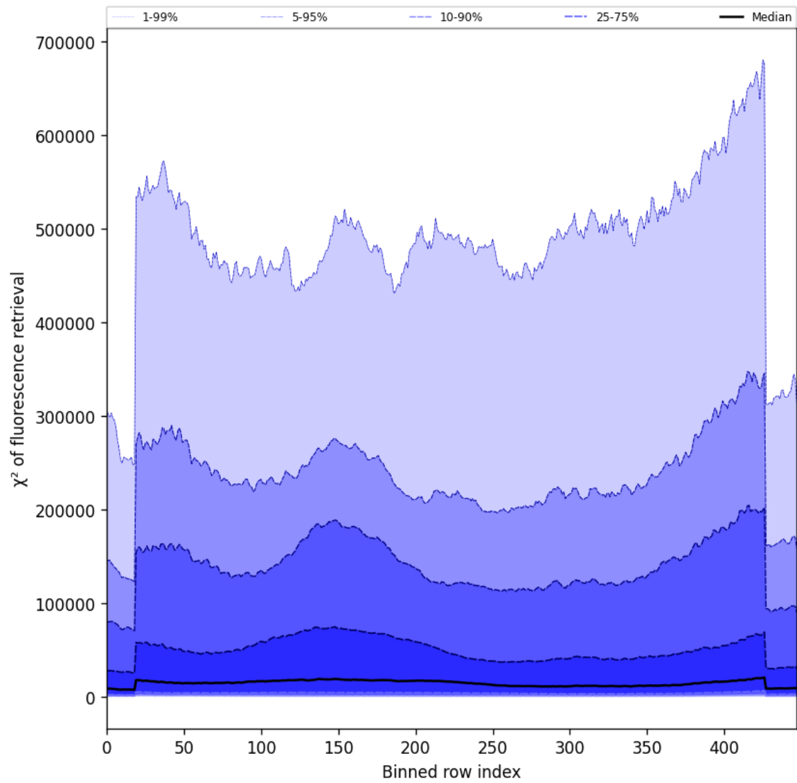
Figure 59: Along track statistics of “ \chi^2 of fluorescence retrieval” for 2025-02-09 to 2025-02-11
