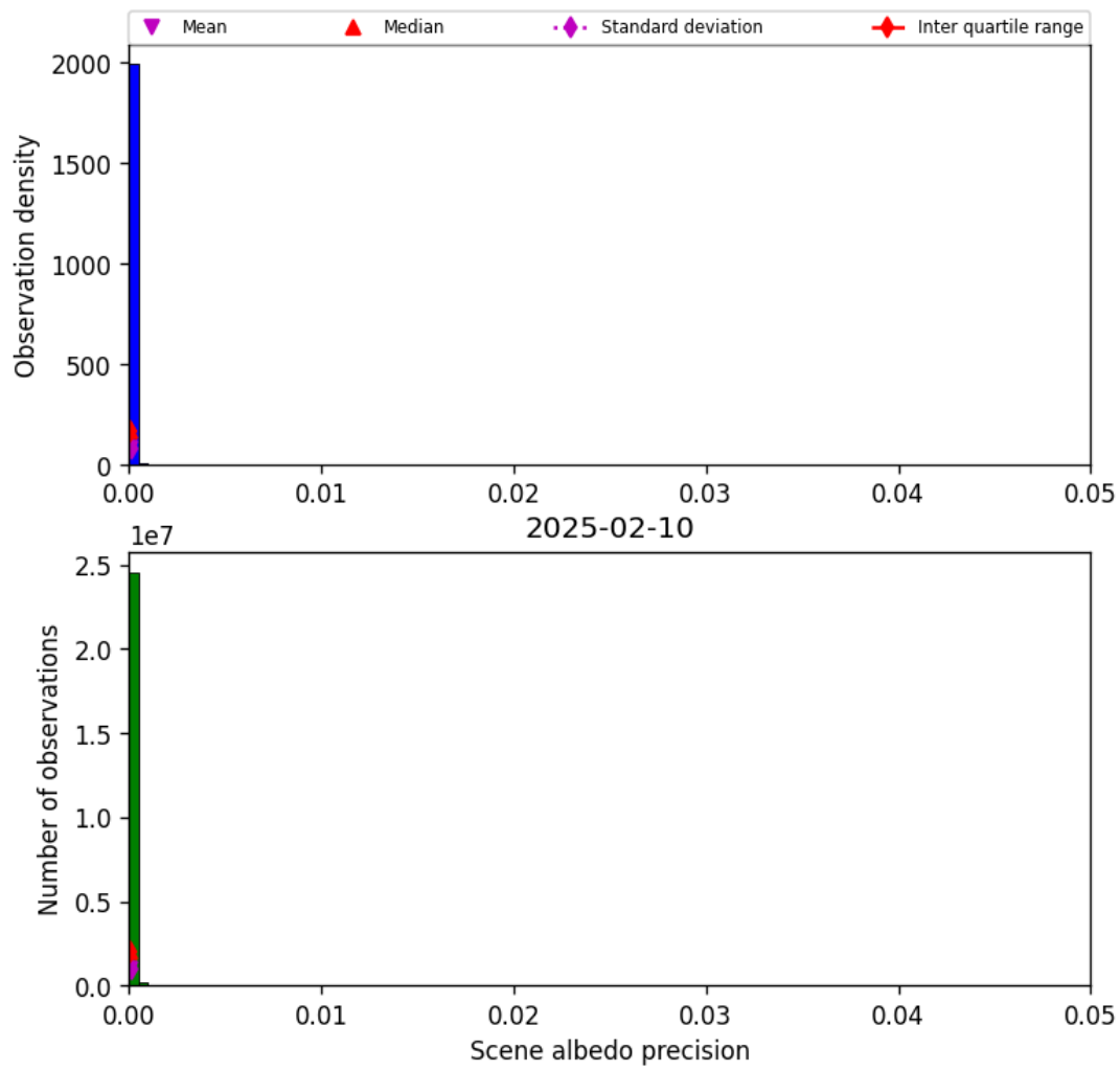
Figure 35: Histogram of “Scene albedo precision” for 2025-02-09 to 2025-02-11
