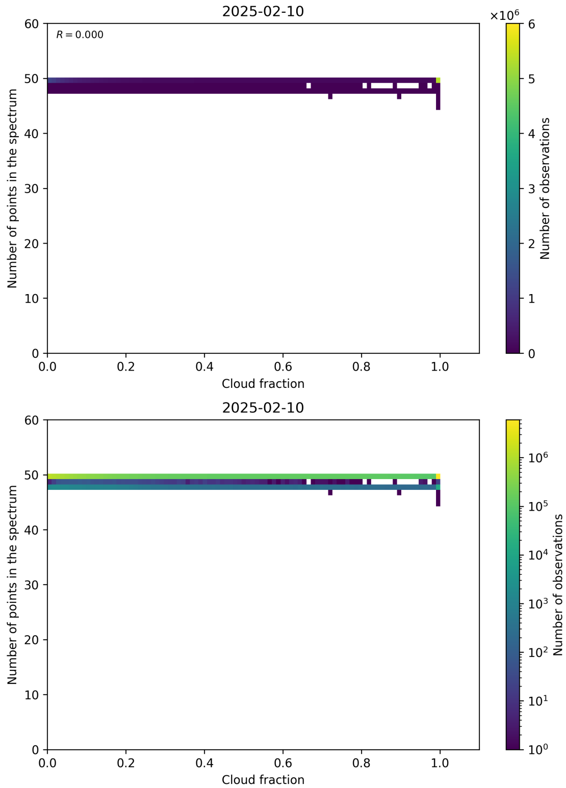
Figure 74: Scatter density plot of “Cloud fraction” against “Number of points in the spectrum” for 2025-02-09 to 2025-02-11.
