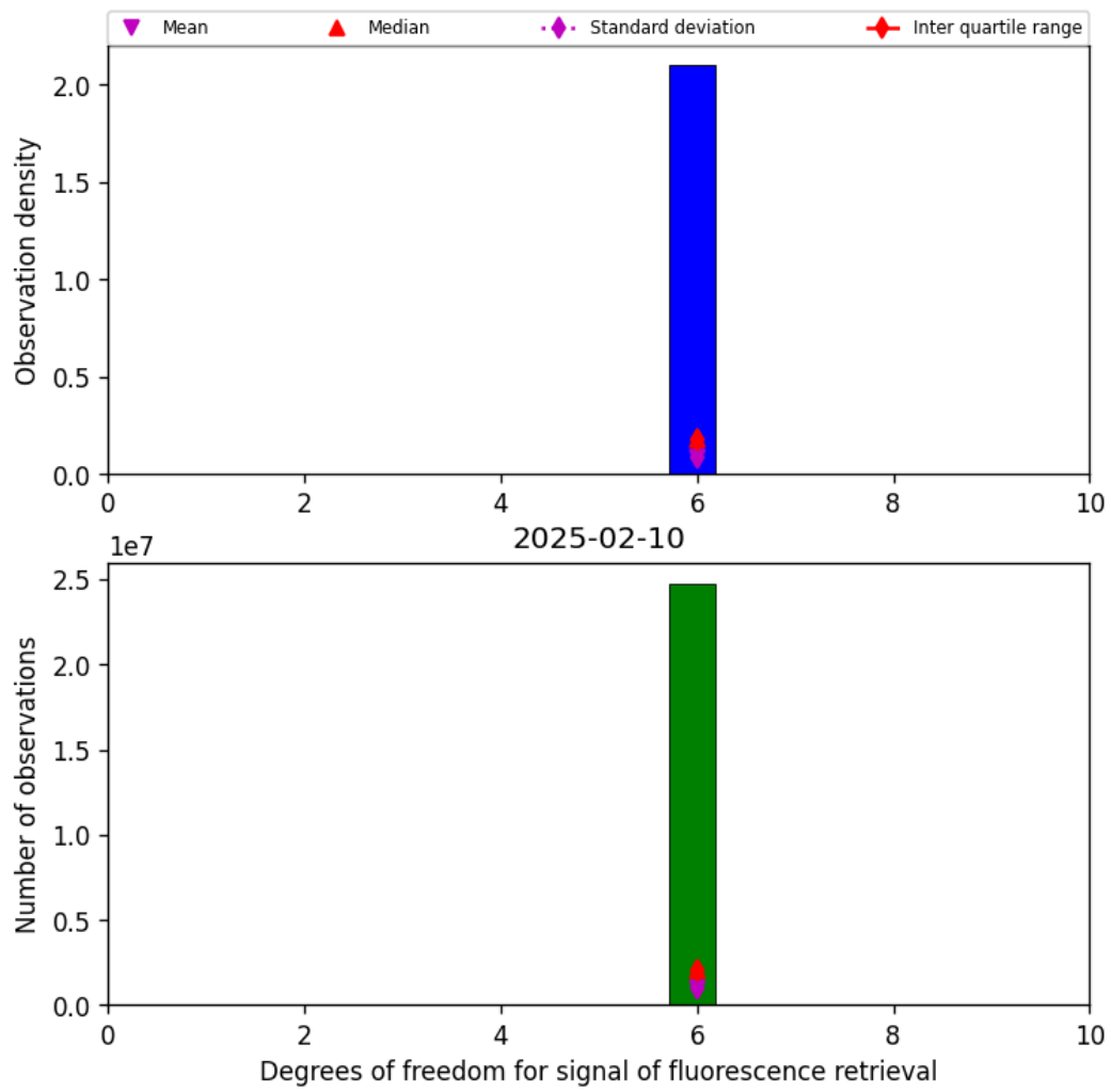
Figure 43: Histogram of "Degrees of freedom for signal of fluorescence retrieval" for 2025-02-09 to 2025-02-11
