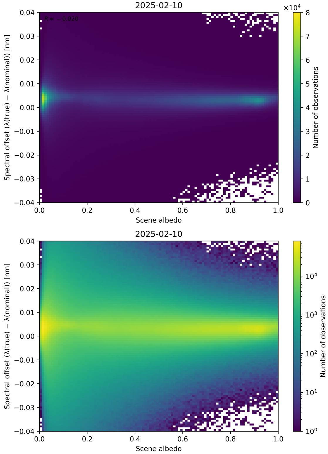
Figure 107: Scatter density plot of “Scene albedo” against “Spectral offset ( \lambda_{\text{true}} - \lambda_{\text{nominal}} )” for 2025-02-09 to 2025-02-11.
