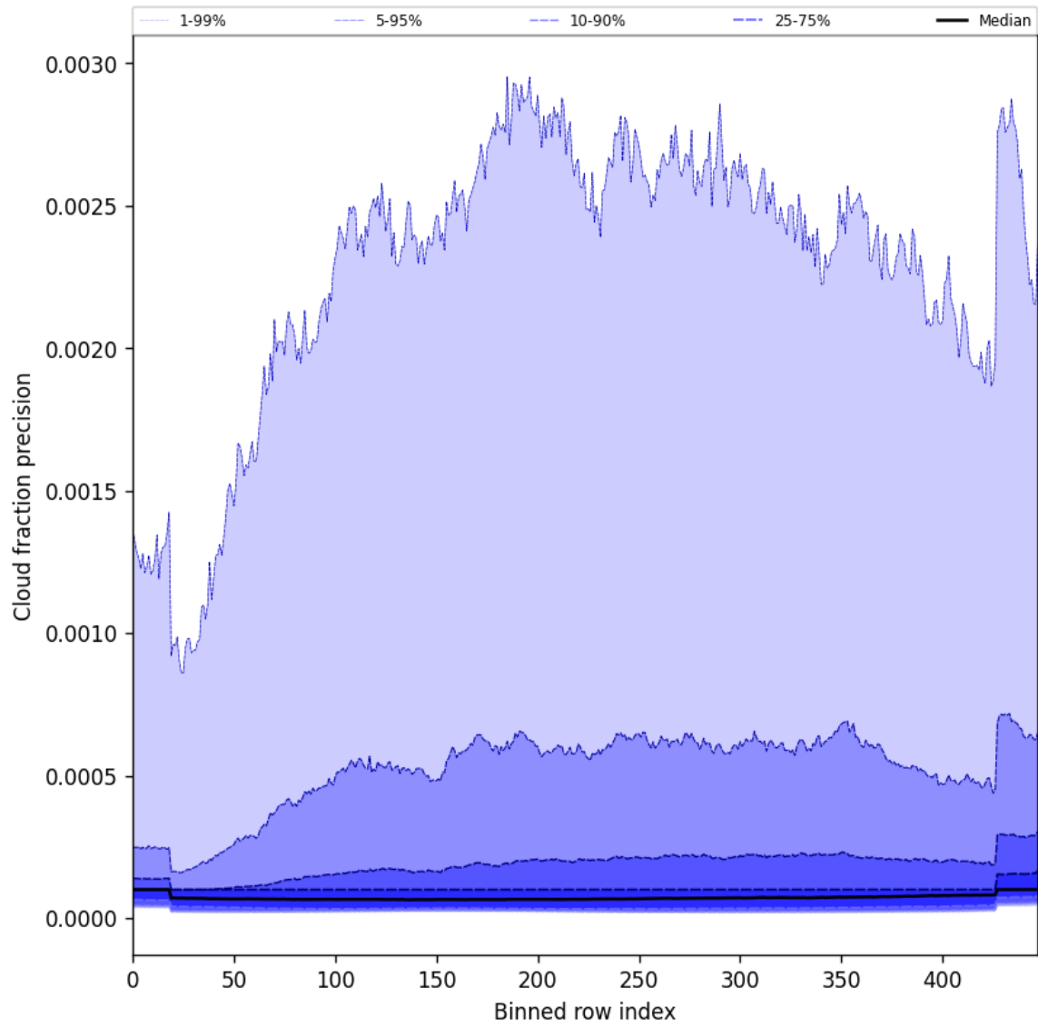
Figure 50: Along track statistics of “Cloud fraction precision” for 2025-02-09 to 2025-02-11
