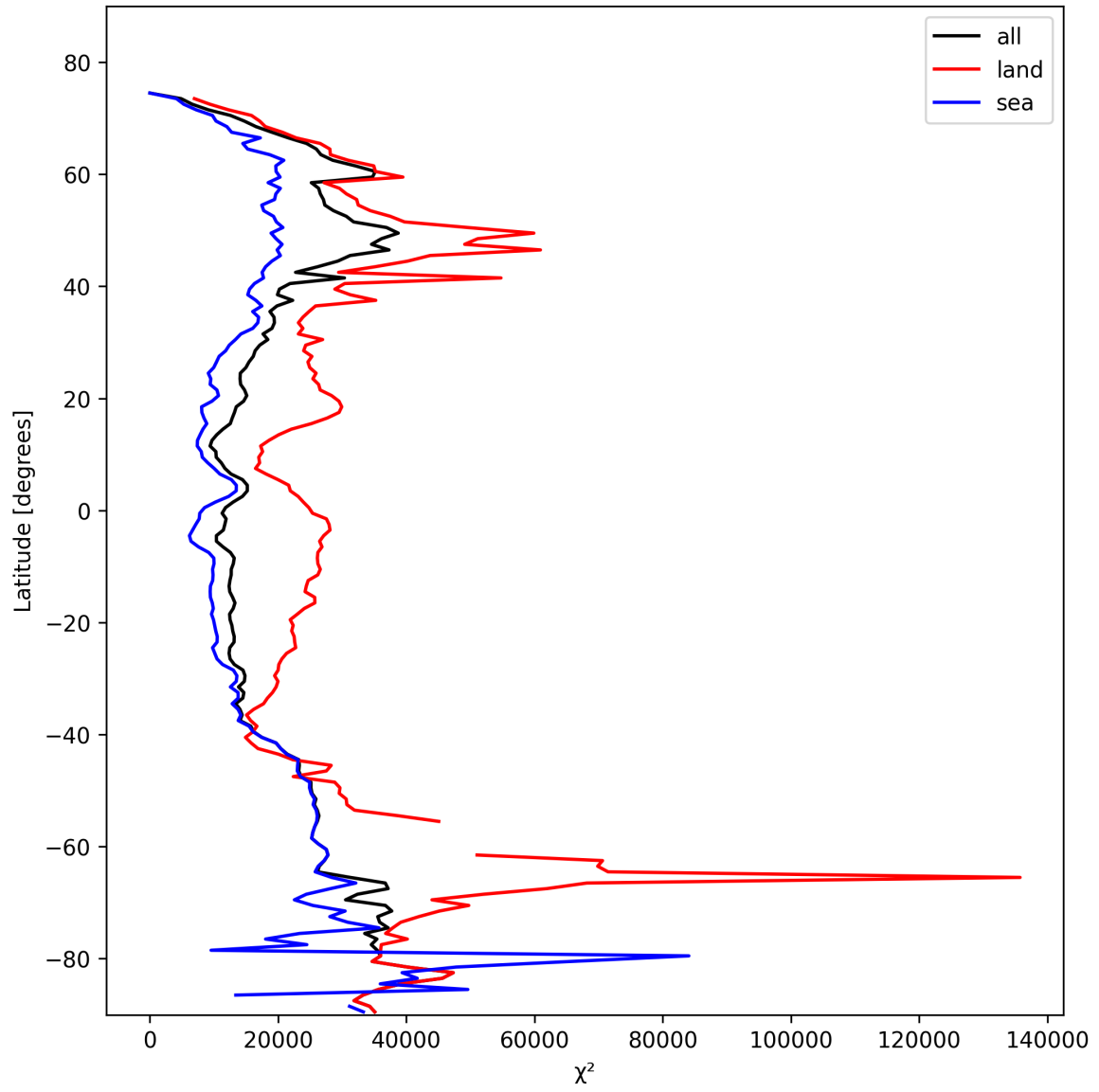
Figure 21: Zonal average of “ \chi^2 ” for 2025-02-09 to 2025-02-11.
