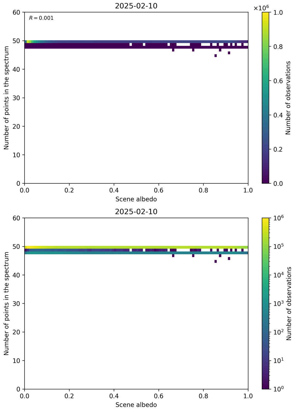
Figure 106: Scatter density plot of “Scene albedo” against “Number of points in the spectrum” for 2025-02-09 to 2025-02-11.
