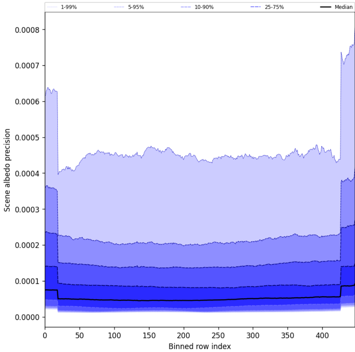
Figure 52: Along track statistics of “Scene albedo precision” for 2025-02-09 to 2025-02-11
