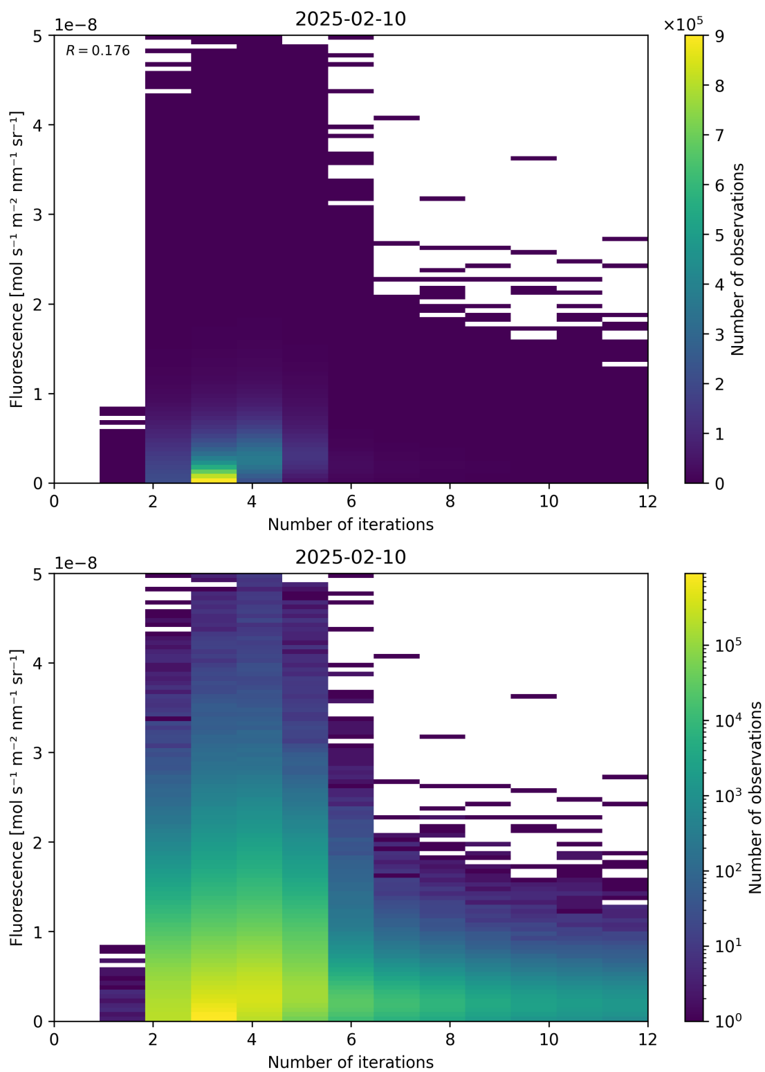
Figure 98: Scatter density plot of “Number of iterations” against “Fluorescence” for 2025-02-09 to 2025-02-11.
