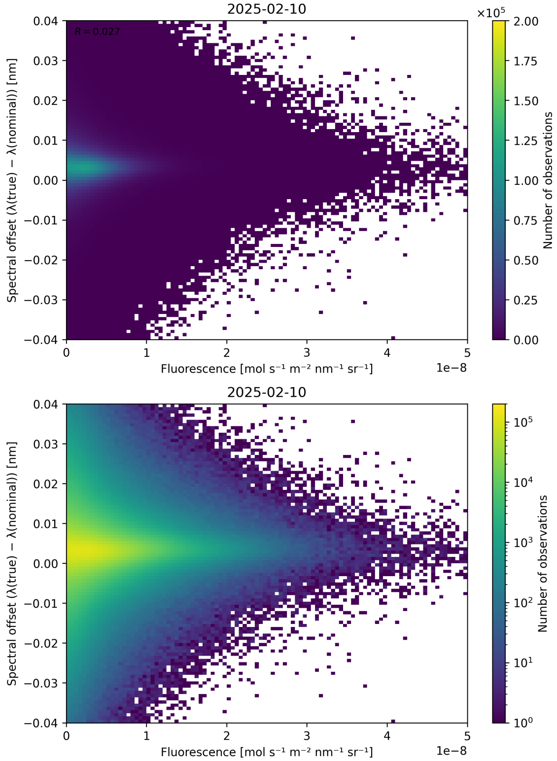
Figure 87: Scatter density plot of “Fluorescence” against “Spectral offset ( \lambda_{\text{true}} - \lambda_{\text{nominal}} )” for 2025-02-09 to 2025-02-11.
