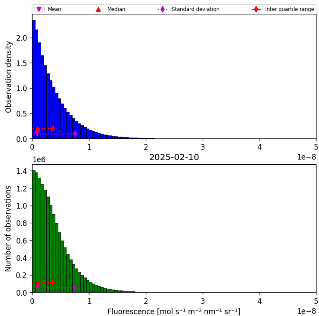
Figure 40: Histogram of “Fluorescence” for 2025-02-09 to 2025-02-11
