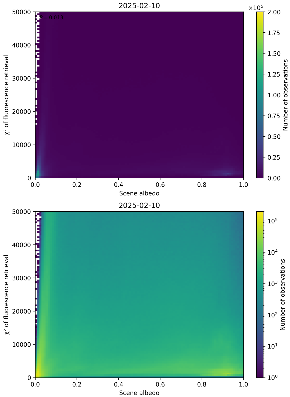
Figure 103: Scatter density plot of “Scene albedo” against “ \chi^2 of fluorescence retrieval” for 2025-02-09 to 2025-02-11.
