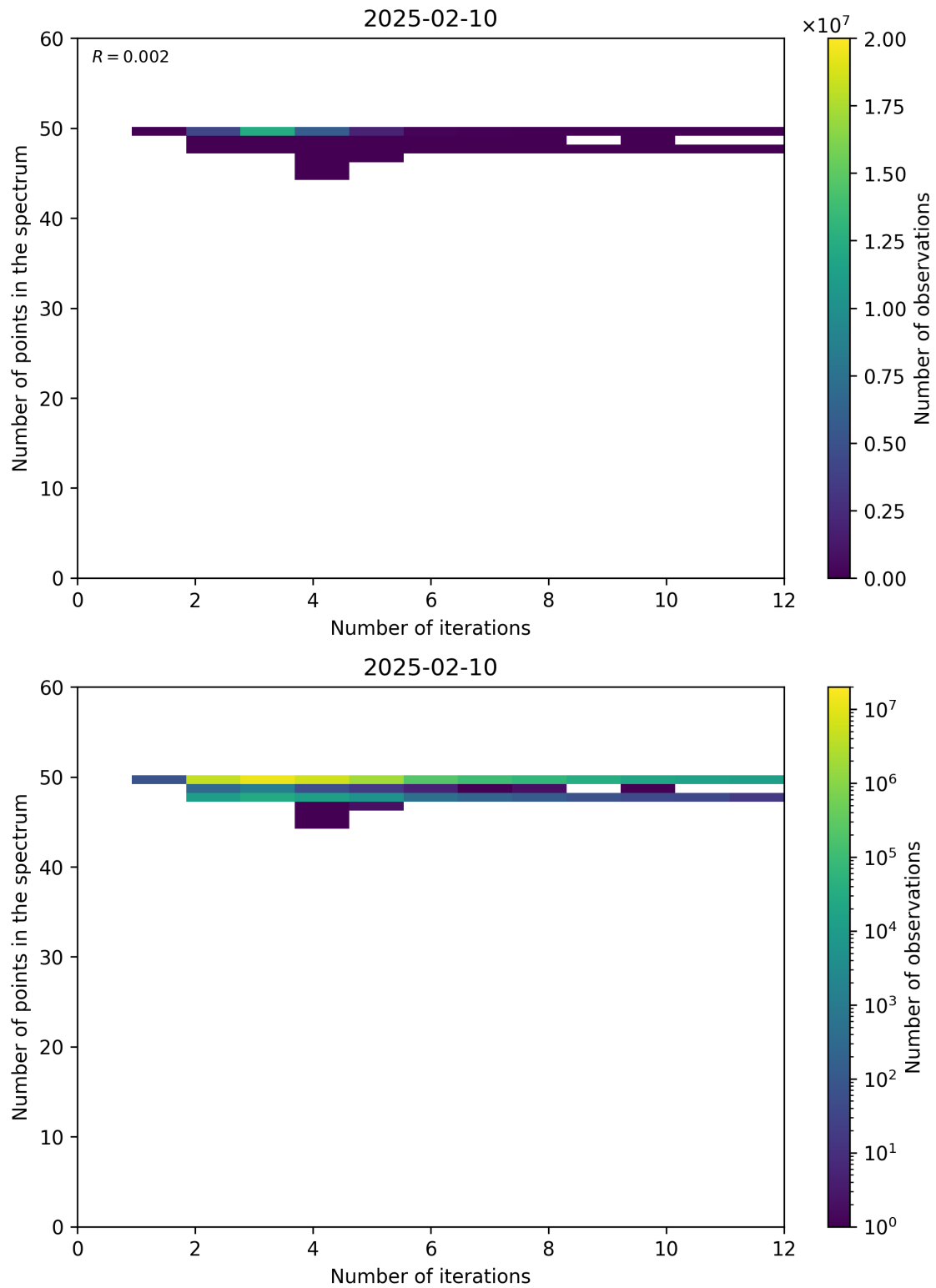
Figure 99: Scatter density plot of “Number of iterations” against “Number of points in the spectrum” for 2025-02-09 to 2025-02-11.
