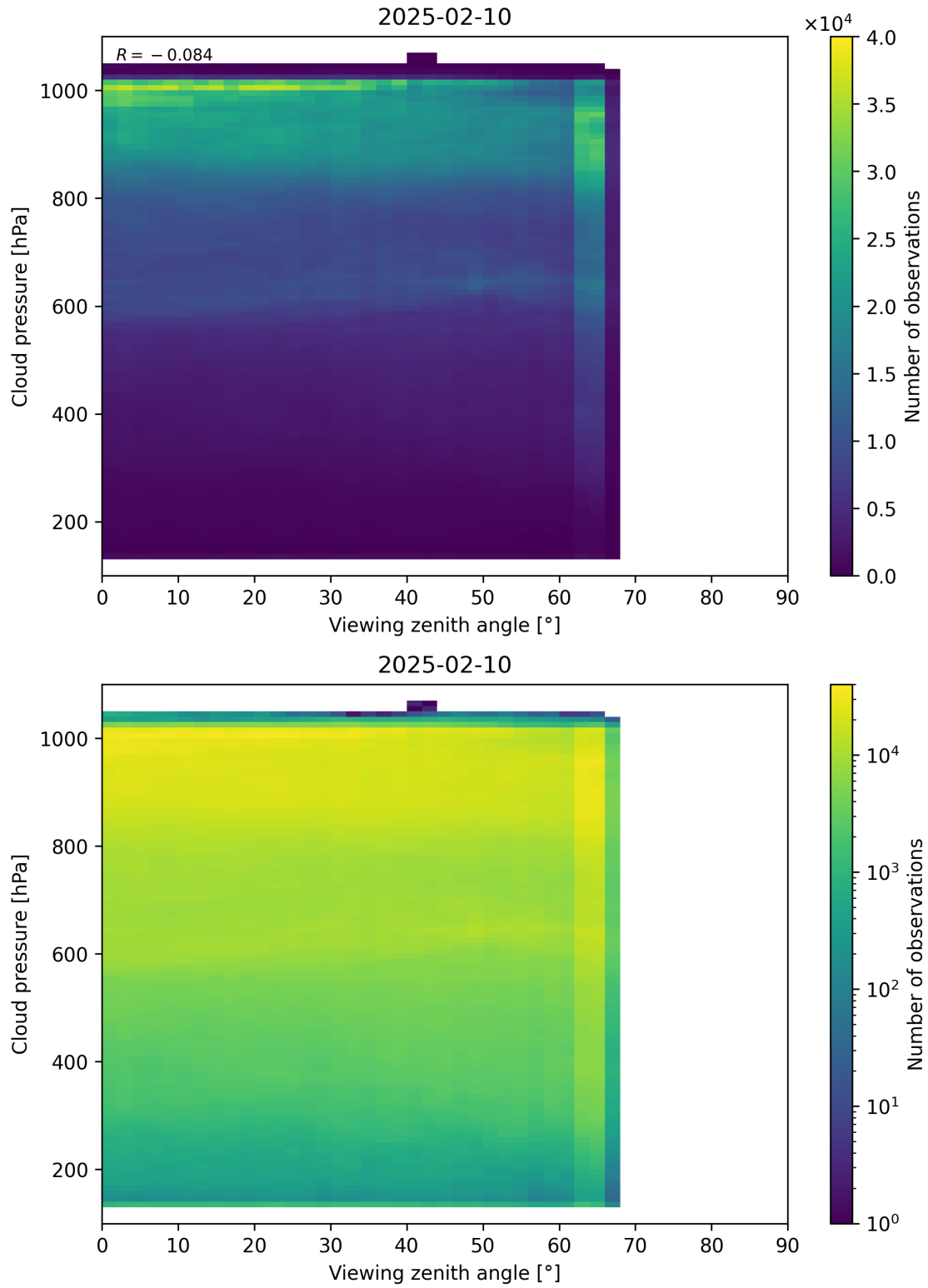
Figure 121: Scatter density plot of “Viewing zenith angle” against “Cloud pressure” for 2025-02-09 to 2025-02-11.
