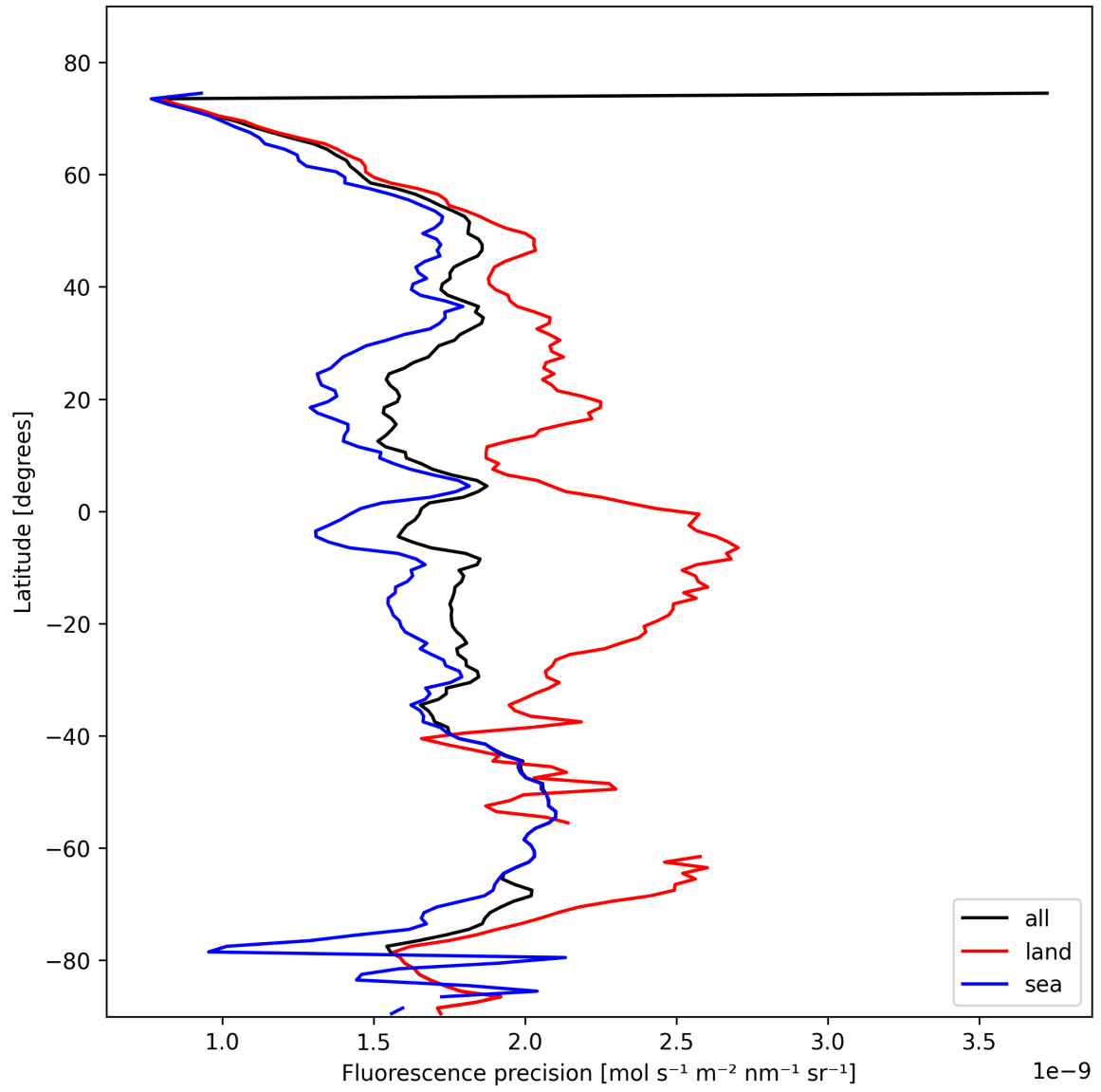
Figure 24: Zonal average of “Fluorescence precision” for 2025-02-09 to 2025-02-11.
