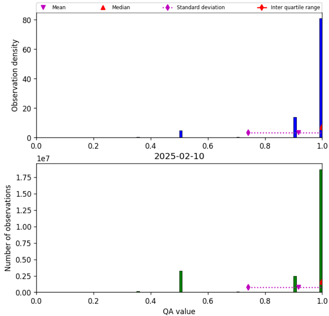
Figure 29: Histogram of “QA value” for 2025-02-09 to 2025-02-11
