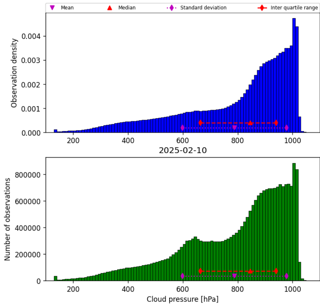
Figure 30: Histogram of “Cloud pressure” for 2025-02-09 to 2025-02-11
