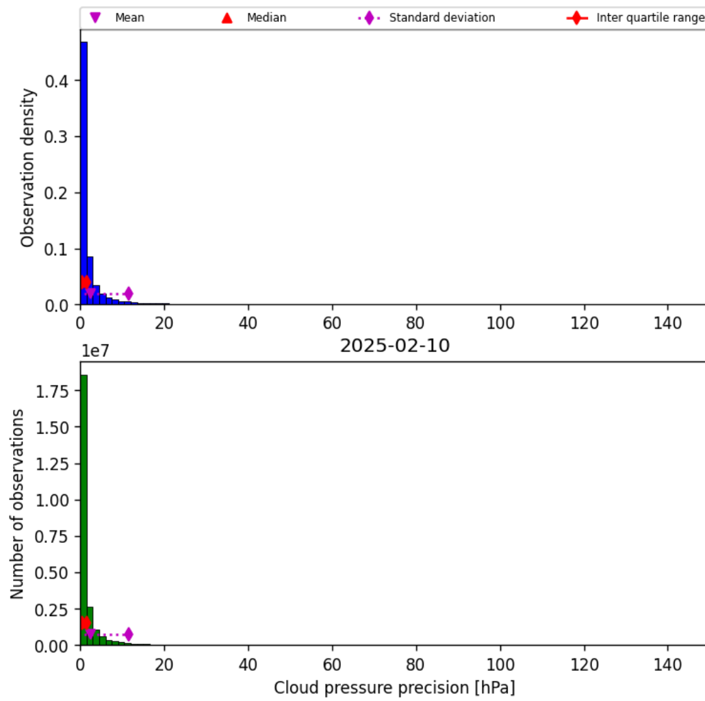
Figure 31: Histogram of “Cloud pressure precision” for 2025-02-09 to 2025-02-11
