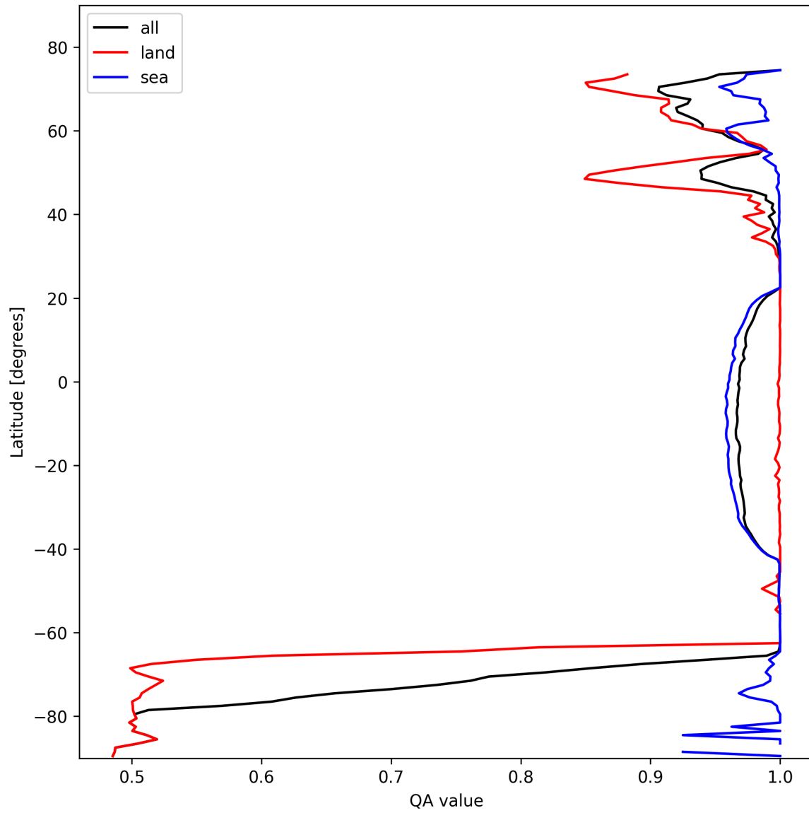
Figure 12: Zonal average of “QA value” for 2025-02-09 to 2025-02-11.
