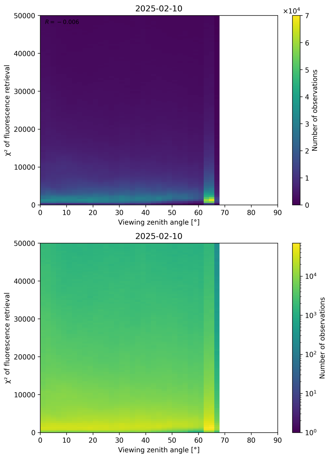
Figure 119: Scatter density plot of “Viewing zenith angle” against “ \chi^2 of fluorescence retrieval” for 2025-02-09 to 2025-02-11.
