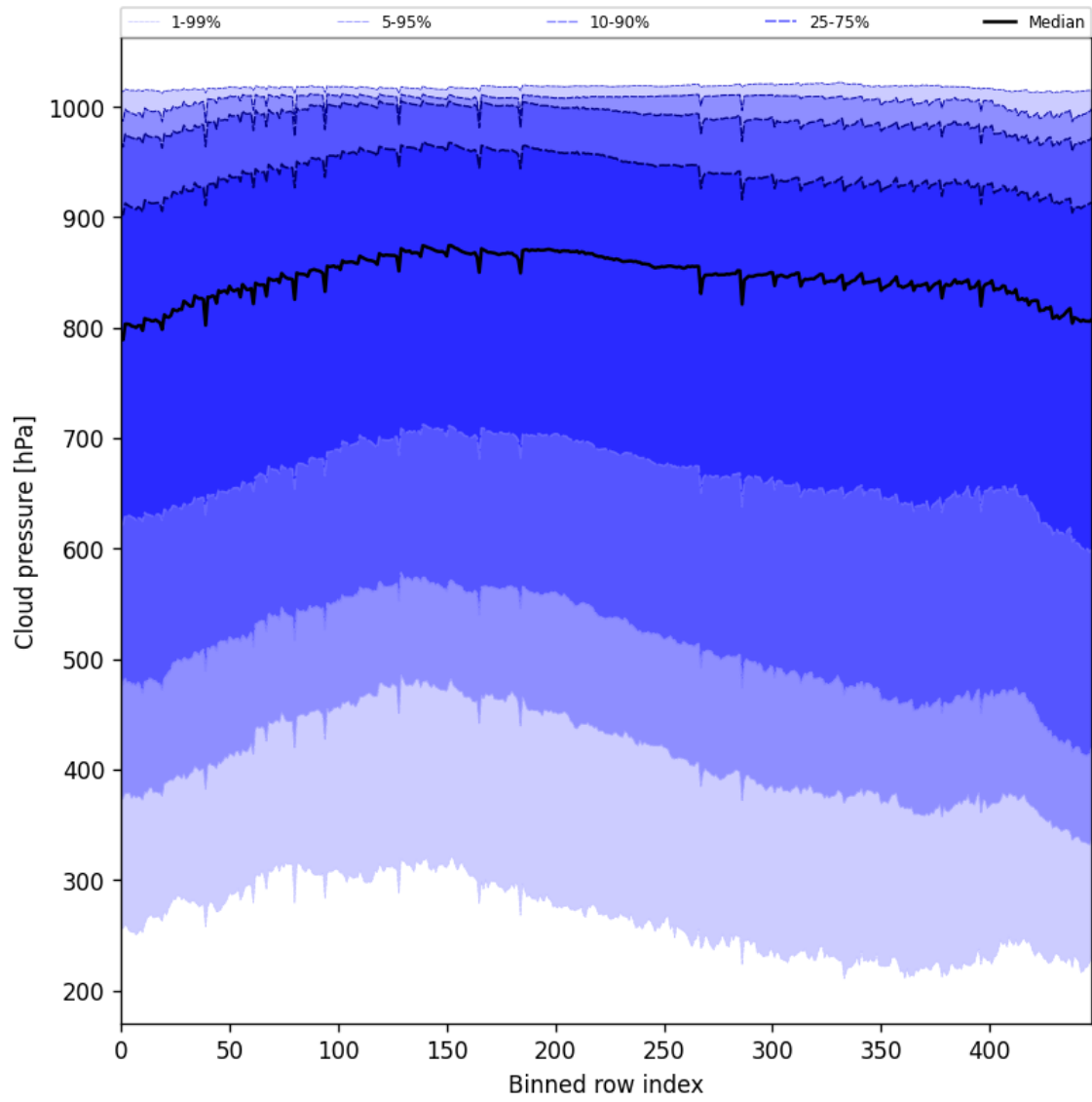
Figure 47: Along track statistics of “Cloud pressure” for 2025-02-09 to 2025-02-11
