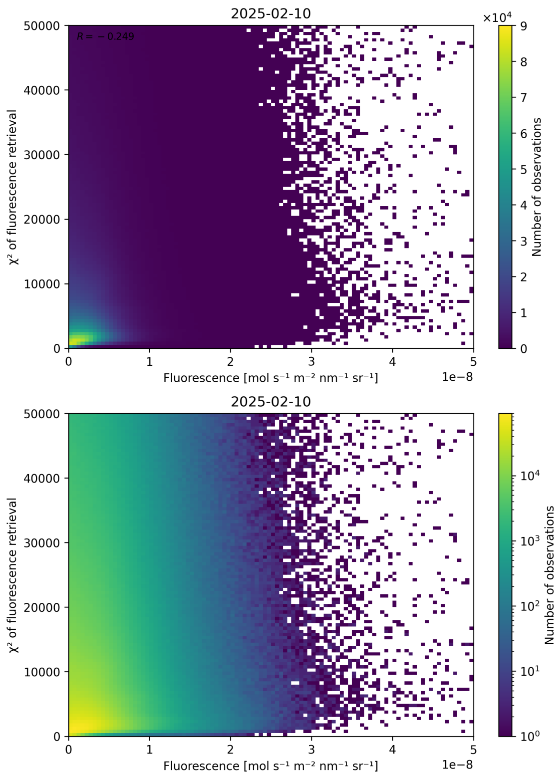
Figure 85: Scatter density plot of “Fluorescence” against “ \chi^2 of fluorescence retrieval” for 2025-02-09 to 2025-02-11.
