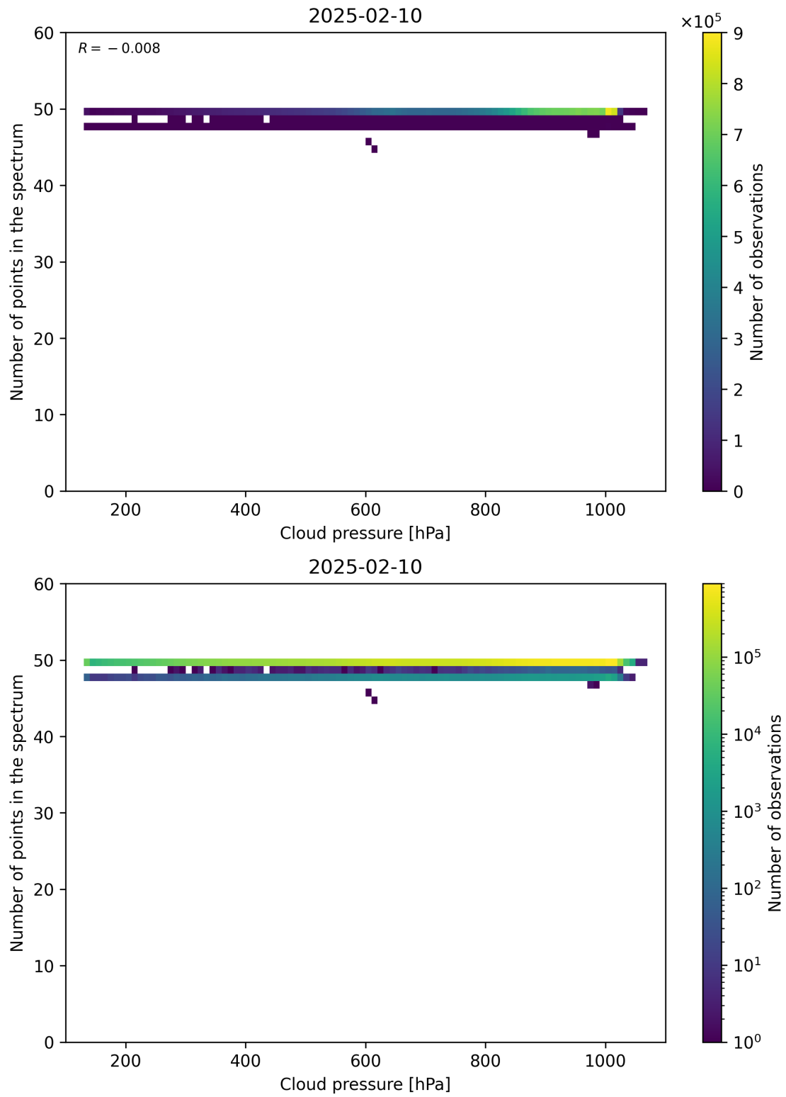
Figure 82: Scatter density plot of “Cloud pressure” against “Number of points in the spectrum” for 2025-02-09 to 2025-02-11.
