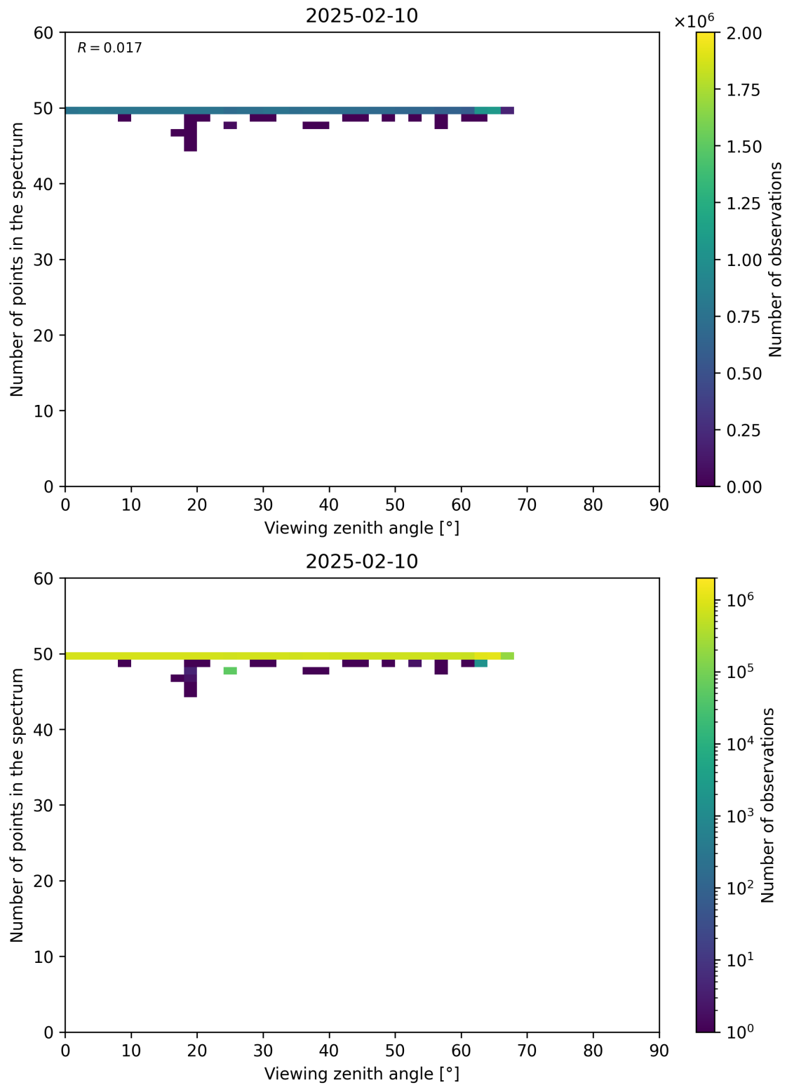
Figure 125: Scatter density plot of “Viewing zenith angle” against “Number of points in the spectrum” for 2025-02-09 to 2025-02-11.
