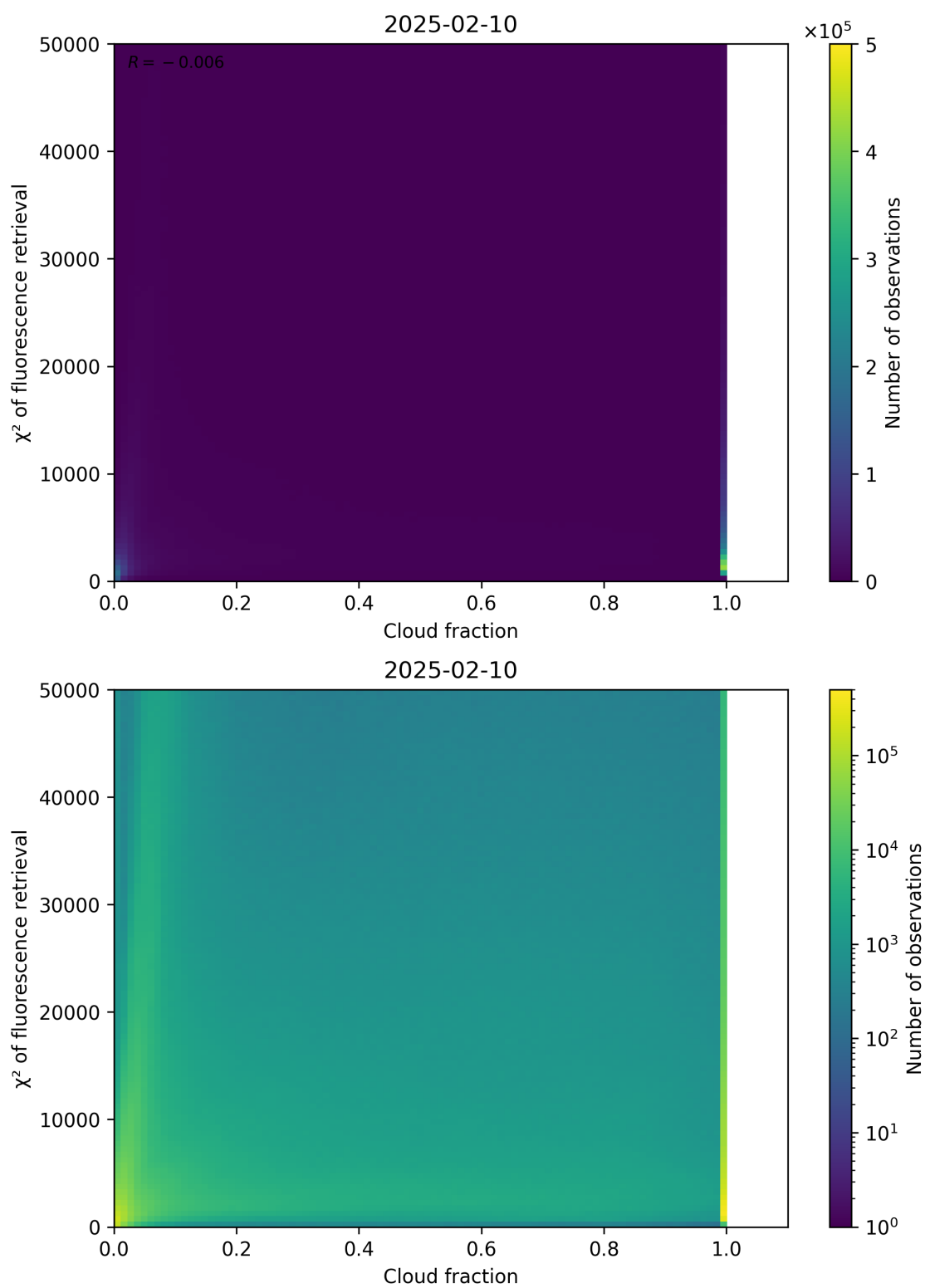
Figure 71: Scatter density plot of “Cloud fraction” against “ \chi^2 of fluorescence retrieval” for 2025-02-09 to 2025-02-11.
