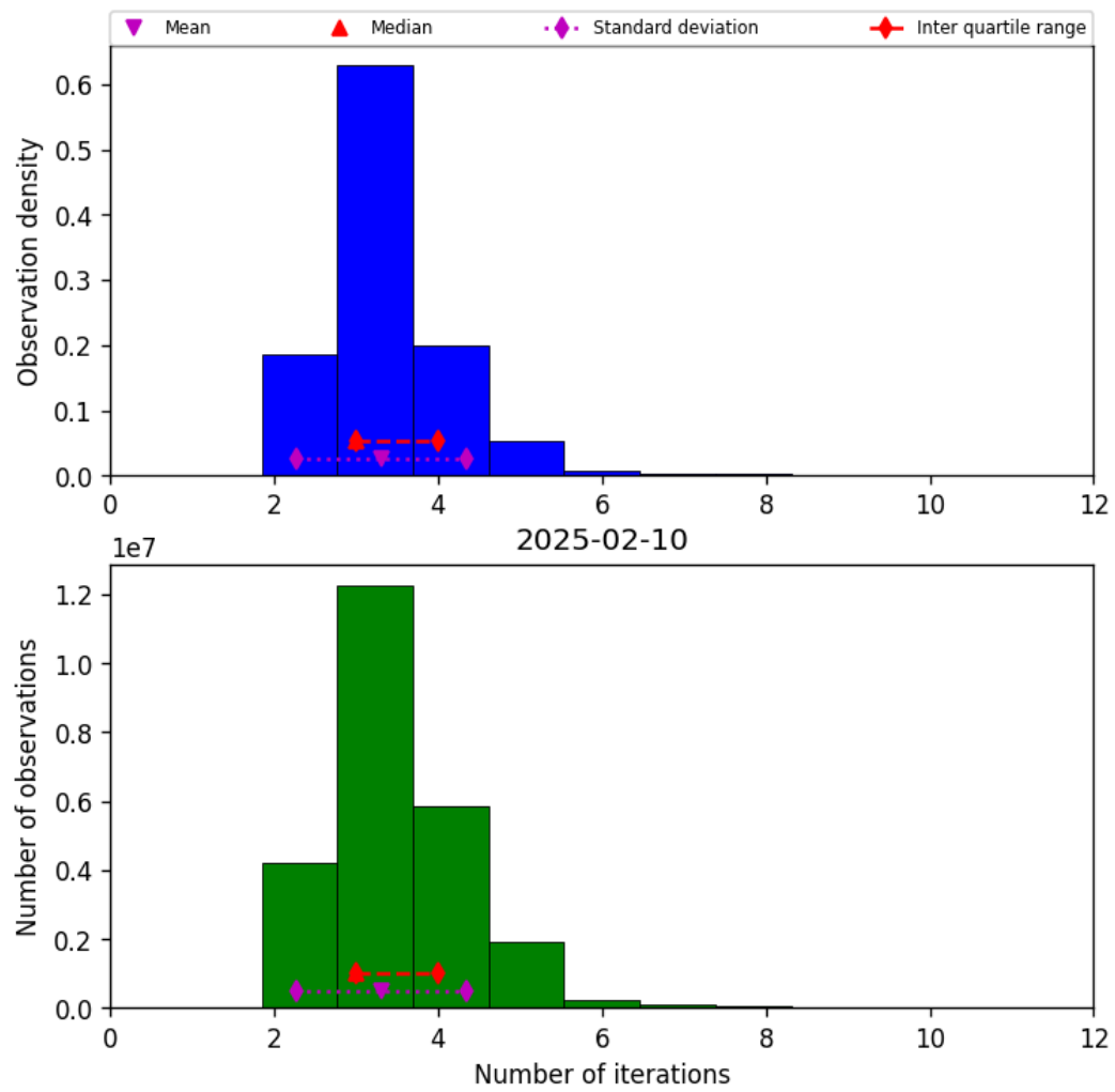
Figure 39: Histogram of “Number of iterations” for 2025-02-09 to 2025-02-11
