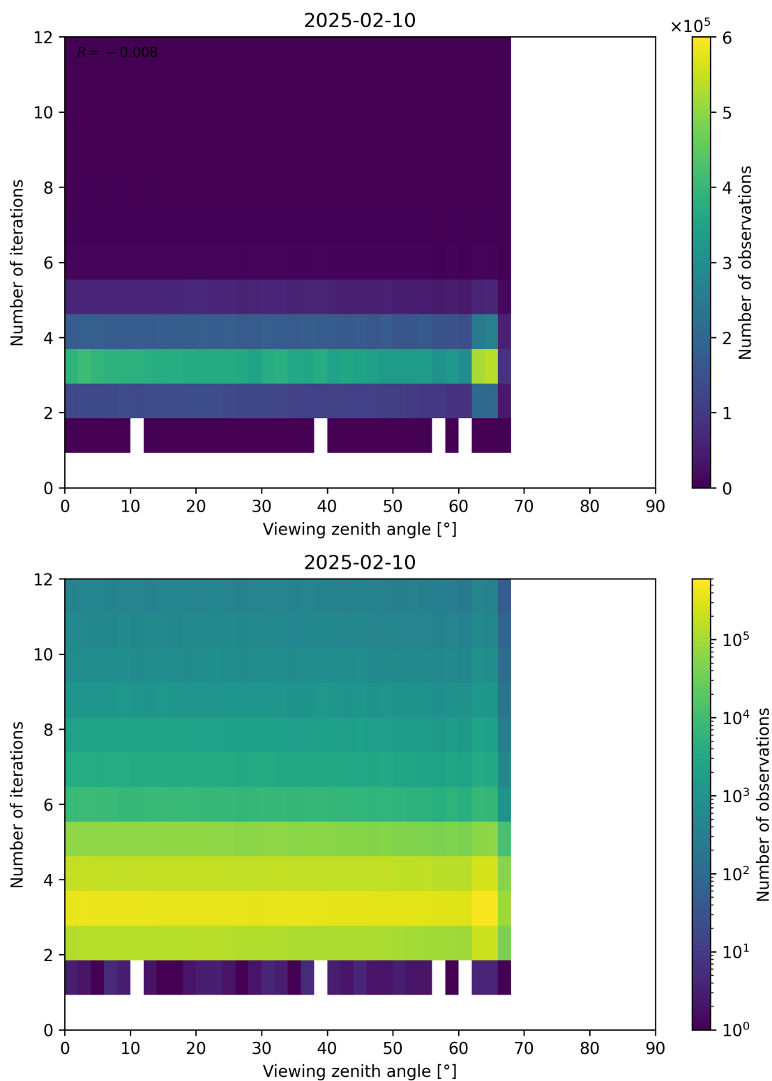
Figure 124: Scatter density plot of “Viewing zenith angle” against “Number of iterations” for 2025-02-09 to 2025-02-11.
