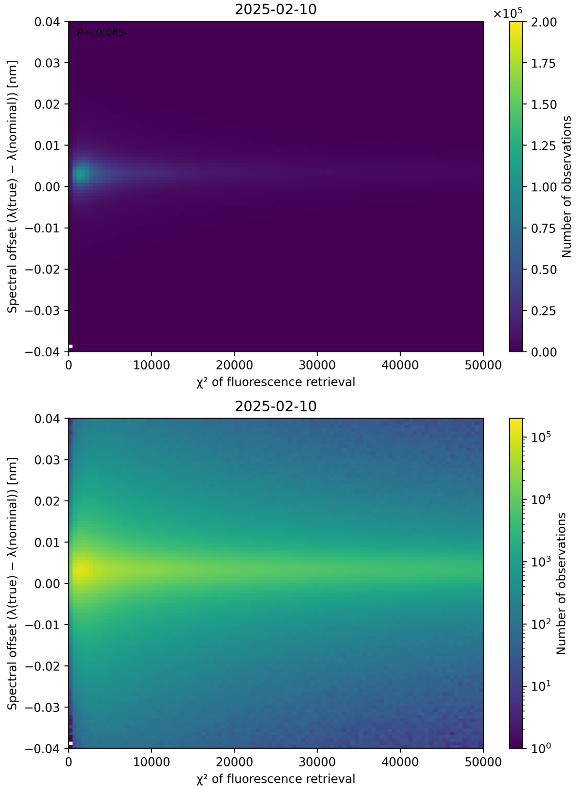
Figure 69: Scatter density plot of “ \chi^2 of fluorescence retrieval” against “Spectral offset ( \lambda_{\text{true}} - \lambda_{\text{nominal}} )” for 2025-02-09 to 2025-02-11.
