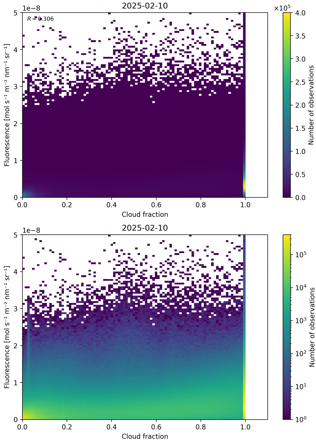
Figure 72: Scatter density plot of “Cloud fraction” against “Fluorescence” for 2025-02-09 to 2025-02-11.
