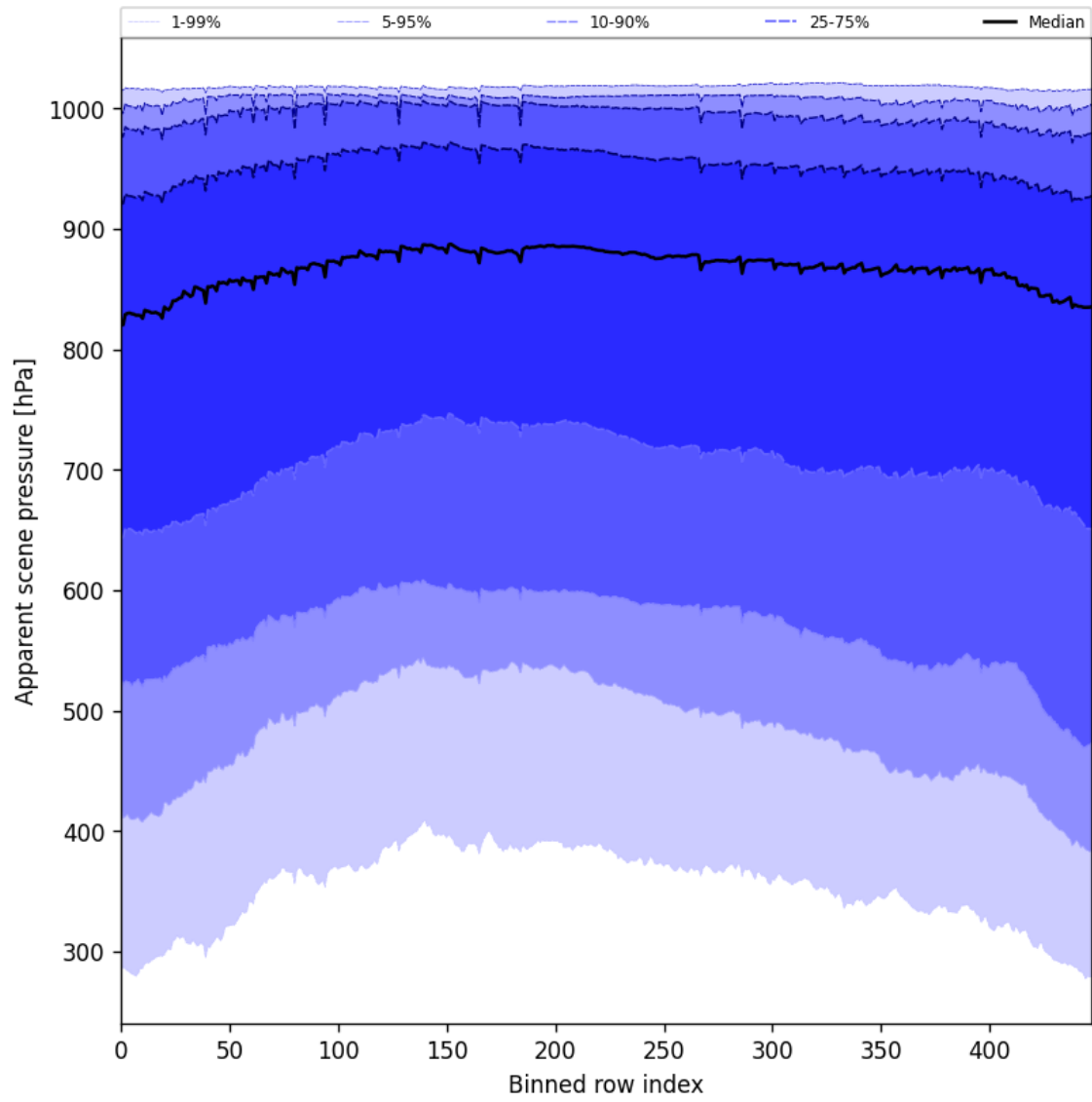
Figure 53: Along track statistics of “Apparent scene pressure” for 2025-02-09 to 2025-02-11
