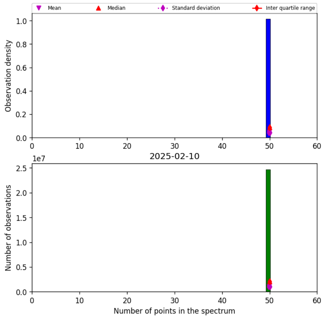
Figure 44: Histogram of “Number of points in the spectrum” for 2025-02-09 to 2025-02-11
