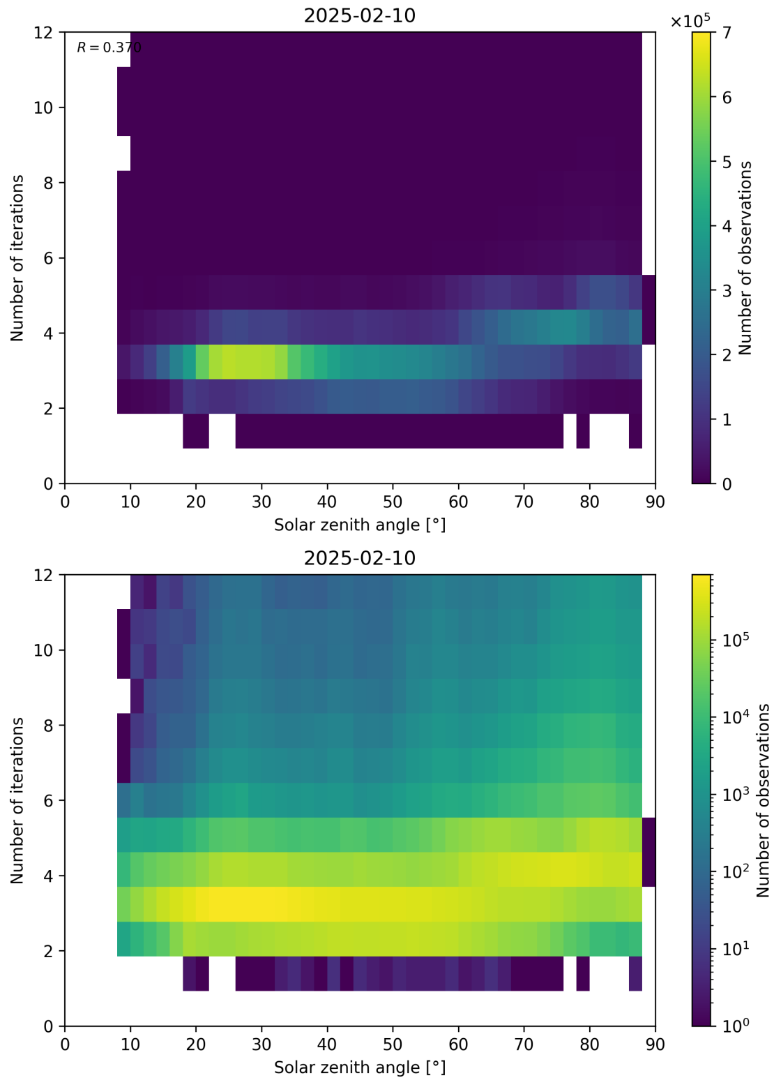
Figure 114: Scatter density plot of “Solar zenith angle” against “Number of iterations” for 2025-02-09 to 2025-02-11.
