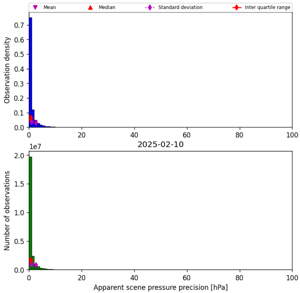
Figure 37: Histogram of “Apparent scene pressure precision” for 2025-02-09 to 2025-02-11
