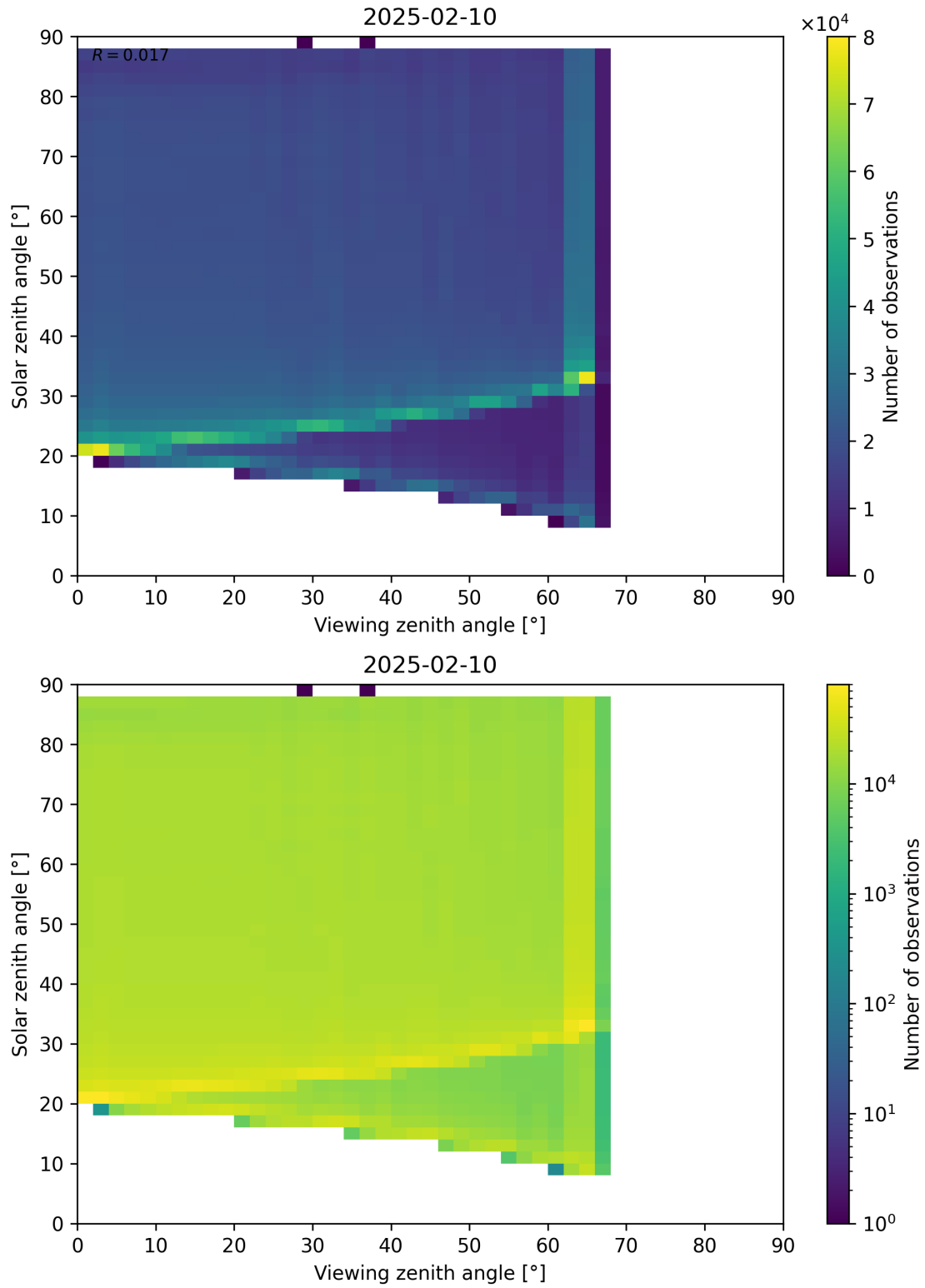
Figure 127: Scatter density plot of “Viewing zenith angle” against “Solar zenith angle” for 2025-02-09 to 2025-02-11.
