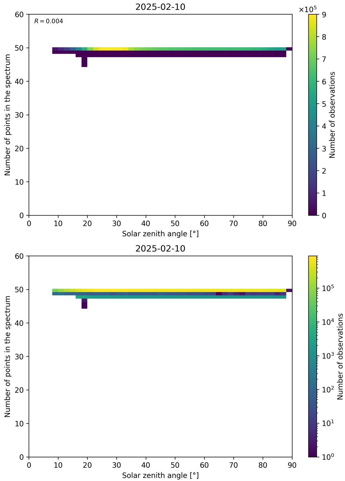
Figure 115: Scatter density plot of “Solar zenith angle” against “Number of points in the spectrum” for 2025-02-09 to 2025-02-11.
