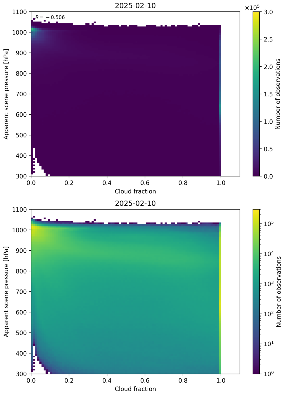
Figure 70: Scatter density plot of “Cloud fraction” against “Apparent scene pressure” for 2025-02-09 to 2025-02-11.
