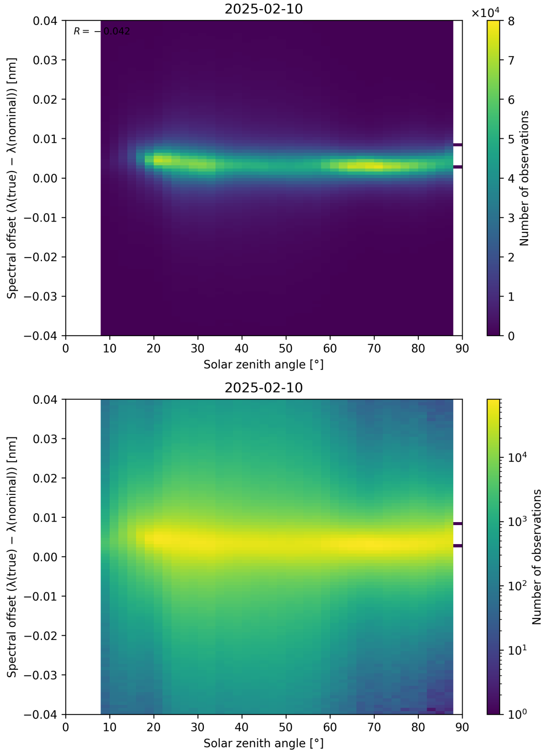
Figure 117: Scatter density plot of “Solar zenith angle” against “Spectral offset ( \lambda_{\text{true}} - \lambda_{\text{nominal}} )” for 2025-02-09 to 2025-02-11.
