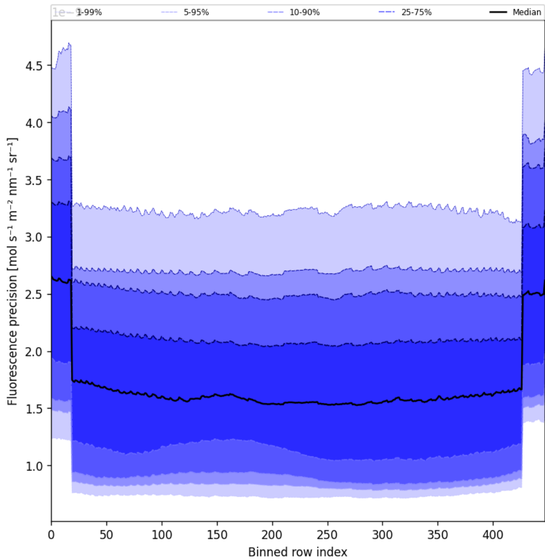
Figure 58: Along track statistics of “Fluorescence precision” for 2025-02-09 to 2025-02-11
