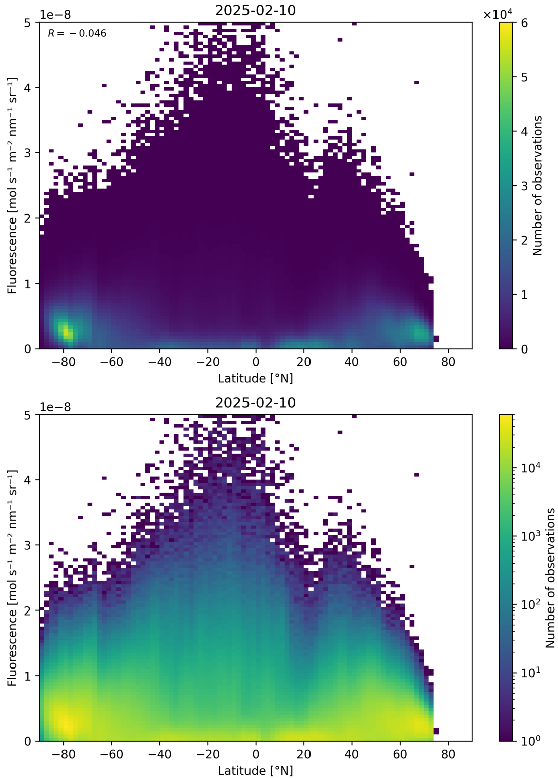
Figure 92: Scatter density plot of “Latitude” against “Fluorescence” for 2025-02-09 to 2025-02-11.
