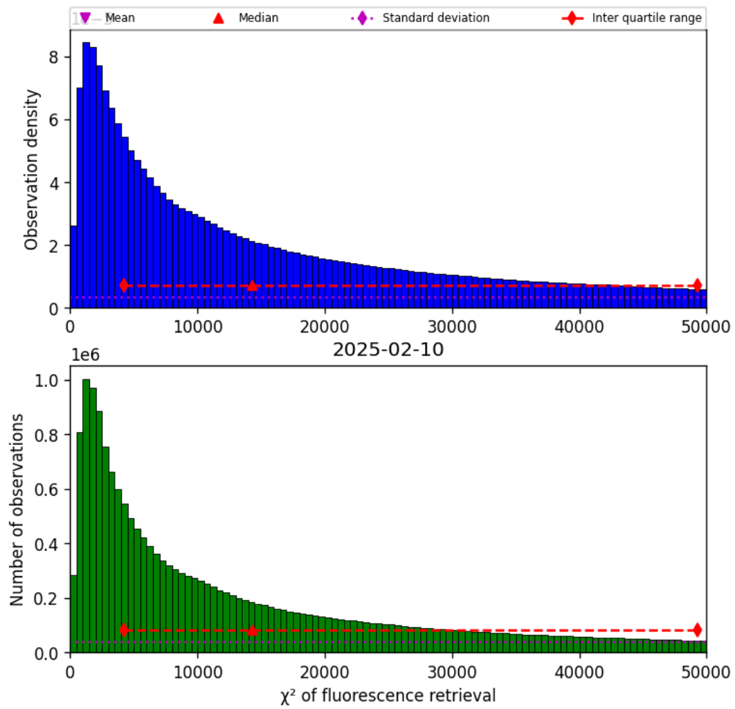
Figure 42: Histogram of “ \chi^2 of fluorescence retrieval” for 2025-02-09 to 2025-02-11
