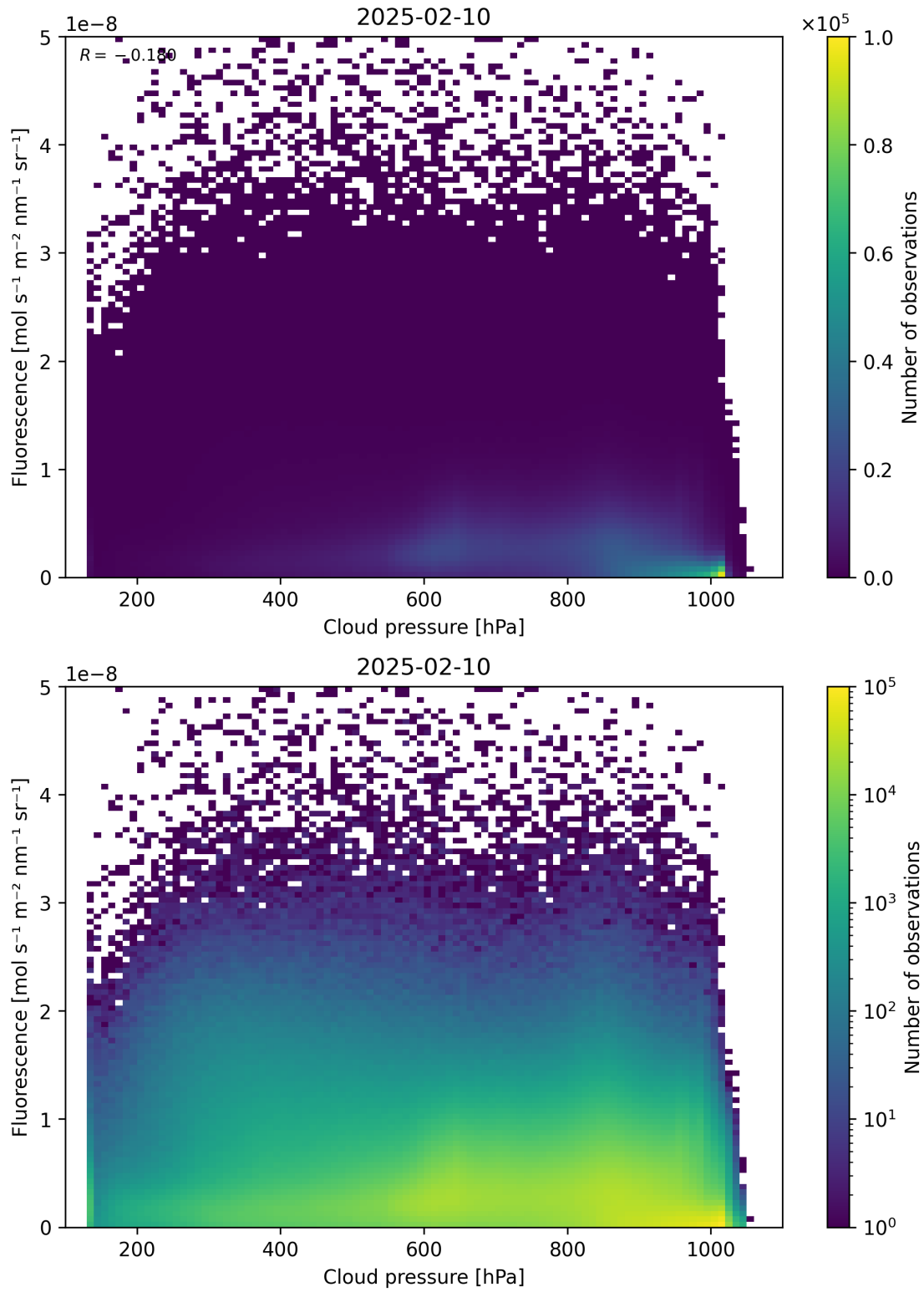
Figure 80: Scatter density plot of “Cloud pressure” against “Fluorescence” for 2025-02-09 to 2025-02-11.
