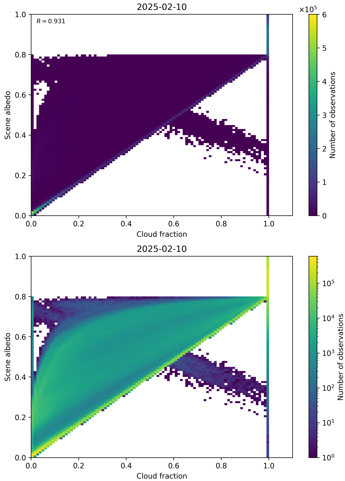
Figure 75: Scatter density plot of “Cloud fraction” against “Scene albedo” for 2025-02-09 to 2025-02-11.
