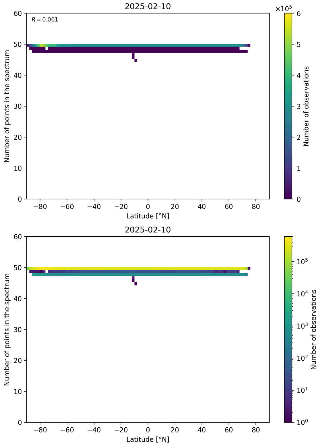
Figure 94: Scatter density plot of “Latitude” against “Number of points in the spectrum” for 2025-02-09 to 2025-02-11.
