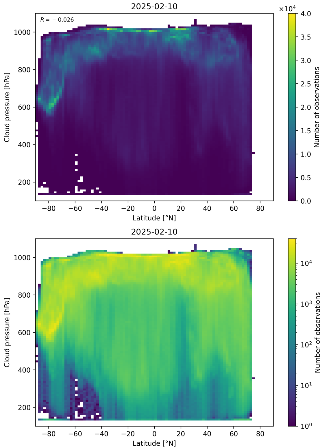
Figure 91: Scatter density plot of “Latitude” against “Cloud pressure” for 2025-02-09 to 2025-02-11.
