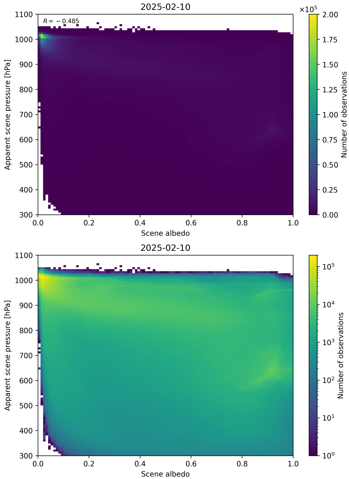
Figure 102: Scatter density plot of “Scene albedo” against “Apparent scene pressure” for 2025-02-09 to 2025-02-11.
