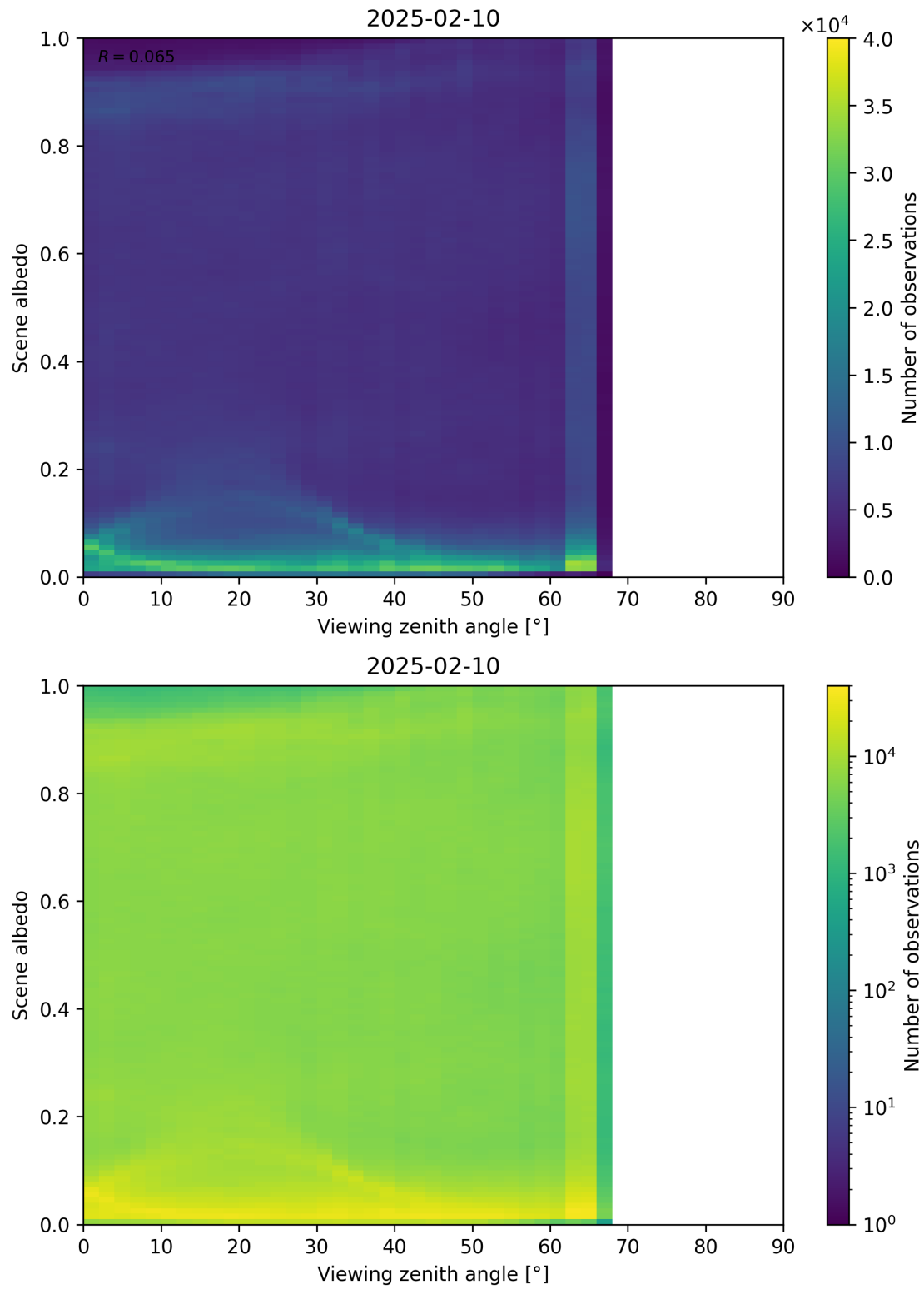
Figure 126: Scatter density plot of “Viewing zenith angle” against “Scene albedo” for 2025-02-09 to 2025-02-11.
