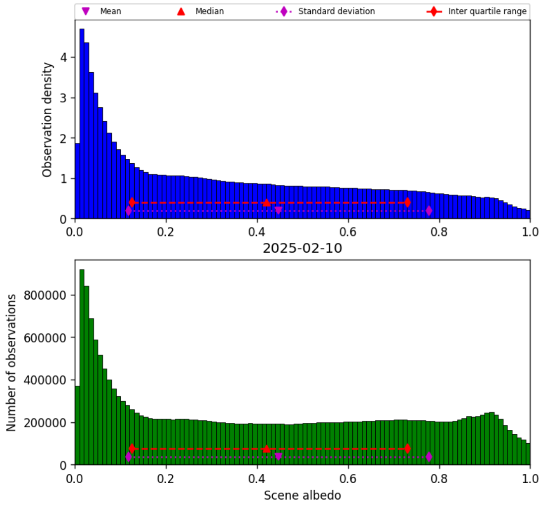
Figure 34: Histogram of “Scene albedo” for 2025-02-09 to 2025-02-11
