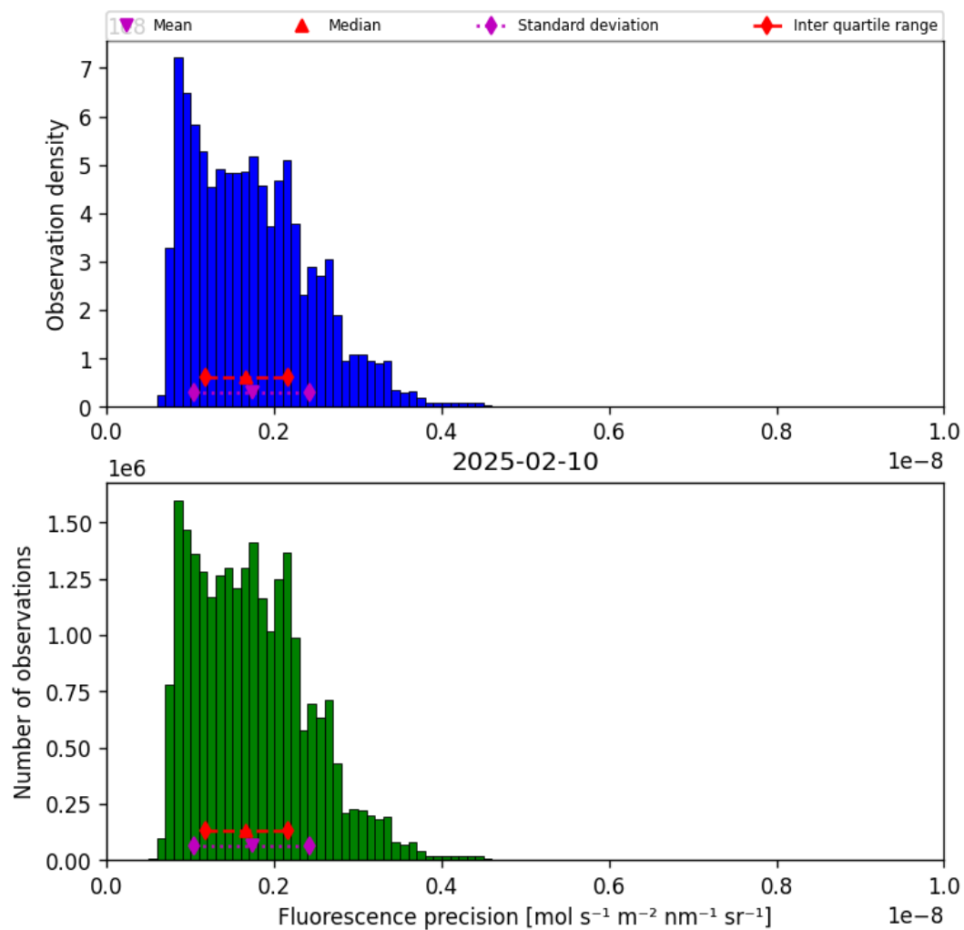
Figure 41: Histogram of “Fluorescence precision” for 2025-02-09 to 2025-02-11
