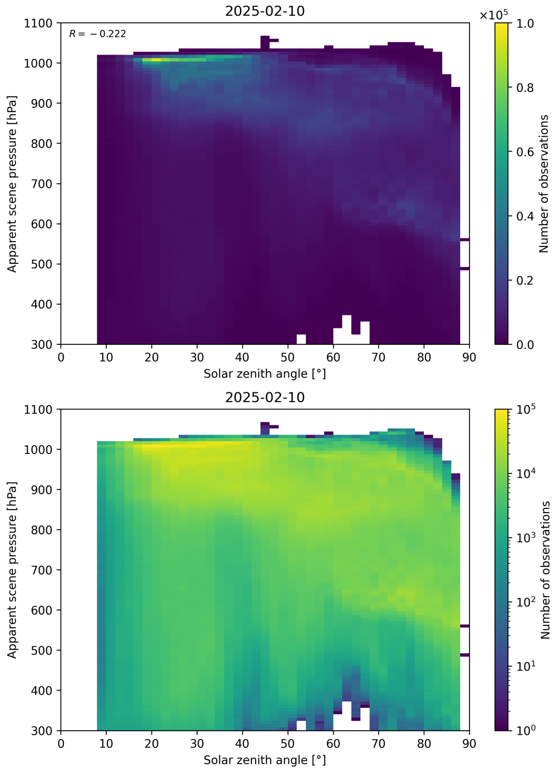
Figure 108: Scatter density plot of “Solar zenith angle” against “Apparent scene pressure” for 2025-02-09 to 2025-02-11.
