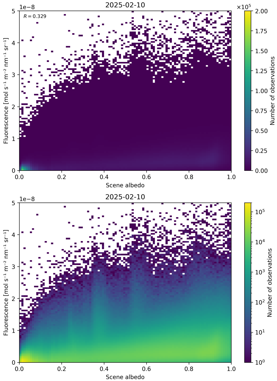
Figure 104: Scatter density plot of “Scene albedo” against “Fluorescence” for 2025-02-09 to 2025-02-11.
