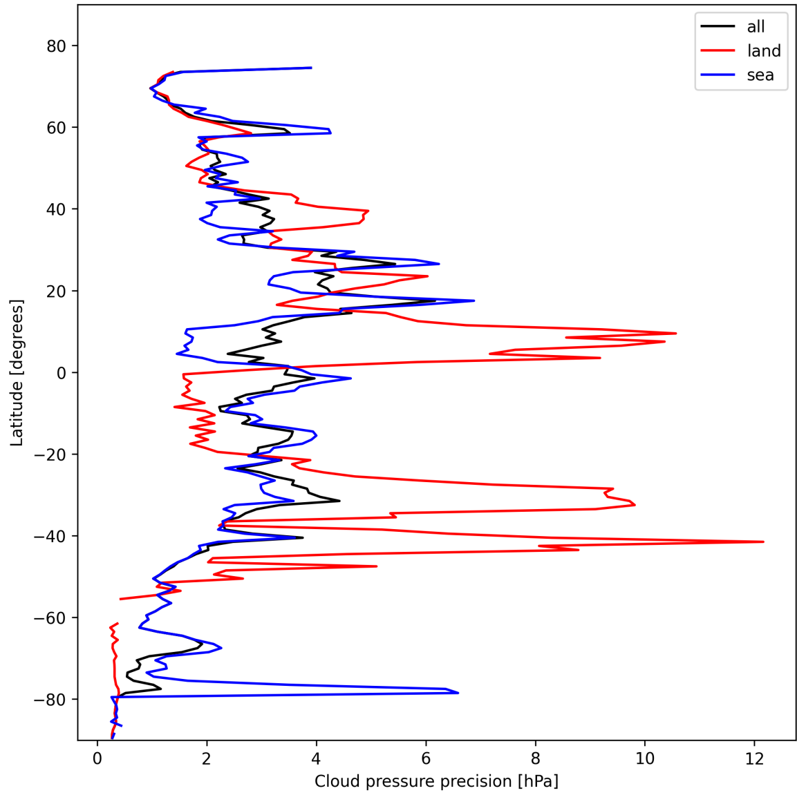
Figure 14: Zonal average of “Cloud pressure precision” for 2025-02-09 to 2025-02-11.
