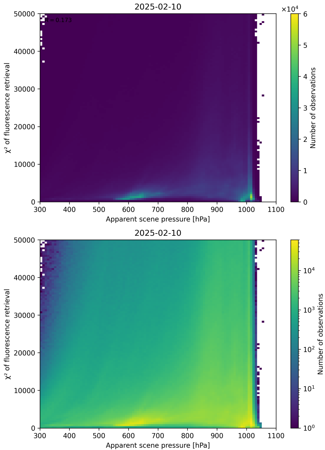
Figure 63: Scatter density plot of “Apparent scene pressure” against “ \chi^2 of fluorescence retrieval” for 2025-02-09 to 2025-02-11.
