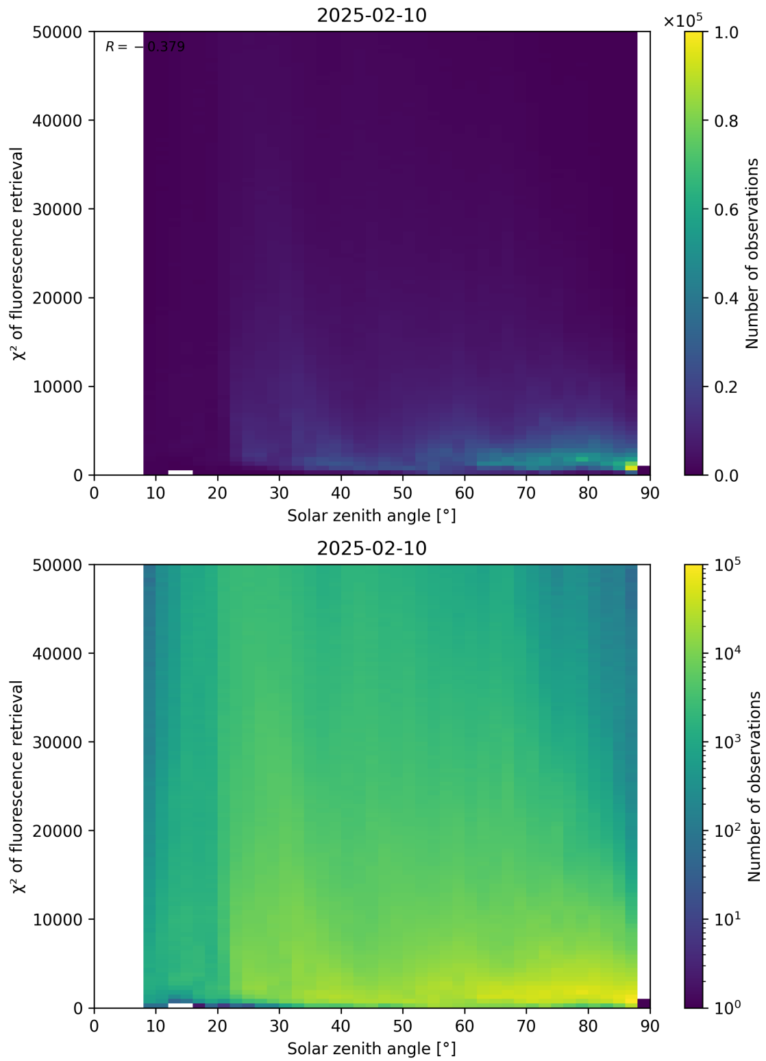
Figure 109: Scatter density plot of “Solar zenith angle” against “ \chi^2 of fluorescence retrieval” for 2025-02-09 to 2025-02-11.
