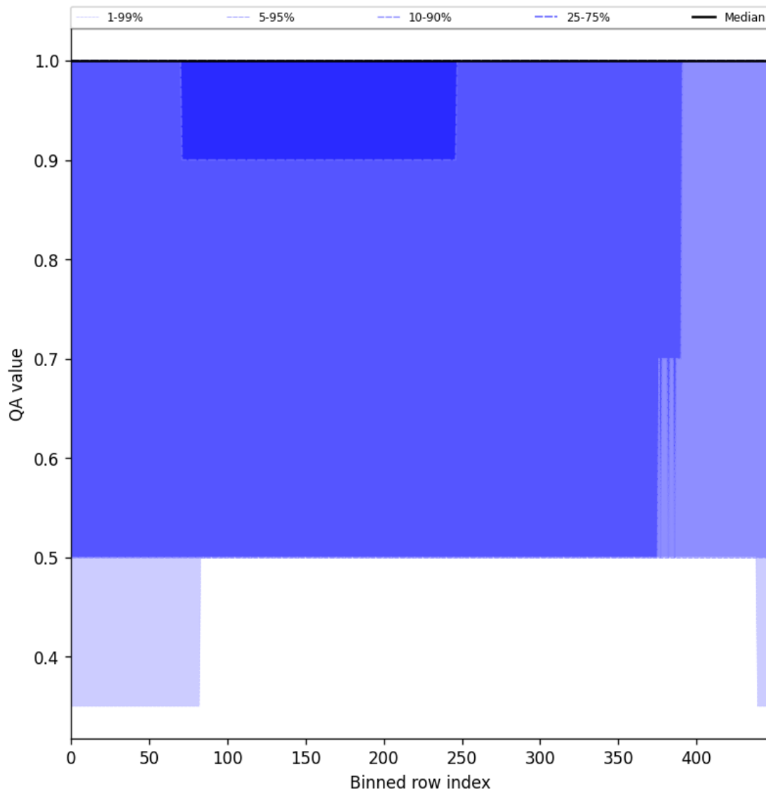
Figure 46: Along track statistics of “QA value” for 2025-02-09 to 2025-02-11
