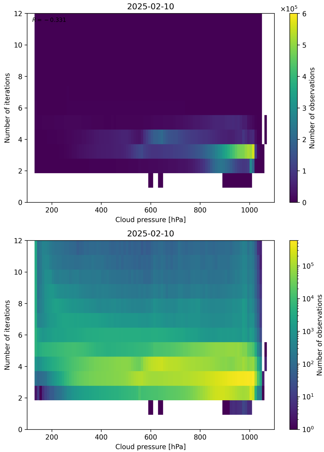
Figure 81: Scatter density plot of “Cloud pressure” against “Number of iterations” for 2025-02-09 to 2025-02-11.
