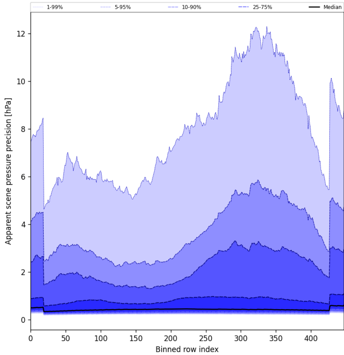
Figure 54: Along track statistics of “Apparent scene pressure precision” for 2025-02-09 to 2025-02-11
