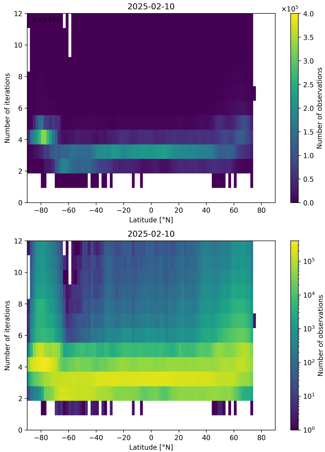
Figure 93: Scatter density plot of “Latitude” against “Number of iterations” for 2025-02-09 to 2025-02-11.
