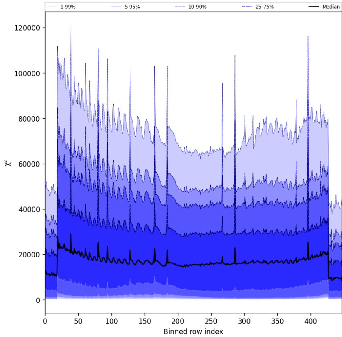
Figure 55: Along track statistics of “ \chi^2 ” for 2025-02-09 to 2025-02-11
