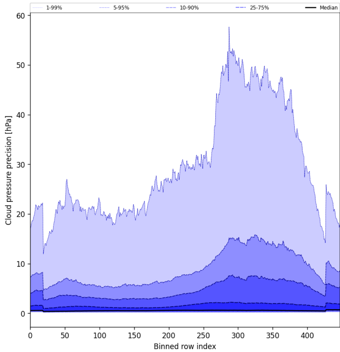
Figure 48: Along track statistics of “Cloud pressure precision” for 2025-02-09 to 2025-02-11
