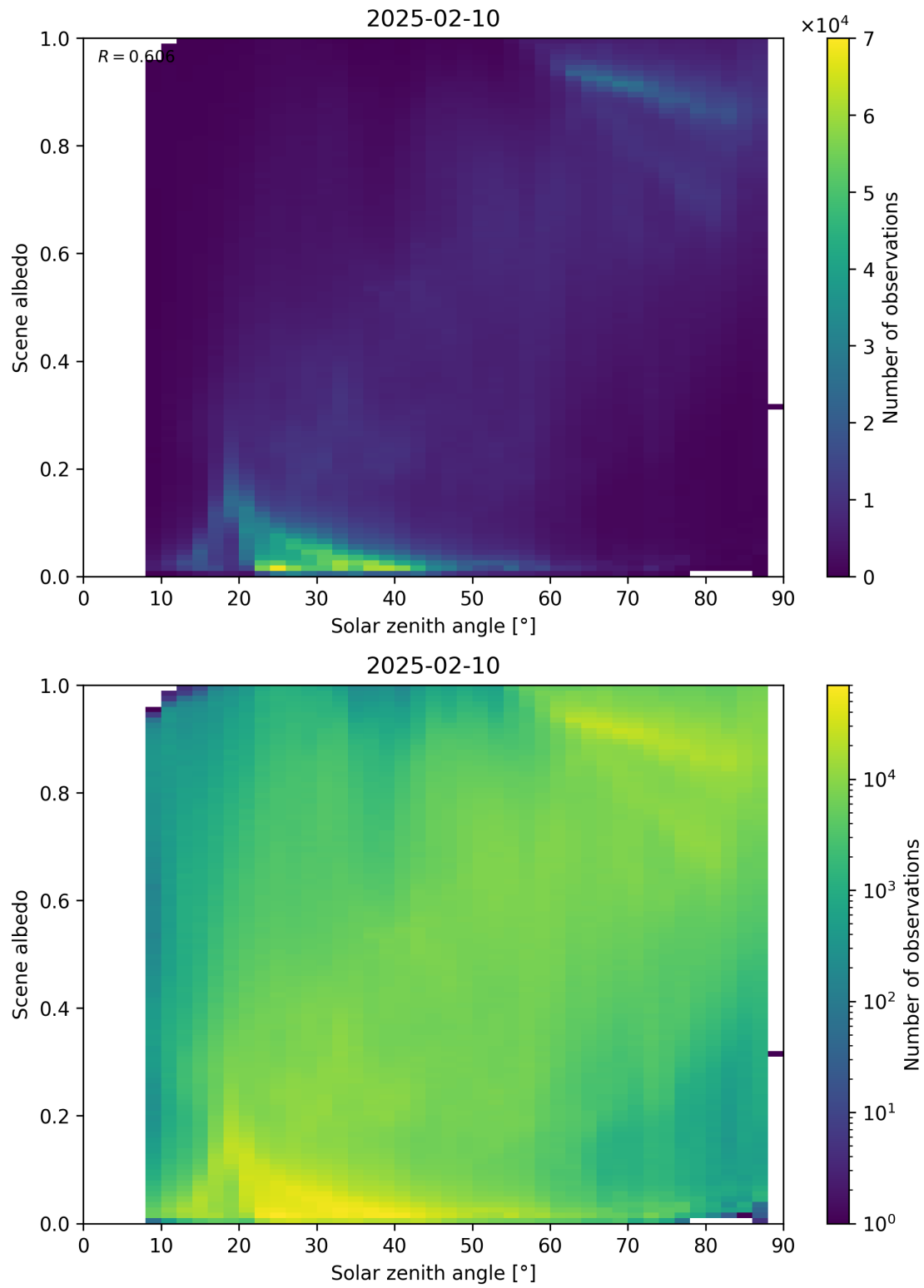
Figure 116: Scatter density plot of “Solar zenith angle” against “Scene albedo” for 2025-02-09 to 2025-02-11.
