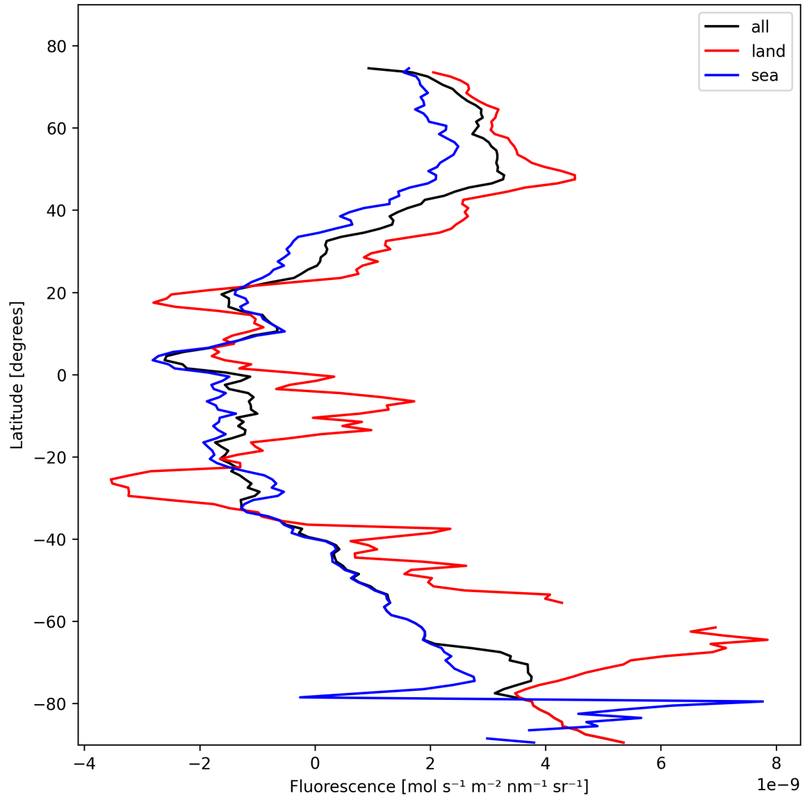
Figure 23: Zonal average of “Fluorescence” for 2025-02-09 to 2025-02-11.
