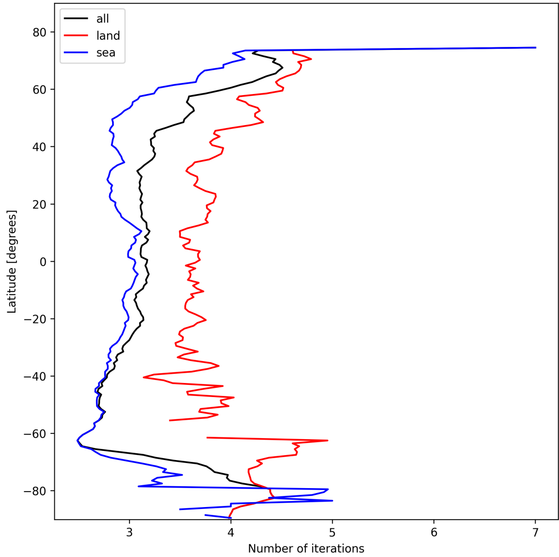
Figure 22: Zonal average of “Number of iterations” for 2025-02-09 to 2025-02-11.
