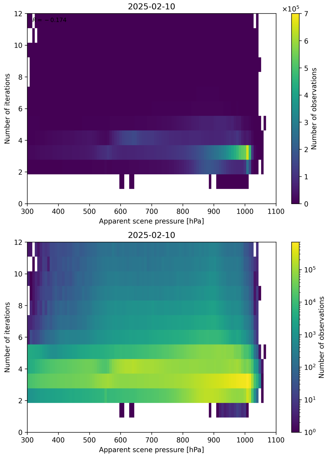
Figure 65: Scatter density plot of “Apparent scene pressure” against “Number of iterations” for 2025-02-09 to 2025-02-11.
