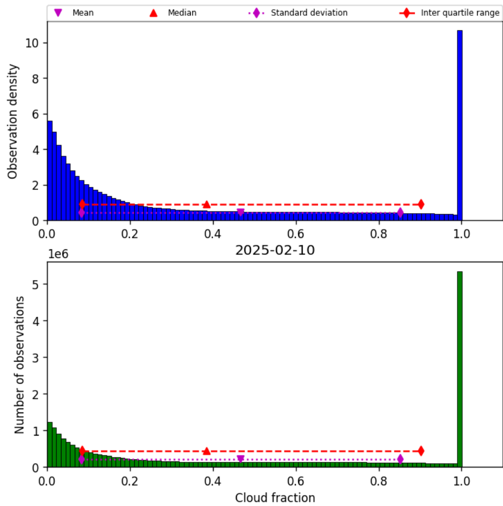
Figure 32: Histogram of “Cloud fraction” for 2025-02-09 to 2025-02-11
