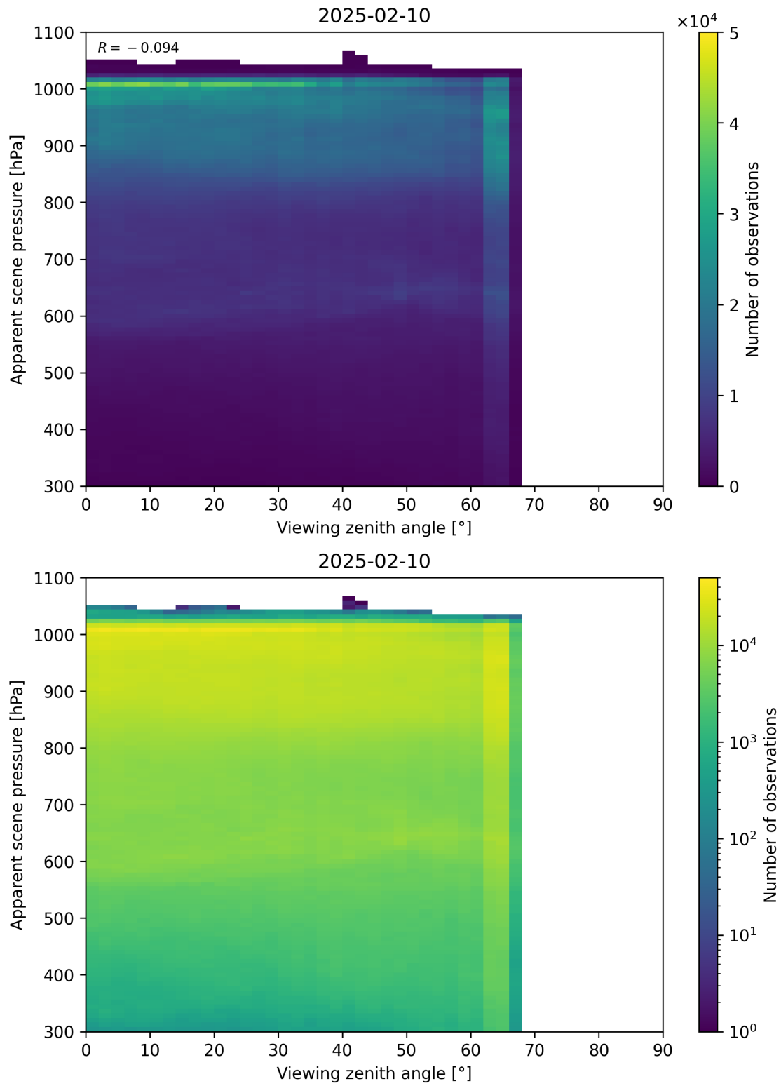
Figure 118: Scatter density plot of “Viewing zenith angle” against “Apparent scene pressure” for 2025-02-09 to 2025-02-11.
