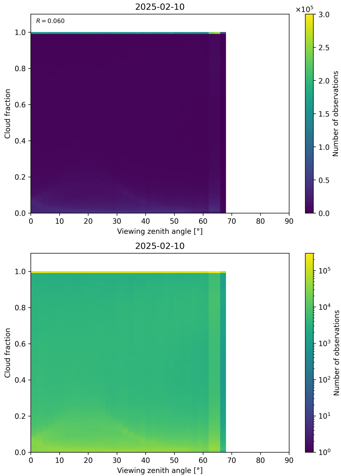
Figure 120: Scatter density plot of “Viewing zenith angle” against “Cloud fraction” for 2025-02-09 to 2025-02-11.
