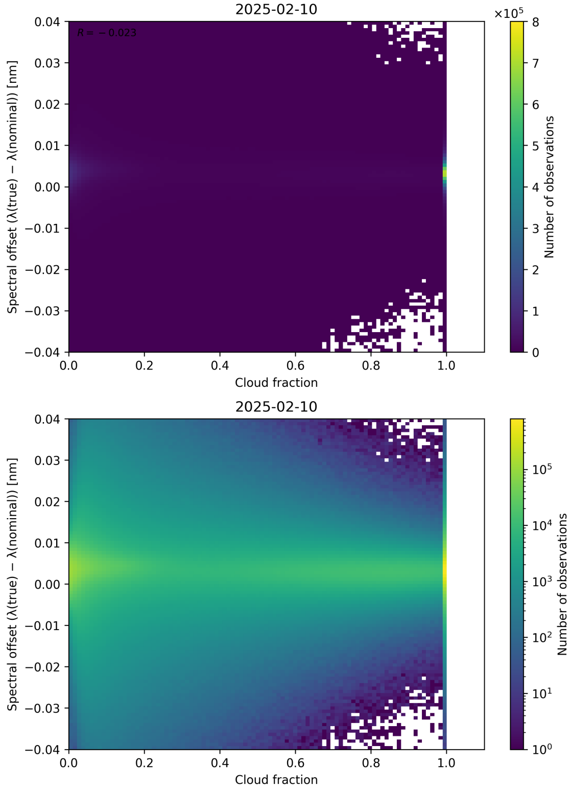
Figure 76: Scatter density plot of “Cloud fraction” against “Spectral offset ( \lambda_{\text{true}} - \lambda_{\text{nominal}} )” for 2025-02-09 to 2025-02-11.
