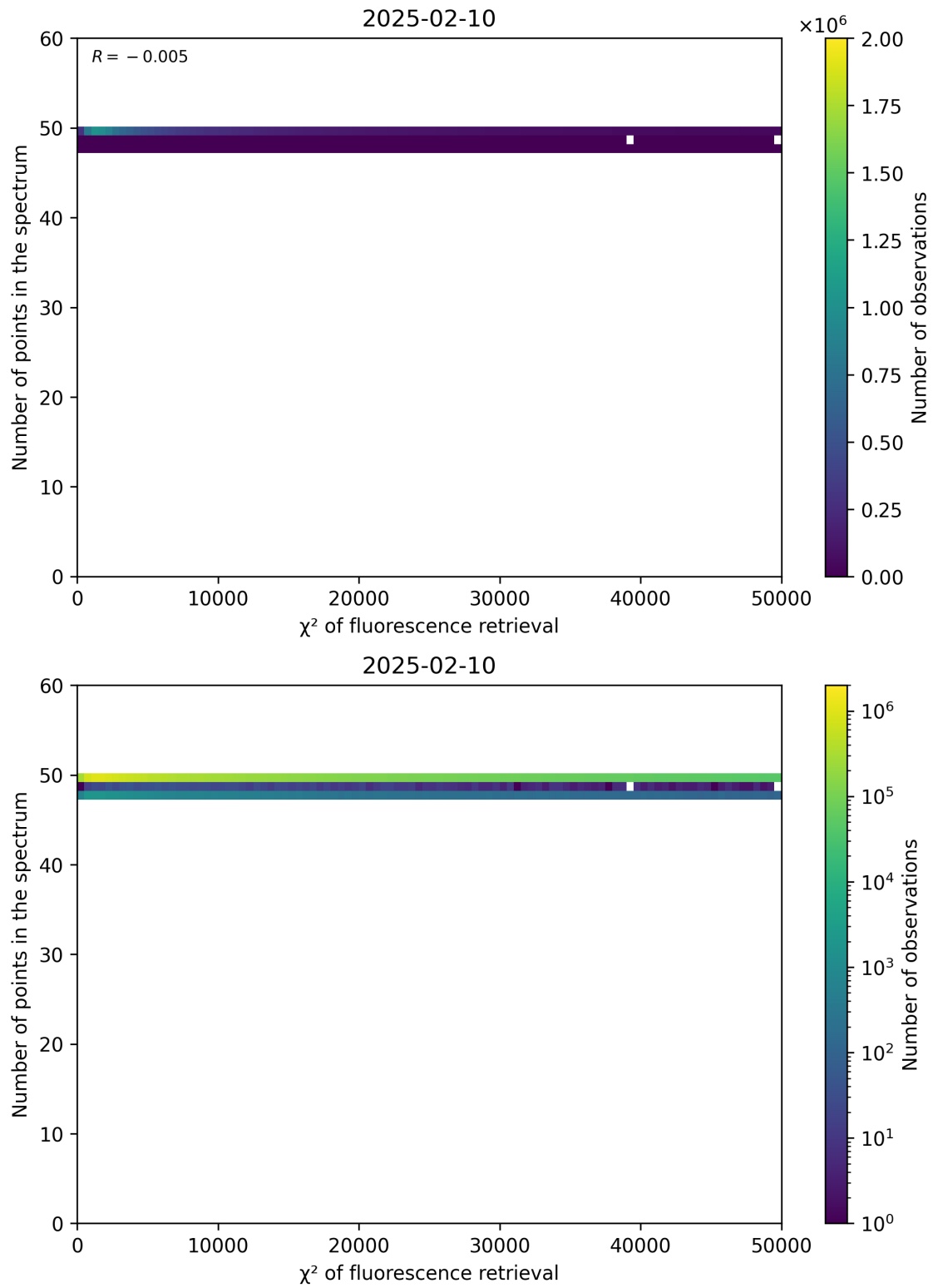
Figure 68: Scatter density plot of " \chi^2 of fluorescence retrieval" against "Number of points in the spectrum" for 2025-02-09 to 2025-02-11.
