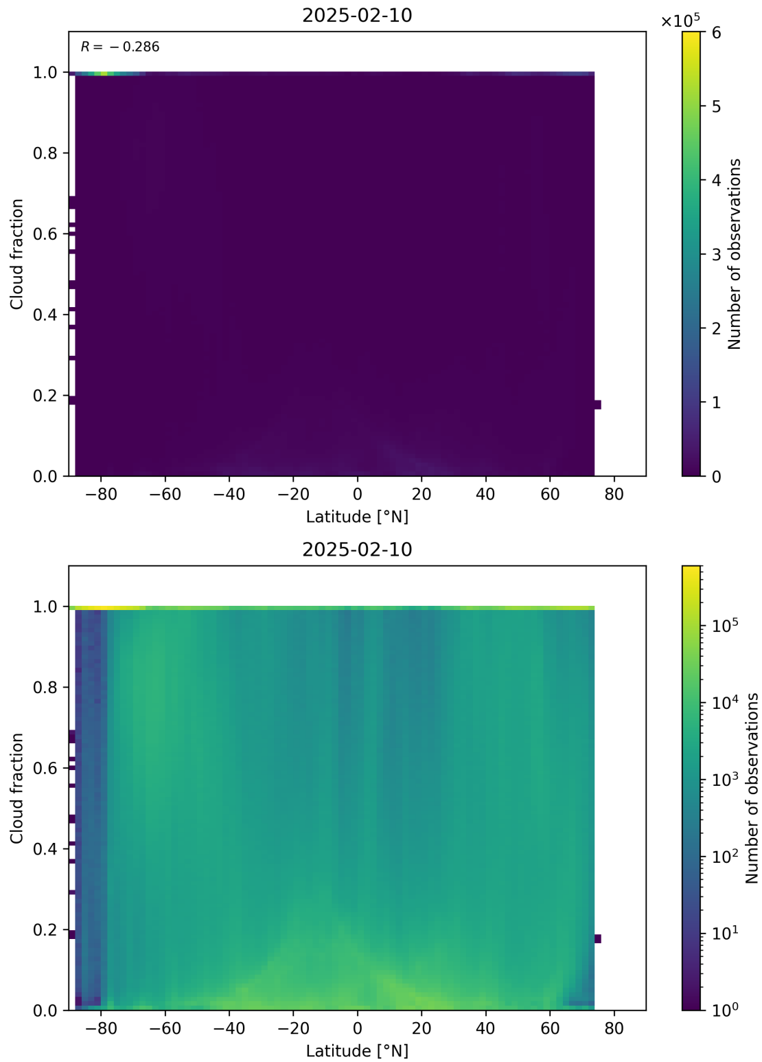
Figure 90: Scatter density plot of “Latitude” against “Cloud fraction” for 2025-02-09 to 2025-02-11.
