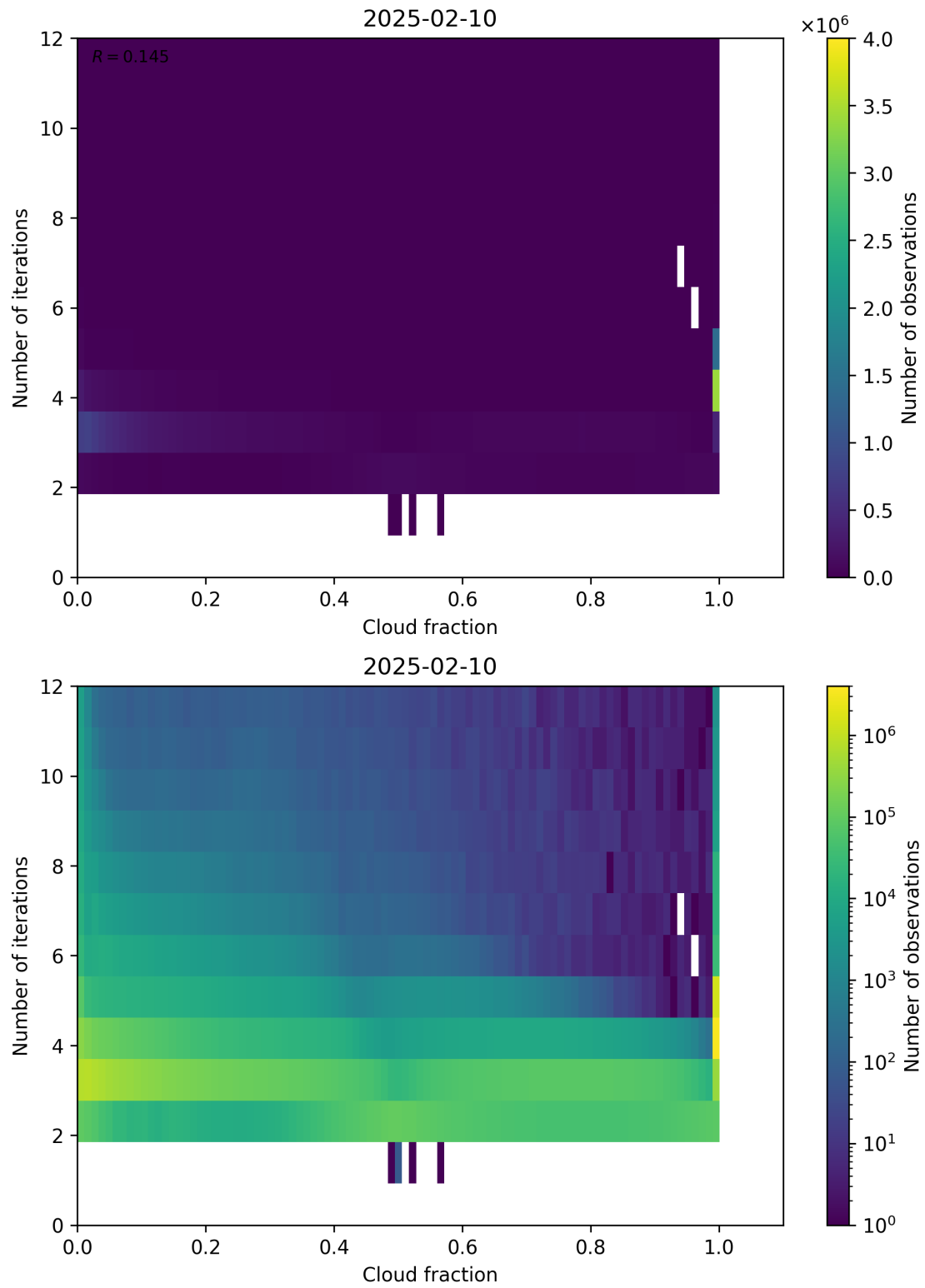
Figure 73: Scatter density plot of “Cloud fraction” against “Number of iterations” for 2025-02-09 to 2025-02-11.
