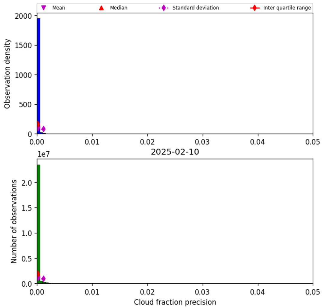
Figure 33: Histogram of “Cloud fraction precision” for 2025-02-09 to 2025-02-11
