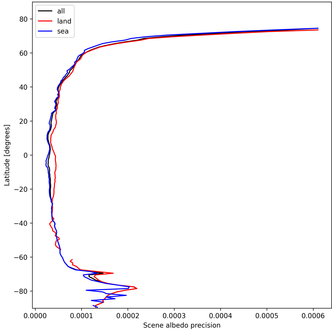
Figure 18: Zonal average of “Scene albedo precision” for 2025-02-09 to 2025-02-11.
