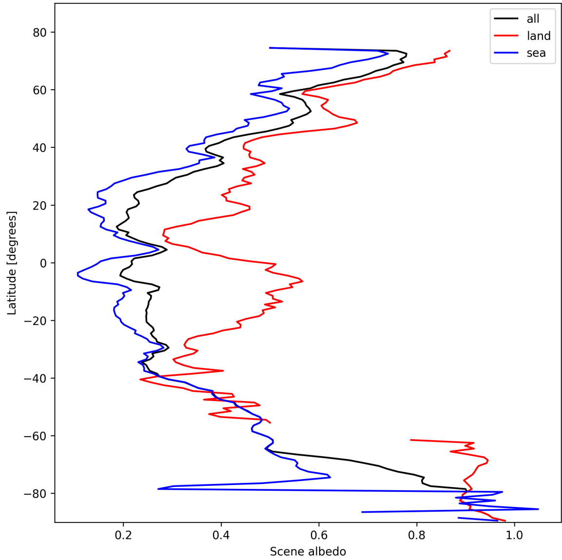
Figure 17: Zonal average of “Scene albedo” for 2025-02-09 to 2025-02-11.
