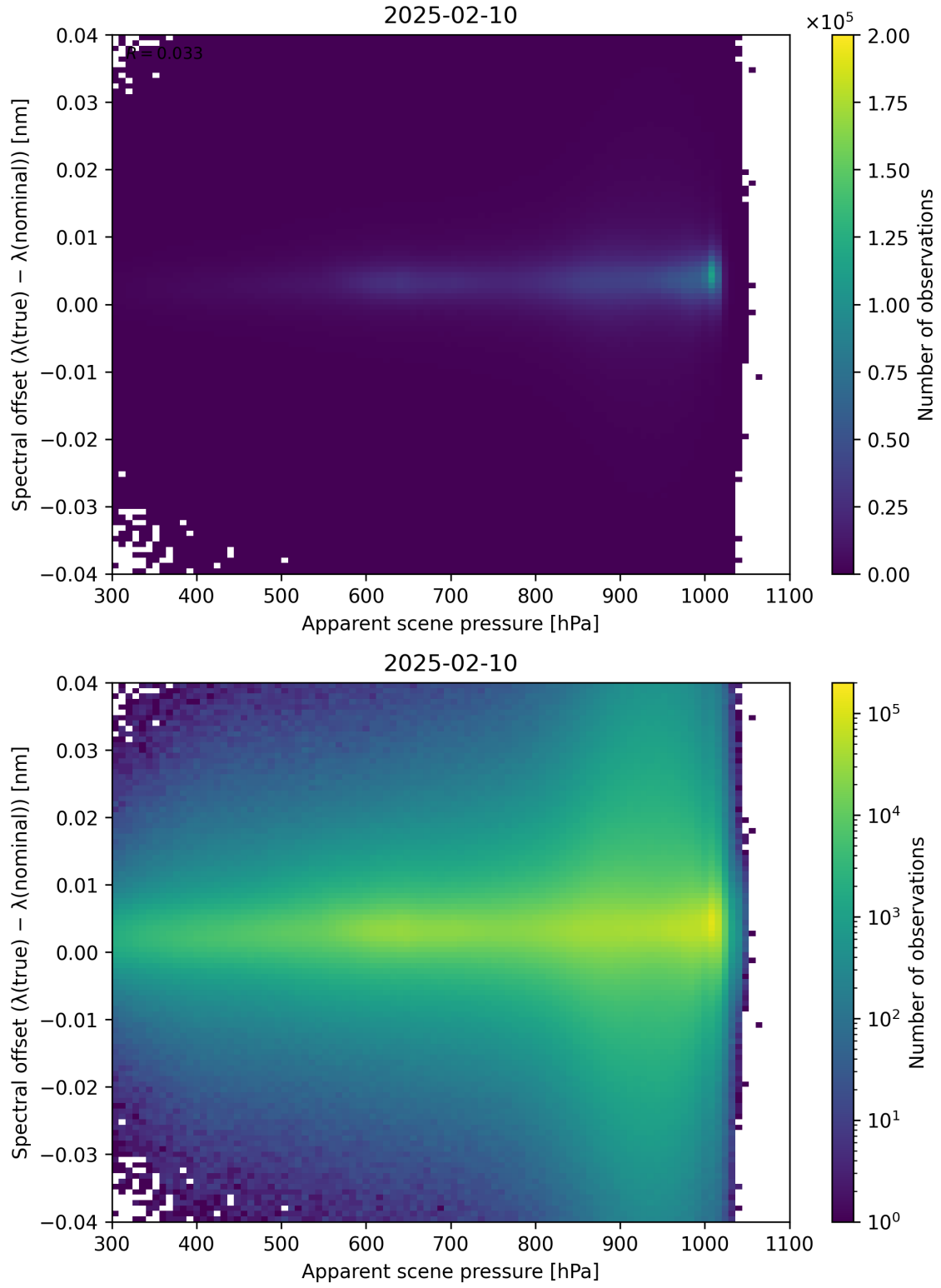
Figure 67: Scatter density plot of “Apparent scene pressure” against “Spectral offset ( \lambda_{\text{true}} - \lambda_{\text{nominal}} )” for 2025-02-09 to 2025-02-11.
