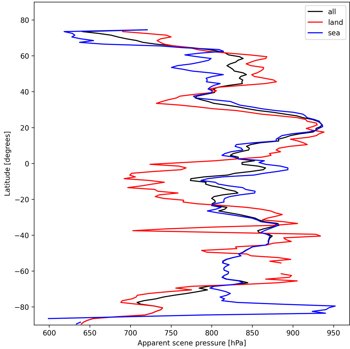
Figure 19: Zonal average of “Apparent scene pressure” for 2025-02-09 to 2025-02-11.
