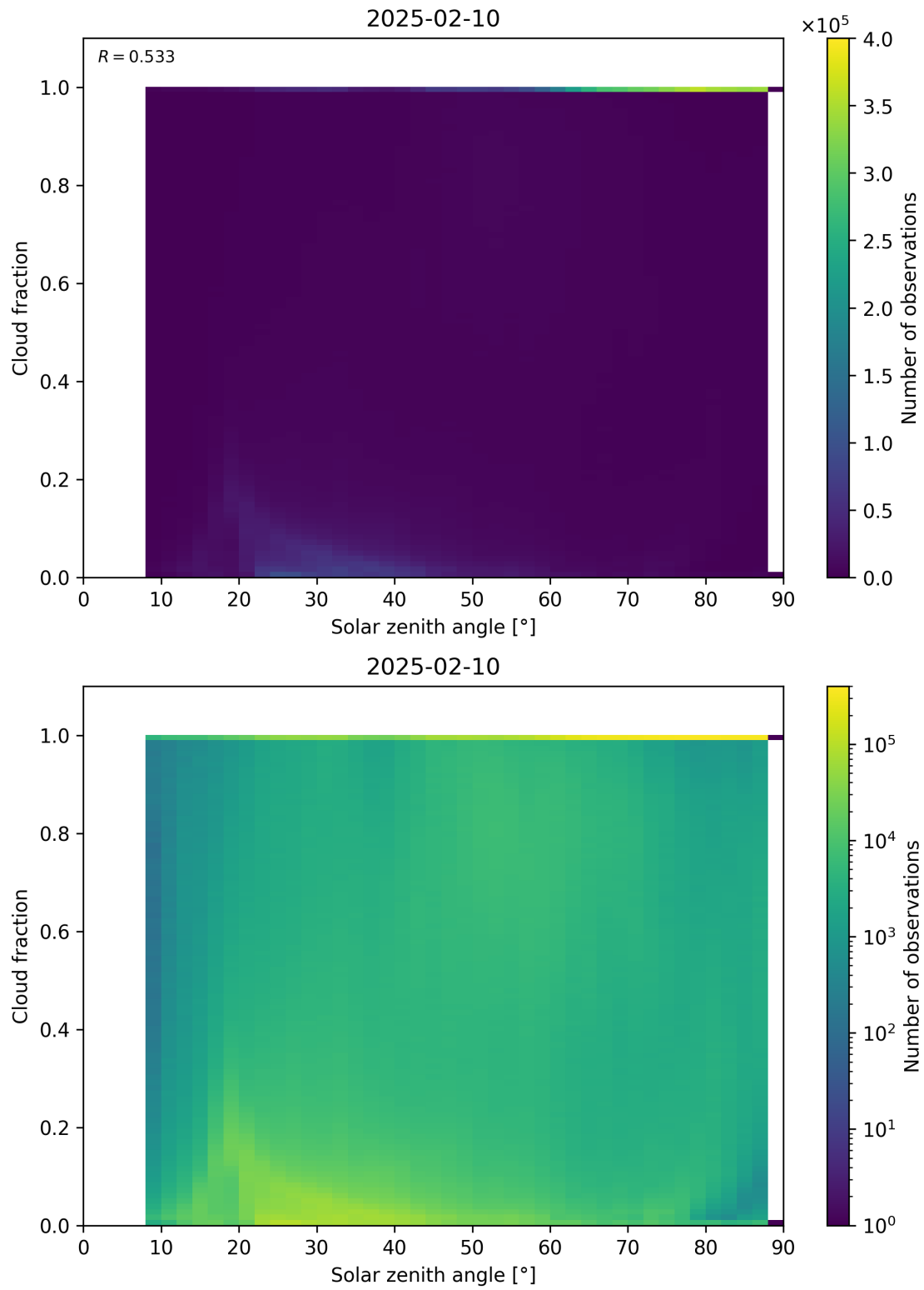
Figure 110: Scatter density plot of “Solar zenith angle” against “Cloud fraction” for 2025-02-09 to 2025-02-11.
