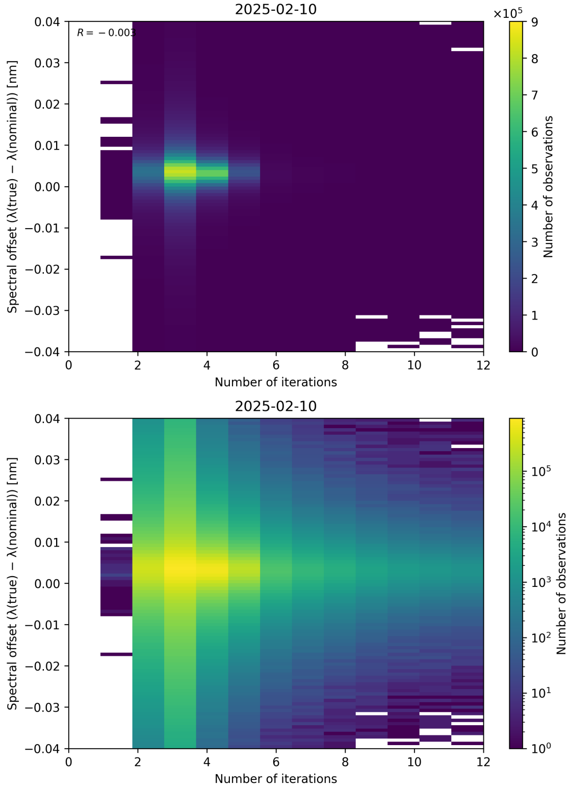
Figure 100: Scatter density plot of “Number of iterations” against “Spectral offset ( \lambda_{\text{true}} - \lambda_{\text{nominal}} )” for 2025-02-09 to 2025-02-11.
