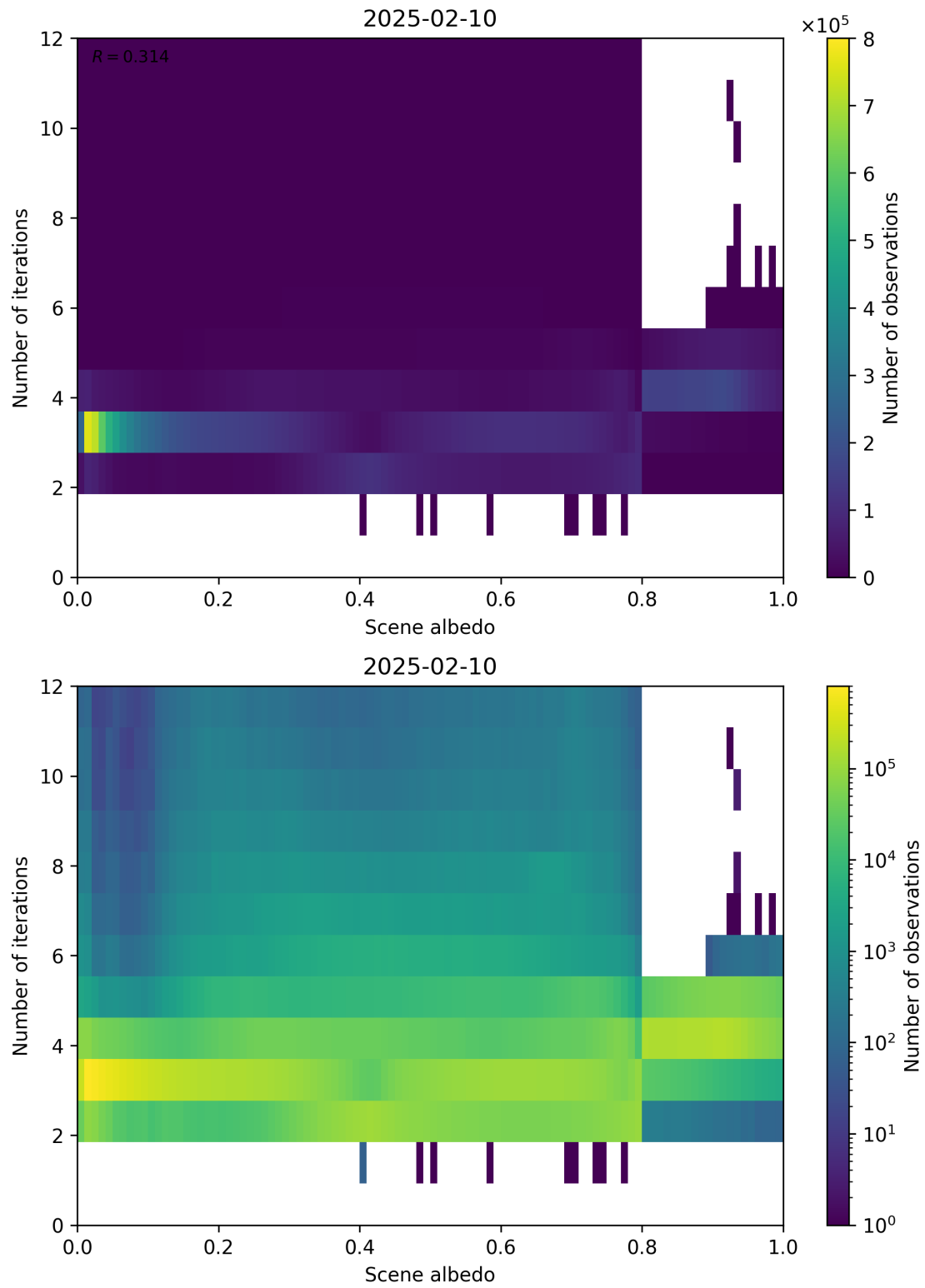
Figure 105: Scatter density plot of “Scene albedo” against “Number of iterations” for 2025-02-09 to 2025-02-11.
