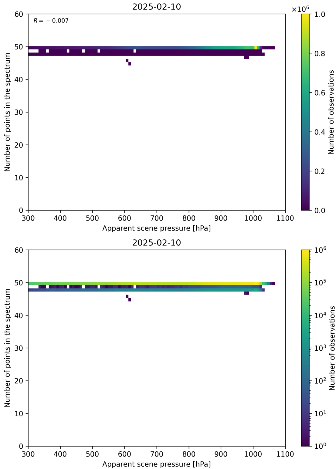
Figure 66: Scatter density plot of “Apparent scene pressure” against “Number of points in the spectrum” for 2025-02-09 to 2025-02-11.
