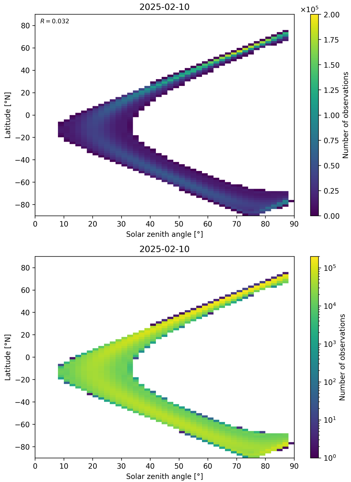
Figure 113: Scatter density plot of “Solar zenith angle” against “Latitude” for 2025-02-09 to 2025-02-11.
