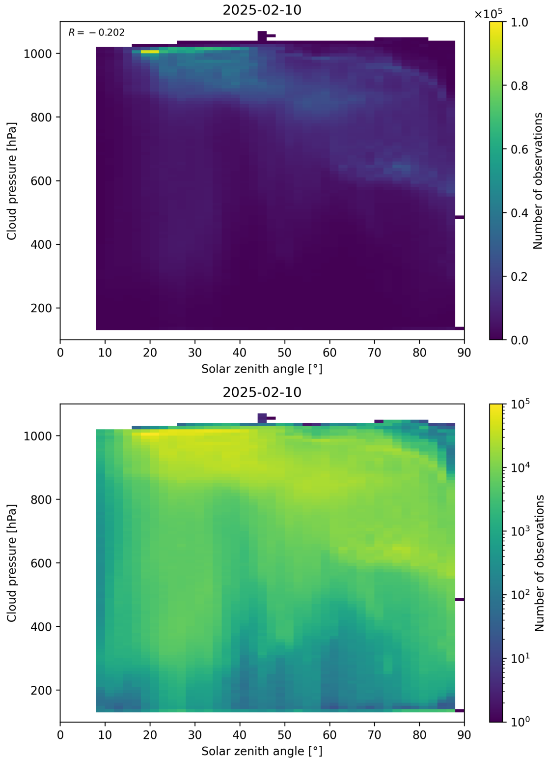
Figure 111: Scatter density plot of “Solar zenith angle” against “Cloud pressure” for 2025-02-09 to 2025-02-11.
