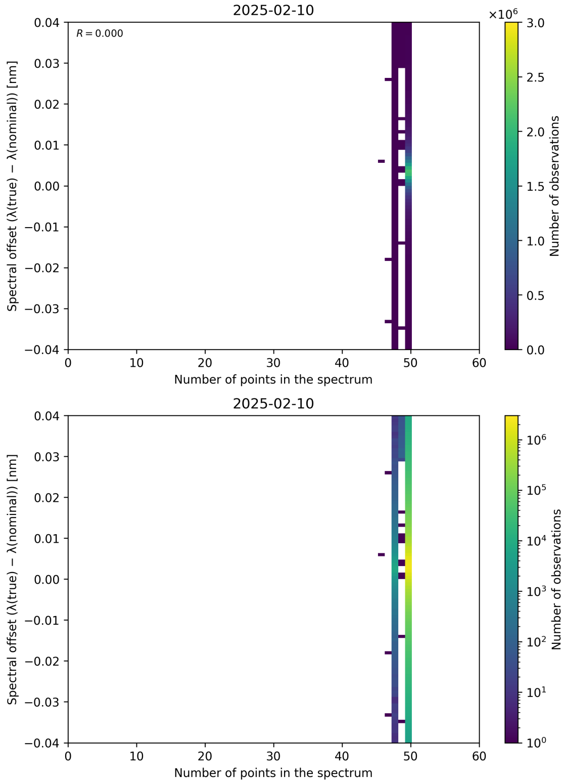
Figure 101: Scatter density plot of “Number of points in the spectrum” against “Spectral offset ( \lambda_{\text{true}} - \lambda_{\text{nominal}} )” for 2025-02-09 to 2025-02-11.
