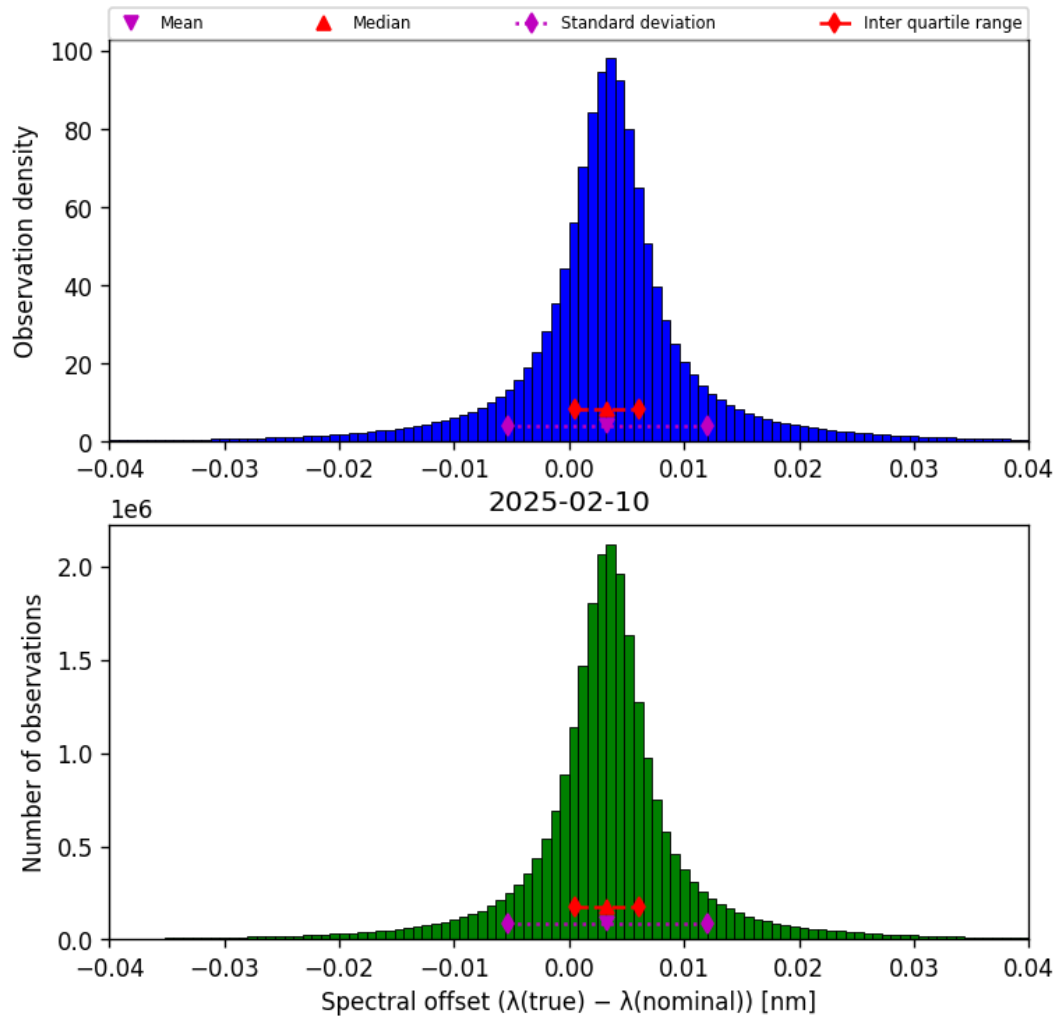
Figure 45: Histogram of “Spectral offset ( \lambda_{\text{true}} - \lambda_{\text{nominal}} )” for 2025-02-09 to 2025-02-11
