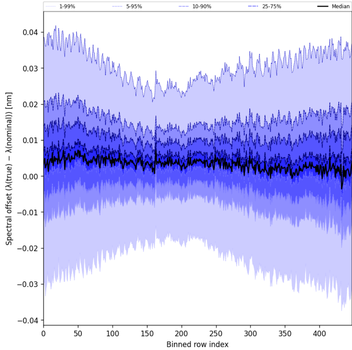
Figure 62: Along track statistics of “Spectral offset ( \lambda_{\text{true}} - \lambda_{\text{nominal}} )” for 2025-02-09 to 2025-02-11
