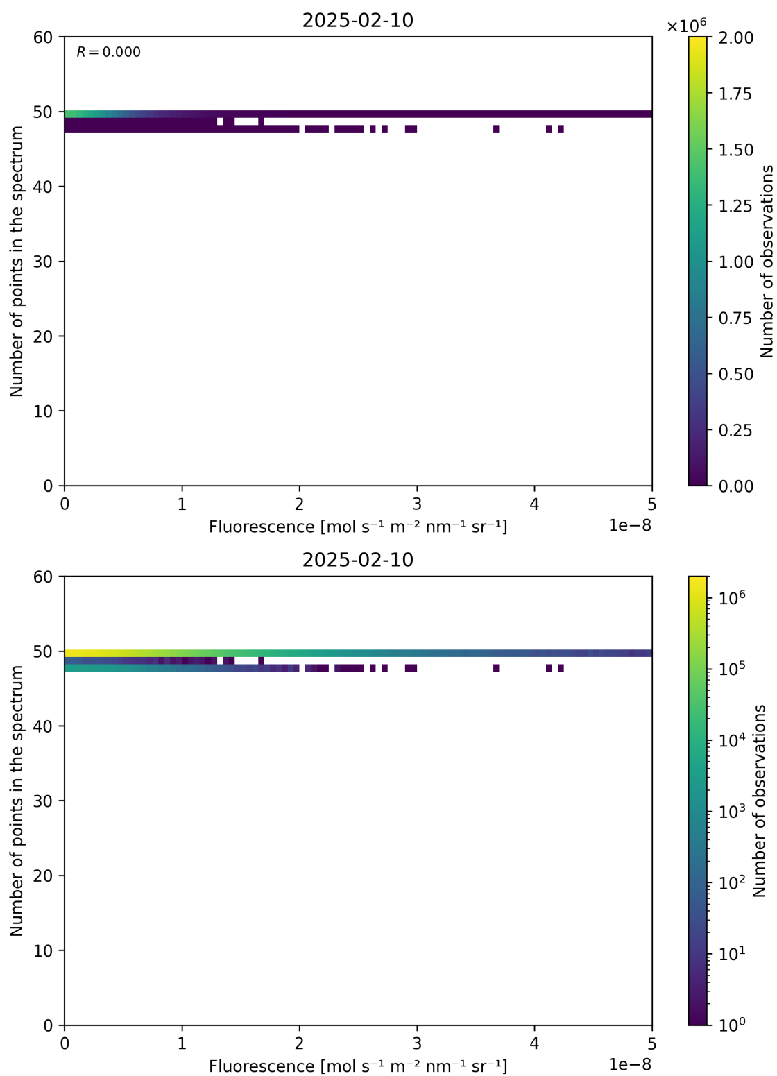
Figure 86: Scatter density plot of “Fluorescence” against “Number of points in the spectrum” for 2025-02-09 to 2025-02-11.
