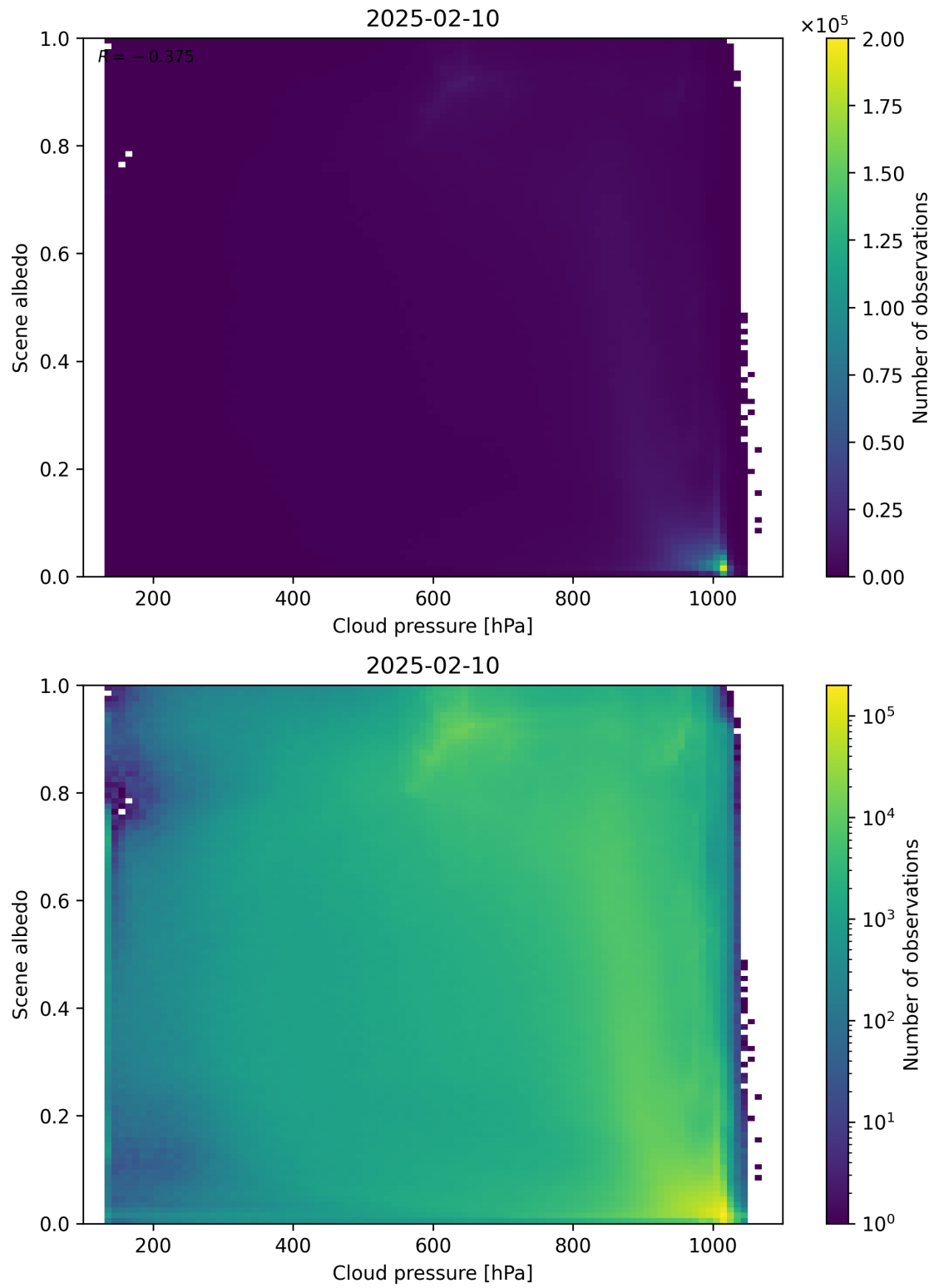
Figure 83: Scatter density plot of “Cloud pressure” against “Scene albedo” for 2025-02-09 to 2025-02-11.
