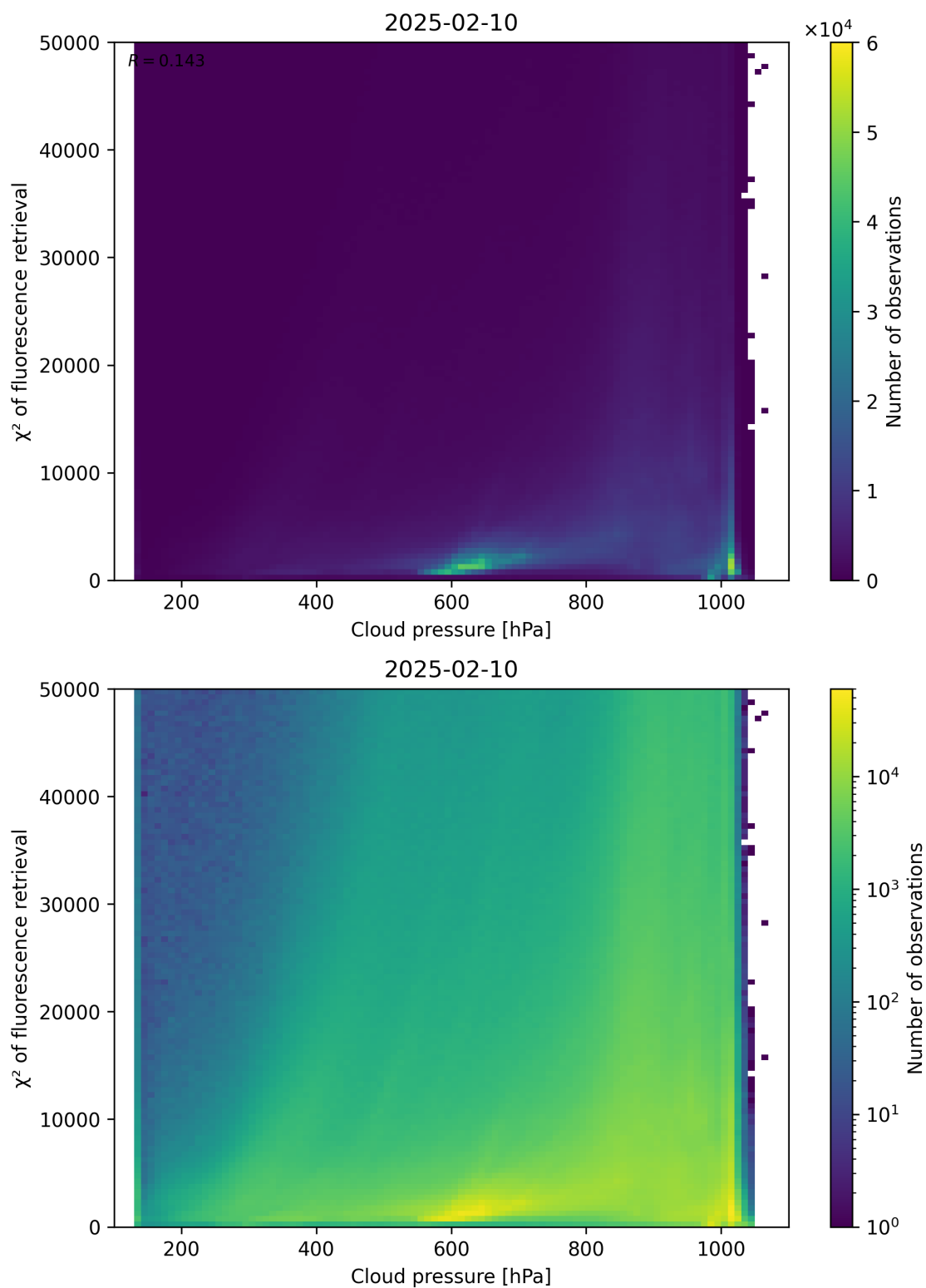
Figure 78: Scatter density plot of “Cloud pressure” against “ \chi^2 of fluorescence retrieval” for 2025-02-09 to 2025-02-11.
