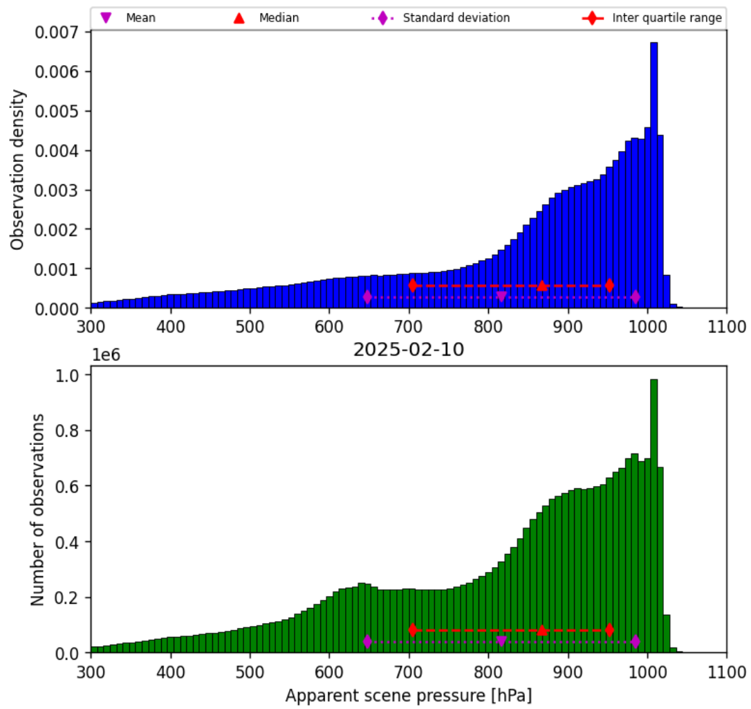
Figure 36: Histogram of “Apparent scene pressure” for 2025-02-09 to 2025-02-11
