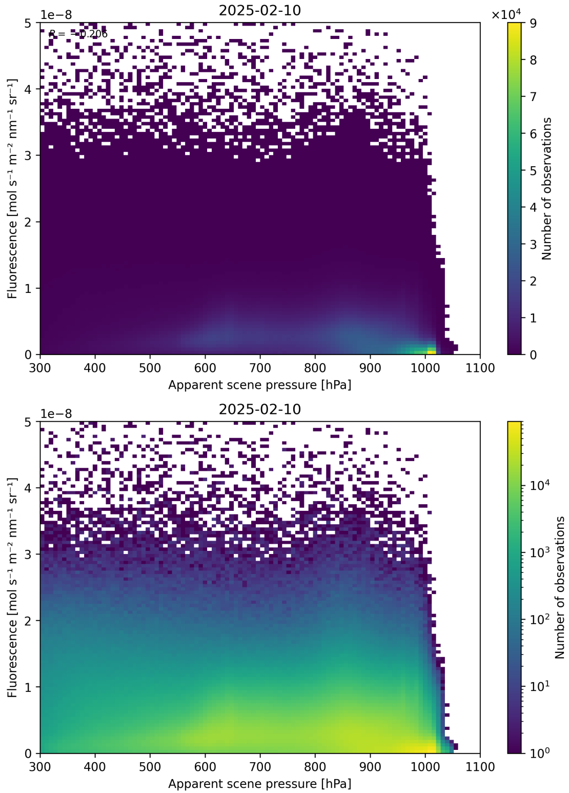
Figure 64: Scatter density plot of “Apparent scene pressure” against “Fluorescence” for 2025-02-09 to 2025-02-11.
