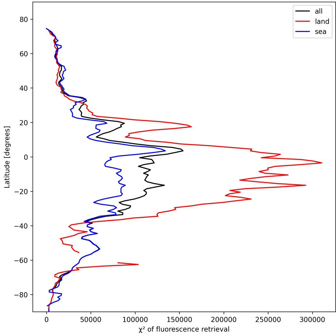
Figure 25: Zonal average of “ \chi^2 of fluorescence retrieval” for 2025-02-09 to 2025-02-11.
