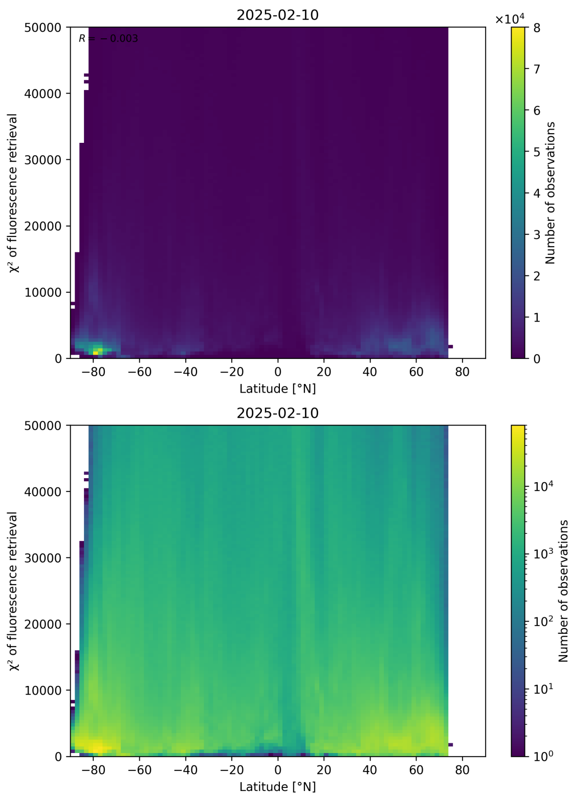
Figure 89: Scatter density plot of “Latitude” against “ \chi^2 of fluorescence retrieval” for 2025-02-09 to 2025-02-11.
