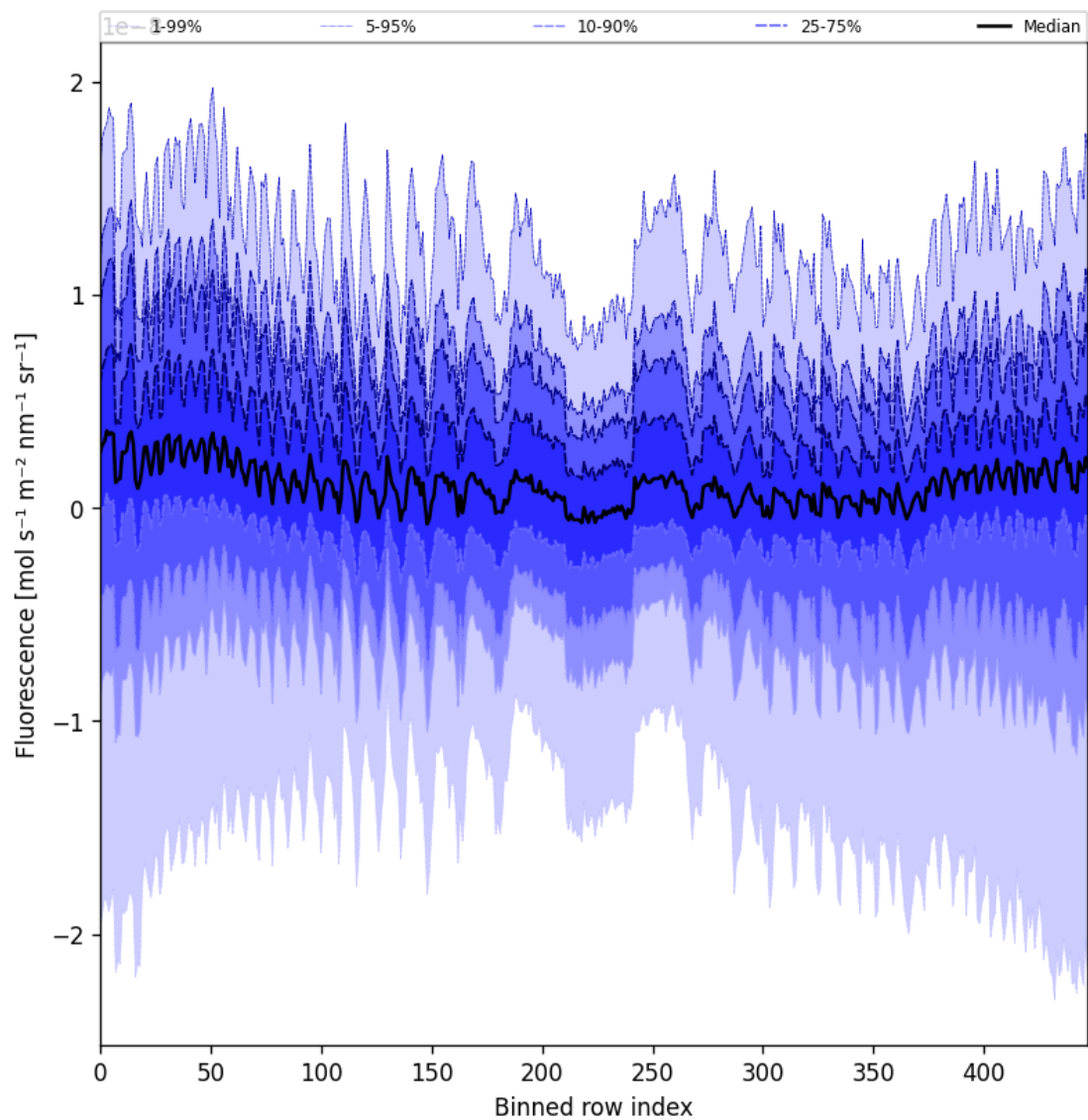
Figure 57: Along track statistics of “Fluorescence” for 2025-02-09 to 2025-02-11
