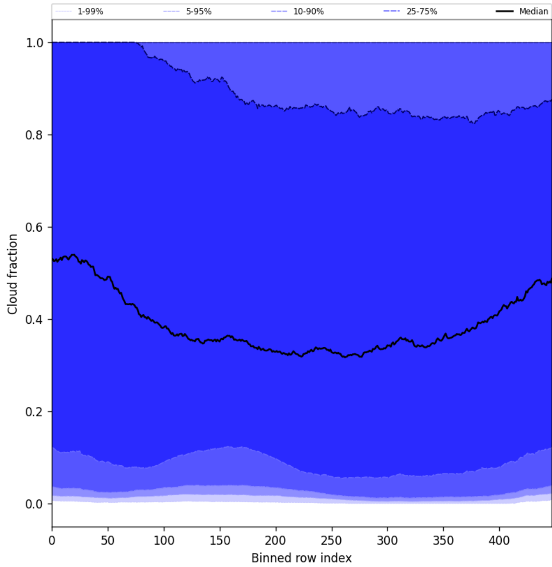
Figure 49: Along track statistics of “Cloud fraction” for 2025-02-09 to 2025-02-11
