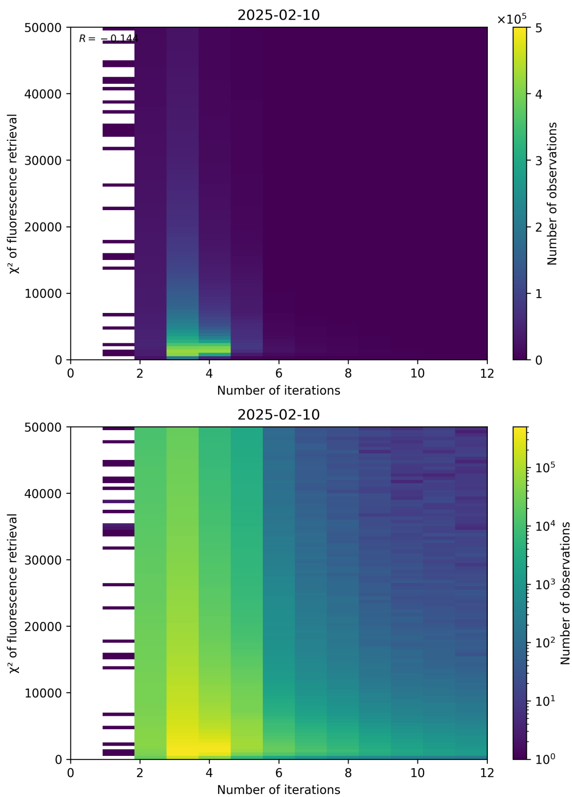
Figure 97: Scatter density plot of “Number of iterations” against “ \chi^2 of fluorescence retrieval” for 2025-02-09 to 2025-02-11.
