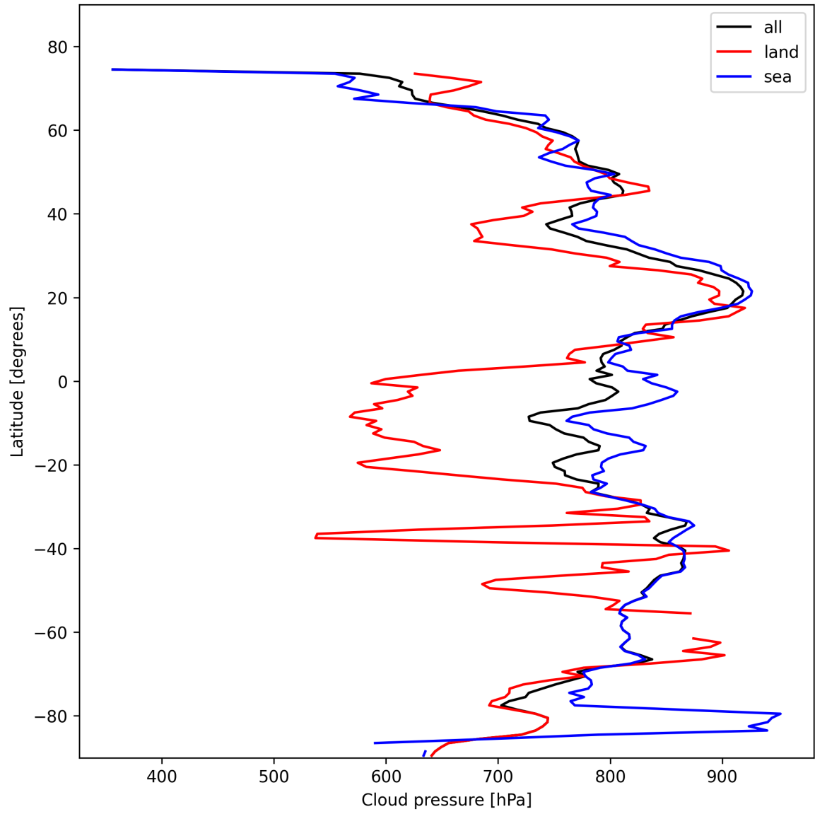
Figure 13: Zonal average of “Cloud pressure” for 2025-02-09 to 2025-02-11.
