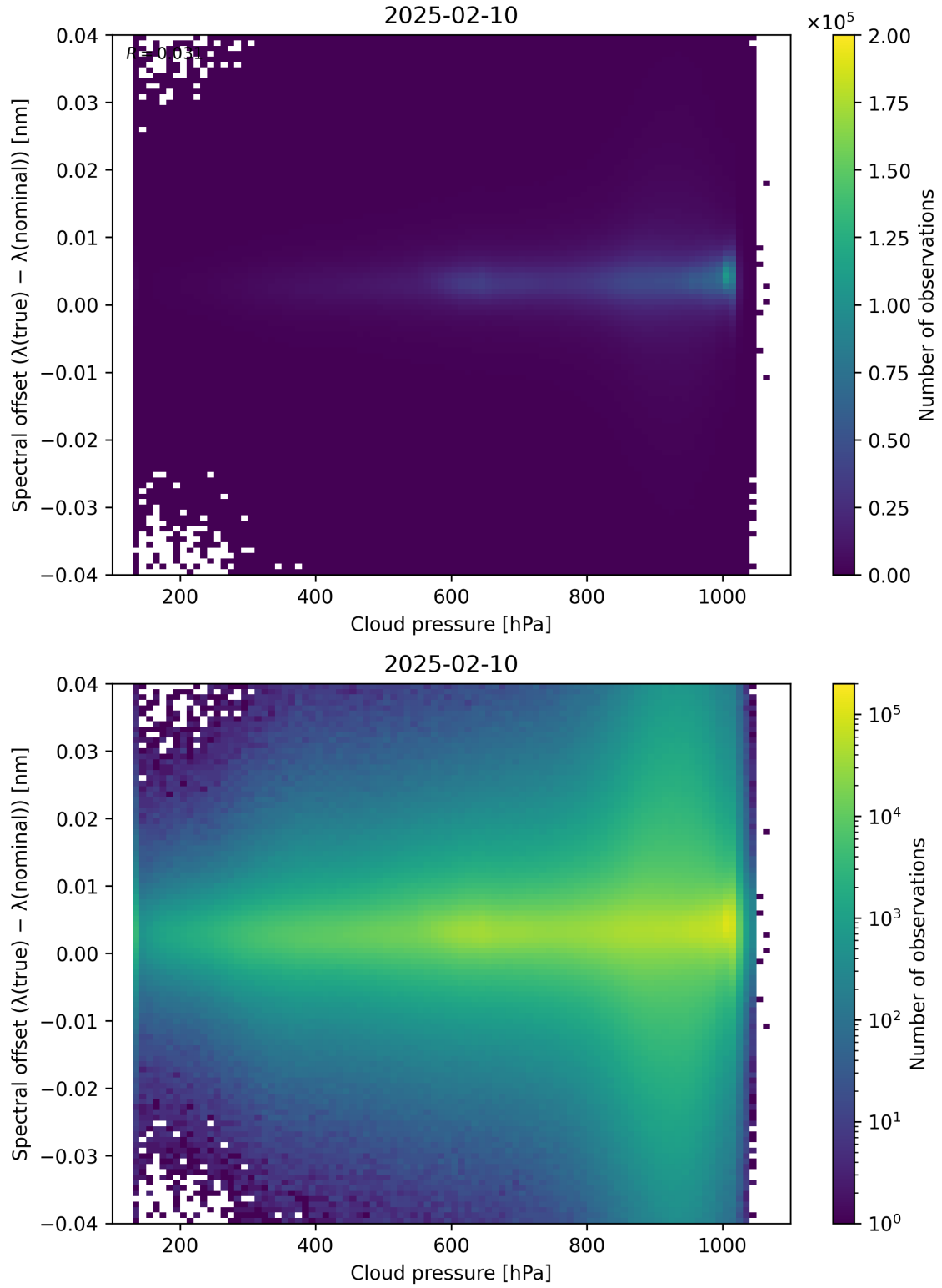
Figure 84: Scatter density plot of “Cloud pressure” against “Spectral offset ( \lambda_{\text{true}} - \lambda_{\text{nominal}} )” for 2025-02-09 to 2025-02-11.
