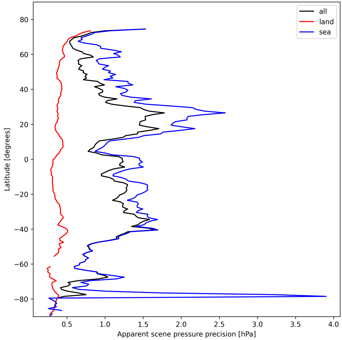
Figure 20: Zonal average of “Apparent scene pressure precision” for 2025-02-09 to 2025-02-11.
