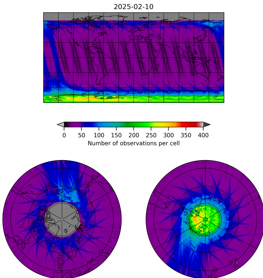
Figure 11: Map of the number of observations for 2025-02-09 to 2025-02-11
