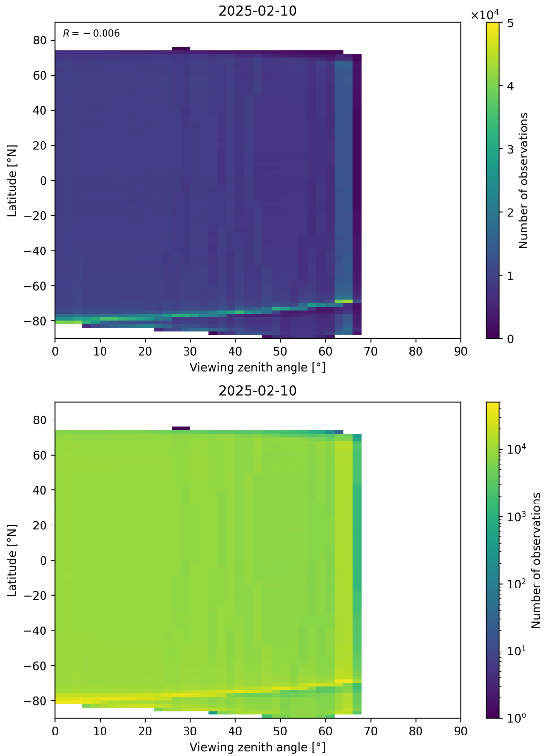
Figure 123: Scatter density plot of “Viewing zenith angle” against “Latitude” for 2025-02-09 to 2025-02-11.
