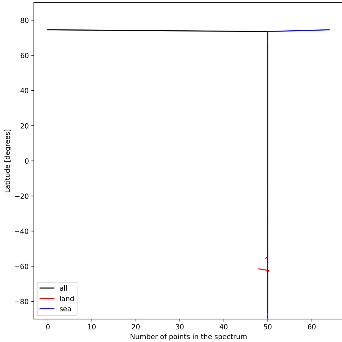
Figure 27: Zonal average of “Number of points in the spectrum” for 2025-02-09 to 2025-02-11.
