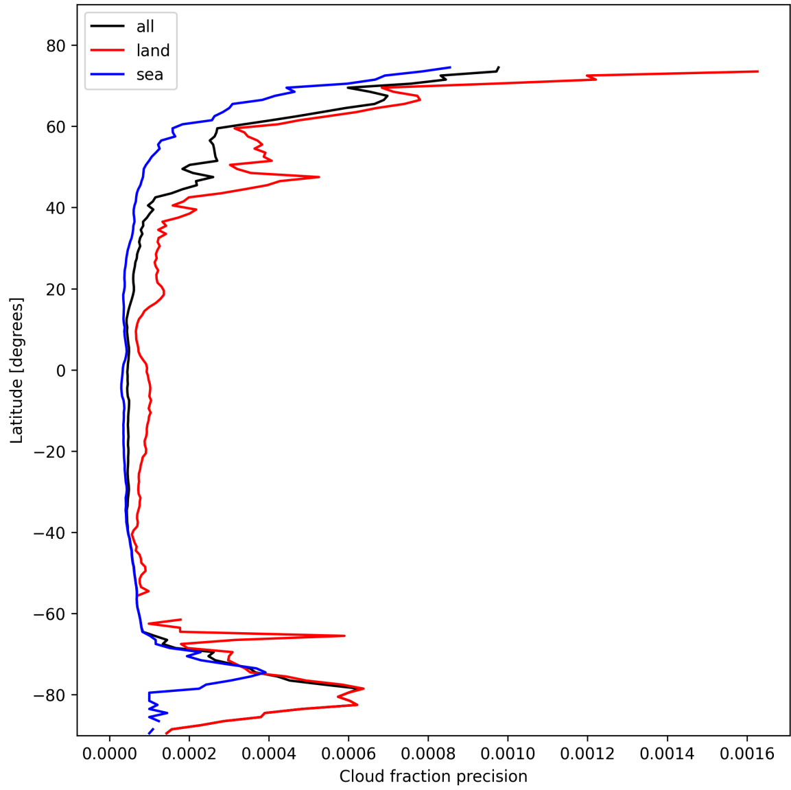
Figure 16: Zonal average of “Cloud fraction precision” for 2025-02-09 to 2025-02-11.
