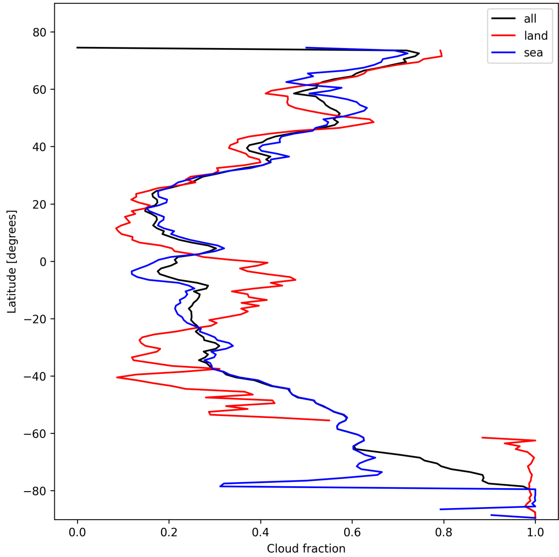
Figure 15: Zonal average of “Cloud fraction” for 2025-02-09 to 2025-02-11.
