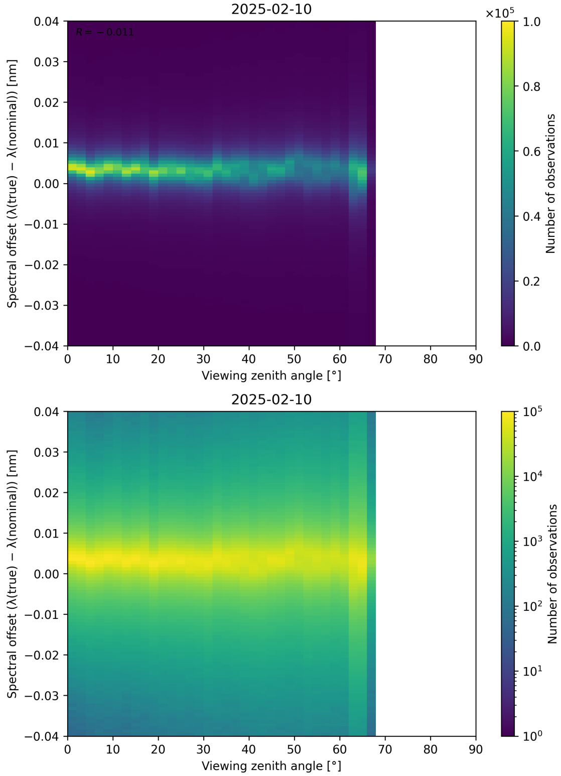
Figure 128: Scatter density plot of “Viewing zenith angle” against “Spectral offset ( \lambda_{\text{true}} - \lambda_{\text{nominal}} )” for 2025-02-09 to 2025-02-11.
