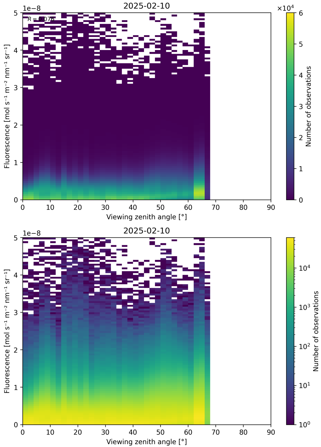
Figure 122: Scatter density plot of “Viewing zenith angle” against “Fluorescence” for 2025-02-09 to 2025-02-11.
