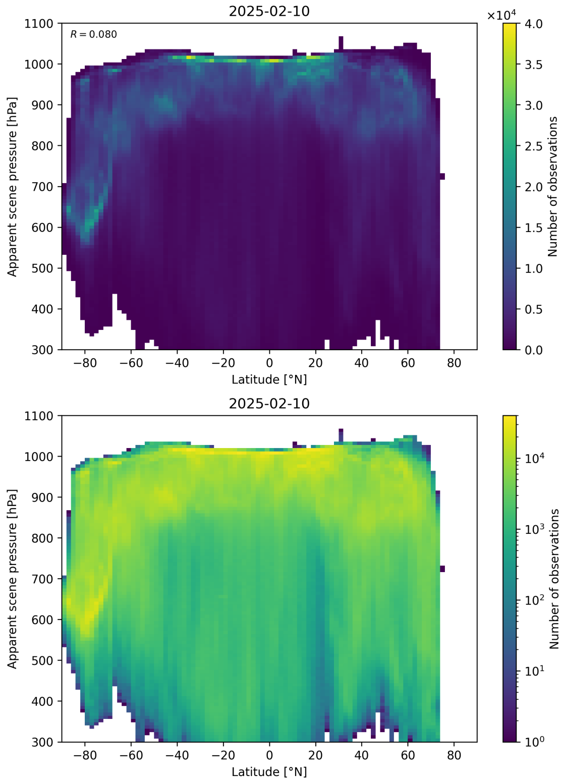
Figure 88: Scatter density plot of “Latitude” against “Apparent scene pressure” for 2025-02-09 to 2025-02-11.
