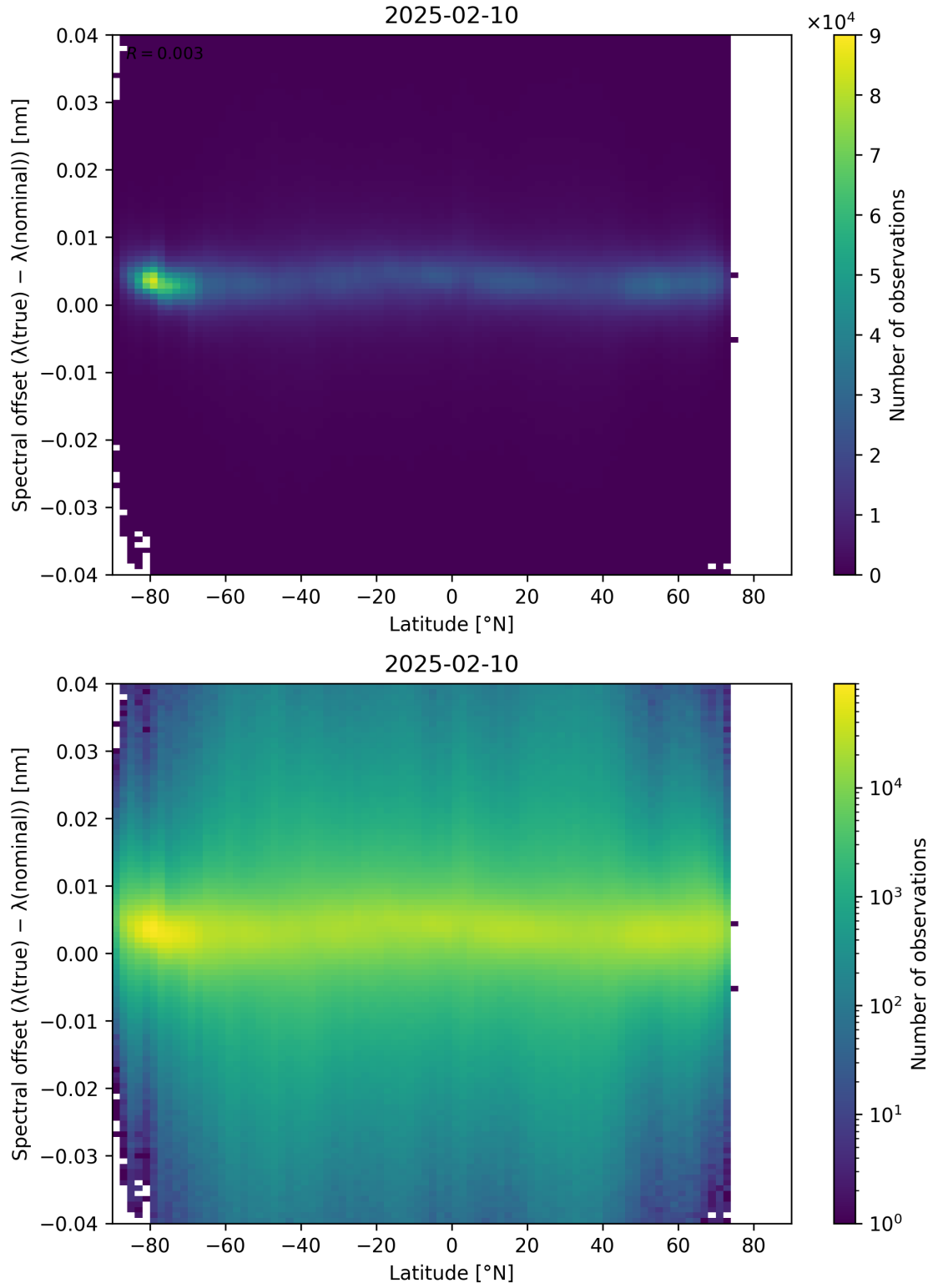
Figure 96: Scatter density plot of “Latitude” against “Spectral offset ( \lambda_{\text{true}} - \lambda_{\text{nominal}} )” for 2025-02-09 to 2025-02-11.
