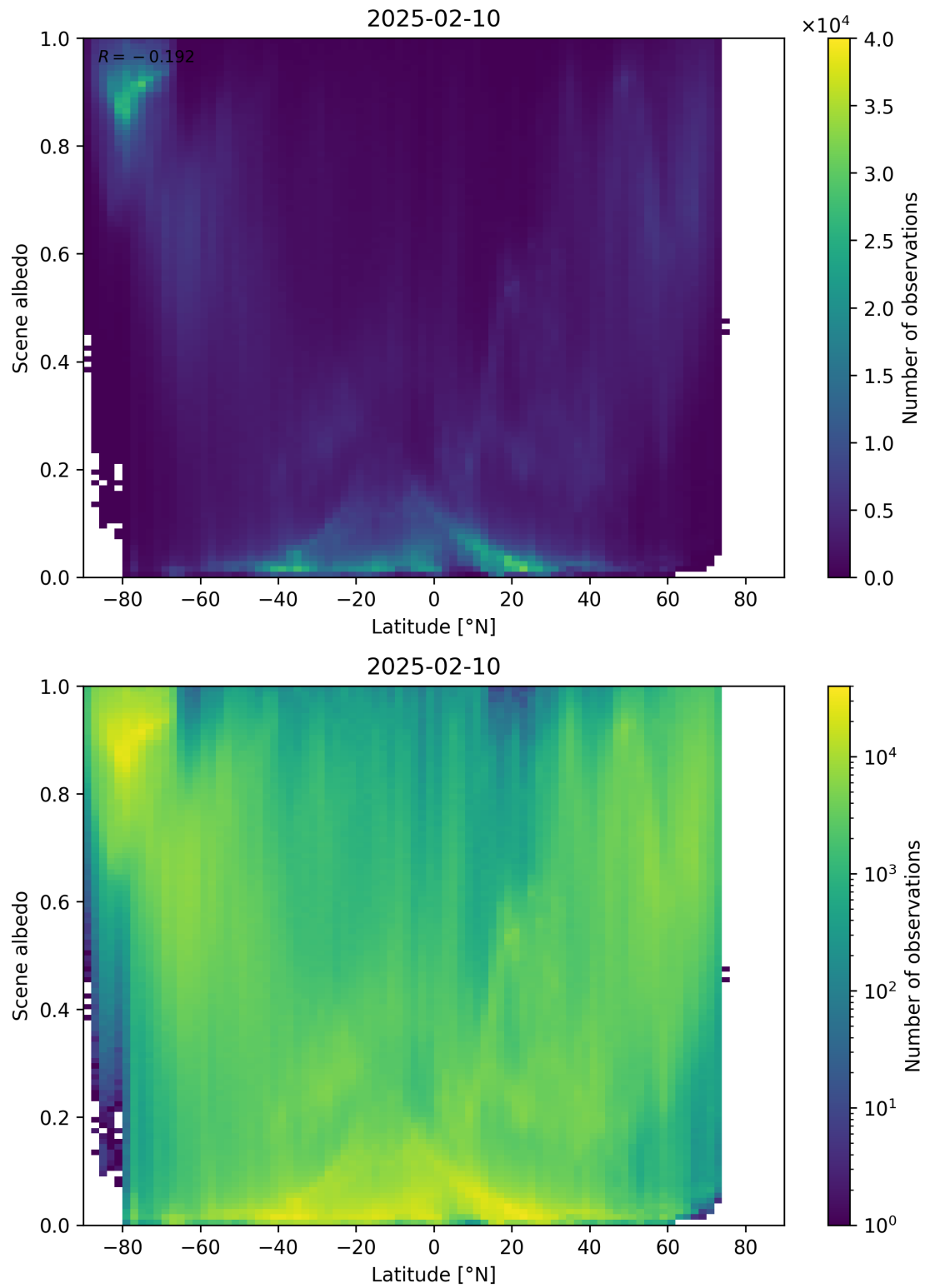
Figure 95: Scatter density plot of “Latitude” against “Scene albedo” for 2025-02-09 to 2025-02-11.
