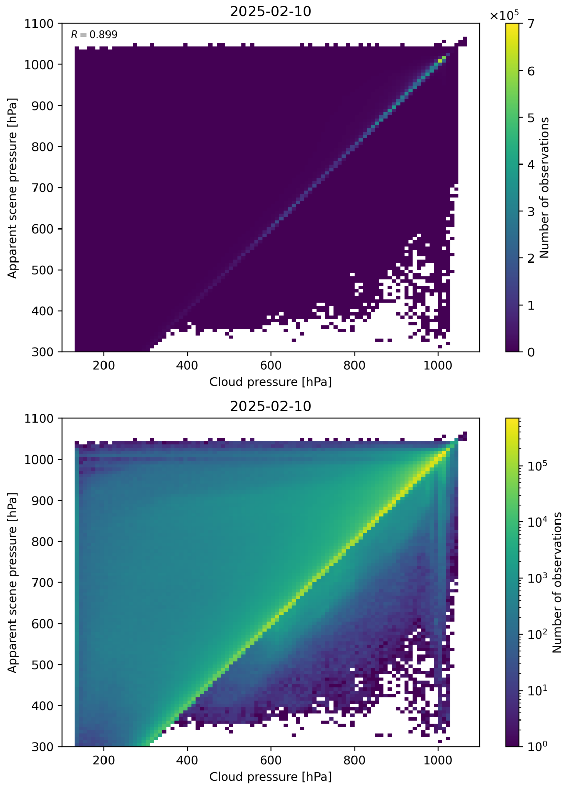
Figure 77: Scatter density plot of “Cloud pressure” against “Apparent scene pressure” for 2025-02-09 to 2025-02-11.
