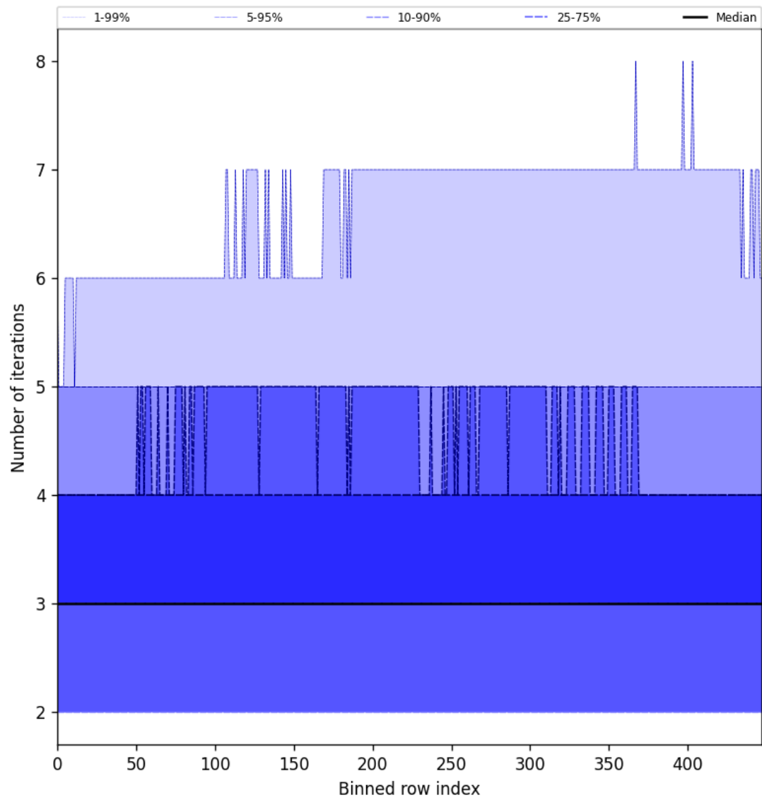
Figure 56: Along track statistics of “Number of iterations” for 2025-02-09 to 2025-02-11
