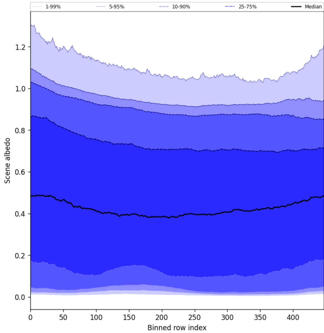
Figure 51: Along track statistics of “Scene albedo” for 2025-02-09 to 2025-02-11
