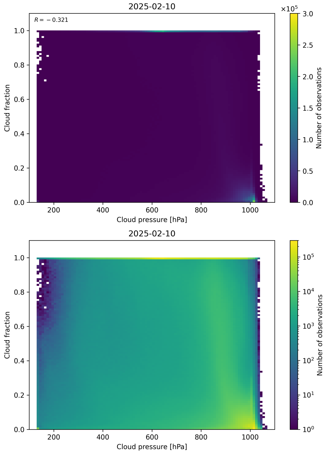
Figure 79: Scatter density plot of “Cloud pressure” against “Cloud fraction” for 2025-02-09 to 2025-02-11.
