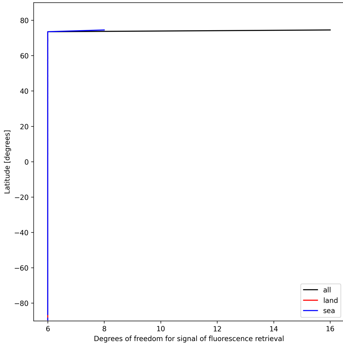
Figure 26: Zonal average of “Degrees of freedom for signal of fluorescence retrieval” for 2025-02-09 to 2025-02-11.
