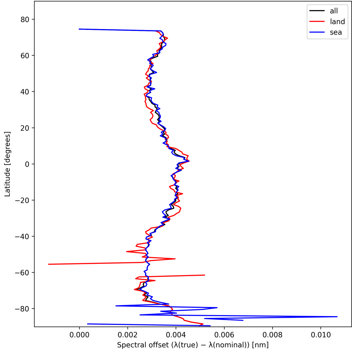
Figure 28: Zonal average of “Spectral offset ( \lambda_{\text{true}} - \lambda_{\text{nominal}} )” for 2025-02-09 to 2025-02-11.
