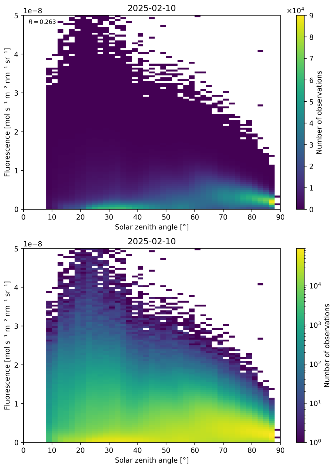
Figure 112: Scatter density plot of “Solar zenith angle” against “Fluorescence” for 2025-02-09 to 2025-02-11.
