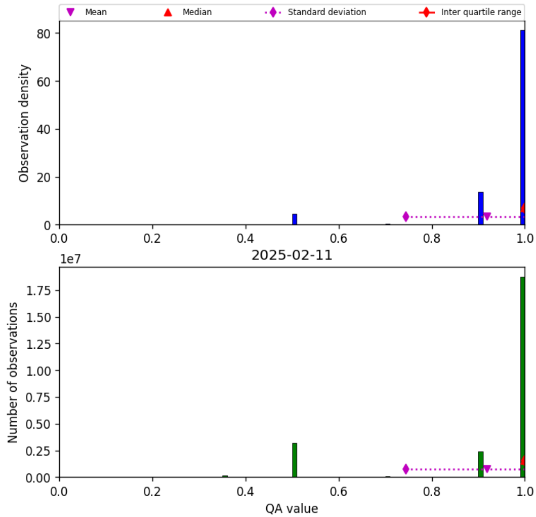
Figure 29: Histogram of “QA value” for 2025-02-10 to 2025-02-12
