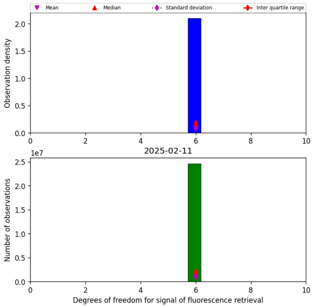
Figure 43: Histogram of “Degrees of freedom for signal of fluorescence retrieval” for 2025-02-10 to 2025-02-12
