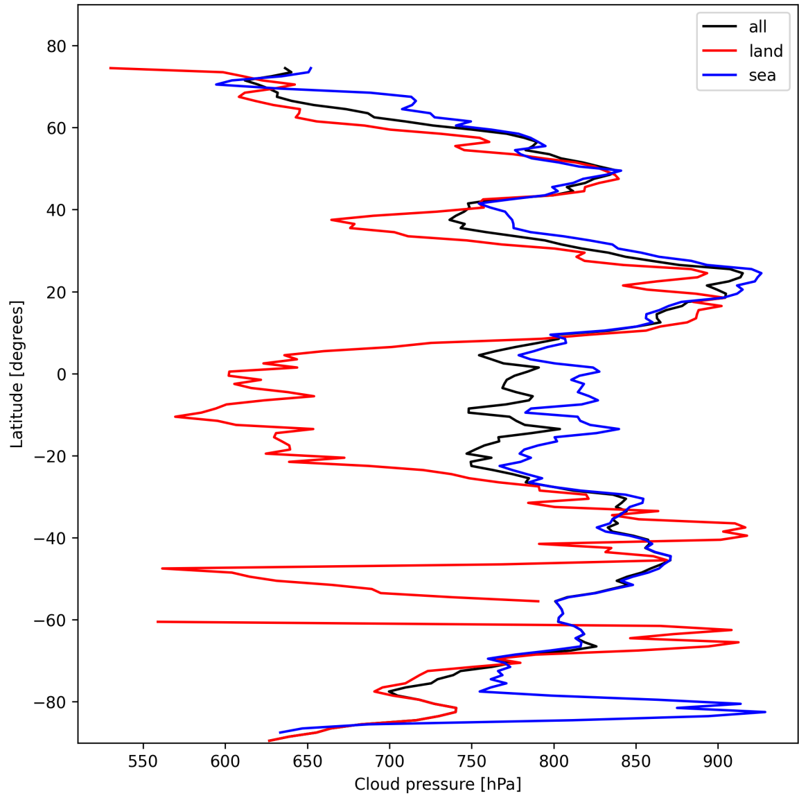
Figure 13: Zonal average of “Cloud pressure” for 2025-02-10 to 2025-02-12.
