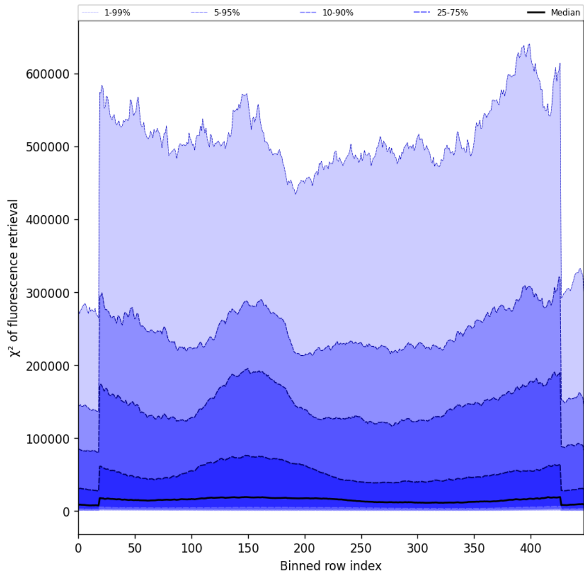
Figure 59: Along track statistics of “ \chi^2 of fluorescence retrieval” for 2025-02-10 to 2025-02-12
