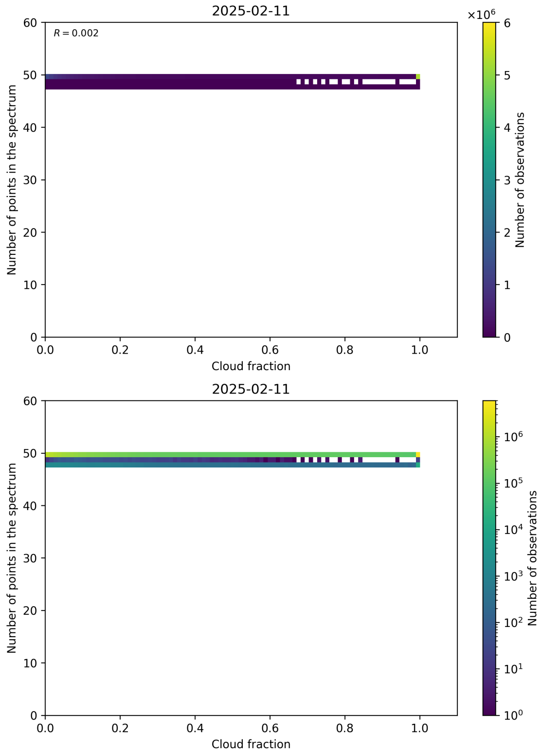
Figure 74: Scatter density plot of “Cloud fraction” against “Number of points in the spectrum” for 2025-02-10 to 2025-02-12.
