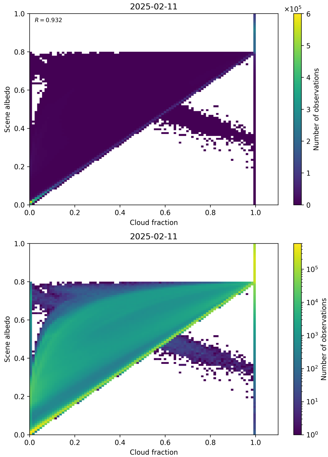
Figure 75: Scatter density plot of “Cloud fraction” against “Scene albedo” for 2025-02-10 to 2025-02-12.
