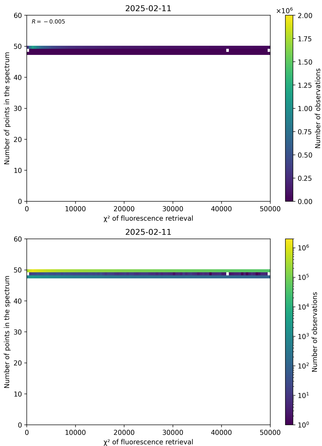
Figure 68: Scatter density plot of “ \chi^2 of fluorescence retrieval” against “Number of points in the spectrum” for 2025-02-10 to 2025-02-12.
