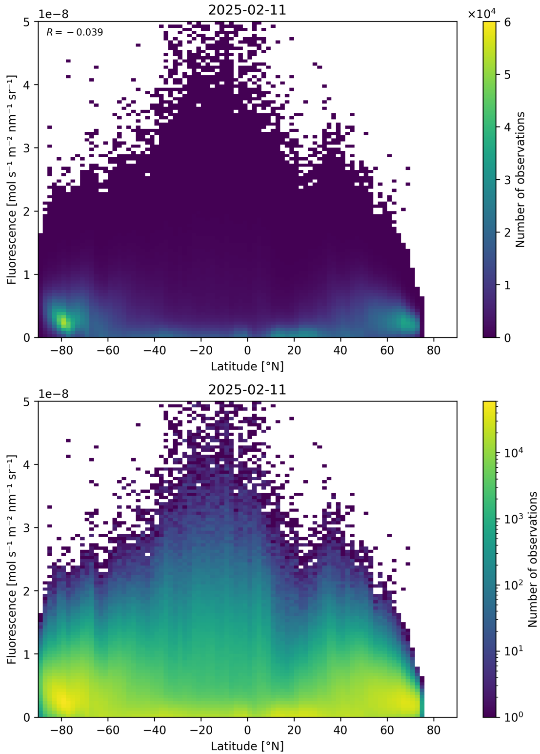
Figure 92: Scatter density plot of “Latitude” against “Fluorescence” for 2025-02-10 to 2025-02-12.
