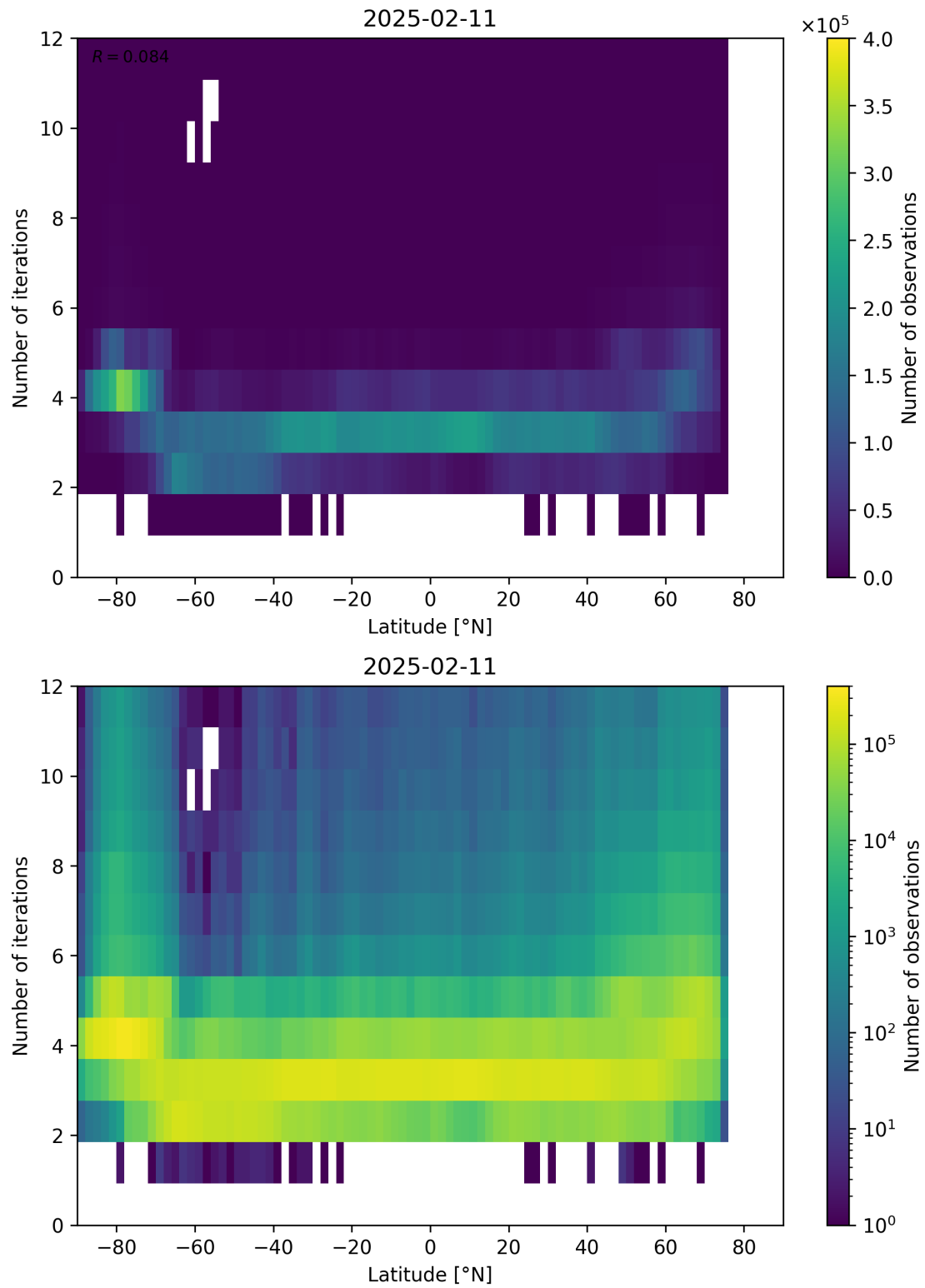
Figure 93: Scatter density plot of “Latitude” against “Number of iterations” for 2025-02-10 to 2025-02-12.
