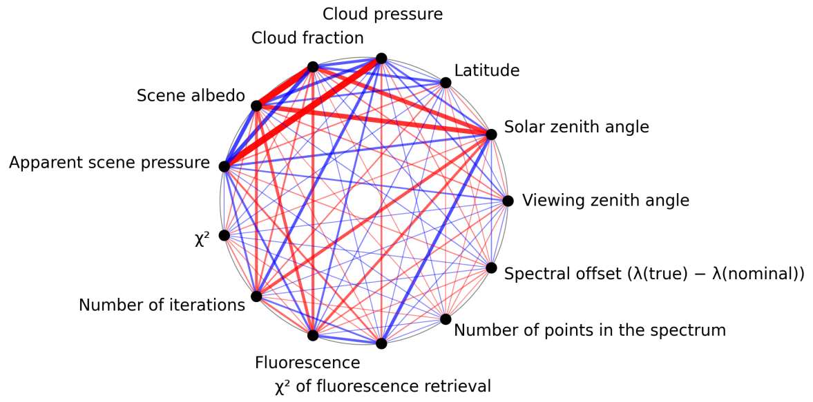
Figure 1: Map of correlation graph for 2025-02-10 to 2025-02-12.
