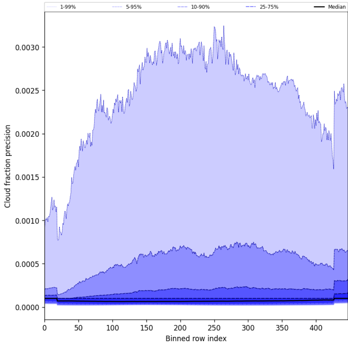
Figure 50: Along track statistics of “Cloud fraction precision” for 2025-02-10 to 2025-02-12
