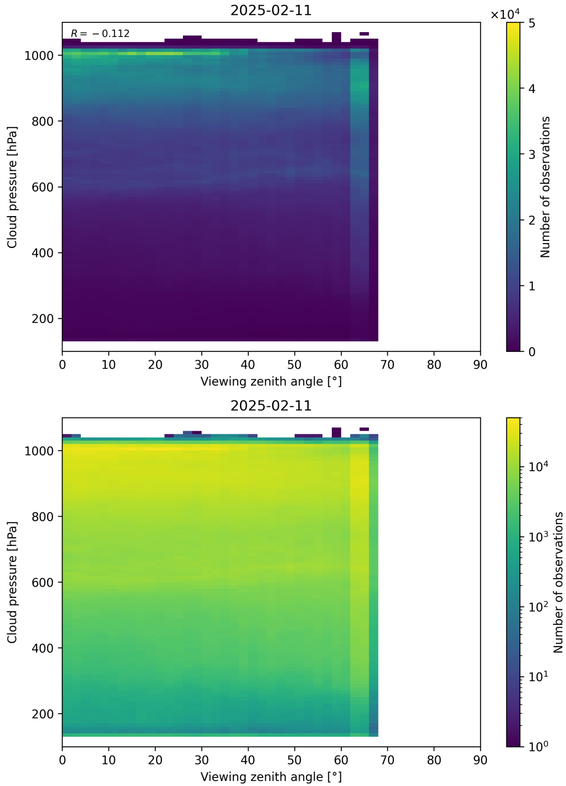
Figure 121: Scatter density plot of “Viewing zenith angle” against “Cloud pressure” for 2025-02-10 to 2025-02-12.
