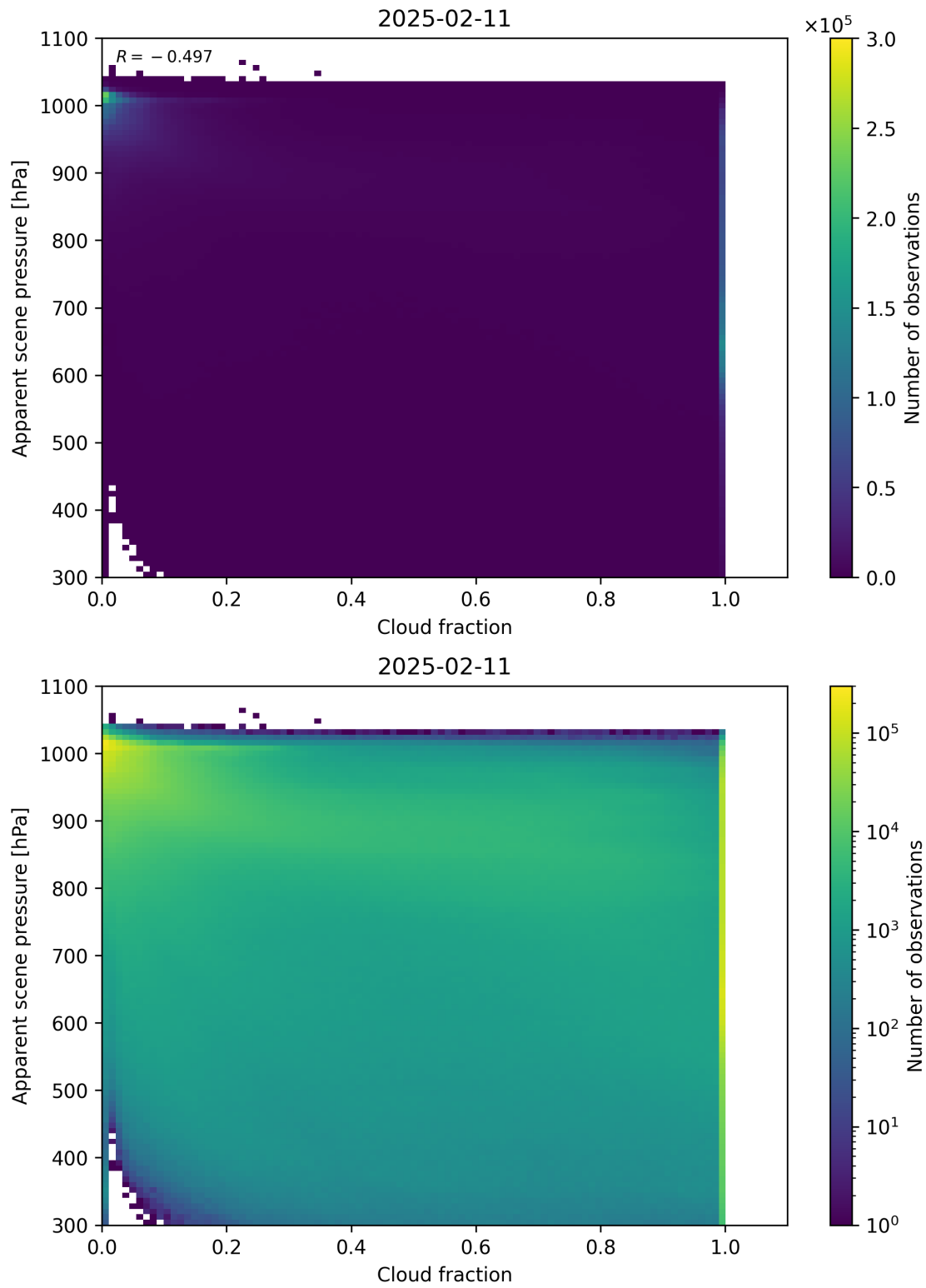
Figure 70: Scatter density plot of “Cloud fraction” against “Apparent scene pressure” for 2025-02-10 to 2025-02-12.
