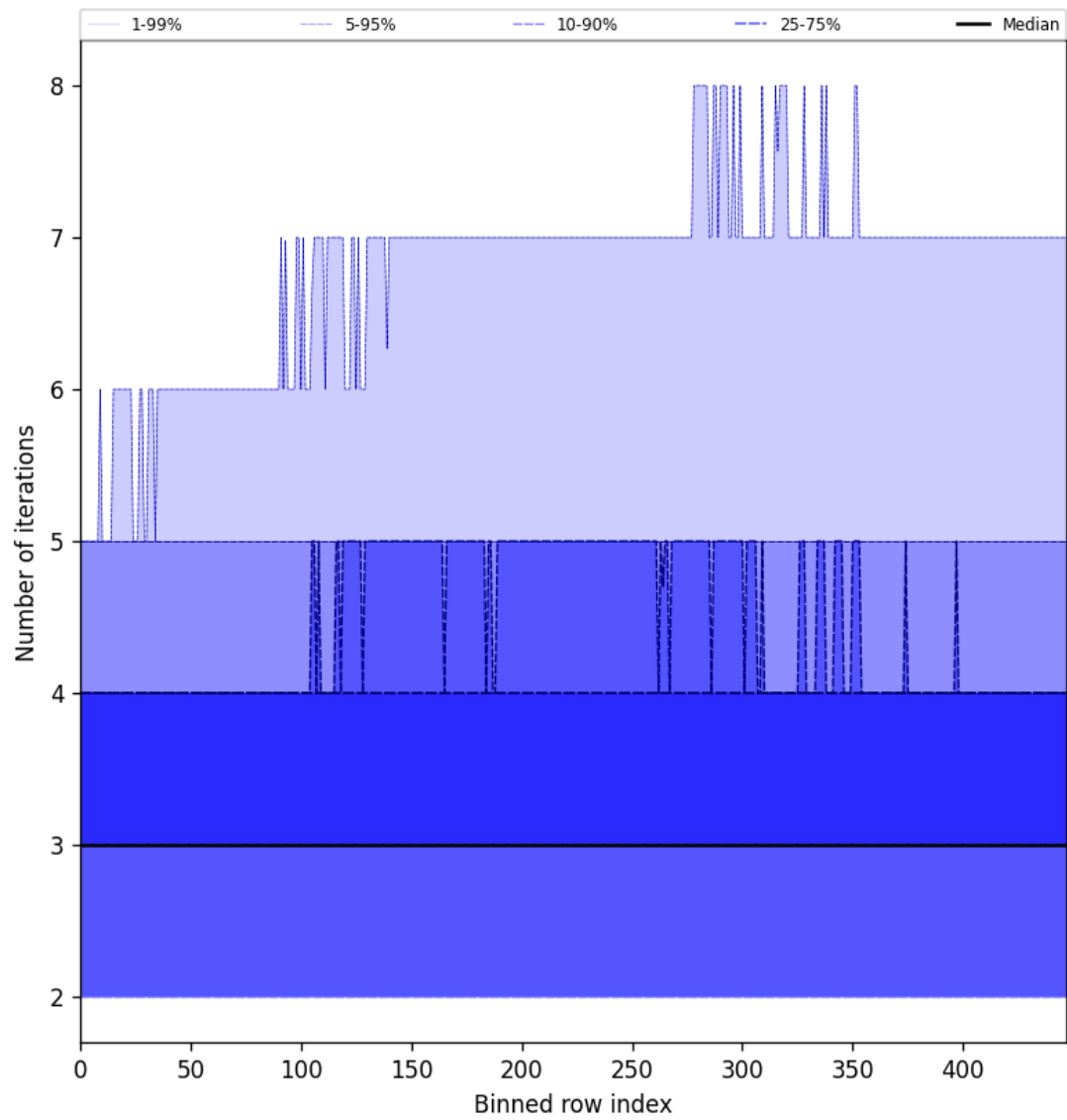
Figure 56: Along track statistics of “Number of iterations” for 2025-02-10 to 2025-02-12
