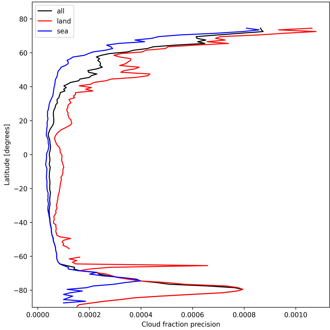
Figure 16: Zonal average of “Cloud fraction precision” for 2025-02-10 to 2025-02-12.
