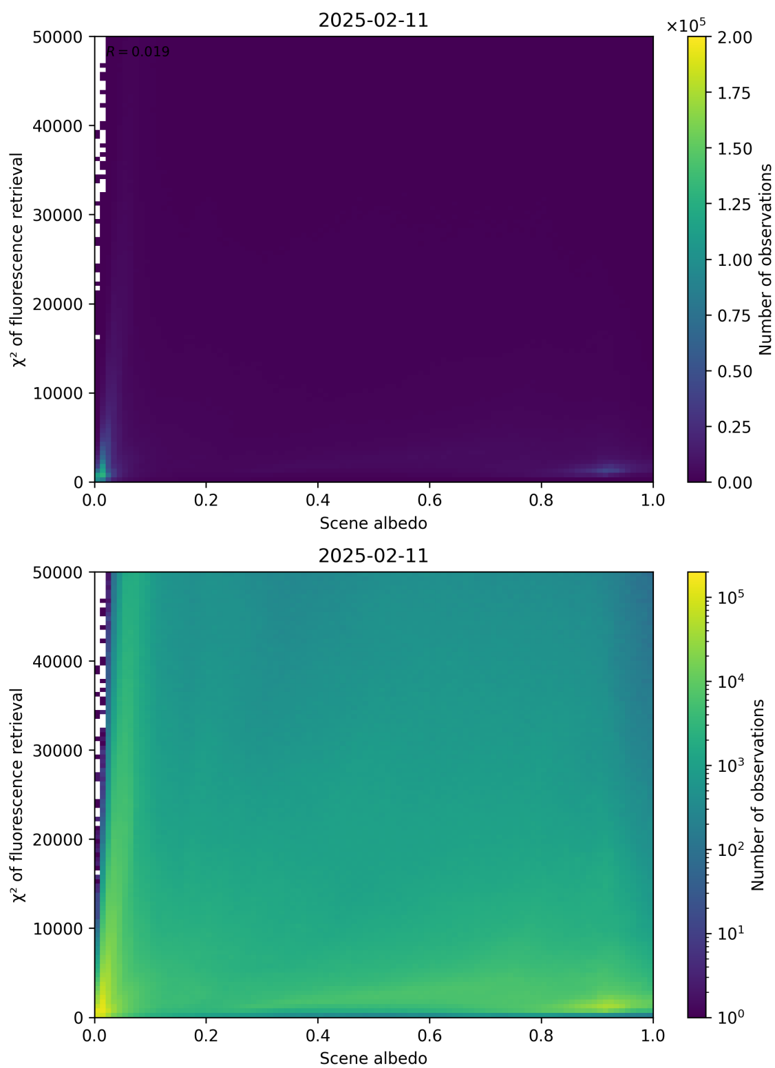
Figure 103: Scatter density plot of “Scene albedo” against “ \chi^2 of fluorescence retrieval” for 2025-02-10 to 2025-02-12.
