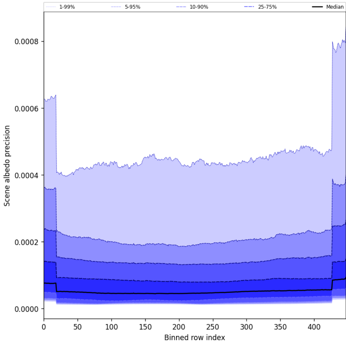
Figure 52: Along track statistics of “Scene albedo precision” for 2025-02-10 to 2025-02-12
