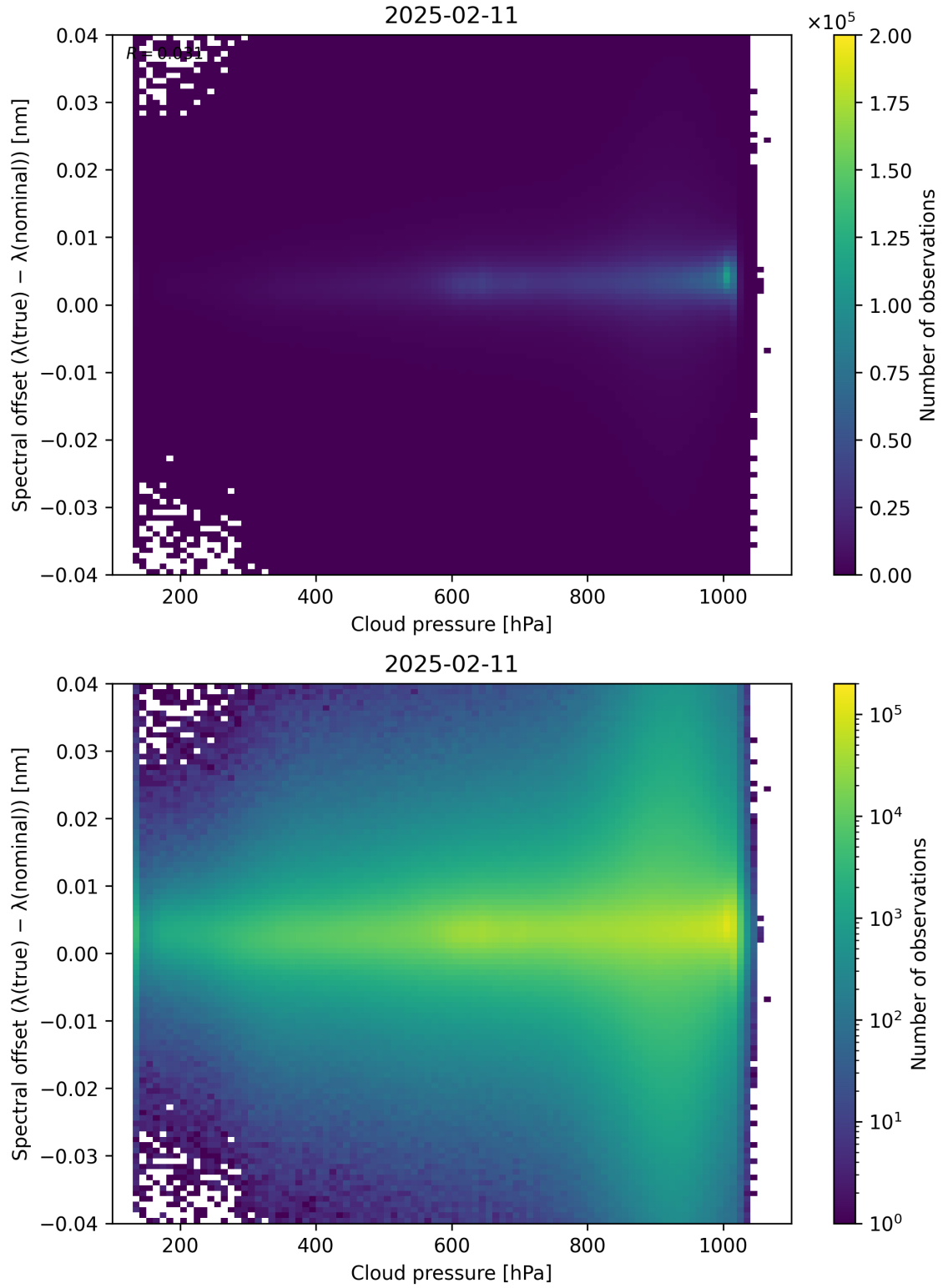
Figure 84: Scatter density plot of “Cloud pressure” against “Spectral offset ( \lambda_{\text{true}} - \lambda_{\text{nominal}} )” for 2025-02-10 to 2025-02-12.
