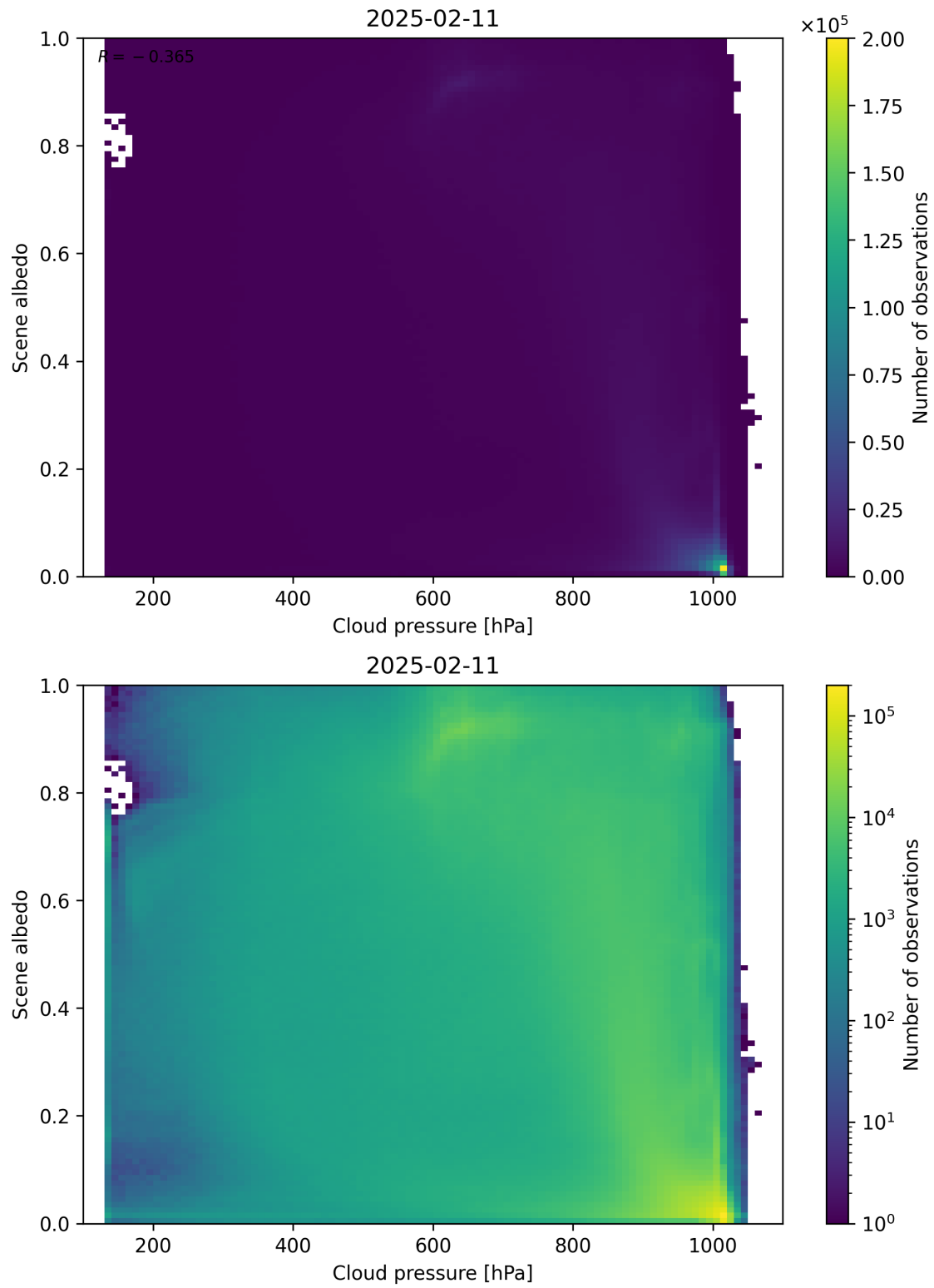
Figure 83: Scatter density plot of “Cloud pressure” against “Scene albedo” for 2025-02-10 to 2025-02-12.
