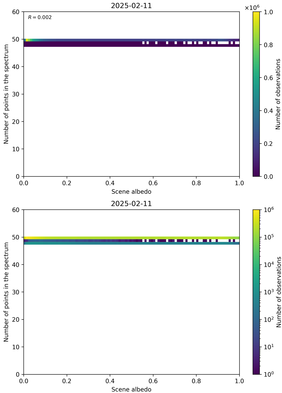
Figure 106: Scatter density plot of “Scene albedo” against “Number of points in the spectrum” for 2025-02-10 to 2025-02-12.
