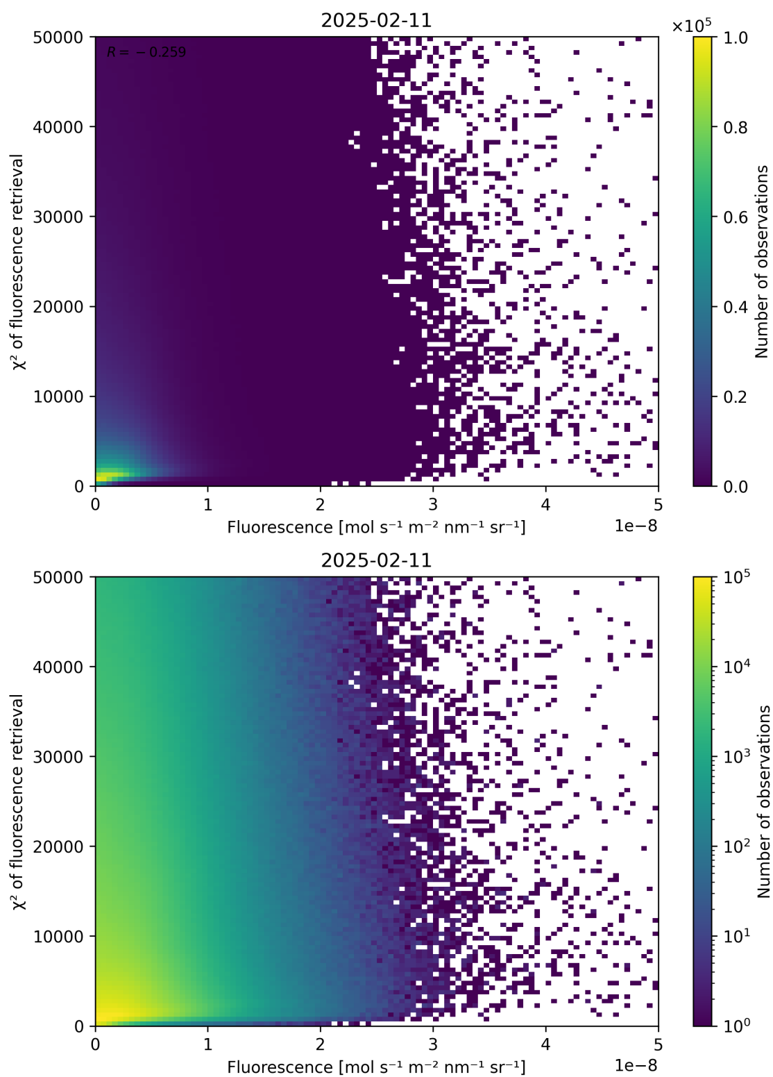
Figure 85: Scatter density plot of “Fluorescence” against “ \chi^2 of fluorescence retrieval” for 2025-02-10 to 2025-02-12.
