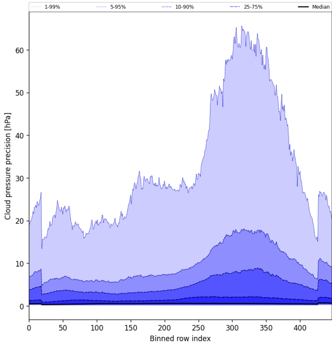
Figure 48: Along track statistics of “Cloud pressure precision” for 2025-02-10 to 2025-02-12
