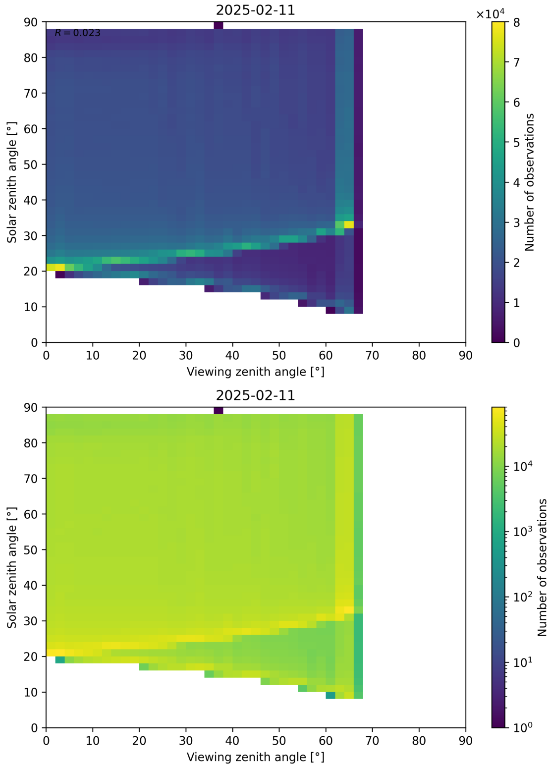
Figure 127: Scatter density plot of “Viewing zenith angle” against “Solar zenith angle” for 2025-02-10 to 2025-02-12.
