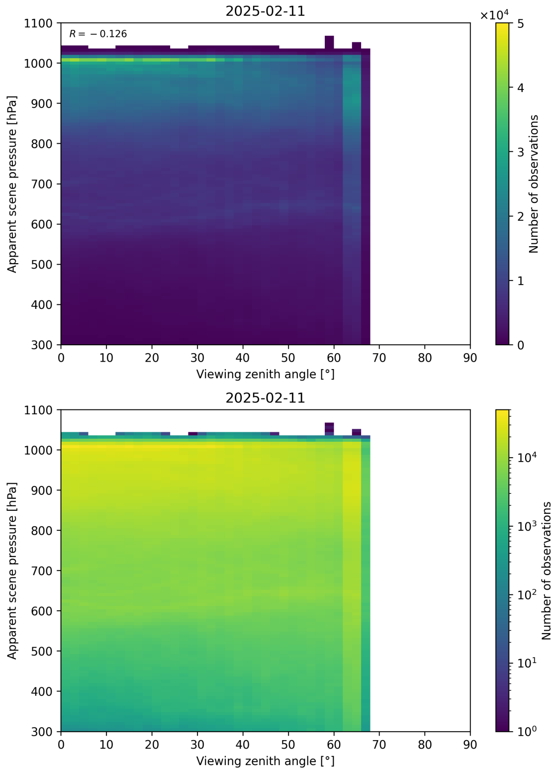
Figure 118: Scatter density plot of “Viewing zenith angle” against “Apparent scene pressure” for 2025-02-10 to 2025-02-12.
