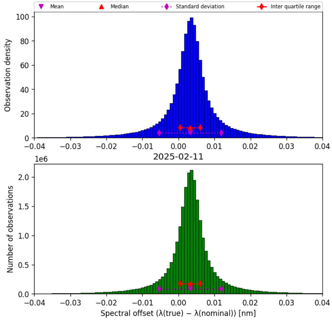
Figure 45: Histogram of “Spectral offset ( \lambda_{\text{true}} - \lambda_{\text{nominal}} )” for 2025-02-10 to 2025-02-12
