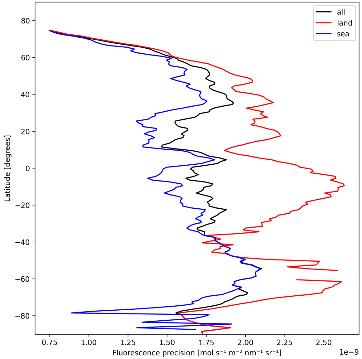
Figure 24: Zonal average of “Fluorescence precision” for 2025-02-10 to 2025-02-12.
