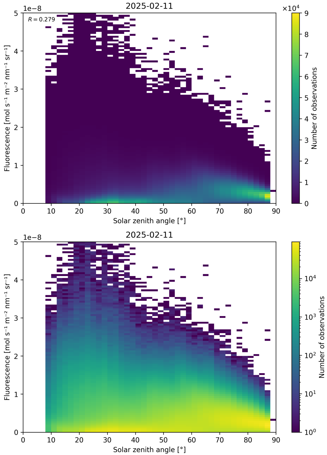
Figure 112: Scatter density plot of “Solar zenith angle” against “Fluorescence” for 2025-02-10 to 2025-02-12.
