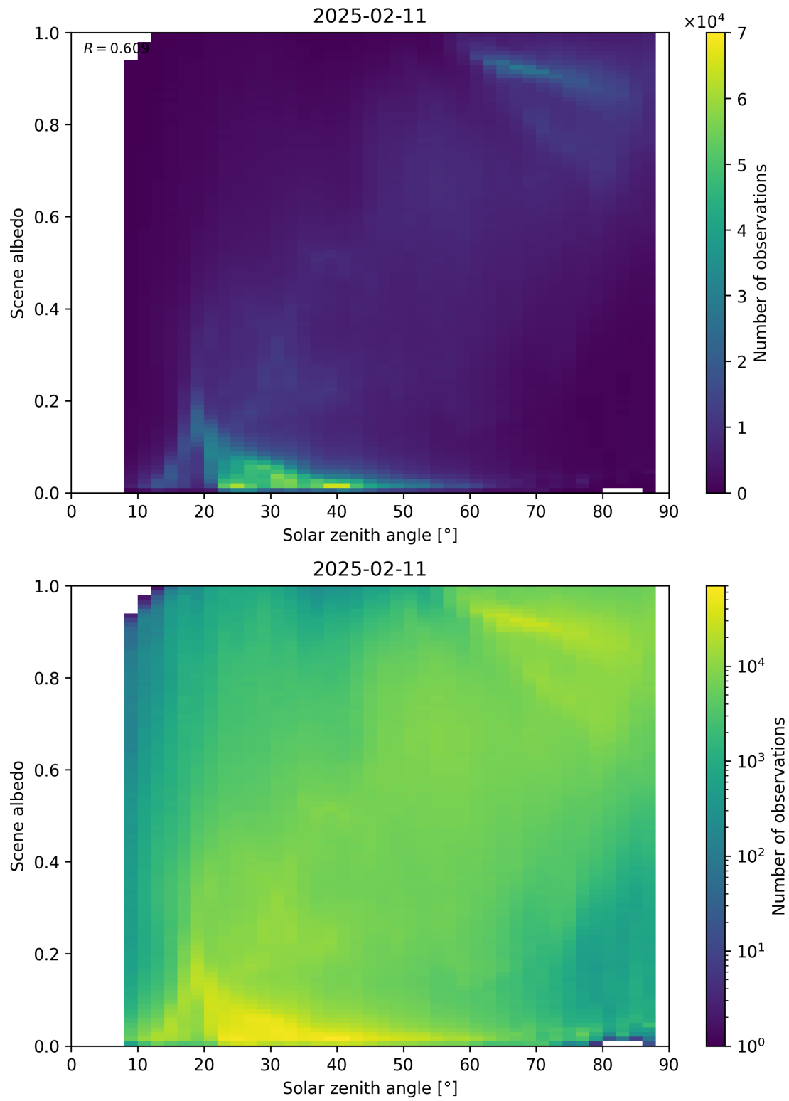
Figure 116: Scatter density plot of “Solar zenith angle” against “Scene albedo” for 2025-02-10 to 2025-02-12.
