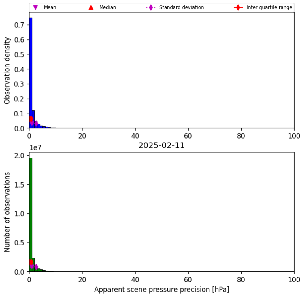
Figure 37: Histogram of “Apparent scene pressure precision” for 2025-02-10 to 2025-02-12
