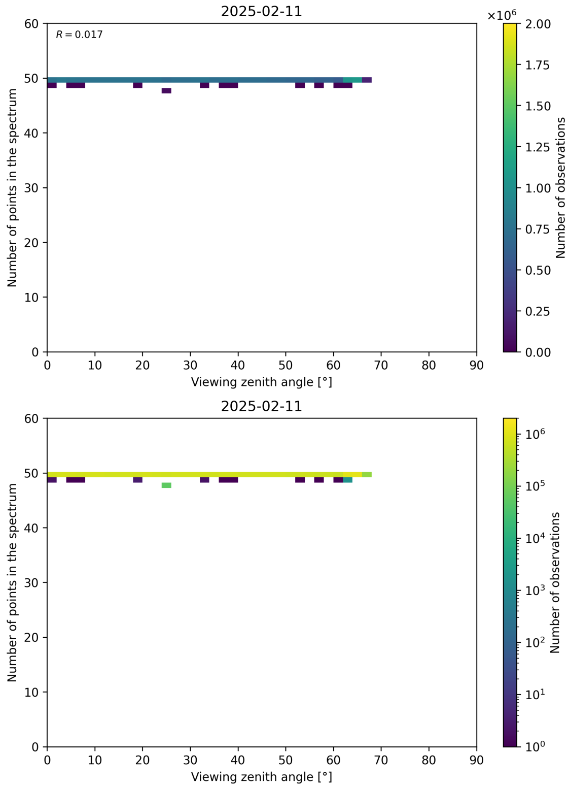
Figure 125: Scatter density plot of “Viewing zenith angle” against “Number of points in the spectrum” for 2025-02-10 to 2025-02-12.
