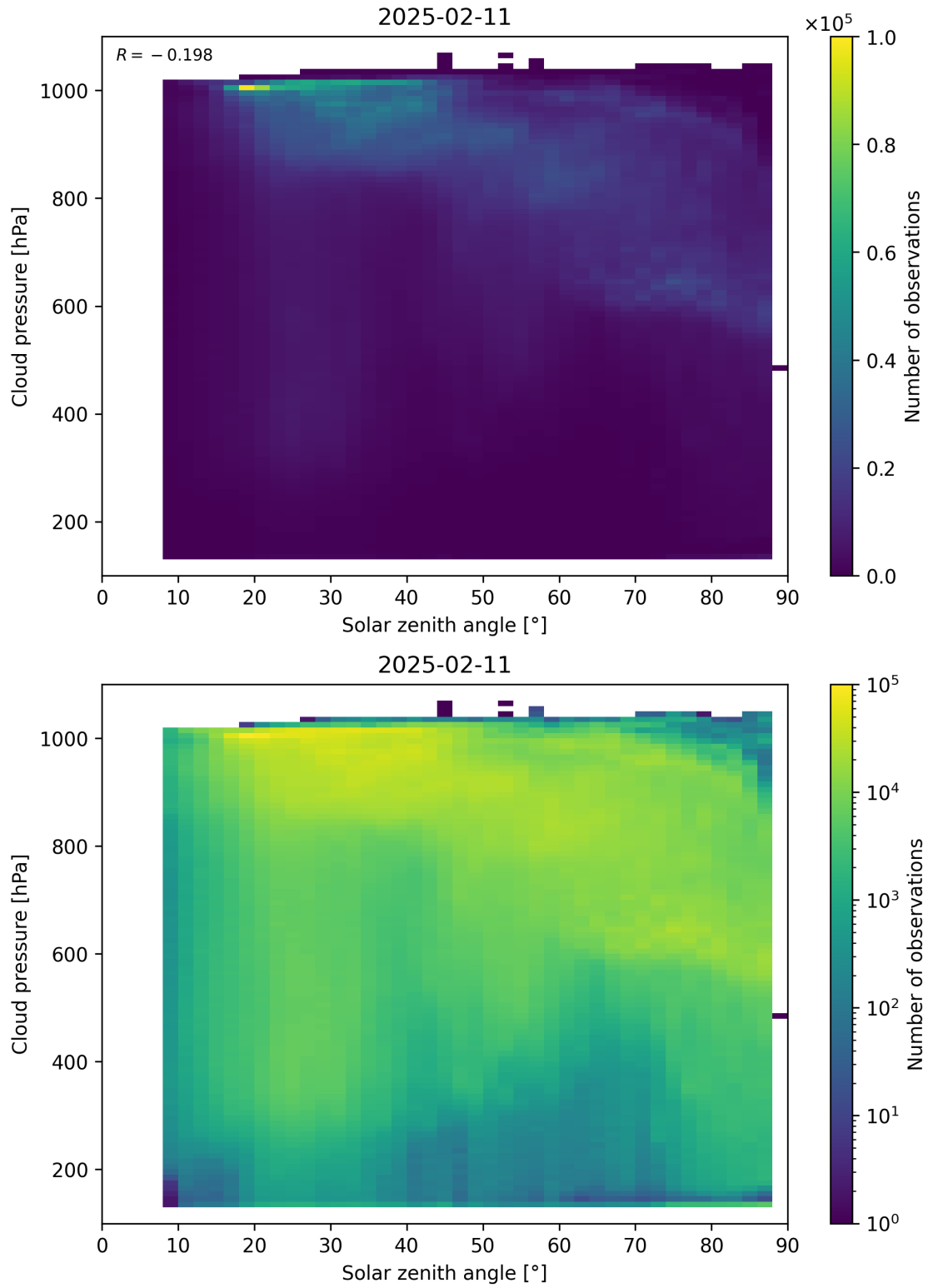
Figure 111: Scatter density plot of “Solar zenith angle” against “Cloud pressure” for 2025-02-10 to 2025-02-12.
