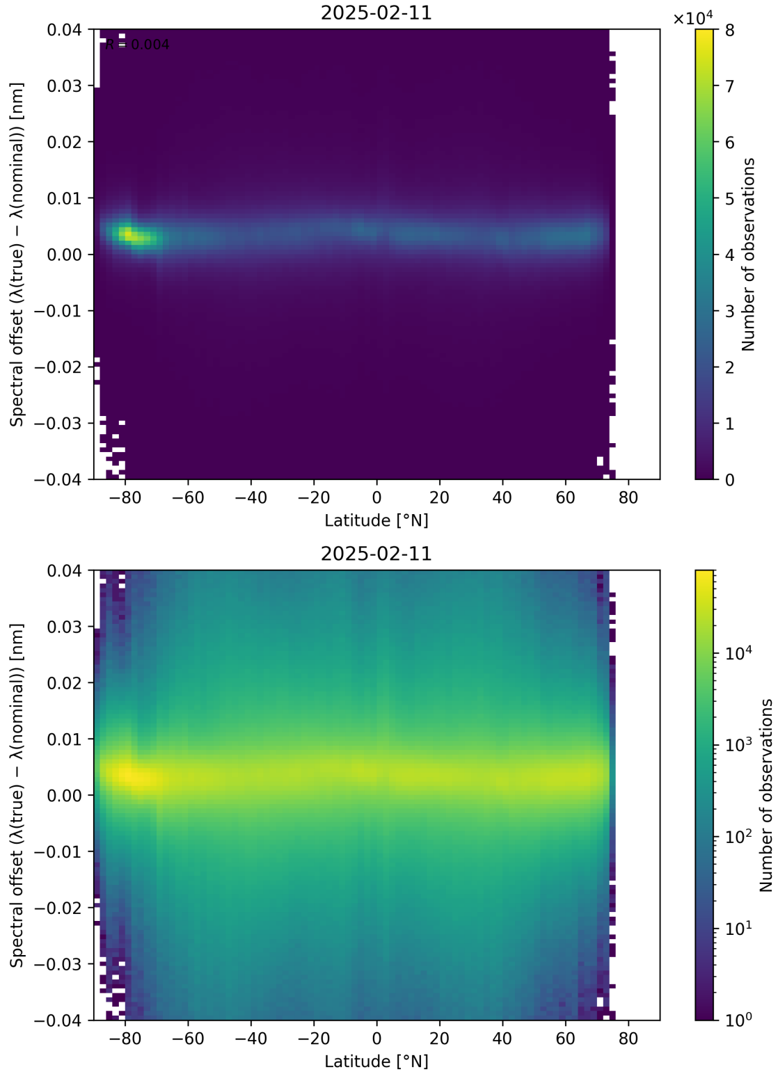
Figure 96: Scatter density plot of “Latitude” against “Spectral offset ( \lambda_{\text{true}} - \lambda_{\text{nominal}} )” for 2025-02-10 to 2025-02-12.
