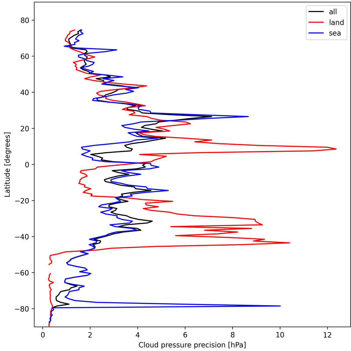
Figure 14: Zonal average of “Cloud pressure precision” for 2025-02-10 to 2025-02-12.
