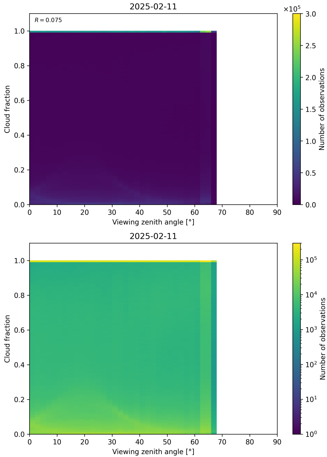
Figure 120: Scatter density plot of “Viewing zenith angle” against “Cloud fraction” for 2025-02-10 to 2025-02-12.
