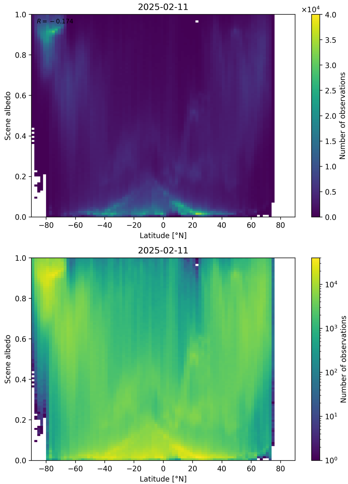
Figure 95: Scatter density plot of “Latitude” against “Scene albedo” for 2025-02-10 to 2025-02-12.
