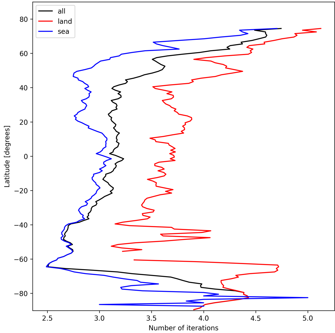
Figure 22: Zonal average of “Number of iterations” for 2025-02-10 to 2025-02-12.
