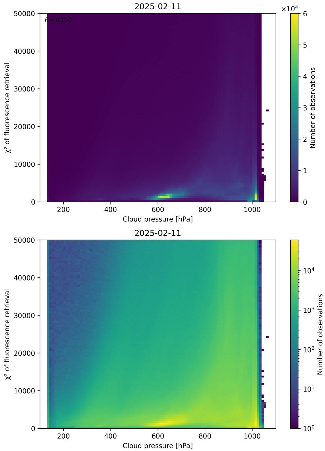
Figure 78: Scatter density plot of “Cloud pressure” against “ \chi^2 of fluorescence retrieval” for 2025-02-10 to 2025-02-12.
