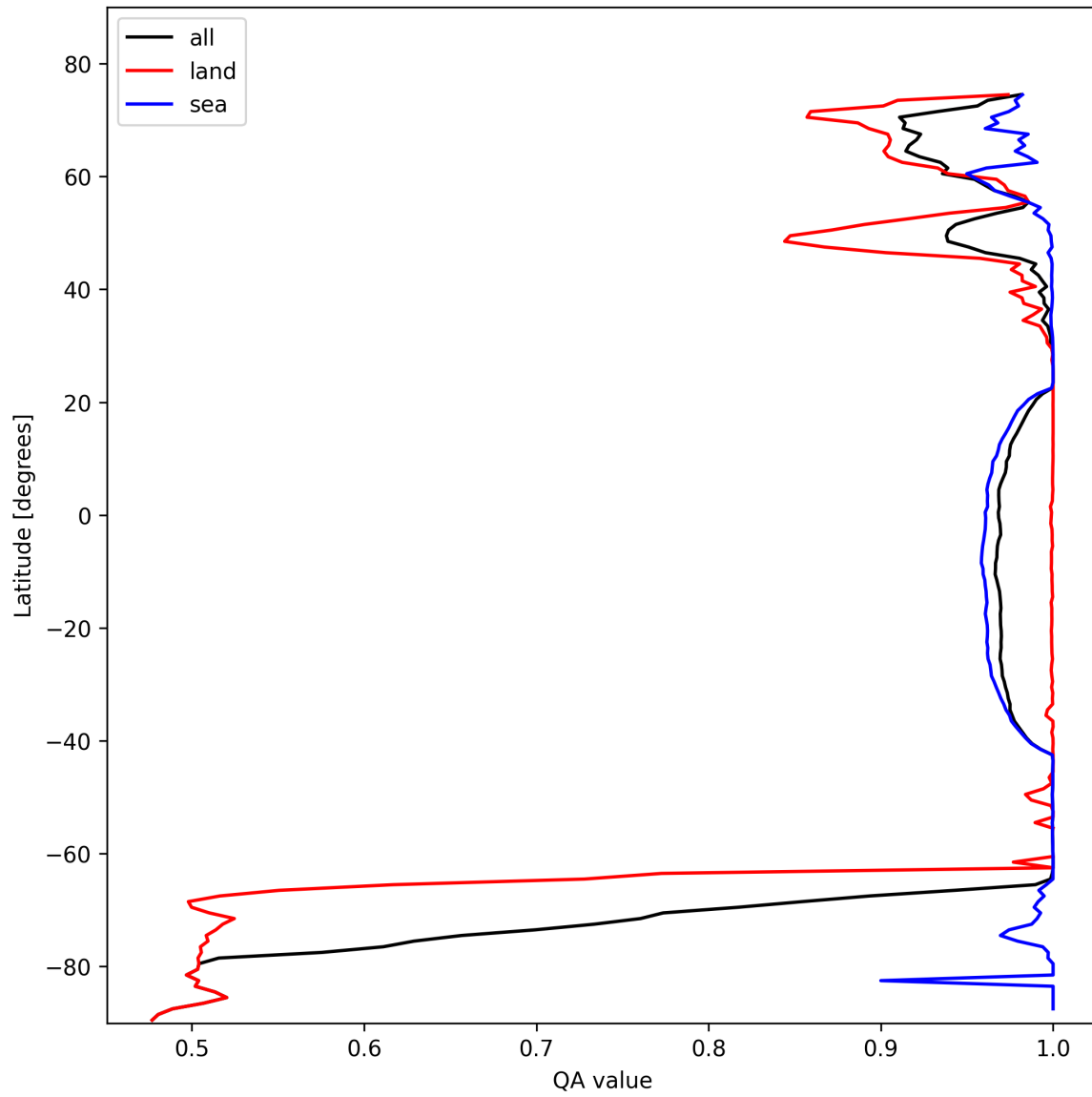
Figure 12: Zonal average of “QA value” for 2025-02-10 to 2025-02-12.
