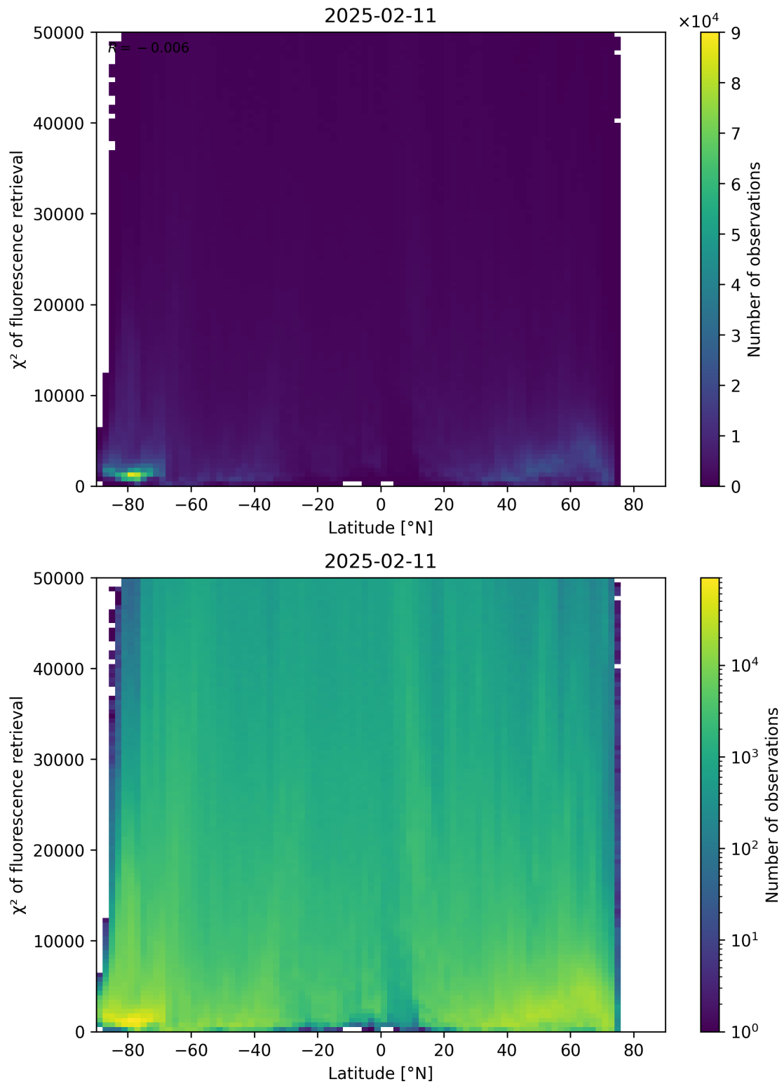
Figure 89: Scatter density plot of “Latitude” against “ \chi^2 of fluorescence retrieval” for 2025-02-10 to 2025-02-12.
