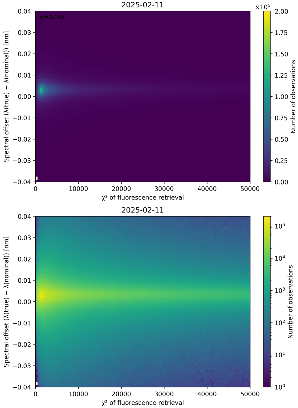
Figure 69: Scatter density plot of “ \chi^2 of fluorescence retrieval” against “Spectral offset ( \lambda_{\text{true}} - \lambda_{\text{nominal}} )” for 2025-02-10 to 2025-02-12.
