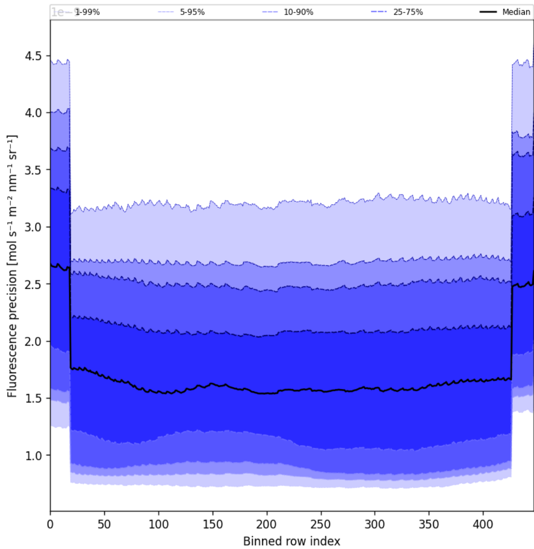
Figure 58: Along track statistics of “Fluorescence precision” for 2025-02-10 to 2025-02-12
