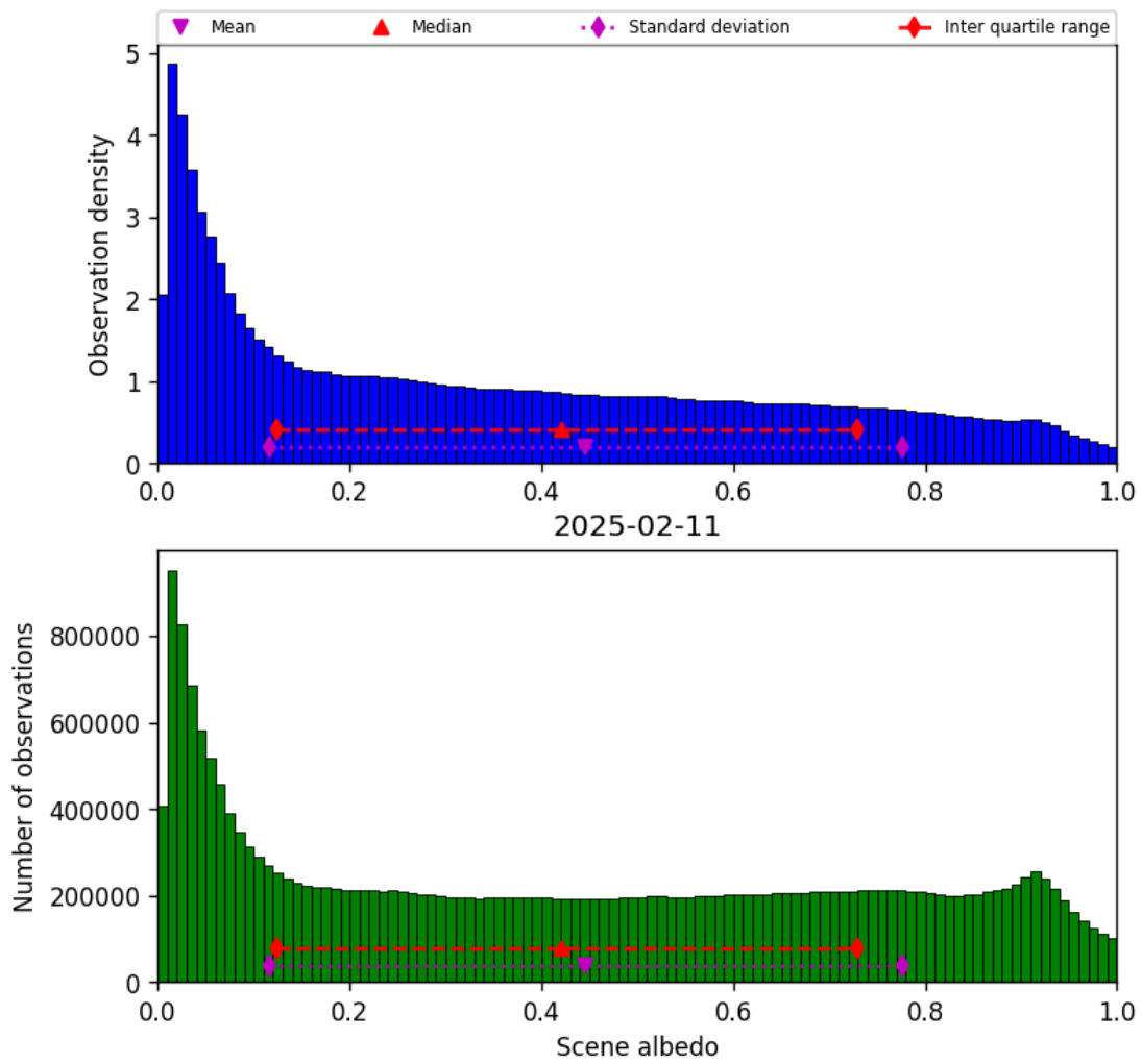
Figure 34: Histogram of “Scene albedo” for 2025-02-10 to 2025-02-12
