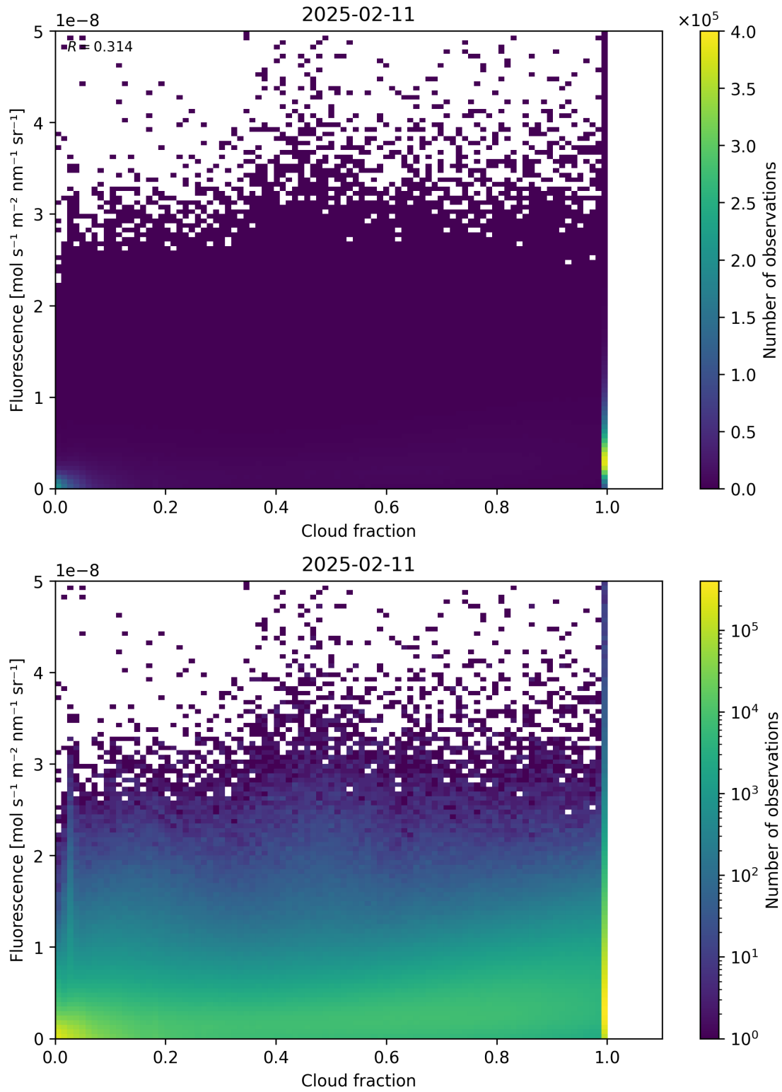
Figure 72: Scatter density plot of “Cloud fraction” against “Fluorescence” for 2025-02-10 to 2025-02-12.
