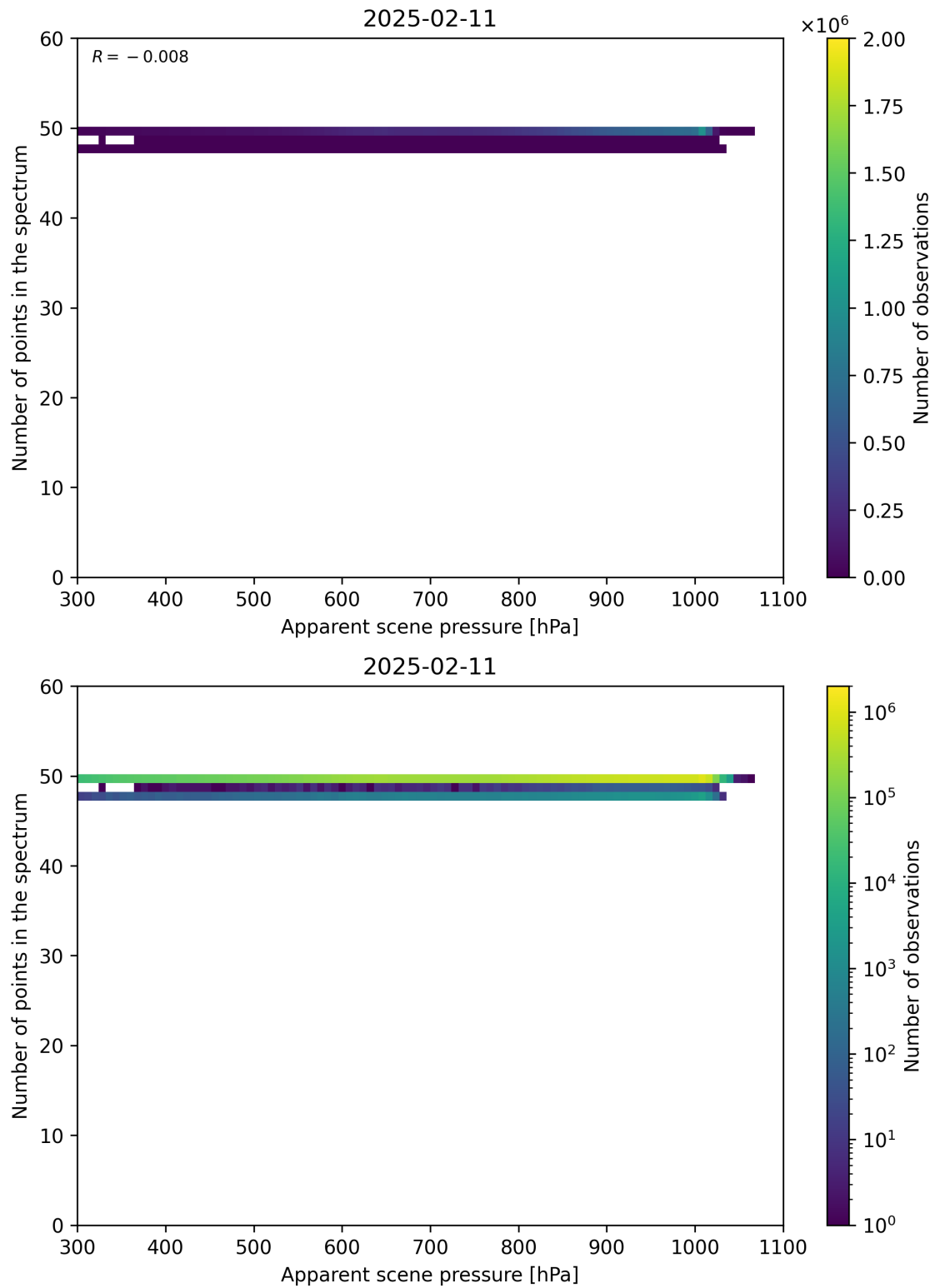
Figure 66: Scatter density plot of “Apparent scene pressure” against “Number of points in the spectrum” for 2025-02-10 to 2025-02-12.
