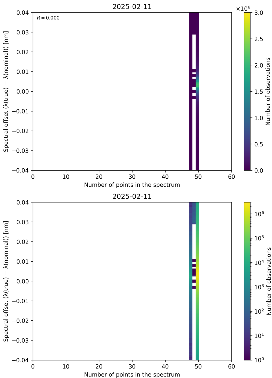
Figure 101: Scatter density plot of “Number of points in the spectrum” against “Spectral offset ( \lambda_{\text{true}} - \lambda_{\text{nominal}} )” for 2025-02-10 to 2025-02-12.
