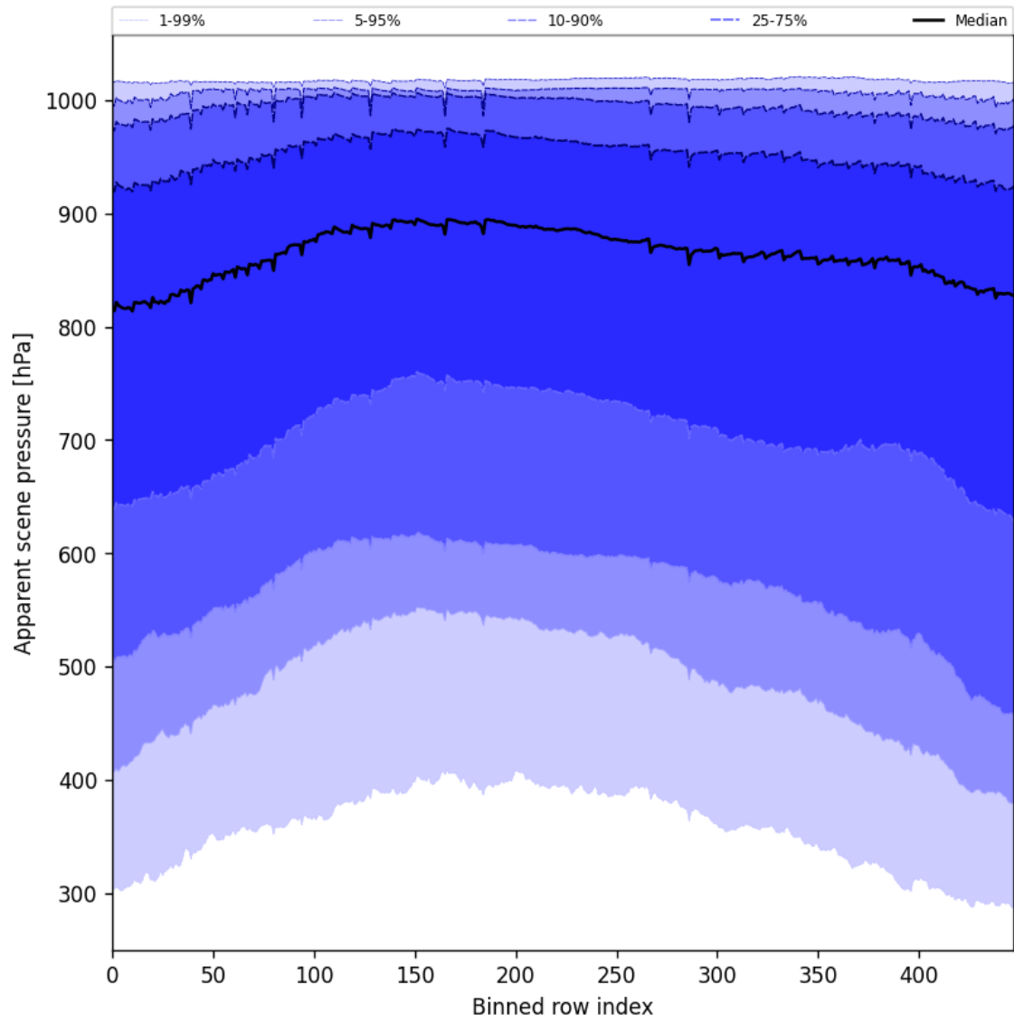
Figure 53: Along track statistics of “Apparent scene pressure” for 2025-02-10 to 2025-02-12
