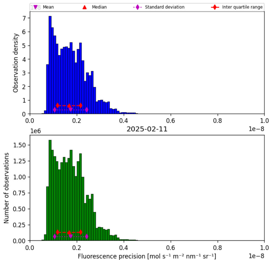
Figure 41: Histogram of “Fluorescence precision” for 2025-02-10 to 2025-02-12
