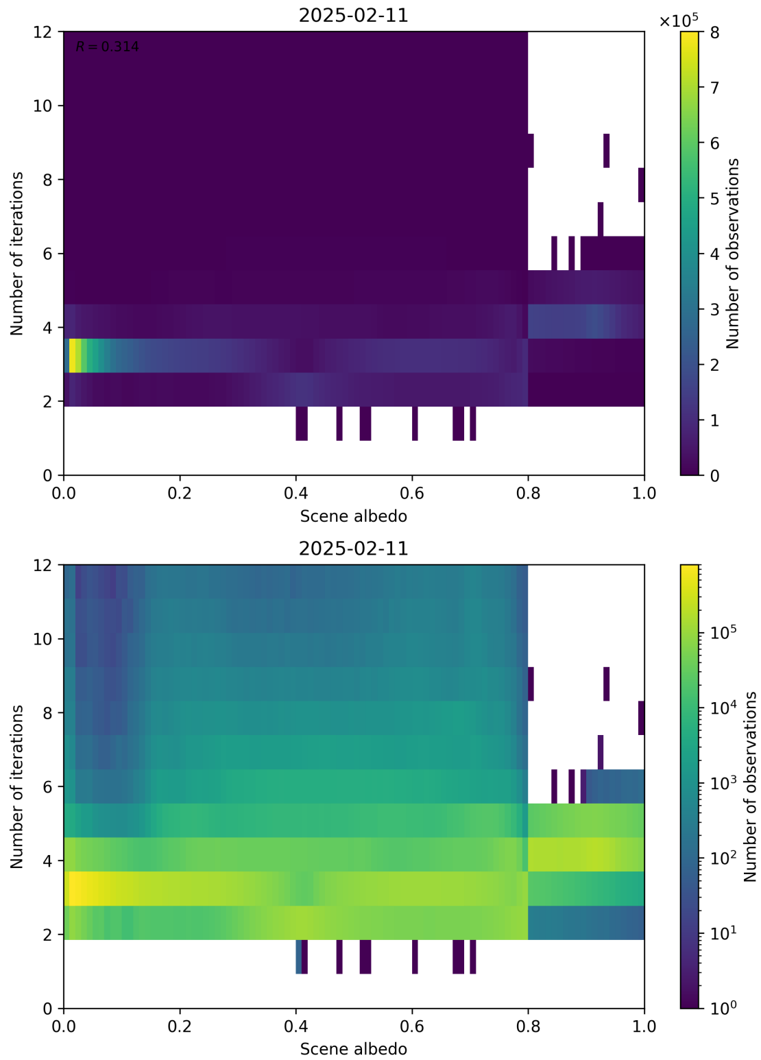
Figure 105: Scatter density plot of “Scene albedo” against “Number of iterations” for 2025-02-10 to 2025-02-12.
