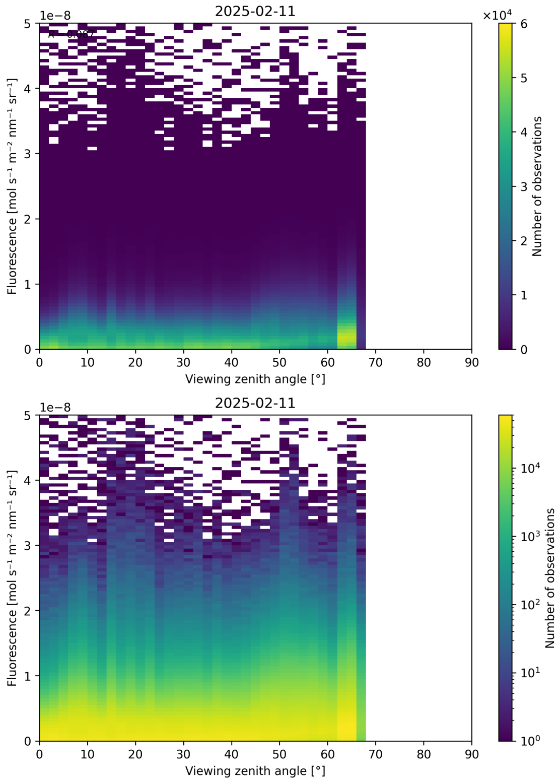
Figure 122: Scatter density plot of “Viewing zenith angle” against “Fluorescence” for 2025-02-10 to 2025-02-12.
