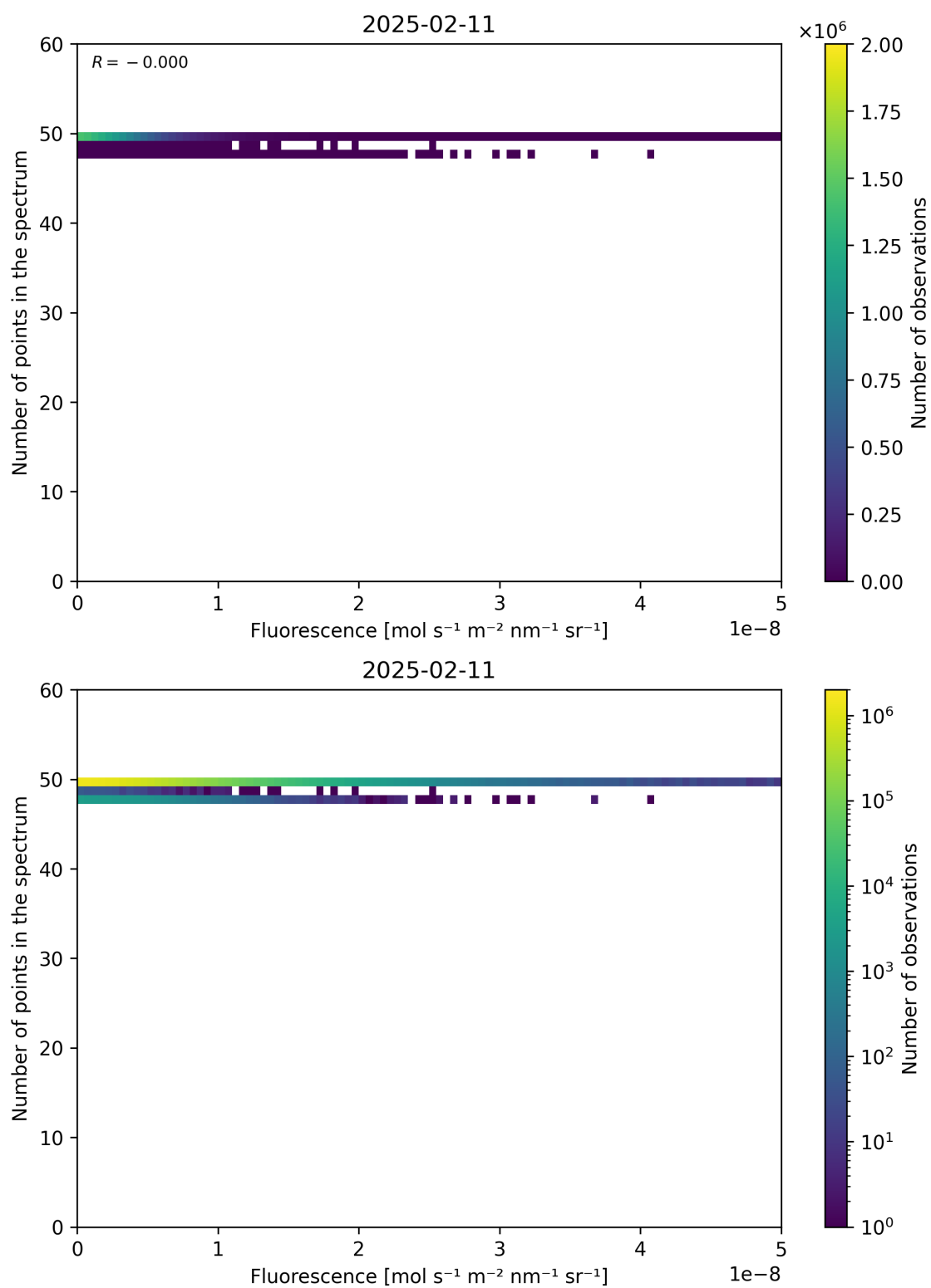
Figure 86: Scatter density plot of “Fluorescence” against “Number of points in the spectrum” for 2025-02-10 to 2025-02-12.
