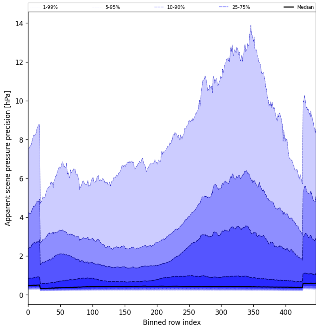
Figure 54: Along track statistics of “Apparent scene pressure precision” for 2025-02-10 to 2025-02-12
