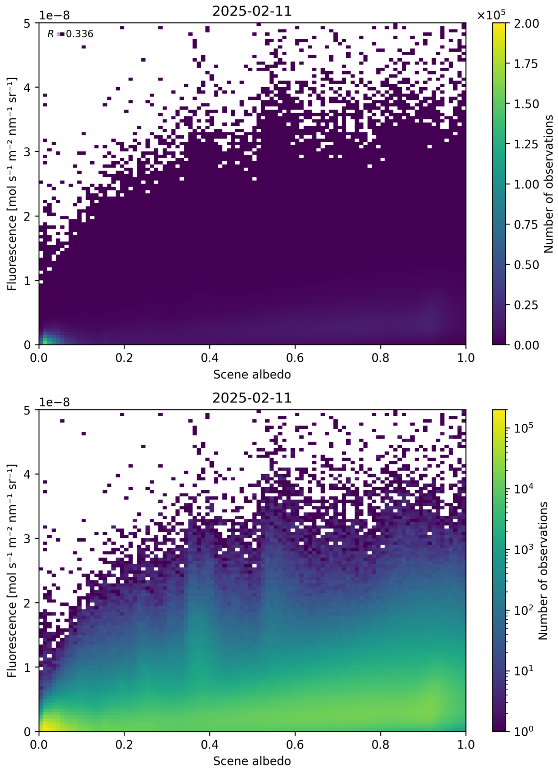
Figure 104: Scatter density plot of “Scene albedo” against “Fluorescence” for 2025-02-10 to 2025-02-12.
