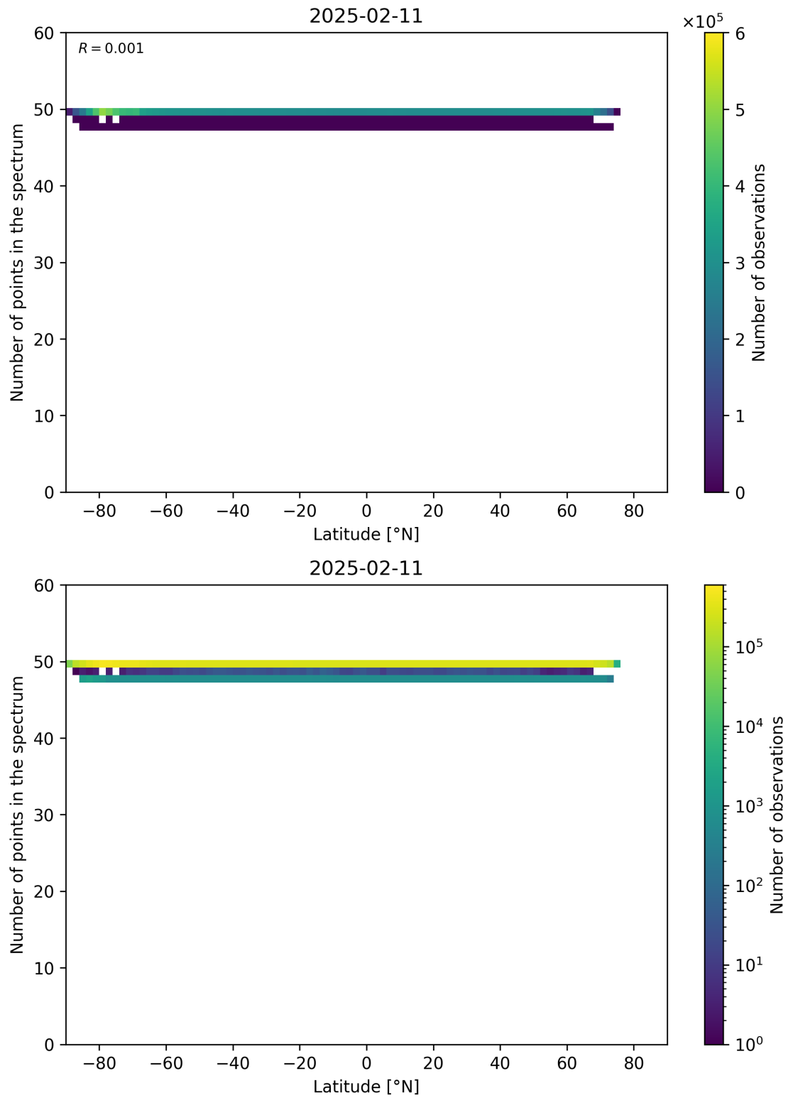
Figure 94: Scatter density plot of “Latitude” against “Number of points in the spectrum” for 2025-02-10 to 2025-02-12.
