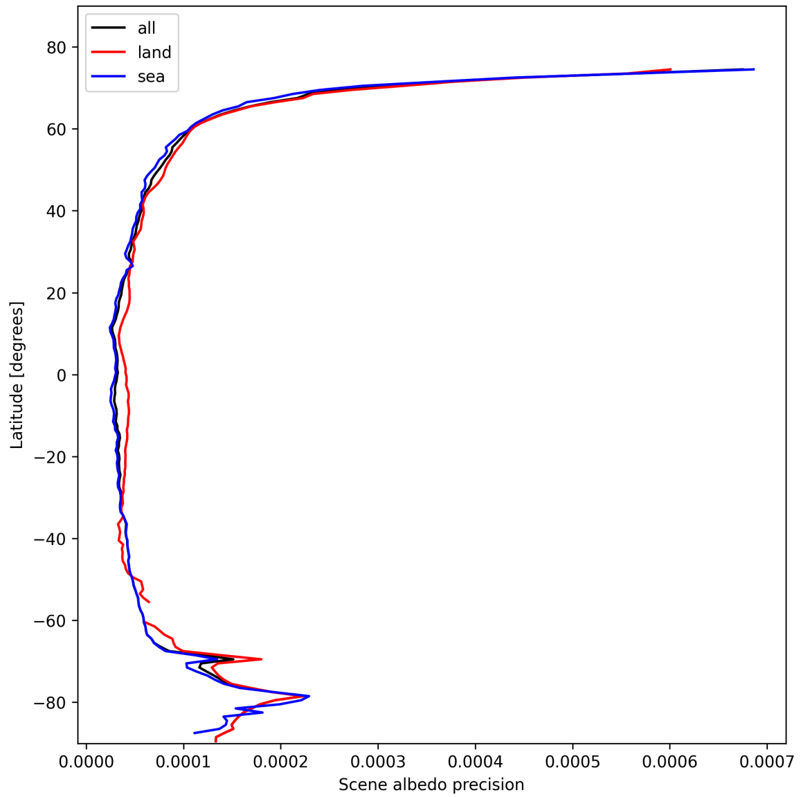
Figure 18: Zonal average of “Scene albedo precision” for 2025-02-10 to 2025-02-12.
