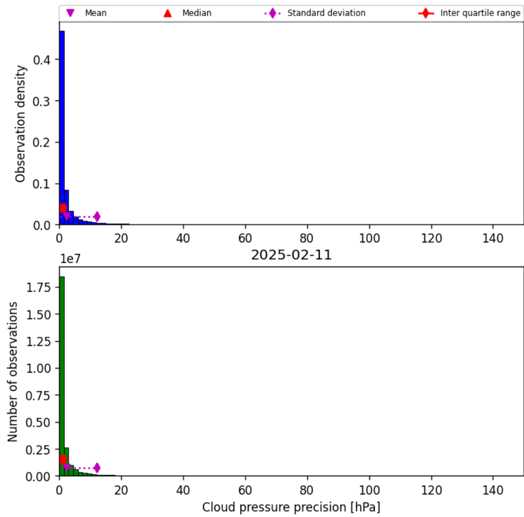
Figure 31: Histogram of “Cloud pressure precision” for 2025-02-10 to 2025-02-12
