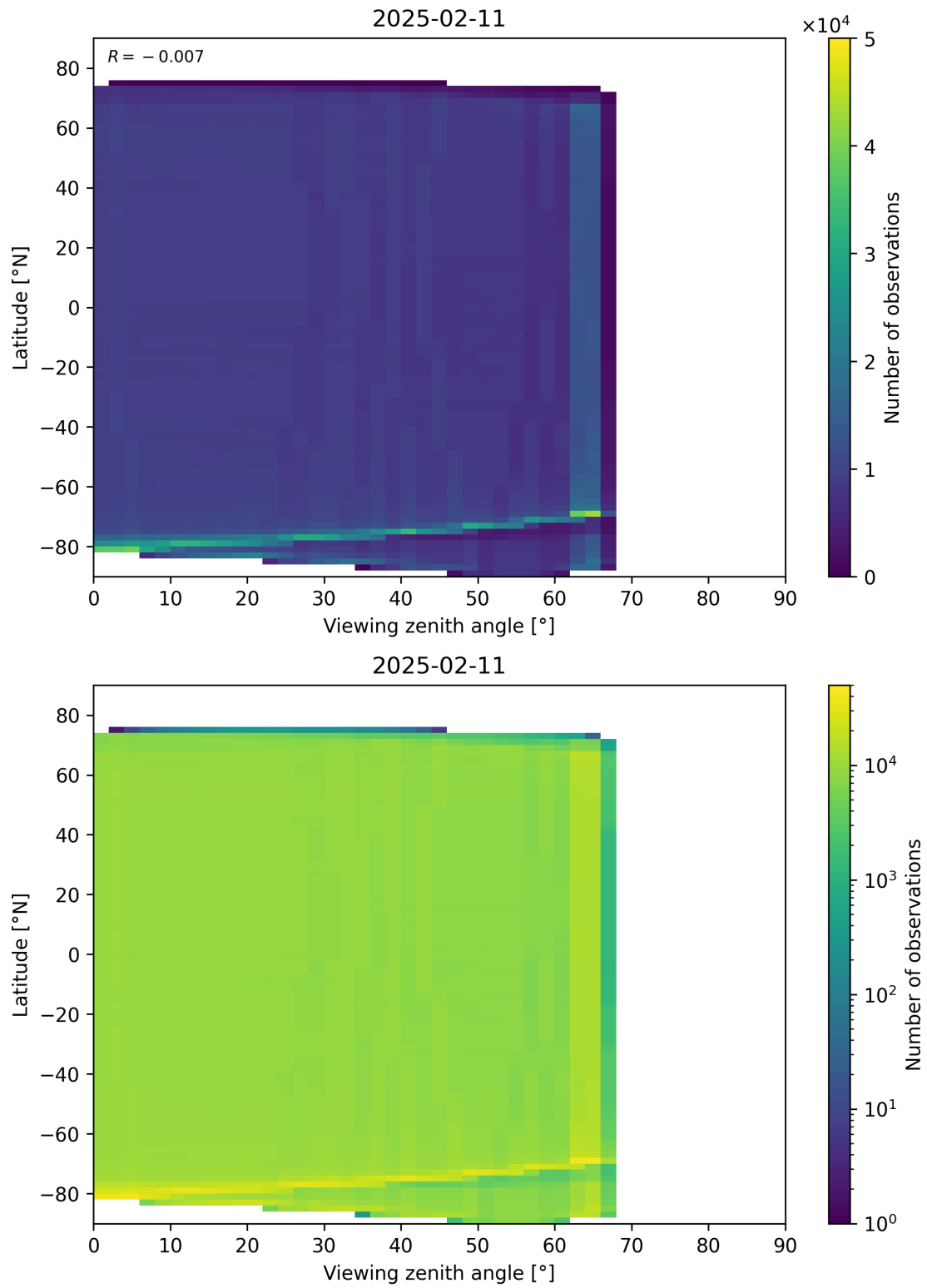
Figure 123: Scatter density plot of “Viewing zenith angle” against “Latitude” for 2025-02-10 to 2025-02-12.
