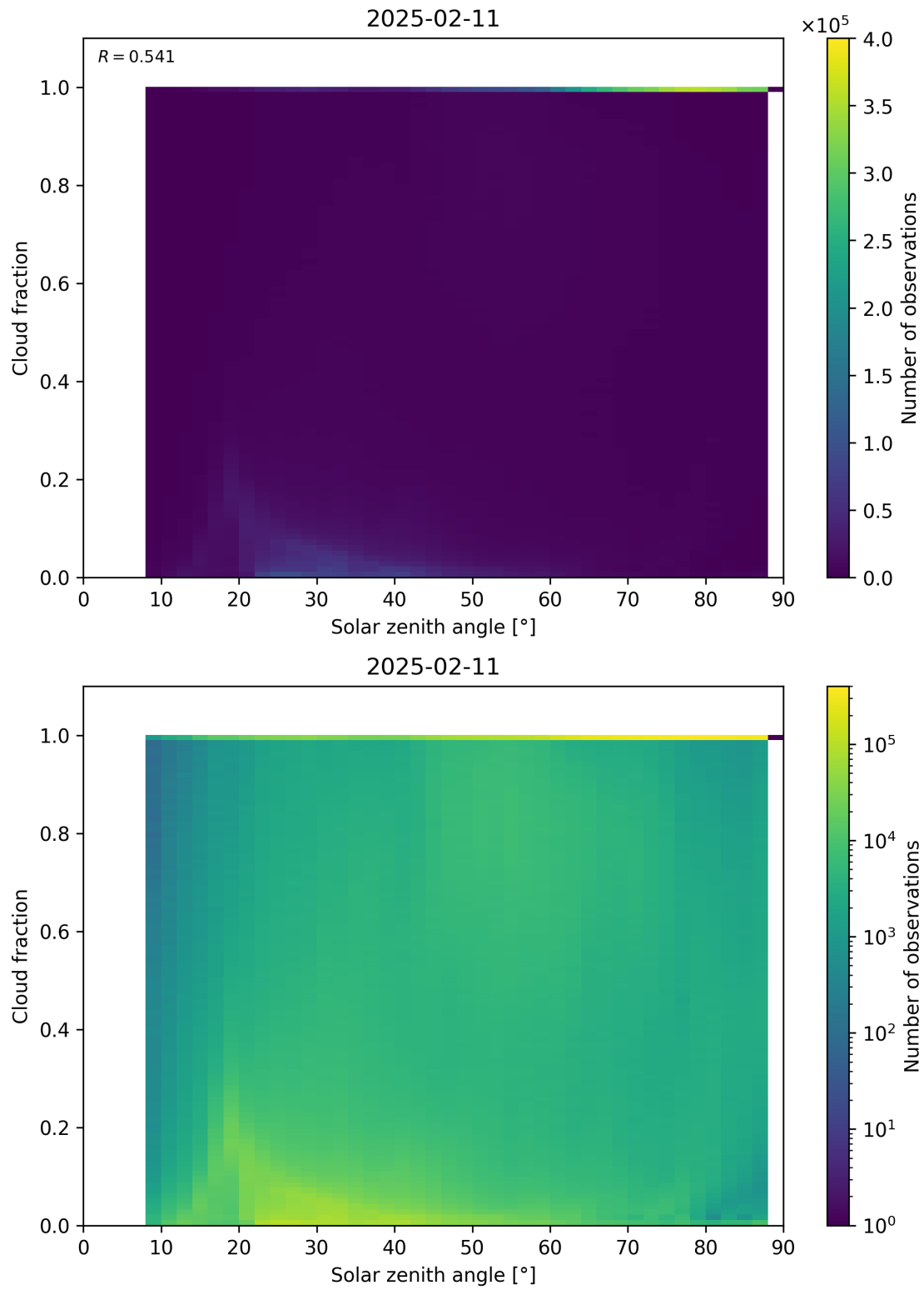
Figure 110: Scatter density plot of “Solar zenith angle” against “Cloud fraction” for 2025-02-10 to 2025-02-12.
