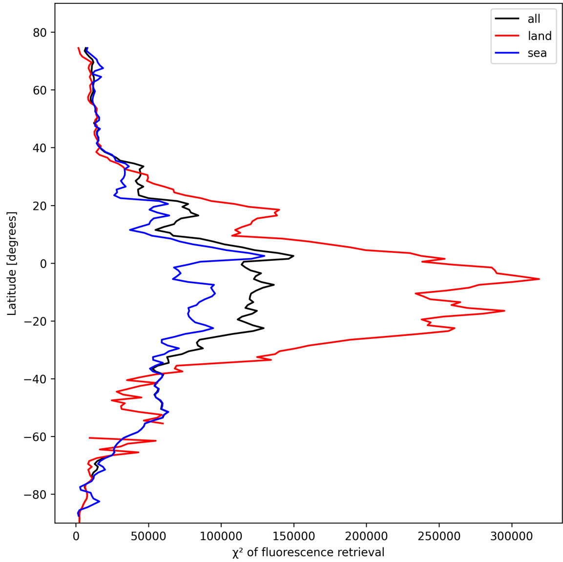
Figure 25: Zonal average of “ \chi^2 of fluorescence retrieval” for 2025-02-10 to 2025-02-12.
