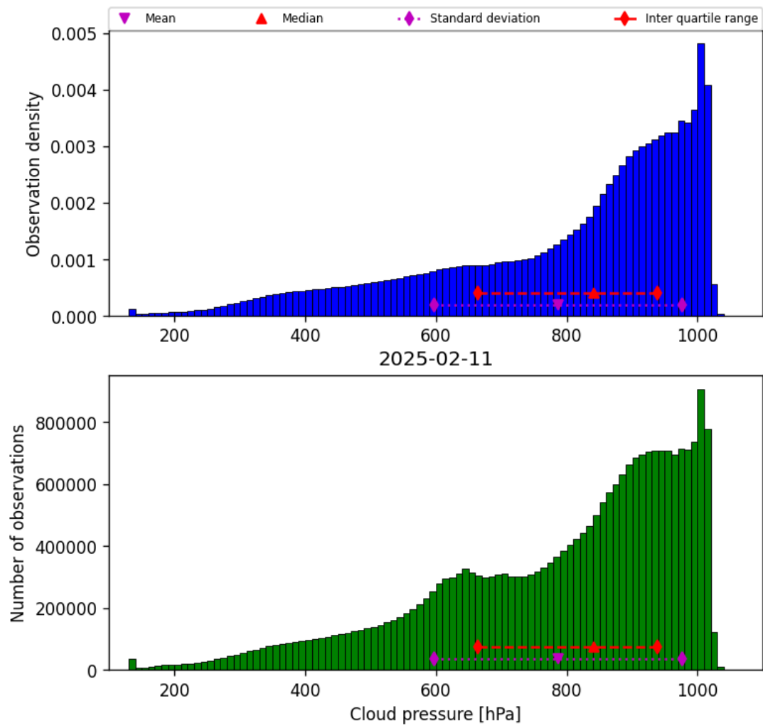
Figure 30: Histogram of “Cloud pressure” for 2025-02-10 to 2025-02-12
