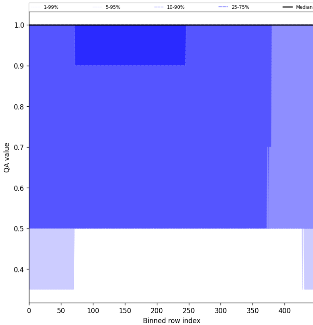
Figure 46: Along track statistics of “QA value” for 2025-02-10 to 2025-02-12
