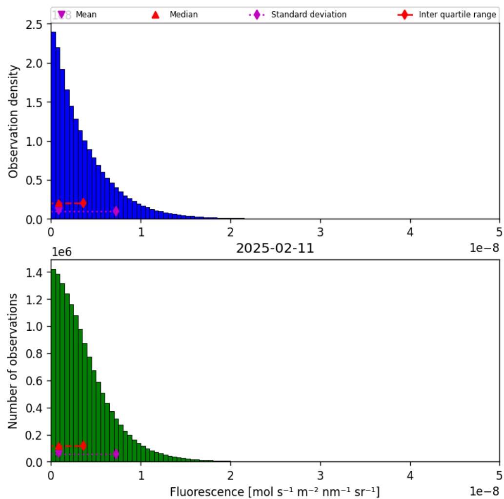
Figure 40: Histogram of “Fluorescence” for 2025-02-10 to 2025-02-12
