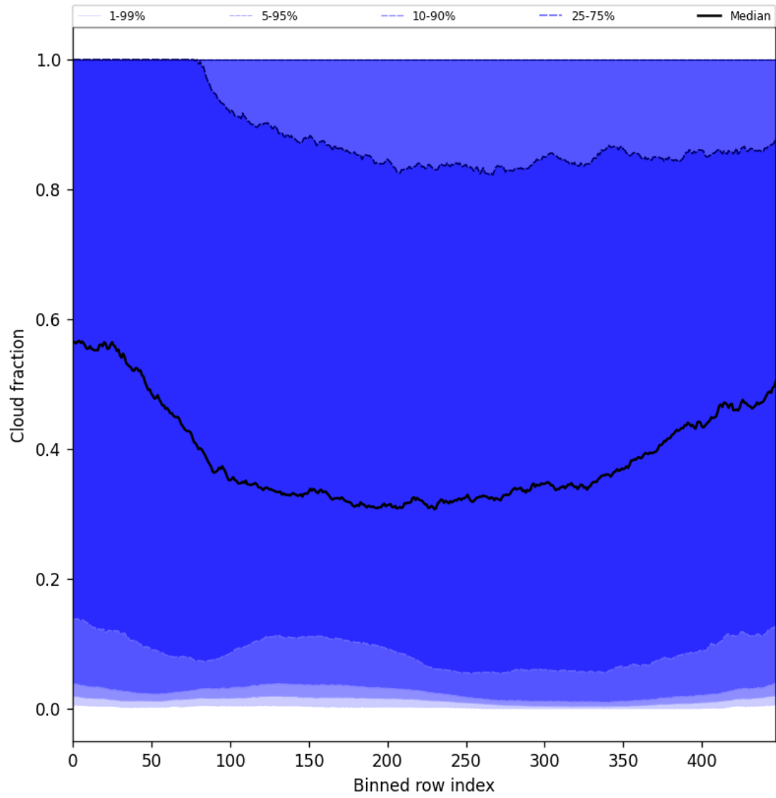
Figure 49: Along track statistics of “Cloud fraction” for 2025-02-10 to 2025-02-12
