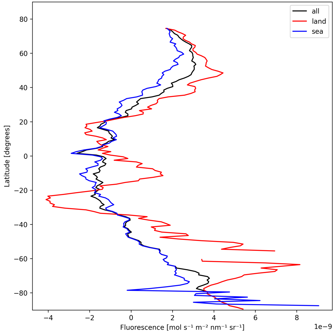
Figure 23: Zonal average of “Fluorescence” for 2025-02-10 to 2025-02-12.
