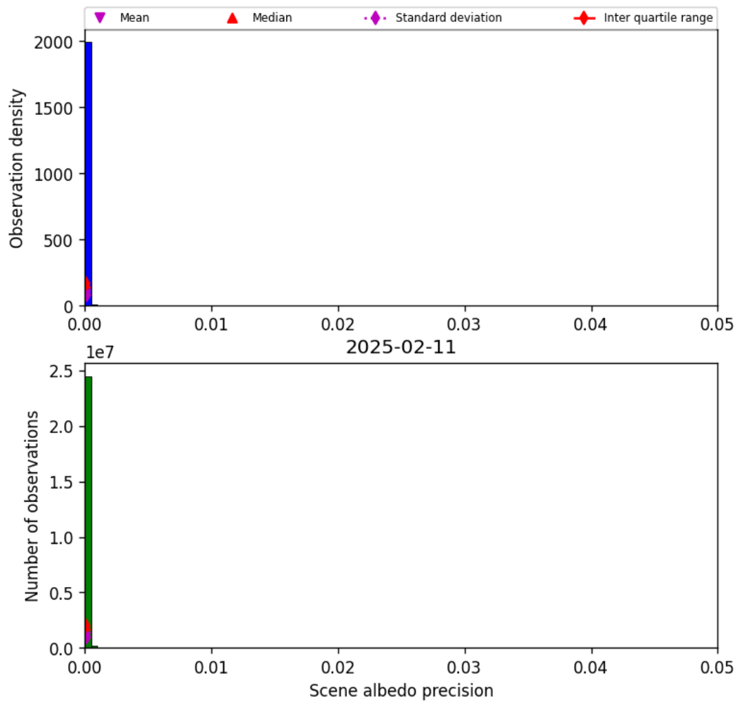
Figure 35: Histogram of “Scene albedo precision” for 2025-02-10 to 2025-02-12
