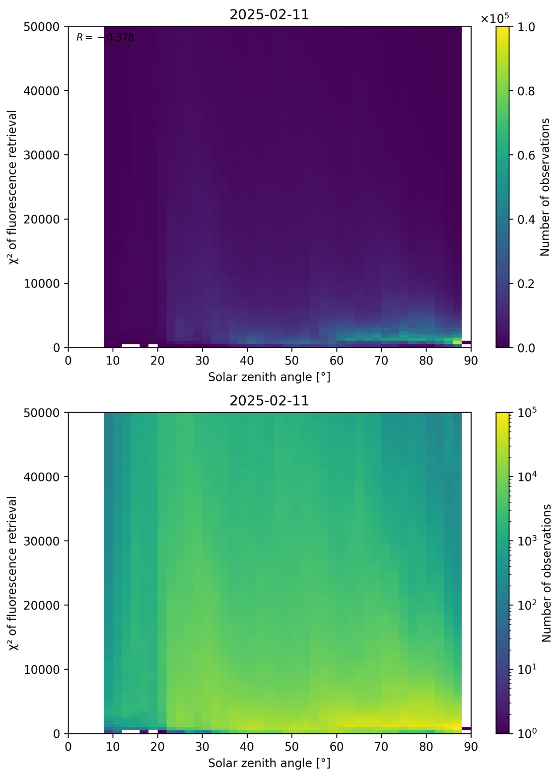
Figure 109: Scatter density plot of “Solar zenith angle” against “ \chi^2 of fluorescence retrieval” for 2025-02-10 to 2025-02-12.
