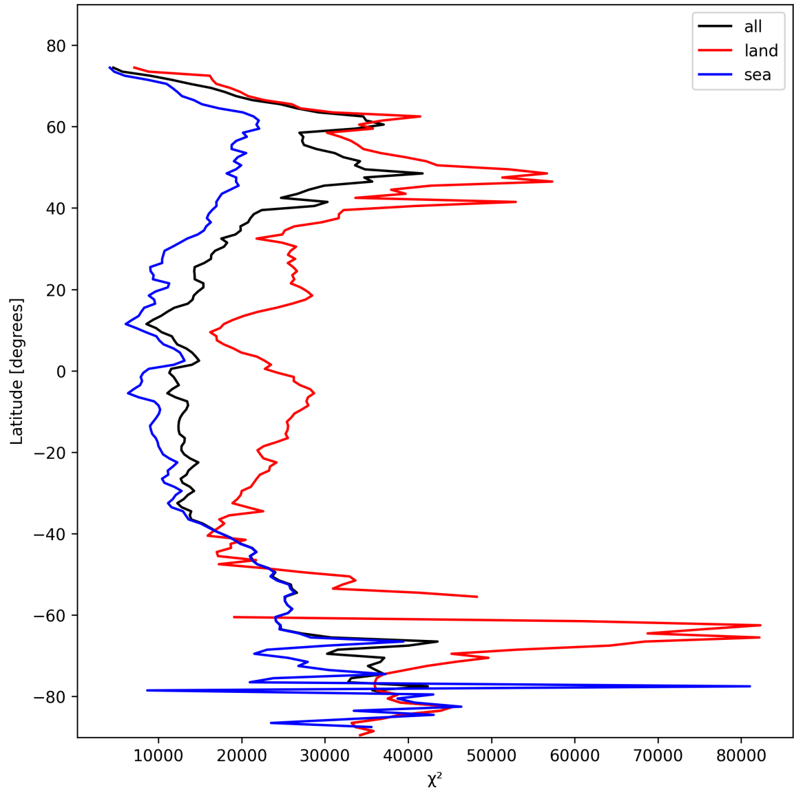
Figure 21: Zonal average of “ \chi^2 ” for 2025-02-10 to 2025-02-12.
