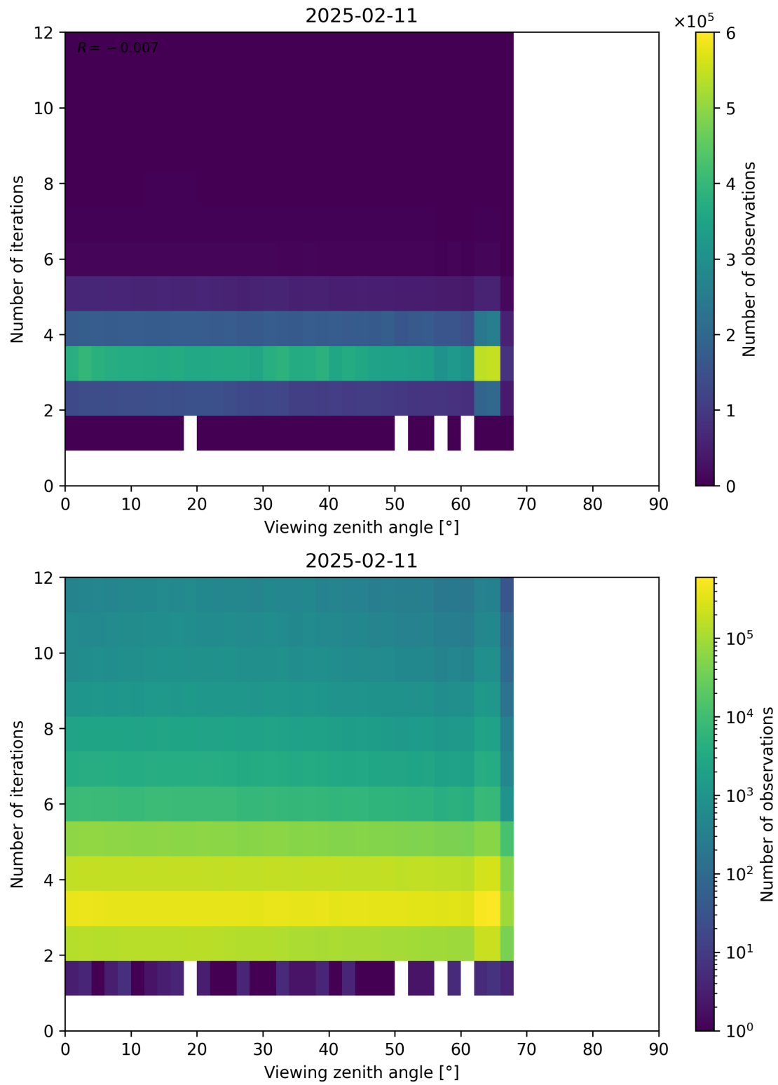
Figure 124: Scatter density plot of “Viewing zenith angle” against “Number of iterations” for 2025-02-10 to 2025-02-12.
