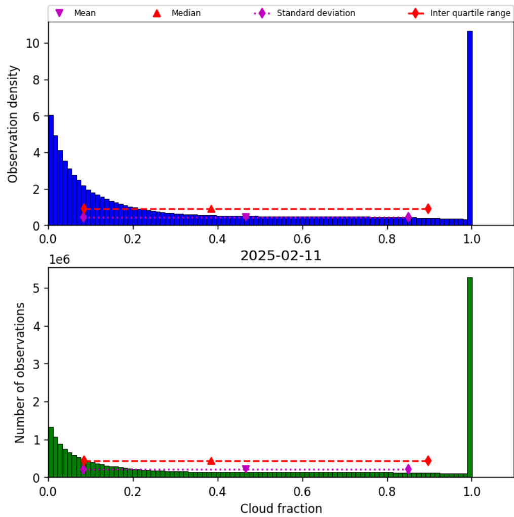
Figure 32: Histogram of “Cloud fraction” for 2025-02-10 to 2025-02-12
