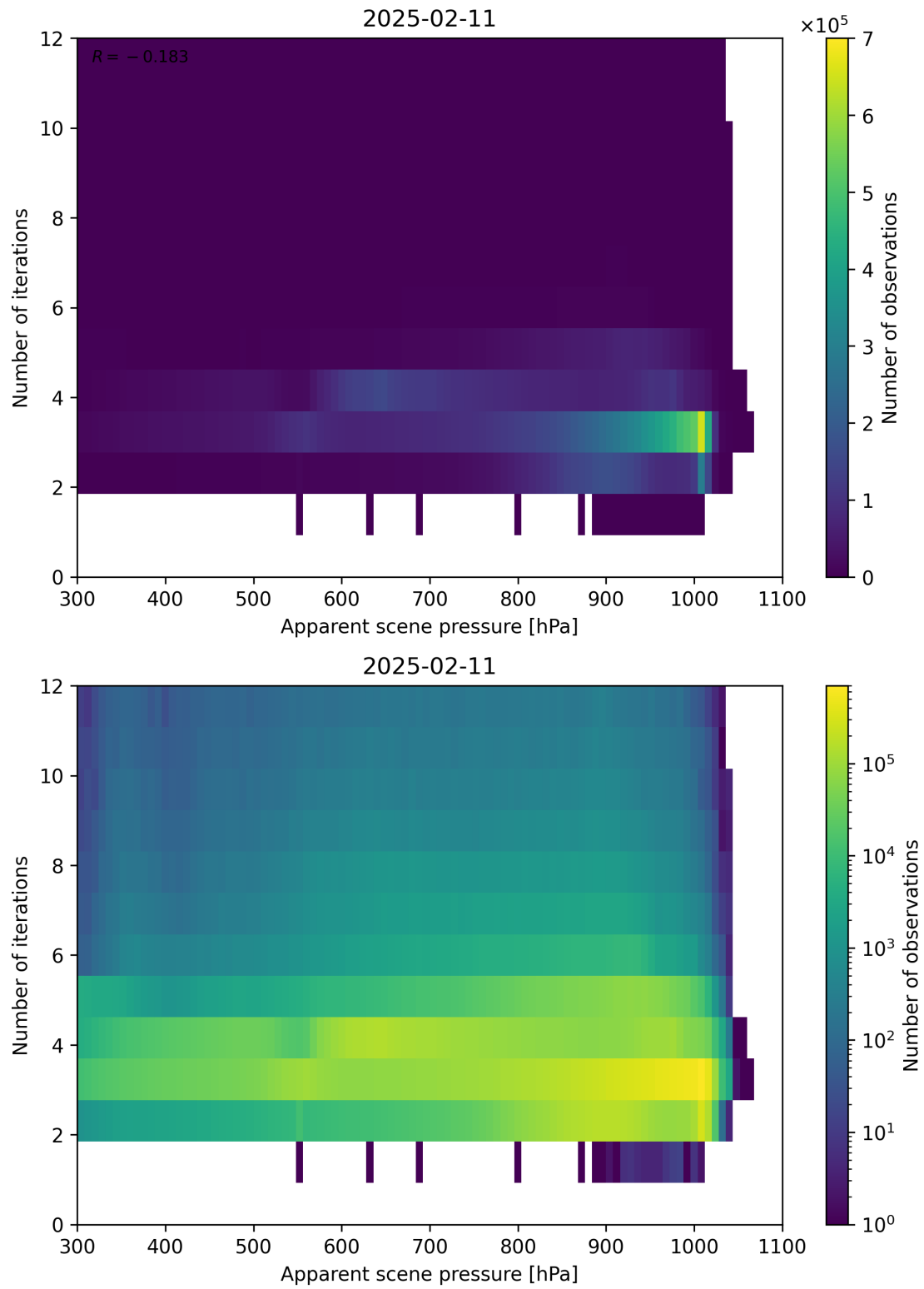
Figure 65: Scatter density plot of “Apparent scene pressure” against “Number of iterations” for 2025-02-10 to 2025-02-12.
