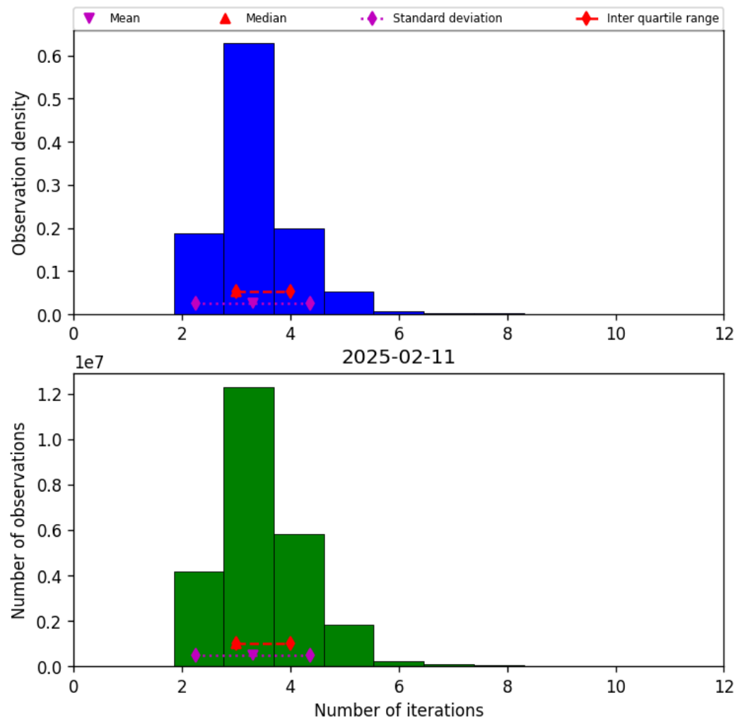
Figure 39: Histogram of “Number of iterations” for 2025-02-10 to 2025-02-12
