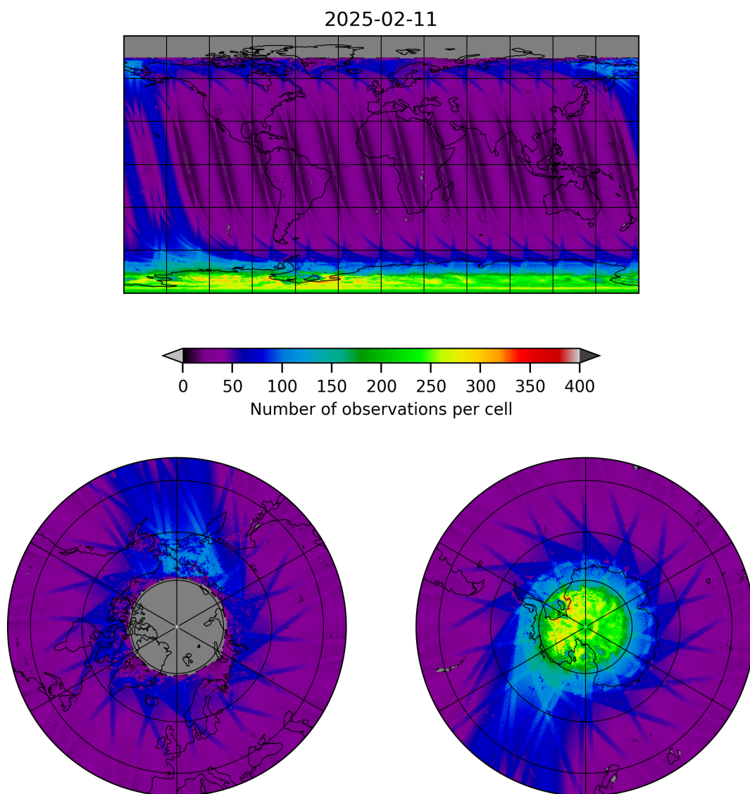
Figure 11: Map of the number of observations for 2025-02-10 to 2025-02-12
