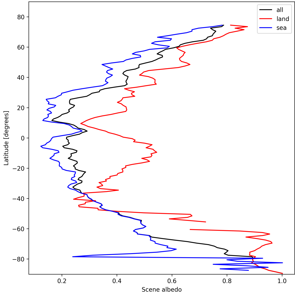
Figure 17: Zonal average of “Scene albedo” for 2025-02-10 to 2025-02-12.
