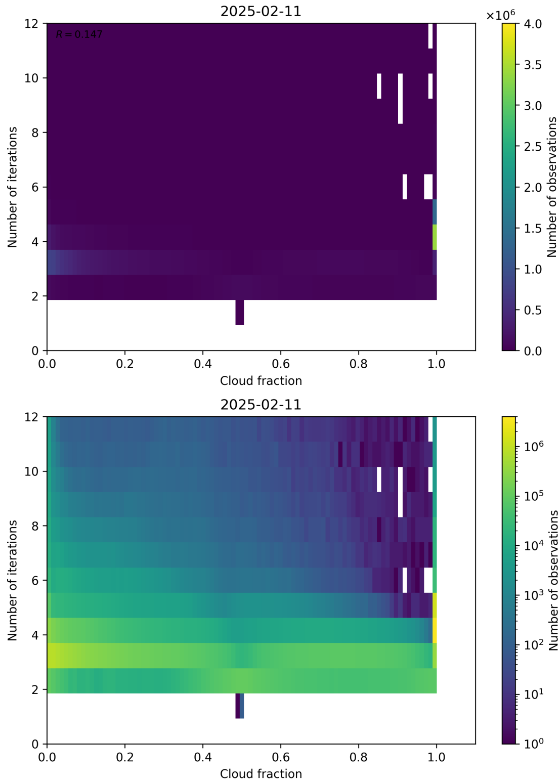
Figure 73: Scatter density plot of “Cloud fraction” against “Number of iterations” for 2025-02-10 to 2025-02-12.
