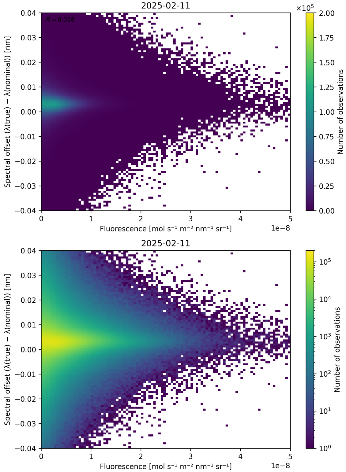
Figure 87: Scatter density plot of “Fluorescence” against “Spectral offset ( \lambda_{\text{true}} - \lambda_{\text{nominal}} )” for 2025-02-10 to 2025-02-12.
