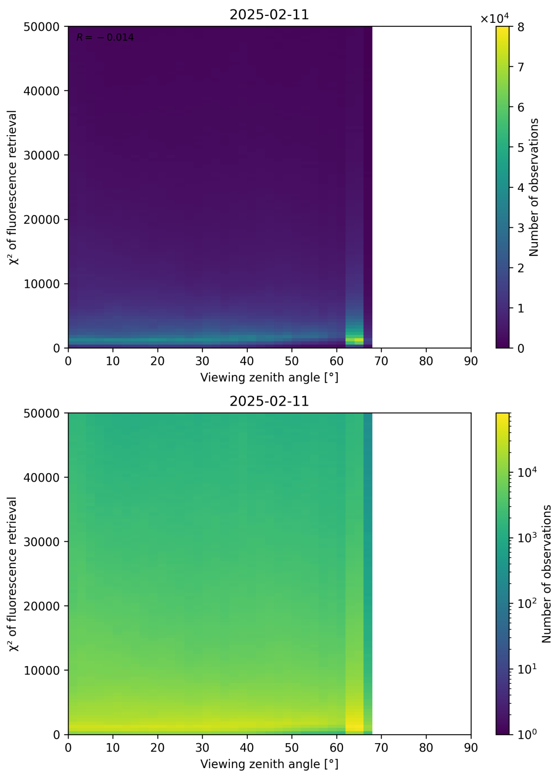
Figure 119: Scatter density plot of “Viewing zenith angle” against “ \chi^2 of fluorescence retrieval” for 2025-02-10 to 2025-02-12.
