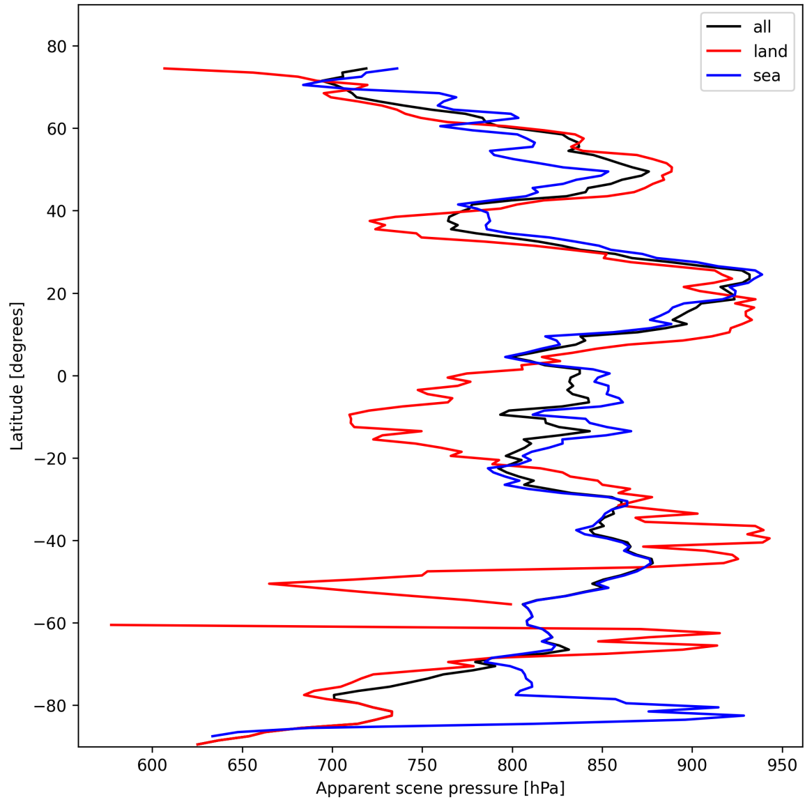
Figure 19: Zonal average of “Apparent scene pressure” for 2025-02-10 to 2025-02-12.
