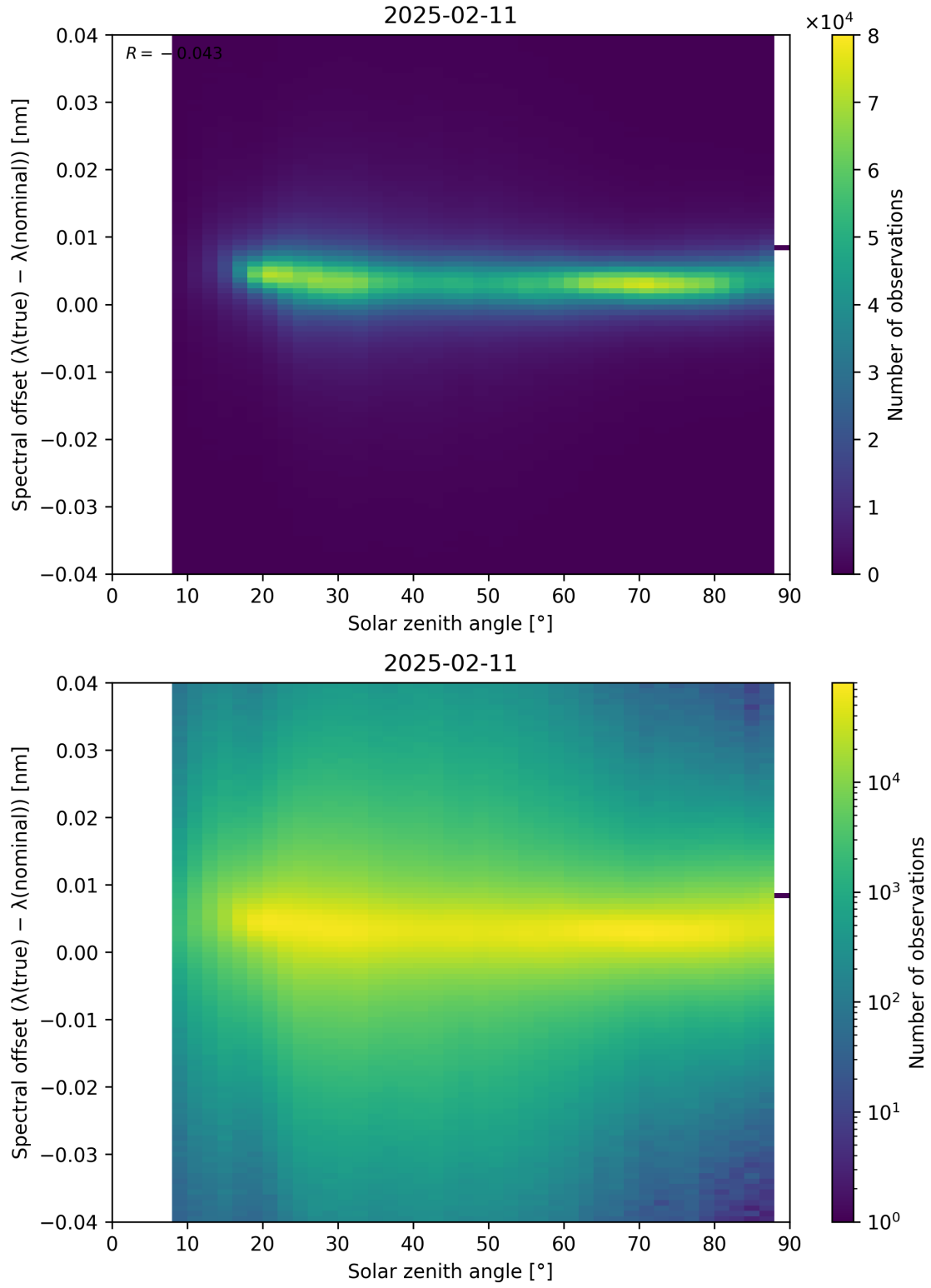
Figure 117: Scatter density plot of “Solar zenith angle” against “Spectral offset ( \lambda_{\text{true}} - \lambda_{\text{nominal}} )” for 2025-02-10 to 2025-02-12.
