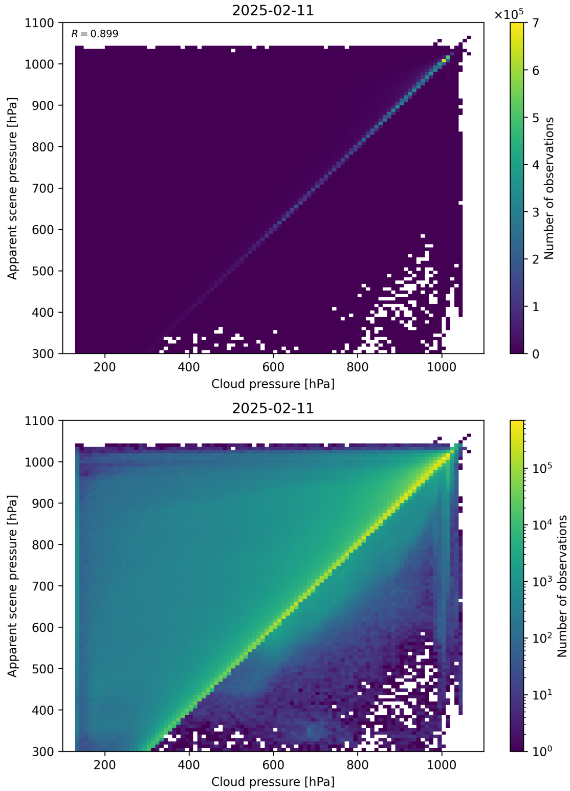
Figure 77: Scatter density plot of “Cloud pressure” against “Apparent scene pressure” for 2025-02-10 to 2025-02-12.
