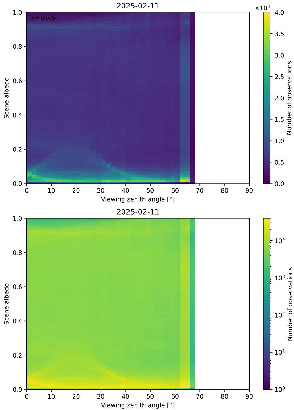
Figure 126: Scatter density plot of “Viewing zenith angle” against “Scene albedo” for 2025-02-10 to 2025-02-12.
