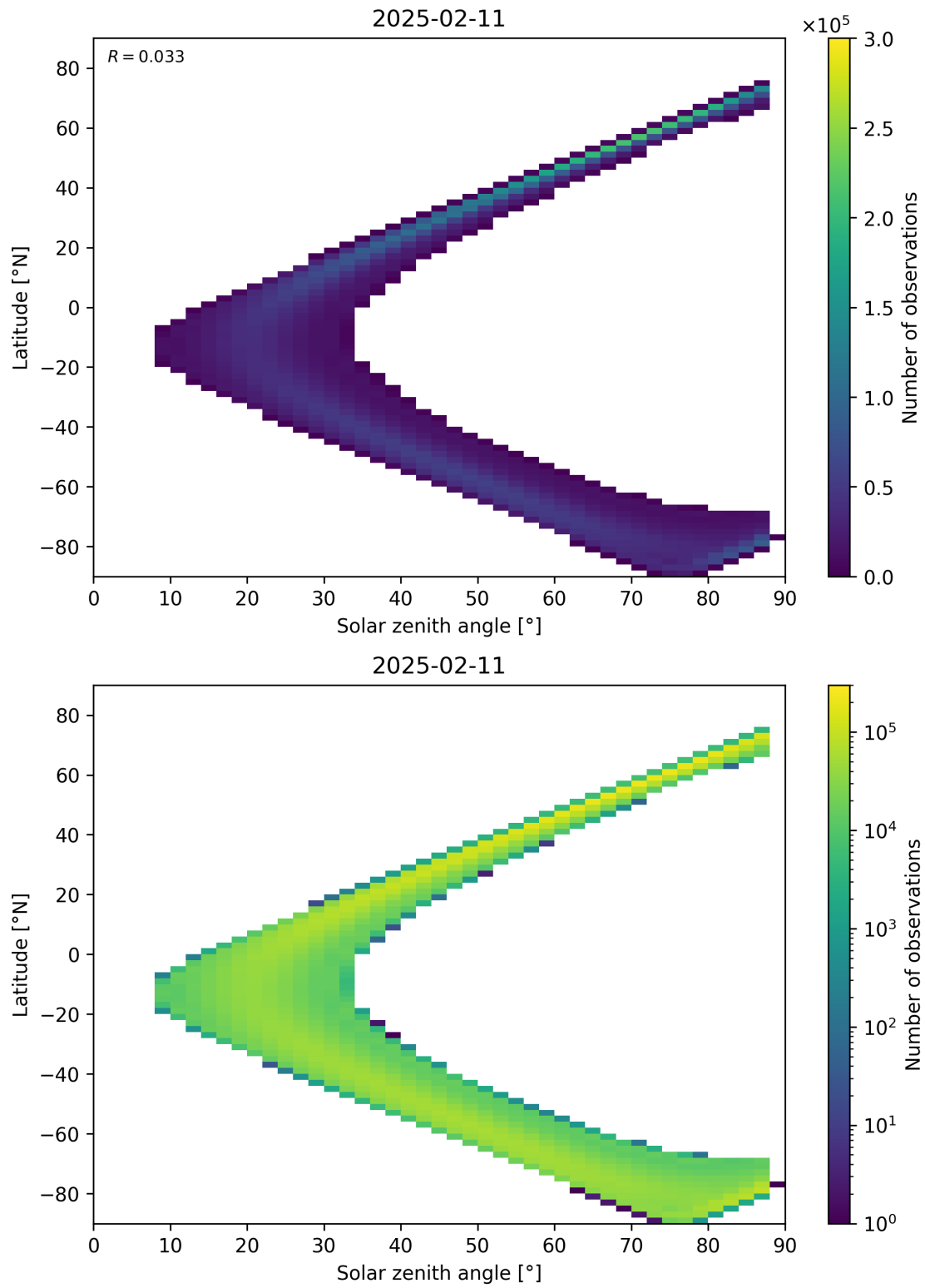
Figure 113: Scatter density plot of “Solar zenith angle” against “Latitude” for 2025-02-10 to 2025-02-12.
