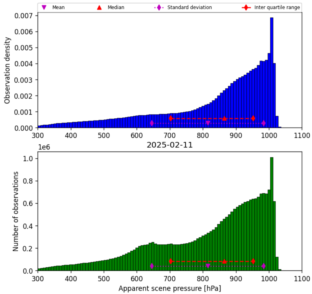
Figure 36: Histogram of “Apparent scene pressure” for 2025-02-10 to 2025-02-12
