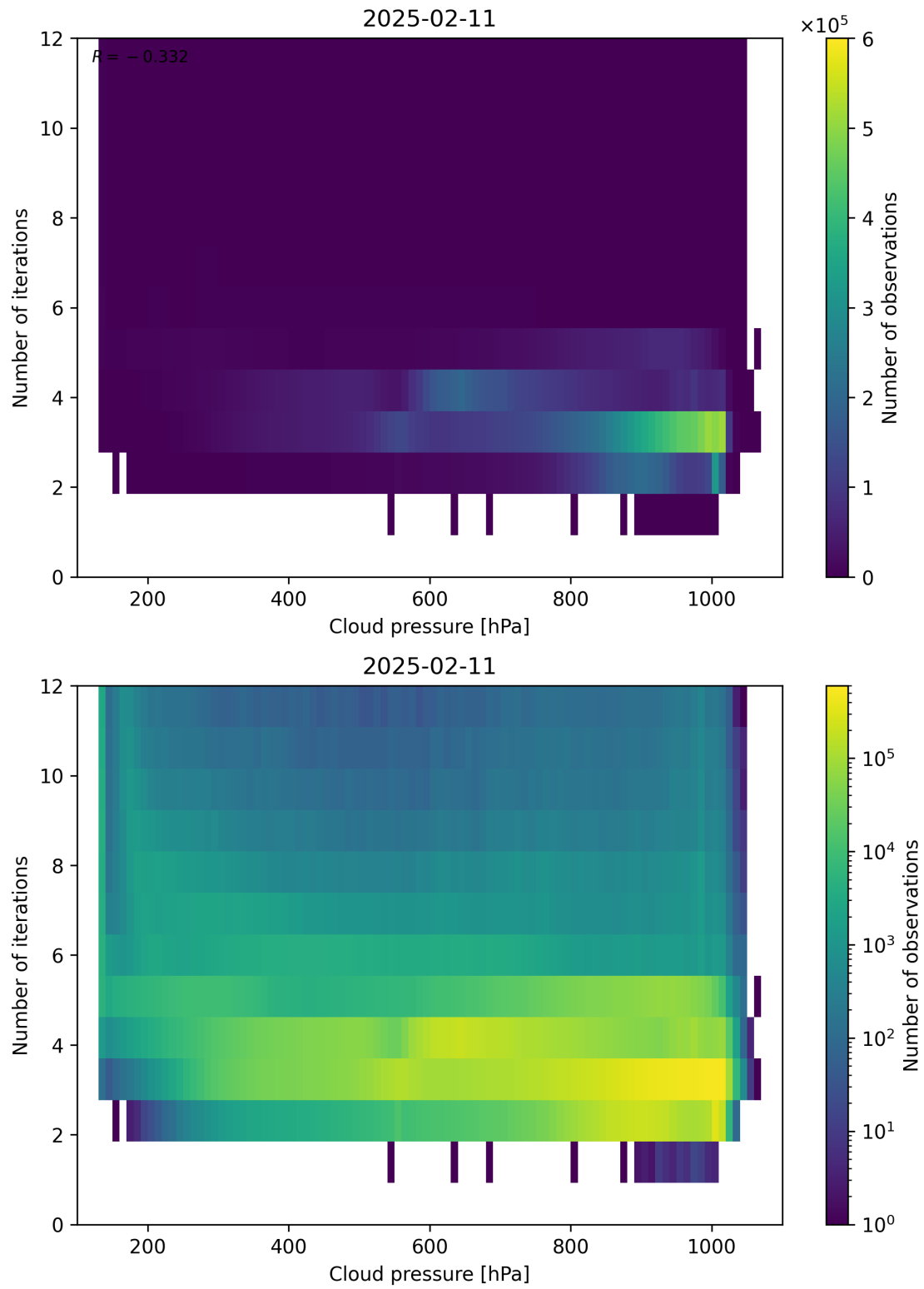
Figure 81: Scatter density plot of “Cloud pressure” against “Number of iterations” for 2025-02-10 to 2025-02-12.
