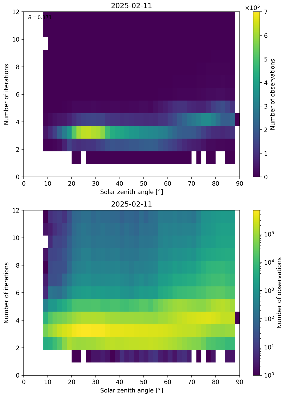
Figure 114: Scatter density plot of “Solar zenith angle” against “Number of iterations” for 2025-02-10 to 2025-02-12.
