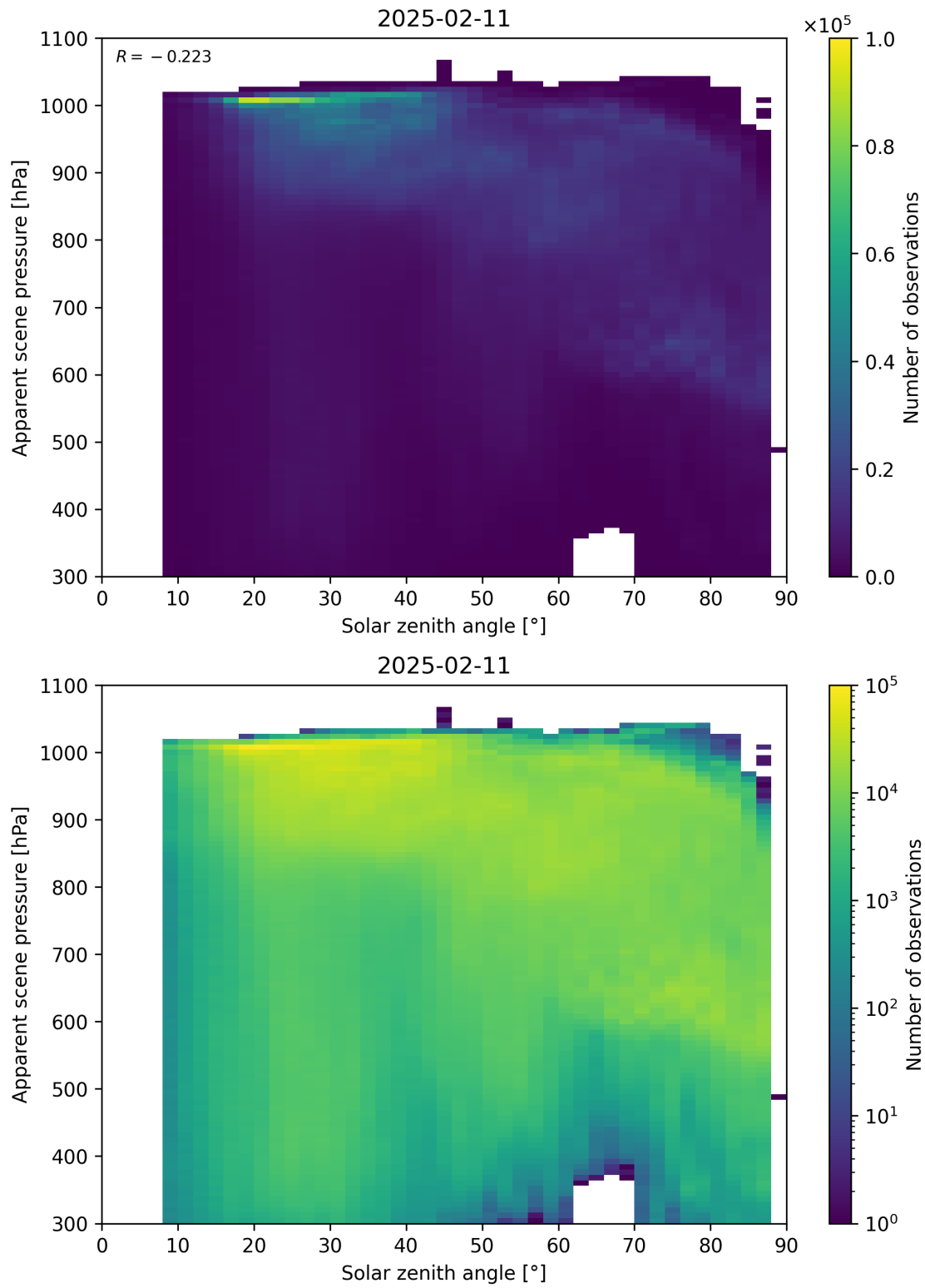
Figure 108: Scatter density plot of “Solar zenith angle” against “Apparent scene pressure” for 2025-02-10 to 2025-02-12.
