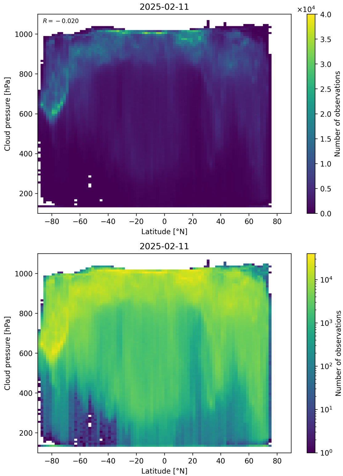
Figure 91: Scatter density plot of “Latitude” against “Cloud pressure” for 2025-02-10 to 2025-02-12.
