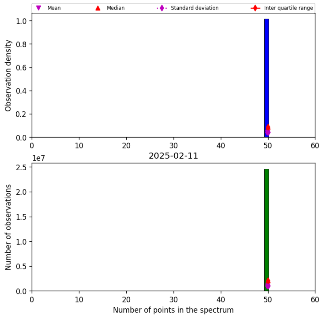
Figure 44: Histogram of "Number of points in the spectrum" for 2025-02-10 to 2025-02-12
