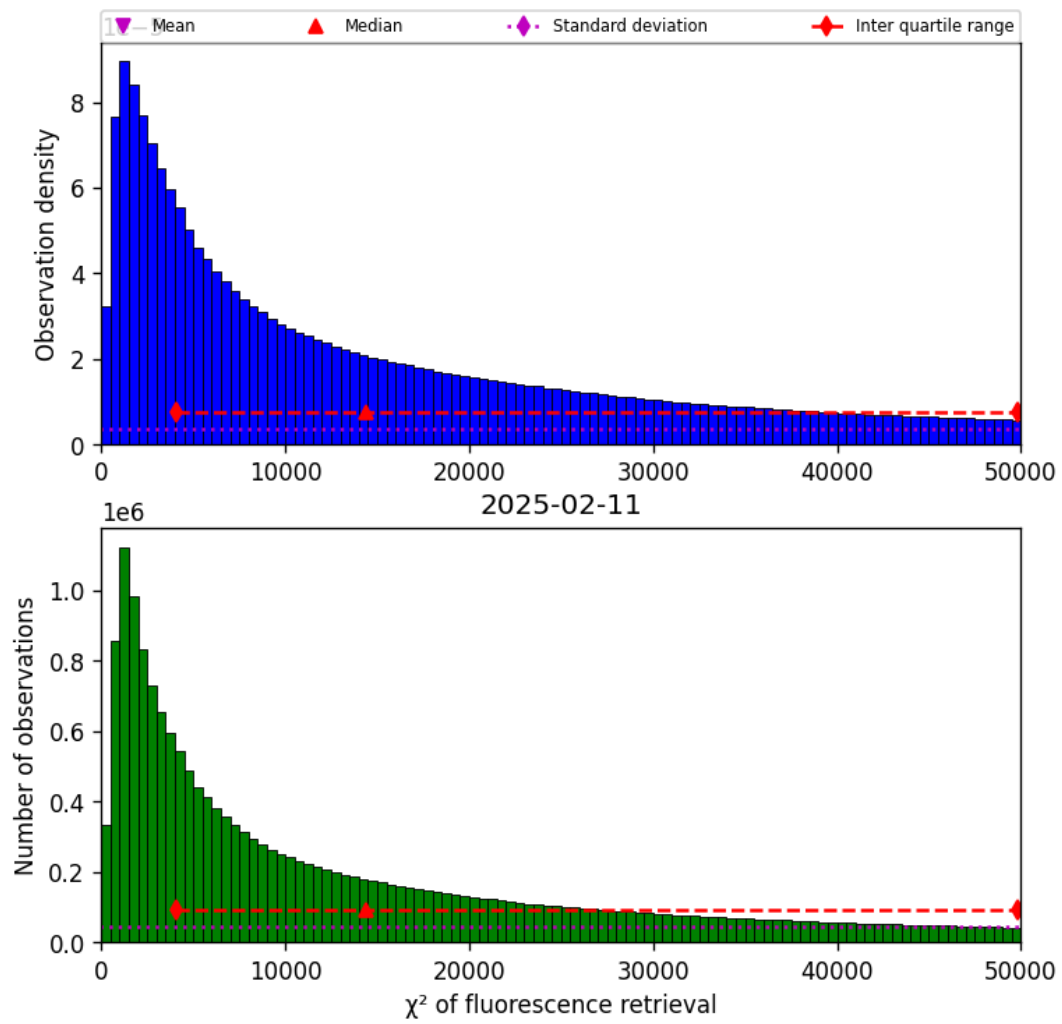
Figure 42: Histogram of “ \chi^2 of fluorescence retrieval” for 2025-02-10 to 2025-02-12
