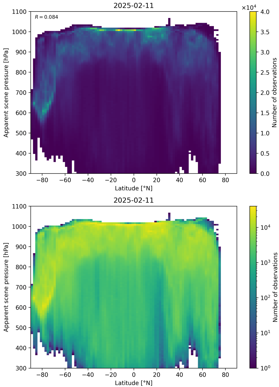
Figure 88: Scatter density plot of “Latitude” against “Apparent scene pressure” for 2025-02-10 to 2025-02-12.
