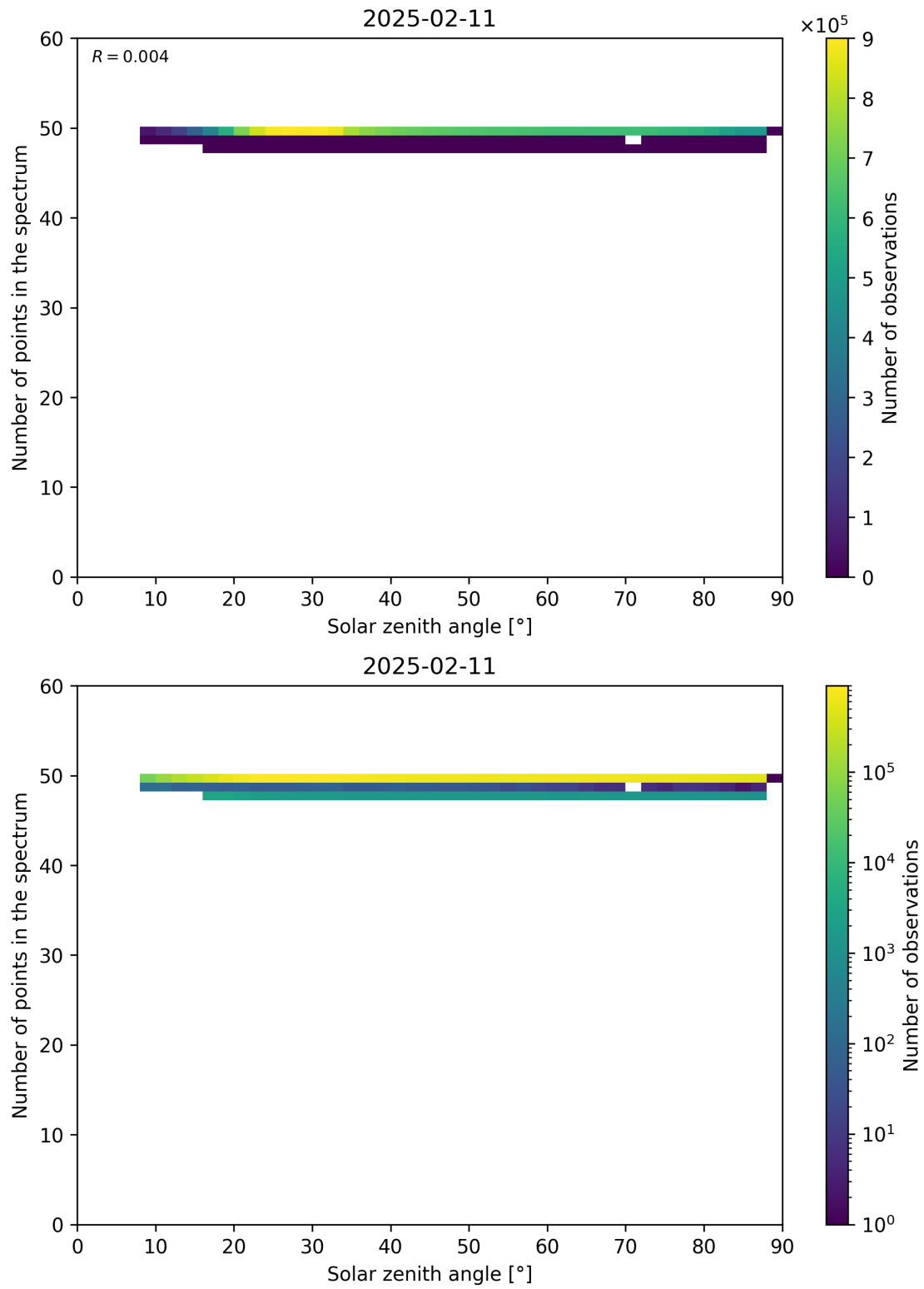
Figure 115: Scatter density plot of “Solar zenith angle” against “Number of points in the spectrum” for 2025-02-10 to 2025-02-12.
