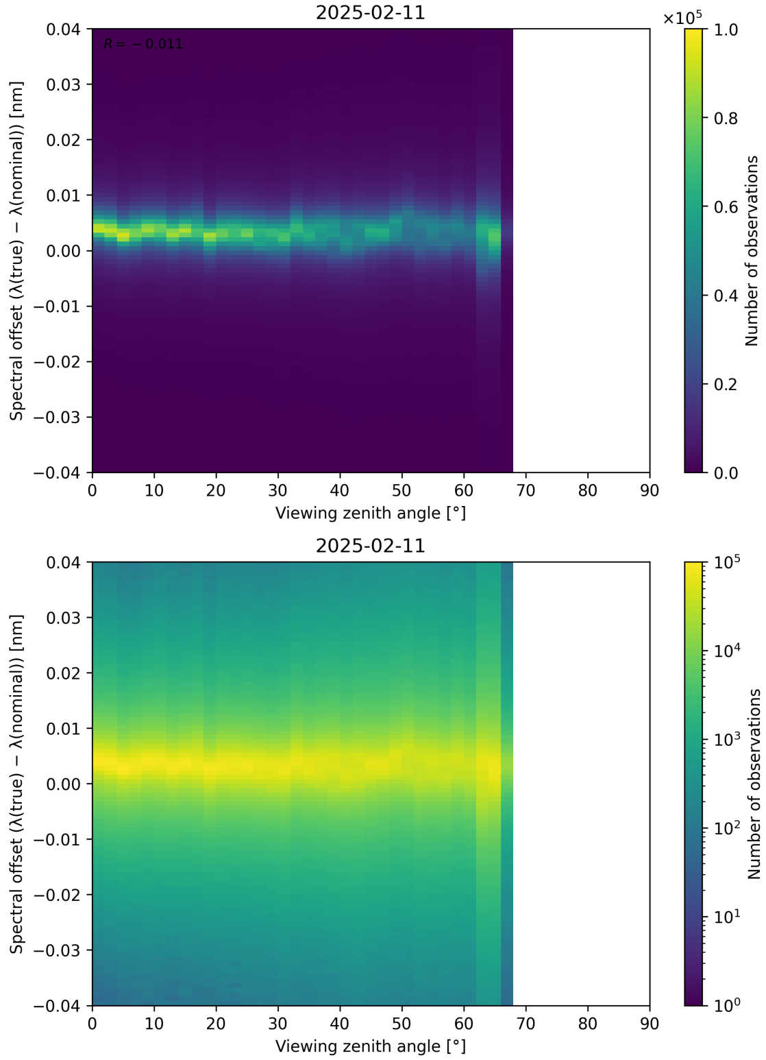
Figure 128: Scatter density plot of “Viewing zenith angle” against “Spectral offset ( \lambda_{\text{true}} - \lambda_{\text{nominal}} )” for 2025-02-10 to 2025-02-12.
