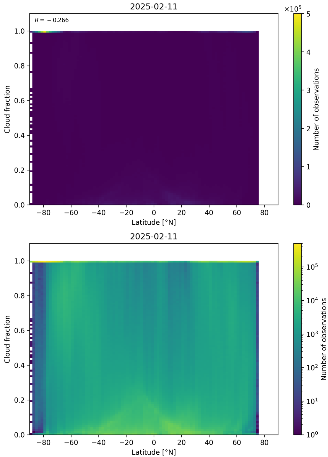
Figure 90: Scatter density plot of “Latitude” against “Cloud fraction” for 2025-02-10 to 2025-02-12.
