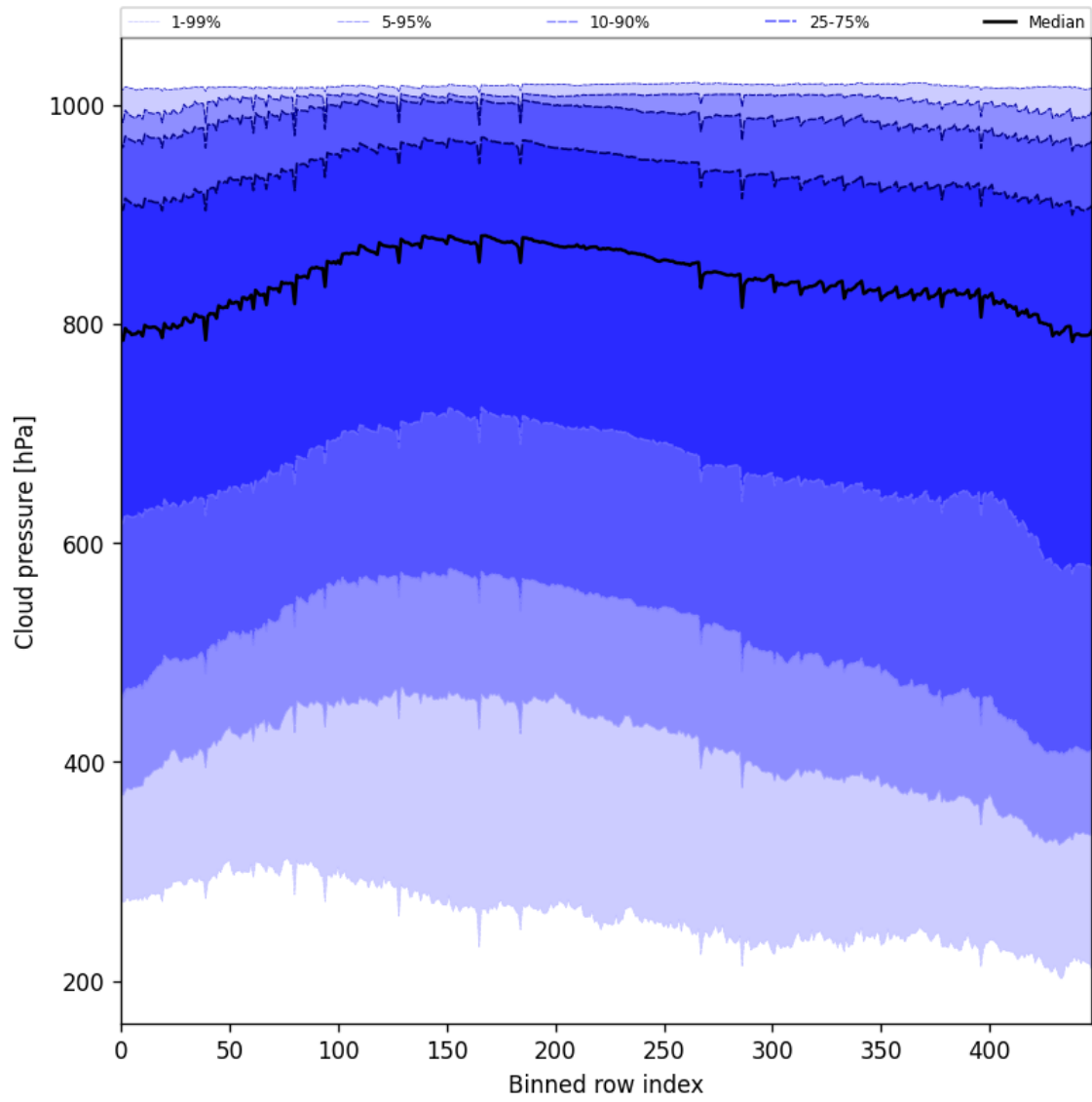
Figure 47: Along track statistics of “Cloud pressure” for 2025-02-10 to 2025-02-12
