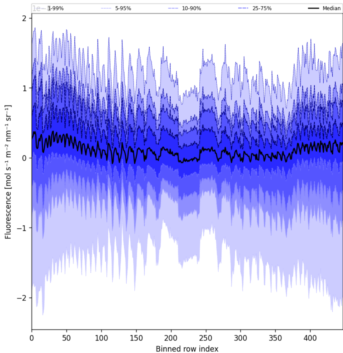
Figure 57: Along track statistics of “Fluorescence” for 2025-02-10 to 2025-02-12
