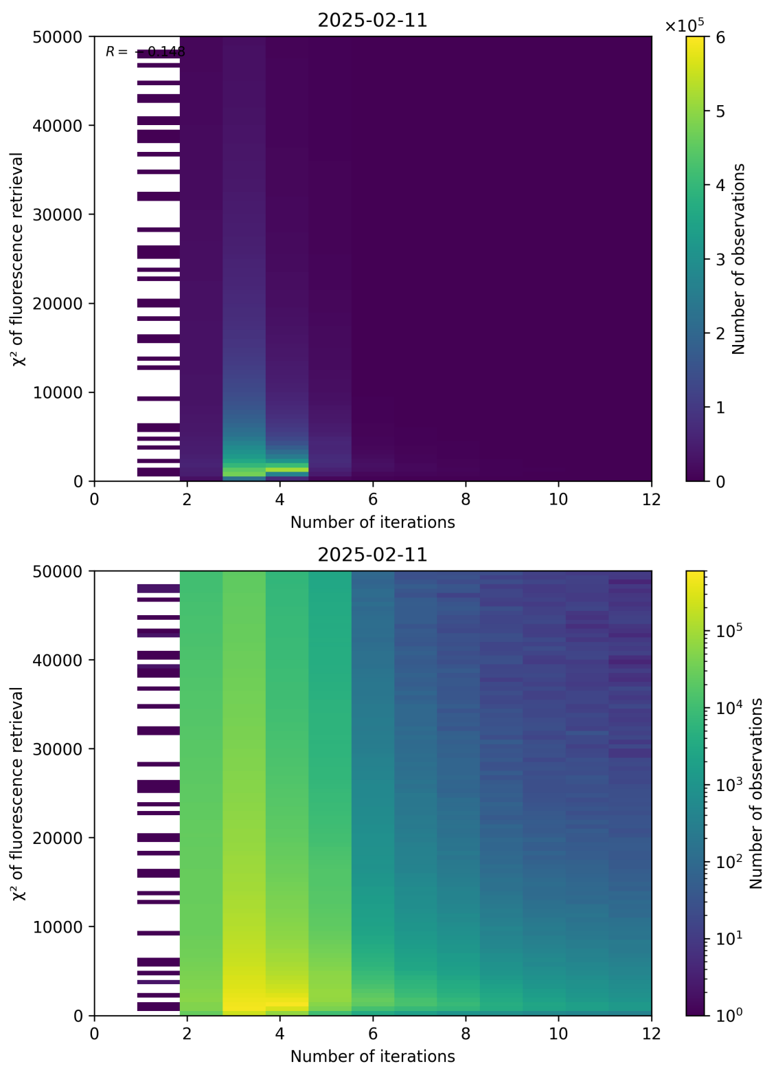
Figure 97: Scatter density plot of “Number of iterations” against “ \chi^2 of fluorescence retrieval” for 2025-02-10 to 2025-02-12.
