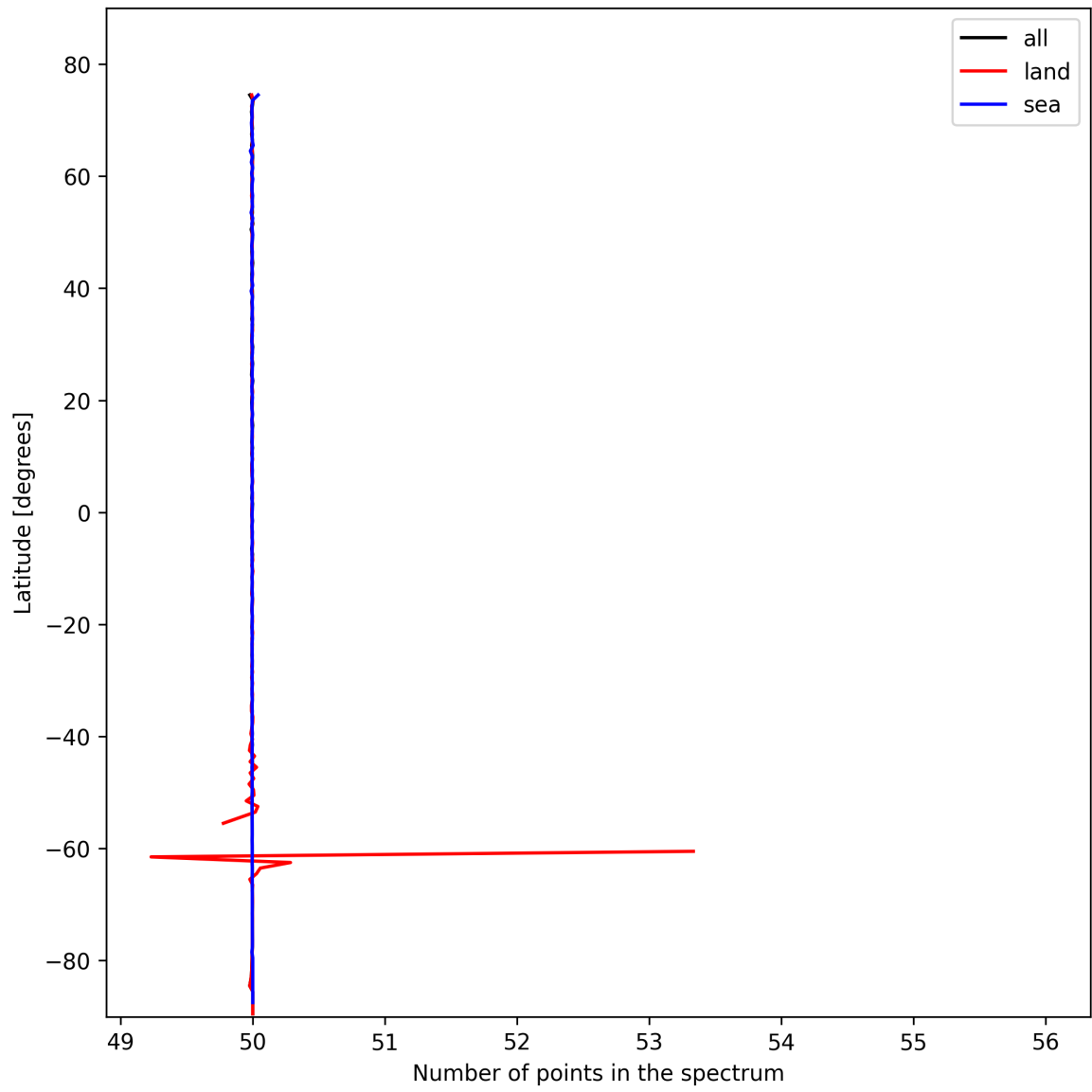
Figure 27: Zonal average of “Number of points in the spectrum” for 2025-02-10 to 2025-02-12.
