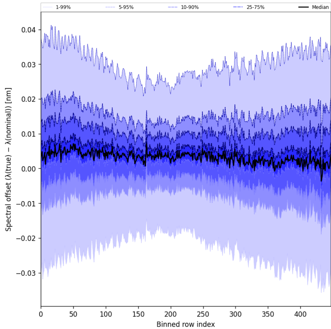
Figure 62: Along track statistics of “Spectral offset ( \lambda_{\text{true}} - \lambda_{\text{nominal}} )” for 2025-02-10 to 2025-02-12
