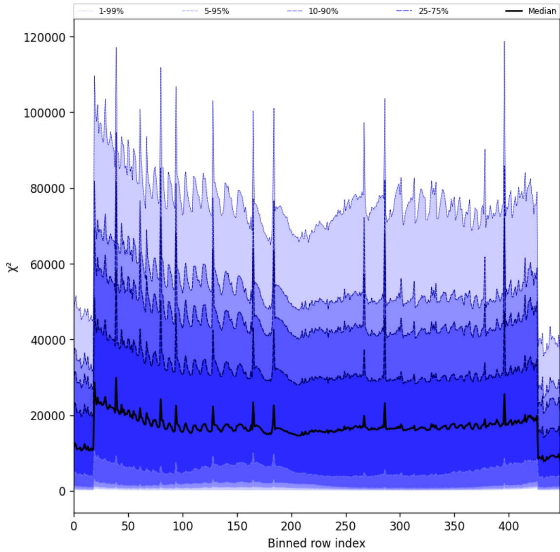
Figure 55: Along track statistics of “ \chi^2 ” for 2025-02-10 to 2025-02-12
