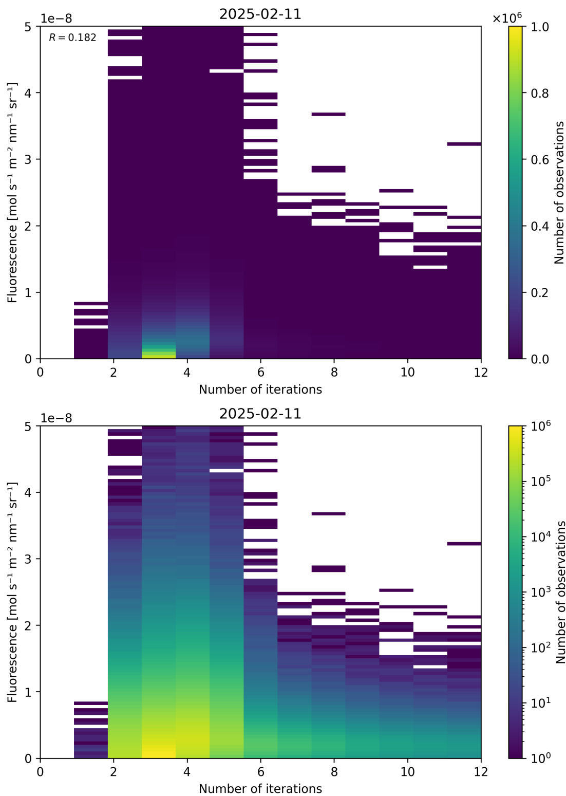
Figure 98: Scatter density plot of “Number of iterations” against “Fluorescence” for 2025-02-10 to 2025-02-12.
