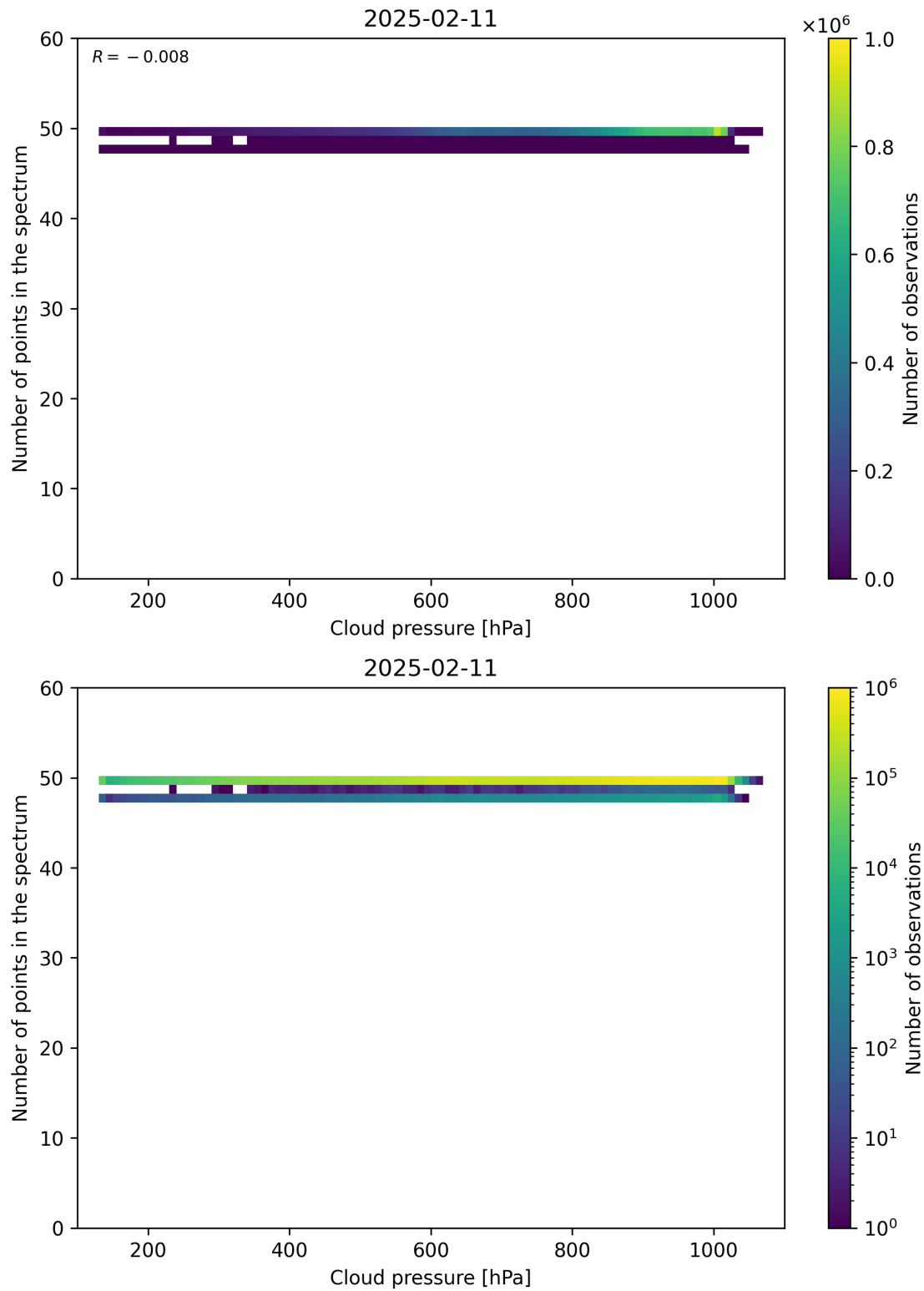
Figure 82: Scatter density plot of “Cloud pressure” against “Number of points in the spectrum” for 2025-02-10 to 2025-02-12.
