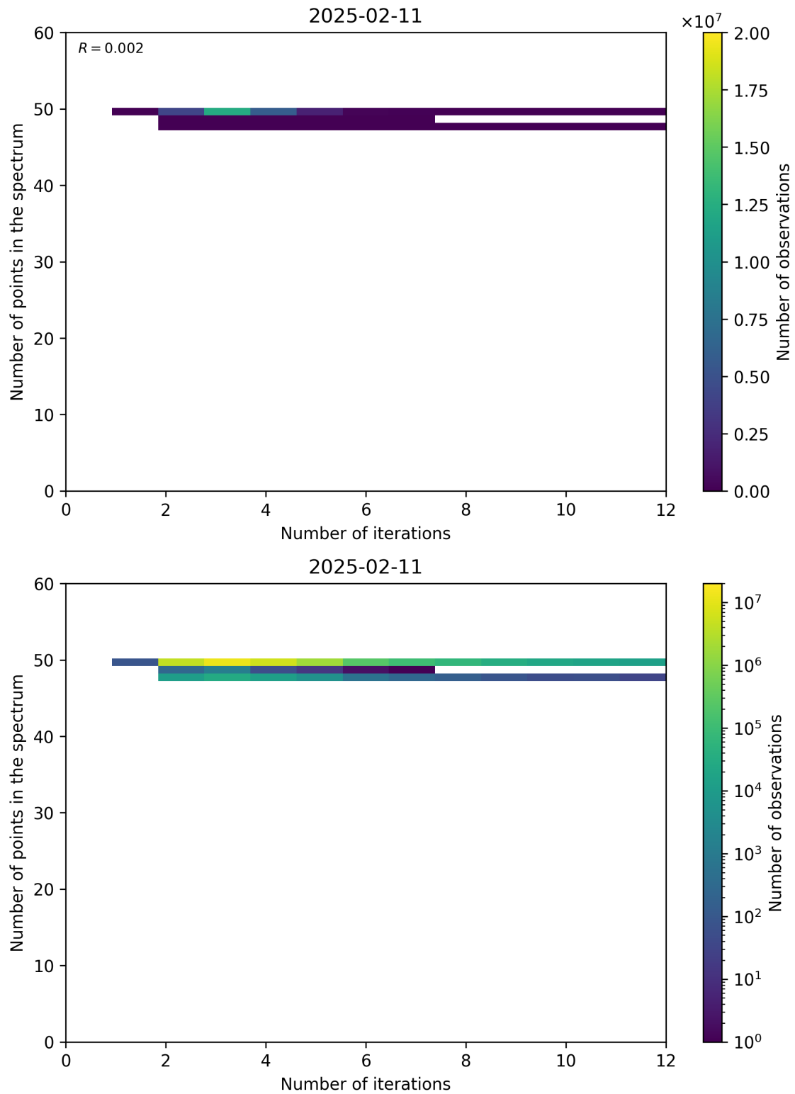
Figure 99: Scatter density plot of “Number of iterations” against “Number of points in the spectrum” for 2025-02-10 to 2025-02-12.
