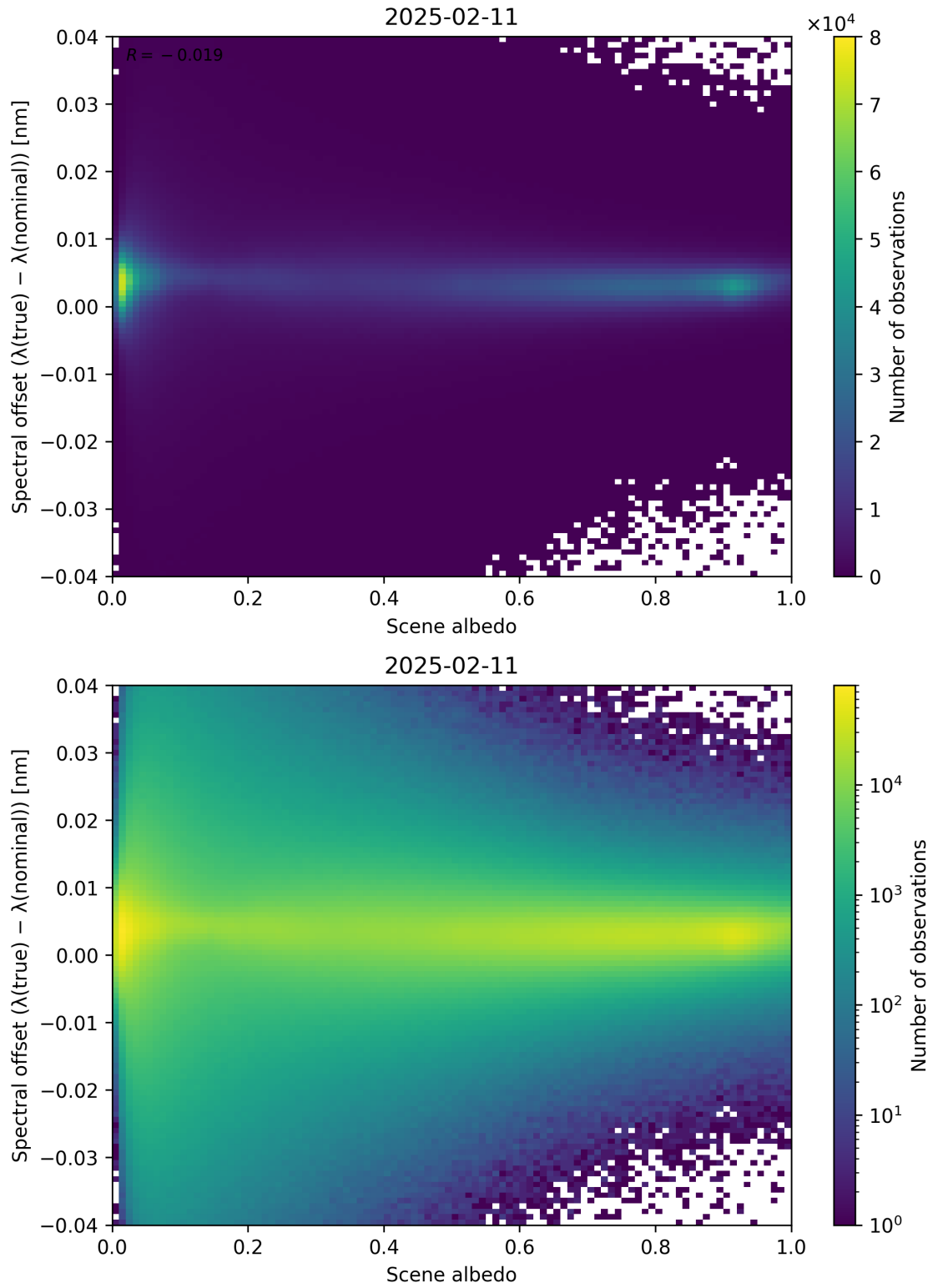
Figure 107: Scatter density plot of “Scene albedo” against “Spectral offset ( \lambda_{\text{true}} - \lambda_{\text{nominal}} )” for 2025-02-10 to 2025-02-12.
