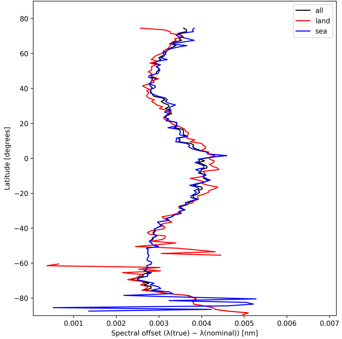
Figure 28: Zonal average of “Spectral offset ( \lambda_{\text{true}} - \lambda_{\text{nominal}} )” for 2025-02-10 to 2025-02-12.
