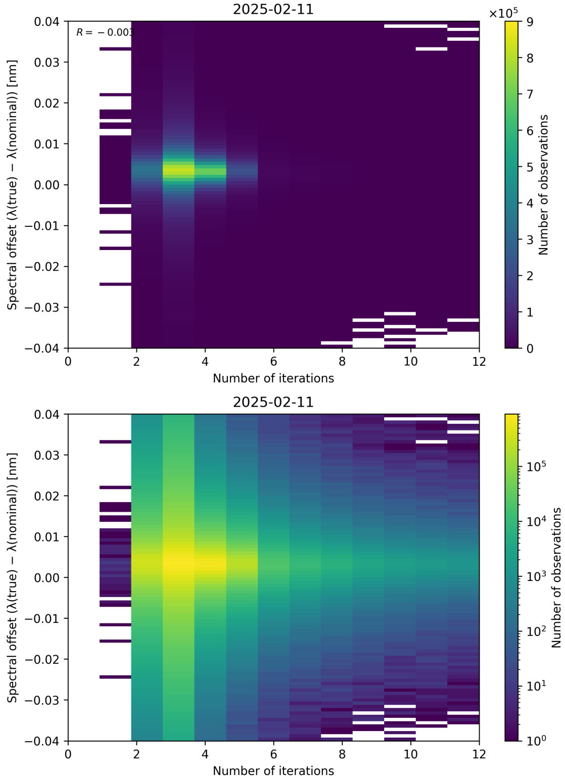
Figure 100: Scatter density plot of “Number of iterations” against “Spectral offset ( \lambda_{\text{true}} - \lambda_{\text{nominal}} )” for 2025-02-10 to 2025-02-12.
