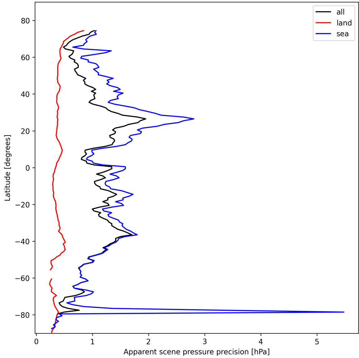
Figure 20: Zonal average of “Apparent scene pressure precision” for 2025-02-10 to 2025-02-12.
