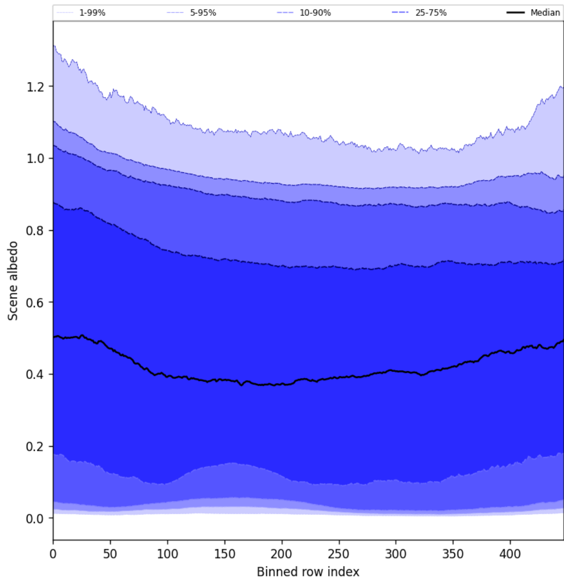
Figure 51: Along track statistics of “Scene albedo” for 2025-02-10 to 2025-02-12
