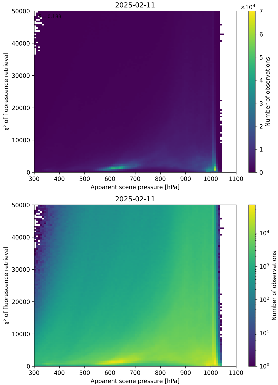
Figure 63: Scatter density plot of “Apparent scene pressure” against “ \chi^2 of fluorescence retrieval” for 2025-02-10 to 2025-02-12.
