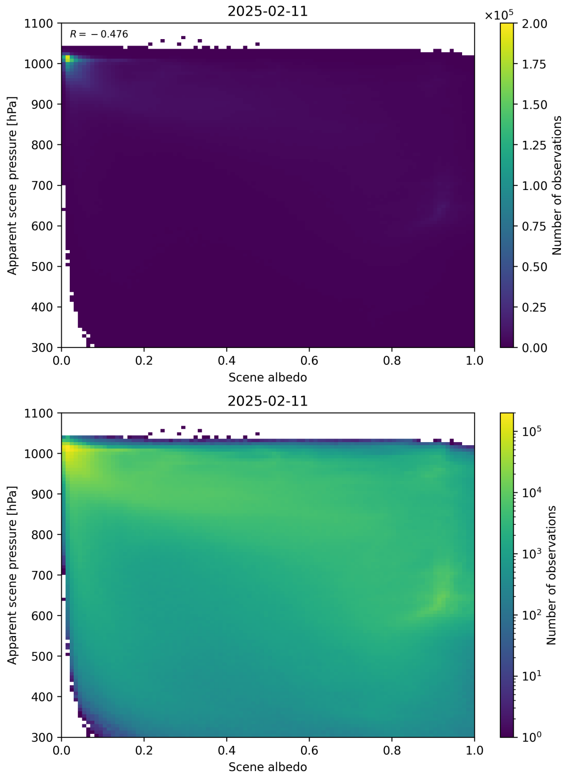
Figure 102: Scatter density plot of “Scene albedo” against “Apparent scene pressure” for 2025-02-10 to 2025-02-12.
