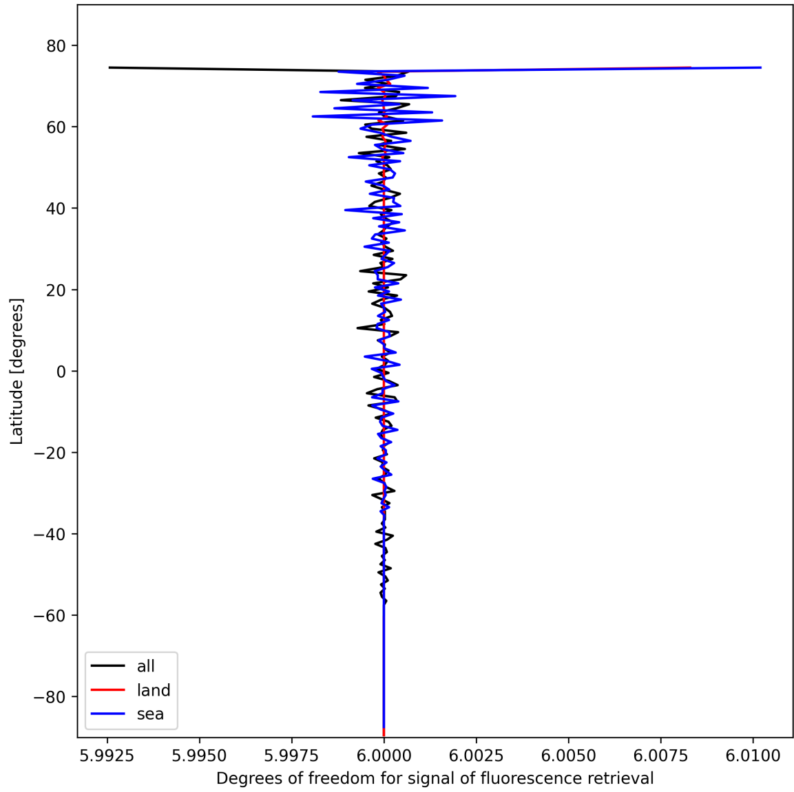
Figure 26: Zonal average of “Degrees of freedom for signal of fluorescence retrieval” for 2025-02-10 to 2025-02-12.
