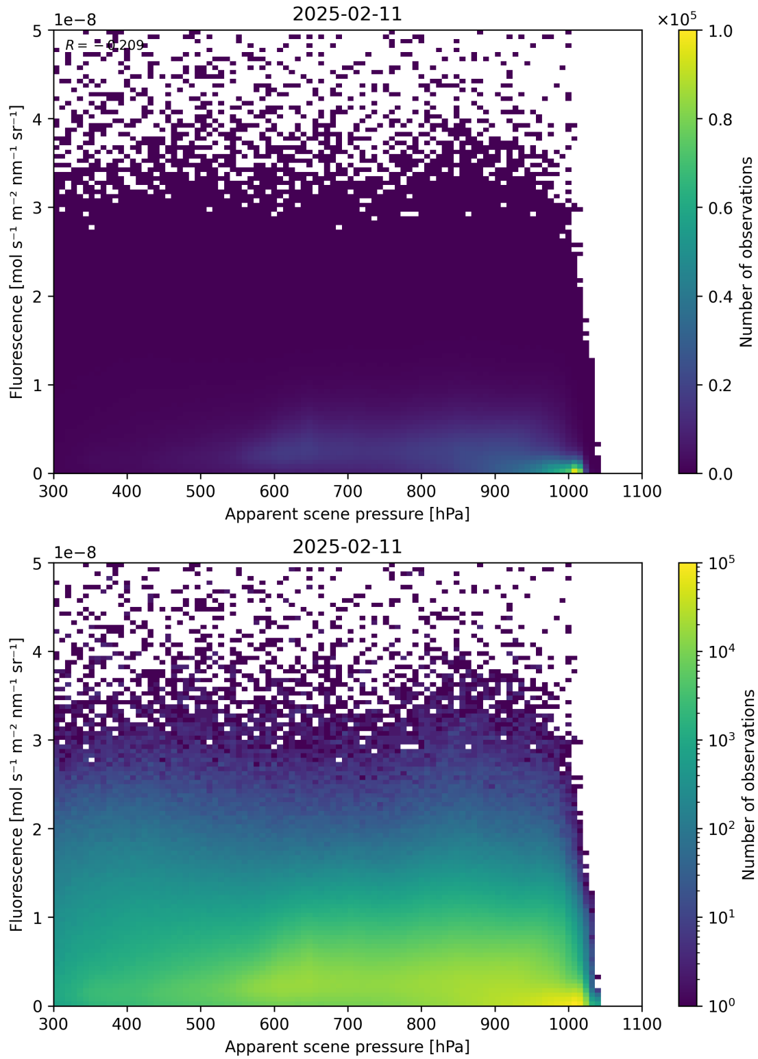
Figure 64: Scatter density plot of “Apparent scene pressure” against “Fluorescence” for 2025-02-10 to 2025-02-12.
