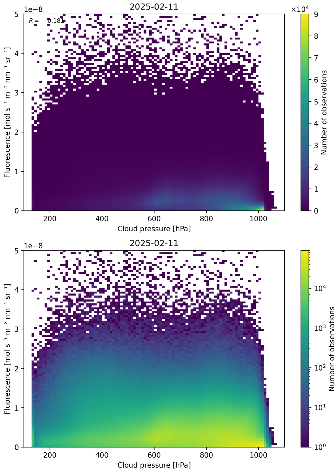
Figure 80: Scatter density plot of “Cloud pressure” against “Fluorescence” for 2025-02-10 to 2025-02-12.
