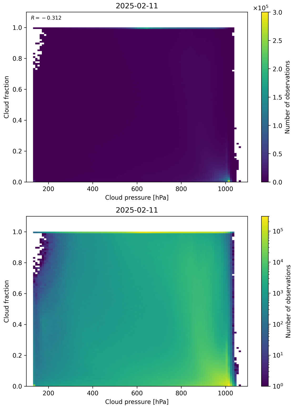
Figure 79: Scatter density plot of “Cloud pressure” against “Cloud fraction” for 2025-02-10 to 2025-02-12.
