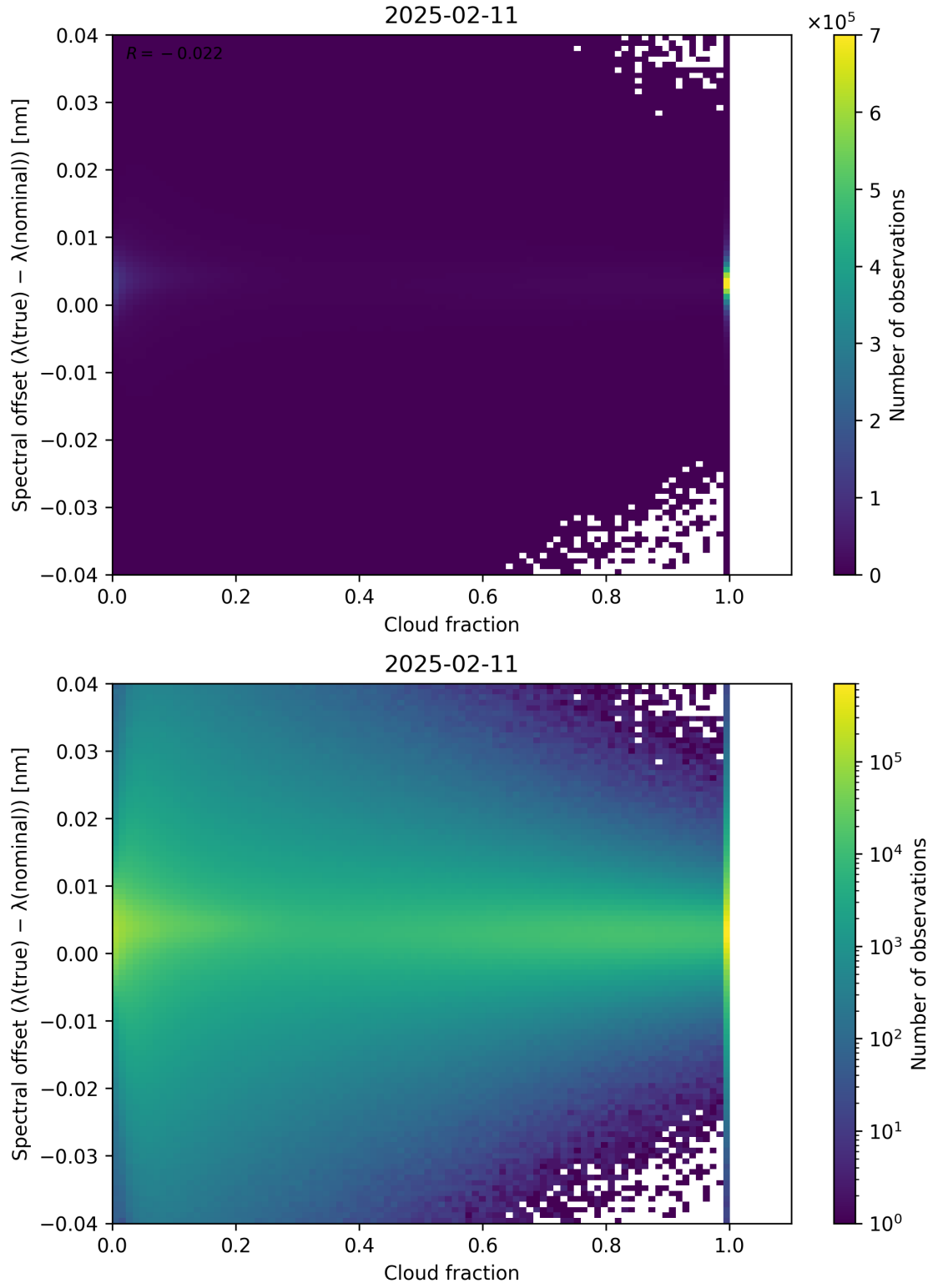
Figure 76: Scatter density plot of “Cloud fraction” against “Spectral offset ( \lambda_{\text{true}} - \lambda_{\text{nominal}} )” for 2025-02-10 to 2025-02-12.
