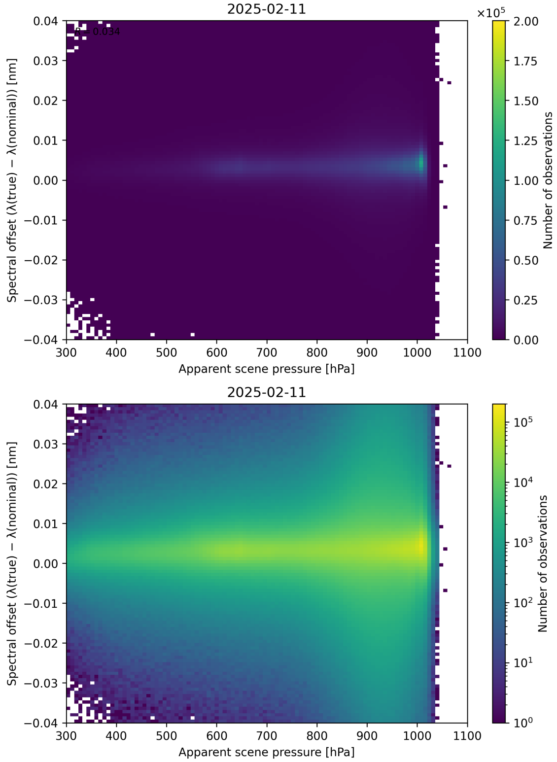
Figure 67: Scatter density plot of “Apparent scene pressure” against “Spectral offset ( \lambda_{\text{true}} - \lambda_{\text{nominal}} )” for 2025-02-10 to 2025-02-12.
