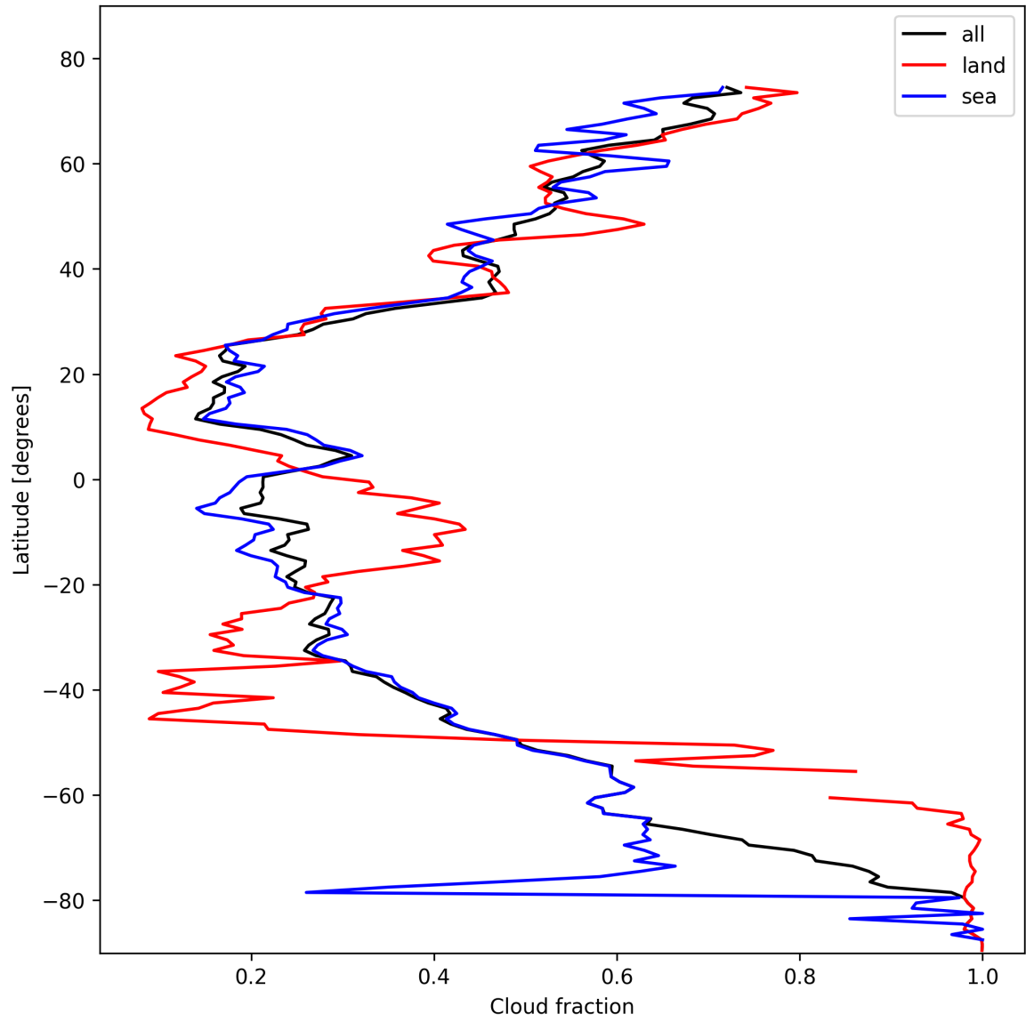
Figure 15: Zonal average of “Cloud fraction” for 2025-02-10 to 2025-02-12.
