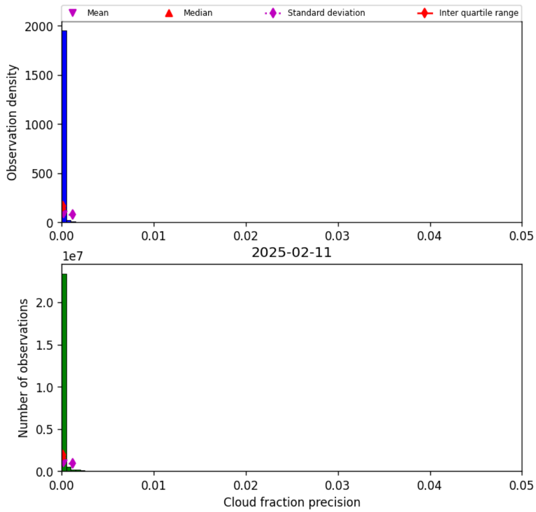
Figure 33: Histogram of “Cloud fraction precision” for 2025-02-10 to 2025-02-12
