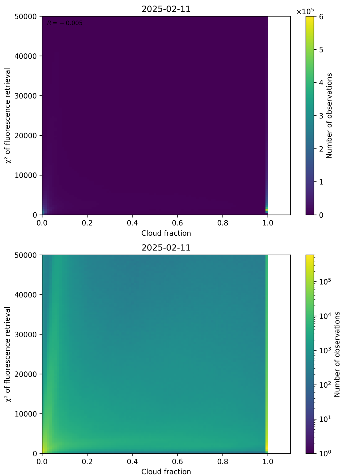
Figure 71: Scatter density plot of “Cloud fraction” against “ \chi^2 of fluorescence retrieval” for 2025-02-10 to 2025-02-12.
