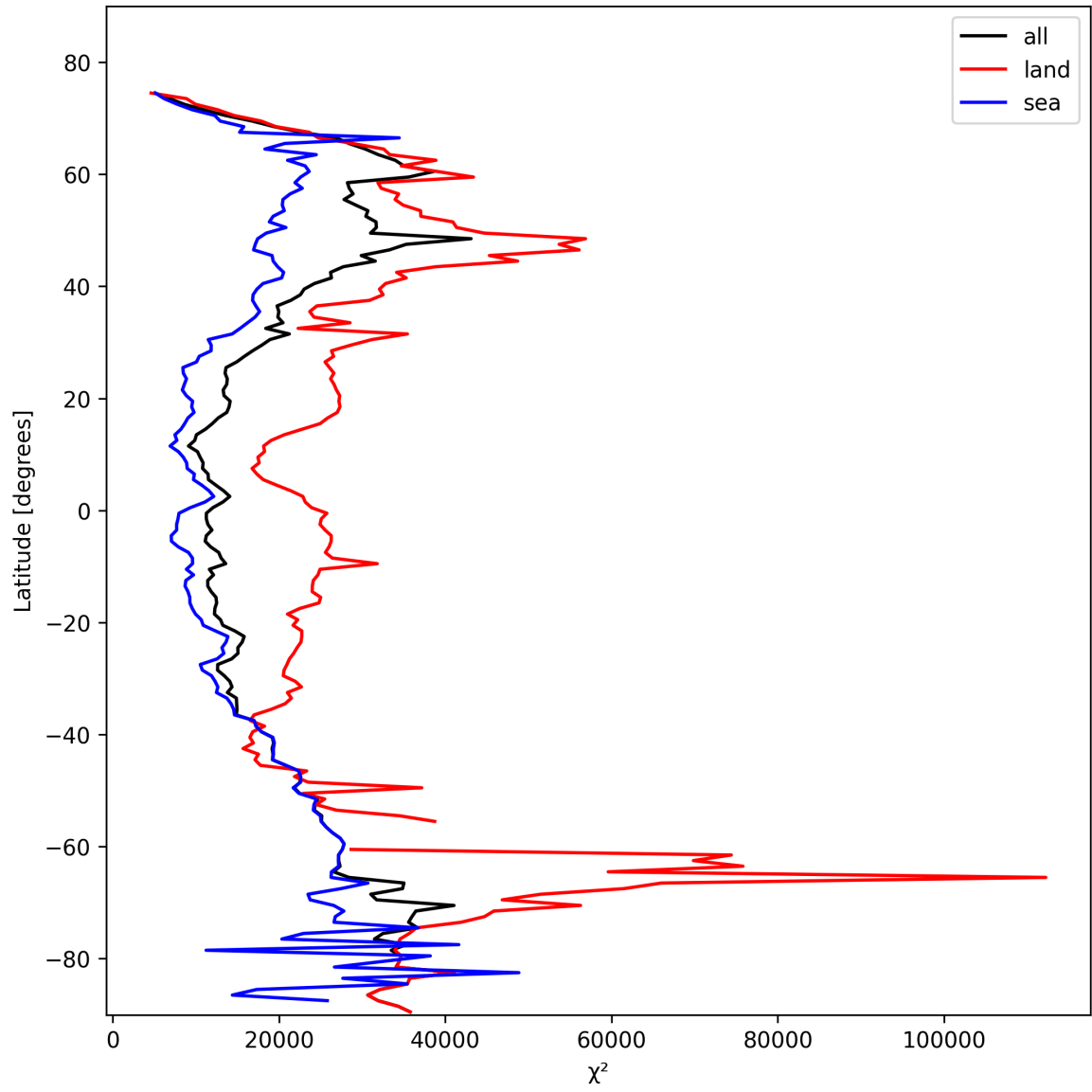
Figure 21: Zonal average of “ \chi^2 ” for 2025-02-11 to 2025-02-13.
