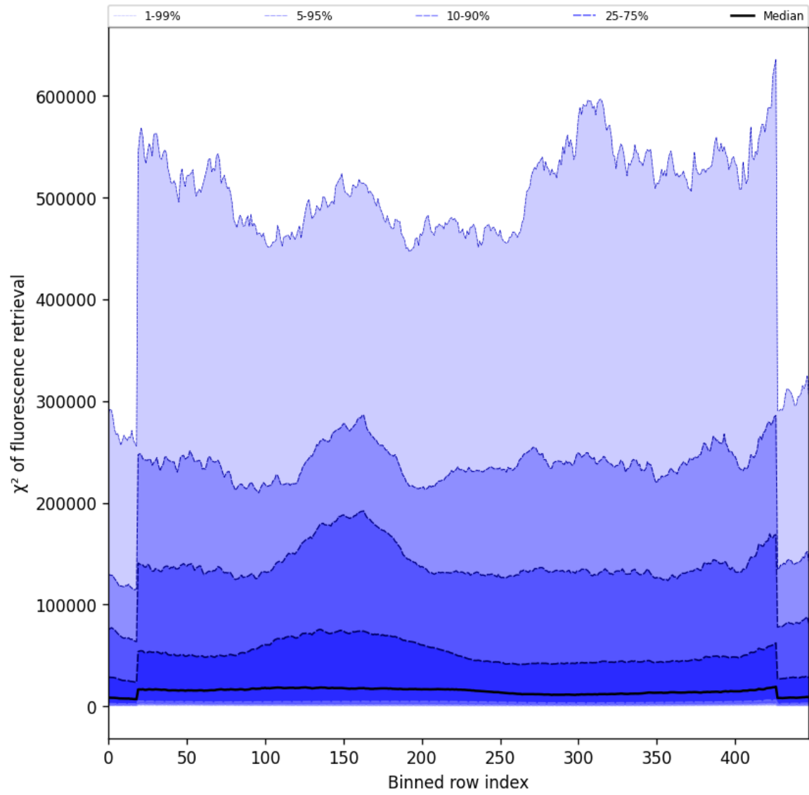
Figure 59: Along track statistics of “ \chi^2 of fluorescence retrieval” for 2025-02-11 to 2025-02-13
