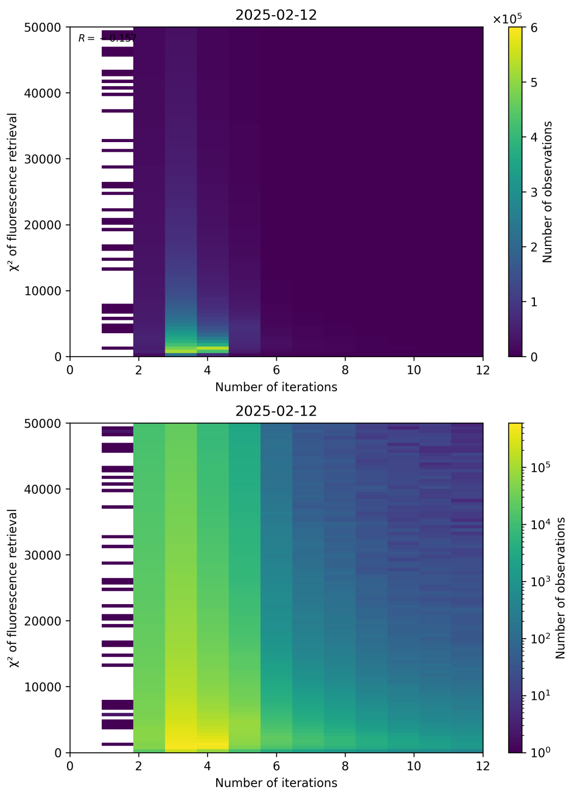
Figure 97: Scatter density plot of “Number of iterations” against “ \chi^2 of fluorescence retrieval” for 2025-02-11 to 2025-02-13.
