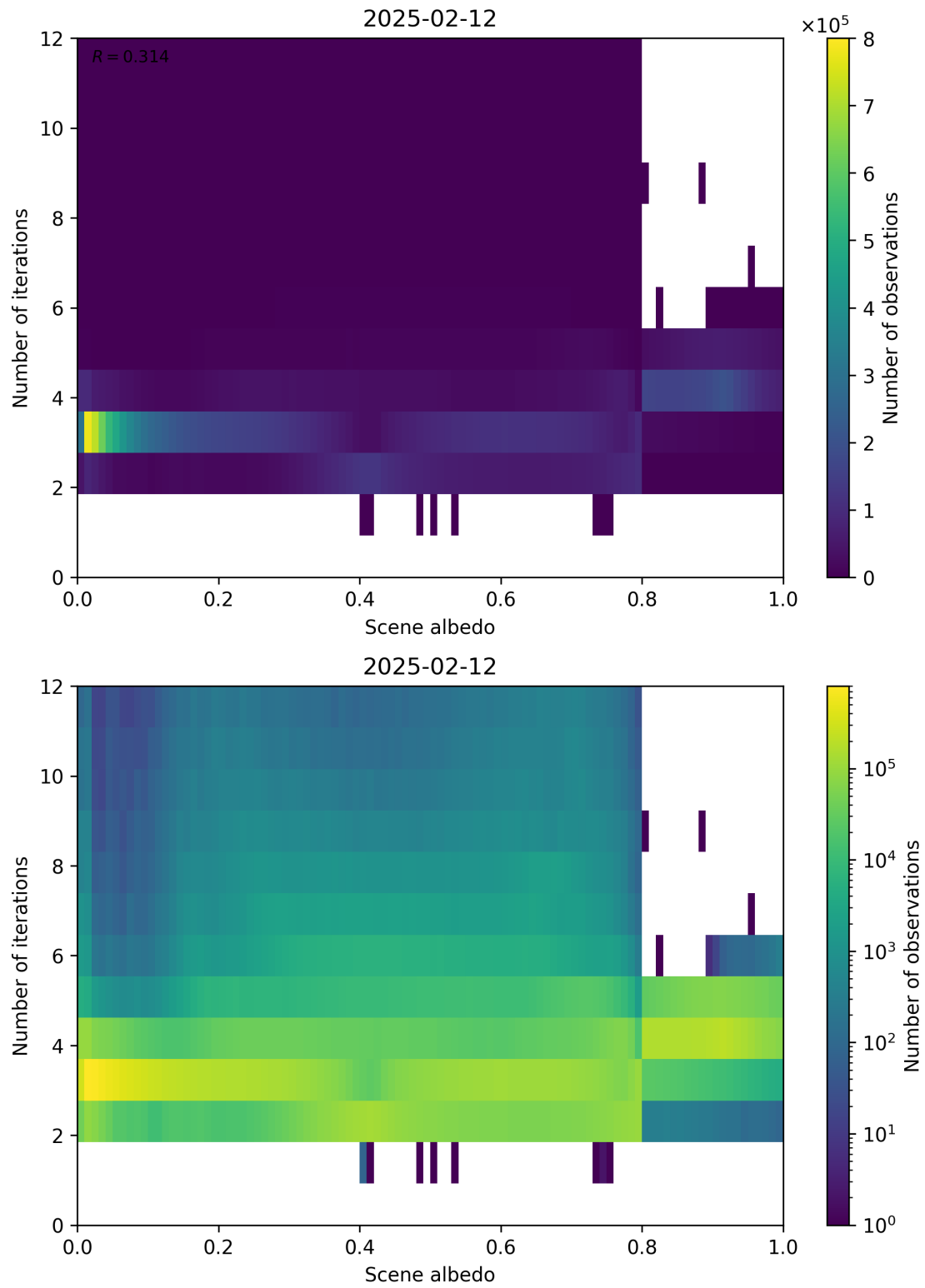
Figure 105: Scatter density plot of “Scene albedo” against “Number of iterations” for 2025-02-11 to 2025-02-13.
