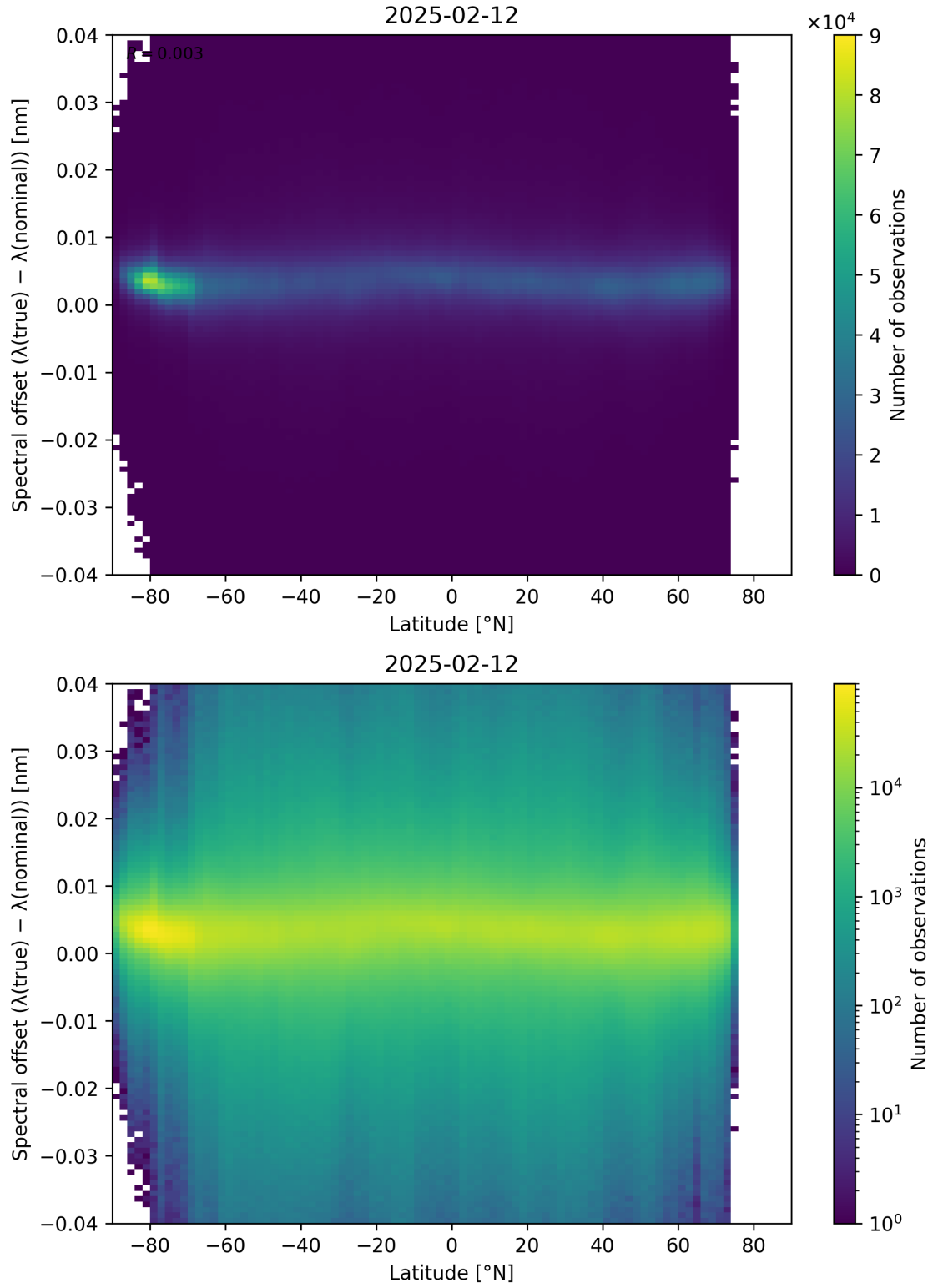
Figure 96: Scatter density plot of “Latitude” against “Spectral offset ( \lambda_{\text{true}} - \lambda_{\text{nominal}} )” for 2025-02-11 to 2025-02-13.
