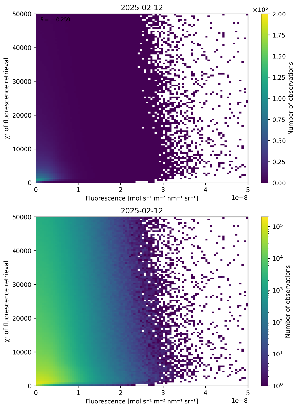
Figure 85: Scatter density plot of “Fluorescence” against “ \chi^2 of fluorescence retrieval” for 2025-02-11 to 2025-02-13.
