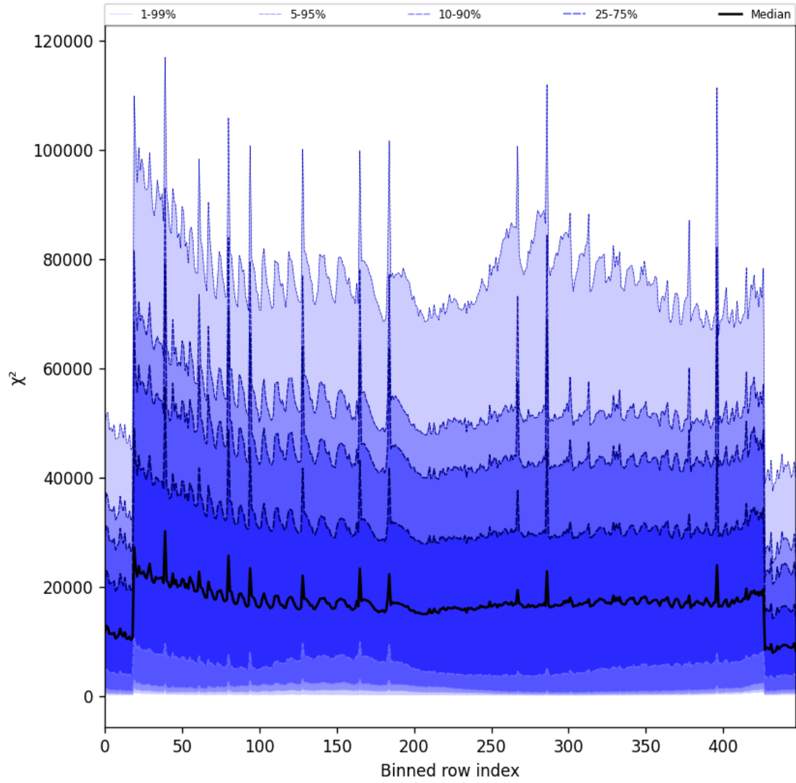
Figure 55: Along track statistics of “ \chi^2 ” for 2025-02-11 to 2025-02-13
