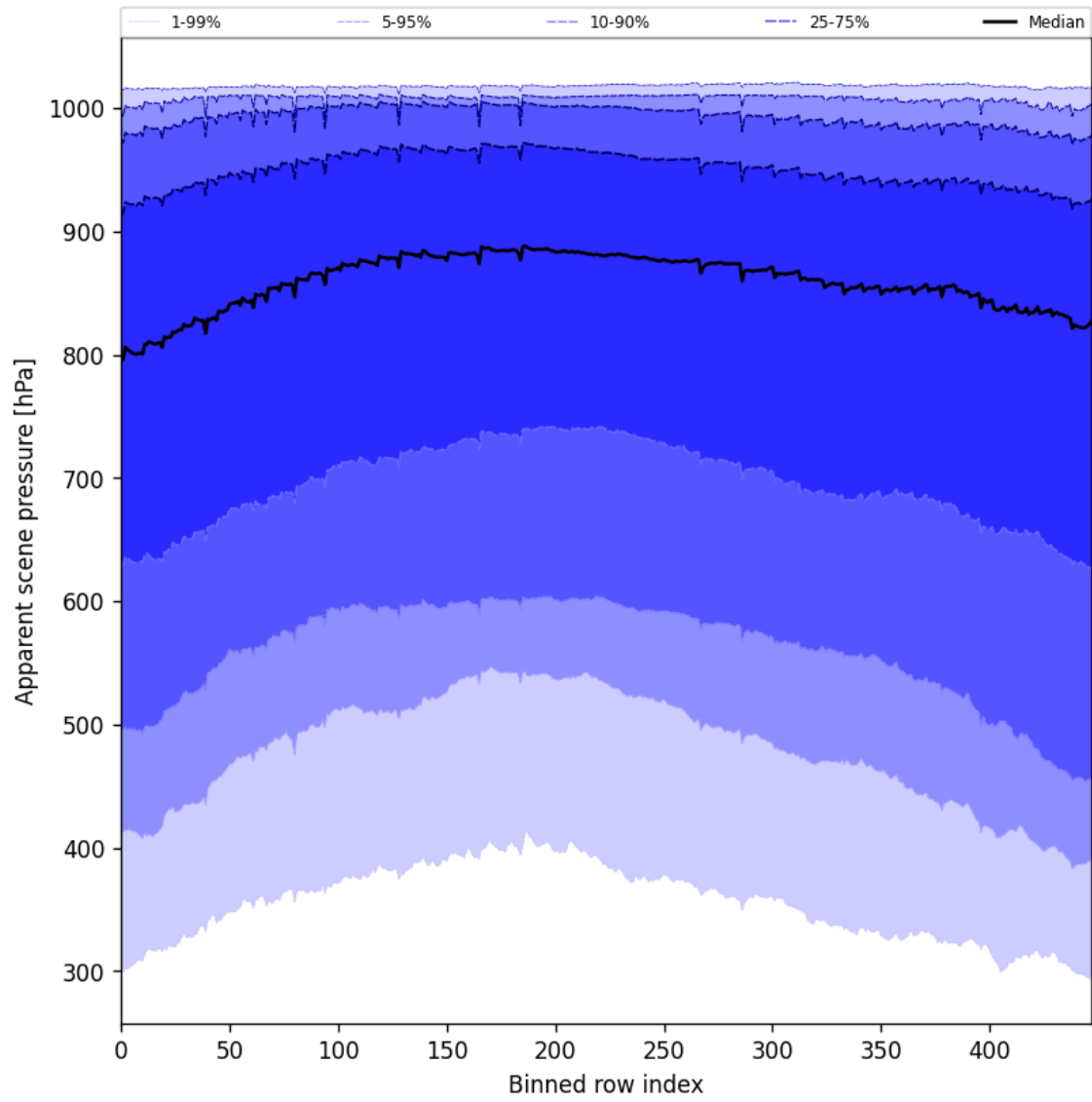
Figure 53: Along track statistics of “Apparent scene pressure” for 2025-02-11 to 2025-02-13
