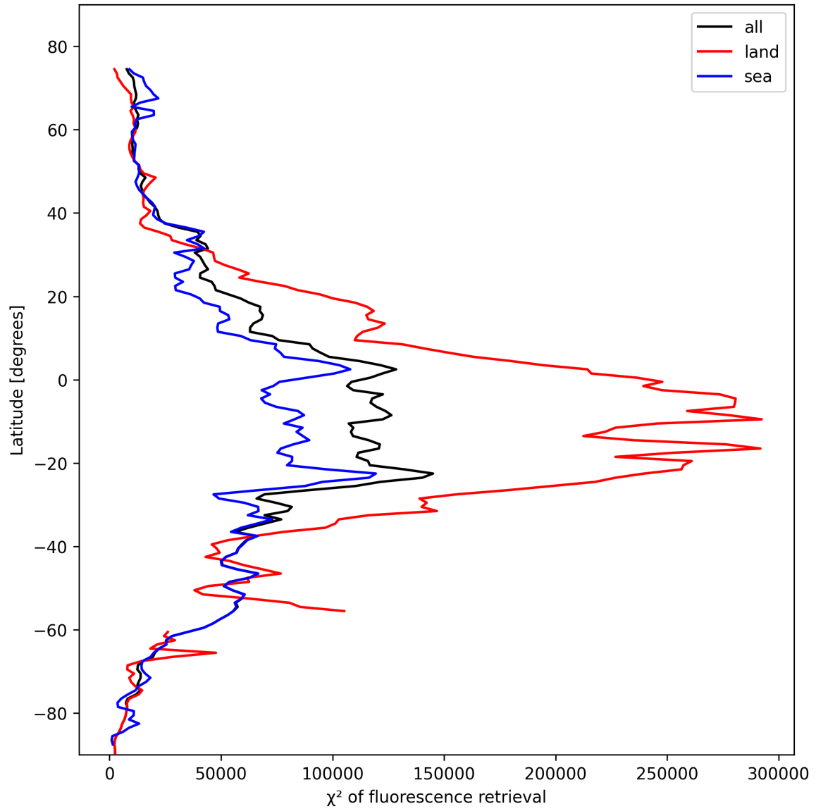
Figure 25: Zonal average of “ \chi^2 of fluorescence retrieval” for 2025-02-11 to 2025-02-13.
