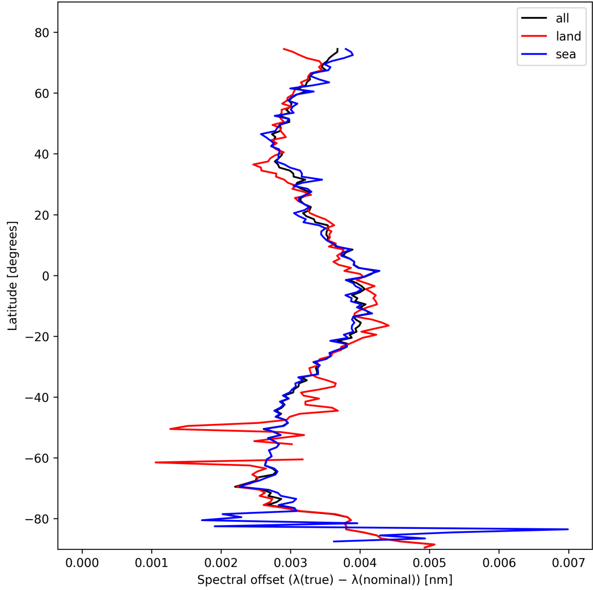
Figure 28: Zonal average of “Spectral offset ( \lambda_{\text{true}} - \lambda_{\text{nominal}} )” for 2025-02-11 to 2025-02-13.
