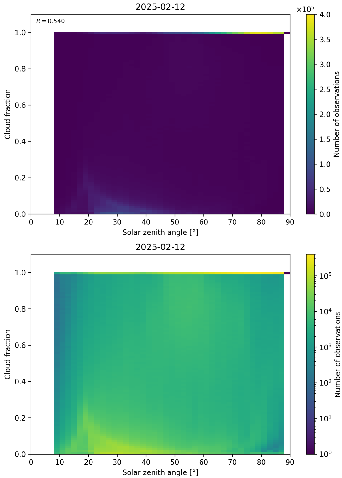
Figure 110: Scatter density plot of “Solar zenith angle” against “Cloud fraction” for 2025-02-11 to 2025-02-13.
