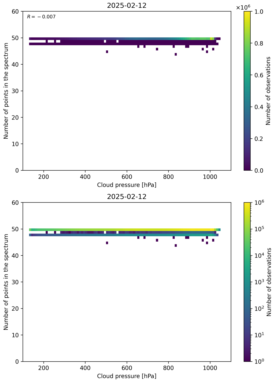
Figure 82: Scatter density plot of “Cloud pressure” against “Number of points in the spectrum” for 2025-02-11 to 2025-02-13.
