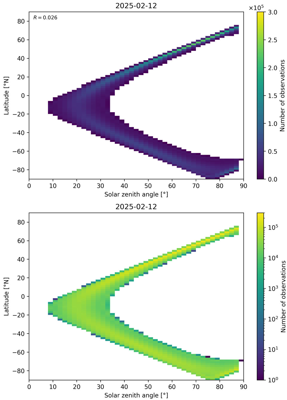
Figure 113: Scatter density plot of “Solar zenith angle” against “Latitude” for 2025-02-11 to 2025-02-13.
