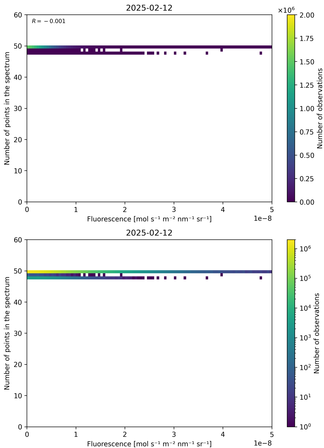
Figure 86: Scatter density plot of “Fluorescence” against “Number of points in the spectrum” for 2025-02-11 to 2025-02-13.
