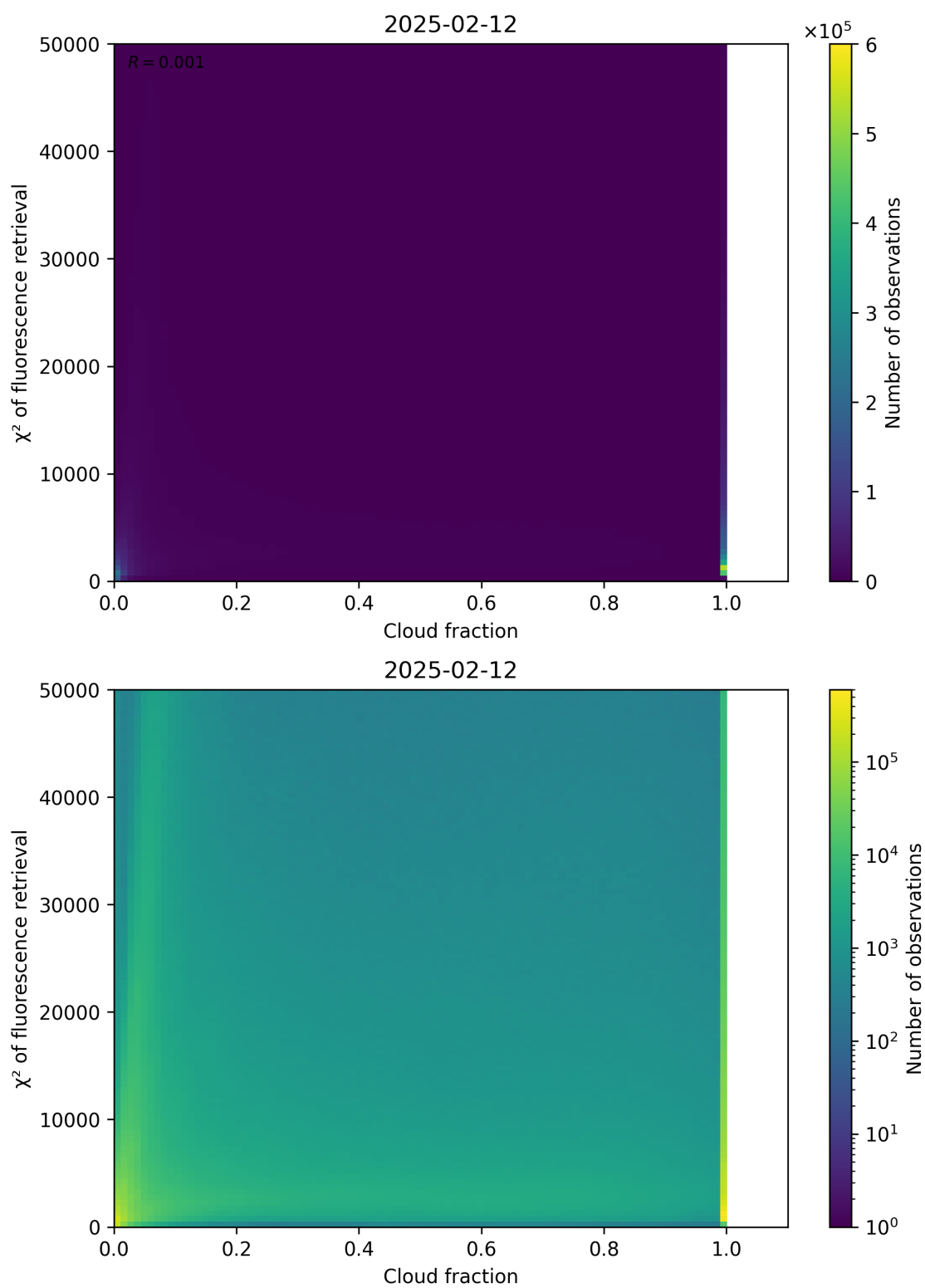
Figure 71: Scatter density plot of “Cloud fraction” against “ \chi^2 of fluorescence retrieval” for 2025-02-11 to 2025-02-13.
