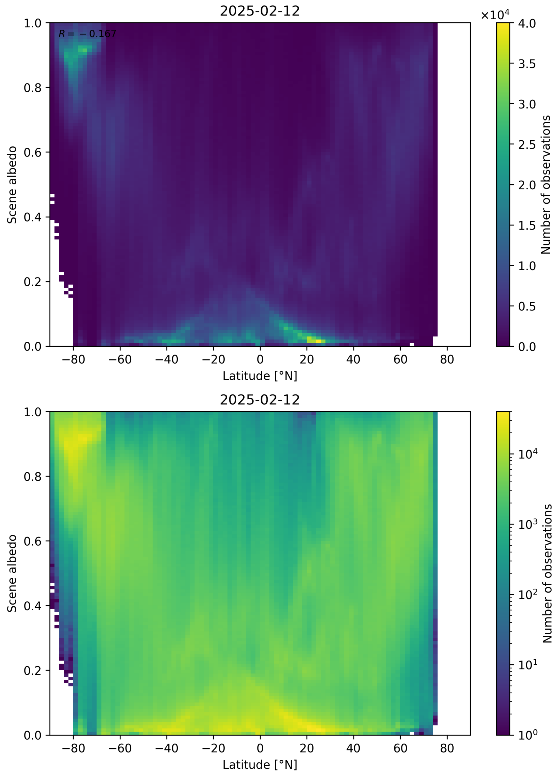
Figure 95: Scatter density plot of “Latitude” against “Scene albedo” for 2025-02-11 to 2025-02-13.
