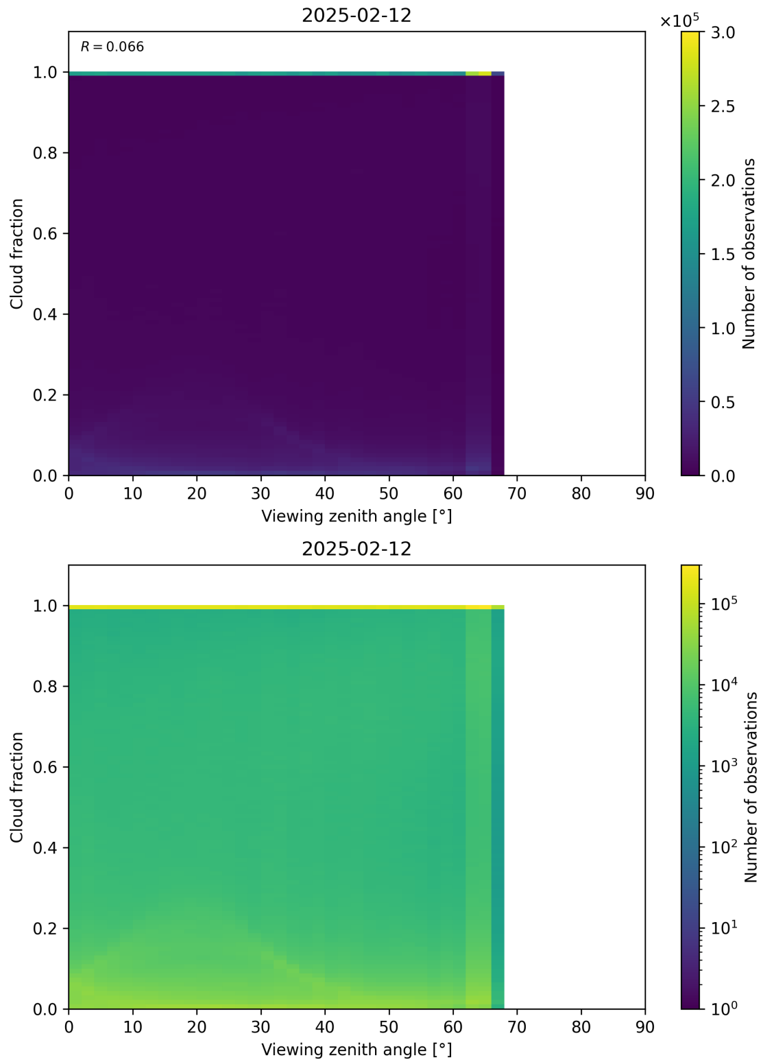
Figure 120: Scatter density plot of “Viewing zenith angle” against “Cloud fraction” for 2025-02-11 to 2025-02-13.
