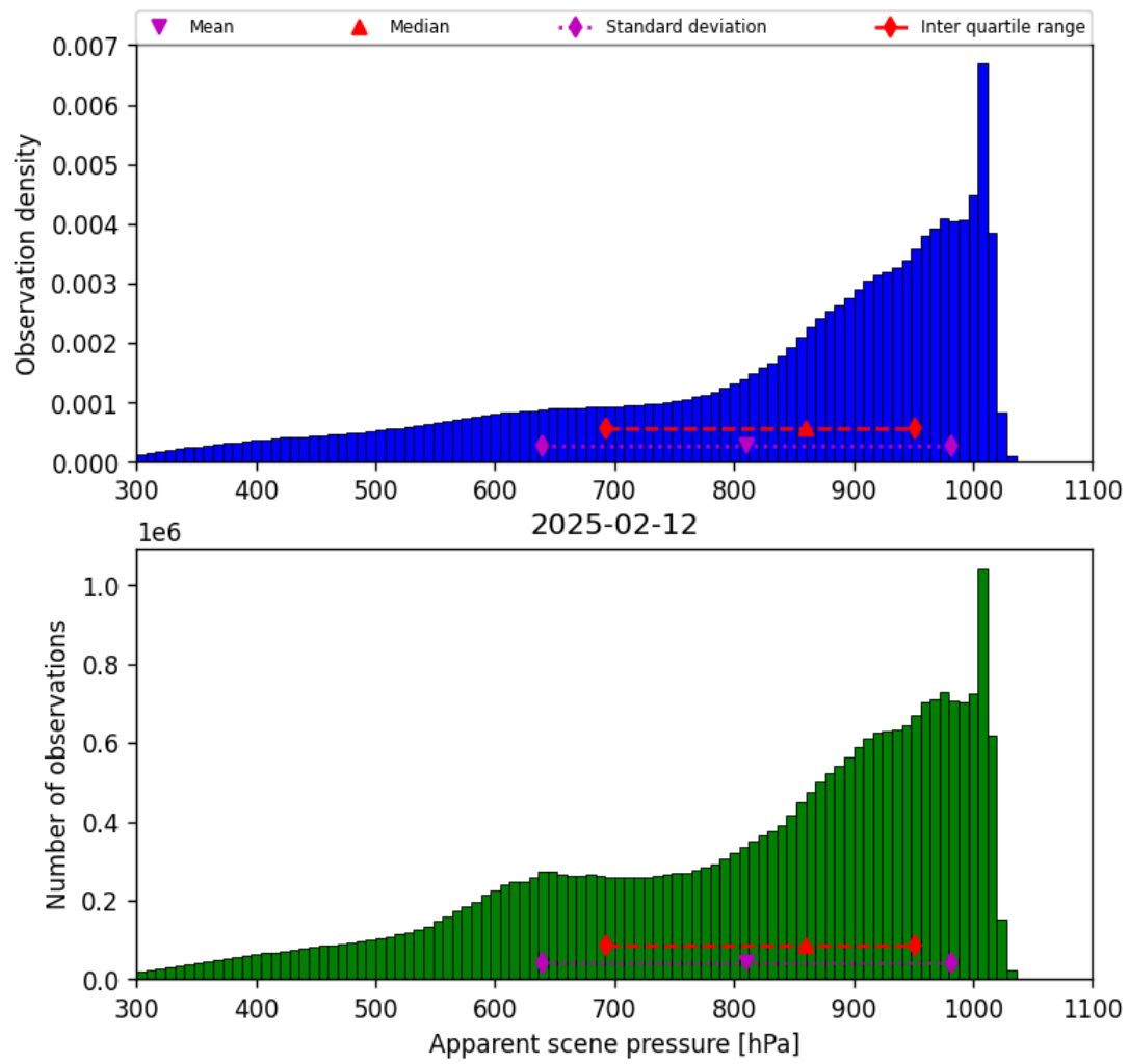
Figure 36: Histogram of “Apparent scene pressure” for 2025-02-11 to 2025-02-13
