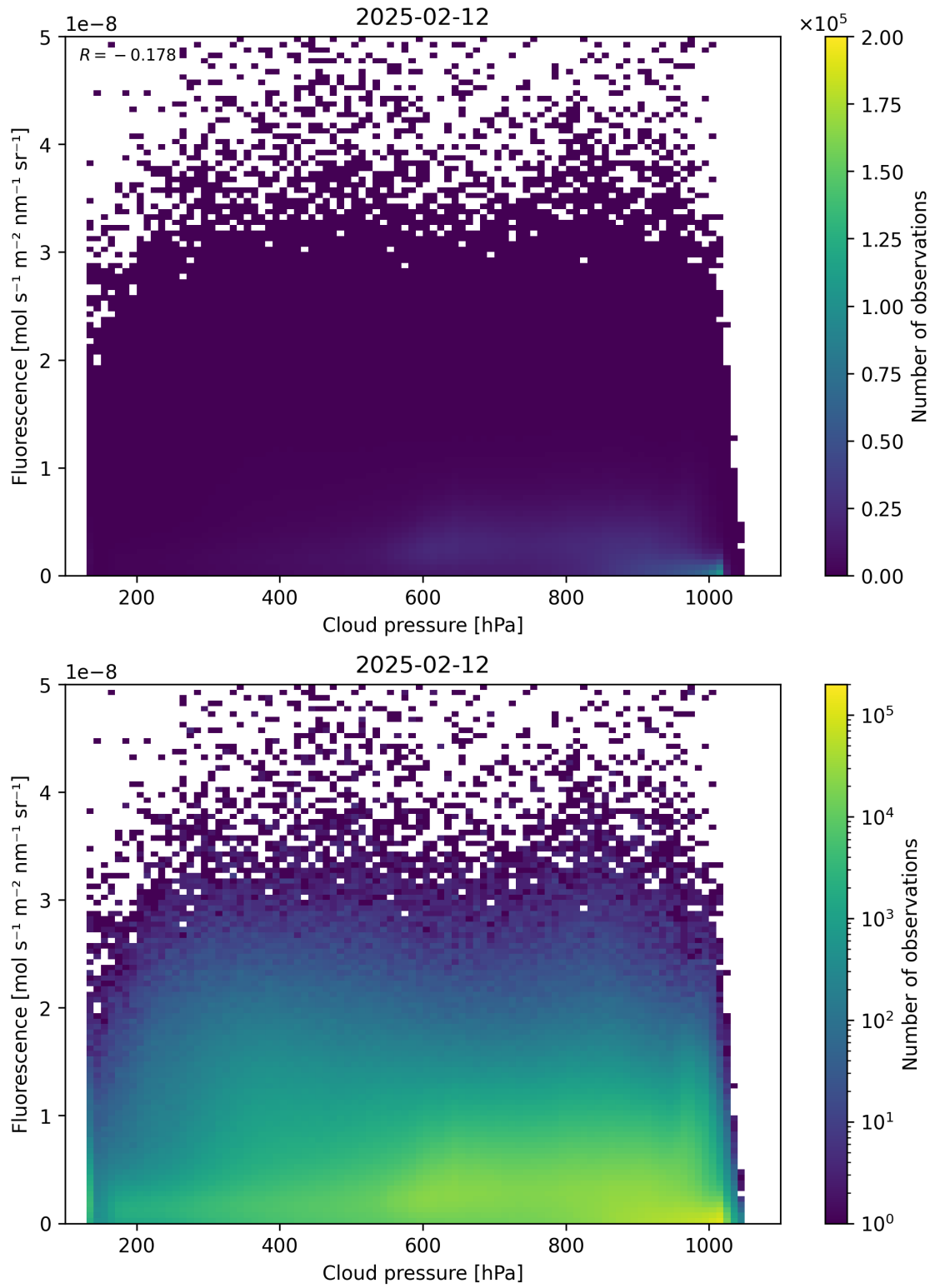
Figure 80: Scatter density plot of “Cloud pressure” against “Fluorescence” for 2025-02-11 to 2025-02-13.
