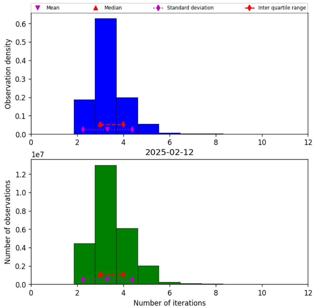
Figure 39: Histogram of “Number of iterations” for 2025-02-11 to 2025-02-13
