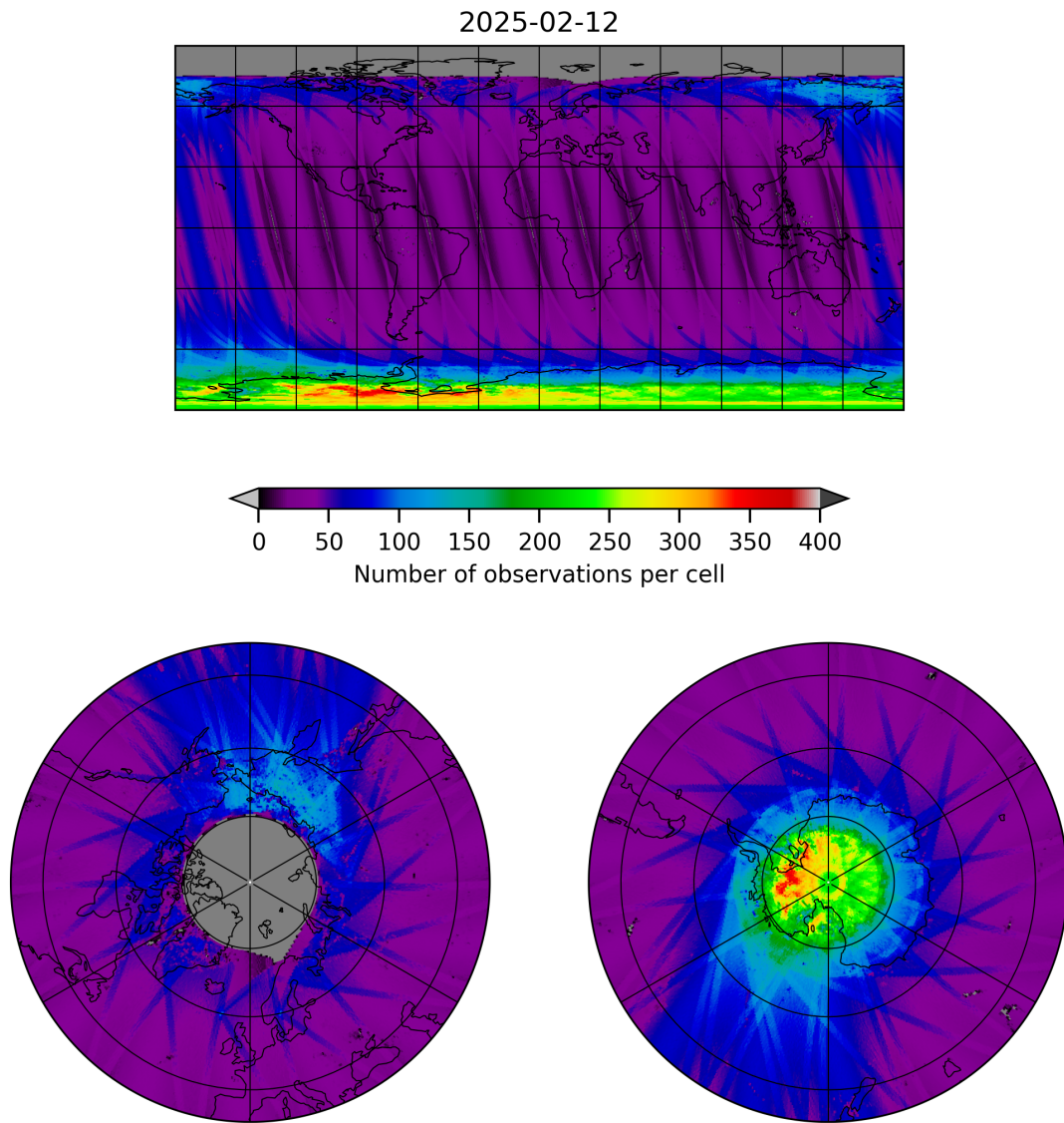
Figure 11: Map of the number of observations for 2025-02-11 to 2025-02-13
