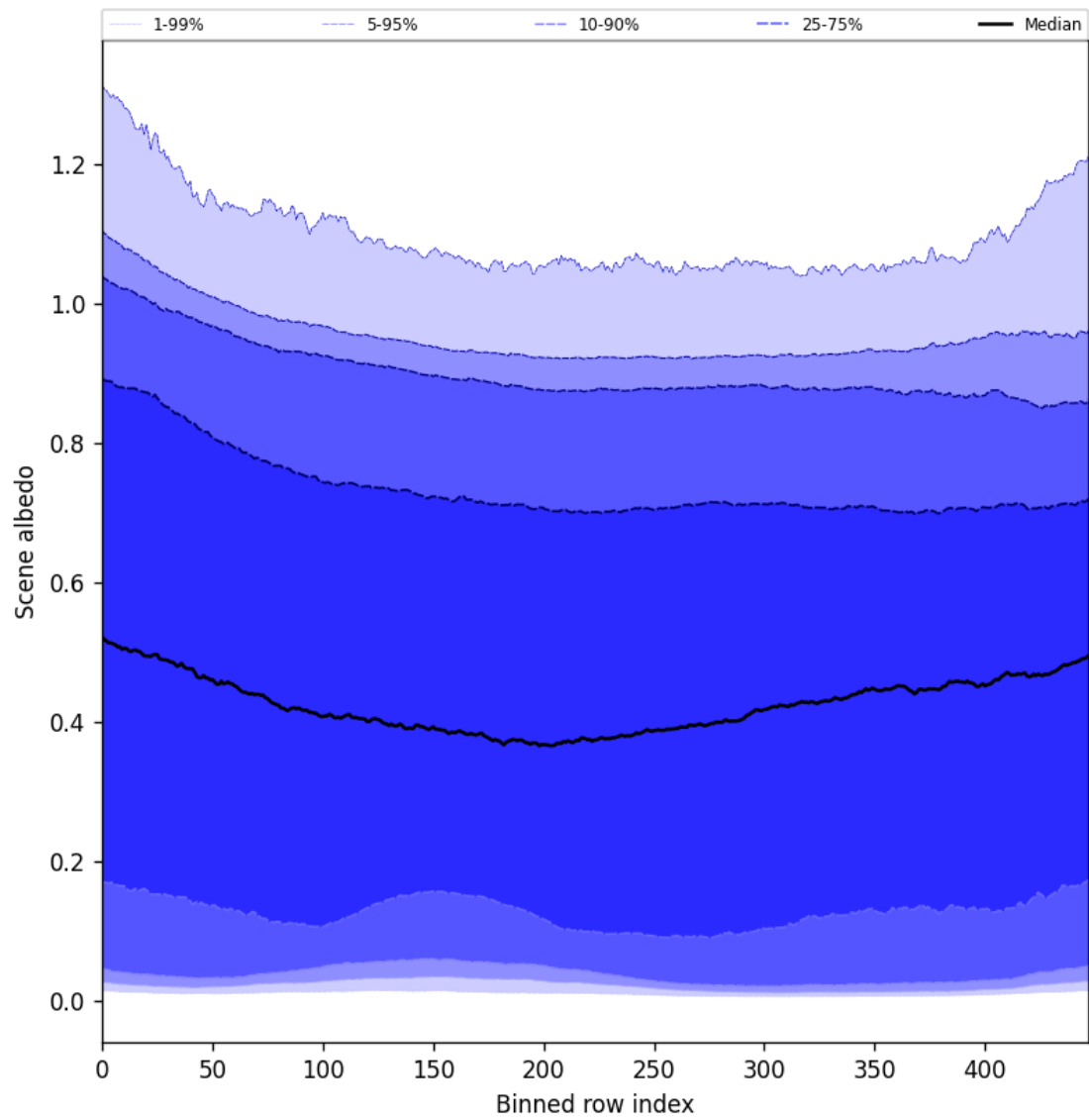
Figure 51: Along track statistics of “Scene albedo” for 2025-02-11 to 2025-02-13
