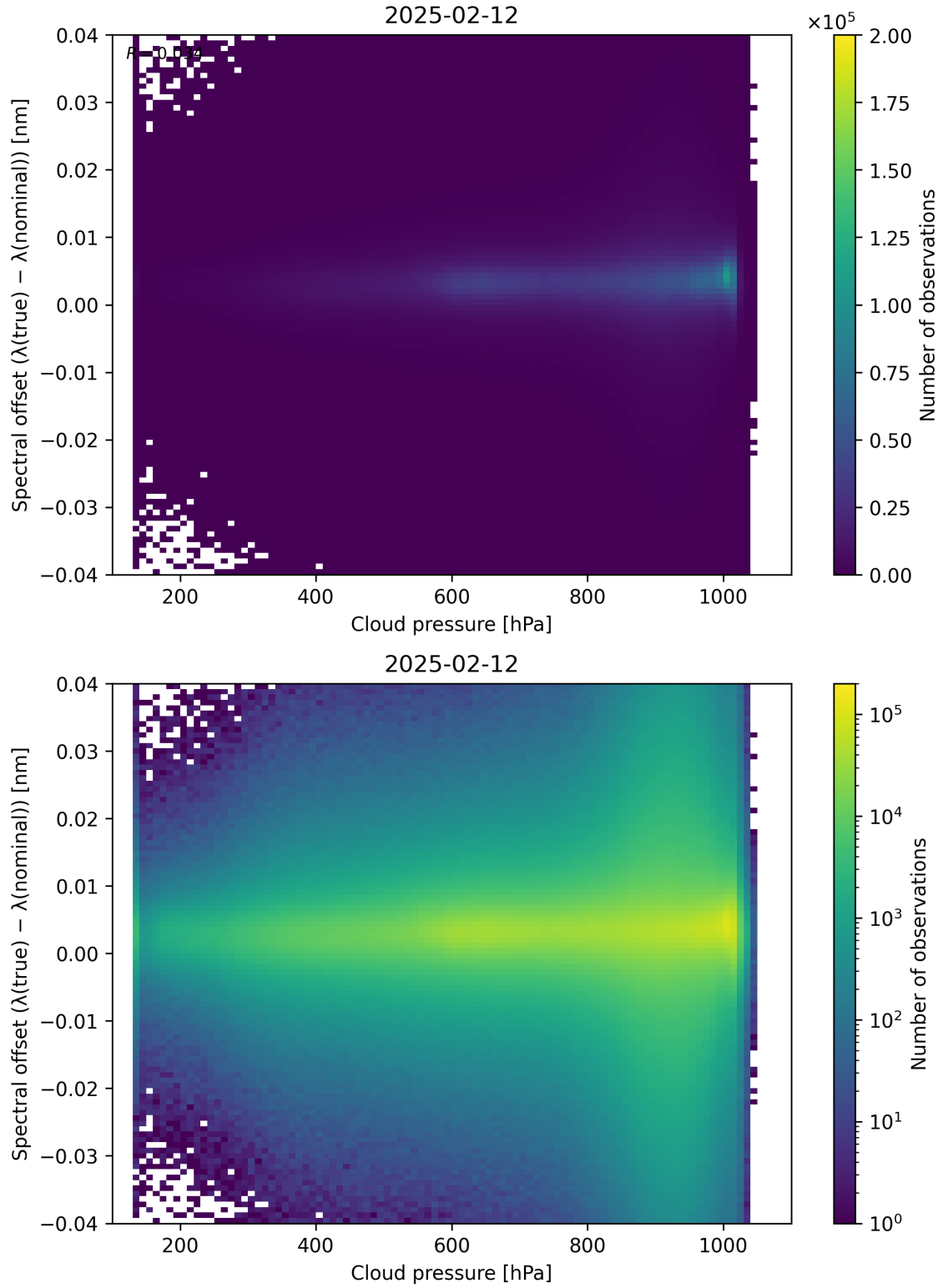
Figure 84: Scatter density plot of “Cloud pressure” against “Spectral offset ( \lambda_{\text{true}} - \lambda_{\text{nominal}} )” for 2025-02-11 to 2025-02-13.
