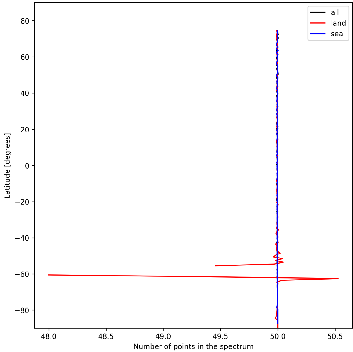
Figure 27: Zonal average of “Number of points in the spectrum” for 2025-02-11 to 2025-02-13.
