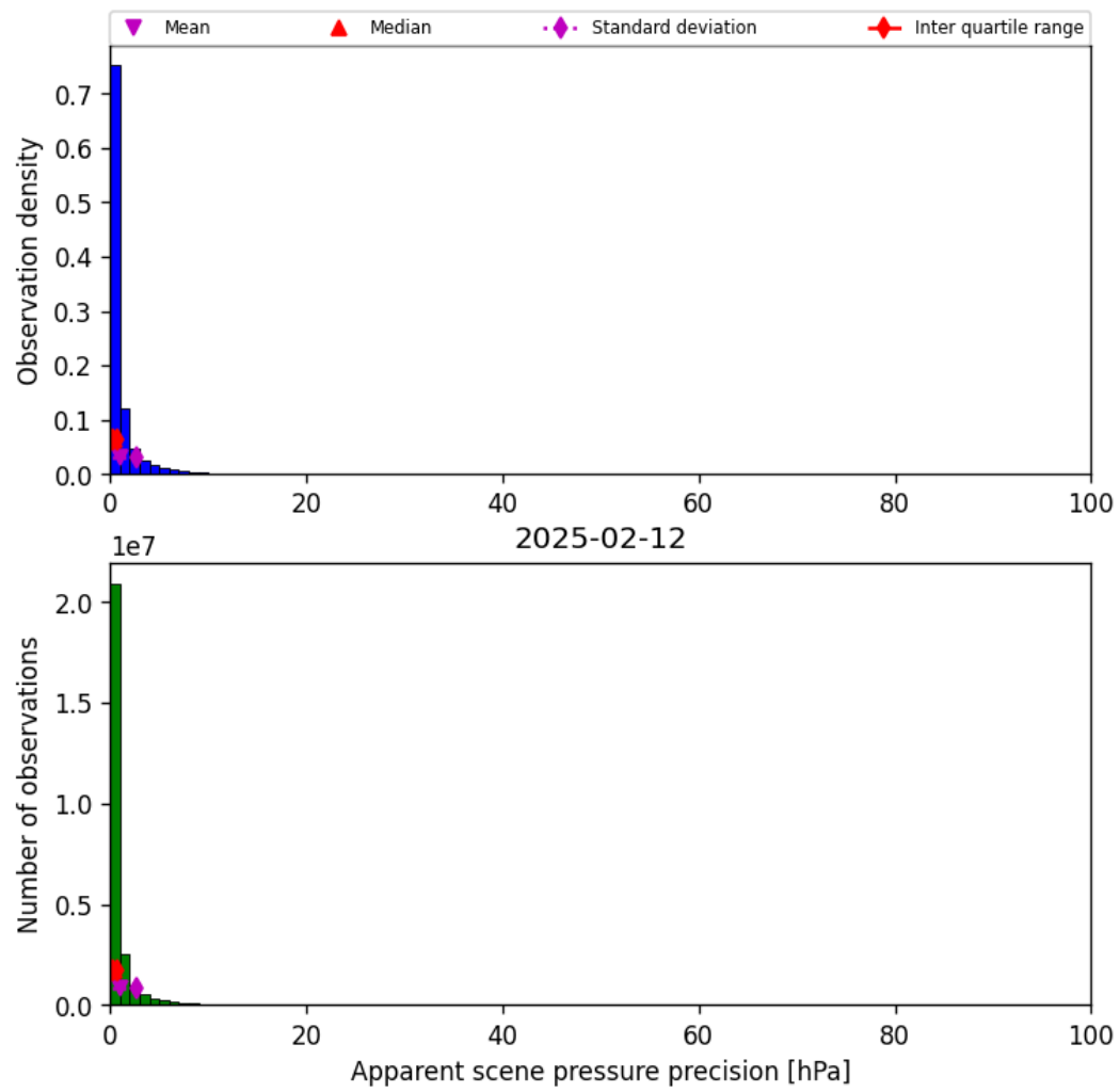
Figure 37: Histogram of “Apparent scene pressure precision” for 2025-02-11 to 2025-02-13
