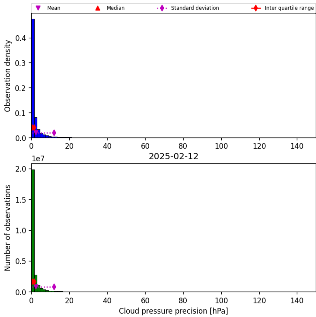
Figure 31: Histogram of “Cloud pressure precision” for 2025-02-11 to 2025-02-13
