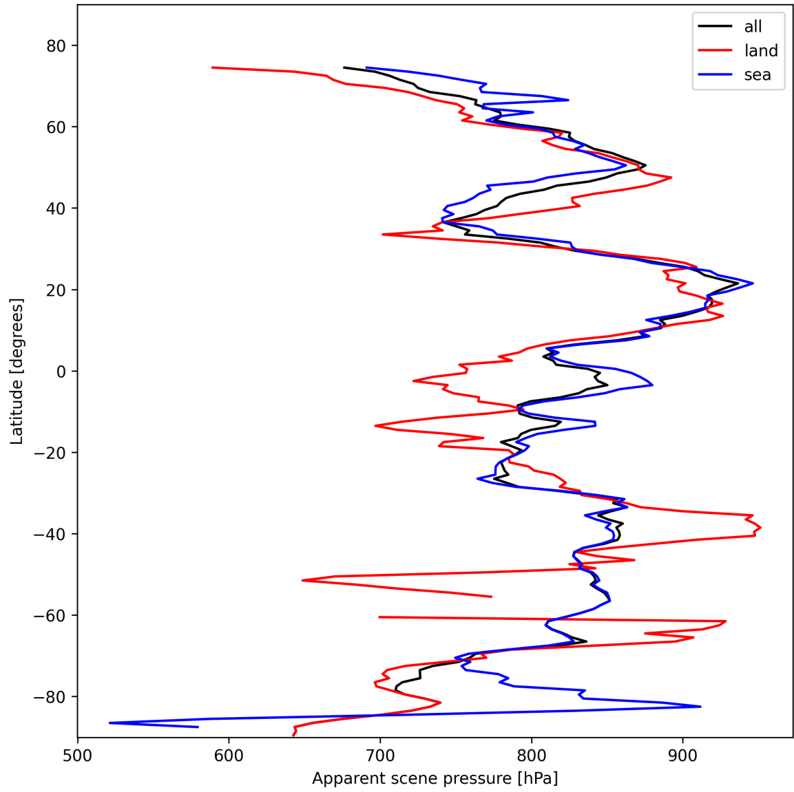
Figure 19: Zonal average of “Apparent scene pressure” for 2025-02-11 to 2025-02-13.
