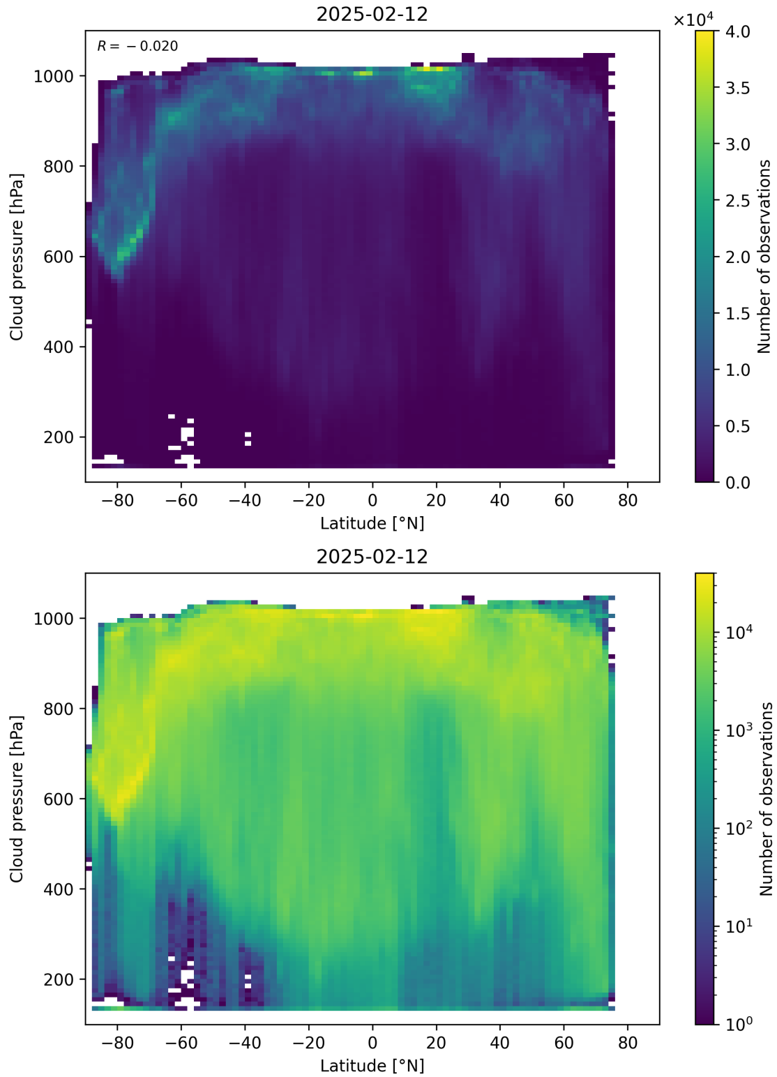
Figure 91: Scatter density plot of “Latitude” against “Cloud pressure” for 2025-02-11 to 2025-02-13.
