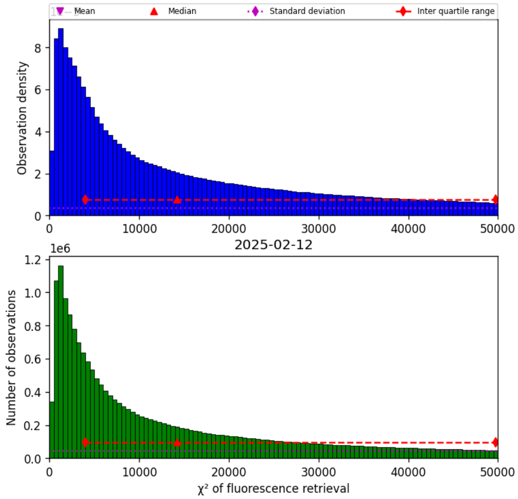
Figure 42: Histogram of “ \chi^2 of fluorescence retrieval” for 2025-02-11 to 2025-02-13
