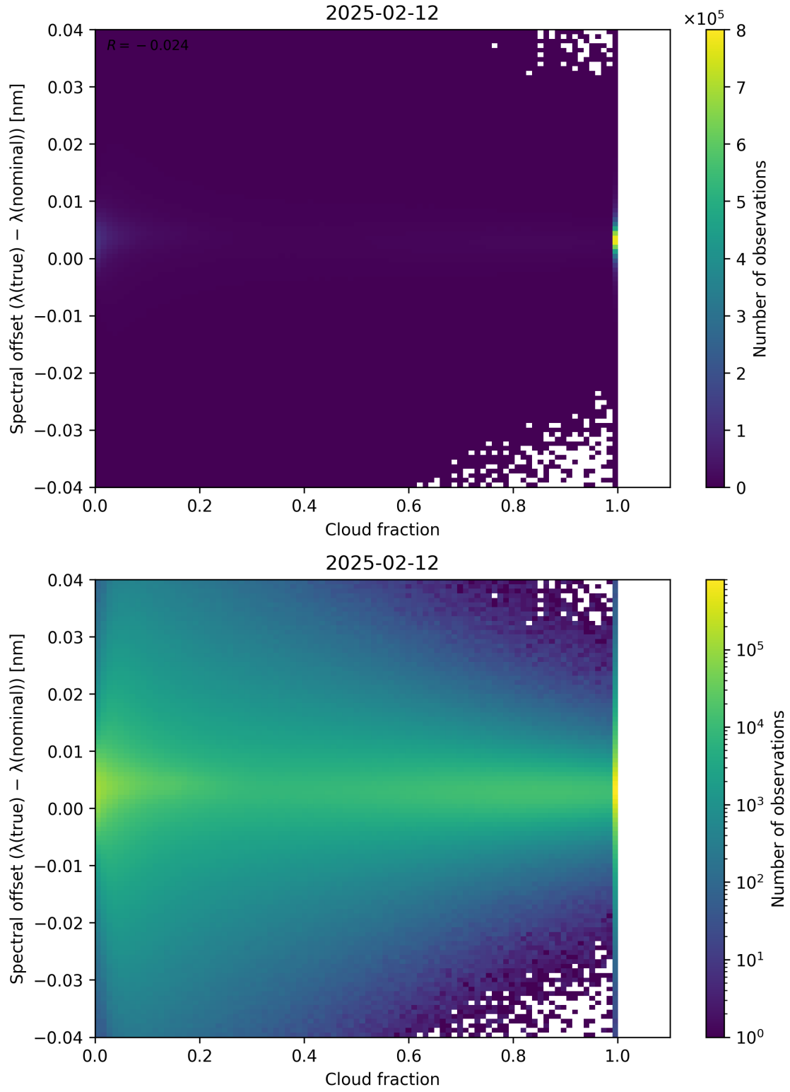
Figure 76: Scatter density plot of “Cloud fraction” against “Spectral offset ( \lambda_{\text{true}} - \lambda_{\text{nominal}} )” for 2025-02-11 to 2025-02-13.
