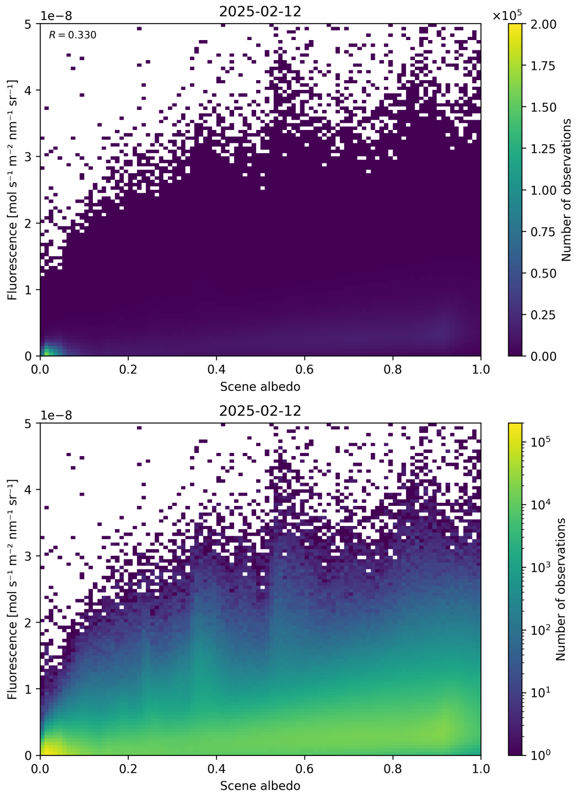
Figure 104: Scatter density plot of “Scene albedo” against “Fluorescence” for 2025-02-11 to 2025-02-13.
