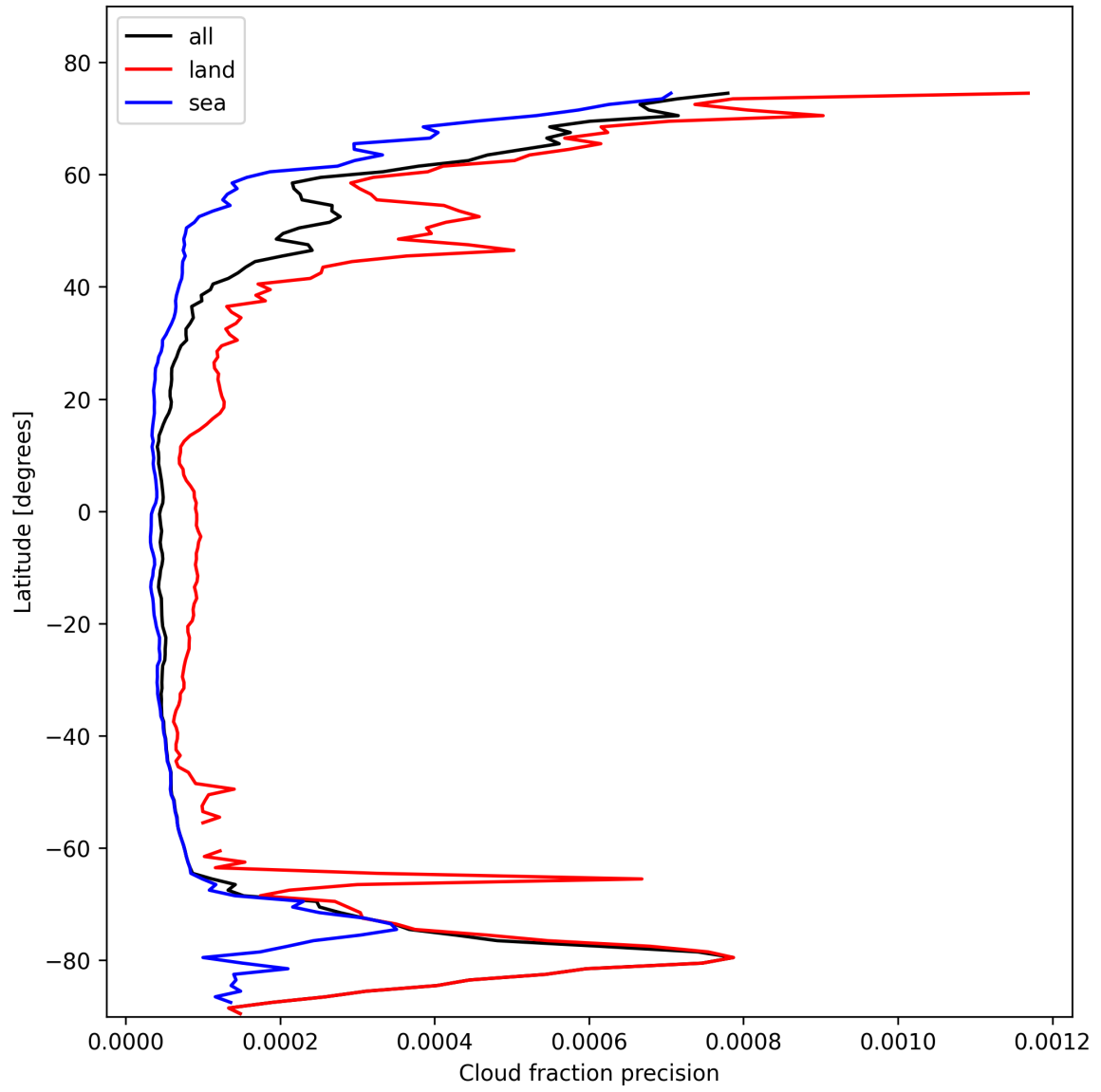
Figure 16: Zonal average of “Cloud fraction precision” for 2025-02-11 to 2025-02-13.
