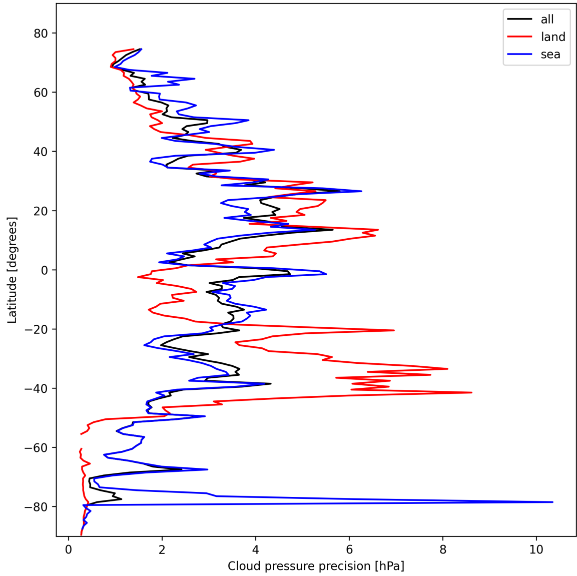
Figure 14: Zonal average of “Cloud pressure precision” for 2025-02-11 to 2025-02-13.
