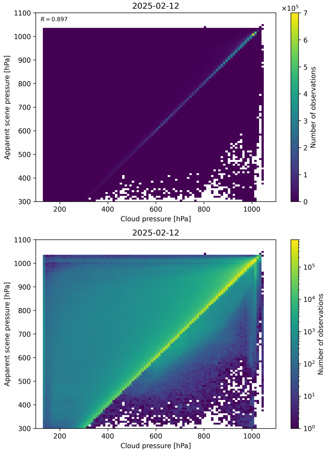
Figure 77: Scatter density plot of “Cloud pressure” against “Apparent scene pressure” for 2025-02-11 to 2025-02-13.
