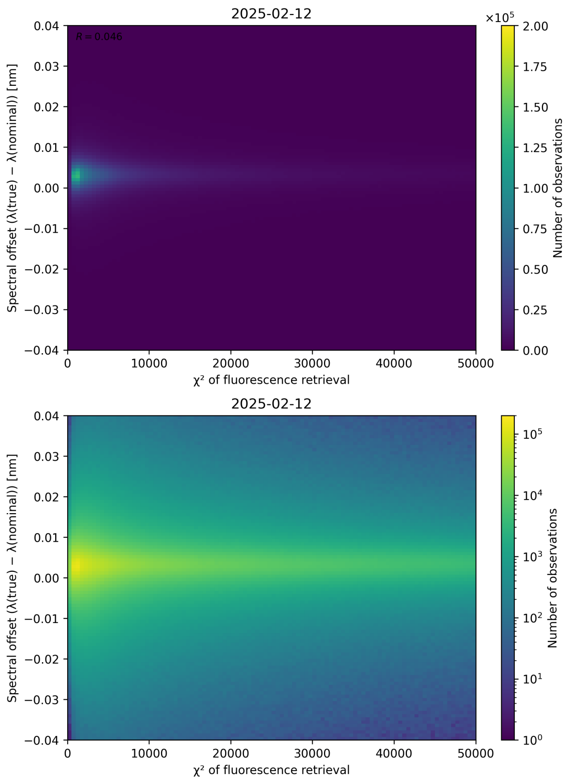
Figure 69: Scatter density plot of “ \chi^2 of fluorescence retrieval” against “Spectral offset ( \lambda_{\text{true}} - \lambda_{\text{nominal}} )” for 2025-02-11 to 2025-02-13.
