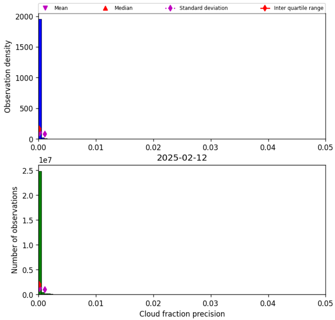
Figure 33: Histogram of “Cloud fraction precision” for 2025-02-11 to 2025-02-13
