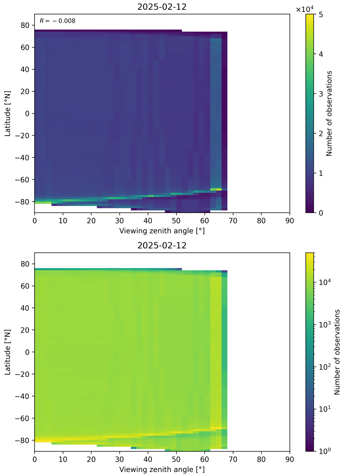
Figure 123: Scatter density plot of “Viewing zenith angle” against “Latitude” for 2025-02-11 to 2025-02-13.
