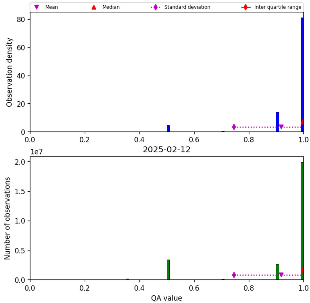
Figure 29: Histogram of “QA value” for 2025-02-11 to 2025-02-13
