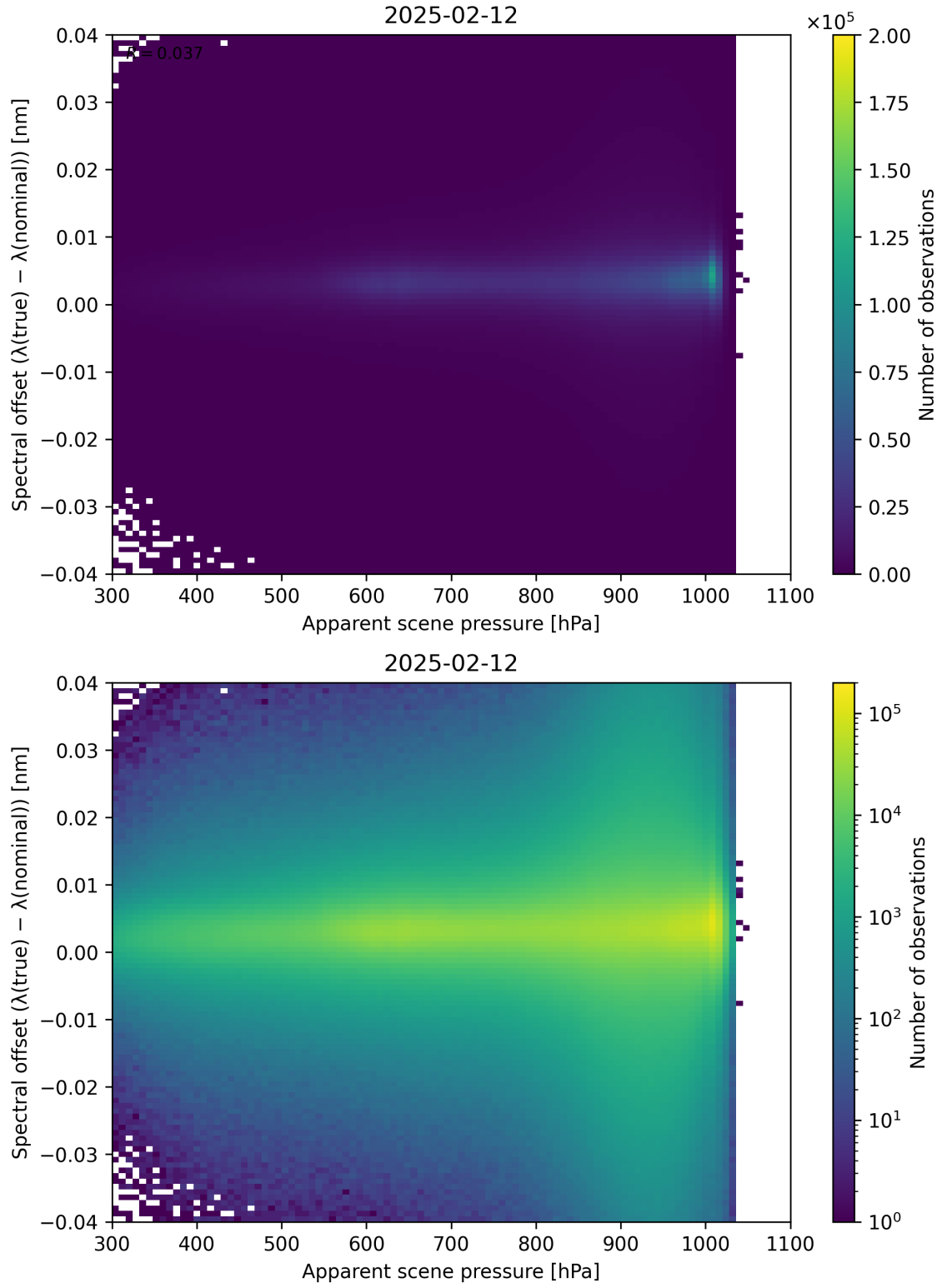
Figure 67: Scatter density plot of “Apparent scene pressure” against “Spectral offset ( \lambda_{\text{true}} - \lambda_{\text{nominal}} )” for 2025-02-11 to 2025-02-13.
