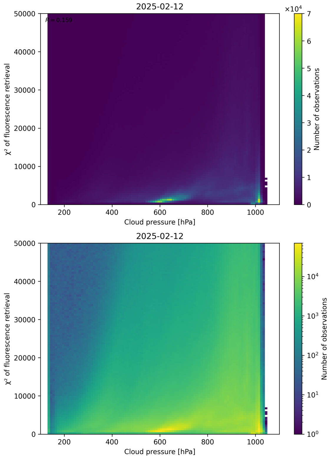
Figure 78: Scatter density plot of “Cloud pressure” against “ \chi^2 of fluorescence retrieval” for 2025-02-11 to 2025-02-13.
