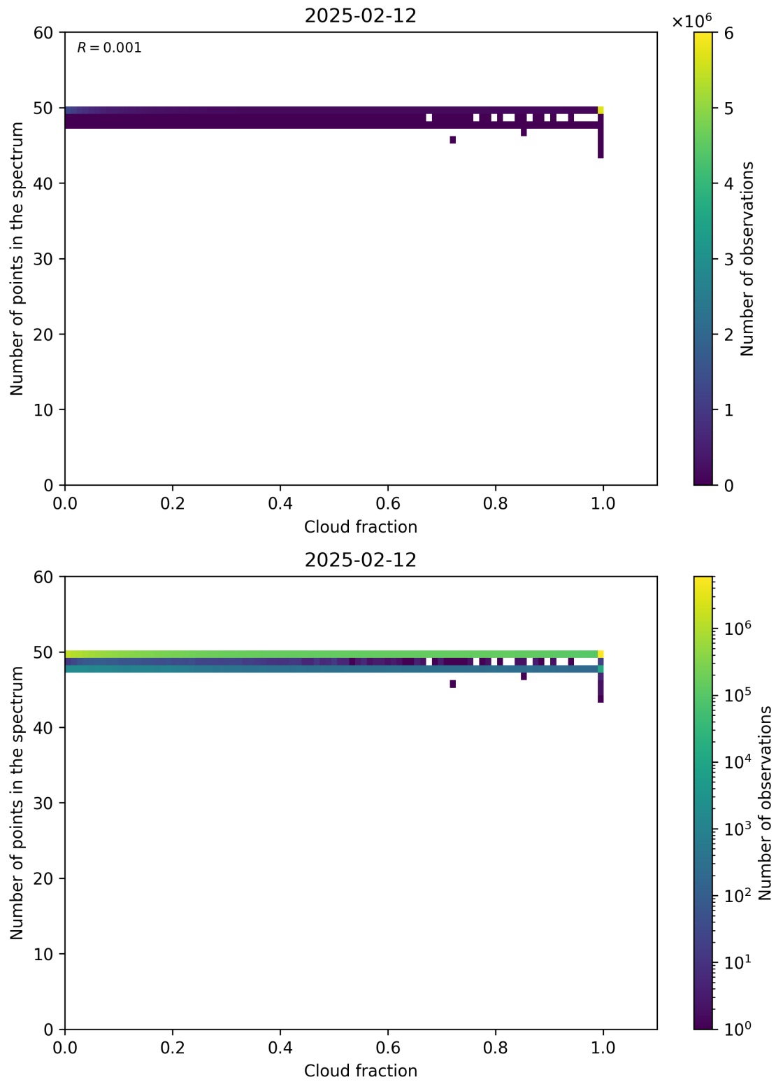
Figure 74: Scatter density plot of “Cloud fraction” against “Number of points in the spectrum” for 2025-02-11 to 2025-02-13.
