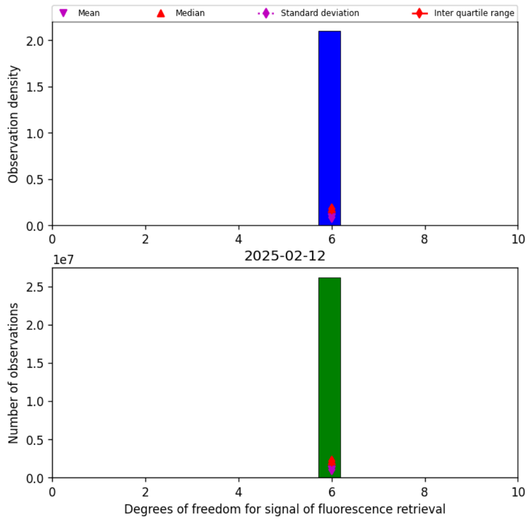
Figure 43: Histogram of “Degrees of freedom for signal of fluorescence retrieval” for 2025-02-11 to 2025-02-13
