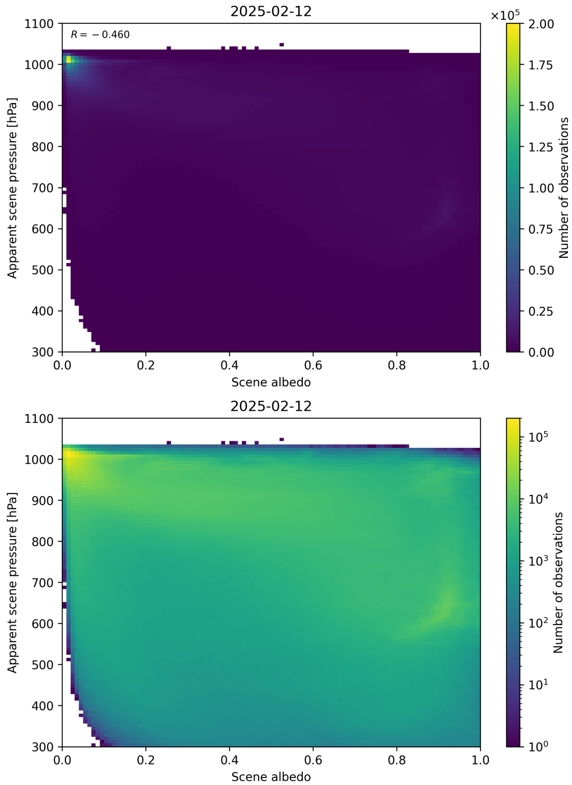
Figure 102: Scatter density plot of “Scene albedo” against “Apparent scene pressure” for 2025-02-11 to 2025-02-13.
