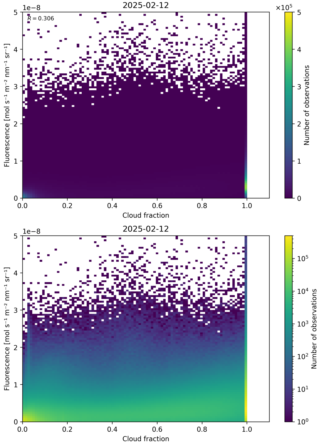
Figure 72: Scatter density plot of “Cloud fraction” against “Fluorescence” for 2025-02-11 to 2025-02-13.
