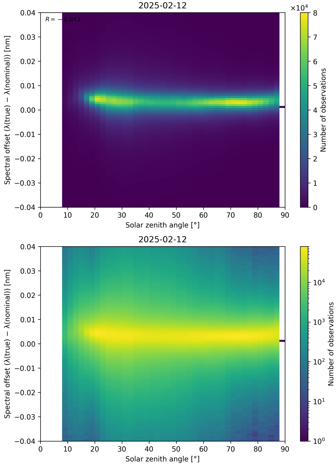
Figure 117: Scatter density plot of “Solar zenith angle” against “Spectral offset ( \lambda_{\text{true}} - \lambda_{\text{nominal}} )” for 2025-02-11 to 2025-02-13.
