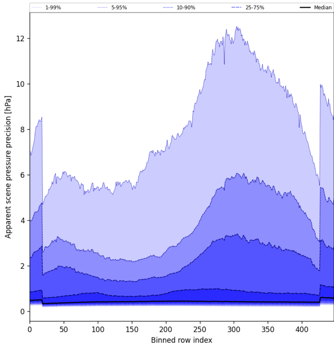
Figure 54: Along track statistics of “Apparent scene pressure precision” for 2025-02-11 to 2025-02-13
