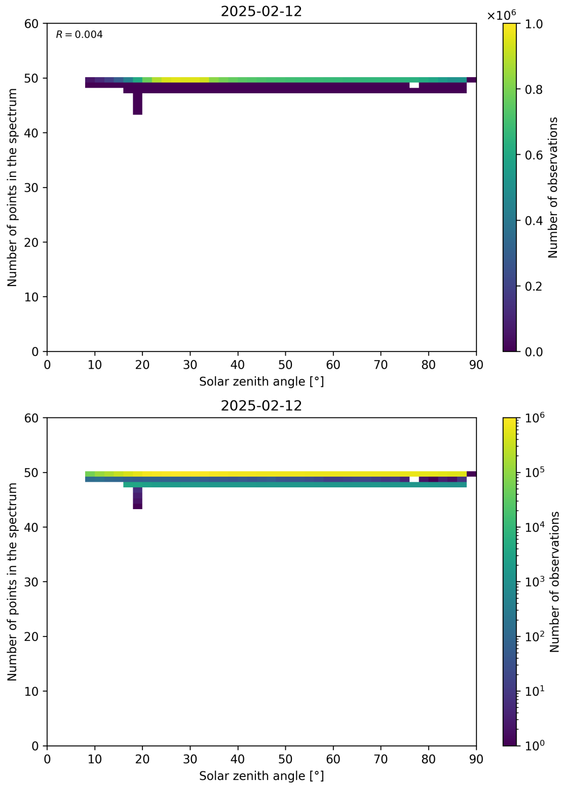
Figure 115: Scatter density plot of “Solar zenith angle” against “Number of points in the spectrum” for 2025-02-11 to 2025-02-13.
