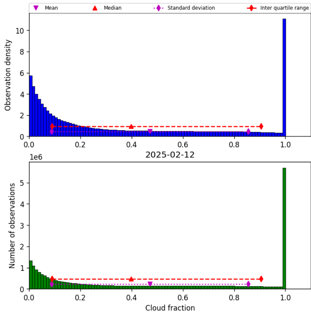
Figure 32: Histogram of “Cloud fraction” for 2025-02-11 to 2025-02-13
