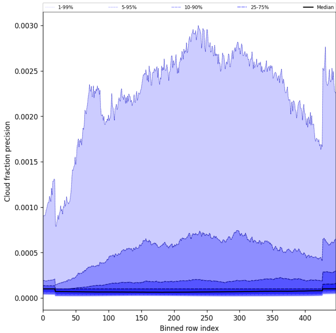
Figure 50: Along track statistics of “Cloud fraction precision” for 2025-02-11 to 2025-02-13
