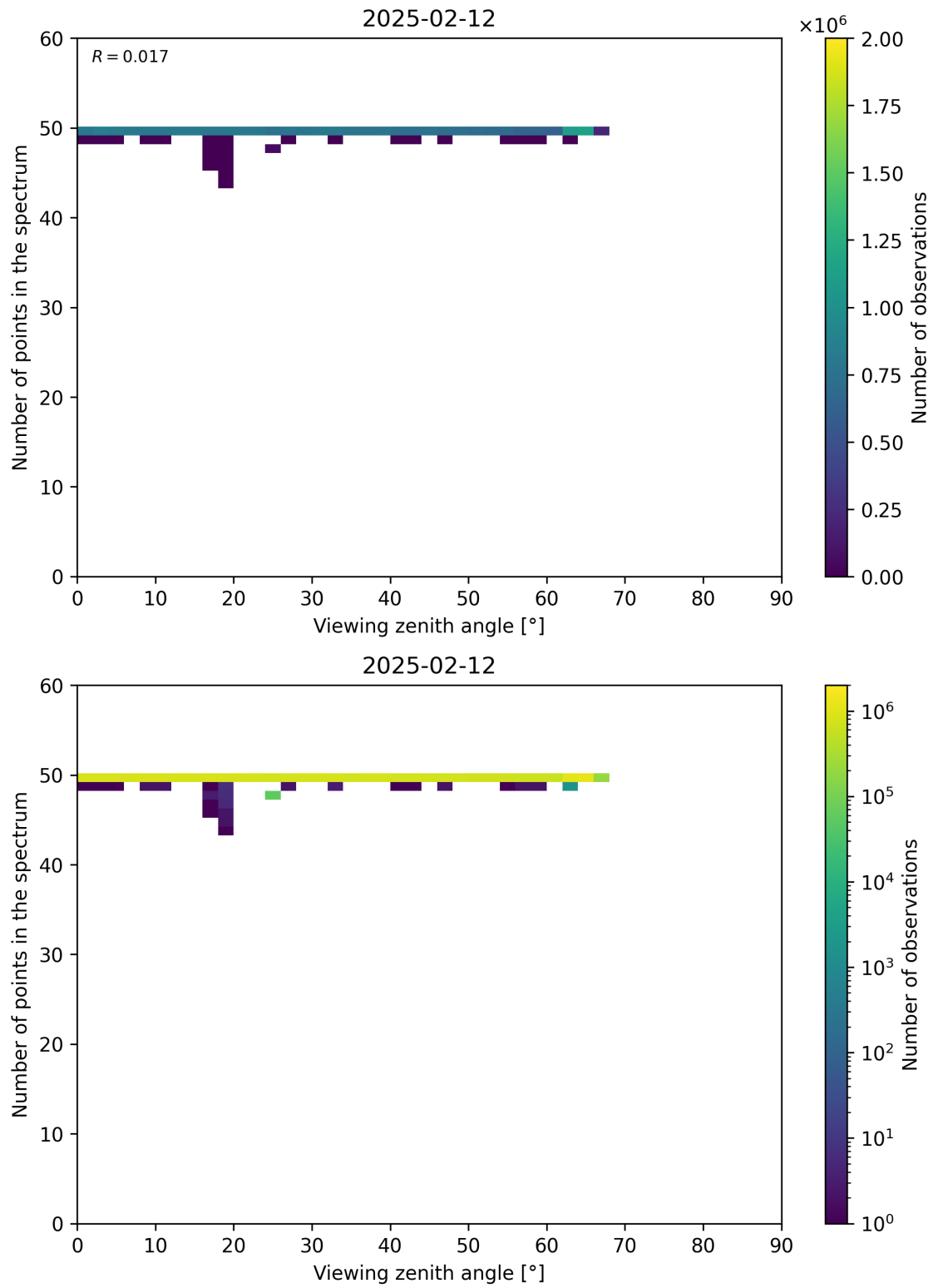
Figure 125: Scatter density plot of “Viewing zenith angle” against “Number of points in the spectrum” for 2025-02-11 to 2025-02-13.
