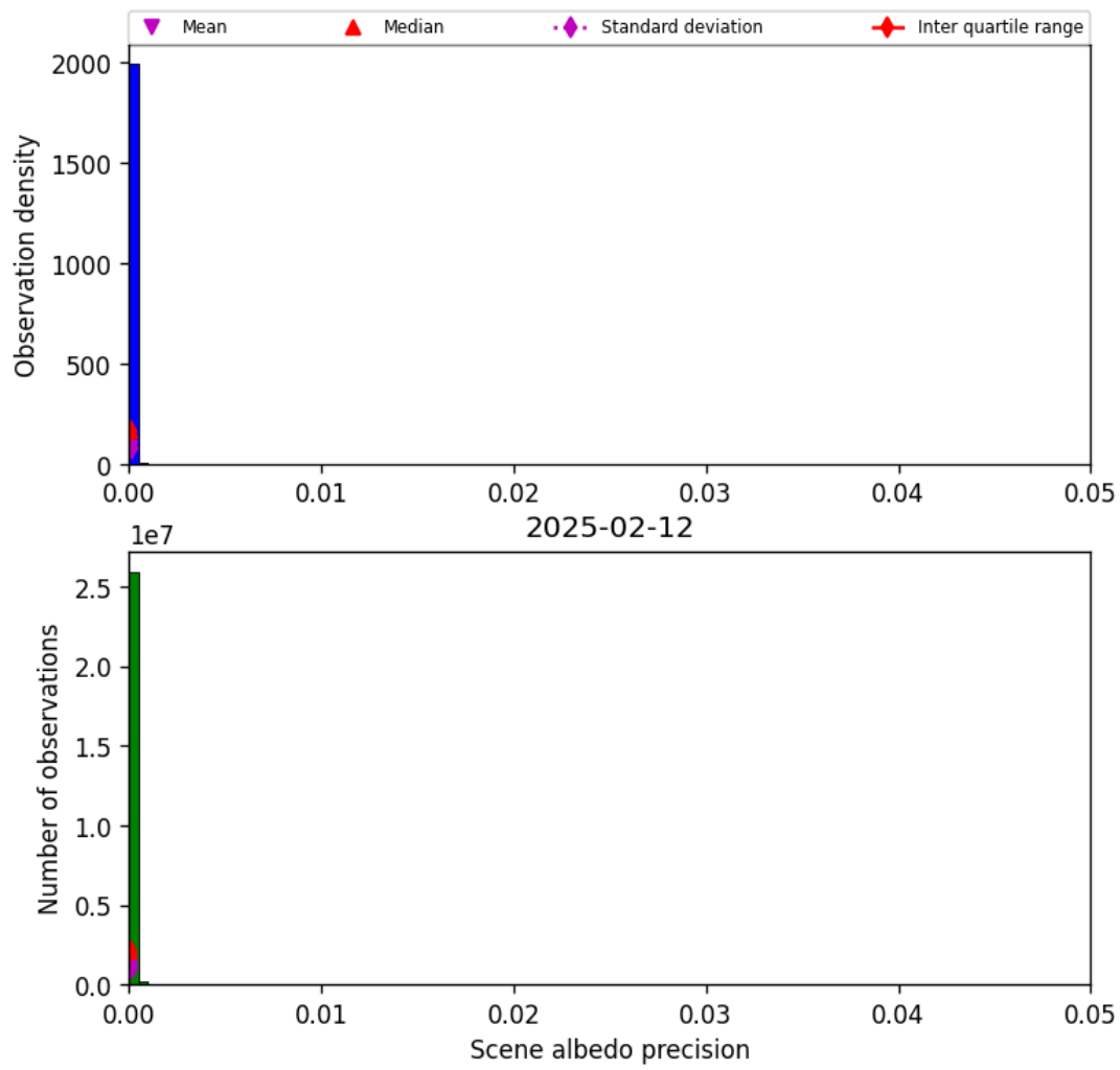
Figure 35: Histogram of “Scene albedo precision” for 2025-02-11 to 2025-02-13
