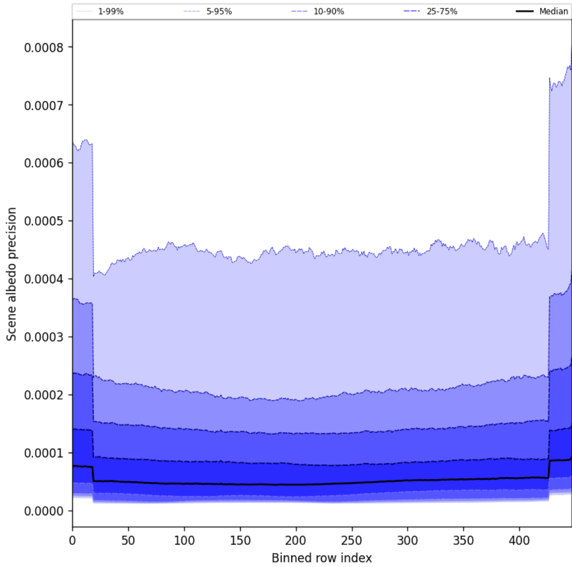
Figure 52: Along track statistics of “Scene albedo precision” for 2025-02-11 to 2025-02-13
