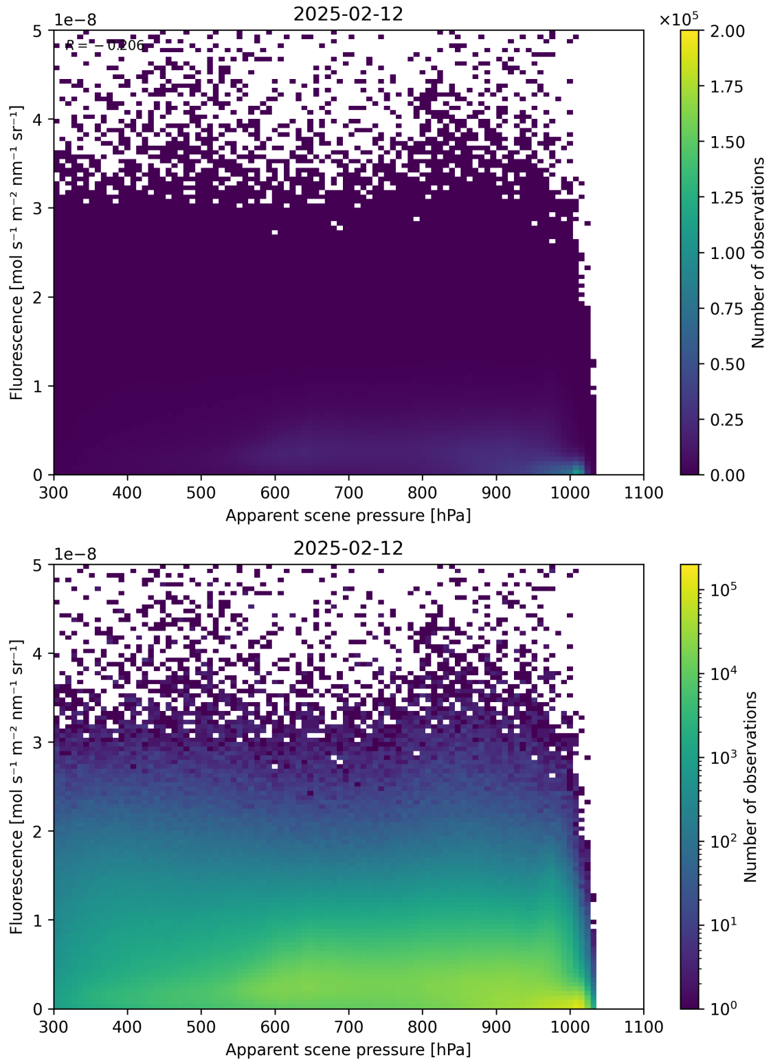
Figure 64: Scatter density plot of “Apparent scene pressure” against “Fluorescence” for 2025-02-11 to 2025-02-13.
