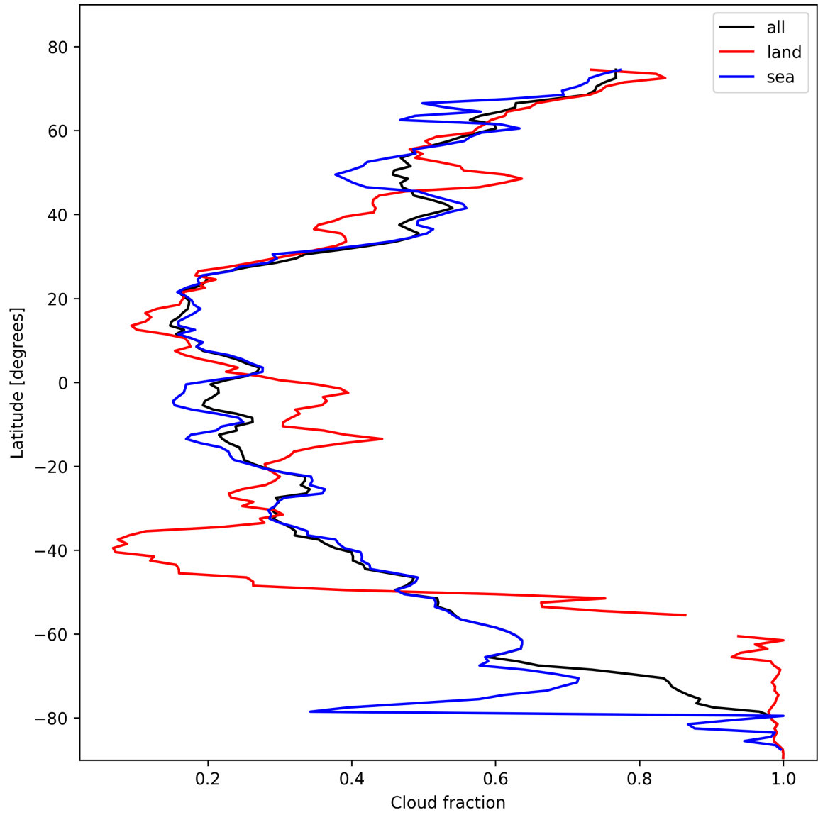
Figure 15: Zonal average of “Cloud fraction” for 2025-02-11 to 2025-02-13.
