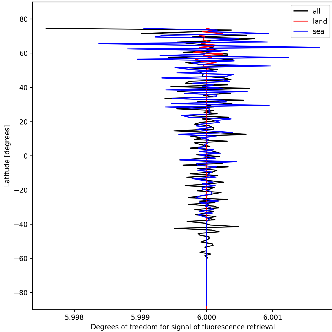
Figure 26: Zonal average of “Degrees of freedom for signal of fluorescence retrieval” for 2025-02-11 to 2025-02-13.
