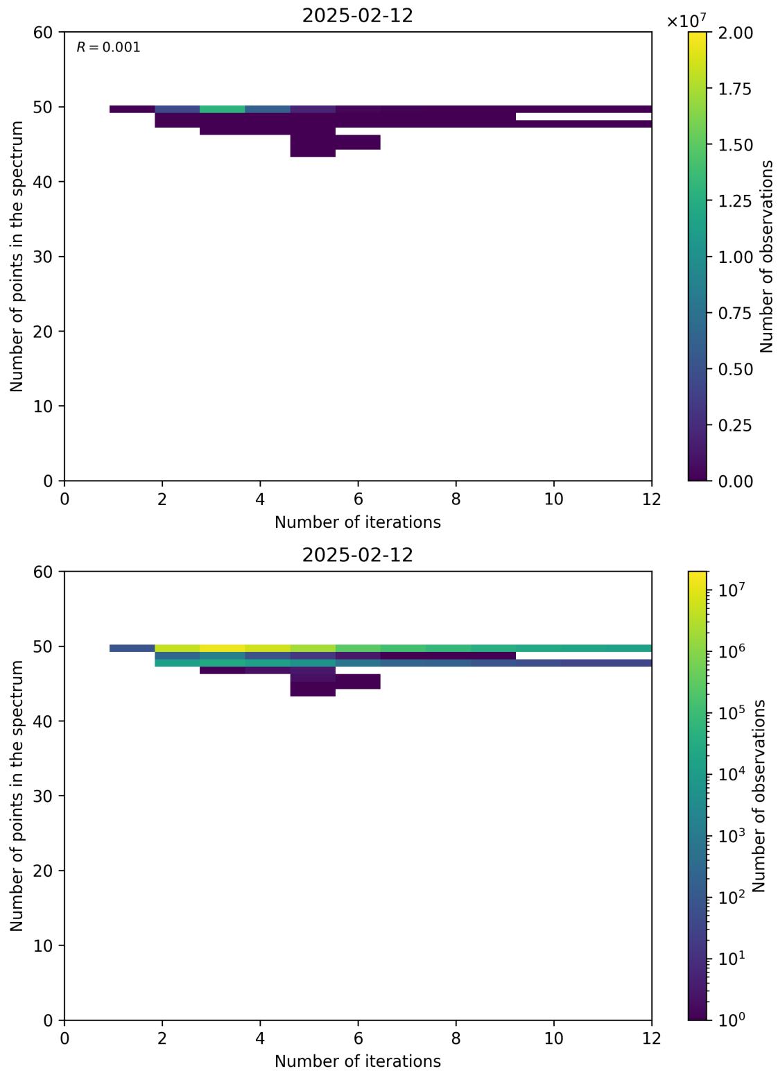
Figure 99: Scatter density plot of “Number of iterations” against “Number of points in the spectrum” for 2025-02-11 to 2025-02-13.
