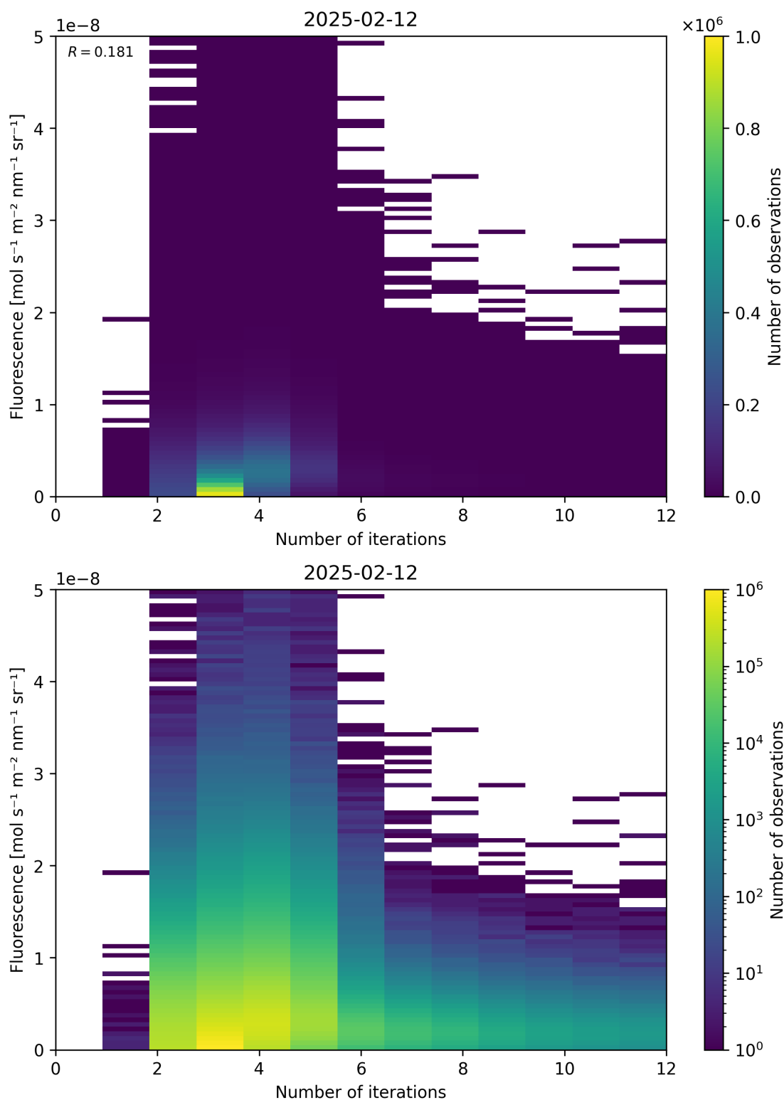
Figure 98: Scatter density plot of “Number of iterations” against “Fluorescence” for 2025-02-11 to 2025-02-13.
