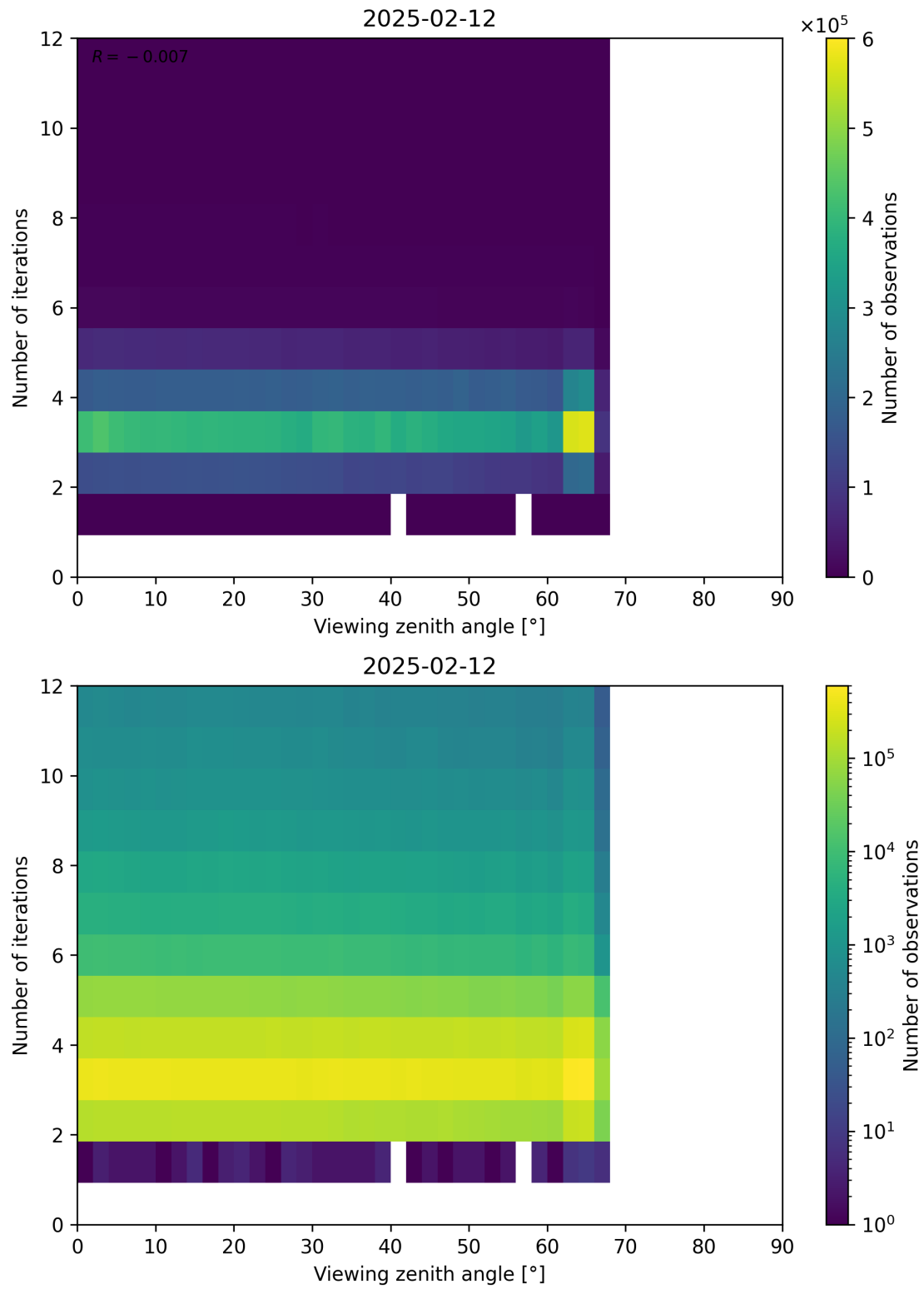
Figure 124: Scatter density plot of “Viewing zenith angle” against “Number of iterations” for 2025-02-11 to 2025-02-13.
