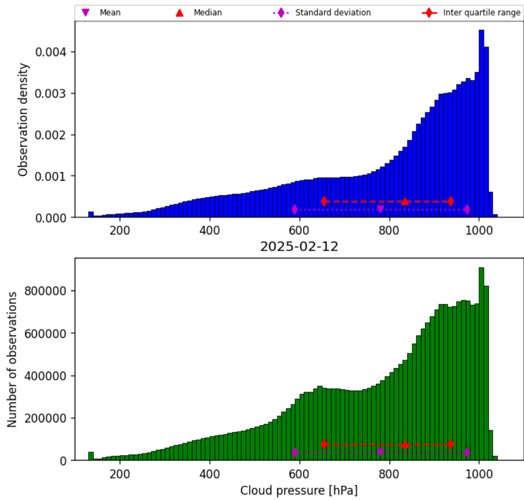
Figure 30: Histogram of “Cloud pressure” for 2025-02-11 to 2025-02-13
