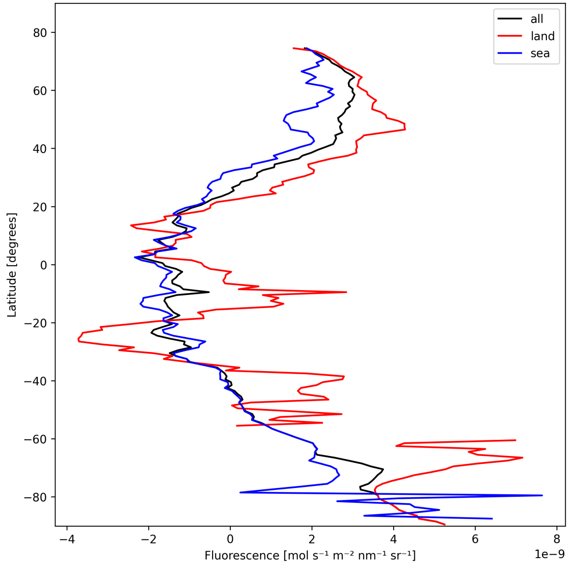
Figure 23: Zonal average of “Fluorescence” for 2025-02-11 to 2025-02-13.
