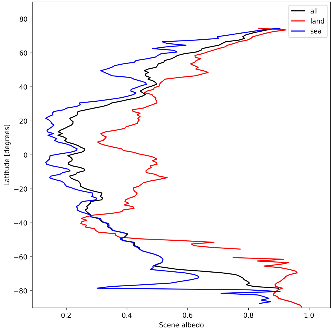
Figure 17: Zonal average of “Scene albedo” for 2025-02-11 to 2025-02-13.
