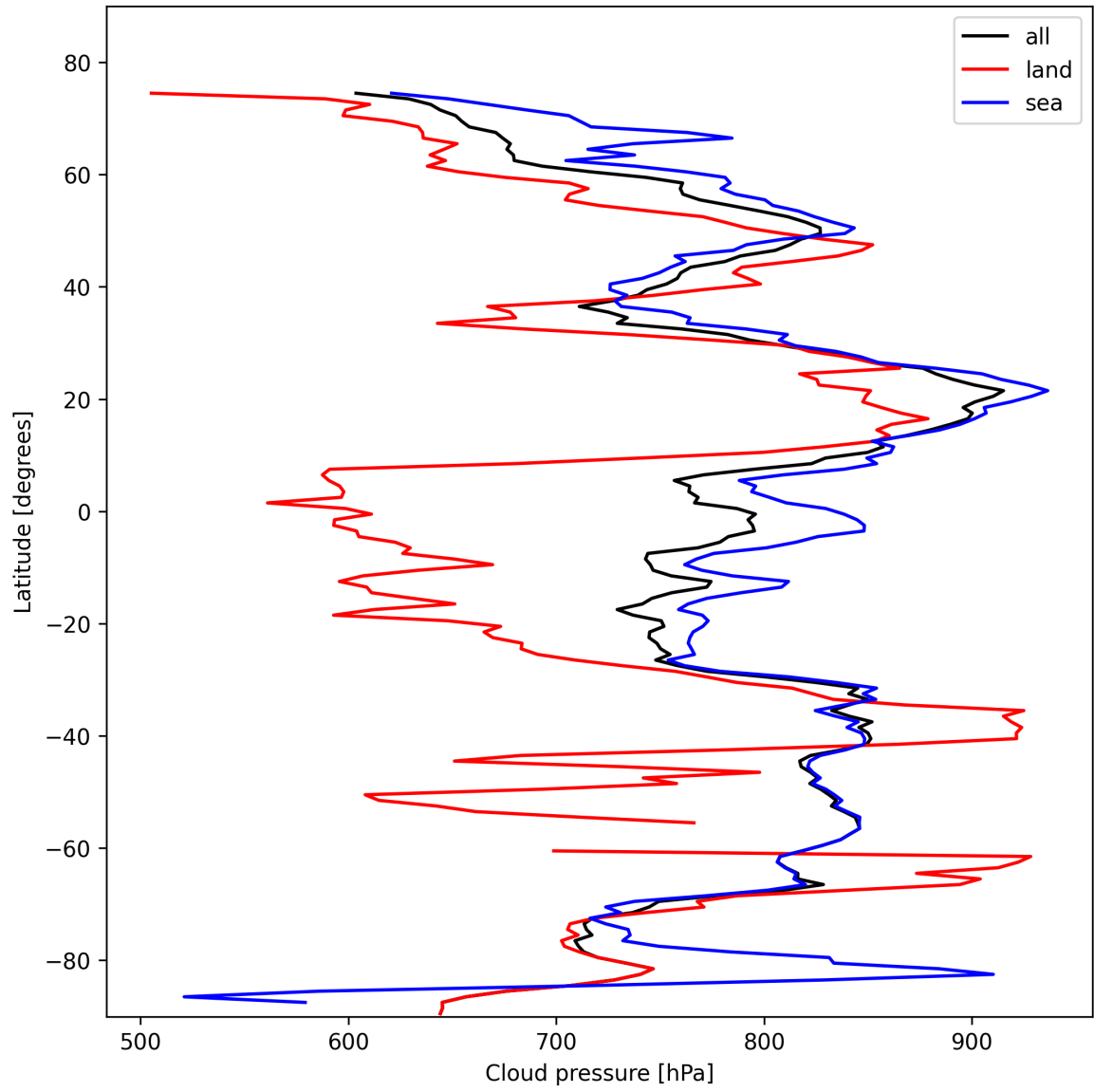
Figure 13: Zonal average of “Cloud pressure” for 2025-02-11 to 2025-02-13.
