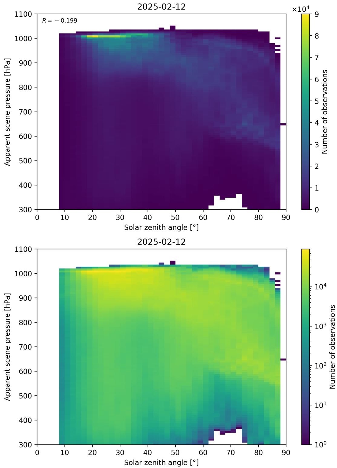
Figure 108: Scatter density plot of “Solar zenith angle” against “Apparent scene pressure” for 2025-02-11 to 2025-02-13.
