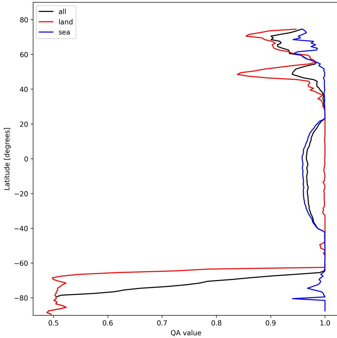
Figure 12: Zonal average of “QA value” for 2025-02-11 to 2025-02-13.
