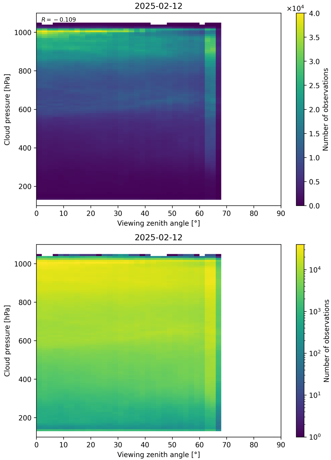
Figure 121: Scatter density plot of “Viewing zenith angle” against “Cloud pressure” for 2025-02-11 to 2025-02-13.
