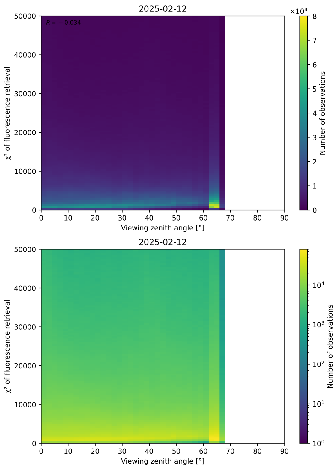
Figure 119: Scatter density plot of “Viewing zenith angle” against “ \chi^2 of fluorescence retrieval” for 2025-02-11 to 2025-02-13.
