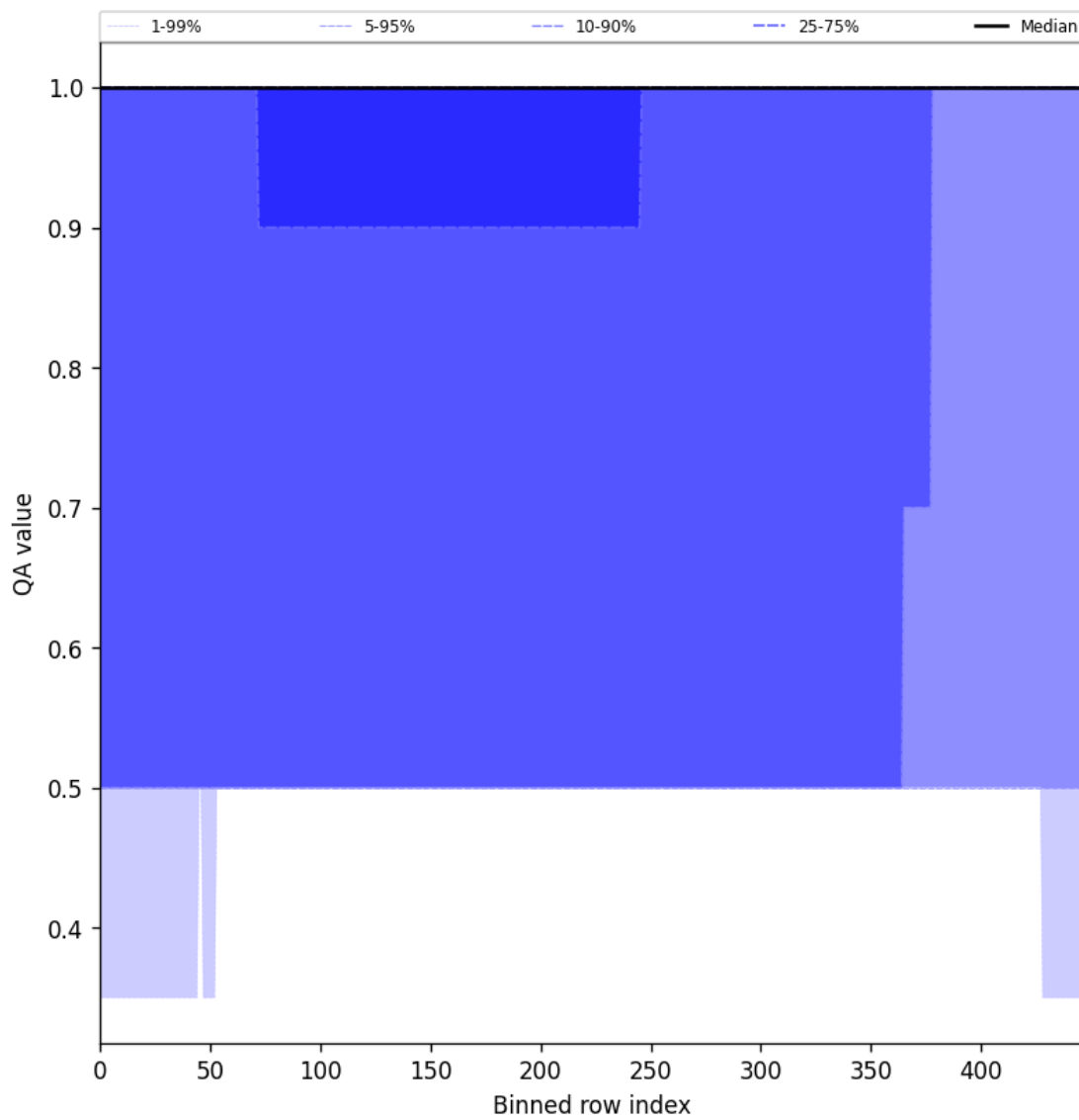
Figure 46: Along track statistics of “QA value” for 2025-02-11 to 2025-02-13
