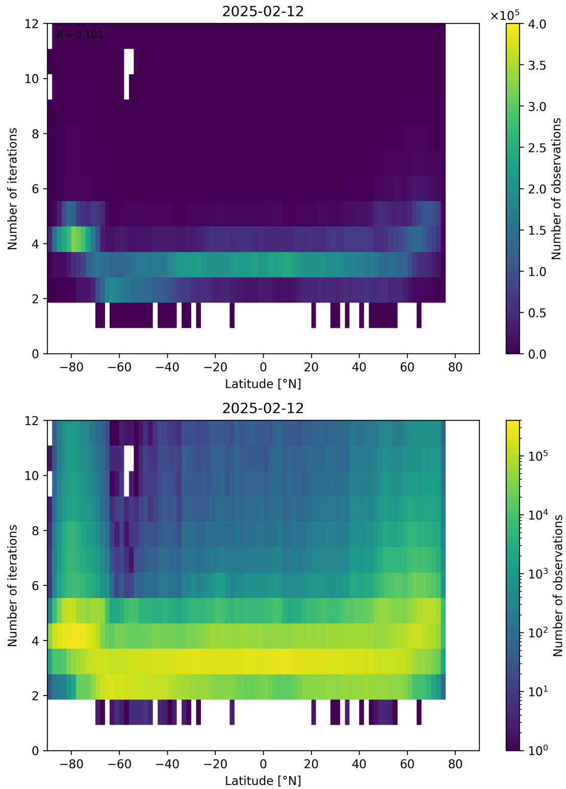
Figure 93: Scatter density plot of “Latitude” against “Number of iterations” for 2025-02-11 to 2025-02-13.
