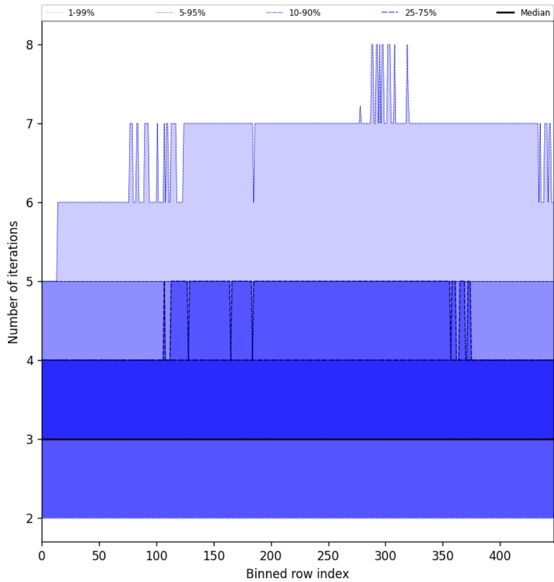
Figure 56: Along track statistics of “Number of iterations” for 2025-02-11 to 2025-02-13
