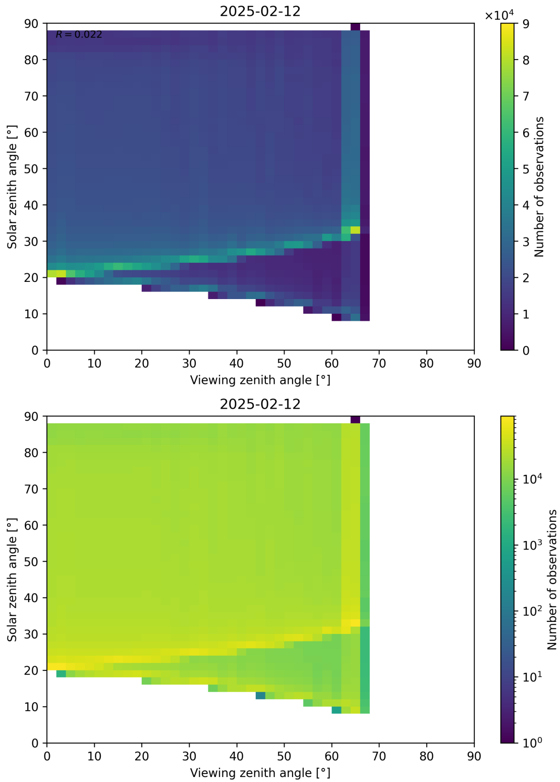
Figure 127: Scatter density plot of “Viewing zenith angle” against “Solar zenith angle” for 2025-02-11 to 2025-02-13.
