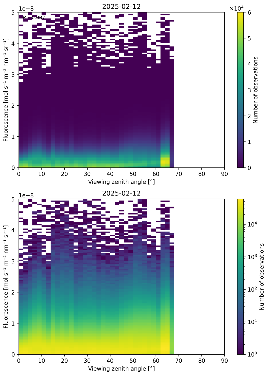
Figure 122: Scatter density plot of “Viewing zenith angle” against “Fluorescence” for 2025-02-11 to 2025-02-13.
