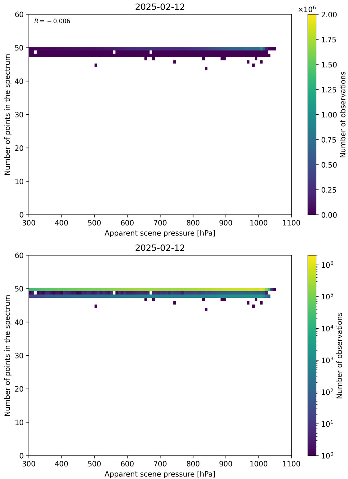
Figure 66: Scatter density plot of “Apparent scene pressure” against “Number of points in the spectrum” for 2025-02-11 to 2025-02-13.
