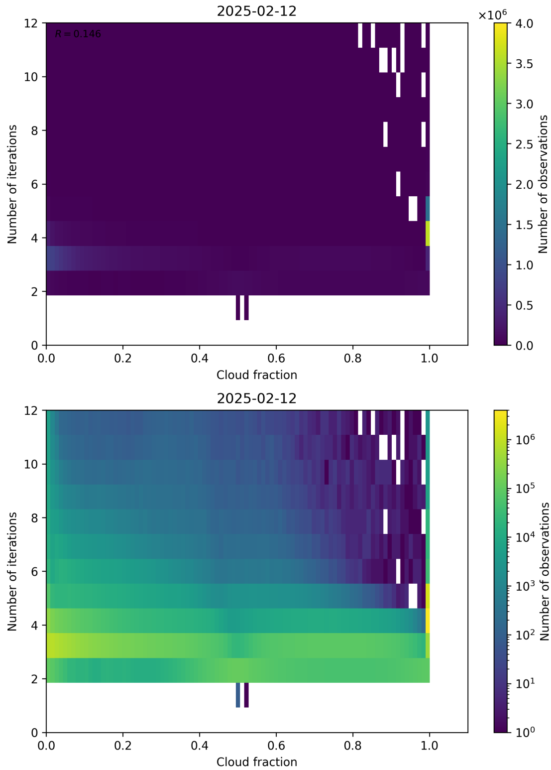
Figure 73: Scatter density plot of “Cloud fraction” against “Number of iterations” for 2025-02-11 to 2025-02-13.
