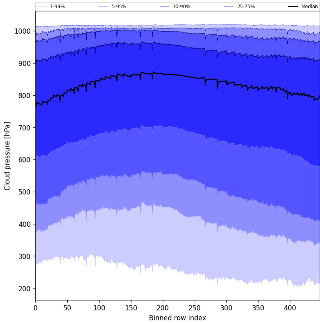
Figure 47: Along track statistics of “Cloud pressure” for 2025-02-11 to 2025-02-13
