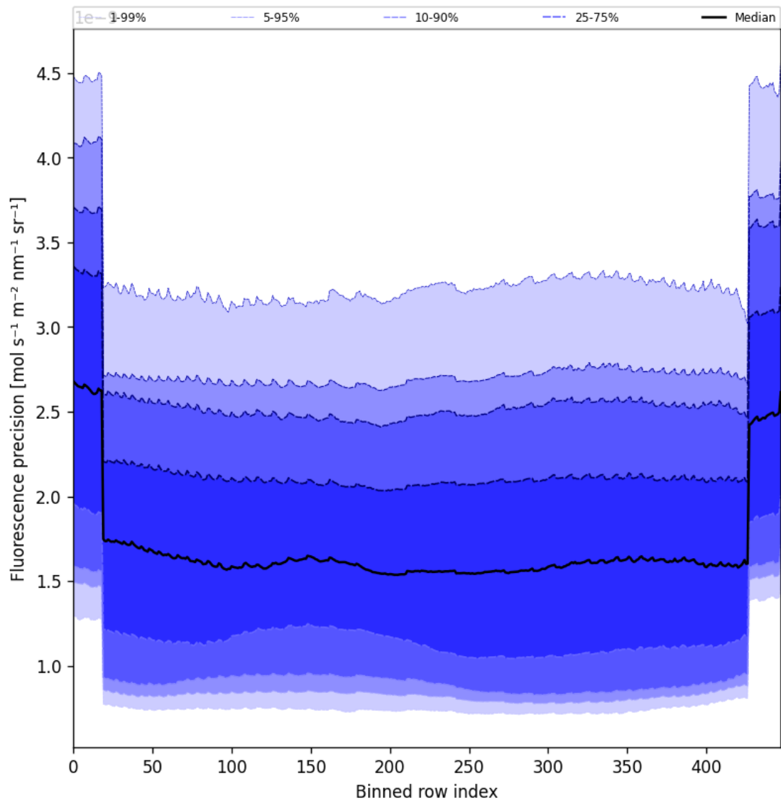
Figure 58: Along track statistics of “Fluorescence precision” for 2025-02-11 to 2025-02-13
