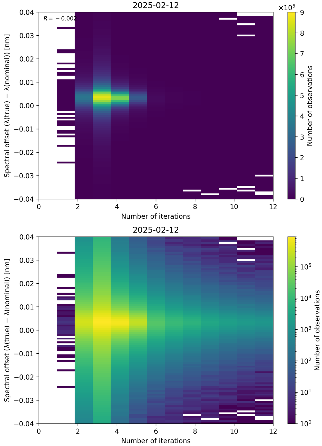
Figure 100: Scatter density plot of “Number of iterations” against “Spectral offset ( \lambda_{\text{true}} - \lambda_{\text{nominal}} )” for 2025-02-11 to 2025-02-13.
