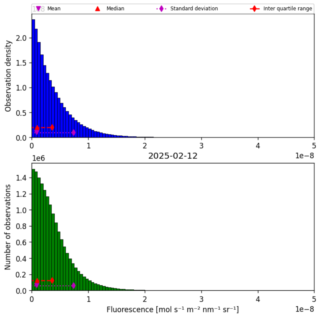
Figure 40: Histogram of “Fluorescence” for 2025-02-11 to 2025-02-13
