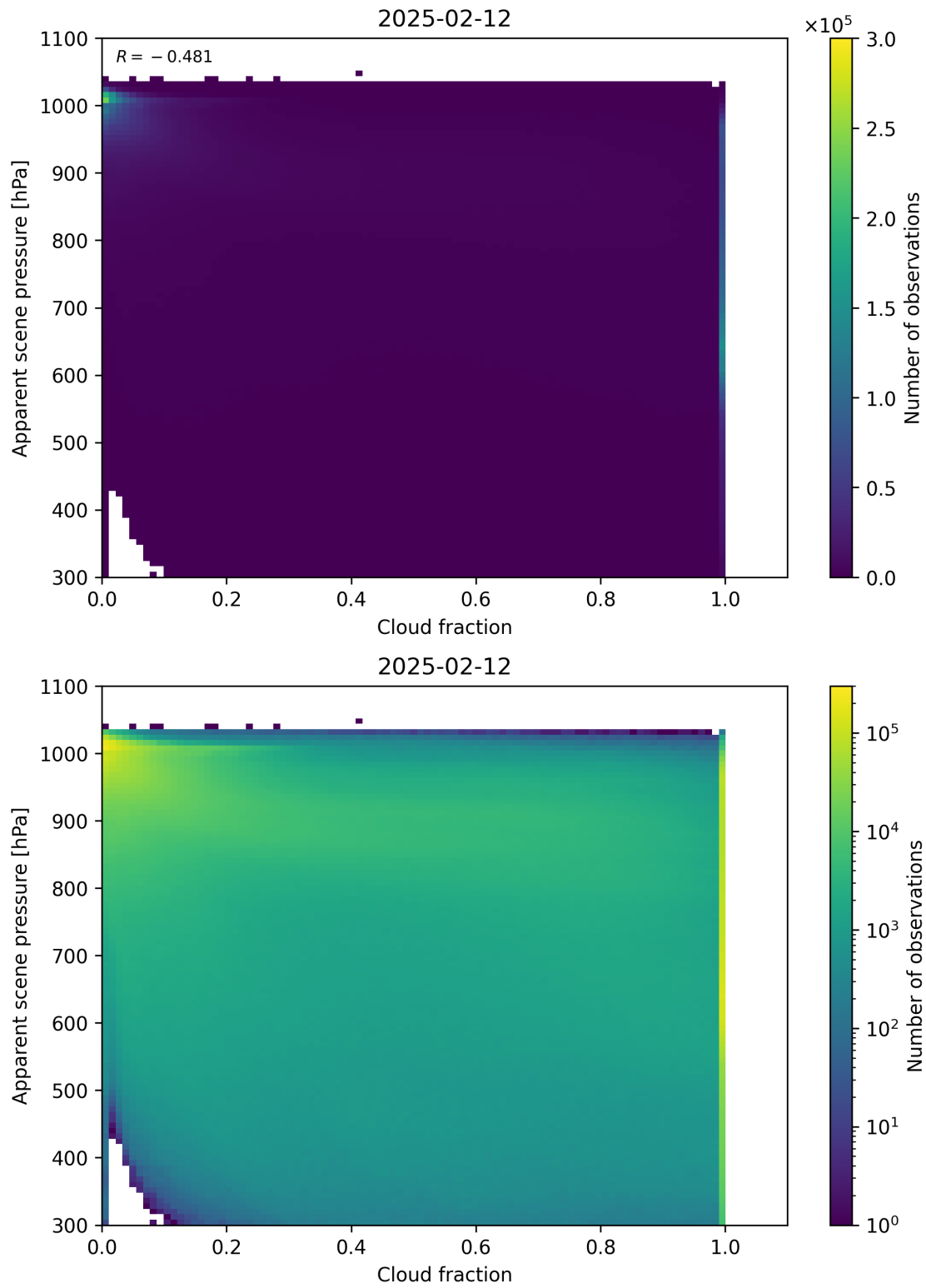
Figure 70: Scatter density plot of “Cloud fraction” against “Apparent scene pressure” for 2025-02-11 to 2025-02-13.
