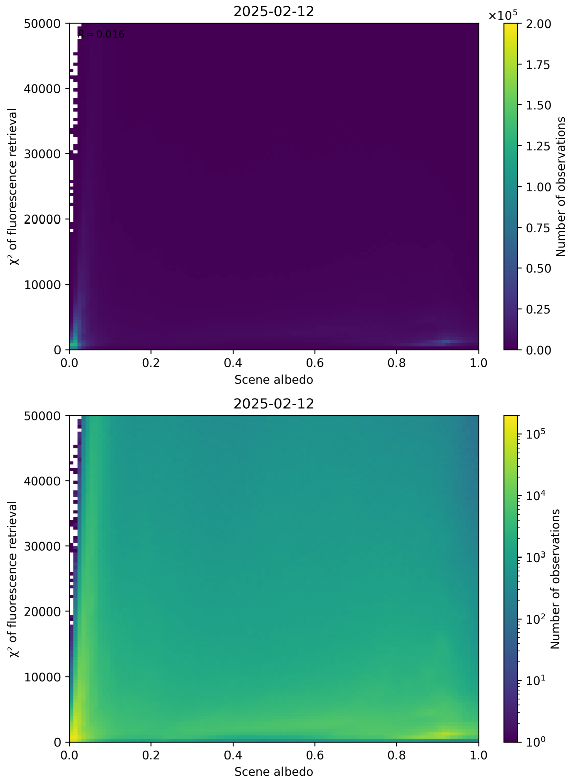
Figure 103: Scatter density plot of “Scene albedo” against “ \chi^2 of fluorescence retrieval” for 2025-02-11 to 2025-02-13.
