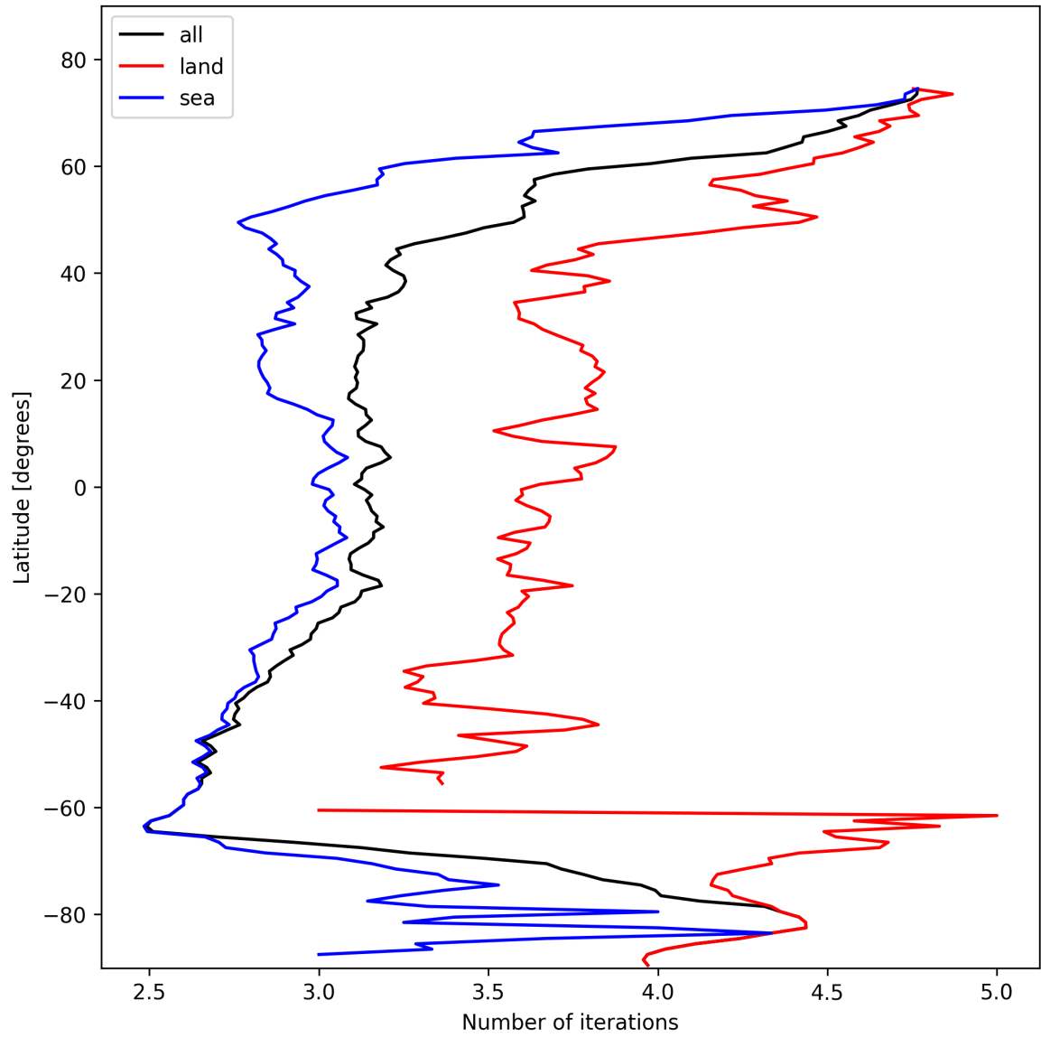
Figure 22: Zonal average of “Number of iterations” for 2025-02-11 to 2025-02-13.
