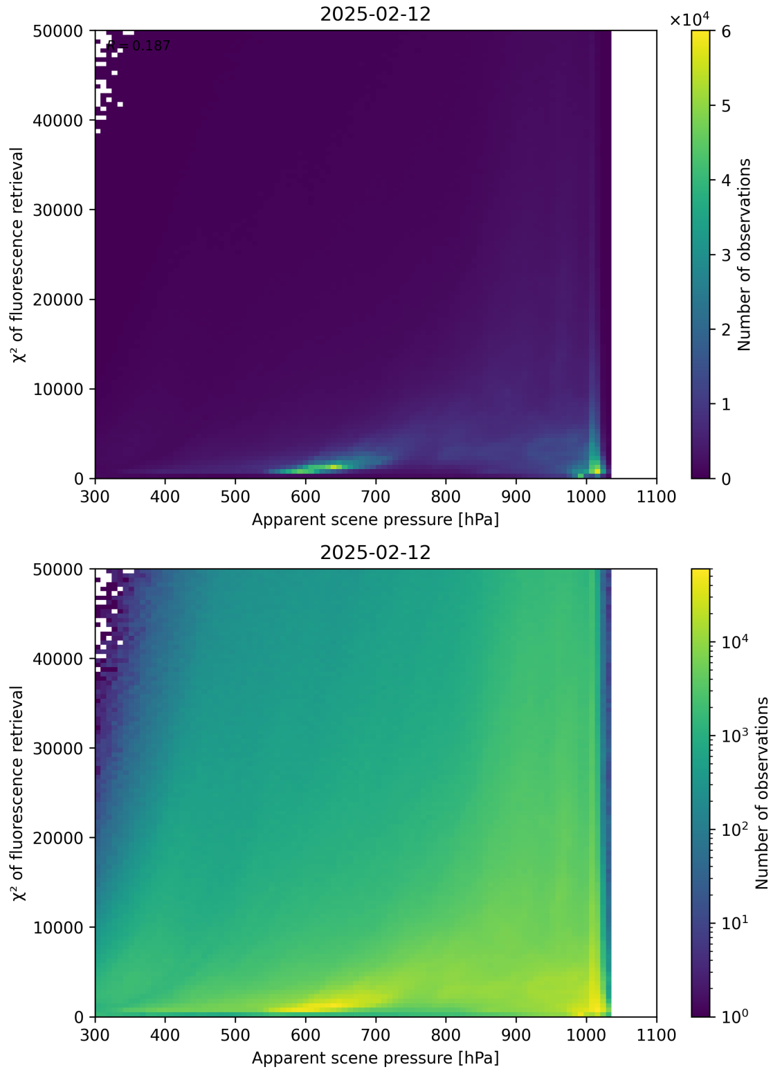
Figure 63: Scatter density plot of “Apparent scene pressure” against “ \chi^2 of fluorescence retrieval” for 2025-02-11 to 2025-02-13.
