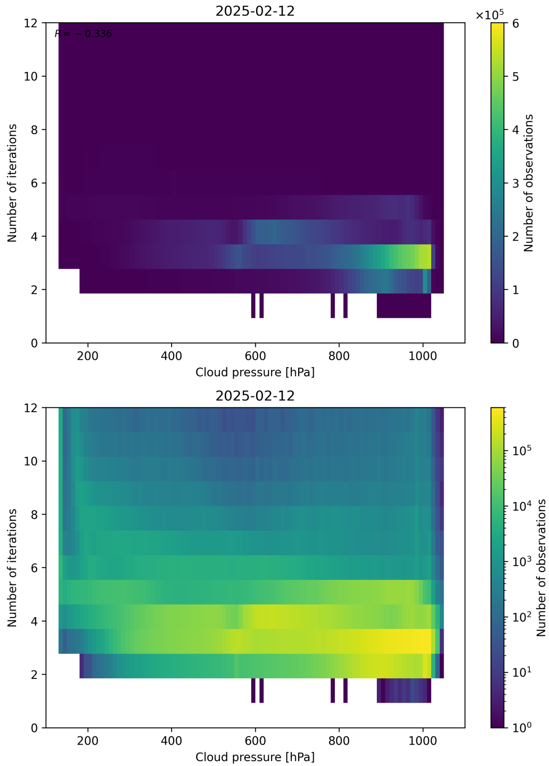
Figure 81: Scatter density plot of “Cloud pressure” against “Number of iterations” for 2025-02-11 to 2025-02-13.
