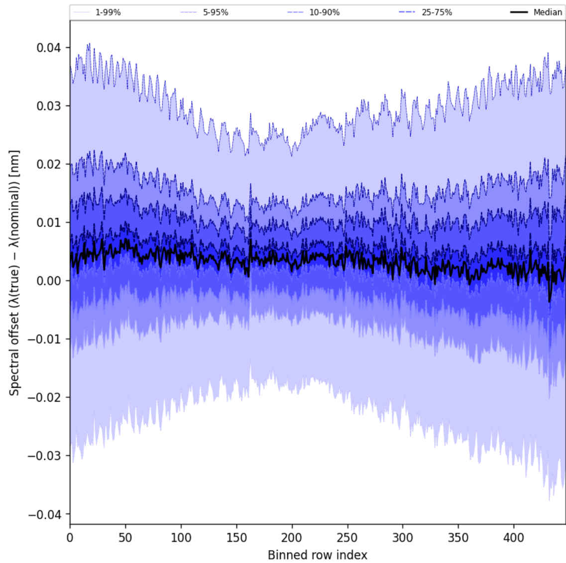
Figure 62: Along track statistics of “Spectral offset ( \lambda_{\text{true}} - \lambda_{\text{nominal}} )” for 2025-02-11 to 2025-02-13
