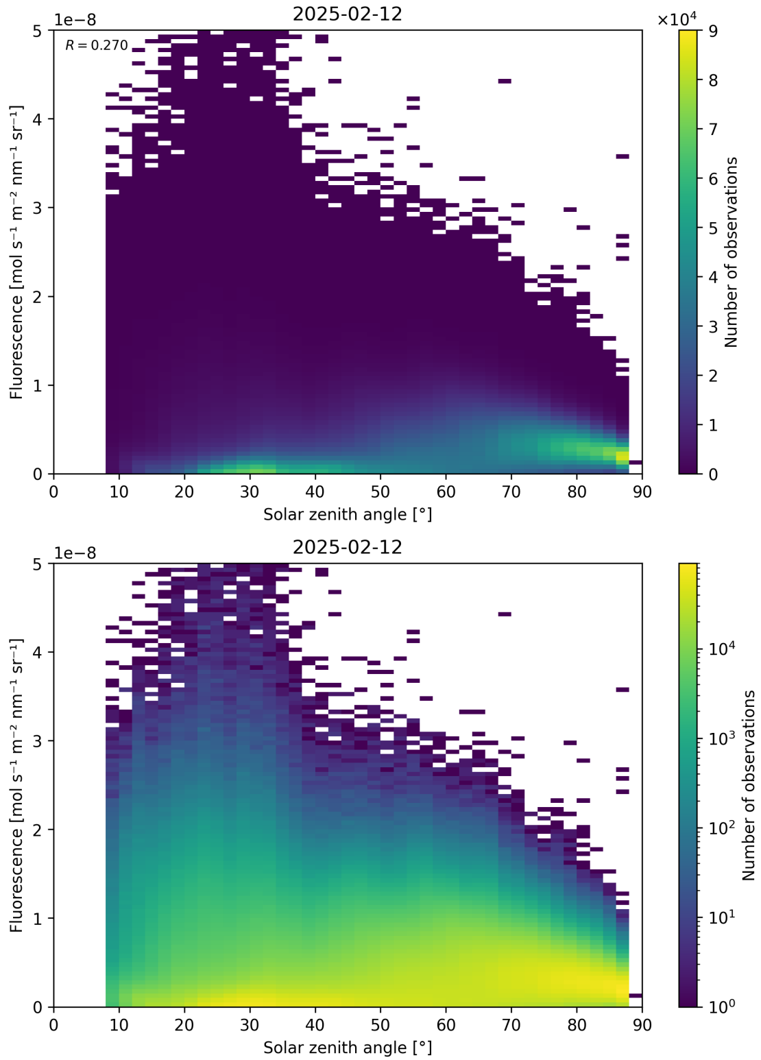
Figure 112: Scatter density plot of “Solar zenith angle” against “Fluorescence” for 2025-02-11 to 2025-02-13.
