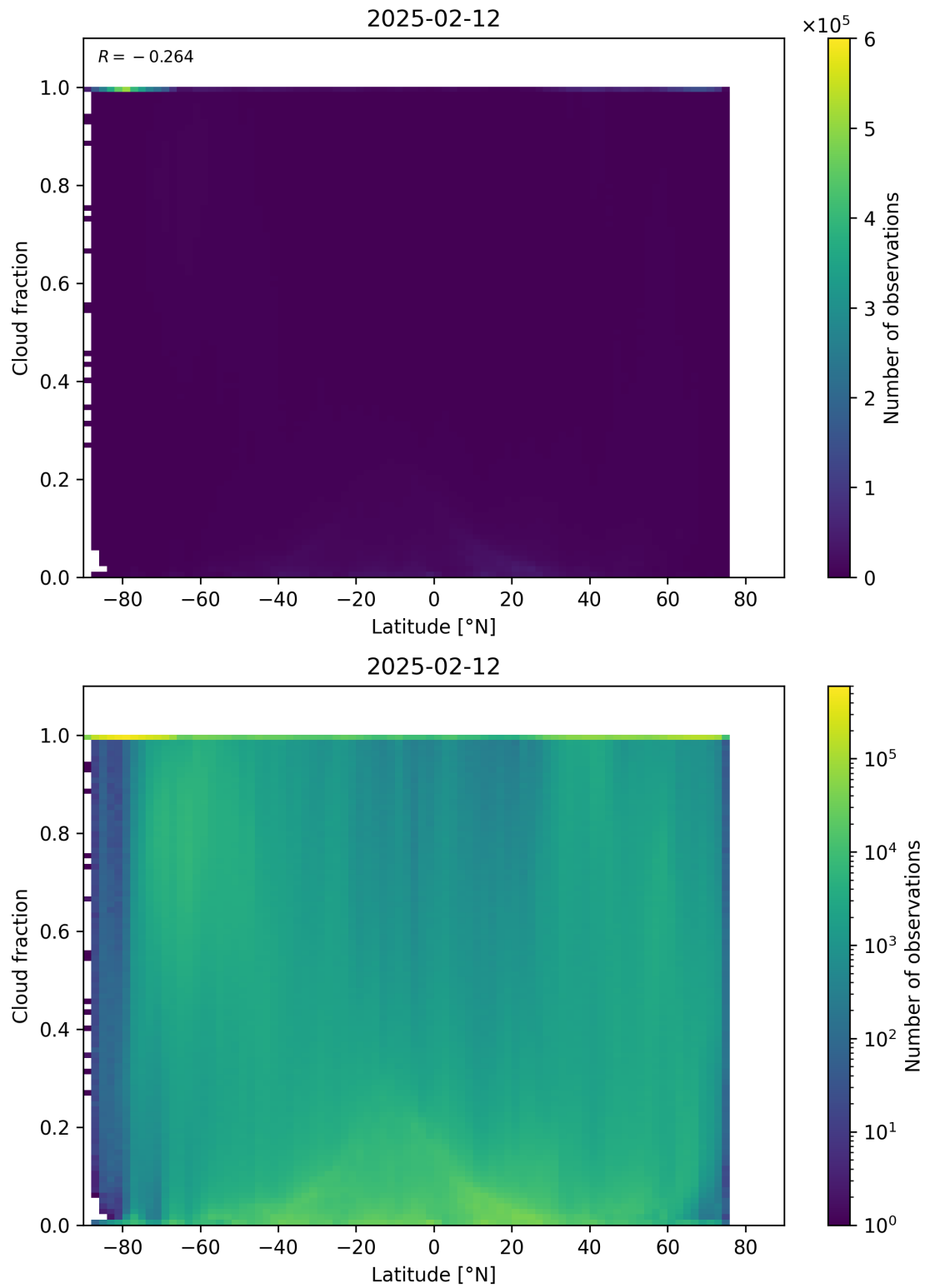
Figure 90: Scatter density plot of “Latitude” against “Cloud fraction” for 2025-02-11 to 2025-02-13.
