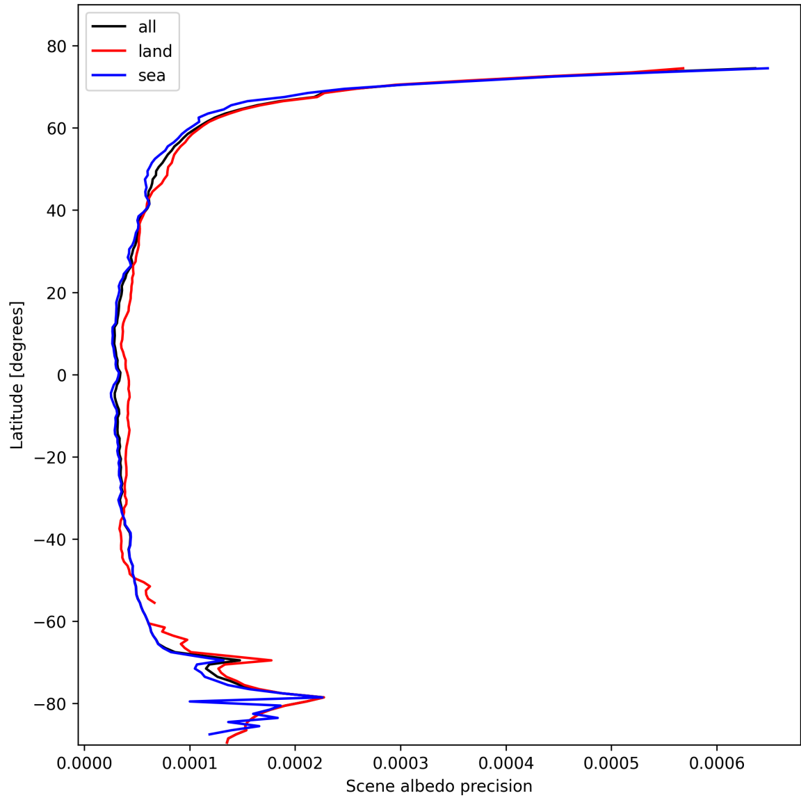
Figure 18: Zonal average of “Scene albedo precision” for 2025-02-11 to 2025-02-13.
