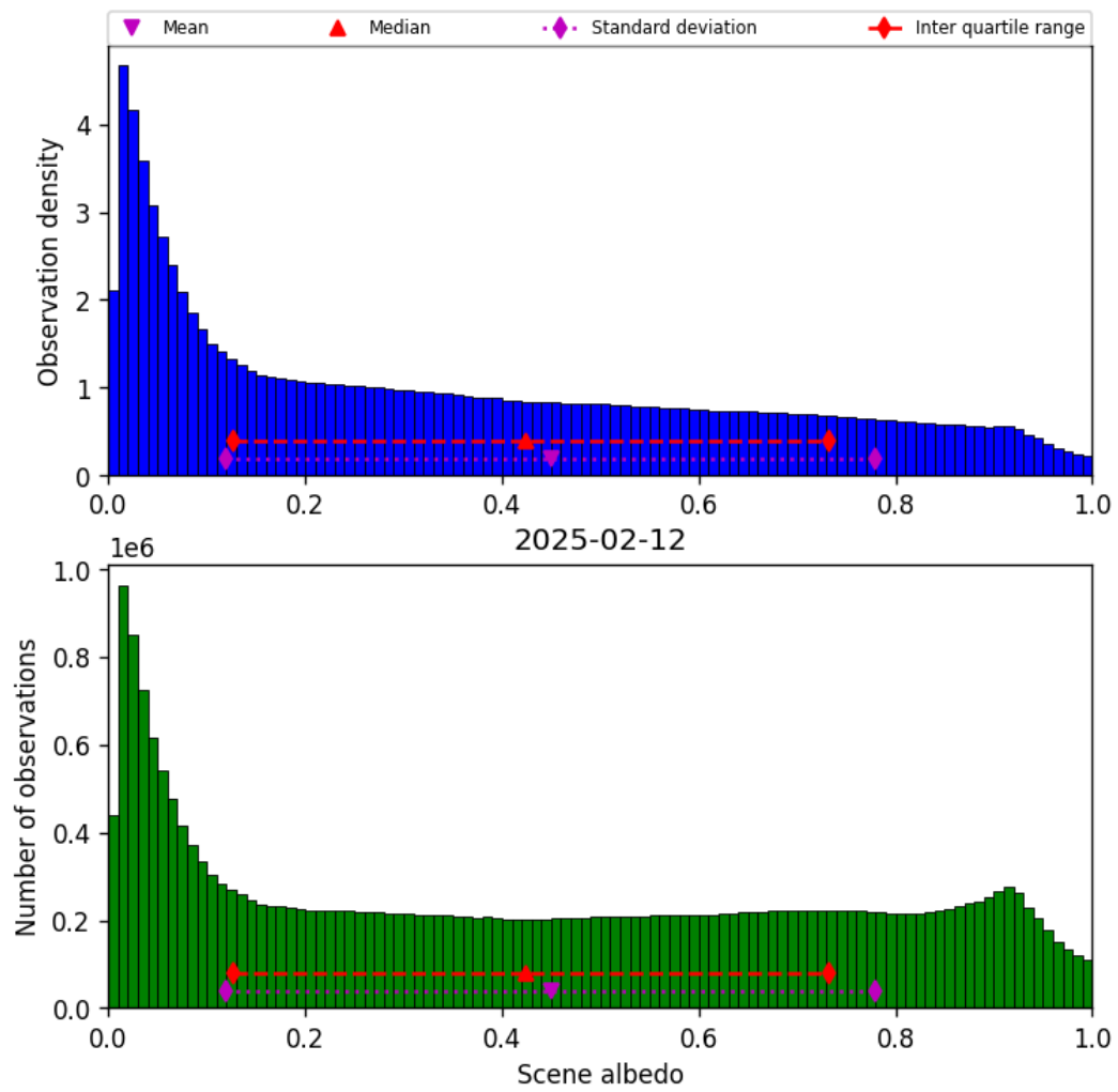
Figure 34: Histogram of “Scene albedo” for 2025-02-11 to 2025-02-13
