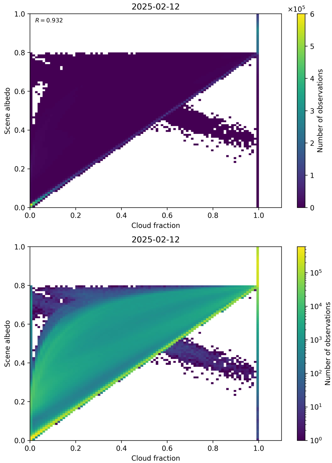
Figure 75: Scatter density plot of “Cloud fraction” against “Scene albedo” for 2025-02-11 to 2025-02-13.
