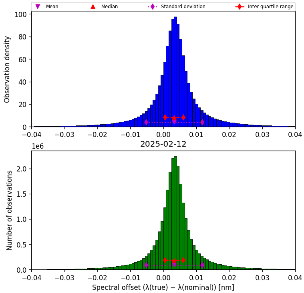
Figure 45: Histogram of “Spectral offset ( \lambda_{\text{true}} - \lambda_{\text{nominal}} )” for 2025-02-11 to 2025-02-13
