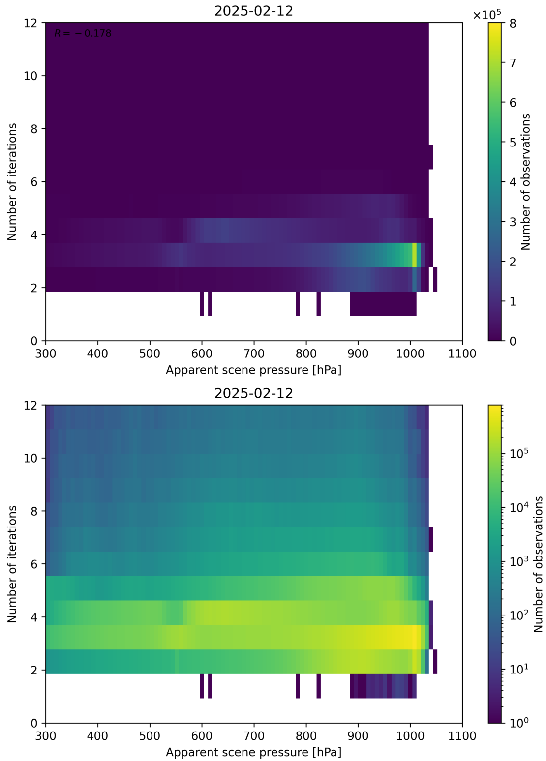
Figure 65: Scatter density plot of “Apparent scene pressure” against “Number of iterations” for 2025-02-11 to 2025-02-13.
