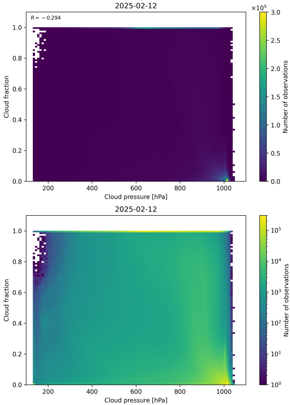
Figure 79: Scatter density plot of “Cloud pressure” against “Cloud fraction” for 2025-02-11 to 2025-02-13.
