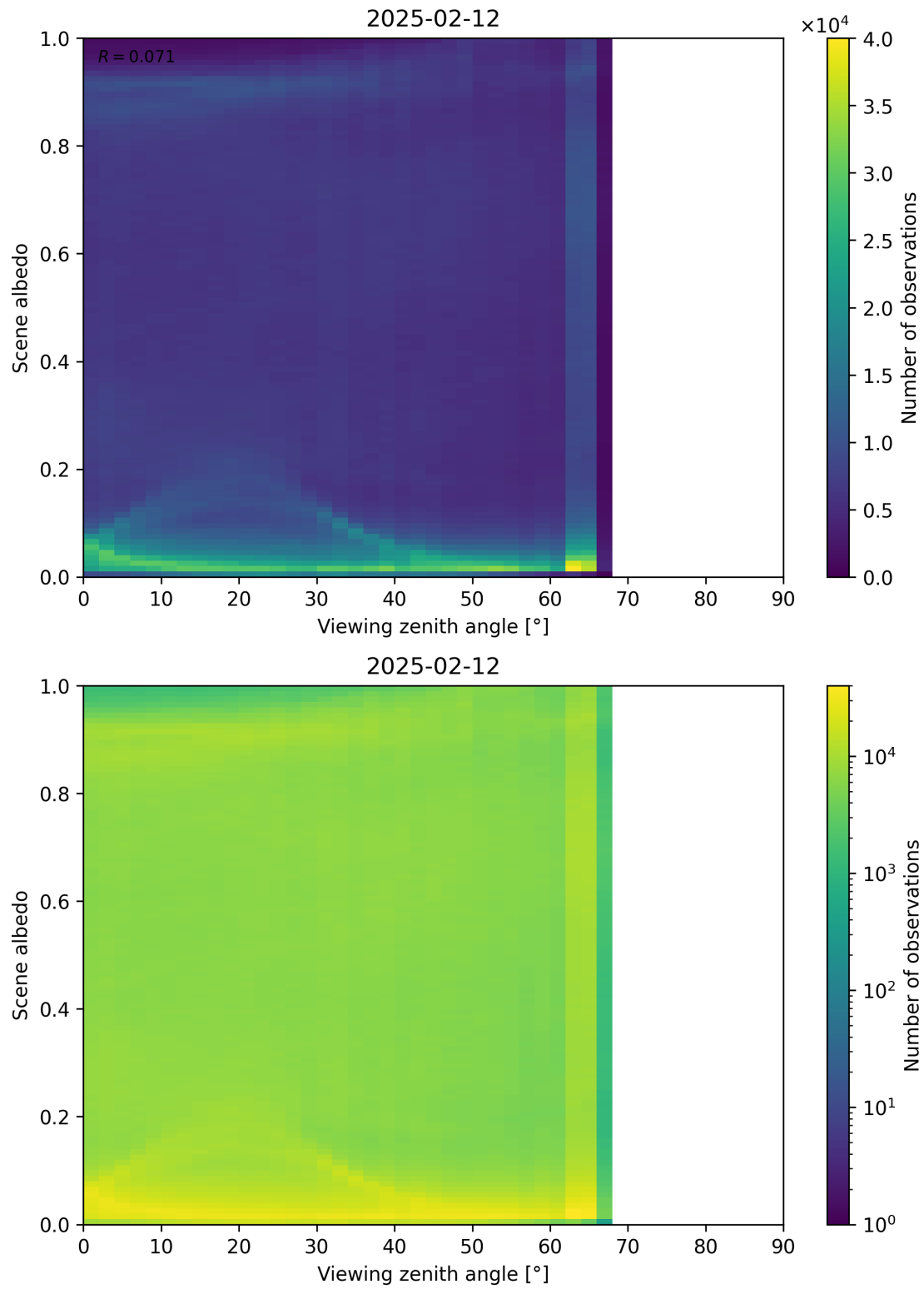
Figure 126: Scatter density plot of “Viewing zenith angle” against “Scene albedo” for 2025-02-11 to 2025-02-13.
