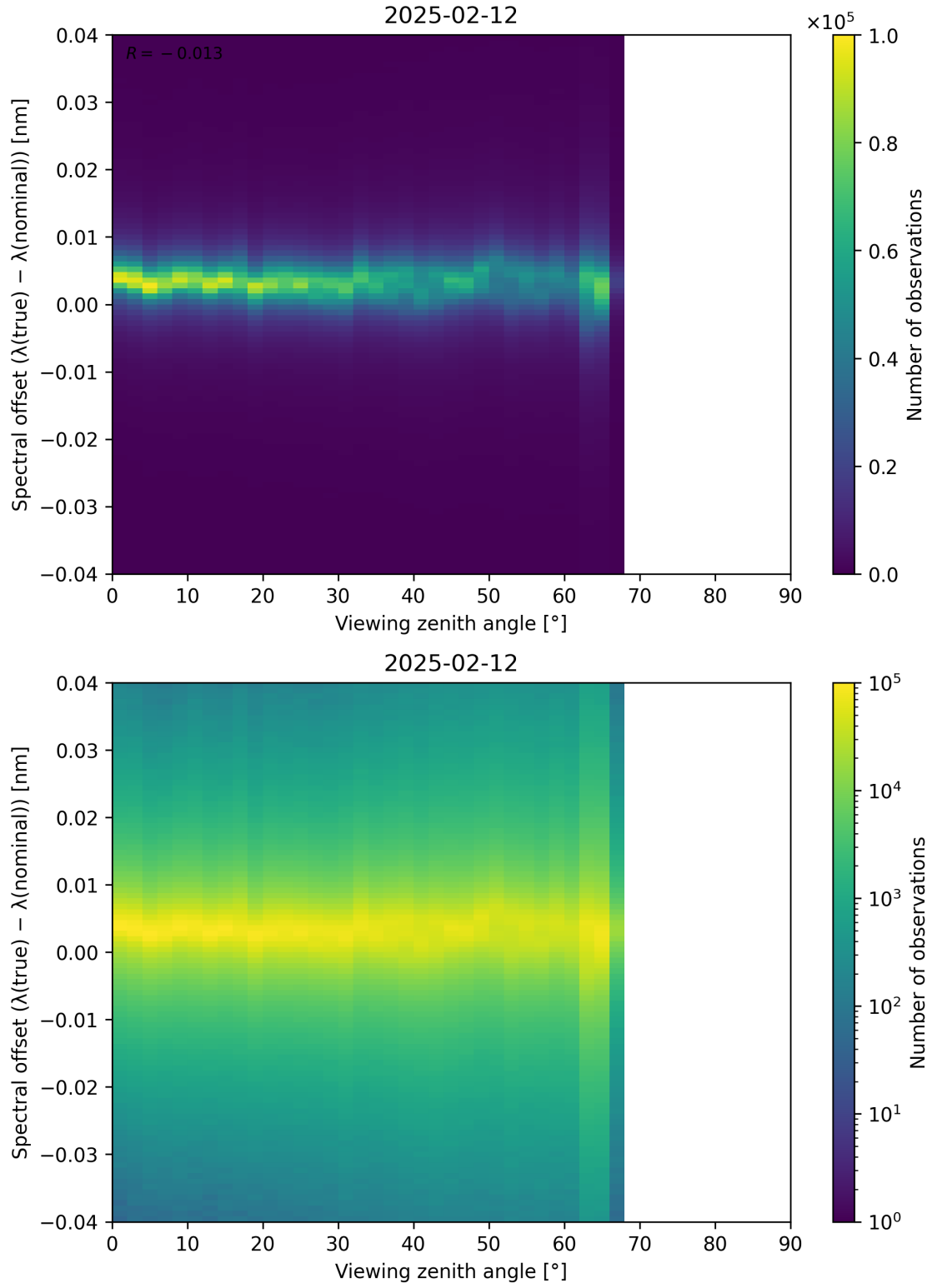
Figure 128: Scatter density plot of “Viewing zenith angle” against “Spectral offset ( \lambda_{\text{true}} - \lambda_{\text{nominal}} )” for 2025-02-11 to 2025-02-13.
