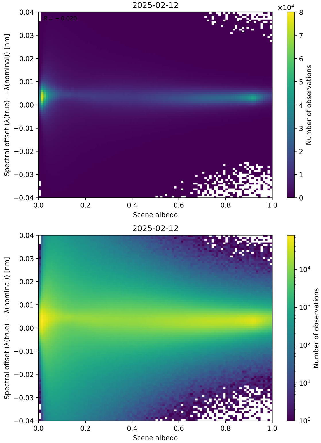
Figure 107: Scatter density plot of “Scene albedo” against “Spectral offset ( \lambda_{\text{true}} - \lambda_{\text{nominal}} )” for 2025-02-11 to 2025-02-13.
