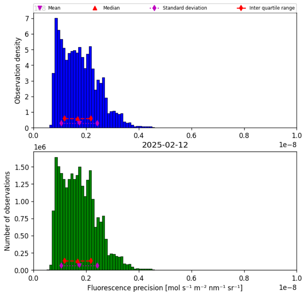
Figure 41: Histogram of “Fluorescence precision” for 2025-02-11 to 2025-02-13
