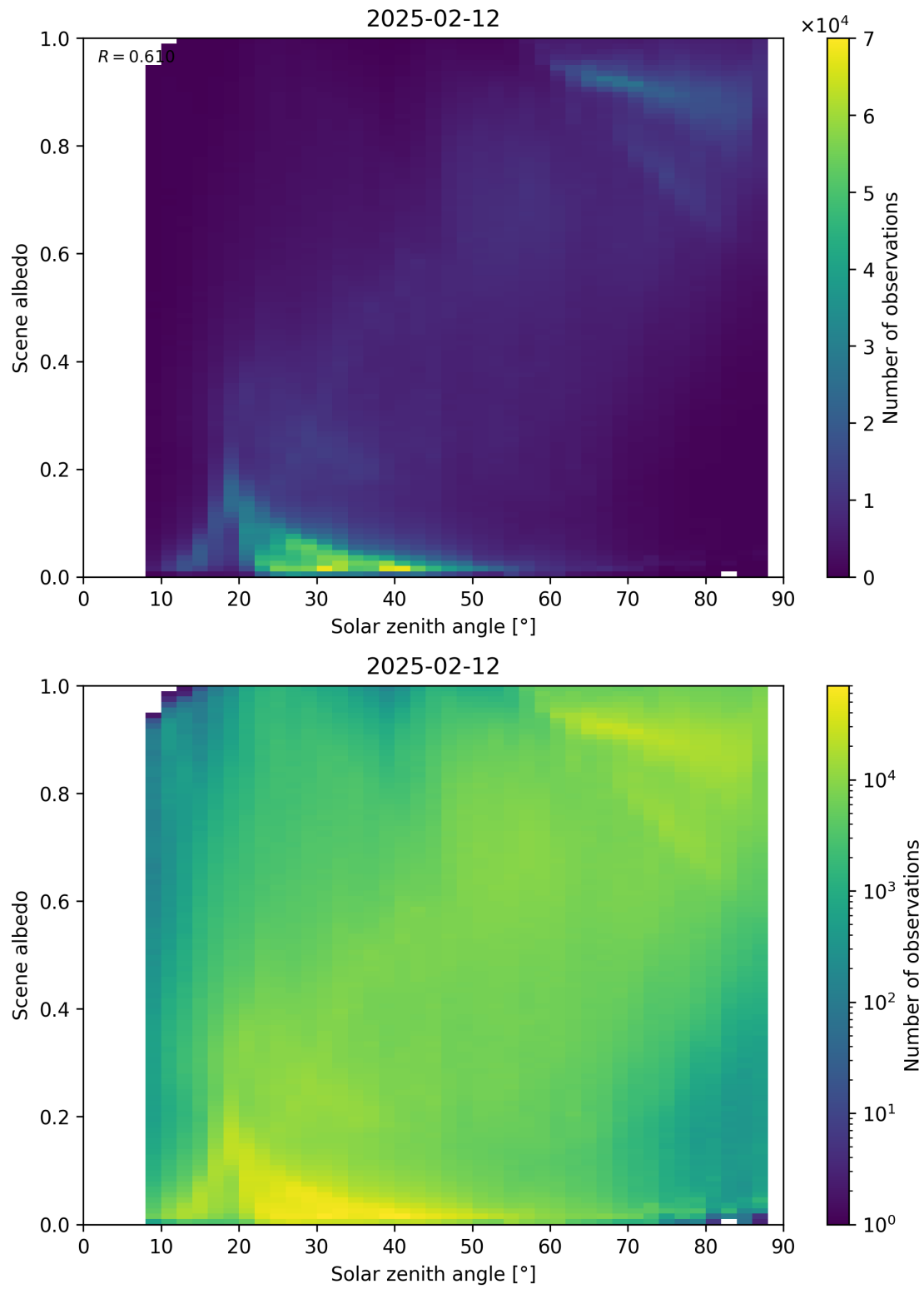
Figure 116: Scatter density plot of “Solar zenith angle” against “Scene albedo” for 2025-02-11 to 2025-02-13.
