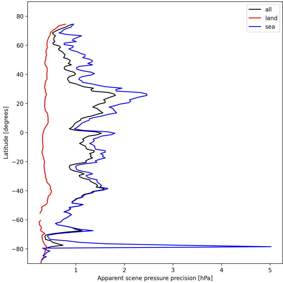
Figure 20: Zonal average of “Apparent scene pressure precision” for 2025-02-11 to 2025-02-13.
