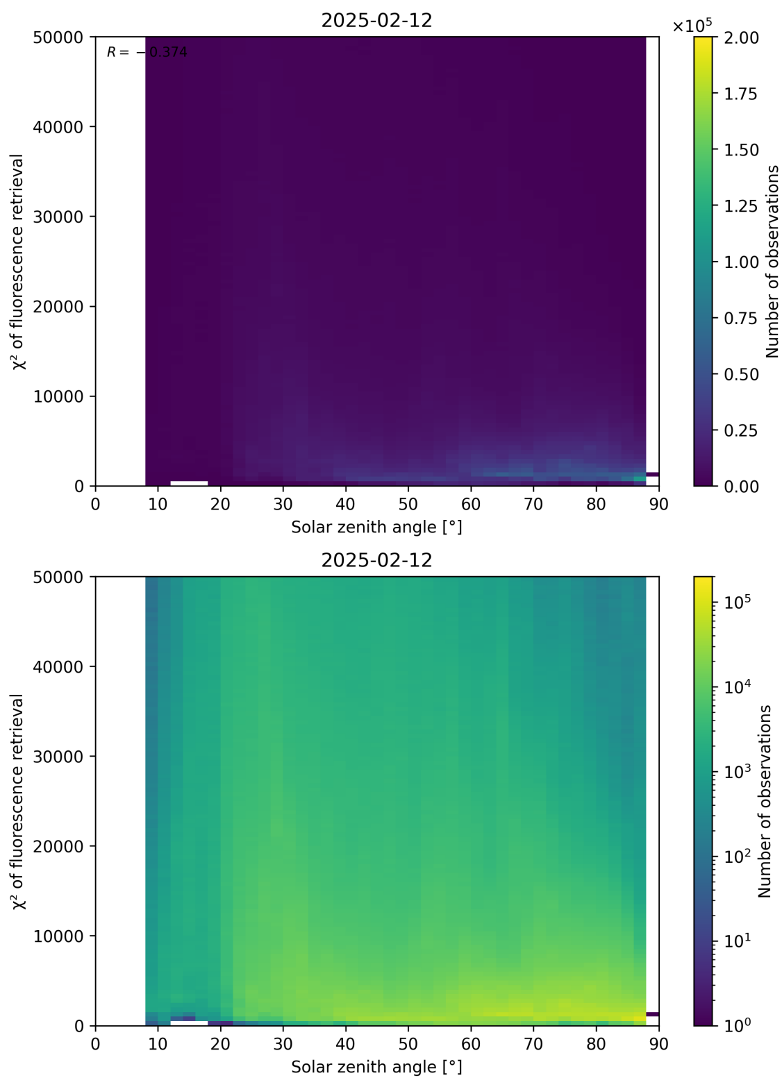
Figure 109: Scatter density plot of “Solar zenith angle” against “ \chi^2 of fluorescence retrieval” for 2025-02-11 to 2025-02-13.
