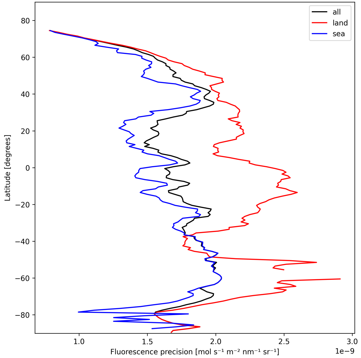
Figure 24: Zonal average of “Fluorescence precision” for 2025-02-11 to 2025-02-13.
