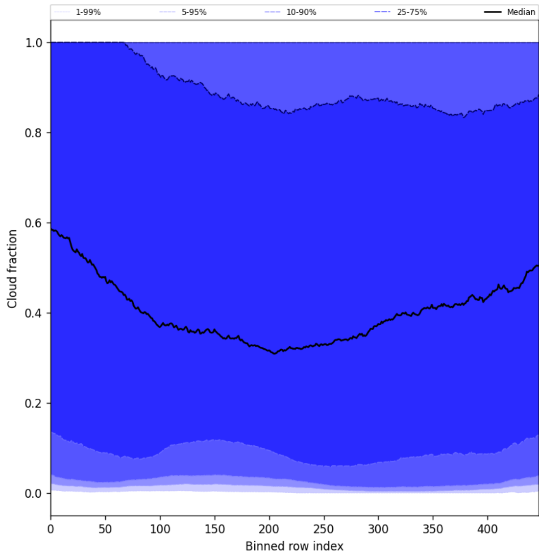
Figure 49: Along track statistics of “Cloud fraction” for 2025-02-11 to 2025-02-13
