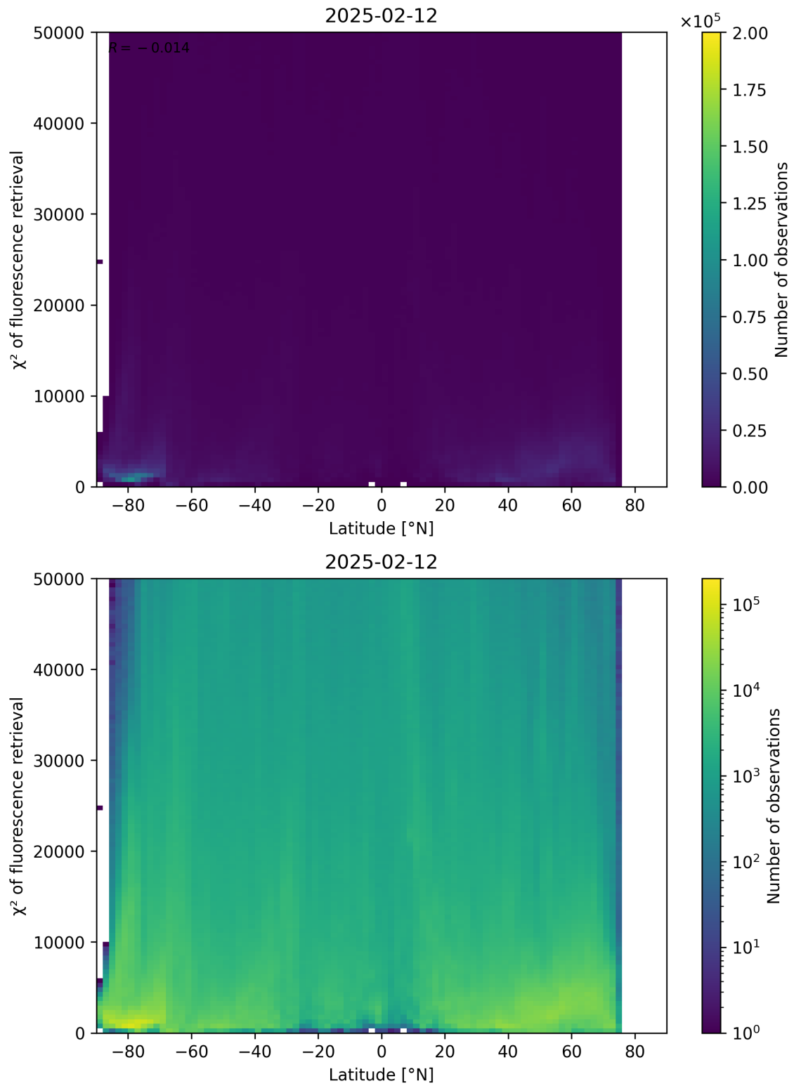
Figure 89: Scatter density plot of “Latitude” against “ \chi^2 of fluorescence retrieval” for 2025-02-11 to 2025-02-13.
