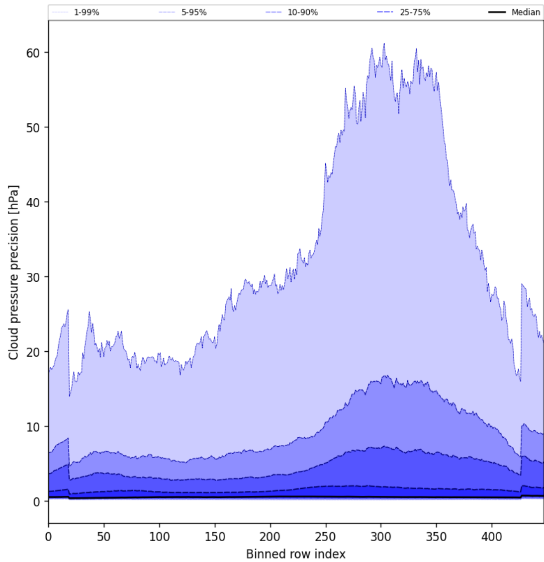
Figure 48: Along track statistics of “Cloud pressure precision” for 2025-02-11 to 2025-02-13
