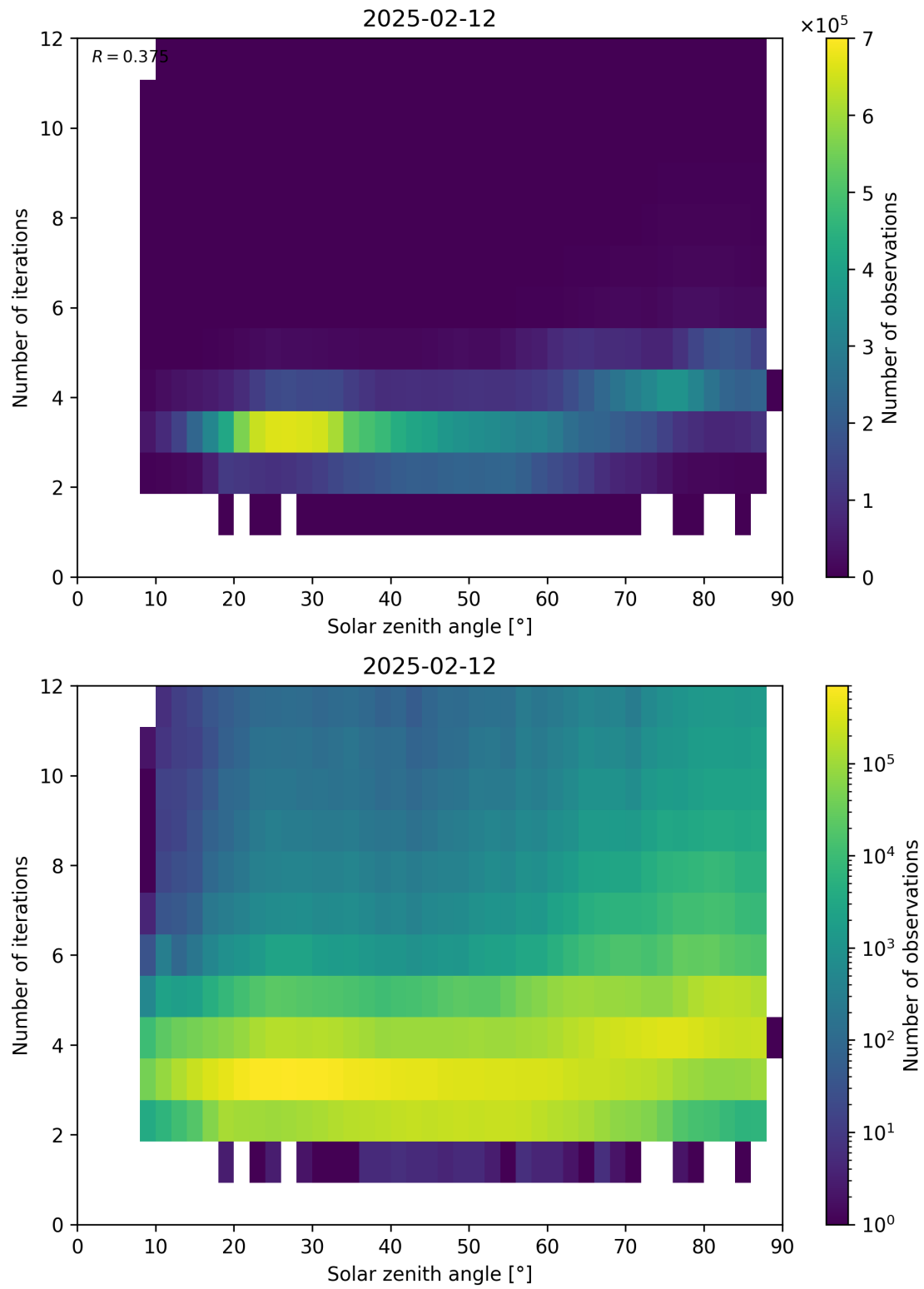
Figure 114: Scatter density plot of “Solar zenith angle” against “Number of iterations” for 2025-02-11 to 2025-02-13.
