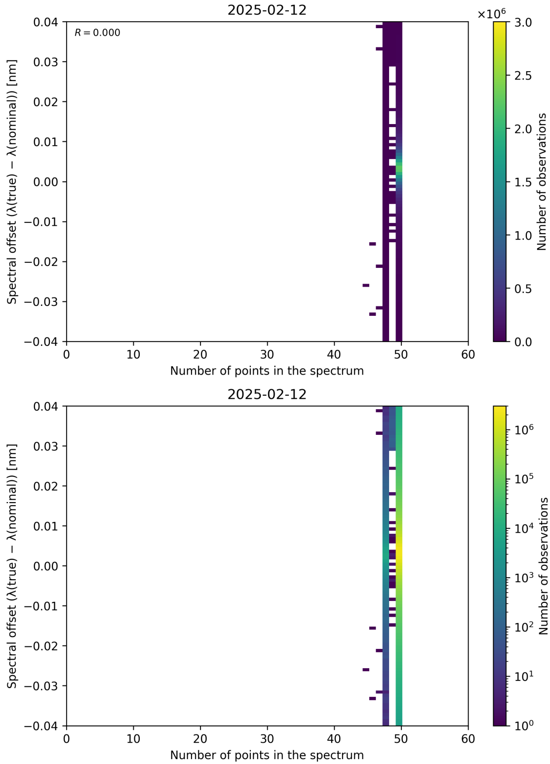
Figure 101: Scatter density plot of “Number of points in the spectrum” against “Spectral offset ( \lambda_{\text{true}} - \lambda_{\text{nominal}} )” for 2025-02-11 to 2025-02-13.
