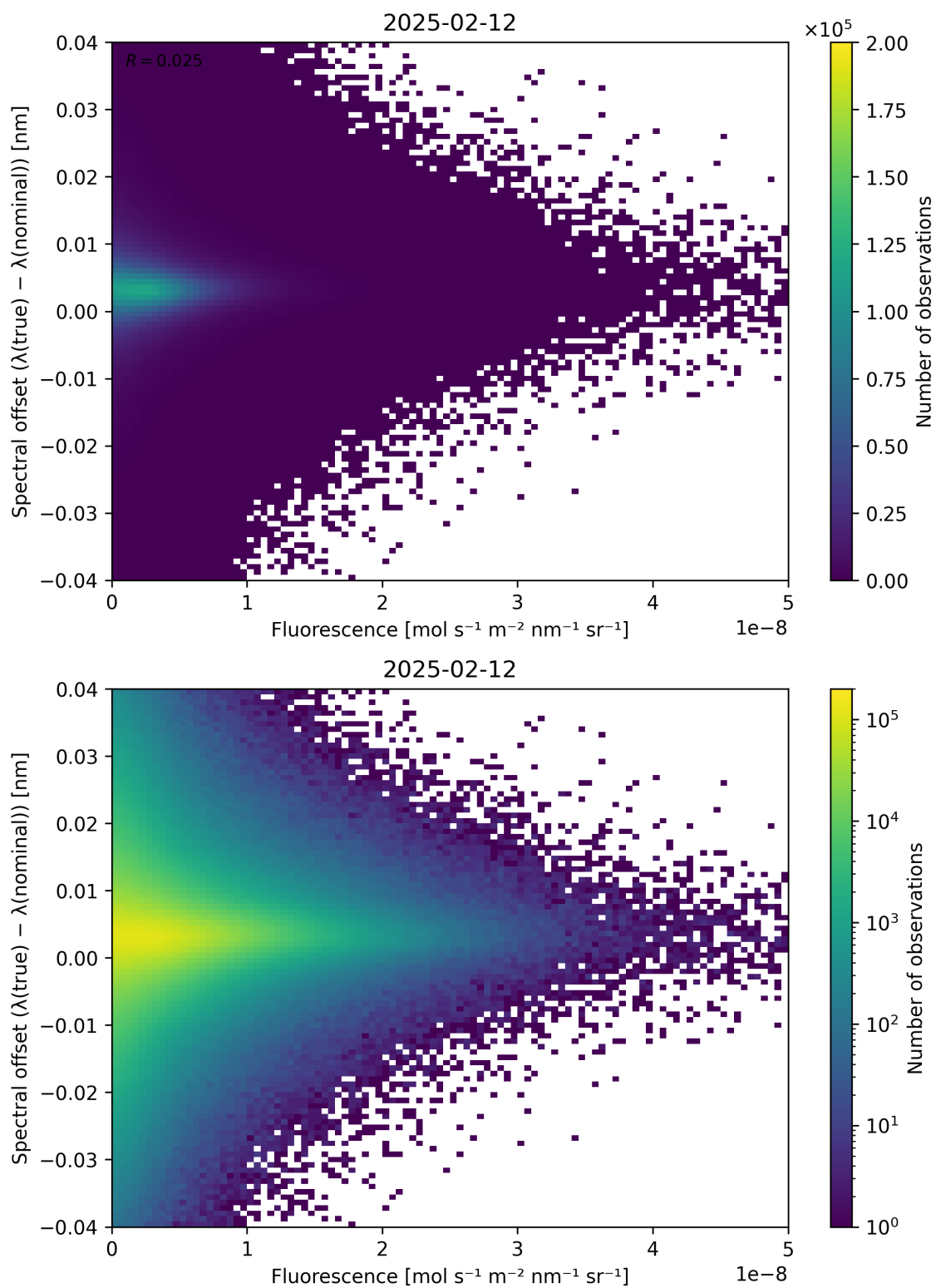
Figure 87: Scatter density plot of “Fluorescence” against “Spectral offset ( \lambda_{\text{true}} - \lambda_{\text{nominal}} )” for 2025-02-11 to 2025-02-13.
