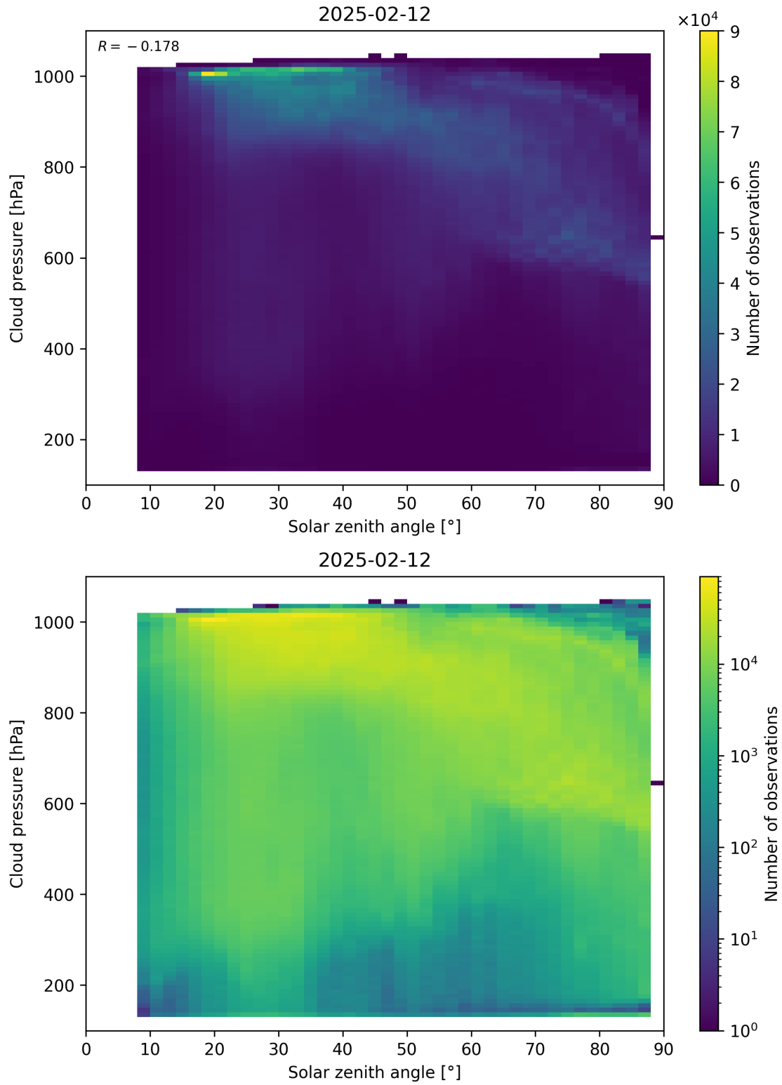
Figure 111: Scatter density plot of “Solar zenith angle” against “Cloud pressure” for 2025-02-11 to 2025-02-13.
