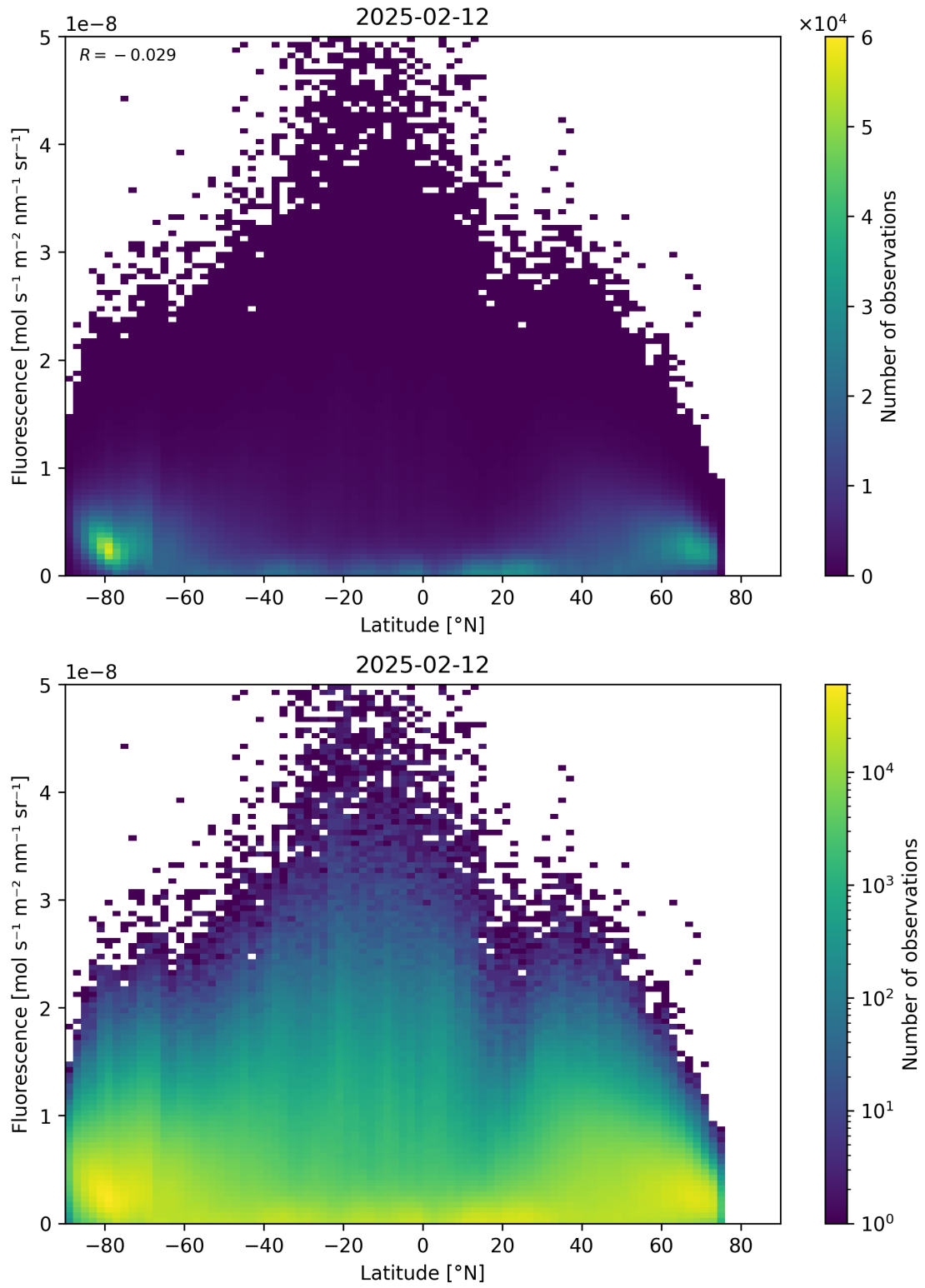
Figure 92: Scatter density plot of “Latitude” against “Fluorescence” for 2025-02-11 to 2025-02-13.
