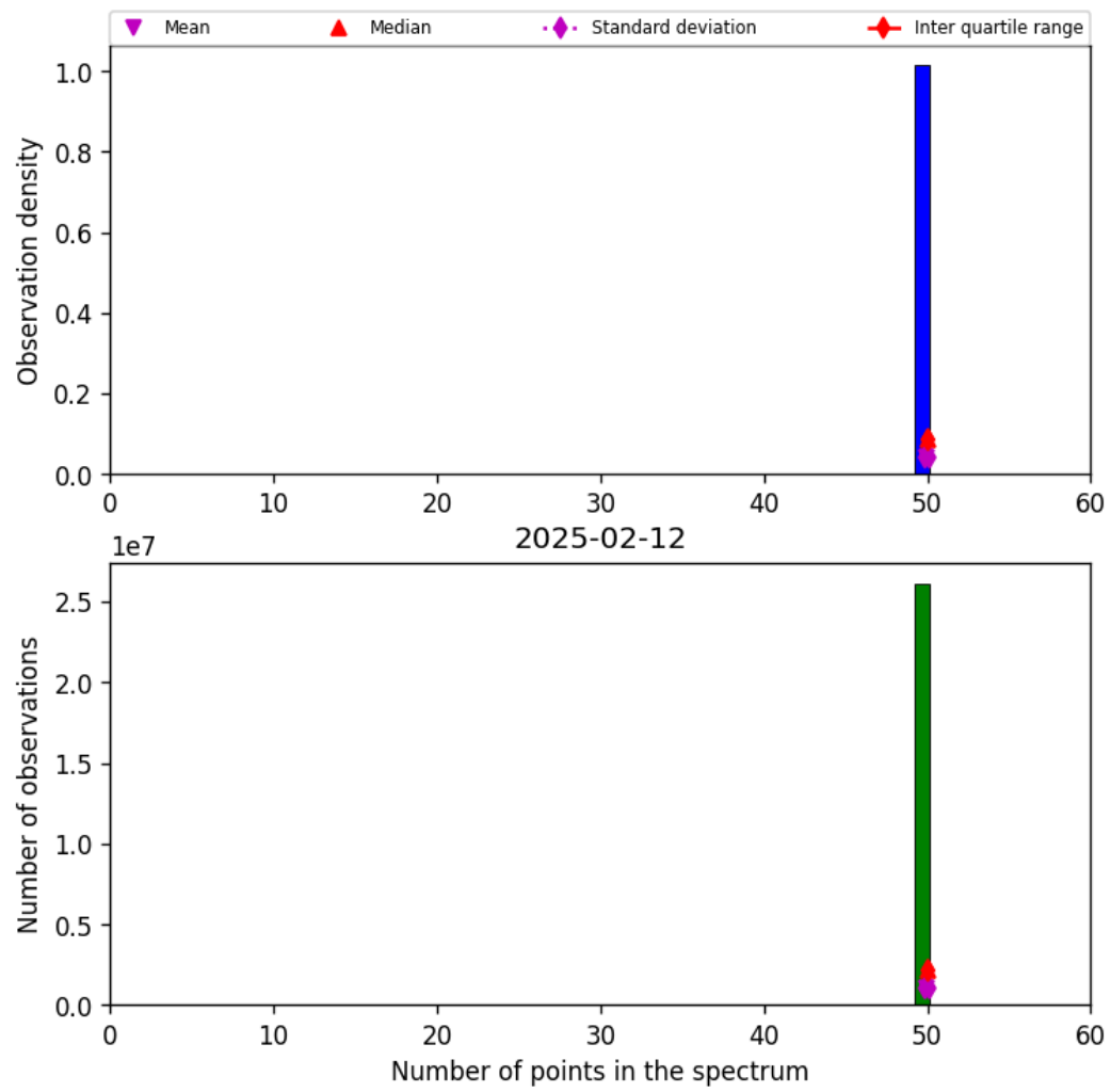
Figure 44: Histogram of "Number of points in the spectrum" for 2025-02-11 to 2025-02-13
