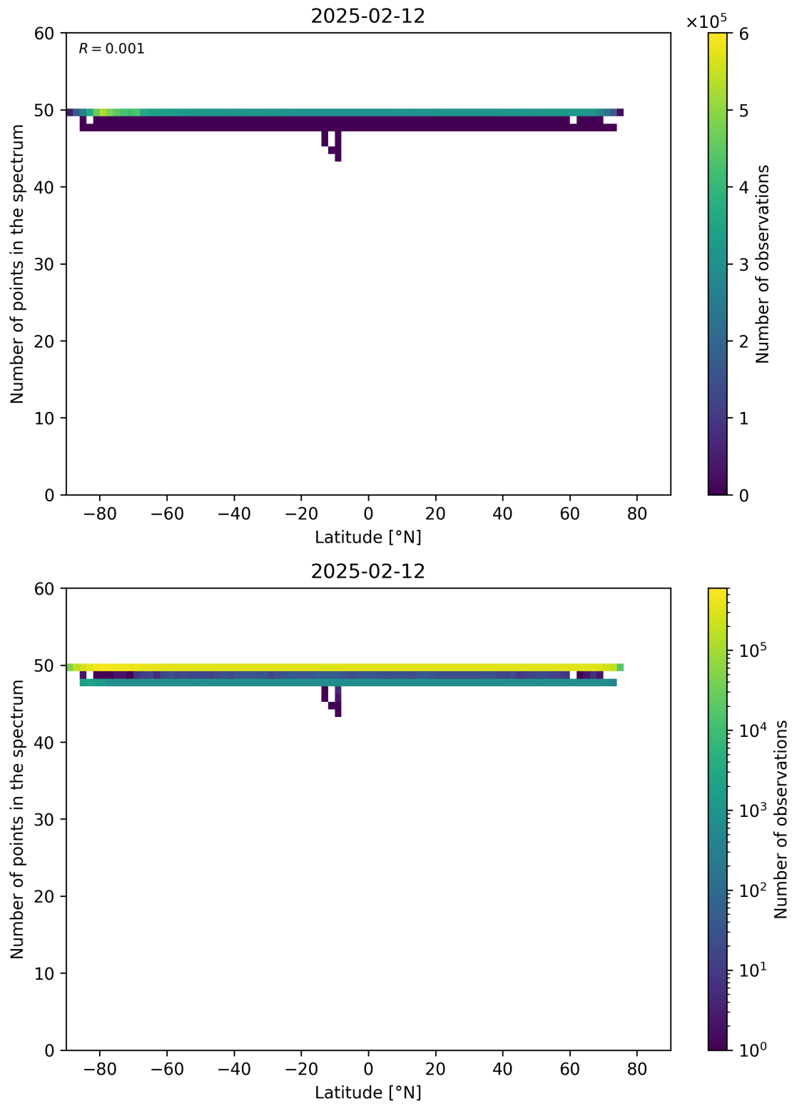
Figure 94: Scatter density plot of “Latitude” against “Number of points in the spectrum” for 2025-02-11 to 2025-02-13.
