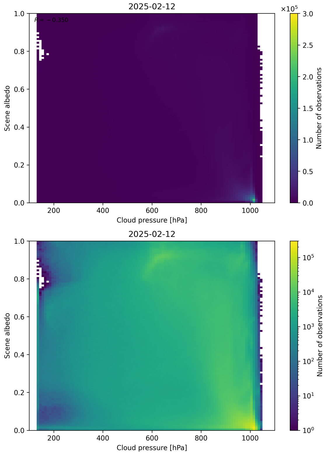
Figure 83: Scatter density plot of “Cloud pressure” against “Scene albedo” for 2025-02-11 to 2025-02-13.
