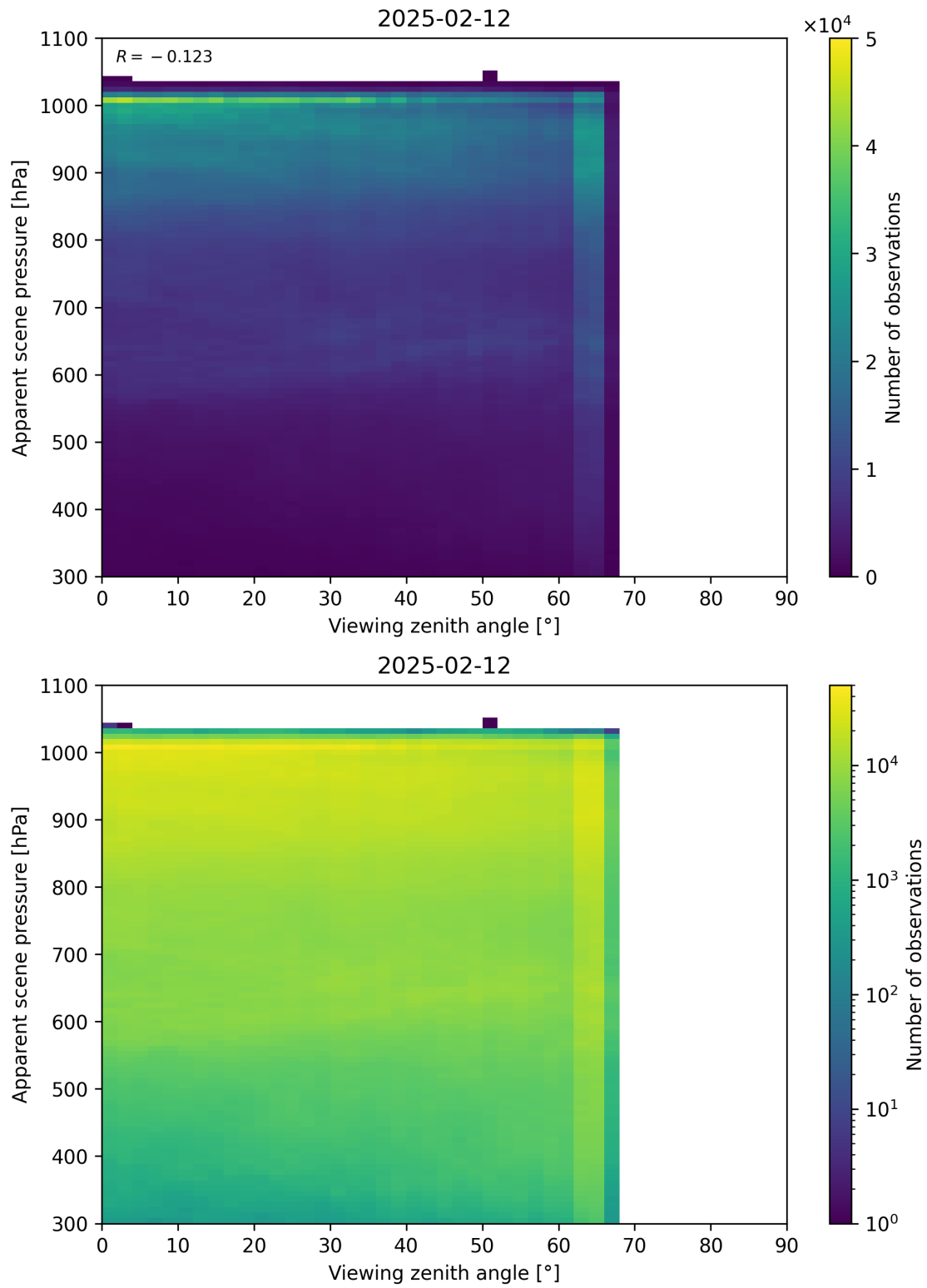
Figure 118: Scatter density plot of “Viewing zenith angle” against “Apparent scene pressure” for 2025-02-11 to 2025-02-13.
