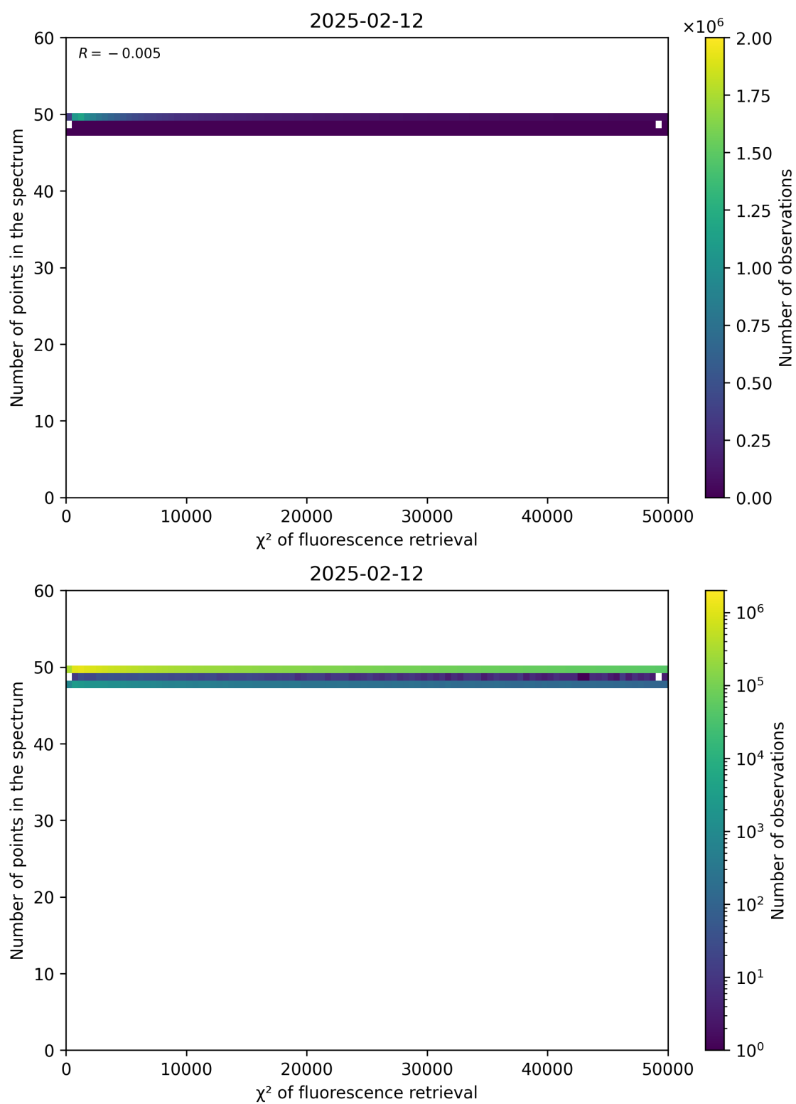
Figure 68: Scatter density plot of “ \chi^2 of fluorescence retrieval” against “Number of points in the spectrum” for 2025-02-11 to 2025-02-13.
