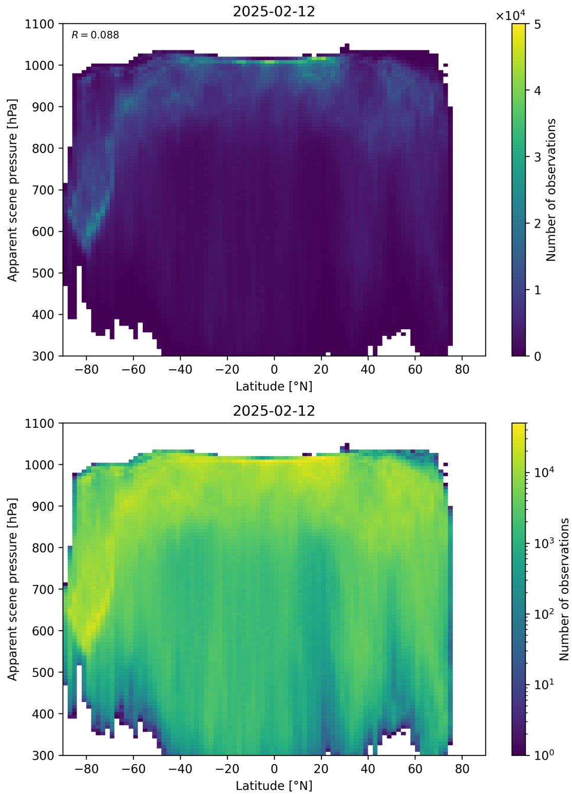
Figure 88: Scatter density plot of “Latitude” against “Apparent scene pressure” for 2025-02-11 to 2025-02-13.
