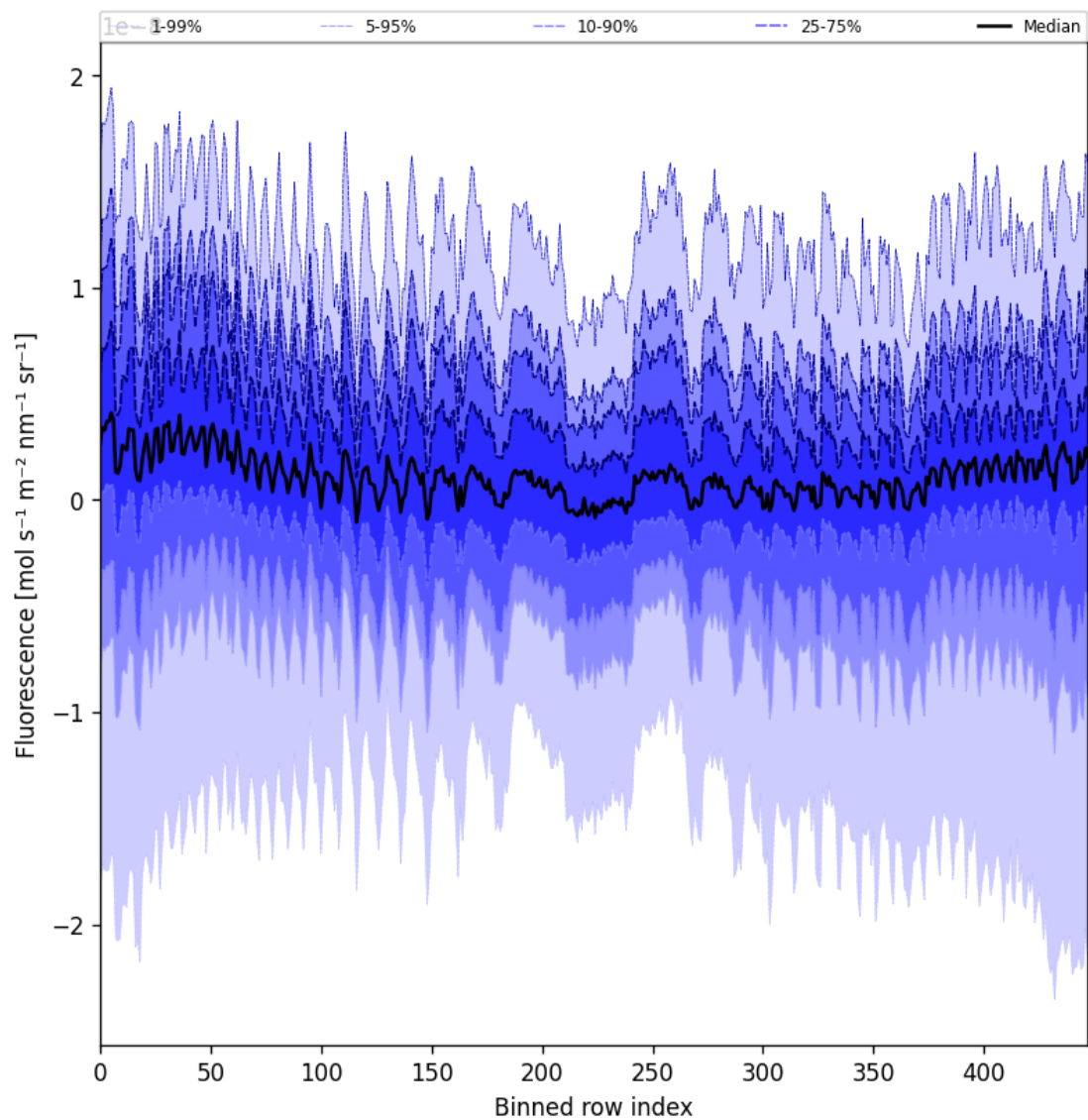
Figure 57: Along track statistics of “Fluorescence” for 2025-02-11 to 2025-02-13
