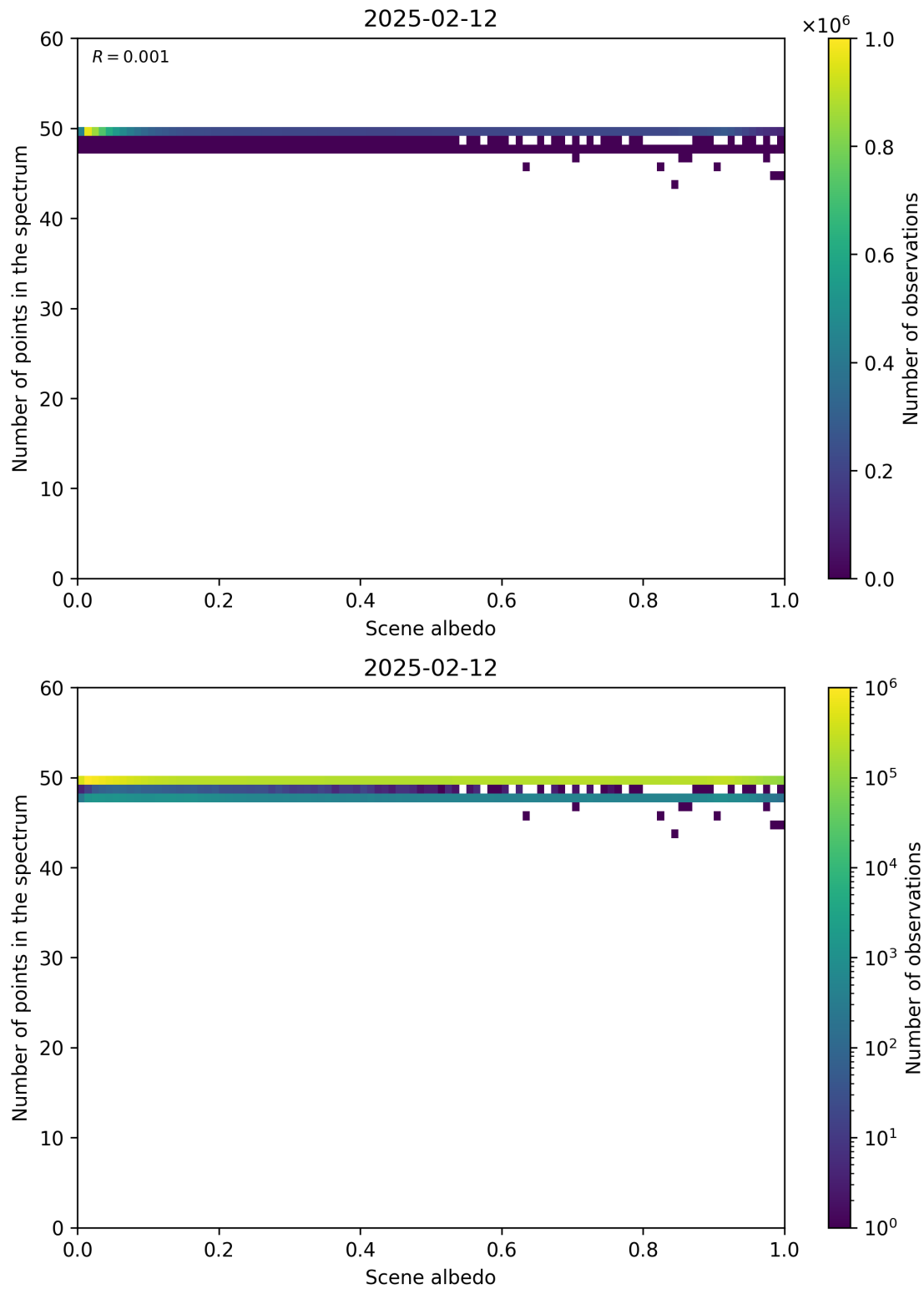
Figure 106: Scatter density plot of “Scene albedo” against “Number of points in the spectrum” for 2025-02-11 to 2025-02-13.
