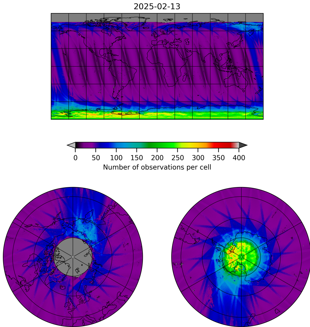
Figure 11: Map of the number of observations for 2025-02-13 to 2025-02-14
