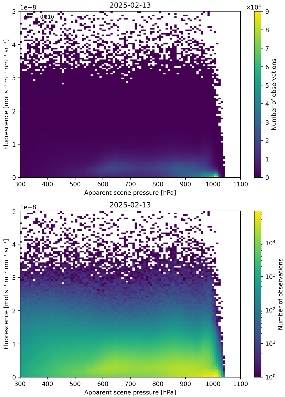
Figure 64: Scatter density plot of “Apparent scene pressure” against “Fluorescence” for 2025-02-13 to 2025-02-14.
