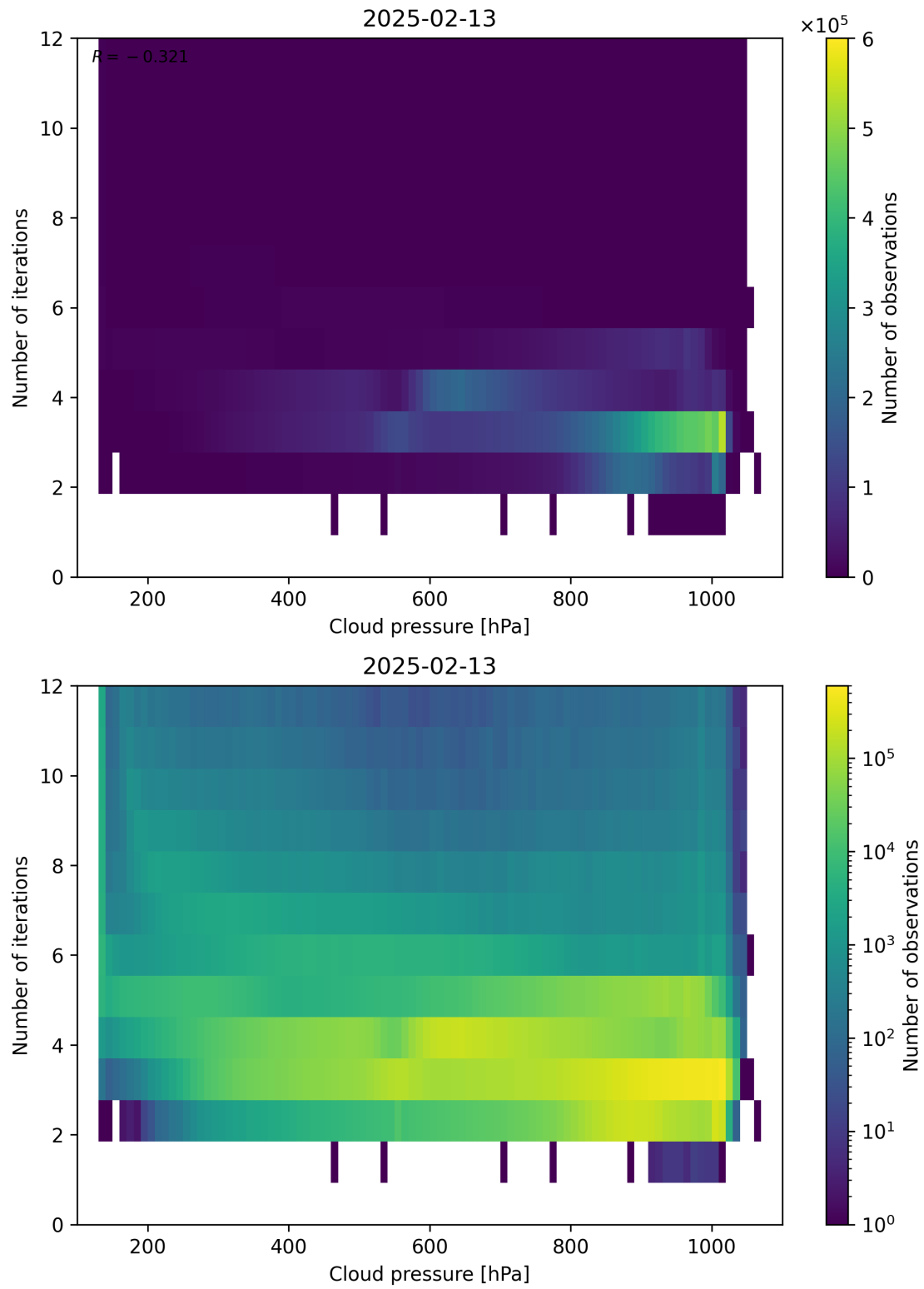
Figure 81: Scatter density plot of “Cloud pressure” against “Number of iterations” for 2025-02-13 to 2025-02-14.
