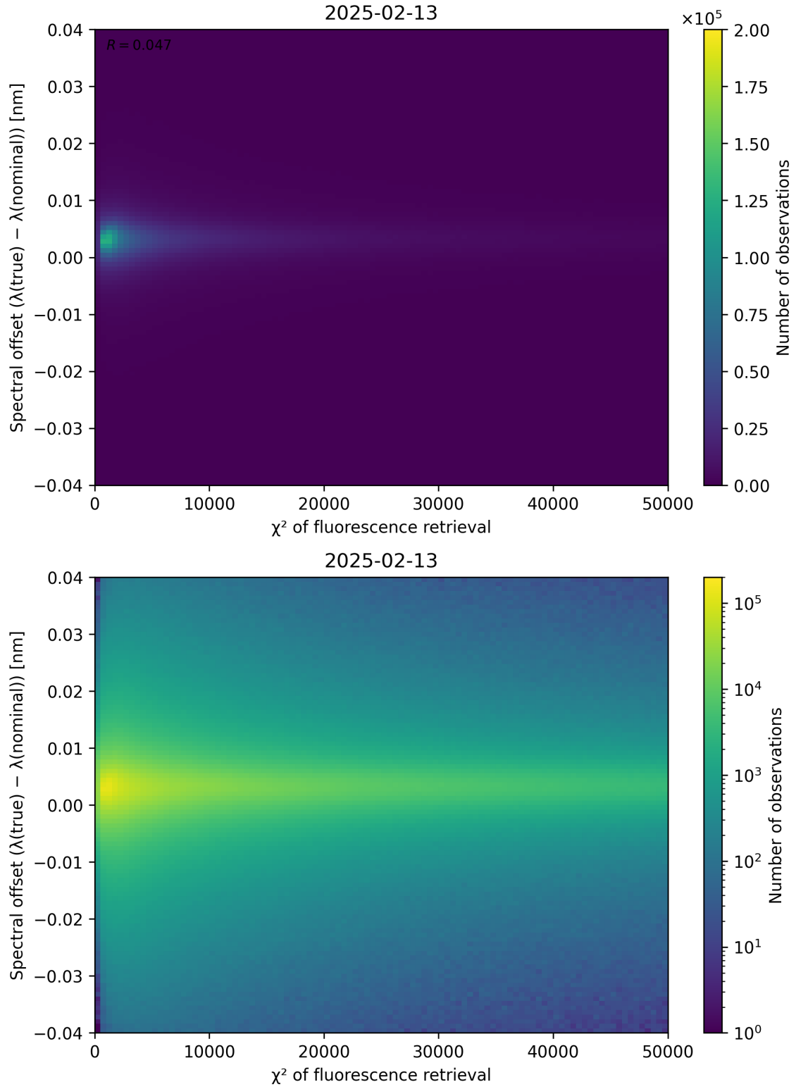
Figure 69: Scatter density plot of “ \chi^2 of fluorescence retrieval” against “Spectral offset ( \lambda_{\text{true}} - \lambda_{\text{nominal}} )” for 2025-02-13 to 2025-02-14.
