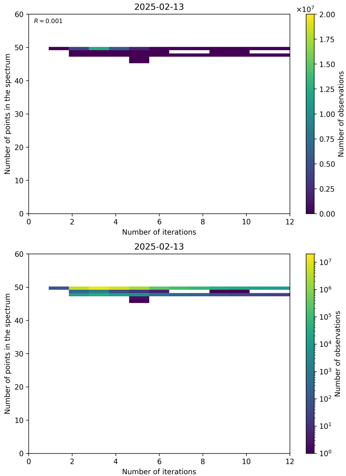
Figure 99: Scatter density plot of “Number of iterations” against “Number of points in the spectrum” for 2025-02-13 to 2025-02-14.
