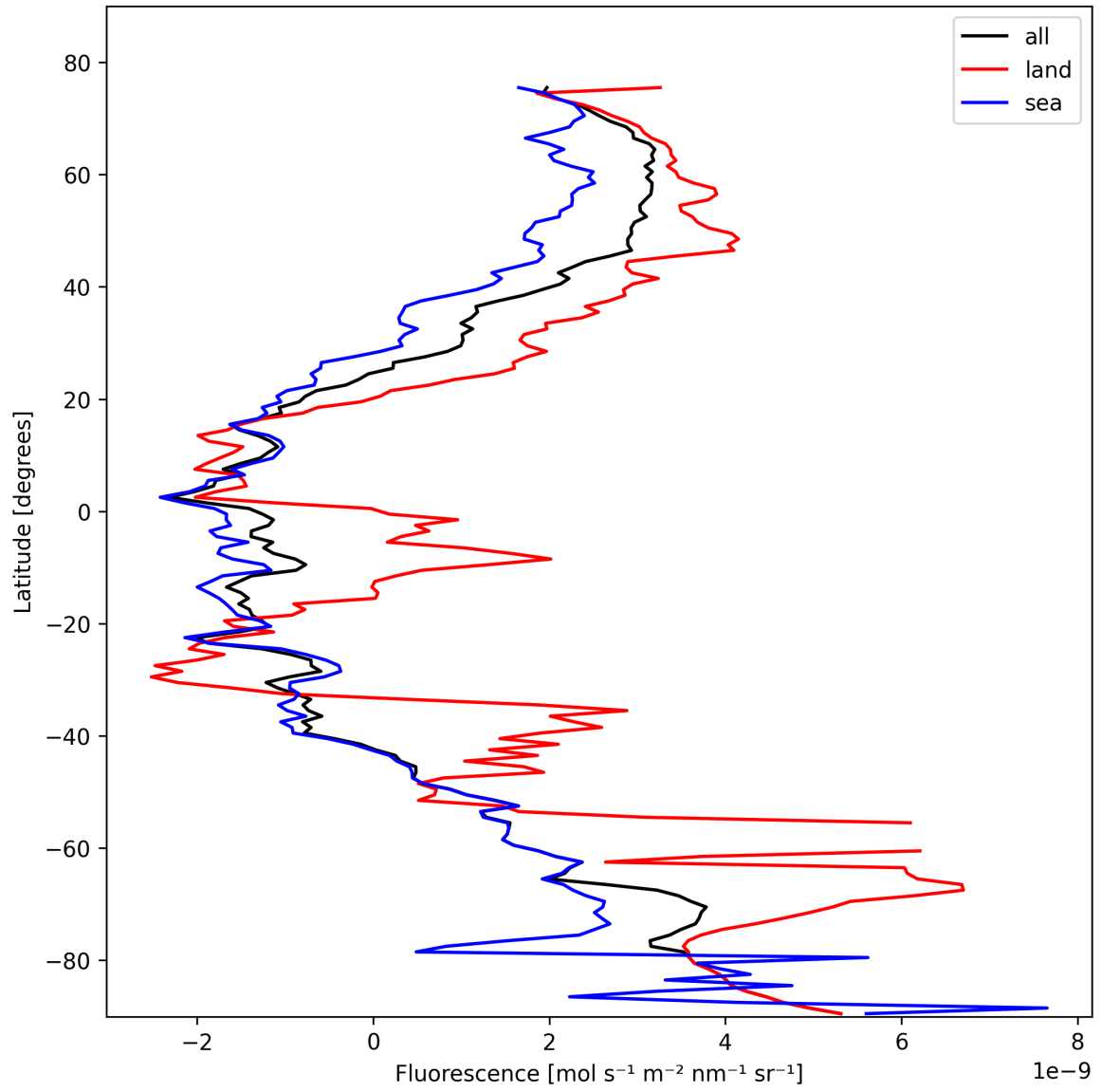
Figure 23: Zonal average of “Fluorescence” for 2025-02-13 to 2025-02-14.
