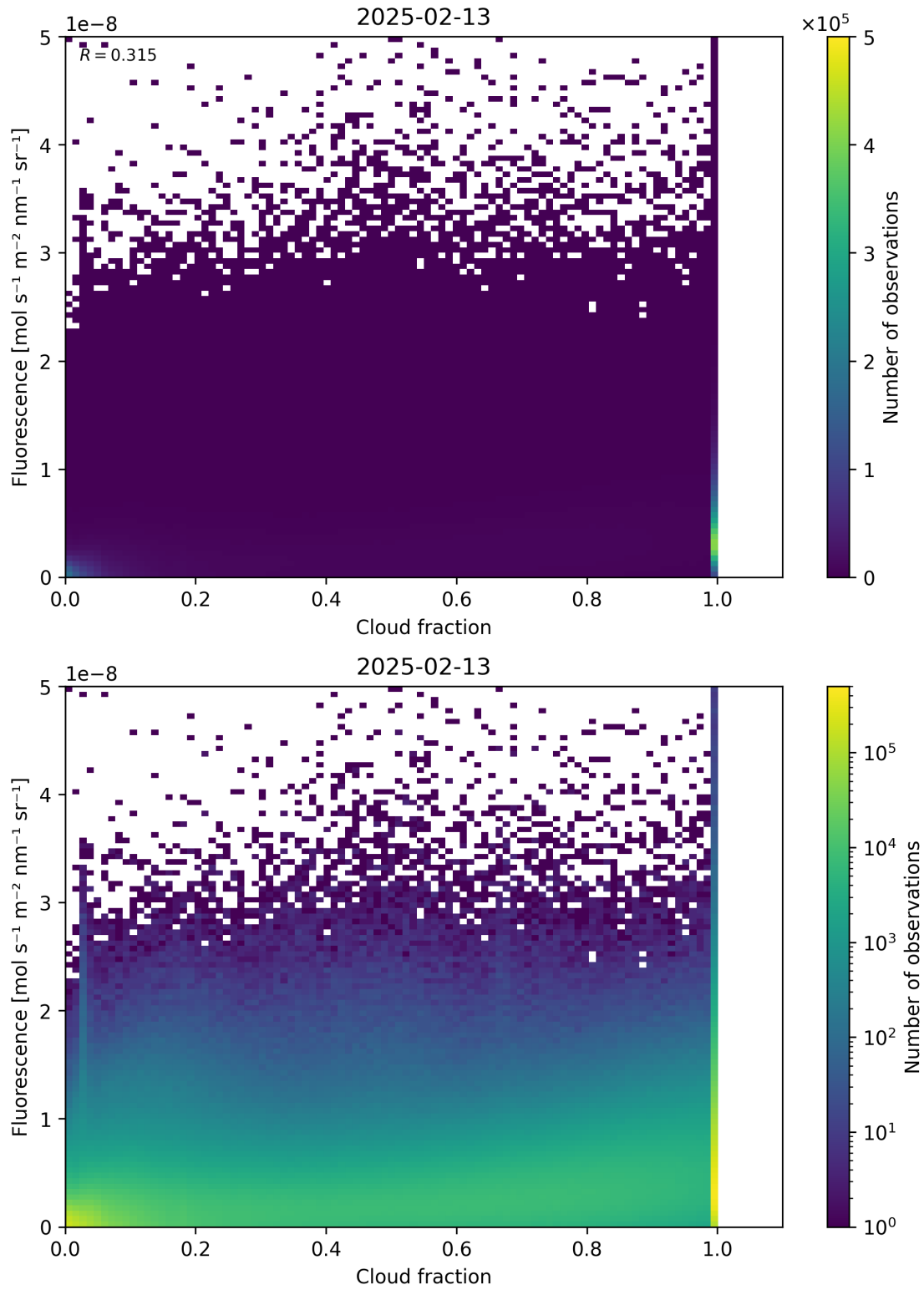
Figure 72: Scatter density plot of “Cloud fraction” against “Fluorescence” for 2025-02-13 to 2025-02-14.
