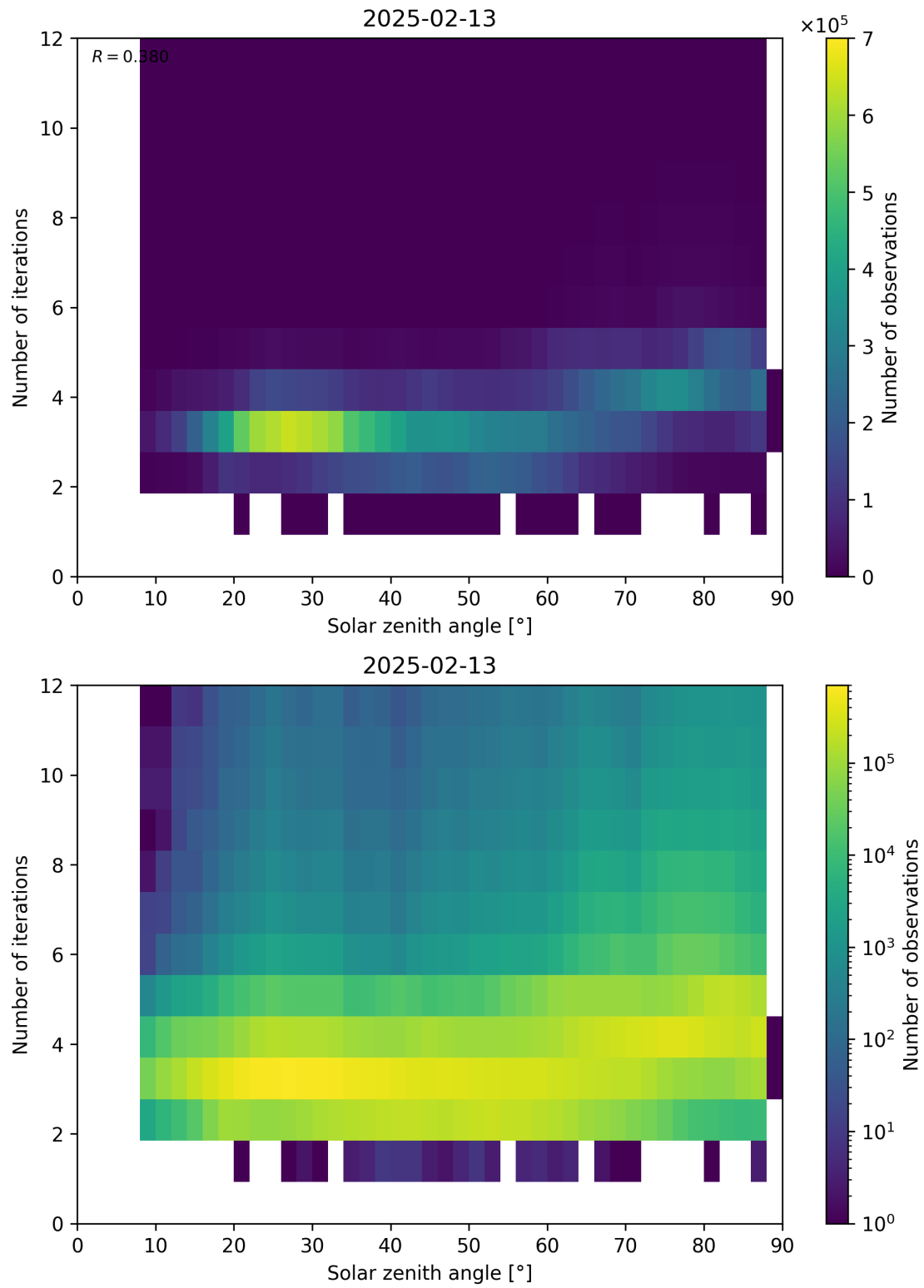
Figure 114: Scatter density plot of “Solar zenith angle” against “Number of iterations” for 2025-02-13 to 2025-02-14.
