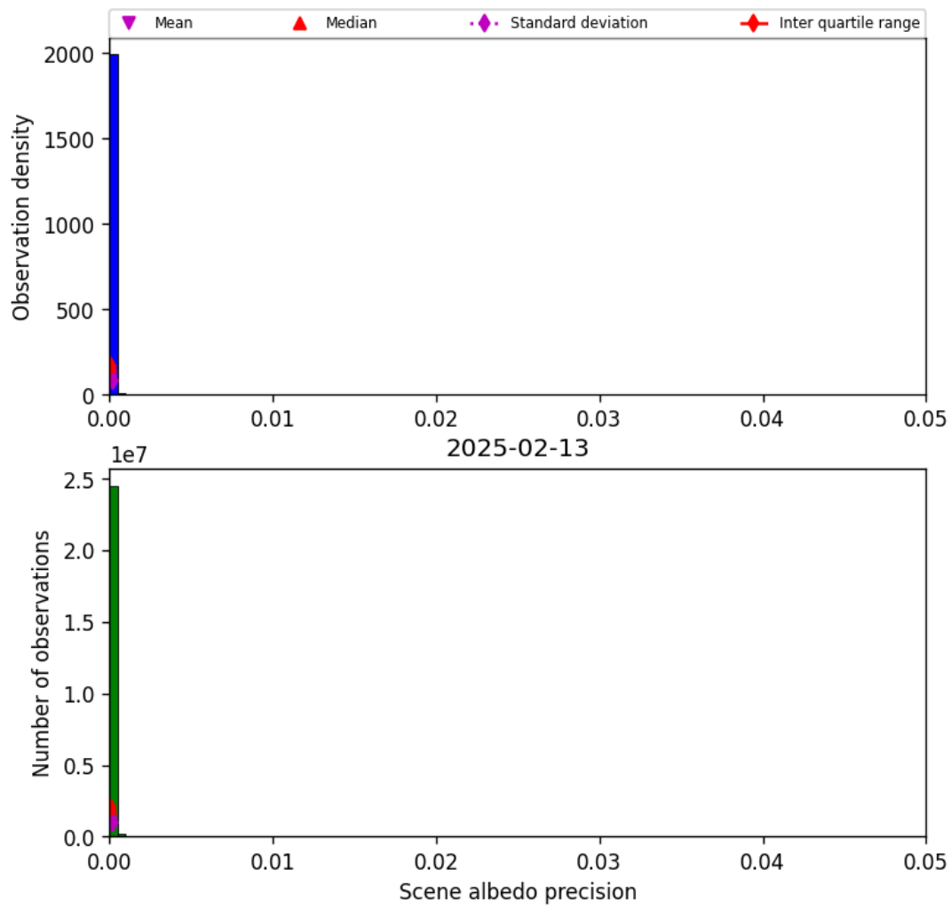
Figure 35: Histogram of “Scene albedo precision” for 2025-02-13 to 2025-02-14
