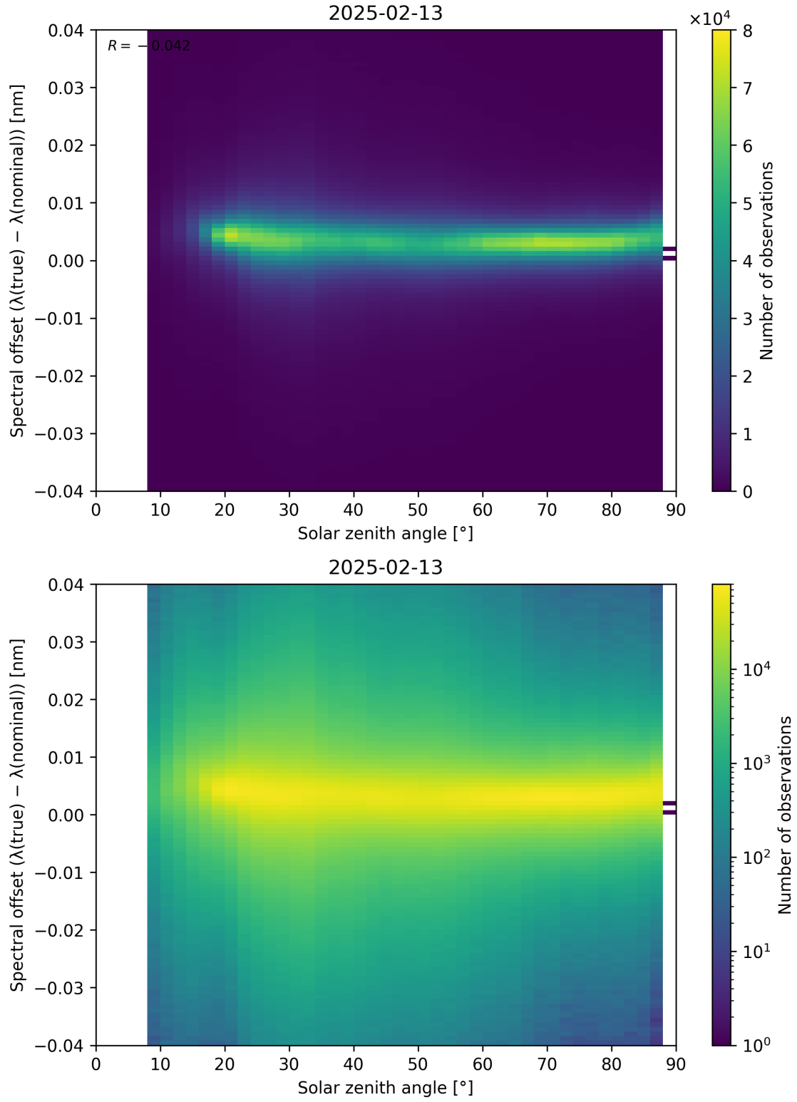
Figure 117: Scatter density plot of “Solar zenith angle” against “Spectral offset ( \lambda_{\text{true}} - \lambda_{\text{nominal}} )” for 2025-02-13 to 2025-02-14.
