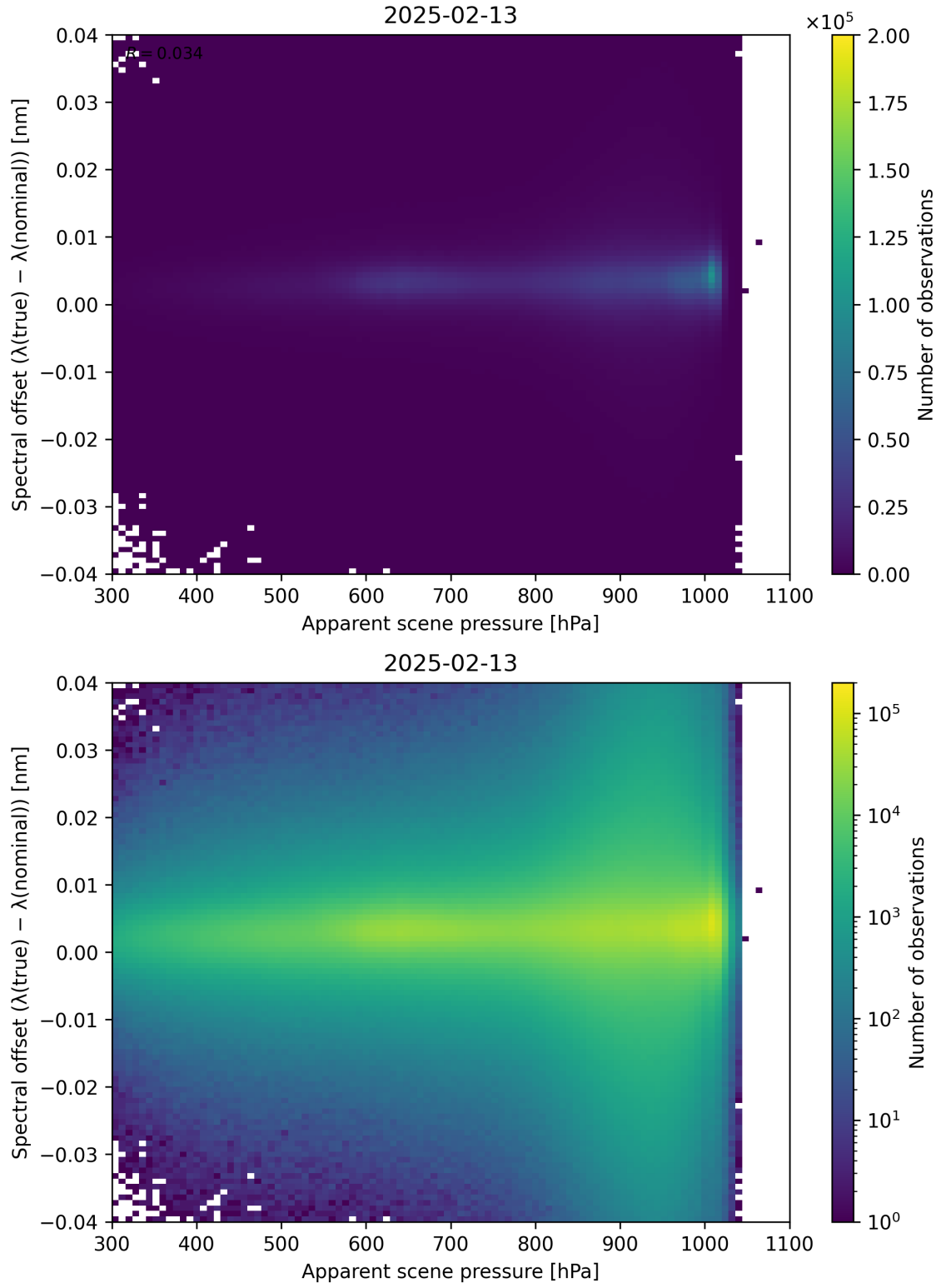
Figure 67: Scatter density plot of “Apparent scene pressure” against “Spectral offset ( \lambda_{\text{true}} - \lambda_{\text{nominal}} )” for 2025-02-13 to 2025-02-14.
