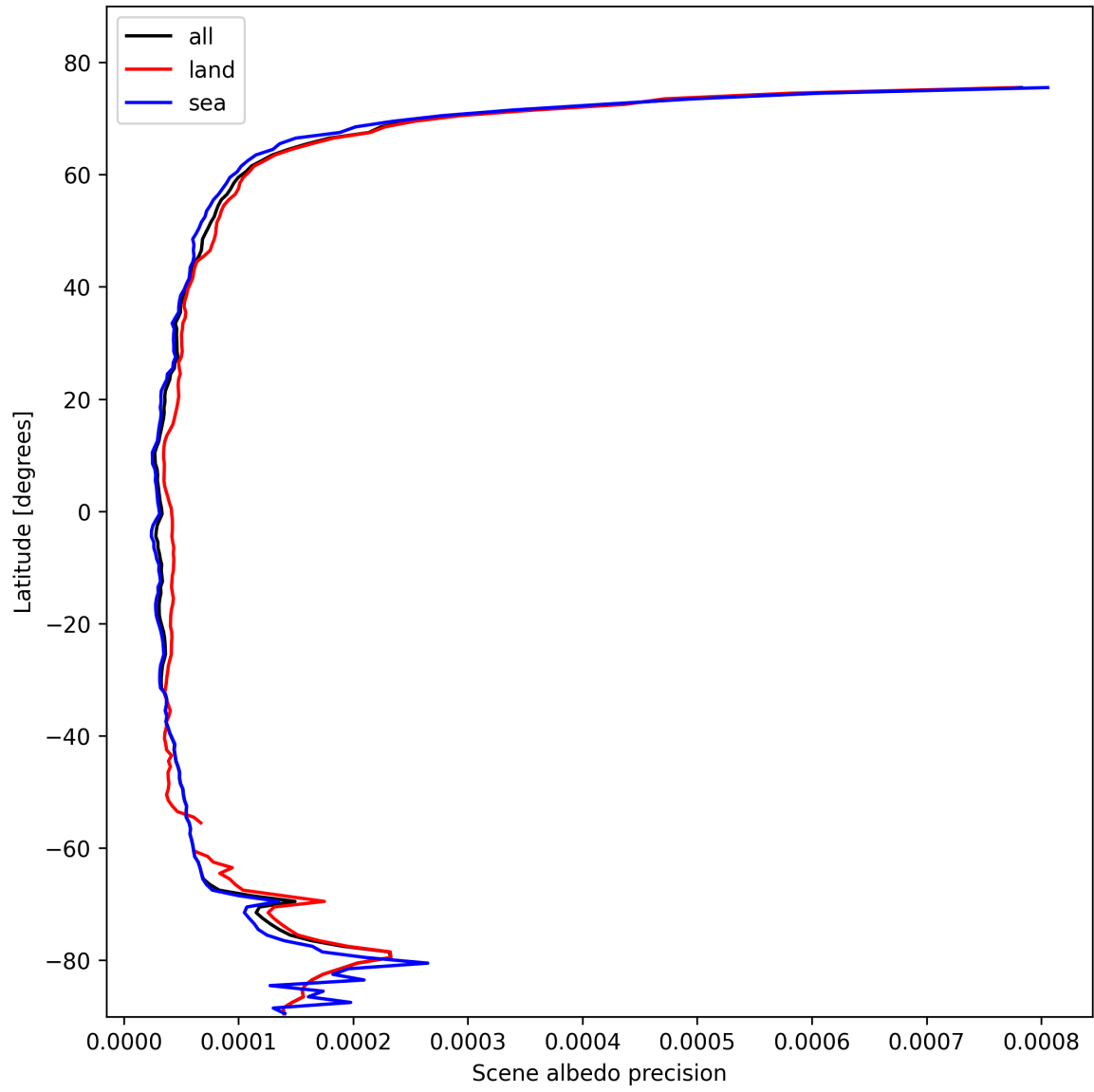
Figure 18: Zonal average of “Scene albedo precision” for 2025-02-13 to 2025-02-14.
