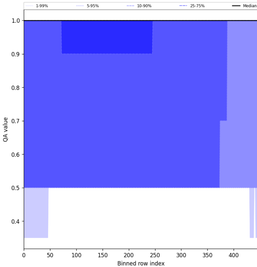
Figure 46: Along track statistics of “QA value” for 2025-02-13 to 2025-02-14
