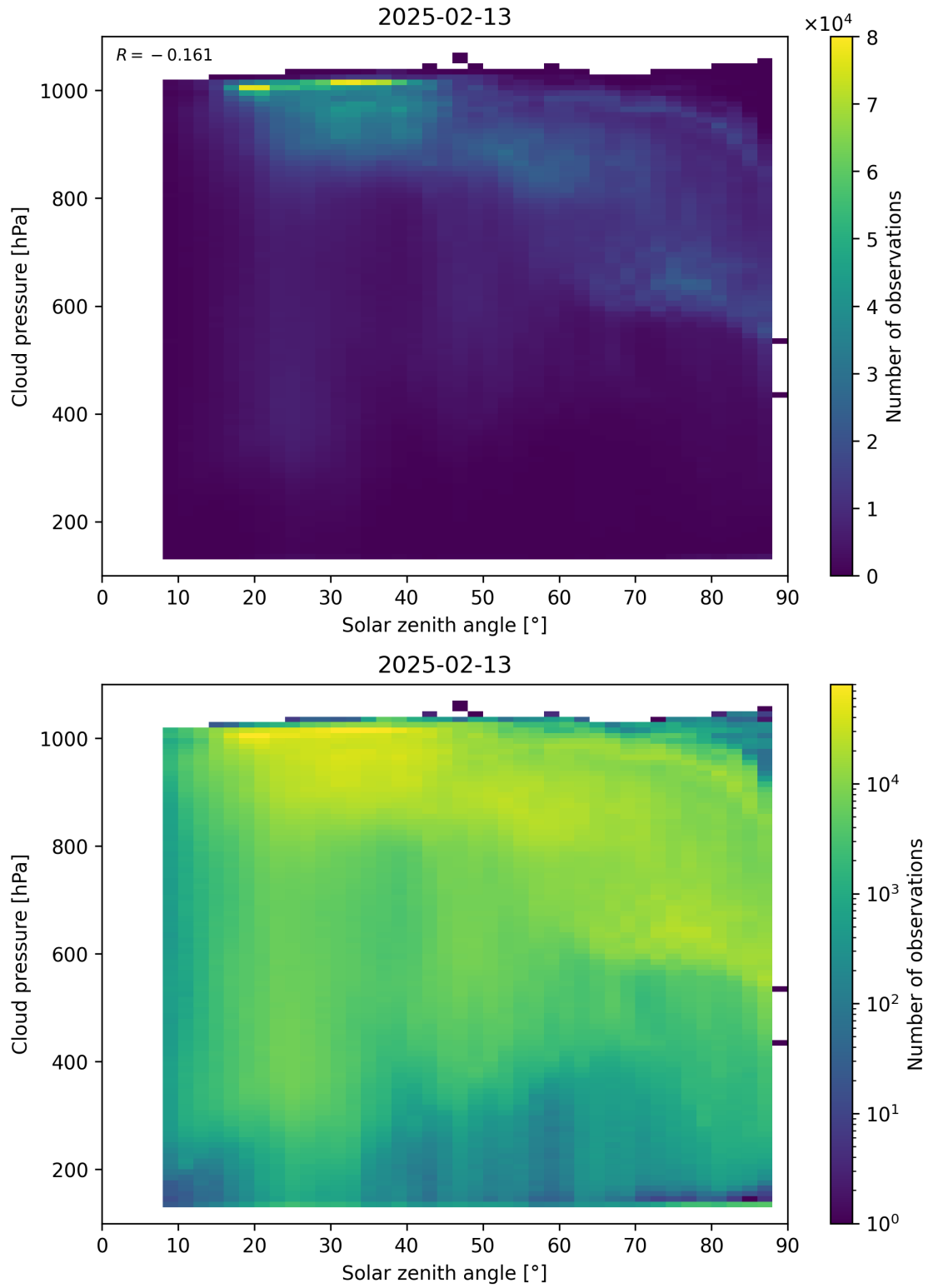
Figure 111: Scatter density plot of “Solar zenith angle” against “Cloud pressure” for 2025-02-13 to 2025-02-14.
