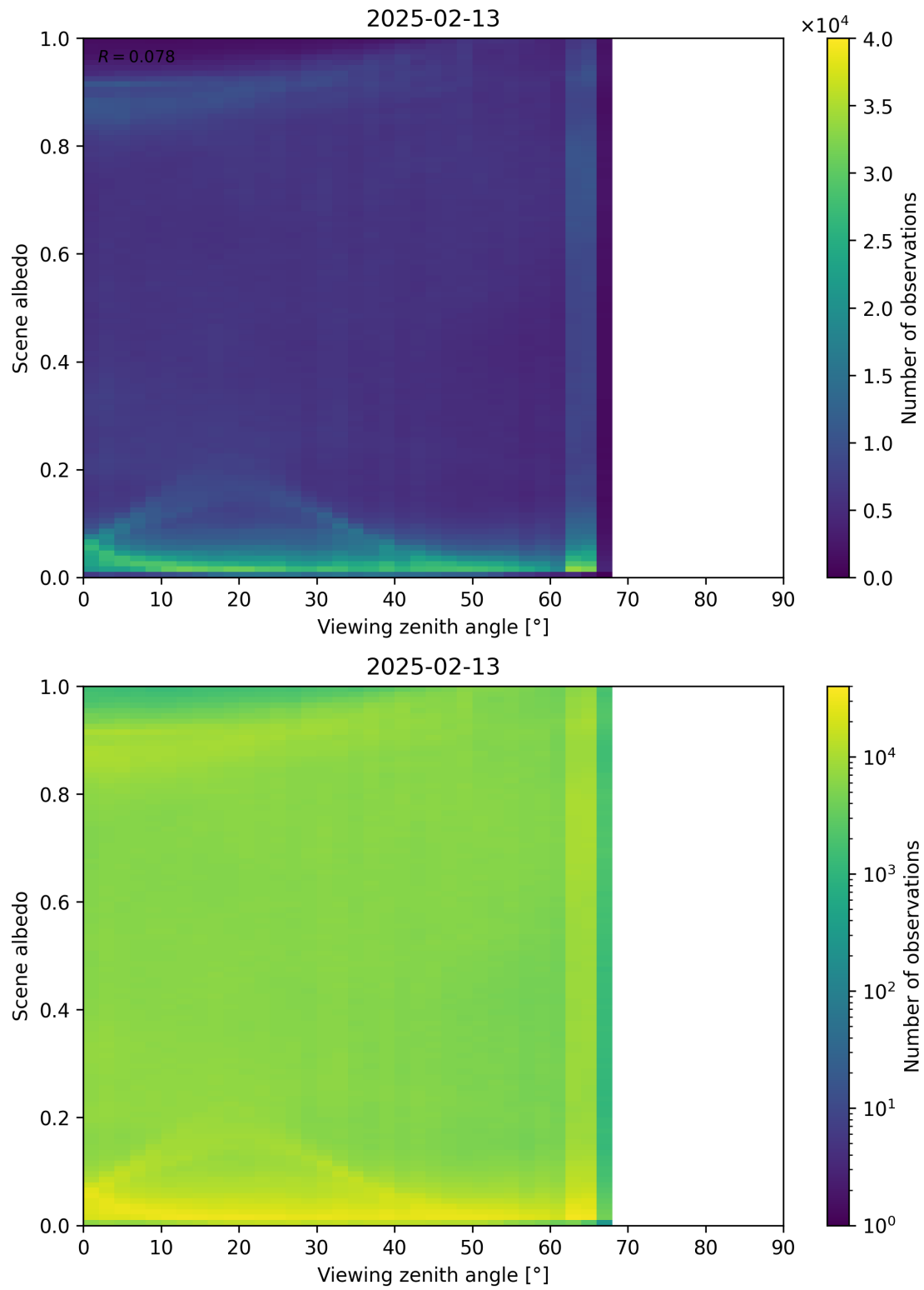
Figure 126: Scatter density plot of “Viewing zenith angle” against “Scene albedo” for 2025-02-13 to 2025-02-14.
