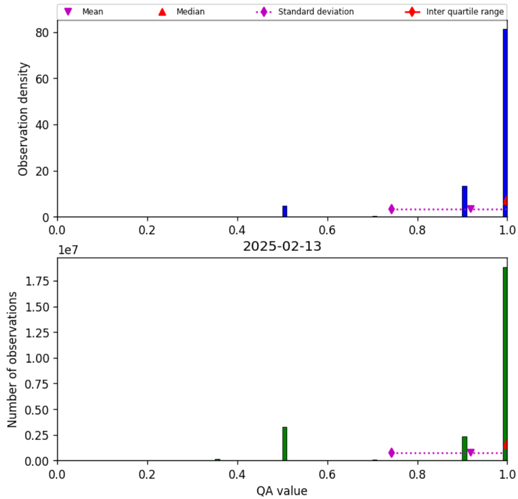
Figure 29: Histogram of “QA value” for 2025-02-13 to 2025-02-14
