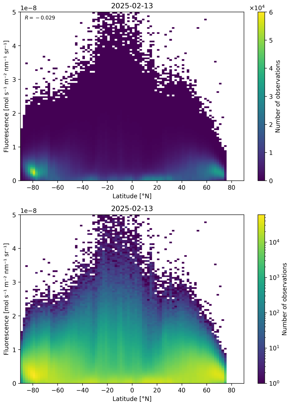
Figure 92: Scatter density plot of “Latitude” against “Fluorescence” for 2025-02-13 to 2025-02-14.
