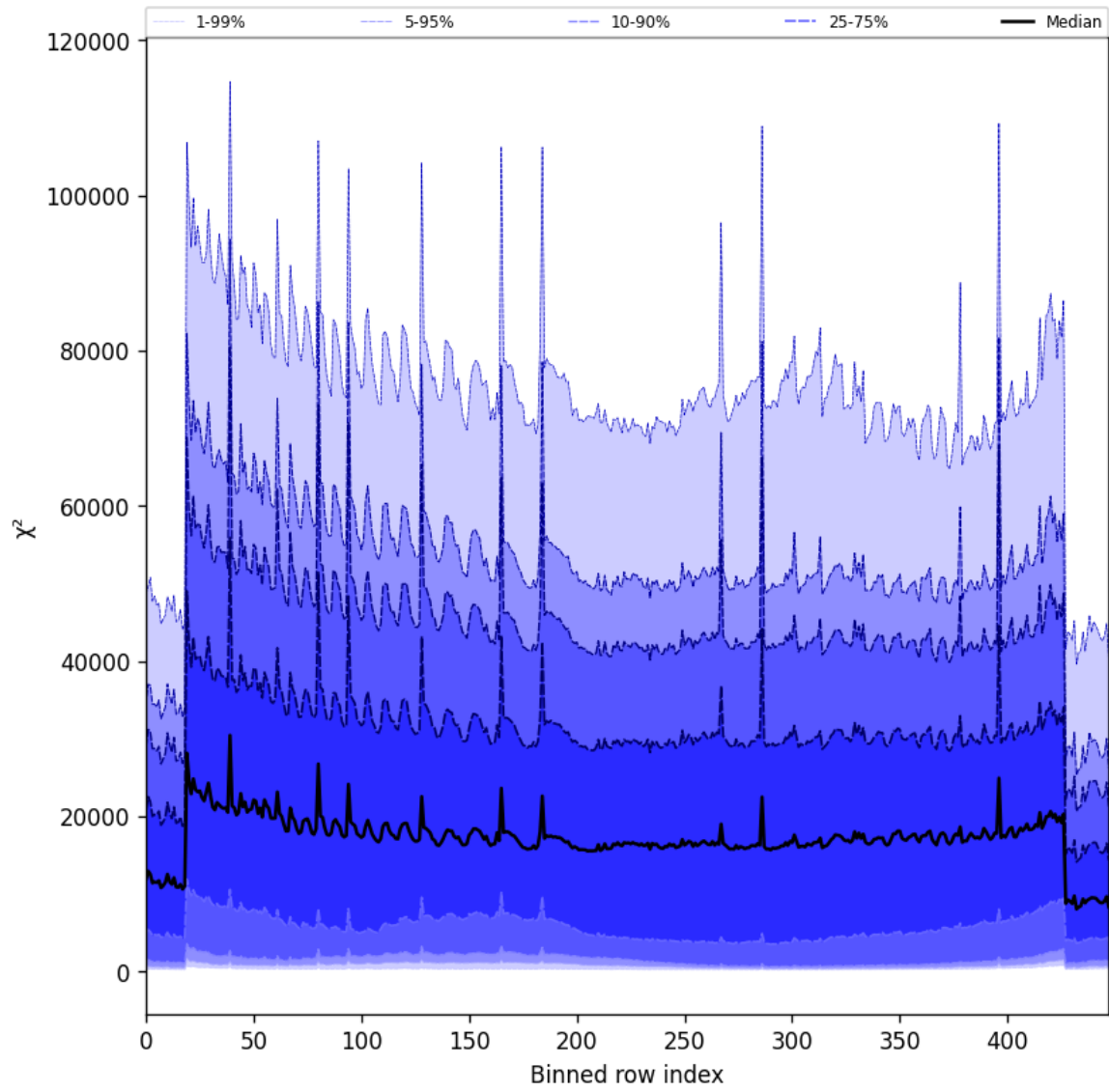
Figure 55: Along track statistics of “ \chi^2 ” for 2025-02-13 to 2025-02-14
