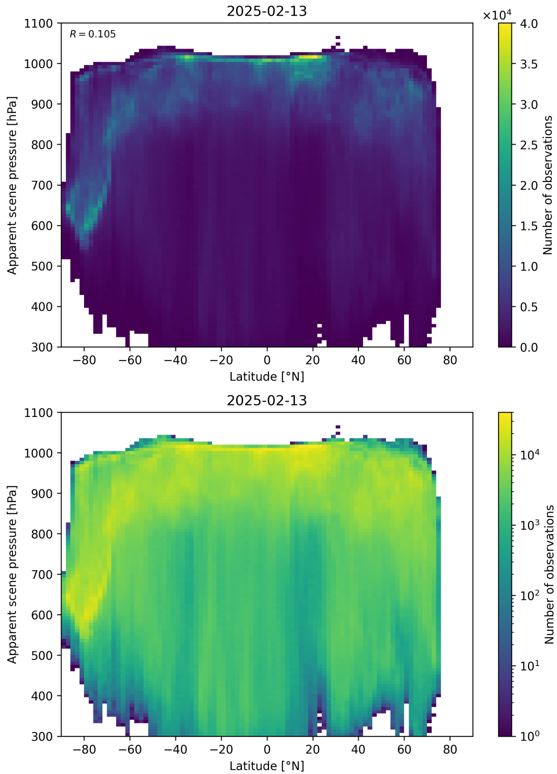
Figure 88: Scatter density plot of “Latitude” against “Apparent scene pressure” for 2025-02-13 to 2025-02-14.
