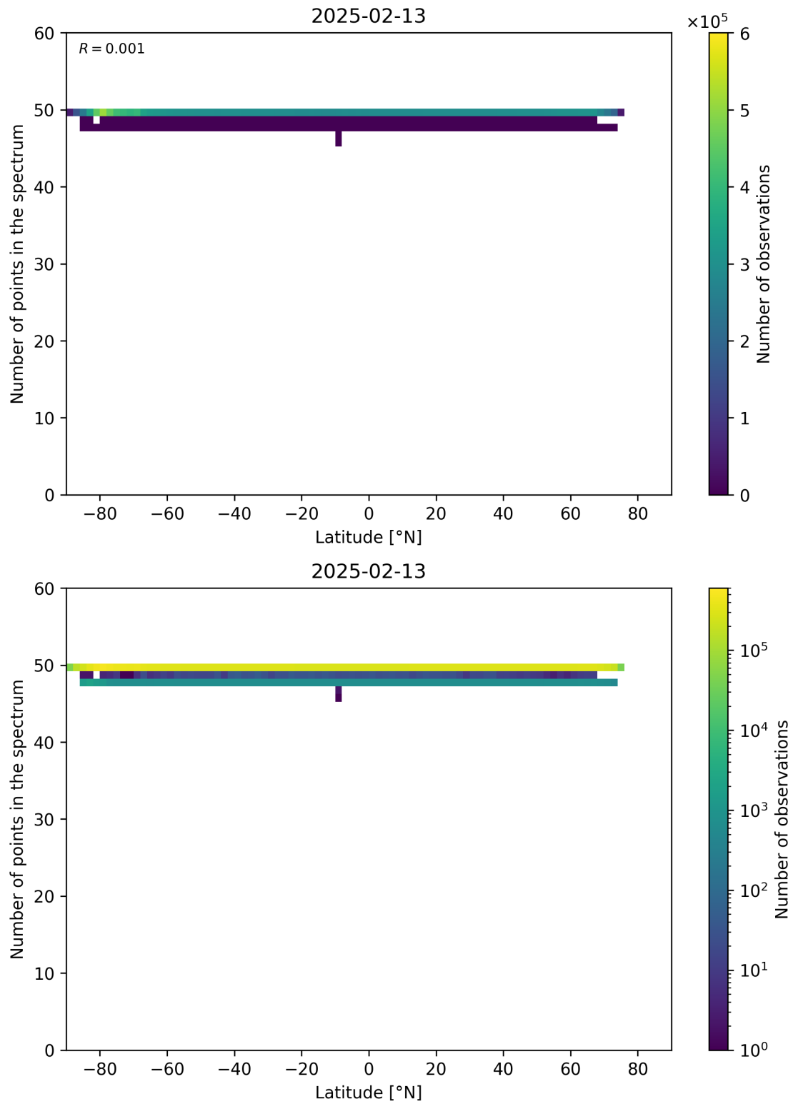
Figure 94: Scatter density plot of “Latitude” against “Number of points in the spectrum” for 2025-02-13 to 2025-02-14.
