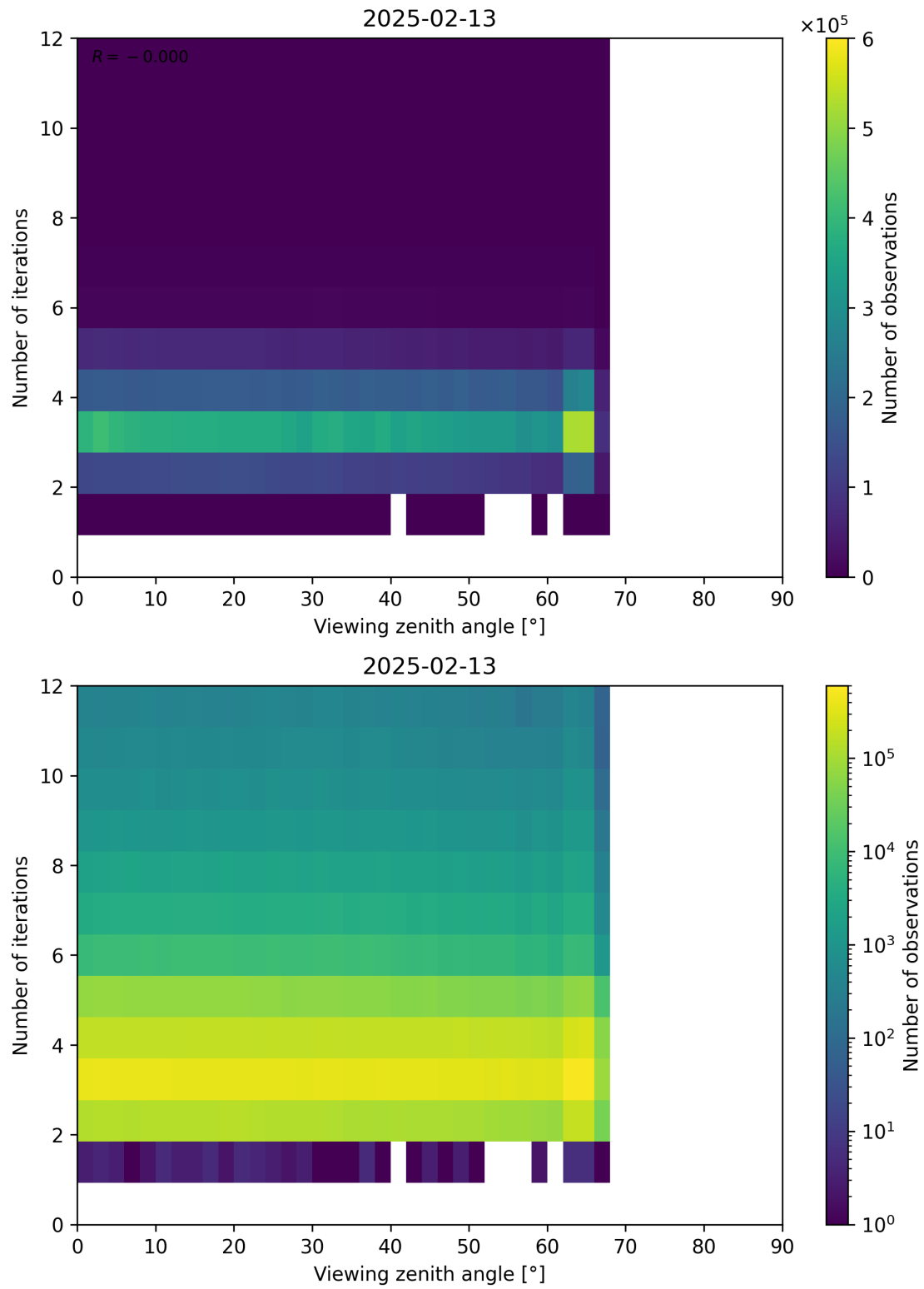
Figure 124: Scatter density plot of “Viewing zenith angle” against “Number of iterations” for 2025-02-13 to 2025-02-14.
