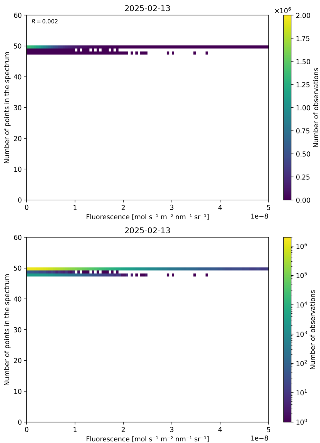
Figure 86: Scatter density plot of “Fluorescence” against “Number of points in the spectrum” for 2025-02-13 to 2025-02-14.
