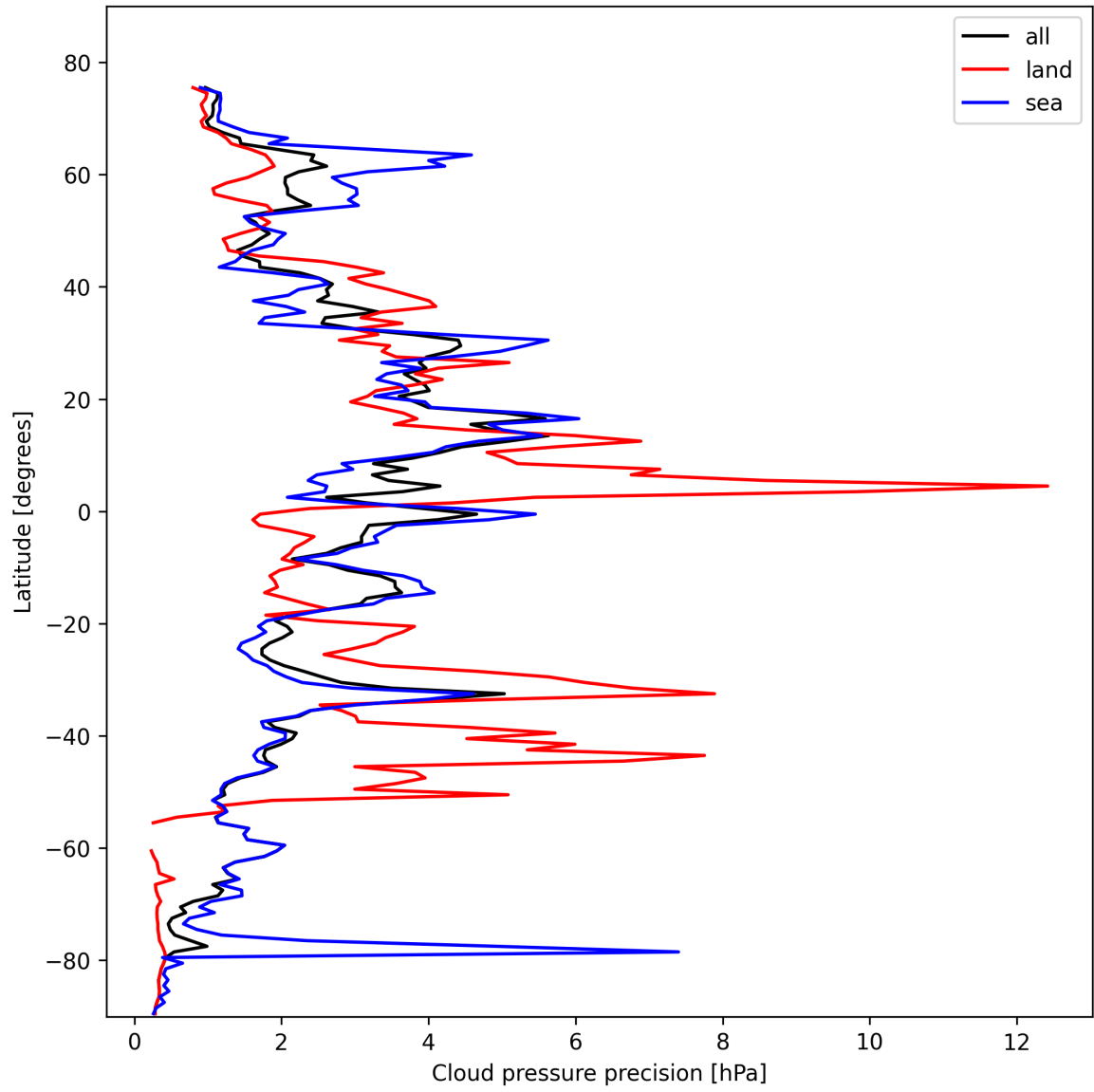
Figure 14: Zonal average of “Cloud pressure precision” for 2025-02-13 to 2025-02-14.
