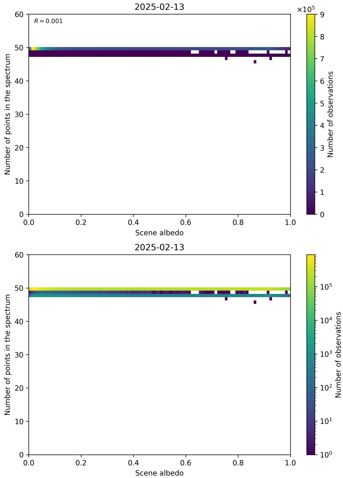
Figure 106: Scatter density plot of “Scene albedo” against “Number of points in the spectrum” for 2025-02-13 to 2025-02-14.
