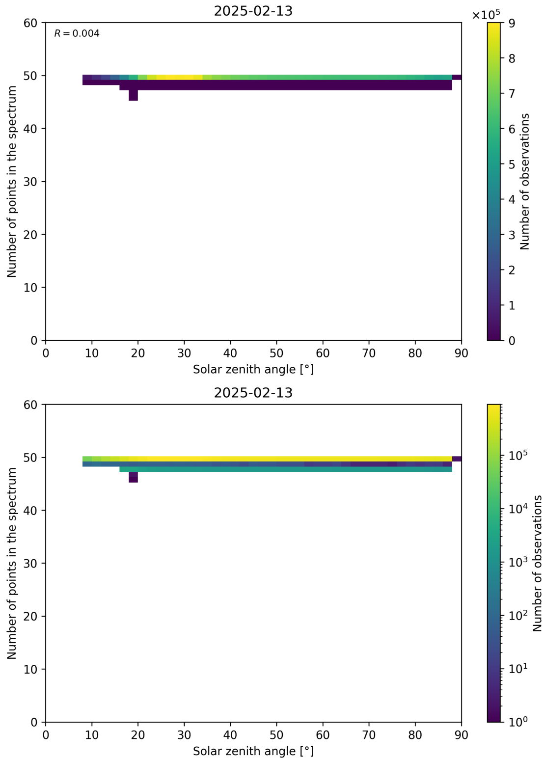
Figure 115: Scatter density plot of “Solar zenith angle” against “Number of points in the spectrum” for 2025-02-13 to 2025-02-14.
