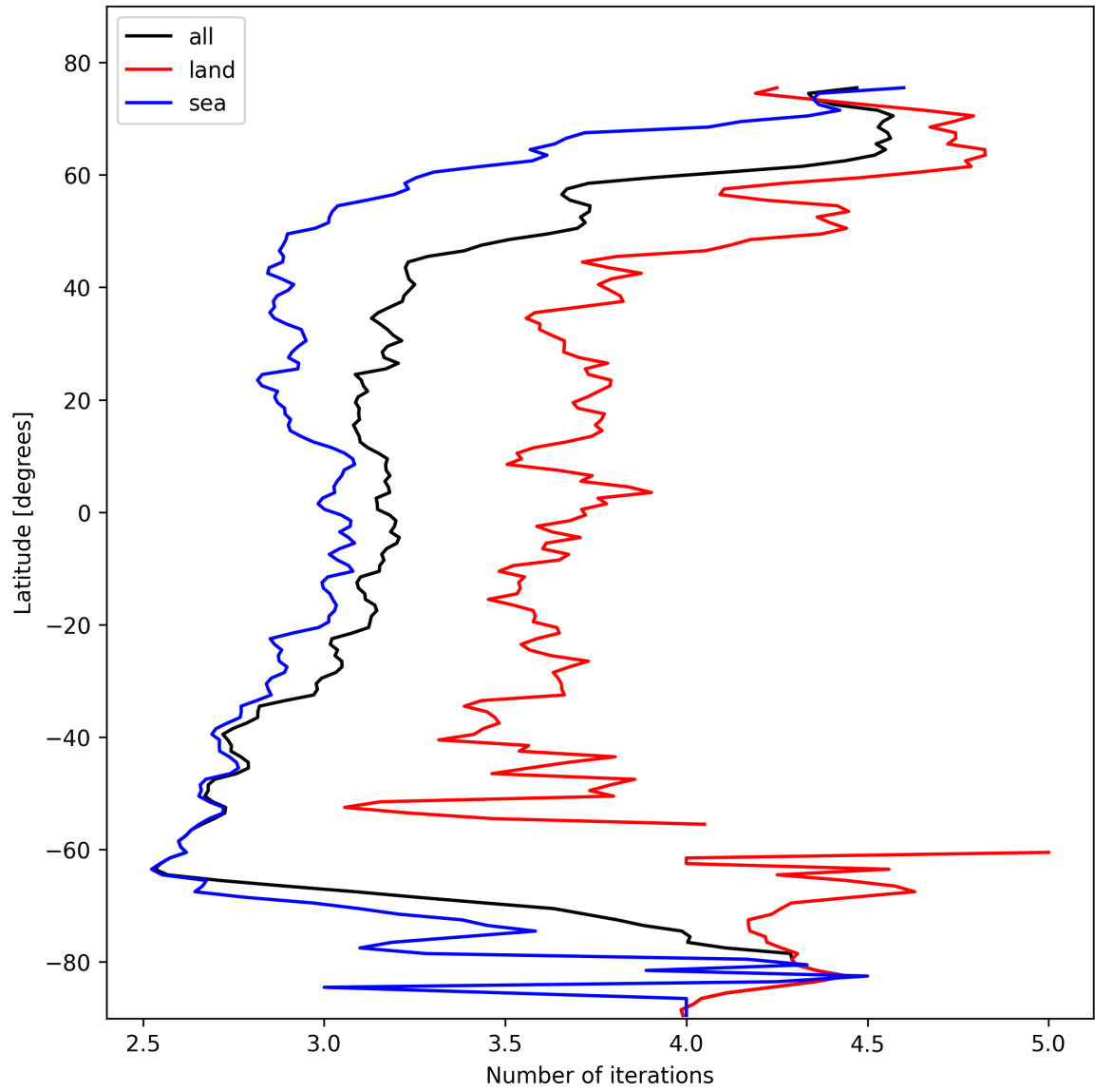
Figure 22: Zonal average of “Number of iterations” for 2025-02-13 to 2025-02-14.
