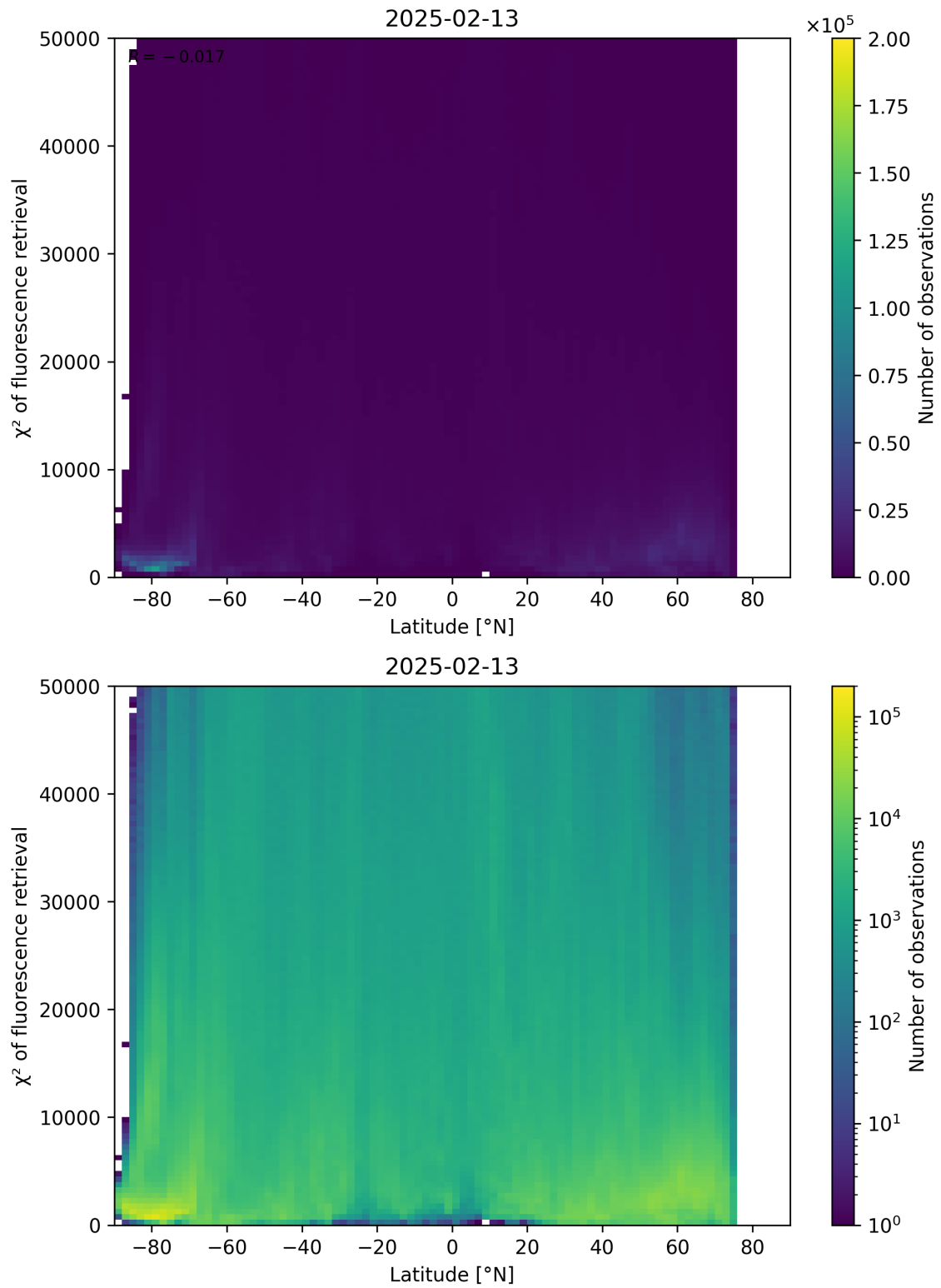
Figure 89: Scatter density plot of “Latitude” against “ \chi^2 of fluorescence retrieval” for 2025-02-13 to 2025-02-14.
