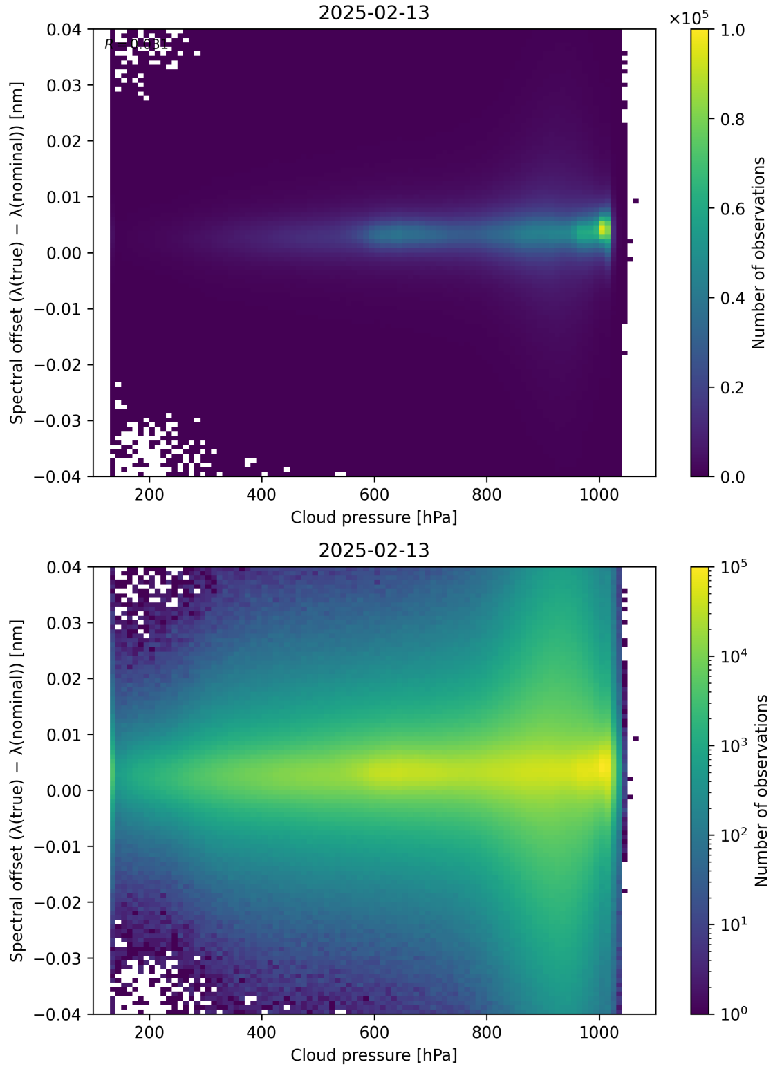
Figure 84: Scatter density plot of “Cloud pressure” against “Spectral offset ( \lambda_{\text{true}} - \lambda_{\text{nominal}} )” for 2025-02-13 to 2025-02-14.
