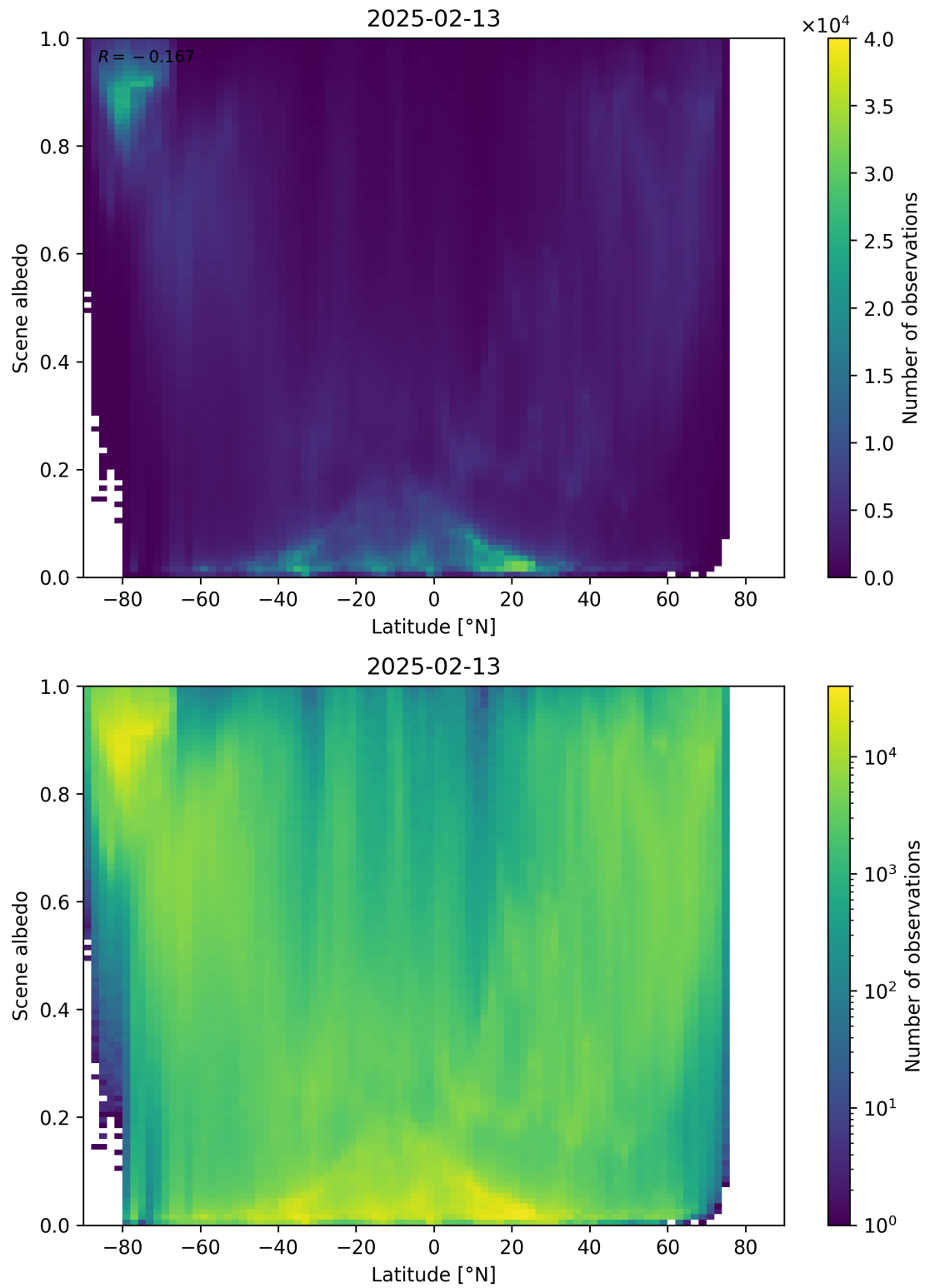
Figure 95: Scatter density plot of “Latitude” against “Scene albedo” for 2025-02-13 to 2025-02-14.
