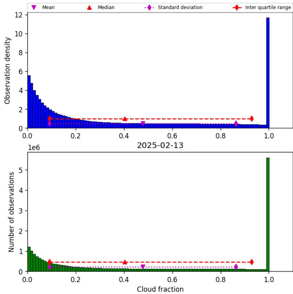
Figure 32: Histogram of “Cloud fraction” for 2025-02-13 to 2025-02-14
