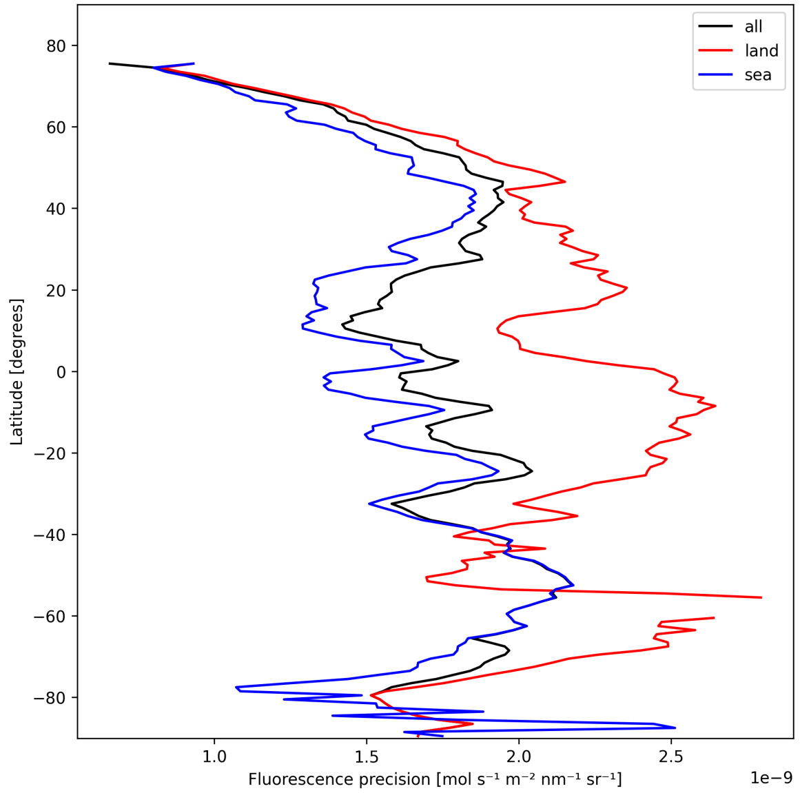
Figure 24: Zonal average of “Fluorescence precision” for 2025-02-13 to 2025-02-14.
