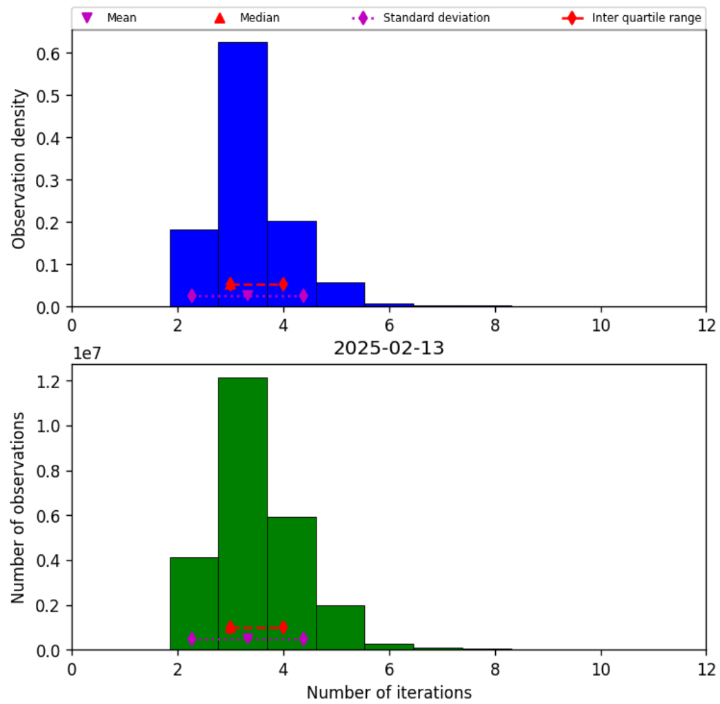
Figure 39: Histogram of “Number of iterations” for 2025-02-13 to 2025-02-14
