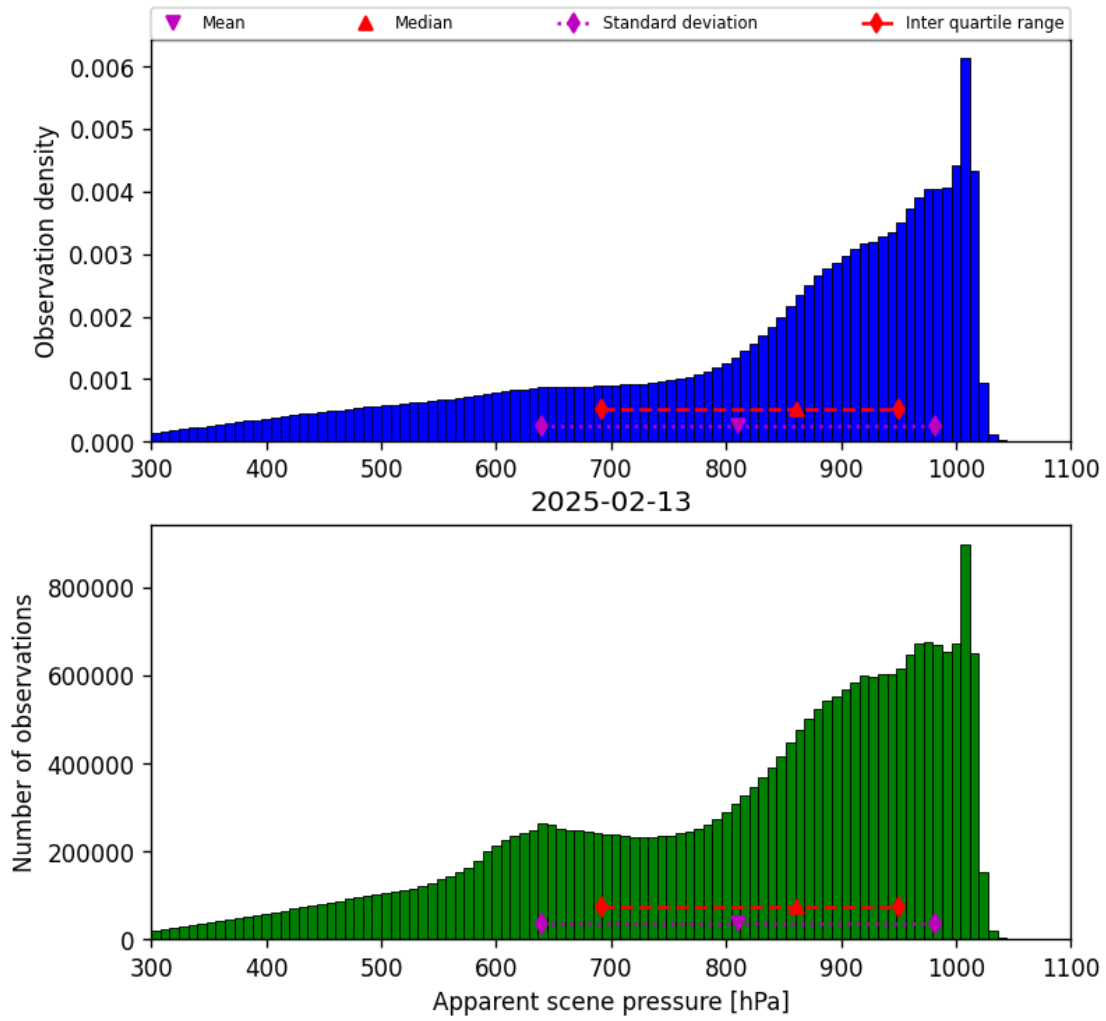
Figure 36: Histogram of “Apparent scene pressure” for 2025-02-13 to 2025-02-14
