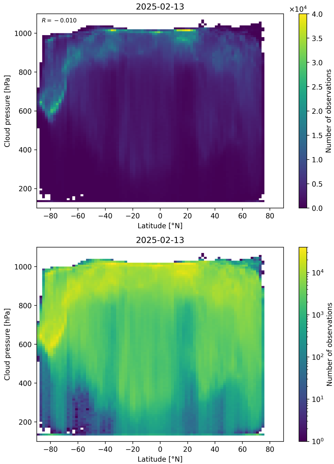
Figure 91: Scatter density plot of “Latitude” against “Cloud pressure” for 2025-02-13 to 2025-02-14.
