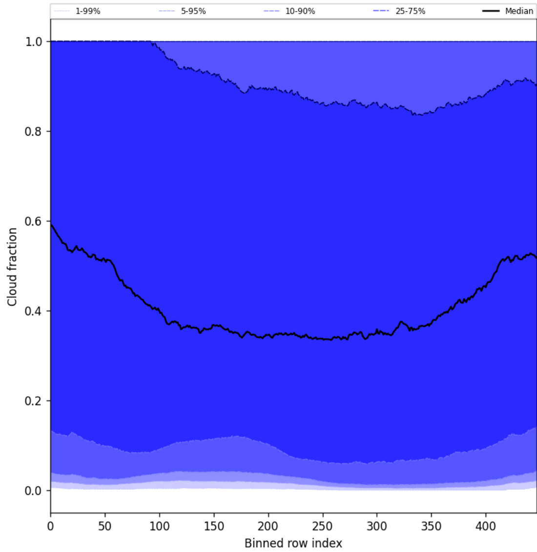
Figure 49: Along track statistics of “Cloud fraction” for 2025-02-13 to 2025-02-14
