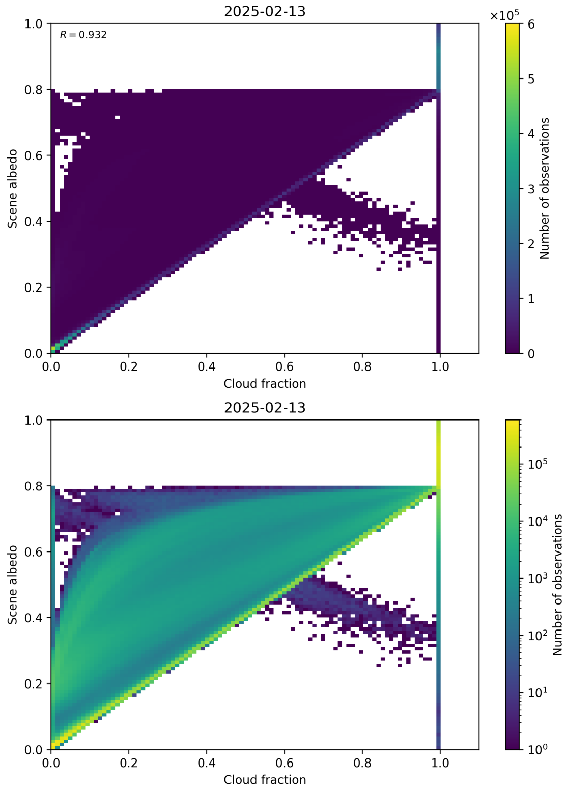
Figure 75: Scatter density plot of “Cloud fraction” against “Scene albedo” for 2025-02-13 to 2025-02-14.
