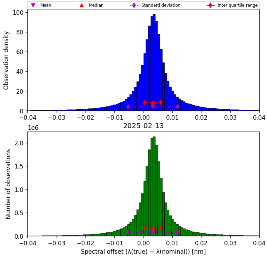
Figure 45: Histogram of “Spectral offset ( \lambda_{\text{true}} - \lambda_{\text{nominal}} )” for 2025-02-13 to 2025-02-14
