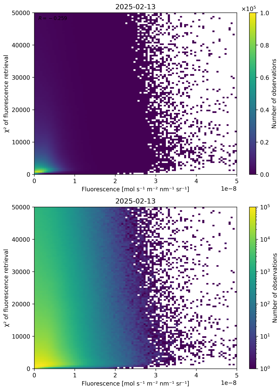
Figure 85: Scatter density plot of “Fluorescence” against “ \chi^2 of fluorescence retrieval” for 2025-02-13 to 2025-02-14.
