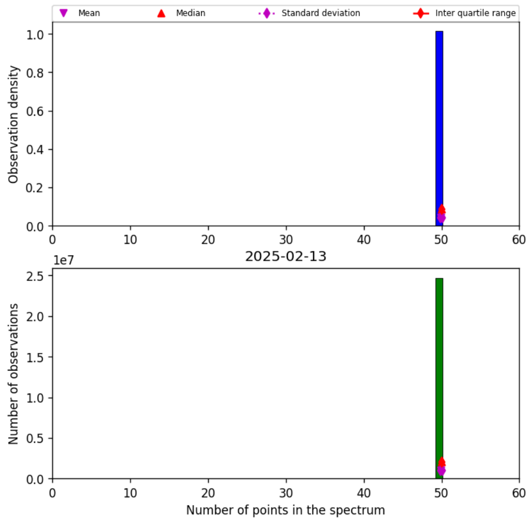
Figure 44: Histogram of “Number of points in the spectrum” for 2025-02-13 to 2025-02-14
