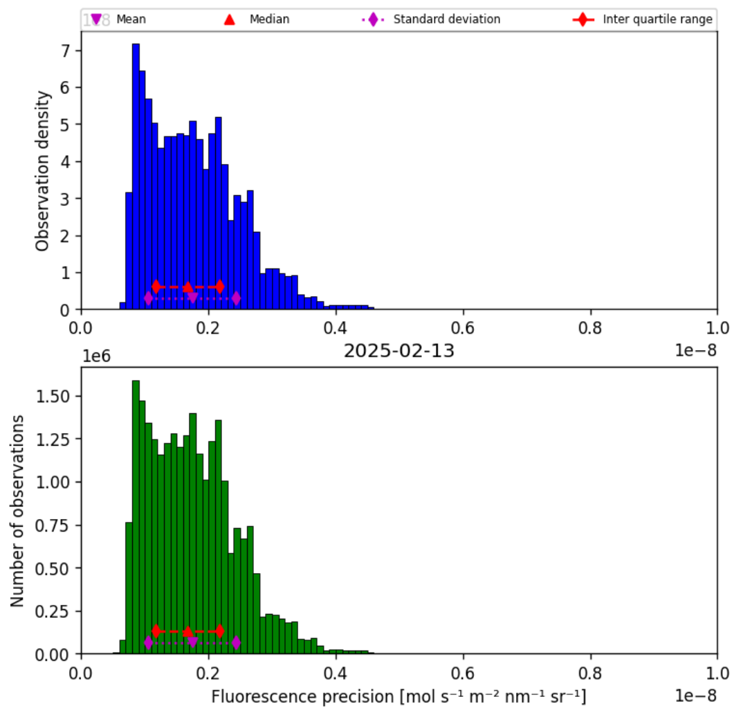
Figure 41: Histogram of “Fluorescence precision” for 2025-02-13 to 2025-02-14
