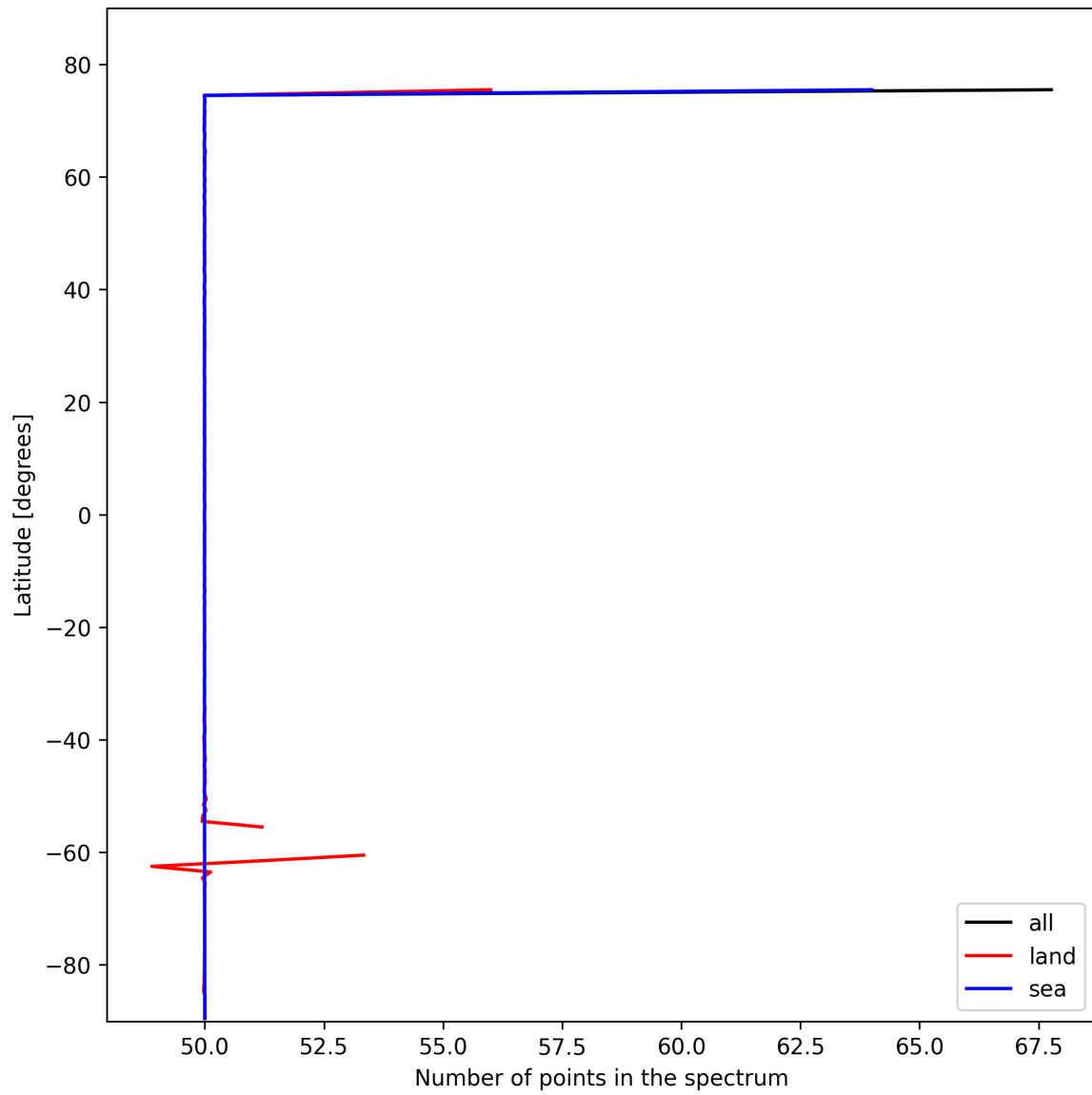
Figure 27: Zonal average of “Number of points in the spectrum” for 2025-02-13 to 2025-02-14.
