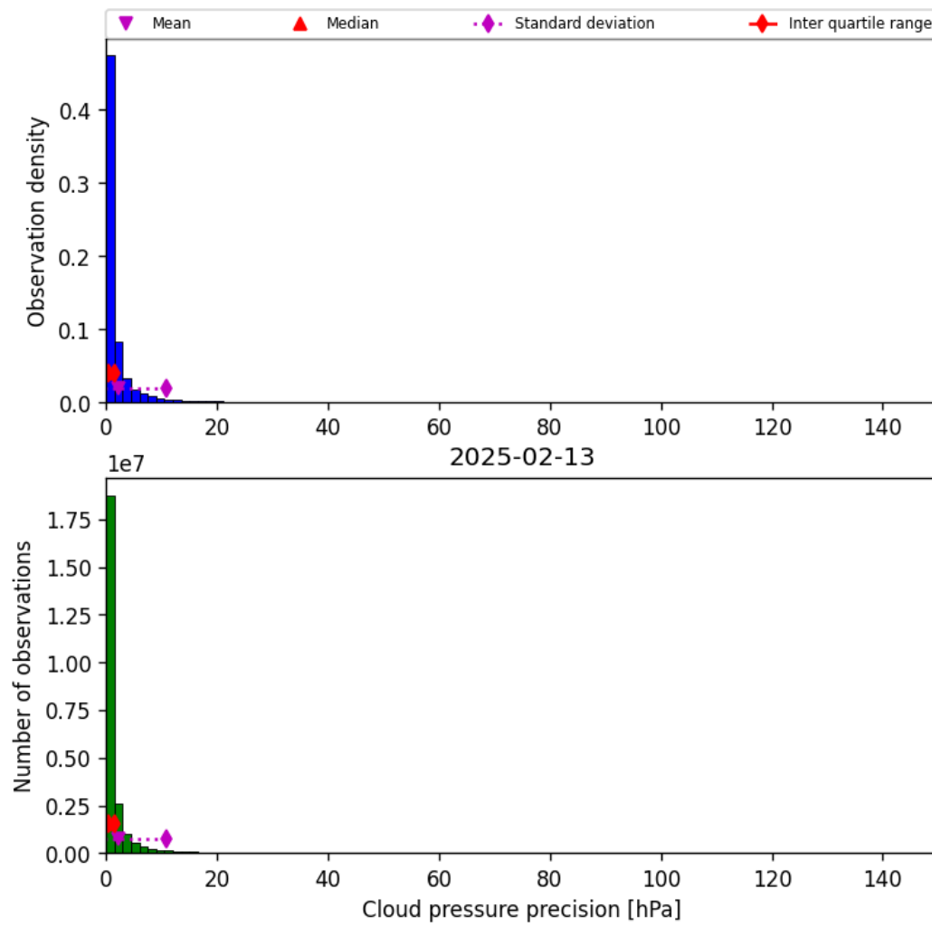
Figure 31: Histogram of “Cloud pressure precision” for 2025-02-13 to 2025-02-14
