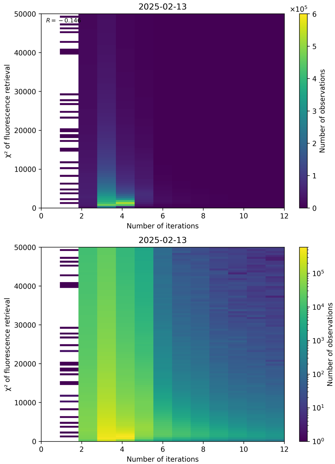
Figure 97: Scatter density plot of “Number of iterations” against “ \chi^2 of fluorescence retrieval” for 2025-02-13 to 2025-02-14.
