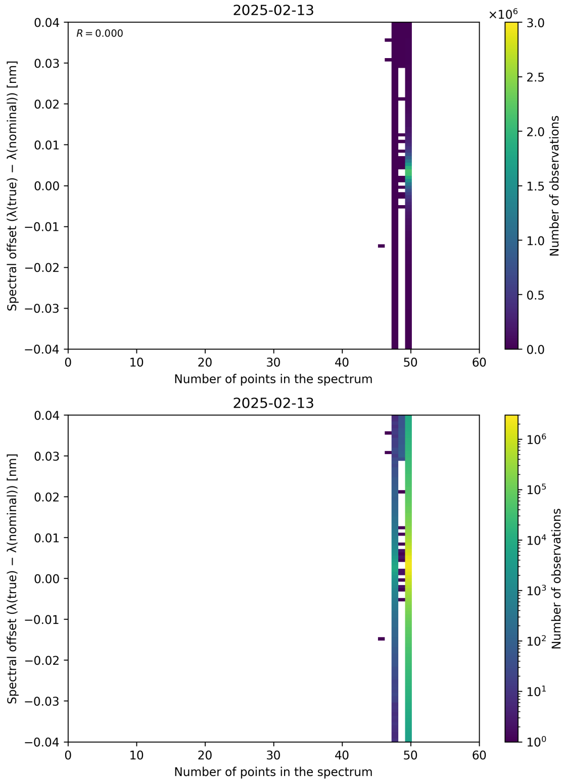
Figure 101: Scatter density plot of “Number of points in the spectrum” against “Spectral offset ( \lambda_{\text{true}} - \lambda_{\text{nominal}} )” for 2025-02-13 to 2025-02-14.
