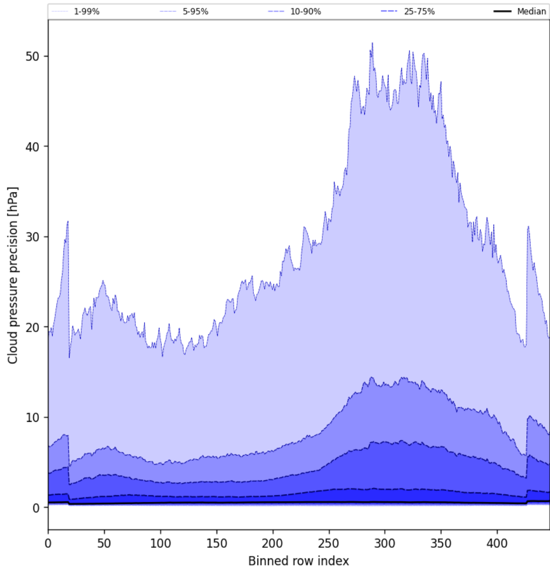
Figure 48: Along track statistics of “Cloud pressure precision” for 2025-02-13 to 2025-02-14
