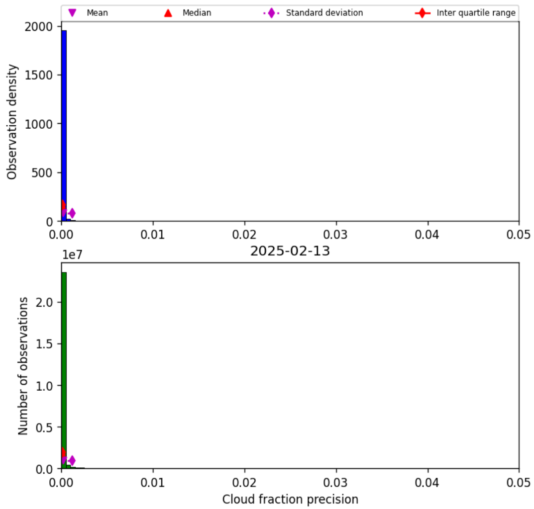
Figure 33: Histogram of “Cloud fraction precision” for 2025-02-13 to 2025-02-14
