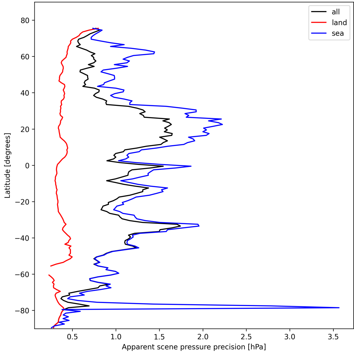
Figure 20: Zonal average of “Apparent scene pressure precision” for 2025-02-13 to 2025-02-14.
