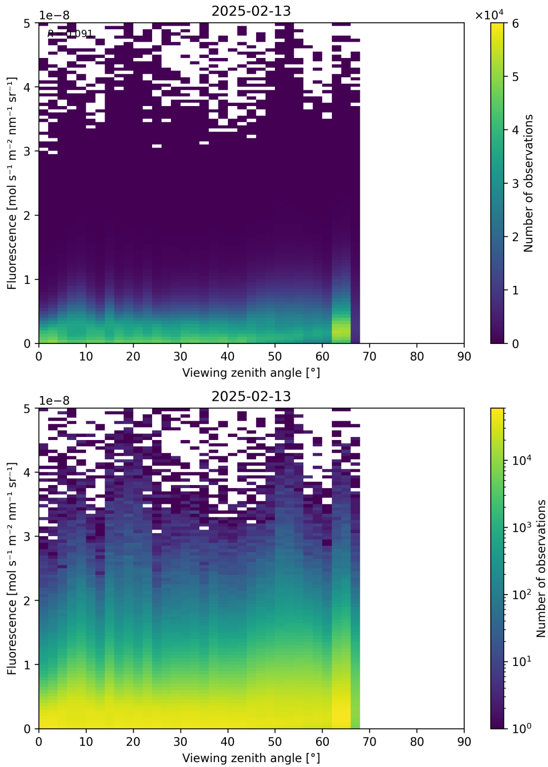
Figure 122: Scatter density plot of “Viewing zenith angle” against “Fluorescence” for 2025-02-13 to 2025-02-14.
