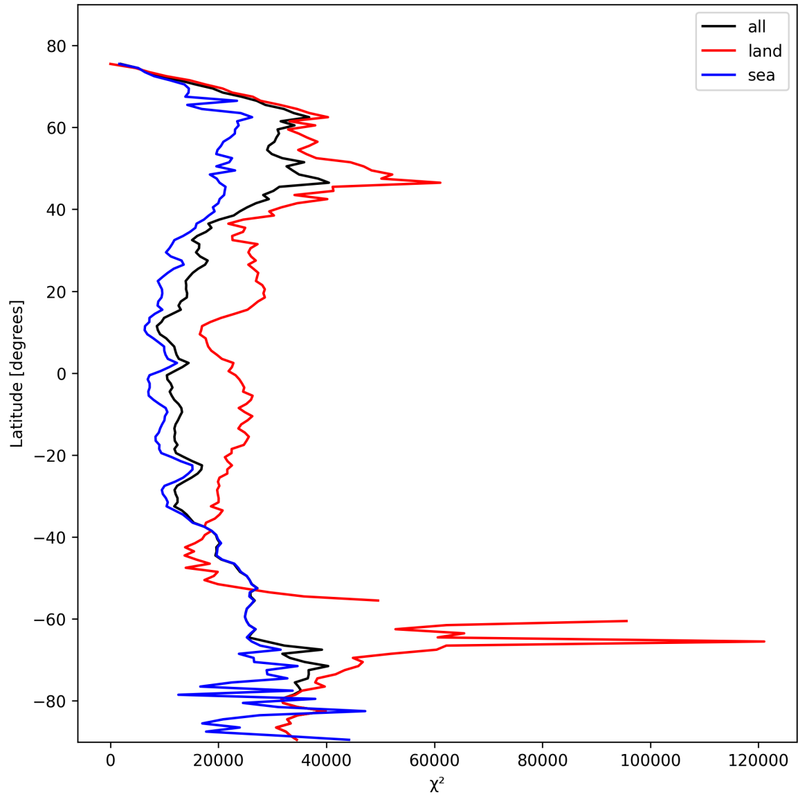
Figure 21: Zonal average of “ \chi^2 ” for 2025-02-13 to 2025-02-14.
