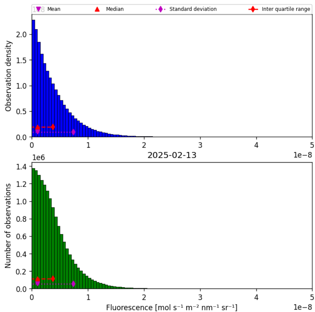
Figure 40: Histogram of “Fluorescence” for 2025-02-13 to 2025-02-14
