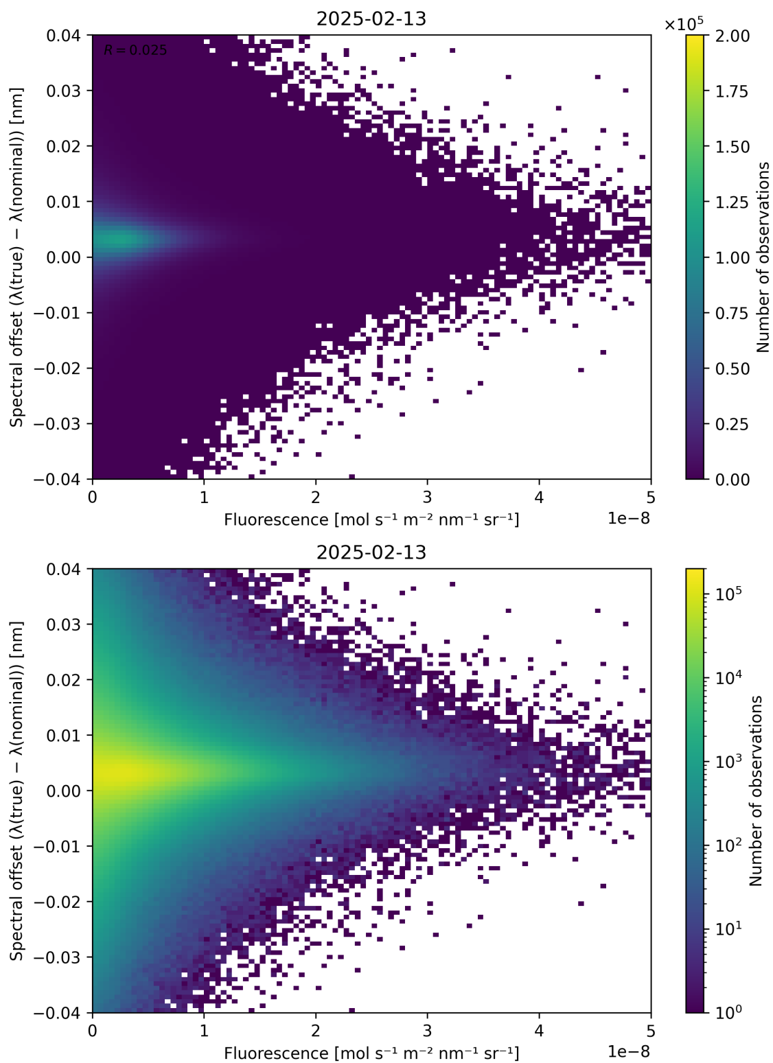
Figure 87: Scatter density plot of “Fluorescence” against “Spectral offset ( \lambda_{\text{true}} - \lambda_{\text{nominal}} )” for 2025-02-13 to 2025-02-14.
