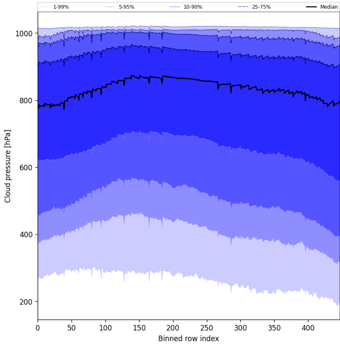
Figure 47: Along track statistics of “Cloud pressure” for 2025-02-13 to 2025-02-14
