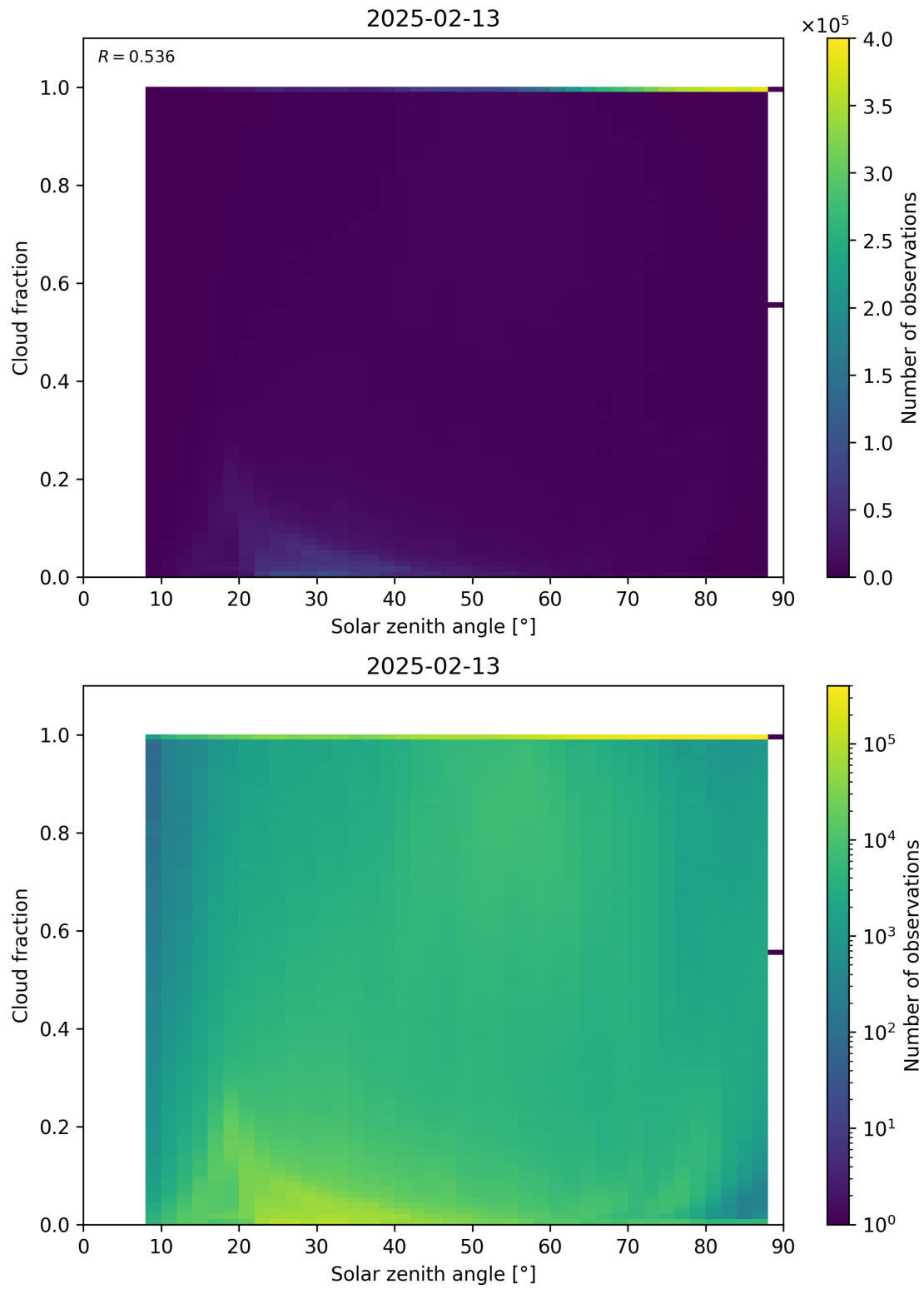
Figure 110: Scatter density plot of “Solar zenith angle” against “Cloud fraction” for 2025-02-13 to 2025-02-14.
