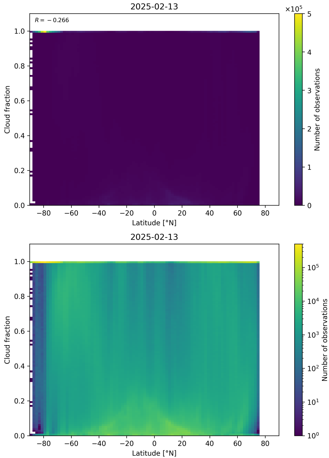
Figure 90: Scatter density plot of “Latitude” against “Cloud fraction” for 2025-02-13 to 2025-02-14.
