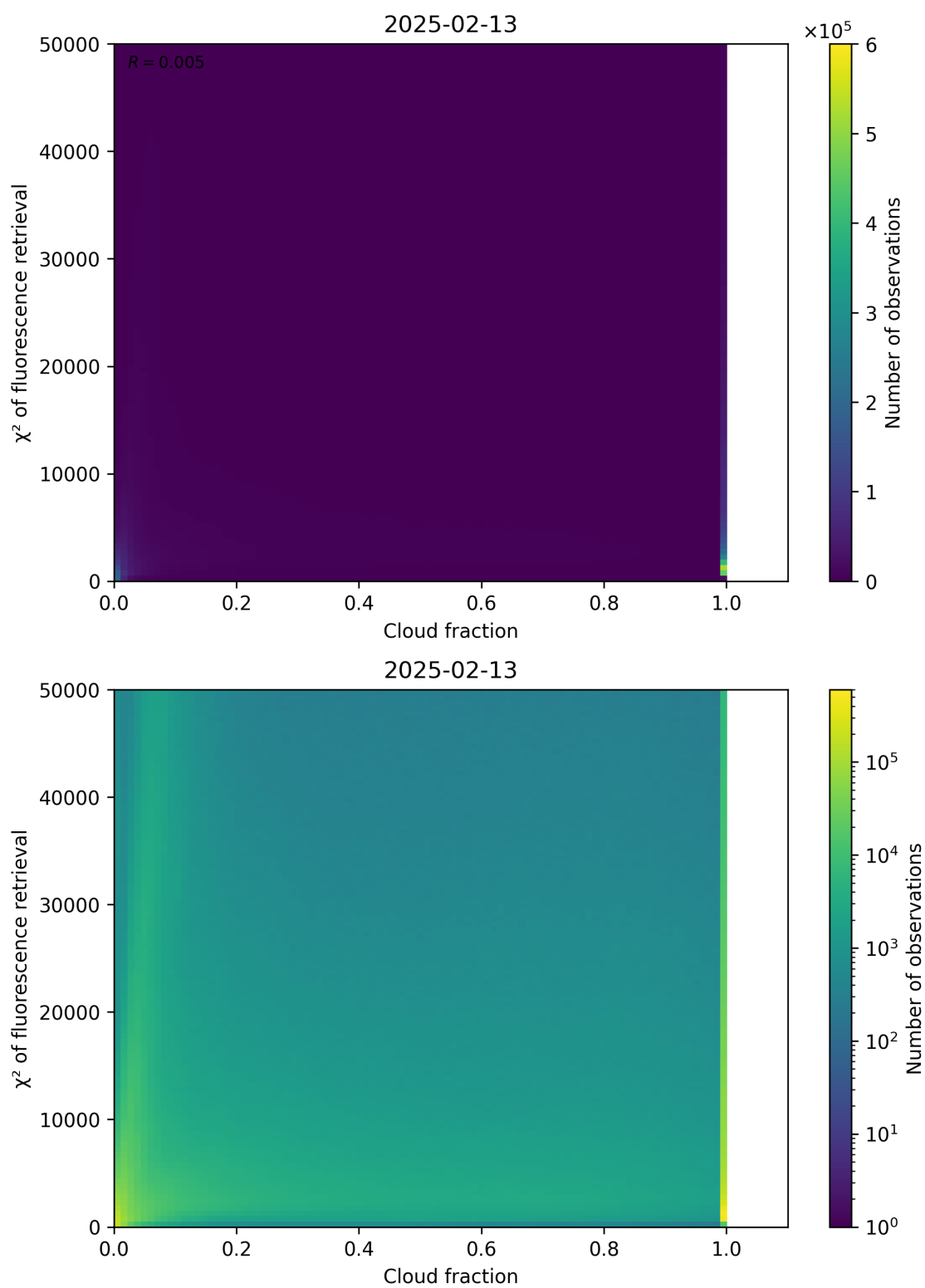
Figure 71: Scatter density plot of “Cloud fraction” against “ \chi^2 of fluorescence retrieval” for 2025-02-13 to 2025-02-14.
