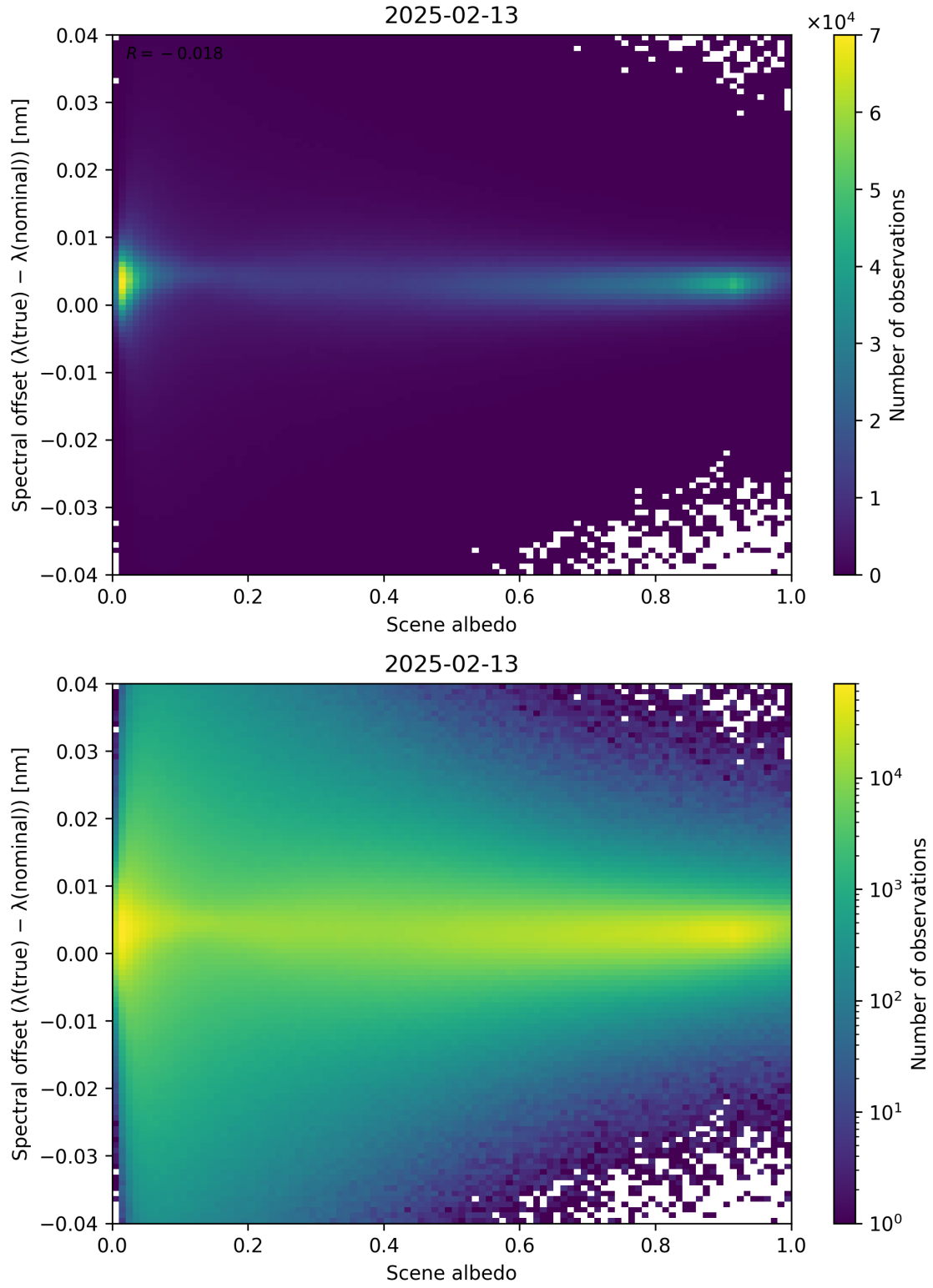
Figure 107: Scatter density plot of “Scene albedo” against “Spectral offset ( \lambda_{\text{true}} - \lambda_{\text{nominal}} )” for 2025-02-13 to 2025-02-14.
