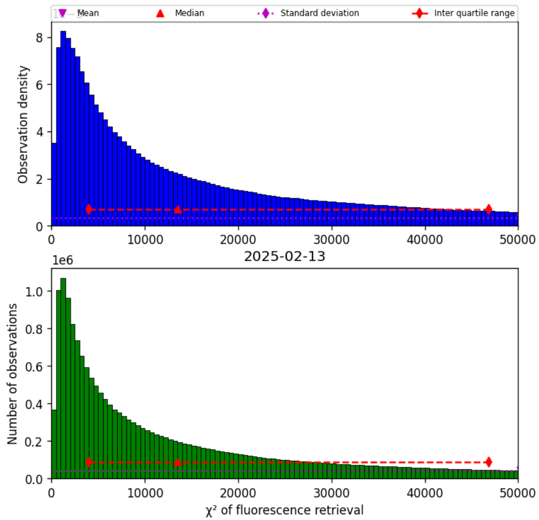
Figure 42: Histogram of “ \chi^2 of fluorescence retrieval” for 2025-02-13 to 2025-02-14
