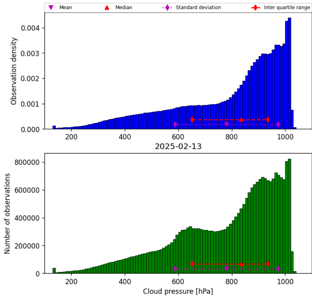
Figure 30: Histogram of “Cloud pressure” for 2025-02-13 to 2025-02-14
