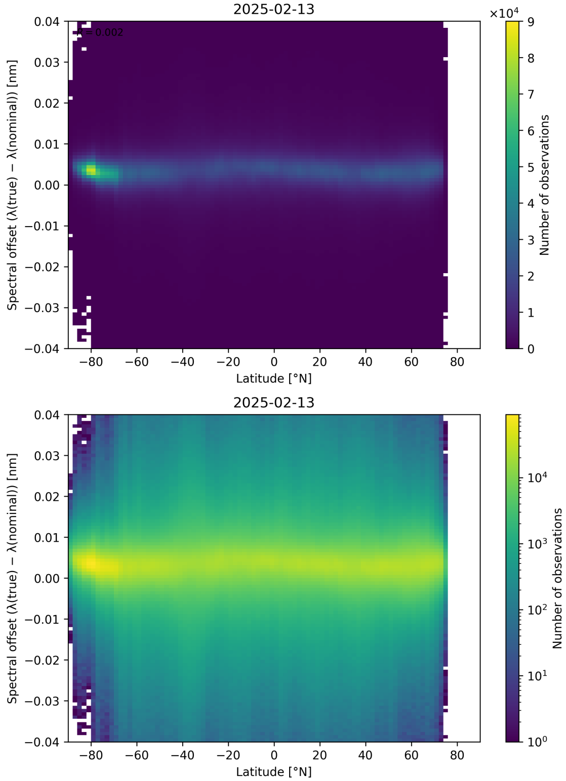
Figure 96: Scatter density plot of “Latitude” against “Spectral offset ( \lambda_{\text{true}} - \lambda_{\text{nominal}} )” for 2025-02-13 to 2025-02-14.
