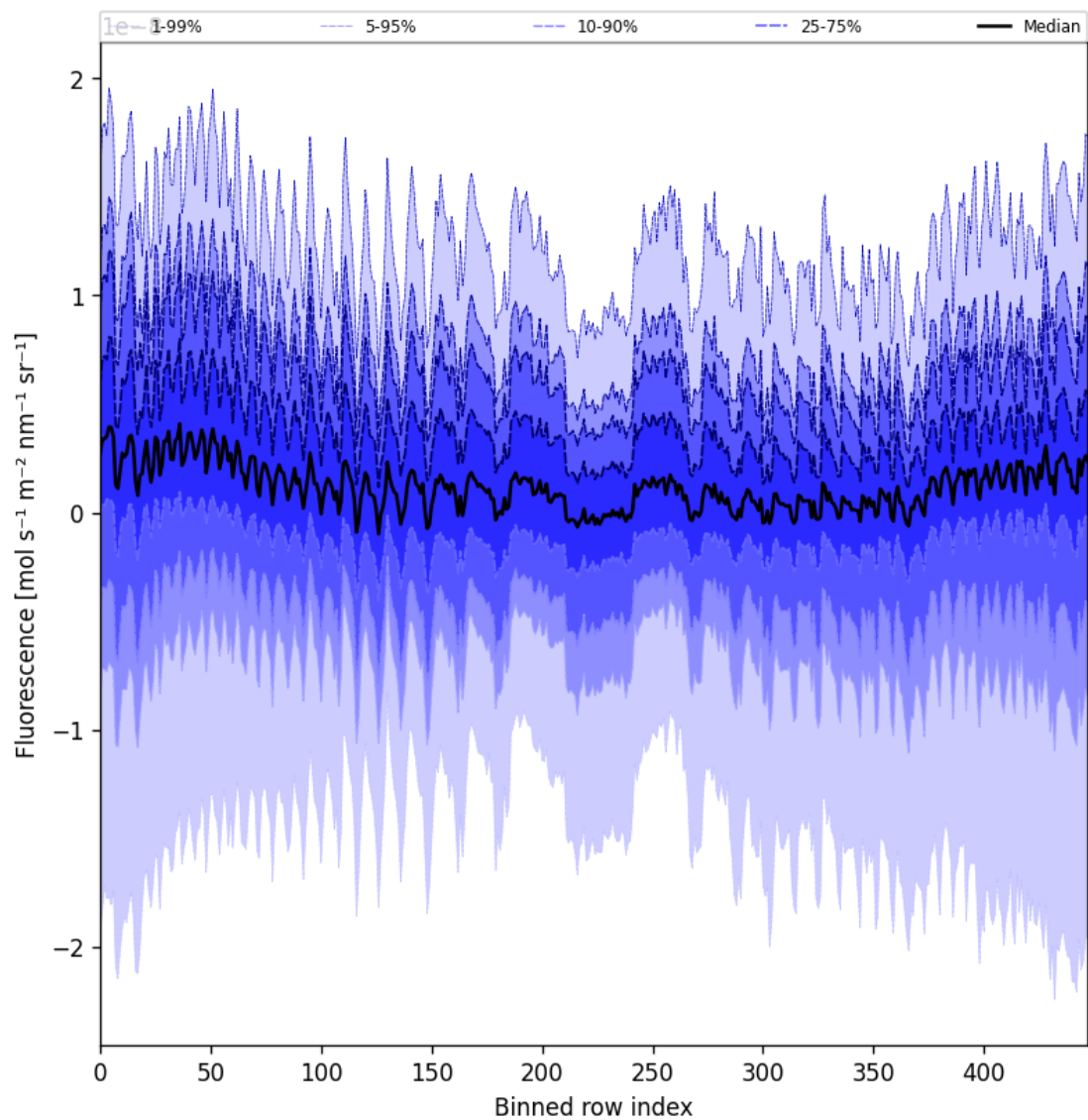
Figure 57: Along track statistics of “Fluorescence” for 2025-02-13 to 2025-02-14
