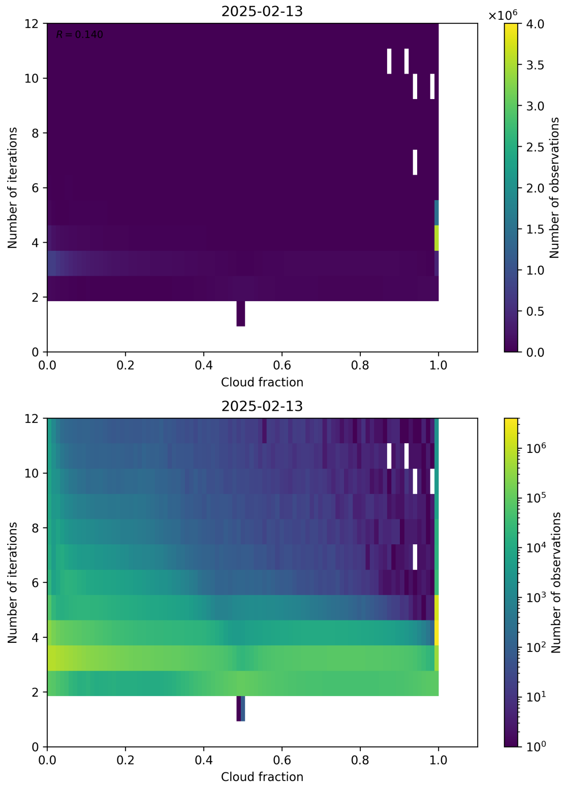
Figure 73: Scatter density plot of “Cloud fraction” against “Number of iterations” for 2025-02-13 to 2025-02-14.
