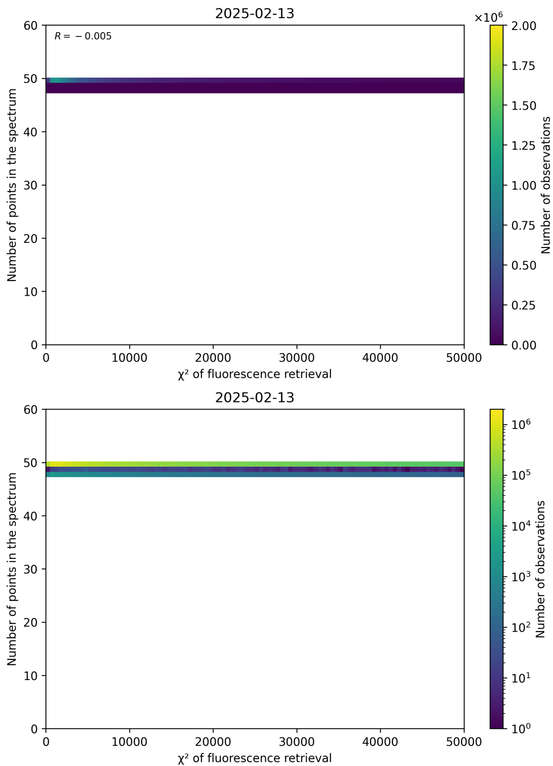
Figure 68: Scatter density plot of “ \chi^2 of fluorescence retrieval” against “Number of points in the spectrum” for 2025-02-13 to 2025-02-14.
