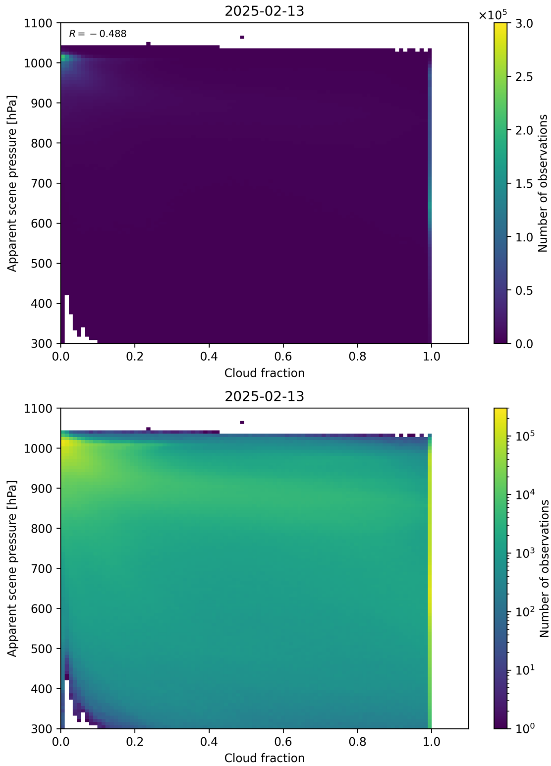
Figure 70: Scatter density plot of “Cloud fraction” against “Apparent scene pressure” for 2025-02-13 to 2025-02-14.
