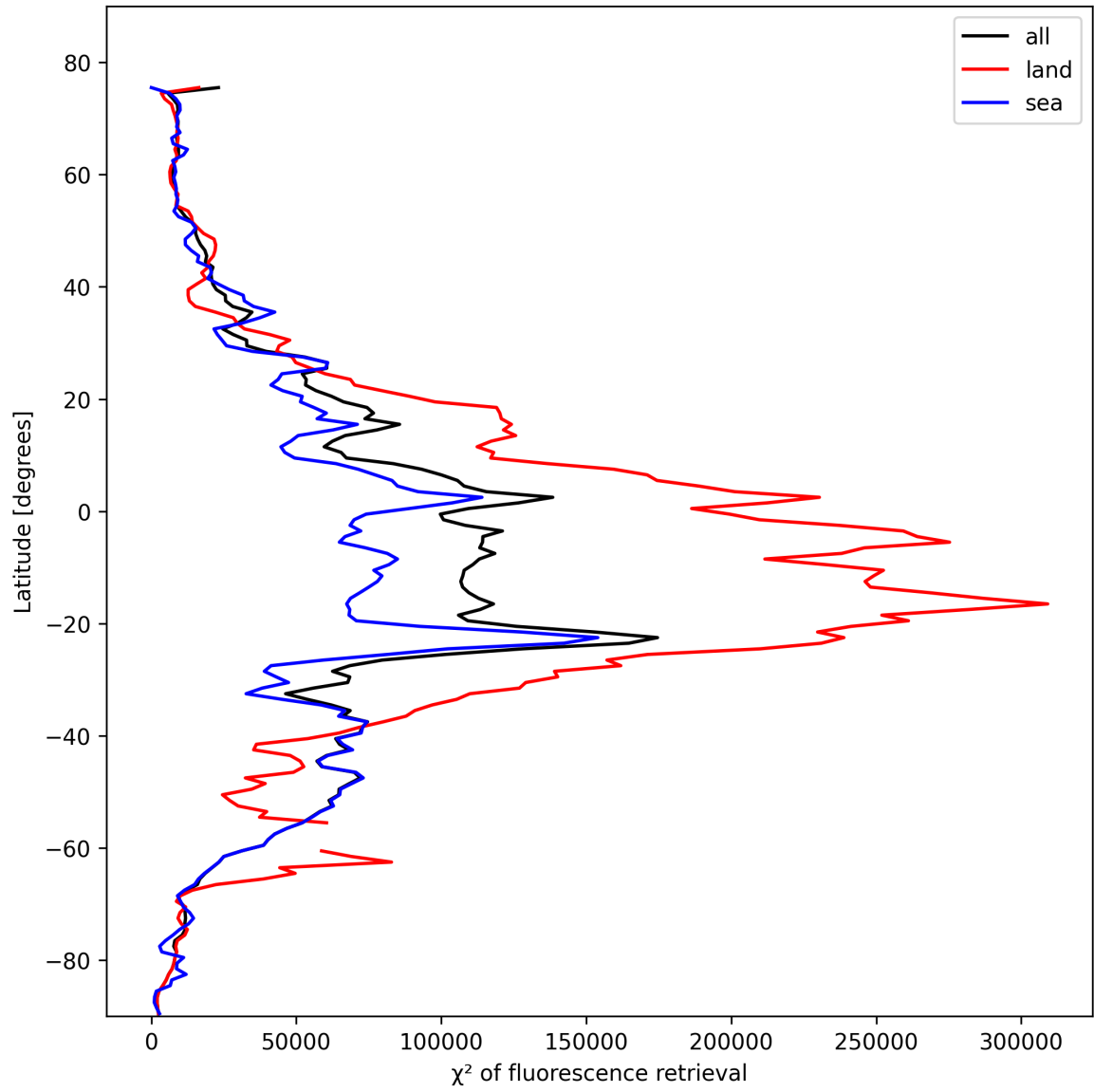
Figure 25: Zonal average of “ \chi^2 of fluorescence retrieval” for 2025-02-13 to 2025-02-14.
