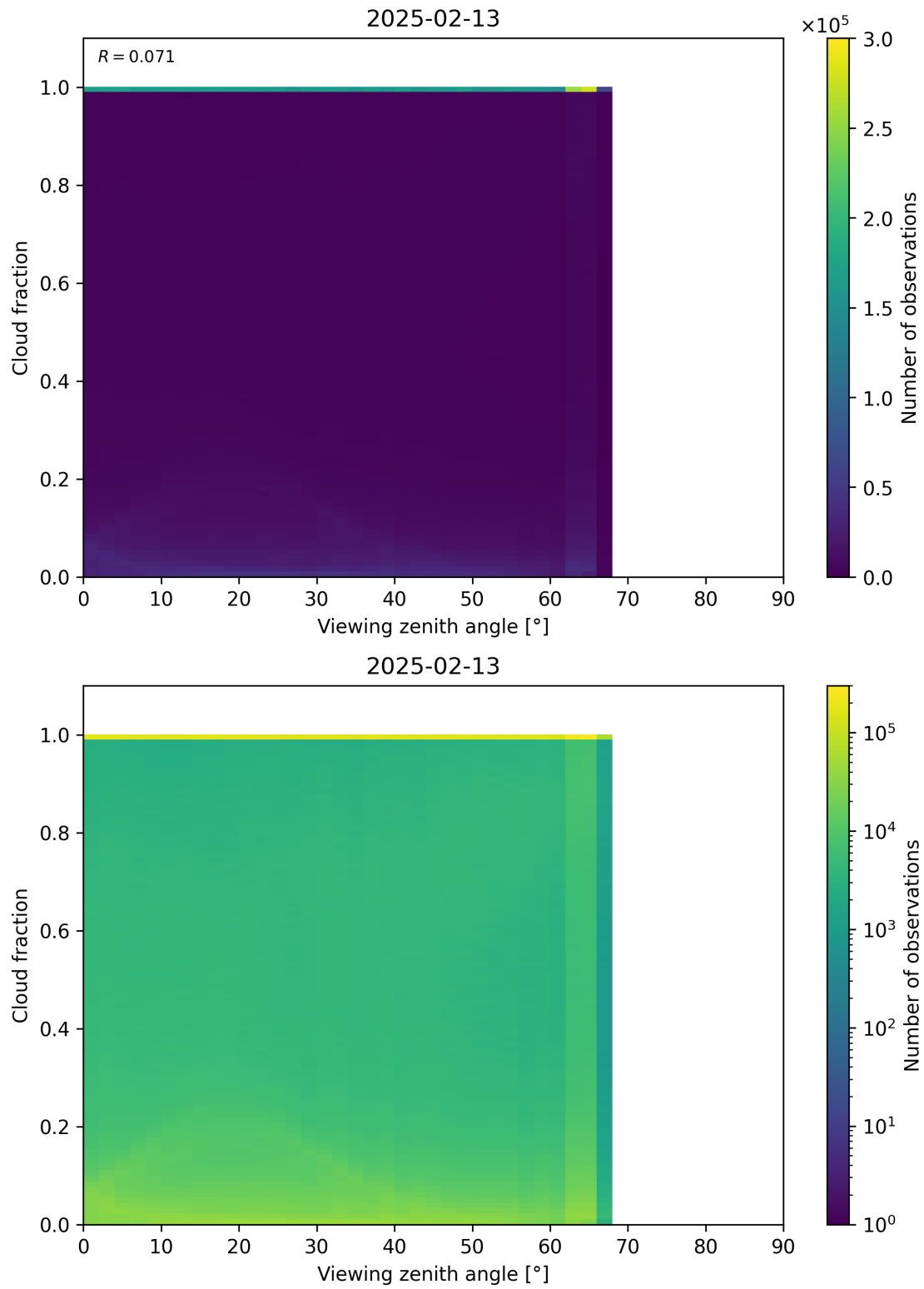
Figure 120: Scatter density plot of “Viewing zenith angle” against “Cloud fraction” for 2025-02-13 to 2025-02-14.
