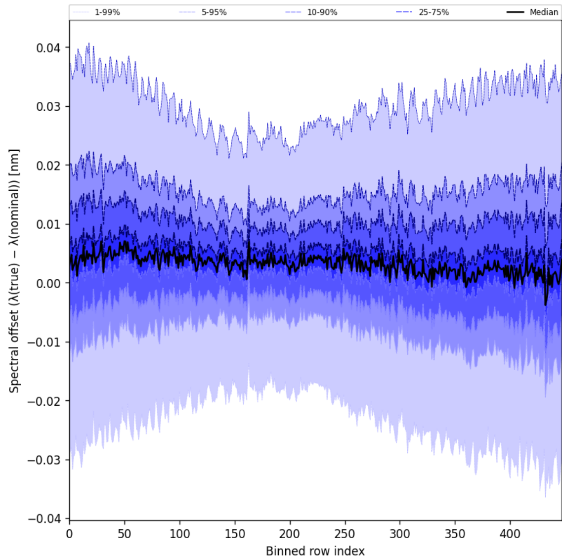
Figure 62: Along track statistics of “Spectral offset ( \lambda_{\text{true}} - \lambda_{\text{nominal}} )” for 2025-02-13 to 2025-02-14
