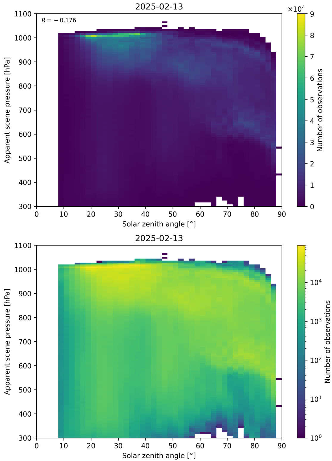
Figure 108: Scatter density plot of “Solar zenith angle” against “Apparent scene pressure” for 2025-02-13 to 2025-02-14.
