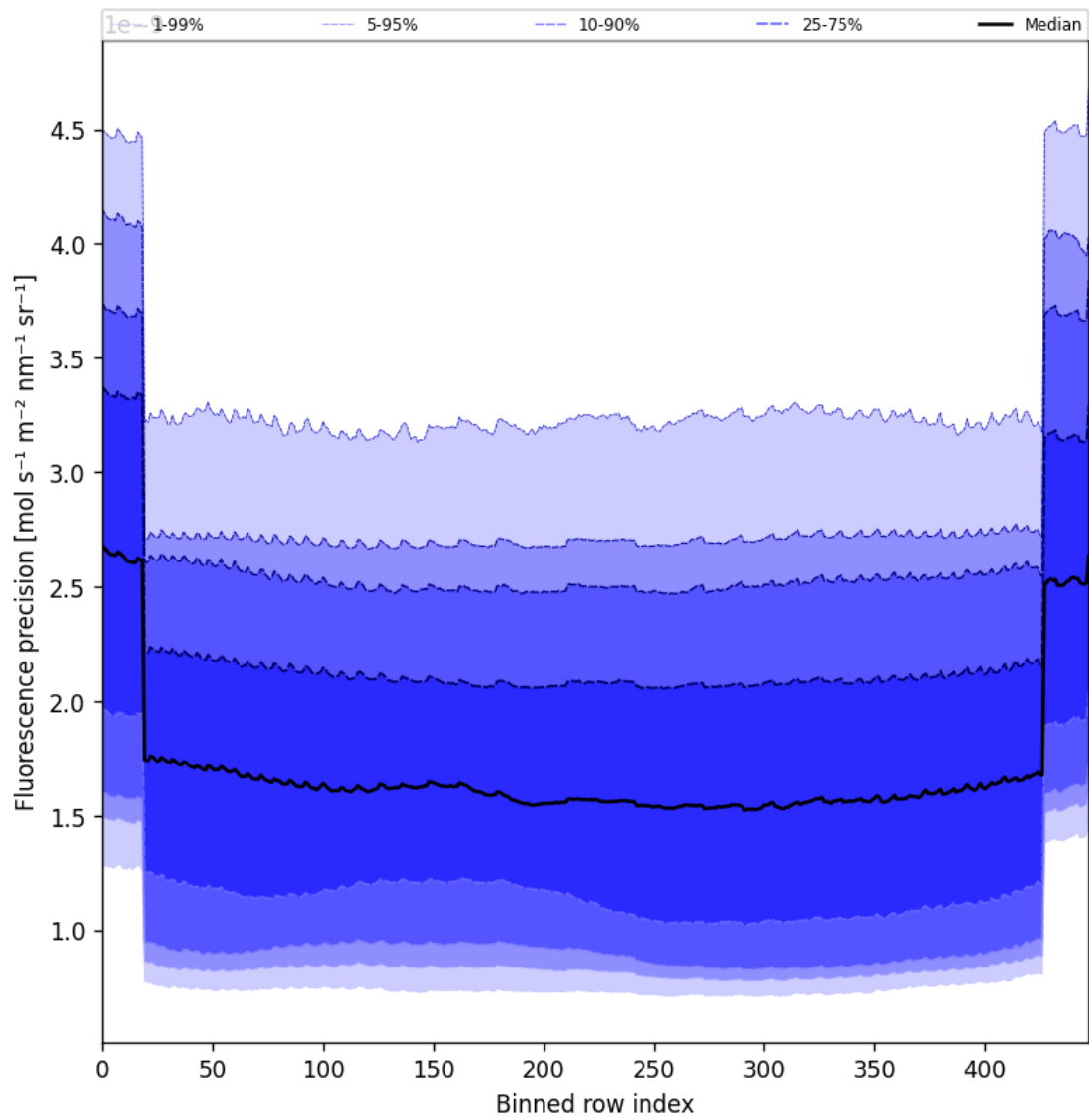
Figure 58: Along track statistics of “Fluorescence precision” for 2025-02-13 to 2025-02-14
