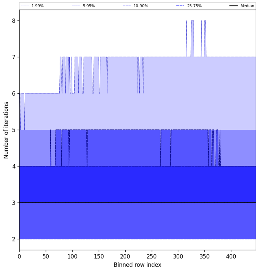
Figure 56: Along track statistics of “Number of iterations” for 2025-02-13 to 2025-02-14
