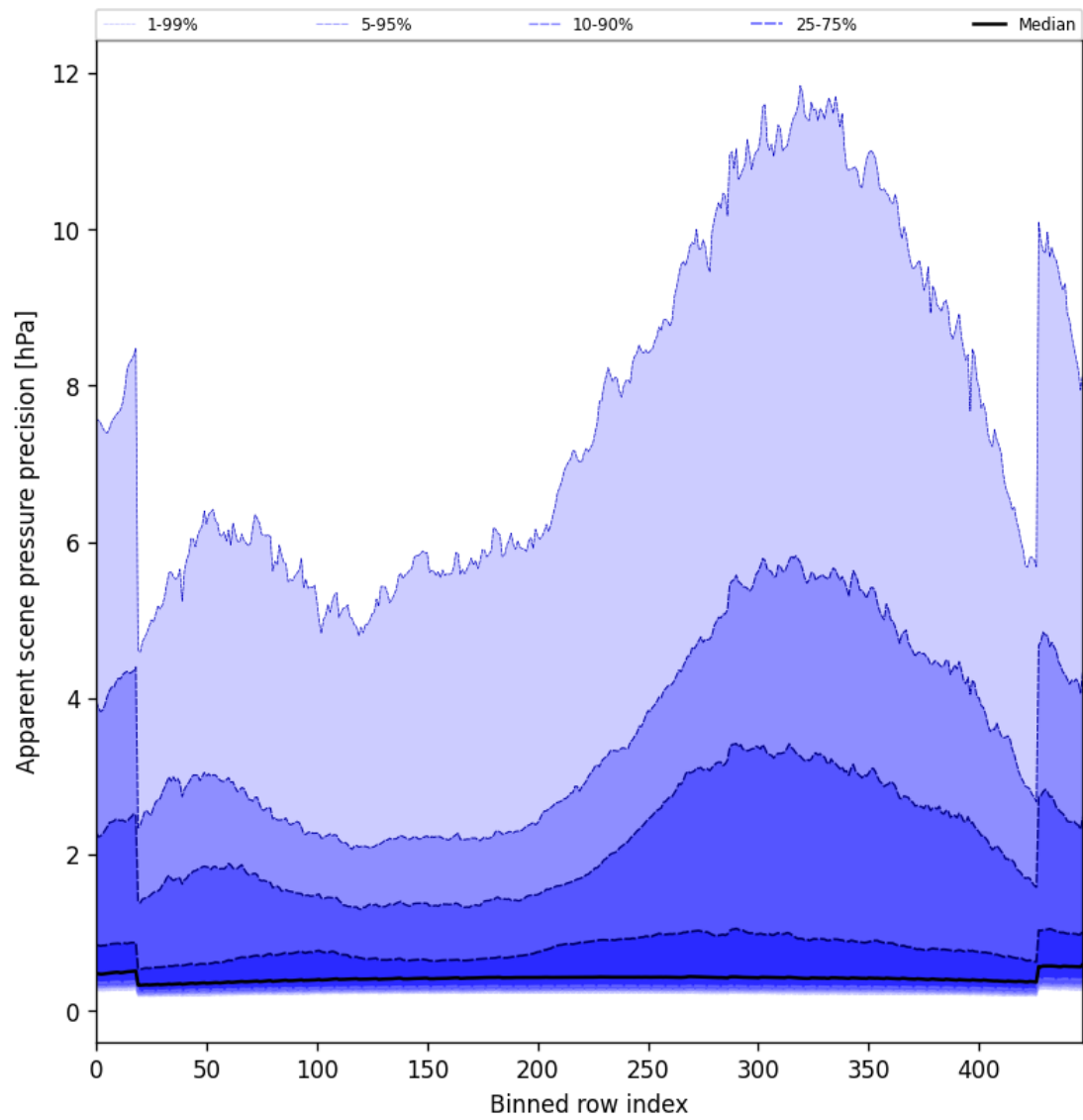
Figure 54: Along track statistics of “Apparent scene pressure precision” for 2025-02-13 to 2025-02-14
