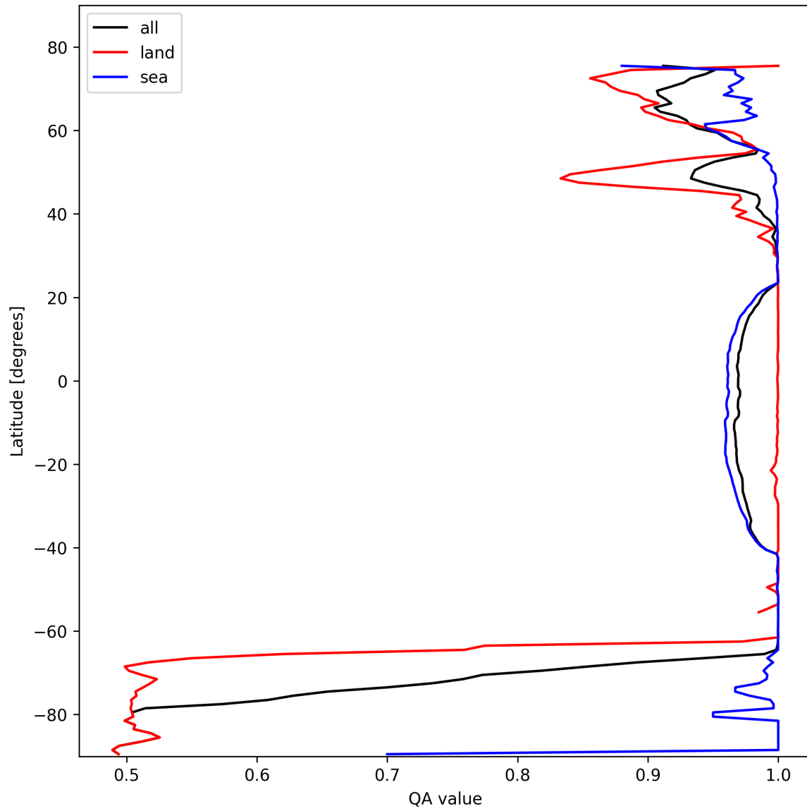
Figure 12: Zonal average of “QA value” for 2025-02-13 to 2025-02-14.
