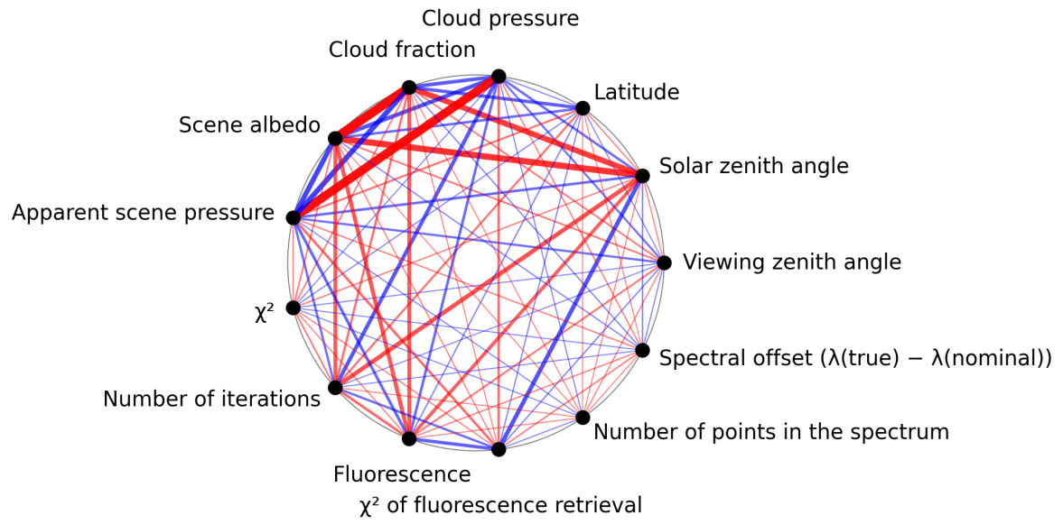
Figure 1: Map of correlation graph for 2025-02-13 to 2025-02-14.
