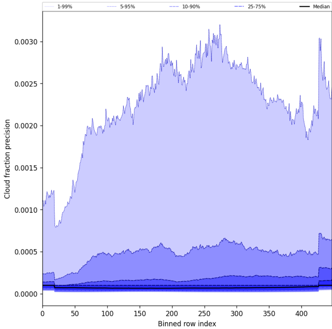
Figure 50: Along track statistics of “Cloud fraction precision” for 2025-02-13 to 2025-02-14
