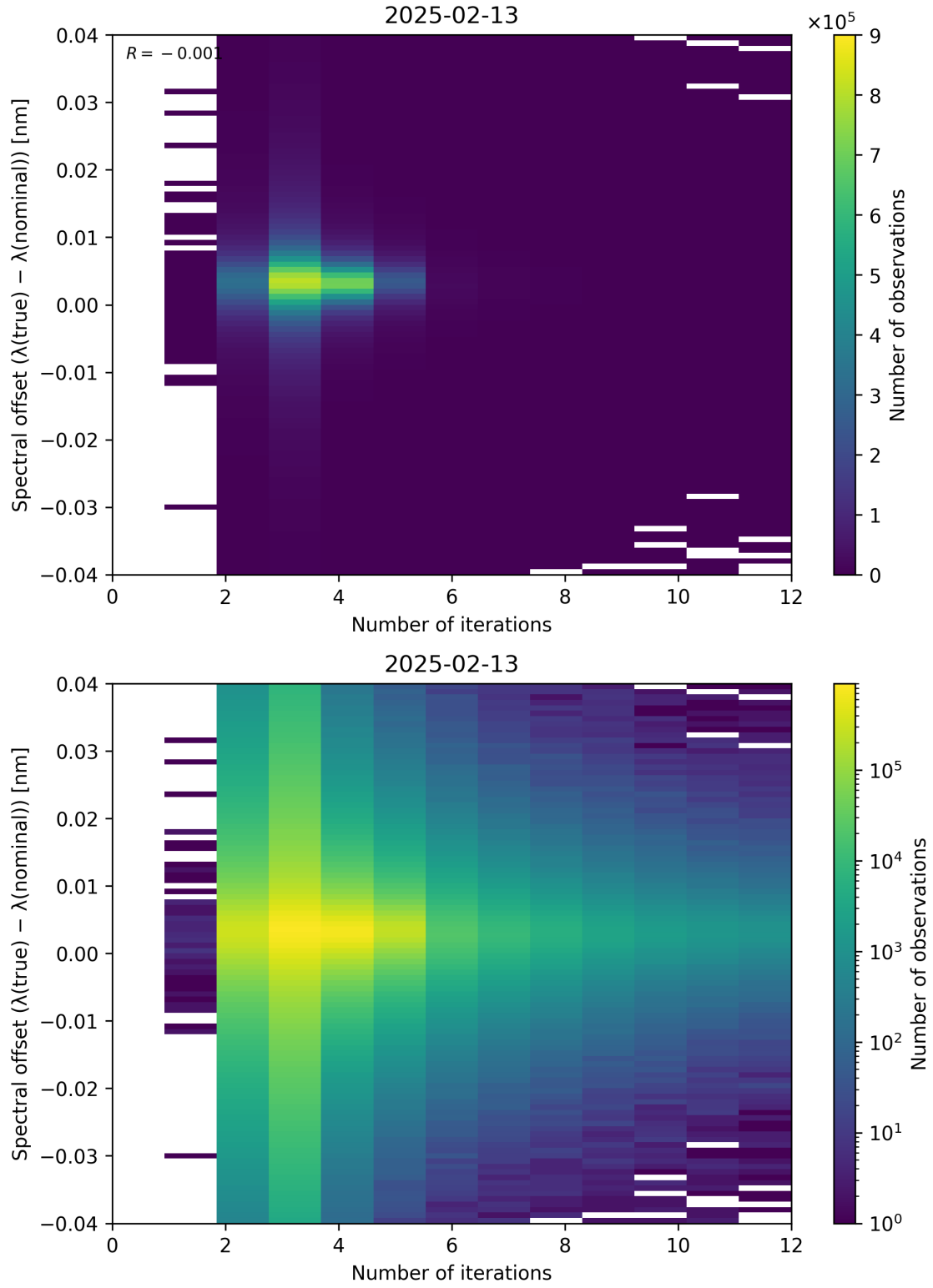
Figure 100: Scatter density plot of “Number of iterations” against “Spectral offset ( \lambda_{\text{true}} - \lambda_{\text{nominal}} )” for 2025-02-13 to 2025-02-14.
