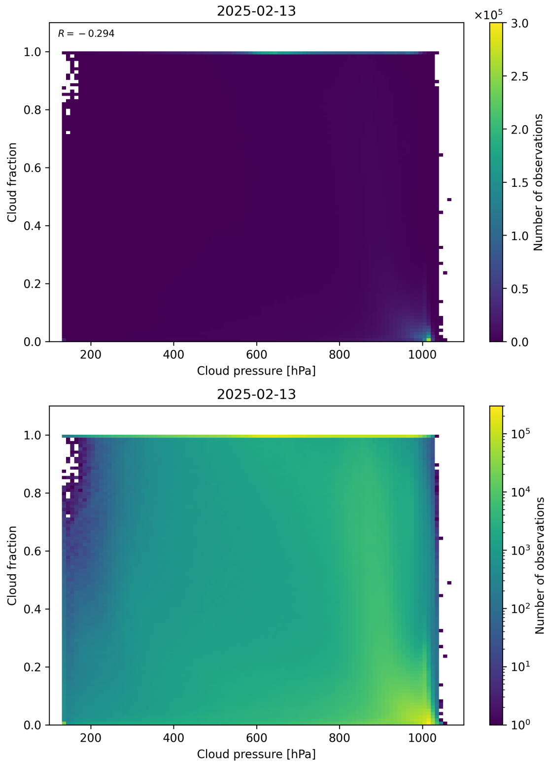
Figure 79: Scatter density plot of “Cloud pressure” against “Cloud fraction” for 2025-02-13 to 2025-02-14.
