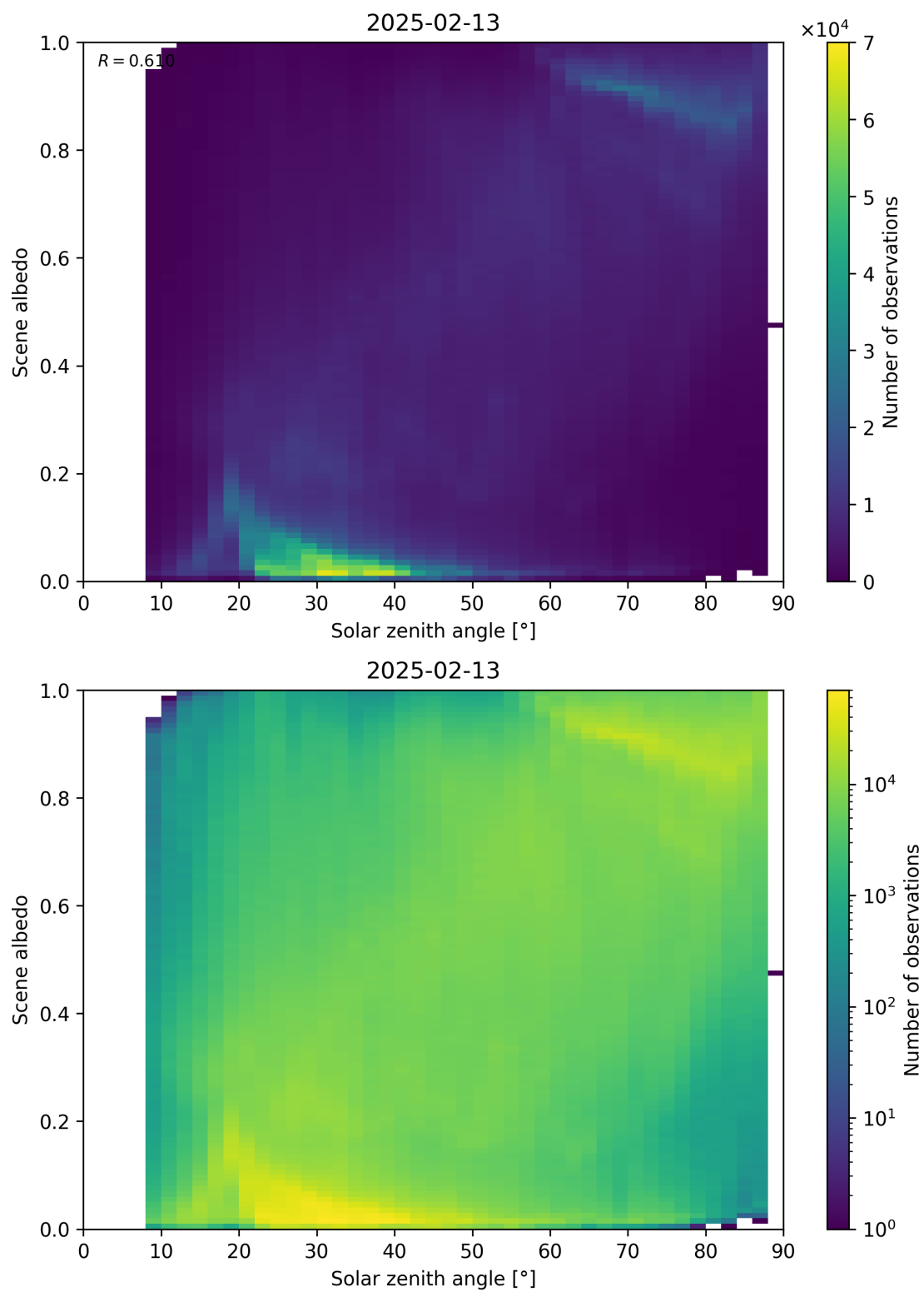
Figure 116: Scatter density plot of “Solar zenith angle” against “Scene albedo” for 2025-02-13 to 2025-02-14.
