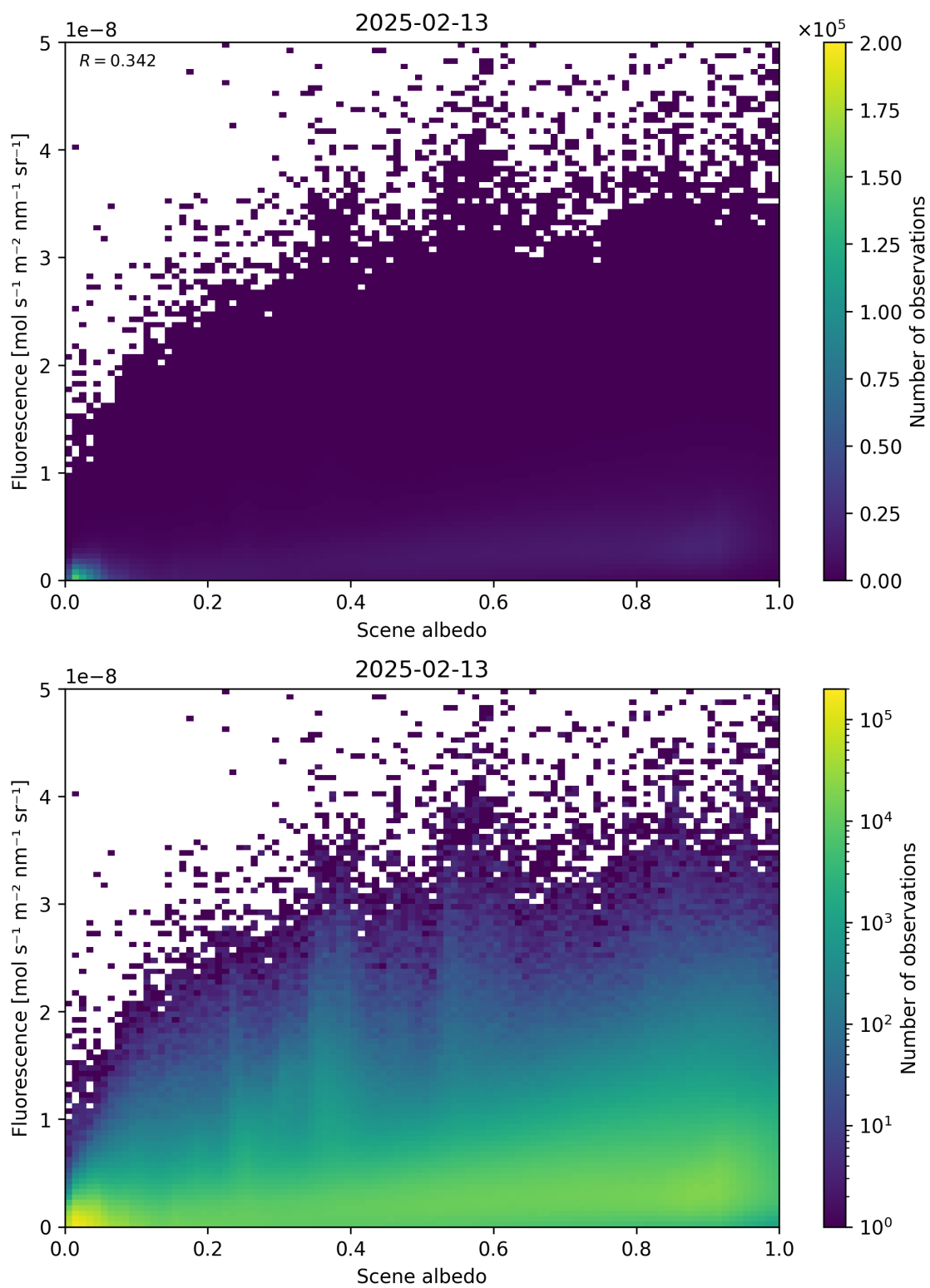
Figure 104: Scatter density plot of “Scene albedo” against “Fluorescence” for 2025-02-13 to 2025-02-14.
