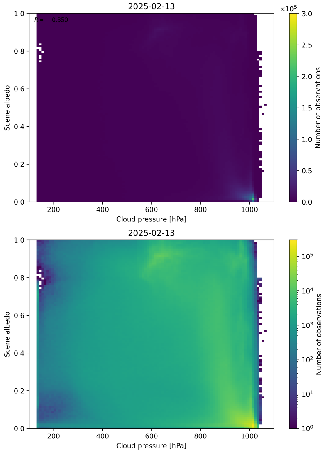
Figure 83: Scatter density plot of “Cloud pressure” against “Scene albedo” for 2025-02-13 to 2025-02-14.
