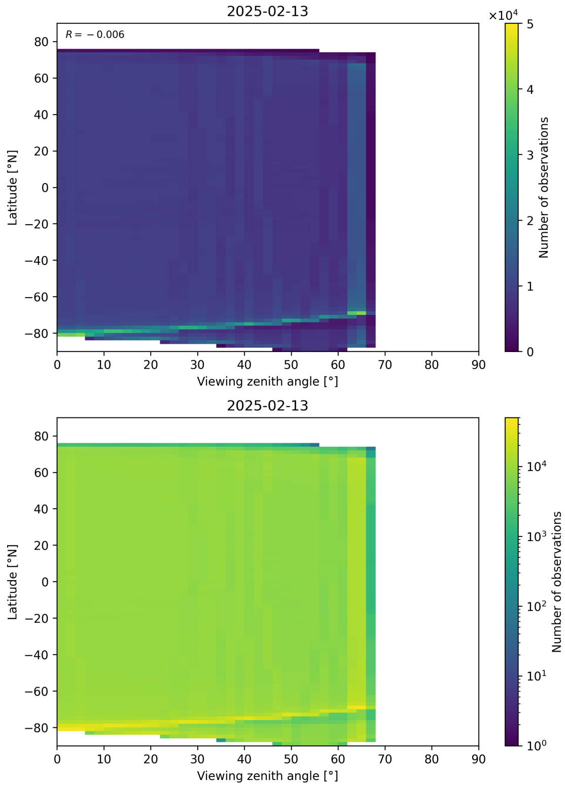
Figure 123: Scatter density plot of “Viewing zenith angle” against “Latitude” for 2025-02-13 to 2025-02-14.
