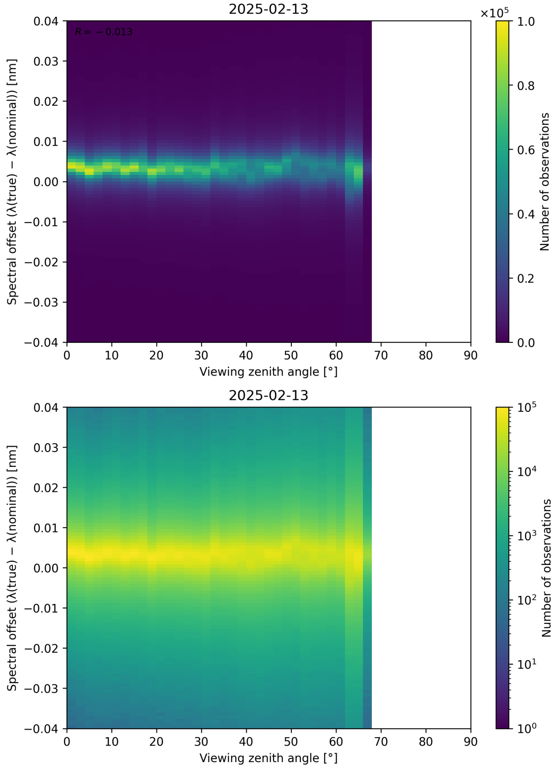
Figure 128: Scatter density plot of “Viewing zenith angle” against “Spectral offset ( \lambda_{\text{true}} - \lambda_{\text{nominal}} )” for 2025-02-13 to 2025-02-14.
