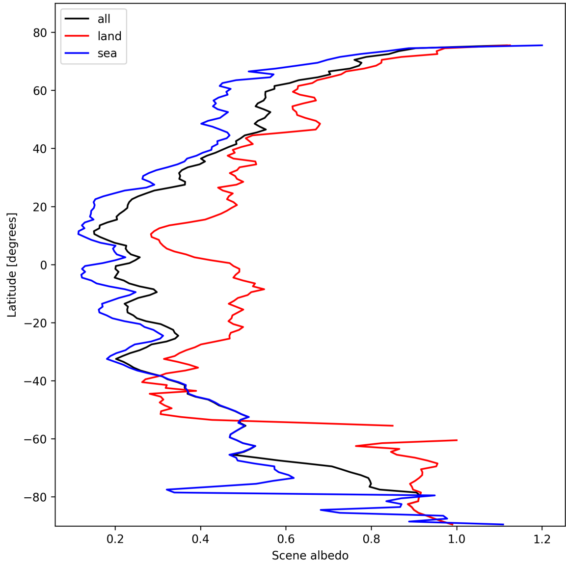
Figure 17: Zonal average of “Scene albedo” for 2025-02-13 to 2025-02-14.
