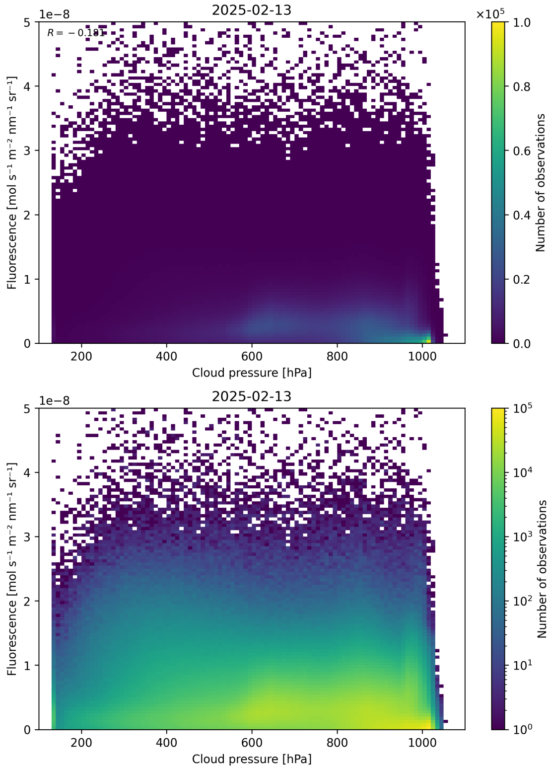
Figure 80: Scatter density plot of “Cloud pressure” against “Fluorescence” for 2025-02-13 to 2025-02-14.
