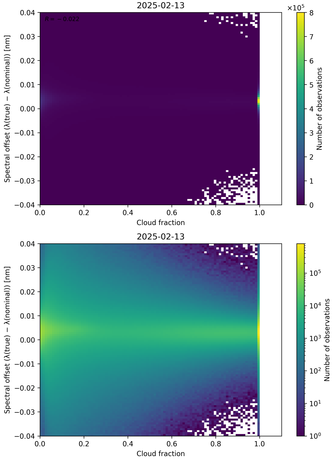
Figure 76: Scatter density plot of “Cloud fraction” against “Spectral offset ( \lambda_{\text{true}} - \lambda_{\text{nominal}} )” for 2025-02-13 to 2025-02-14.
