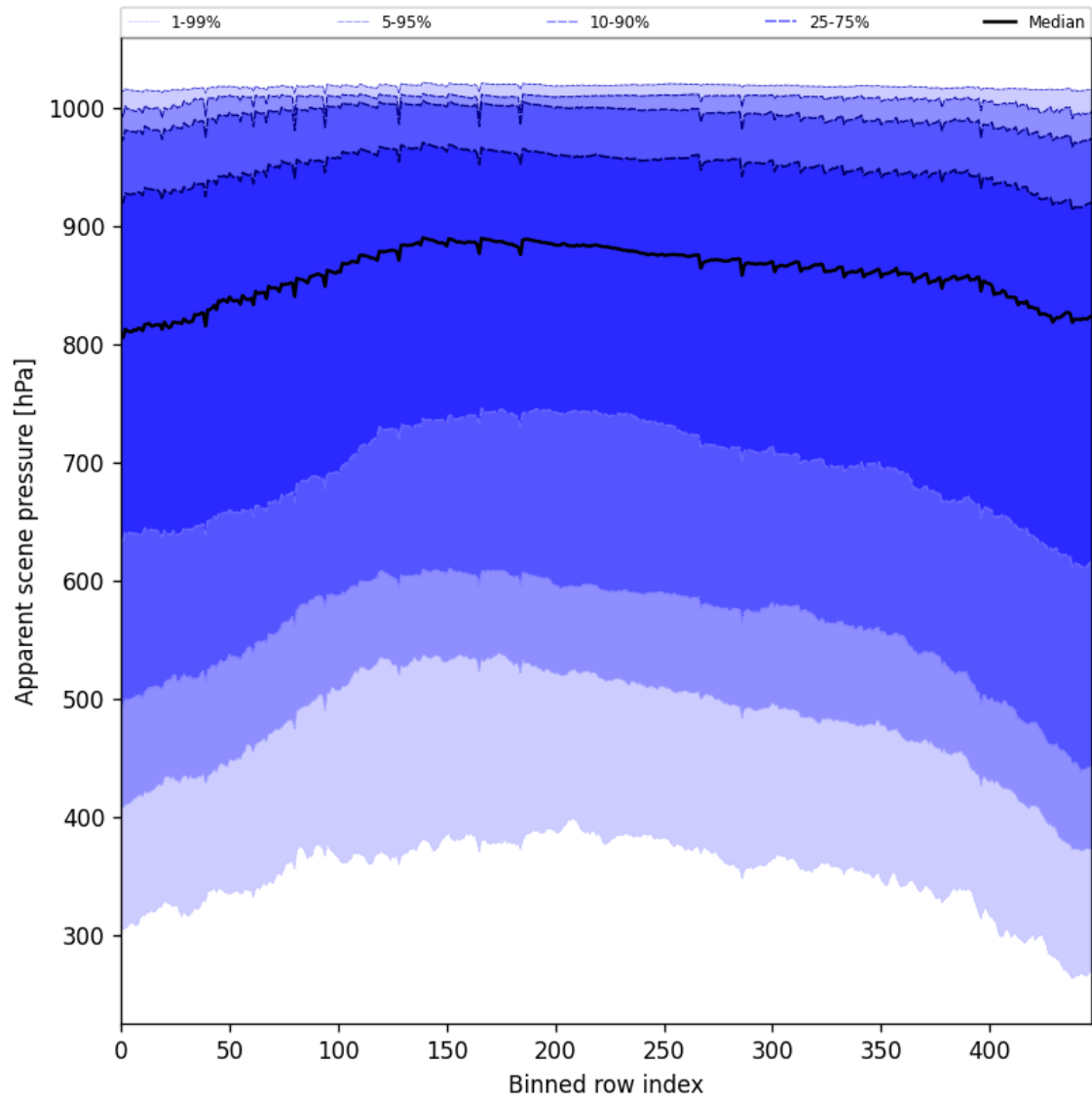
Figure 53: Along track statistics of “Apparent scene pressure” for 2025-02-13 to 2025-02-14
