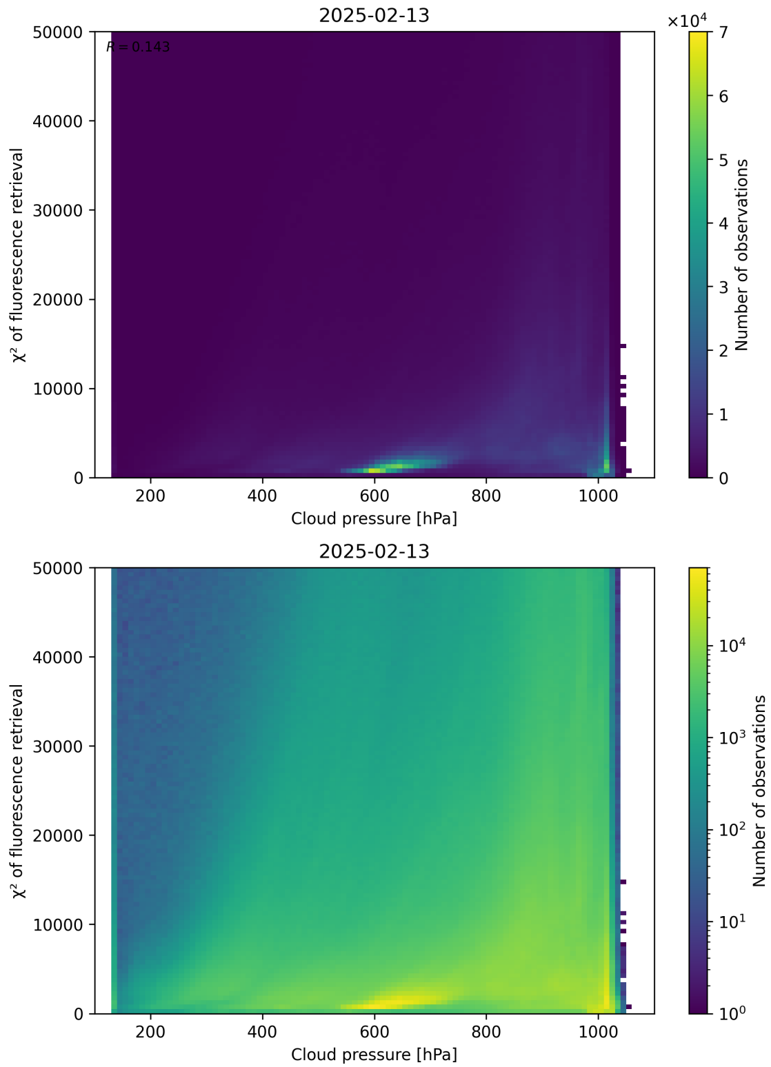
Figure 78: Scatter density plot of “Cloud pressure” against “ \chi^2 of fluorescence retrieval” for 2025-02-13 to 2025-02-14.
