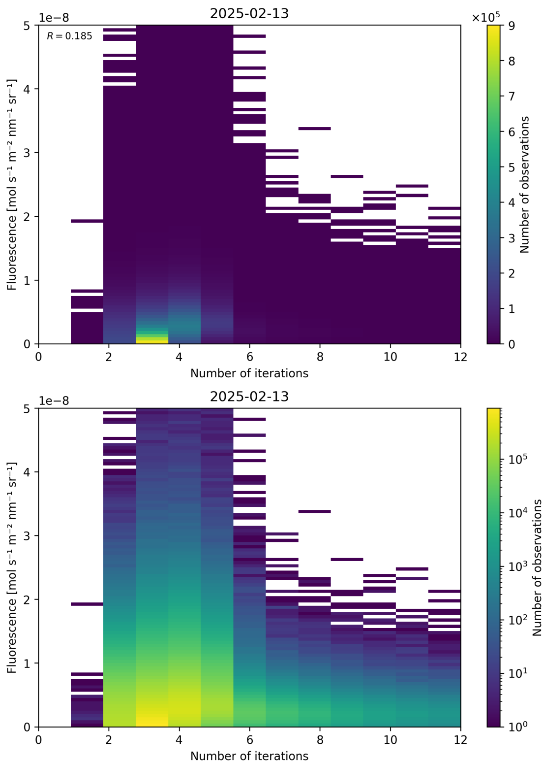
Figure 98: Scatter density plot of “Number of iterations” against “Fluorescence” for 2025-02-13 to 2025-02-14.
