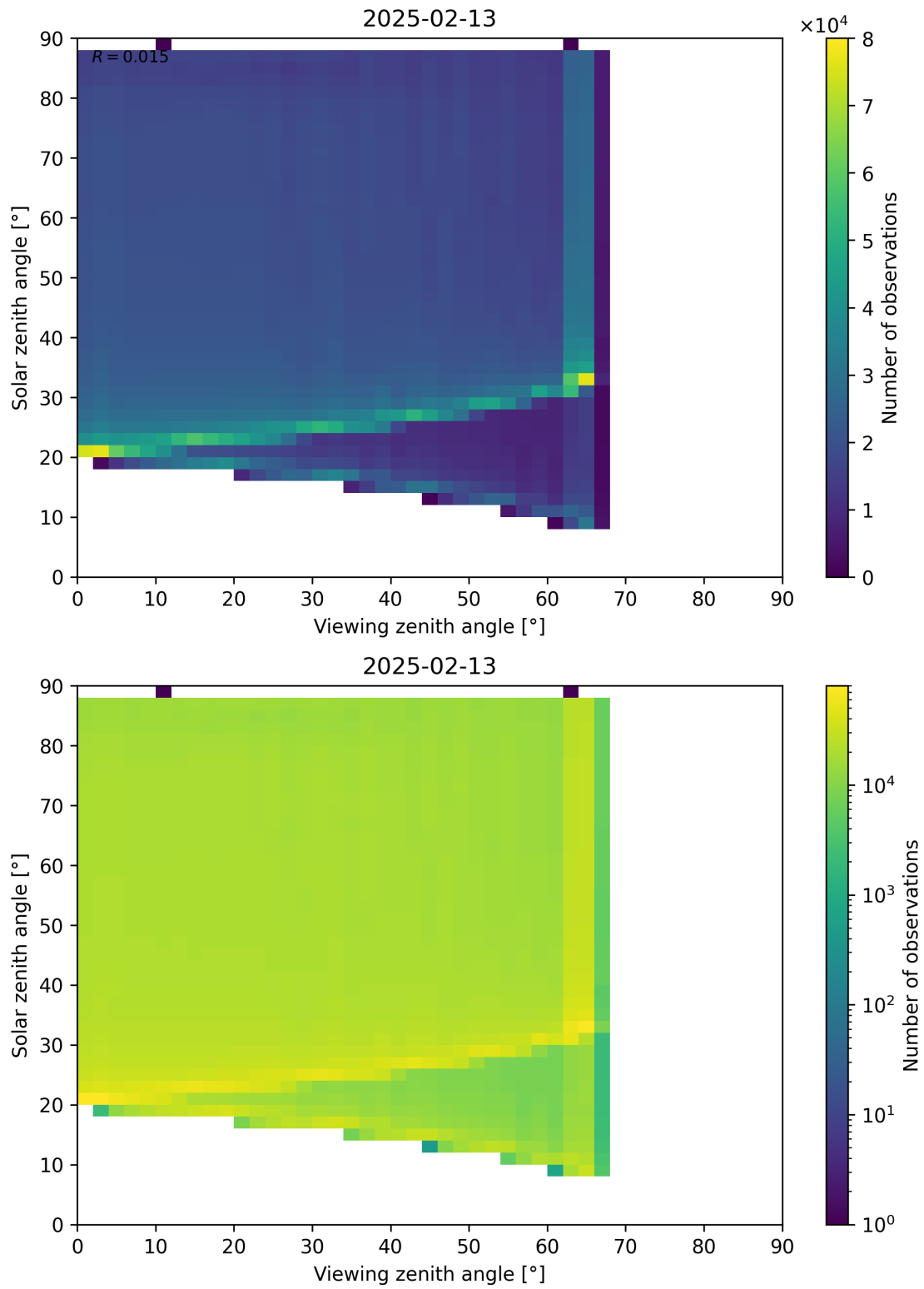
Figure 127: Scatter density plot of “Viewing zenith angle” against “Solar zenith angle” for 2025-02-13 to 2025-02-14.
