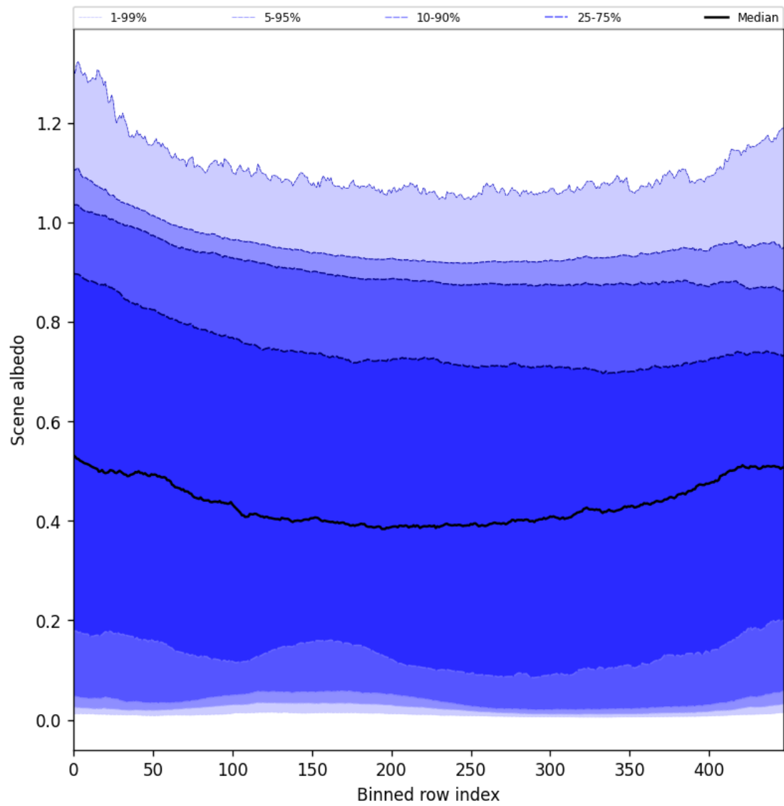
Figure 51: Along track statistics of “Scene albedo” for 2025-02-13 to 2025-02-14
