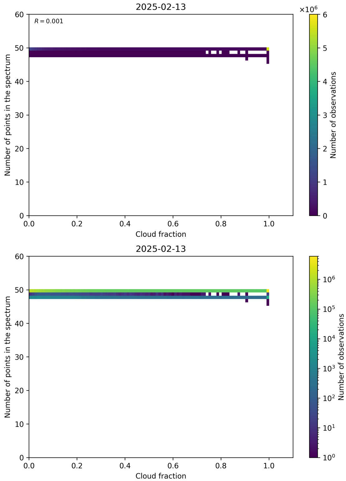
Figure 74: Scatter density plot of “Cloud fraction” against “Number of points in the spectrum” for 2025-02-13 to 2025-02-14.
