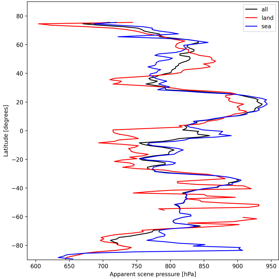
Figure 19: Zonal average of “Apparent scene pressure” for 2025-02-13 to 2025-02-14.
