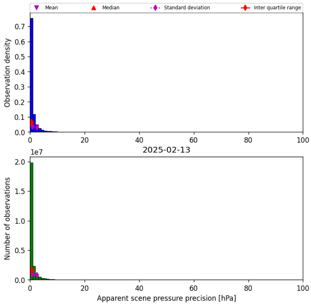
Figure 37: Histogram of “Apparent scene pressure precision” for 2025-02-13 to 2025-02-14
