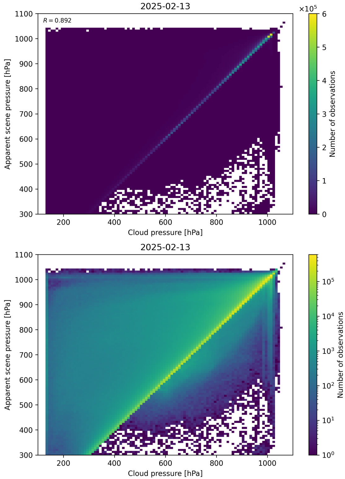
Figure 77: Scatter density plot of “Cloud pressure” against “Apparent scene pressure” for 2025-02-13 to 2025-02-14.
