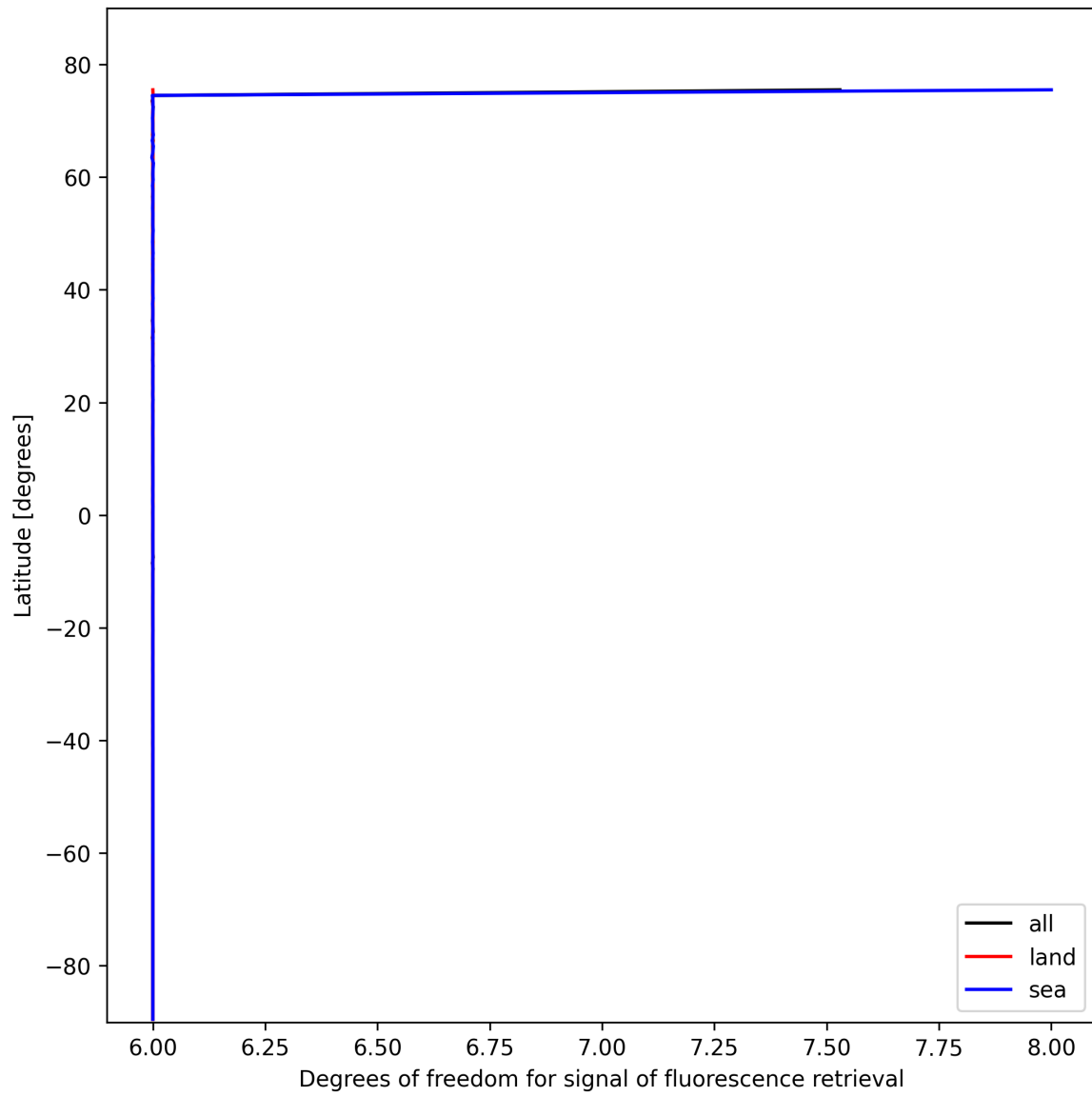
Figure 26: Zonal average of “Degrees of freedom for signal of fluorescence retrieval” for 2025-02-13 to 2025-02-14.
