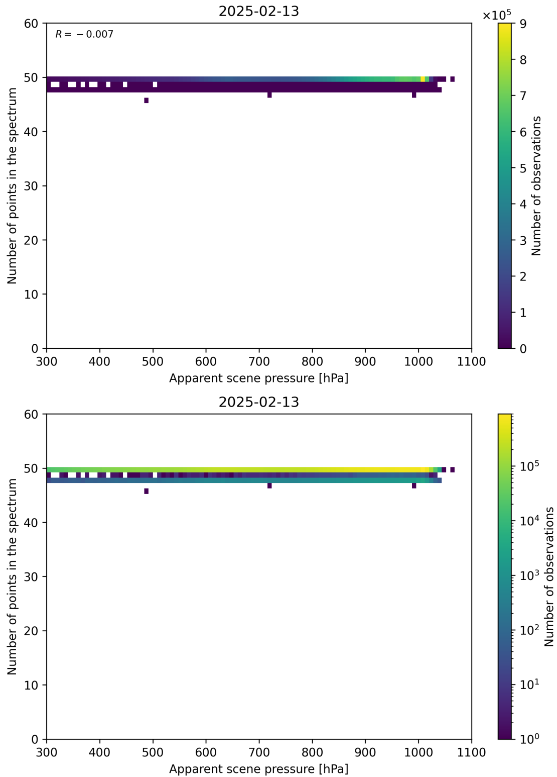
Figure 66: Scatter density plot of “Apparent scene pressure” against “Number of points in the spectrum” for 2025-02-13 to 2025-02-14.
