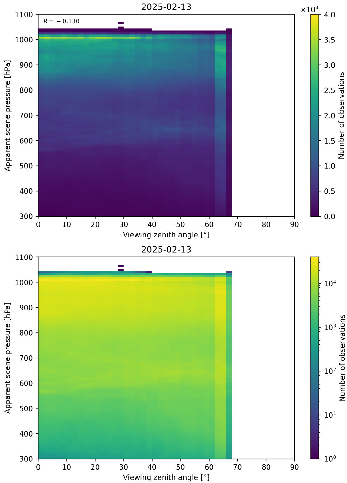
Figure 118: Scatter density plot of “Viewing zenith angle” against “Apparent scene pressure” for 2025-02-13 to 2025-02-14.
