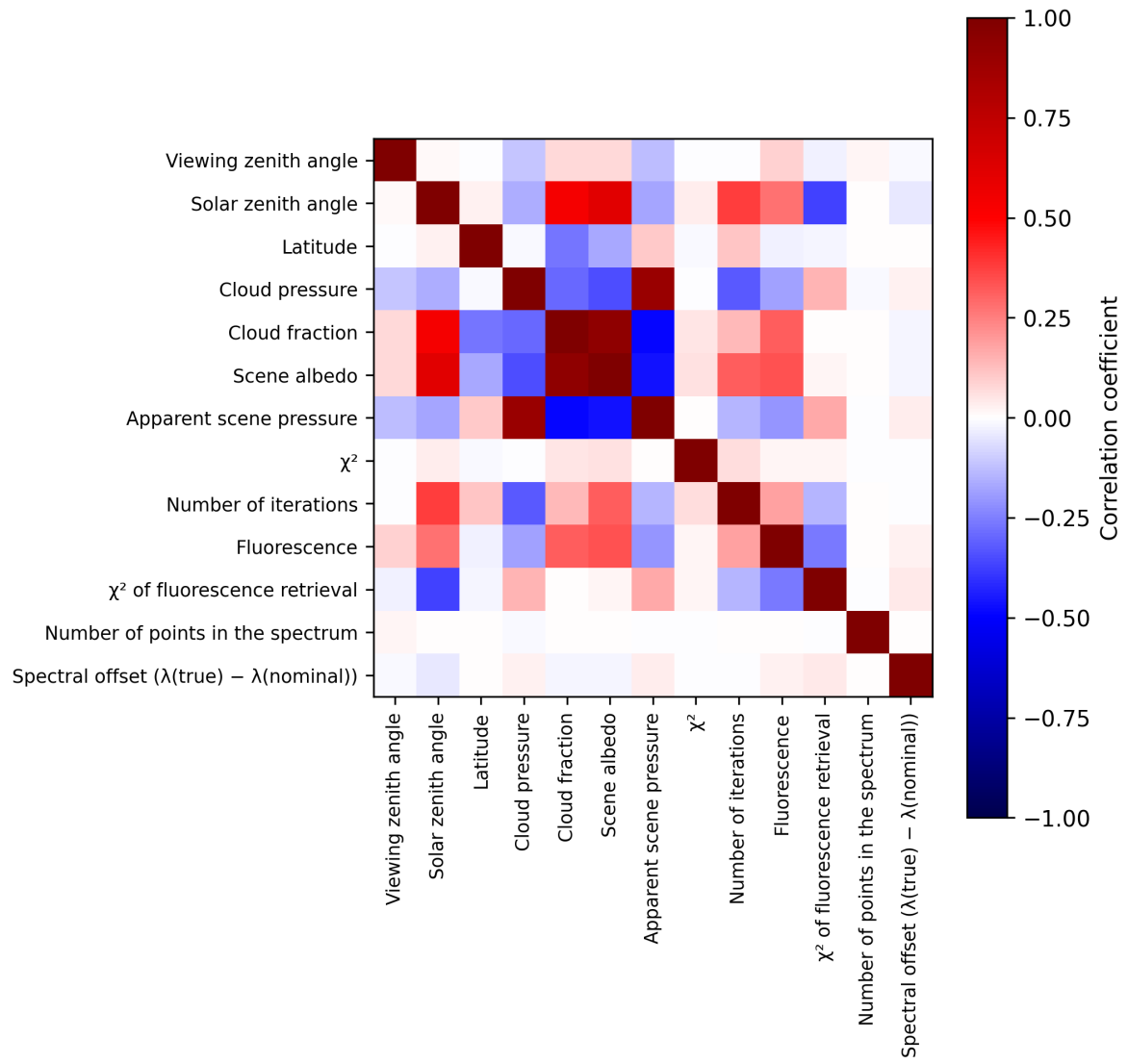
Figure 2: Map of correlation matrix for 2025-02-13 to 2025-02-14.
