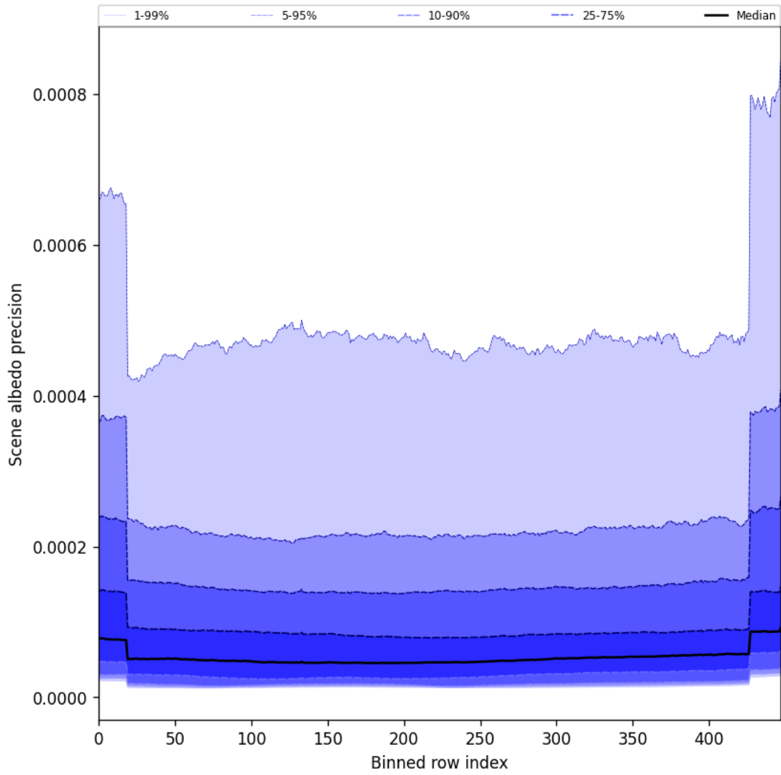
Figure 52: Along track statistics of “Scene albedo precision” for 2025-02-13 to 2025-02-14
