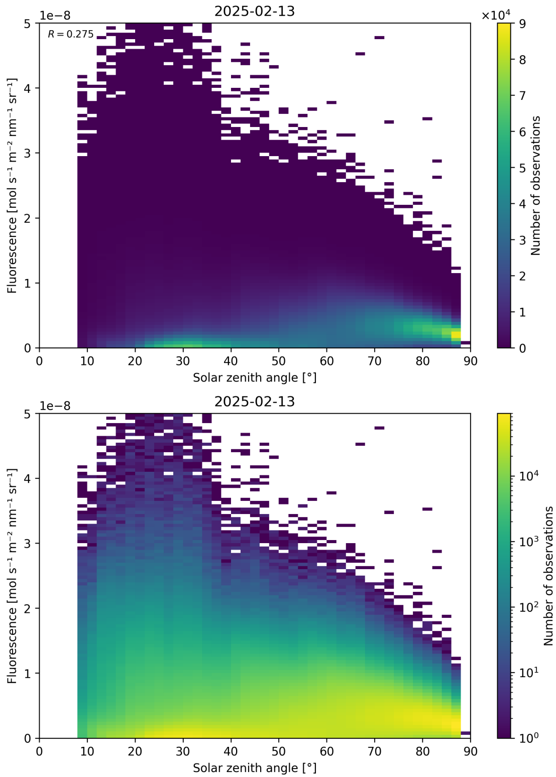
Figure 112: Scatter density plot of “Solar zenith angle” against “Fluorescence” for 2025-02-13 to 2025-02-14.
