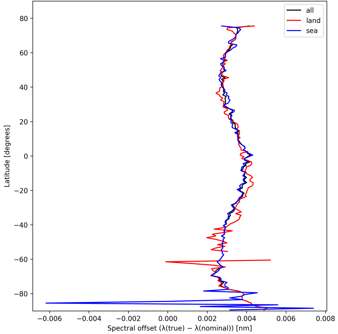
Figure 28: Zonal average of “Spectral offset ( \lambda_{\text{true}} - \lambda_{\text{nominal}} )” for 2025-02-13 to 2025-02-14.
