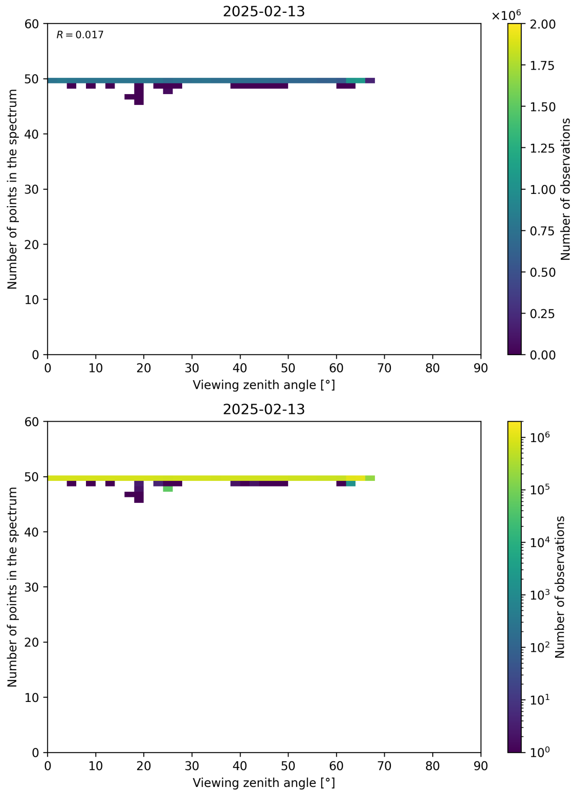
Figure 125: Scatter density plot of “Viewing zenith angle” against “Number of points in the spectrum” for 2025-02-13 to 2025-02-14.
