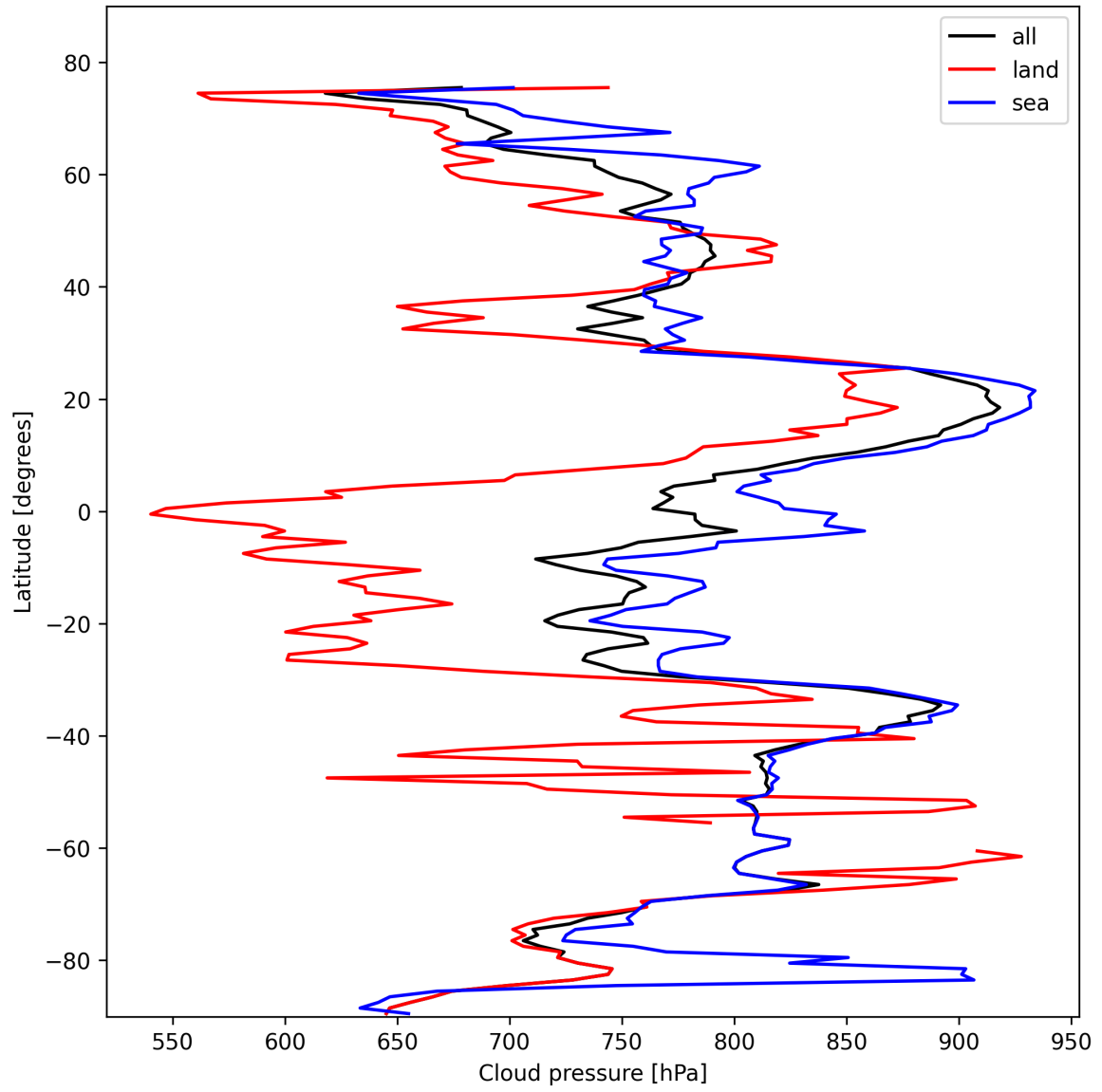
Figure 13: Zonal average of “Cloud pressure” for 2025-02-13 to 2025-02-14.
