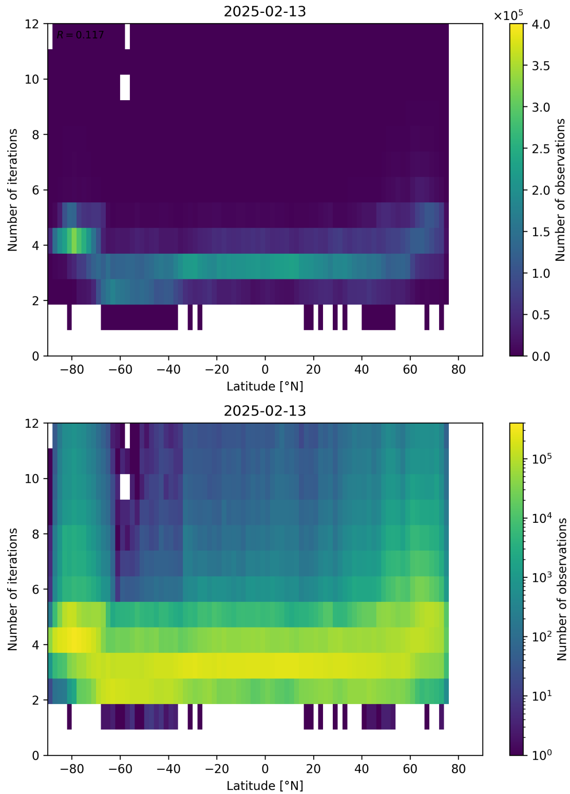
Figure 93: Scatter density plot of “Latitude” against “Number of iterations” for 2025-02-13 to 2025-02-14.
