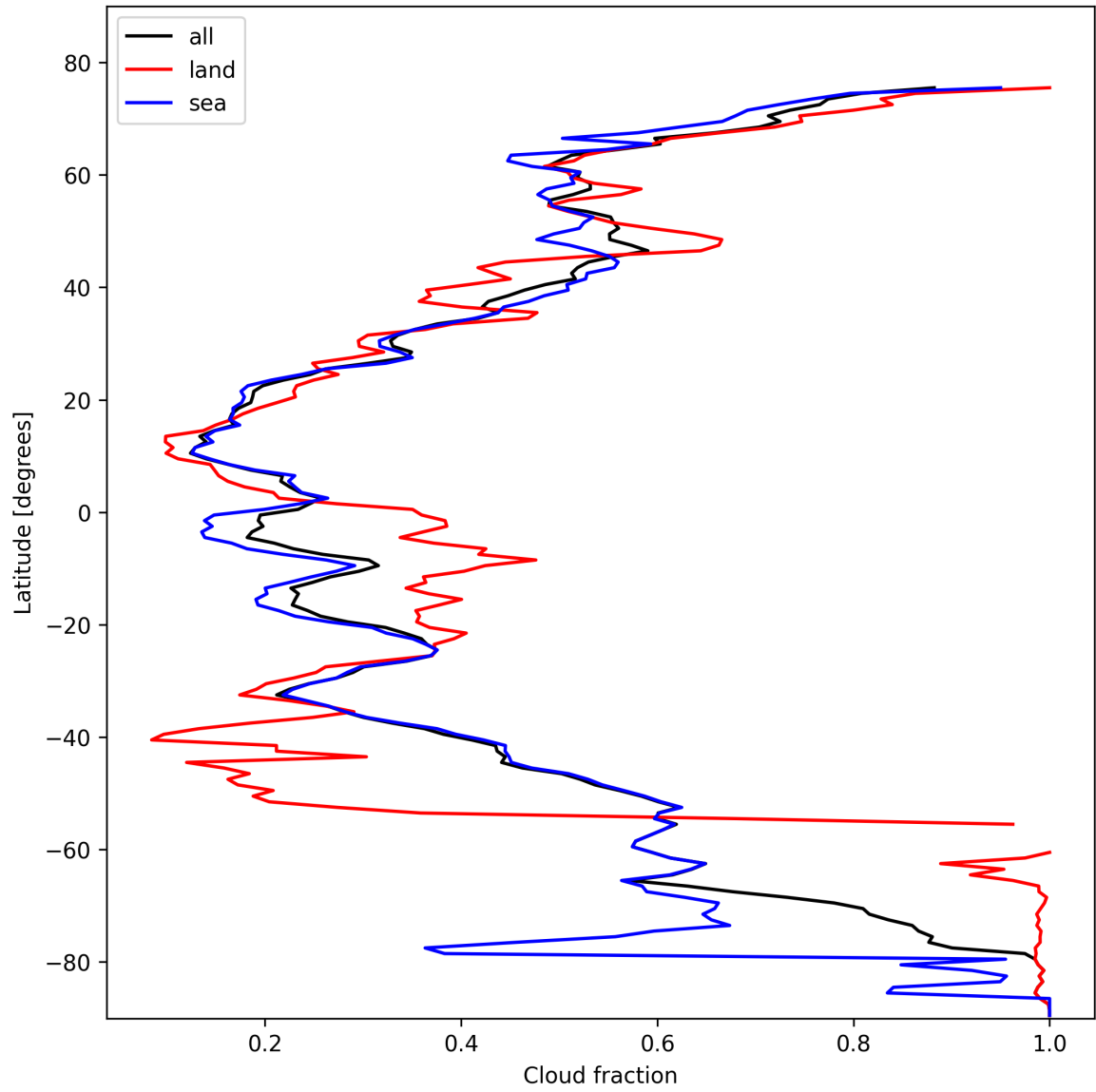
Figure 15: Zonal average of “Cloud fraction” for 2025-02-13 to 2025-02-14.
