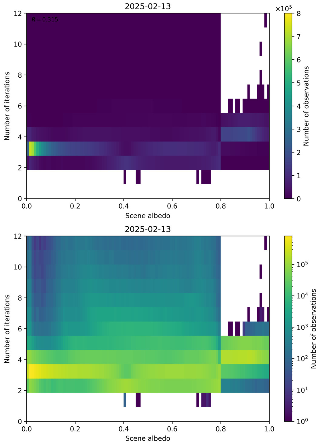
Figure 105: Scatter density plot of “Scene albedo” against “Number of iterations” for 2025-02-13 to 2025-02-14.
