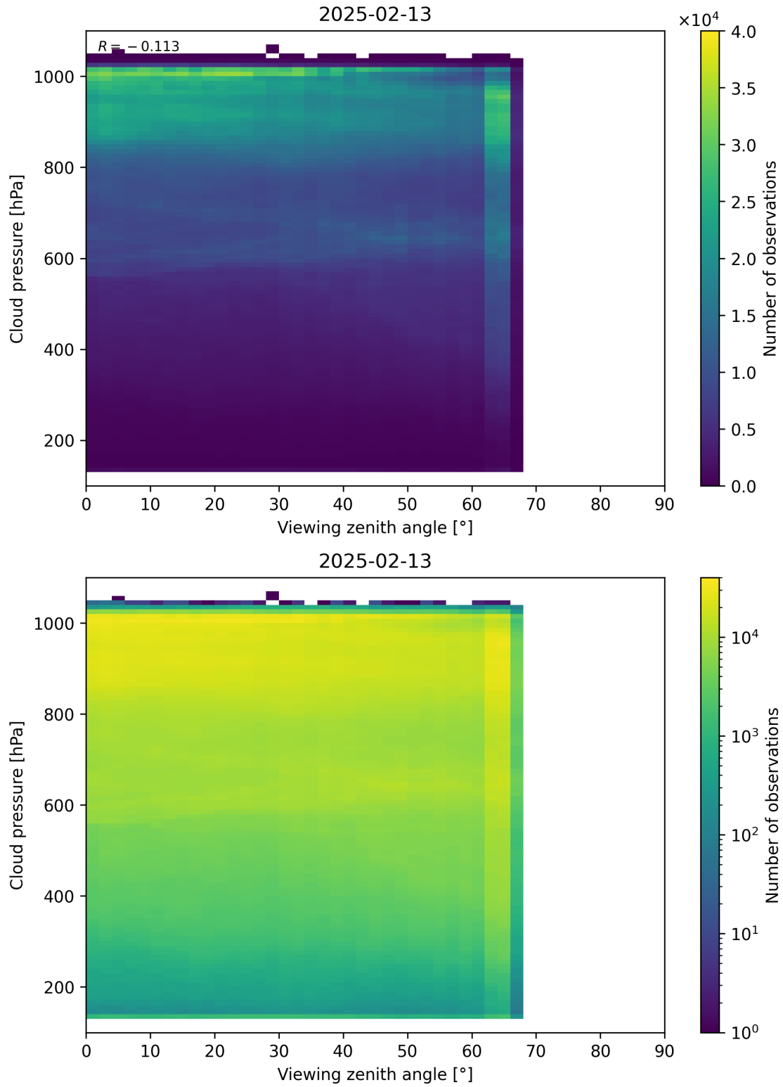
Figure 121: Scatter density plot of “Viewing zenith angle” against “Cloud pressure” for 2025-02-13 to 2025-02-14.
