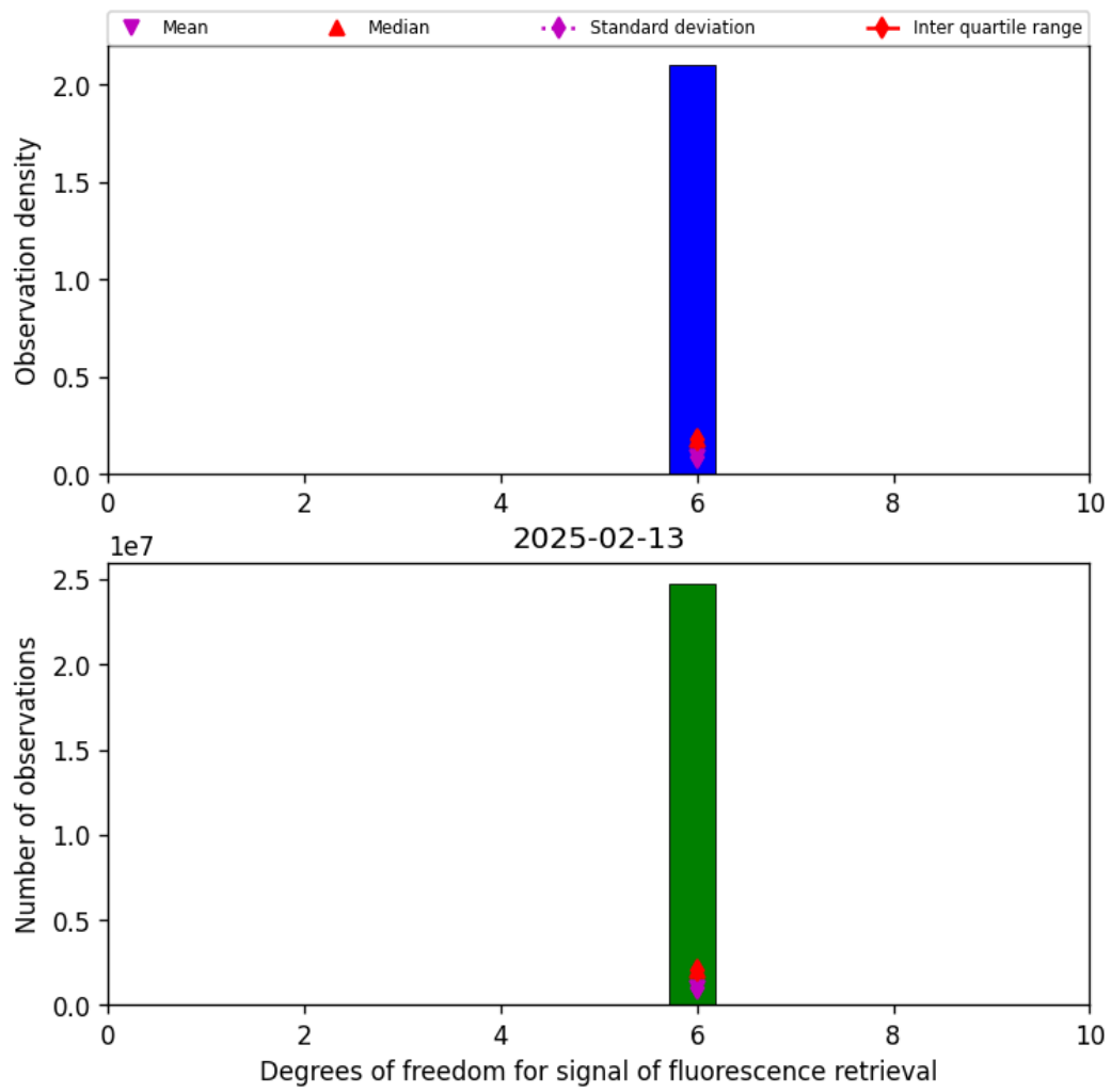
Figure 43: Histogram of “Degrees of freedom for signal of fluorescence retrieval” for 2025-02-13 to 2025-02-14
