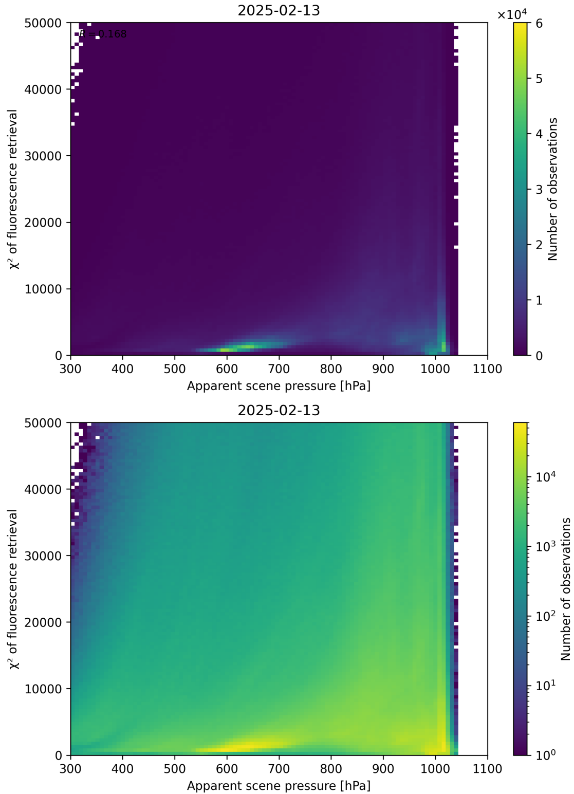
Figure 63: Scatter density plot of “Apparent scene pressure” against “ \chi^2 of fluorescence retrieval” for 2025-02-13 to 2025-02-14.
