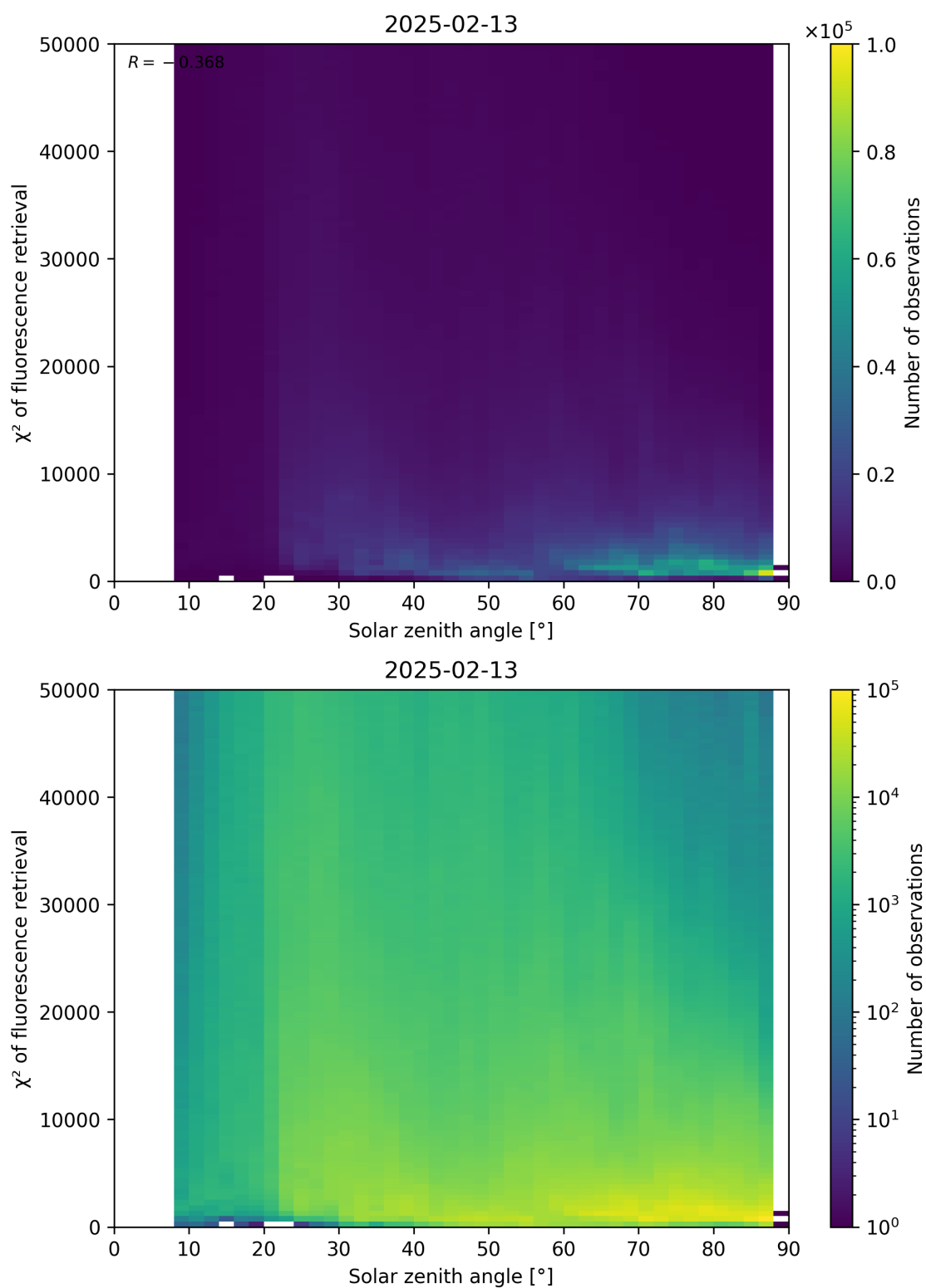
Figure 109: Scatter density plot of “Solar zenith angle” against “ \chi^2 of fluorescence retrieval” for 2025-02-13 to 2025-02-14.
