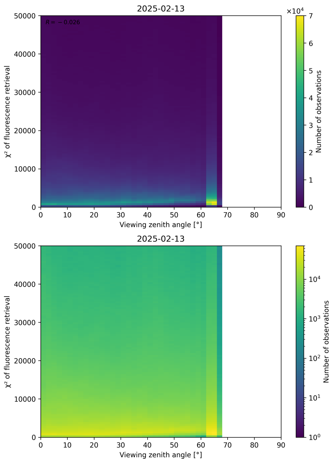
Figure 119: Scatter density plot of “Viewing zenith angle” against “ \chi^2 of fluorescence retrieval” for 2025-02-13 to 2025-02-14.
