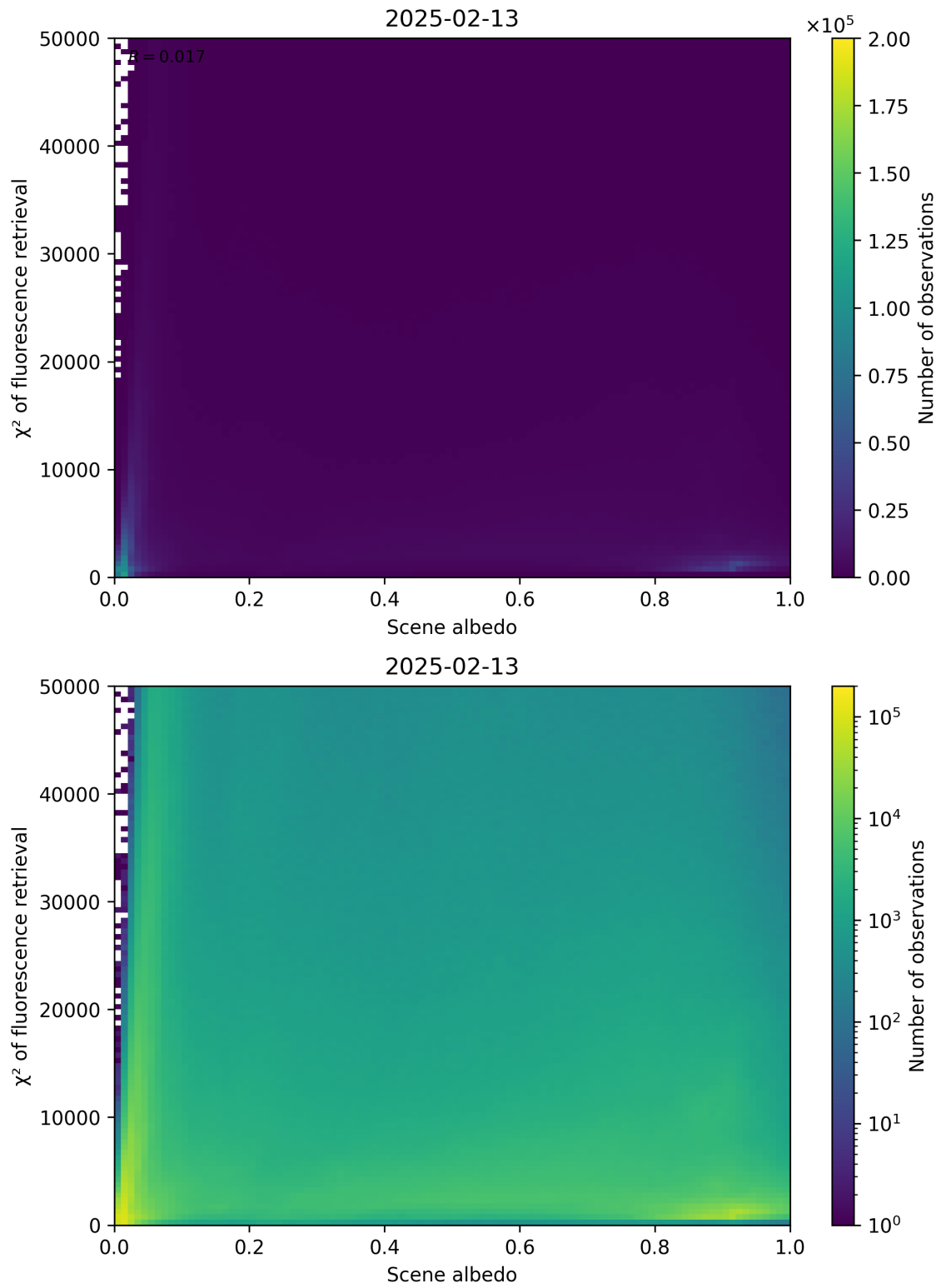
Figure 103: Scatter density plot of “Scene albedo” against “ \chi^2 of fluorescence retrieval” for 2025-02-13 to 2025-02-14.
