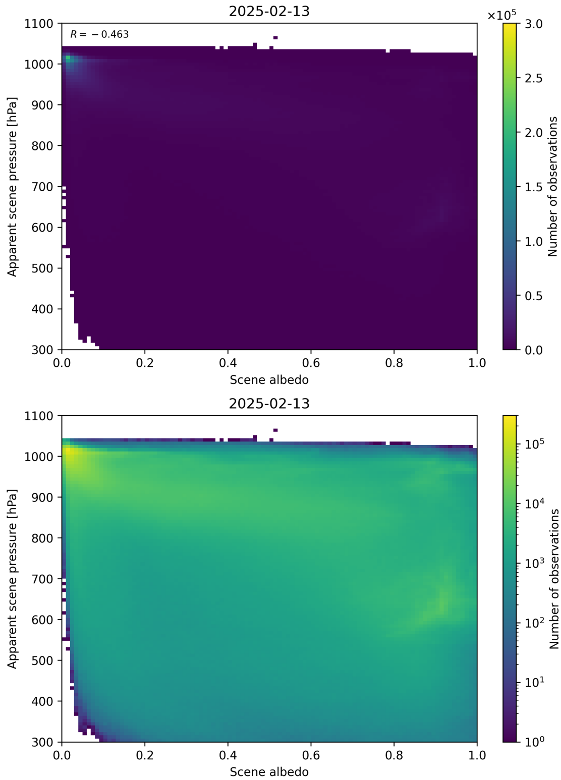
Figure 102: Scatter density plot of “Scene albedo” against “Apparent scene pressure” for 2025-02-13 to 2025-02-14.
