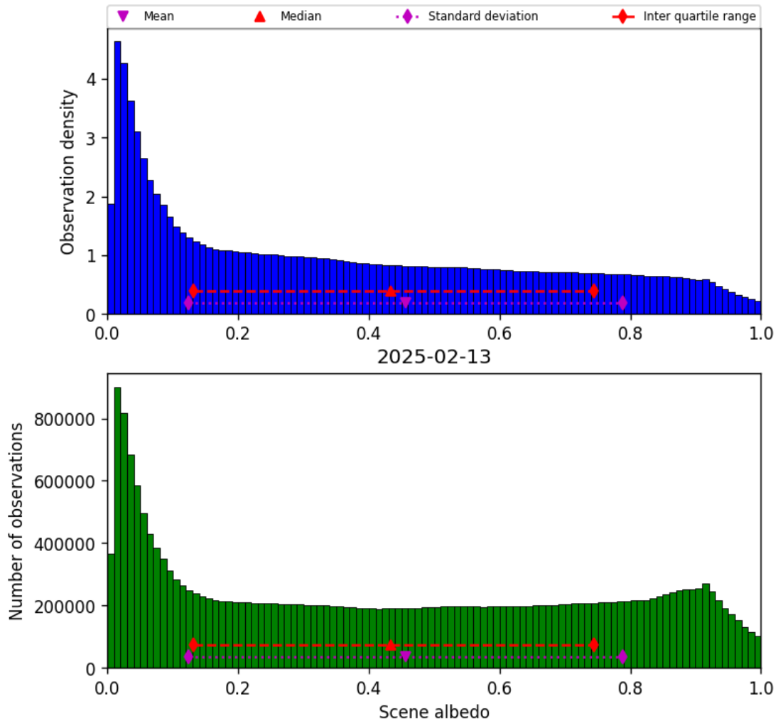
Figure 34: Histogram of “Scene albedo” for 2025-02-13 to 2025-02-14
