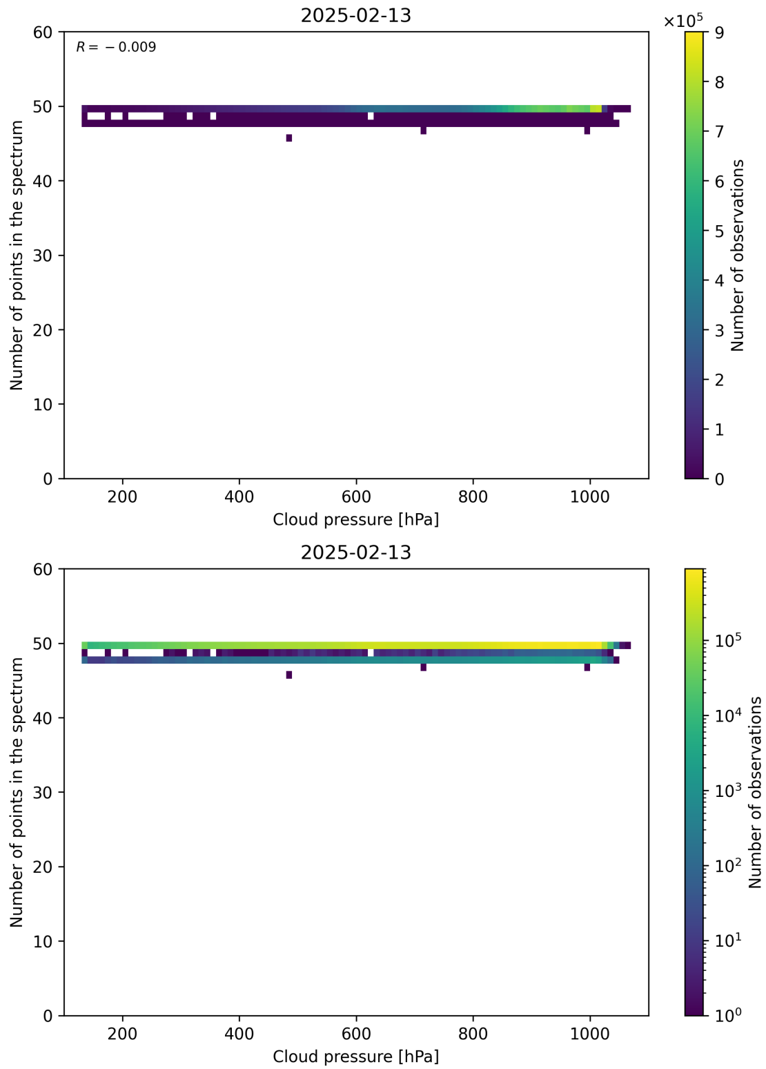
Figure 82: Scatter density plot of “Cloud pressure” against “Number of points in the spectrum” for 2025-02-13 to 2025-02-14.
