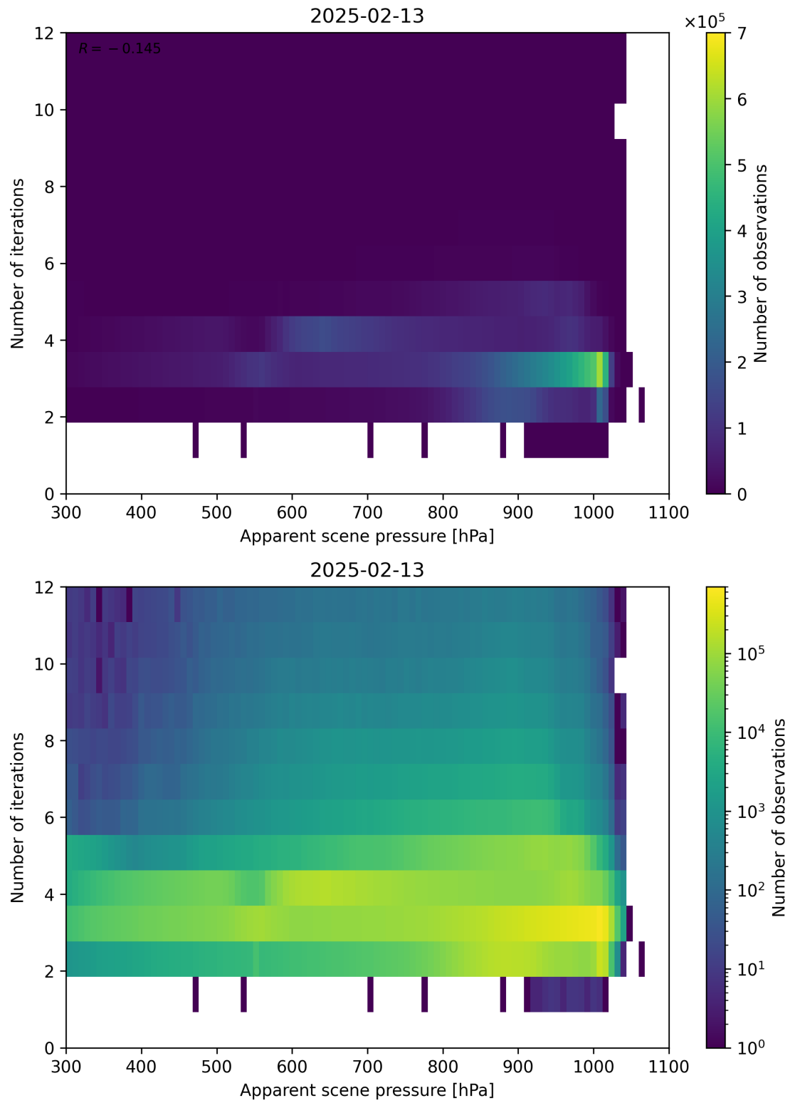
Figure 65: Scatter density plot of “Apparent scene pressure” against “Number of iterations” for 2025-02-13 to 2025-02-14.
