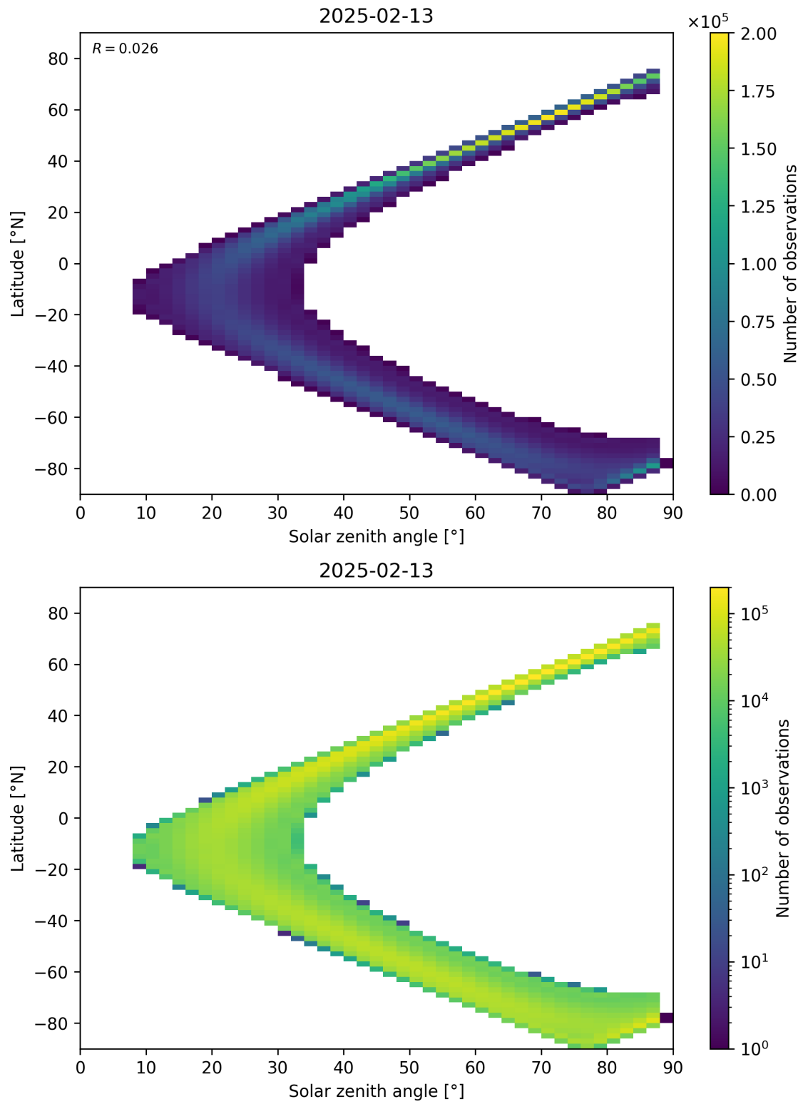
Figure 113: Scatter density plot of “Solar zenith angle” against “Latitude” for 2025-02-13 to 2025-02-14.
