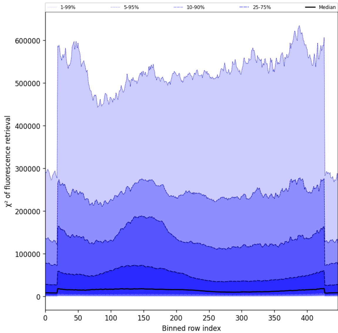
Figure 59: Along track statistics of “ \chi^2 of fluorescence retrieval” for 2025-02-13 to 2025-02-14
