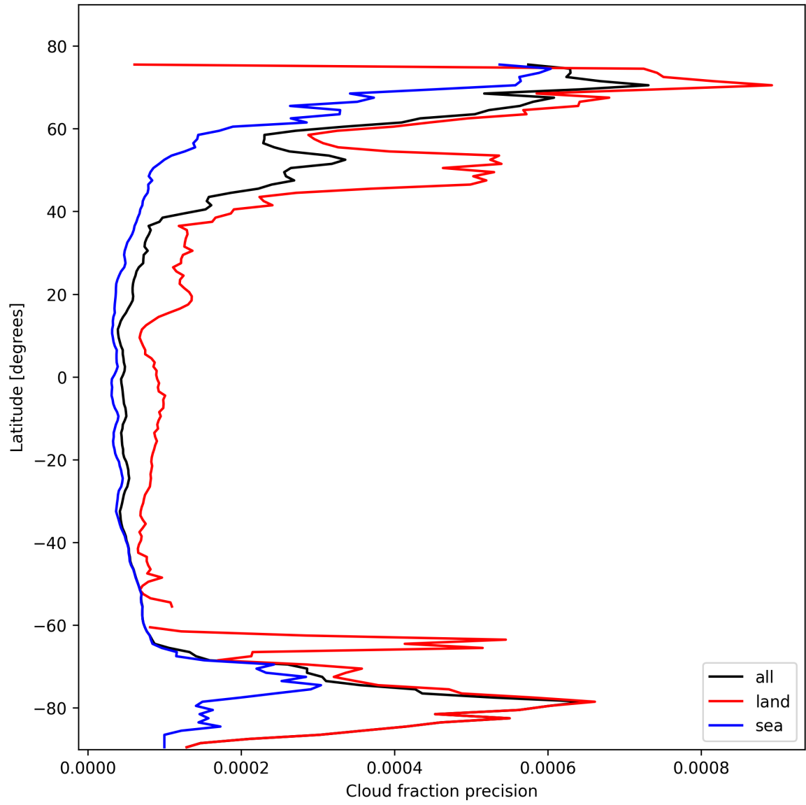
Figure 16: Zonal average of “Cloud fraction precision” for 2025-02-13 to 2025-02-14.
