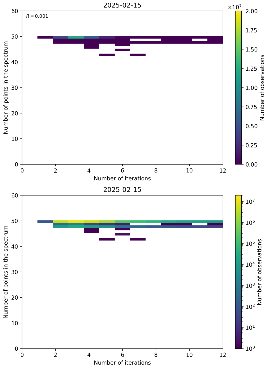
Figure 99: Scatter density plot of “Number of iterations” against “Number of points in the spectrum” for 2025-02-14 to 2025-02-16.
