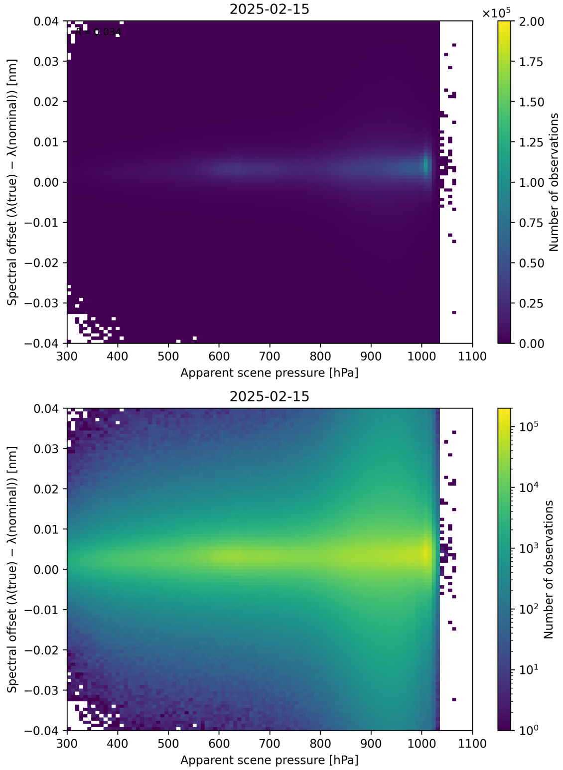
Figure 67: Scatter density plot of “Apparent scene pressure” against “Spectral offset ( \lambda_{\text{true}} - \lambda_{\text{nominal}} )” for 2025-02-14 to 2025-02-16.
