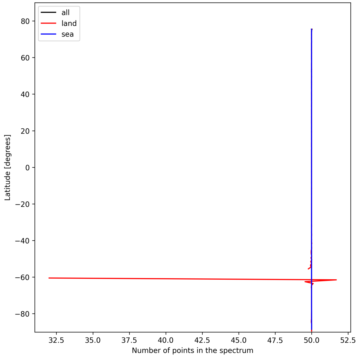
Figure 27: Zonal average of “Number of points in the spectrum” for 2025-02-14 to 2025-02-16.
