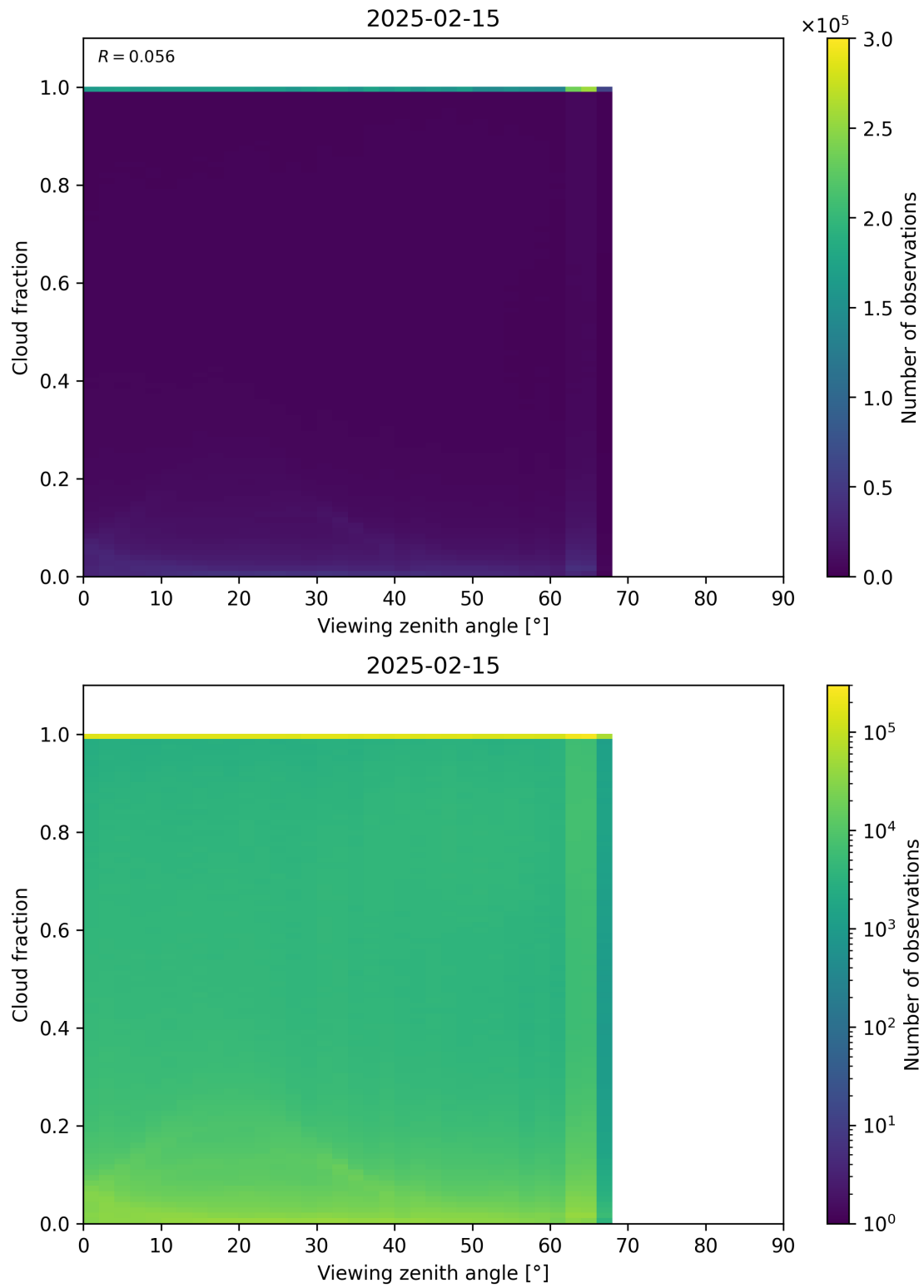
Figure 120: Scatter density plot of “Viewing zenith angle” against “Cloud fraction” for 2025-02-14 to 2025-02-16.
