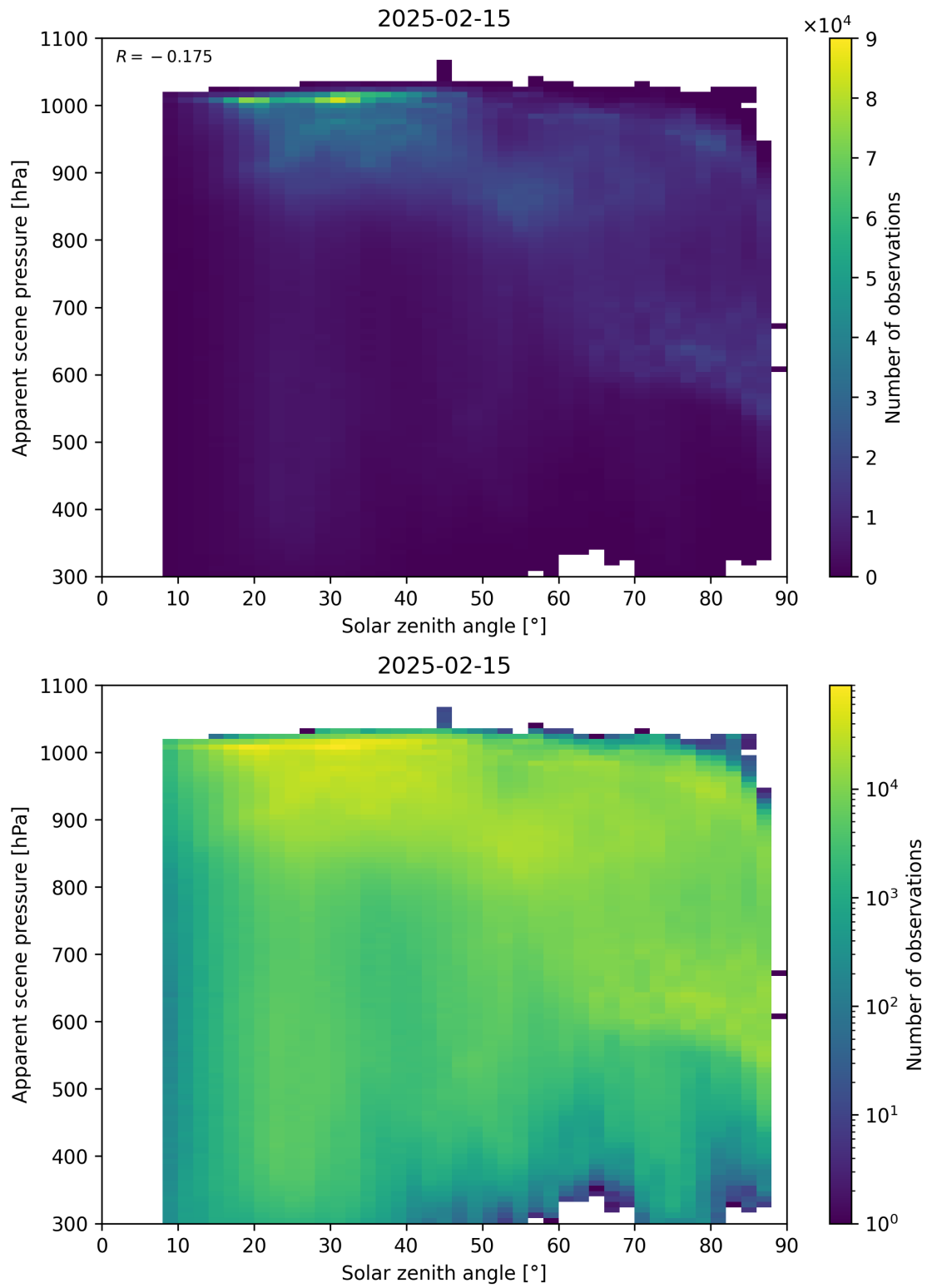
Figure 108: Scatter density plot of “Solar zenith angle” against “Apparent scene pressure” for 2025-02-14 to 2025-02-16.
