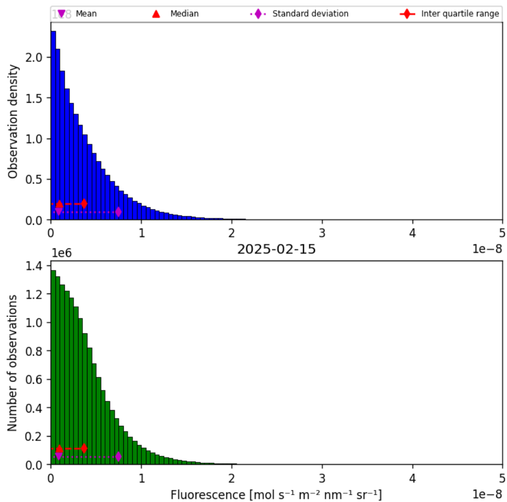
Figure 40: Histogram of “Fluorescence” for 2025-02-14 to 2025-02-16
