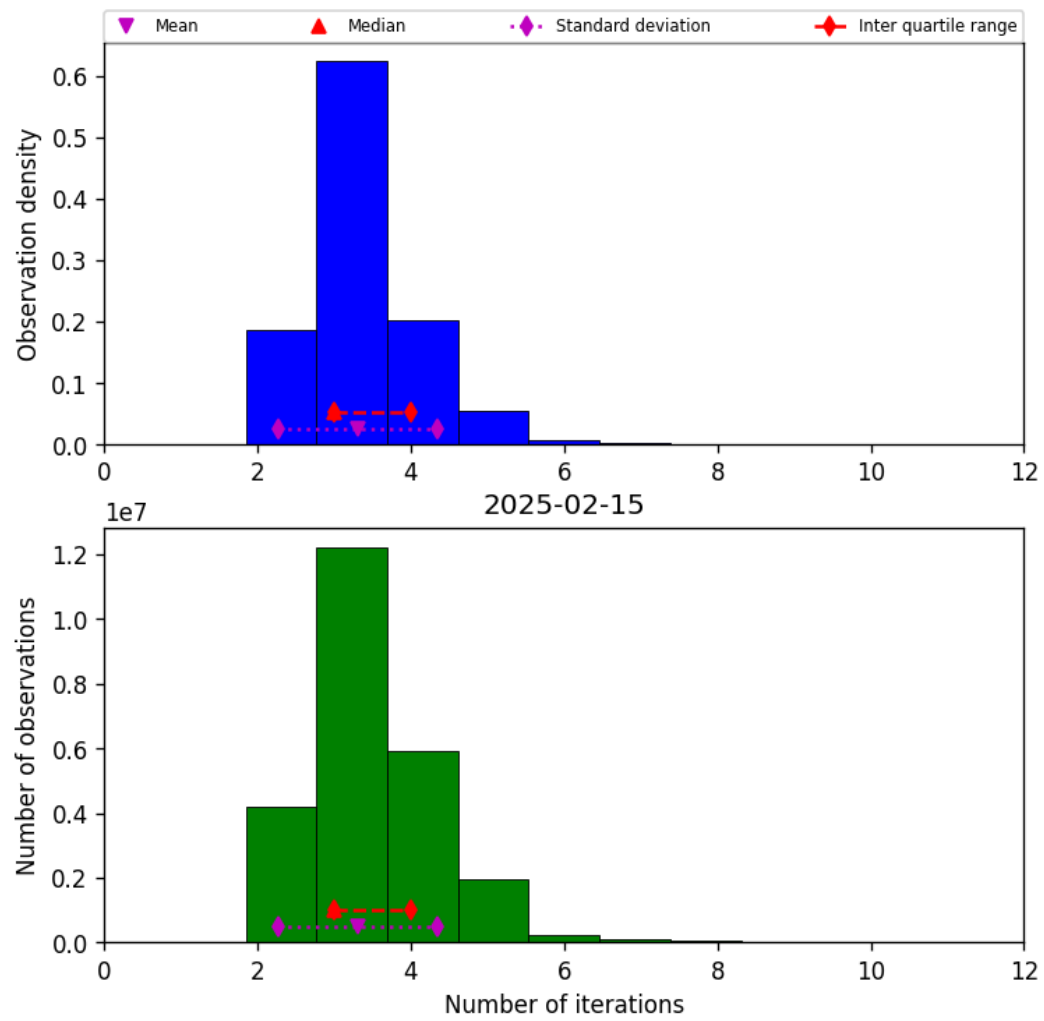
Figure 39: Histogram of “Number of iterations” for 2025-02-14 to 2025-02-16
