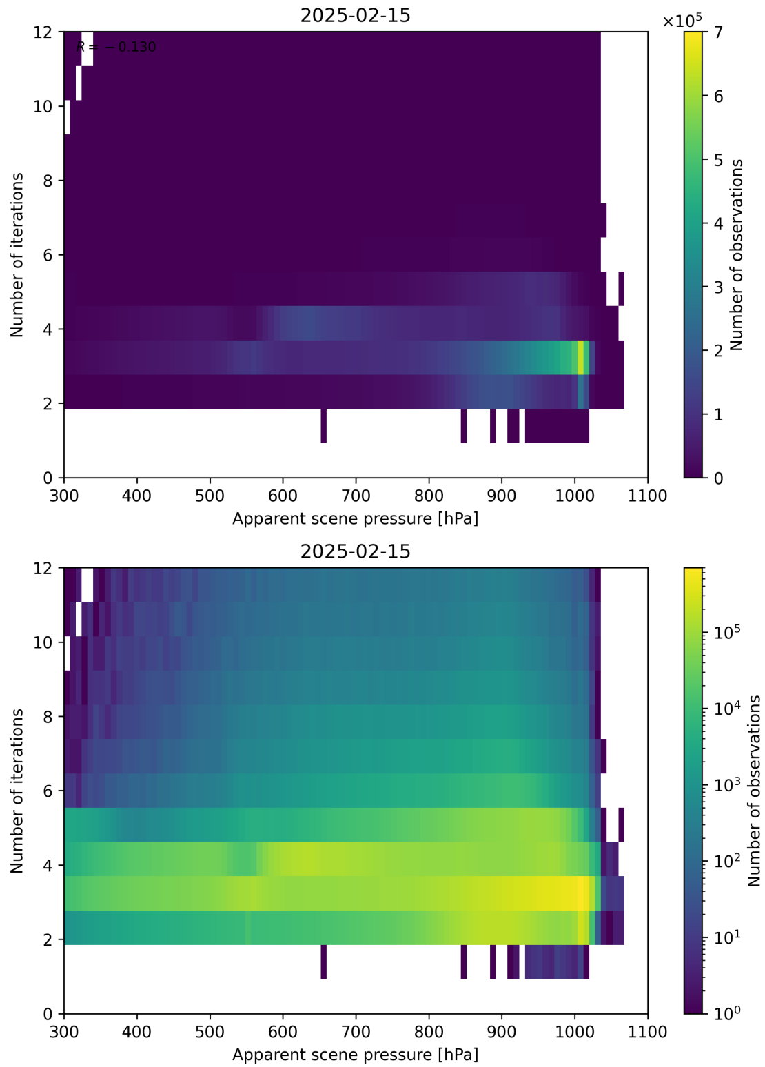
Figure 65: Scatter density plot of “Apparent scene pressure” against “Number of iterations” for 2025-02-14 to 2025-02-16.
