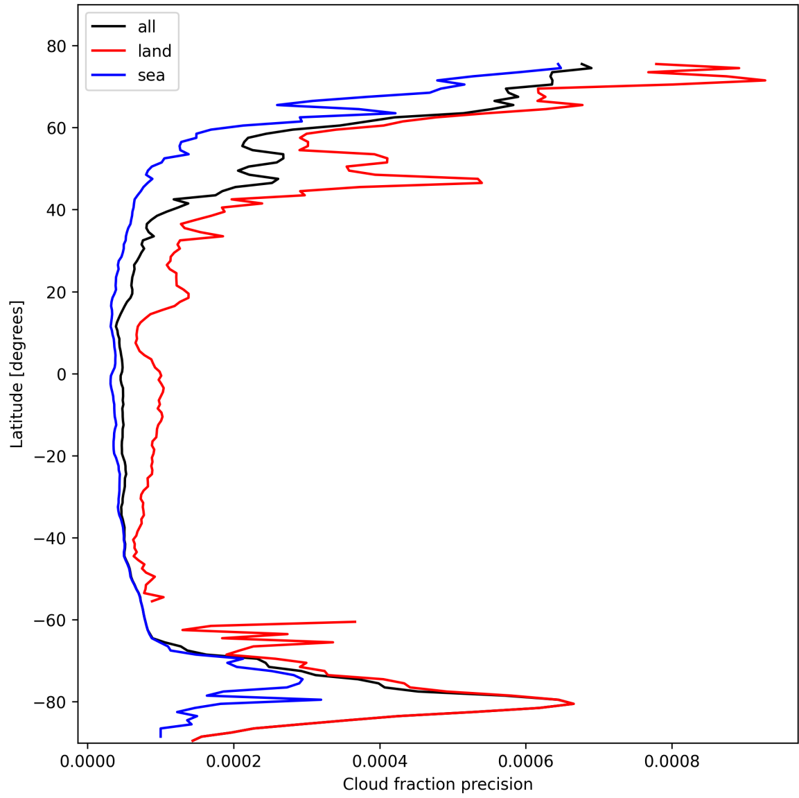
Figure 16: Zonal average of “Cloud fraction precision” for 2025-02-14 to 2025-02-16.
