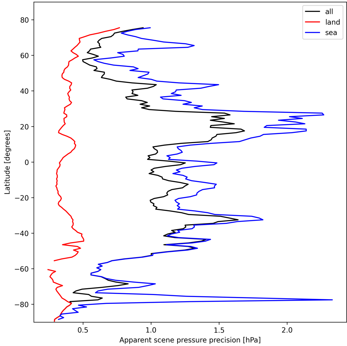
Figure 20: Zonal average of “Apparent scene pressure precision” for 2025-02-14 to 2025-02-16.
