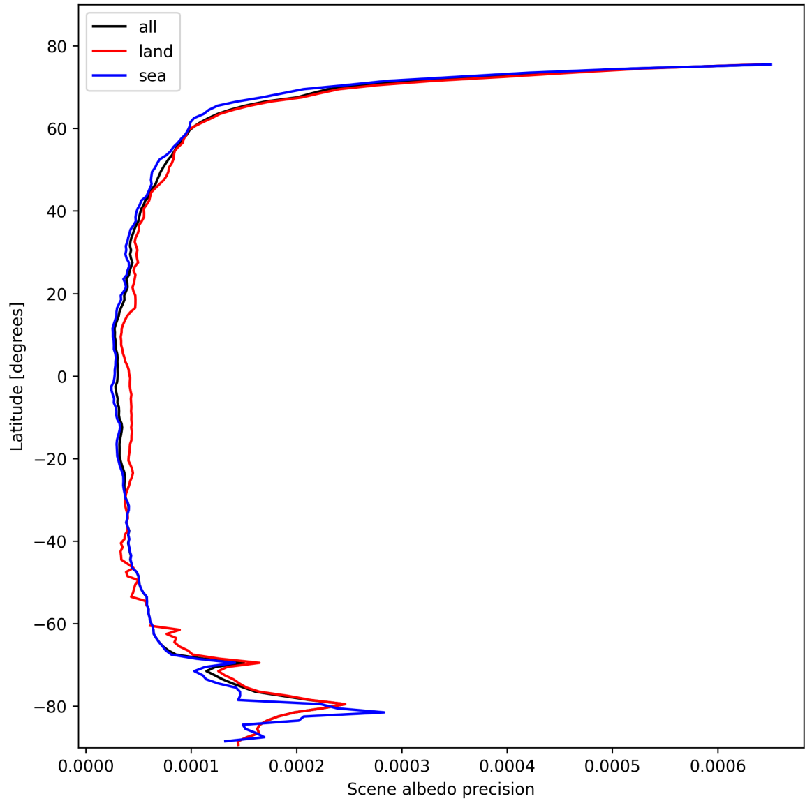
Figure 18: Zonal average of “Scene albedo precision” for 2025-02-14 to 2025-02-16.
