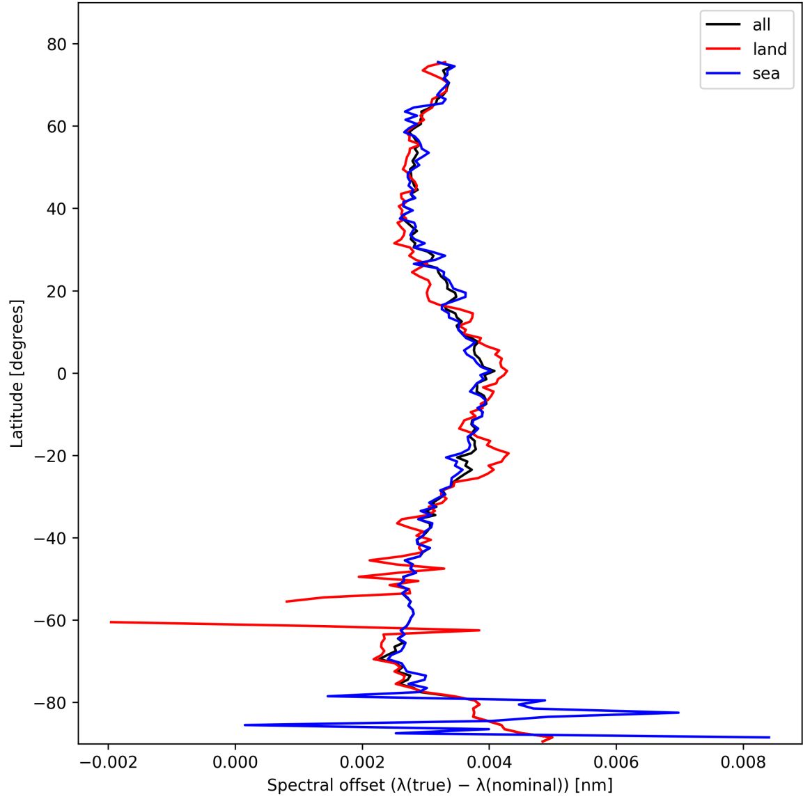
Figure 28: Zonal average of “Spectral offset ( \lambda_{\text{true}} - \lambda_{\text{nominal}} )” for 2025-02-14 to 2025-02-16.
