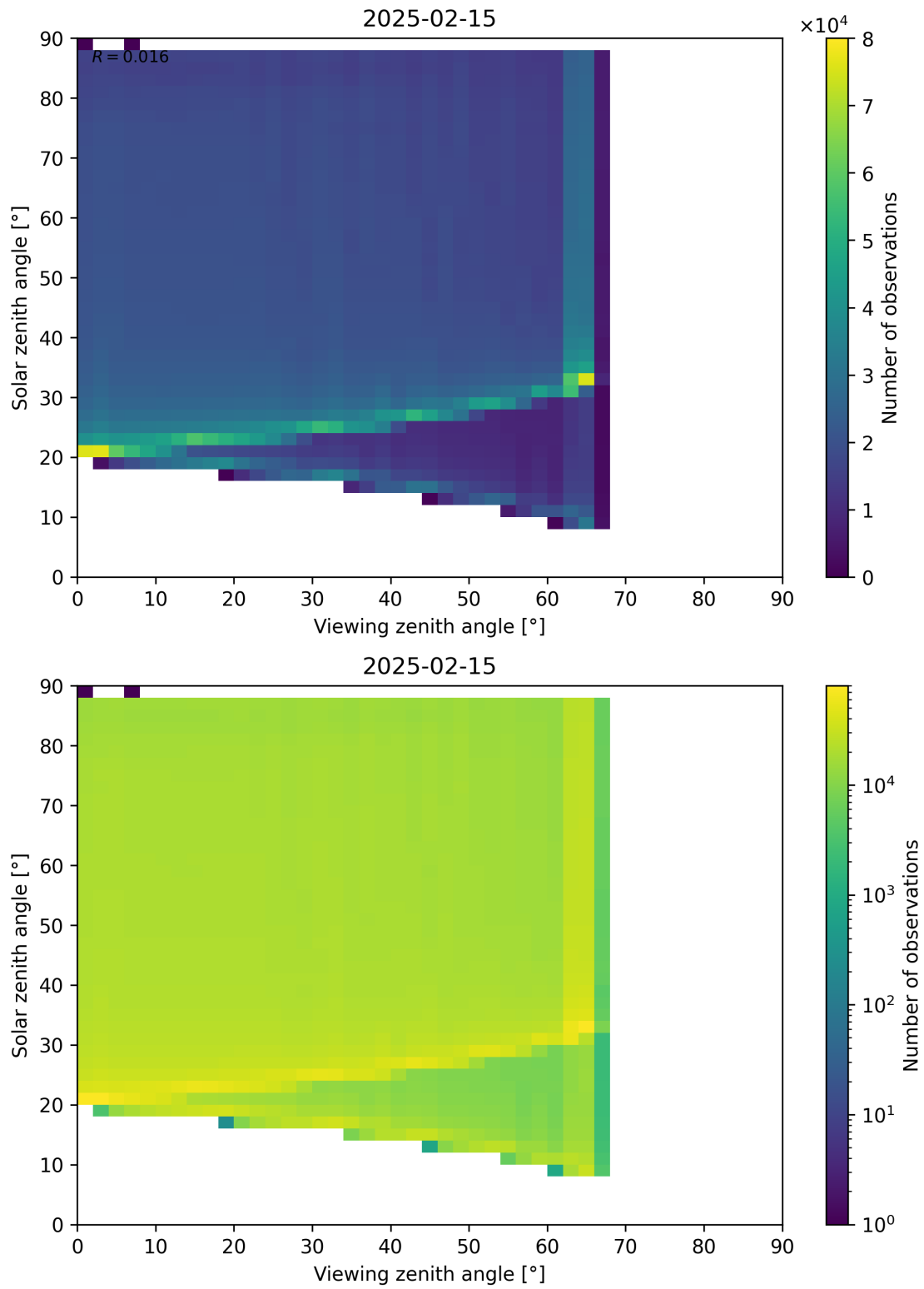
Figure 127: Scatter density plot of “Viewing zenith angle” against “Solar zenith angle” for 2025-02-14 to 2025-02-16.
