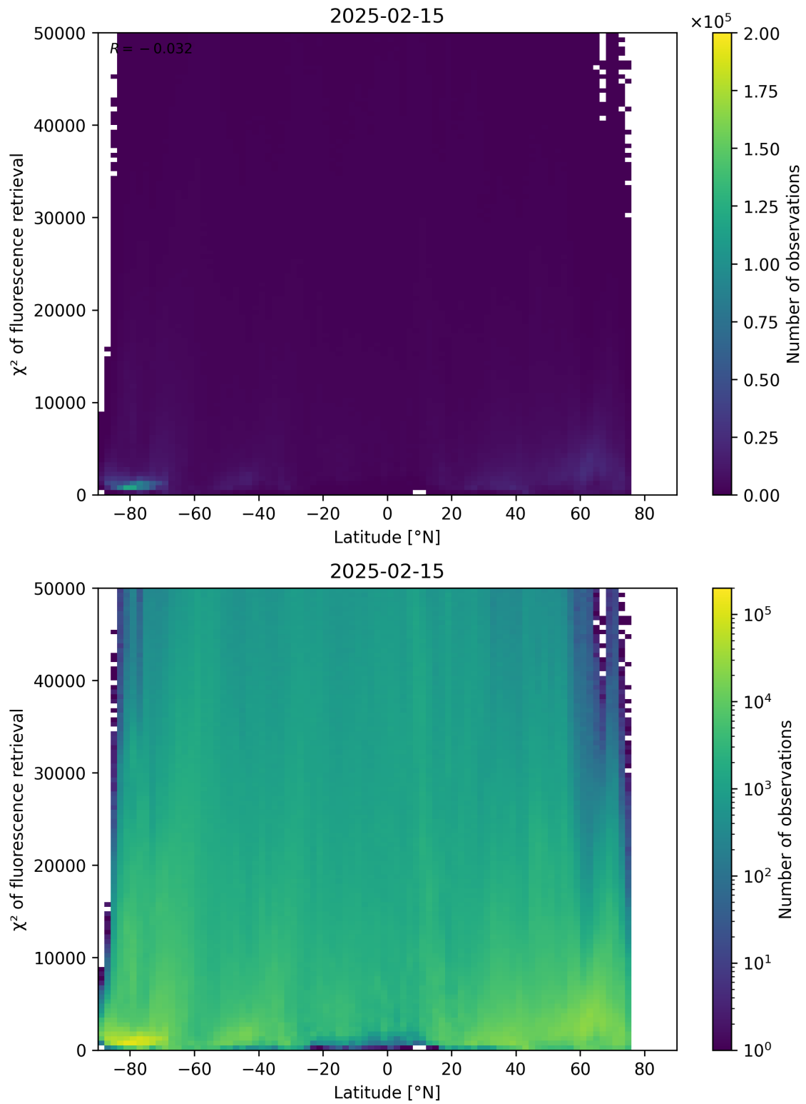
Figure 89: Scatter density plot of “Latitude” against “ \chi^2 of fluorescence retrieval” for 2025-02-14 to 2025-02-16.
