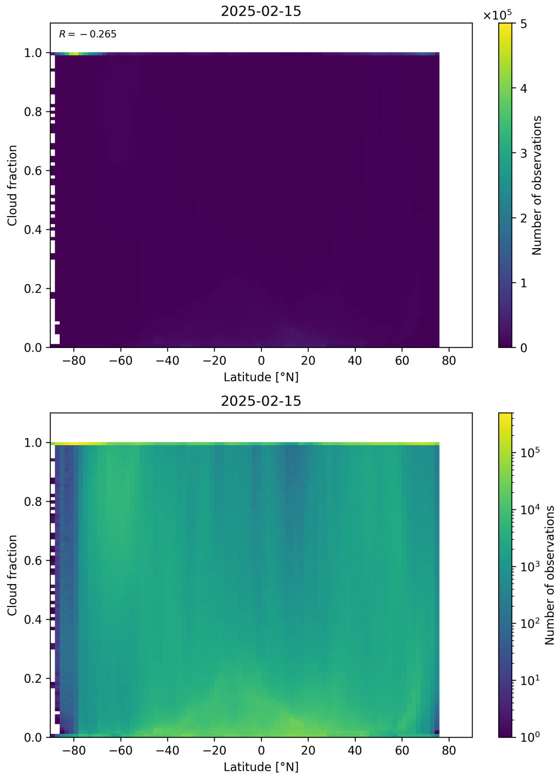
Figure 90: Scatter density plot of “Latitude” against “Cloud fraction” for 2025-02-14 to 2025-02-16.
