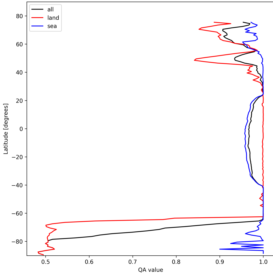
Figure 12: Zonal average of “QA value” for 2025-02-14 to 2025-02-16.
