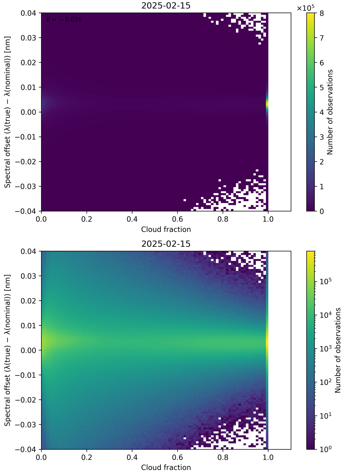
Figure 76: Scatter density plot of “Cloud fraction” against “Spectral offset ( \lambda_{\text{true}} - \lambda_{\text{nominal}} )” for 2025-02-14 to 2025-02-16.
