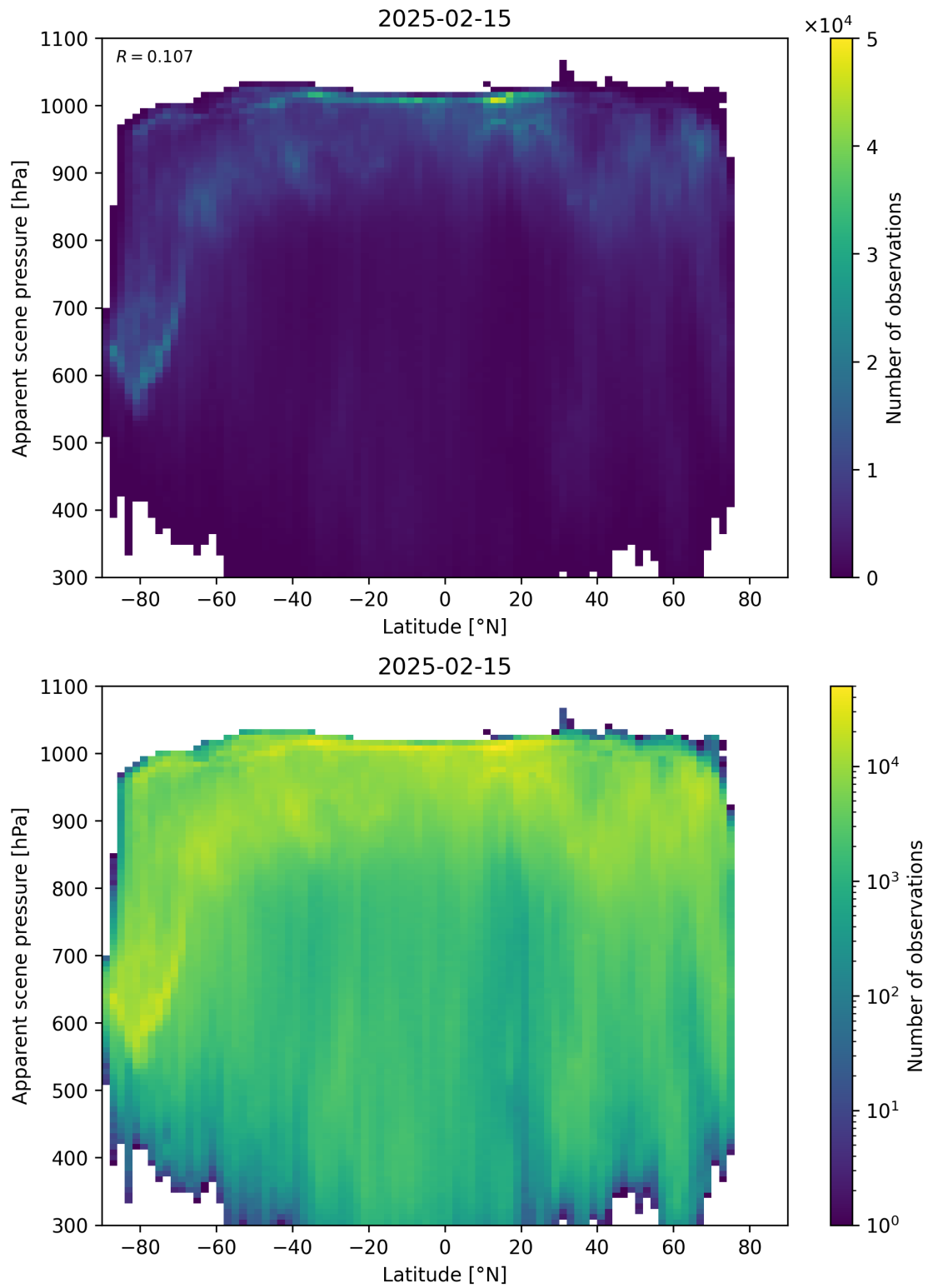
Figure 88: Scatter density plot of “Latitude” against “Apparent scene pressure” for 2025-02-14 to 2025-02-16.
