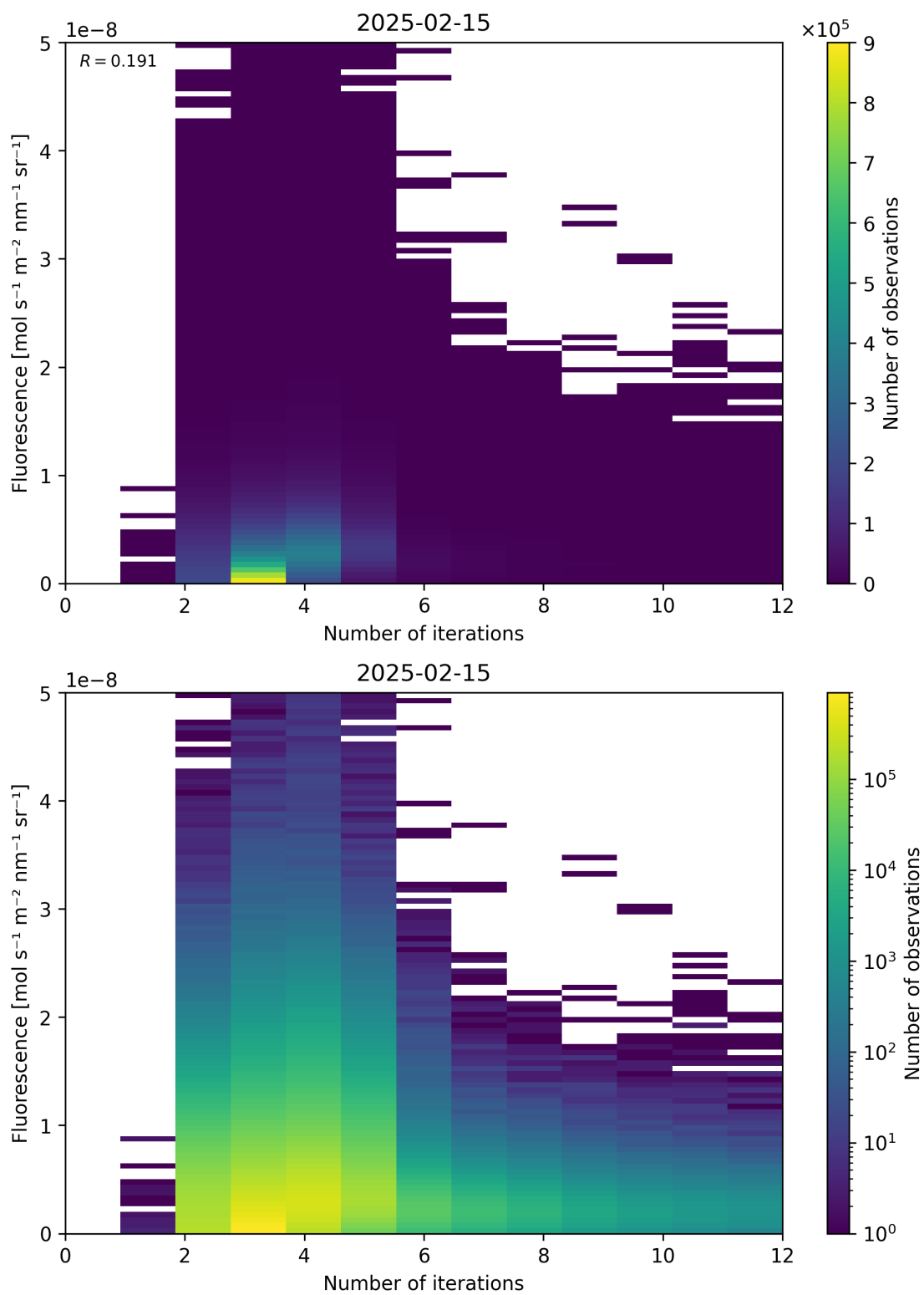
Figure 98: Scatter density plot of “Number of iterations” against “Fluorescence” for 2025-02-14 to 2025-02-16.
