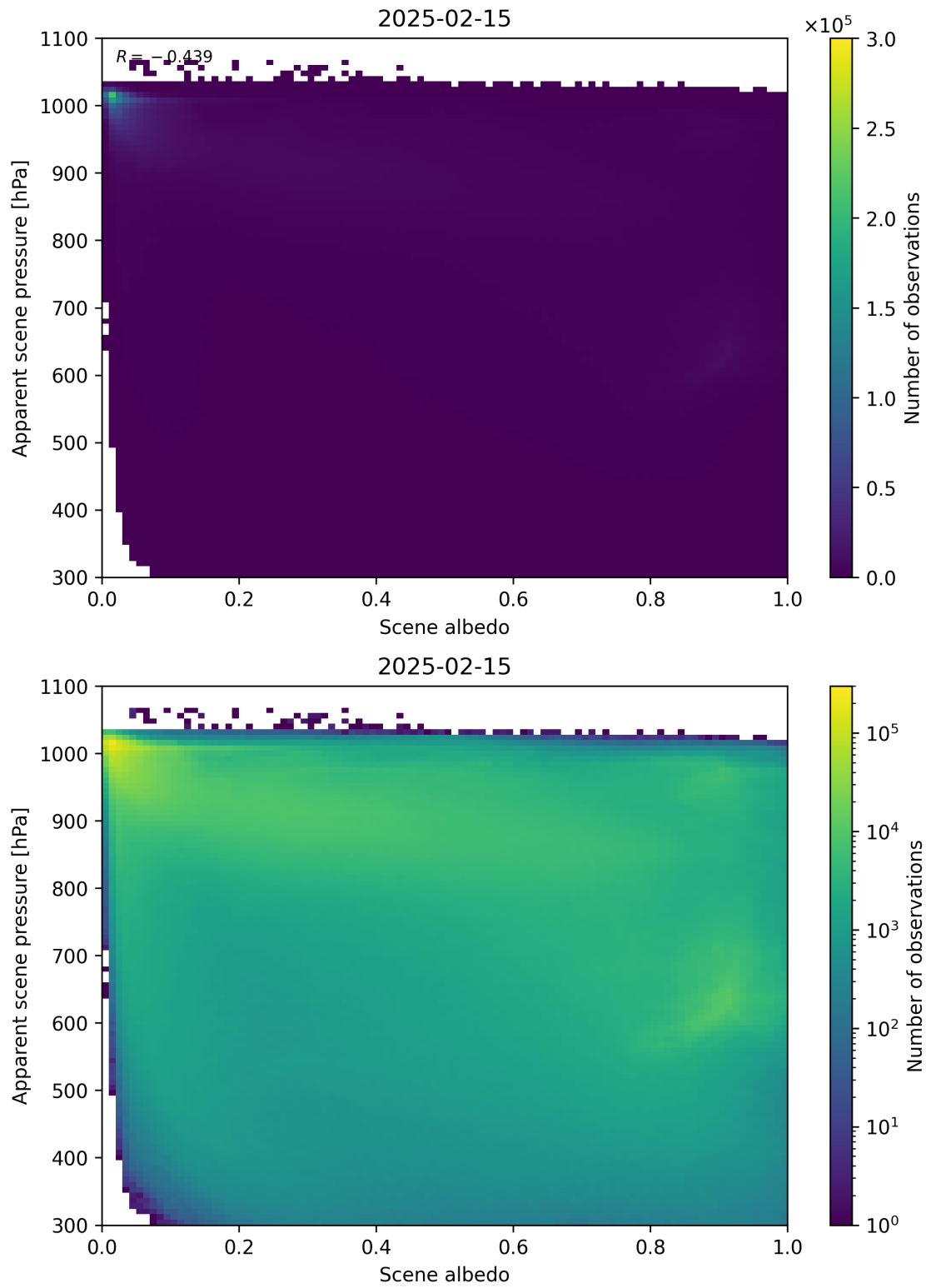
Figure 102: Scatter density plot of “Scene albedo” against “Apparent scene pressure” for 2025-02-14 to 2025-02-16.
