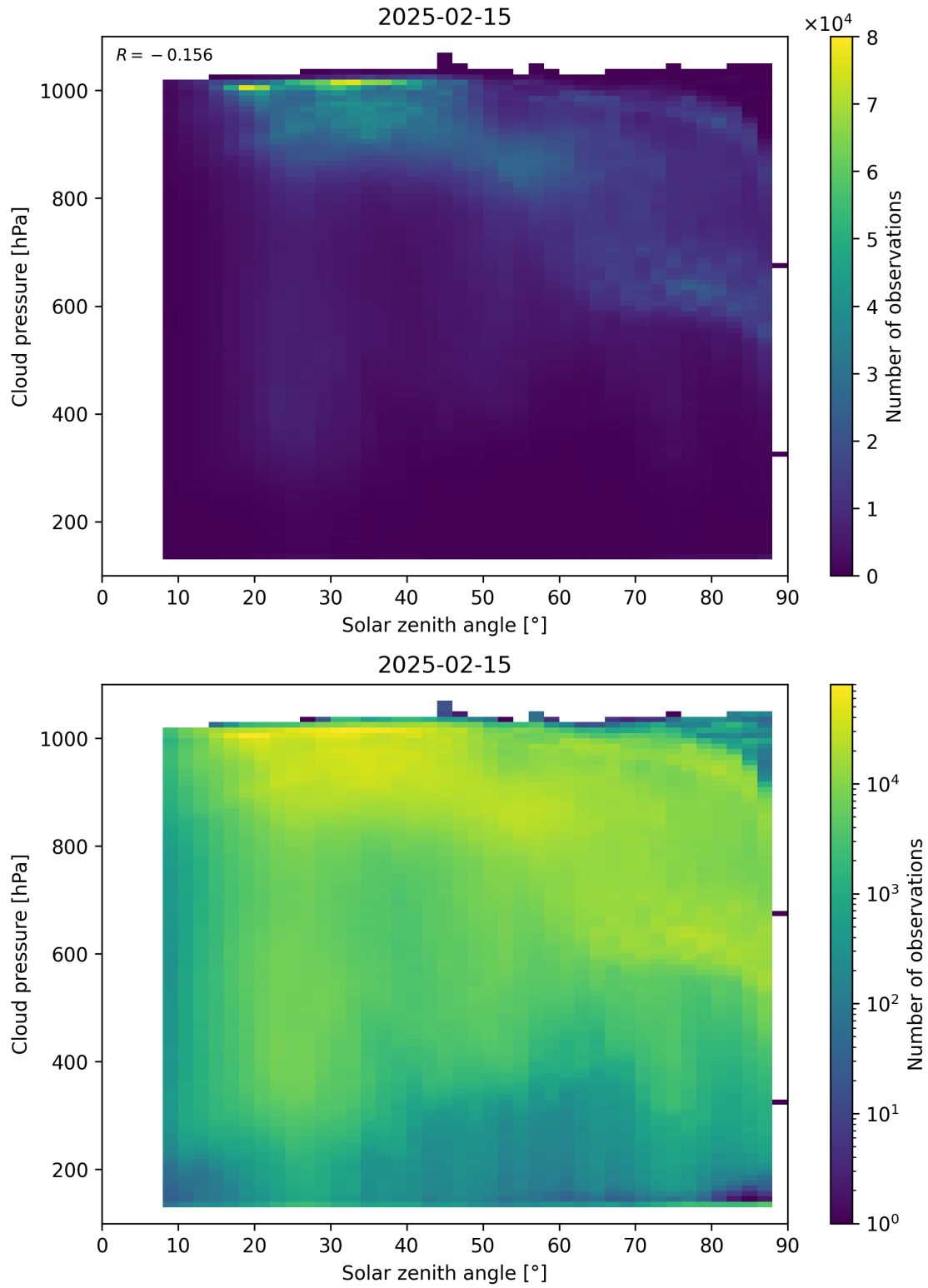
Figure 111: Scatter density plot of “Solar zenith angle” against “Cloud pressure” for 2025-02-14 to 2025-02-16.
