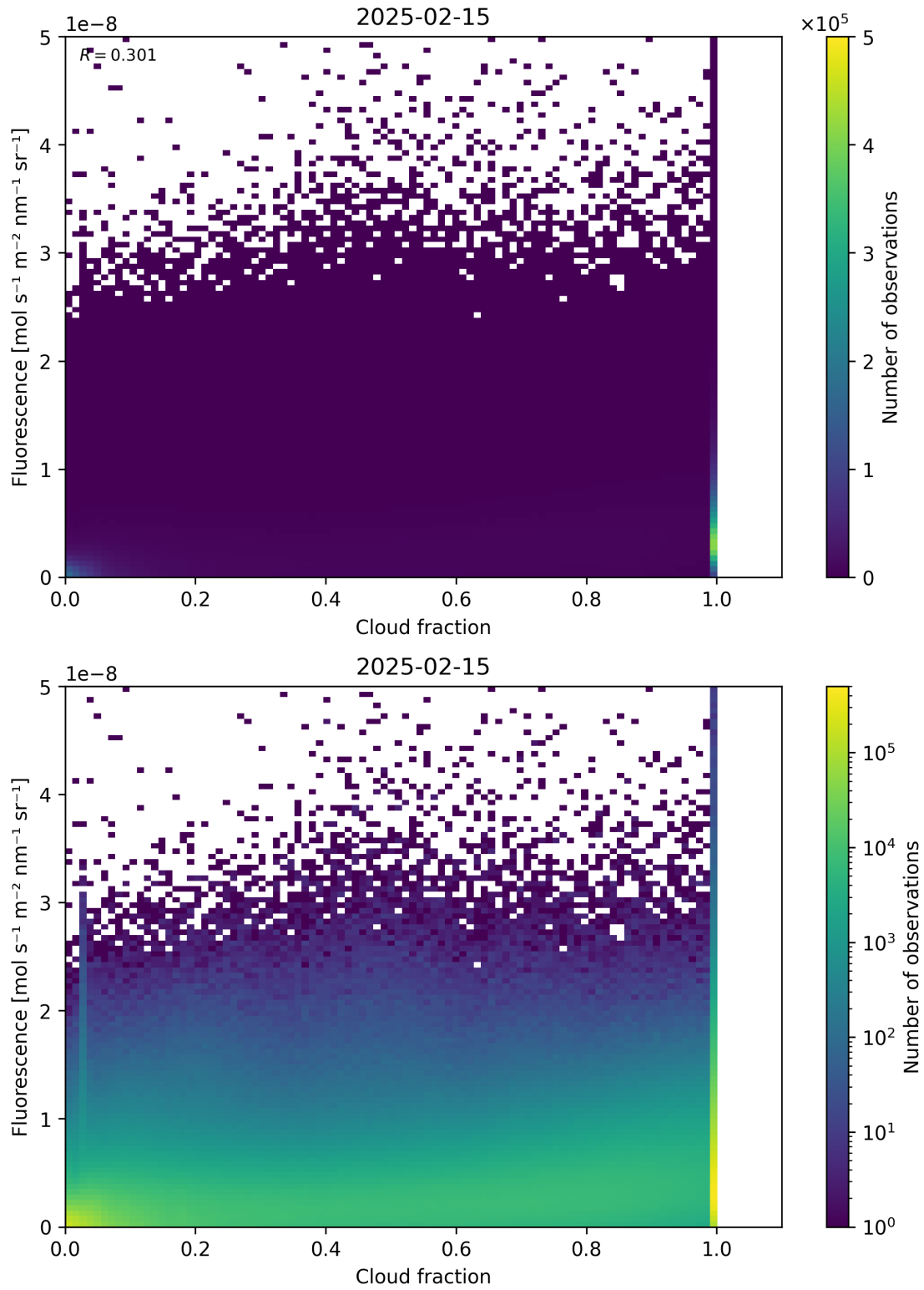
Figure 72: Scatter density plot of “Cloud fraction” against “Fluorescence” for 2025-02-14 to 2025-02-16.
