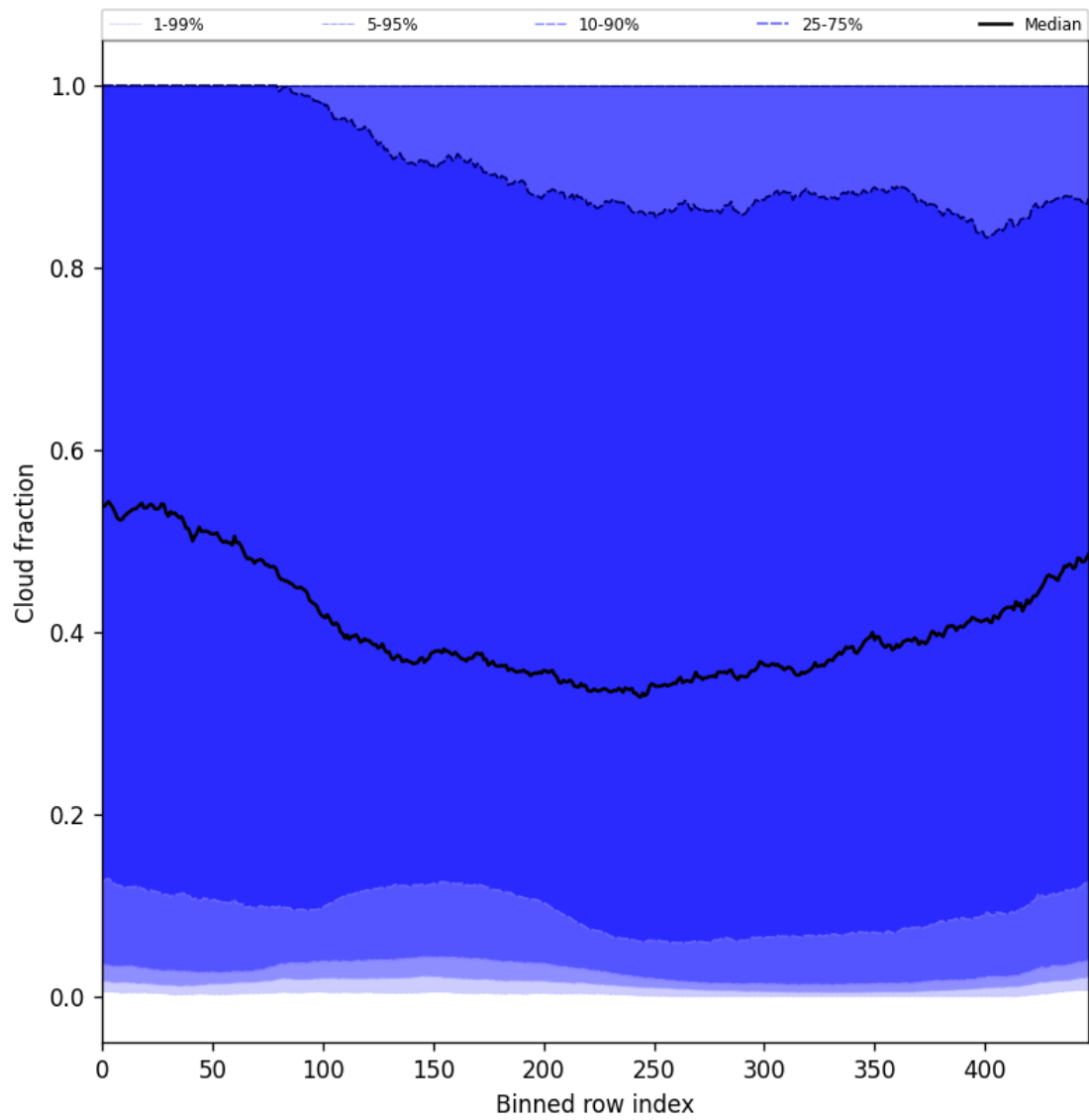
Figure 49: Along track statistics of “Cloud fraction” for 2025-02-14 to 2025-02-16
