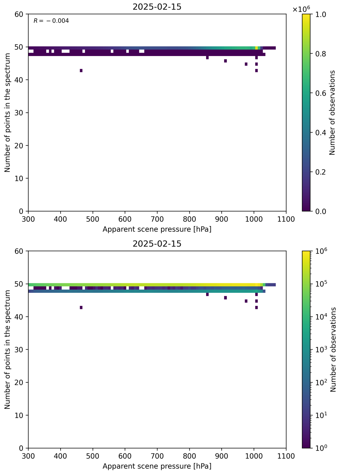
Figure 66: Scatter density plot of “Apparent scene pressure” against “Number of points in the spectrum” for 2025-02-14 to 2025-02-16.
