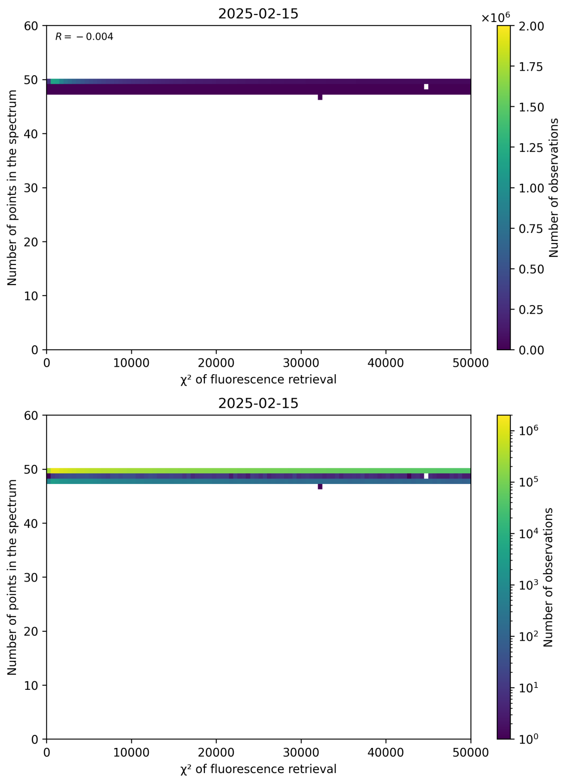
Figure 68: Scatter density plot of “ \chi^2 of fluorescence retrieval” against “Number of points in the spectrum” for 2025-02-14 to 2025-02-16.
