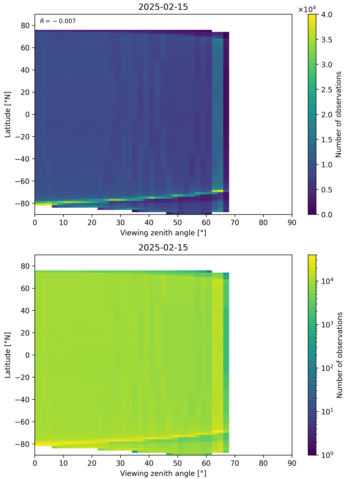
Figure 123: Scatter density plot of “Viewing zenith angle” against “Latitude” for 2025-02-14 to 2025-02-16.
