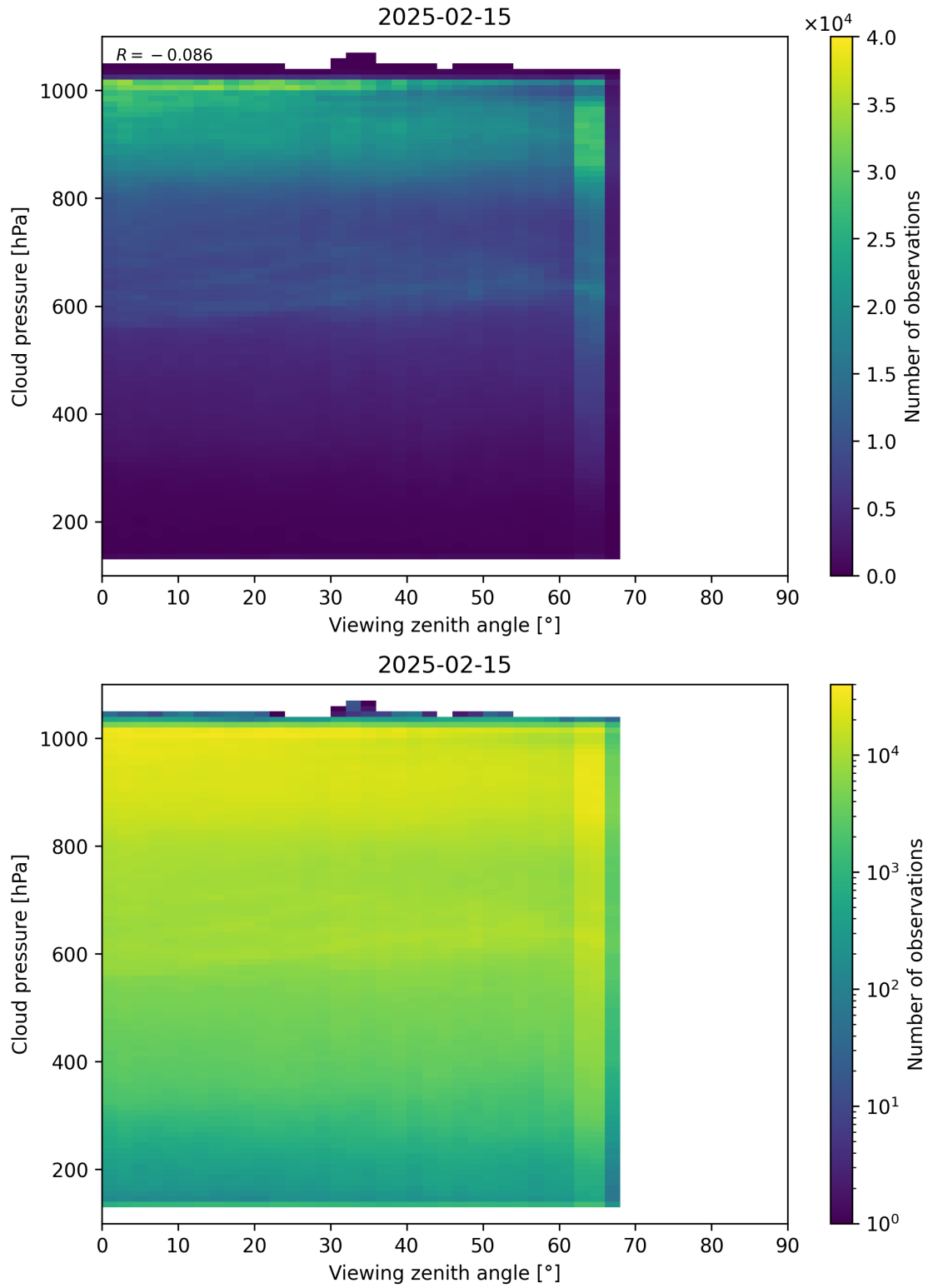
Figure 121: Scatter density plot of “Viewing zenith angle” against “Cloud pressure” for 2025-02-14 to 2025-02-16.
