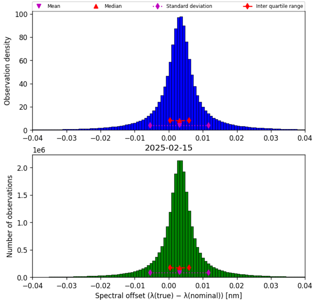
Figure 45: Histogram of “Spectral offset ( \lambda_{\text{true}} - \lambda_{\text{nominal}} )” for 2025-02-14 to 2025-02-16
