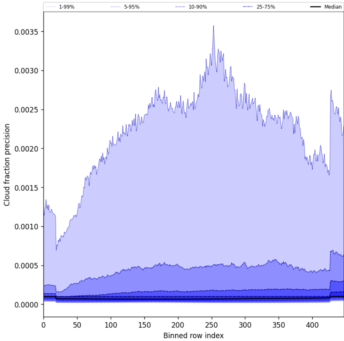
Figure 50: Along track statistics of “Cloud fraction precision” for 2025-02-14 to 2025-02-16
