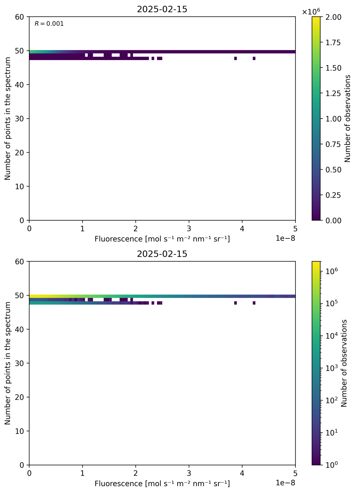
Figure 86: Scatter density plot of “Fluorescence” against “Number of points in the spectrum” for 2025-02-14 to 2025-02-16.
