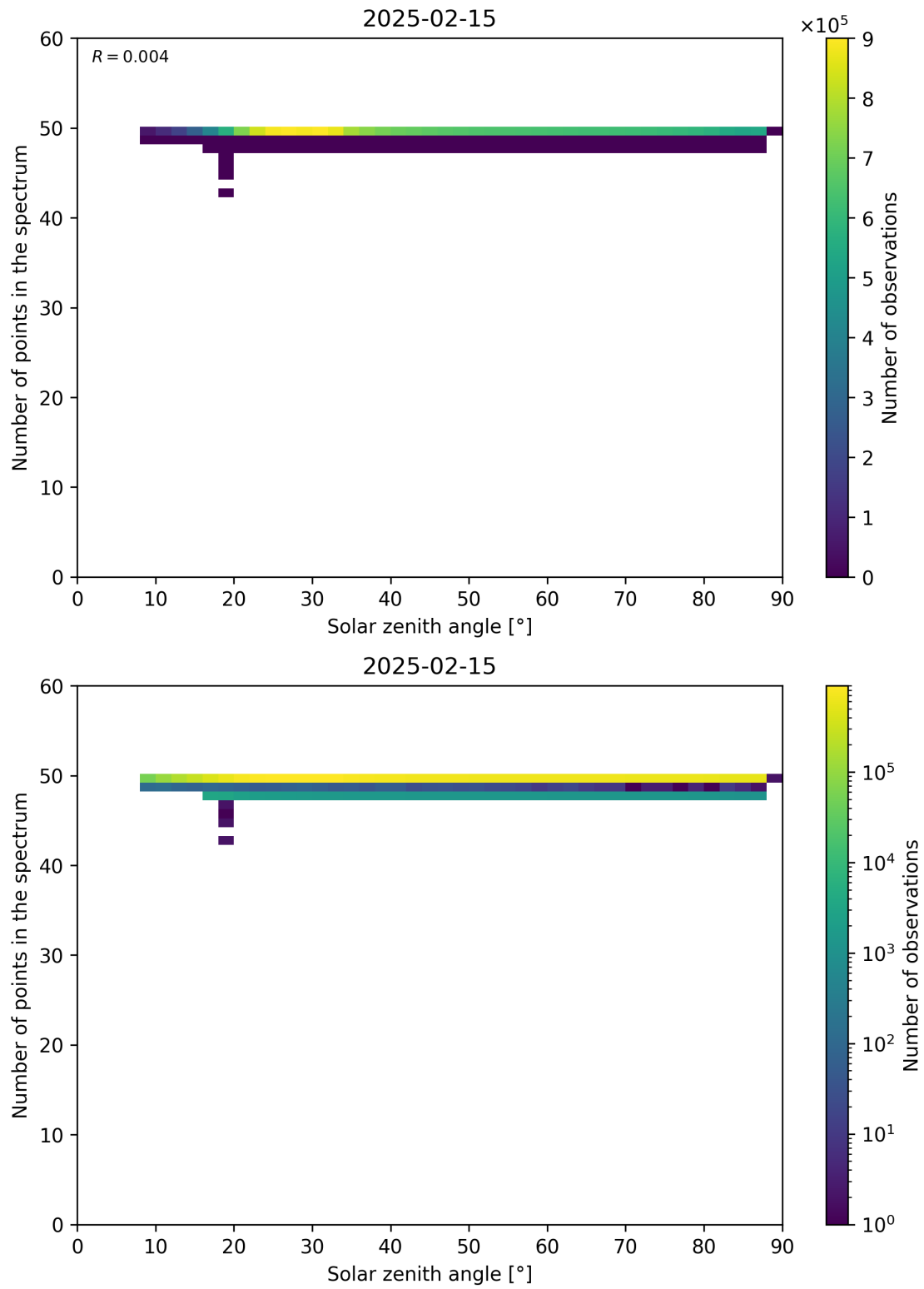
Figure 115: Scatter density plot of “Solar zenith angle” against “Number of points in the spectrum” for 2025-02-14 to 2025-02-16.
