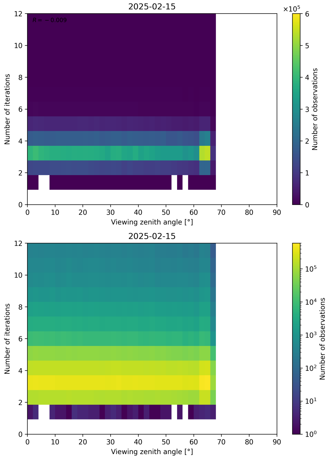
Figure 124: Scatter density plot of “Viewing zenith angle” against “Number of iterations” for 2025-02-14 to 2025-02-16.
