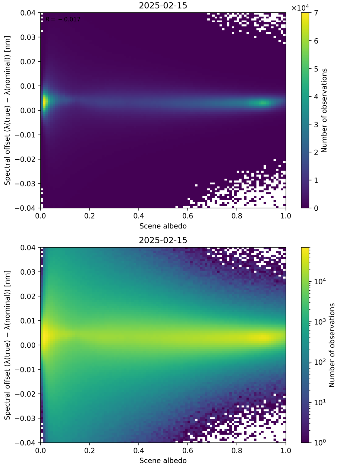
Figure 107: Scatter density plot of “Scene albedo” against “Spectral offset ( \lambda_{\text{true}} - \lambda_{\text{nominal}} )” for 2025-02-14 to 2025-02-16.
