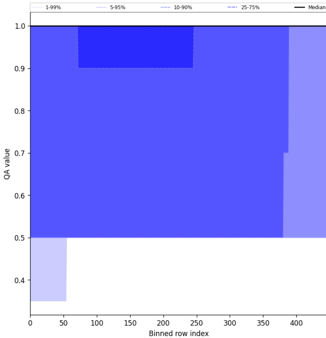
Figure 46: Along track statistics of “QA value” for 2025-02-14 to 2025-02-16
