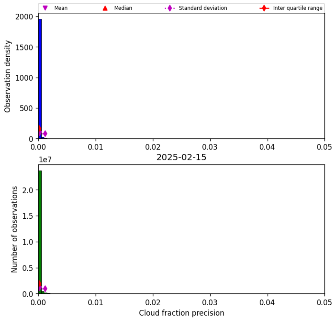
Figure 33: Histogram of “Cloud fraction precision” for 2025-02-14 to 2025-02-16
