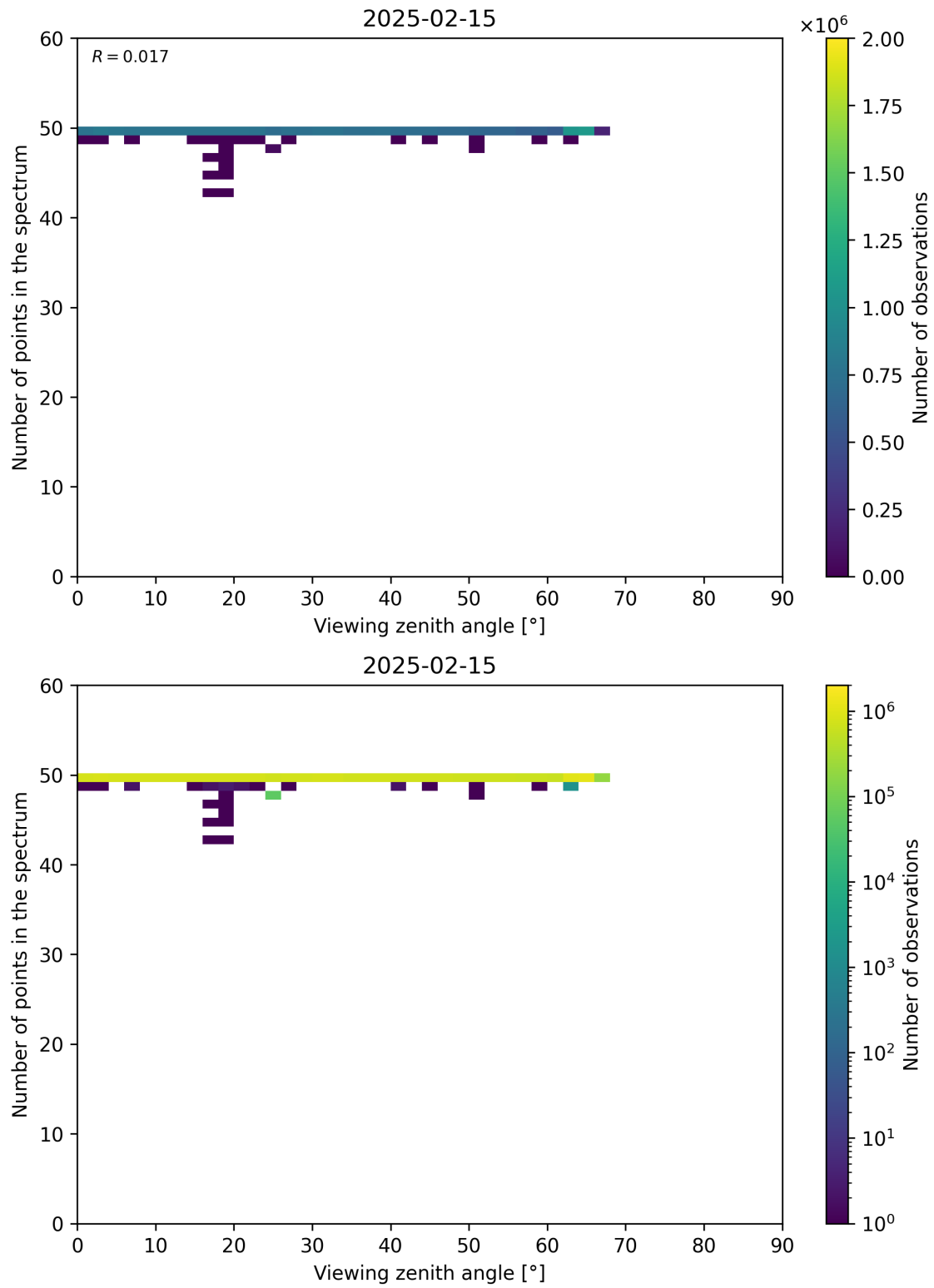
Figure 125: Scatter density plot of “Viewing zenith angle” against “Number of points in the spectrum” for 2025-02-14 to 2025-02-16.
