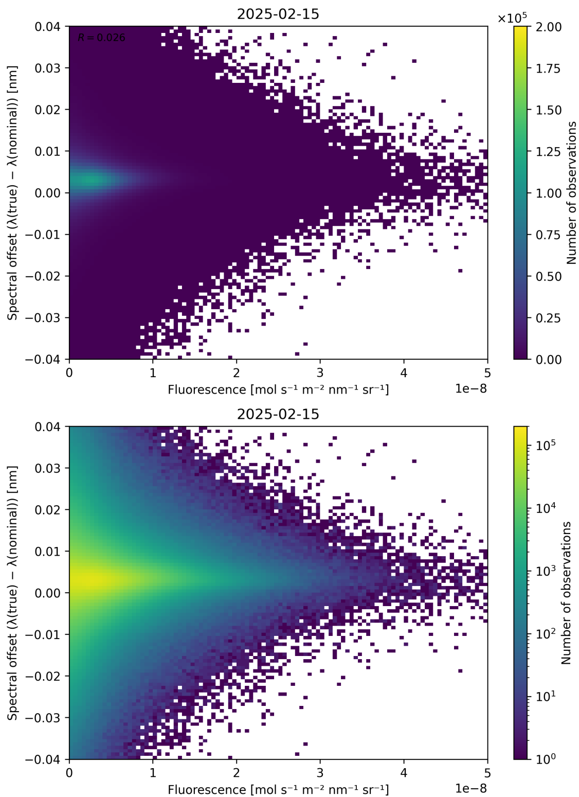
Figure 87: Scatter density plot of “Fluorescence” against “Spectral offset ( \lambda_{\text{true}} - \lambda_{\text{nominal}} )” for 2025-02-14 to 2025-02-16.
