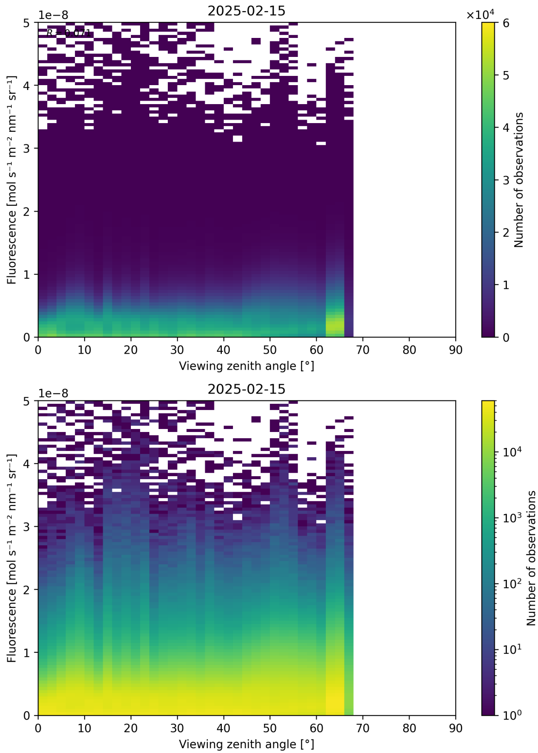
Figure 122: Scatter density plot of “Viewing zenith angle” against “Fluorescence” for 2025-02-14 to 2025-02-16.
