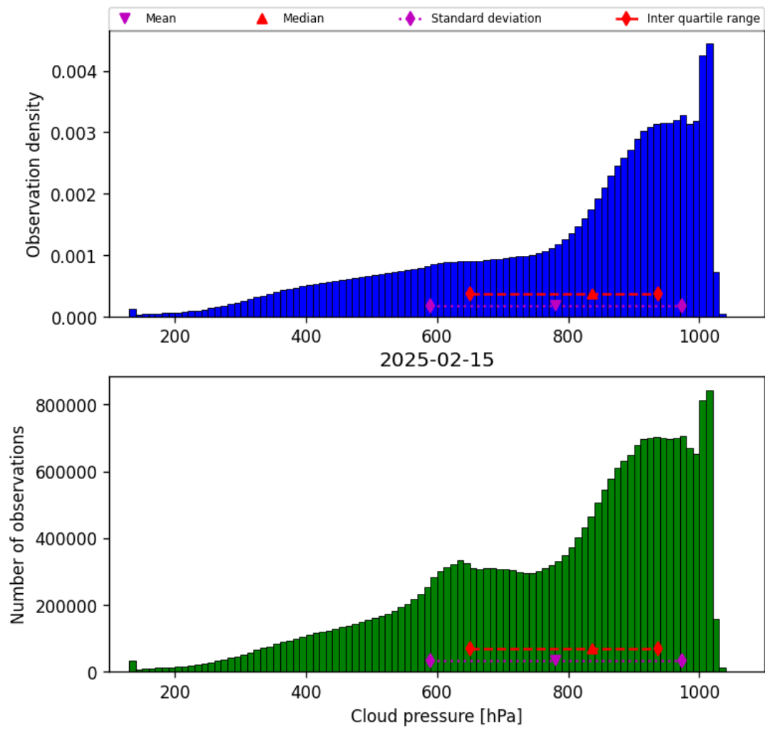
Figure 30: Histogram of “Cloud pressure” for 2025-02-14 to 2025-02-16
