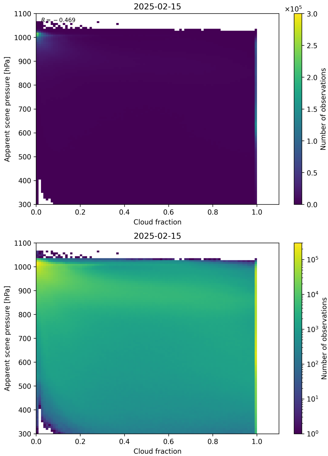
Figure 70: Scatter density plot of “Cloud fraction” against “Apparent scene pressure” for 2025-02-14 to 2025-02-16.
