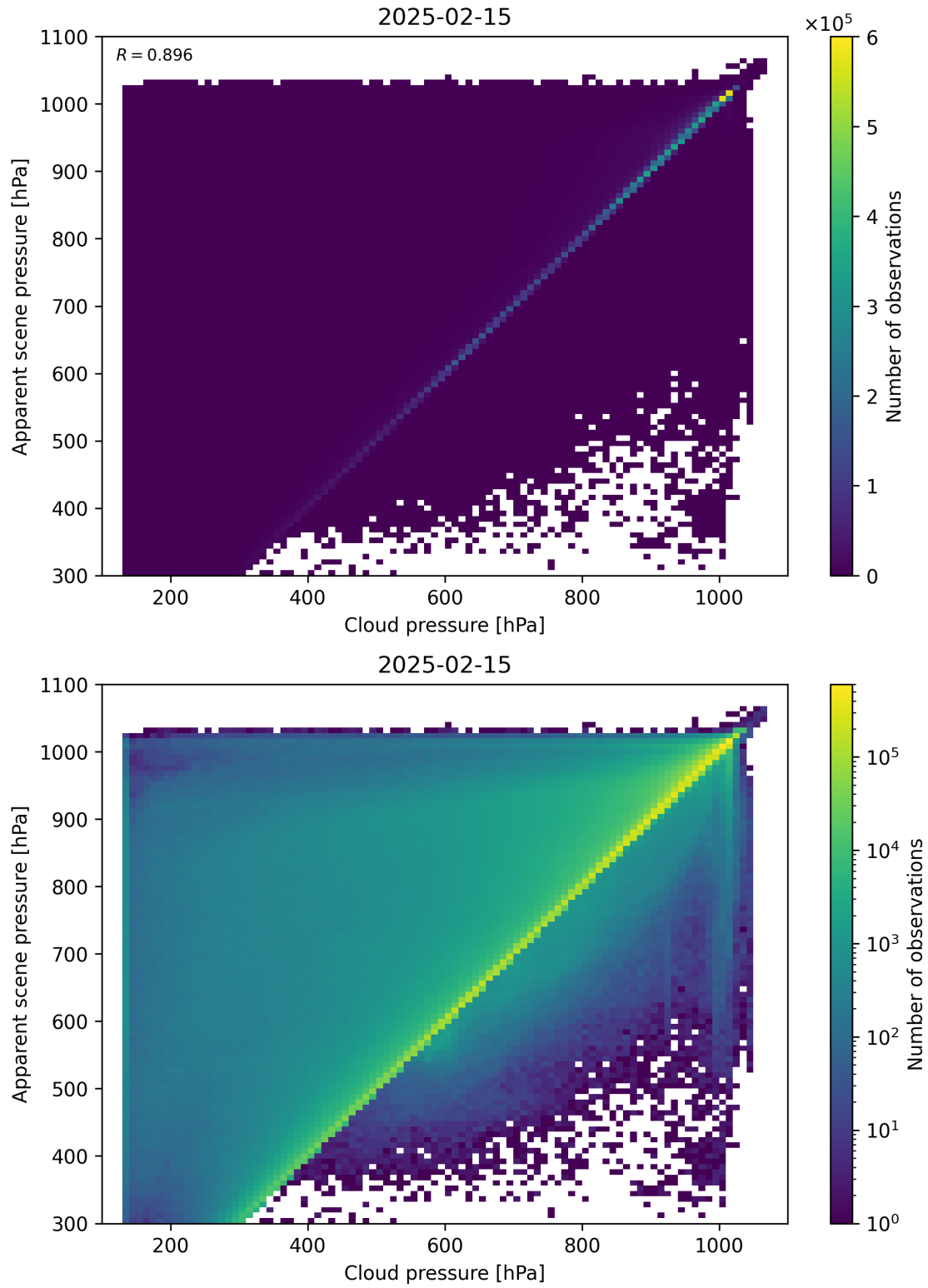
Figure 77: Scatter density plot of “Cloud pressure” against “Apparent scene pressure” for 2025-02-14 to 2025-02-16.
