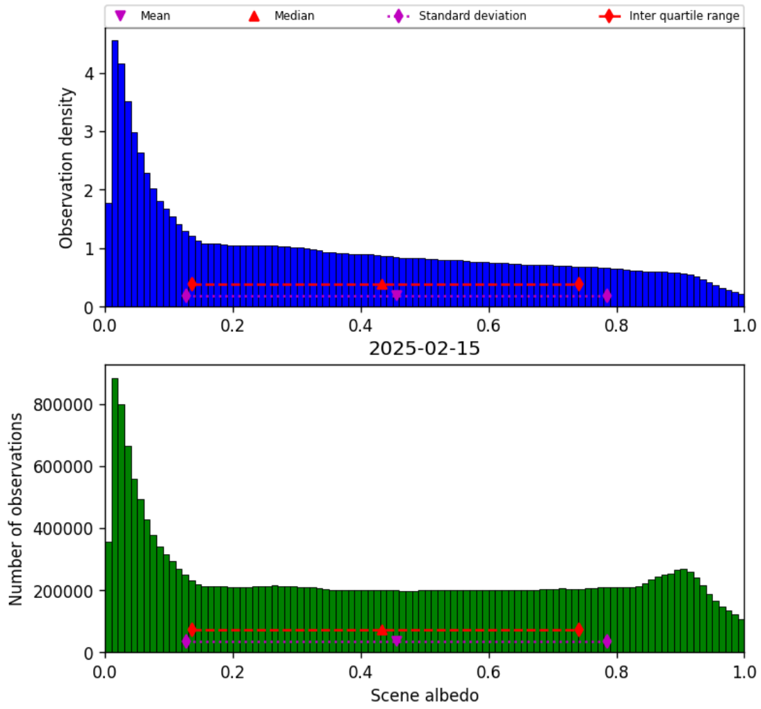
Figure 34: Histogram of “Scene albedo” for 2025-02-14 to 2025-02-16
