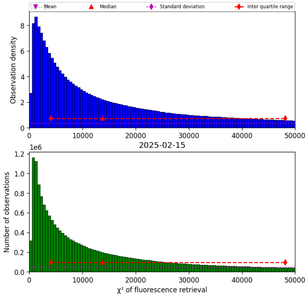
Figure 42: Histogram of “ \chi^2 of fluorescence retrieval” for 2025-02-14 to 2025-02-16
