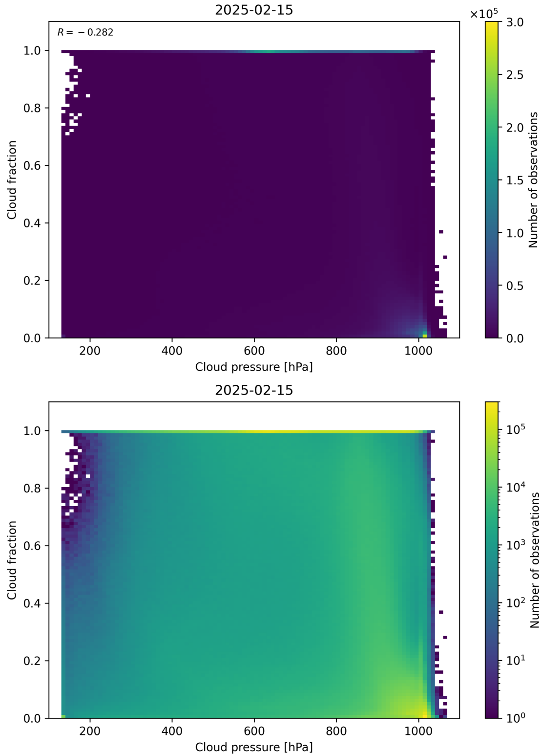
Figure 79: Scatter density plot of “Cloud pressure” against “Cloud fraction” for 2025-02-14 to 2025-02-16.
