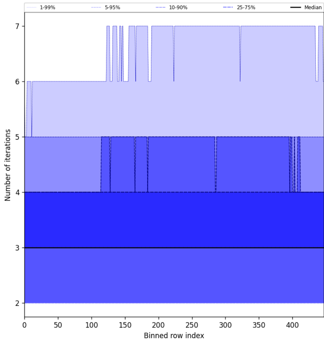
Figure 56: Along track statistics of “Number of iterations” for 2025-02-14 to 2025-02-16
