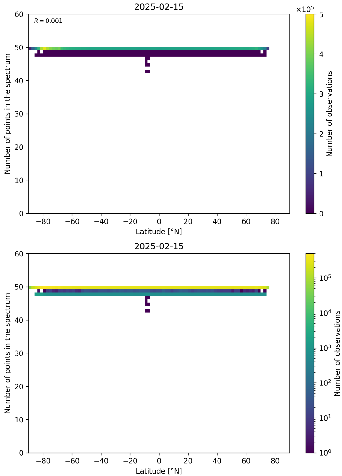
Figure 94: Scatter density plot of “Latitude” against “Number of points in the spectrum” for 2025-02-14 to 2025-02-16.
