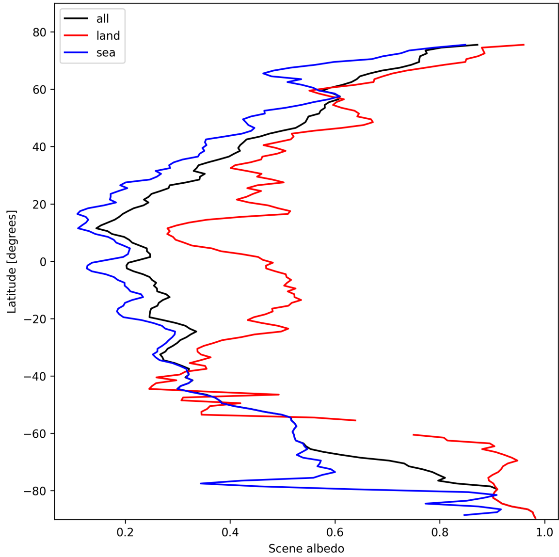
Figure 17: Zonal average of “Scene albedo” for 2025-02-14 to 2025-02-16.
