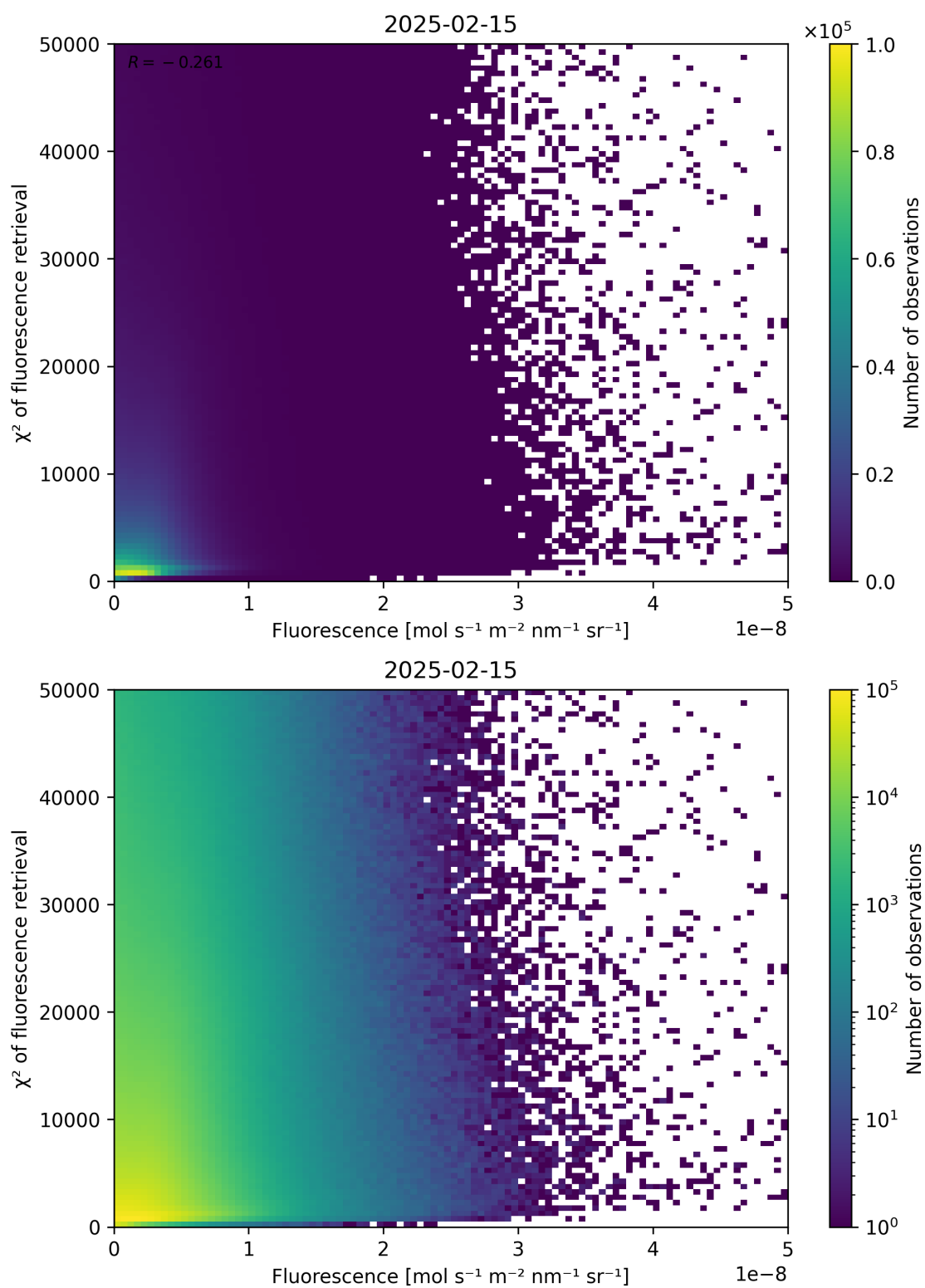
Figure 85: Scatter density plot of “Fluorescence” against “ \chi^2 of fluorescence retrieval” for 2025-02-14 to 2025-02-16.
