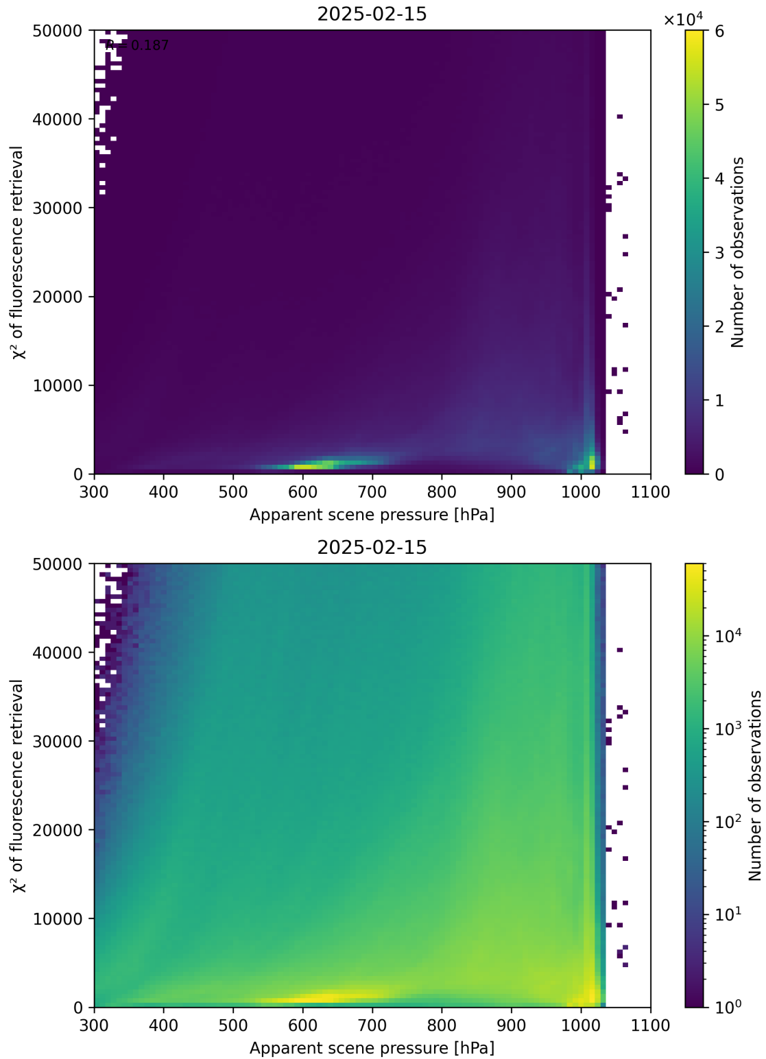
Figure 63: Scatter density plot of “Apparent scene pressure” against “ \chi^2 of fluorescence retrieval” for 2025-02-14 to 2025-02-16.
