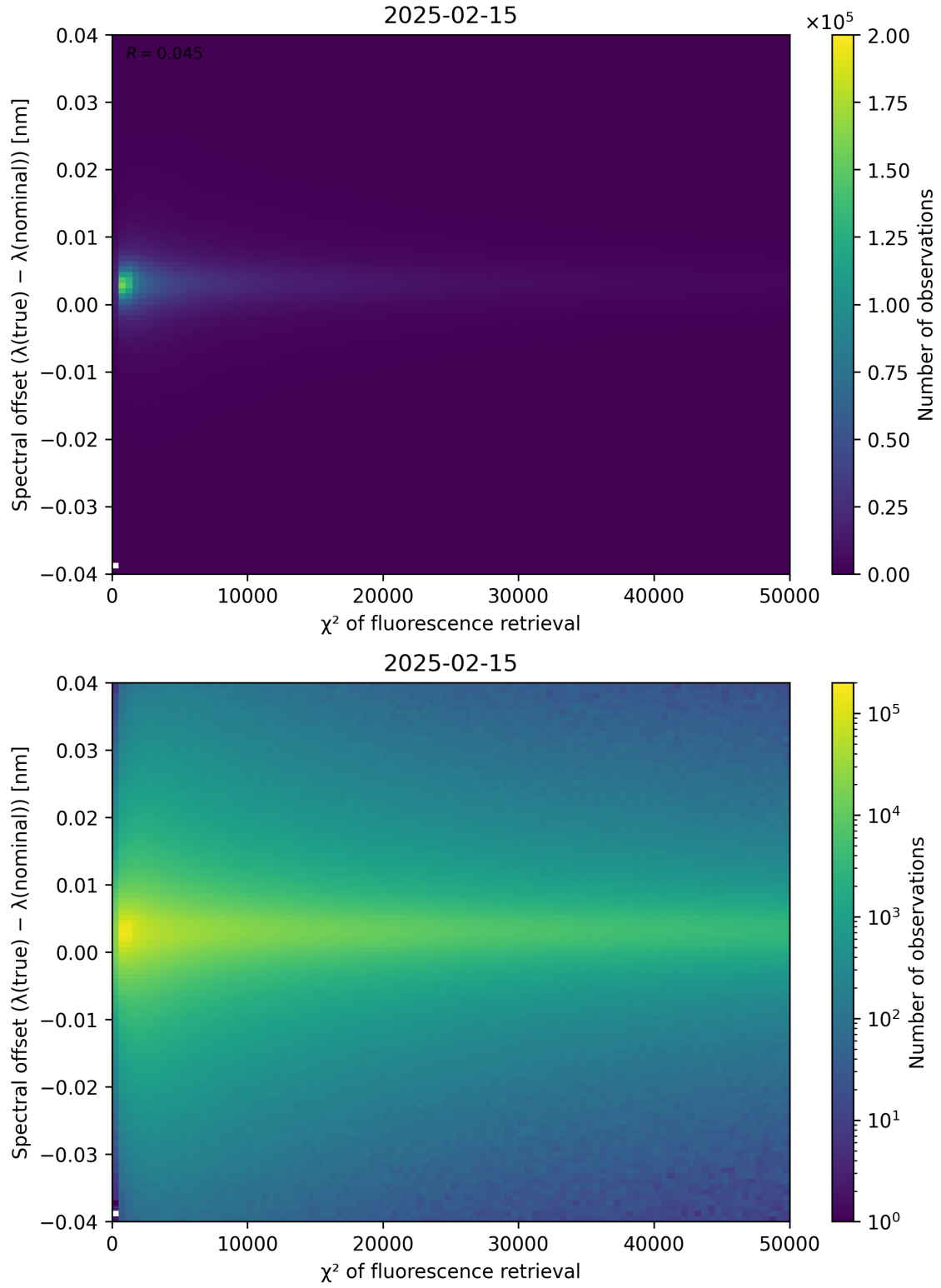
Figure 69: Scatter density plot of “ \chi^2 of fluorescence retrieval” against “Spectral offset ( \lambda_{\text{true}} - \lambda_{\text{nominal}} )” for 2025-02-14 to 2025-02-16.
