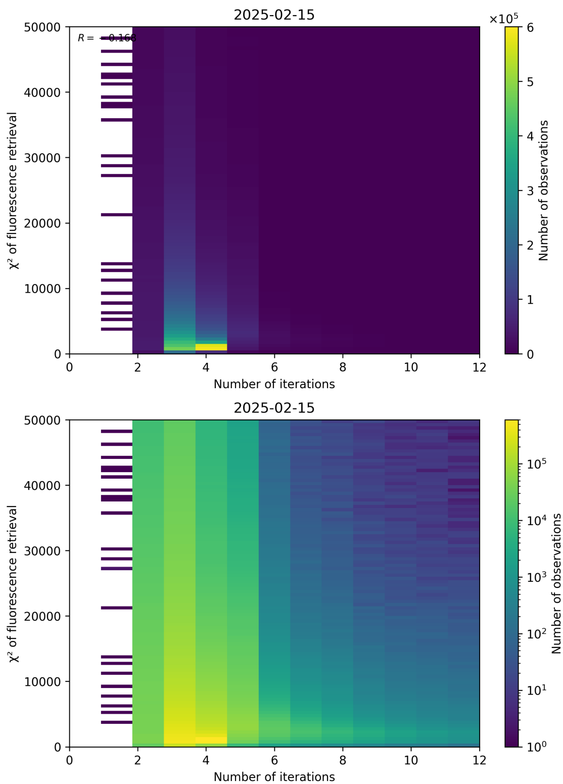
Figure 97: Scatter density plot of “Number of iterations” against “ \chi^2 of fluorescence retrieval” for 2025-02-14 to 2025-02-16.
