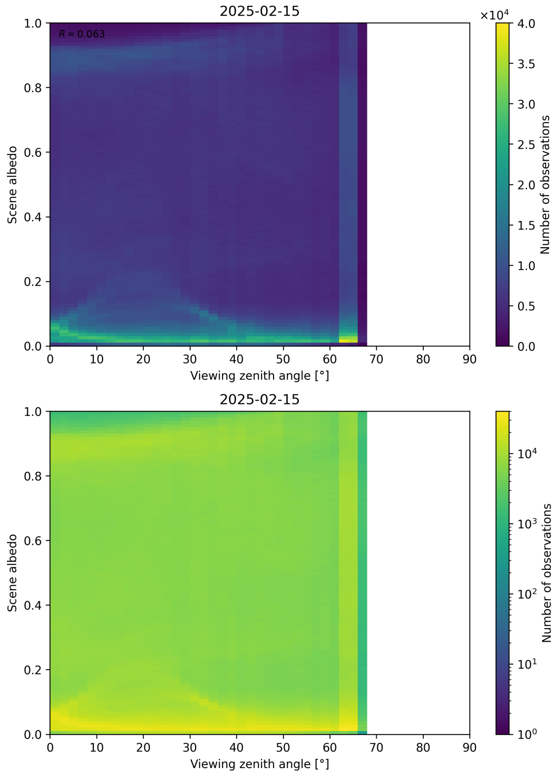
Figure 126: Scatter density plot of “Viewing zenith angle” against “Scene albedo” for 2025-02-14 to 2025-02-16.
