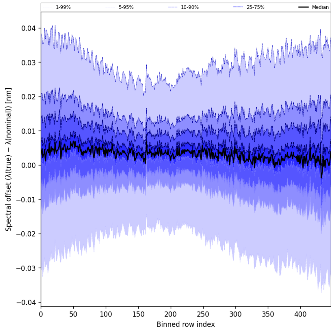
Figure 62: Along track statistics of “Spectral offset ( \lambda_{\text{true}} - \lambda_{\text{nominal}} )” for 2025-02-14 to 2025-02-16
