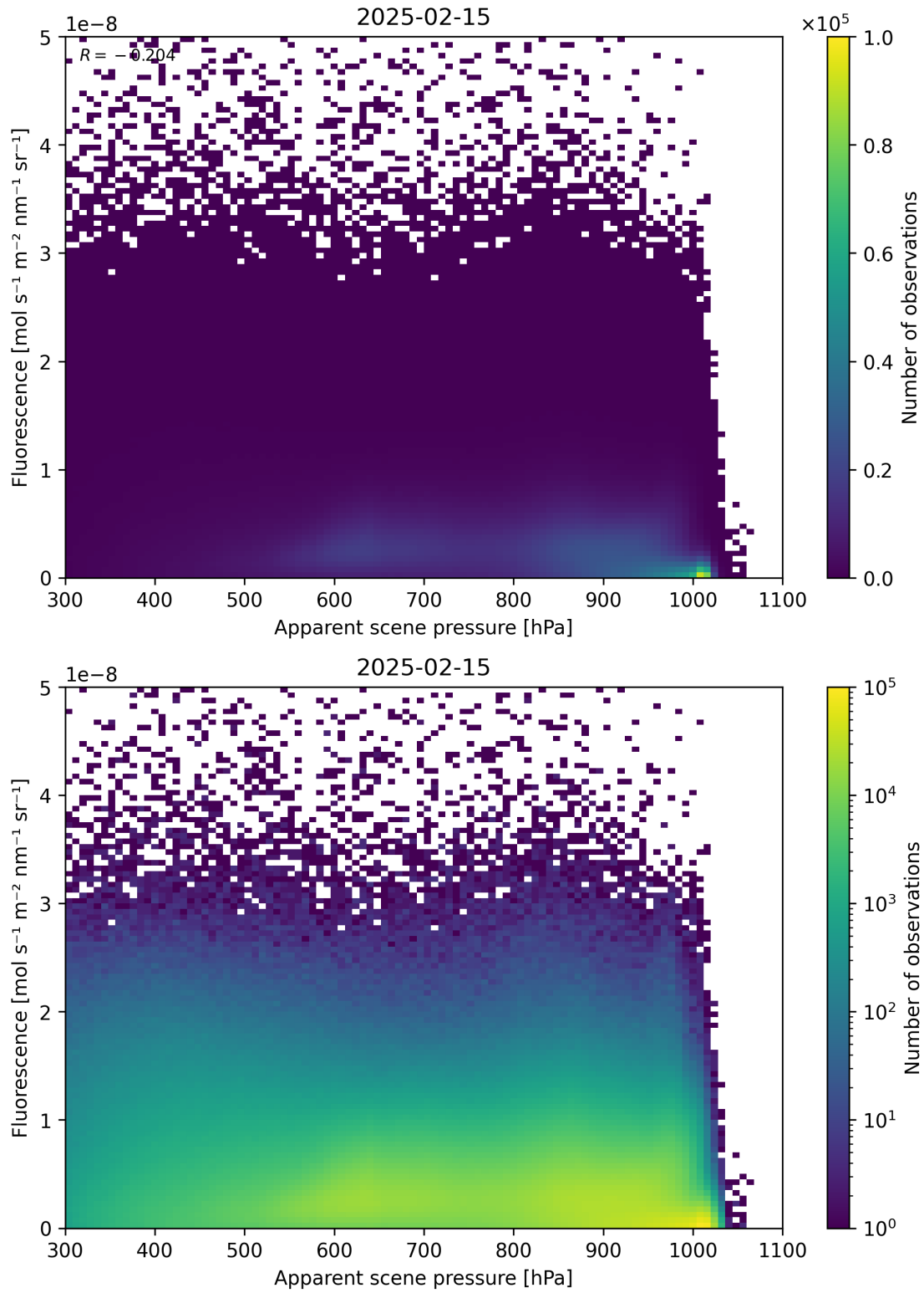
Figure 64: Scatter density plot of “Apparent scene pressure” against “Fluorescence” for 2025-02-14 to 2025-02-16.
