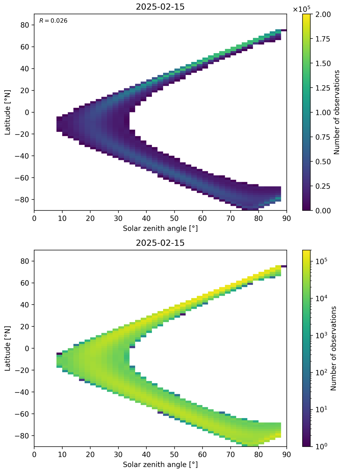
Figure 113: Scatter density plot of “Solar zenith angle” against “Latitude” for 2025-02-14 to 2025-02-16.
