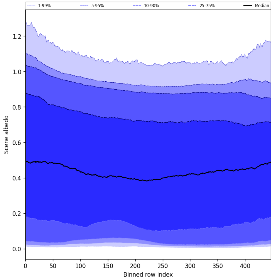
Figure 51: Along track statistics of “Scene albedo” for 2025-02-14 to 2025-02-16
