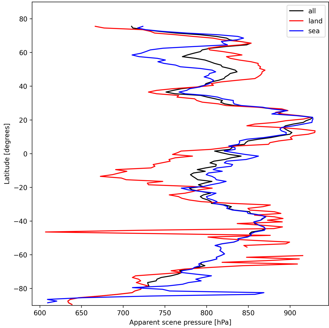
Figure 19: Zonal average of “Apparent scene pressure” for 2025-02-14 to 2025-02-16.
