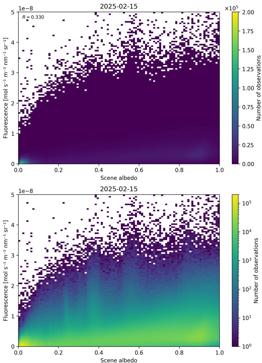
Figure 104: Scatter density plot of “Scene albedo” against “Fluorescence” for 2025-02-14 to 2025-02-16.
