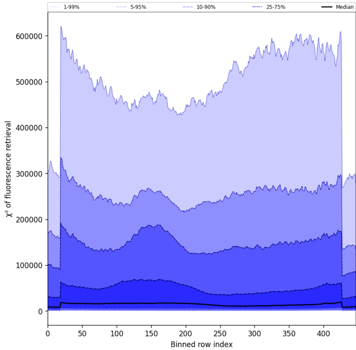
Figure 59: Along track statistics of “ \chi^2 of fluorescence retrieval” for 2025-02-14 to 2025-02-16
