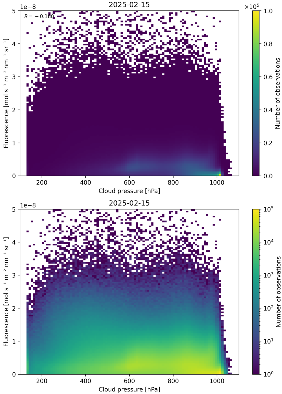
Figure 80: Scatter density plot of “Cloud pressure” against “Fluorescence” for 2025-02-14 to 2025-02-16.
