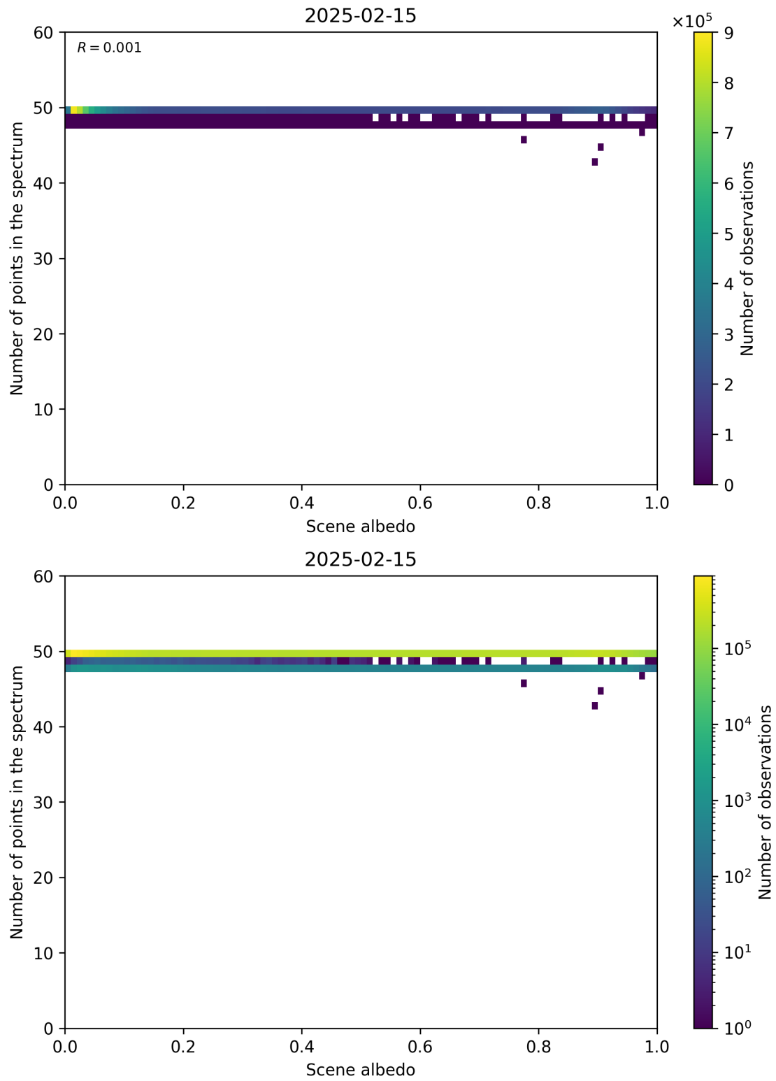
Figure 106: Scatter density plot of “Scene albedo” against “Number of points in the spectrum” for 2025-02-14 to 2025-02-16.
