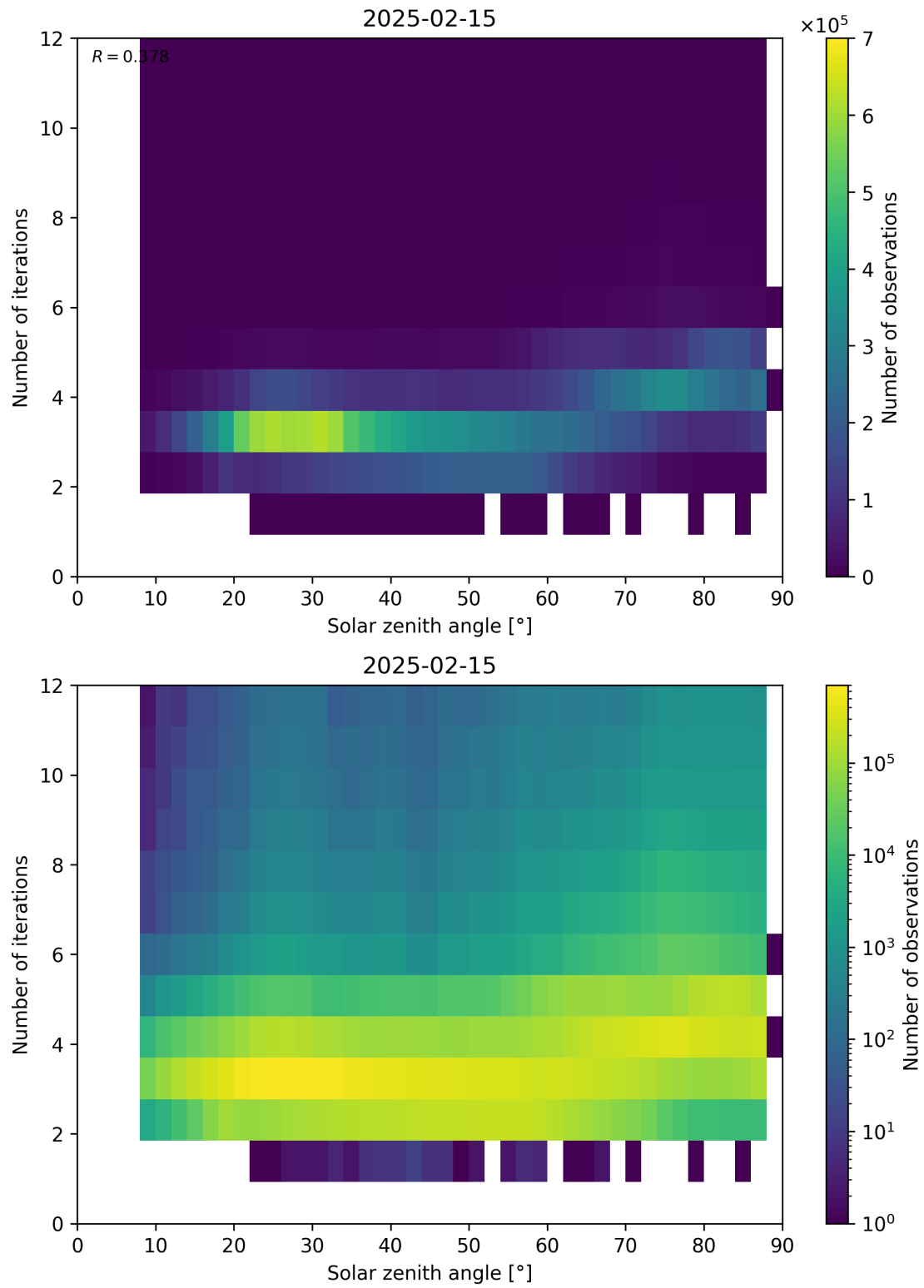
Figure 114: Scatter density plot of “Solar zenith angle” against “Number of iterations” for 2025-02-14 to 2025-02-16.
