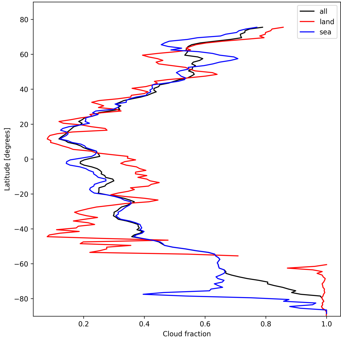
Figure 15: Zonal average of “Cloud fraction” for 2025-02-14 to 2025-02-16.
