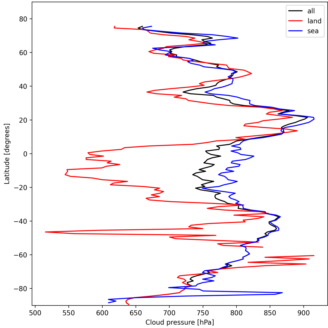
Figure 13: Zonal average of “Cloud pressure” for 2025-02-14 to 2025-02-16.
