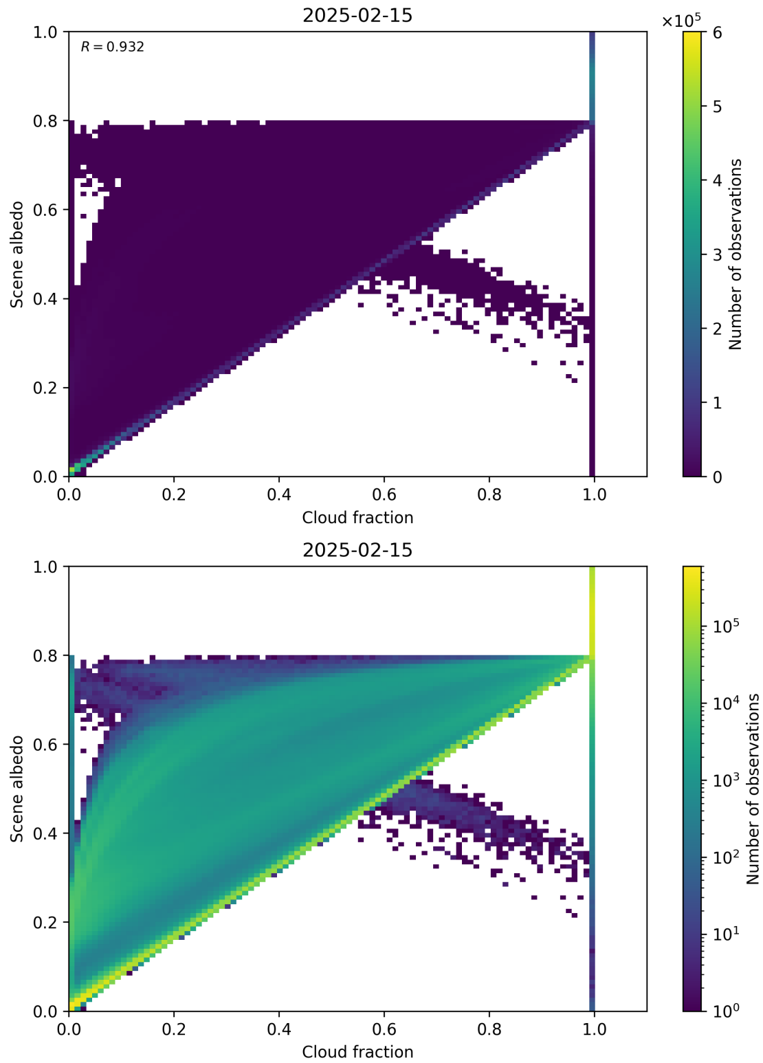
Figure 75: Scatter density plot of “Cloud fraction” against “Scene albedo” for 2025-02-14 to 2025-02-16.
