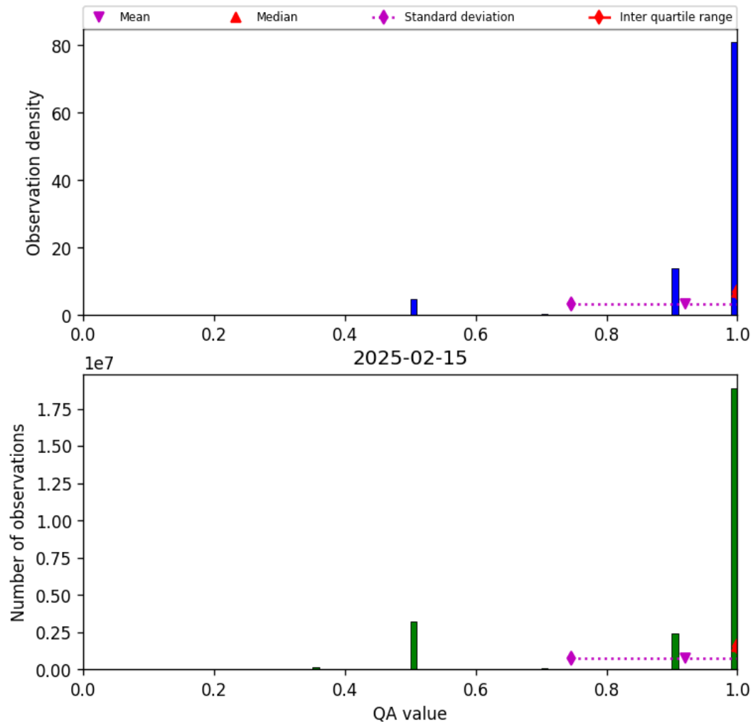
Figure 29: Histogram of “QA value” for 2025-02-14 to 2025-02-16
