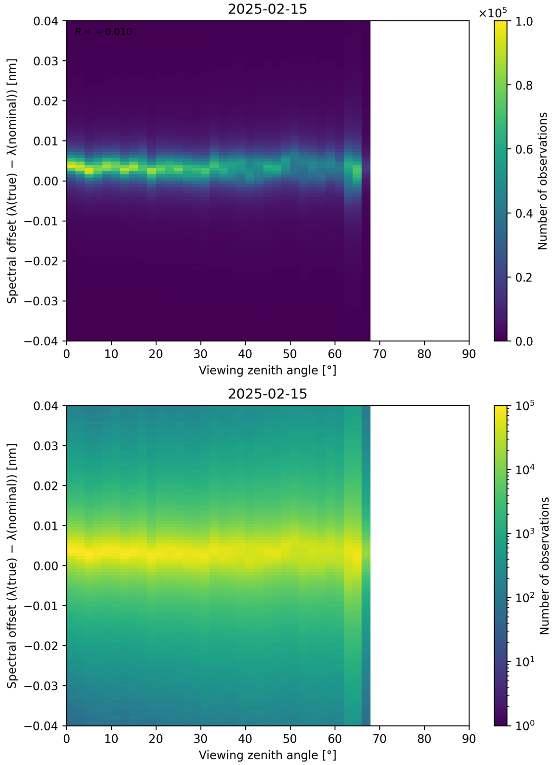
Figure 128: Scatter density plot of “Viewing zenith angle” against “Spectral offset ( \lambda_{\text{true}} - \lambda_{\text{nominal}} )” for 2025-02-14 to 2025-02-16.
