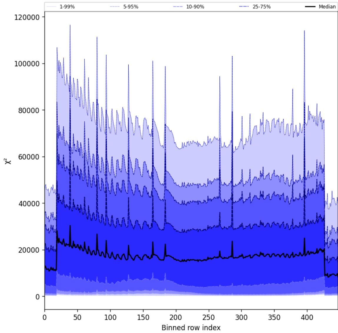
Figure 55: Along track statistics of “ \chi^2 ” for 2025-02-14 to 2025-02-16
