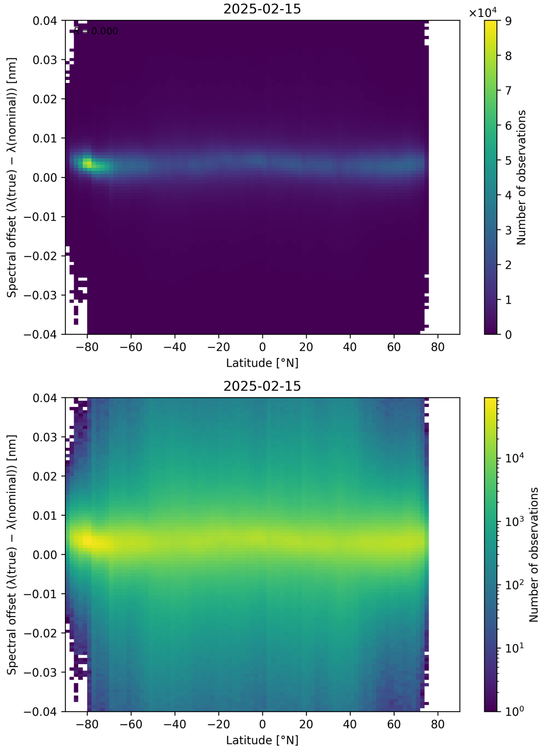
Figure 96: Scatter density plot of “Latitude” against “Spectral offset ( \lambda_{\text{true}} - \lambda_{\text{nominal}} )” for 2025-02-14 to 2025-02-16.
