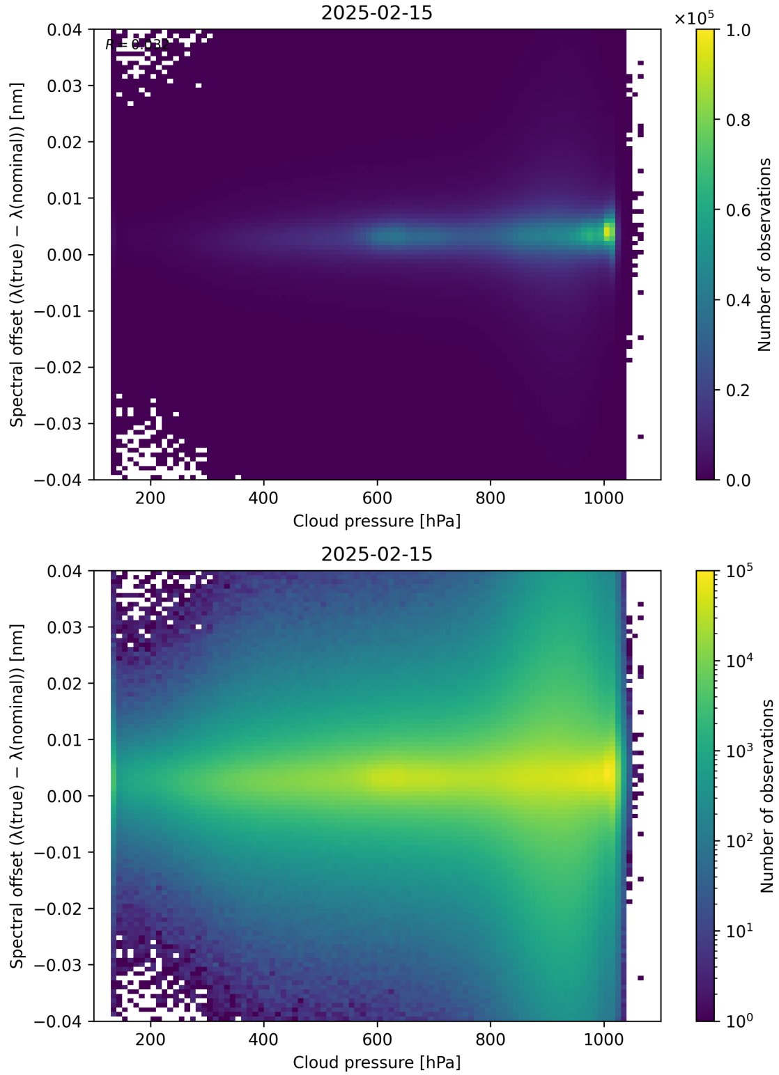
Figure 84: Scatter density plot of “Cloud pressure” against “Spectral offset ( \lambda_{\text{true}} - \lambda_{\text{nominal}} )” for 2025-02-14 to 2025-02-16.
