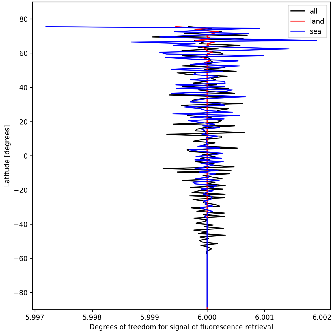
Figure 26: Zonal average of “Degrees of freedom for signal of fluorescence retrieval” for 2025-02-14 to 2025-02-16.
