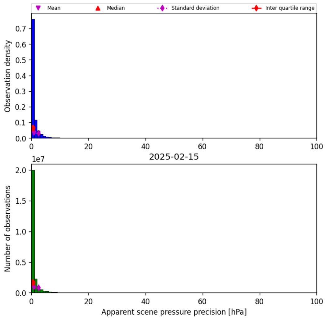
Figure 37: Histogram of “Apparent scene pressure precision” for 2025-02-14 to 2025-02-16
