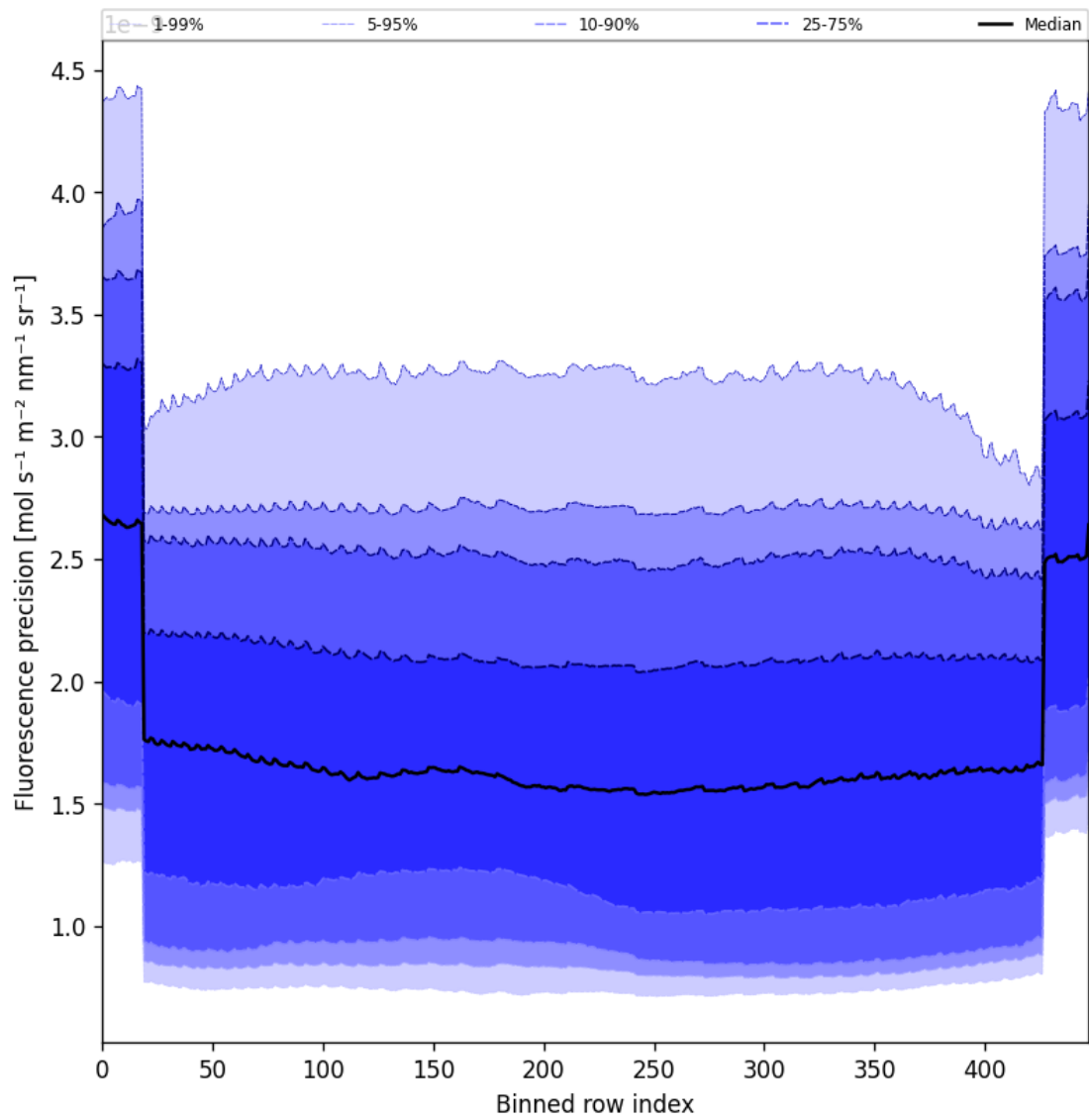
Figure 58: Along track statistics of “Fluorescence precision” for 2025-02-14 to 2025-02-16
