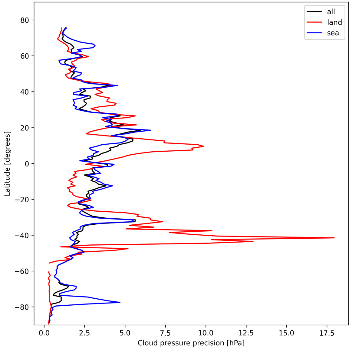
Figure 14: Zonal average of “Cloud pressure precision” for 2025-02-14 to 2025-02-16.
