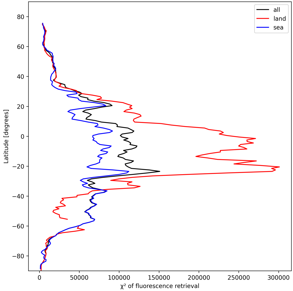
Figure 25: Zonal average of “ \chi^2 of fluorescence retrieval” for 2025-02-14 to 2025-02-16.
