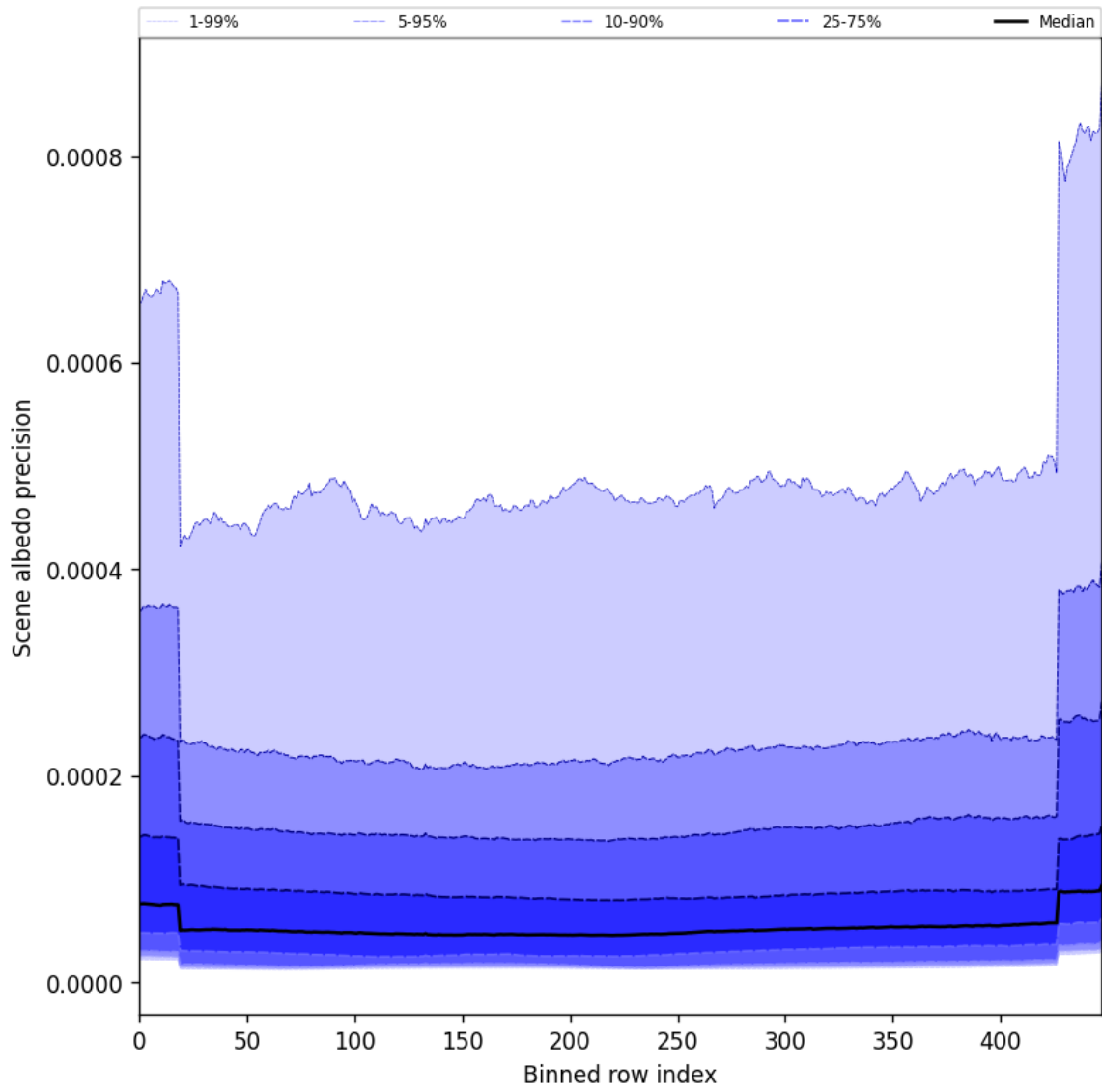
Figure 52: Along track statistics of “Scene albedo precision” for 2025-02-14 to 2025-02-16
