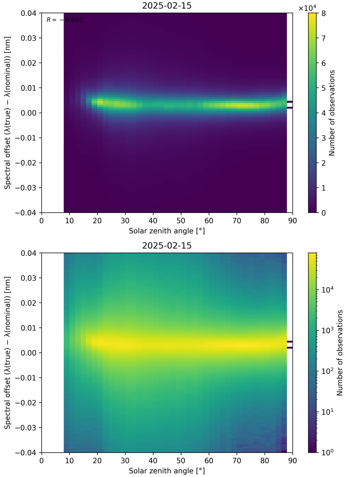
Figure 117: Scatter density plot of “Solar zenith angle” against “Spectral offset ( \lambda_{\text{true}} - \lambda_{\text{nominal}} )” for 2025-02-14 to 2025-02-16.
