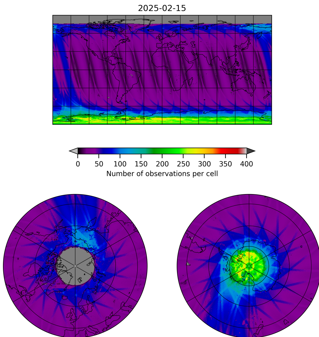
Figure 11: Map of the number of observations for 2025-02-14 to 2025-02-16
