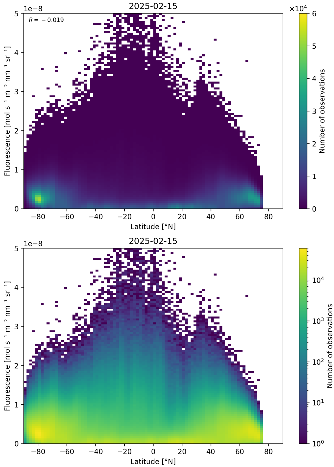
Figure 92: Scatter density plot of “Latitude” against “Fluorescence” for 2025-02-14 to 2025-02-16.
