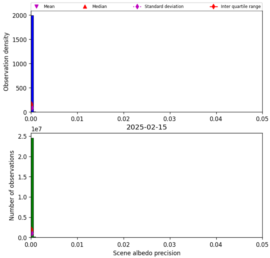
Figure 35: Histogram of “Scene albedo precision” for 2025-02-14 to 2025-02-16
