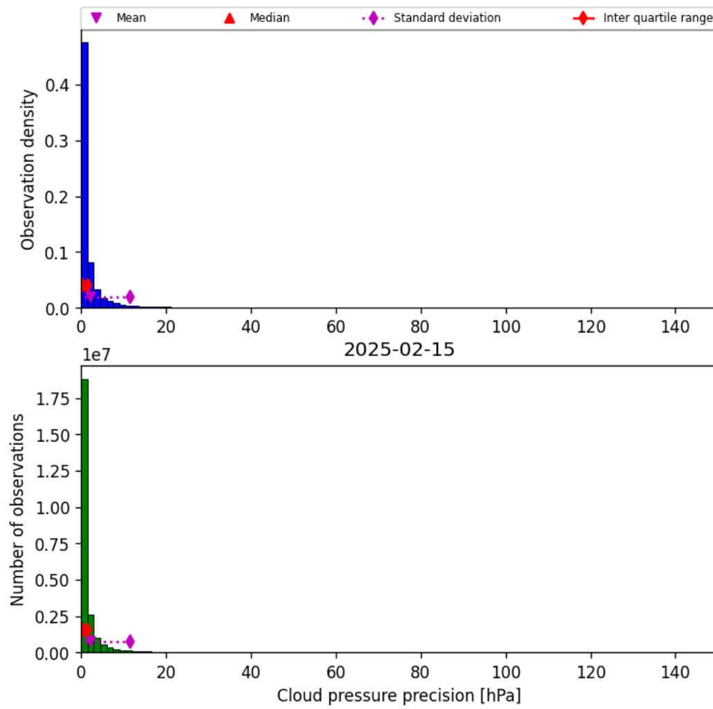
Figure 31: Histogram of “Cloud pressure precision” for 2025-02-14 to 2025-02-16
