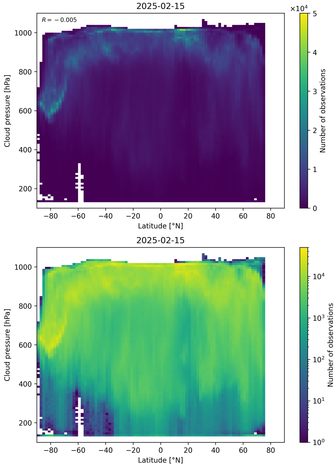
Figure 91: Scatter density plot of “Latitude” against “Cloud pressure” for 2025-02-14 to 2025-02-16.
