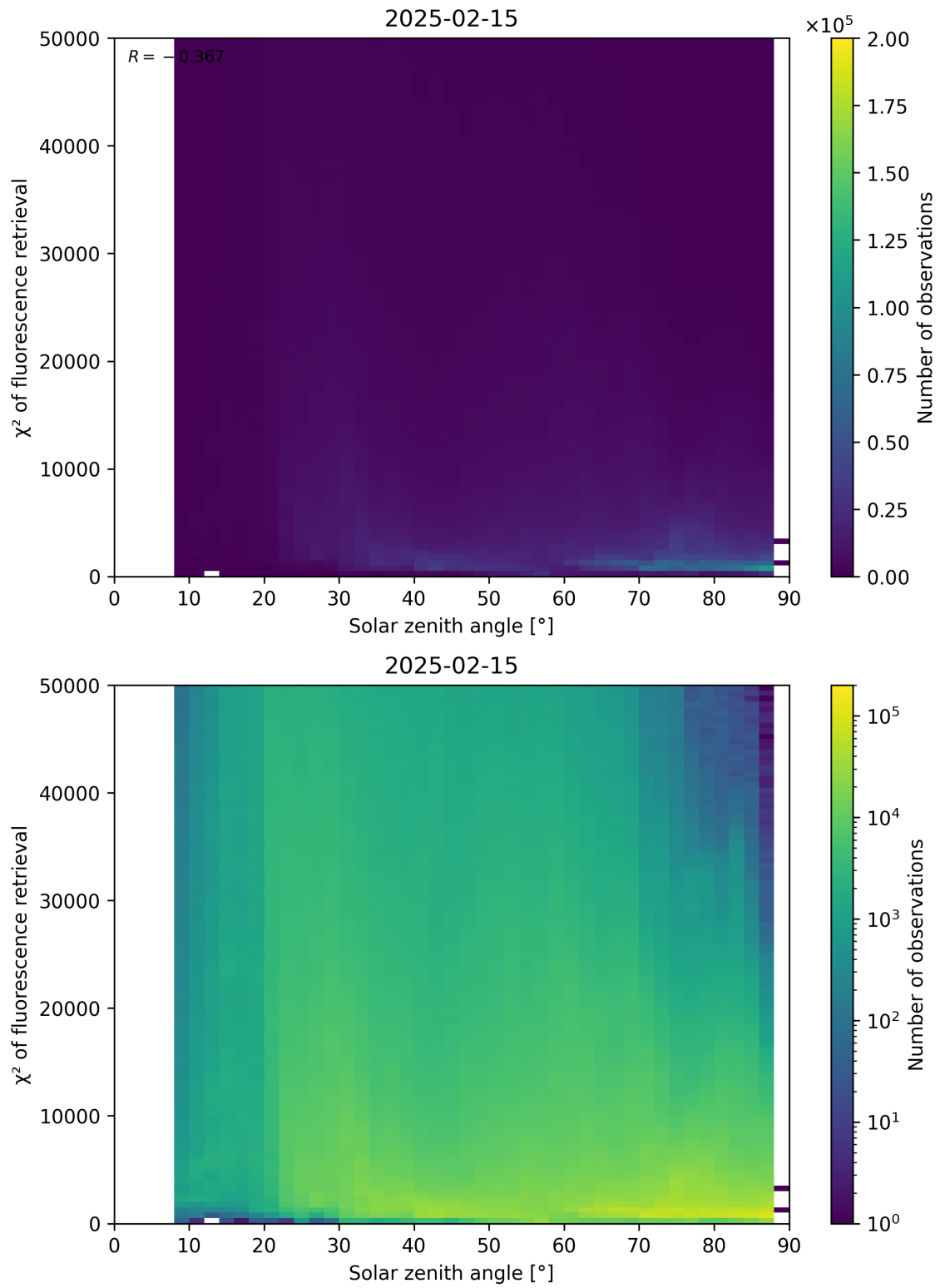
Figure 109: Scatter density plot of “Solar zenith angle” against “ \chi^2 of fluorescence retrieval” for 2025-02-14 to 2025-02-16.
