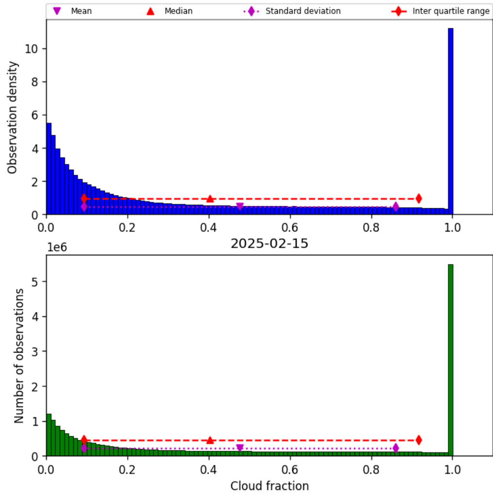
Figure 32: Histogram of “Cloud fraction” for 2025-02-14 to 2025-02-16
