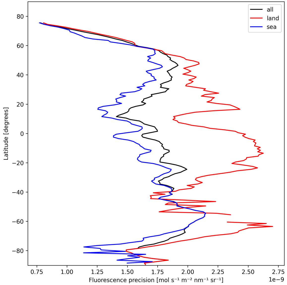
Figure 24: Zonal average of “Fluorescence precision” for 2025-02-14 to 2025-02-16.
