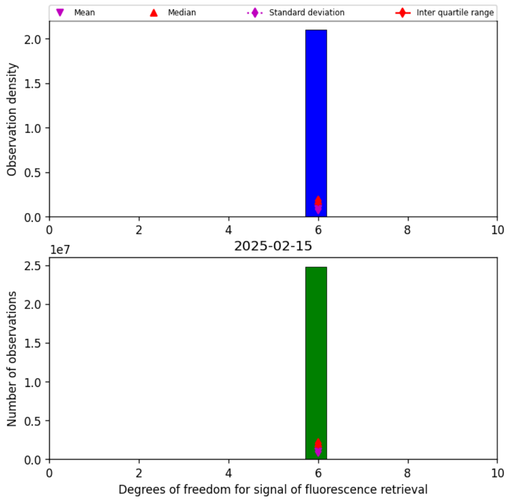
Figure 43: Histogram of “Degrees of freedom for signal of fluorescence retrieval” for 2025-02-14 to 2025-02-16
