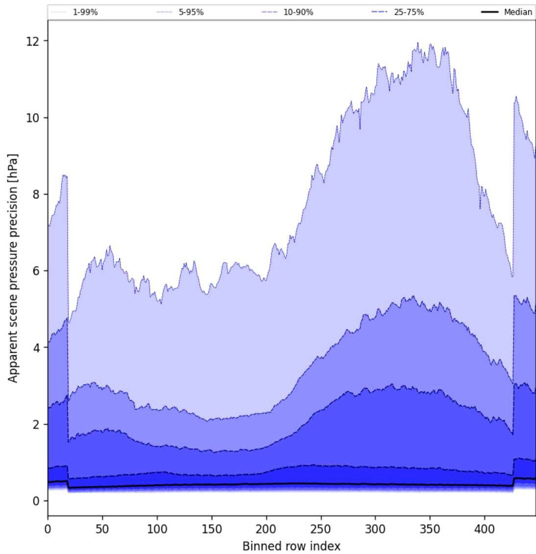
Figure 54: Along track statistics of “Apparent scene pressure precision” for 2025-02-14 to 2025-02-16
