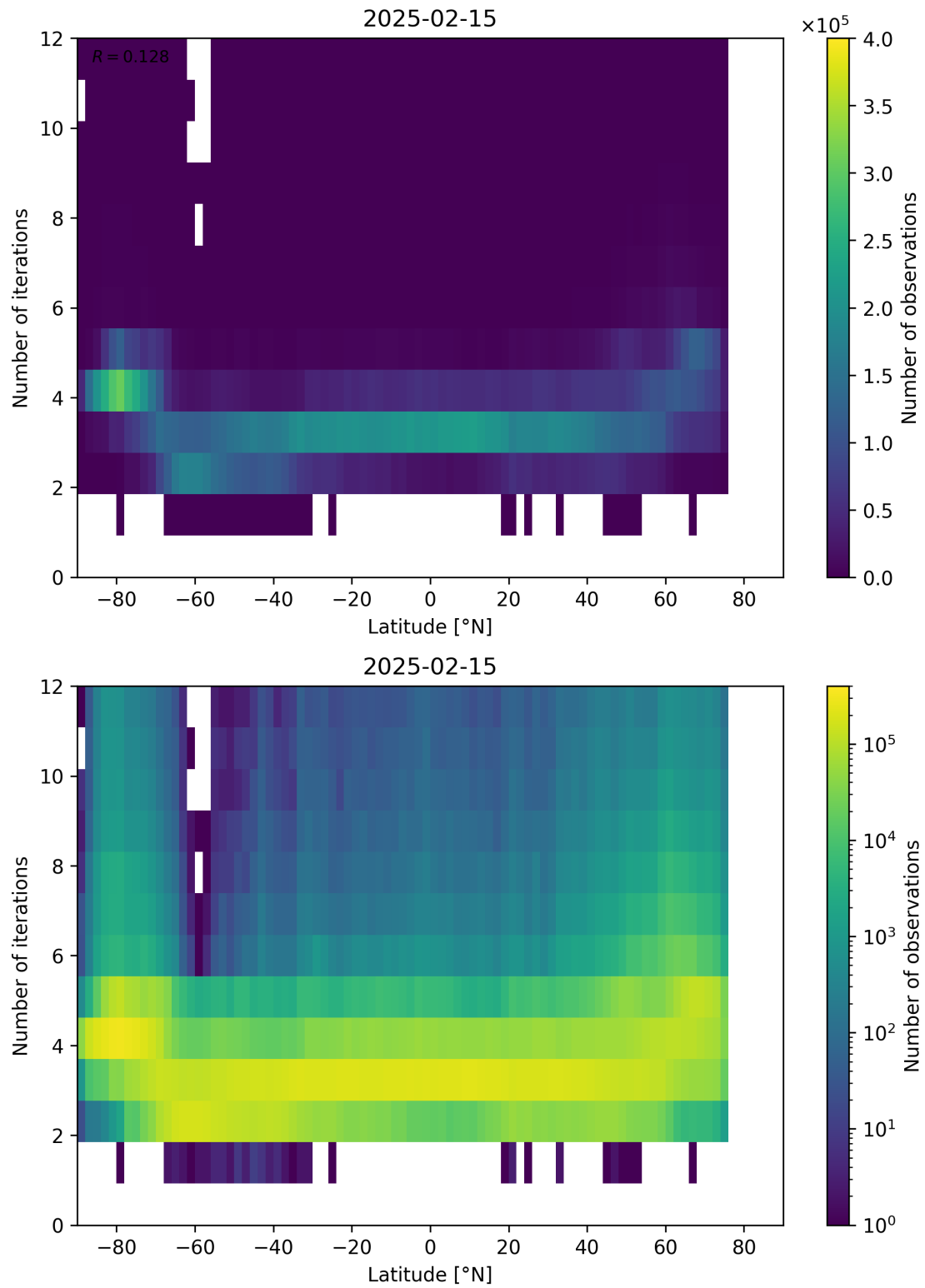
Figure 93: Scatter density plot of “Latitude” against “Number of iterations” for 2025-02-14 to 2025-02-16.
