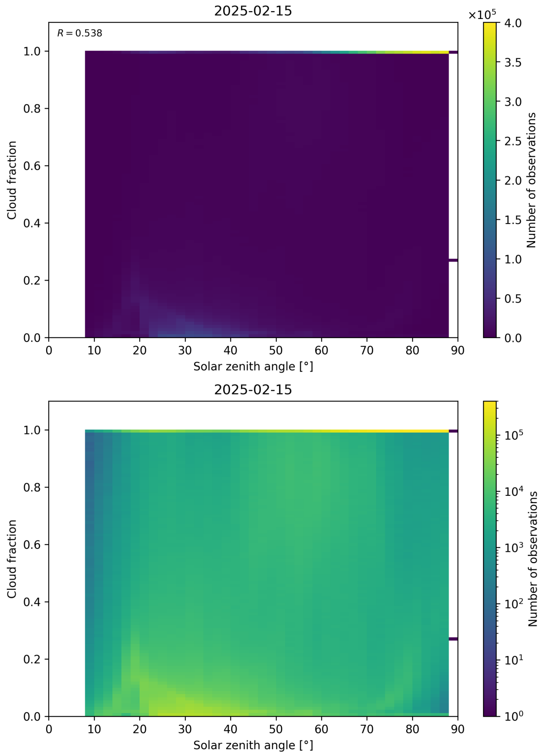
Figure 110: Scatter density plot of “Solar zenith angle” against “Cloud fraction” for 2025-02-14 to 2025-02-16.
