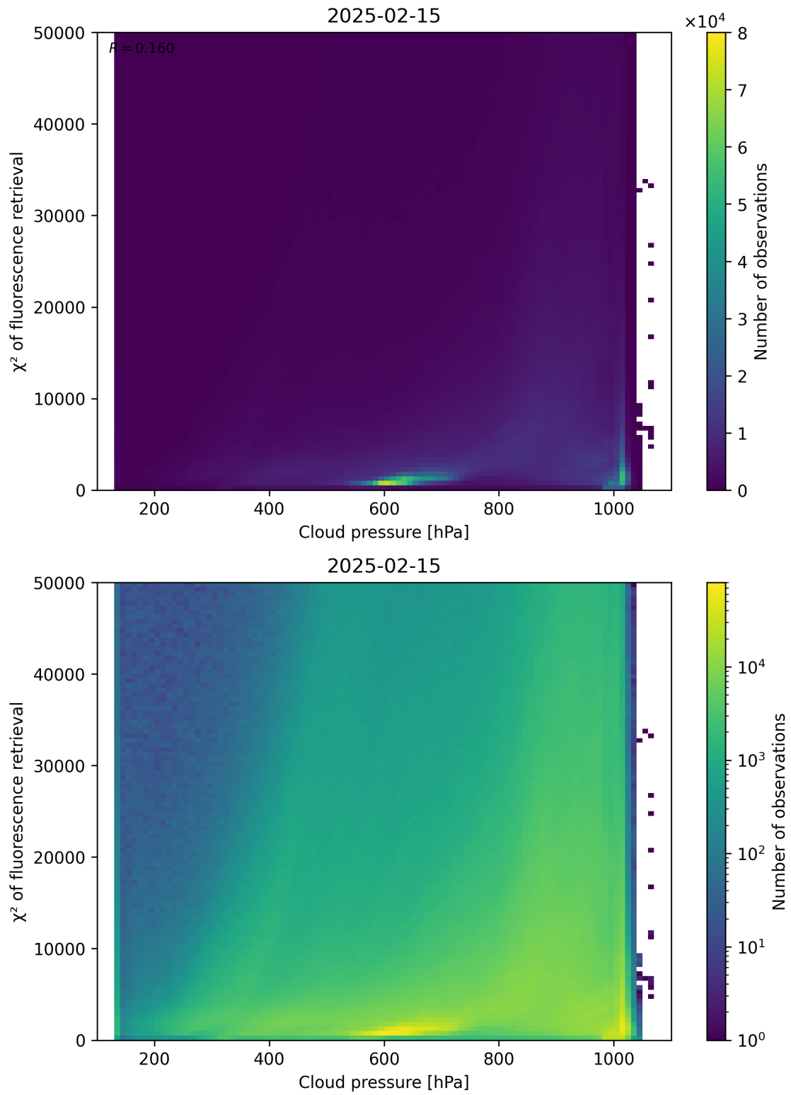
Figure 78: Scatter density plot of “Cloud pressure” against “ \chi^2 of fluorescence retrieval” for 2025-02-14 to 2025-02-16.
