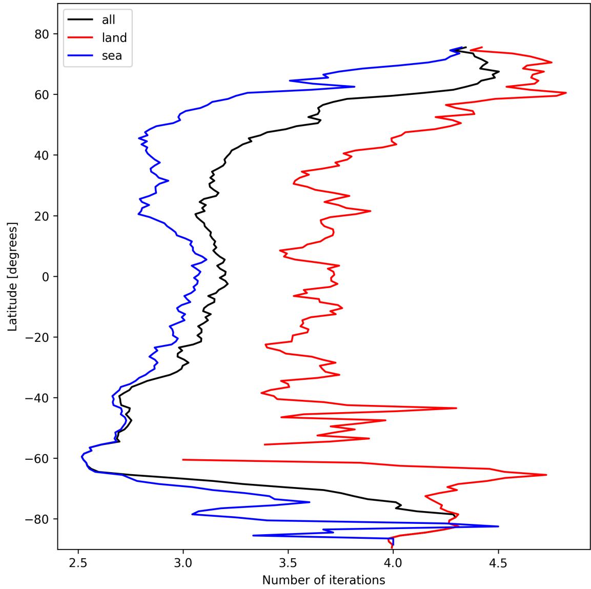
Figure 22: Zonal average of “Number of iterations” for 2025-02-14 to 2025-02-16.
