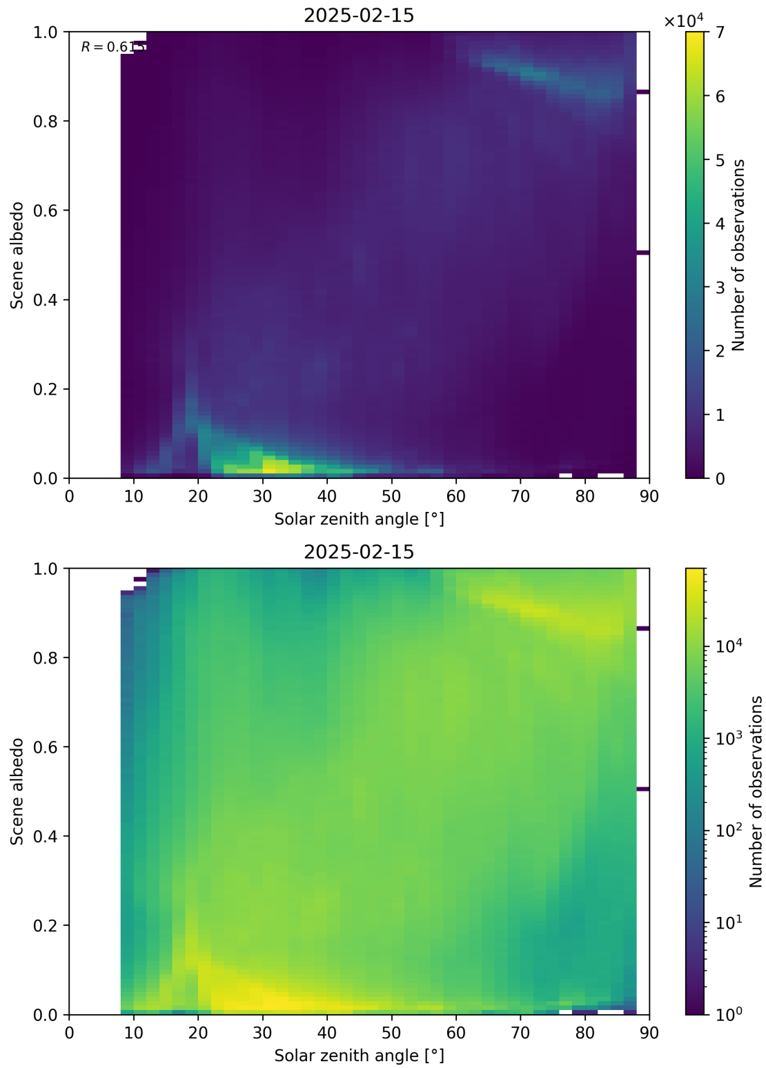
Figure 116: Scatter density plot of “Solar zenith angle” against “Scene albedo” for 2025-02-14 to 2025-02-16.
