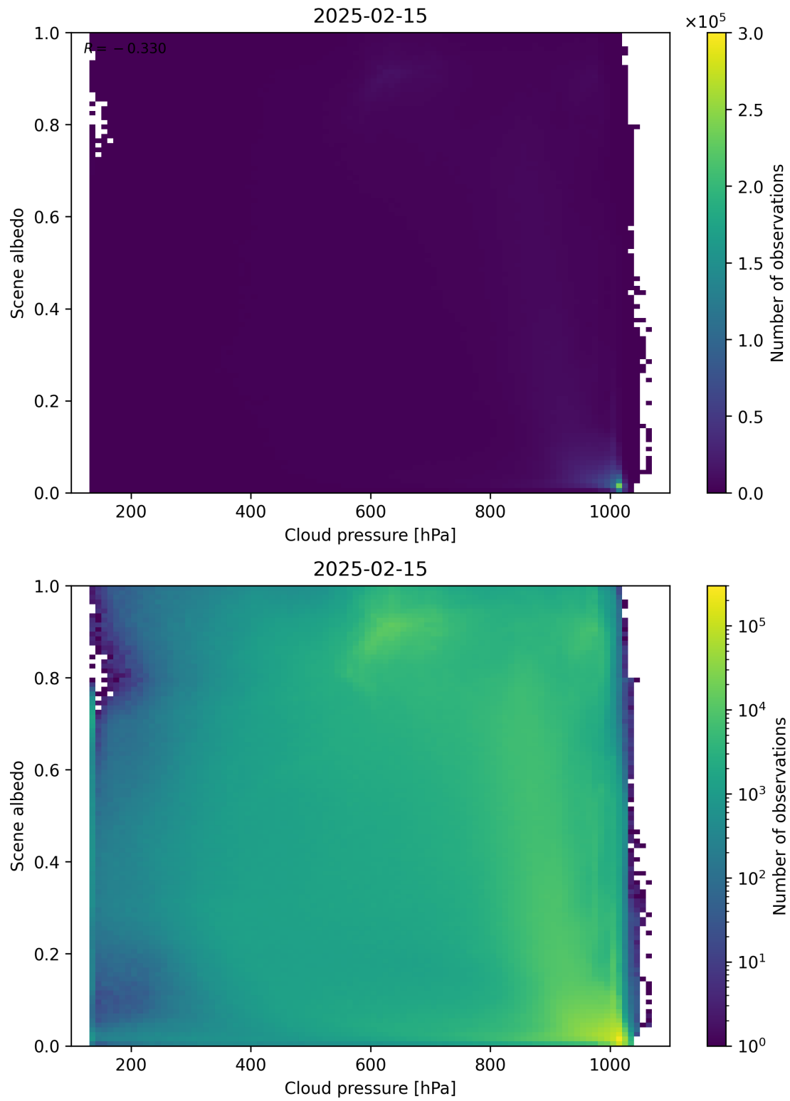
Figure 83: Scatter density plot of “Cloud pressure” against “Scene albedo” for 2025-02-14 to 2025-02-16.
