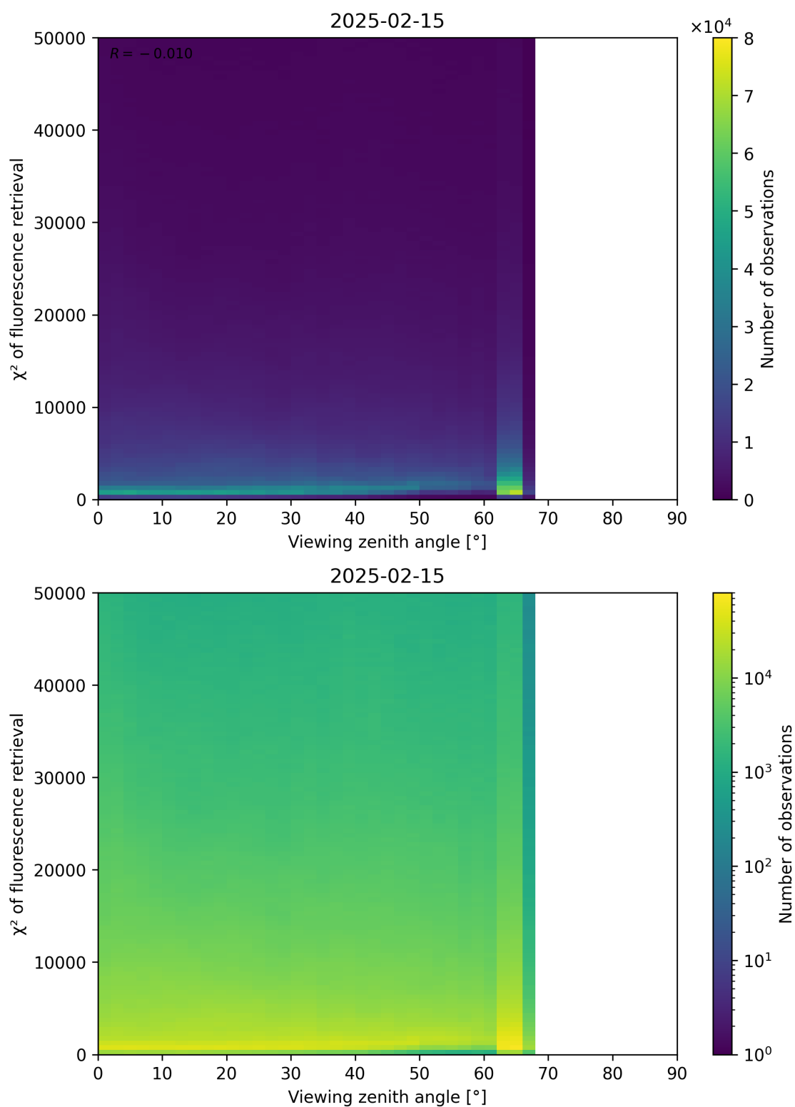
Figure 119: Scatter density plot of “Viewing zenith angle” against “ \chi^2 of fluorescence retrieval” for 2025-02-14 to 2025-02-16.
