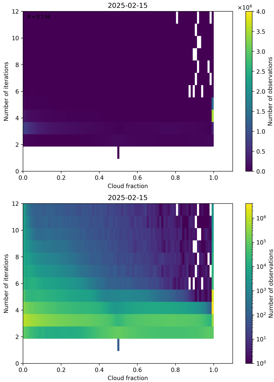
Figure 73: Scatter density plot of “Cloud fraction” against “Number of iterations” for 2025-02-14 to 2025-02-16.
