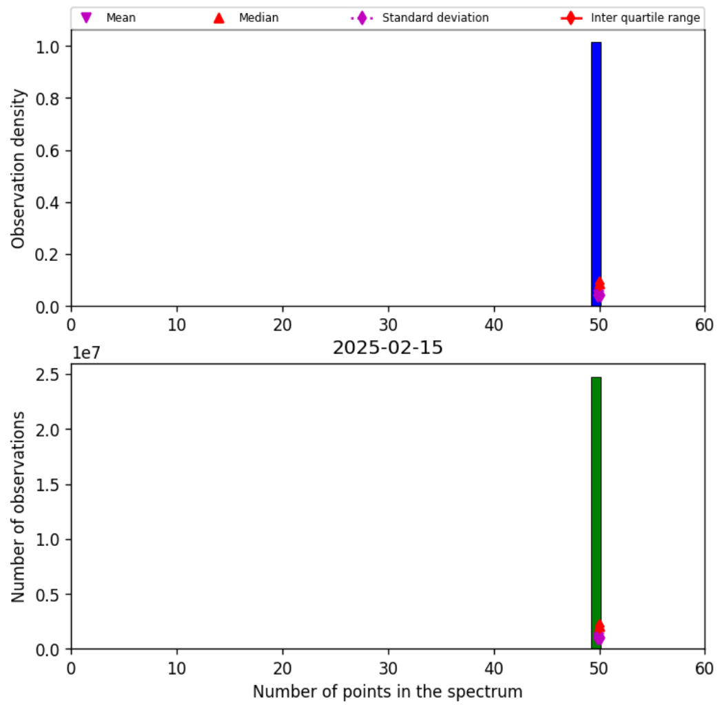
Figure 44: Histogram of “Number of points in the spectrum” for 2025-02-14 to 2025-02-16
