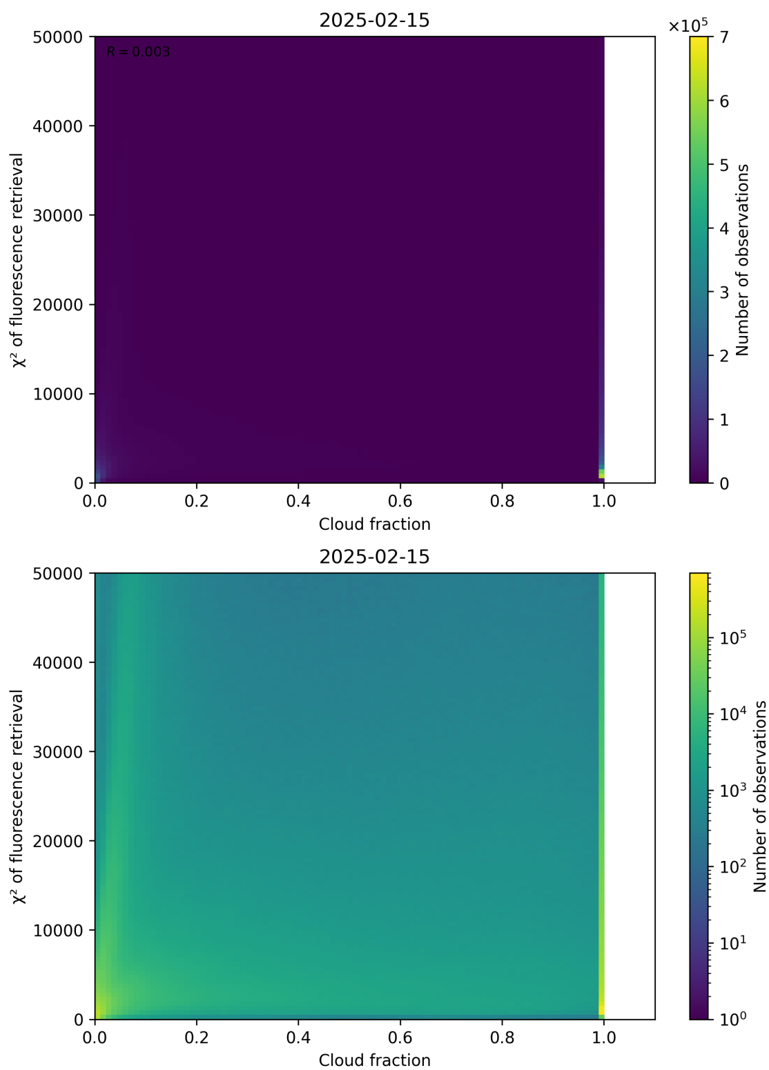
Figure 71: Scatter density plot of “Cloud fraction” against “ \chi^2 of fluorescence retrieval” for 2025-02-14 to 2025-02-16.
