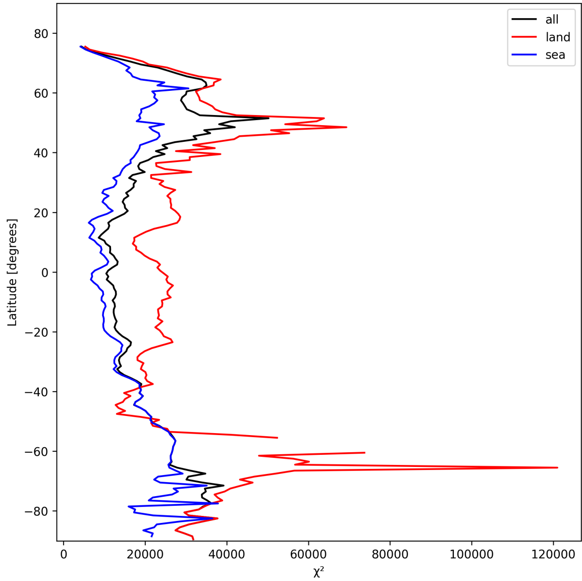
Figure 21: Zonal average of “ \chi^2 ” for 2025-02-14 to 2025-02-16.
