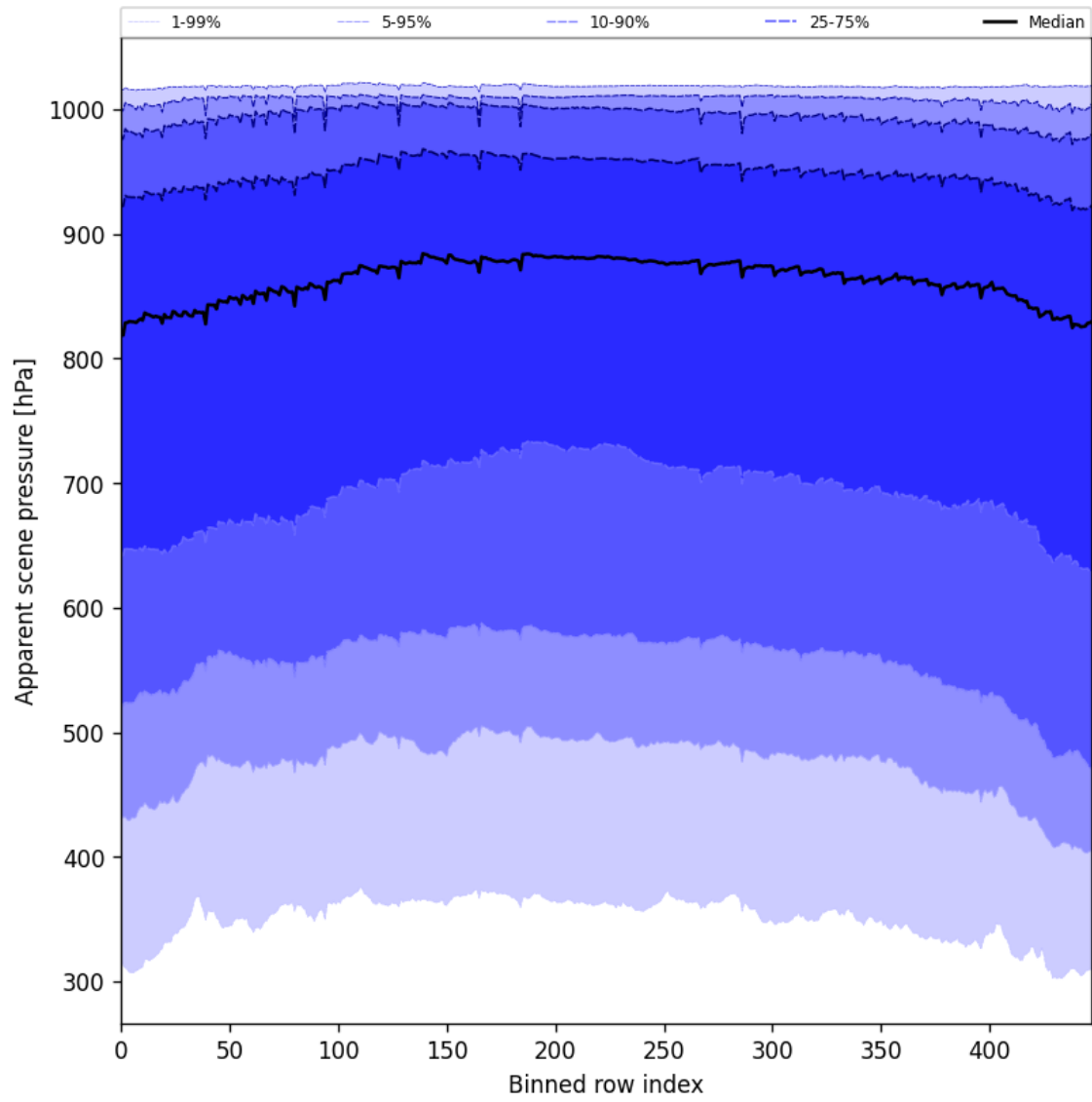
Figure 53: Along track statistics of “Apparent scene pressure” for 2025-02-14 to 2025-02-16
