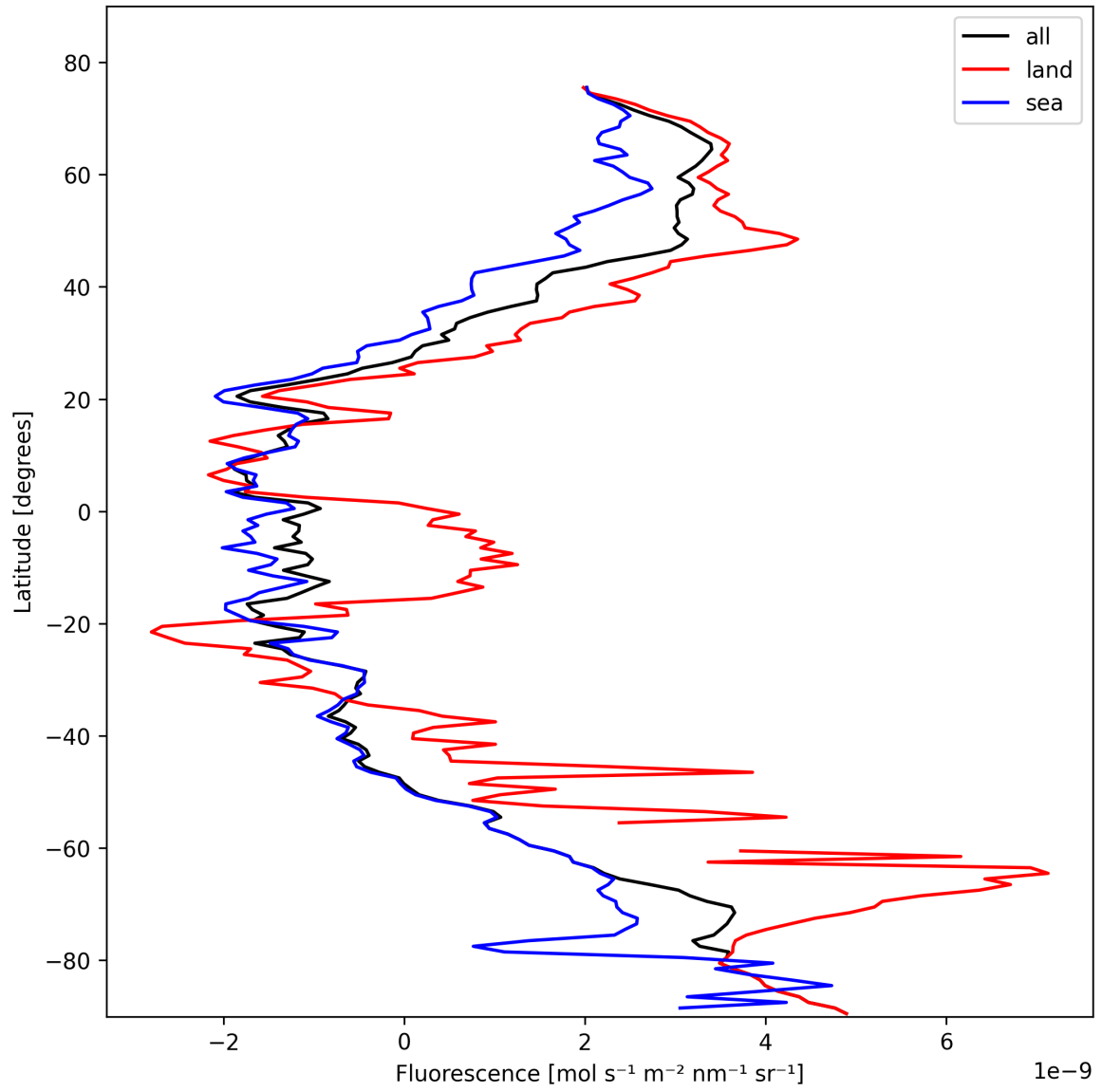
Figure 23: Zonal average of “Fluorescence” for 2025-02-14 to 2025-02-16.
