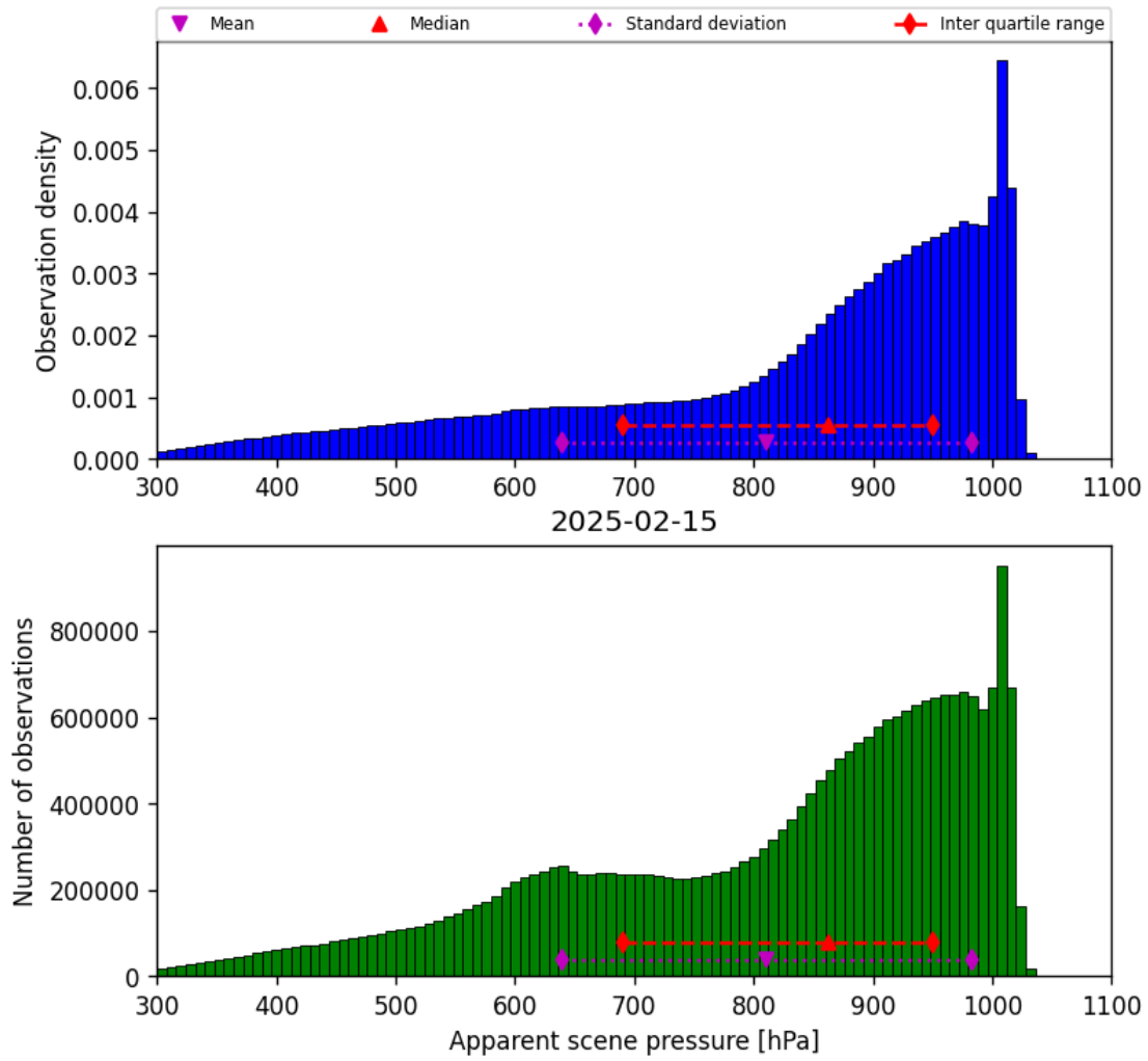
Figure 36: Histogram of “Apparent scene pressure” for 2025-02-14 to 2025-02-16
