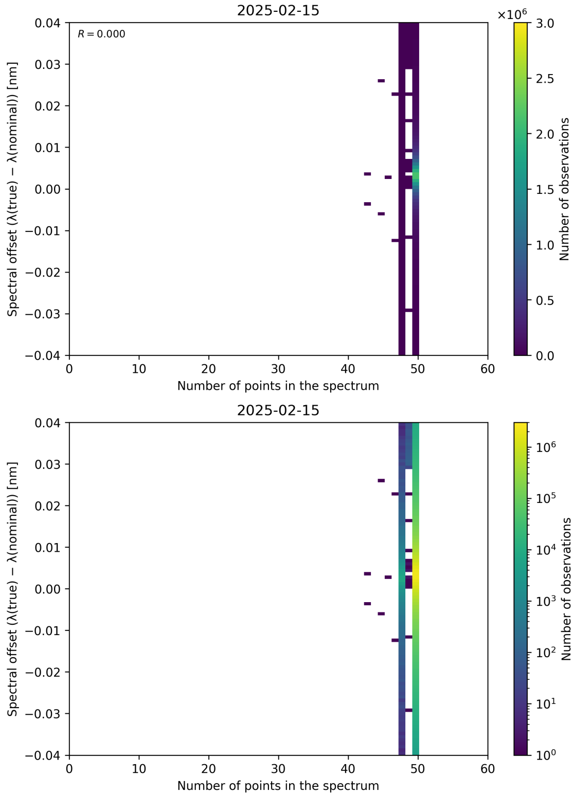
Figure 101: Scatter density plot of “Number of points in the spectrum” against “Spectral offset ( \lambda_{\text{true}} - \lambda_{\text{nominal}} )” for 2025-02-14 to 2025-02-16.
