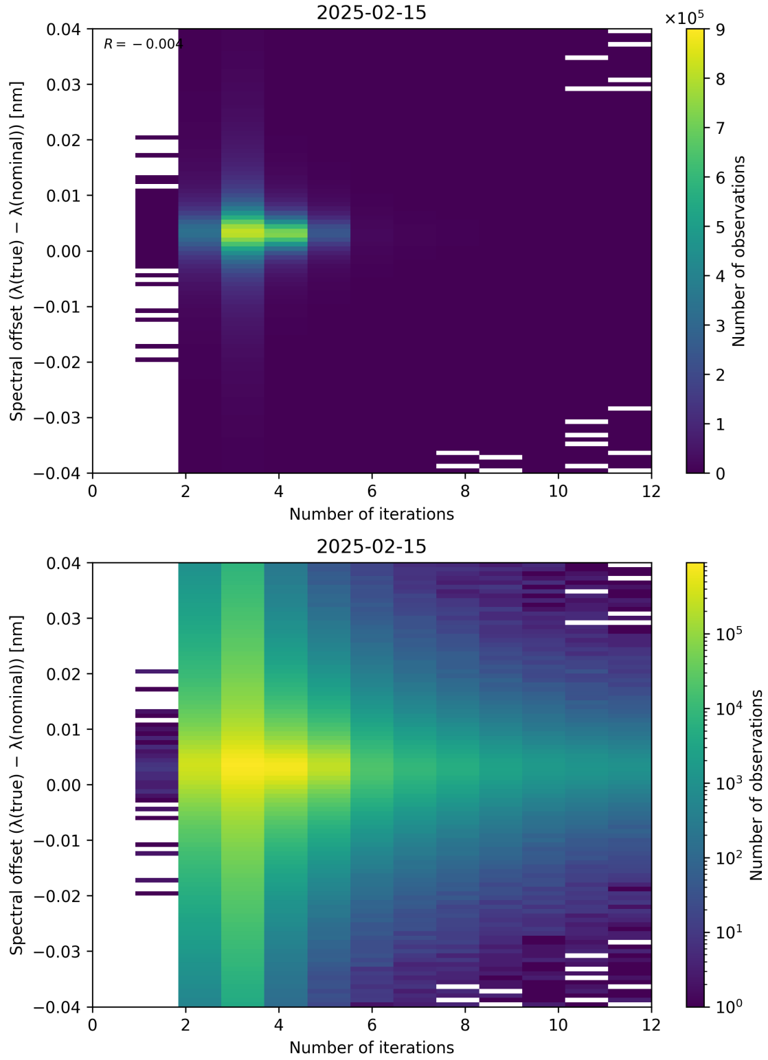
Figure 100: Scatter density plot of “Number of iterations” against “Spectral offset ( \lambda_{\text{true}} - \lambda_{\text{nominal}} )” for 2025-02-14 to 2025-02-16.
