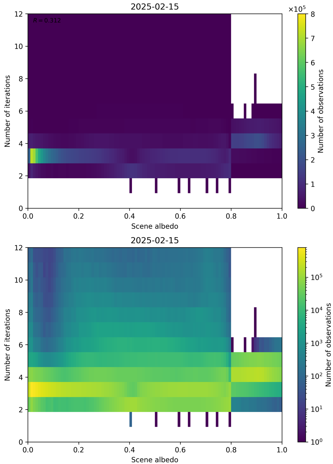
Figure 105: Scatter density plot of “Scene albedo” against “Number of iterations” for 2025-02-14 to 2025-02-16.
