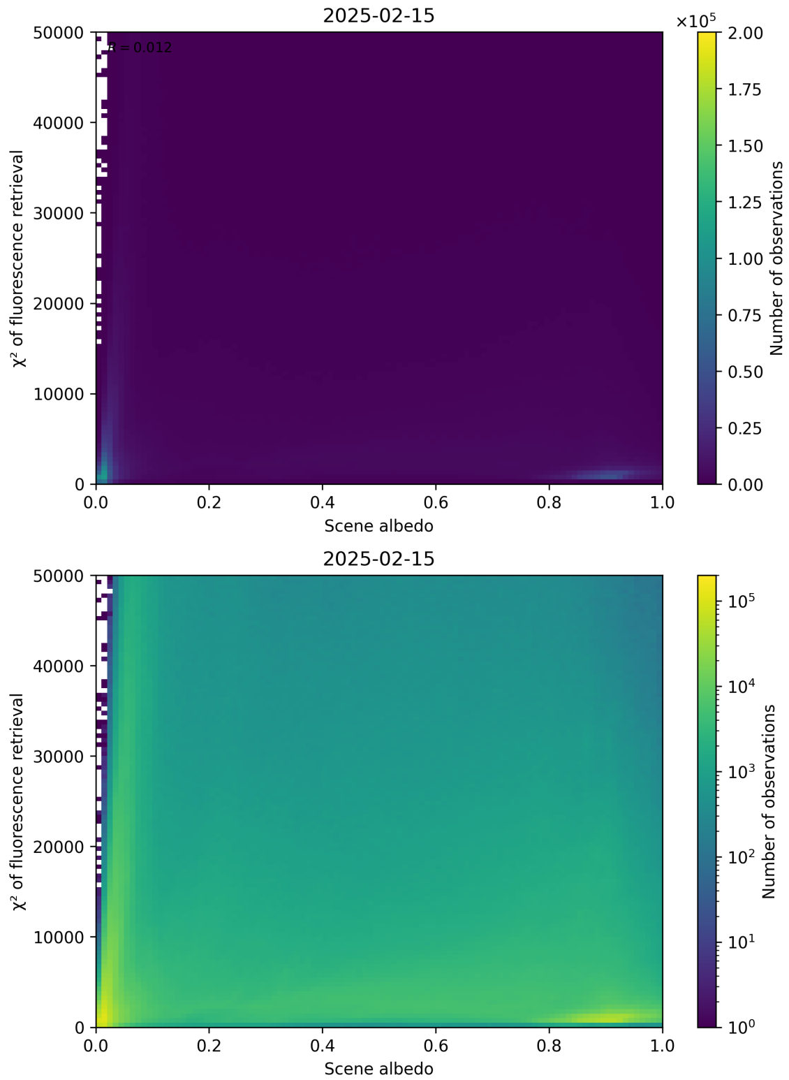
Figure 103: Scatter density plot of “Scene albedo” against “ \chi^2 of fluorescence retrieval” for 2025-02-14 to 2025-02-16.
