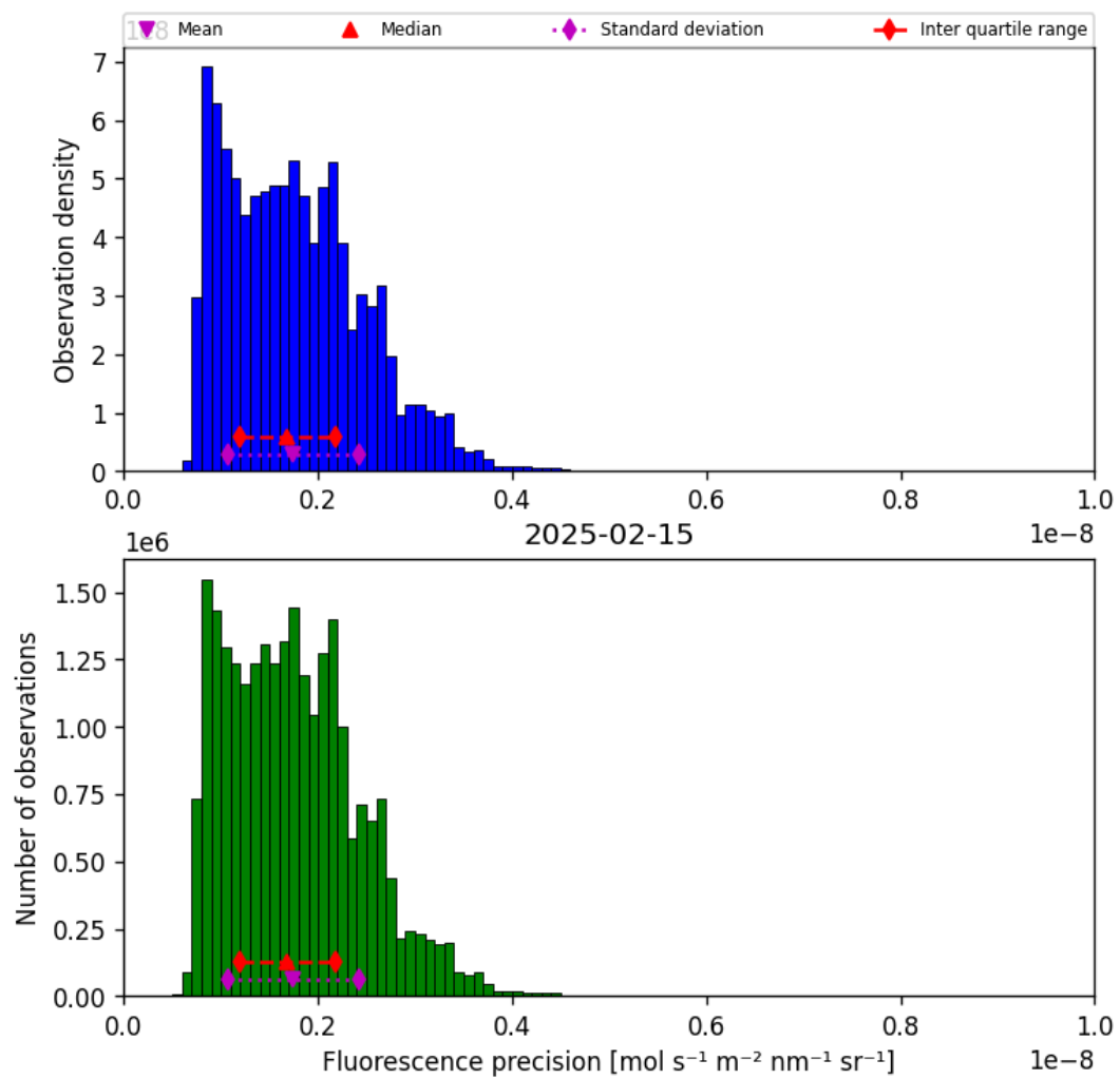
Figure 41: Histogram of “Fluorescence precision” for 2025-02-14 to 2025-02-16
