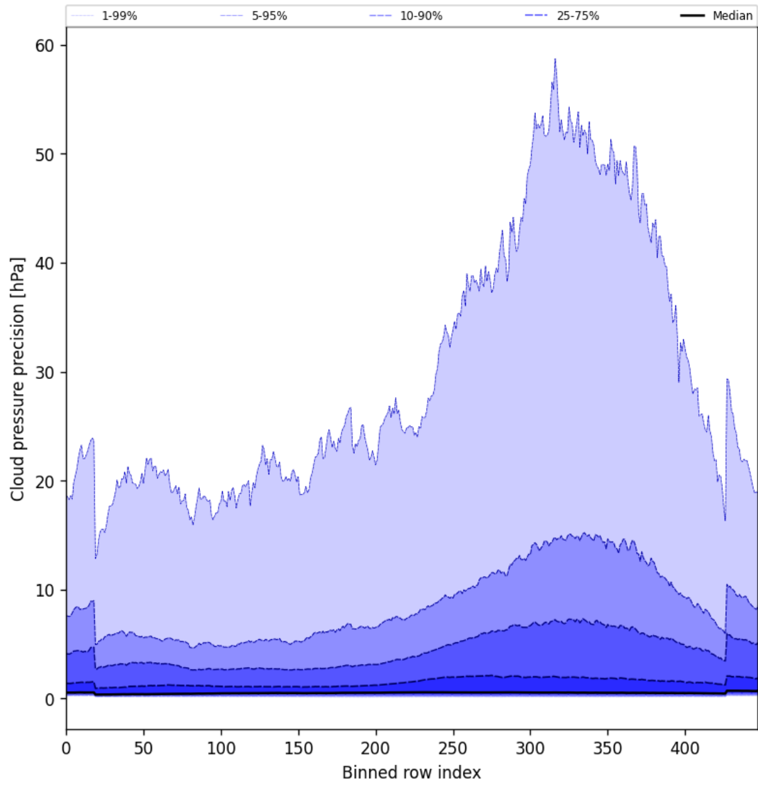
Figure 48: Along track statistics of “Cloud pressure precision” for 2025-02-14 to 2025-02-16
