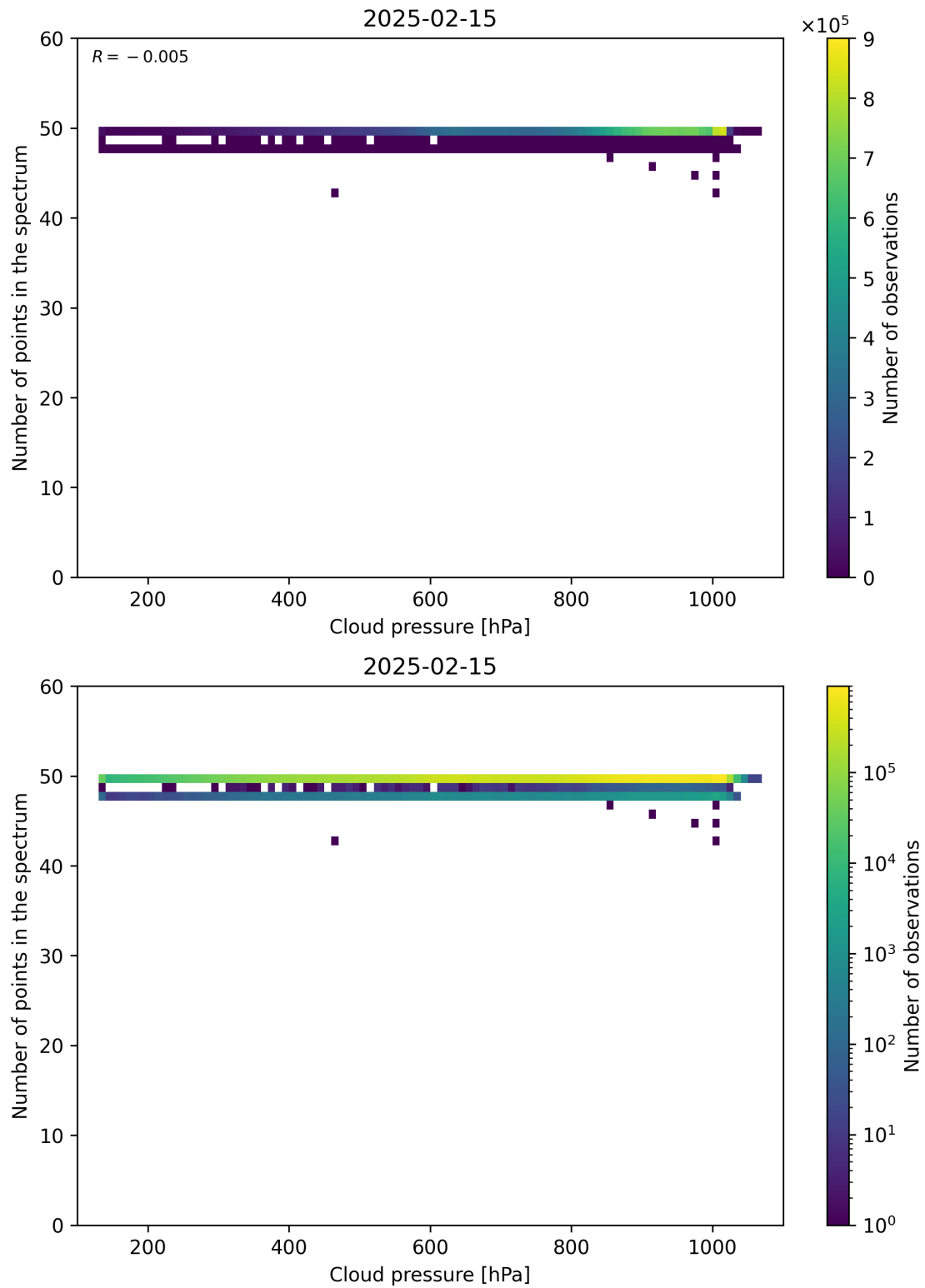
Figure 82: Scatter density plot of “Cloud pressure” against “Number of points in the spectrum” for 2025-02-14 to 2025-02-16.
