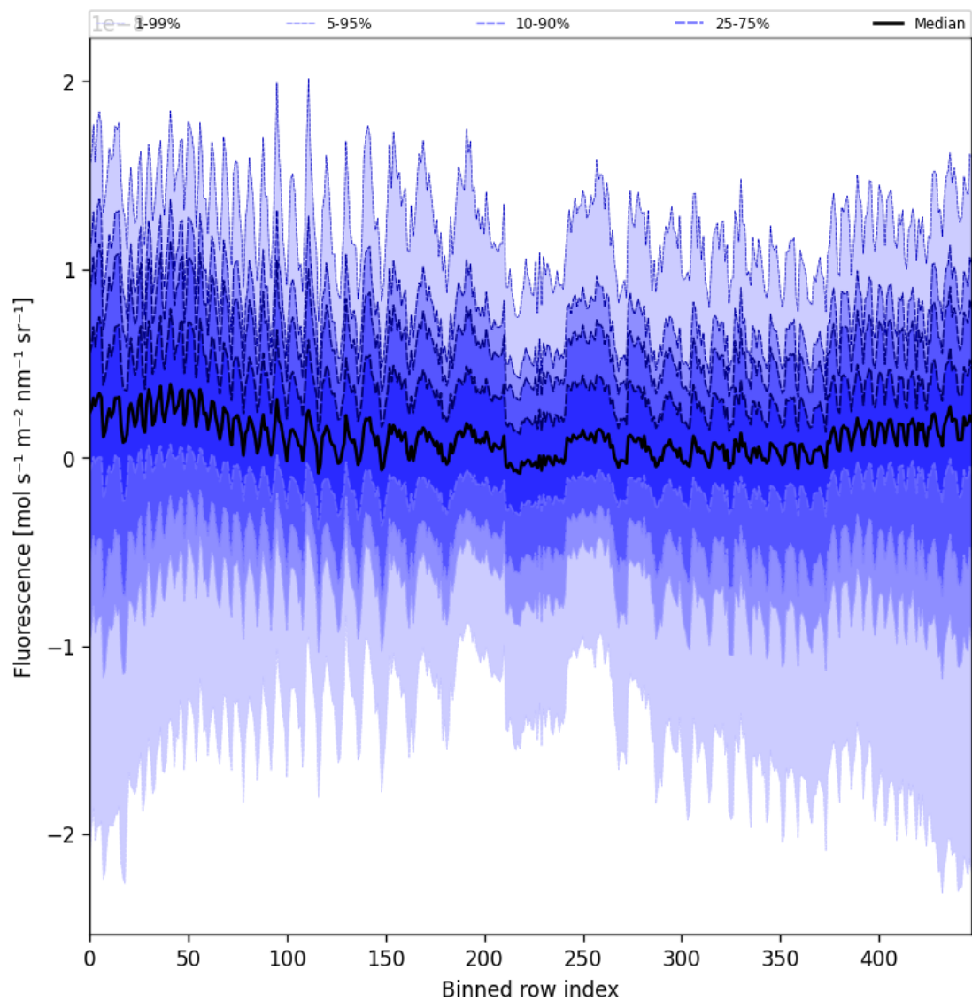
Figure 57: Along track statistics of “Fluorescence” for 2025-02-14 to 2025-02-16
