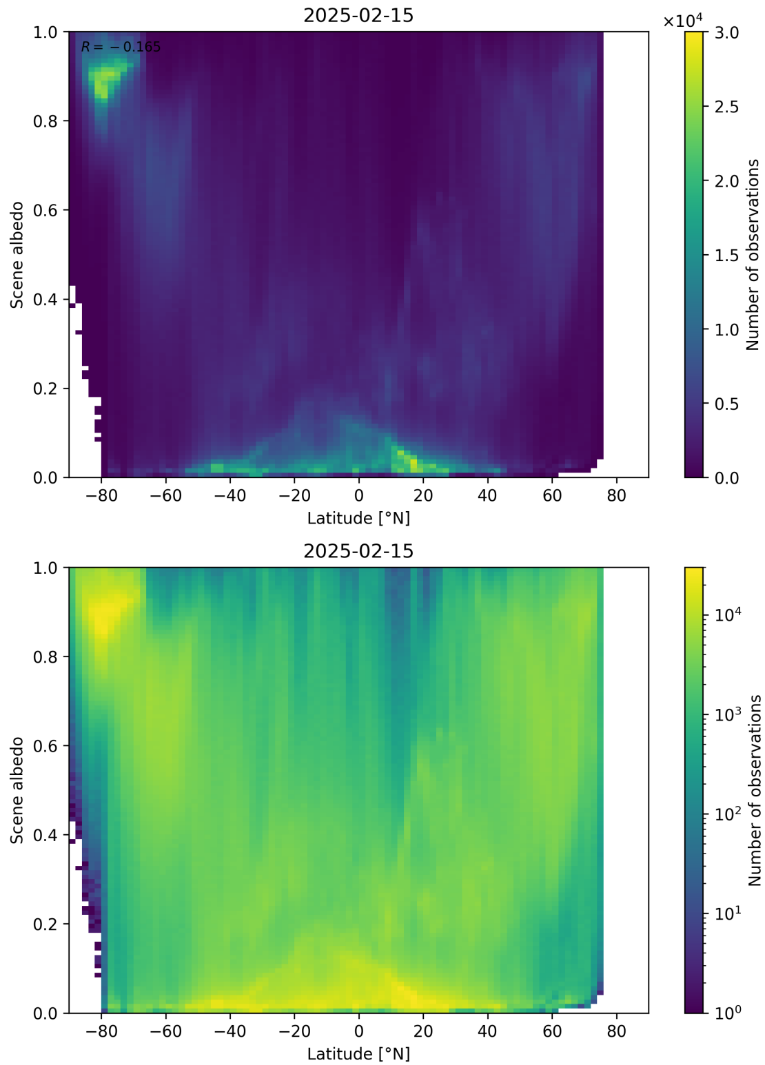
Figure 95: Scatter density plot of “Latitude” against “Scene albedo” for 2025-02-14 to 2025-02-16.
