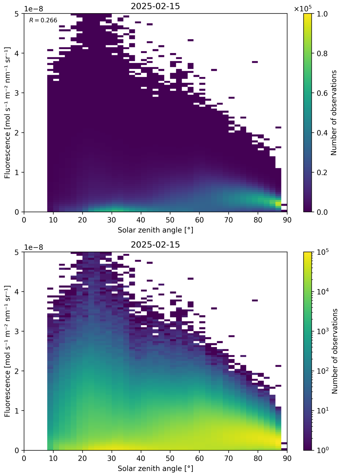
Figure 112: Scatter density plot of “Solar zenith angle” against “Fluorescence” for 2025-02-14 to 2025-02-16.
