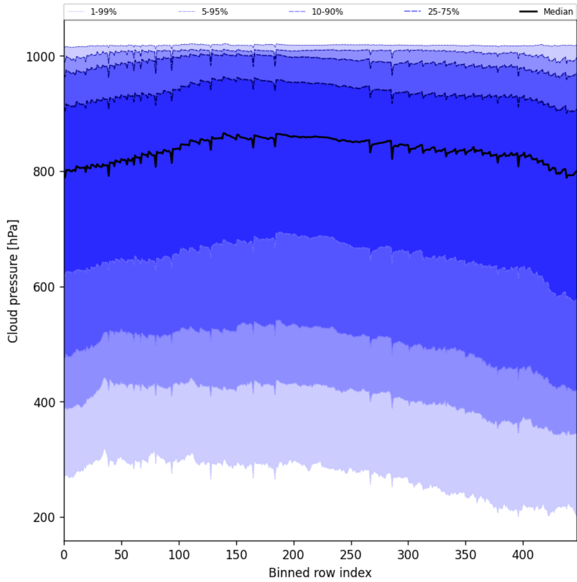
Figure 47: Along track statistics of “Cloud pressure” for 2025-02-14 to 2025-02-16
