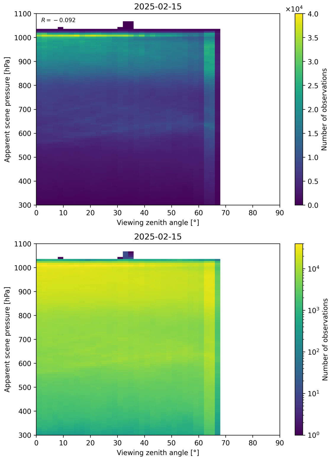
Figure 118: Scatter density plot of “Viewing zenith angle” against “Apparent scene pressure” for 2025-02-14 to 2025-02-16.
