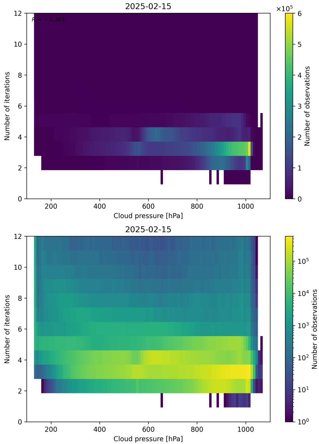
Figure 81: Scatter density plot of “Cloud pressure” against “Number of iterations” for 2025-02-14 to 2025-02-16.
