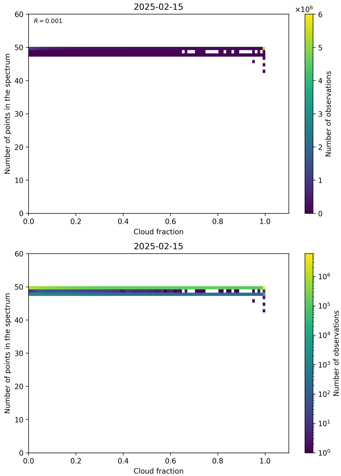
Figure 74: Scatter density plot of “Cloud fraction” against “Number of points in the spectrum” for 2025-02-14 to 2025-02-16.
