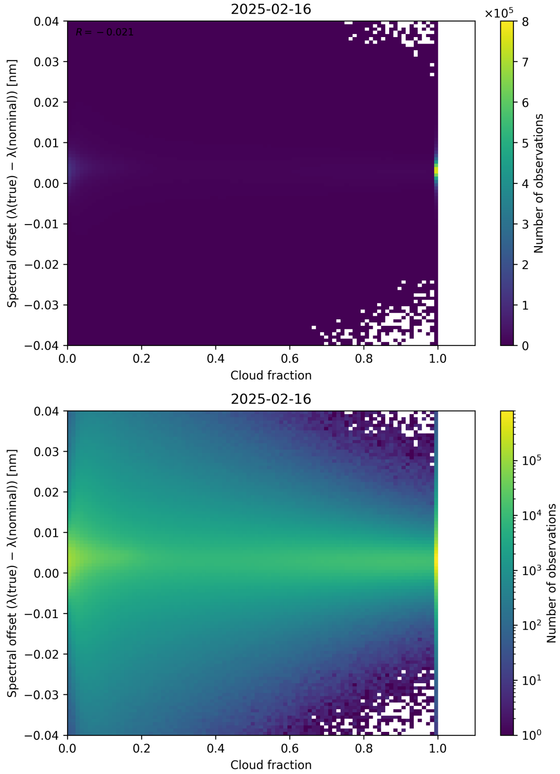
Figure 76: Scatter density plot of “Cloud fraction” against “Spectral offset ( \lambda_{\text{true}} - \lambda_{\text{nominal}} )” for 2025-02-15 to 2025-02-17.
