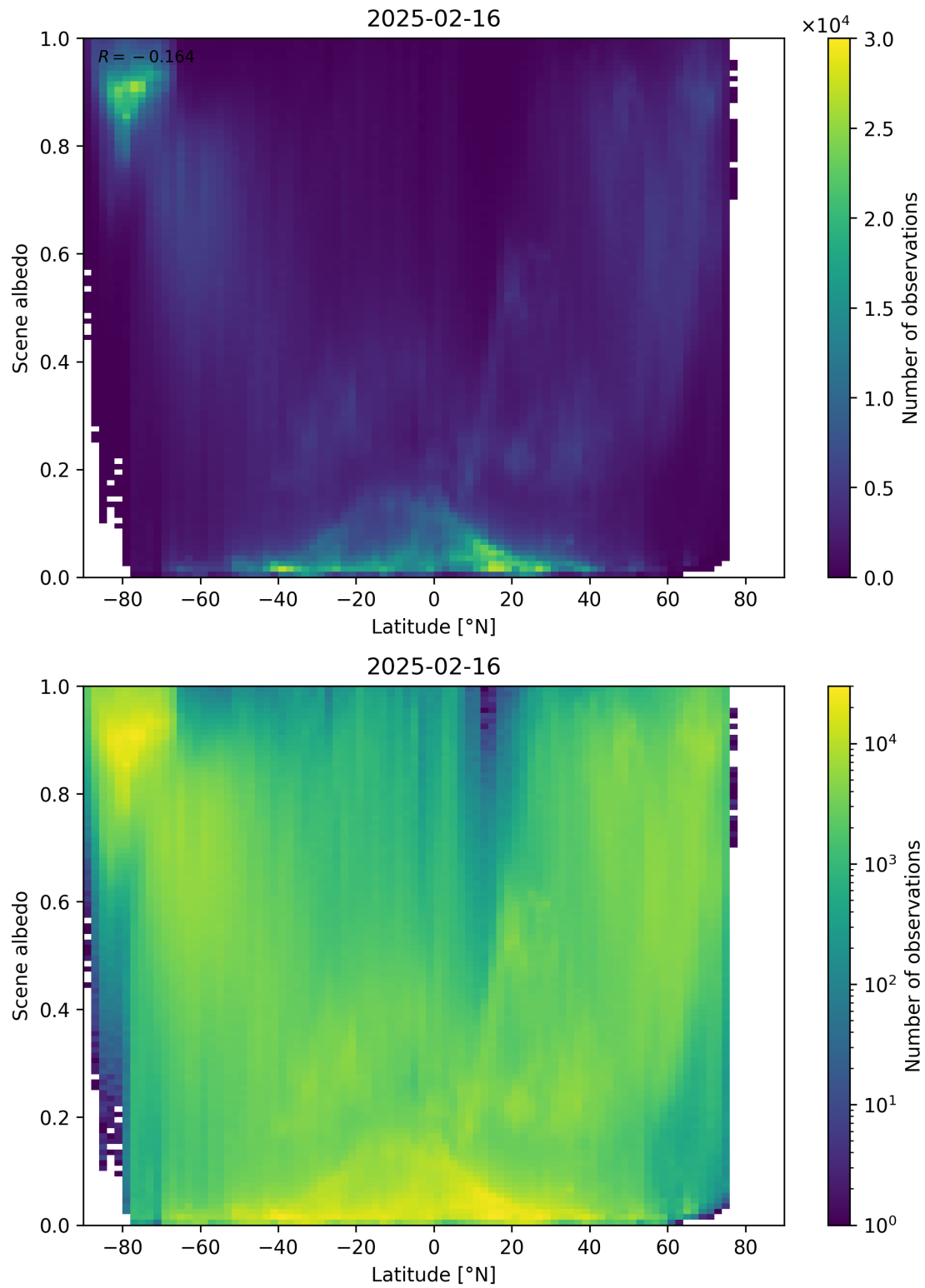
Figure 95: Scatter density plot of “Latitude” against “Scene albedo” for 2025-02-15 to 2025-02-17.
