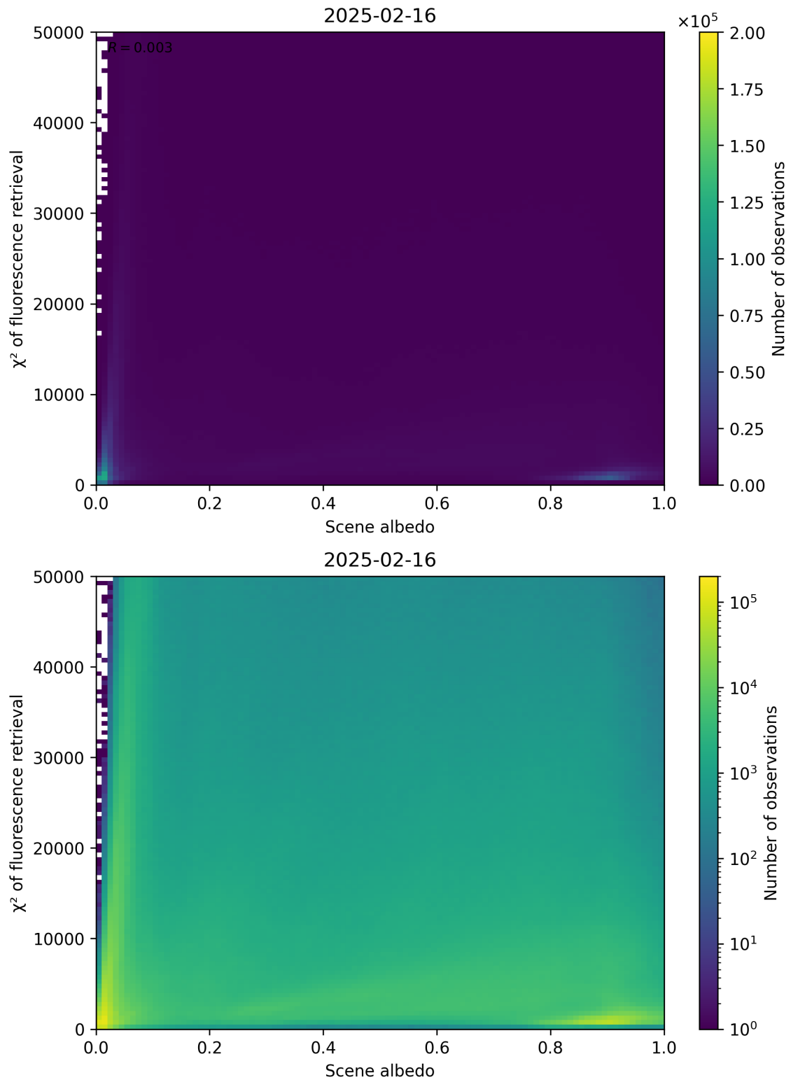
Figure 103: Scatter density plot of “Scene albedo” against “ \chi^2 of fluorescence retrieval” for 2025-02-15 to 2025-02-17.
