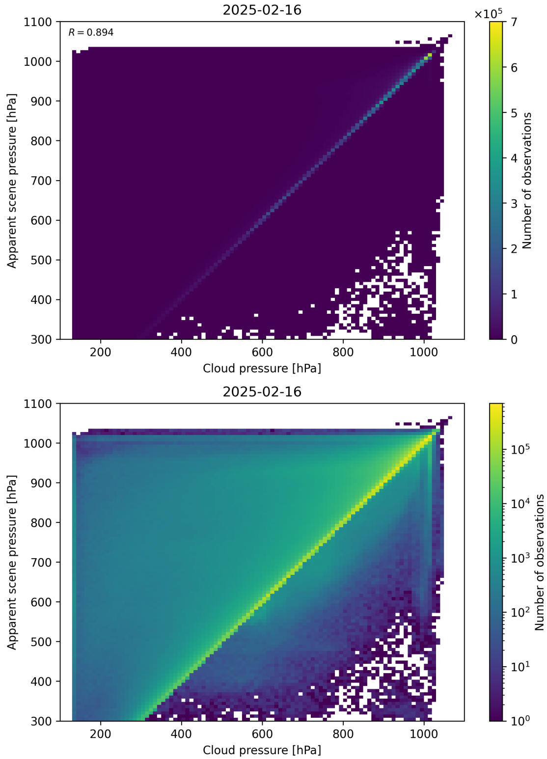
Figure 77: Scatter density plot of “Cloud pressure” against “Apparent scene pressure” for 2025-02-15 to 2025-02-17.
