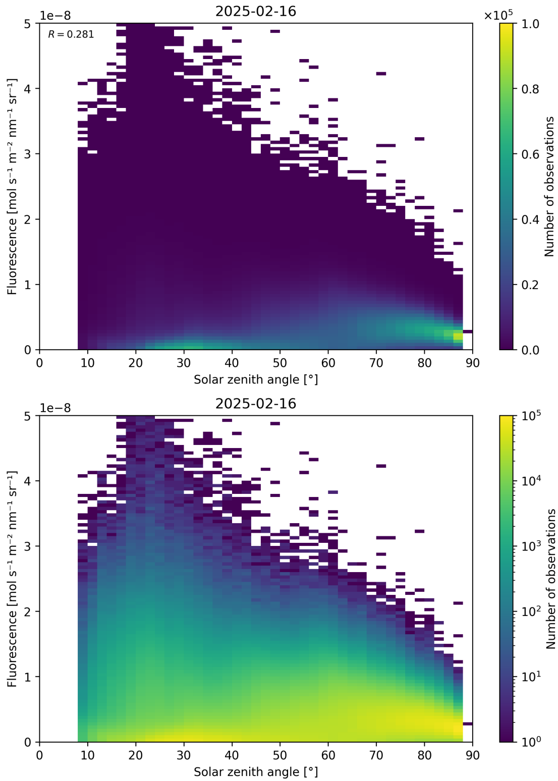
Figure 112: Scatter density plot of “Solar zenith angle” against “Fluorescence” for 2025-02-15 to 2025-02-17.
