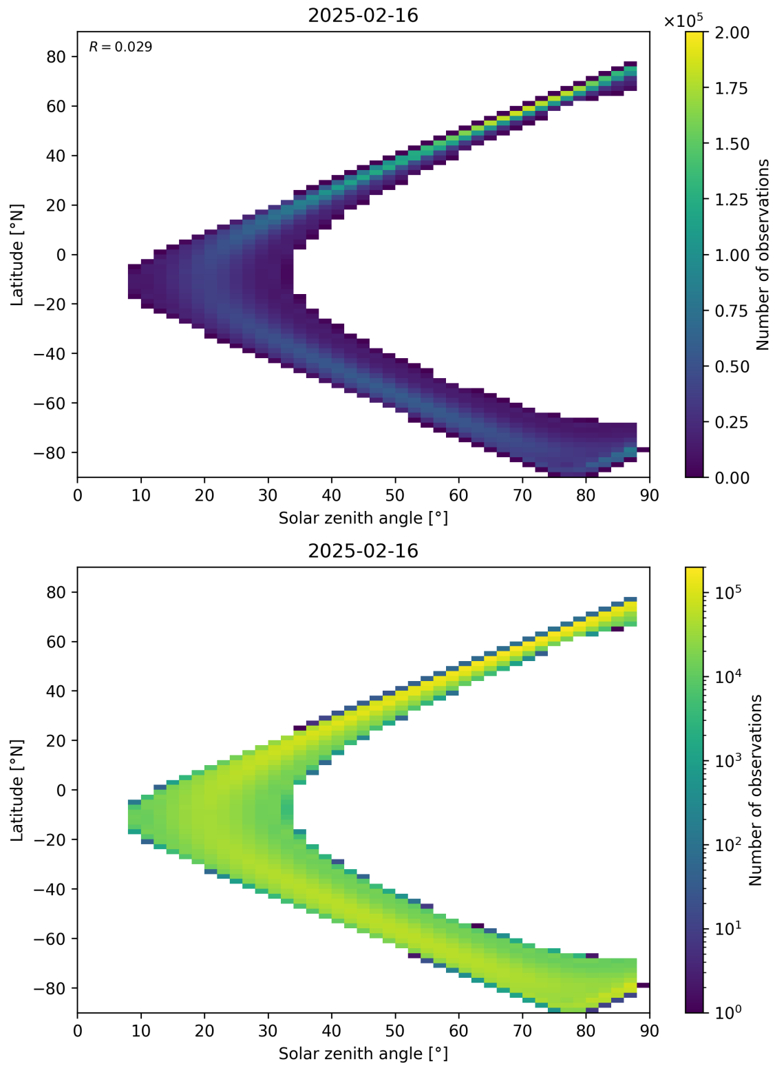
Figure 113: Scatter density plot of “Solar zenith angle” against “Latitude” for 2025-02-15 to 2025-02-17.
