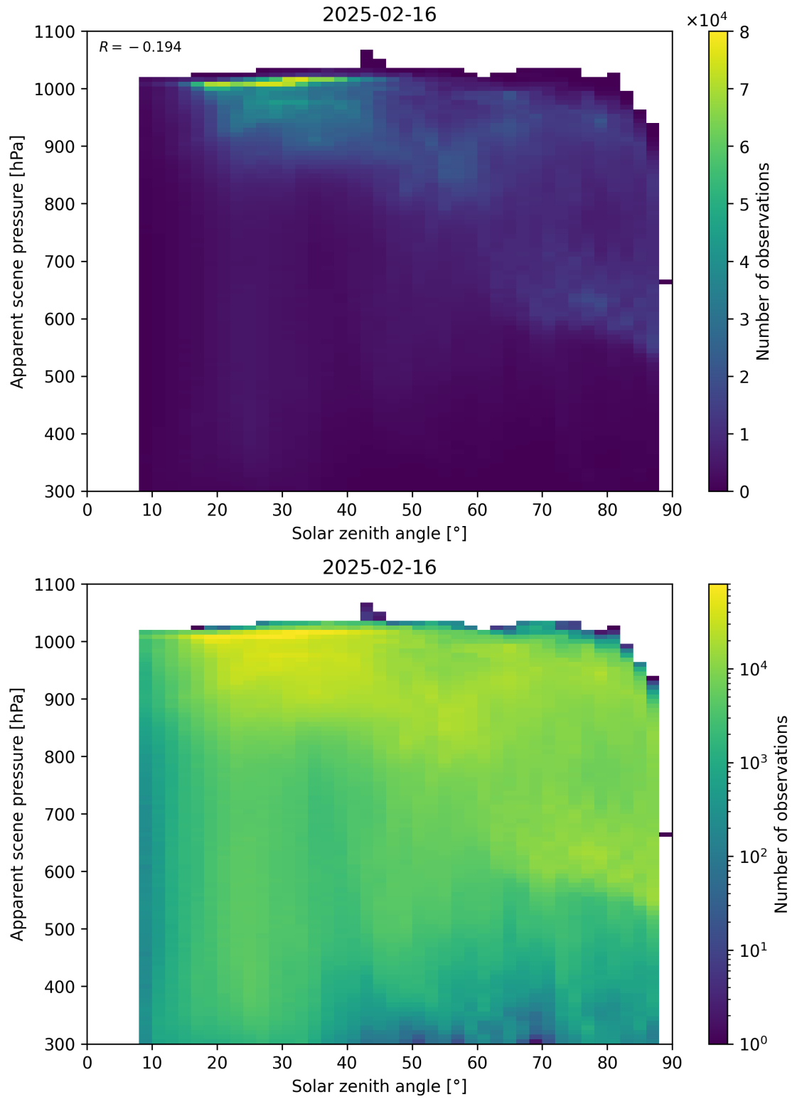
Figure 108: Scatter density plot of “Solar zenith angle” against “Apparent scene pressure” for 2025-02-15 to 2025-02-17.
