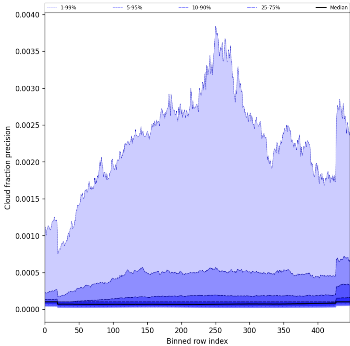
Figure 50: Along track statistics of “Cloud fraction precision” for 2025-02-15 to 2025-02-17
