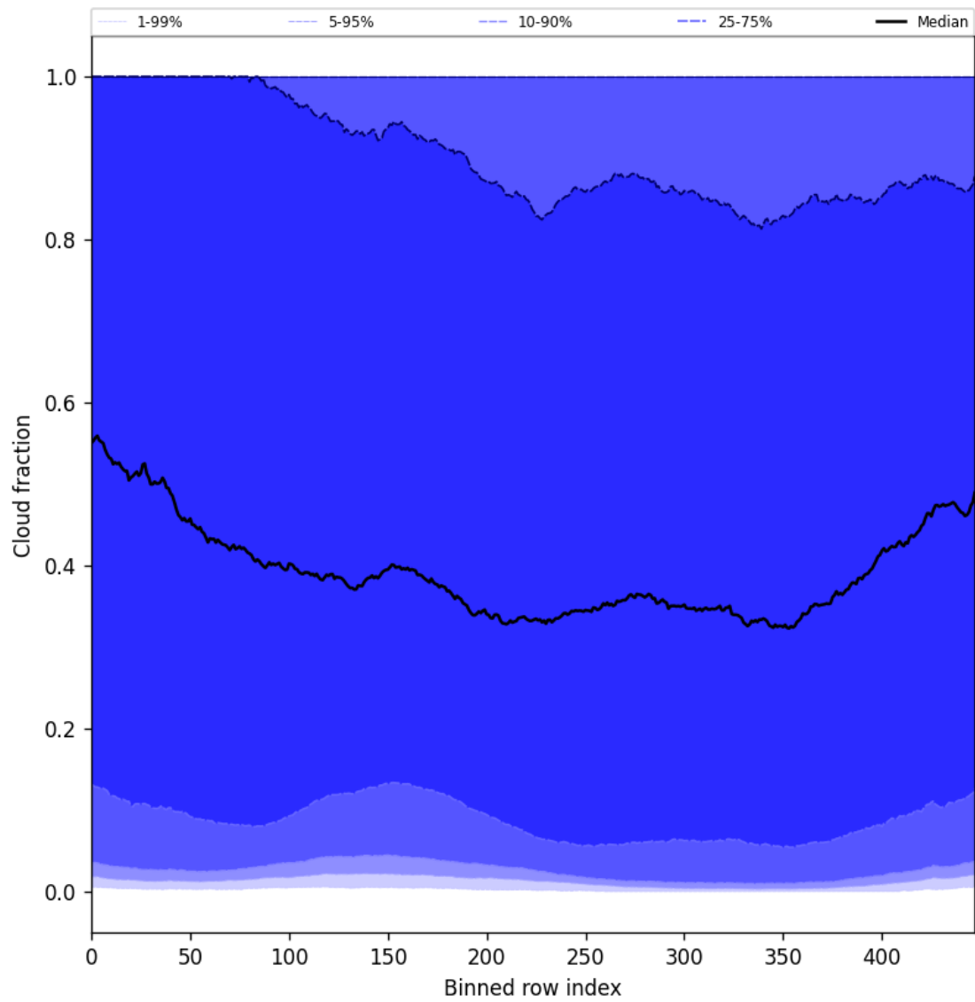
Figure 49: Along track statistics of “Cloud fraction” for 2025-02-15 to 2025-02-17
