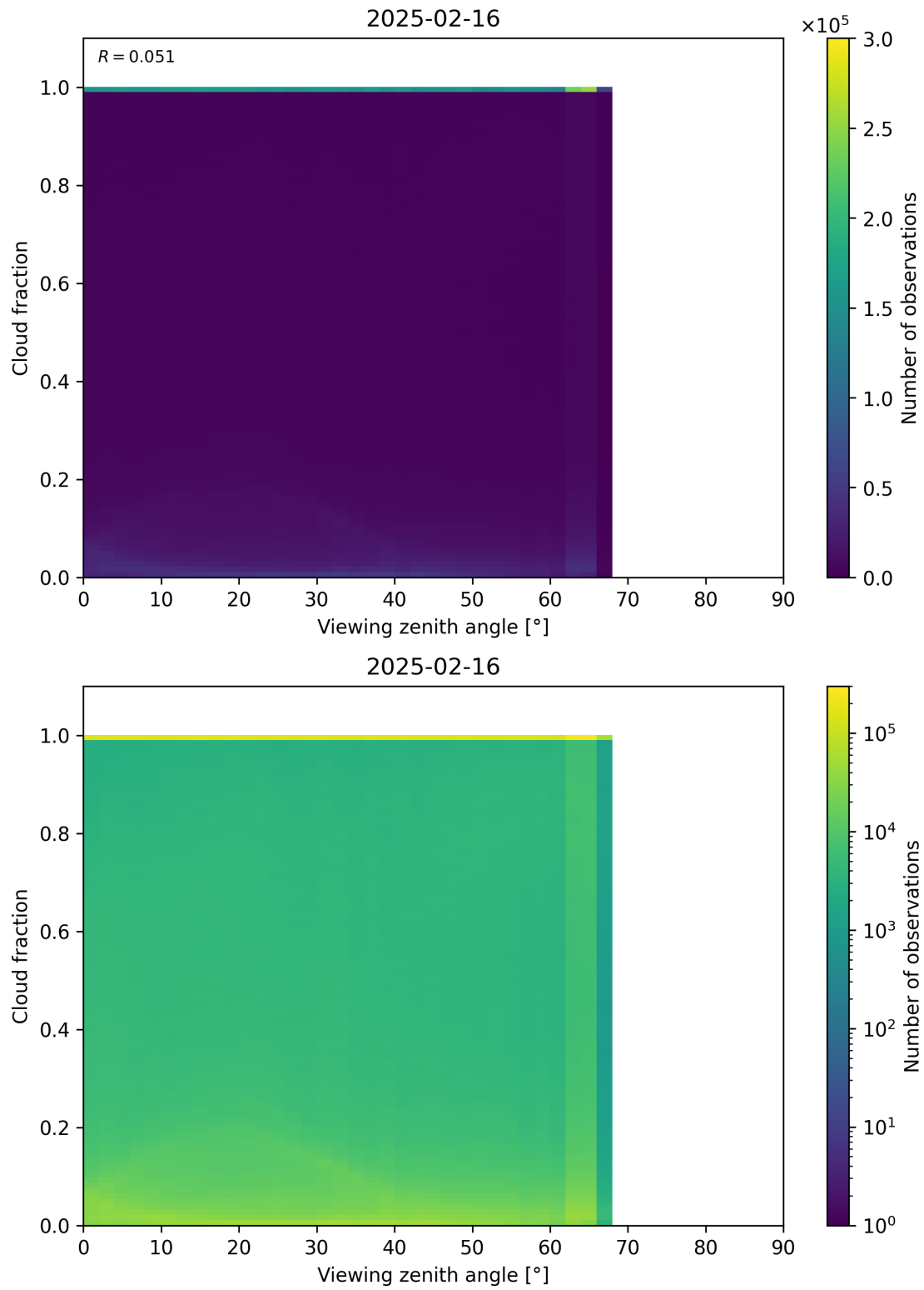
Figure 120: Scatter density plot of “Viewing zenith angle” against “Cloud fraction” for 2025-02-15 to 2025-02-17.
