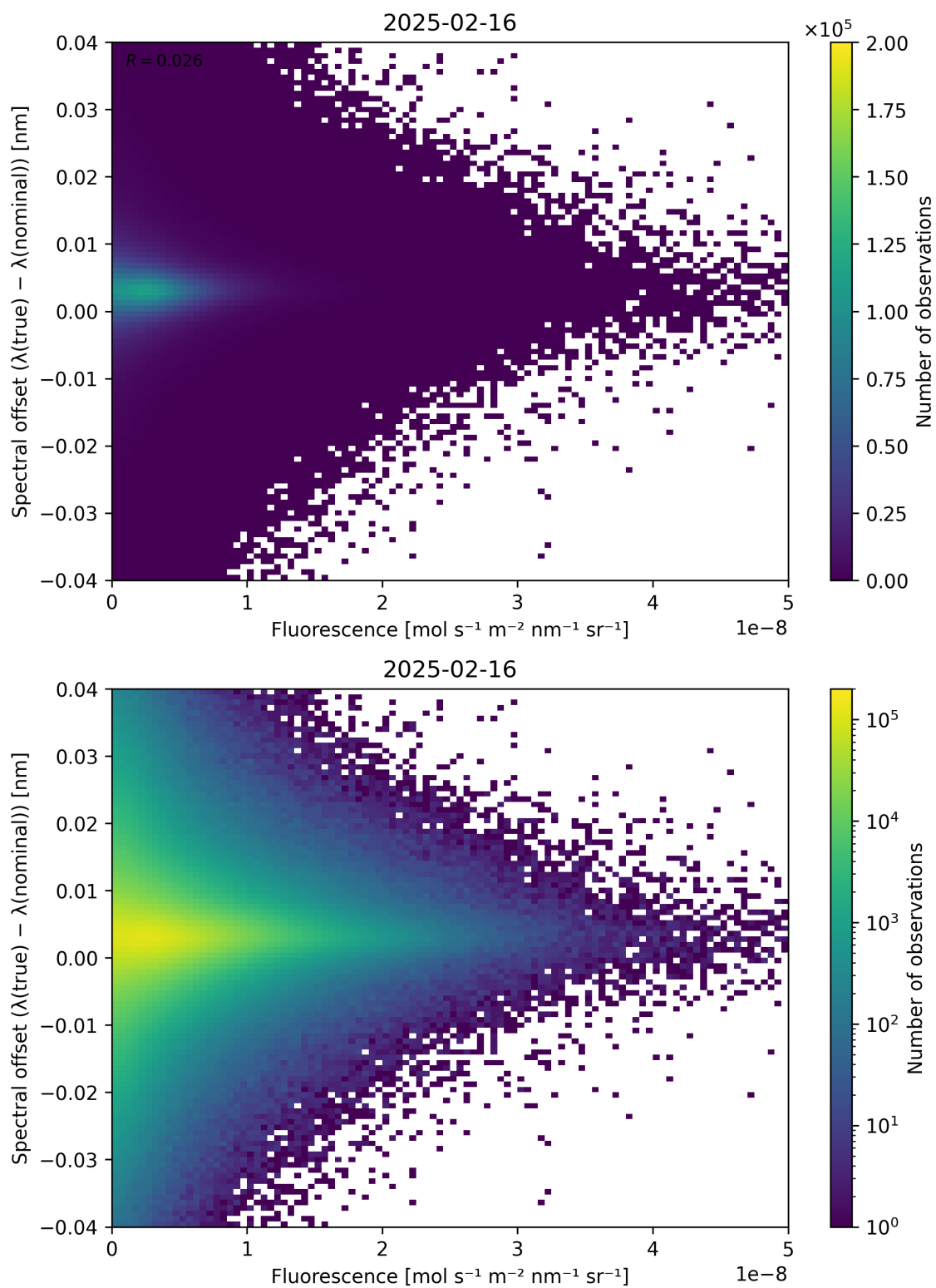
Figure 87: Scatter density plot of “Fluorescence” against “Spectral offset ( \lambda_{\text{true}} - \lambda_{\text{nominal}} )” for 2025-02-15 to 2025-02-17.
