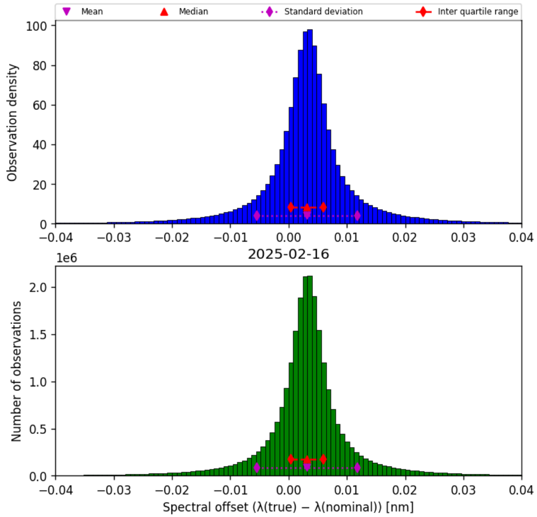
Figure 45: Histogram of “Spectral offset ( \lambda_{\text{true}} - \lambda_{\text{nominal}} )” for 2025-02-15 to 2025-02-17
