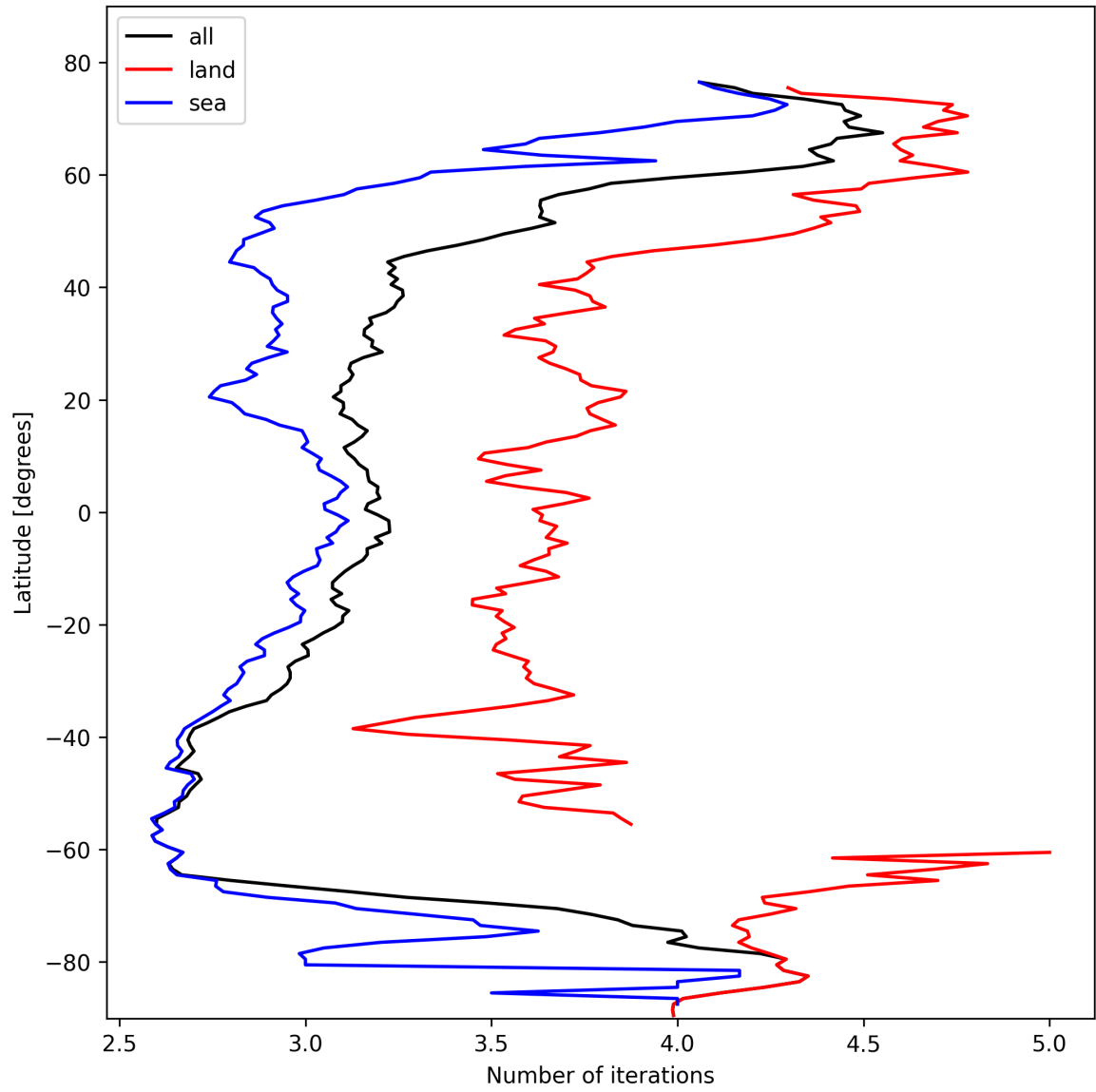
Figure 22: Zonal average of “Number of iterations” for 2025-02-15 to 2025-02-17.
