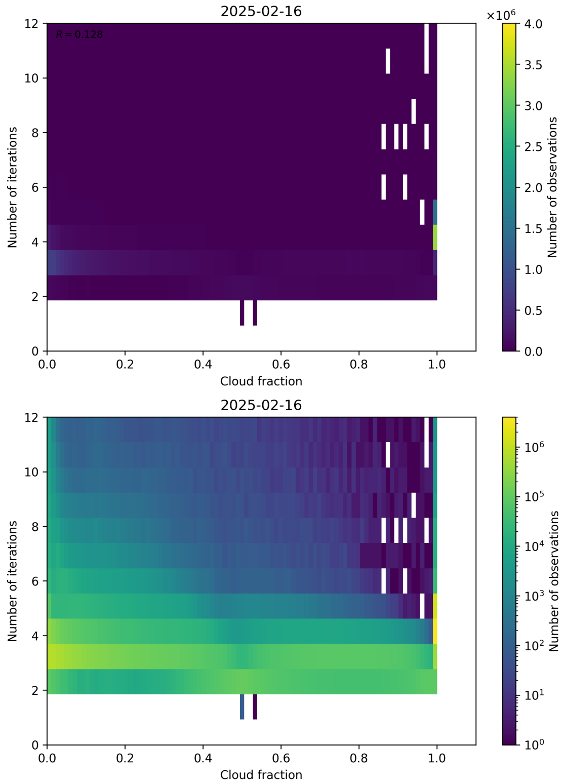
Figure 73: Scatter density plot of “Cloud fraction” against “Number of iterations” for 2025-02-15 to 2025-02-17.
