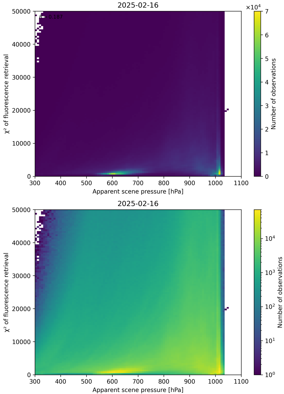
Figure 63: Scatter density plot of “Apparent scene pressure” against “ \chi^2 of fluorescence retrieval” for 2025-02-15 to 2025-02-17.
