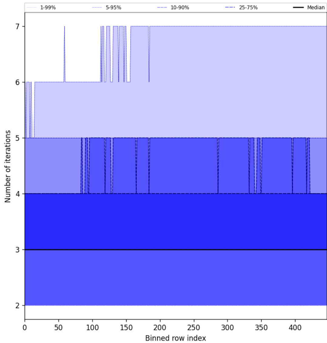
Figure 56: Along track statistics of “Number of iterations” for 2025-02-15 to 2025-02-17
