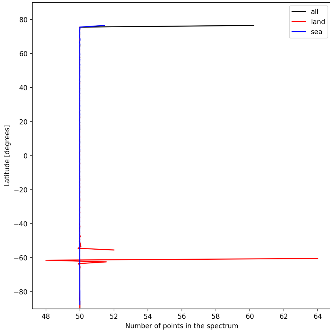
Figure 27: Zonal average of “Number of points in the spectrum” for 2025-02-15 to 2025-02-17.
