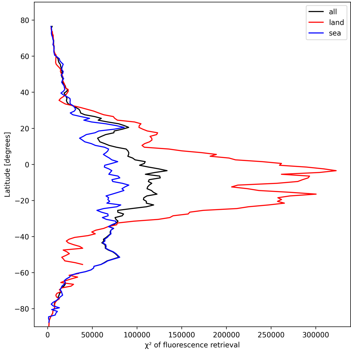
Figure 25: Zonal average of “ \chi^2 of fluorescence retrieval” for 2025-02-15 to 2025-02-17.
