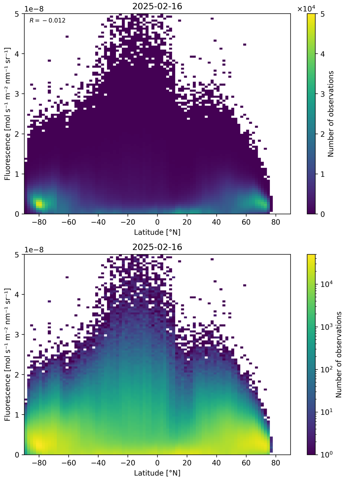
Figure 92: Scatter density plot of “Latitude” against “Fluorescence” for 2025-02-15 to 2025-02-17.
