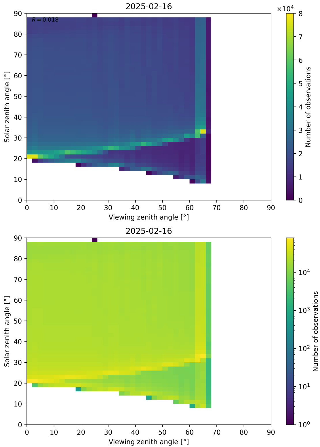
Figure 127: Scatter density plot of “Viewing zenith angle” against “Solar zenith angle” for 2025-02-15 to 2025-02-17.
