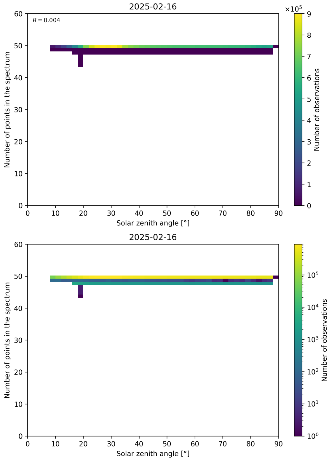
Figure 115: Scatter density plot of “Solar zenith angle” against “Number of points in the spectrum” for 2025-02-15 to 2025-02-17.
