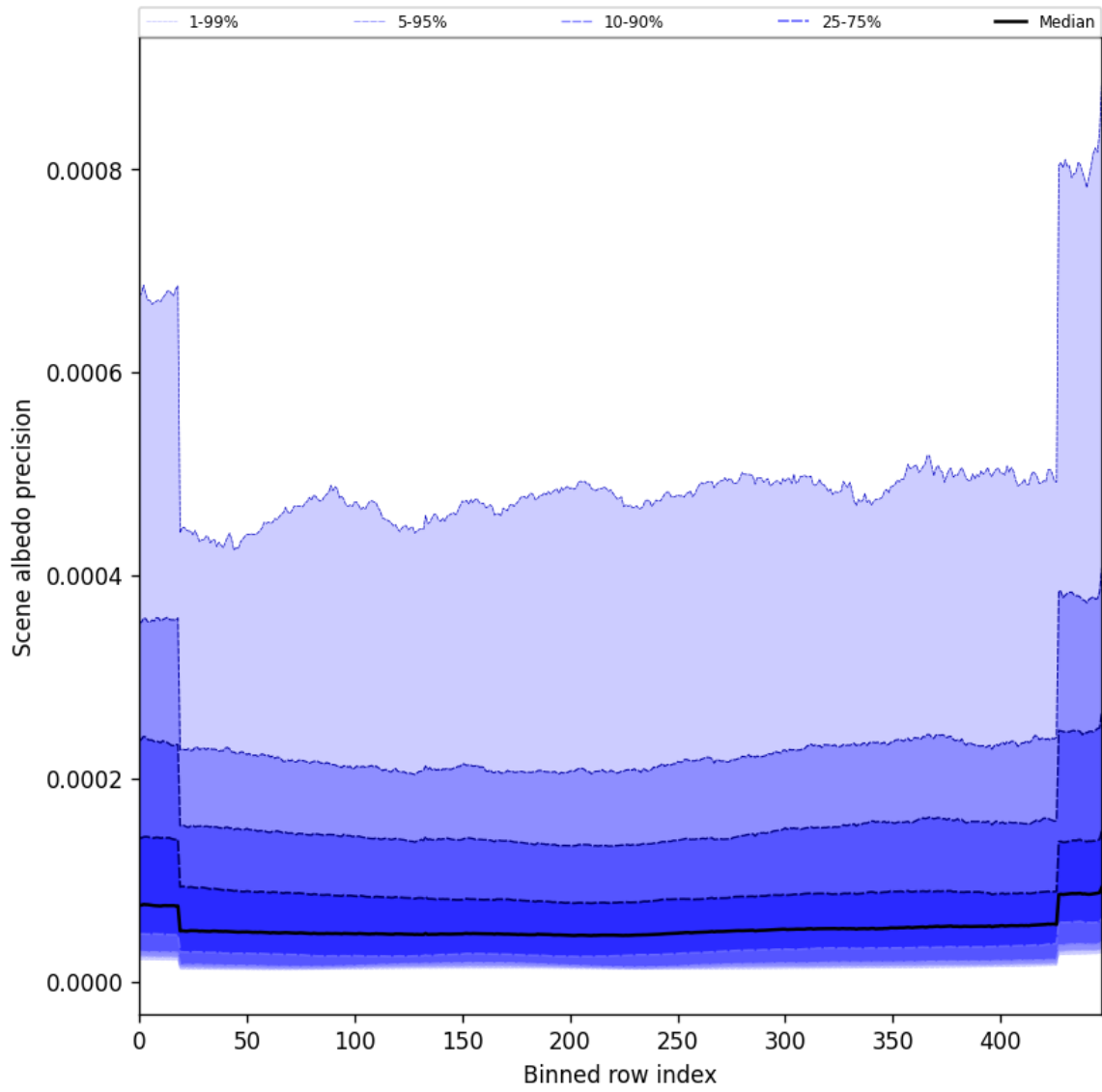
Figure 52: Along track statistics of “Scene albedo precision” for 2025-02-15 to 2025-02-17
