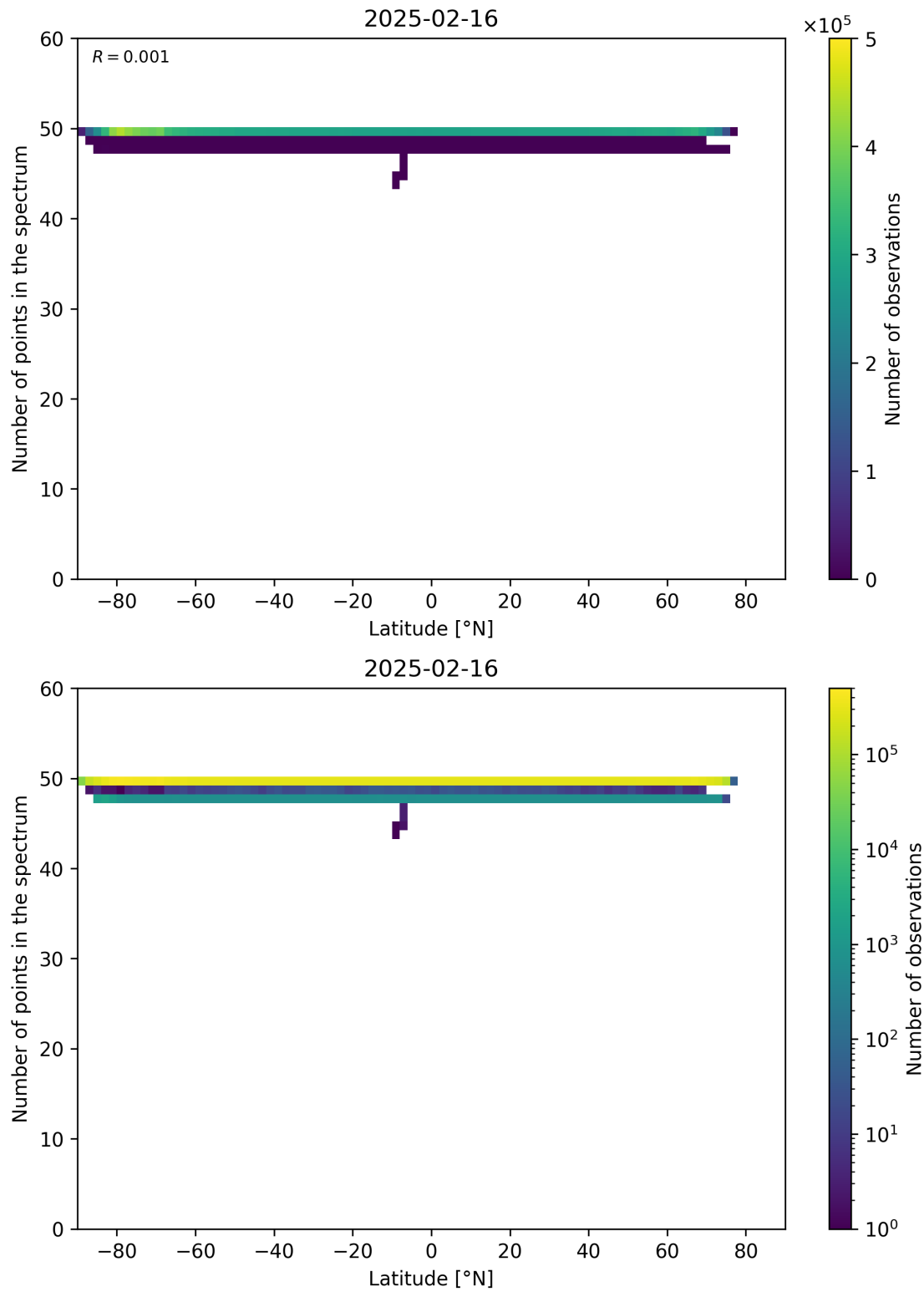
Figure 94: Scatter density plot of “Latitude” against “Number of points in the spectrum” for 2025-02-15 to 2025-02-17.
