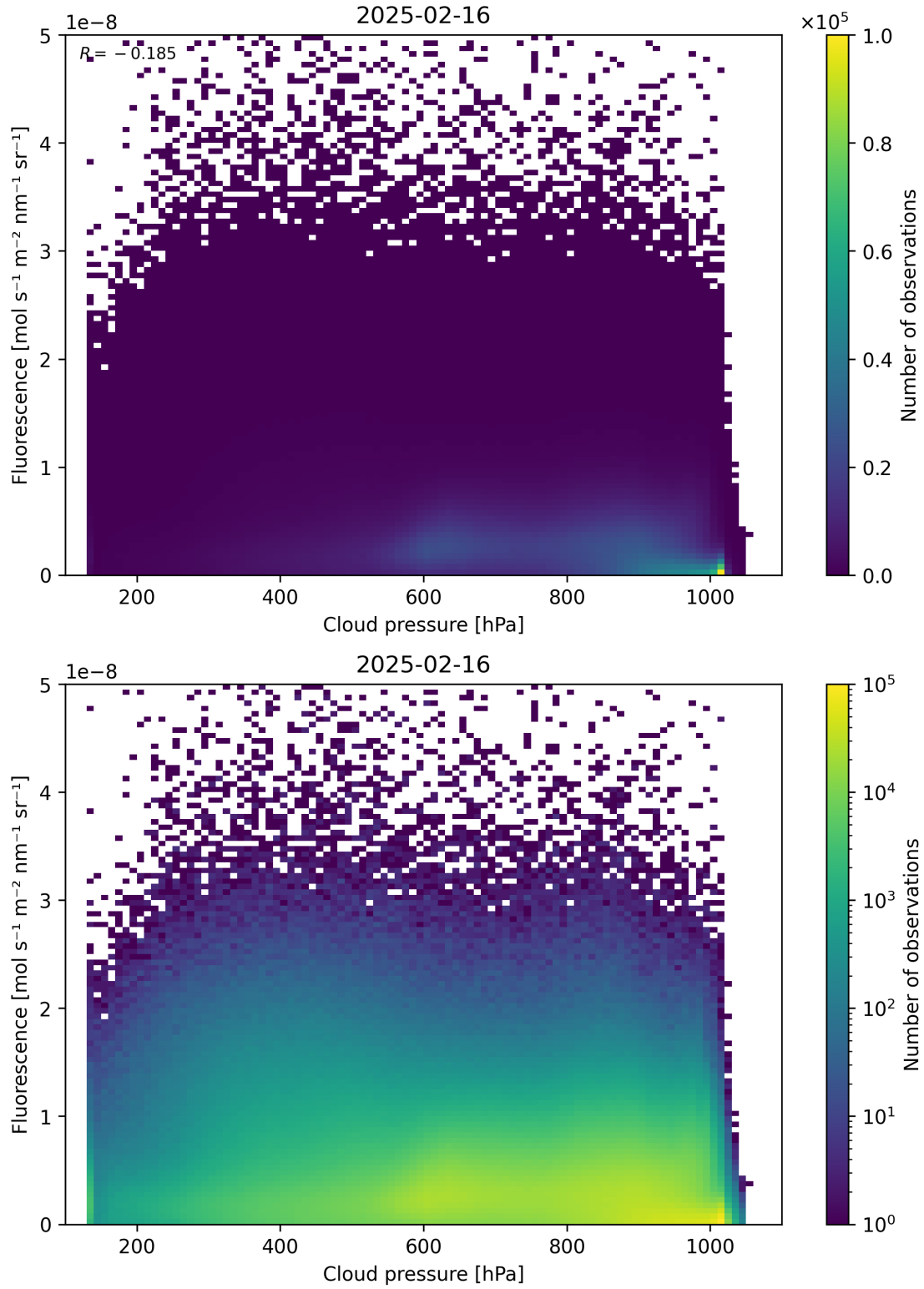
Figure 80: Scatter density plot of “Cloud pressure” against “Fluorescence” for 2025-02-15 to 2025-02-17.
