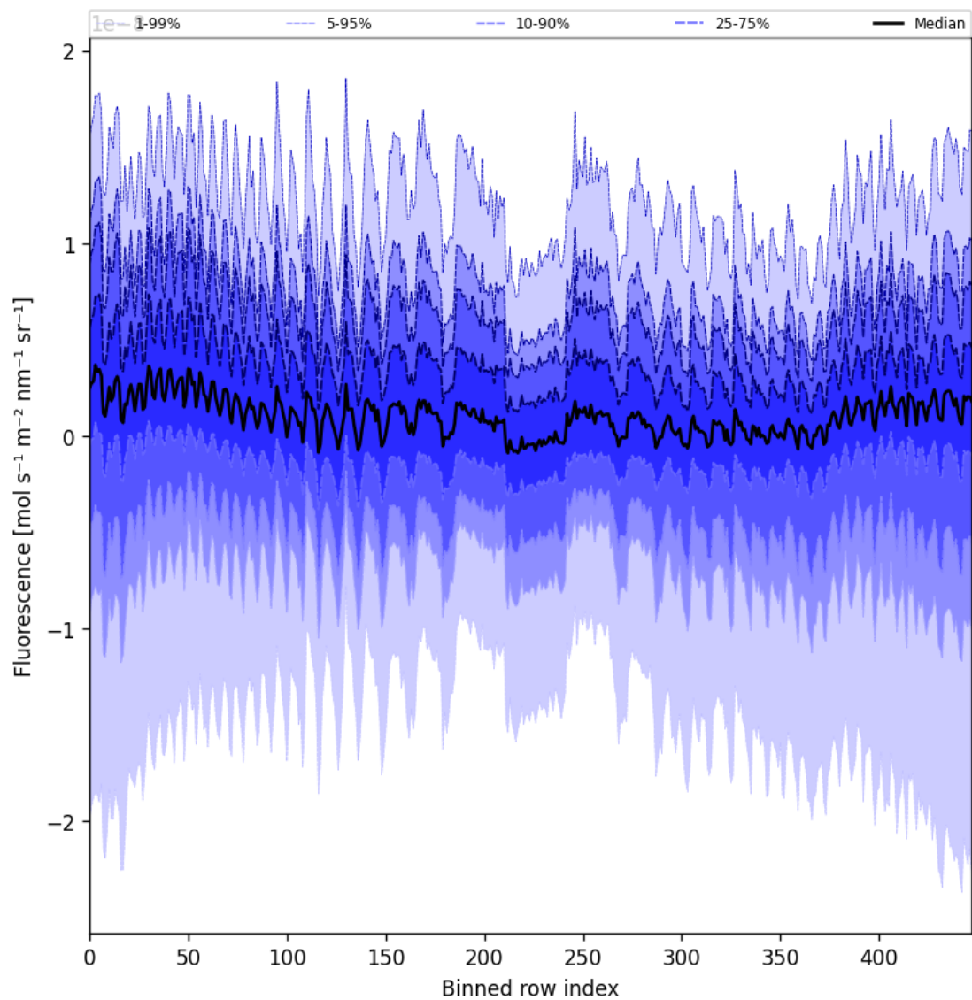
Figure 57: Along track statistics of “Fluorescence” for 2025-02-15 to 2025-02-17
