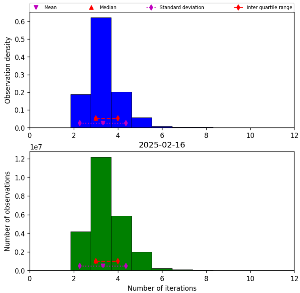
Figure 39: Histogram of “Number of iterations” for 2025-02-15 to 2025-02-17
