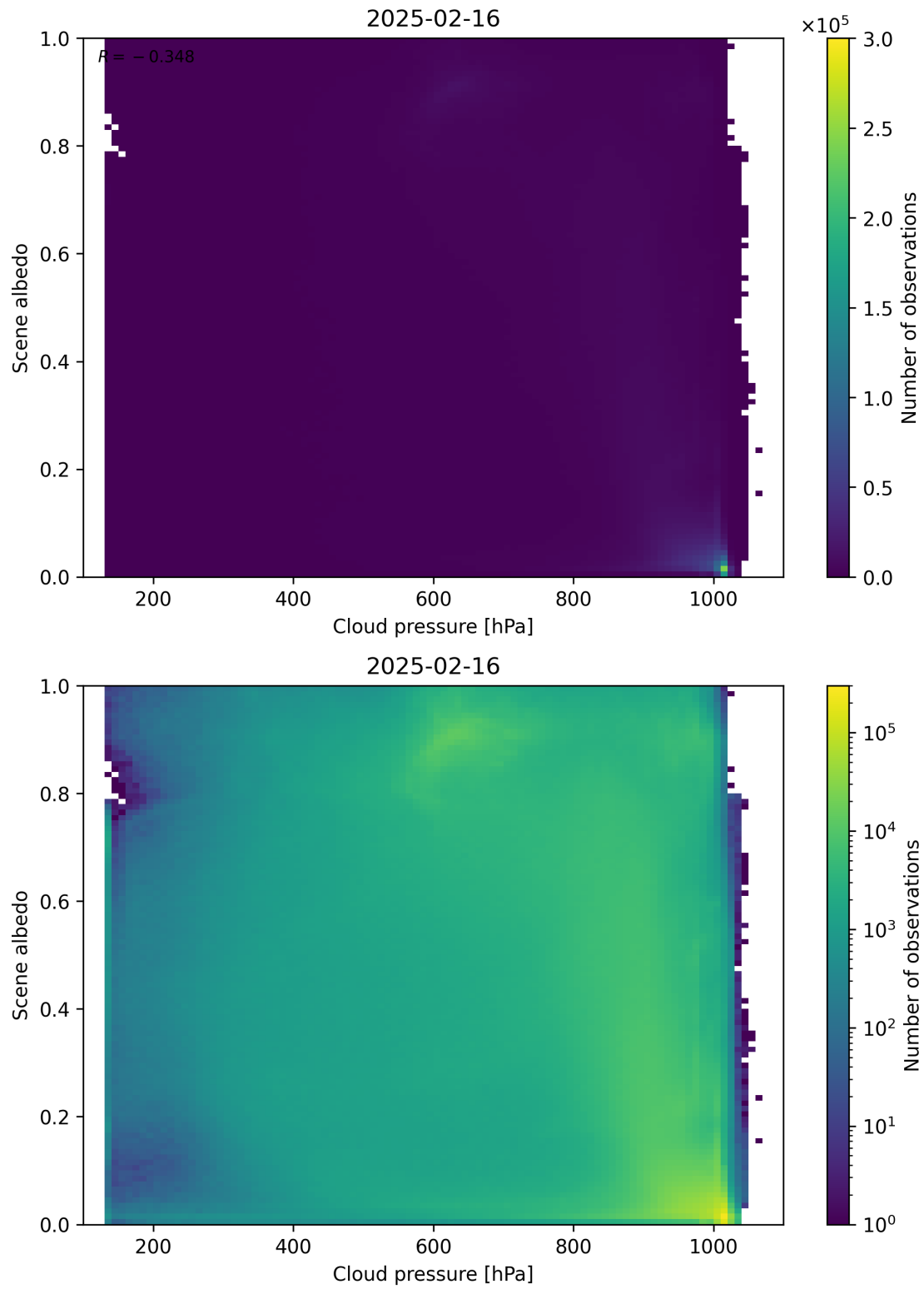
Figure 83: Scatter density plot of “Cloud pressure” against “Scene albedo” for 2025-02-15 to 2025-02-17.
