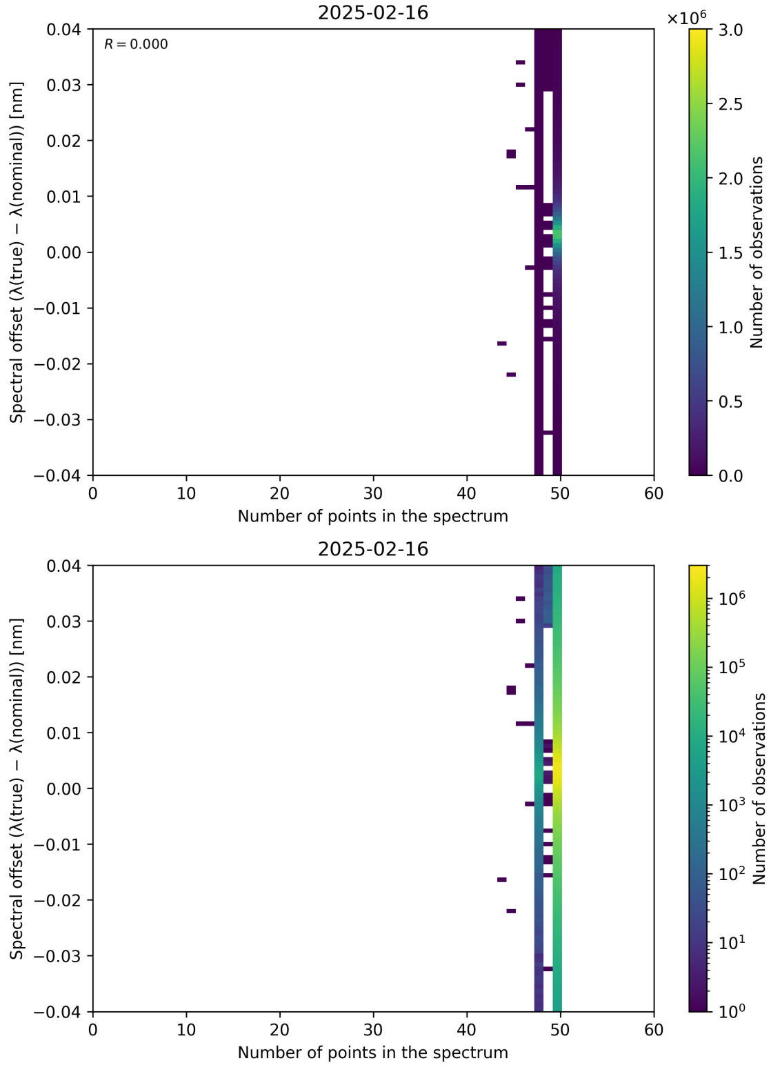
Figure 101: Scatter density plot of “Number of points in the spectrum” against “Spectral offset ( \lambda_{\text{true}} - \lambda_{\text{nominal}} )” for 2025-02-15 to 2025-02-17.
