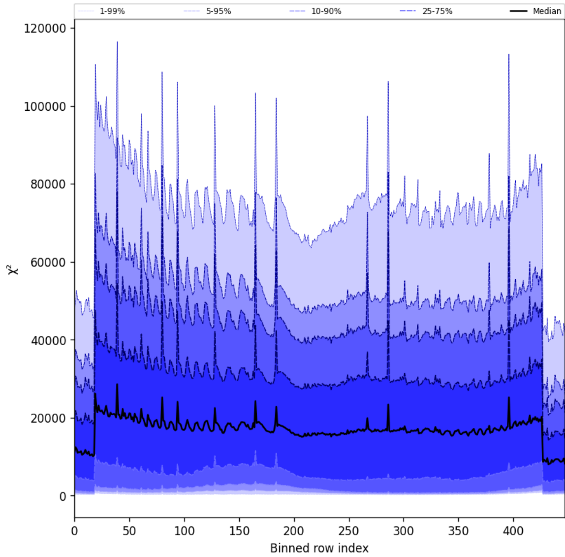
Figure 55: Along track statistics of “ \chi^2 ” for 2025-02-15 to 2025-02-17
