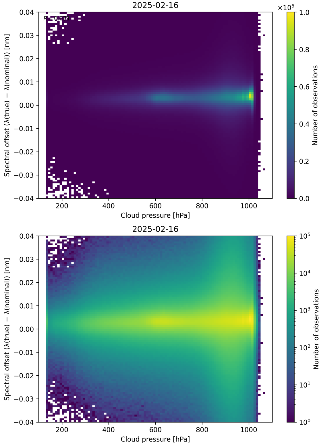
Figure 84: Scatter density plot of “Cloud pressure” against “Spectral offset ( \lambda_{\text{true}} - \lambda_{\text{nominal}} )” for 2025-02-15 to 2025-02-17.
