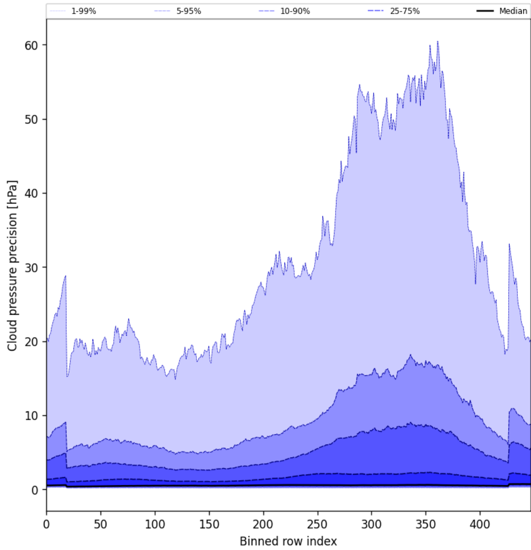
Figure 48: Along track statistics of “Cloud pressure precision” for 2025-02-15 to 2025-02-17
