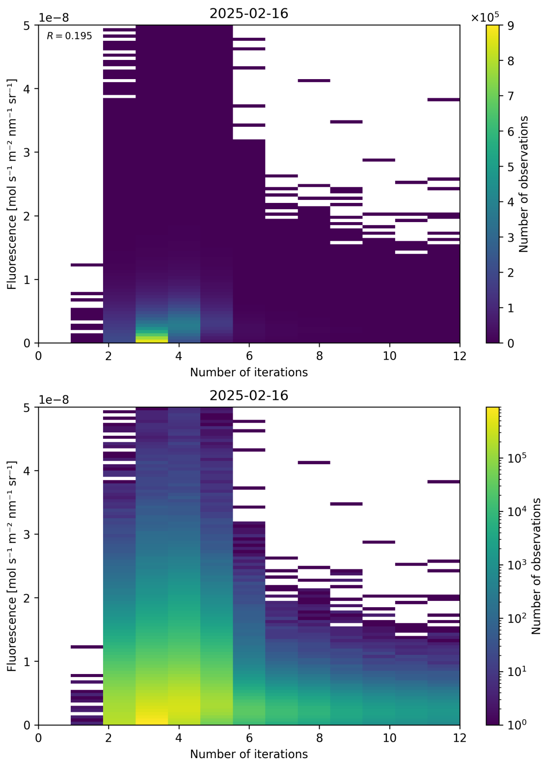
Figure 98: Scatter density plot of “Number of iterations” against “Fluorescence” for 2025-02-15 to 2025-02-17.
