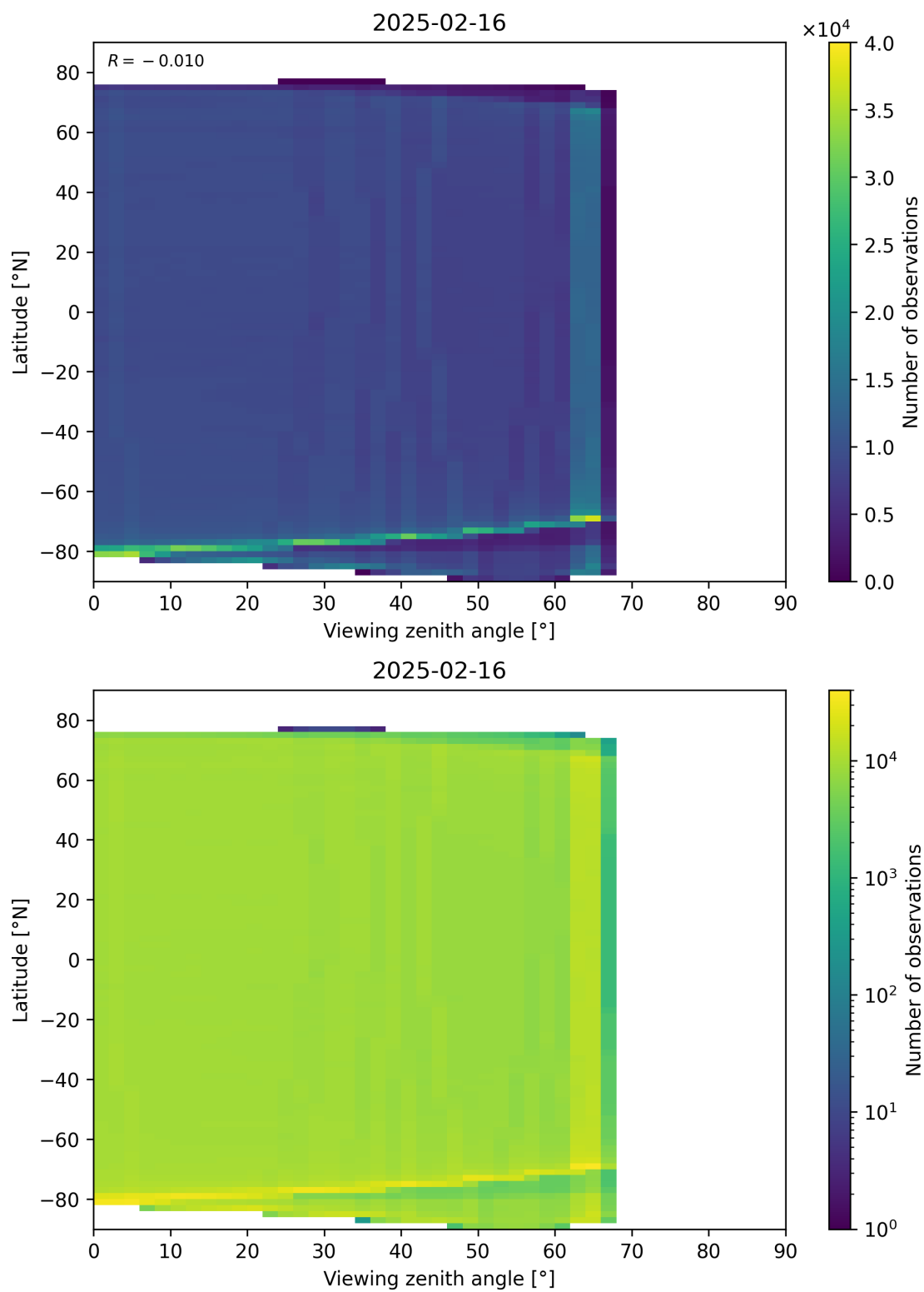
Figure 123: Scatter density plot of “Viewing zenith angle” against “Latitude” for 2025-02-15 to 2025-02-17.
