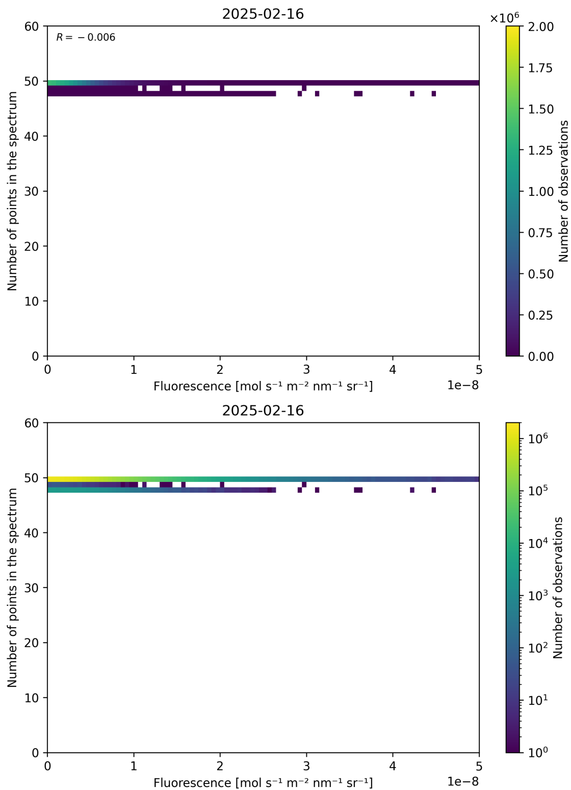
Figure 86: Scatter density plot of “Fluorescence” against “Number of points in the spectrum” for 2025-02-15 to 2025-02-17.
