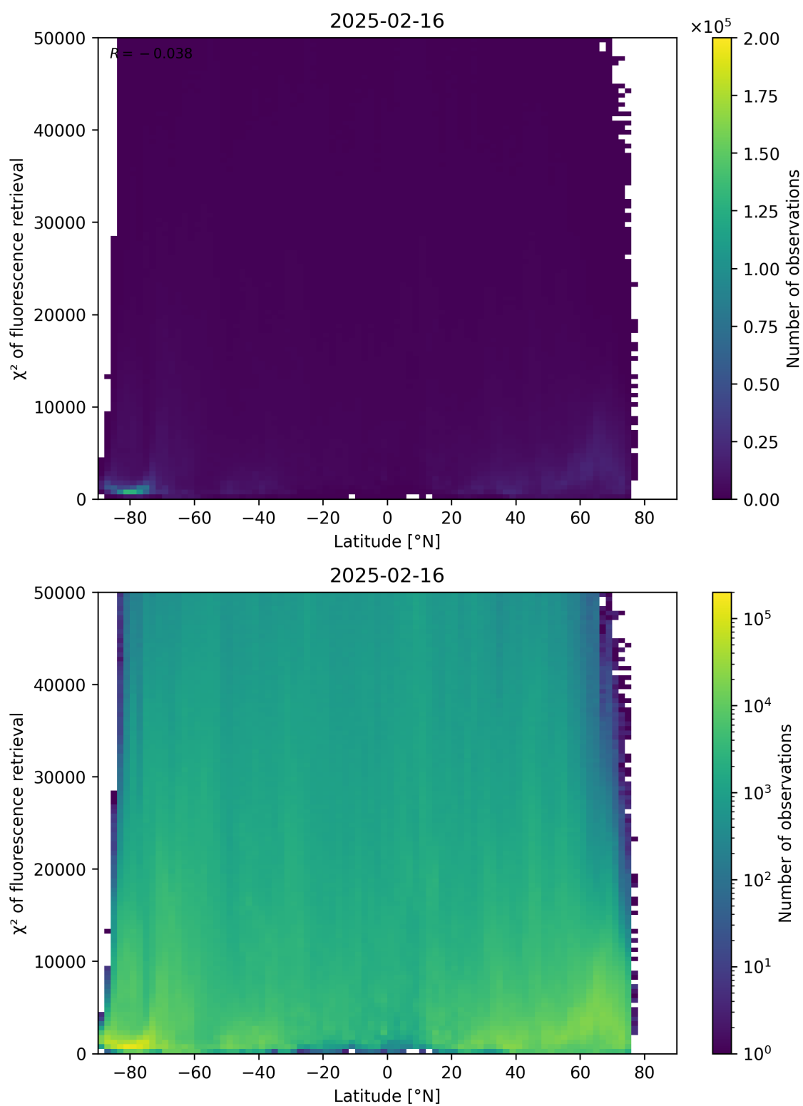
Figure 89: Scatter density plot of “Latitude” against “ \chi^2 of fluorescence retrieval” for 2025-02-15 to 2025-02-17.
