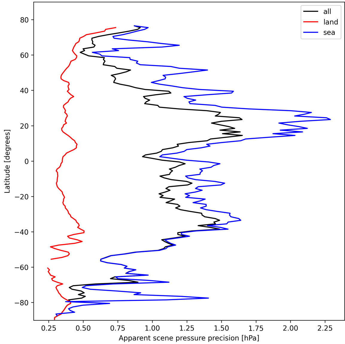
Figure 20: Zonal average of “Apparent scene pressure precision” for 2025-02-15 to 2025-02-17.
