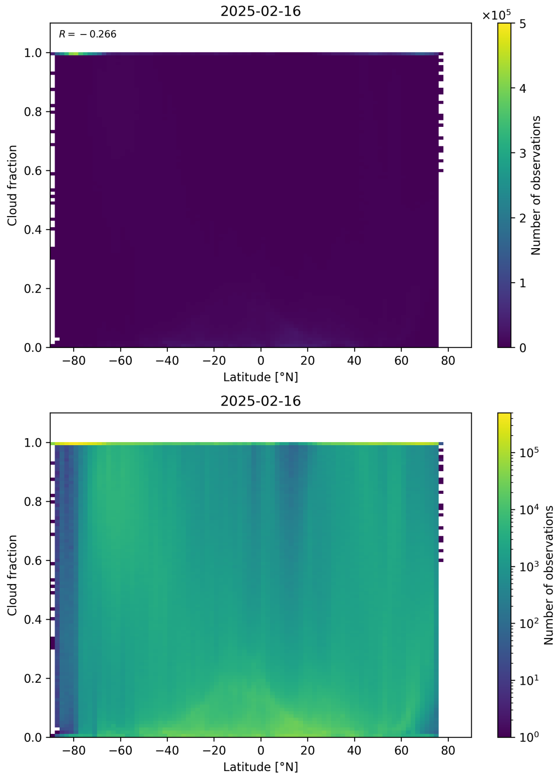
Figure 90: Scatter density plot of “Latitude” against “Cloud fraction” for 2025-02-15 to 2025-02-17.
