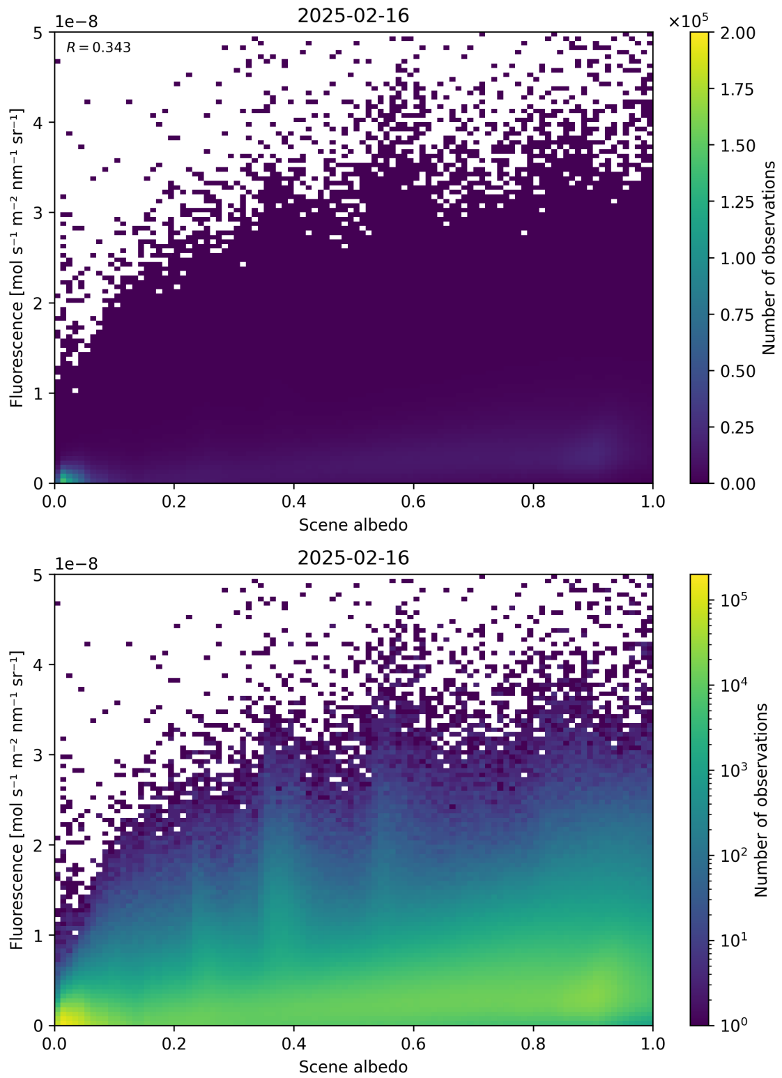
Figure 104: Scatter density plot of “Scene albedo” against “Fluorescence” for 2025-02-15 to 2025-02-17.
