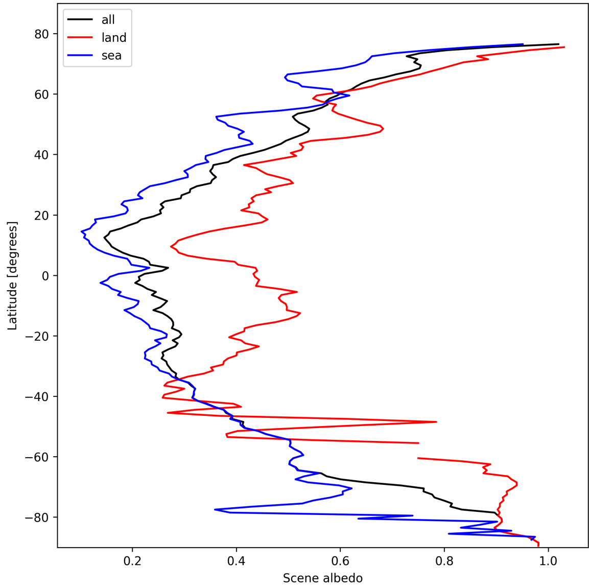
Figure 17: Zonal average of “Scene albedo” for 2025-02-15 to 2025-02-17.
