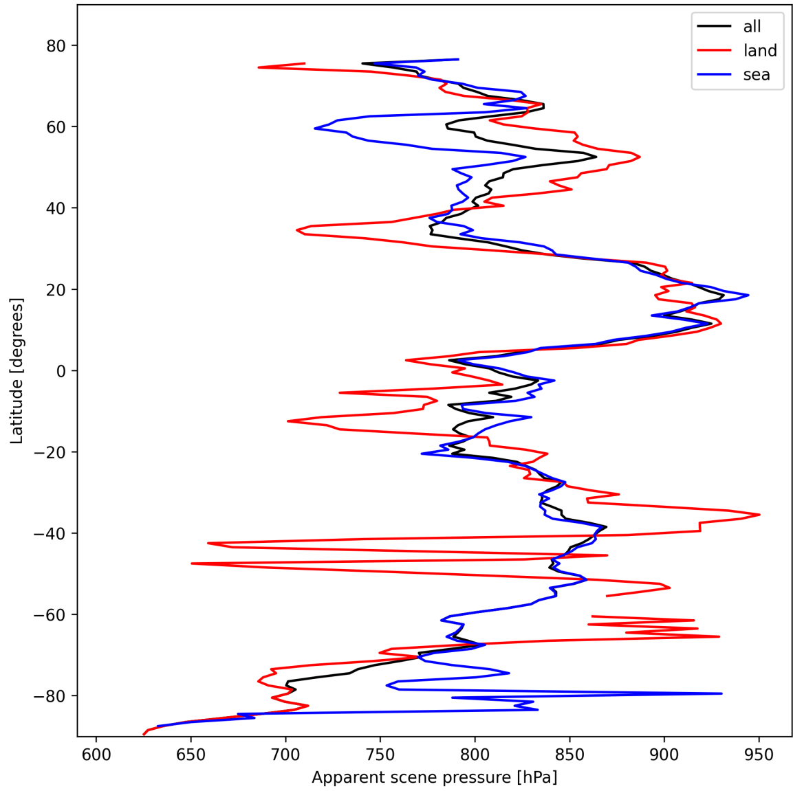
Figure 19: Zonal average of “Apparent scene pressure” for 2025-02-15 to 2025-02-17.
