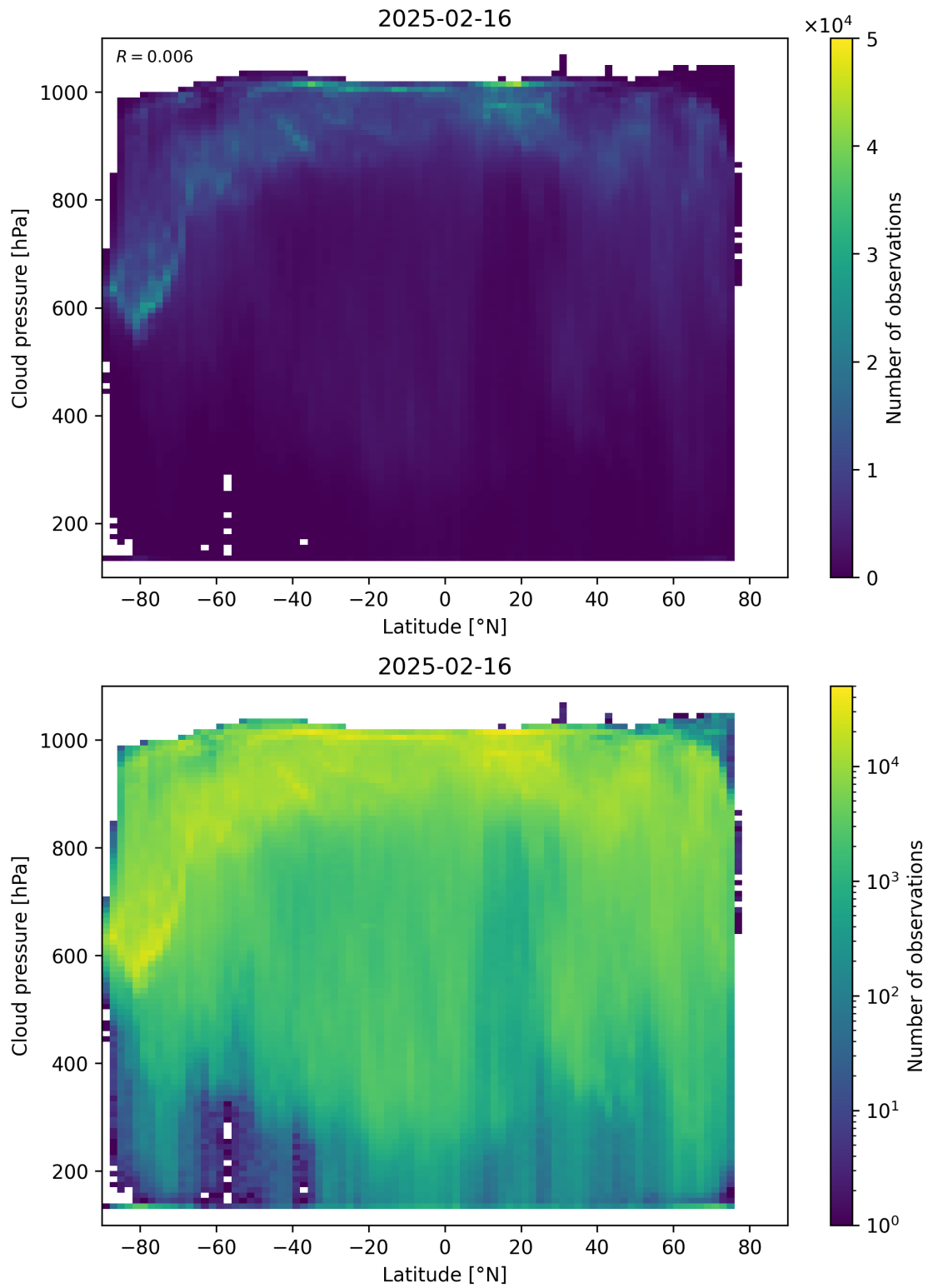
Figure 91: Scatter density plot of “Latitude” against “Cloud pressure” for 2025-02-15 to 2025-02-17.
