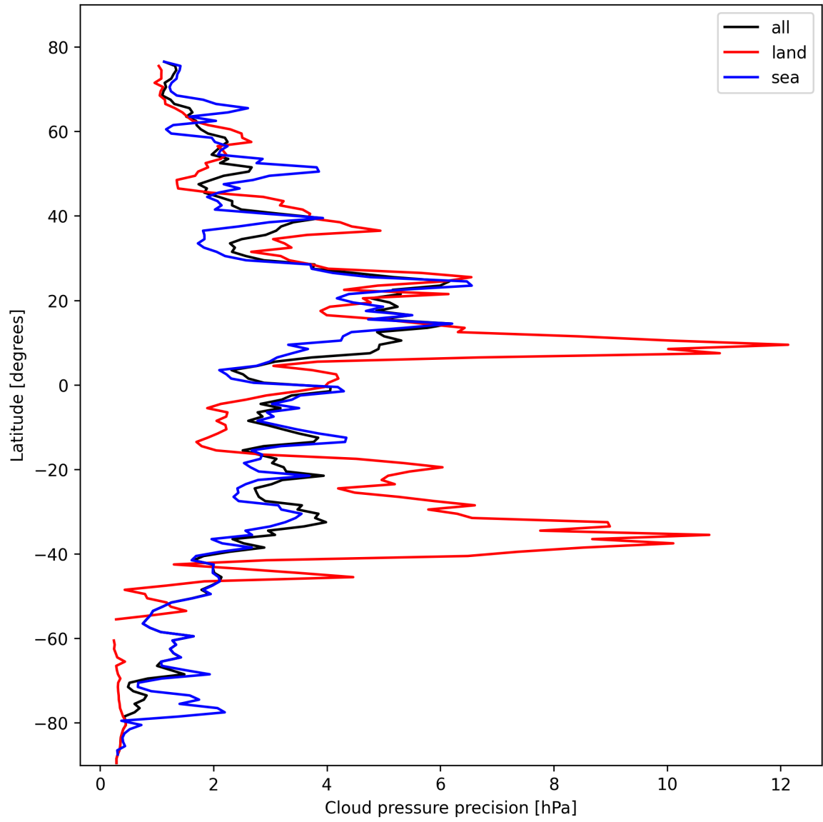
Figure 14: Zonal average of “Cloud pressure precision” for 2025-02-15 to 2025-02-17.
