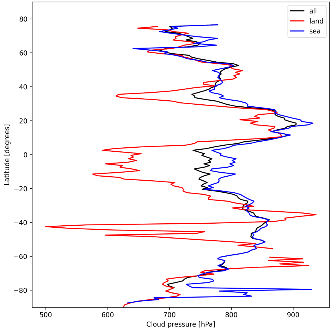
Figure 13: Zonal average of “Cloud pressure” for 2025-02-15 to 2025-02-17.
