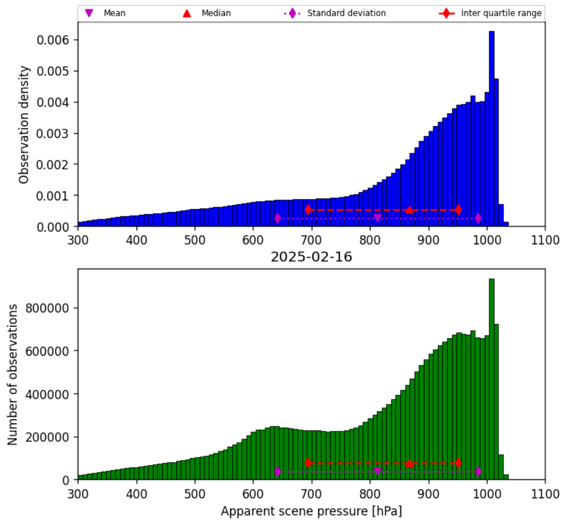
Figure 36: Histogram of “Apparent scene pressure” for 2025-02-15 to 2025-02-17
