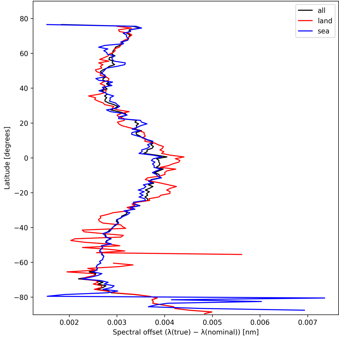
Figure 28: Zonal average of “Spectral offset ( \lambda_{\text{true}} - \lambda_{\text{nominal}} )” for 2025-02-15 to 2025-02-17.
