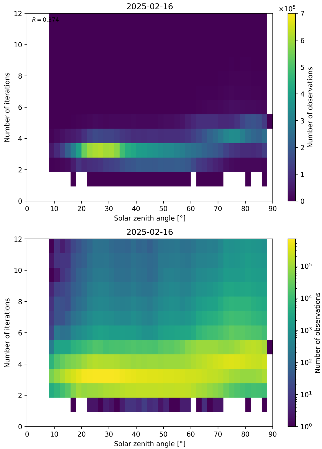
Figure 114: Scatter density plot of “Solar zenith angle” against “Number of iterations” for 2025-02-15 to 2025-02-17.
