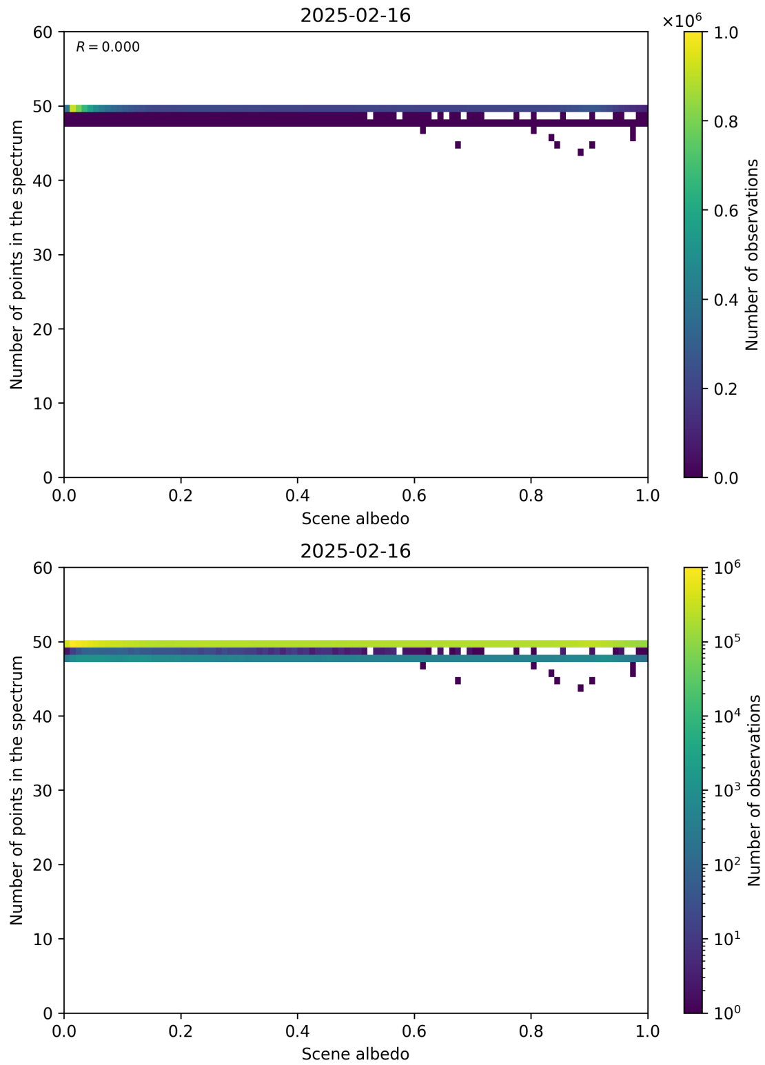
Figure 106: Scatter density plot of “Scene albedo” against “Number of points in the spectrum” for 2025-02-15 to 2025-02-17.
