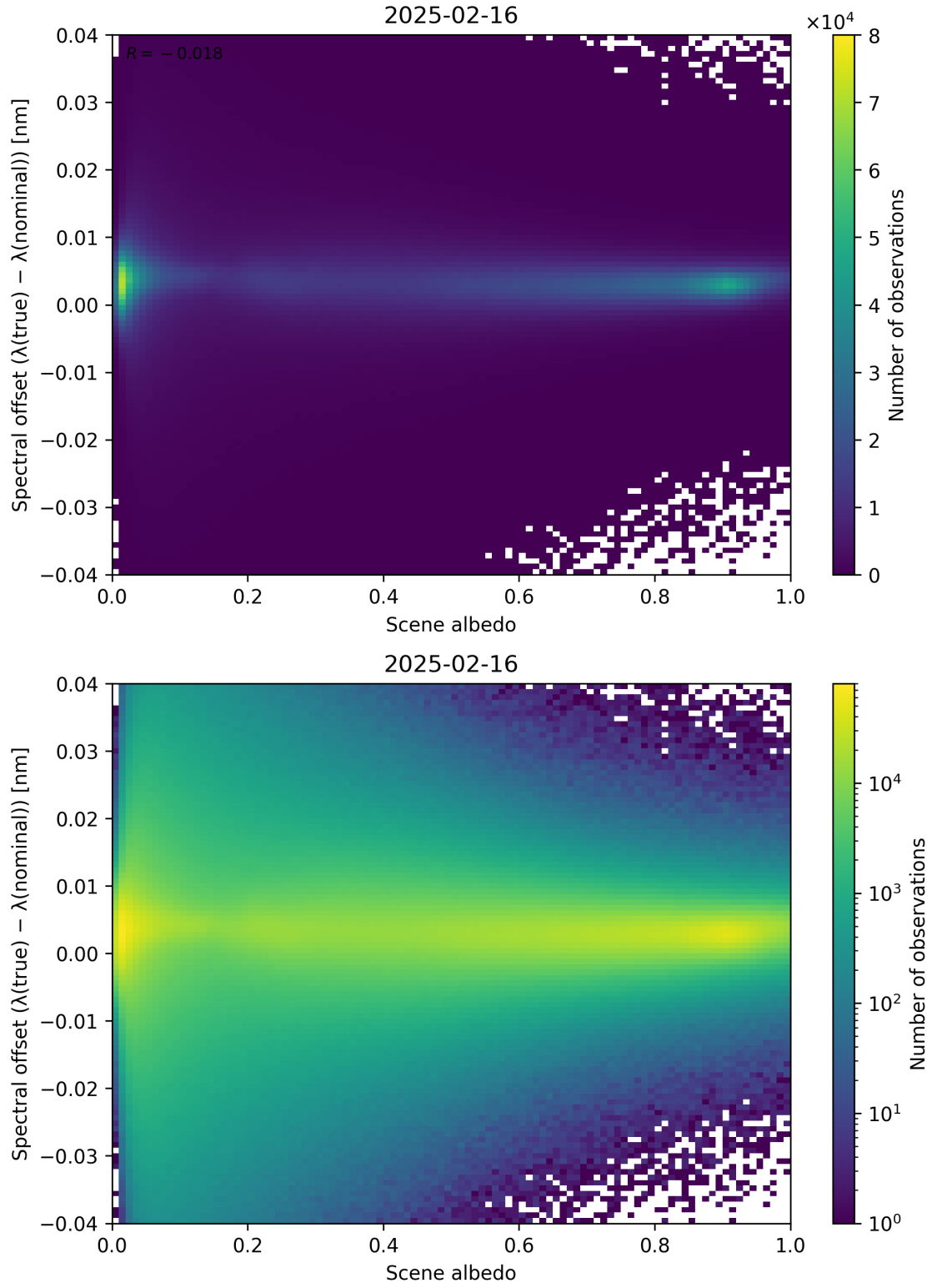
Figure 107: Scatter density plot of “Scene albedo” against “Spectral offset ( \lambda_{\text{true}} - \lambda_{\text{nominal}} )” for 2025-02-15 to 2025-02-17.
