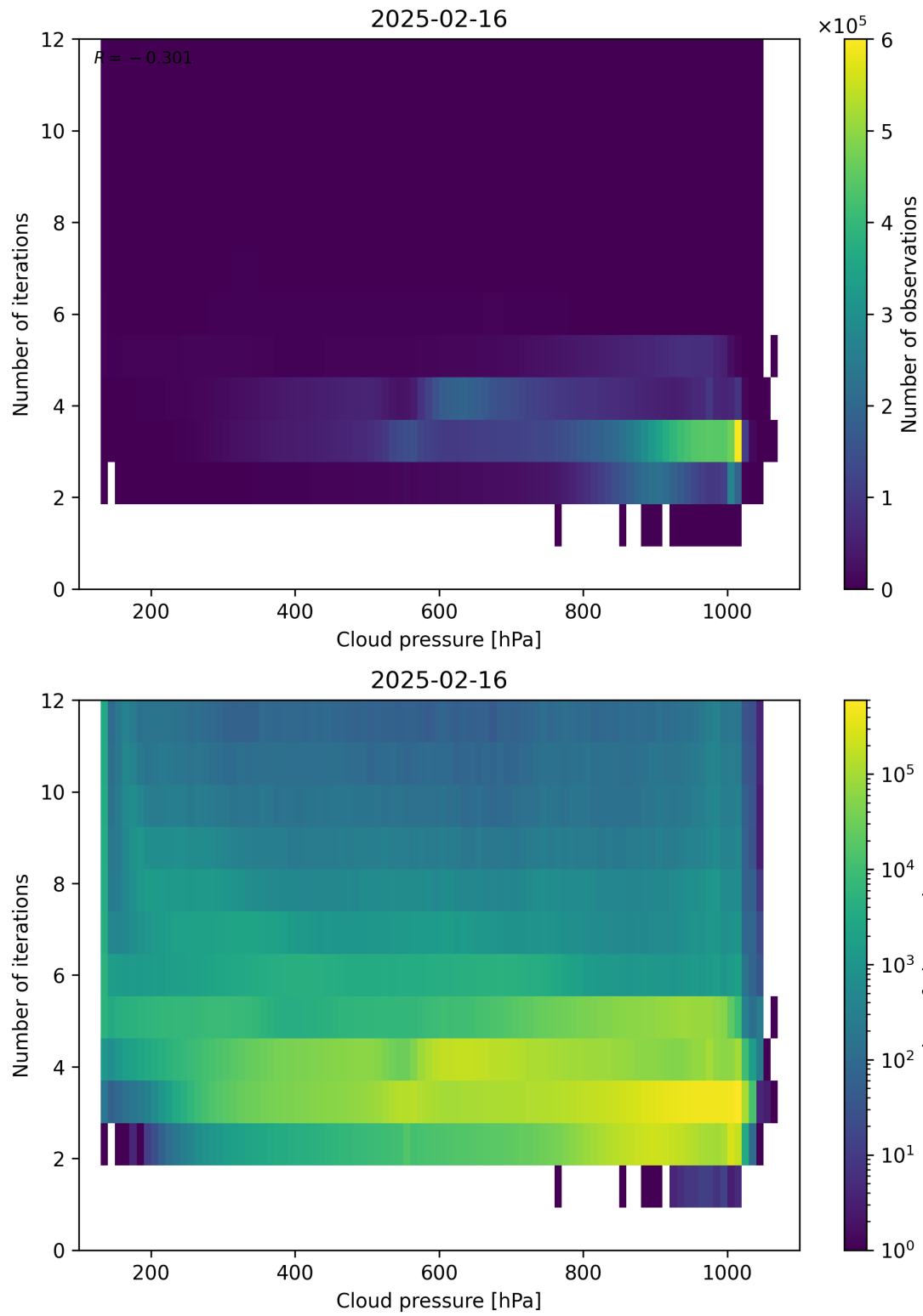
Figure 81: Scatter density plot of “Cloud pressure” against “Number of iterations” for 2025-02-15 to 2025-02-17.
