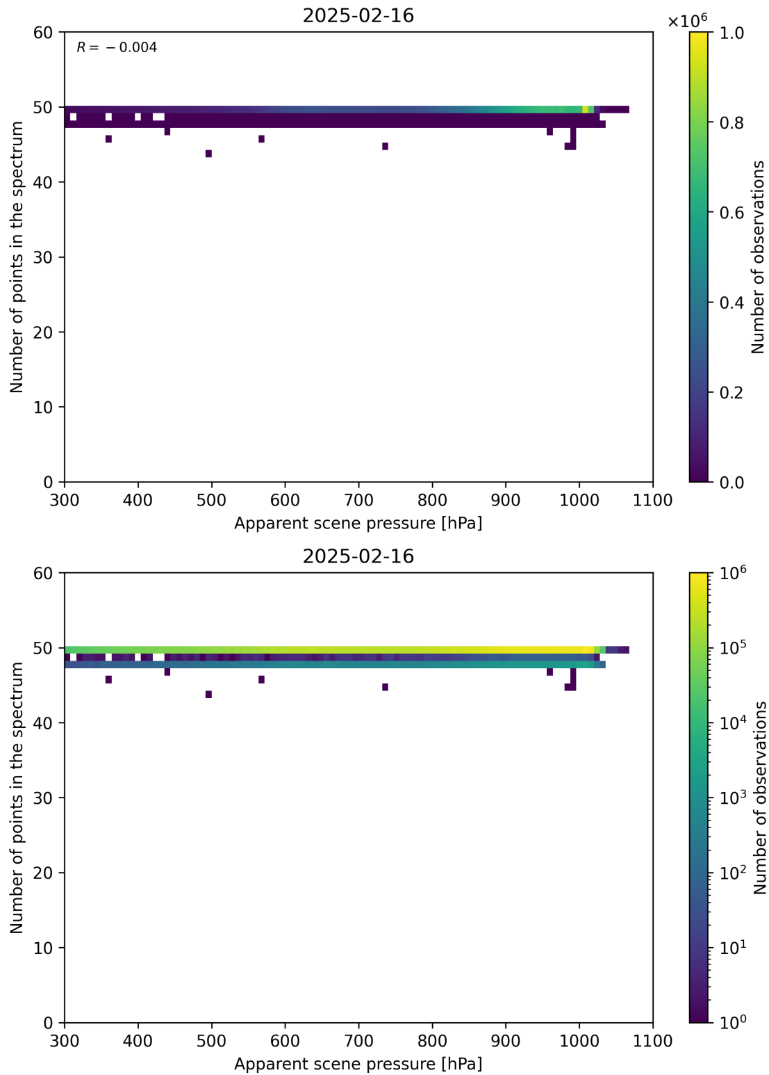
Figure 66: Scatter density plot of “Apparent scene pressure” against “Number of points in the spectrum” for 2025-02-15 to 2025-02-17.
