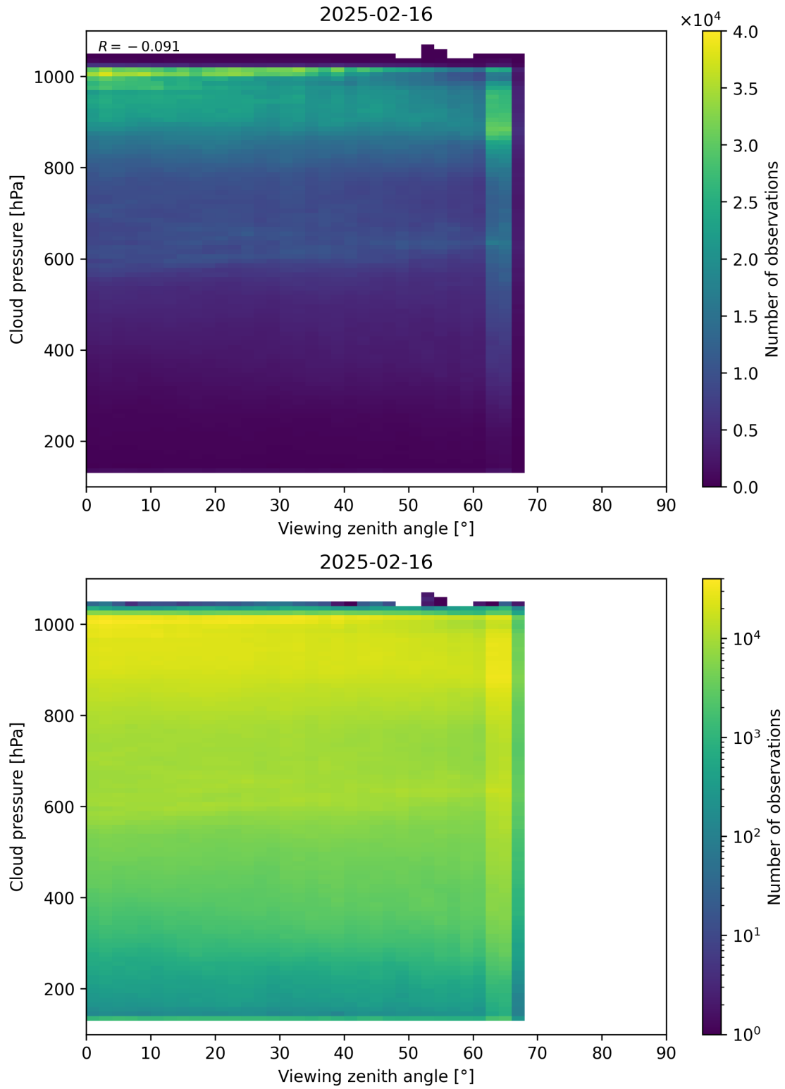
Figure 121: Scatter density plot of “Viewing zenith angle” against “Cloud pressure” for 2025-02-15 to 2025-02-17.
