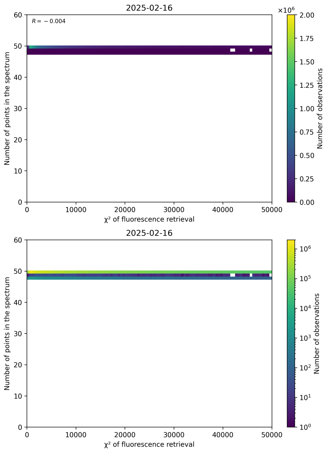
Figure 68: Scatter density plot of “ \chi^2 of fluorescence retrieval” against “Number of points in the spectrum” for 2025-02-15 to 2025-02-17.
