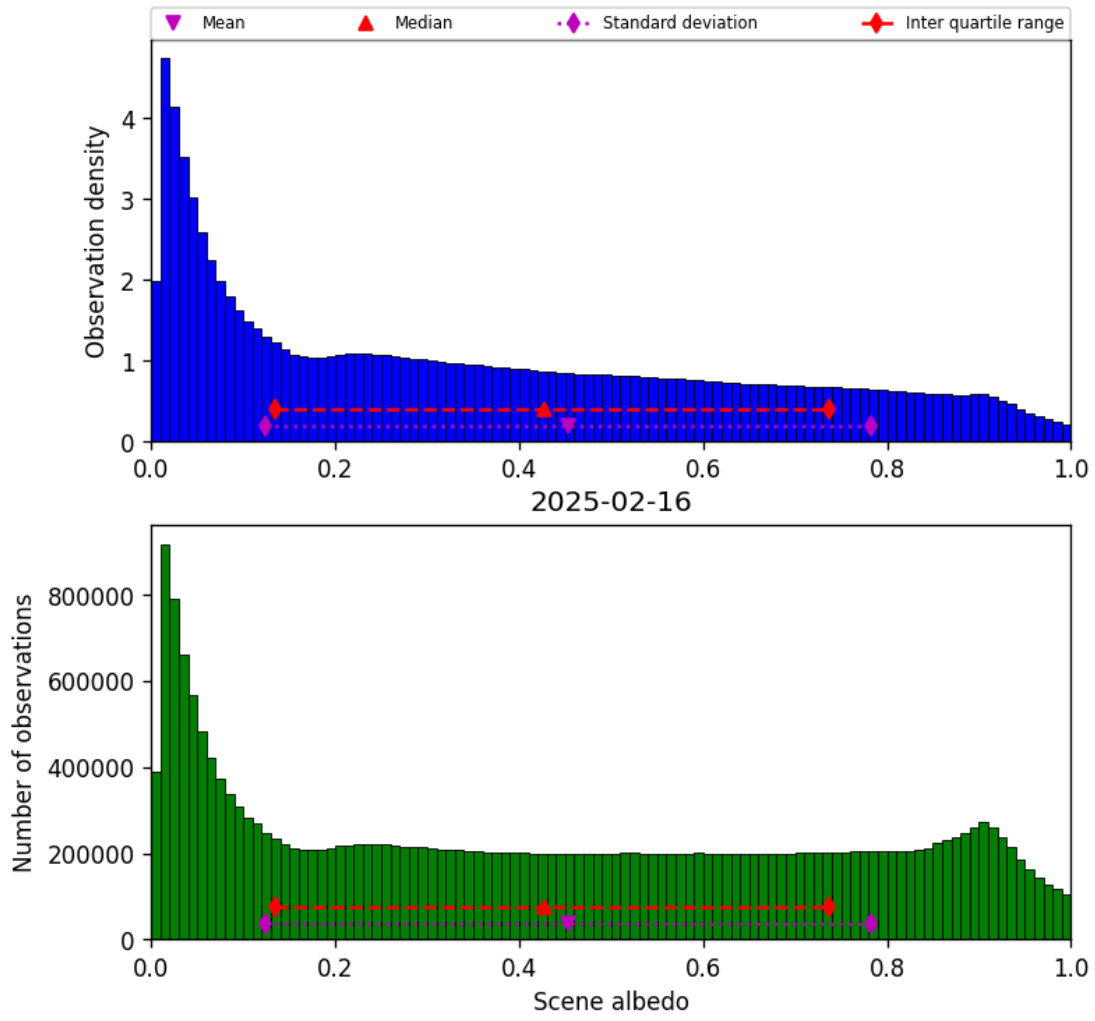
Figure 34: Histogram of “Scene albedo” for 2025-02-15 to 2025-02-17
