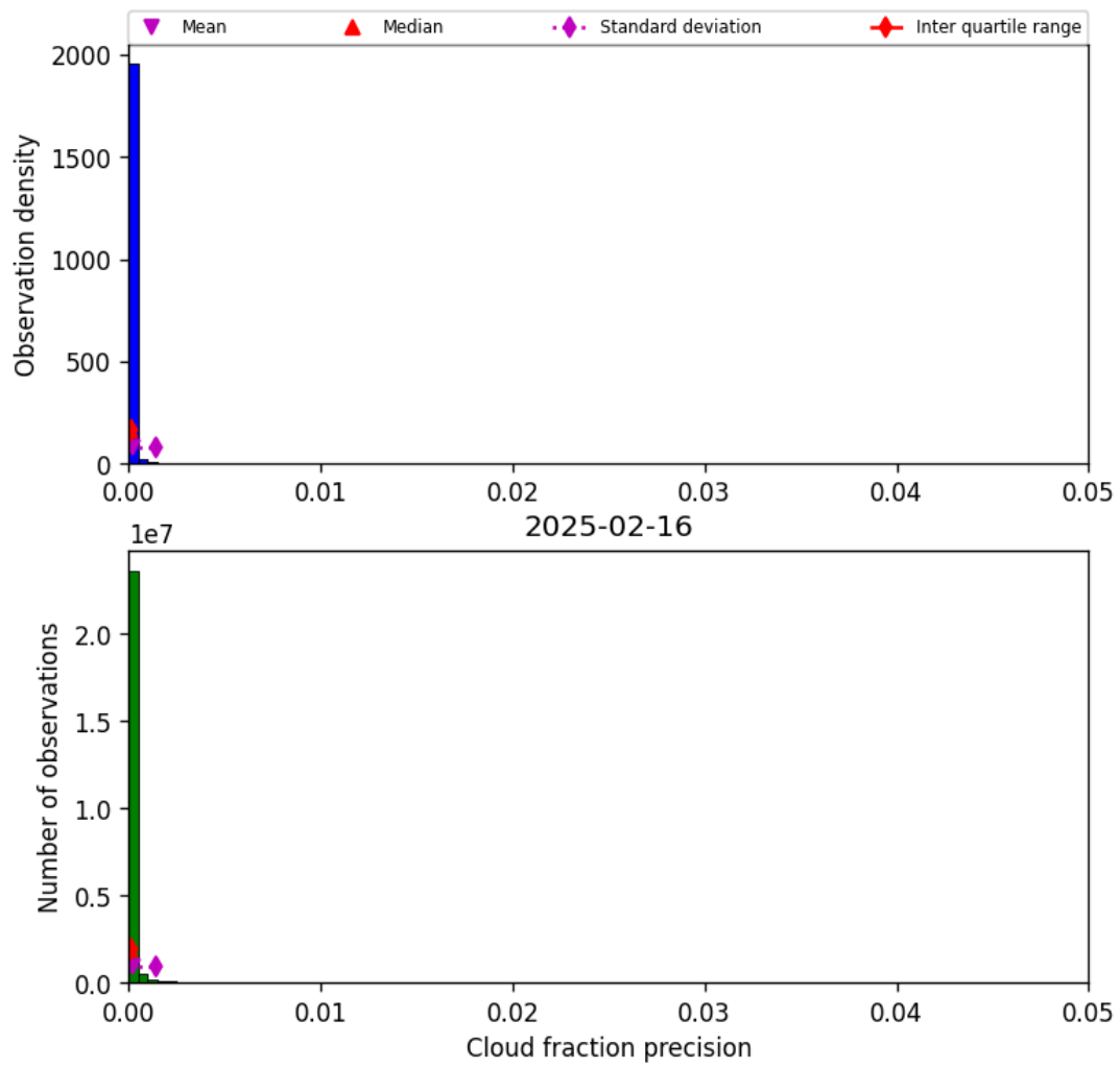
Figure 33: Histogram of “Cloud fraction precision” for 2025-02-15 to 2025-02-17
