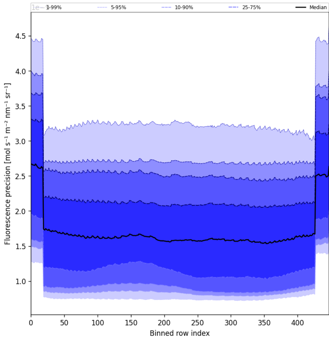
Figure 58: Along track statistics of “Fluorescence precision” for 2025-02-15 to 2025-02-17
