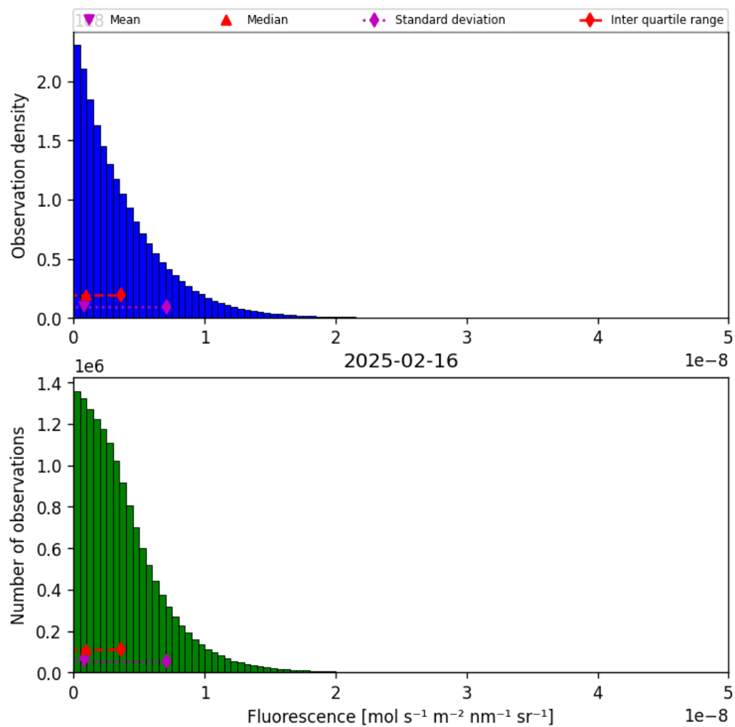
Figure 40: Histogram of “Fluorescence” for 2025-02-15 to 2025-02-17
