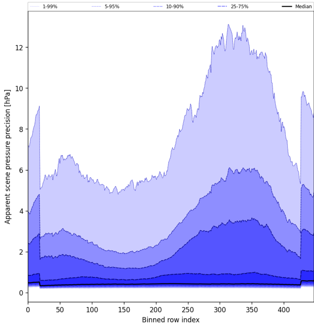
Figure 54: Along track statistics of “Apparent scene pressure precision” for 2025-02-15 to 2025-02-17
