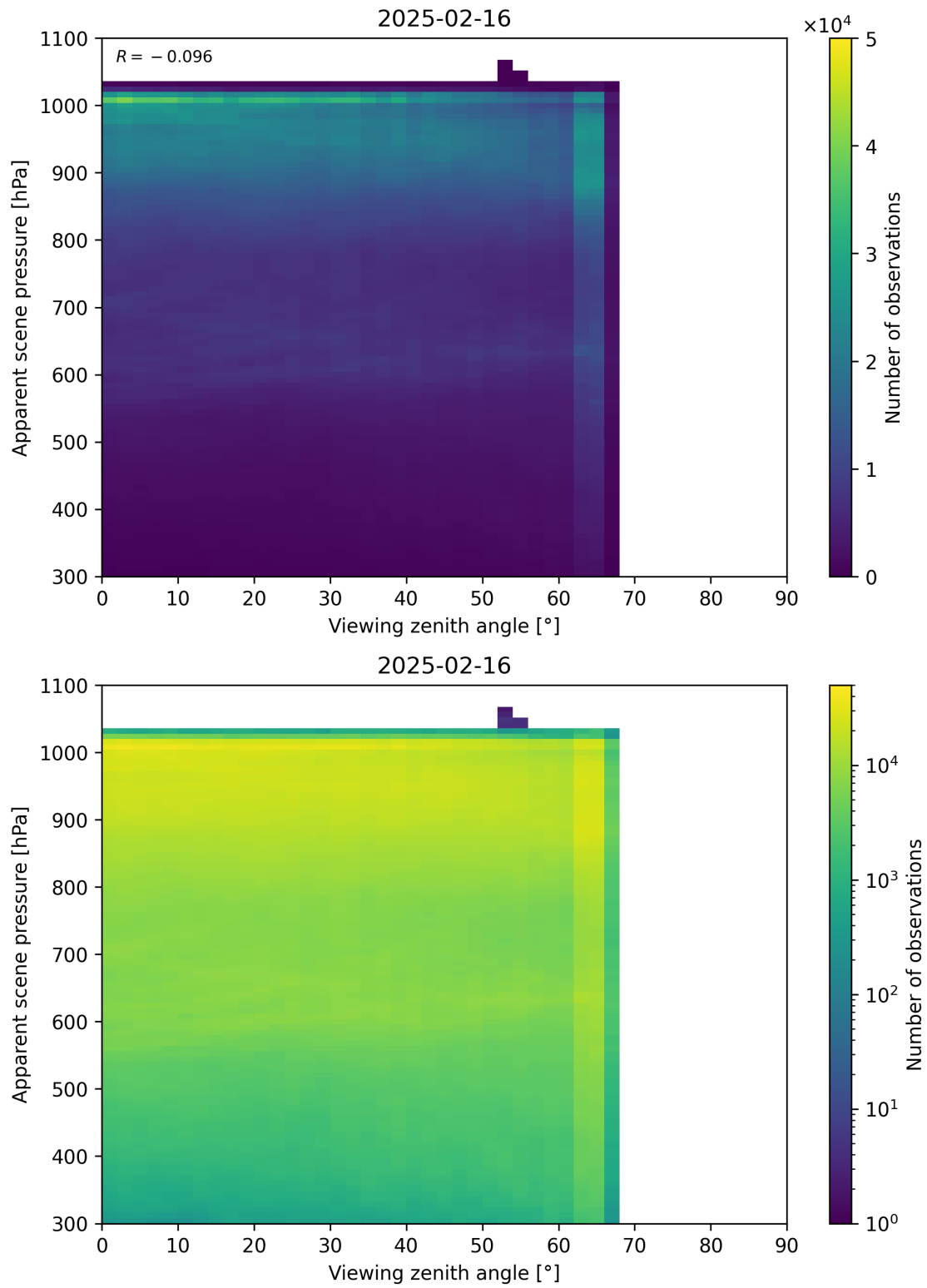
Figure 118: Scatter density plot of “Viewing zenith angle” against “Apparent scene pressure” for 2025-02-15 to 2025-02-17.
