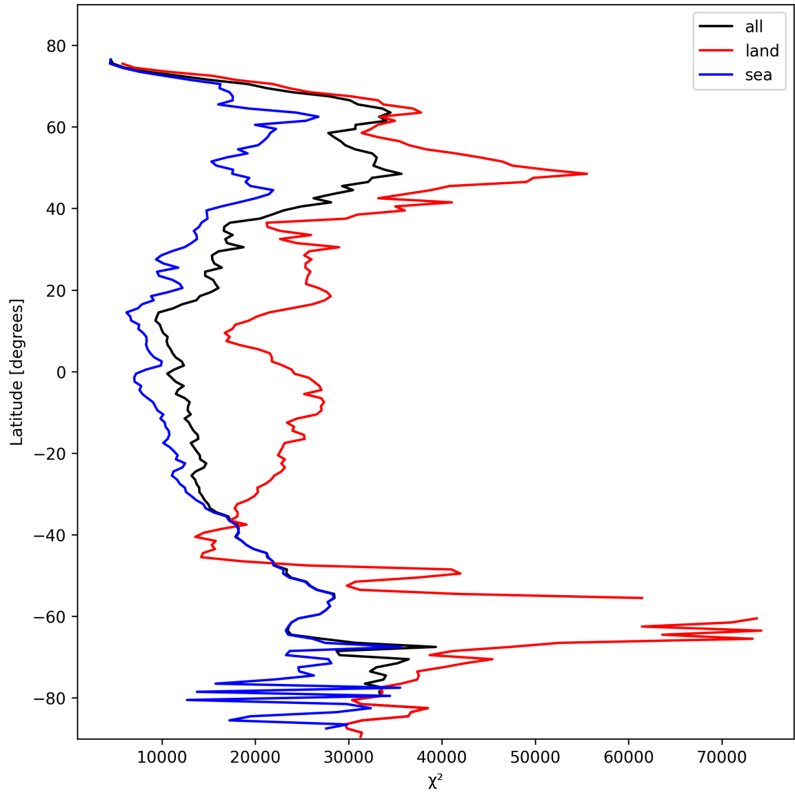
Figure 21: Zonal average of “ \chi^2 ” for 2025-02-15 to 2025-02-17.
