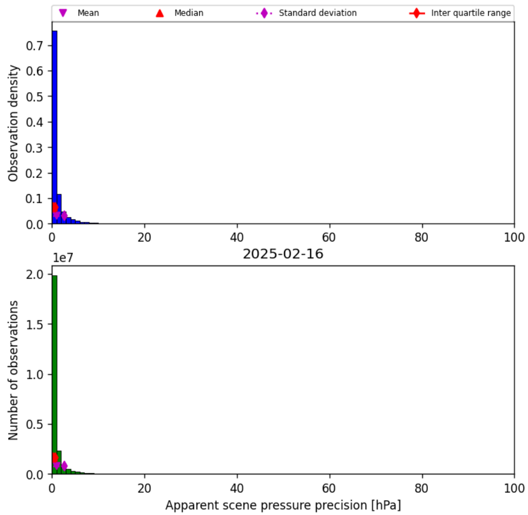
Figure 37: Histogram of “Apparent scene pressure precision” for 2025-02-15 to 2025-02-17
