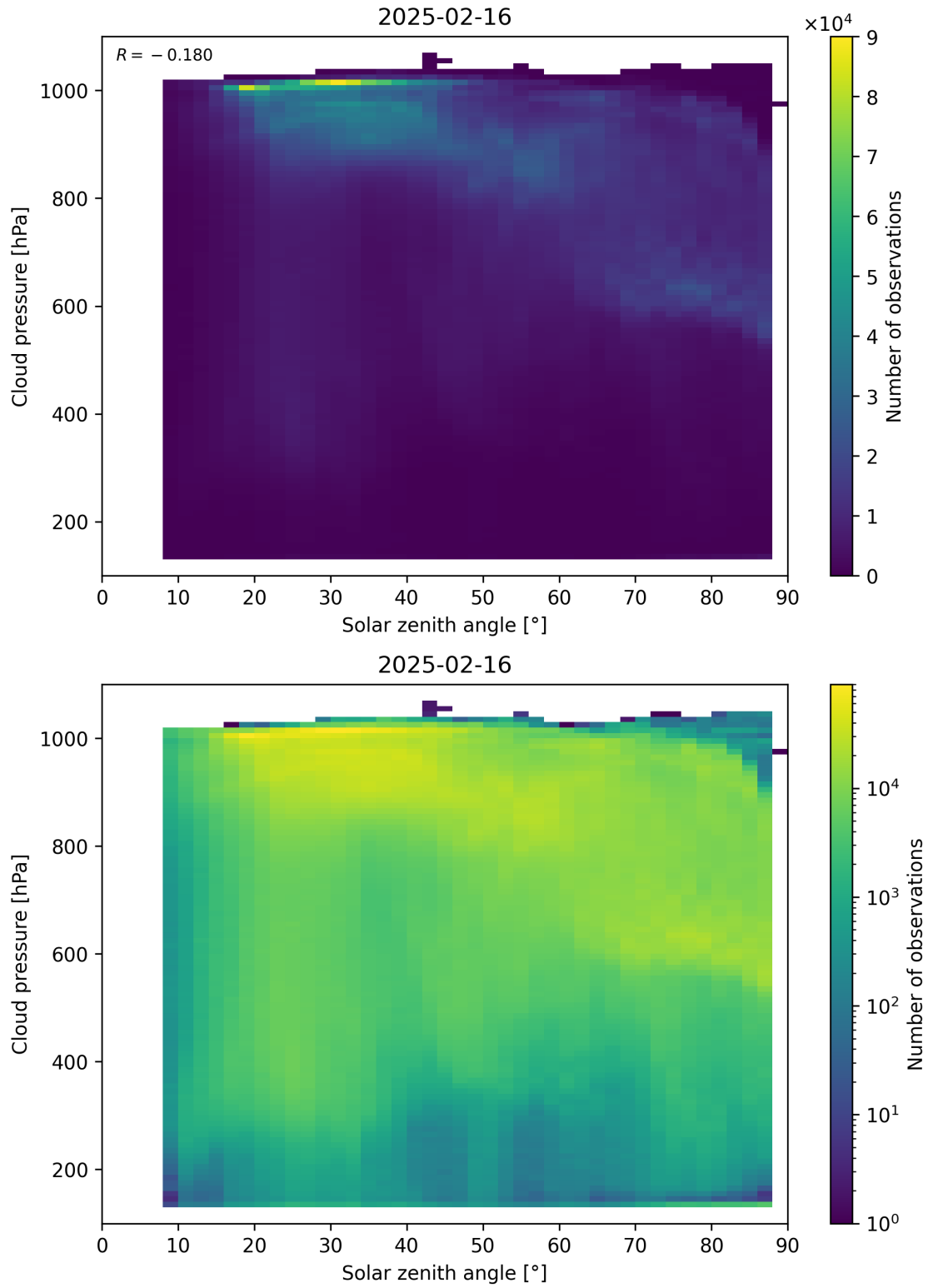
Figure 111: Scatter density plot of “Solar zenith angle” against “Cloud pressure” for 2025-02-15 to 2025-02-17.
