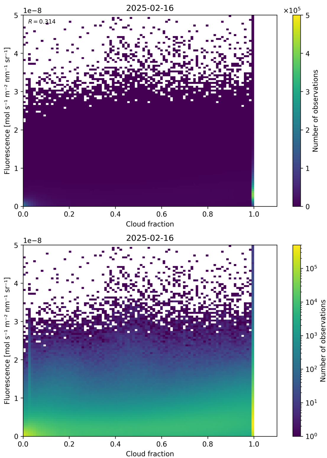
Figure 72: Scatter density plot of “Cloud fraction” against “Fluorescence” for 2025-02-15 to 2025-02-17.
