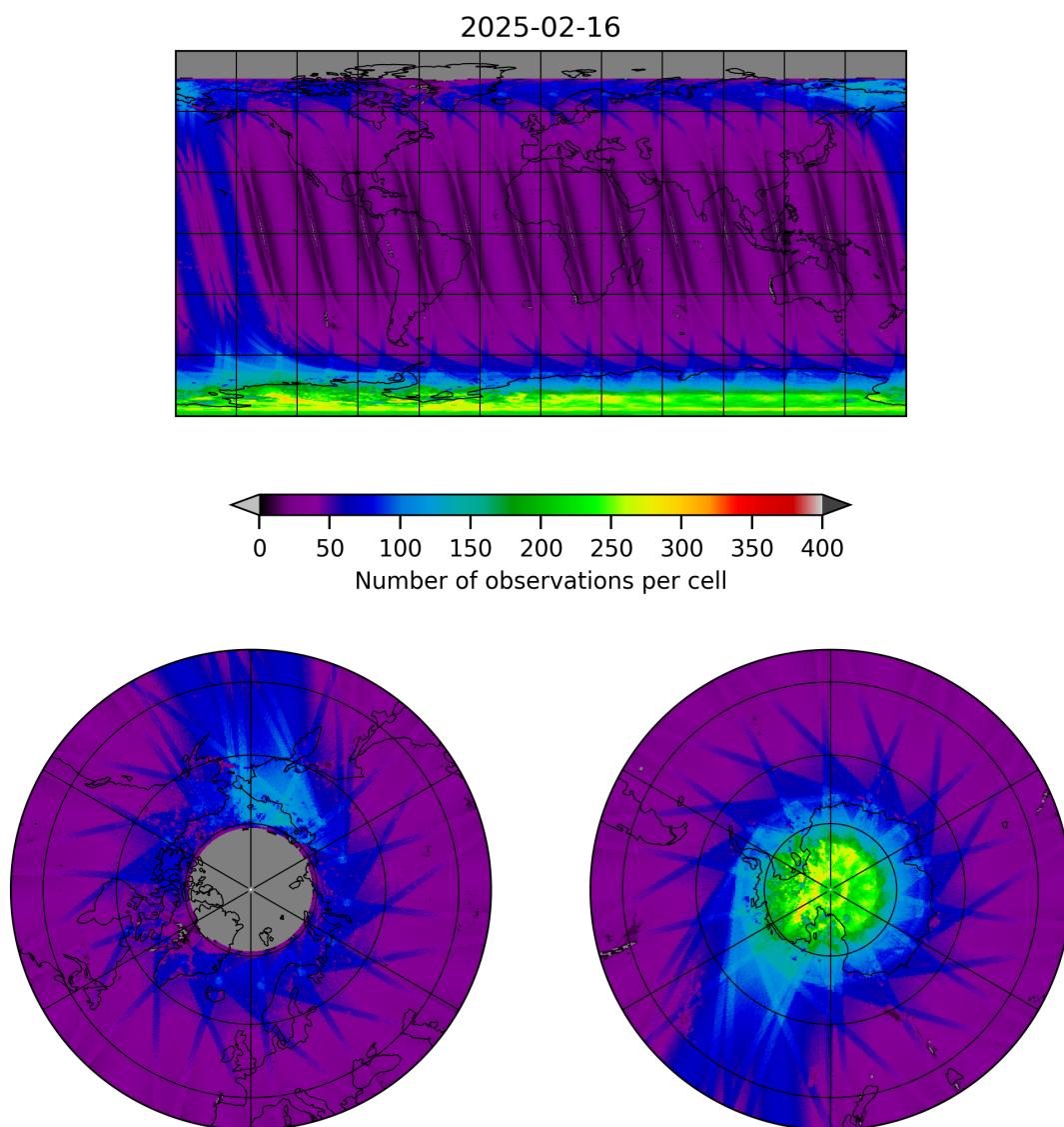
Figure 11: Map of the number of observations for 2025-02-15 to 2025-02-17
