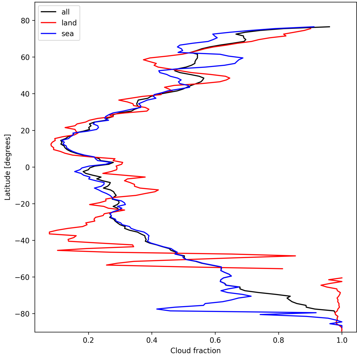
Figure 15: Zonal average of “Cloud fraction” for 2025-02-15 to 2025-02-17.
