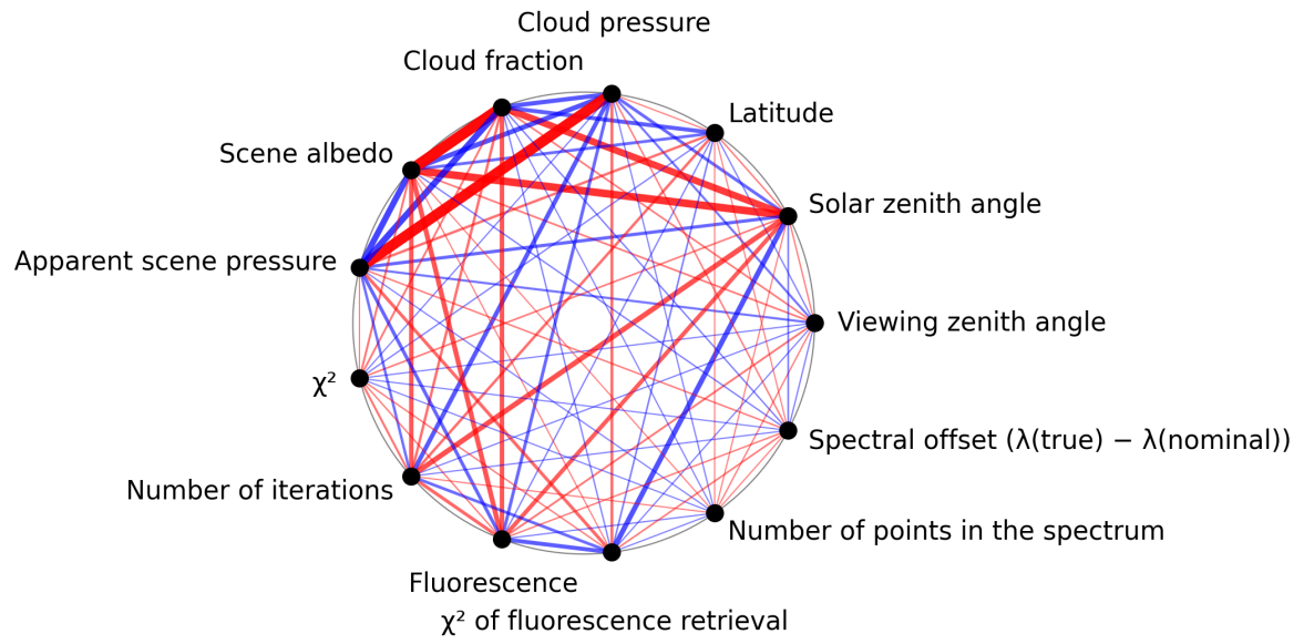
Figure 1: Map of correlation graph for 2025-02-15 to 2025-02-17.
