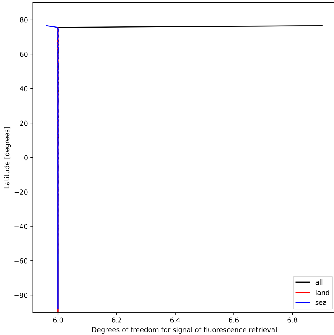
Figure 26: Zonal average of “Degrees of freedom for signal of fluorescence retrieval” for 2025-02-15 to 2025-02-17.
