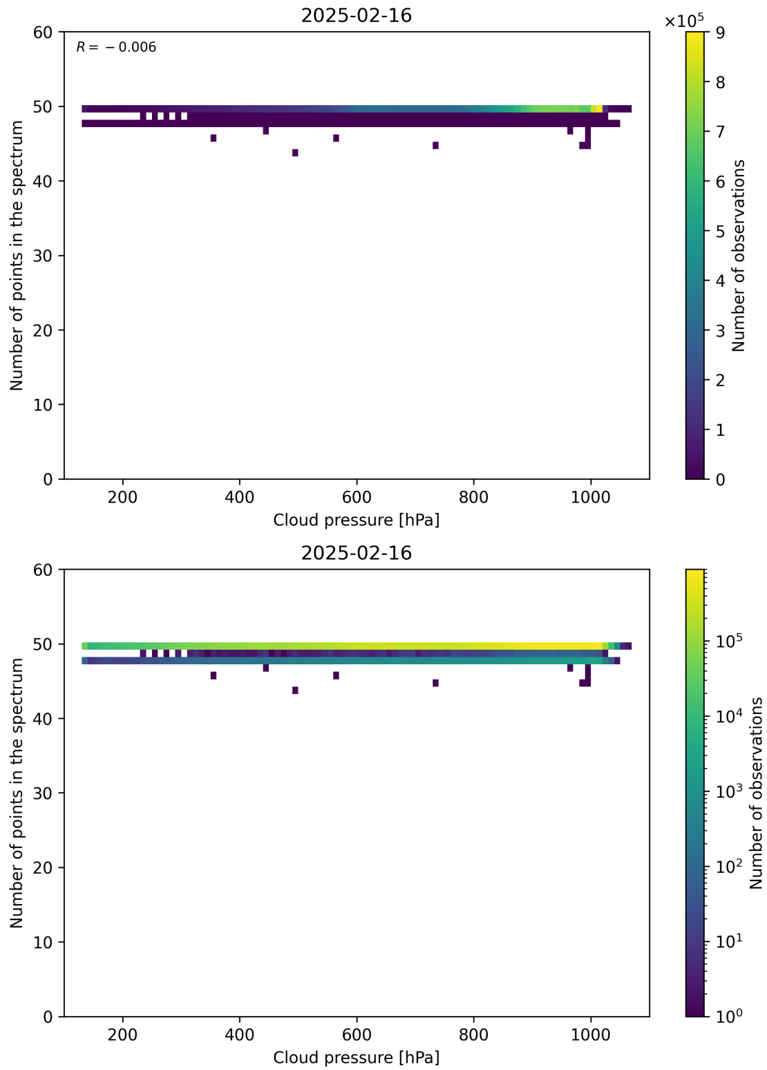
Figure 82: Scatter density plot of “Cloud pressure” against “Number of points in the spectrum” for 2025-02-15 to 2025-02-17.
