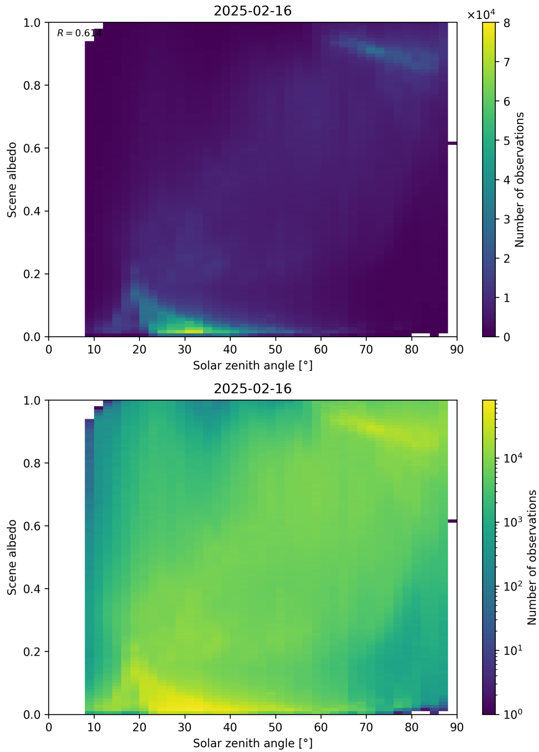
Figure 116: Scatter density plot of “Solar zenith angle” against “Scene albedo” for 2025-02-15 to 2025-02-17.
