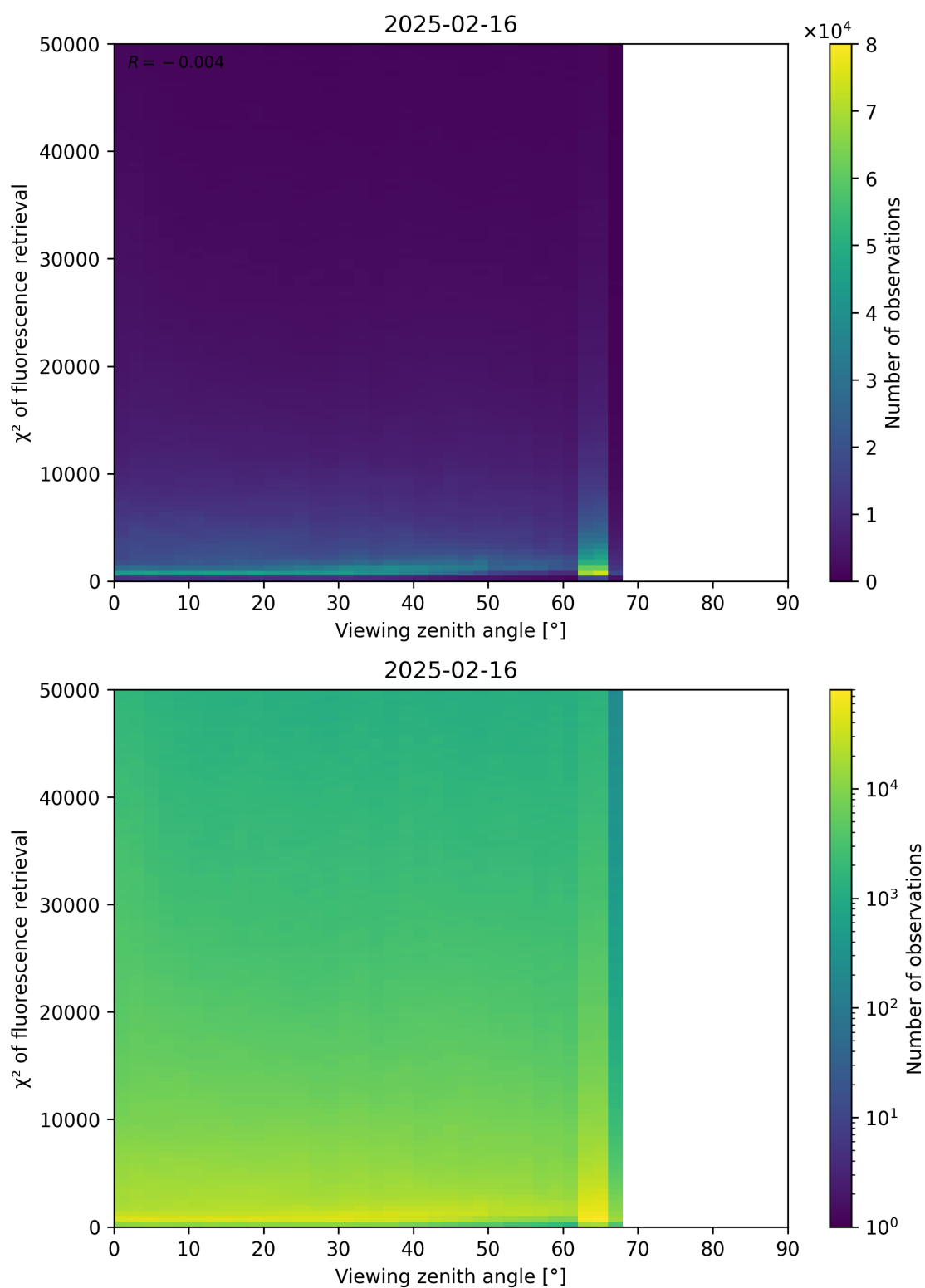
Figure 119: Scatter density plot of “Viewing zenith angle” against “ \chi^2 of fluorescence retrieval” for 2025-02-15 to 2025-02-17.
