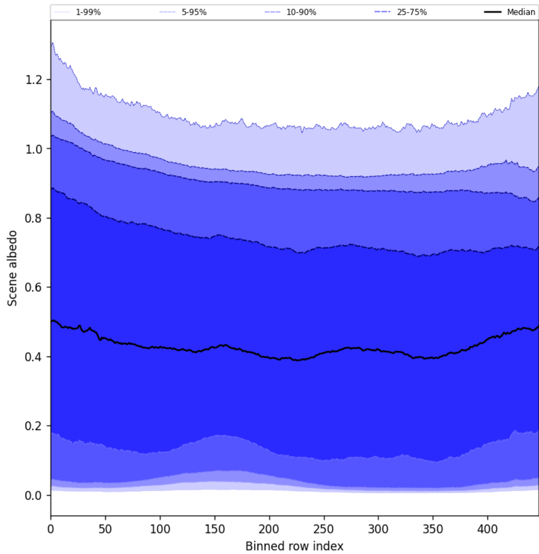
Figure 51: Along track statistics of “Scene albedo” for 2025-02-15 to 2025-02-17
