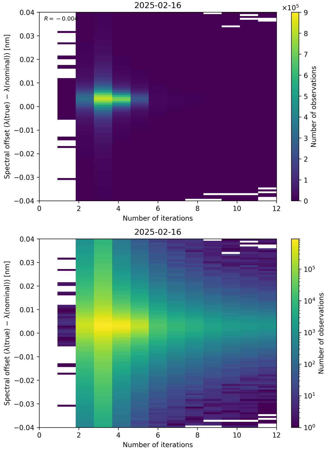
Figure 100: Scatter density plot of “Number of iterations” against “Spectral offset ( \lambda_{\text{true}} - \lambda_{\text{nominal}} )” for 2025-02-15 to 2025-02-17.
