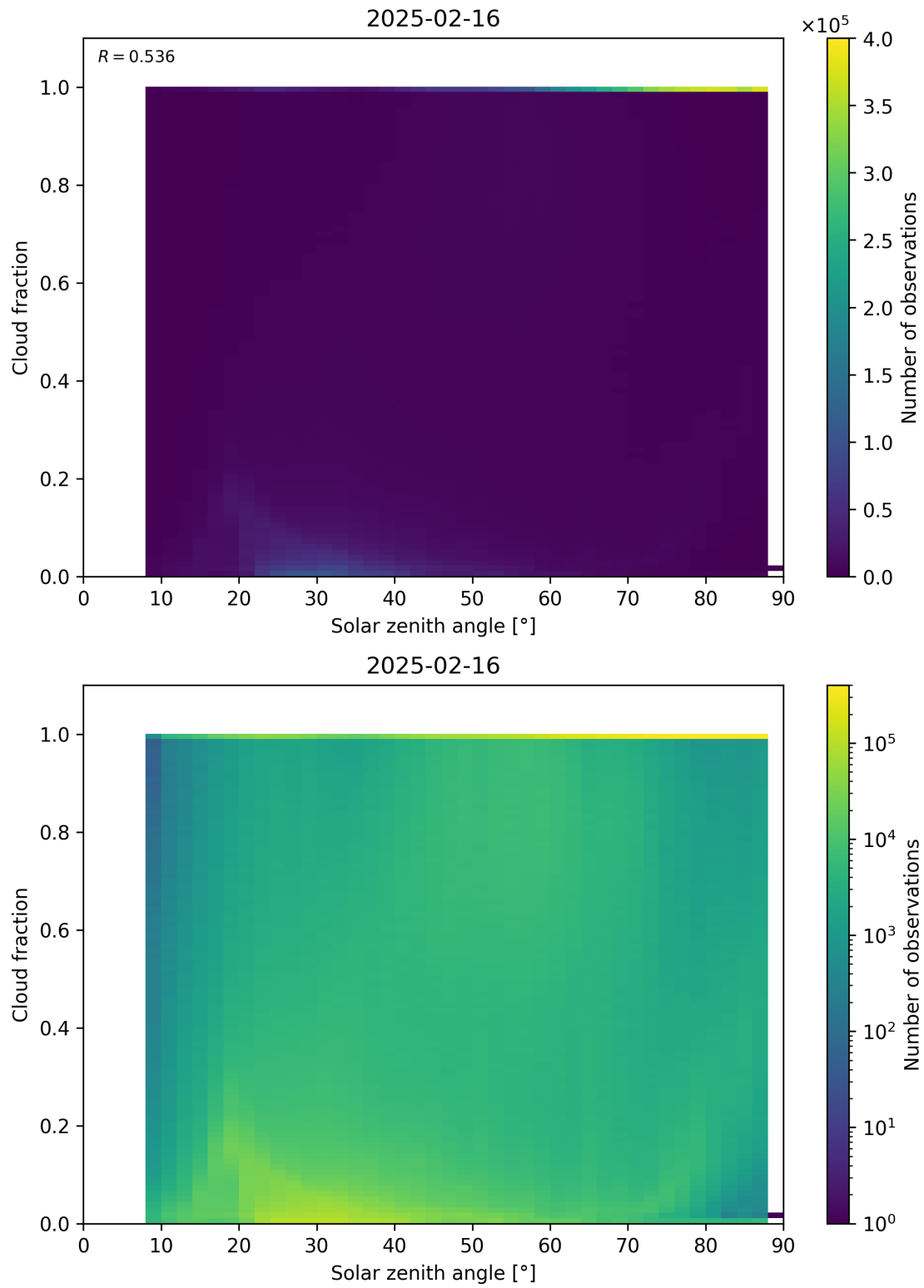
Figure 110: Scatter density plot of “Solar zenith angle” against “Cloud fraction” for 2025-02-15 to 2025-02-17.
