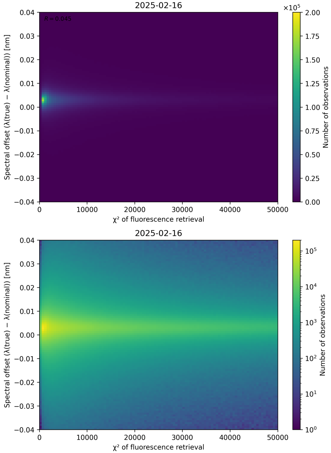
Figure 69: Scatter density plot of “ \chi^2 of fluorescence retrieval” against “Spectral offset ( \lambda_{\text{true}} - \lambda_{\text{nominal}} )” for 2025-02-15 to 2025-02-17.
