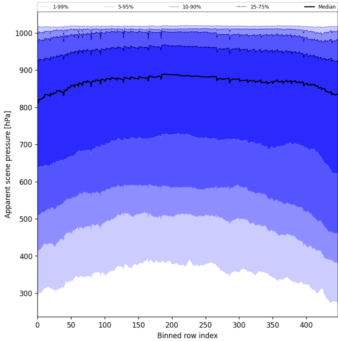
Figure 53: Along track statistics of “Apparent scene pressure” for 2025-02-15 to 2025-02-17
