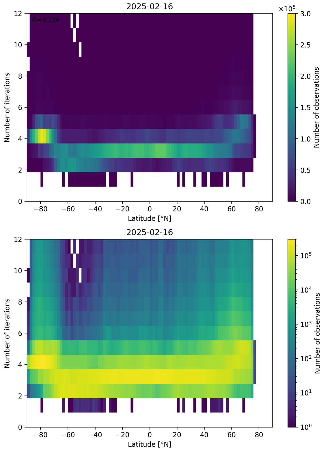
Figure 93: Scatter density plot of “Latitude” against “Number of iterations” for 2025-02-15 to 2025-02-17.
