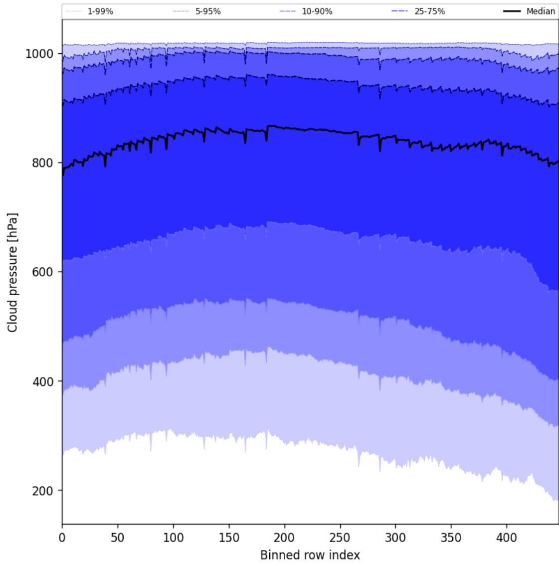
Figure 47: Along track statistics of “Cloud pressure” for 2025-02-15 to 2025-02-17
