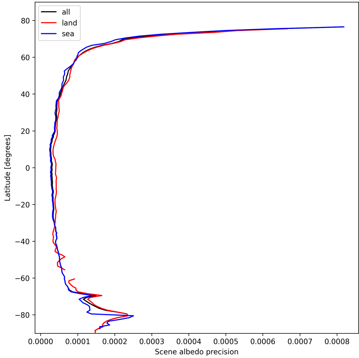
Figure 18: Zonal average of “Scene albedo precision” for 2025-02-15 to 2025-02-17.
