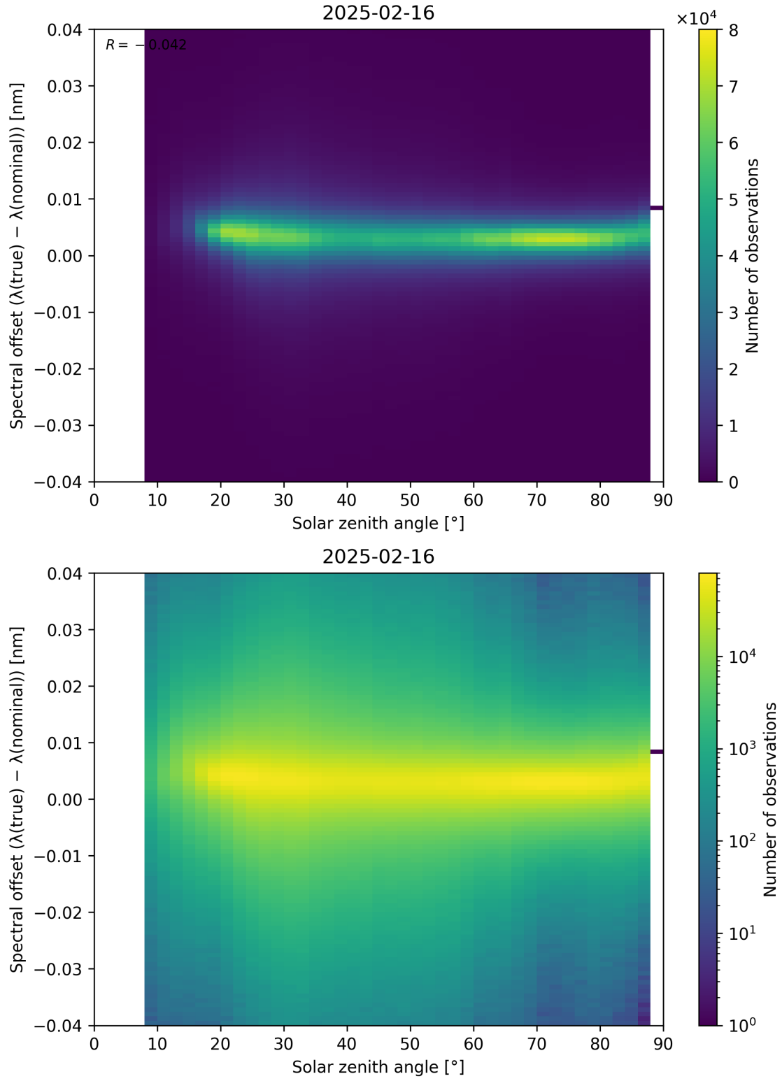
Figure 117: Scatter density plot of “Solar zenith angle” against “Spectral offset ( \lambda_{\text{true}} - \lambda_{\text{nominal}} )” for 2025-02-15 to 2025-02-17.
