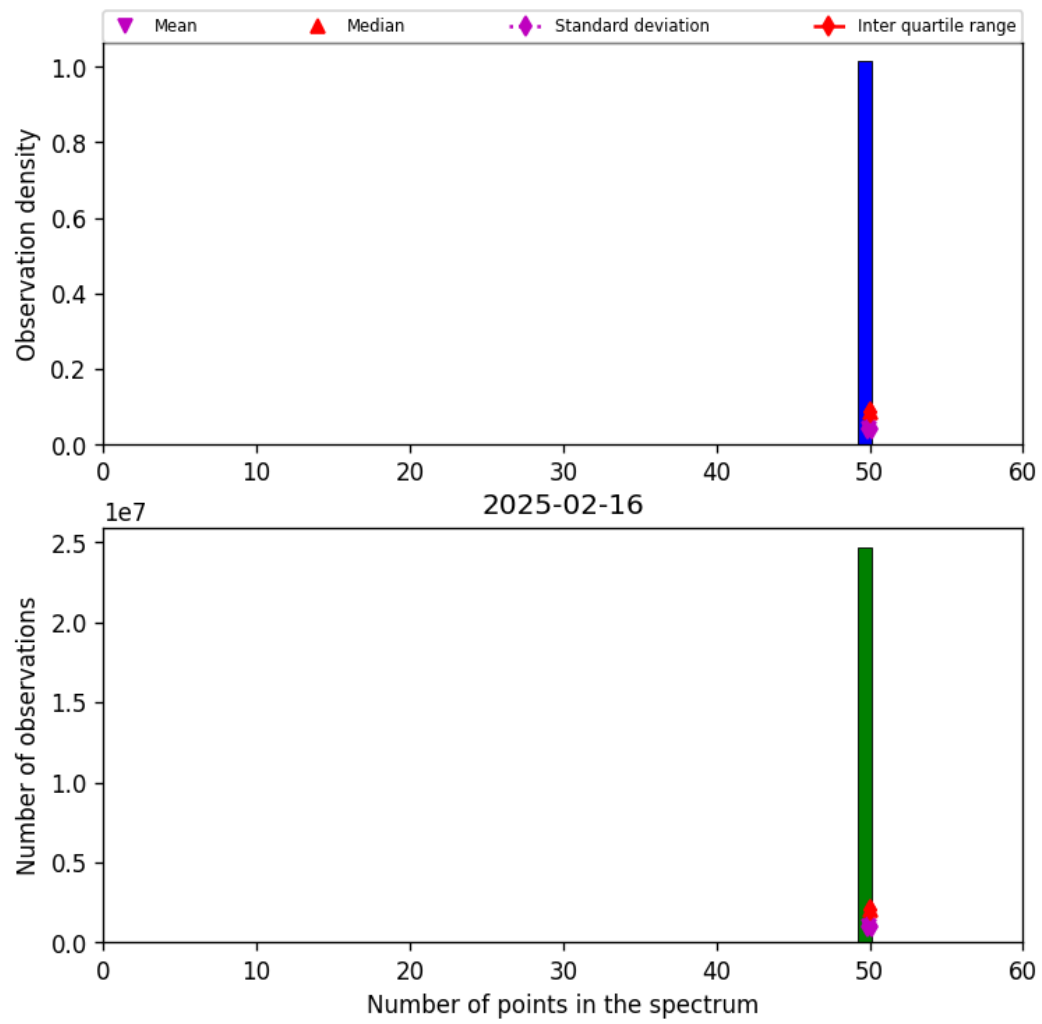
Figure 44: Histogram of “Number of points in the spectrum” for 2025-02-15 to 2025-02-17
