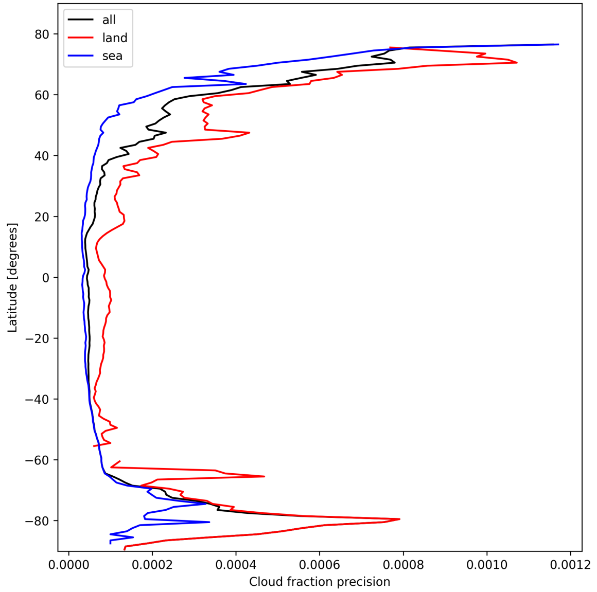
Figure 16: Zonal average of “Cloud fraction precision” for 2025-02-15 to 2025-02-17.
