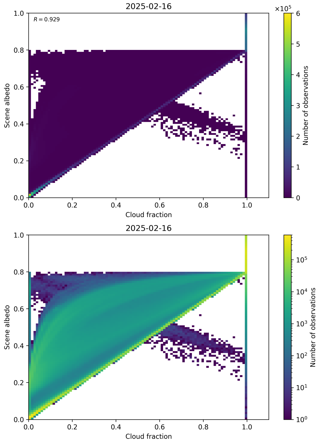
Figure 75: Scatter density plot of “Cloud fraction” against “Scene albedo” for 2025-02-15 to 2025-02-17.
