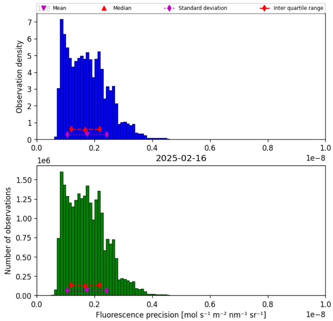
Figure 41: Histogram of “Fluorescence precision” for 2025-02-15 to 2025-02-17
