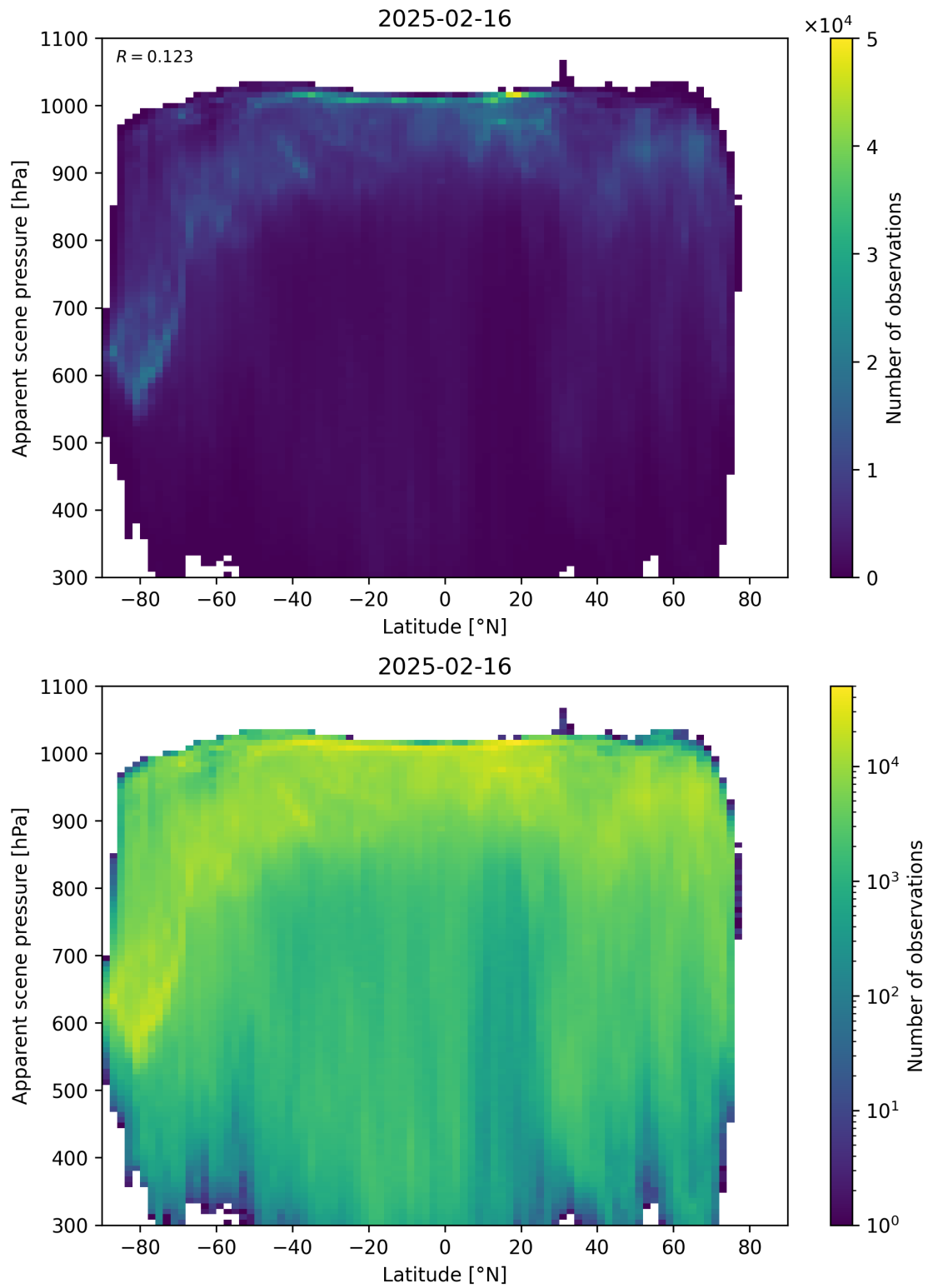
Figure 88: Scatter density plot of “Latitude” against “Apparent scene pressure” for 2025-02-15 to 2025-02-17.
