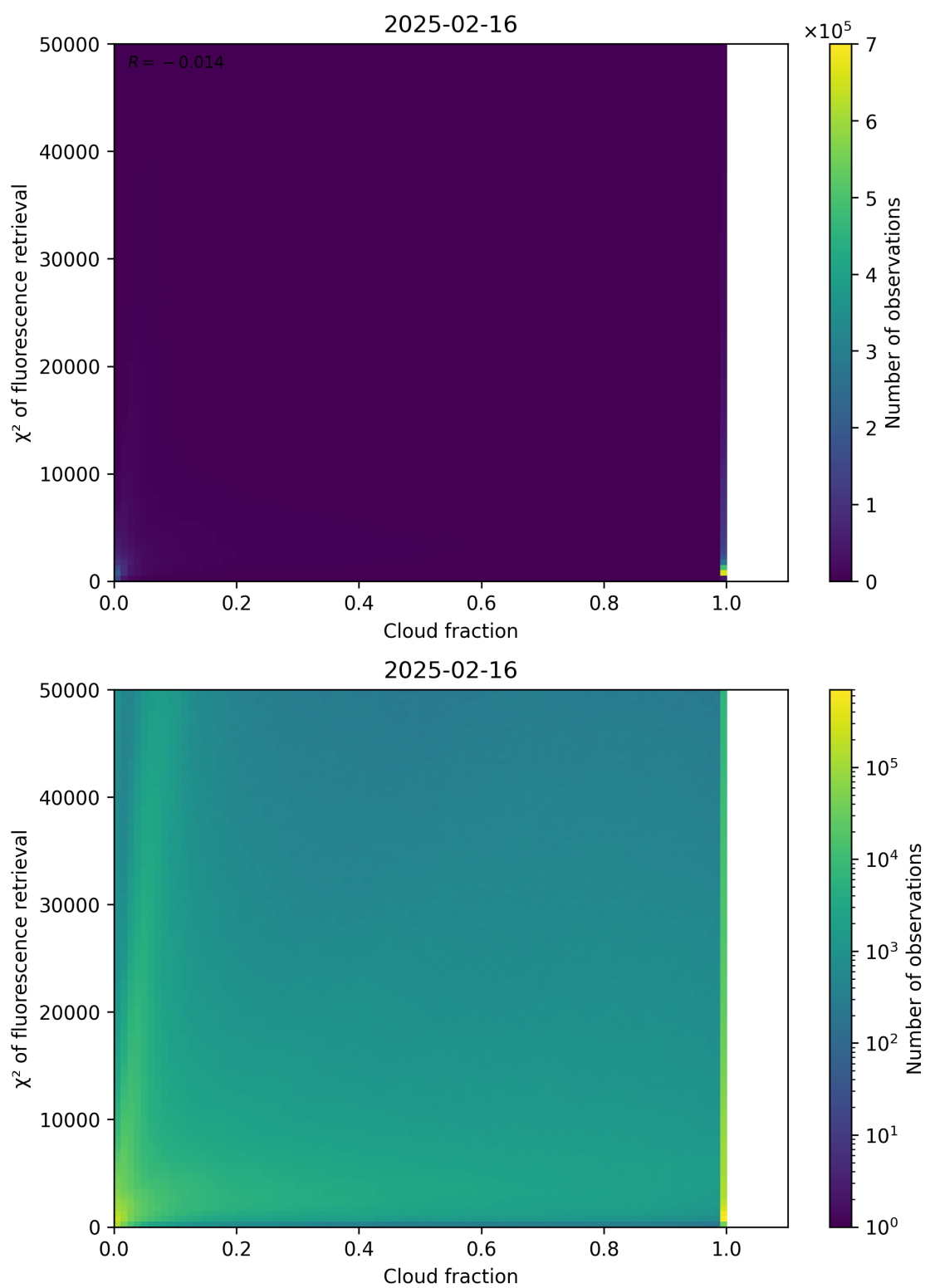
Figure 71: Scatter density plot of “Cloud fraction” against “ \chi^2 of fluorescence retrieval” for 2025-02-15 to 2025-02-17.
