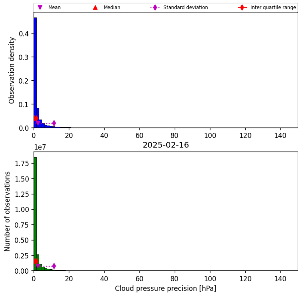
Figure 31: Histogram of “Cloud pressure precision” for 2025-02-15 to 2025-02-17
