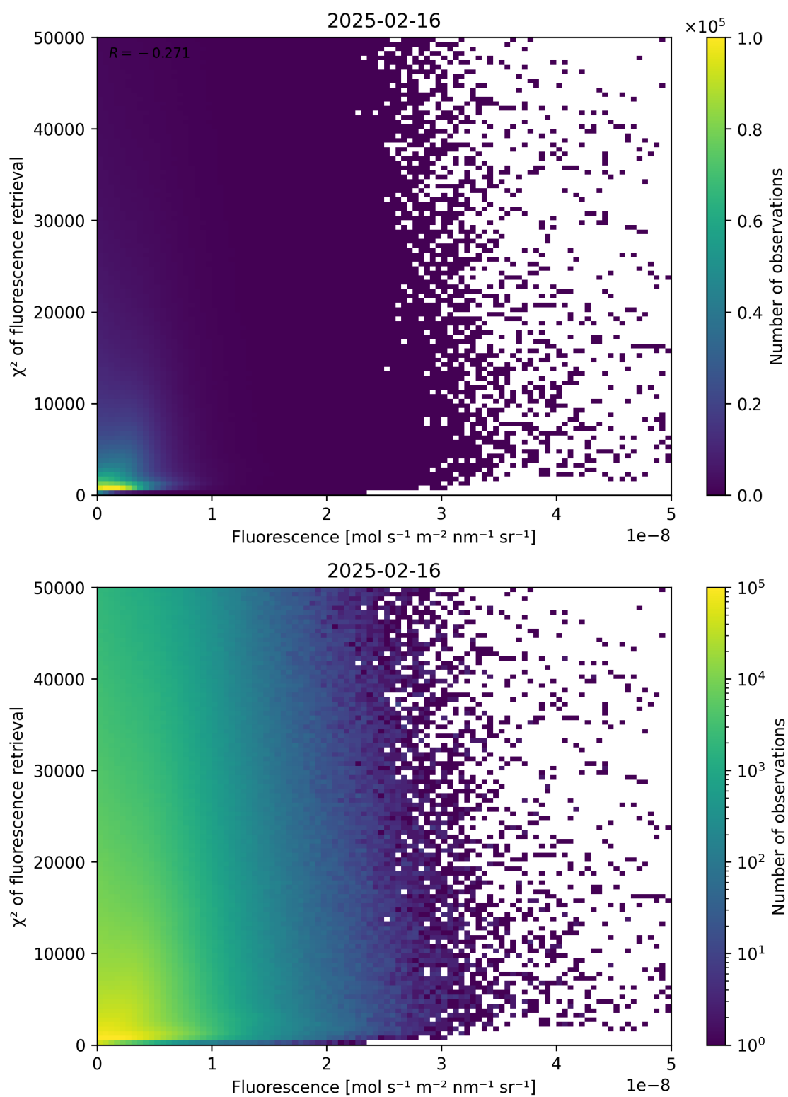
Figure 85: Scatter density plot of “Fluorescence” against “ \chi^2 of fluorescence retrieval” for 2025-02-15 to 2025-02-17.
