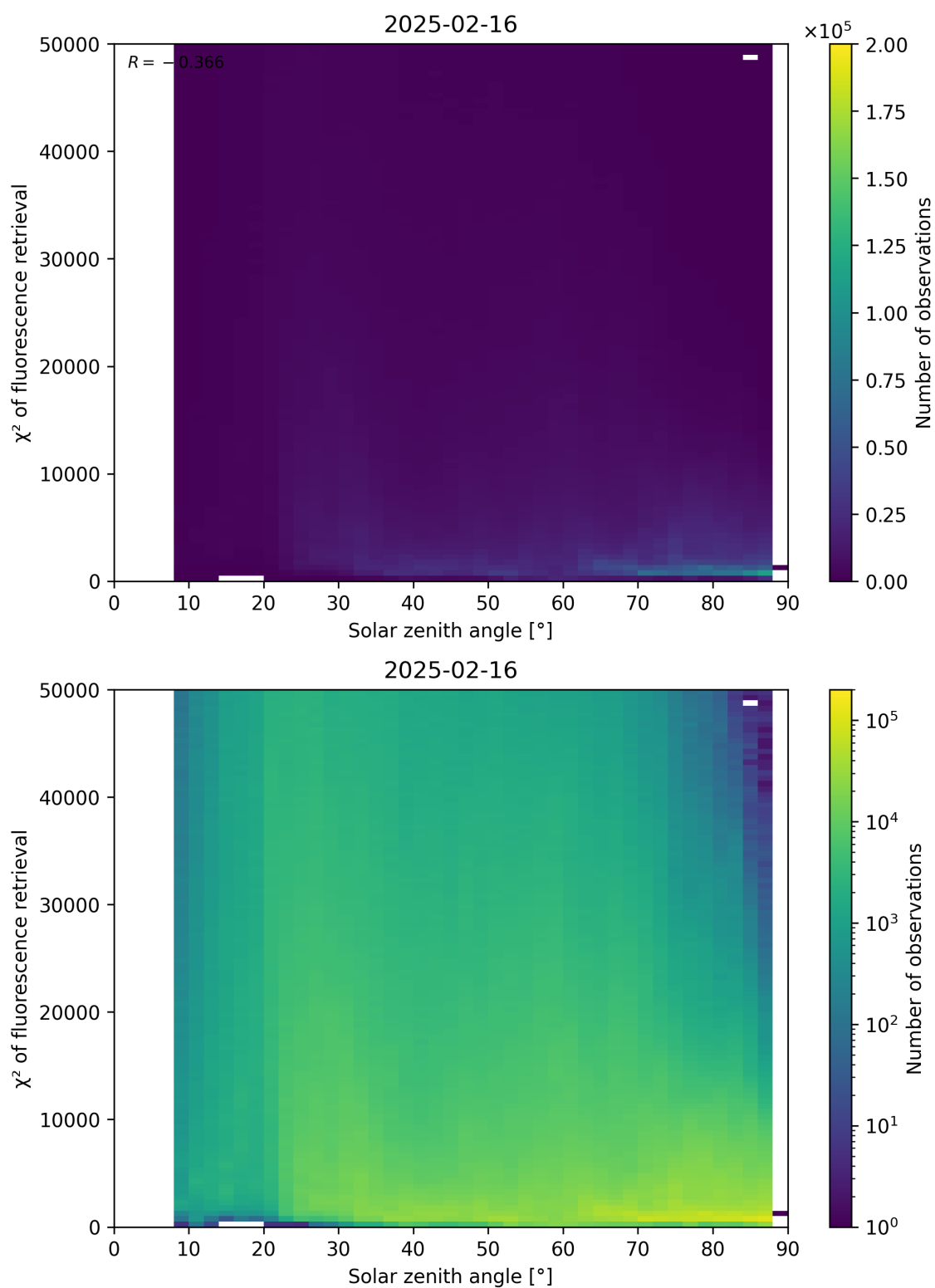
Figure 109: Scatter density plot of “Solar zenith angle” against “ \chi^2 of fluorescence retrieval” for 2025-02-15 to 2025-02-17.
