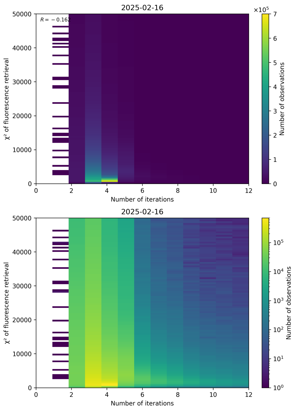
Figure 97: Scatter density plot of “Number of iterations” against “ \chi^2 of fluorescence retrieval” for 2025-02-15 to 2025-02-17.
