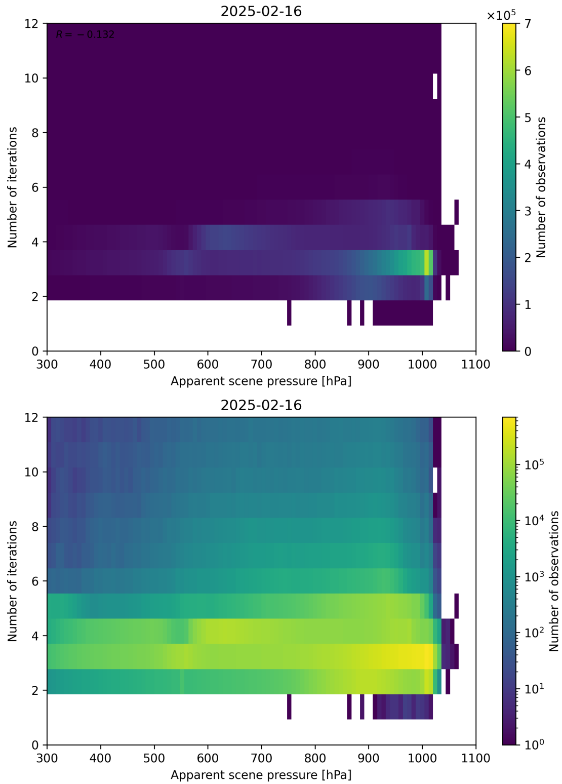
Figure 65: Scatter density plot of “Apparent scene pressure” against “Number of iterations” for 2025-02-15 to 2025-02-17.
