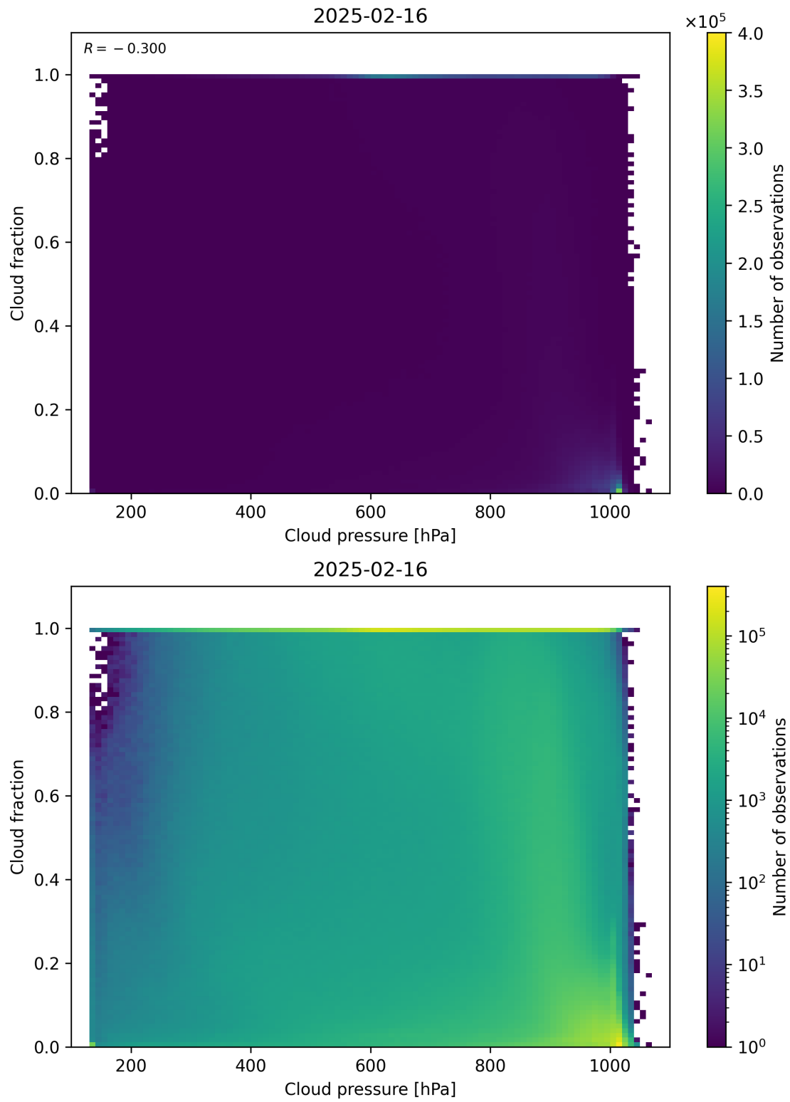
Figure 79: Scatter density plot of “Cloud pressure” against “Cloud fraction” for 2025-02-15 to 2025-02-17.
