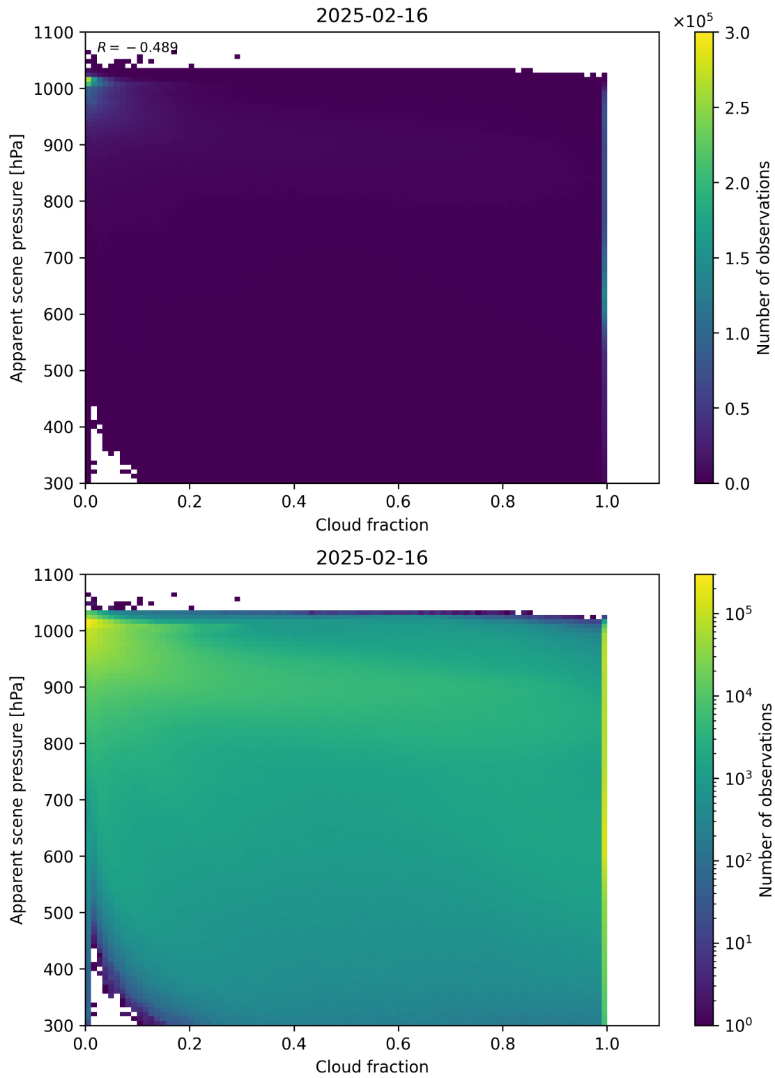
Figure 70: Scatter density plot of “Cloud fraction” against “Apparent scene pressure” for 2025-02-15 to 2025-02-17.
