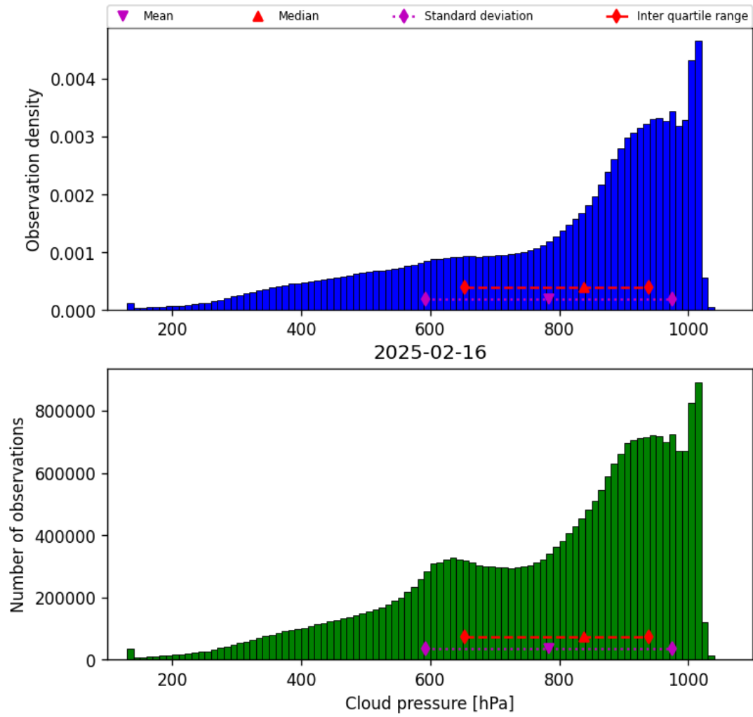
Figure 30: Histogram of “Cloud pressure” for 2025-02-15 to 2025-02-17
