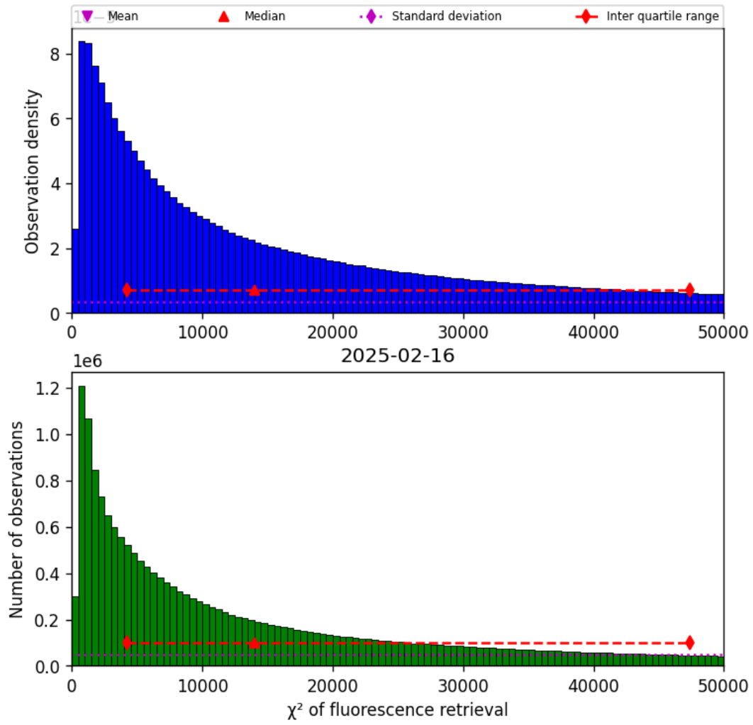
Figure 42: Histogram of “ \chi^2 of fluorescence retrieval” for 2025-02-15 to 2025-02-17
