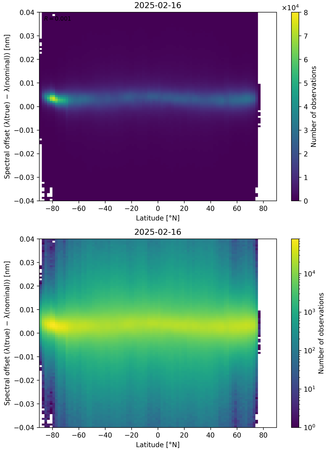
Figure 96: Scatter density plot of “Latitude” against “Spectral offset ( \lambda_{\text{true}} - \lambda_{\text{nominal}} )” for 2025-02-15 to 2025-02-17.
