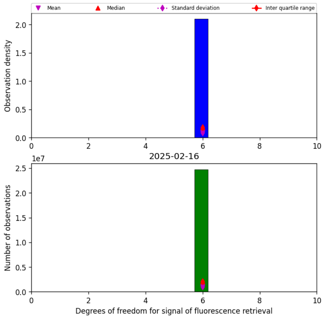
Figure 43: Histogram of “Degrees of freedom for signal of fluorescence retrieval” for 2025-02-15 to 2025-02-17
