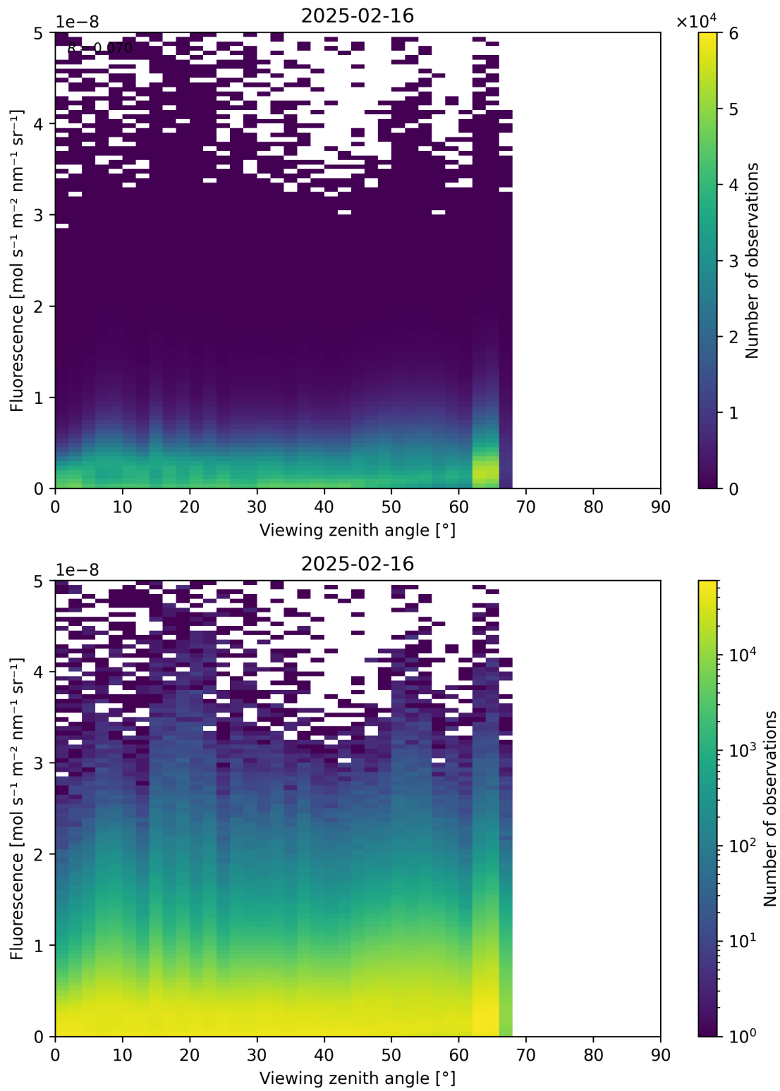
Figure 122: Scatter density plot of “Viewing zenith angle” against “Fluorescence” for 2025-02-15 to 2025-02-17.
