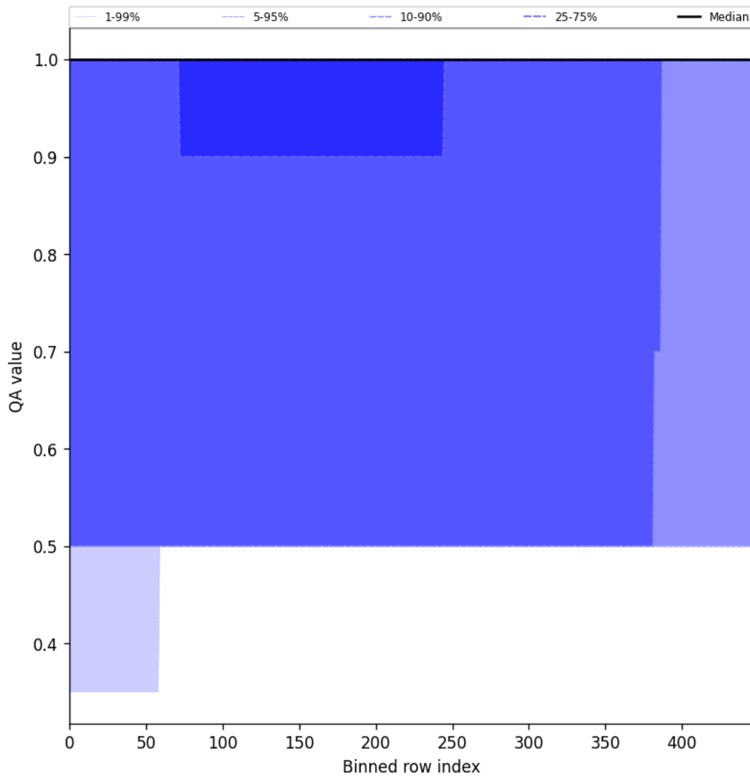
Figure 46: Along track statistics of “QA value” for 2025-02-15 to 2025-02-17
