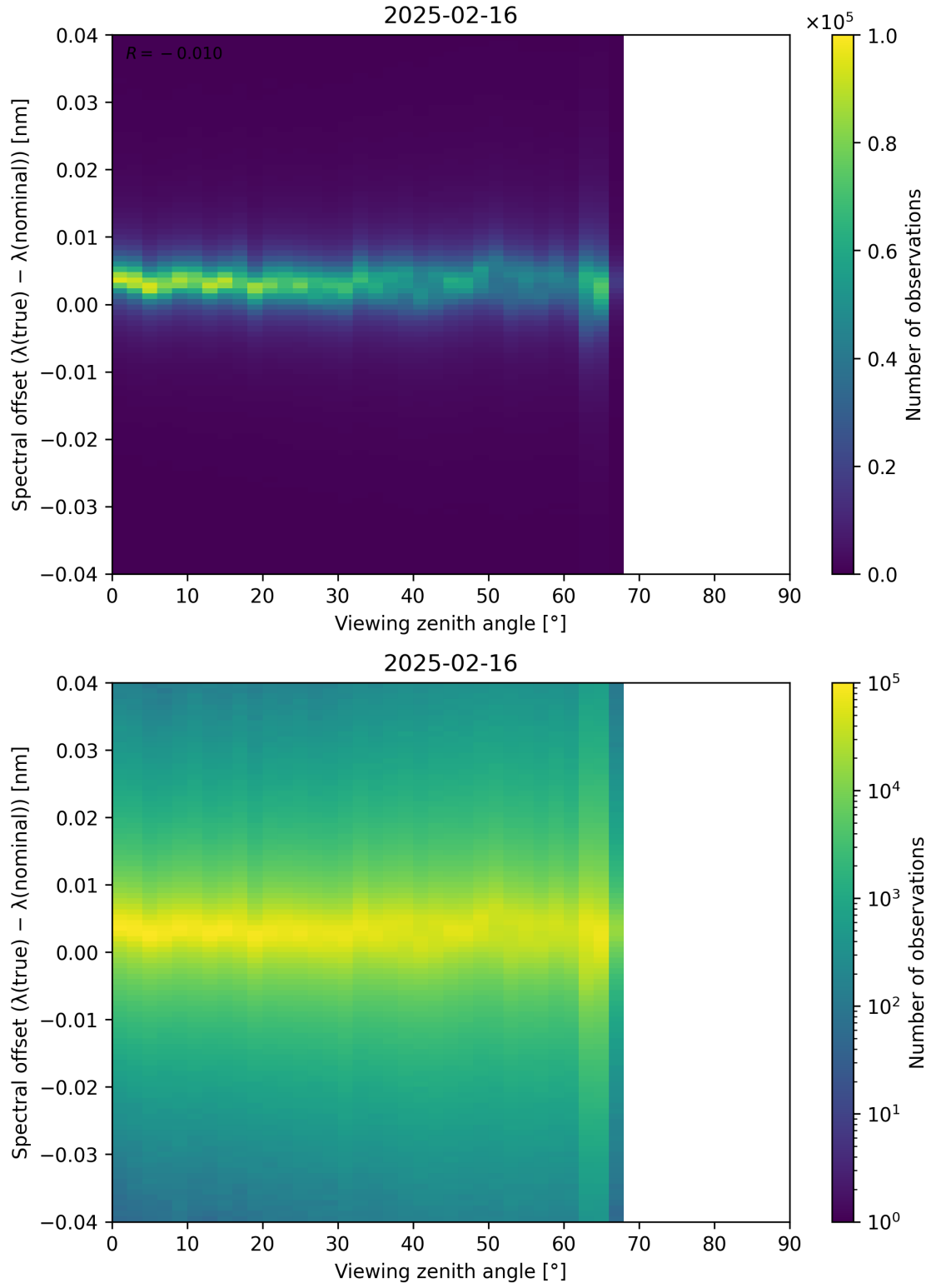
Figure 128: Scatter density plot of “Viewing zenith angle” against “Spectral offset ( \lambda_{\text{true}} - \lambda_{\text{nominal}} )” for 2025-02-15 to 2025-02-17.
