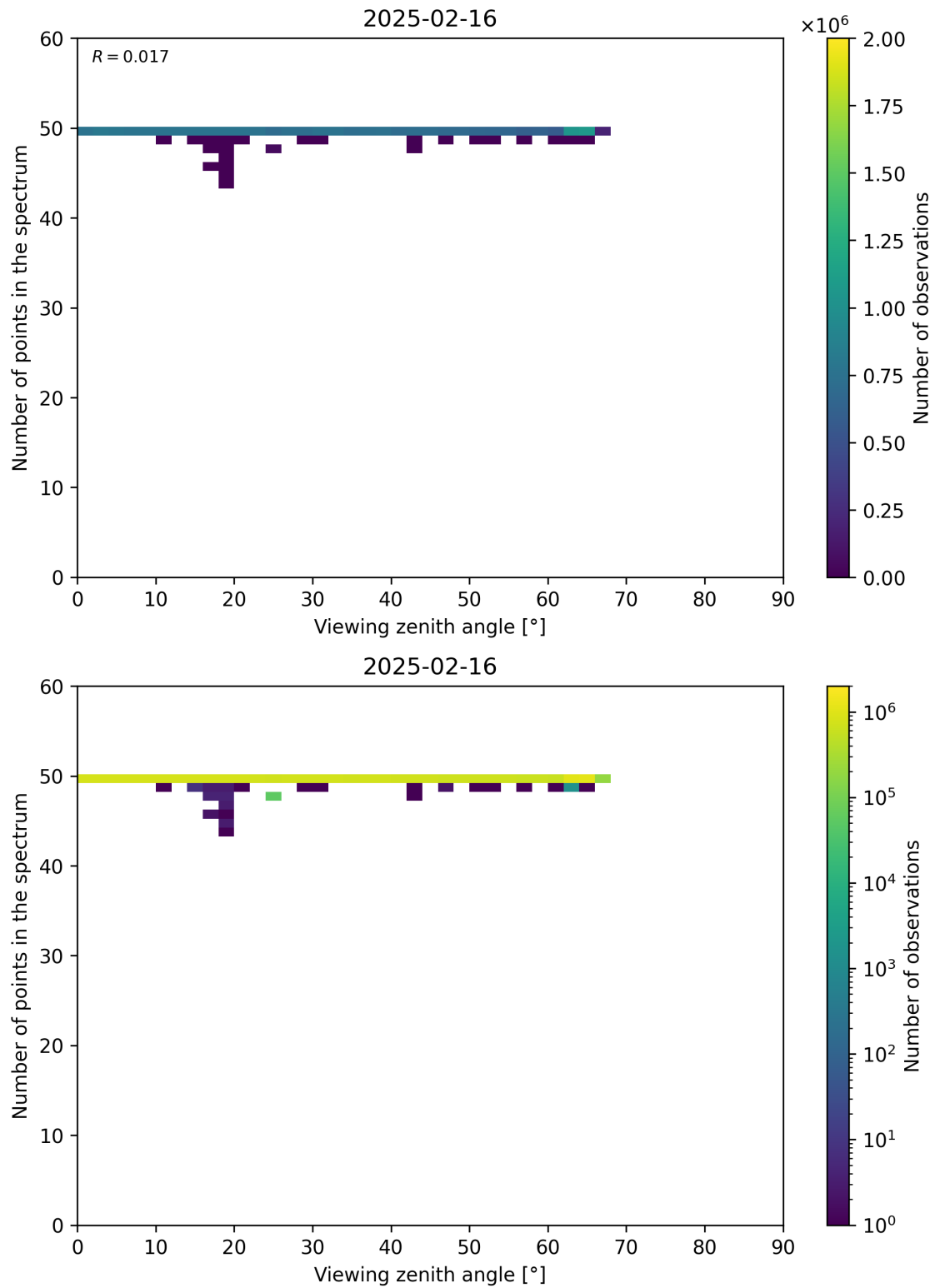
Figure 125: Scatter density plot of “Viewing zenith angle” against “Number of points in the spectrum” for 2025-02-15 to 2025-02-17.
