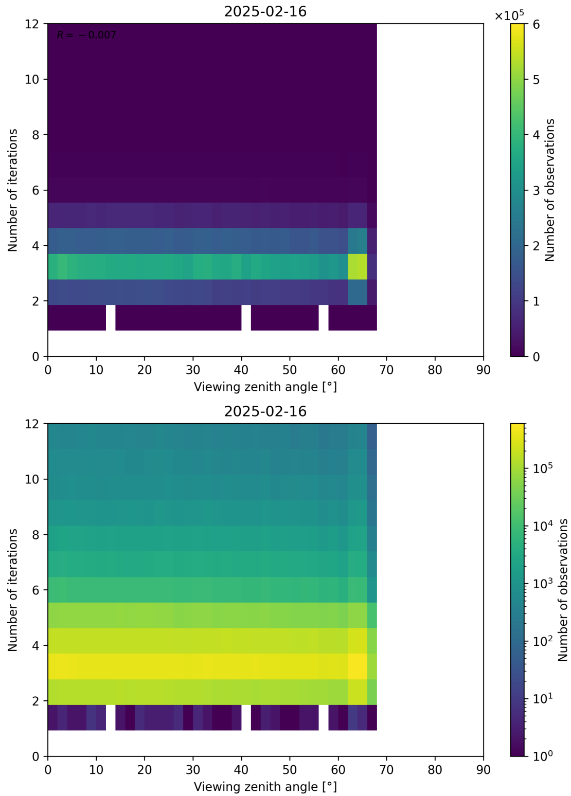
Figure 124: Scatter density plot of “Viewing zenith angle” against “Number of iterations” for 2025-02-15 to 2025-02-17.
