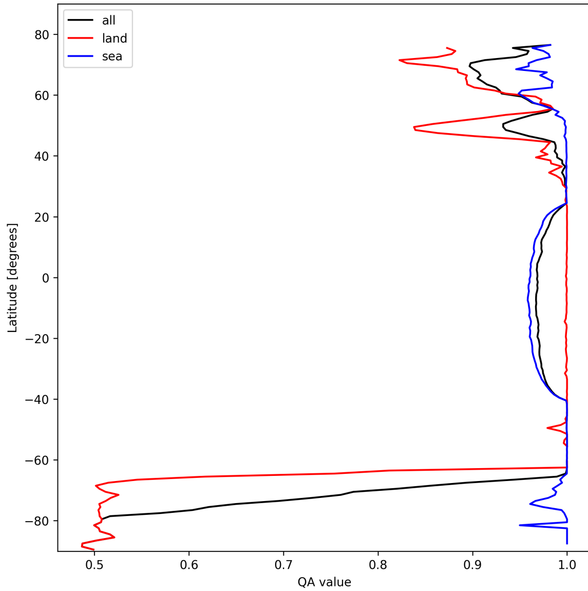
Figure 12: Zonal average of “QA value” for 2025-02-15 to 2025-02-17.
