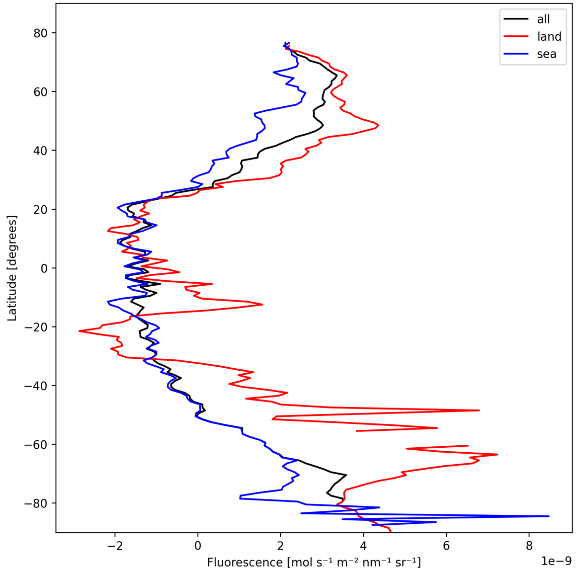
Figure 23: Zonal average of “Fluorescence” for 2025-02-15 to 2025-02-17.
