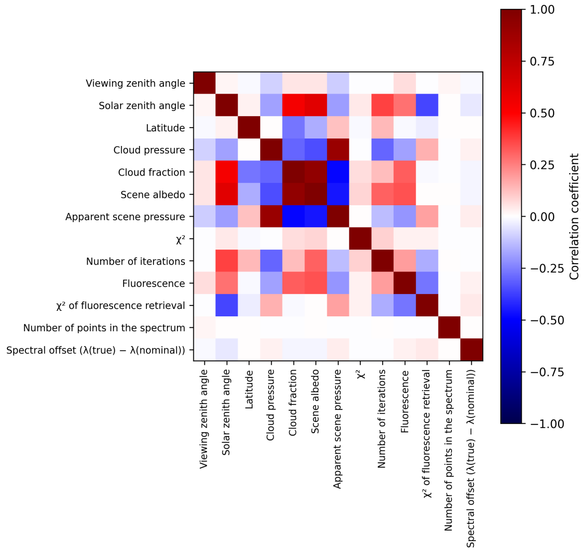
Figure 2: Map of correlation matrix for 2025-02-15 to 2025-02-17.
