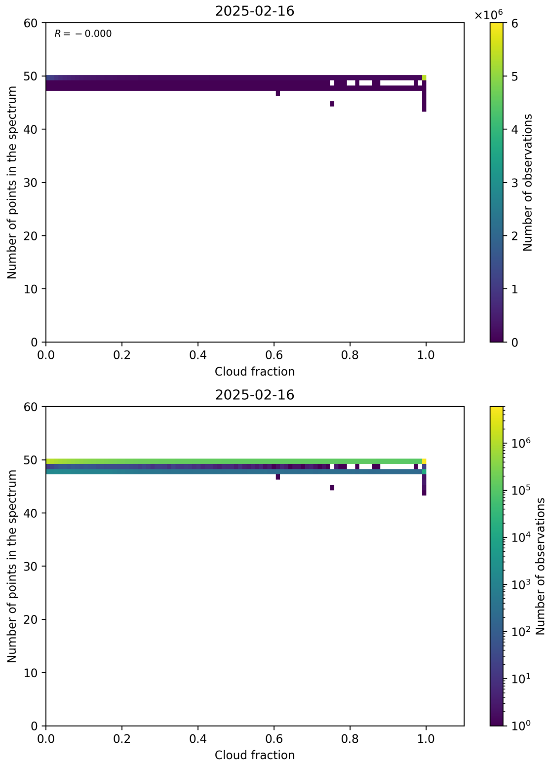
Figure 74: Scatter density plot of “Cloud fraction” against “Number of points in the spectrum” for 2025-02-15 to 2025-02-17.
