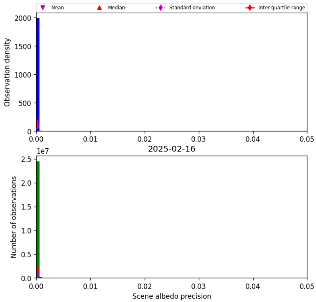
Figure 35: Histogram of “Scene albedo precision” for 2025-02-15 to 2025-02-17
