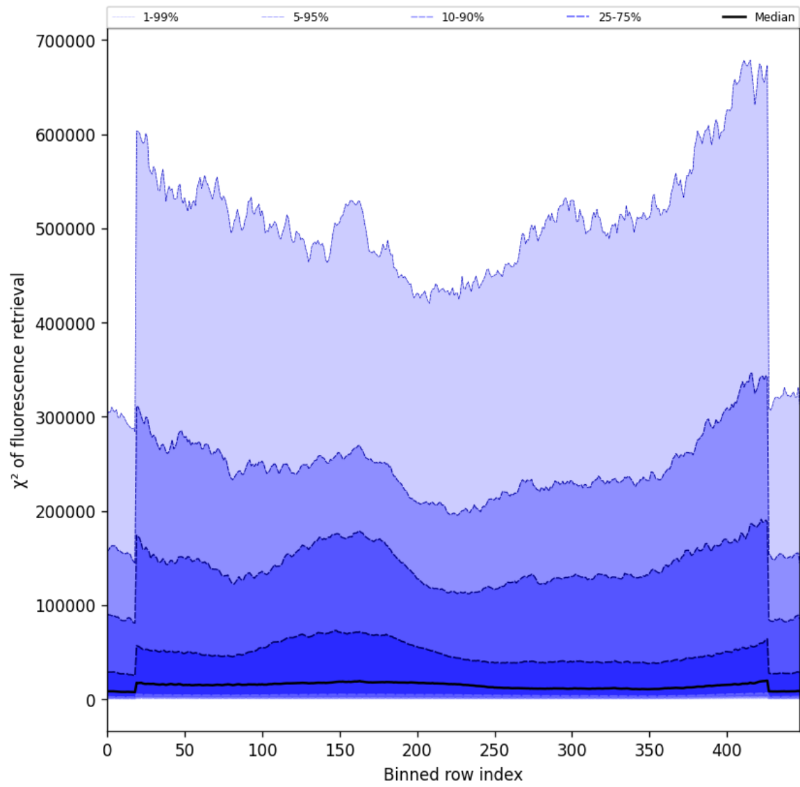
Figure 59: Along track statistics of “ \chi^2 of fluorescence retrieval” for 2025-02-15 to 2025-02-17
