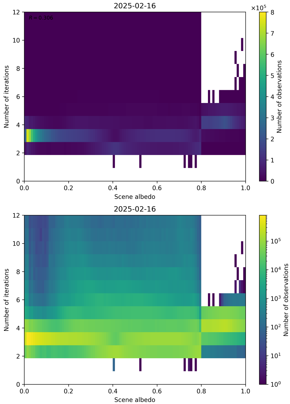
Figure 105: Scatter density plot of “Scene albedo” against “Number of iterations” for 2025-02-15 to 2025-02-17.
