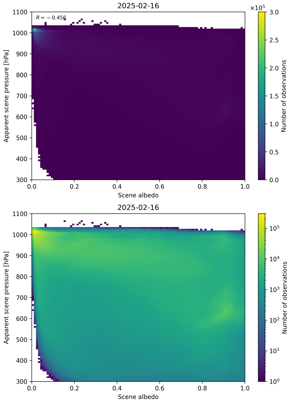
Figure 102: Scatter density plot of “Scene albedo” against “Apparent scene pressure” for 2025-02-15 to 2025-02-17.
