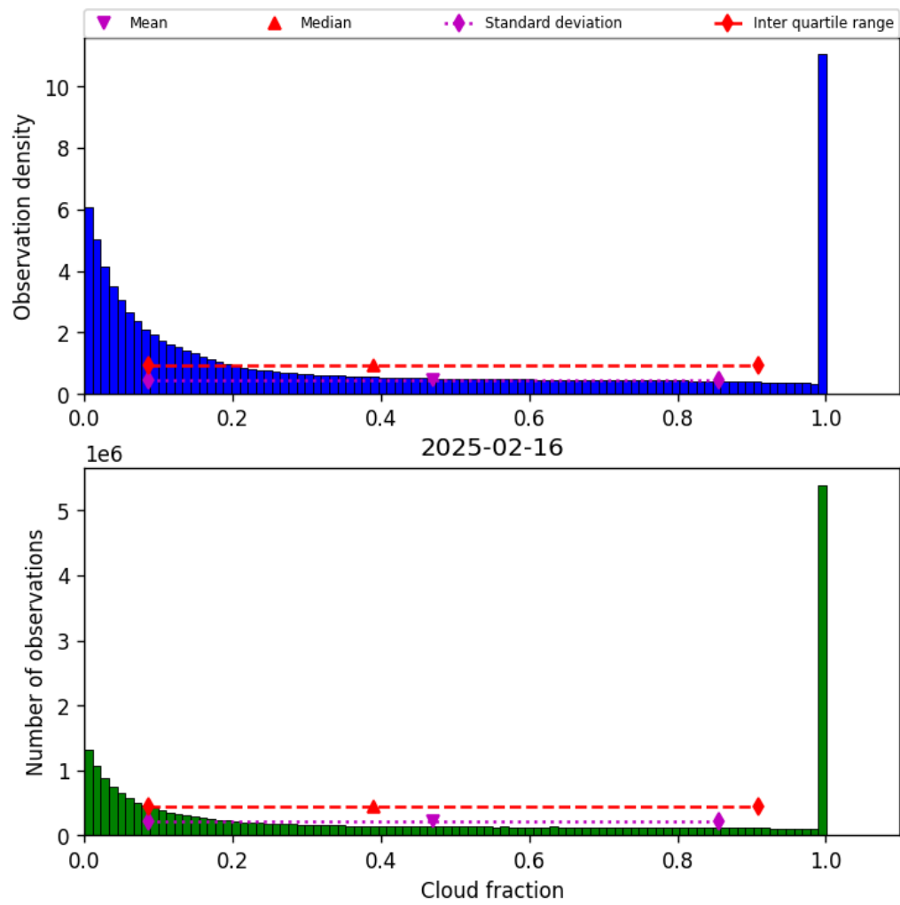
Figure 32: Histogram of “Cloud fraction” for 2025-02-15 to 2025-02-17
