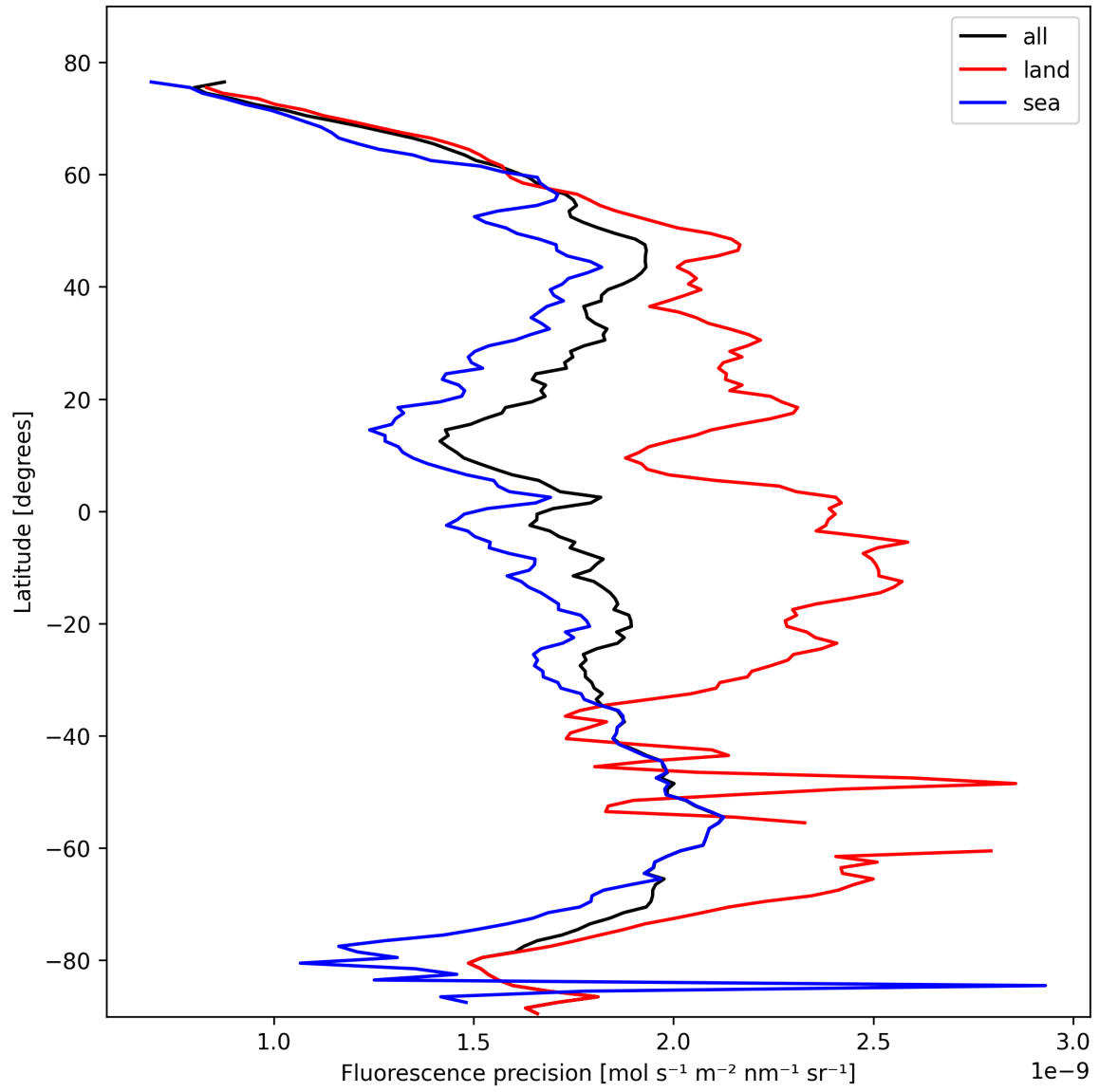
Figure 24: Zonal average of “Fluorescence precision” for 2025-02-15 to 2025-02-17.
