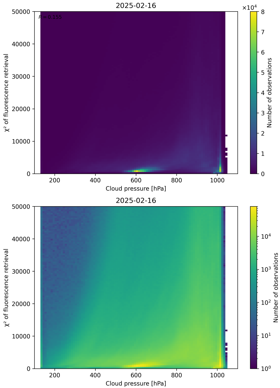
Figure 78: Scatter density plot of “Cloud pressure” against “ \chi^2 of fluorescence retrieval” for 2025-02-15 to 2025-02-17.
