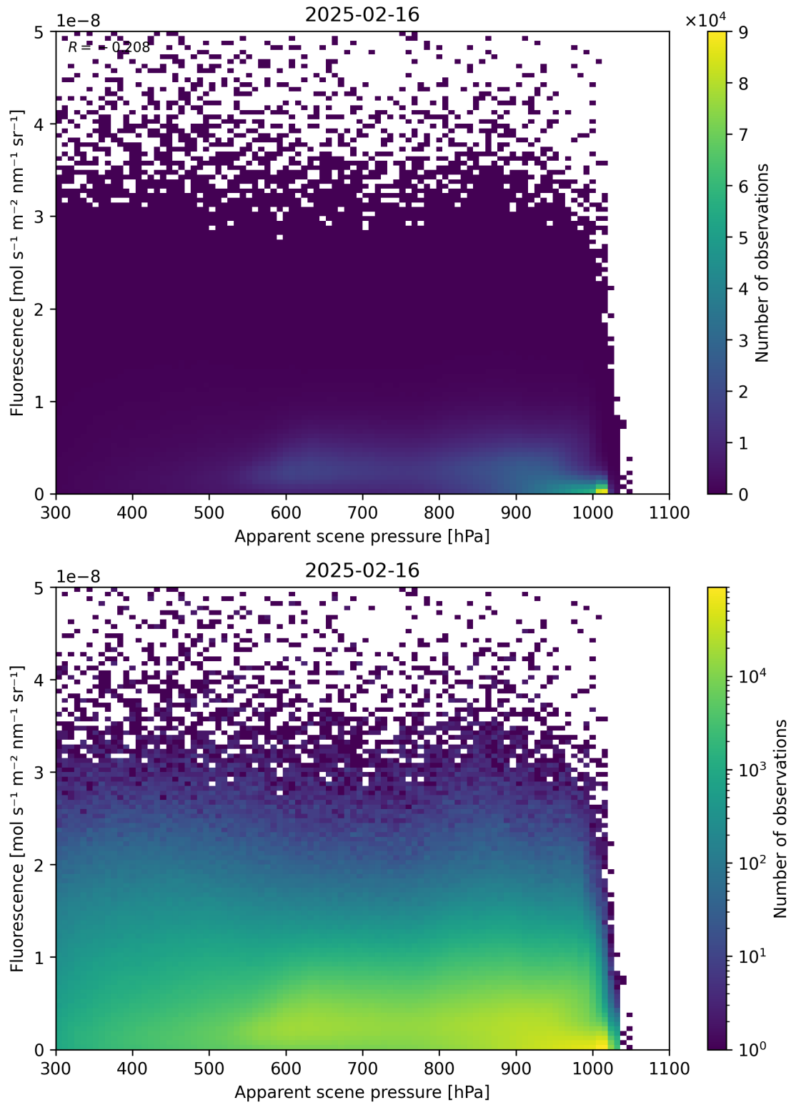
Figure 64: Scatter density plot of “Apparent scene pressure” against “Fluorescence” for 2025-02-15 to 2025-02-17.
