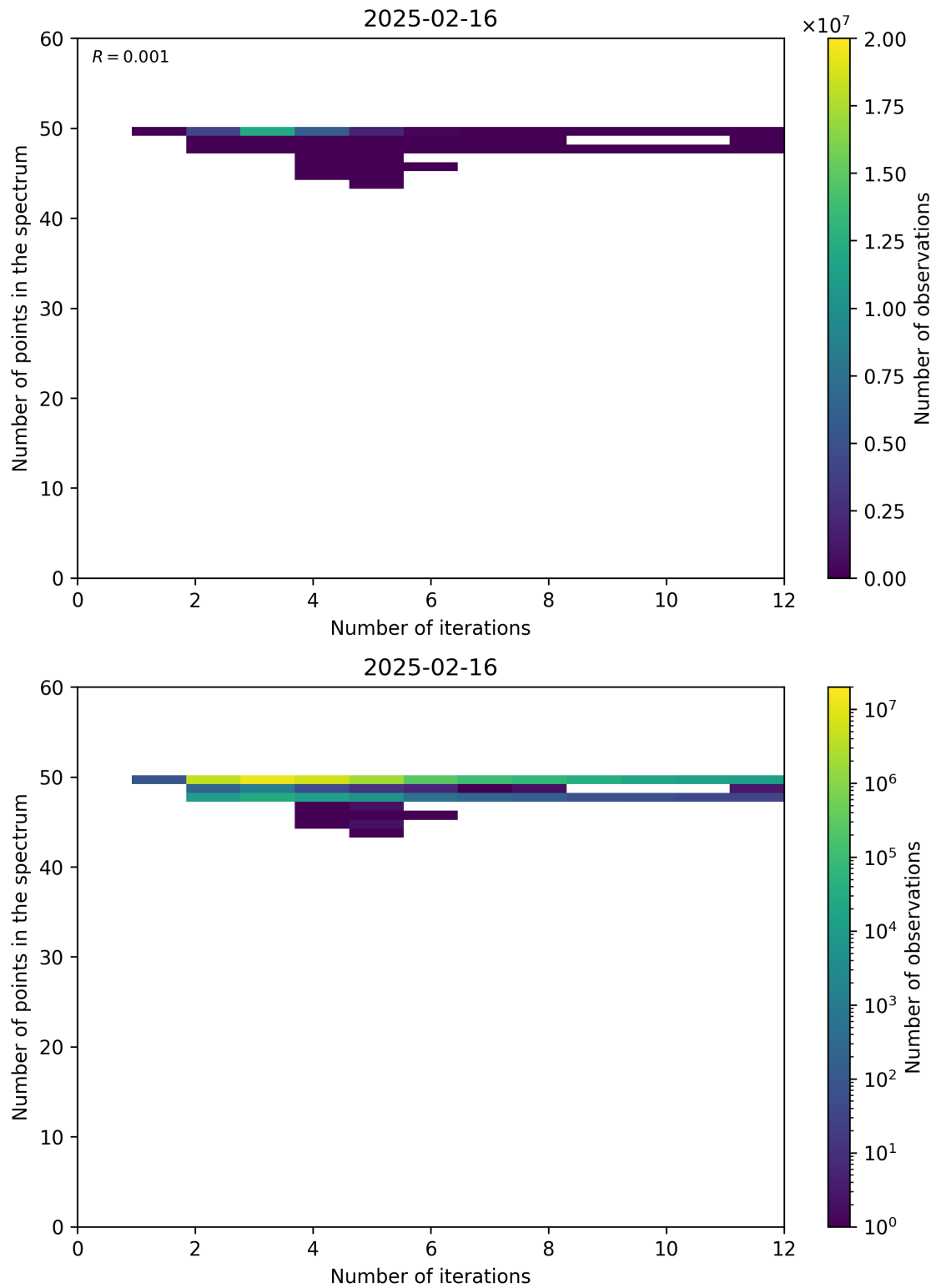
Figure 99: Scatter density plot of “Number of iterations” against “Number of points in the spectrum” for 2025-02-15 to 2025-02-17.
