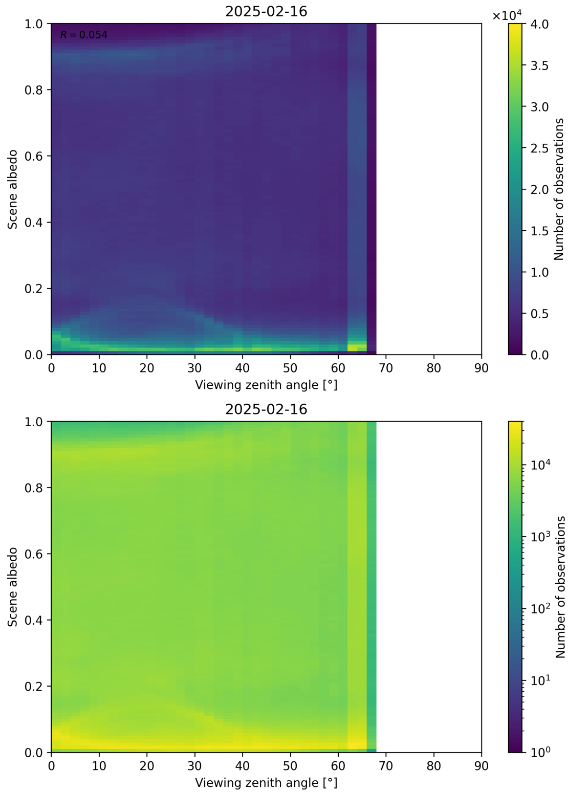
Figure 126: Scatter density plot of “Viewing zenith angle” against “Scene albedo” for 2025-02-15 to 2025-02-17.
