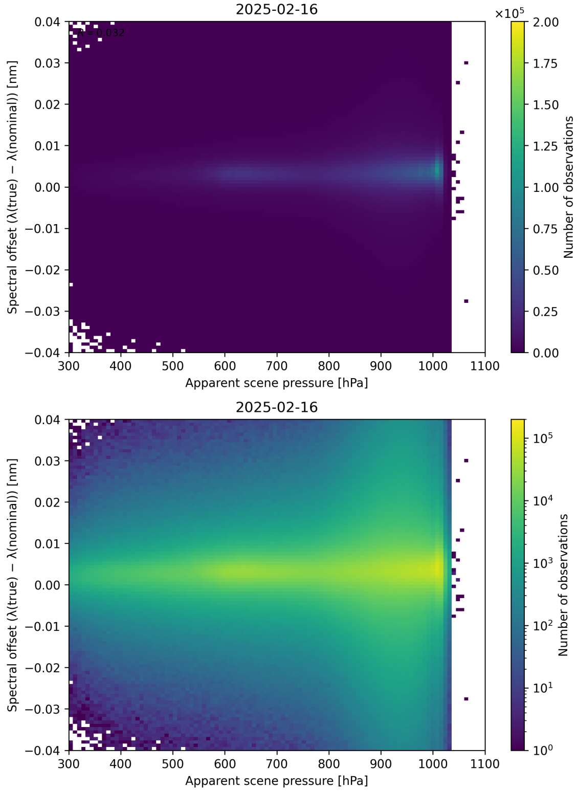
Figure 67: Scatter density plot of “Apparent scene pressure” against “Spectral offset ( \lambda_{\text{true}} - \lambda_{\text{nominal}} )” for 2025-02-15 to 2025-02-17.
