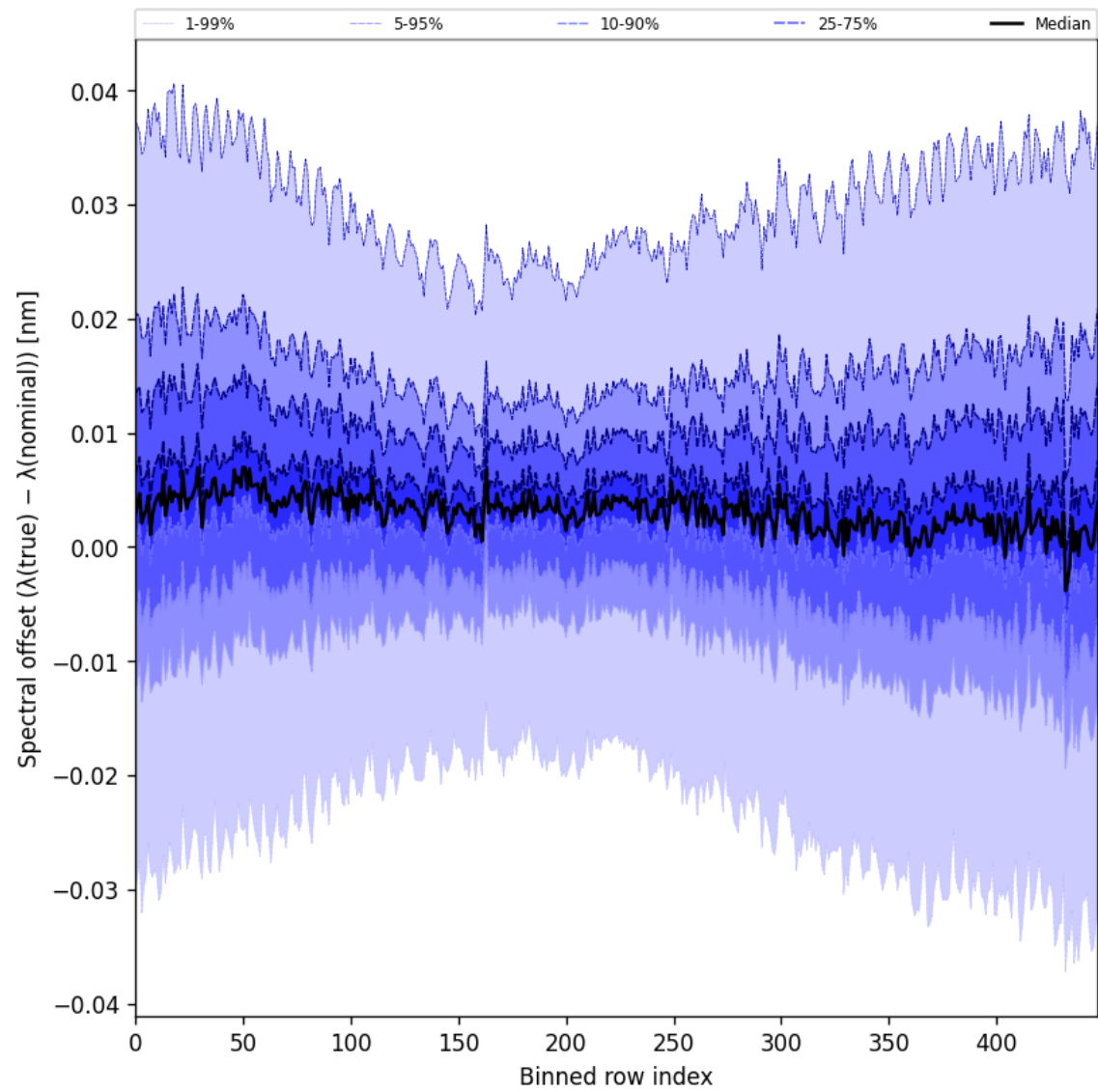
Figure 62: Along track statistics of “Spectral offset ( \lambda_{\text{true}} - \lambda_{\text{nominal}} )” for 2025-02-15 to 2025-02-17
