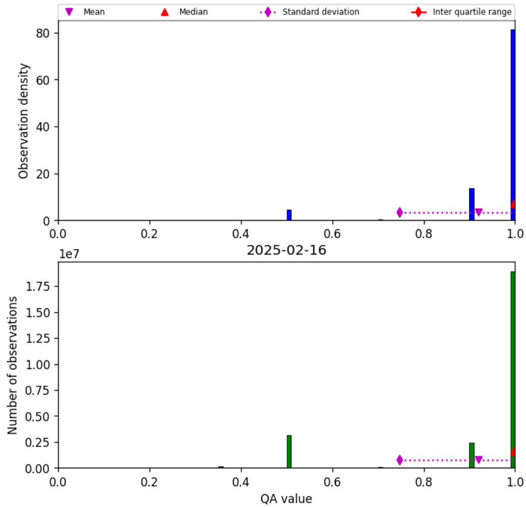
Figure 29: Histogram of “QA value” for 2025-02-15 to 2025-02-17
