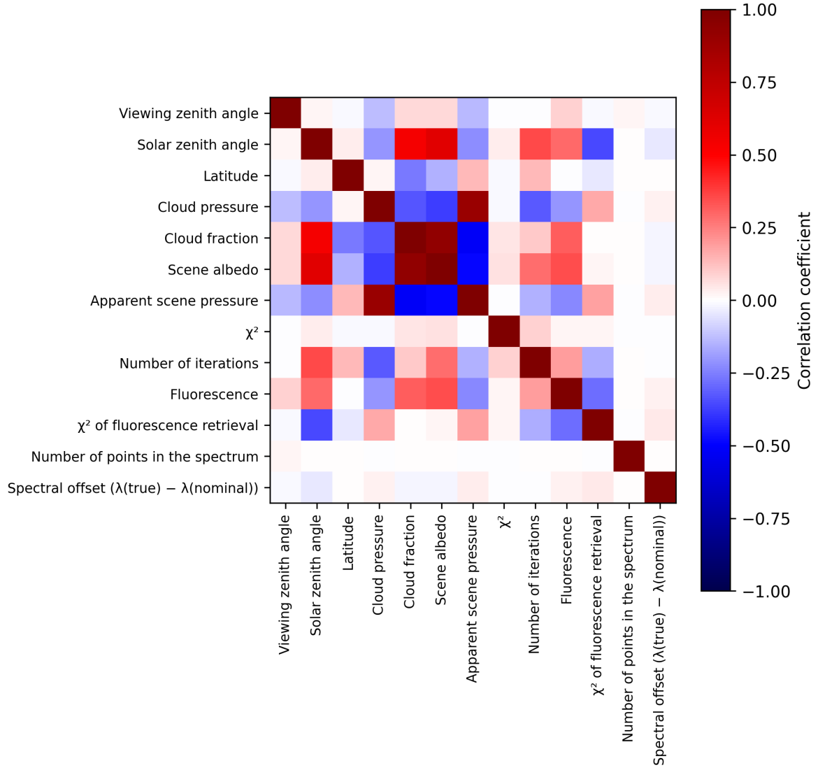
Figure 2: Map of correlation matrix for 2025-02-16 to 2025-02-18.
