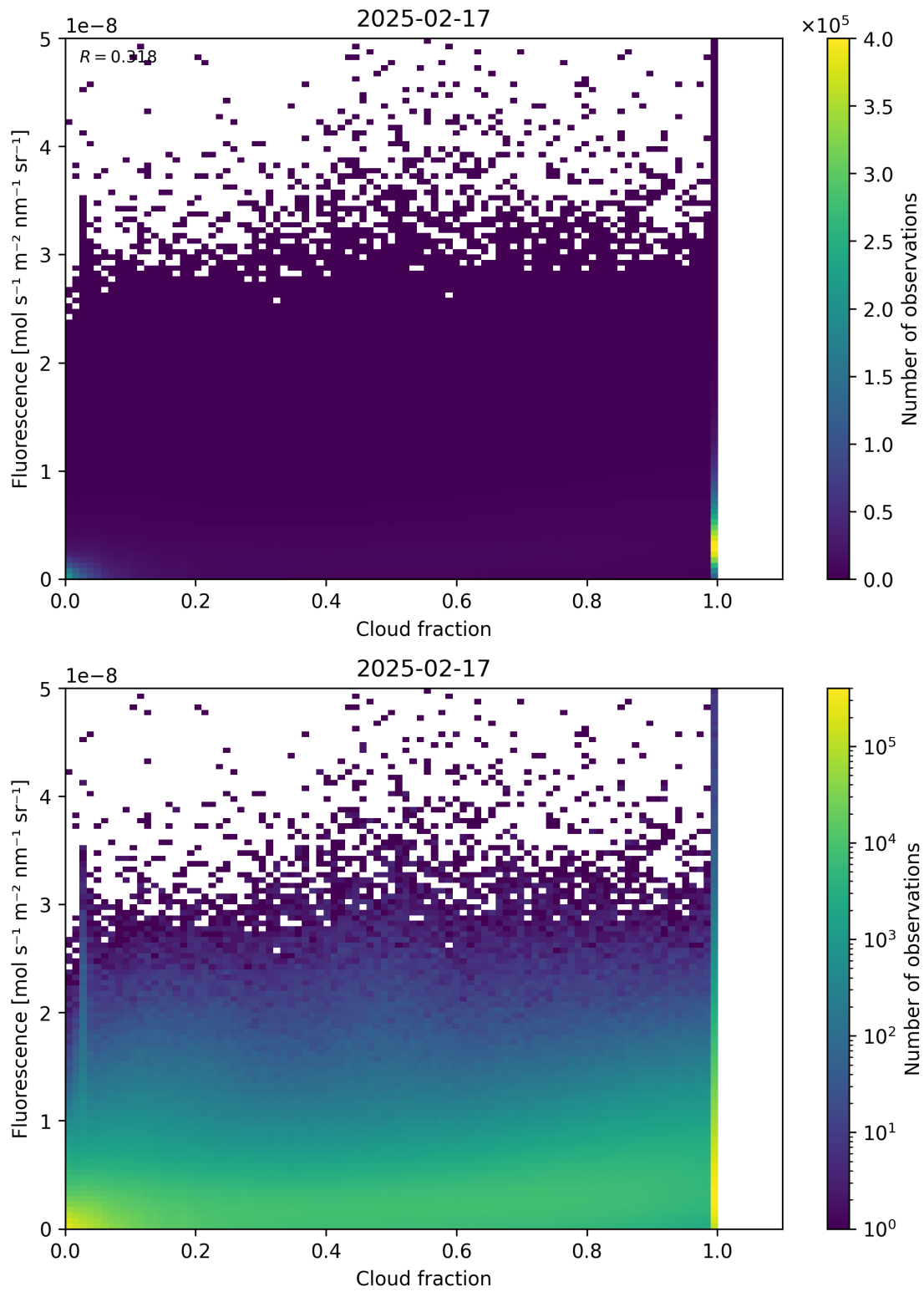
Figure 72: Scatter density plot of “Cloud fraction” against “Fluorescence” for 2025-02-16 to 2025-02-18.
