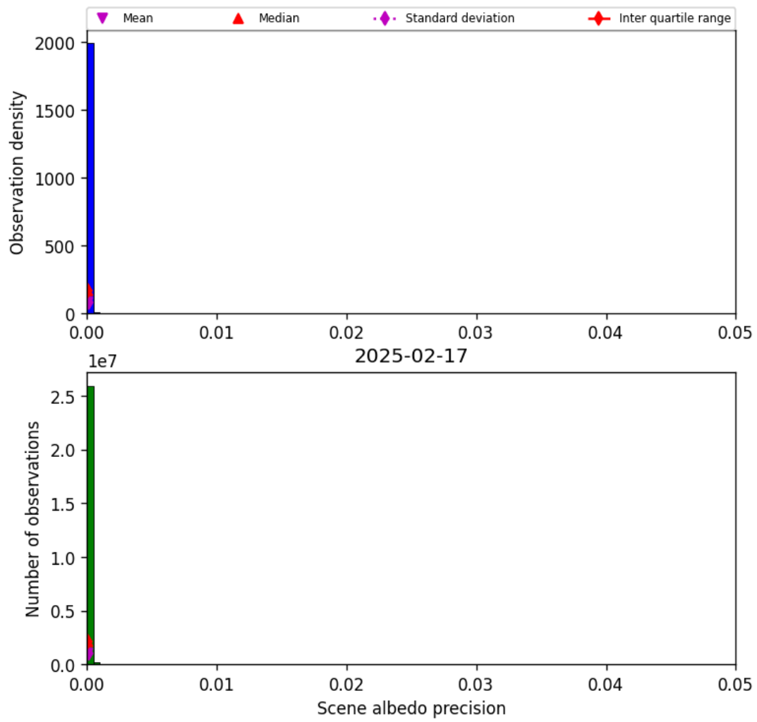
Figure 35: Histogram of “Scene albedo precision” for 2025-02-16 to 2025-02-18
