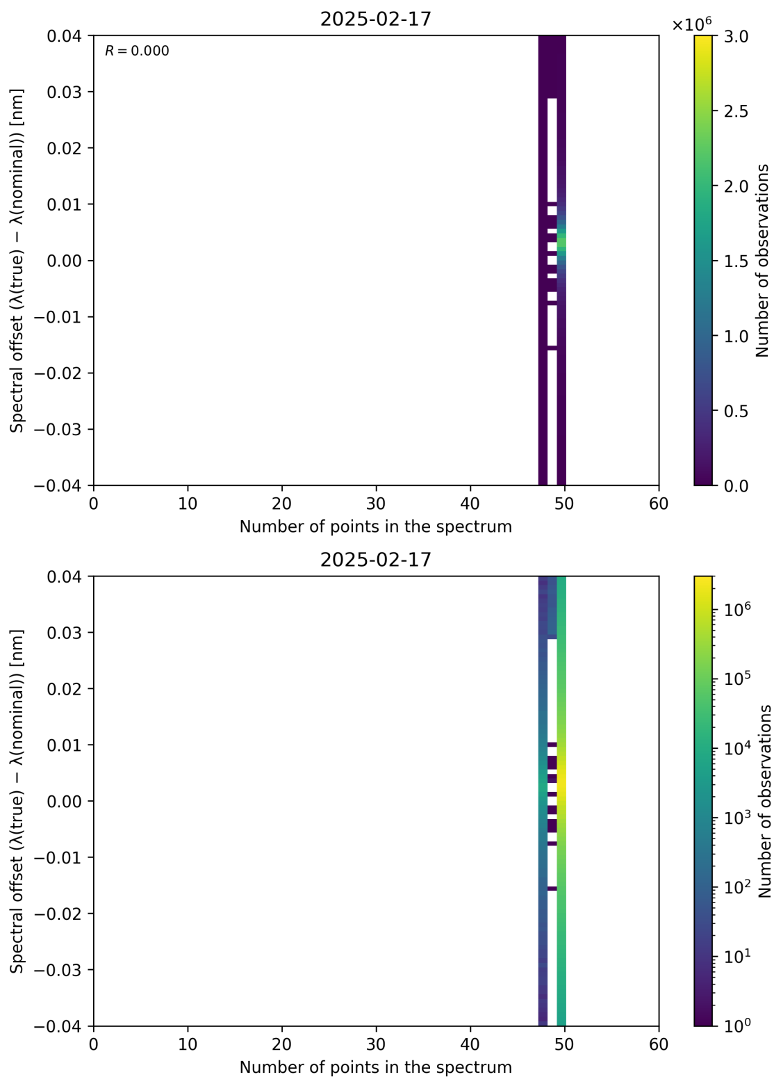
Figure 101: Scatter density plot of “Number of points in the spectrum” against “Spectral offset ( \lambda_{\text{true}} - \lambda_{\text{nominal}} )” for 2025-02-16 to 2025-02-18.
