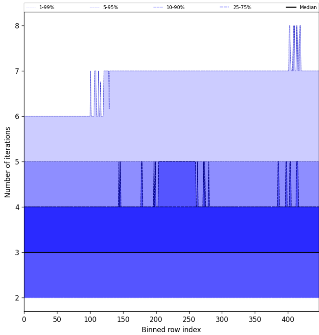
Figure 56: Along track statistics of “Number of iterations” for 2025-02-16 to 2025-02-18
