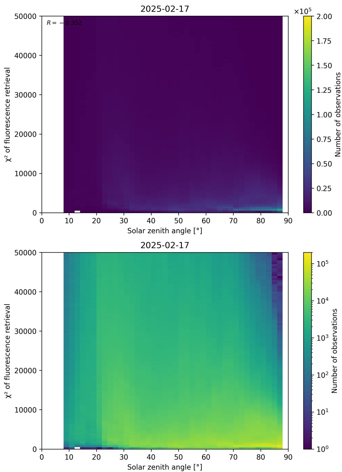
Figure 109: Scatter density plot of “Solar zenith angle” against “ \chi^2 of fluorescence retrieval” for 2025-02-16 to 2025-02-18.
