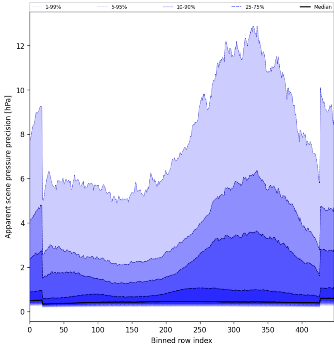
Figure 54: Along track statistics of “Apparent scene pressure precision” for 2025-02-16 to 2025-02-18
