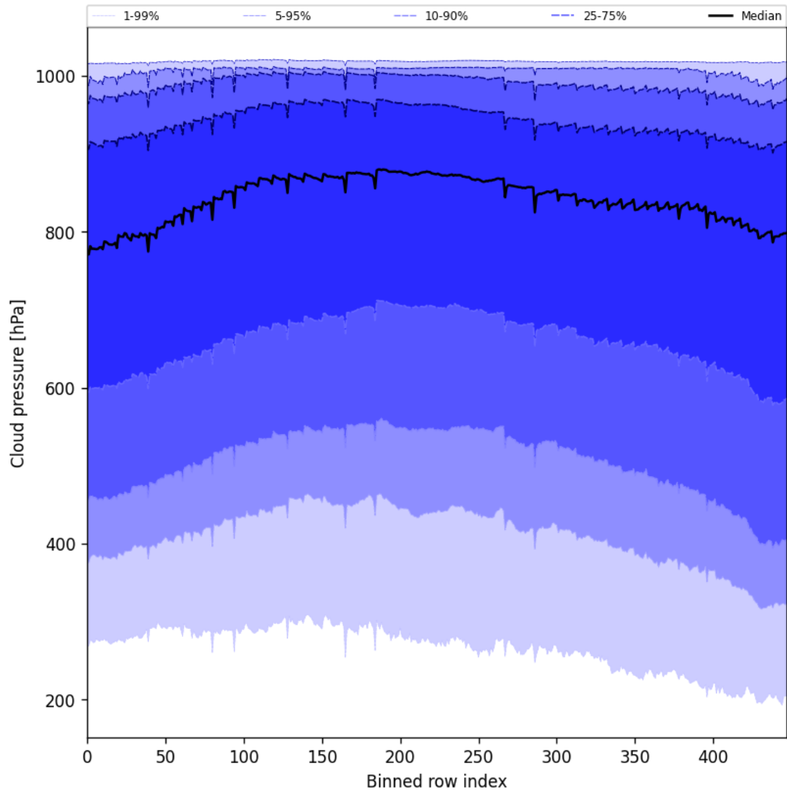
Figure 47: Along track statistics of “Cloud pressure” for 2025-02-16 to 2025-02-18
