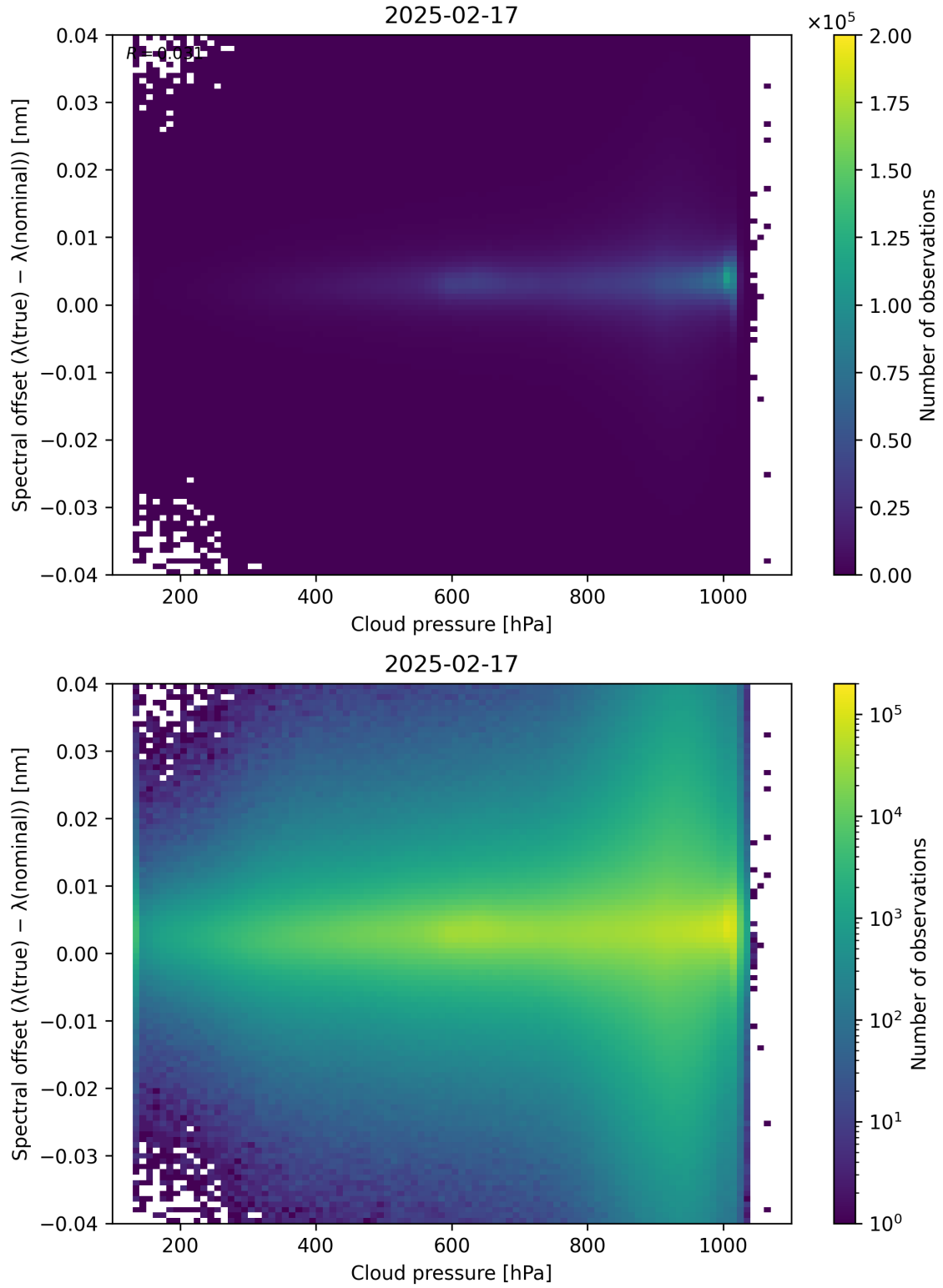
Figure 84: Scatter density plot of “Cloud pressure” against “Spectral offset ( \lambda_{\text{true}} - \lambda_{\text{nominal}} )” for 2025-02-16 to 2025-02-18.
