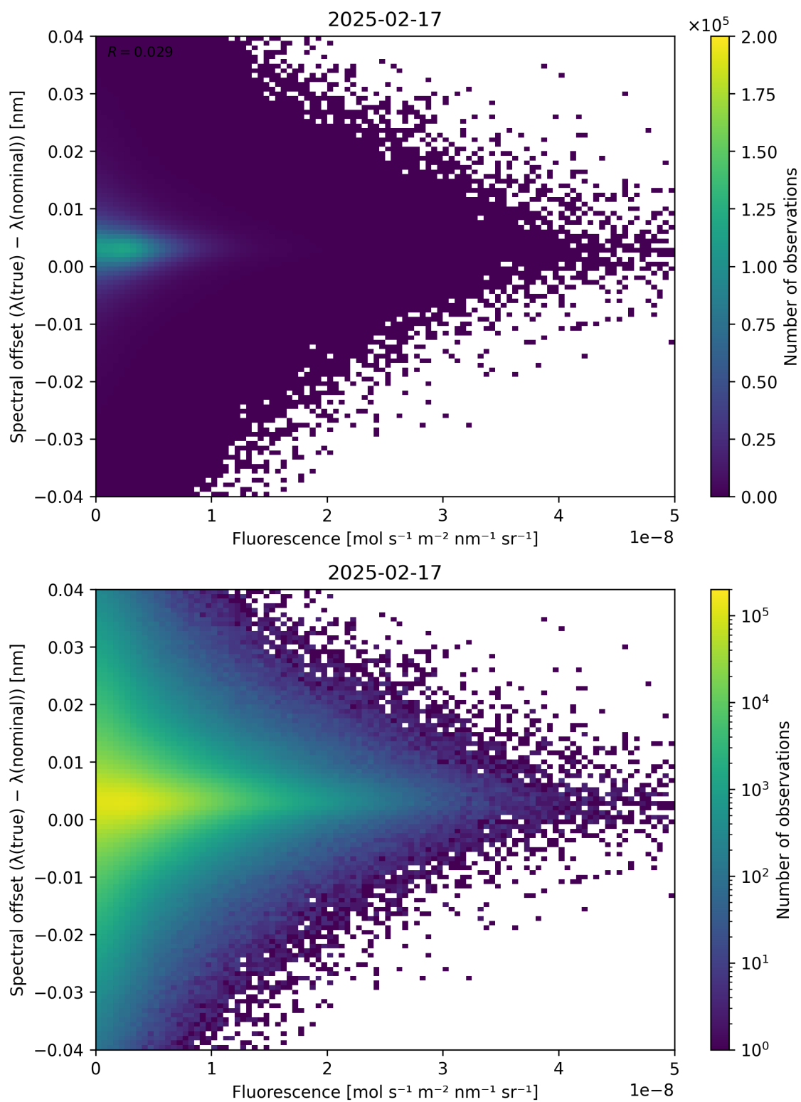
Figure 87: Scatter density plot of “Fluorescence” against “Spectral offset ( \lambda_{\text{true}} - \lambda_{\text{nominal}} )” for 2025-02-16 to 2025-02-18.
