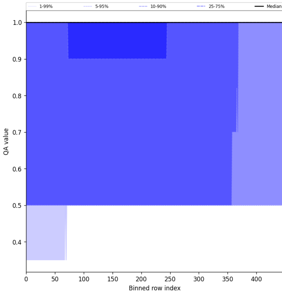
Figure 46: Along track statistics of “QA value” for 2025-02-16 to 2025-02-18
