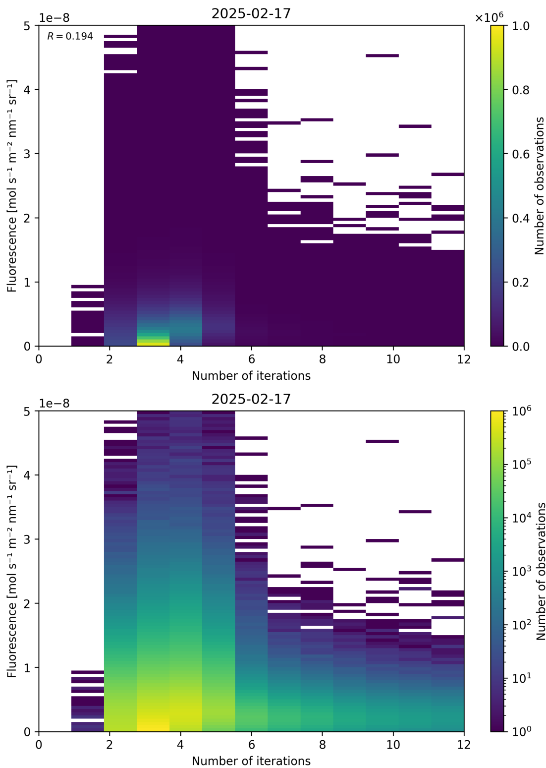
Figure 98: Scatter density plot of “Number of iterations” against “Fluorescence” for 2025-02-16 to 2025-02-18.
