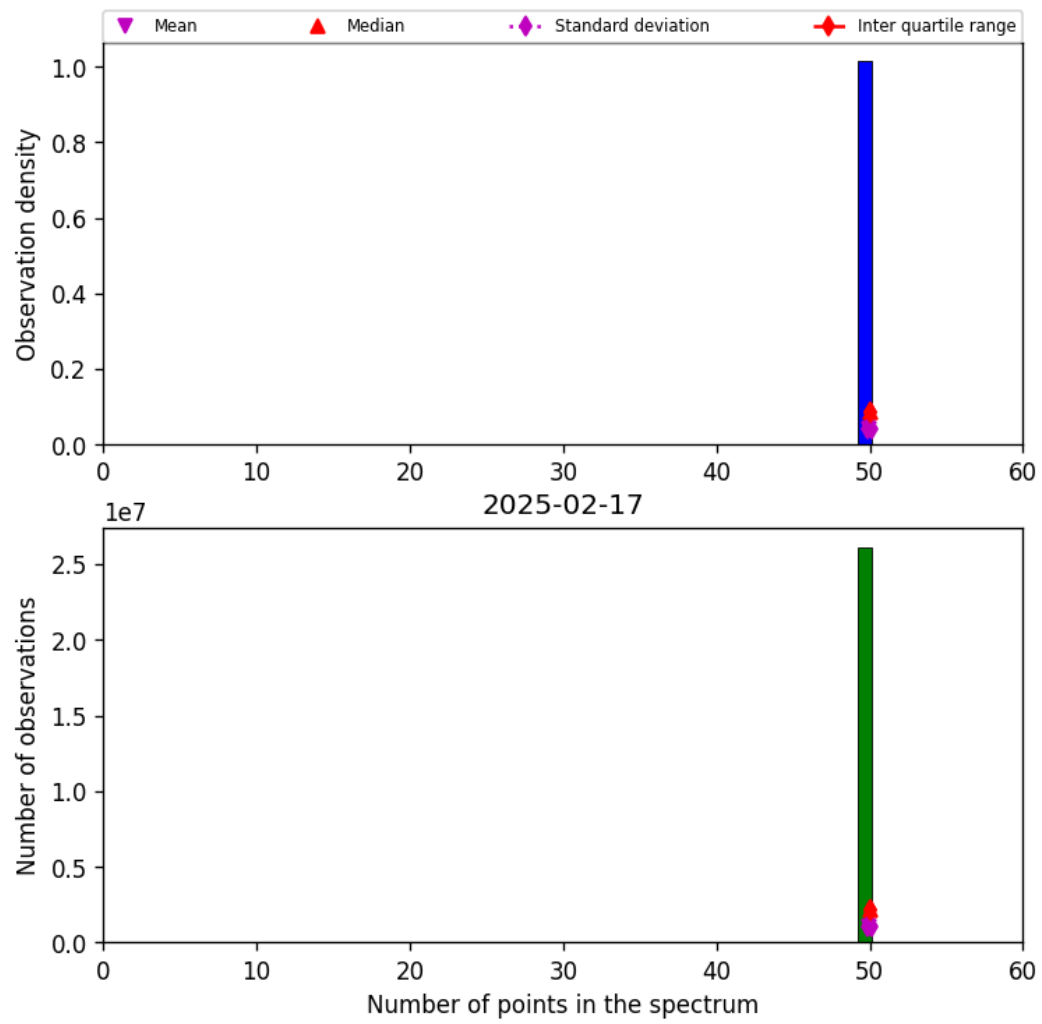
Figure 44: Histogram of "Number of points in the spectrum" for 2025-02-16 to 2025-02-18
