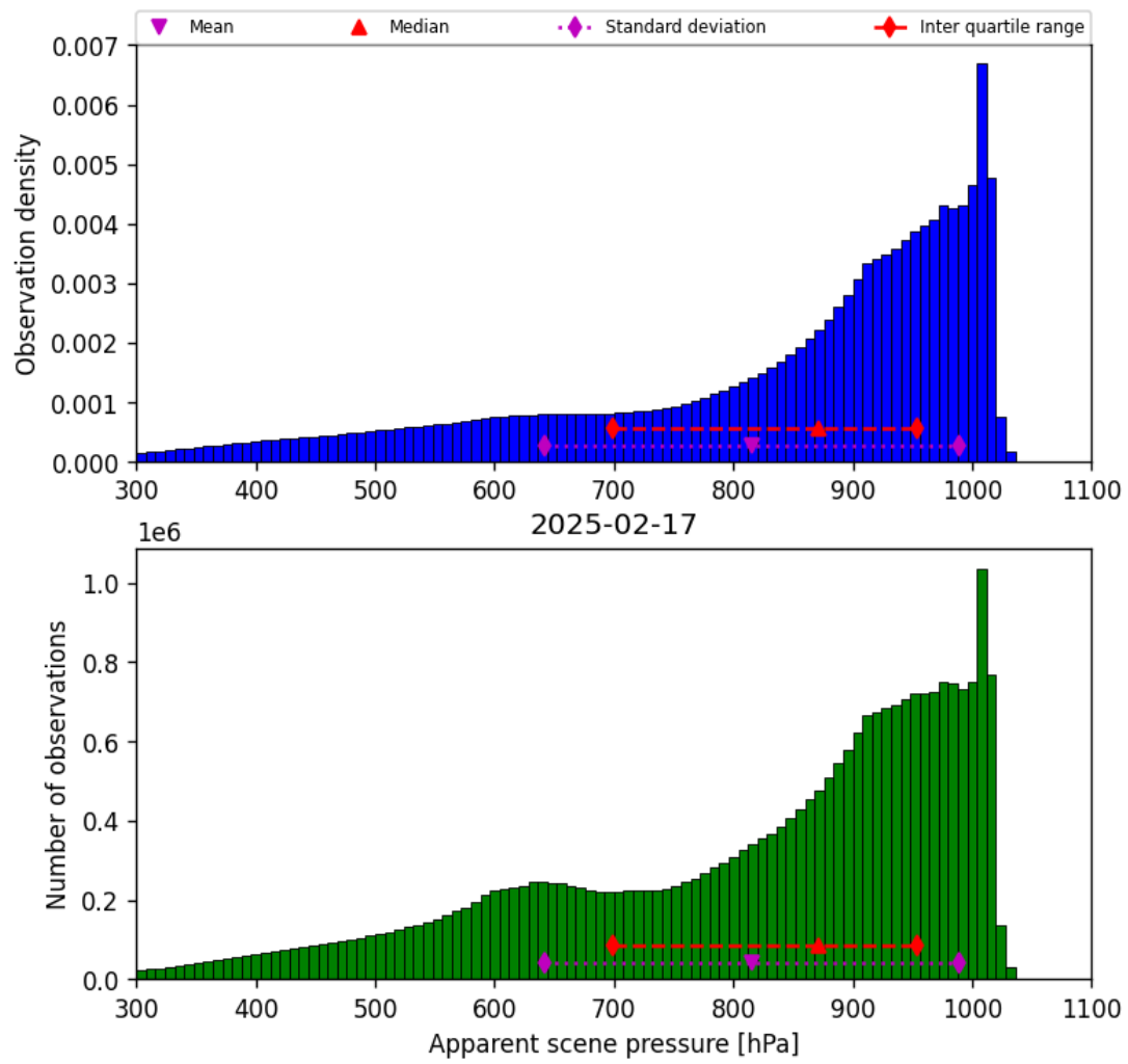
Figure 36: Histogram of “Apparent scene pressure” for 2025-02-16 to 2025-02-18
