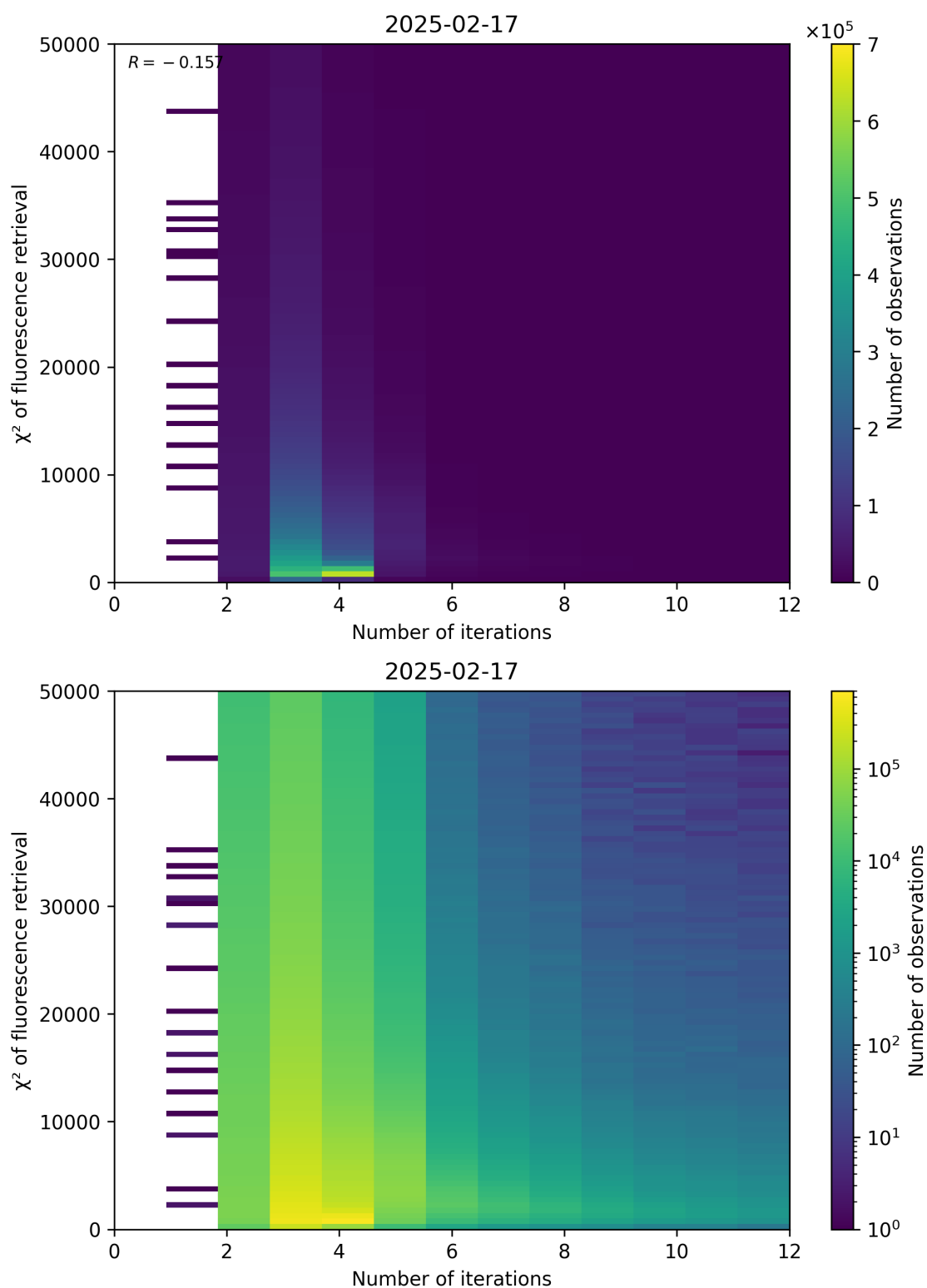
Figure 97: Scatter density plot of “Number of iterations” against “ \chi^2 of fluorescence retrieval” for 2025-02-16 to 2025-02-18.
