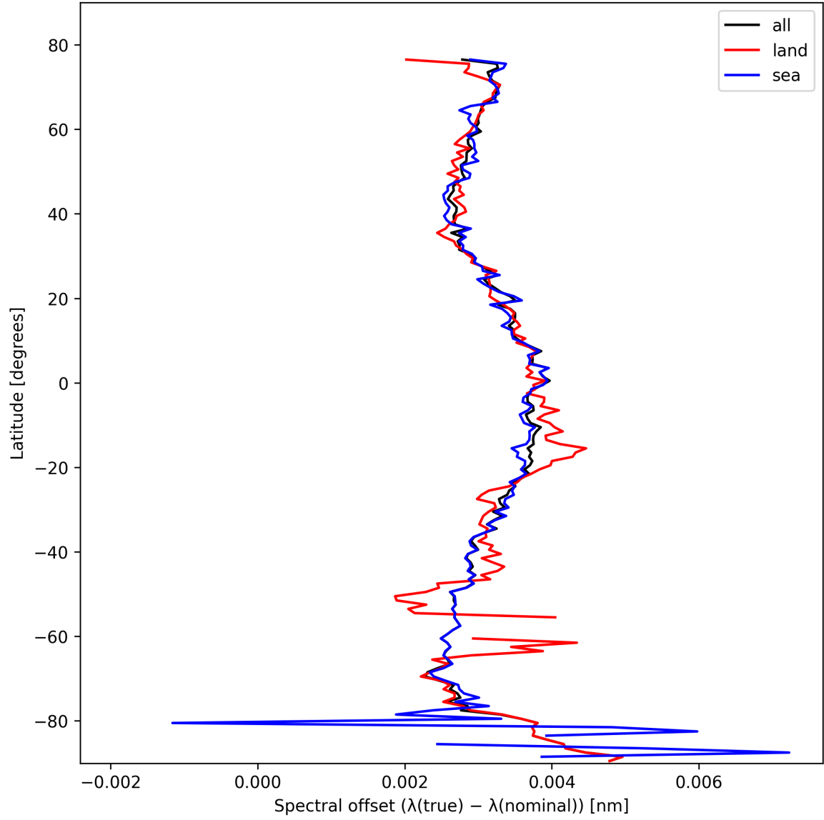
Figure 28: Zonal average of “Spectral offset ( \lambda_{\text{true}} - \lambda_{\text{nominal}} )” for 2025-02-16 to 2025-02-18.
