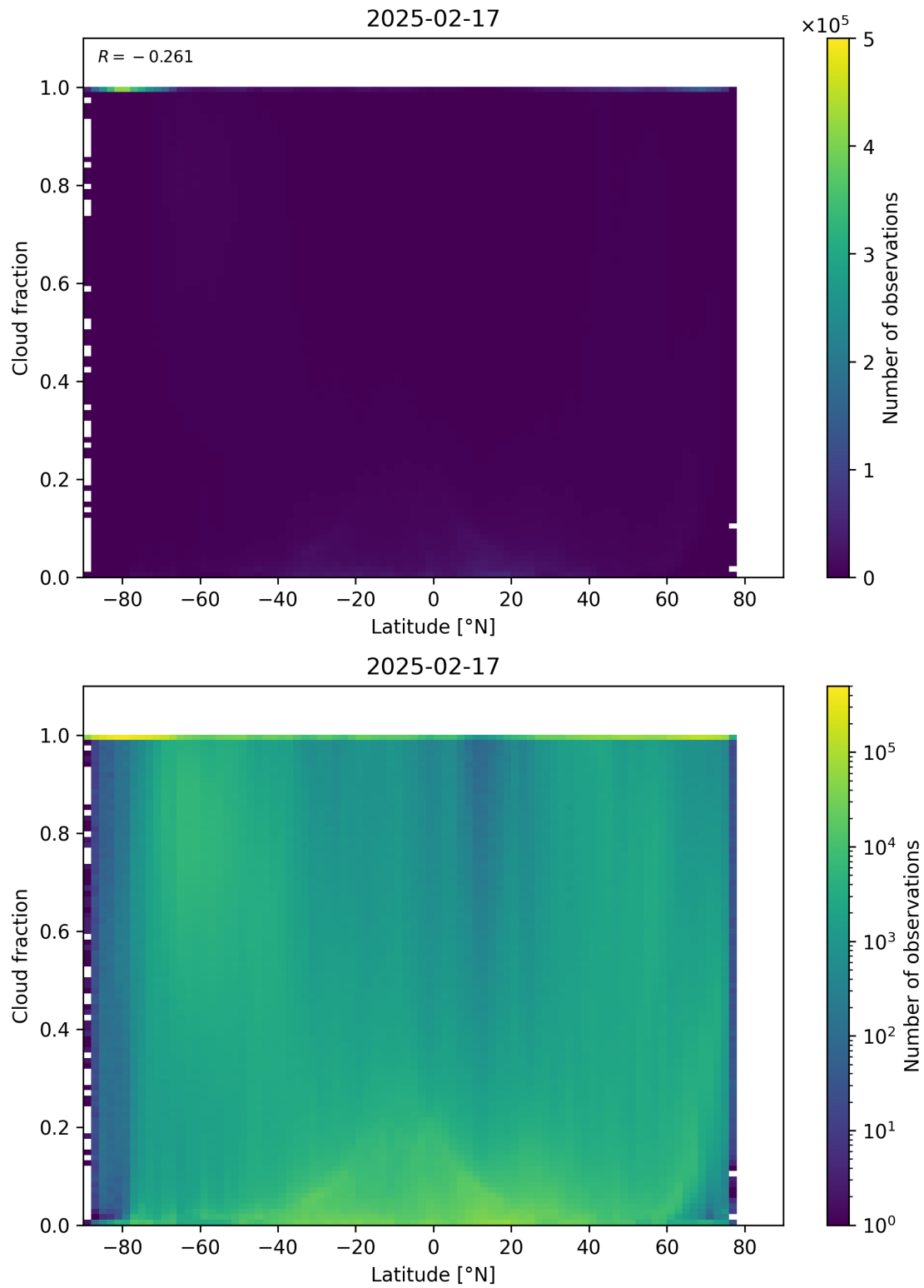
Figure 90: Scatter density plot of “Latitude” against “Cloud fraction” for 2025-02-16 to 2025-02-18.
