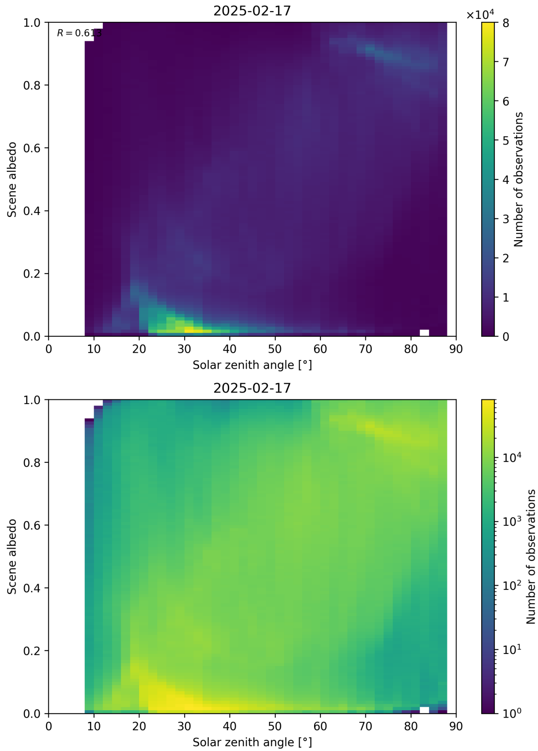
Figure 116: Scatter density plot of “Solar zenith angle” against “Scene albedo” for 2025-02-16 to 2025-02-18.
