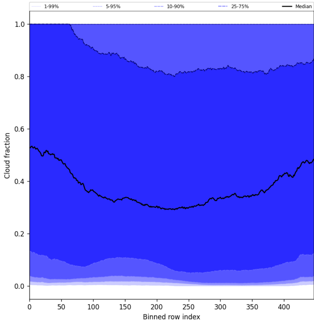
Figure 49: Along track statistics of “Cloud fraction” for 2025-02-16 to 2025-02-18
