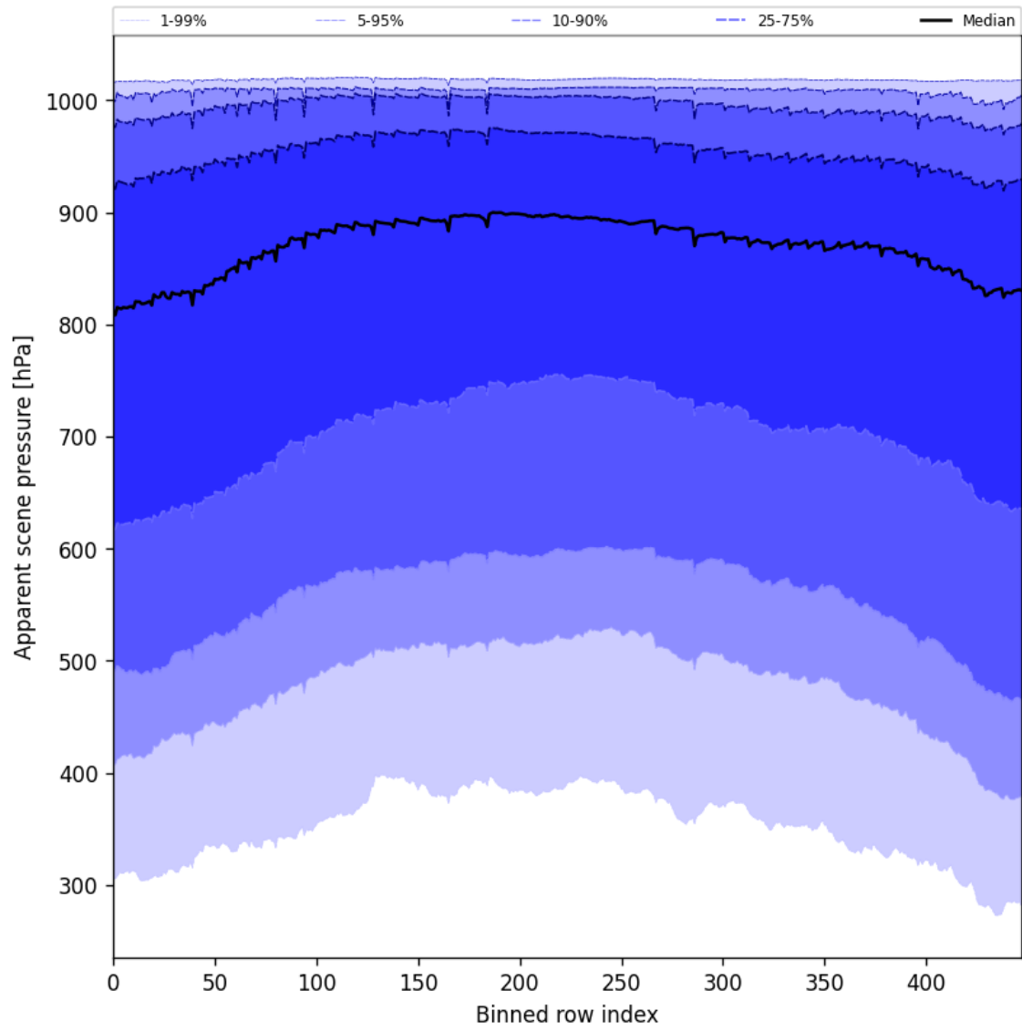
Figure 53: Along track statistics of “Apparent scene pressure” for 2025-02-16 to 2025-02-18
