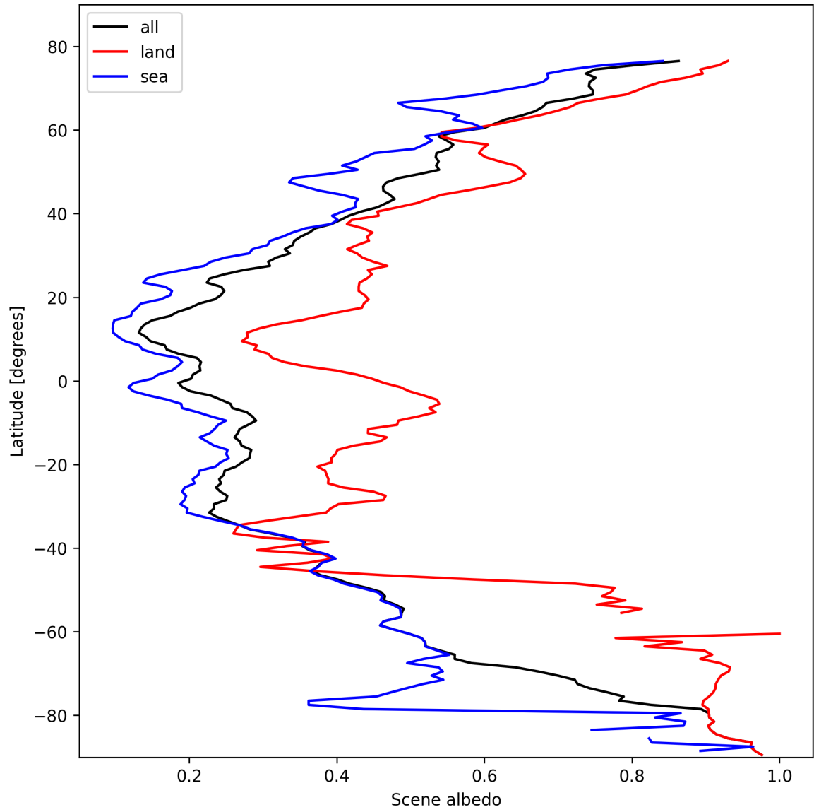
Figure 17: Zonal average of “Scene albedo” for 2025-02-16 to 2025-02-18.
