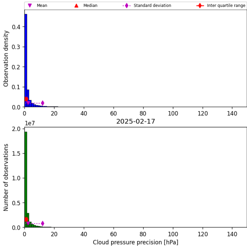
Figure 31: Histogram of “Cloud pressure precision” for 2025-02-16 to 2025-02-18
