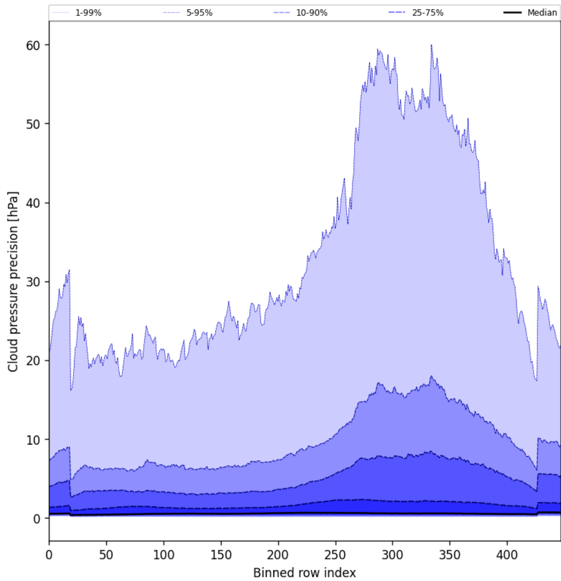
Figure 48: Along track statistics of “Cloud pressure precision” for 2025-02-16 to 2025-02-18
