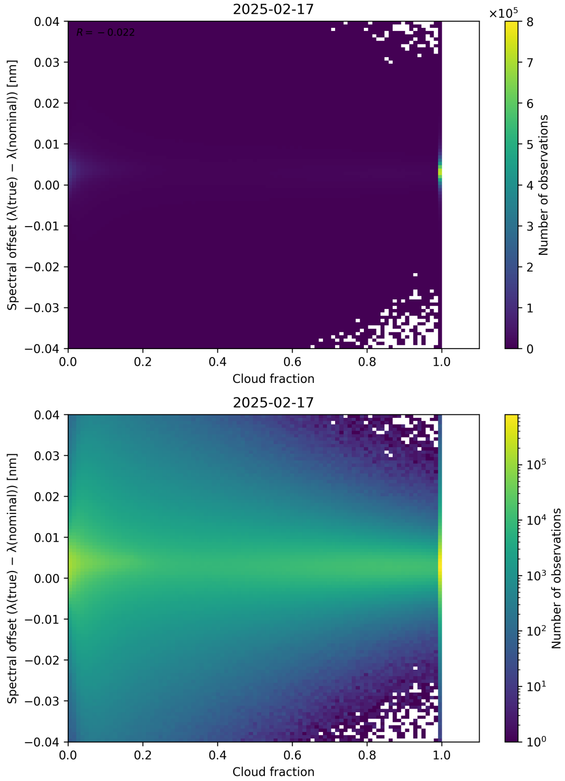
Figure 76: Scatter density plot of “Cloud fraction” against “Spectral offset ( \lambda_{\text{true}} - \lambda_{\text{nominal}} )” for 2025-02-16 to 2025-02-18.
