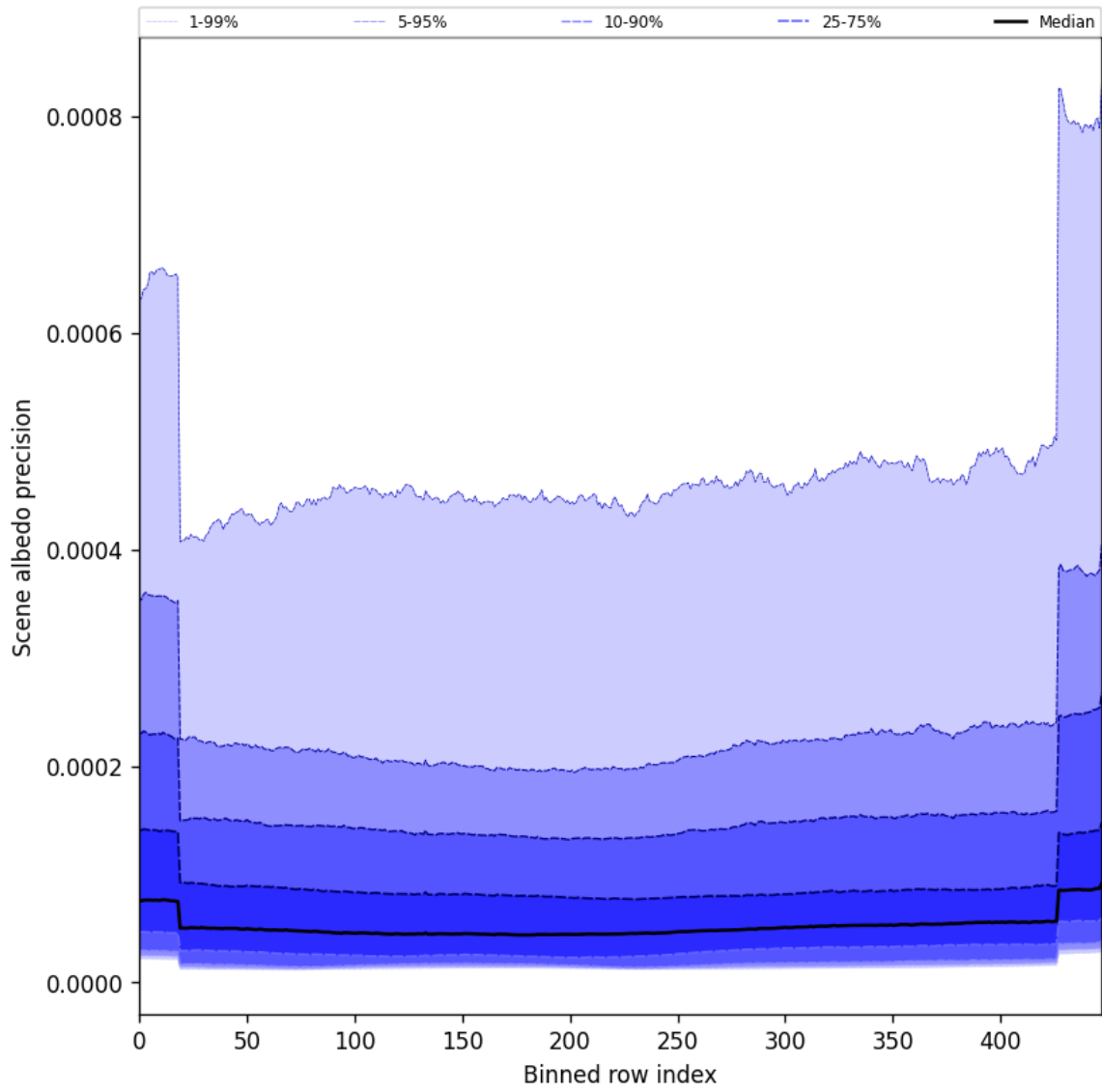
Figure 52: Along track statistics of “Scene albedo precision” for 2025-02-16 to 2025-02-18
