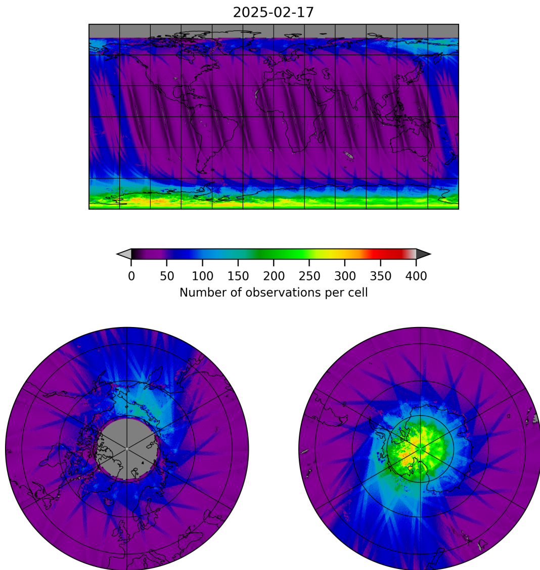
Figure 11: Map of the number of observations for 2025-02-16 to 2025-02-18
