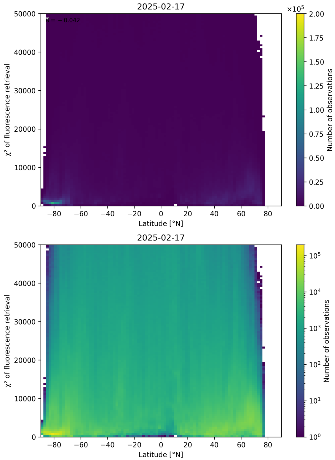
Figure 89: Scatter density plot of “Latitude” against “ \chi^2 of fluorescence retrieval” for 2025-02-16 to 2025-02-18.
