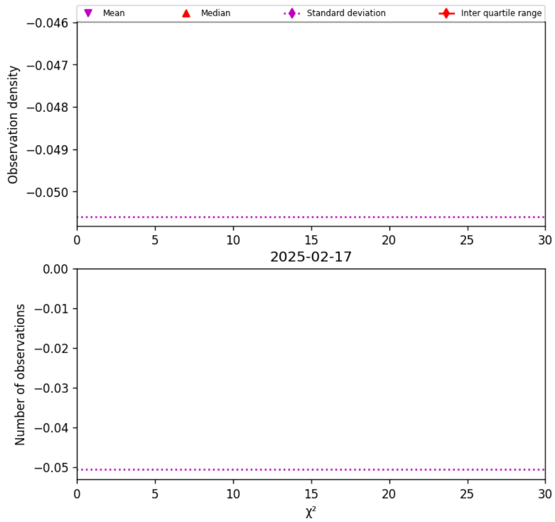
Figure 38: Histogram of " \chi^2 " for 2025-02-16 to 2025-02-18
