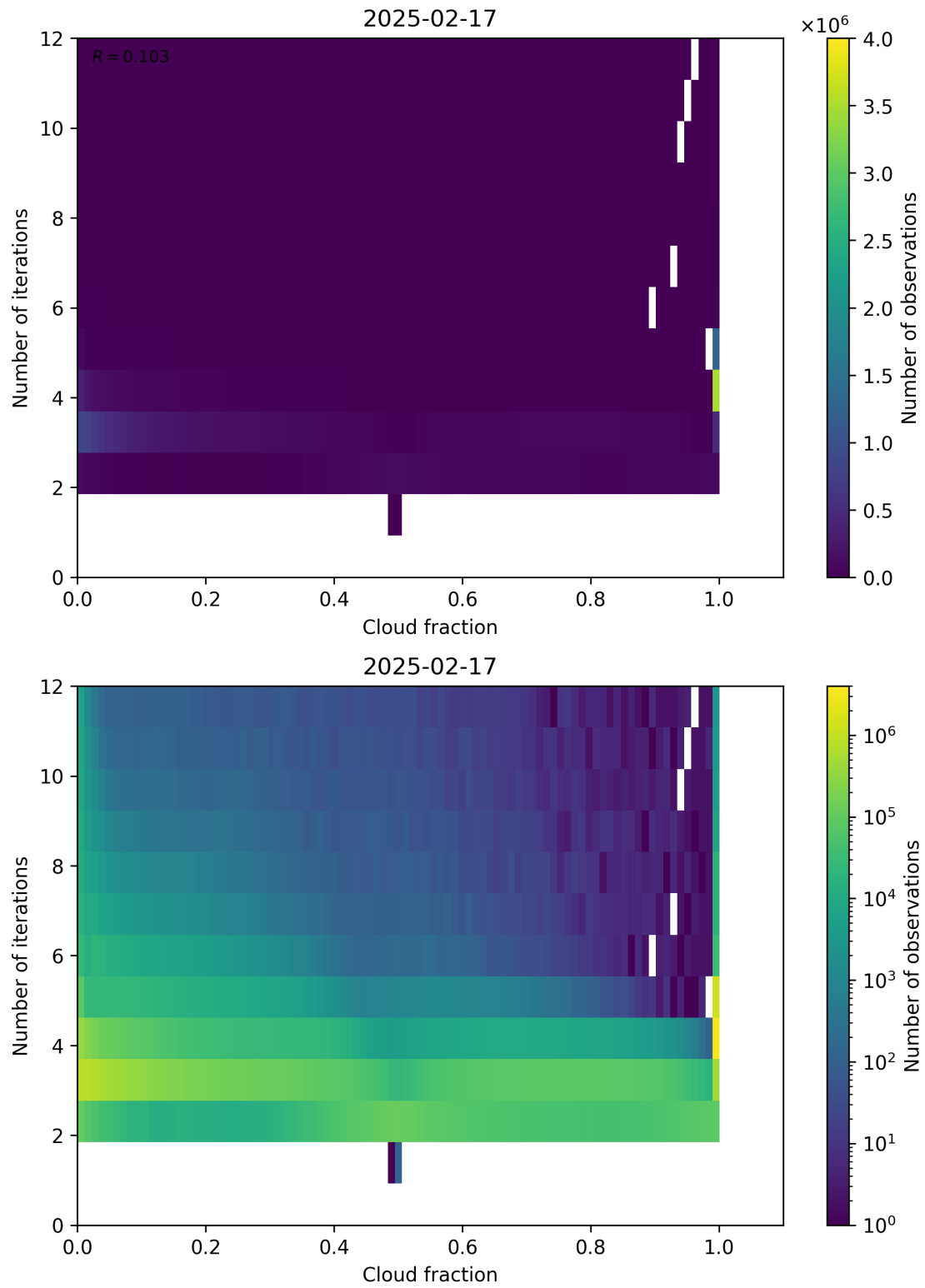
Figure 73: Scatter density plot of “Cloud fraction” against “Number of iterations” for 2025-02-16 to 2025-02-18.
