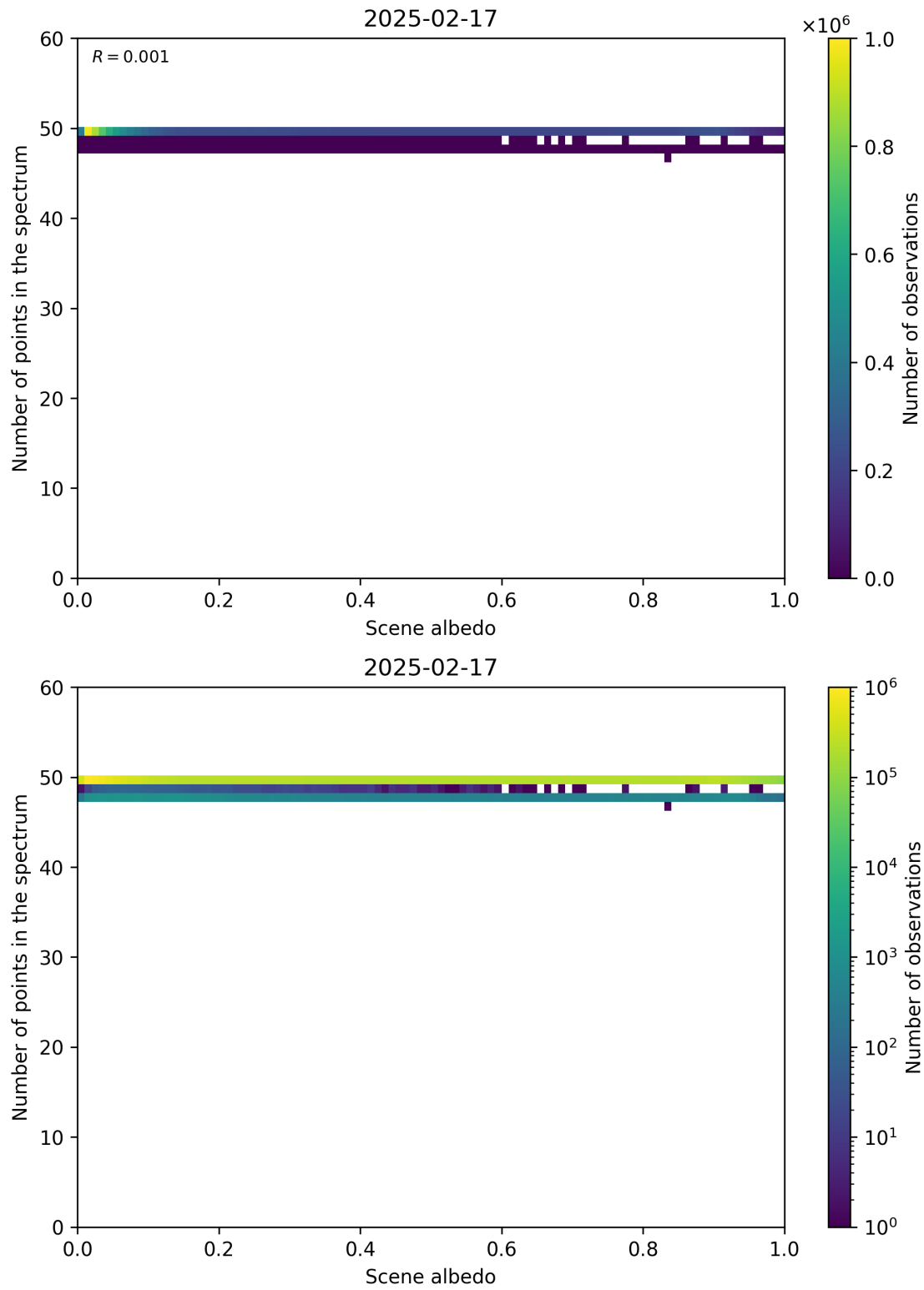
Figure 106: Scatter density plot of “Scene albedo” against “Number of points in the spectrum” for 2025-02-16 to 2025-02-18.
