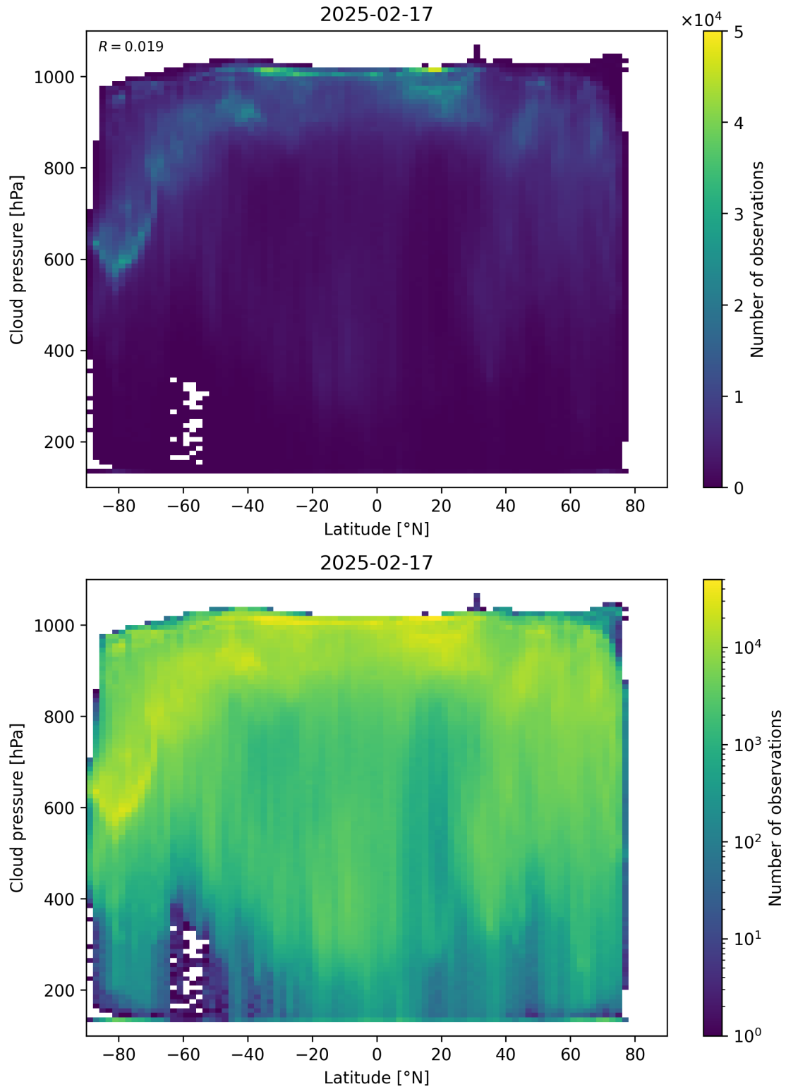
Figure 91: Scatter density plot of “Latitude” against “Cloud pressure” for 2025-02-16 to 2025-02-18.
