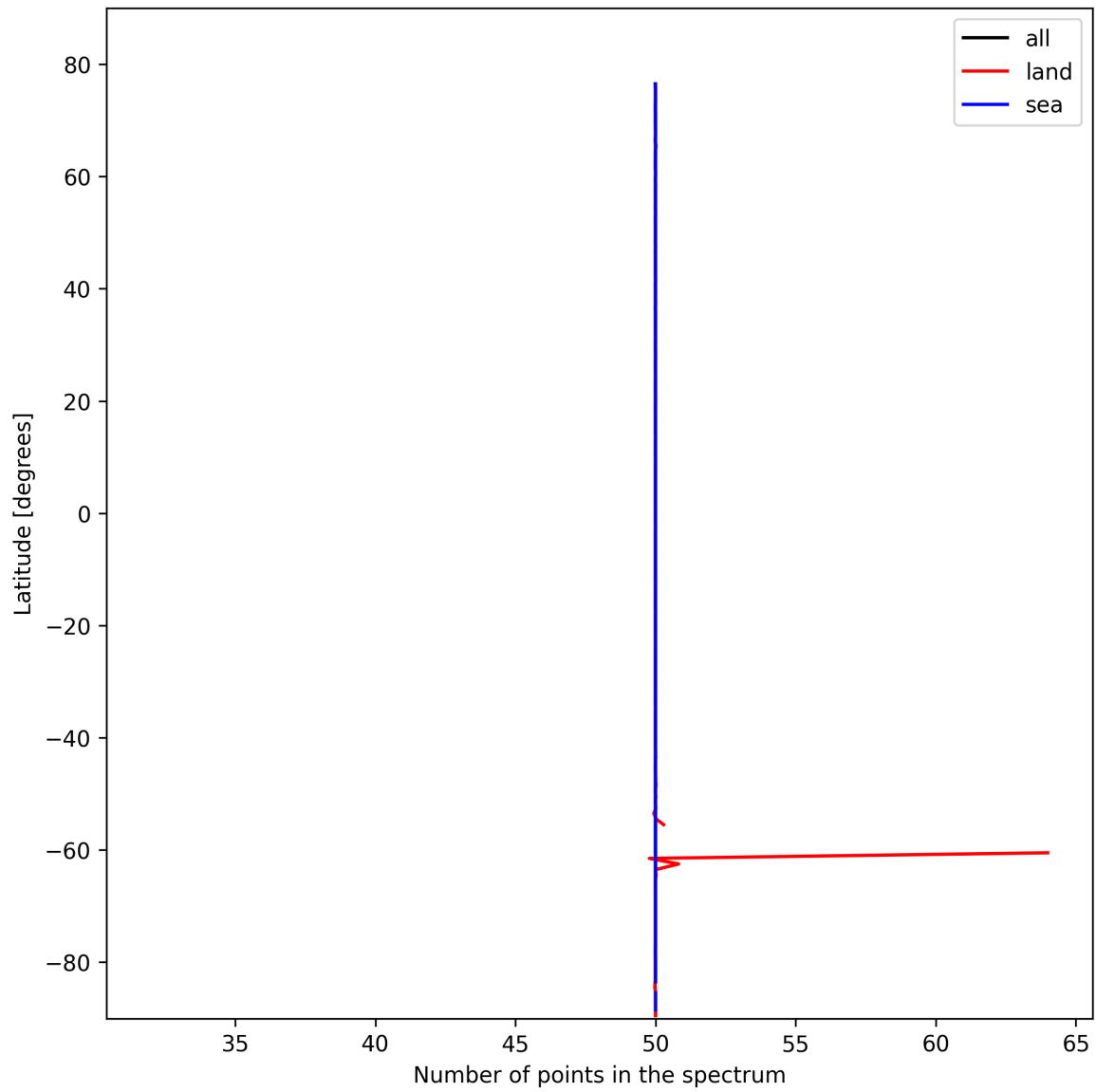
Figure 27: Zonal average of “Number of points in the spectrum” for 2025-02-16 to 2025-02-18.
