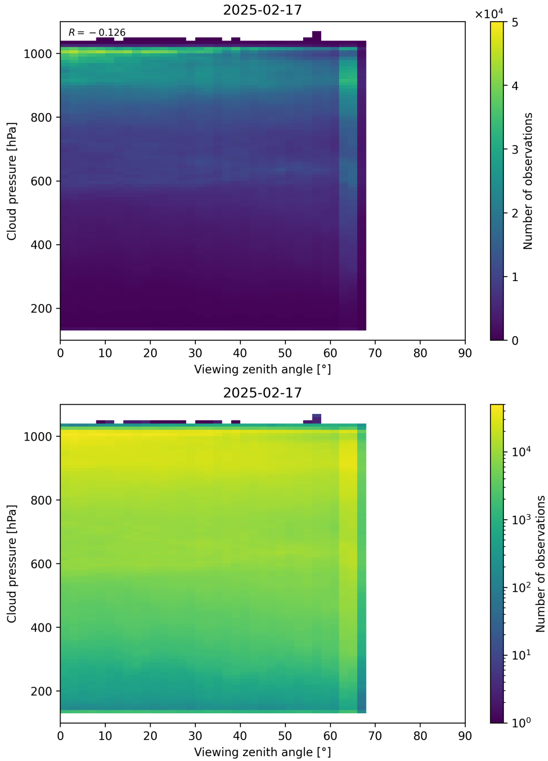
Figure 121: Scatter density plot of “Viewing zenith angle” against “Cloud pressure” for 2025-02-16 to 2025-02-18.
