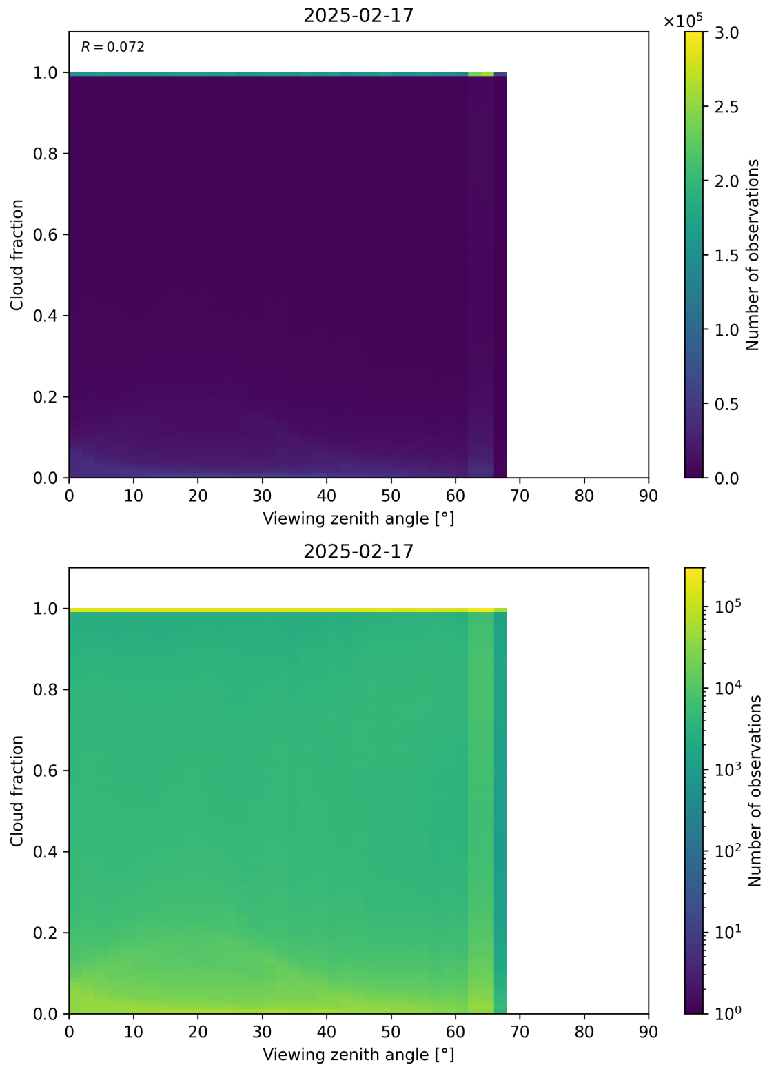
Figure 120: Scatter density plot of “Viewing zenith angle” against “Cloud fraction” for 2025-02-16 to 2025-02-18.
