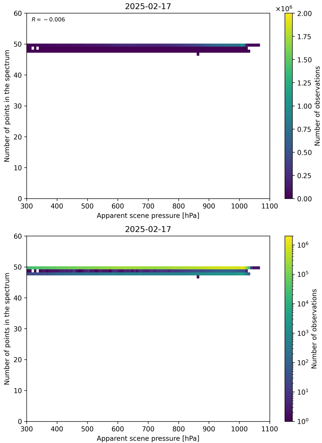
Figure 66: Scatter density plot of “Apparent scene pressure” against “Number of points in the spectrum” for 2025-02-16 to 2025-02-18.
