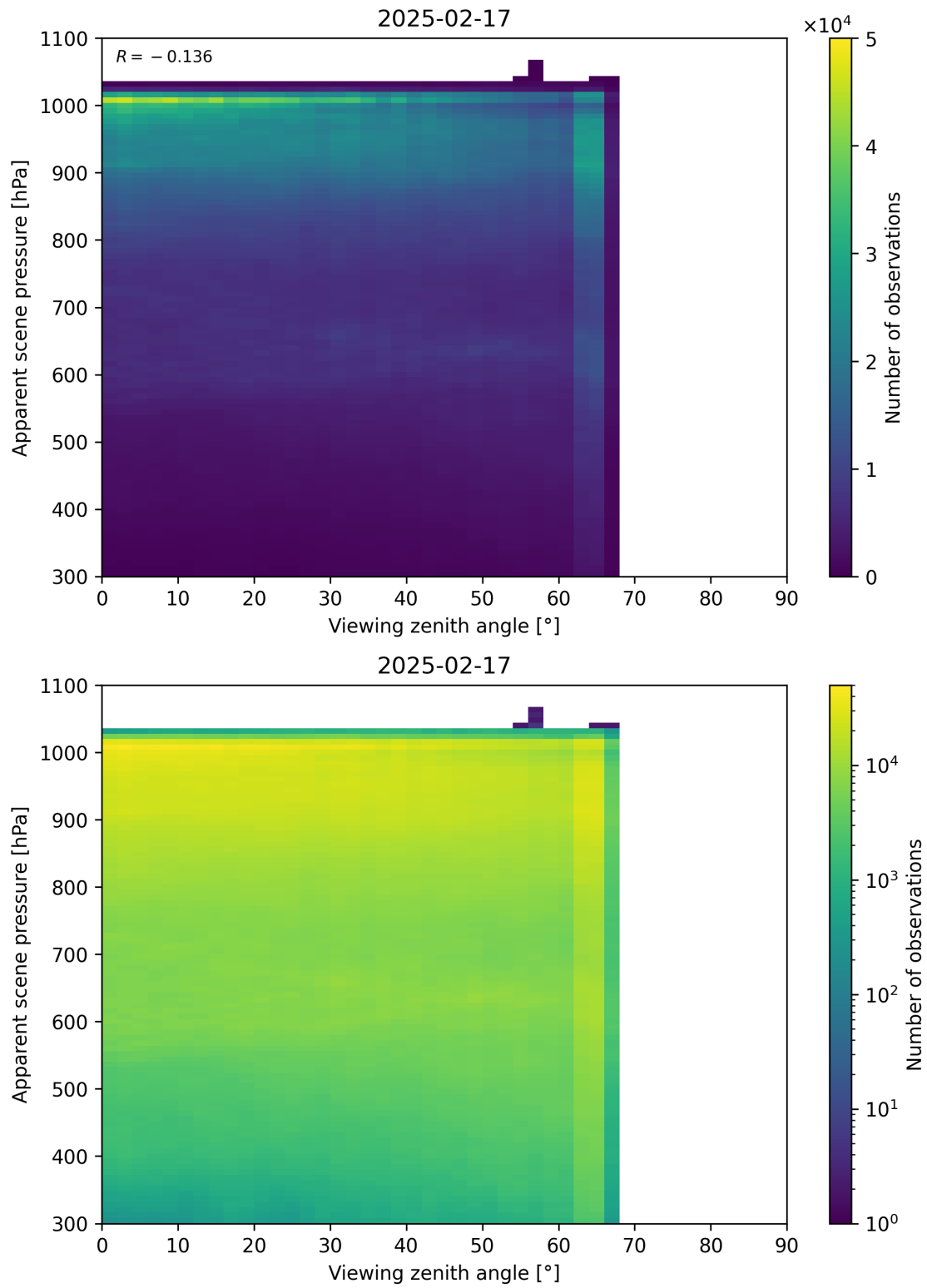
Figure 118: Scatter density plot of “Viewing zenith angle” against “Apparent scene pressure” for 2025-02-16 to 2025-02-18.
