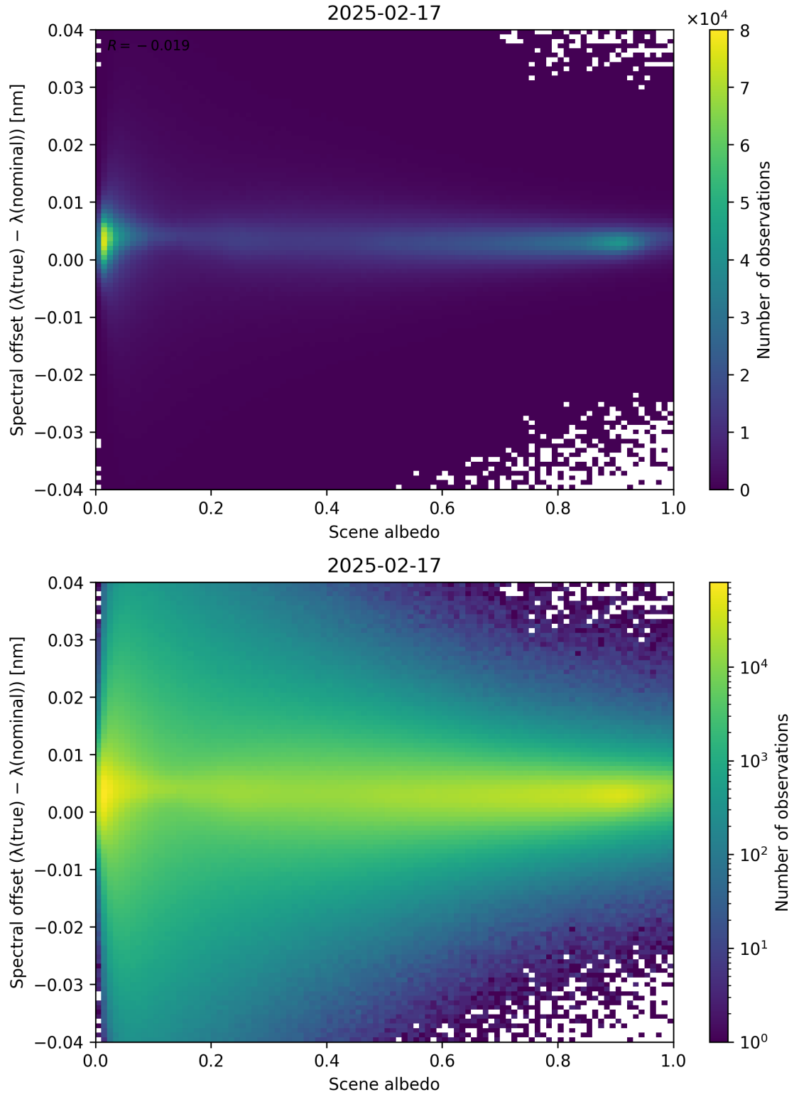
Figure 107: Scatter density plot of “Scene albedo” against “Spectral offset ( \lambda_{\text{true}} - \lambda_{\text{nominal}} )” for 2025-02-16 to 2025-02-18.
