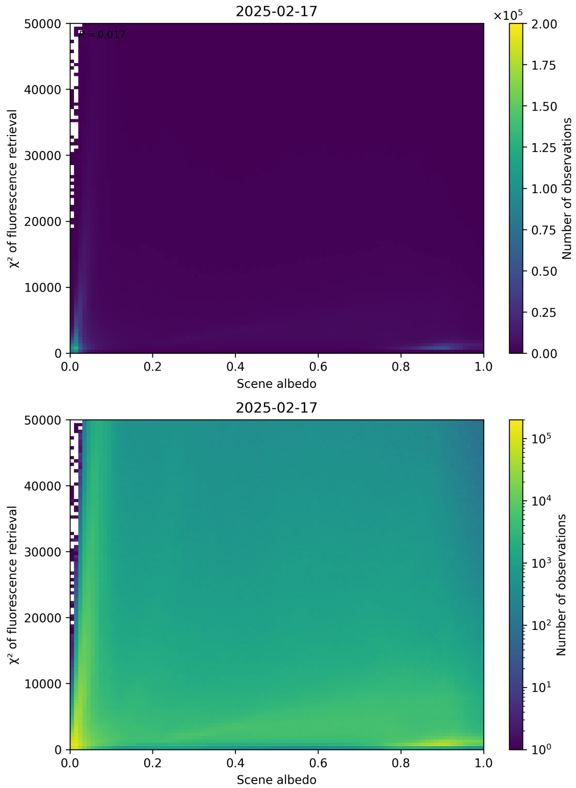
Figure 103: Scatter density plot of “Scene albedo” against “ \chi^2 of fluorescence retrieval” for 2025-02-16 to 2025-02-18.
