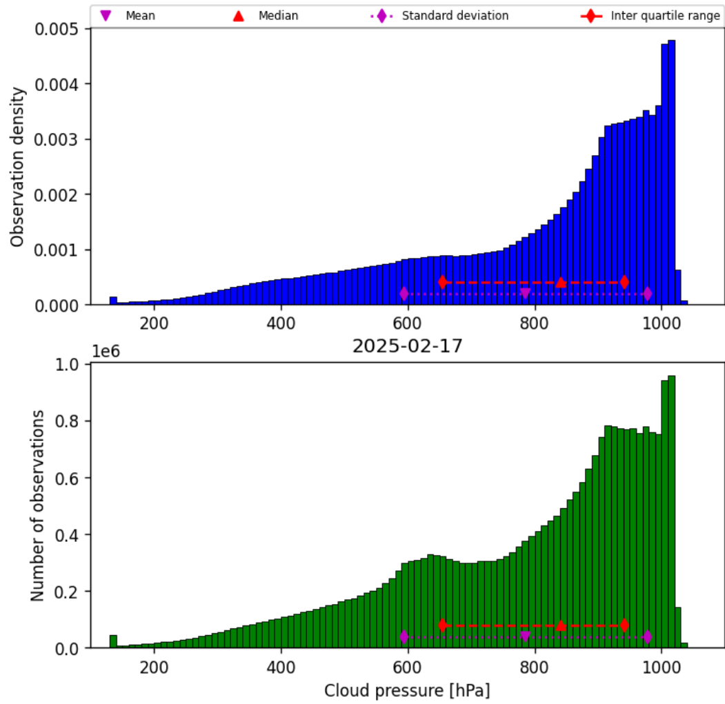
Figure 30: Histogram of “Cloud pressure” for 2025-02-16 to 2025-02-18
