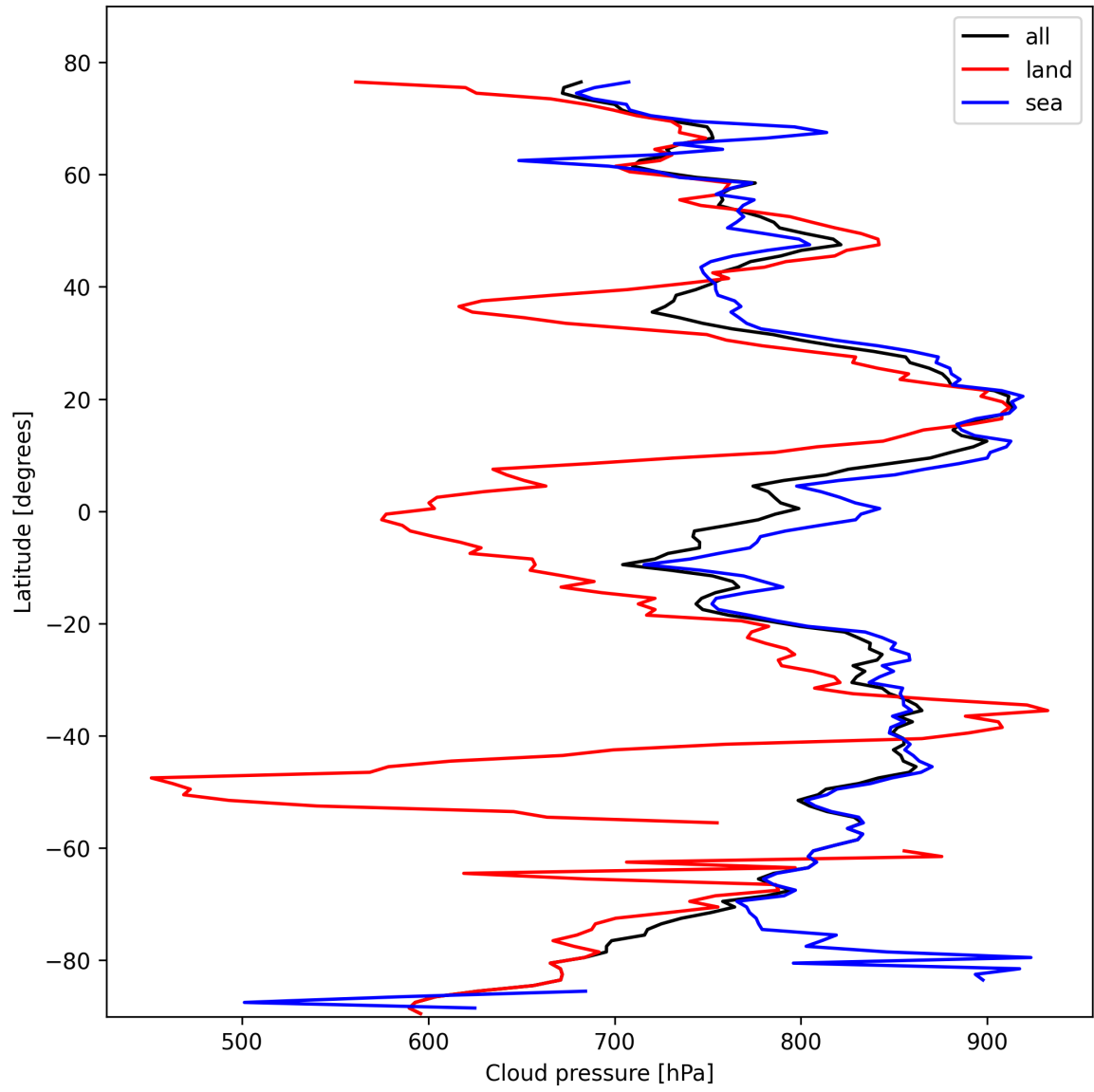
Figure 13: Zonal average of “Cloud pressure” for 2025-02-16 to 2025-02-18.
