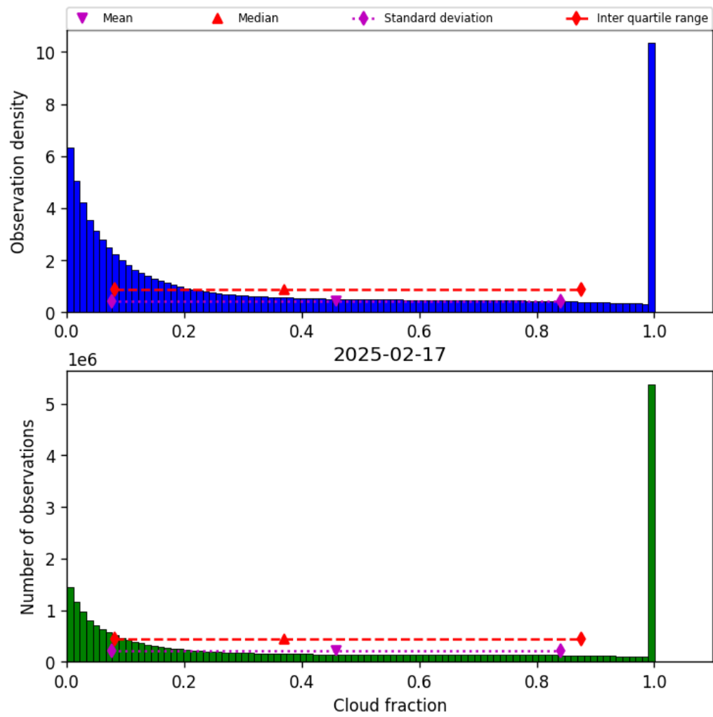
Figure 32: Histogram of “Cloud fraction” for 2025-02-16 to 2025-02-18
