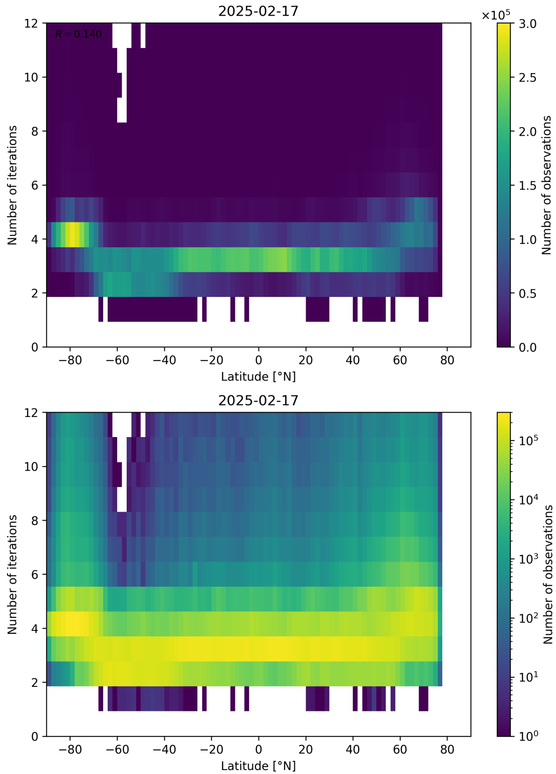
Figure 93: Scatter density plot of “Latitude” against “Number of iterations” for 2025-02-16 to 2025-02-18.
