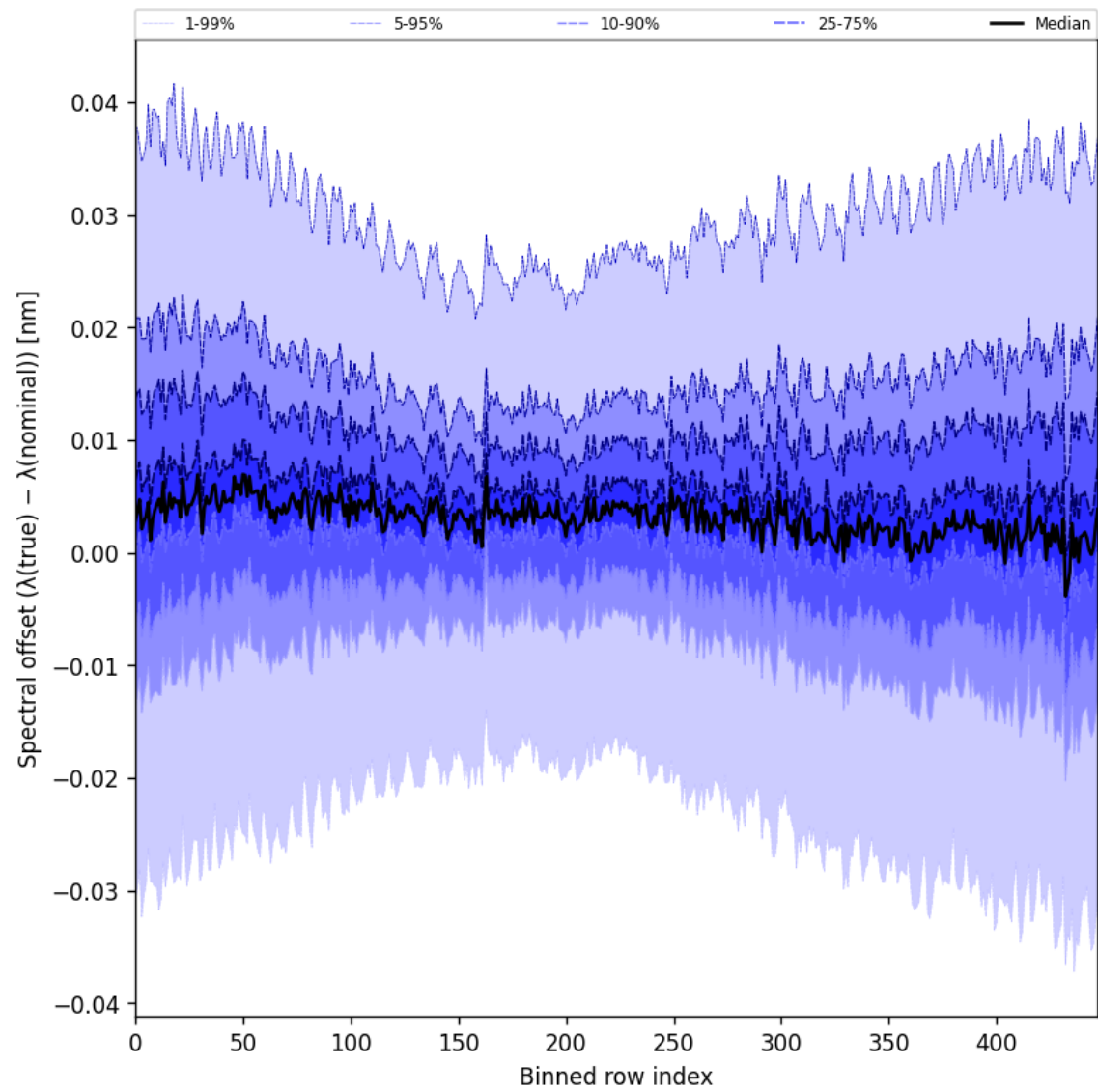
Figure 62: Along track statistics of “Spectral offset ( \lambda_{\text{true}} - \lambda_{\text{nominal}} )” for 2025-02-16 to 2025-02-18
