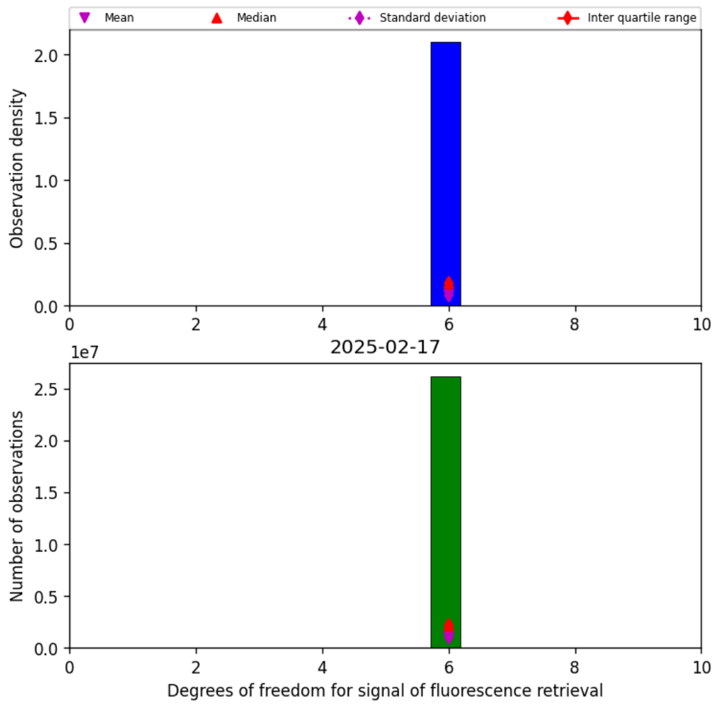
Figure 43: Histogram of “Degrees of freedom for signal of fluorescence retrieval” for 2025-02-16 to 2025-02-18
