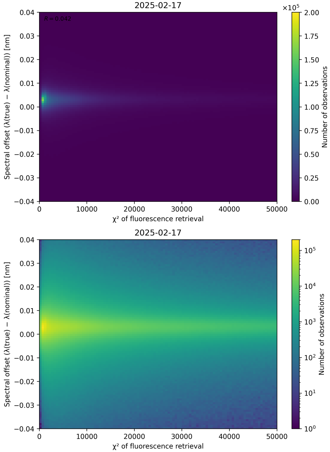
Figure 69: Scatter density plot of “ \chi^2 of fluorescence retrieval” against “Spectral offset ( \lambda_{\text{true}} - \lambda_{\text{nominal}} )” for 2025-02-16 to 2025-02-18.
