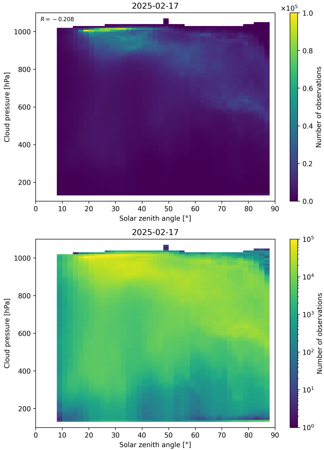
Figure 111: Scatter density plot of “Solar zenith angle” against “Cloud pressure” for 2025-02-16 to 2025-02-18.
