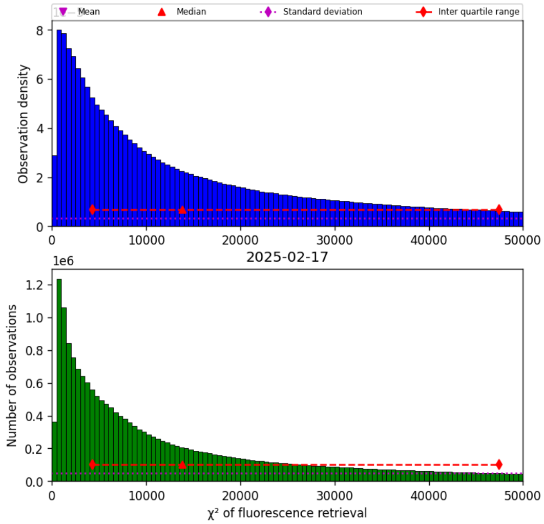
Figure 42: Histogram of “ \chi^2 of fluorescence retrieval” for 2025-02-16 to 2025-02-18
