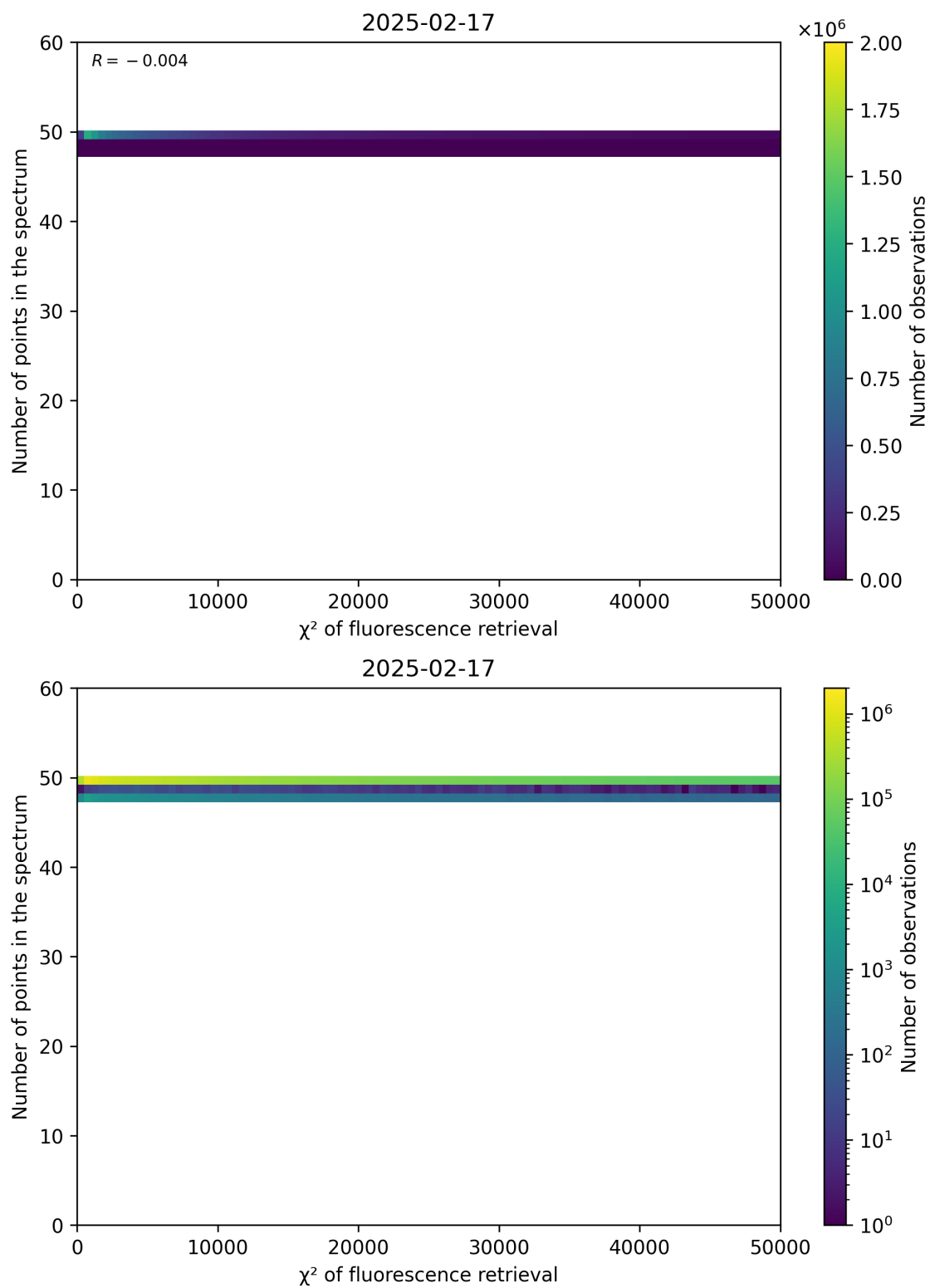
Figure 68: Scatter density plot of " \chi^2 of fluorescence retrieval" against "Number of points in the spectrum" for 2025-02-16 to 2025-02-18.
