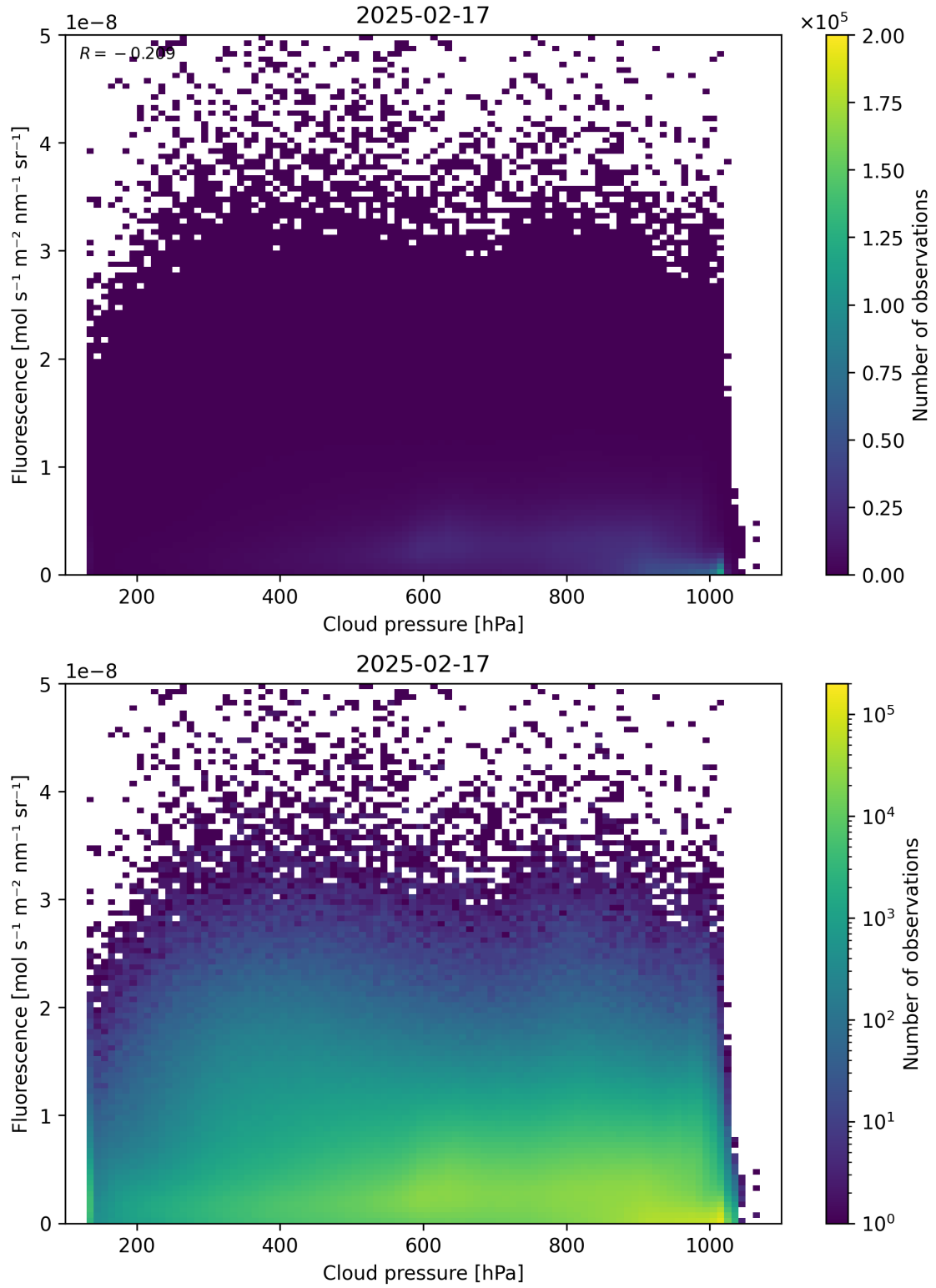
Figure 80: Scatter density plot of “Cloud pressure” against “Fluorescence” for 2025-02-16 to 2025-02-18.
