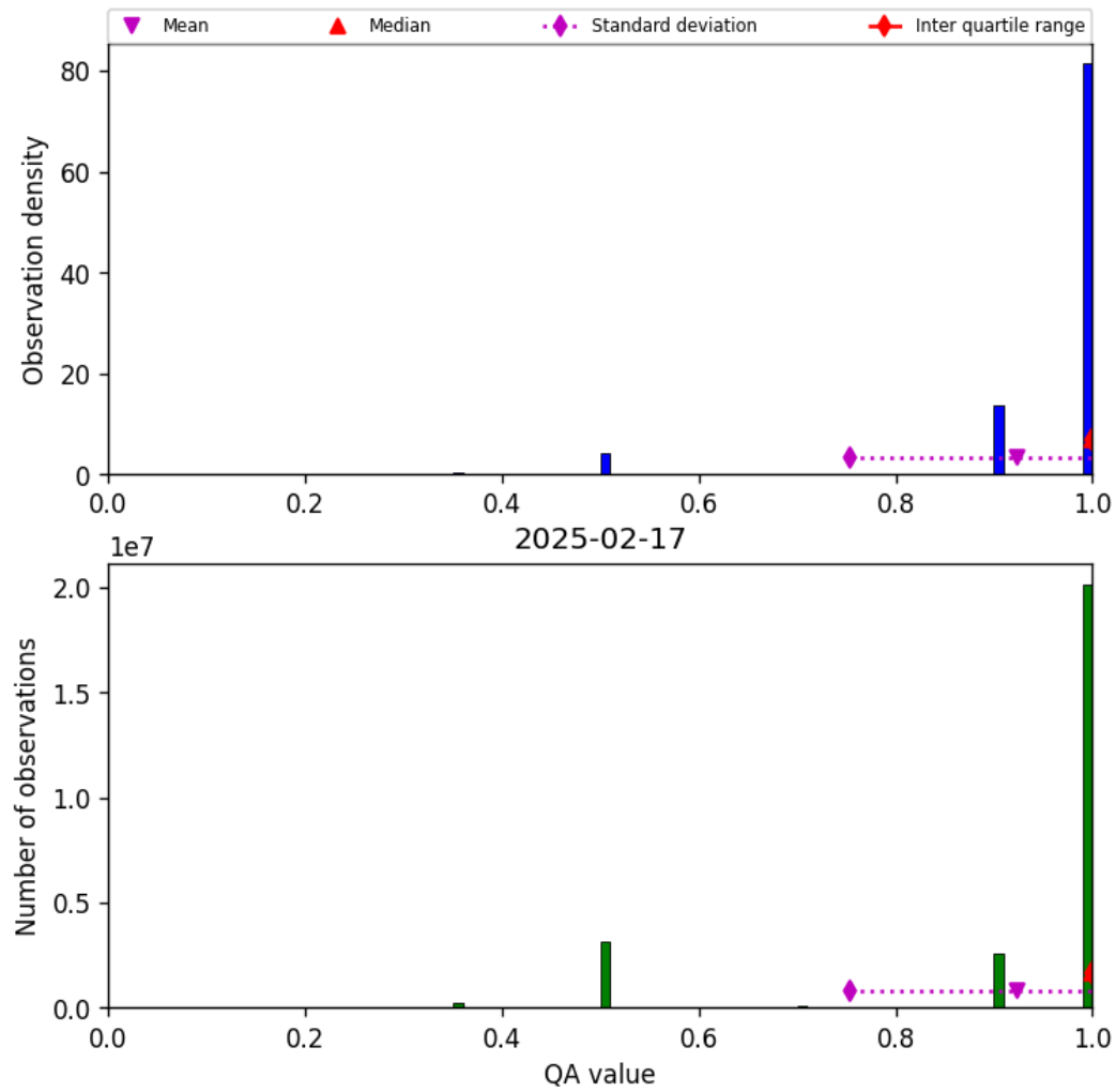
Figure 29: Histogram of “QA value” for 2025-02-16 to 2025-02-18
