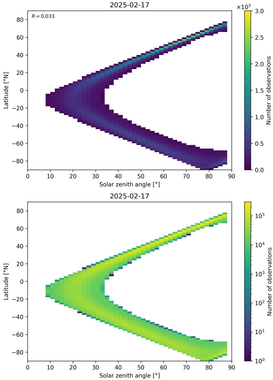
Figure 113: Scatter density plot of “Solar zenith angle” against “Latitude” for 2025-02-16 to 2025-02-18.
