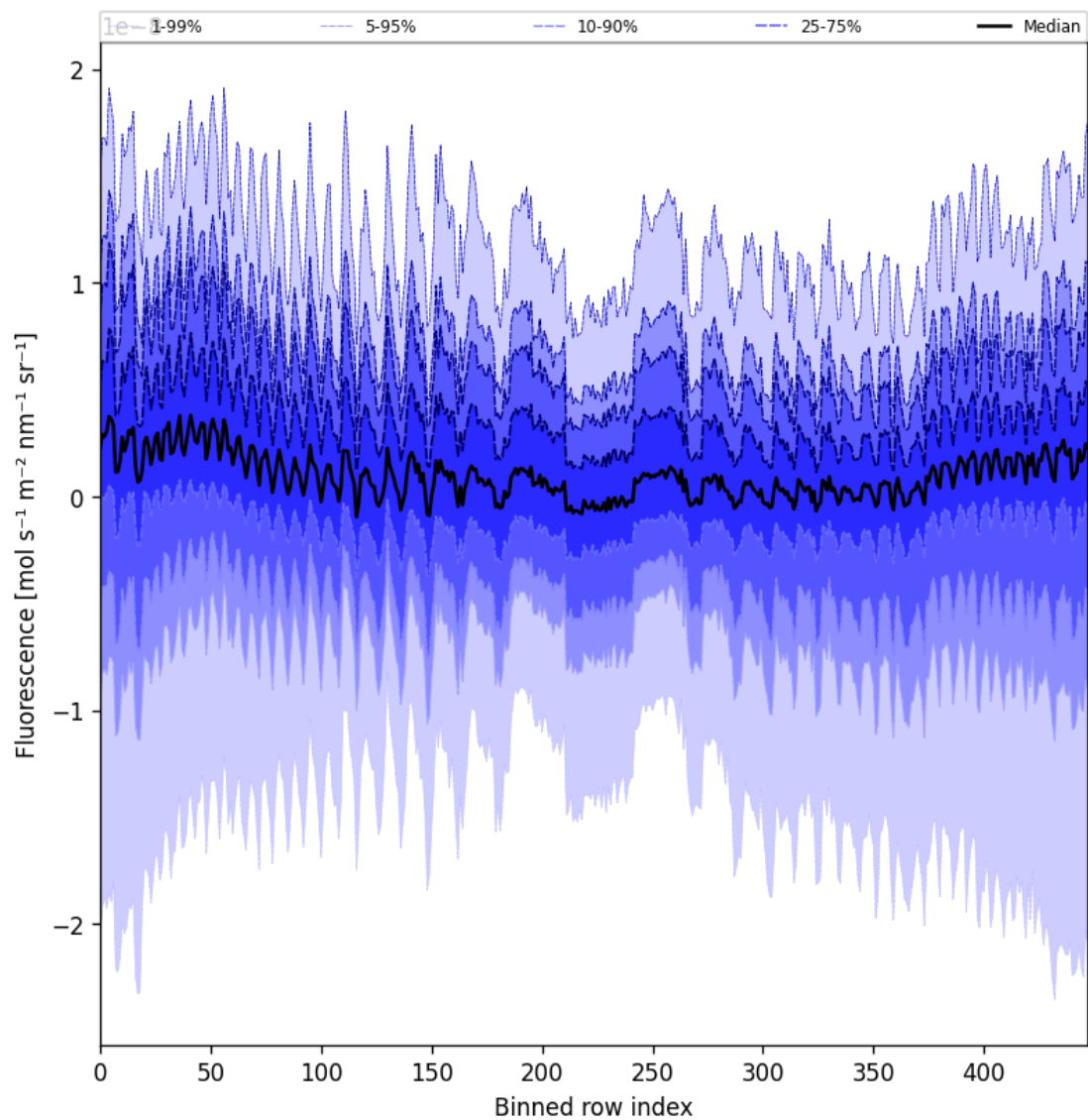
Figure 57: Along track statistics of “Fluorescence” for 2025-02-16 to 2025-02-18
