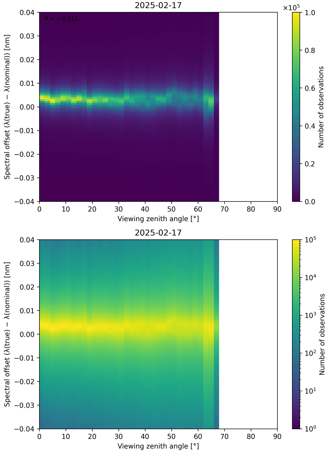
Figure 128: Scatter density plot of “Viewing zenith angle” against “Spectral offset ( \lambda_{\text{true}} - \lambda_{\text{nominal}} )” for 2025-02-16 to 2025-02-18.
