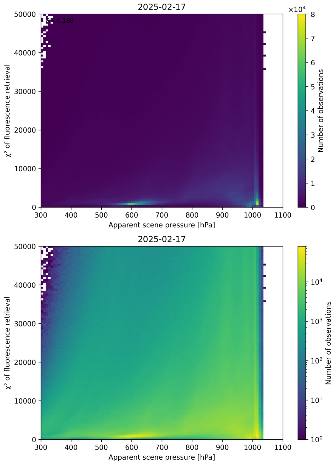
Figure 63: Scatter density plot of “Apparent scene pressure” against “ \chi^2 of fluorescence retrieval” for 2025-02-16 to 2025-02-18.
