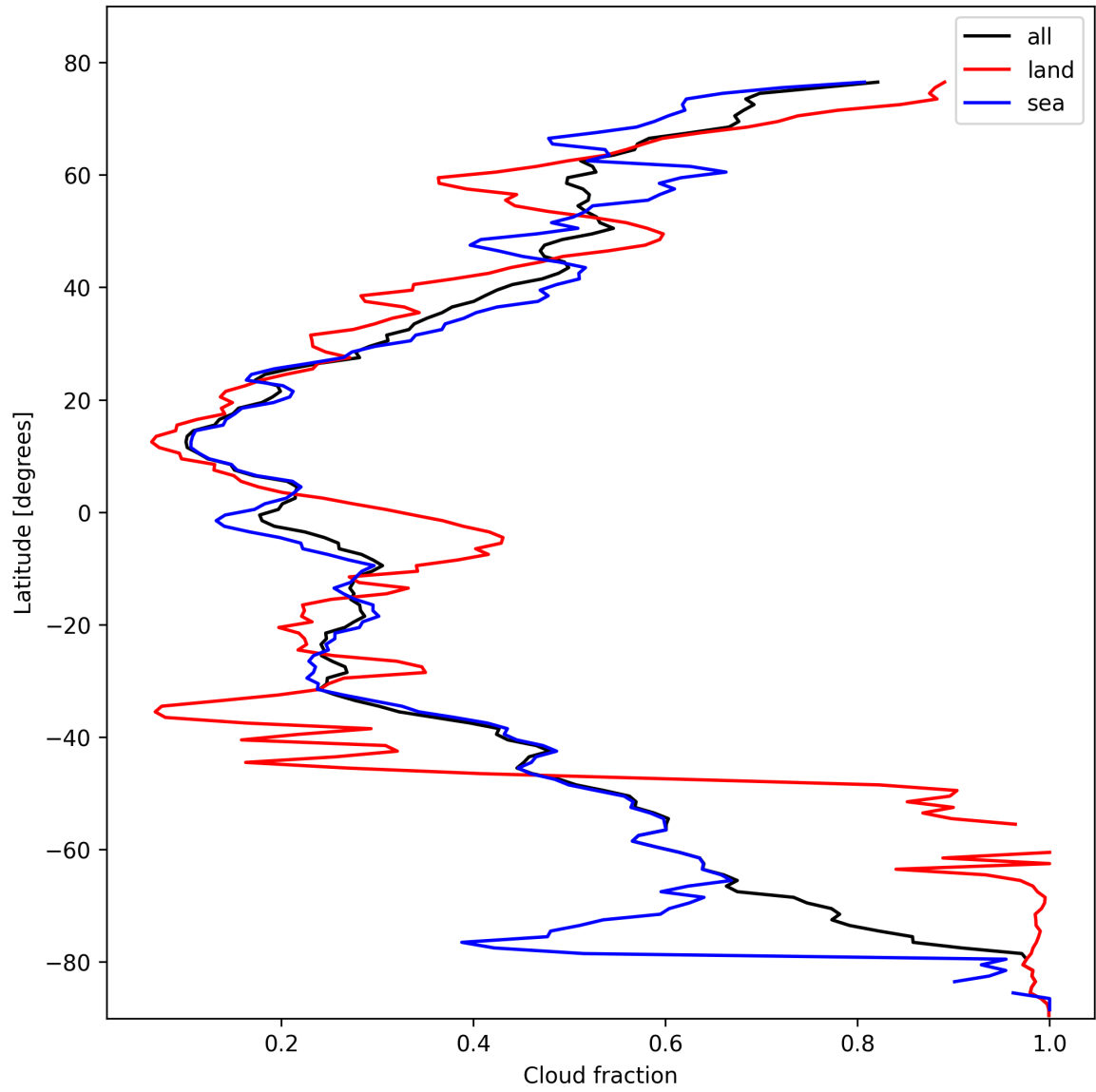
Figure 15: Zonal average of “Cloud fraction” for 2025-02-16 to 2025-02-18.
