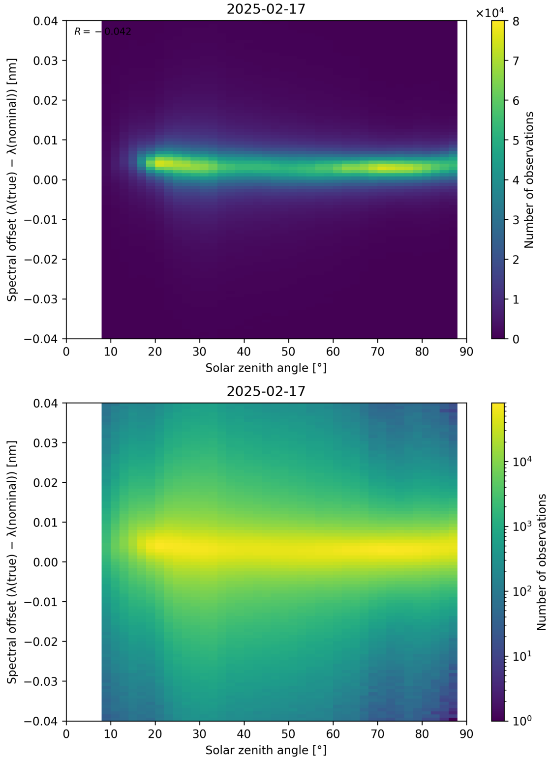
Figure 117: Scatter density plot of “Solar zenith angle” against “Spectral offset ( \lambda_{\text{true}} - \lambda_{\text{nominal}} )” for 2025-02-16 to 2025-02-18.
