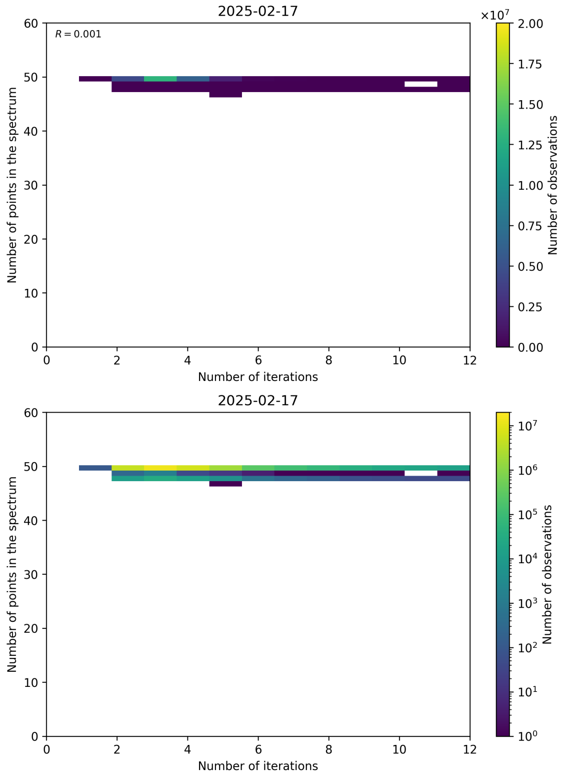
Figure 99: Scatter density plot of “Number of iterations” against “Number of points in the spectrum” for 2025-02-16 to 2025-02-18.
