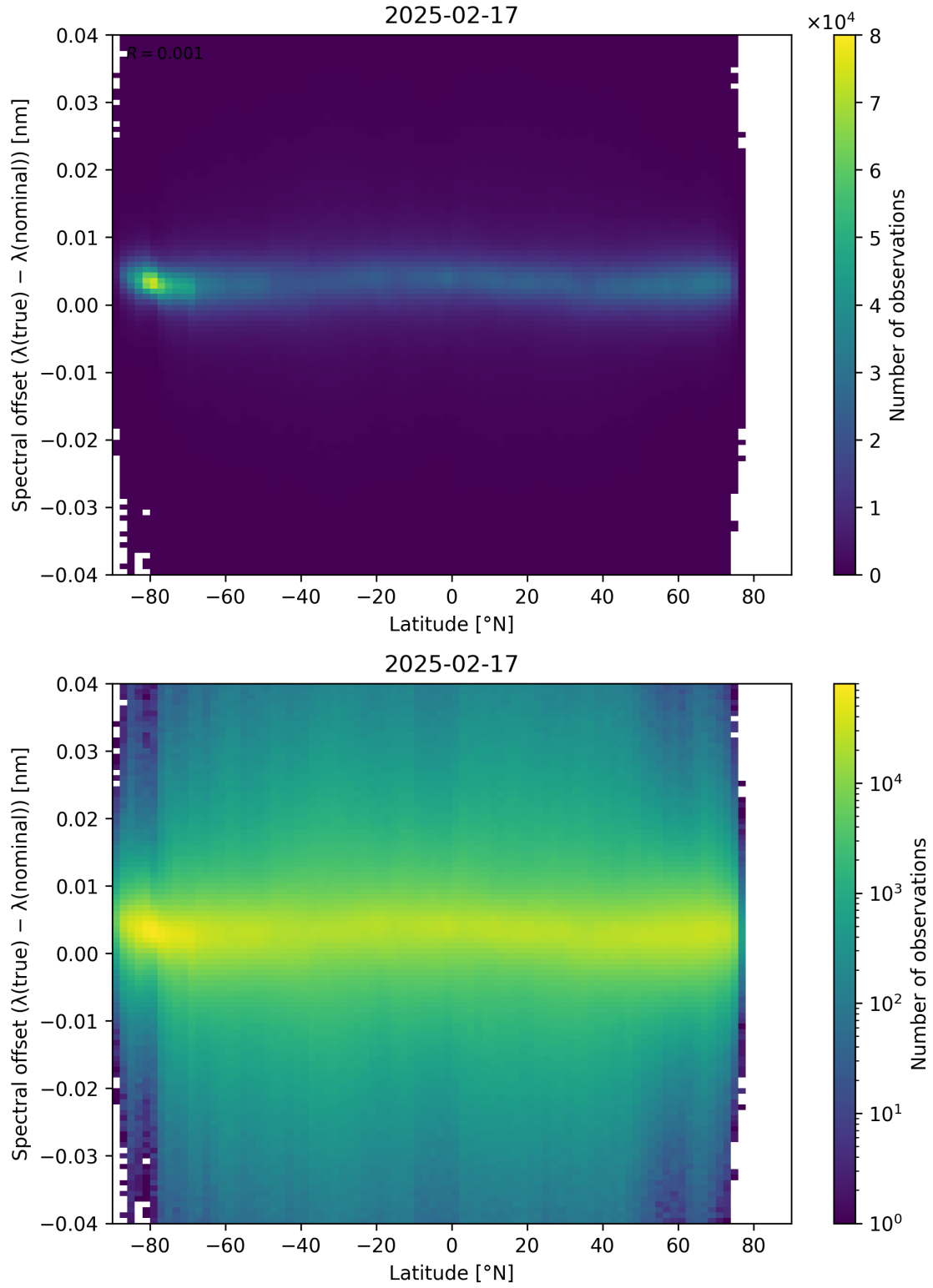
Figure 96: Scatter density plot of “Latitude” against “Spectral offset ( \lambda_{\text{true}} - \lambda_{\text{nominal}} )” for 2025-02-16 to 2025-02-18.
