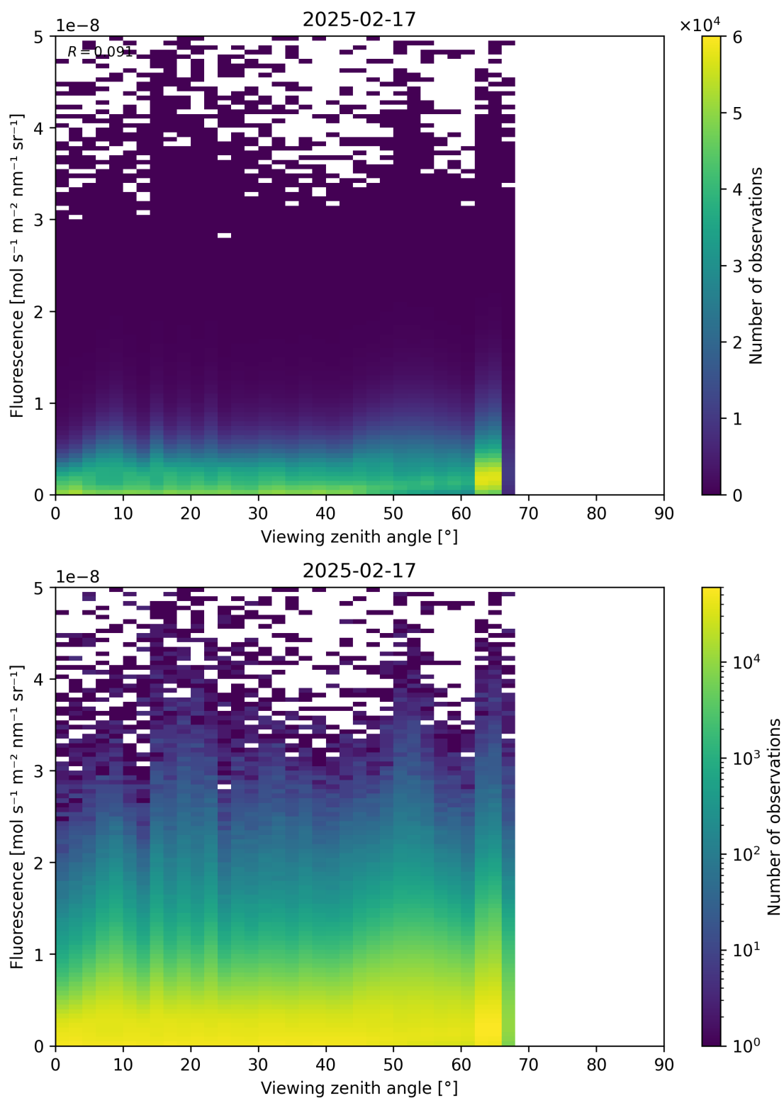
Figure 122: Scatter density plot of “Viewing zenith angle” against “Fluorescence” for 2025-02-16 to 2025-02-18.
