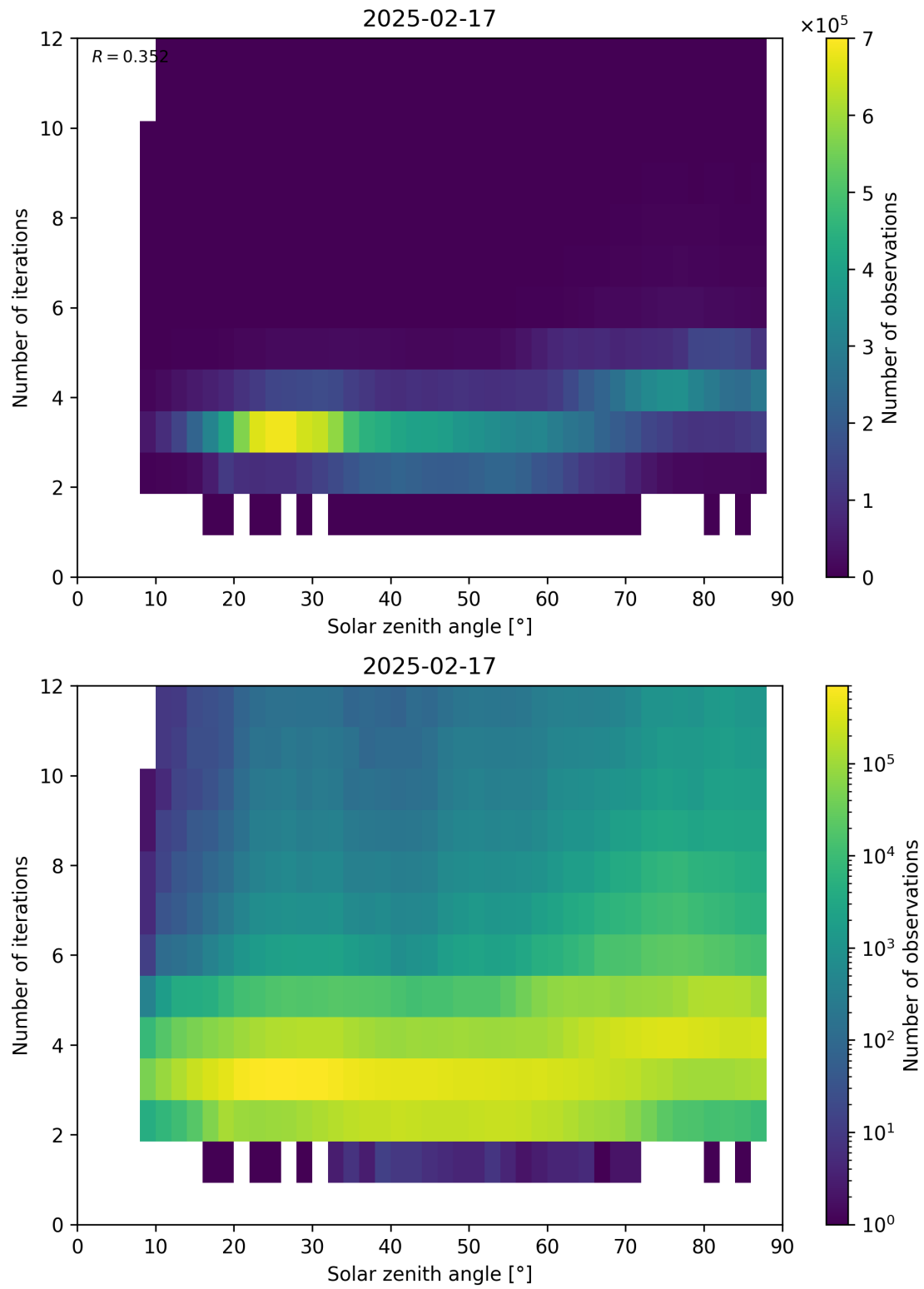
Figure 114: Scatter density plot of “Solar zenith angle” against “Number of iterations” for 2025-02-16 to 2025-02-18.
