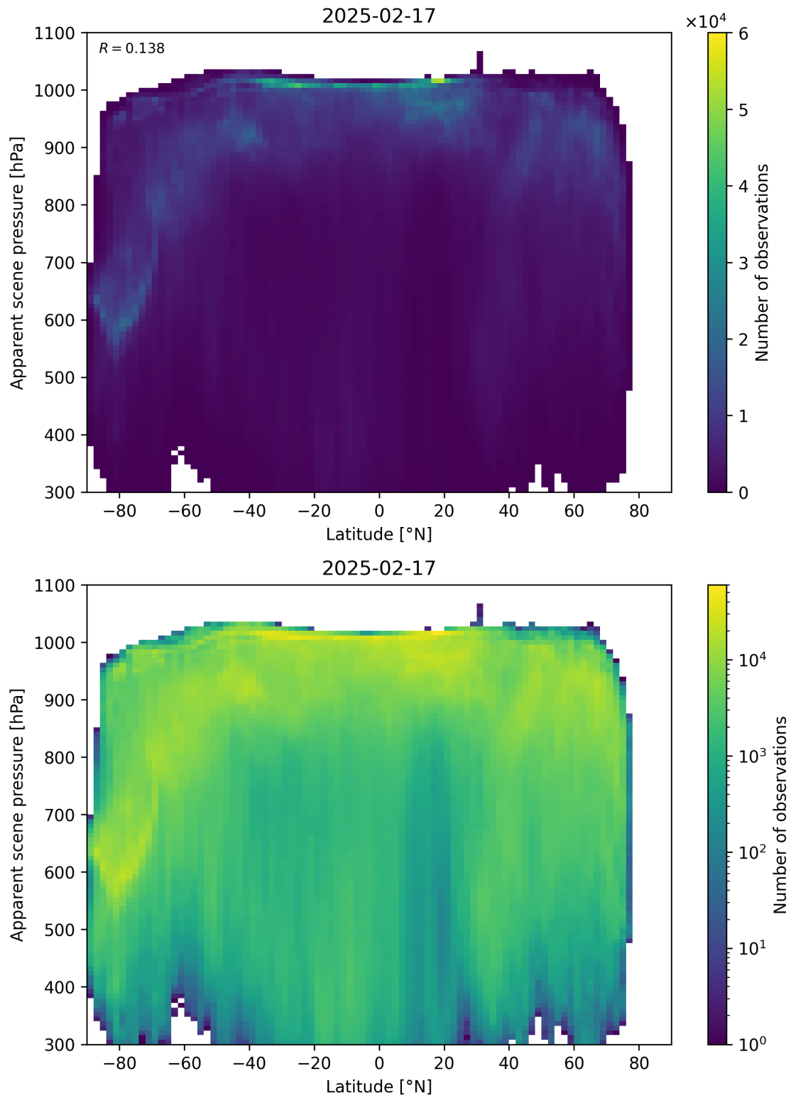
Figure 88: Scatter density plot of “Latitude” against “Apparent scene pressure” for 2025-02-16 to 2025-02-18.
