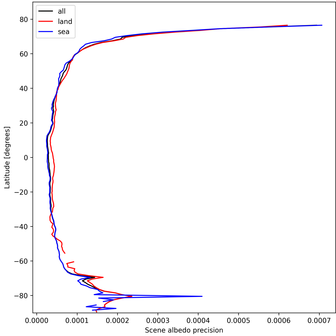
Figure 18: Zonal average of “Scene albedo precision” for 2025-02-16 to 2025-02-18.
