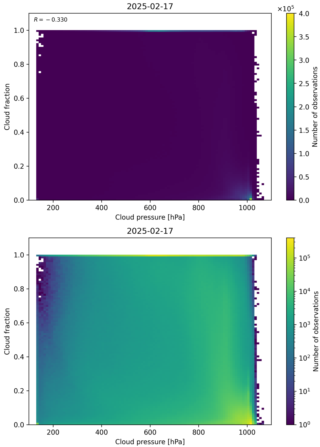
Figure 79: Scatter density plot of “Cloud pressure” against “Cloud fraction” for 2025-02-16 to 2025-02-18.
