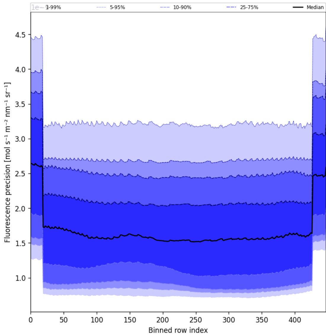
Figure 58: Along track statistics of “Fluorescence precision” for 2025-02-16 to 2025-02-18
