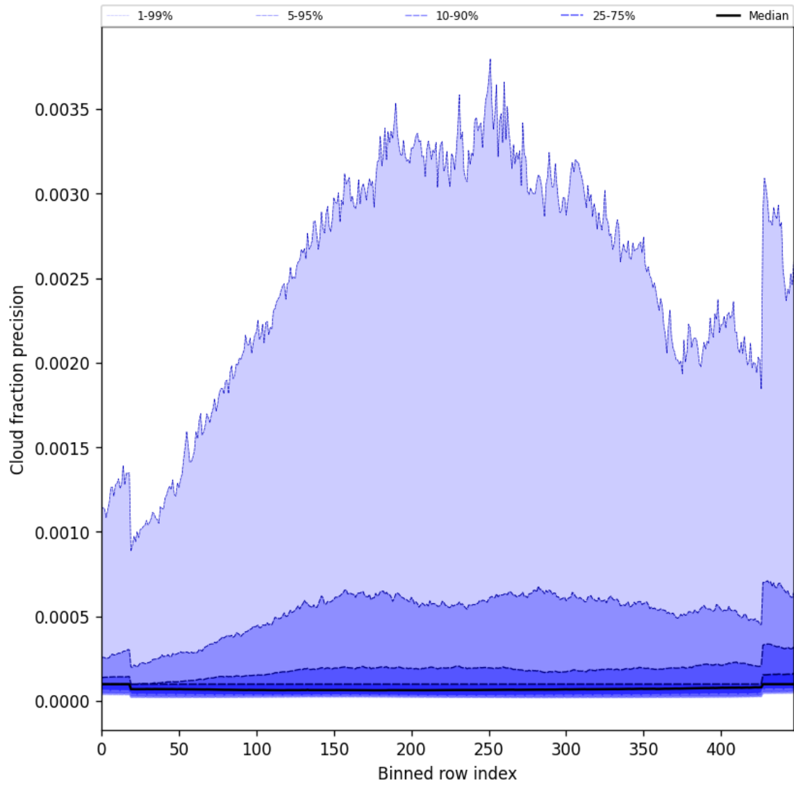
Figure 50: Along track statistics of “Cloud fraction precision” for 2025-02-16 to 2025-02-18
