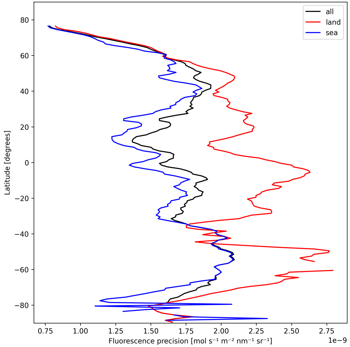
Figure 24: Zonal average of "Fluorescence precision" for 2025-02-16 to 2025-02-18.
