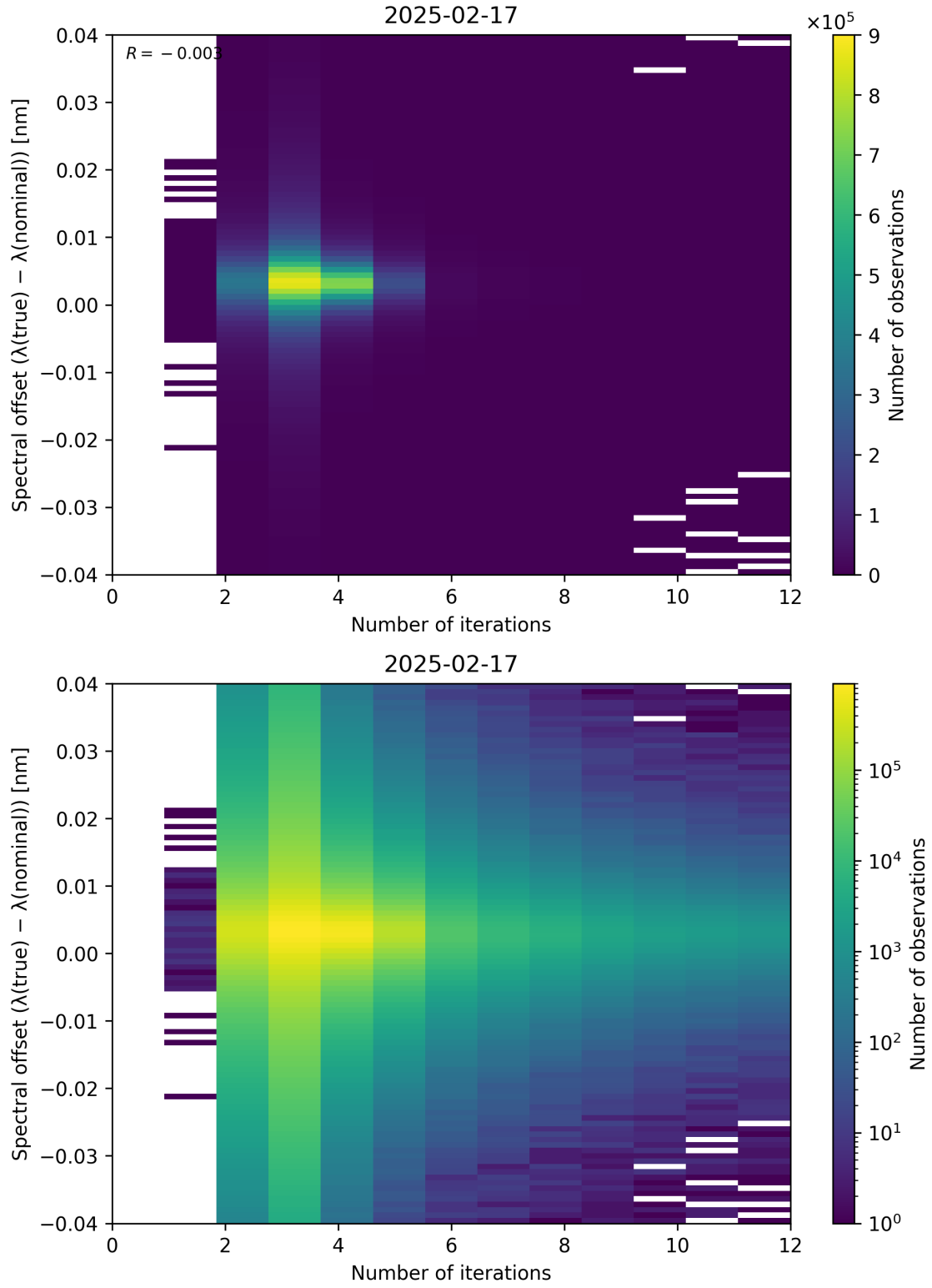
Figure 100: Scatter density plot of “Number of iterations” against “Spectral offset ( \lambda_{\text{true}} - \lambda_{\text{nominal}} )” for 2025-02-16 to 2025-02-18.
