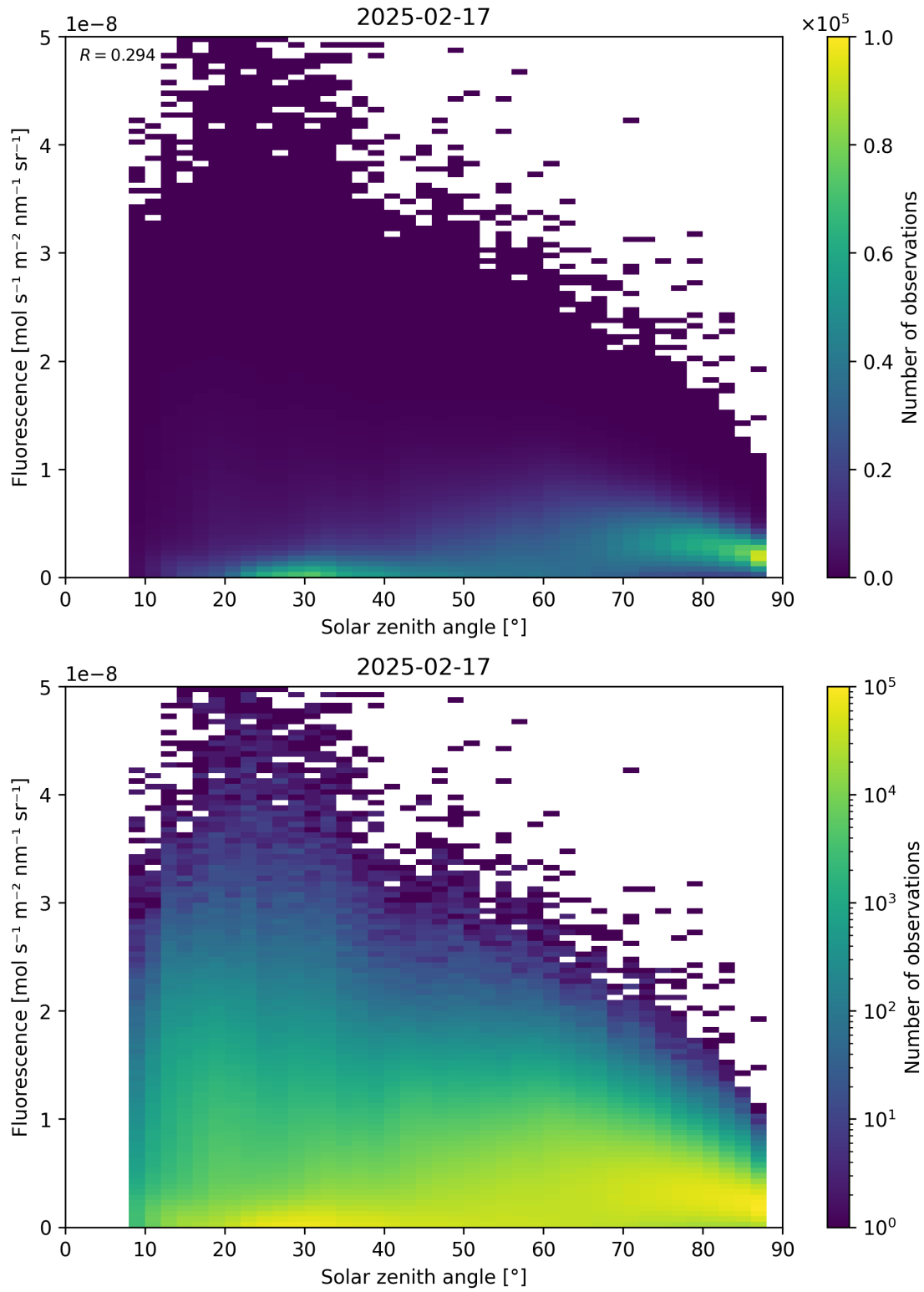
Figure 112: Scatter density plot of “Solar zenith angle” against “Fluorescence” for 2025-02-16 to 2025-02-18.
