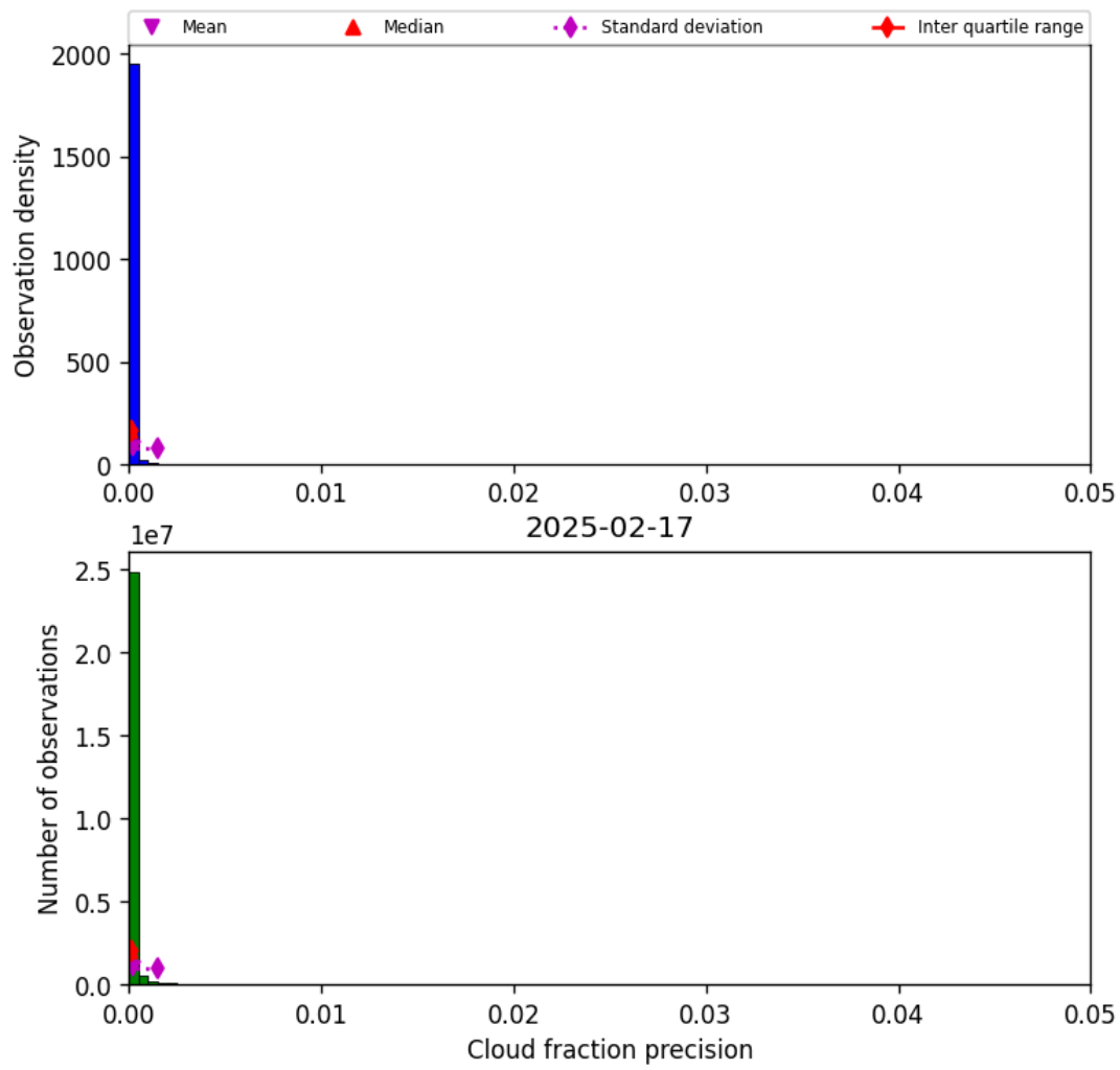
Figure 33: Histogram of “Cloud fraction precision” for 2025-02-16 to 2025-02-18
