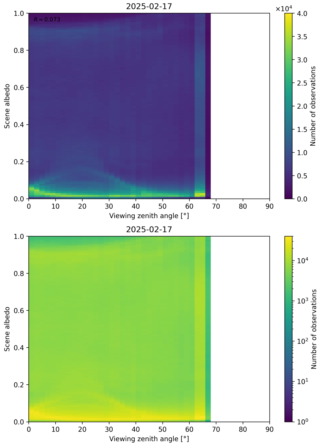
Figure 126: Scatter density plot of “Viewing zenith angle” against “Scene albedo” for 2025-02-16 to 2025-02-18.
