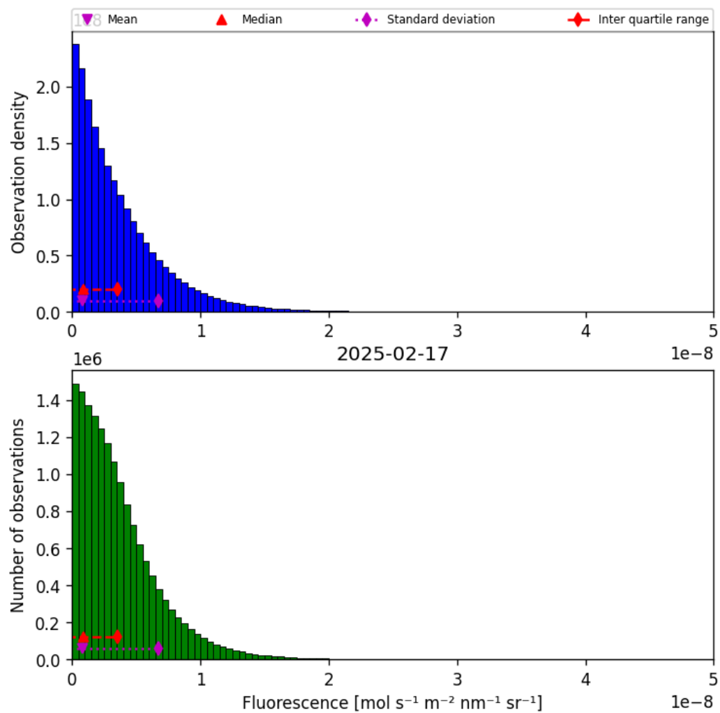
Figure 40: Histogram of “Fluorescence” for 2025-02-16 to 2025-02-18
