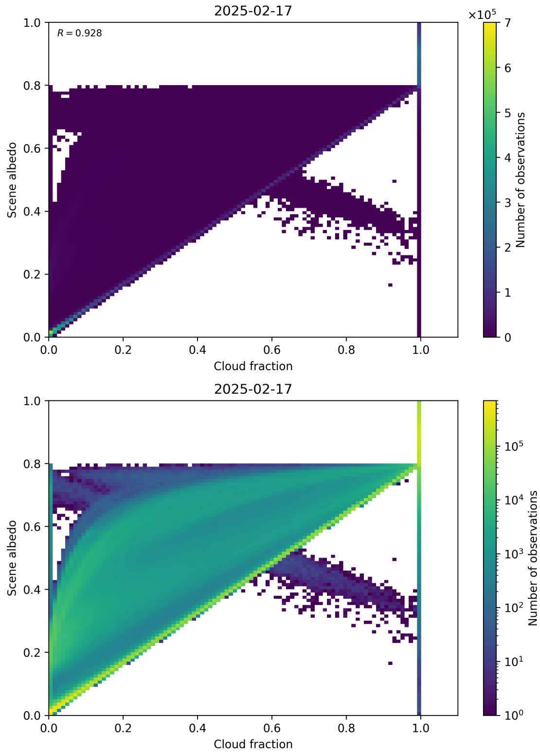
Figure 75: Scatter density plot of “Cloud fraction” against “Scene albedo” for 2025-02-16 to 2025-02-18.
