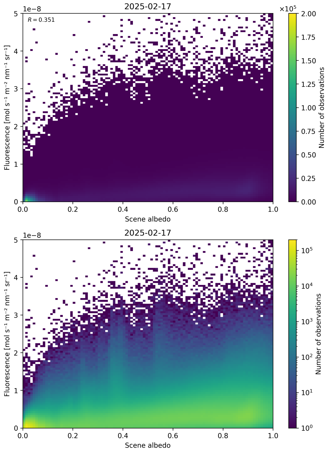
Figure 104: Scatter density plot of “Scene albedo” against “Fluorescence” for 2025-02-16 to 2025-02-18.
