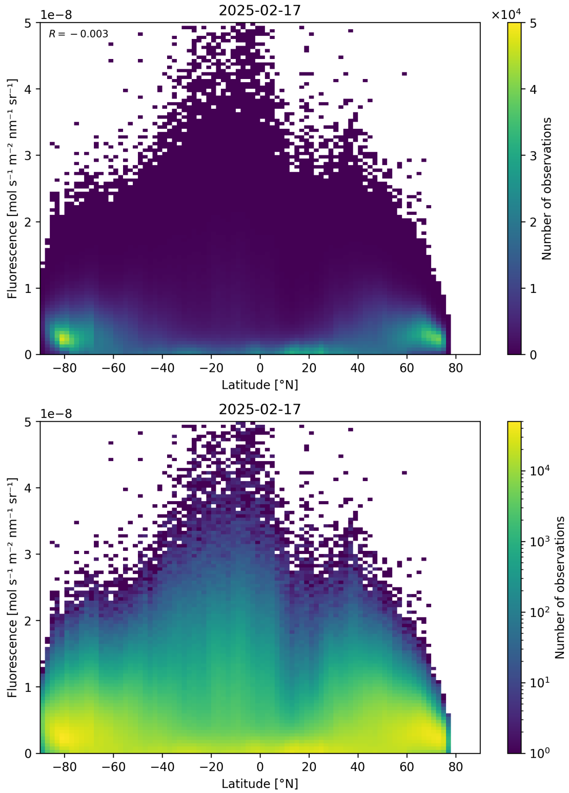
Figure 92: Scatter density plot of “Latitude” against “Fluorescence” for 2025-02-16 to 2025-02-18.
