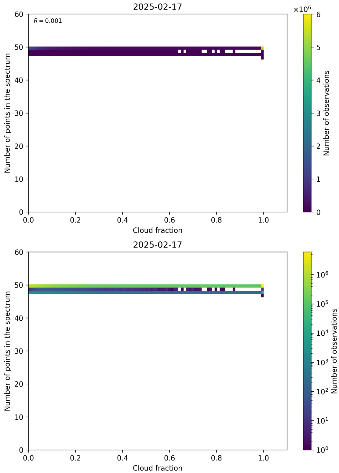
Figure 74: Scatter density plot of “Cloud fraction” against “Number of points in the spectrum” for 2025-02-16 to 2025-02-18.
