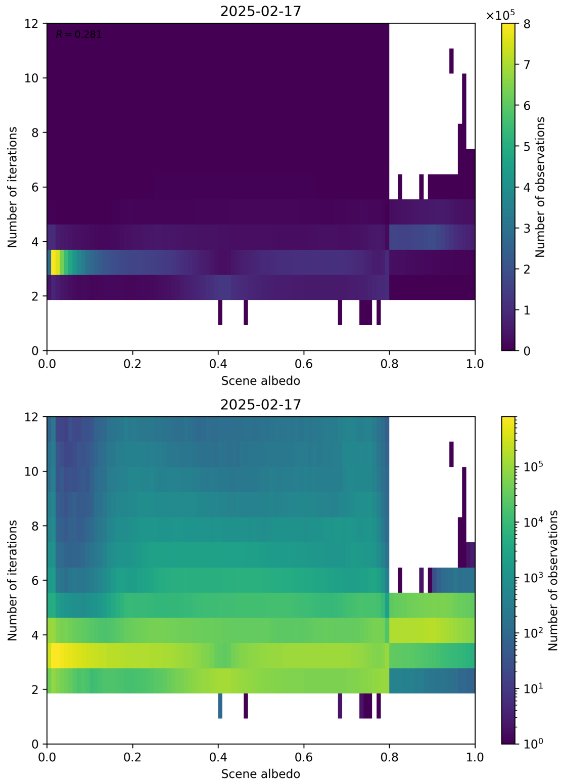
Figure 105: Scatter density plot of “Scene albedo” against “Number of iterations” for 2025-02-16 to 2025-02-18.
