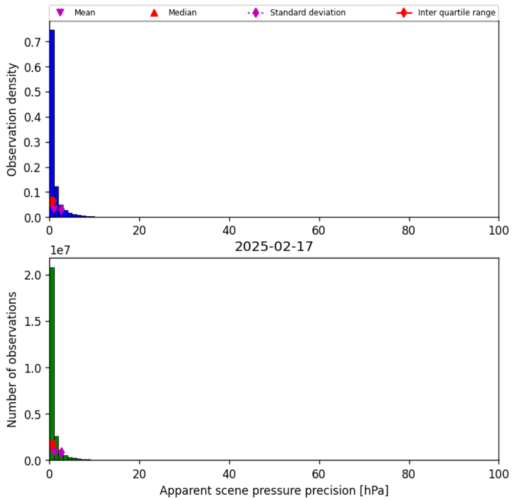
Figure 37: Histogram of “Apparent scene pressure precision” for 2025-02-16 to 2025-02-18
