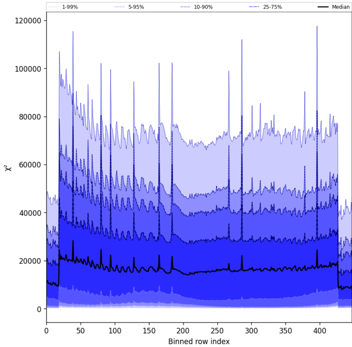
Figure 55: Along track statistics of “ \chi^2 ” for 2025-02-16 to 2025-02-18
