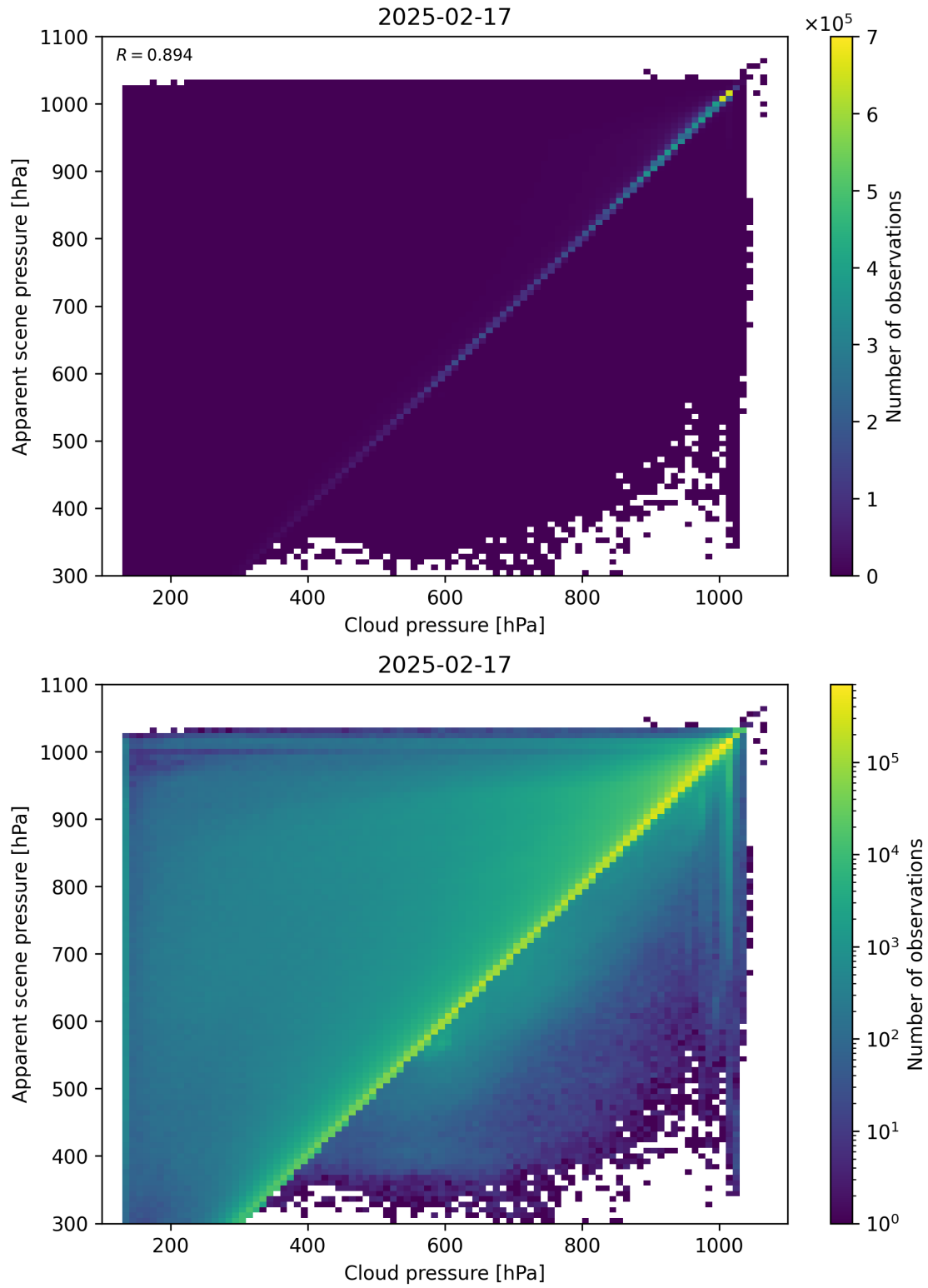
Figure 77: Scatter density plot of “Cloud pressure” against “Apparent scene pressure” for 2025-02-16 to 2025-02-18.
