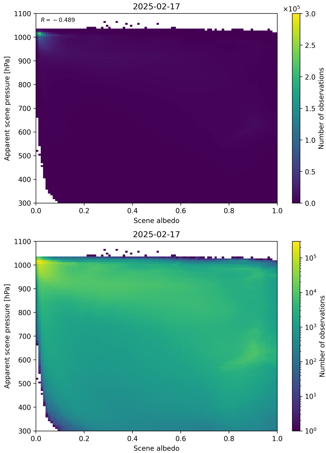
Figure 102: Scatter density plot of “Scene albedo” against “Apparent scene pressure” for 2025-02-16 to 2025-02-18.
