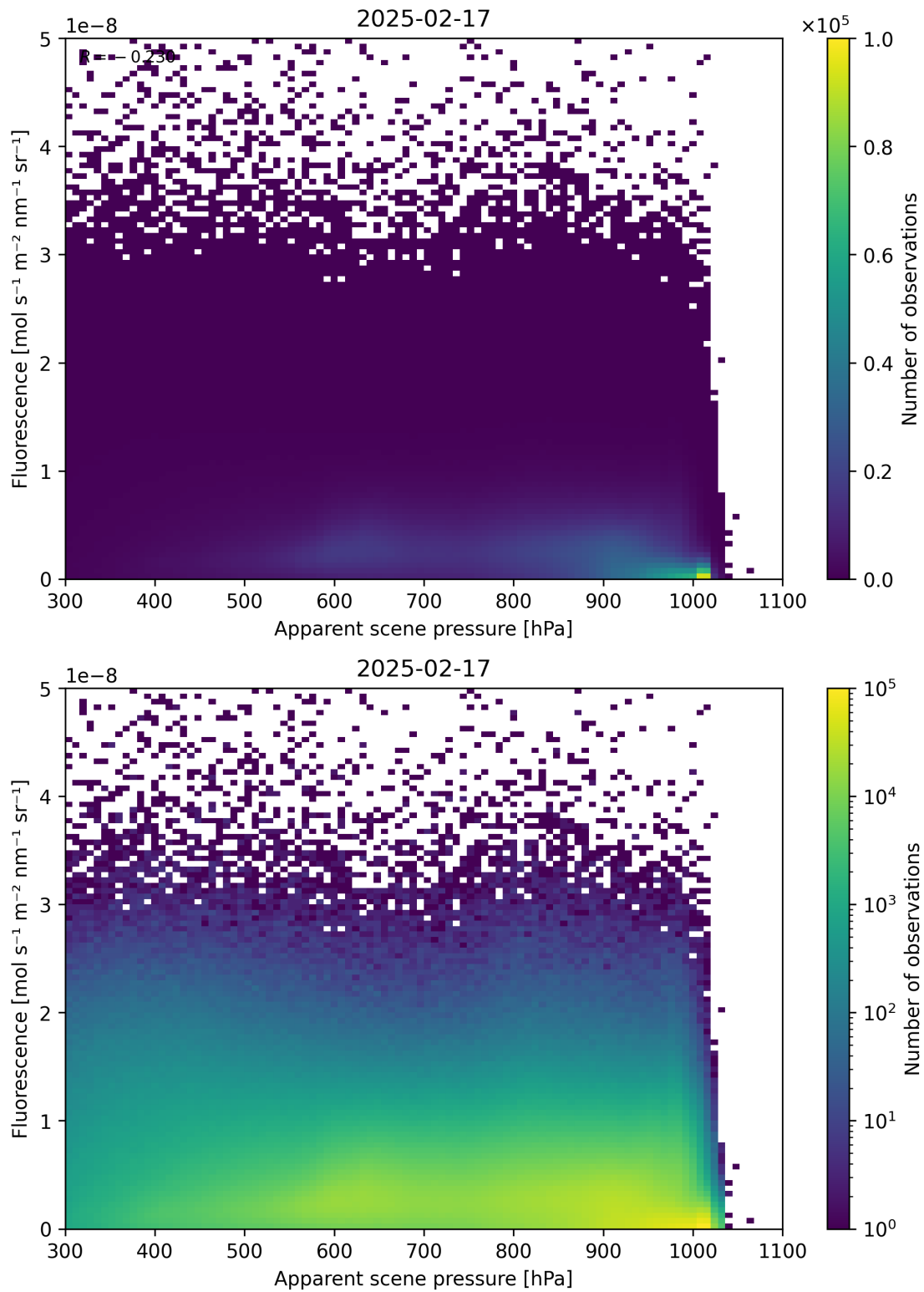
Figure 64: Scatter density plot of “Apparent scene pressure” against “Fluorescence” for 2025-02-16 to 2025-02-18.
