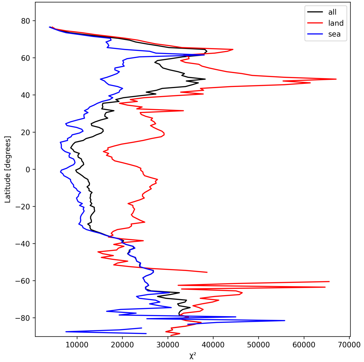
Figure 21: Zonal average of “ \chi^2 ” for 2025-02-16 to 2025-02-18.
