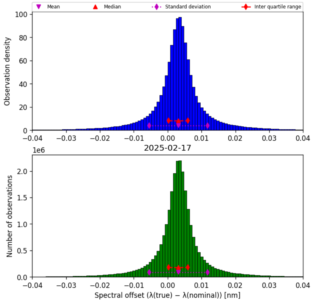
Figure 45: Histogram of “Spectral offset ( \lambda_{\text{true}} - \lambda_{\text{nominal}} )” for 2025-02-16 to 2025-02-18
