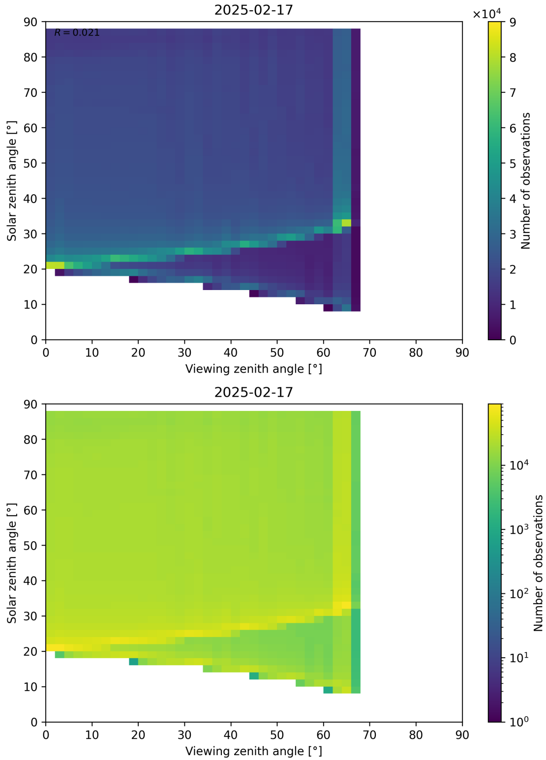
Figure 127: Scatter density plot of “Viewing zenith angle” against “Solar zenith angle” for 2025-02-16 to 2025-02-18.
