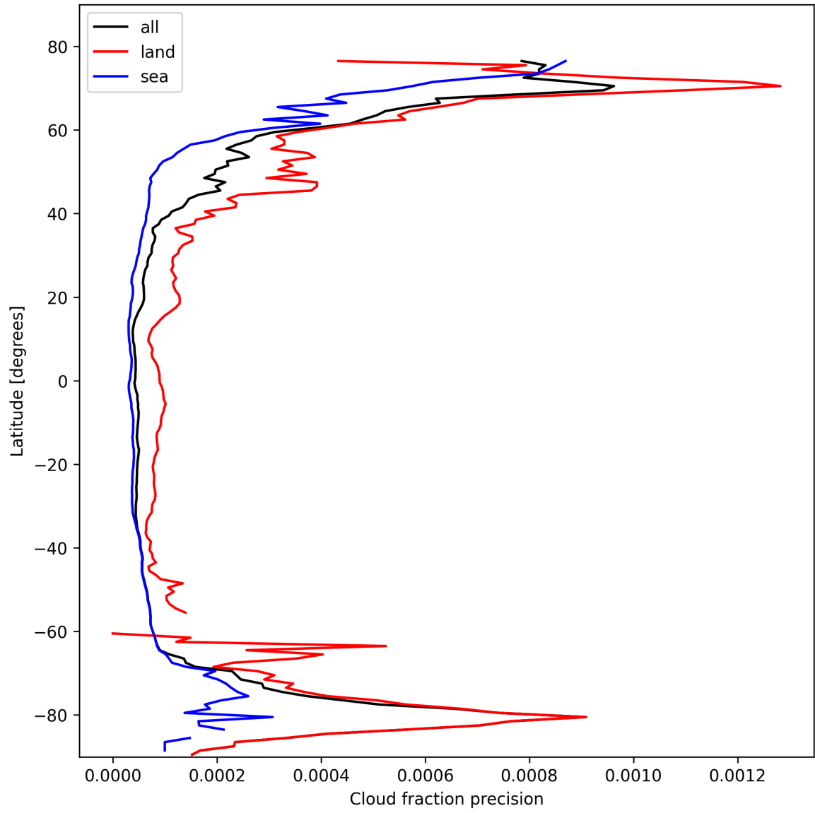
Figure 16: Zonal average of “Cloud fraction precision” for 2025-02-16 to 2025-02-18.
