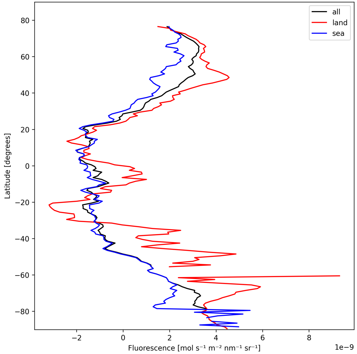
Figure 23: Zonal average of “Fluorescence” for 2025-02-16 to 2025-02-18.
