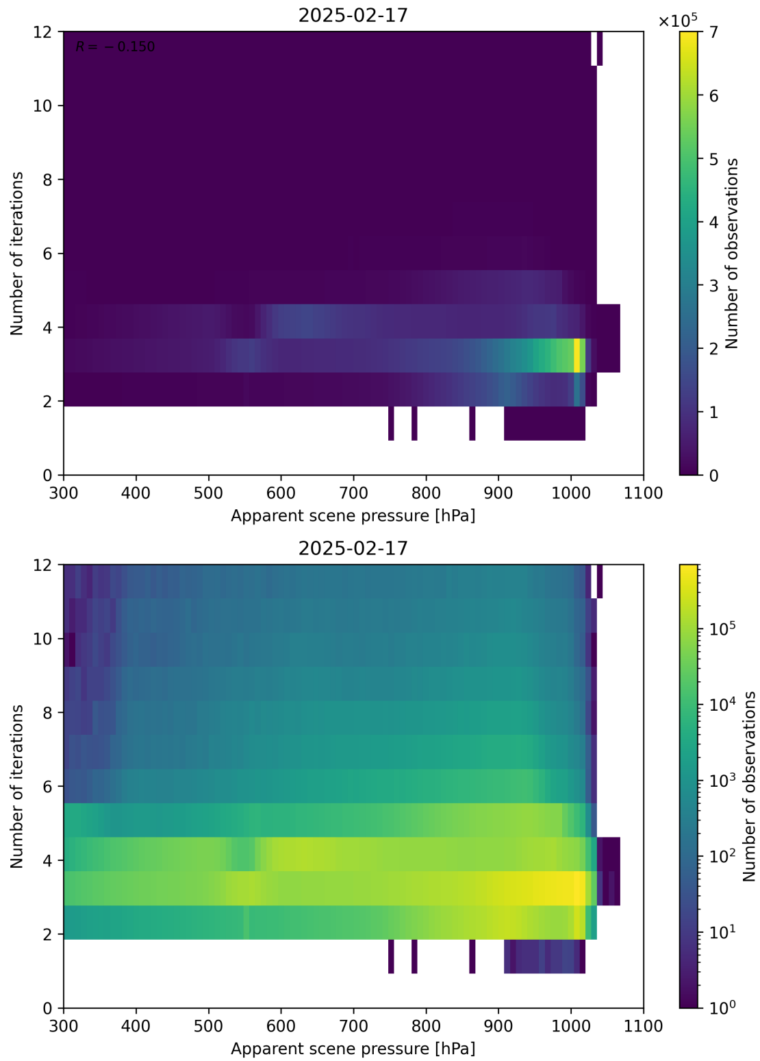
Figure 65: Scatter density plot of “Apparent scene pressure” against “Number of iterations” for 2025-02-16 to 2025-02-18.
