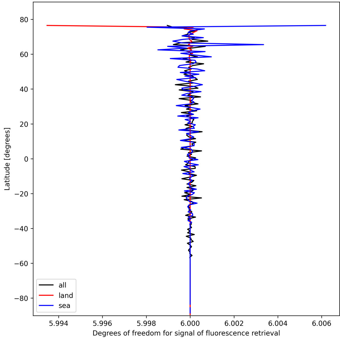
Figure 26: Zonal average of “Degrees of freedom for signal of fluorescence retrieval” for 2025-02-16 to 2025-02-18.
