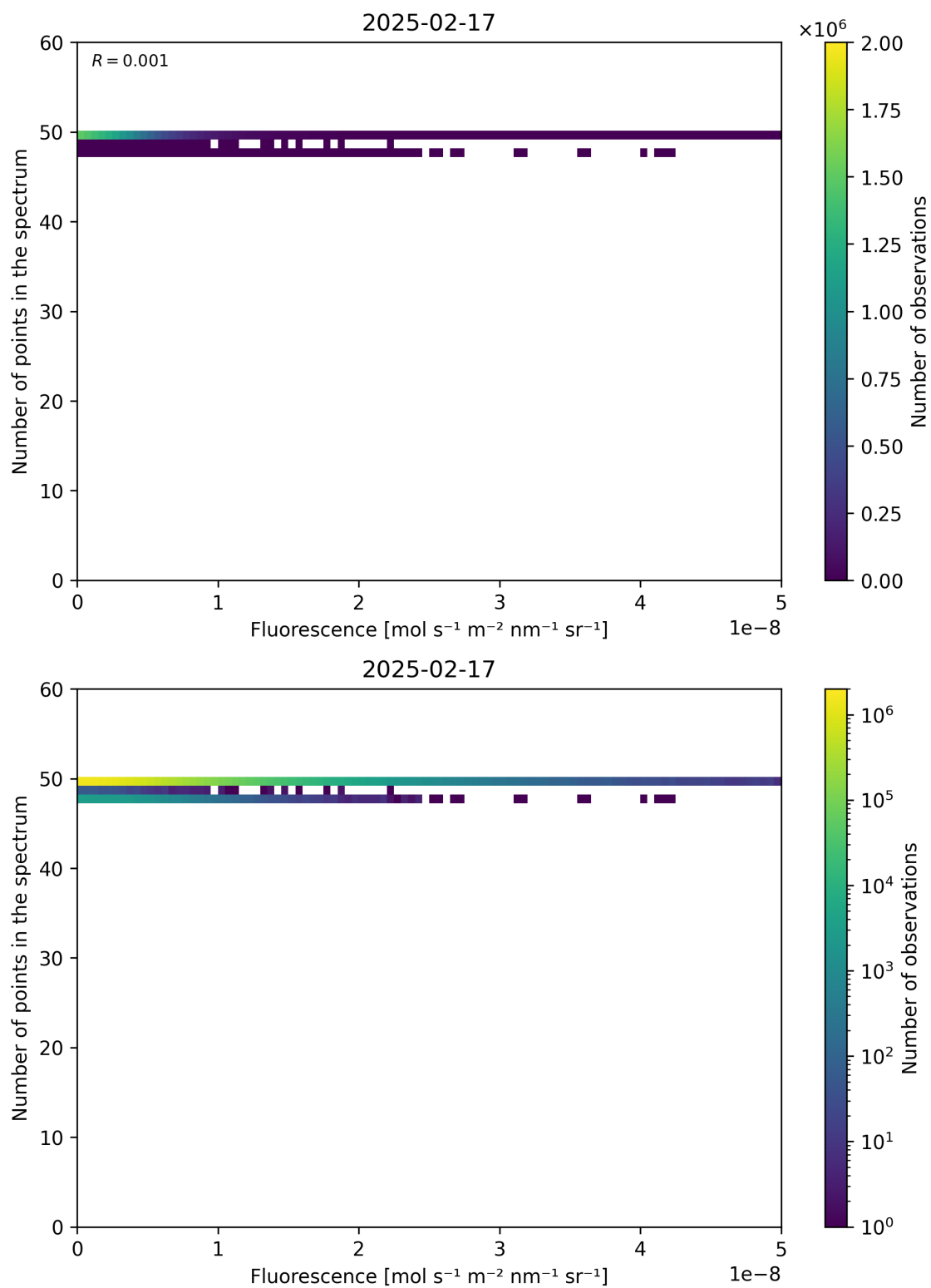
Figure 86: Scatter density plot of “Fluorescence” against “Number of points in the spectrum” for 2025-02-16 to 2025-02-18.
