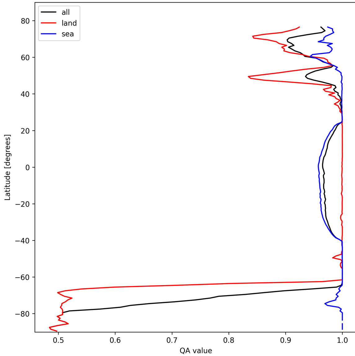
Figure 12: Zonal average of “QA value” for 2025-02-16 to 2025-02-18.
