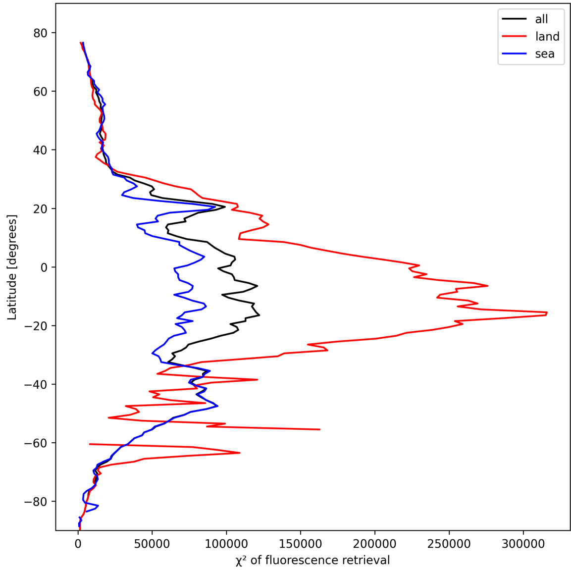
Figure 25: Zonal average of “ \chi^2 of fluorescence retrieval” for 2025-02-16 to 2025-02-18.
