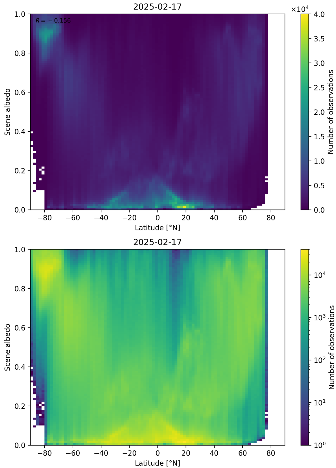
Figure 95: Scatter density plot of “Latitude” against “Scene albedo” for 2025-02-16 to 2025-02-18.
