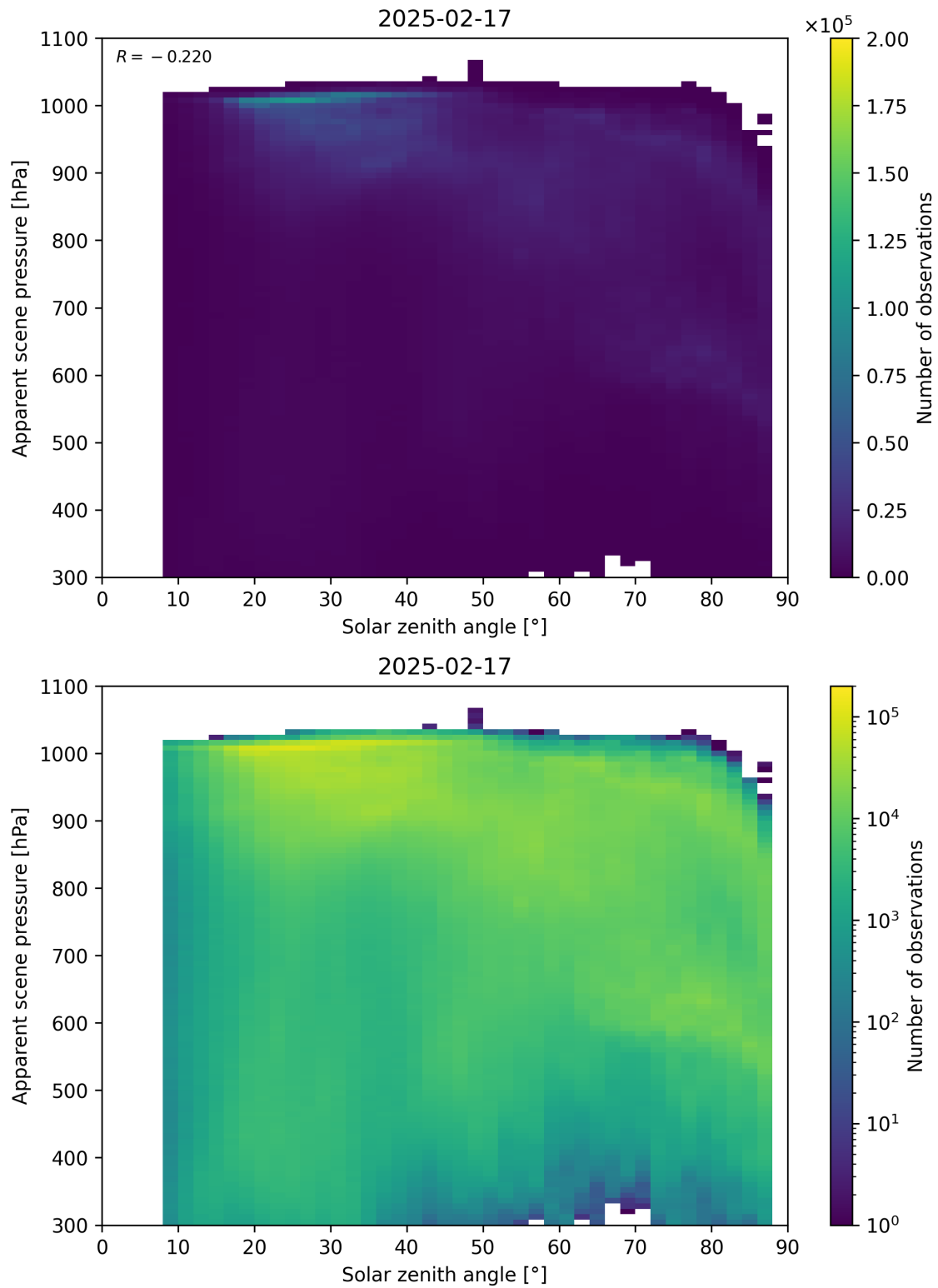
Figure 108: Scatter density plot of “Solar zenith angle” against “Apparent scene pressure” for 2025-02-16 to 2025-02-18.
