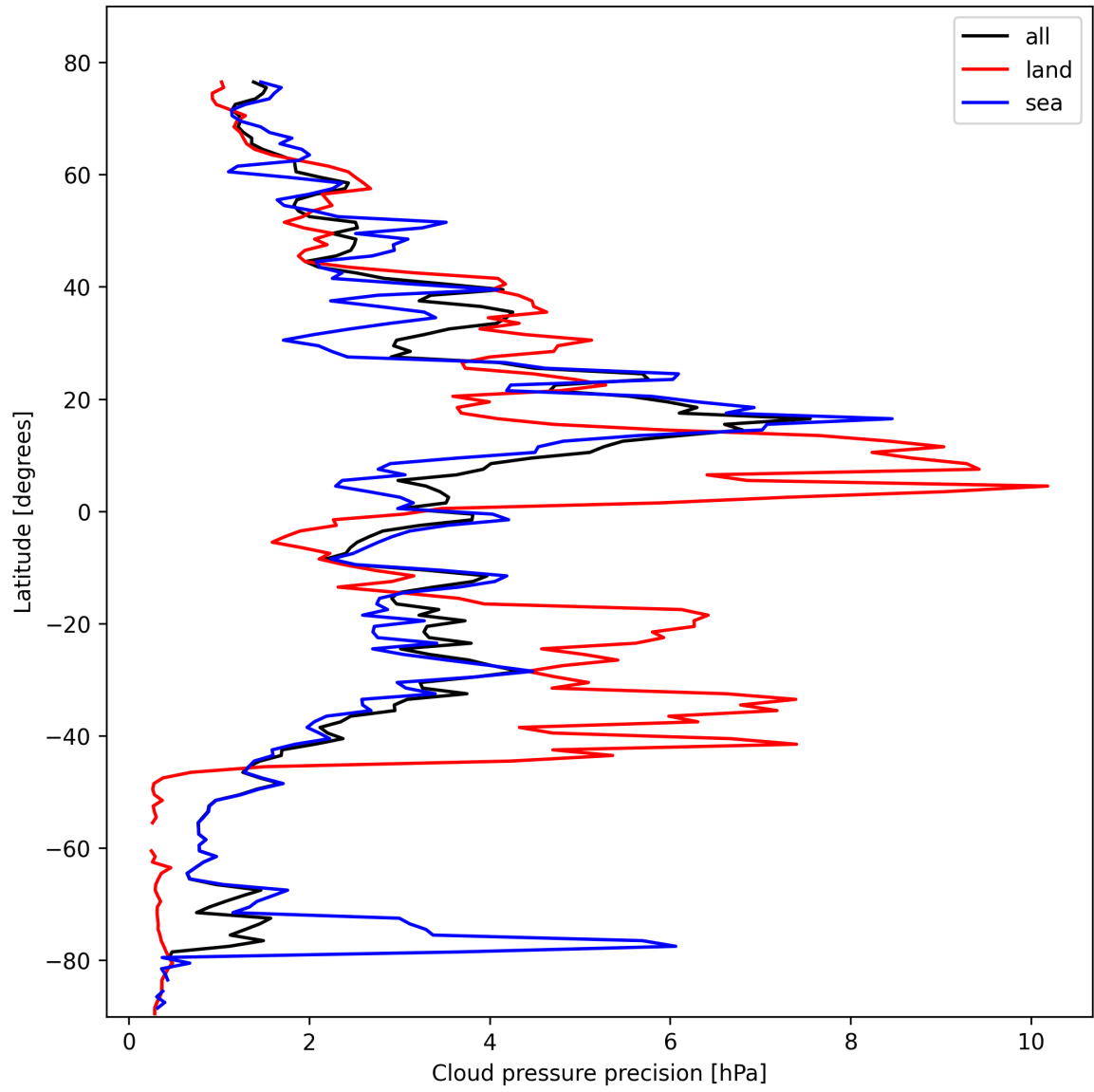
Figure 14: Zonal average of “Cloud pressure precision” for 2025-02-16 to 2025-02-18.
