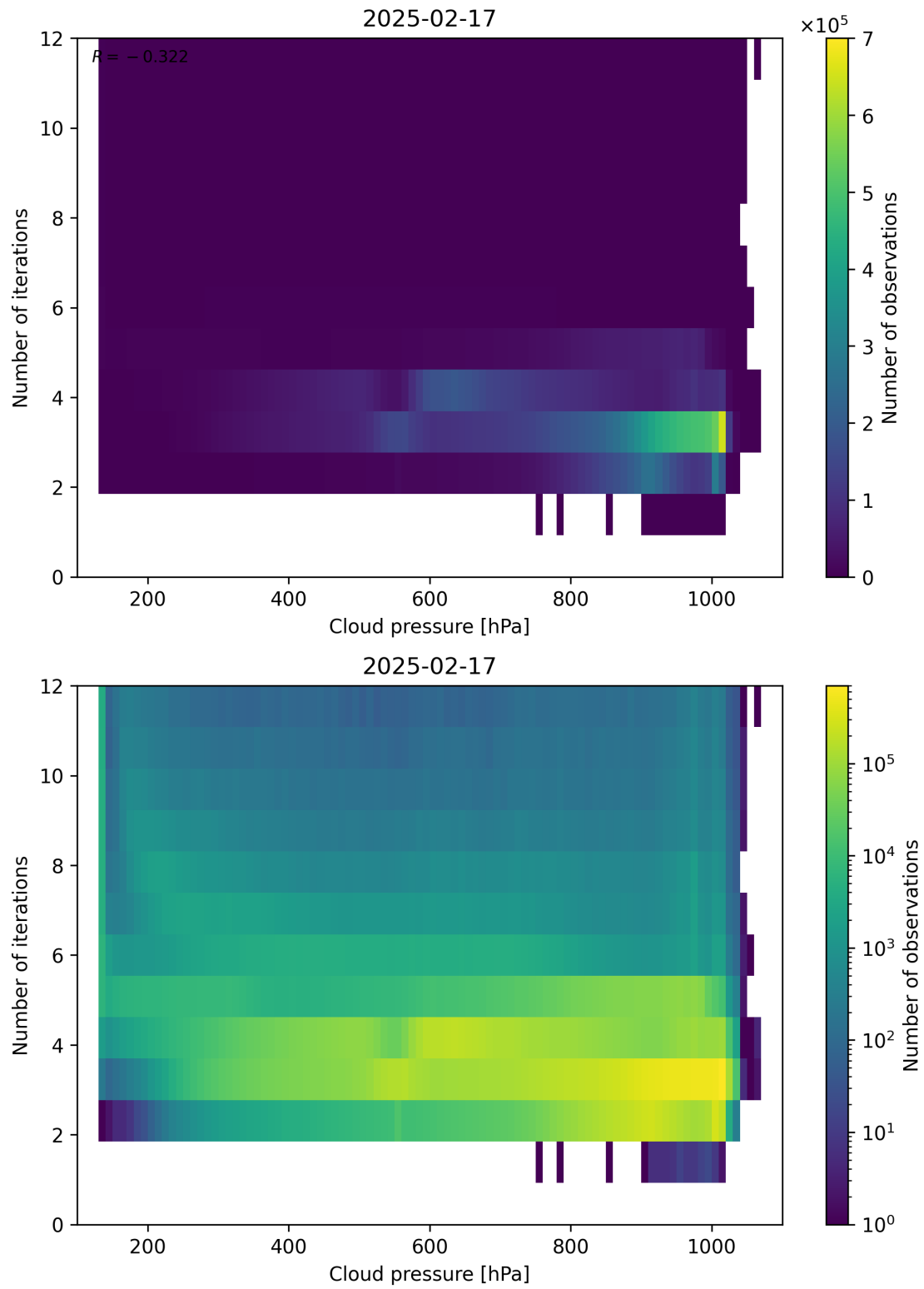
Figure 81: Scatter density plot of “Cloud pressure” against “Number of iterations” for 2025-02-16 to 2025-02-18.
