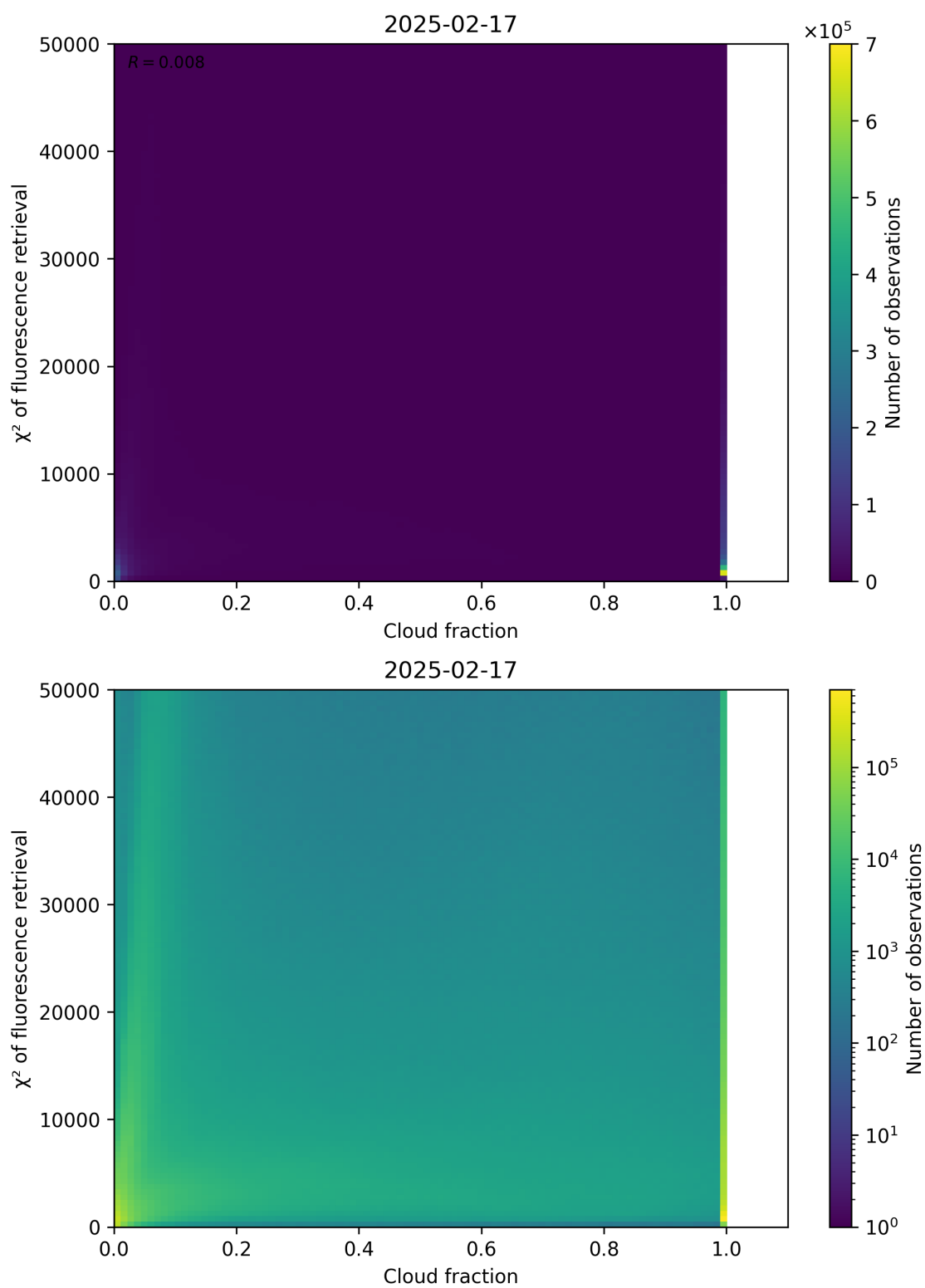
Figure 71: Scatter density plot of “Cloud fraction” against “ \chi^2 of fluorescence retrieval” for 2025-02-16 to 2025-02-18.
