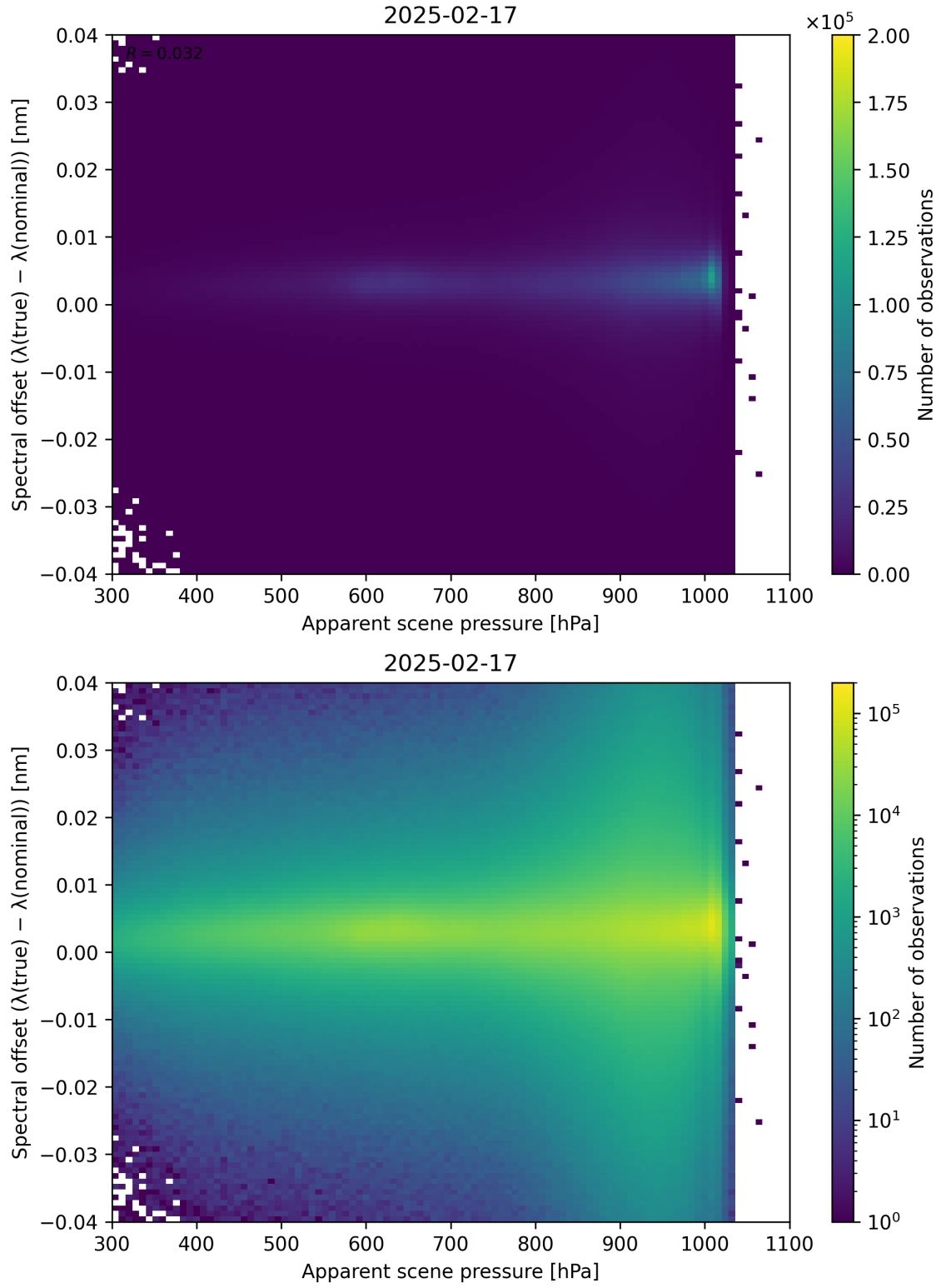
Figure 67: Scatter density plot of “Apparent scene pressure” against “Spectral offset ( \lambda_{\text{true}} - \lambda_{\text{nominal}} )” for 2025-02-16 to 2025-02-18.
