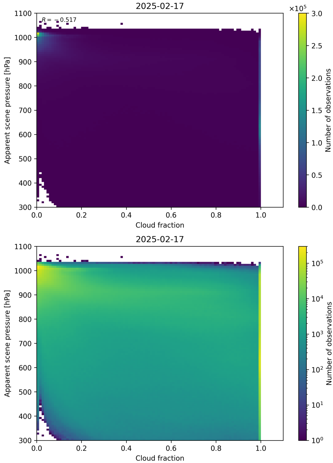
Figure 70: Scatter density plot of “Cloud fraction” against “Apparent scene pressure” for 2025-02-16 to 2025-02-18.
