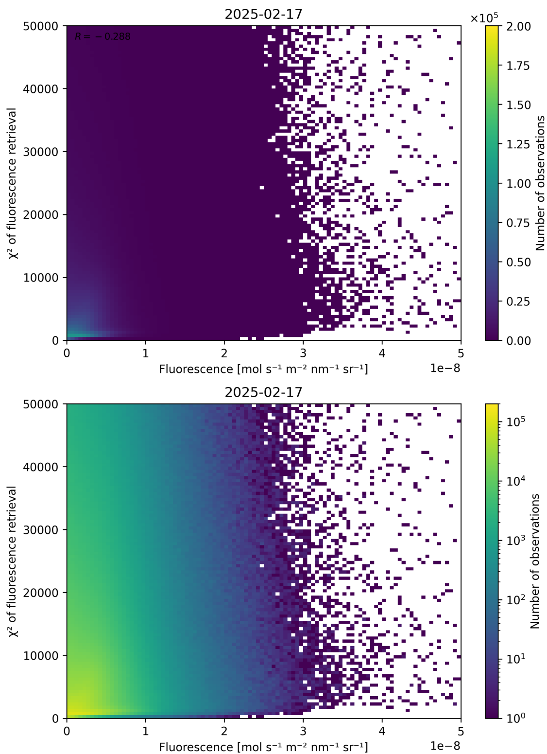
Figure 85: Scatter density plot of “Fluorescence” against “ \chi^2 of fluorescence retrieval” for 2025-02-16 to 2025-02-18.
