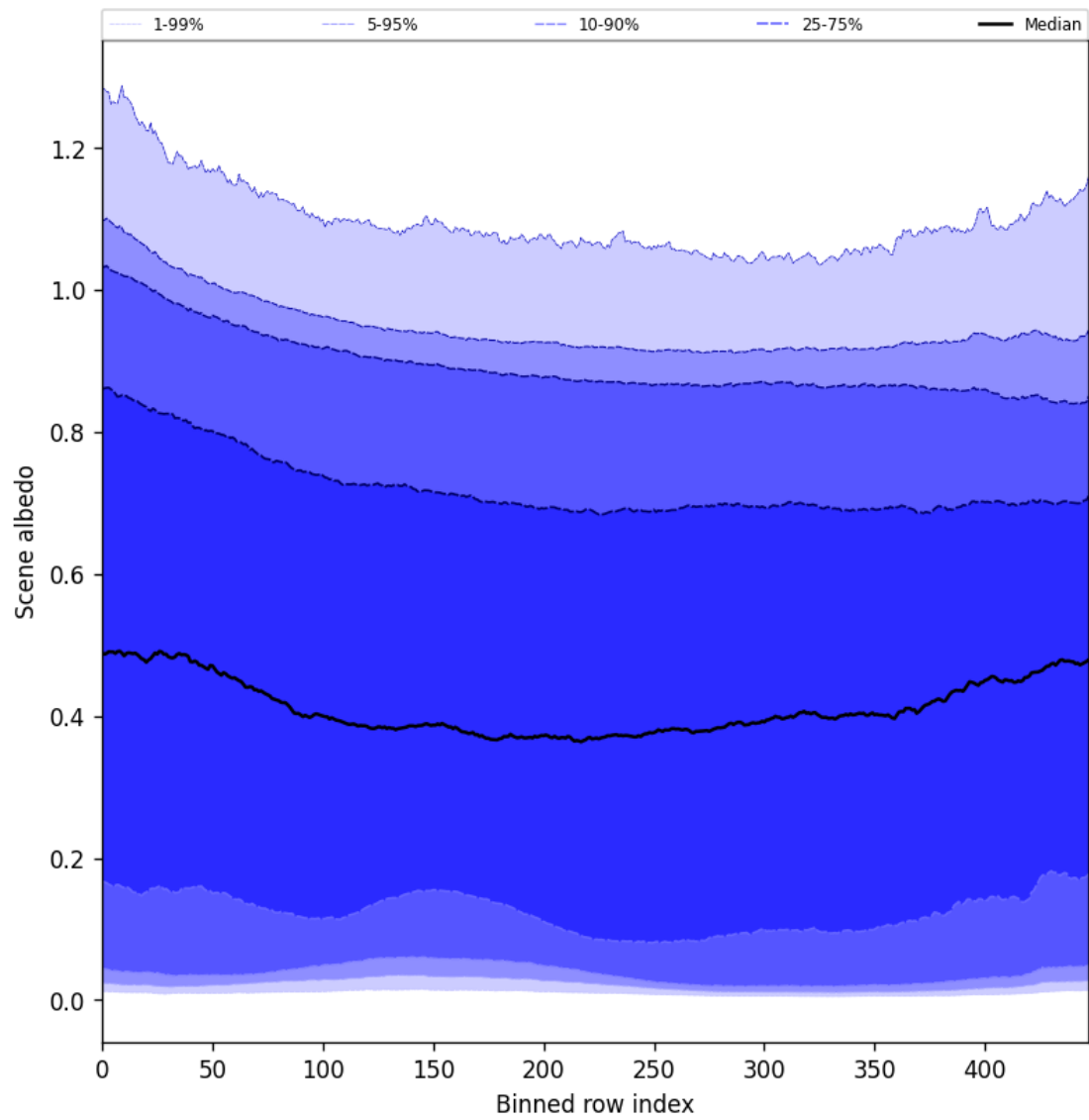
Figure 51: Along track statistics of “Scene albedo” for 2025-02-16 to 2025-02-18
