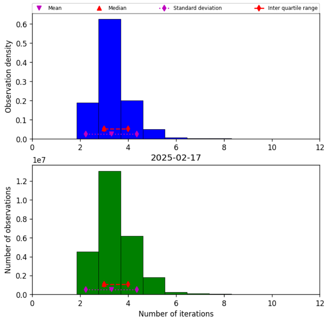
Figure 39: Histogram of “Number of iterations” for 2025-02-16 to 2025-02-18
