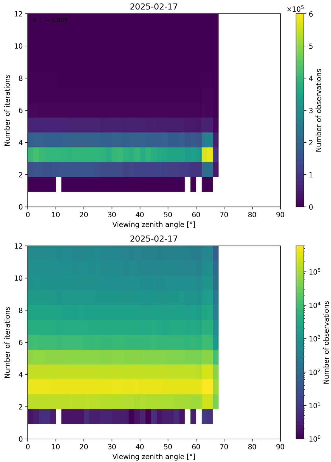
Figure 124: Scatter density plot of “Viewing zenith angle” against “Number of iterations” for 2025-02-16 to 2025-02-18.
