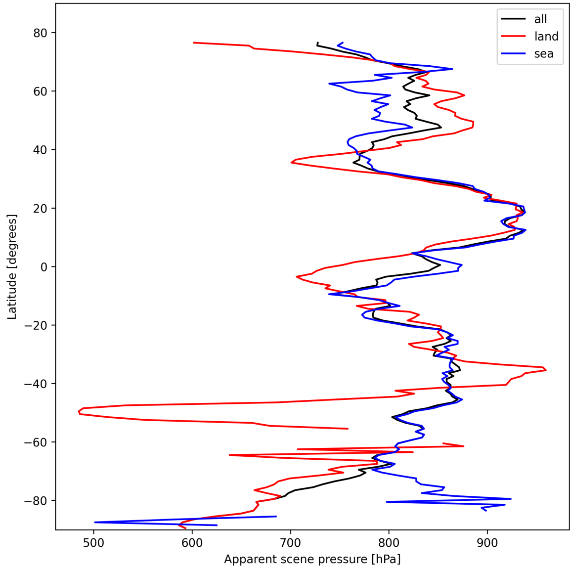
Figure 19: Zonal average of “Apparent scene pressure” for 2025-02-16 to 2025-02-18.
