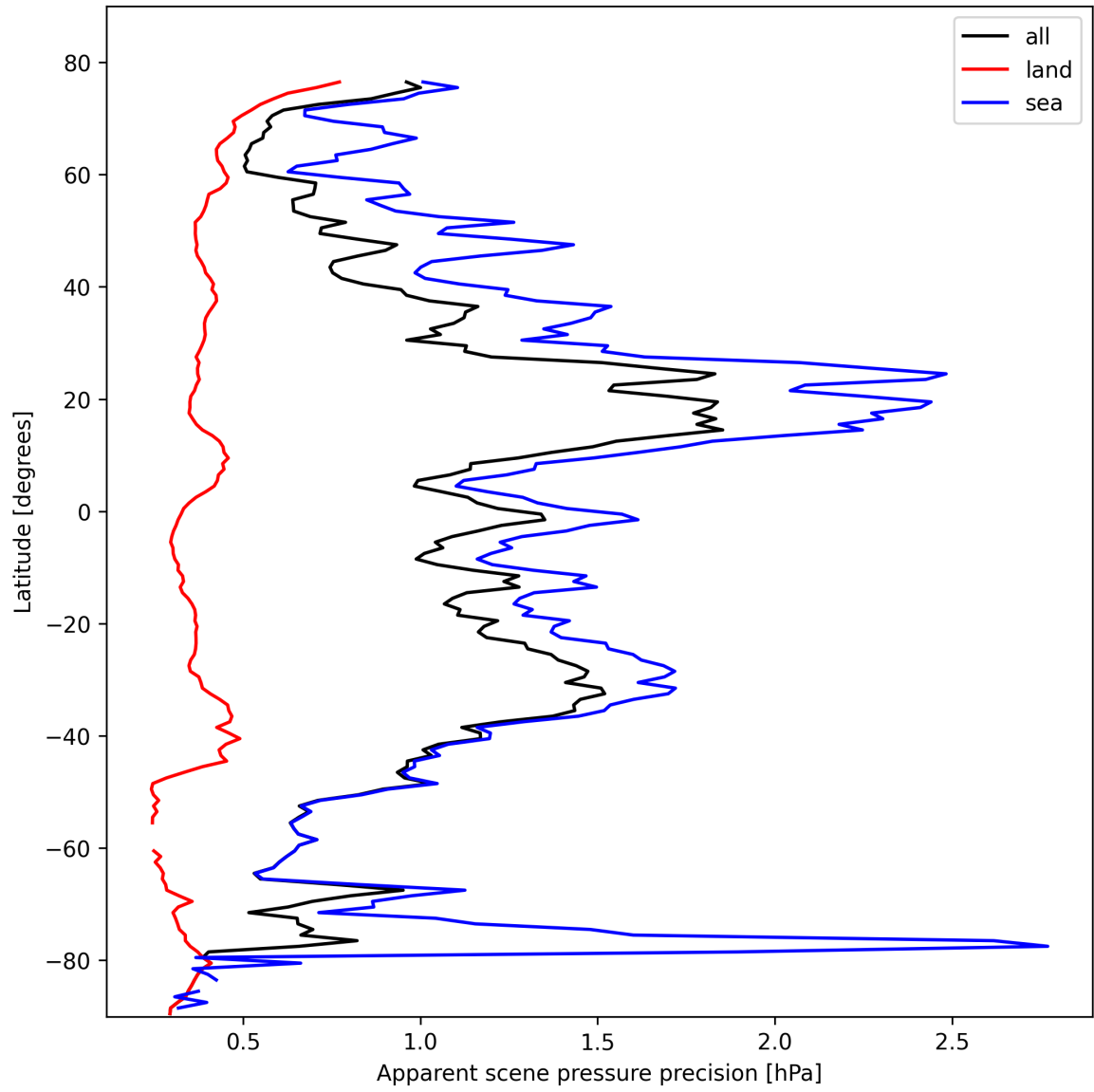
Figure 20: Zonal average of “Apparent scene pressure precision” for 2025-02-16 to 2025-02-18.
