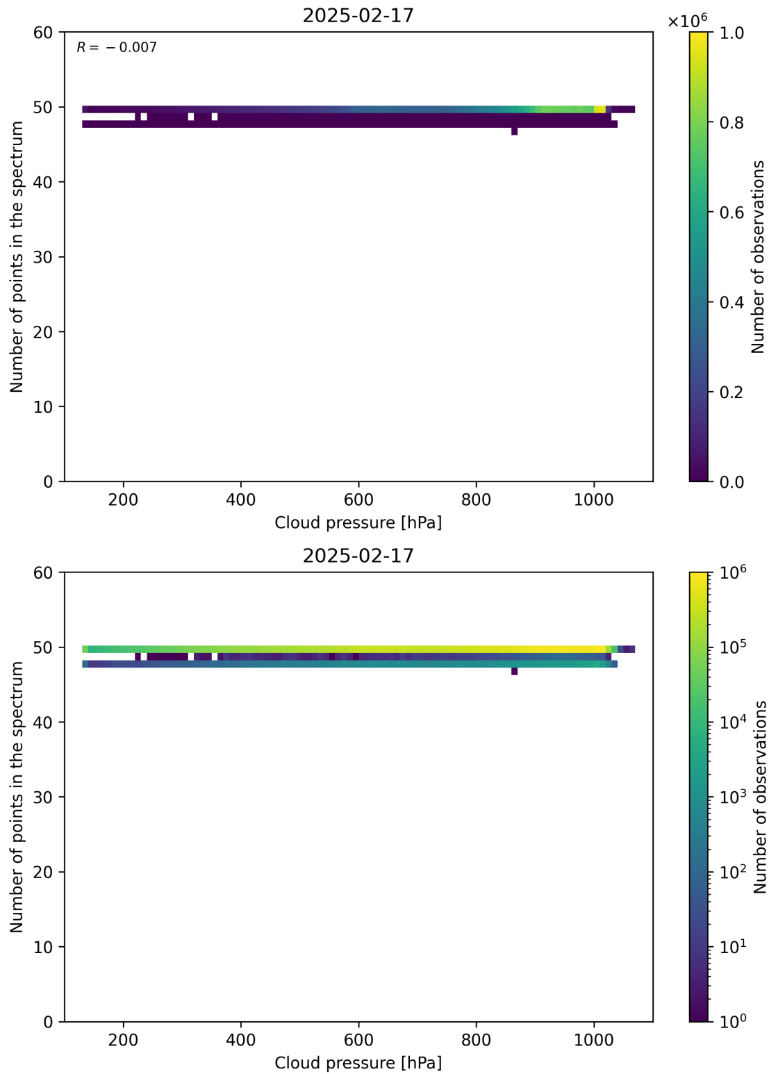
Figure 82: Scatter density plot of “Cloud pressure” against “Number of points in the spectrum” for 2025-02-16 to 2025-02-18.
