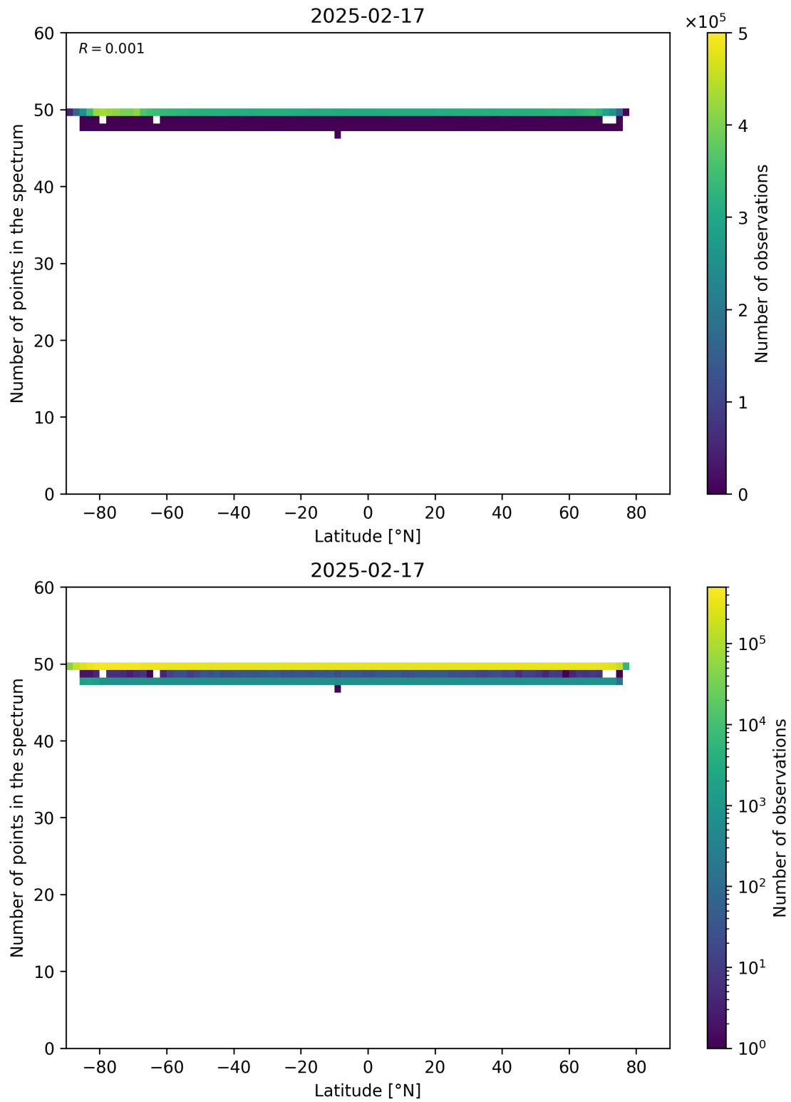
Figure 94: Scatter density plot of “Latitude” against “Number of points in the spectrum” for 2025-02-16 to 2025-02-18.
