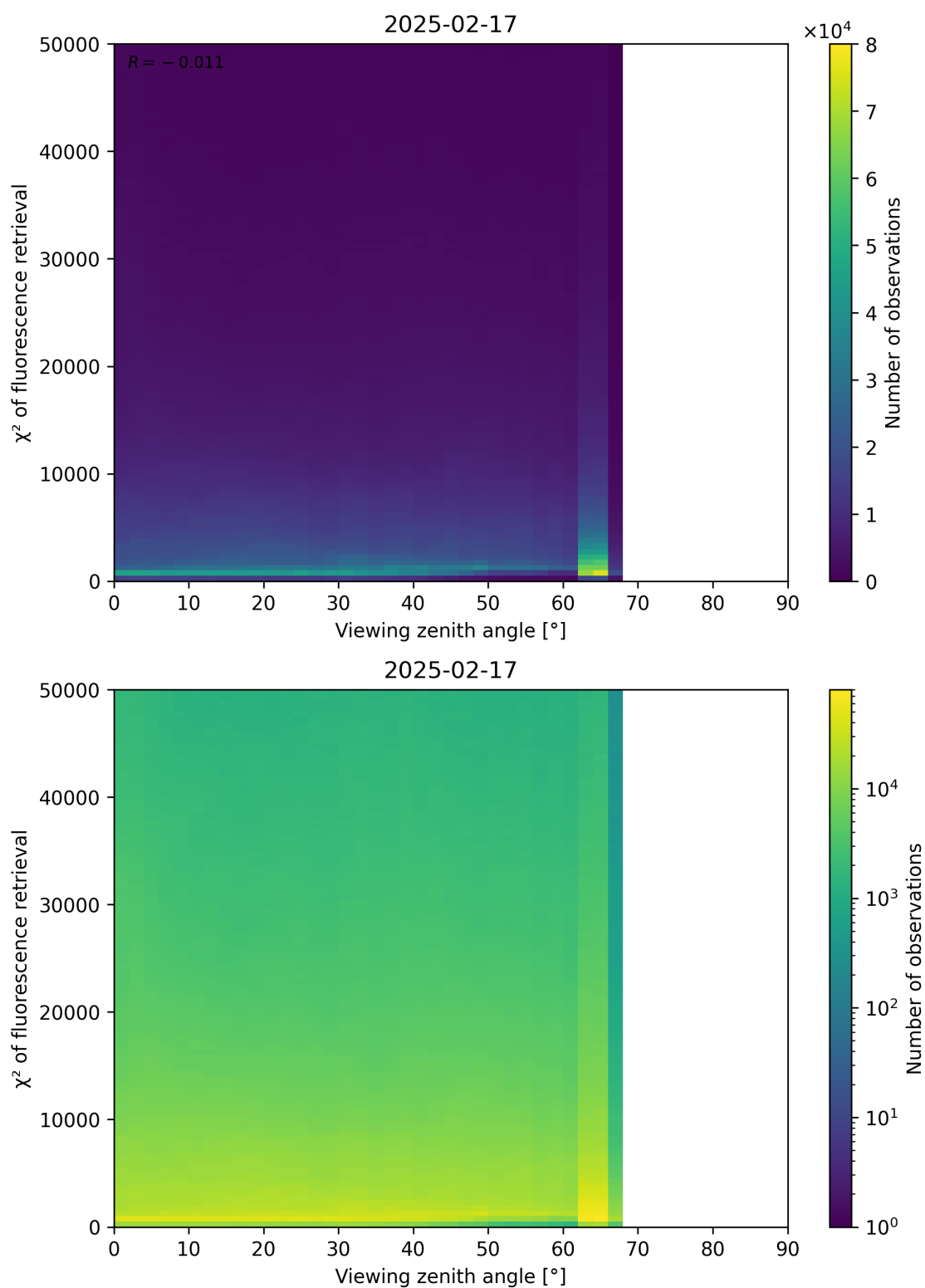
Figure 119: Scatter density plot of “Viewing zenith angle” against “ \chi^2 of fluorescence retrieval” for 2025-02-16 to 2025-02-18.
