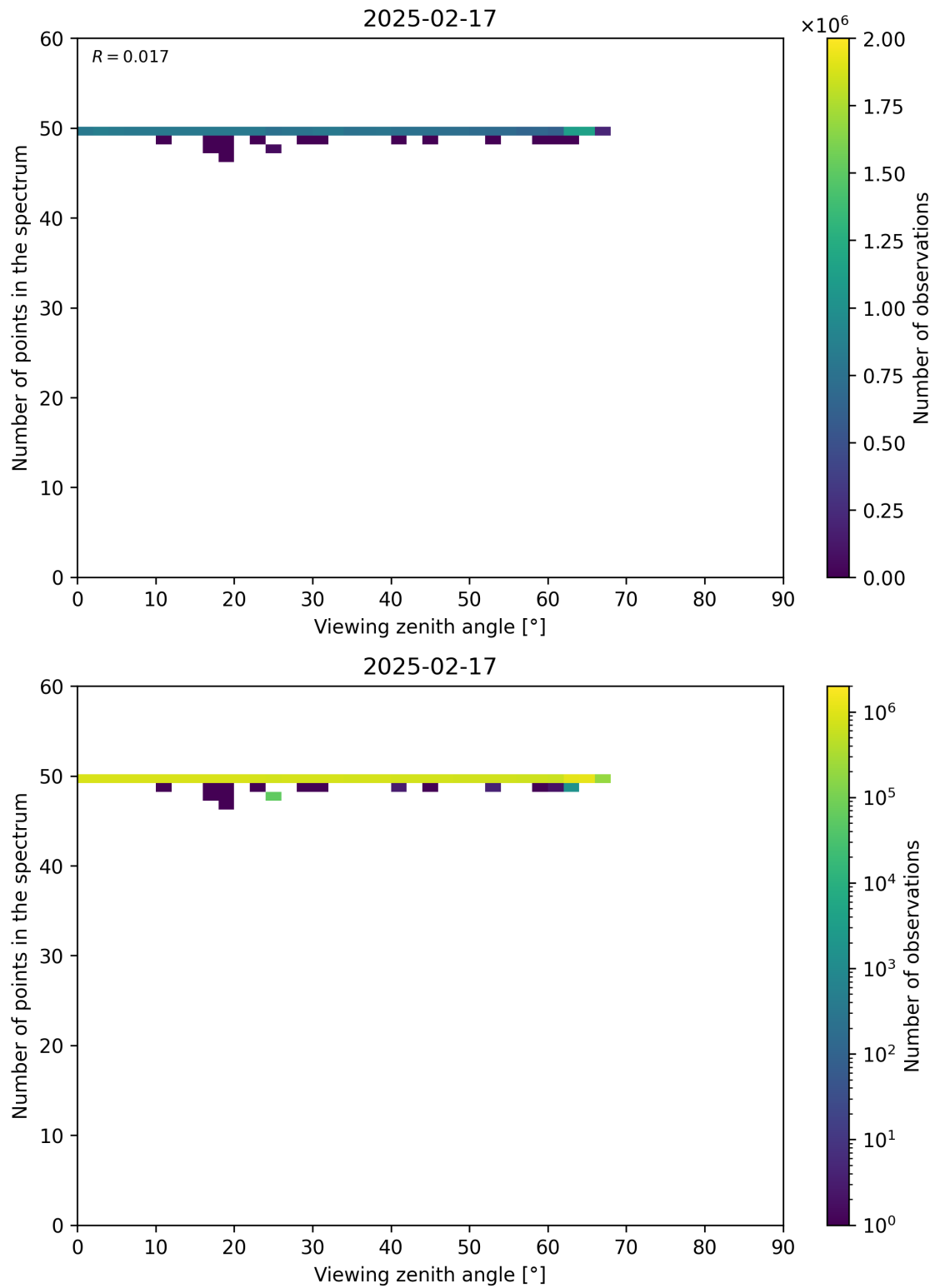
Figure 125: Scatter density plot of “Viewing zenith angle” against “Number of points in the spectrum” for 2025-02-16 to 2025-02-18.
