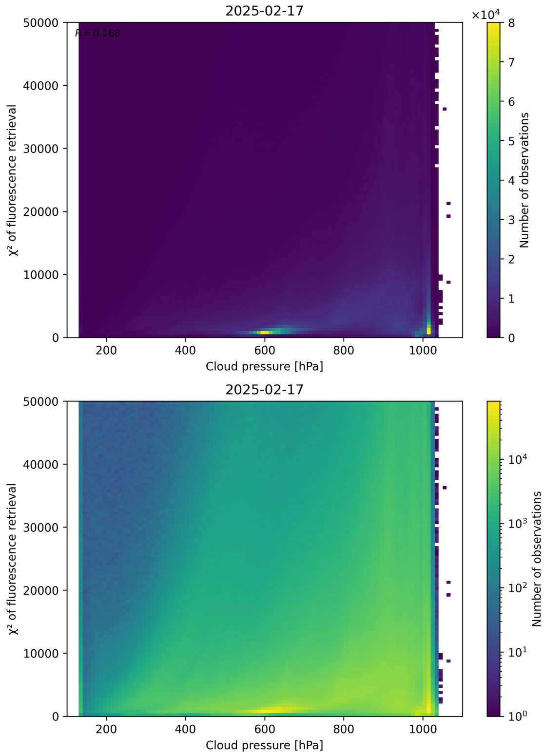
Figure 78: Scatter density plot of “Cloud pressure” against “ \chi^2 of fluorescence retrieval” for 2025-02-16 to 2025-02-18.
