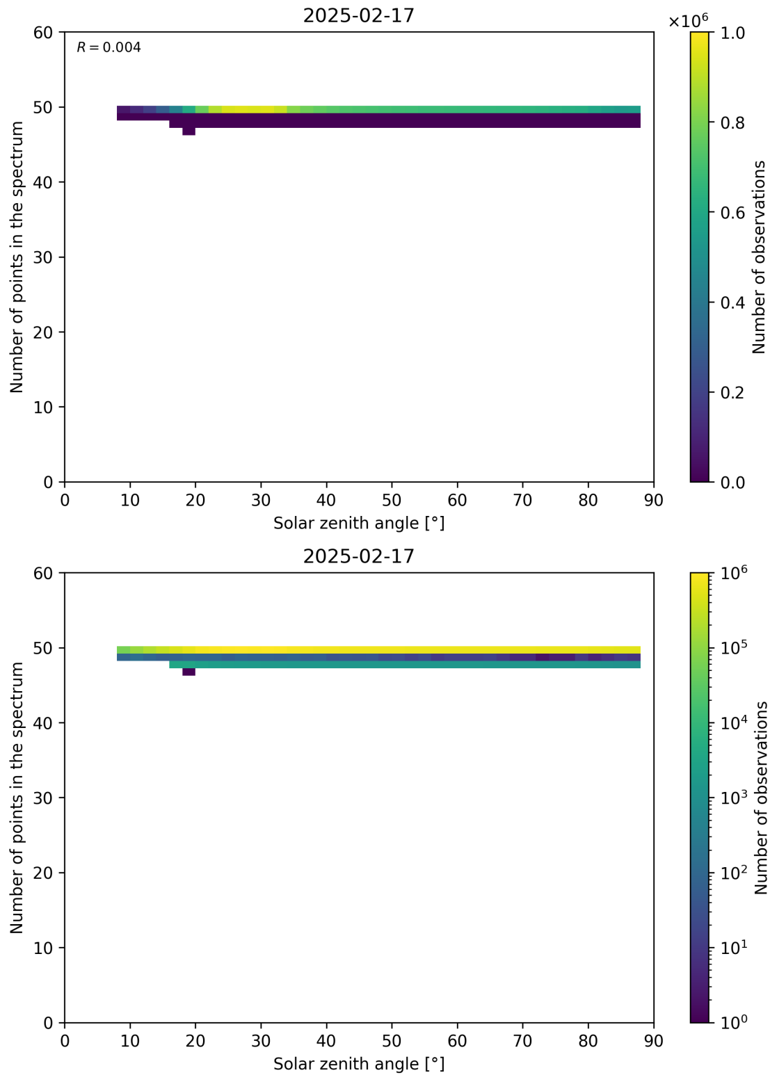
Figure 115: Scatter density plot of “Solar zenith angle” against “Number of points in the spectrum” for 2025-02-16 to 2025-02-18.
