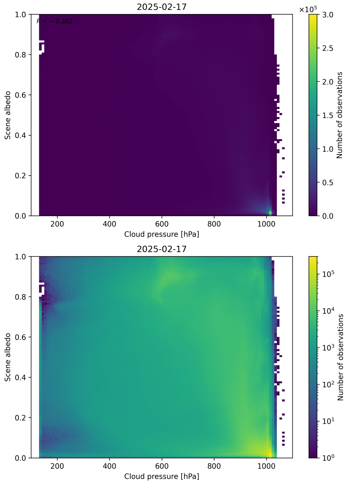
Figure 83: Scatter density plot of “Cloud pressure” against “Scene albedo” for 2025-02-16 to 2025-02-18.
