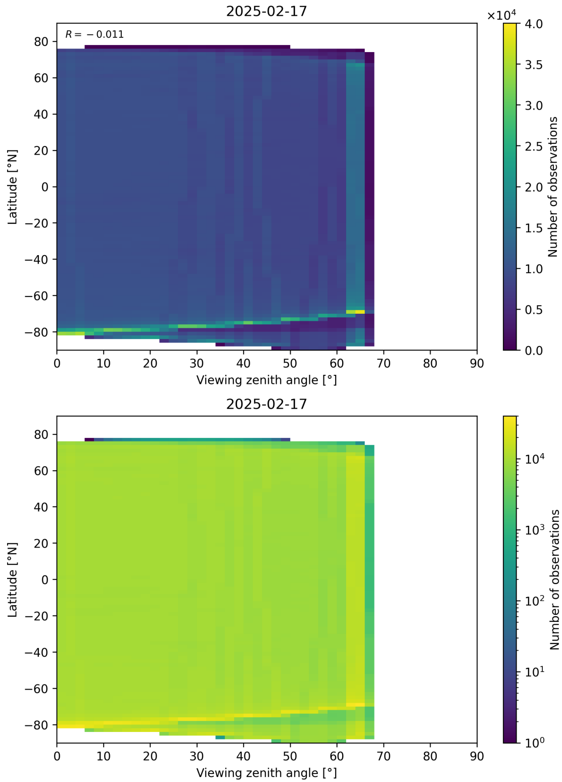
Figure 123: Scatter density plot of “Viewing zenith angle” against “Latitude” for 2025-02-16 to 2025-02-18.
