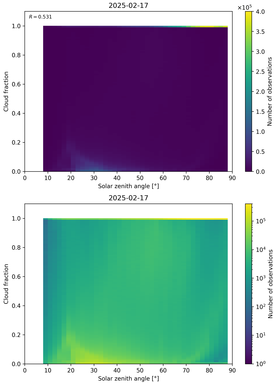
Figure 110: Scatter density plot of “Solar zenith angle” against “Cloud fraction” for 2025-02-16 to 2025-02-18.
