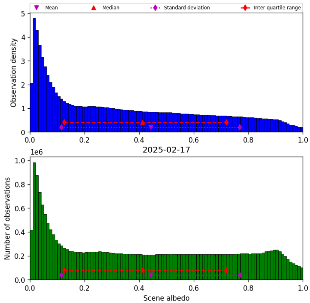
Figure 34: Histogram of “Scene albedo” for 2025-02-16 to 2025-02-18
