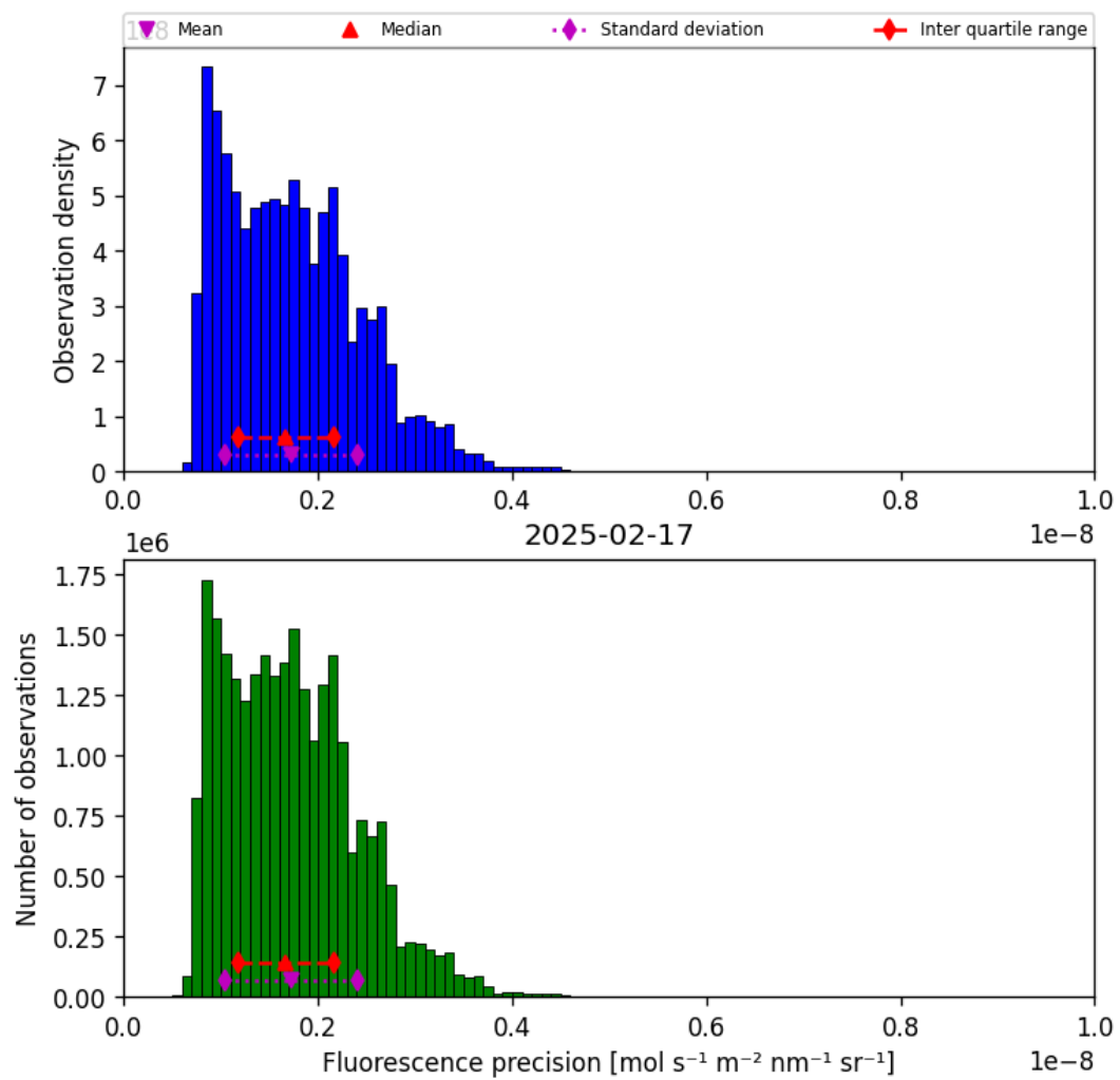
Figure 41: Histogram of “Fluorescence precision” for 2025-02-16 to 2025-02-18
