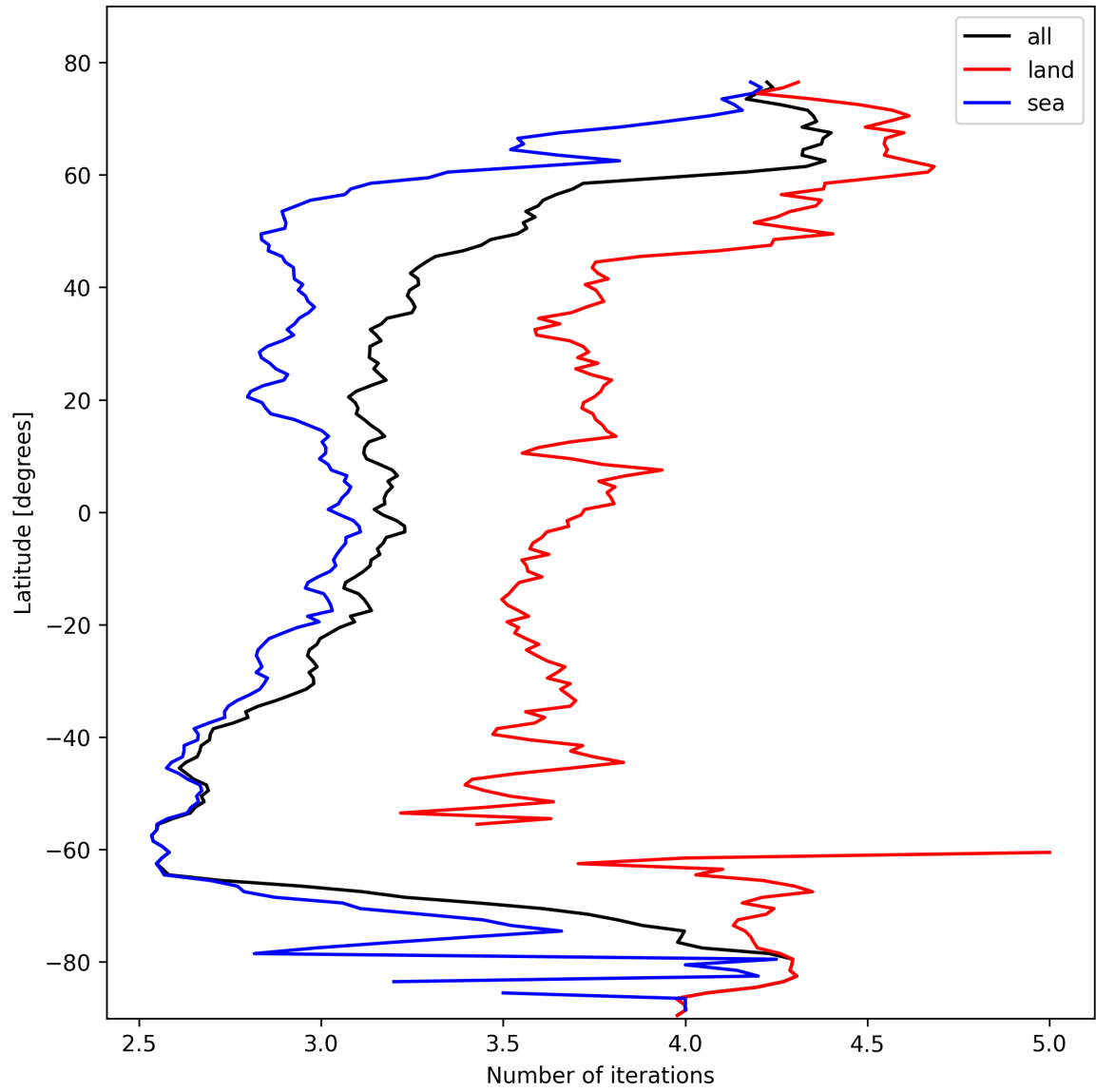
Figure 22: Zonal average of “Number of iterations” for 2025-02-16 to 2025-02-18.
