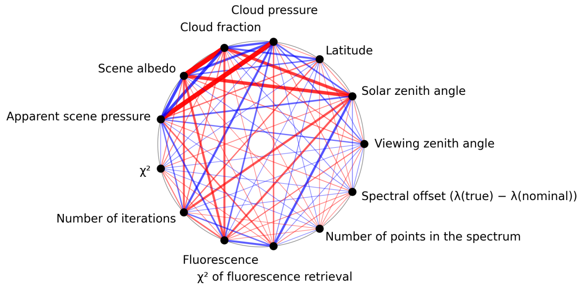
Figure 1: Map of correlation graph for 2025-02-16 to 2025-02-18.
