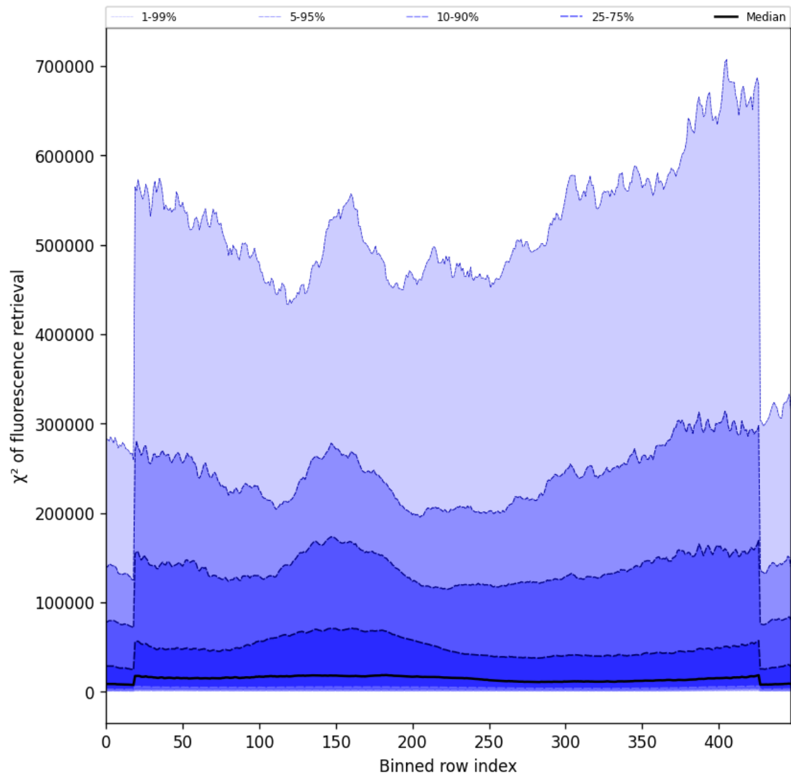
Figure 59: Along track statistics of “ \chi^2 of fluorescence retrieval” for 2025-02-16 to 2025-02-18
