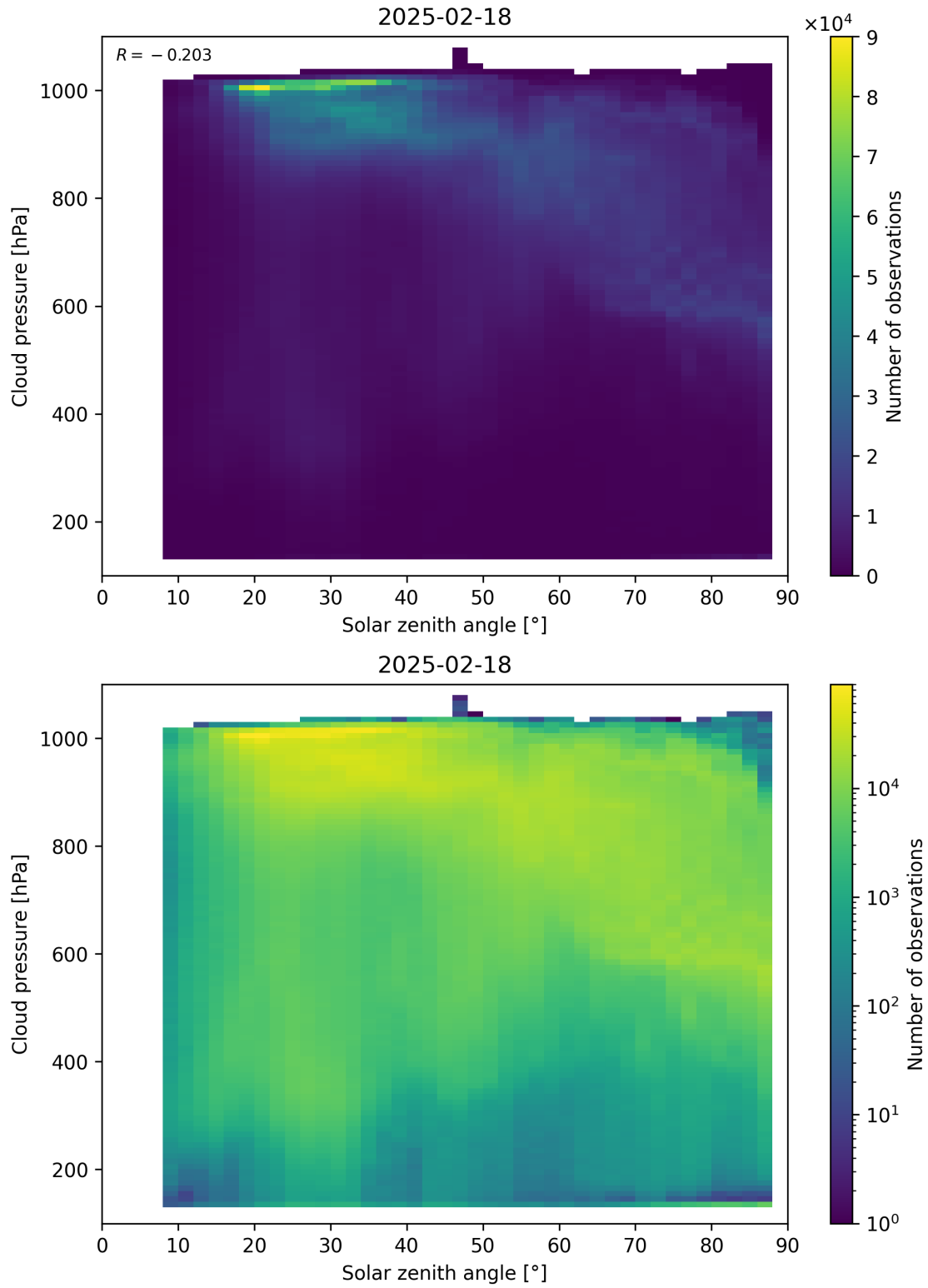
Figure 111: Scatter density plot of “Solar zenith angle” against “Cloud pressure” for 2025-02-18 to 2025-02-19.
