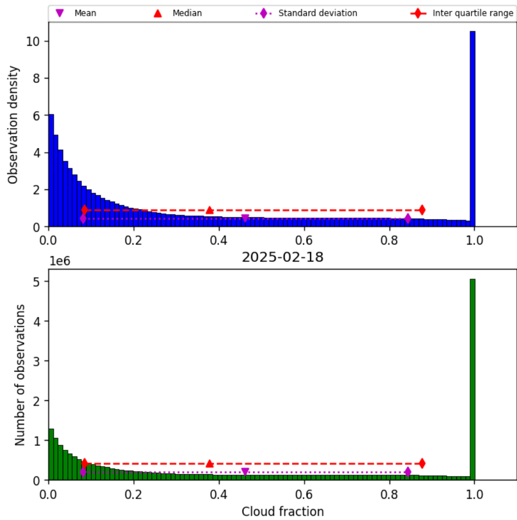
Figure 32: Histogram of “Cloud fraction” for 2025-02-18 to 2025-02-19
