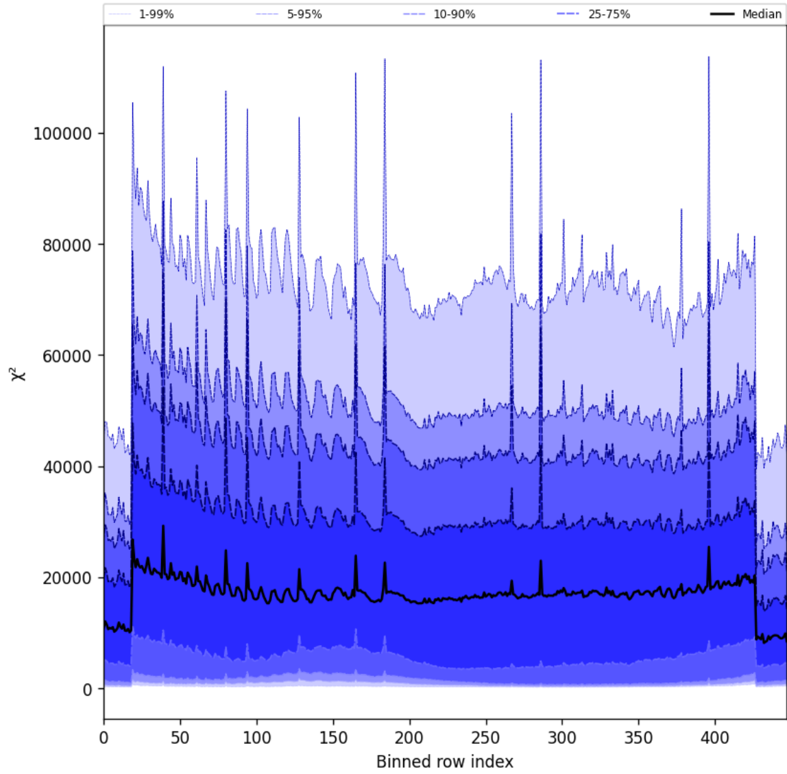
Figure 55: Along track statistics of “ \chi^2 ” for 2025-02-18 to 2025-02-19
