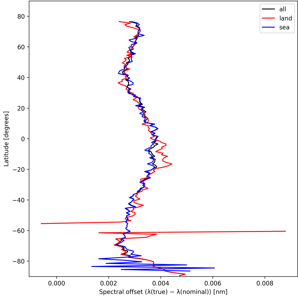
Figure 28: Zonal average of “Spectral offset ( \lambda_{\text{true}} - \lambda_{\text{nominal}} )” for 2025-02-18 to 2025-02-19.
