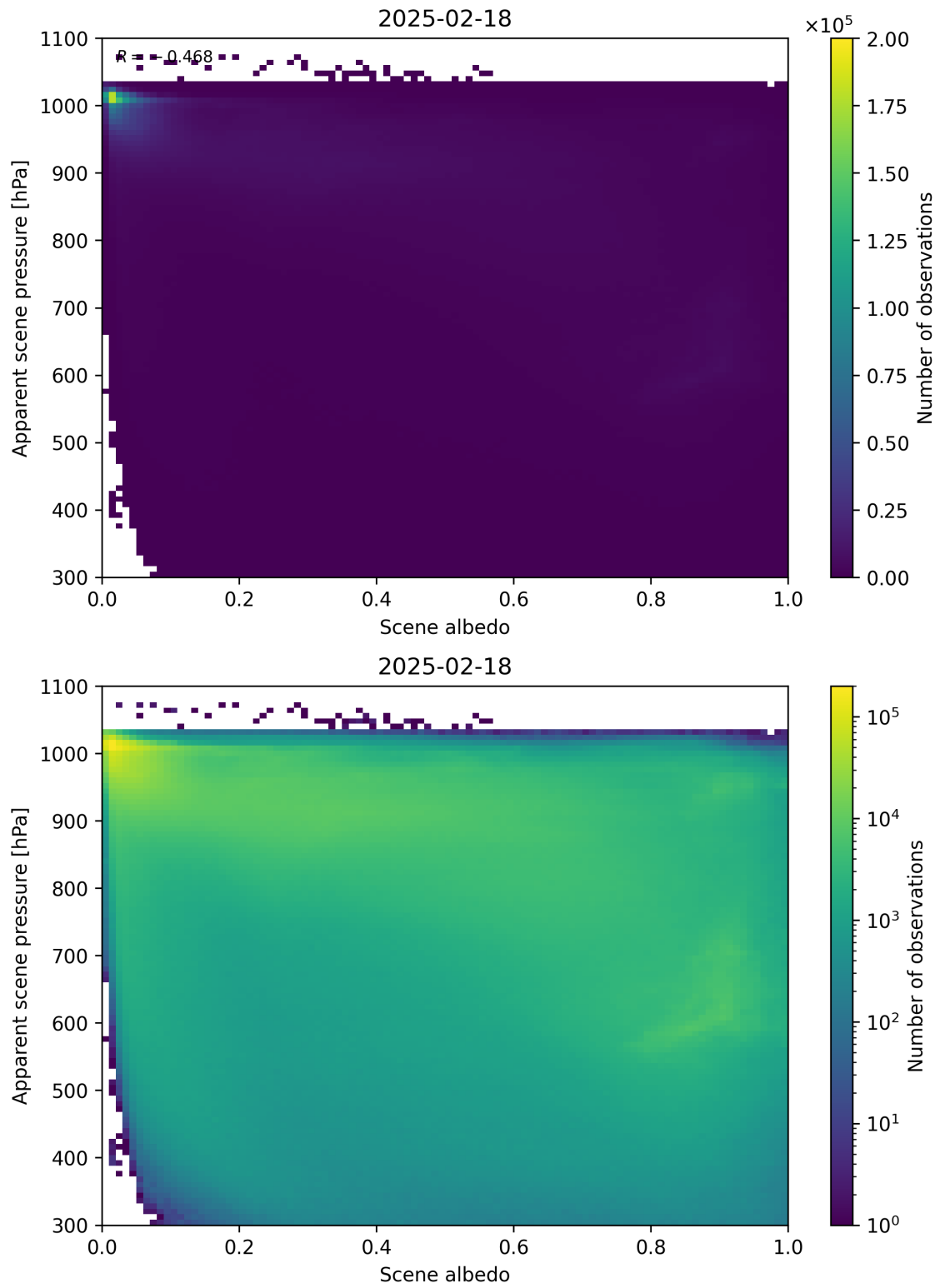
Figure 102: Scatter density plot of “Scene albedo” against “Apparent scene pressure” for 2025-02-18 to 2025-02-19.
