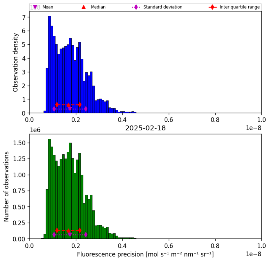
Figure 41: Histogram of “Fluorescence precision” for 2025-02-18 to 2025-02-19
