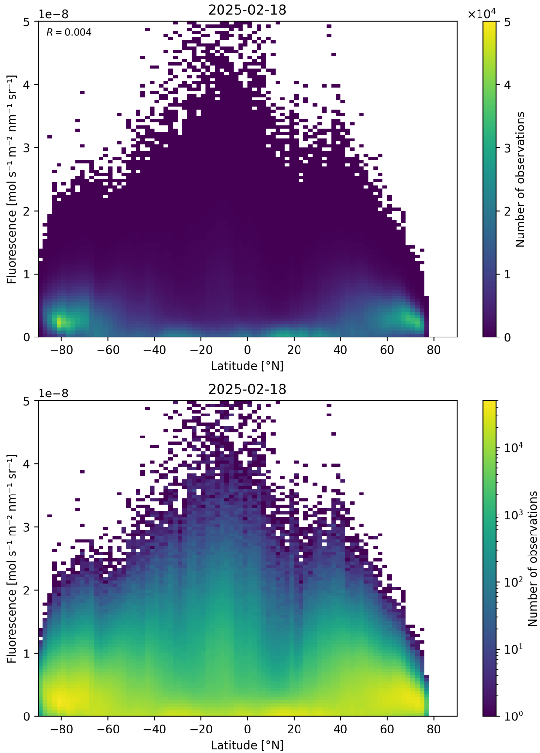
Figure 92: Scatter density plot of “Latitude” against “Fluorescence” for 2025-02-18 to 2025-02-19.
