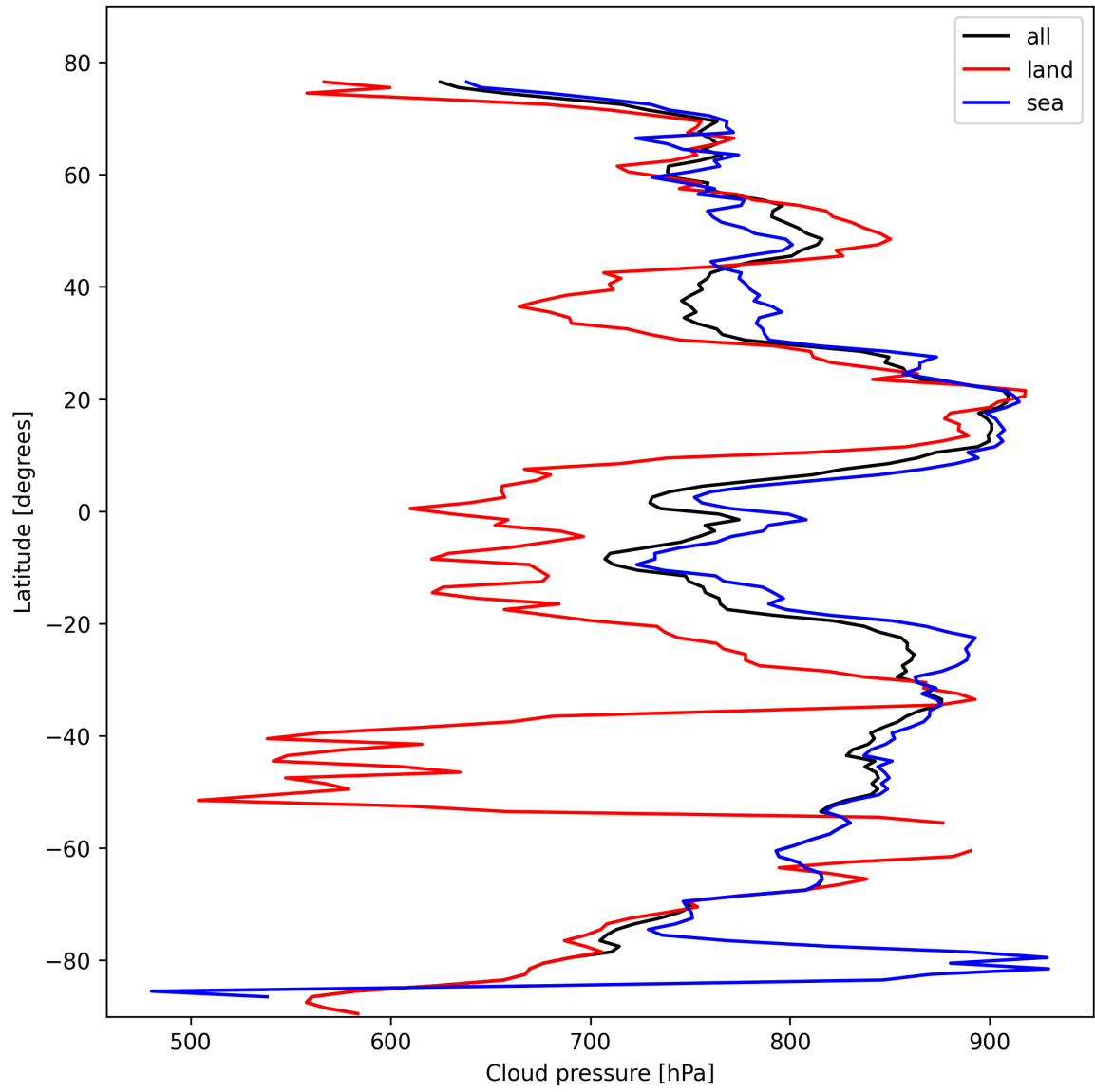
Figure 13: Zonal average of “Cloud pressure” for 2025-02-18 to 2025-02-19.
