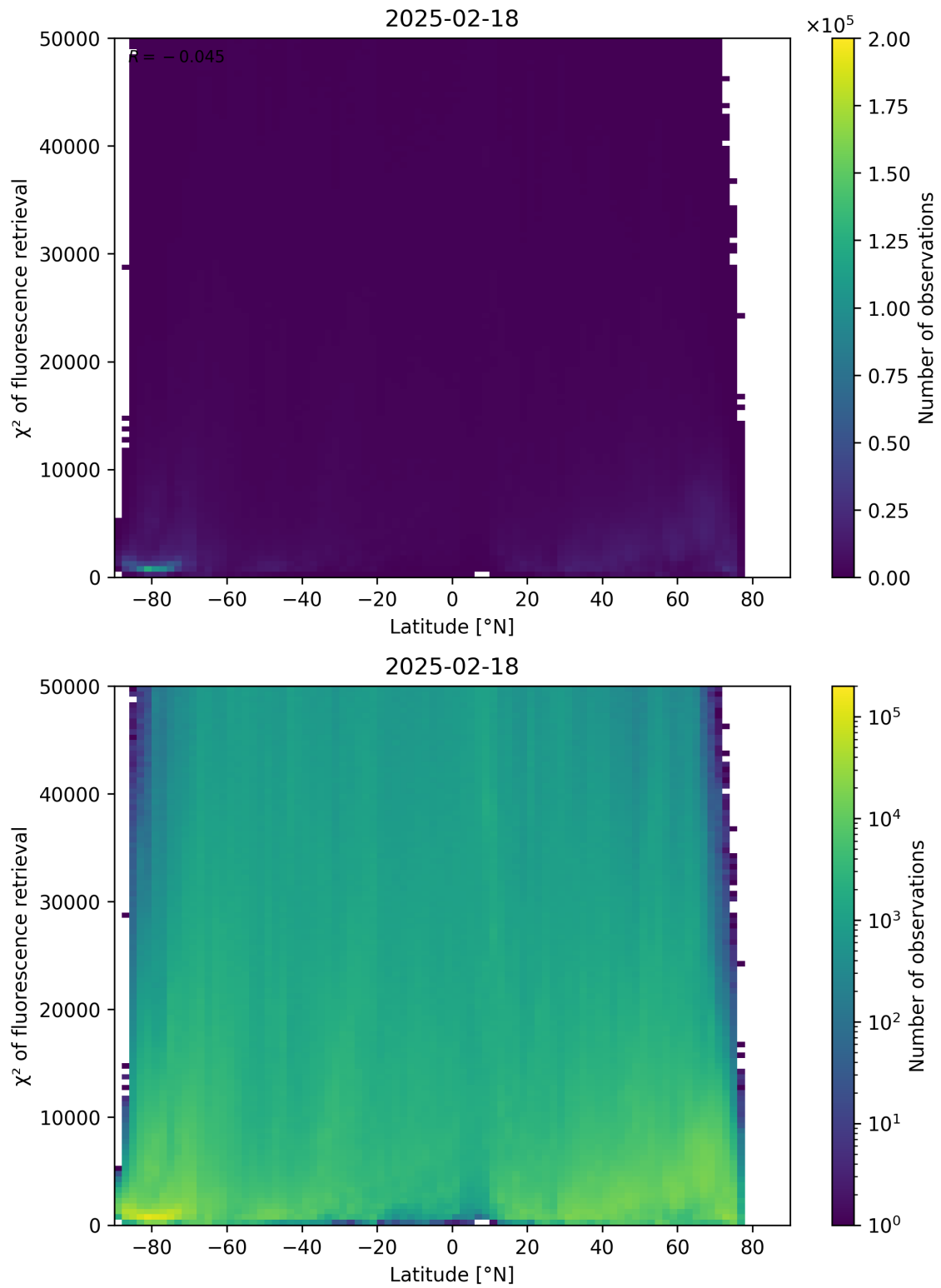
Figure 89: Scatter density plot of “Latitude” against “ \chi^2 of fluorescence retrieval” for 2025-02-18 to 2025-02-19.
