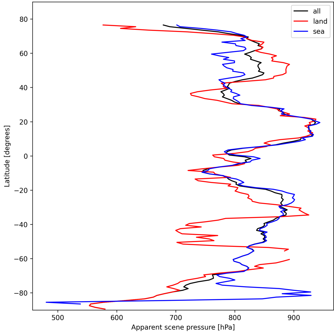
Figure 19: Zonal average of “Apparent scene pressure” for 2025-02-18 to 2025-02-19.
