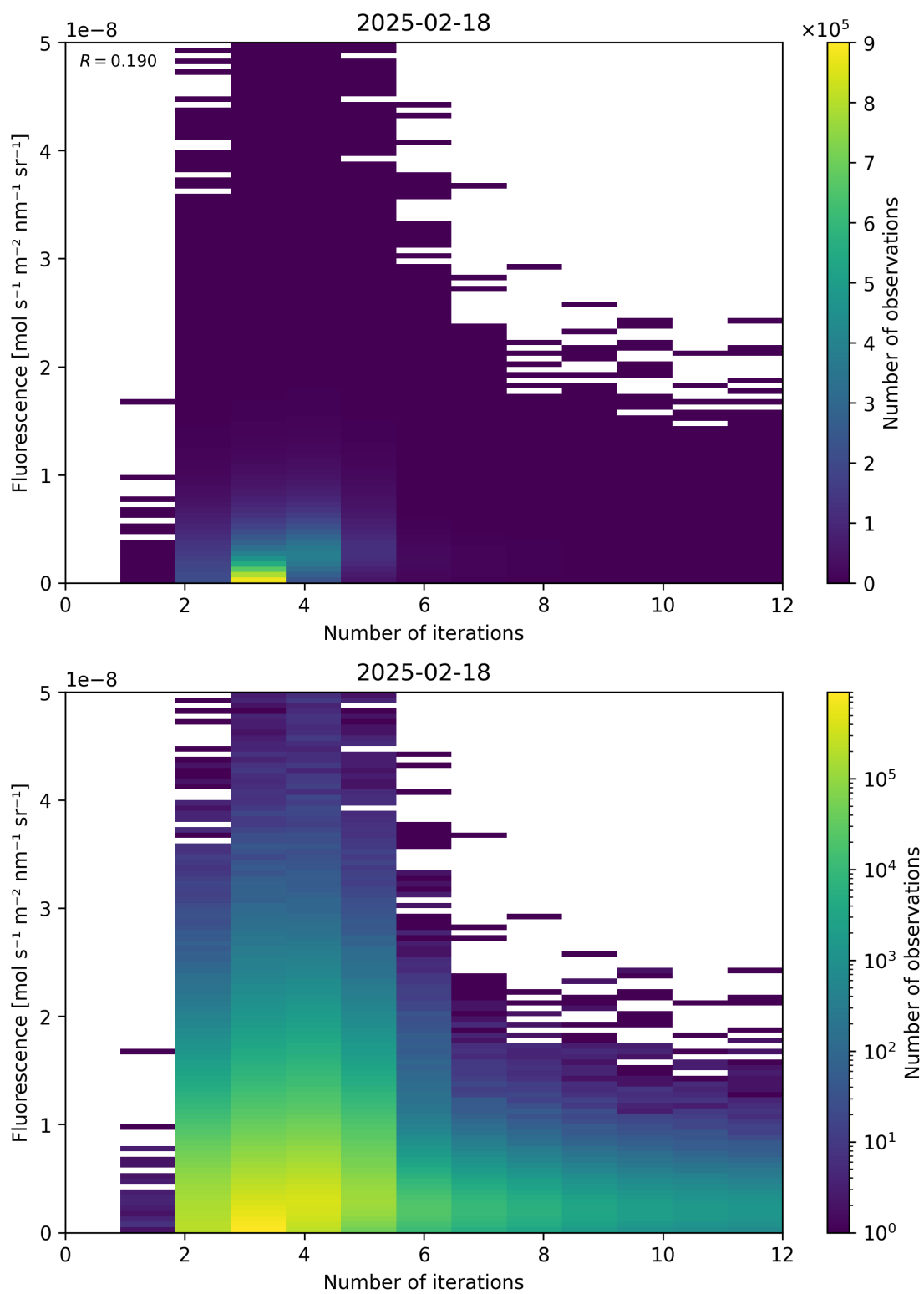
Figure 98: Scatter density plot of "Number of iterations" against "Fluorescence" for 2025-02-18 to 2025-02-19.
