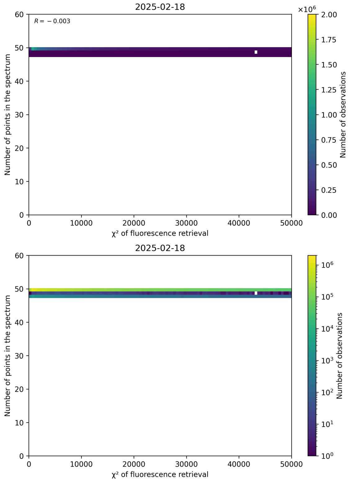
Figure 68: Scatter density plot of “ \chi^2 of fluorescence retrieval” against “Number of points in the spectrum” for 2025-02-18 to 2025-02-19.
