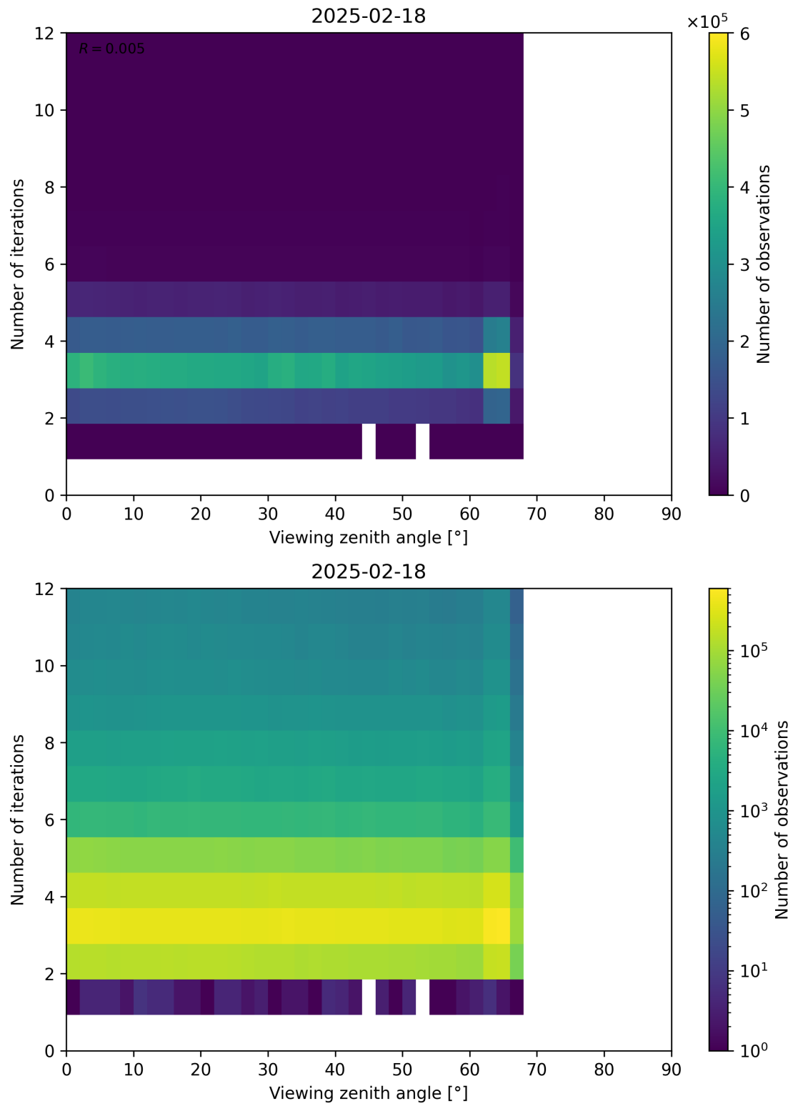
Figure 124: Scatter density plot of “Viewing zenith angle” against “Number of iterations” for 2025-02-18 to 2025-02-19.
