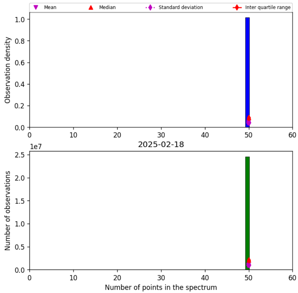
Figure 44: Histogram of “Number of points in the spectrum” for 2025-02-18 to 2025-02-19
