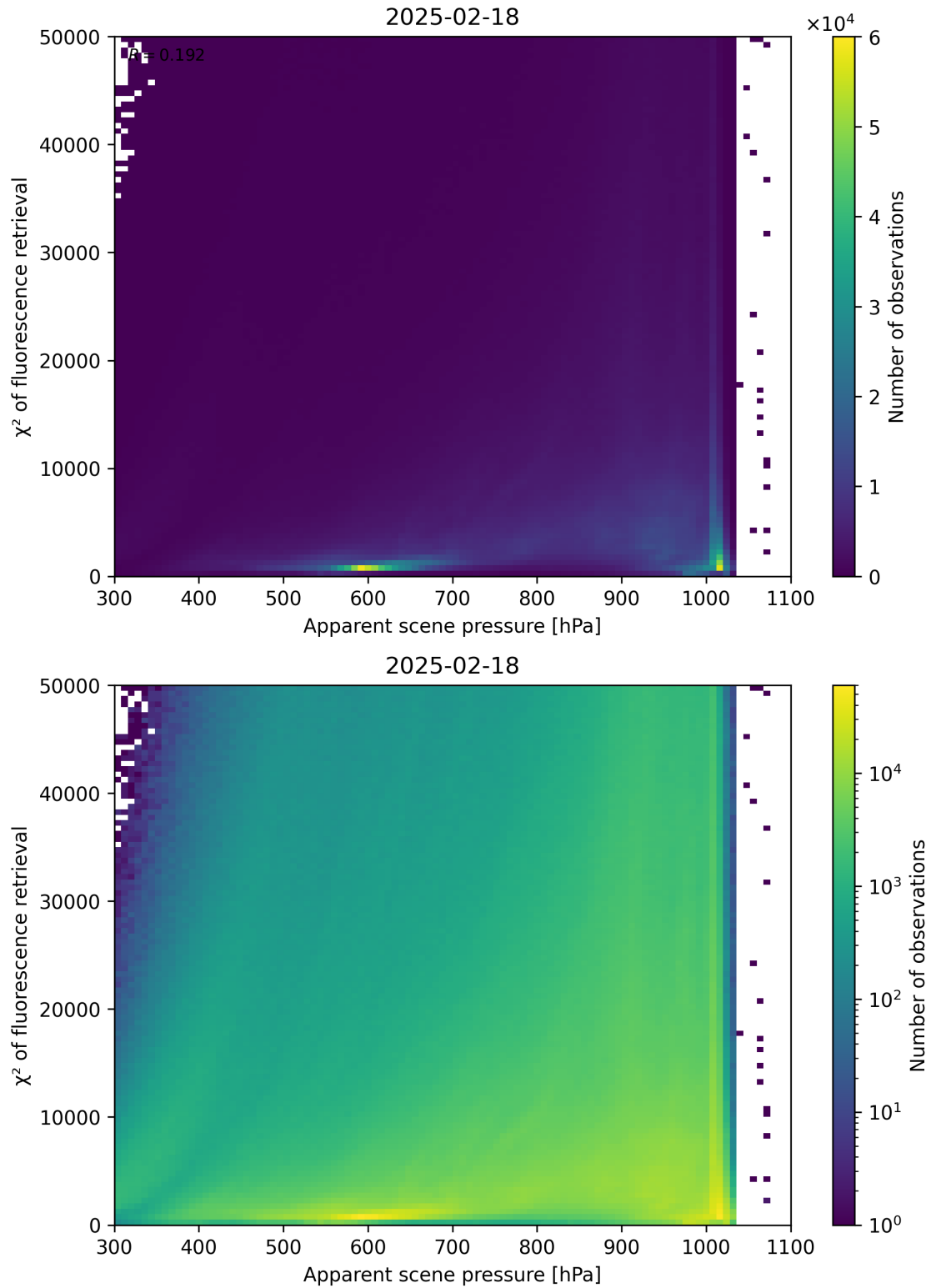
Figure 63: Scatter density plot of “Apparent scene pressure” against “ \chi^2 of fluorescence retrieval” for 2025-02-18 to 2025-02-19.
