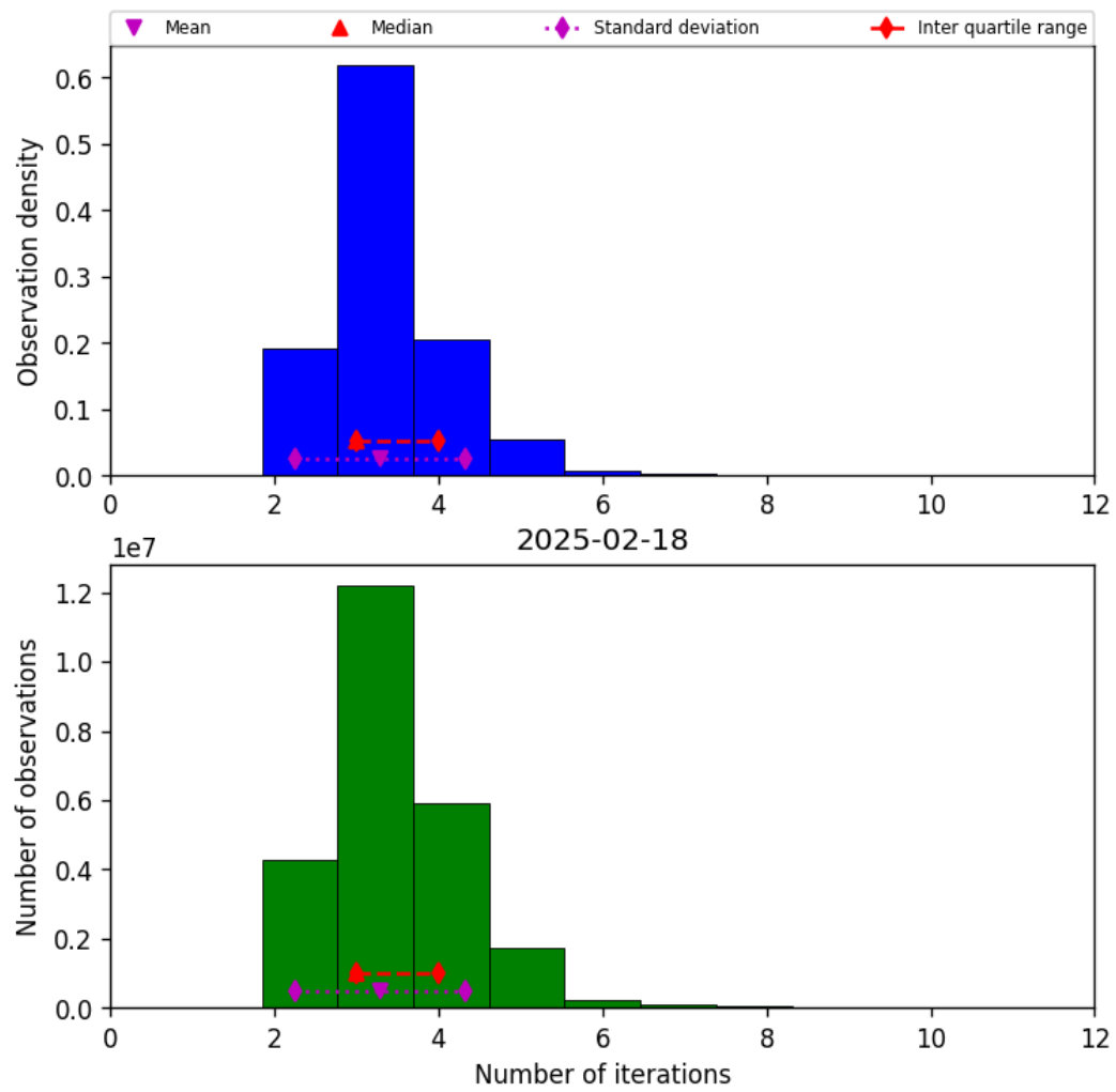
Figure 39: Histogram of “Number of iterations” for 2025-02-18 to 2025-02-19
