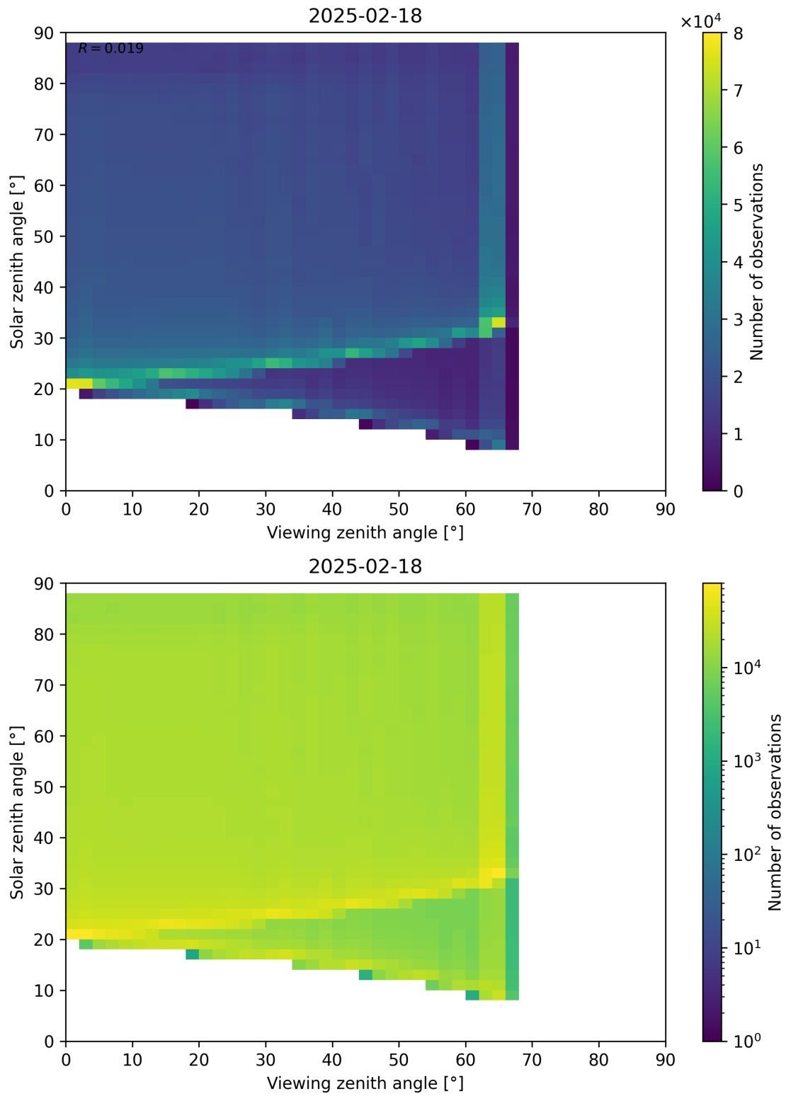
Figure 127: Scatter density plot of “Viewing zenith angle” against “Solar zenith angle” for 2025-02-18 to 2025-02-19.
