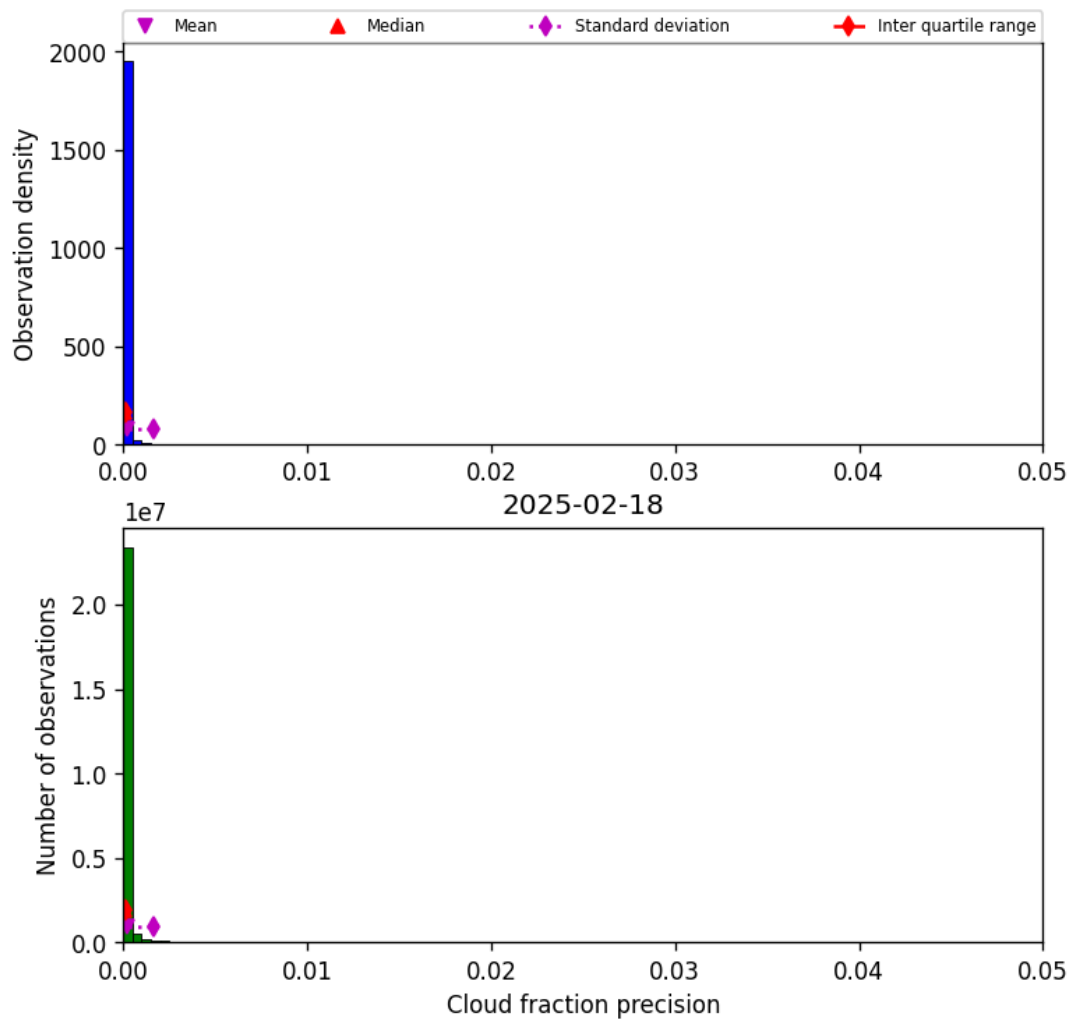
Figure 33: Histogram of “Cloud fraction precision” for 2025-02-18 to 2025-02-19
