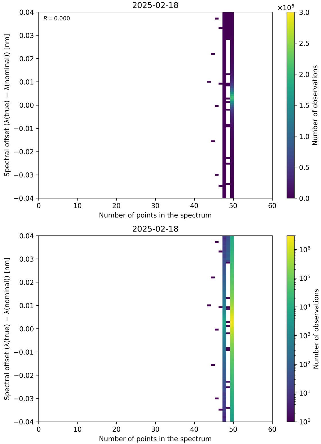
Figure 101: Scatter density plot of “Number of points in the spectrum” against “Spectral offset ( \lambda_{\text{true}} - \lambda_{\text{nominal}} )” for 2025-02-18 to 2025-02-19.
