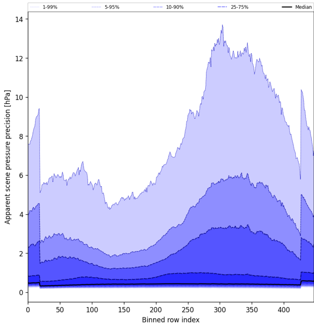
Figure 54: Along track statistics of “Apparent scene pressure precision” for 2025-02-18 to 2025-02-19
