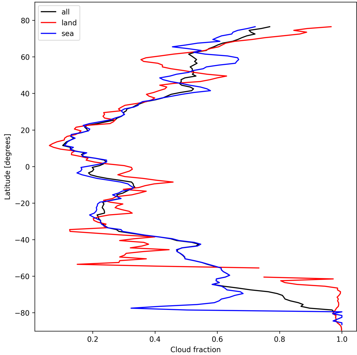
Figure 15: Zonal average of “Cloud fraction” for 2025-02-18 to 2025-02-19.
