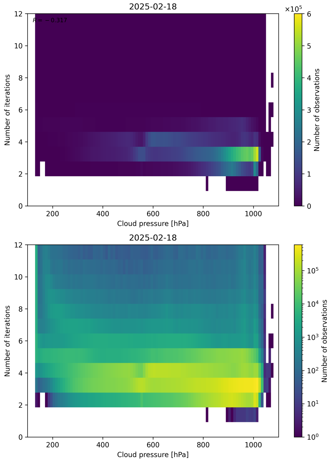
Figure 81: Scatter density plot of “Cloud pressure” against “Number of iterations” for 2025-02-18 to 2025-02-19.
