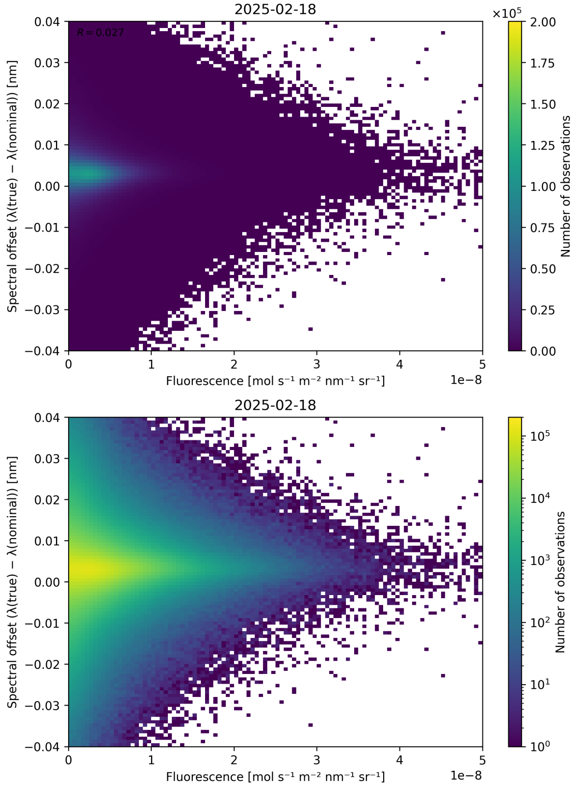
Figure 87: Scatter density plot of “Fluorescence” against “Spectral offset ( \lambda_{\text{true}} - \lambda_{\text{nominal}} )” for 2025-02-18 to 2025-02-19.
