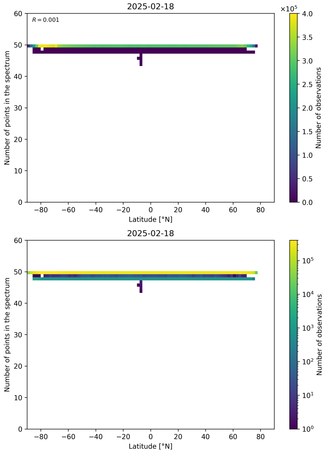
Figure 94: Scatter density plot of “Latitude” against “Number of points in the spectrum” for 2025-02-18 to 2025-02-19.
