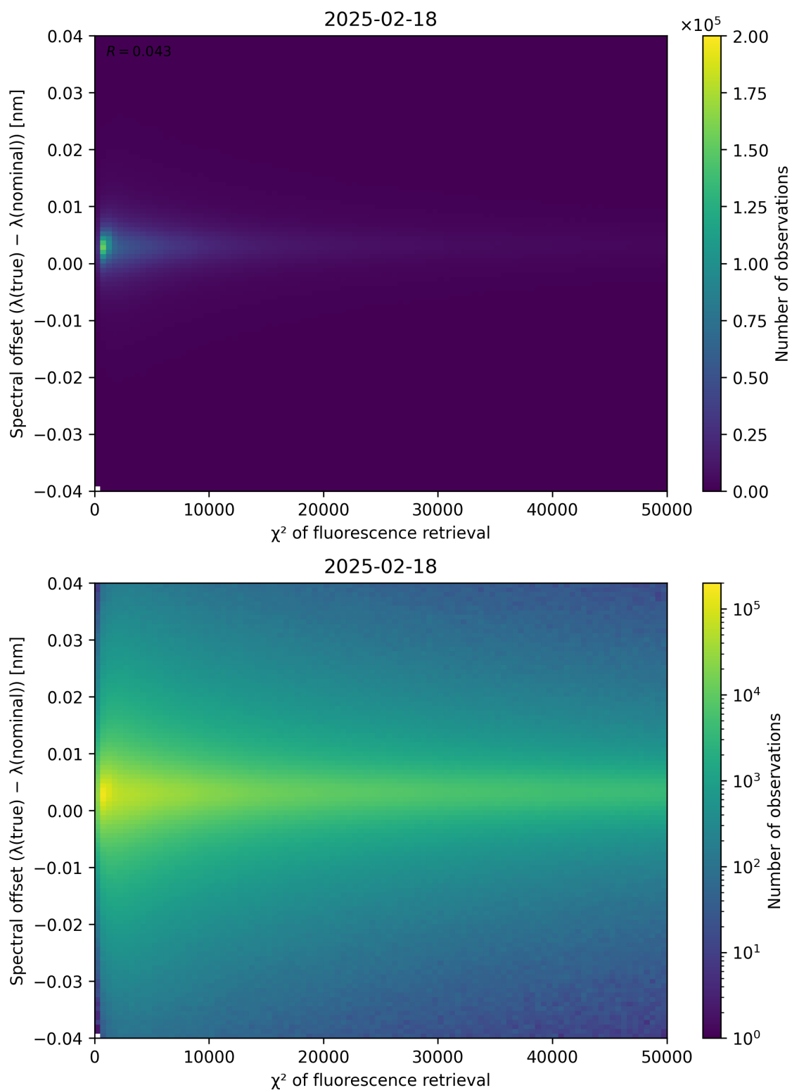
Figure 69: Scatter density plot of “ \chi^2 of fluorescence retrieval” against “Spectral offset ( \lambda_{\text{true}} - \lambda_{\text{nominal}} )” for 2025-02-18 to 2025-02-19.
