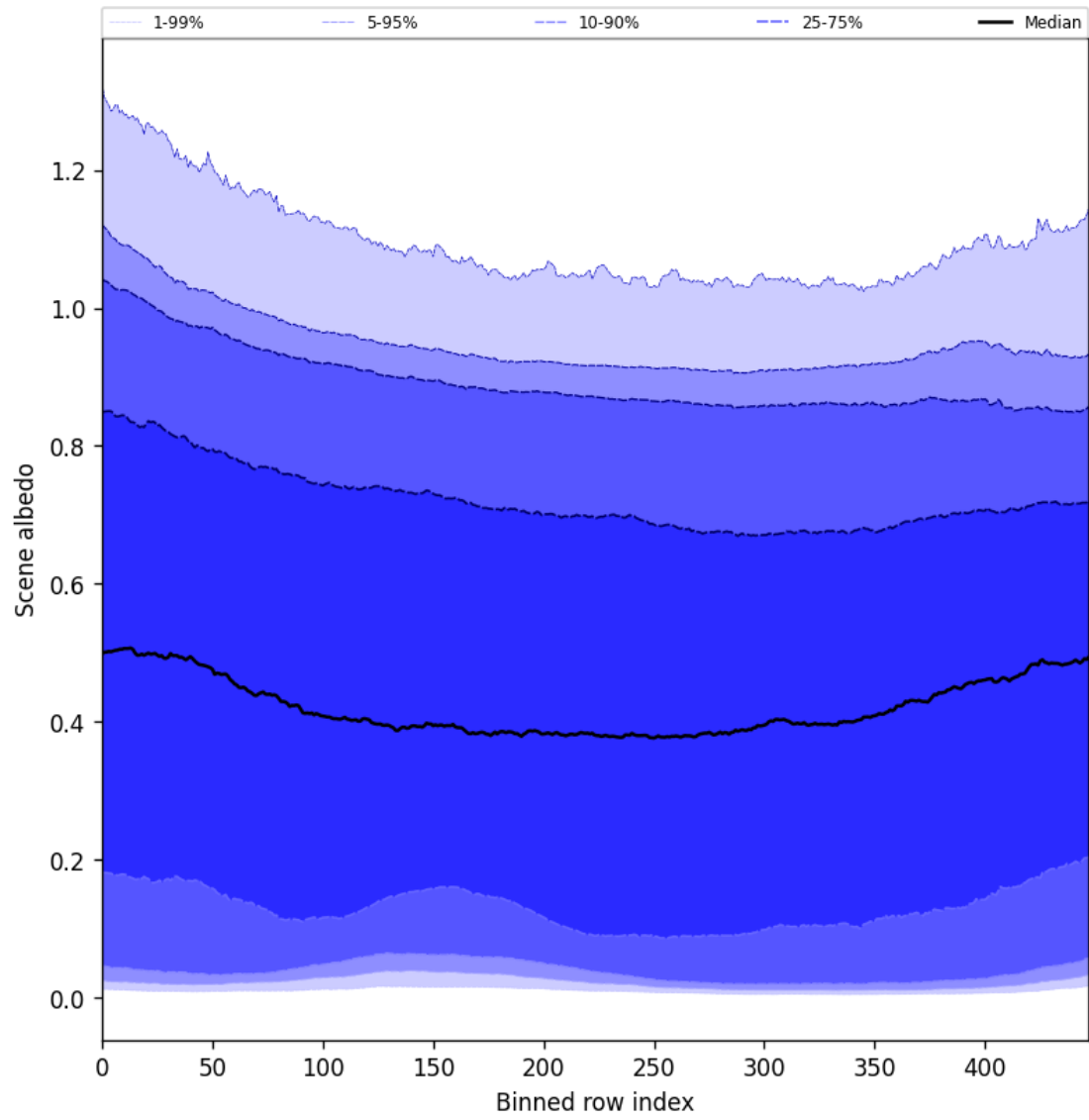
Figure 51: Along track statistics of “Scene albedo” for 2025-02-18 to 2025-02-19
