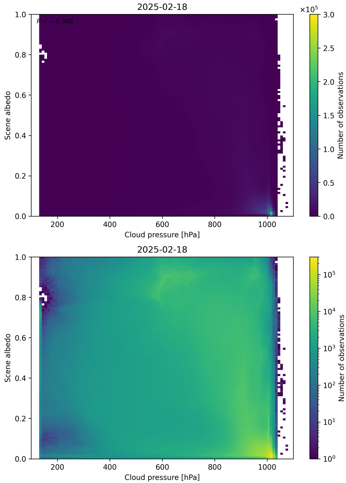
Figure 83: Scatter density plot of “Cloud pressure” against “Scene albedo” for 2025-02-18 to 2025-02-19.
