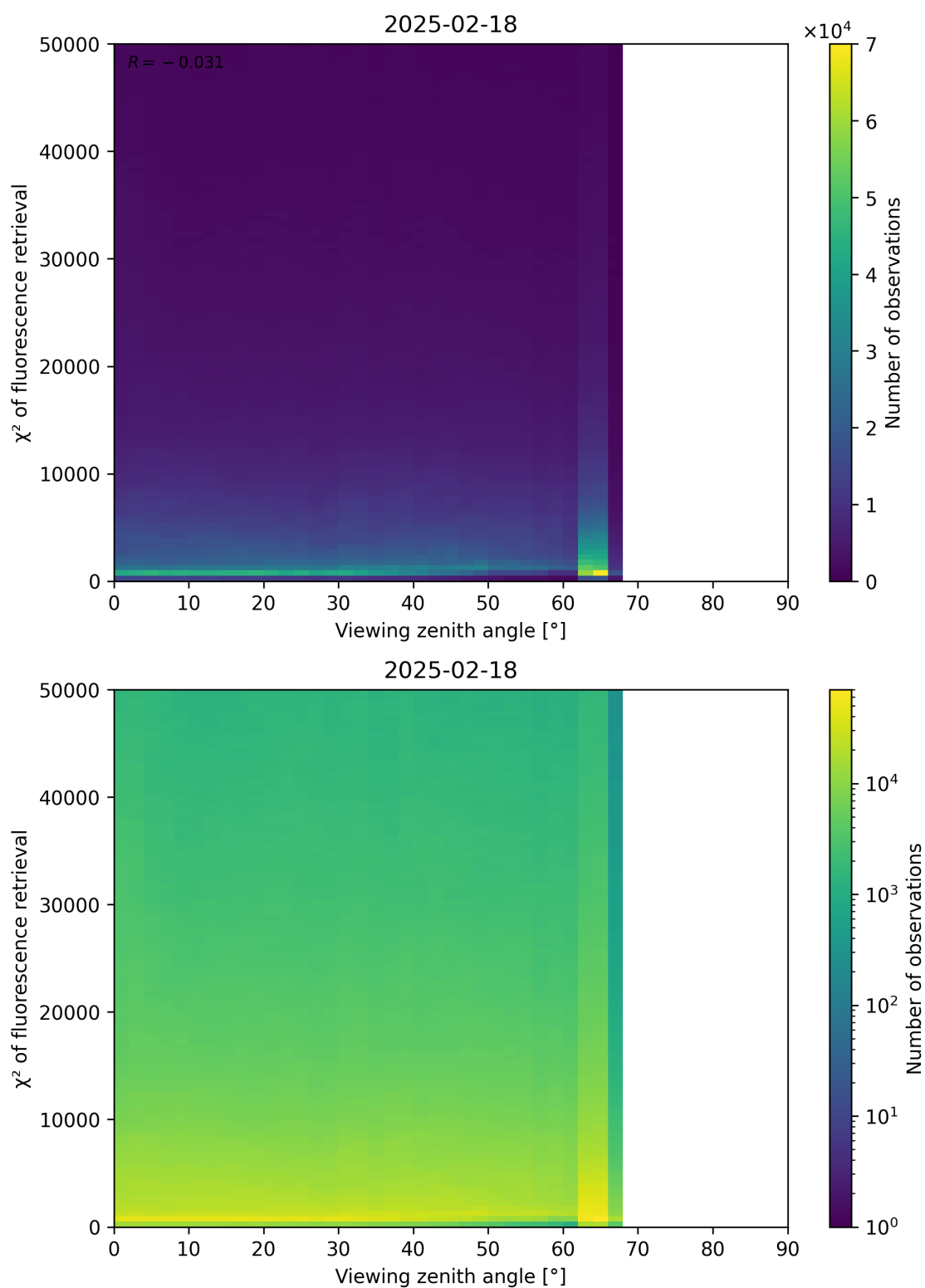
Figure 119: Scatter density plot of “Viewing zenith angle” against “ \chi^2 of fluorescence retrieval” for 2025-02-18 to 2025-02-19.
