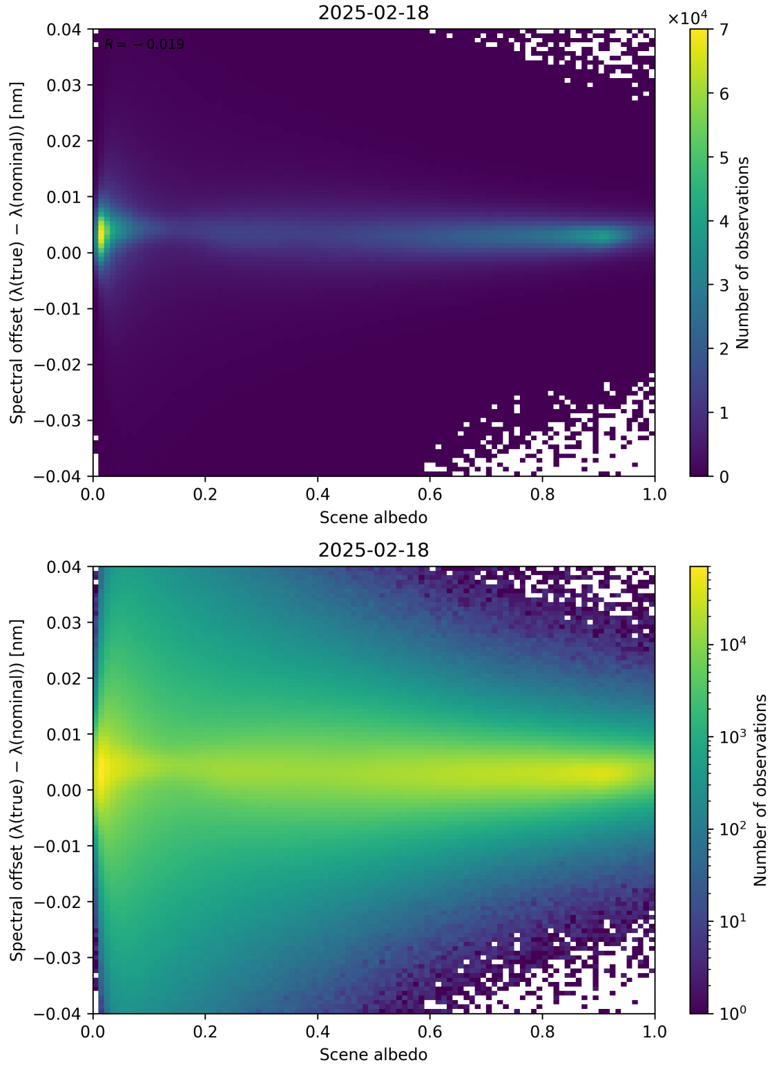
Figure 107: Scatter density plot of “Scene albedo” against “Spectral offset ( \lambda_{\text{true}} - \lambda_{\text{nominal}} )” for 2025-02-18 to 2025-02-19.
