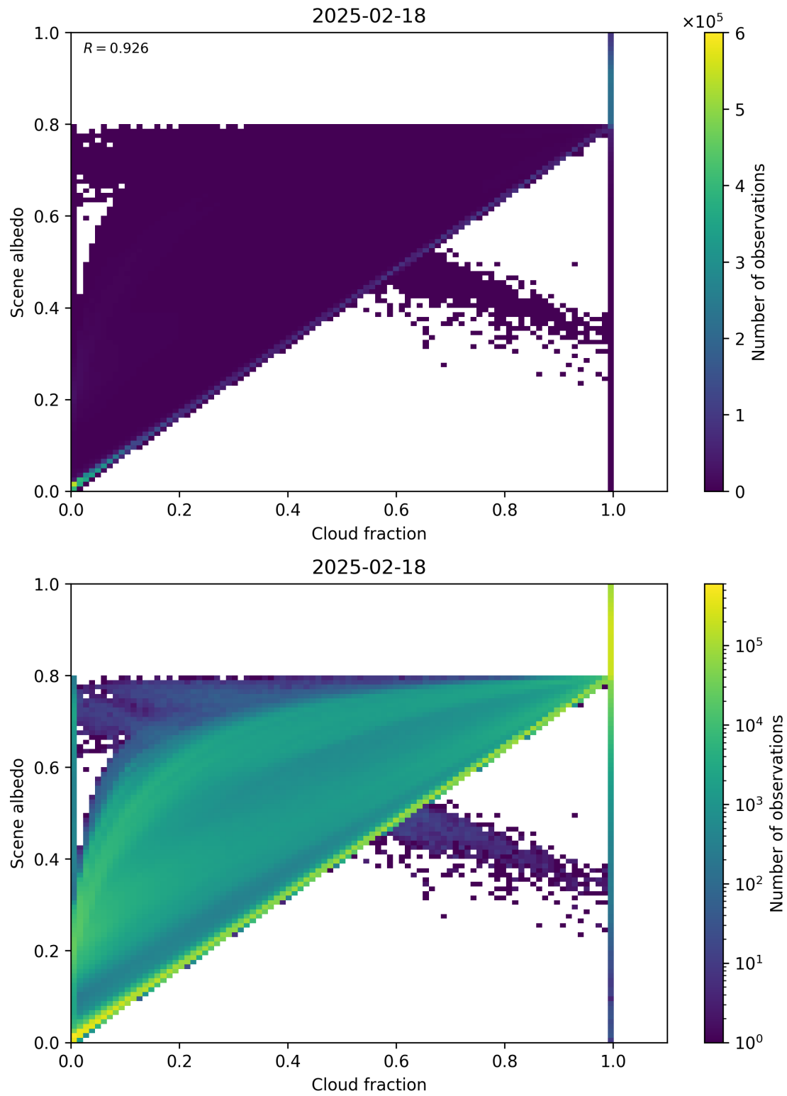
Figure 75: Scatter density plot of “Cloud fraction” against “Scene albedo” for 2025-02-18 to 2025-02-19.
