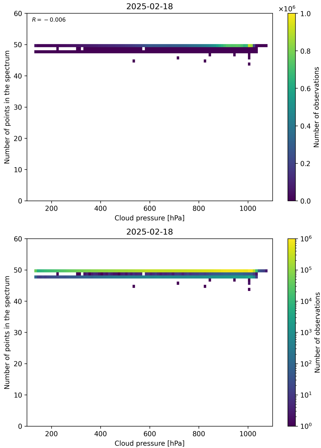
Figure 82: Scatter density plot of “Cloud pressure” against “Number of points in the spectrum” for 2025-02-18 to 2025-02-19.
