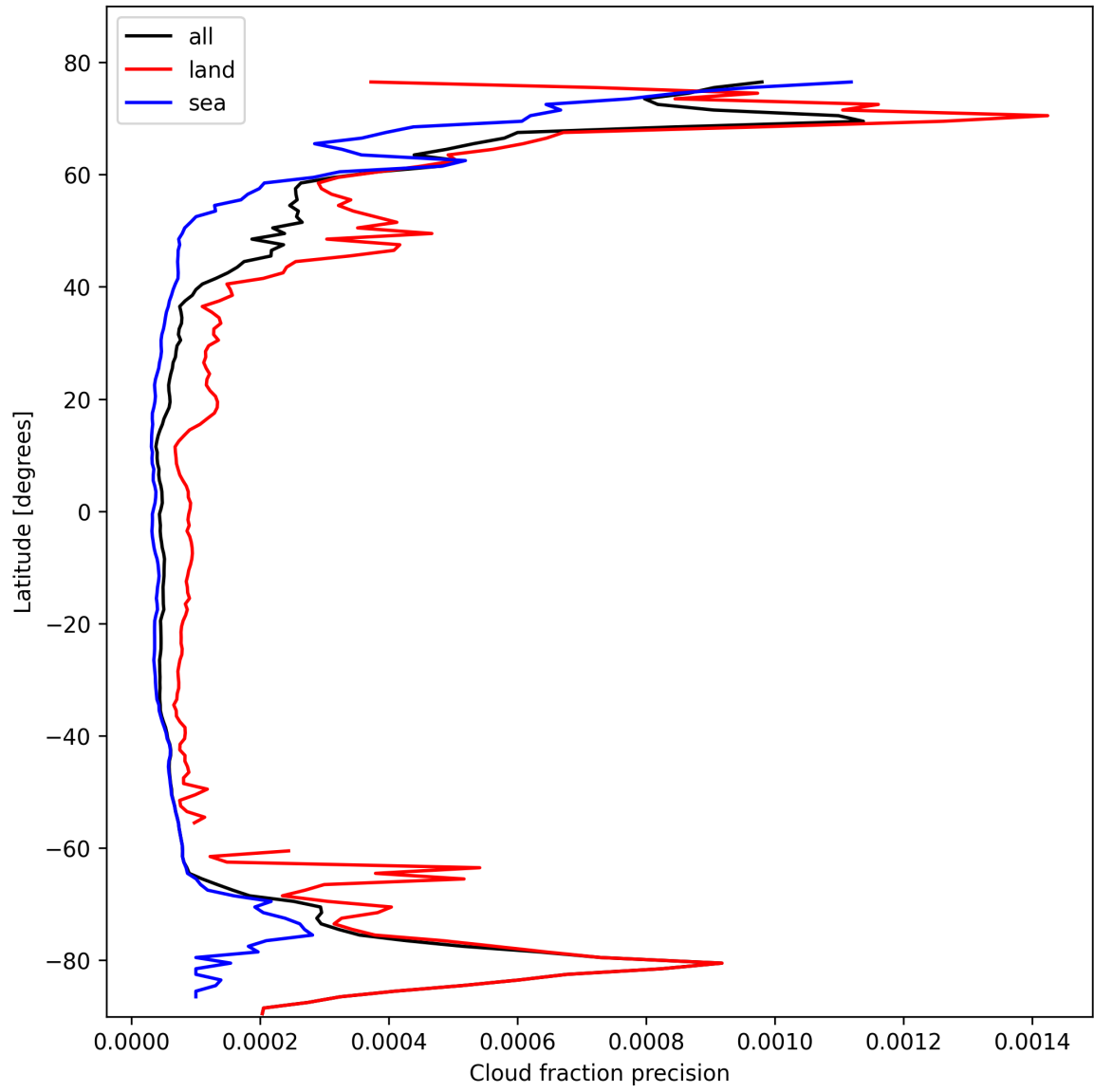
Figure 16: Zonal average of “Cloud fraction precision” for 2025-02-18 to 2025-02-19.
