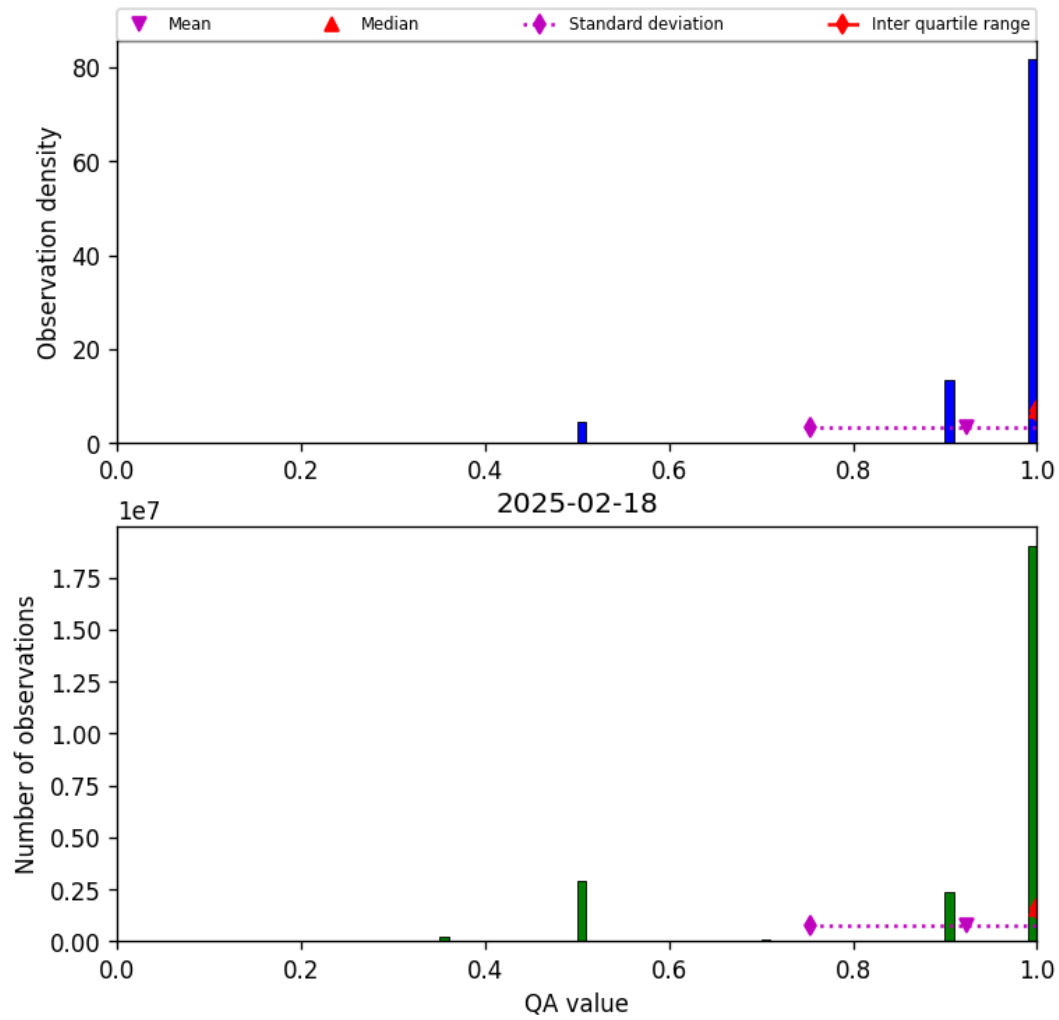
Figure 29: Histogram of “QA value” for 2025-02-18 to 2025-02-19
