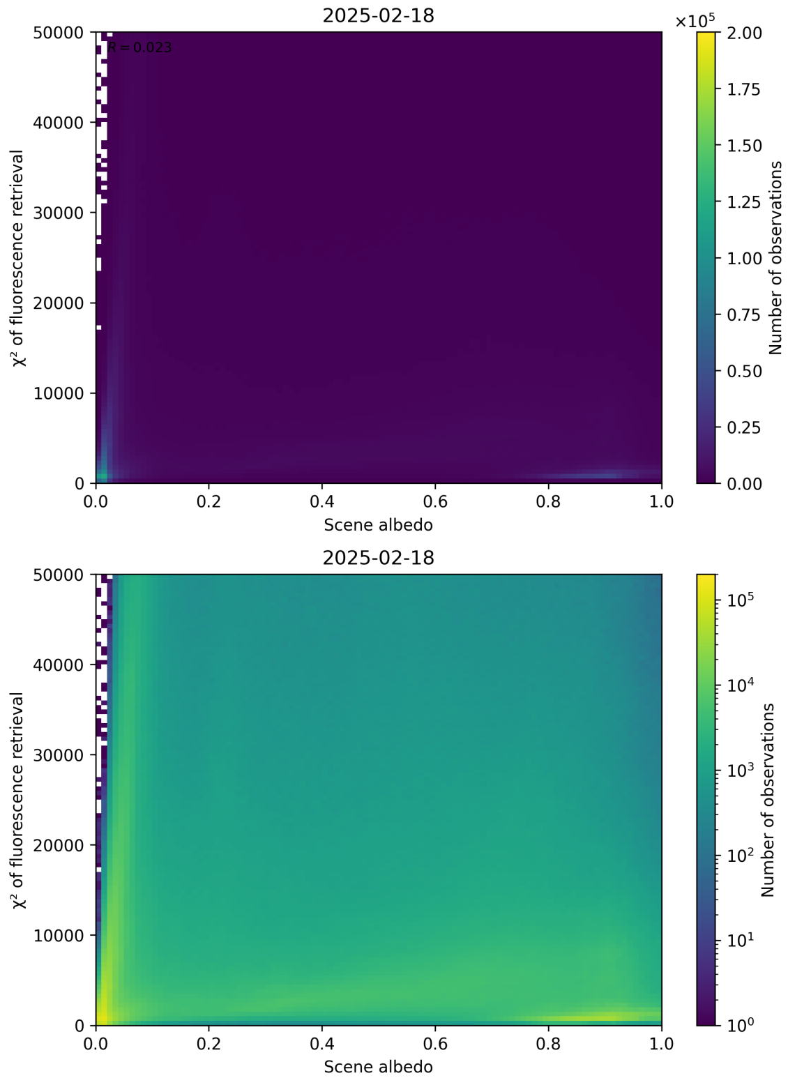
Figure 103: Scatter density plot of “Scene albedo” against “ \chi^2 of fluorescence retrieval” for 2025-02-18 to 2025-02-19.
