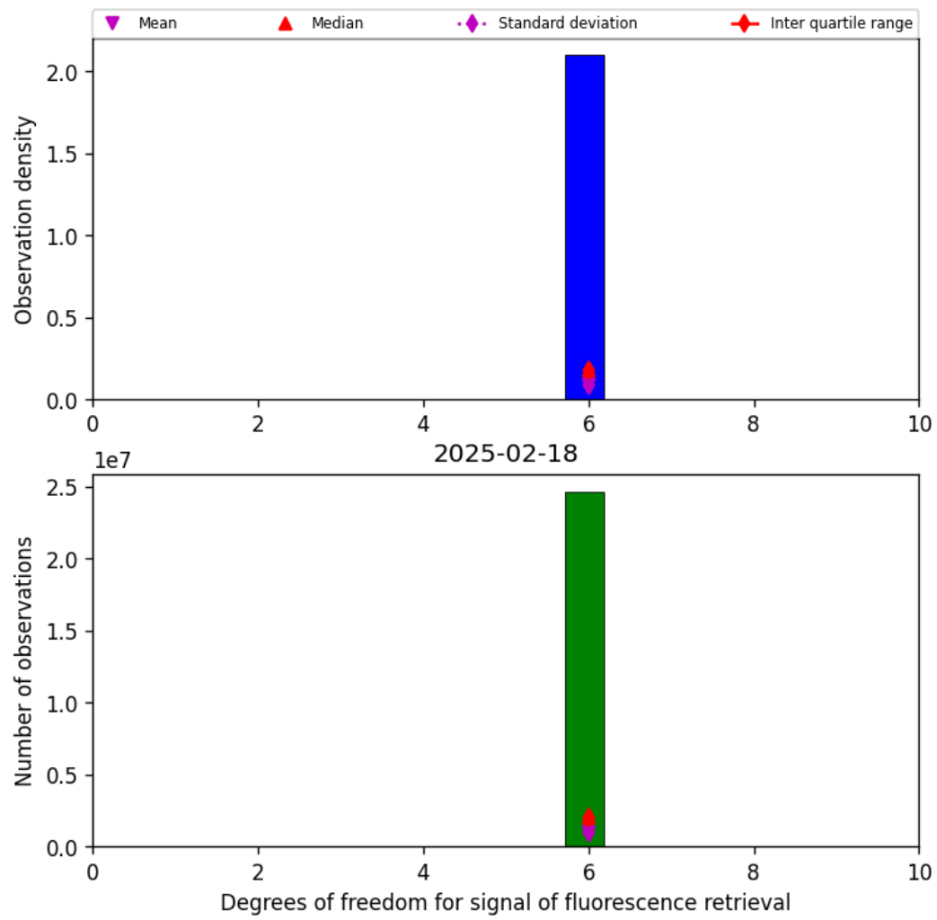
Figure 43: Histogram of “Degrees of freedom for signal of fluorescence retrieval” for 2025-02-18 to 2025-02-19
