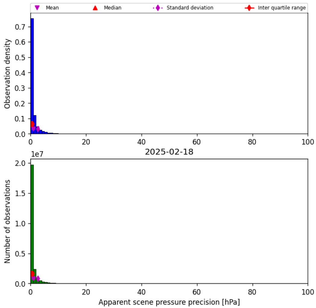
Figure 37: Histogram of “Apparent scene pressure precision” for 2025-02-18 to 2025-02-19
