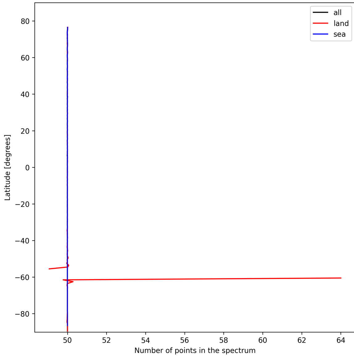
Figure 27: Zonal average of “Number of points in the spectrum” for 2025-02-18 to 2025-02-19.
