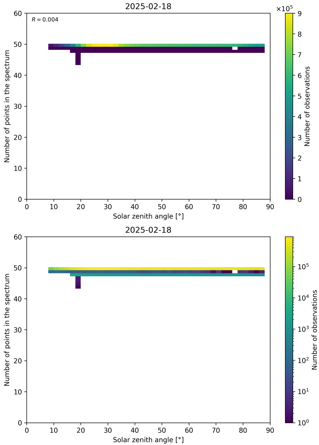
Figure 115: Scatter density plot of “Solar zenith angle” against “Number of points in the spectrum” for 2025-02-18 to 2025-02-19.
