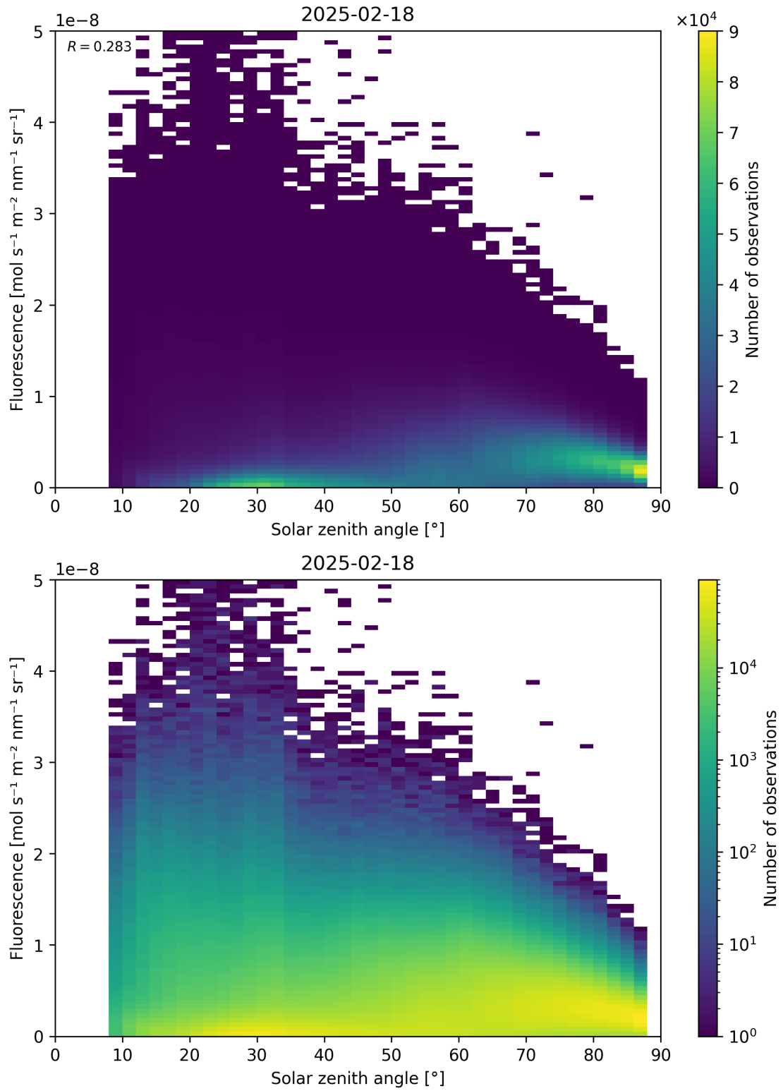
Figure 112: Scatter density plot of “Solar zenith angle” against “Fluorescence” for 2025-02-18 to 2025-02-19.
