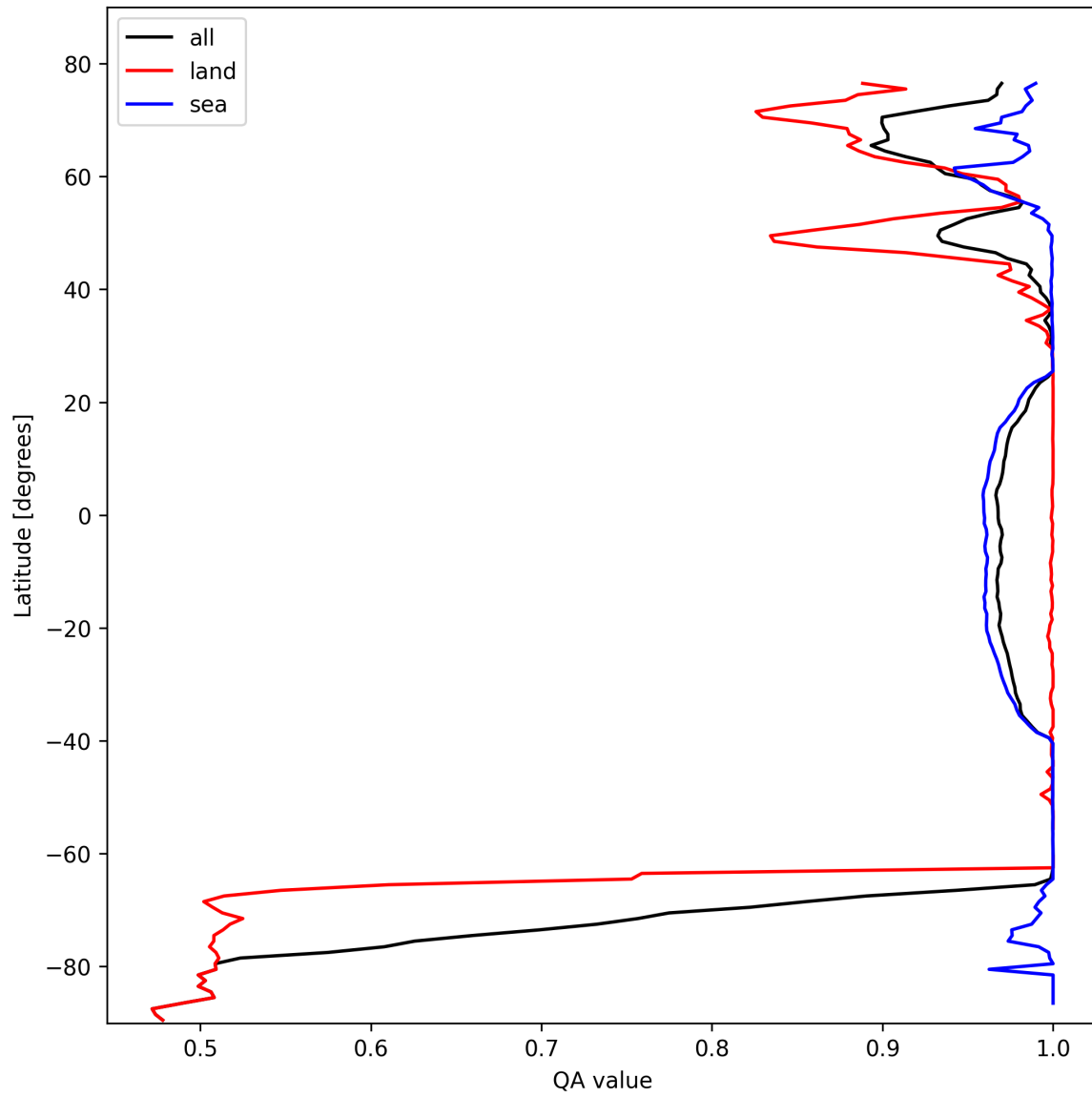
Figure 12: Zonal average of “QA value” for 2025-02-18 to 2025-02-19.
