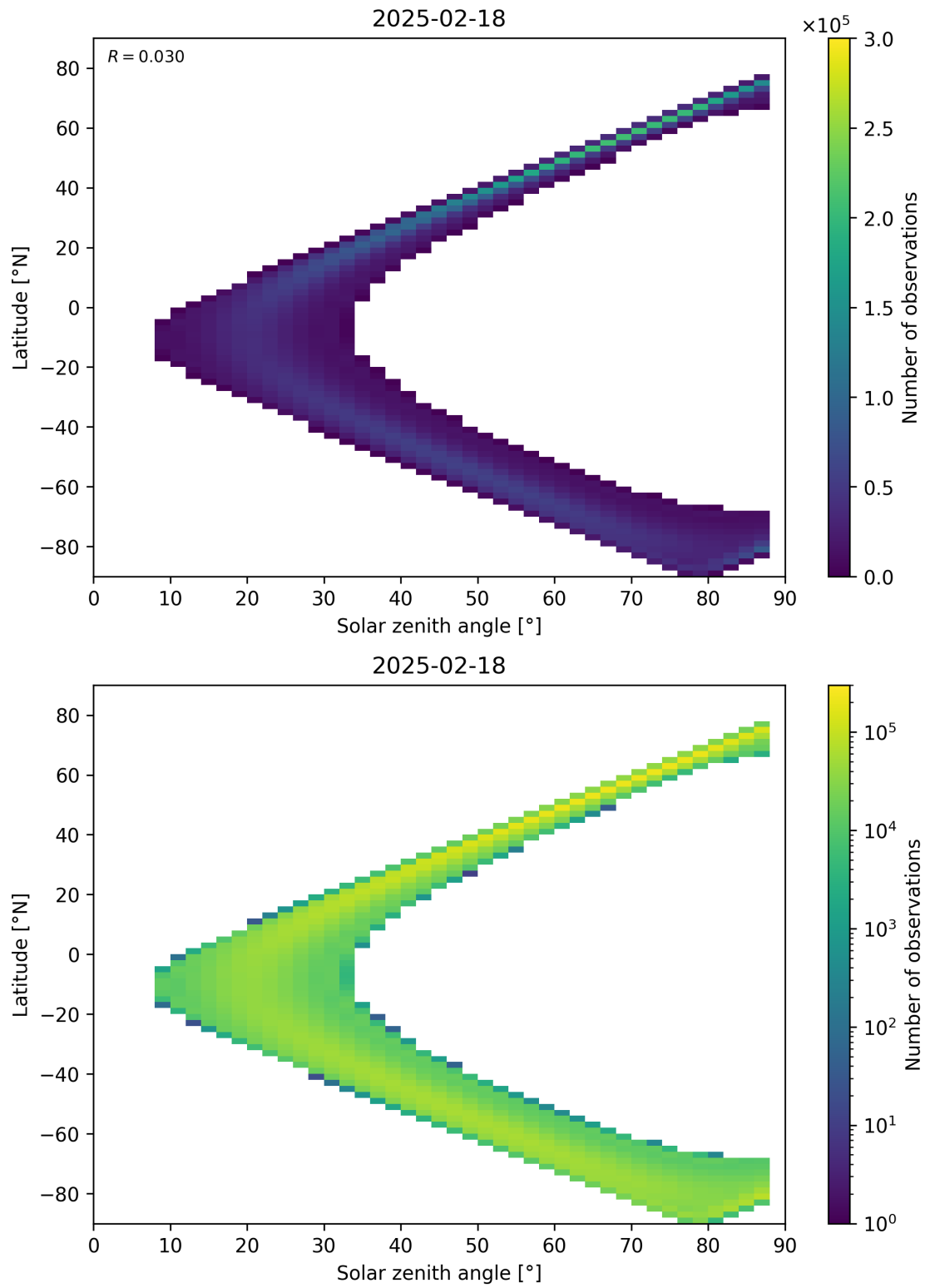
Figure 113: Scatter density plot of “Solar zenith angle” against “Latitude” for 2025-02-18 to 2025-02-19.
