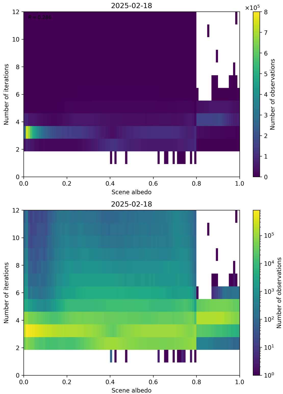
Figure 105: Scatter density plot of “Scene albedo” against “Number of iterations” for 2025-02-18 to 2025-02-19.
