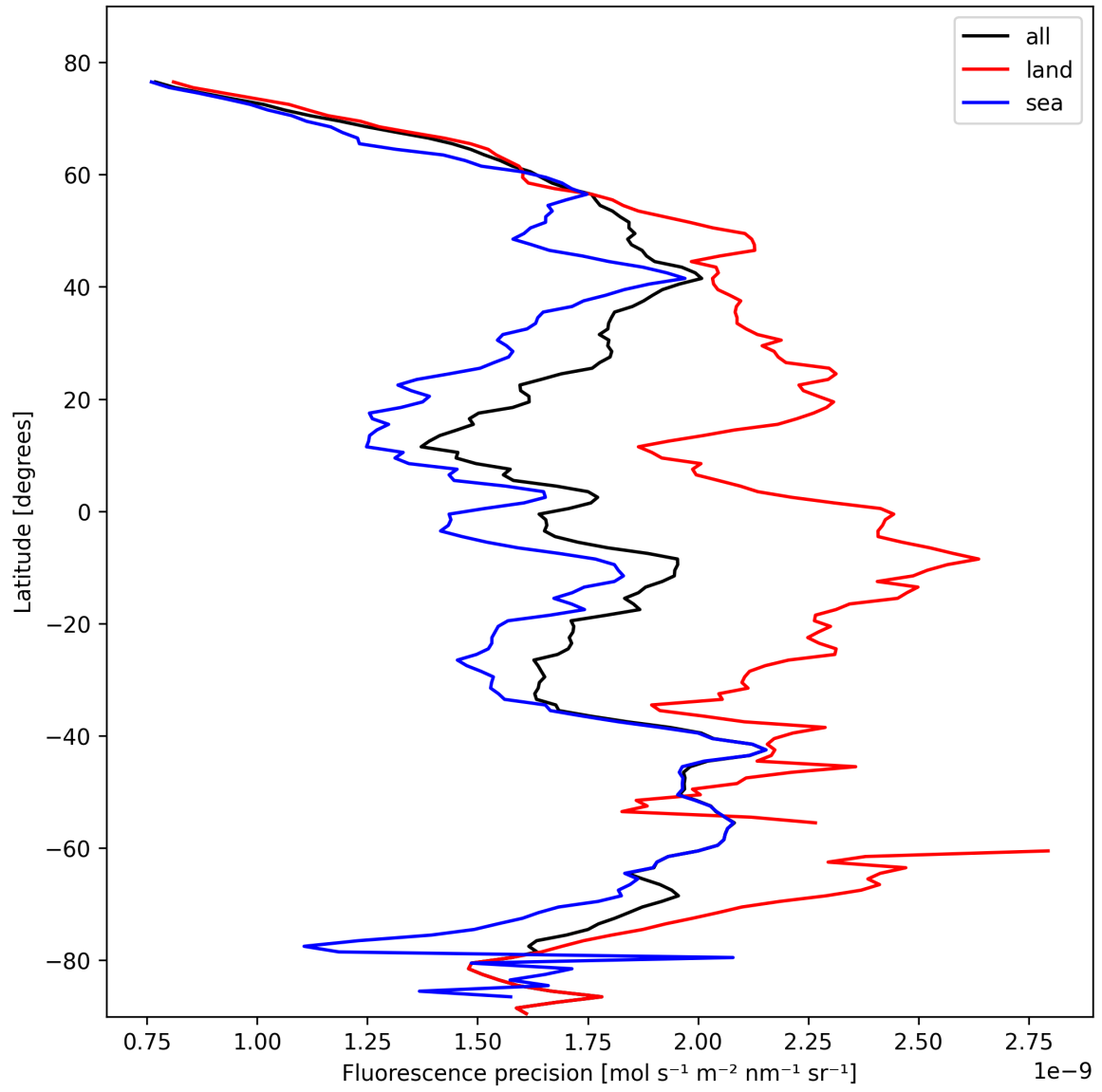
Figure 24: Zonal average of “Fluorescence precision” for 2025-02-18 to 2025-02-19.
