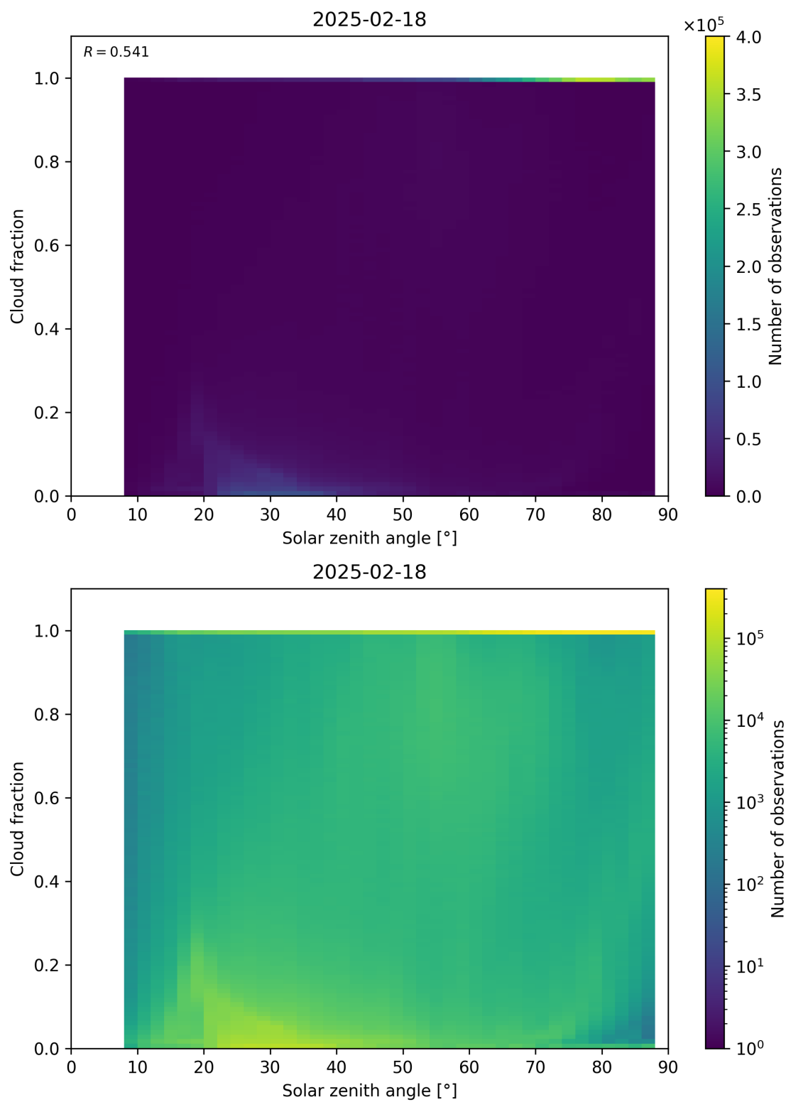
Figure 110: Scatter density plot of “Solar zenith angle” against “Cloud fraction” for 2025-02-18 to 2025-02-19.
