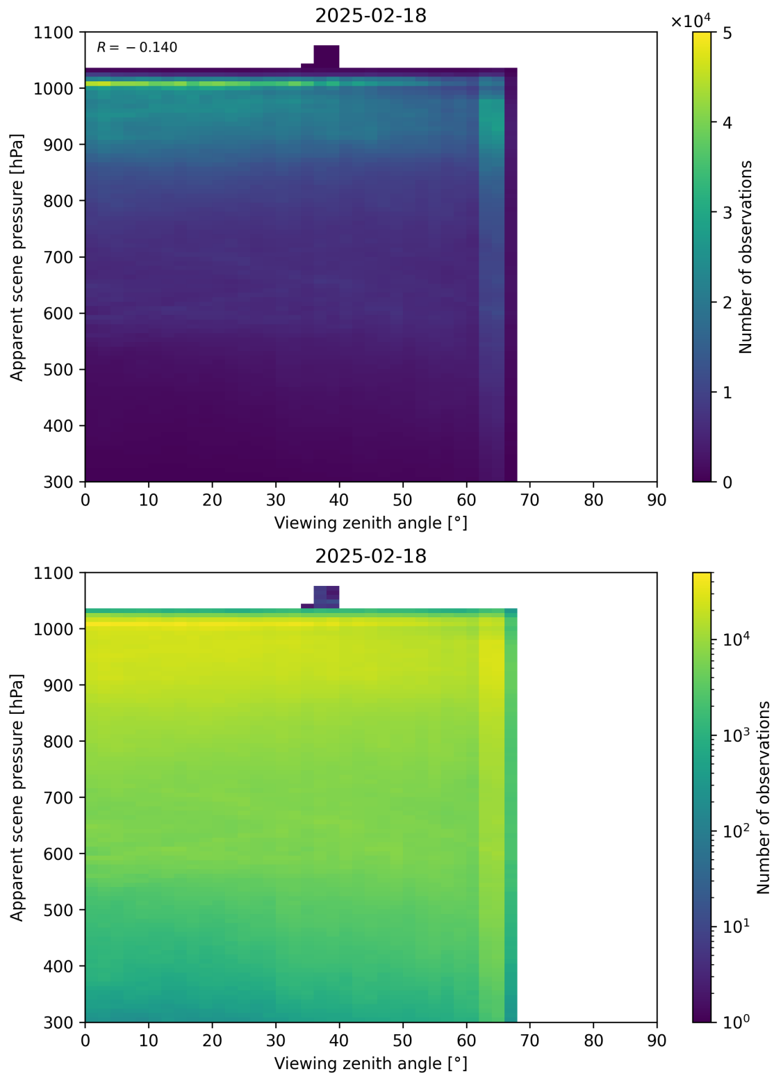
Figure 118: Scatter density plot of “Viewing zenith angle” against “Apparent scene pressure” for 2025-02-18 to 2025-02-19.
