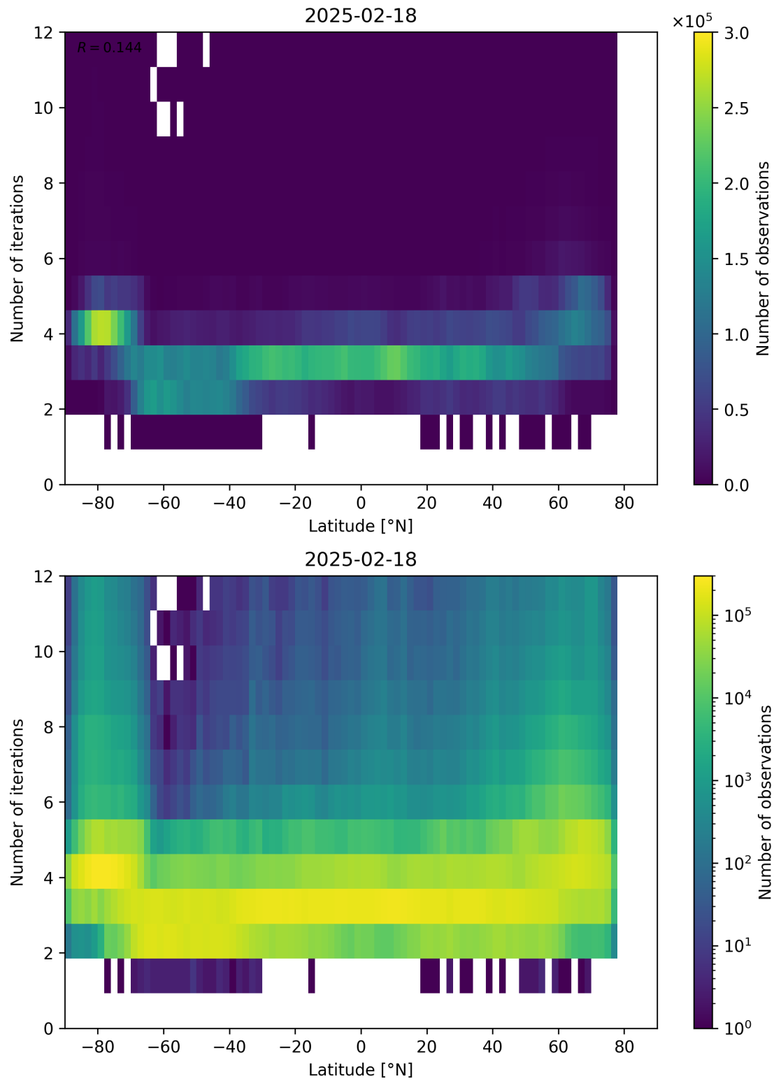
Figure 93: Scatter density plot of “Latitude” against “Number of iterations” for 2025-02-18 to 2025-02-19.
