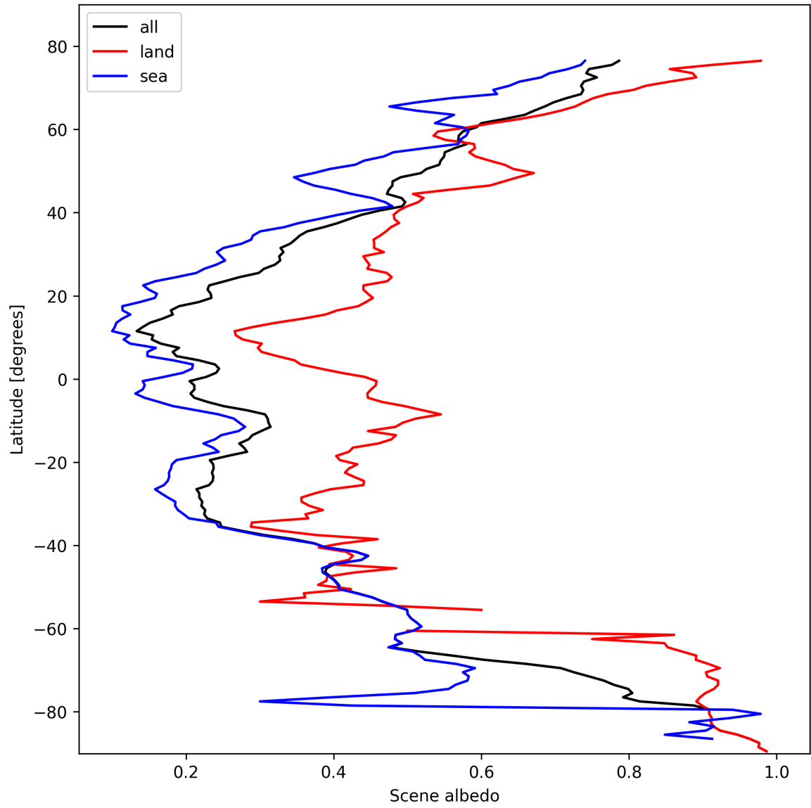
Figure 17: Zonal average of “Scene albedo” for 2025-02-18 to 2025-02-19.
