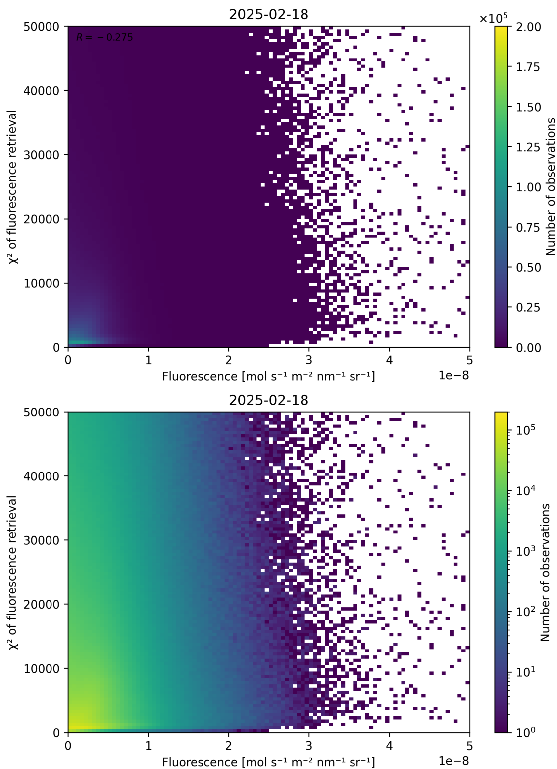
Figure 85: Scatter density plot of “Fluorescence” against “ \chi^2 of fluorescence retrieval” for 2025-02-18 to 2025-02-19.
