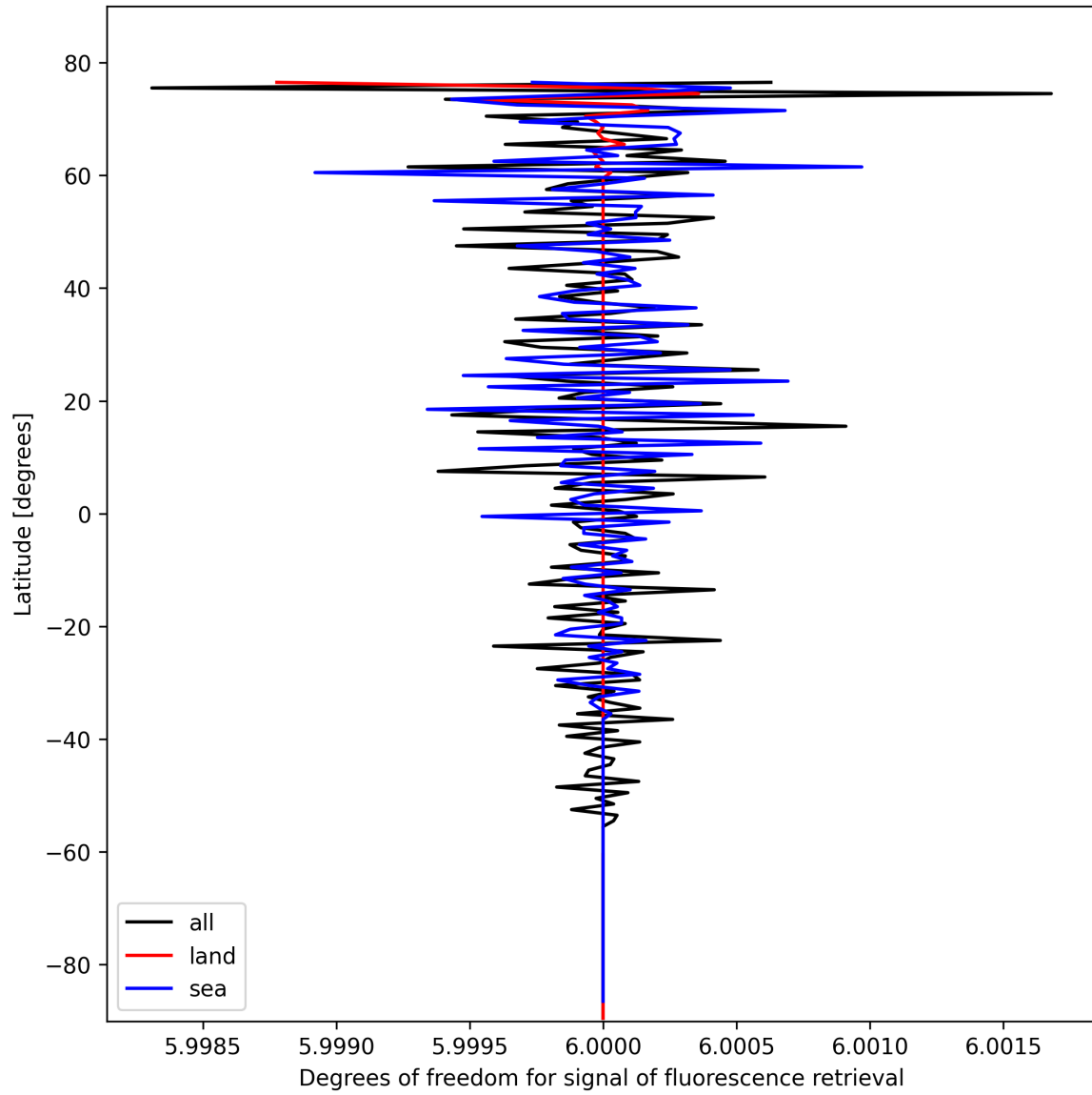
Figure 26: Zonal average of “Degrees of freedom for signal of fluorescence retrieval” for 2025-02-18 to 2025-02-19.
