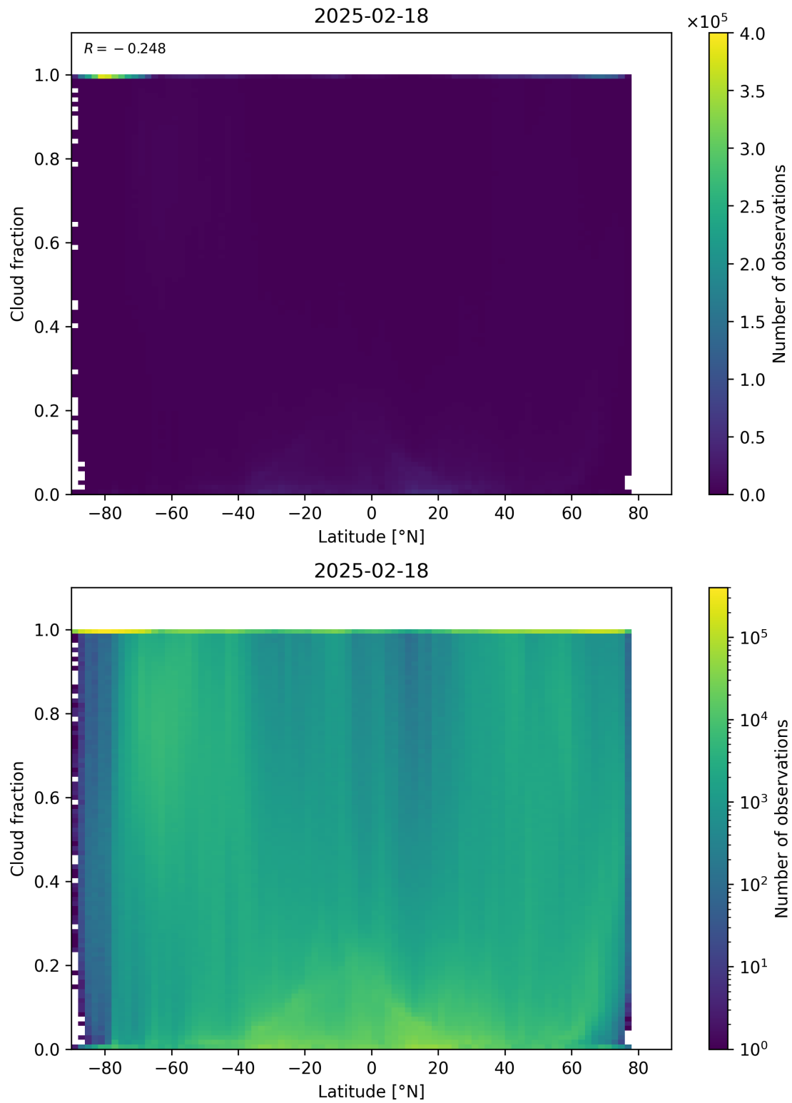
Figure 90: Scatter density plot of “Latitude” against “Cloud fraction” for 2025-02-18 to 2025-02-19.
