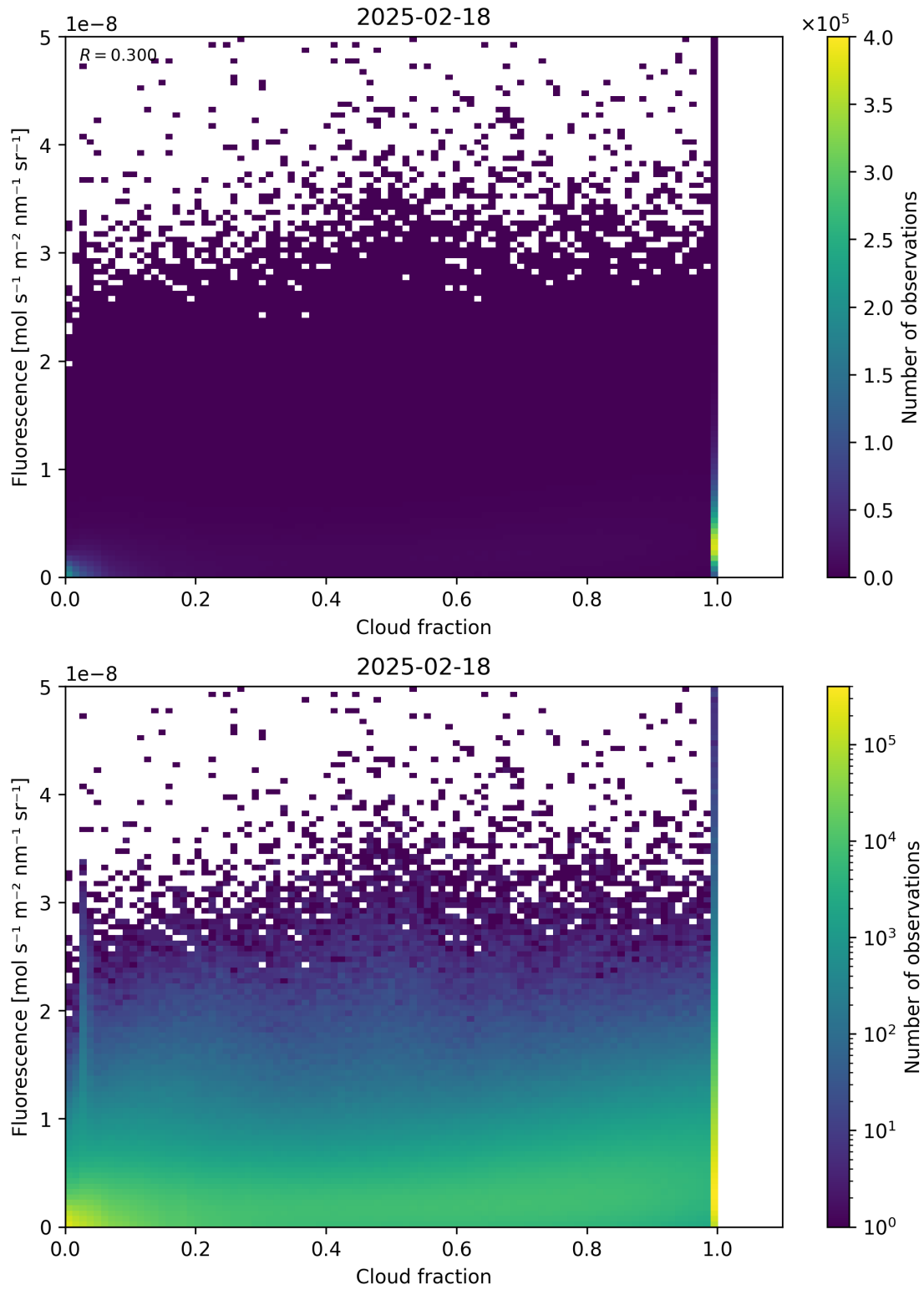
Figure 72: Scatter density plot of “Cloud fraction” against “Fluorescence” for 2025-02-18 to 2025-02-19.
