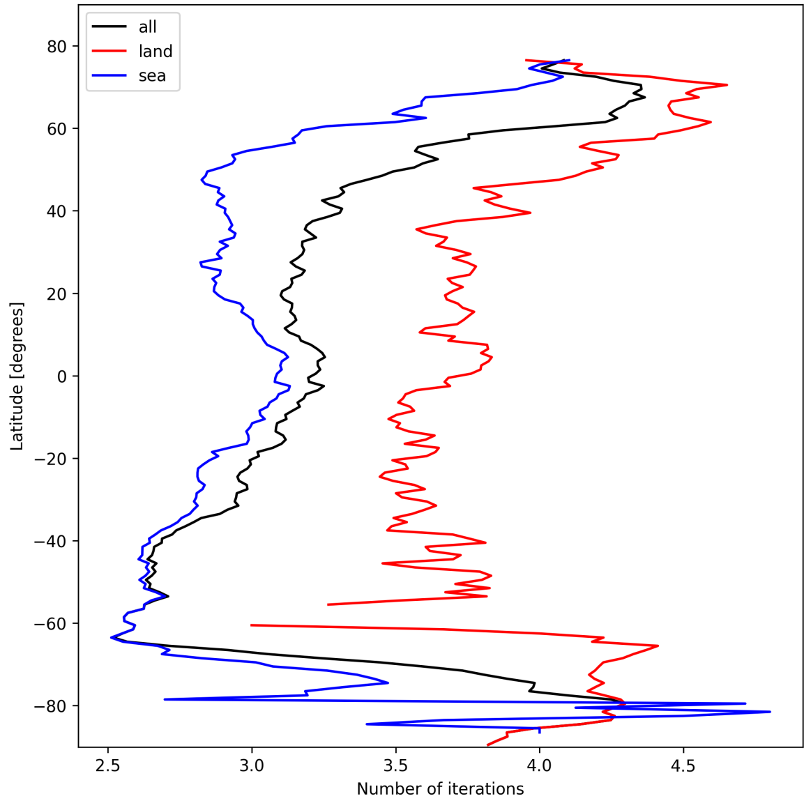
Figure 22: Zonal average of “Number of iterations” for 2025-02-18 to 2025-02-19.
