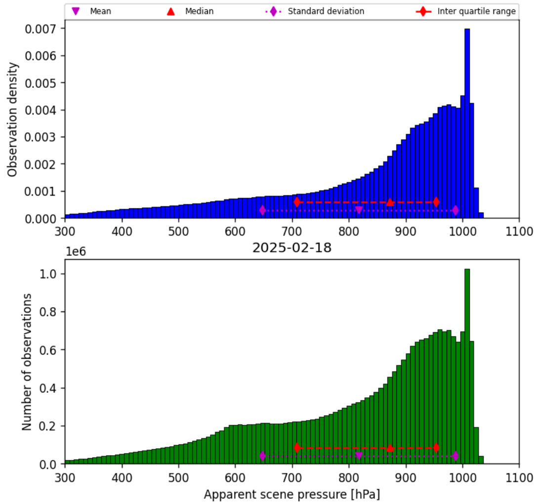
Figure 36: Histogram of “Apparent scene pressure” for 2025-02-18 to 2025-02-19
