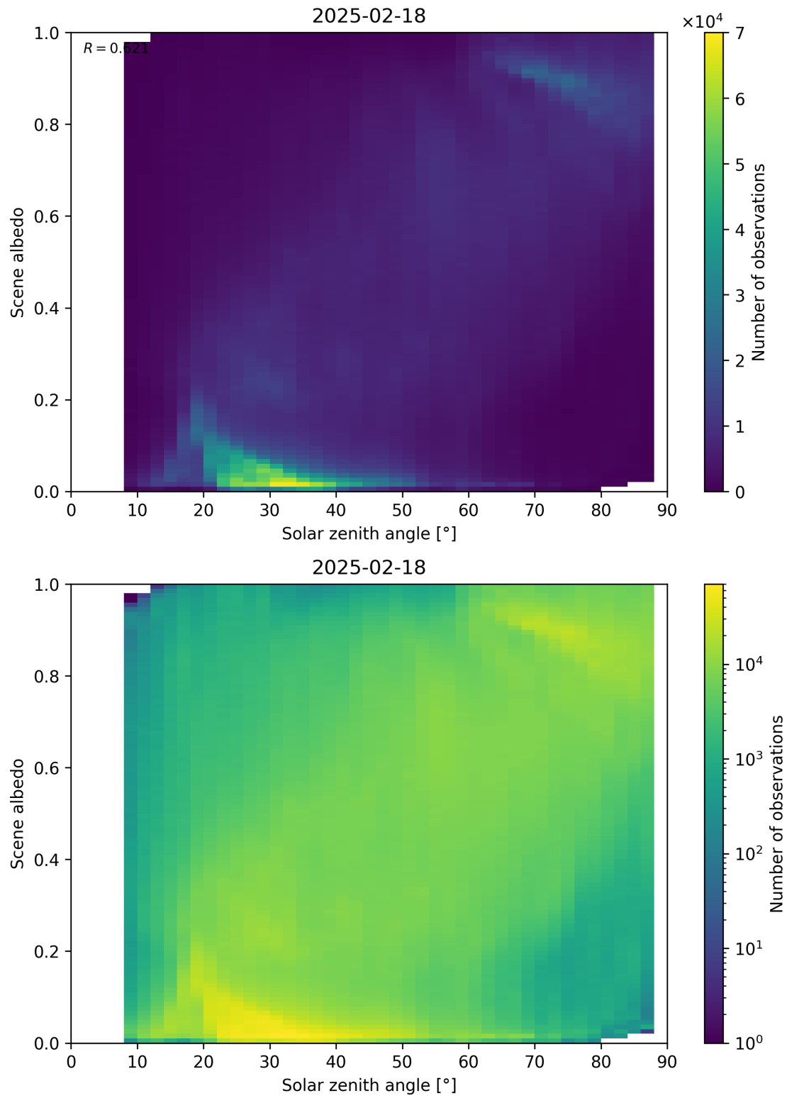
Figure 116: Scatter density plot of “Solar zenith angle” against “Scene albedo” for 2025-02-18 to 2025-02-19.
