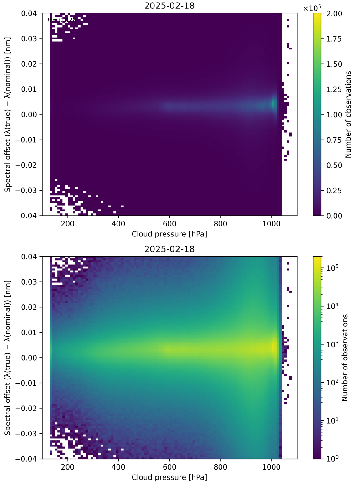
Figure 84: Scatter density plot of “Cloud pressure” against “Spectral offset ( \lambda_{\text{true}} - \lambda_{\text{nominal}} )” for 2025-02-18 to 2025-02-19.
