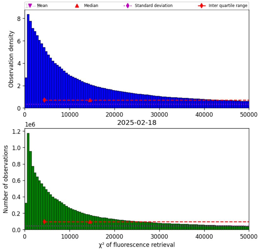
Figure 42: Histogram of “ \chi^2 of fluorescence retrieval” for 2025-02-18 to 2025-02-19
