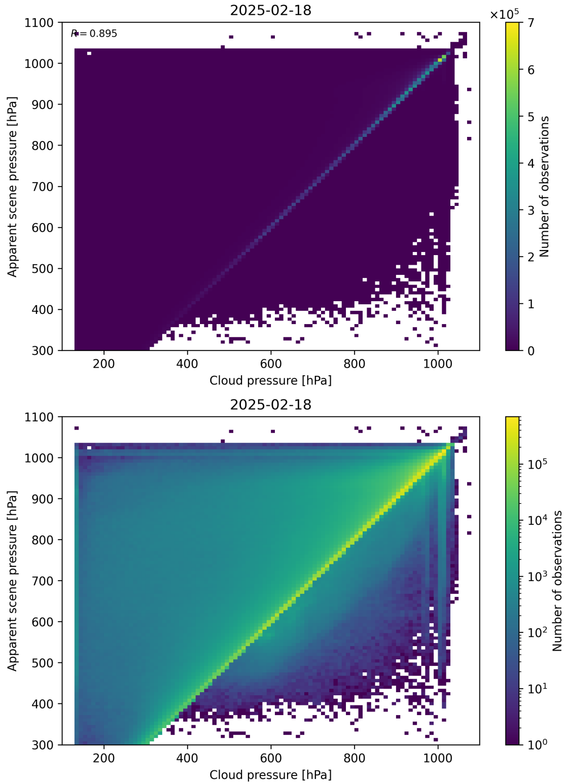
Figure 77: Scatter density plot of “Cloud pressure” against “Apparent scene pressure” for 2025-02-18 to 2025-02-19.
