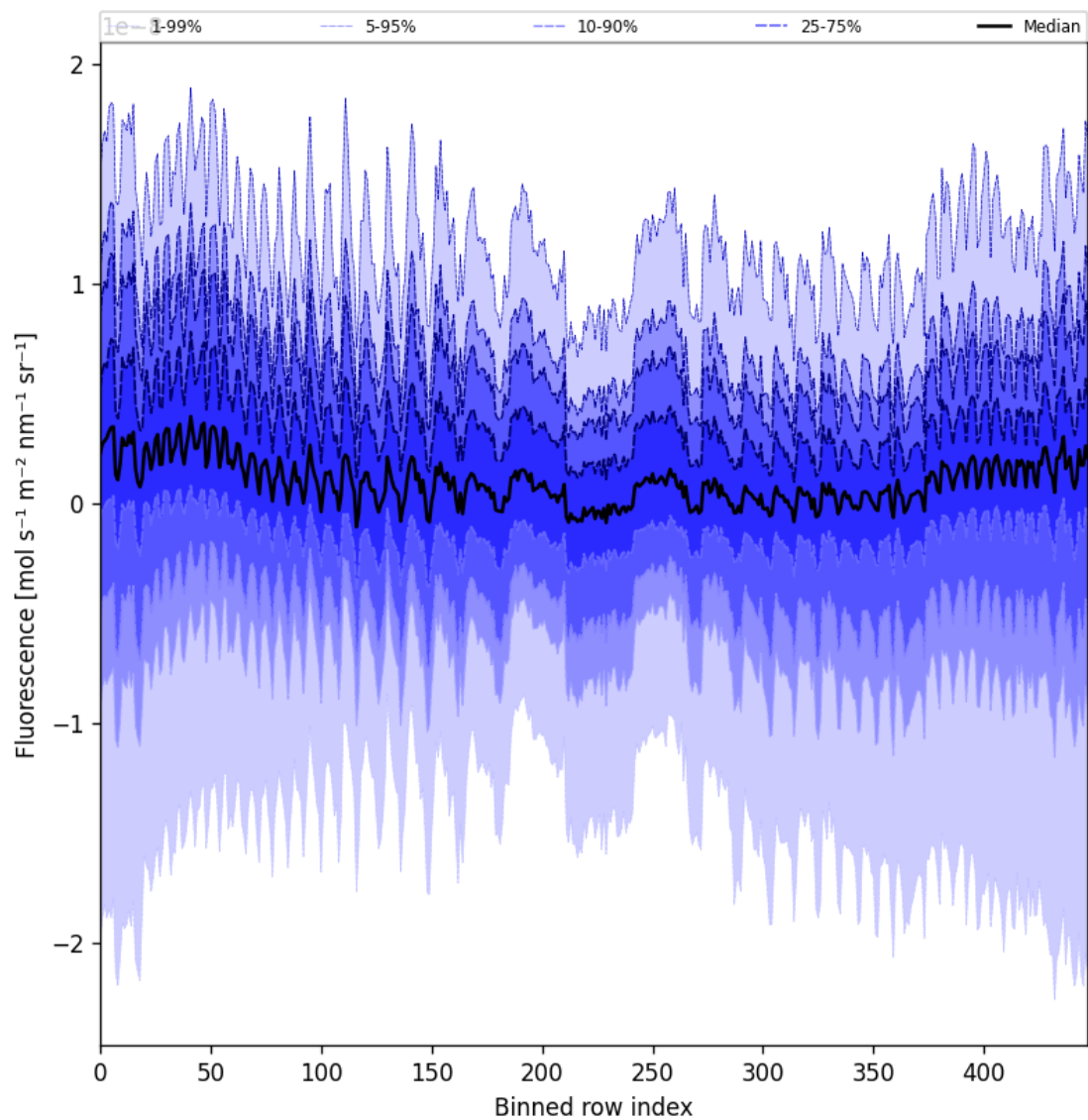
Figure 57: Along track statistics of “Fluorescence” for 2025-02-18 to 2025-02-19
