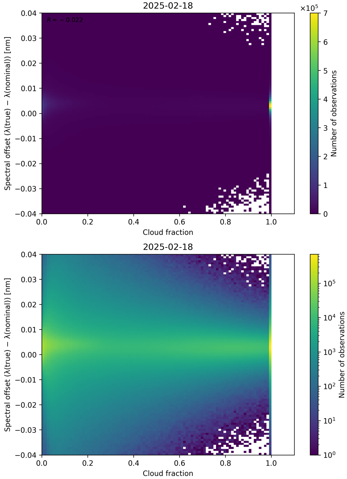
Figure 76: Scatter density plot of “Cloud fraction” against “Spectral offset ( \lambda_{\text{true}} - \lambda_{\text{nominal}} )” for 2025-02-18 to 2025-02-19.
