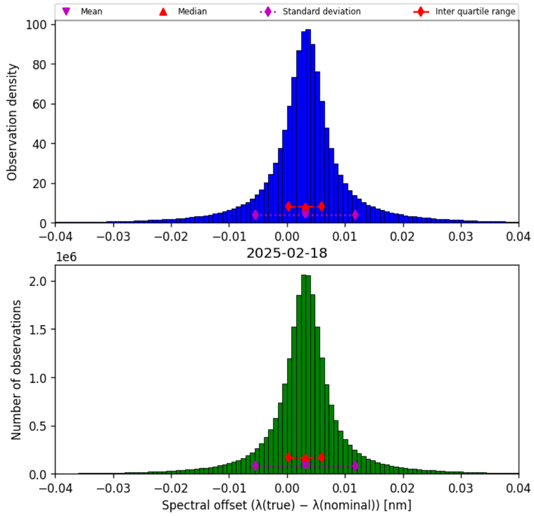
Figure 45: Histogram of “Spectral offset ( \lambda_{\text{true}} - \lambda_{\text{nominal}} )” for 2025-02-18 to 2025-02-19
