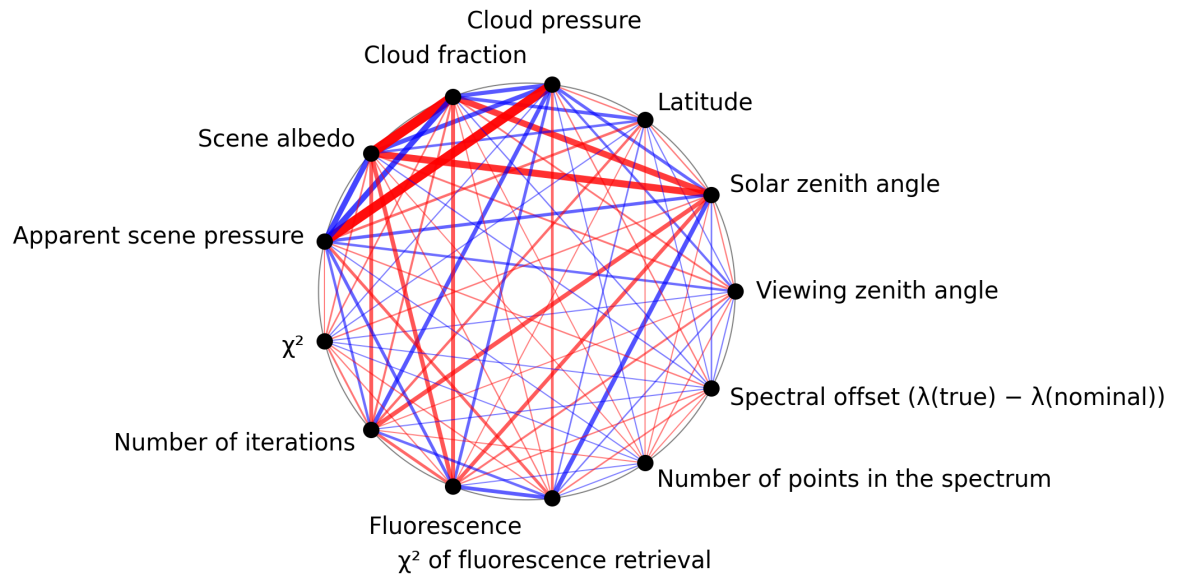
Figure 1: Map of correlation graph for 2025-02-18 to 2025-02-19.
