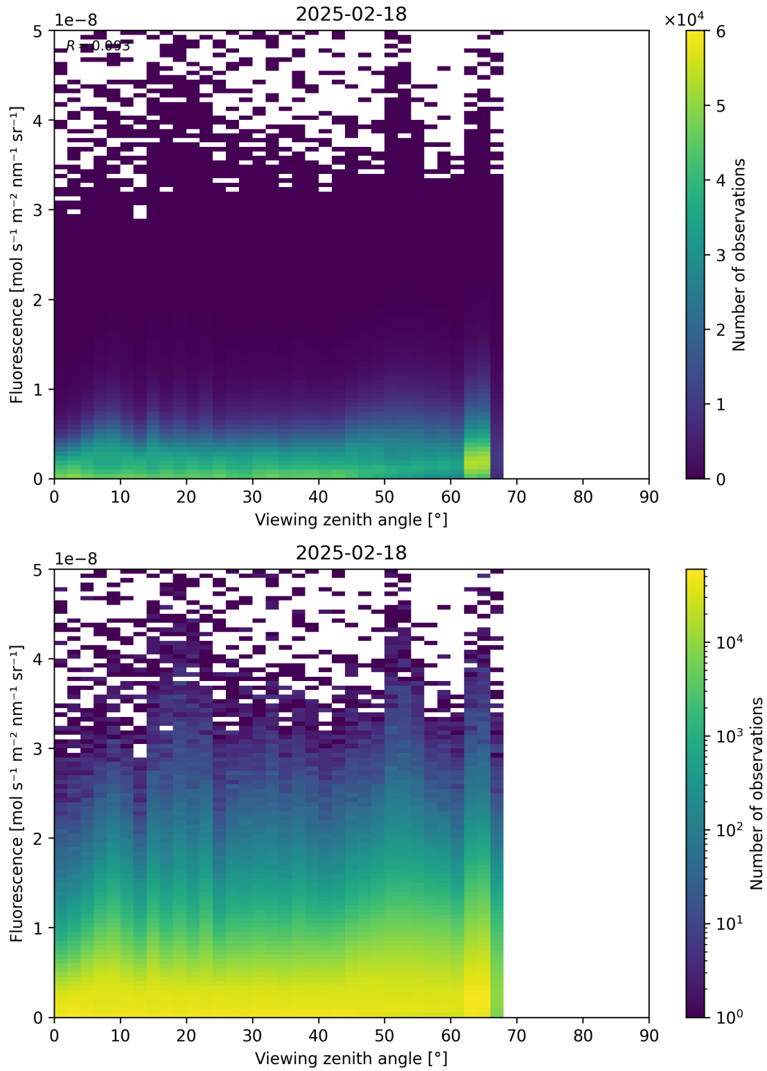
Figure 122: Scatter density plot of “Viewing zenith angle” against “Fluorescence” for 2025-02-18 to 2025-02-19.
