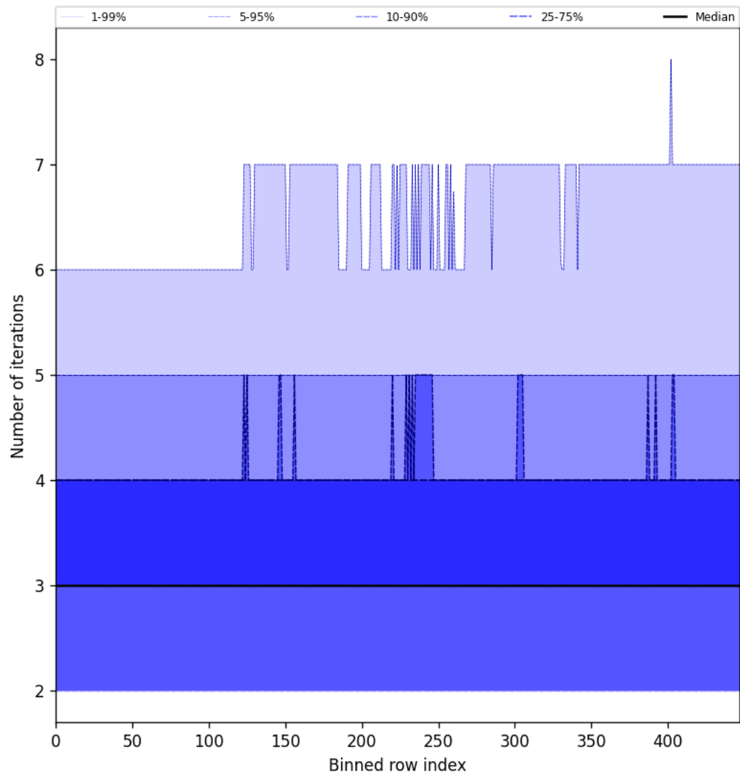
Figure 56: Along track statistics of “Number of iterations” for 2025-02-18 to 2025-02-19
