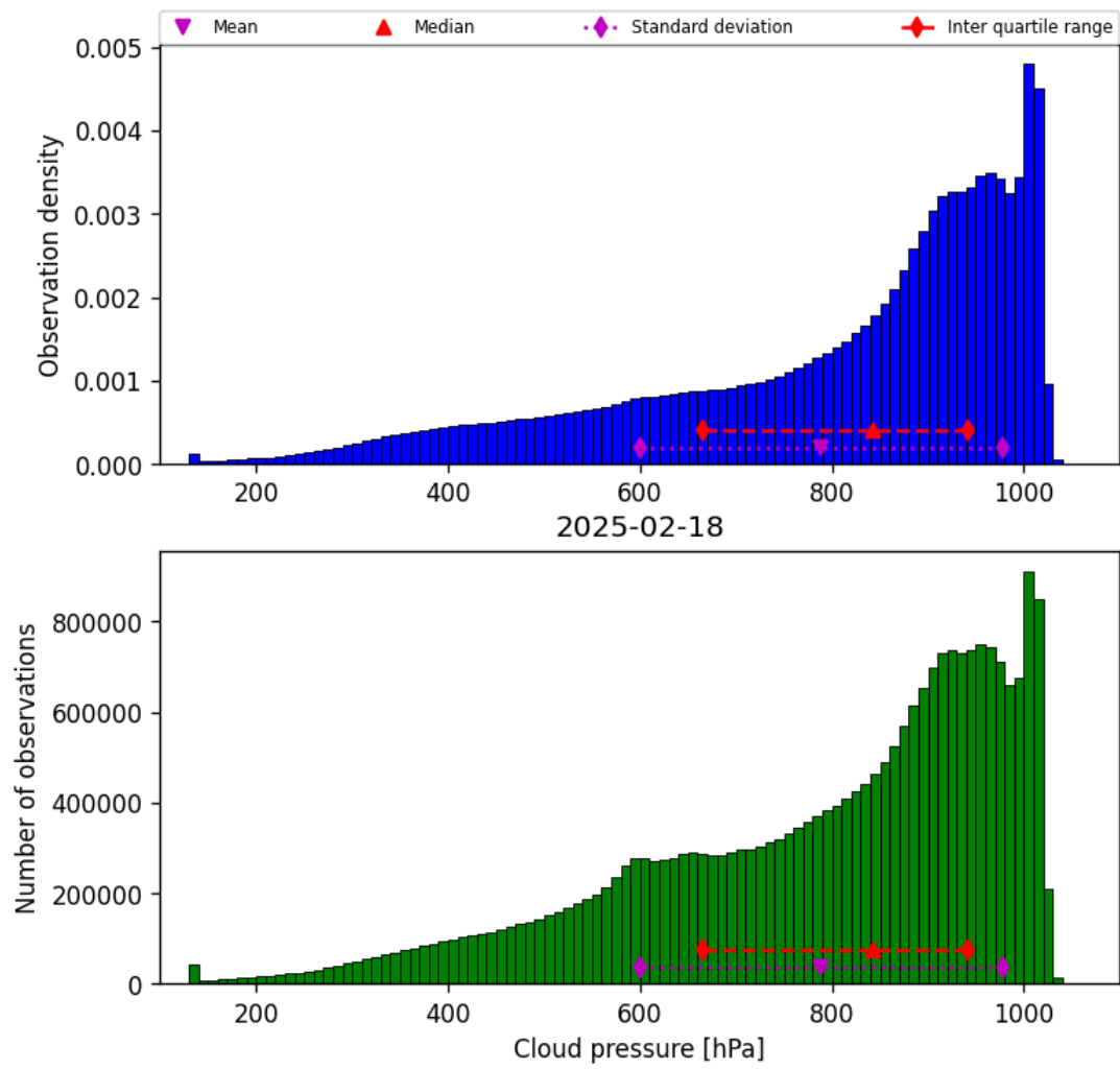
Figure 30: Histogram of “Cloud pressure” for 2025-02-18 to 2025-02-19
