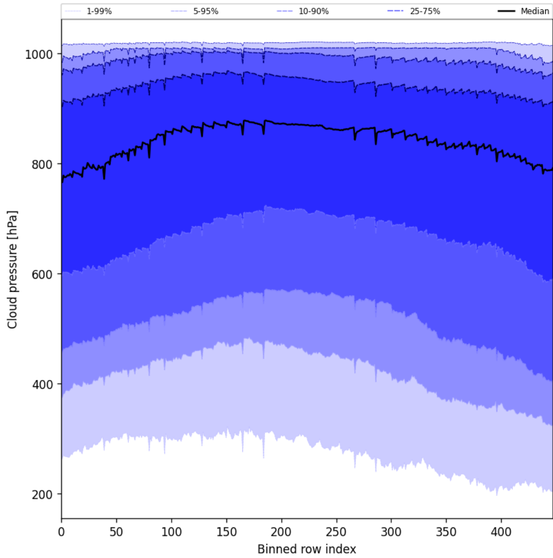
Figure 47: Along track statistics of “Cloud pressure” for 2025-02-18 to 2025-02-19
