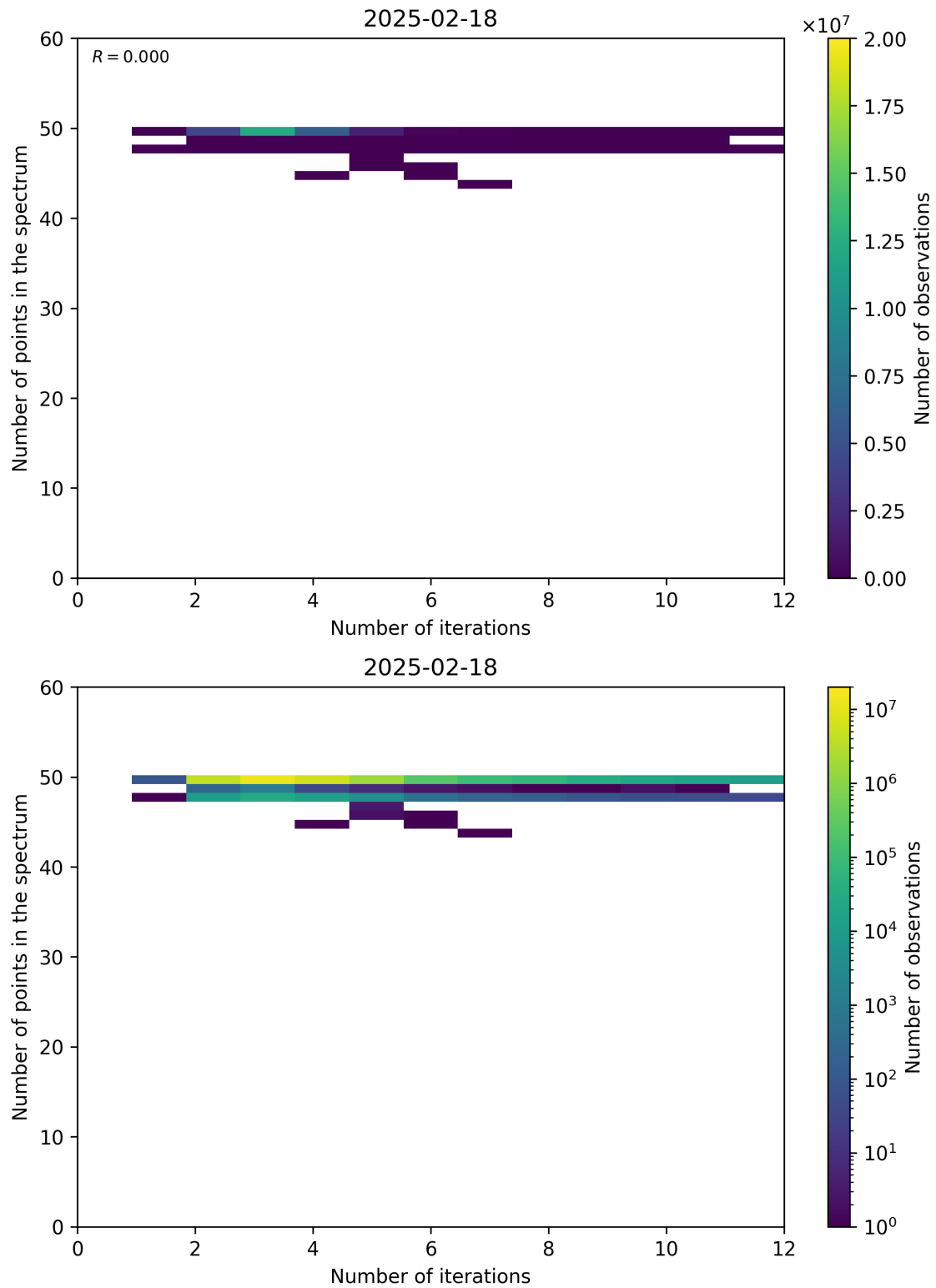
Figure 99: Scatter density plot of “Number of iterations” against “Number of points in the spectrum” for 2025-02-18 to 2025-02-19.
