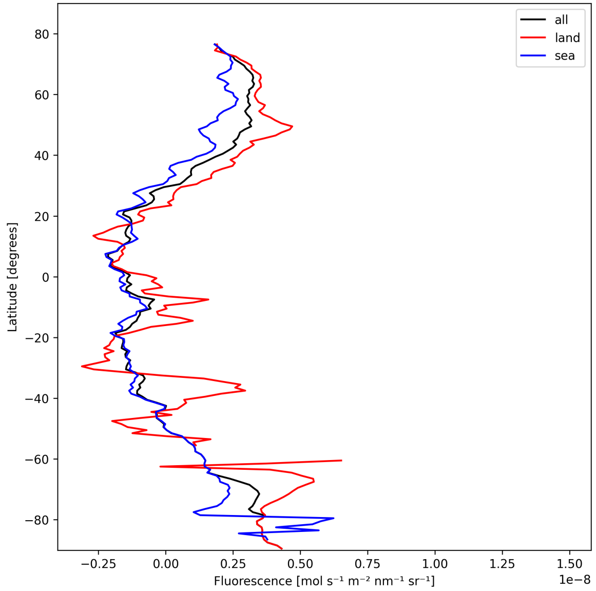
Figure 23: Zonal average of “Fluorescence” for 2025-02-18 to 2025-02-19.
