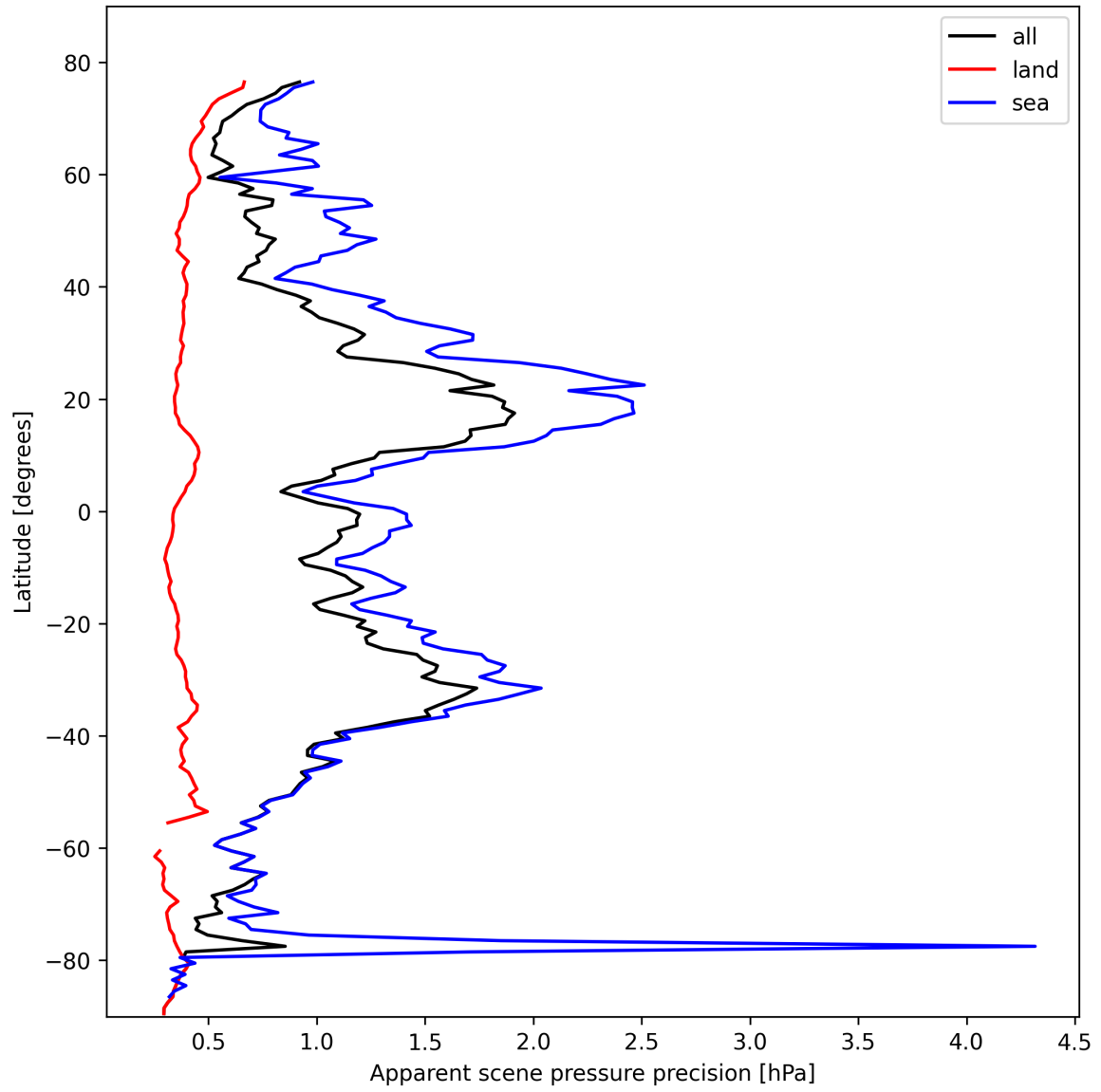
Figure 20: Zonal average of “Apparent scene pressure precision” for 2025-02-18 to 2025-02-19.
