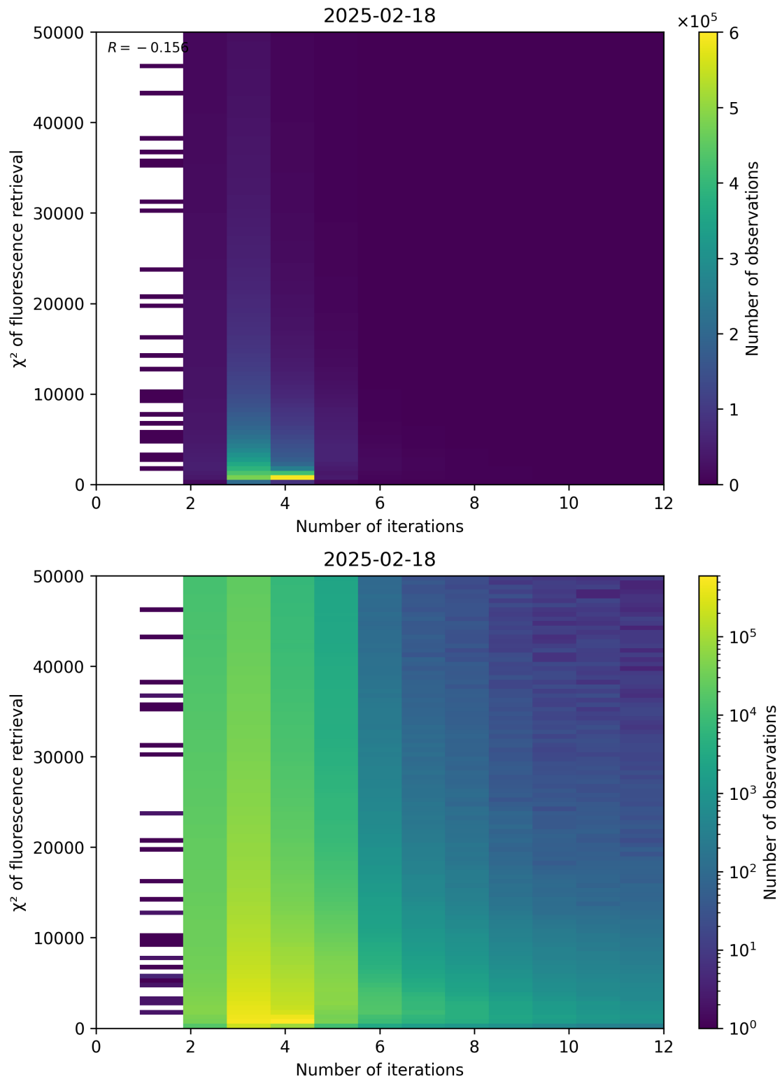
Figure 97: Scatter density plot of “Number of iterations” against “ \chi^2 of fluorescence retrieval” for 2025-02-18 to 2025-02-19.
