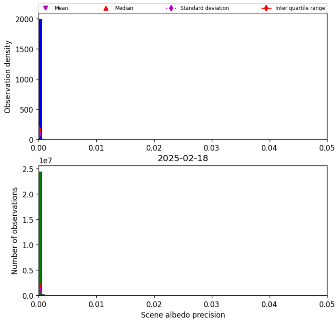
Figure 35: Histogram of “Scene albedo precision” for 2025-02-18 to 2025-02-19
