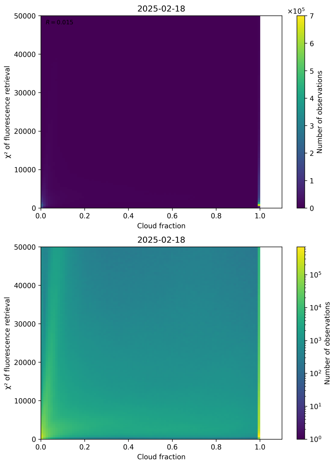
Figure 71: Scatter density plot of “Cloud fraction” against “ \chi^2 of fluorescence retrieval” for 2025-02-18 to 2025-02-19.
