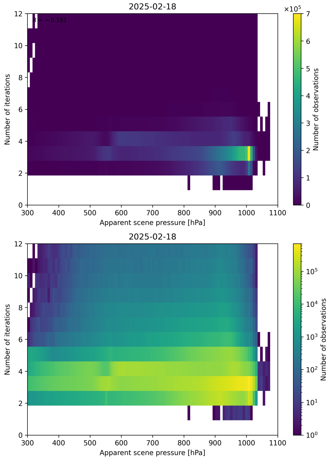
Figure 65: Scatter density plot of “Apparent scene pressure” against “Number of iterations” for 2025-02-18 to 2025-02-19.
