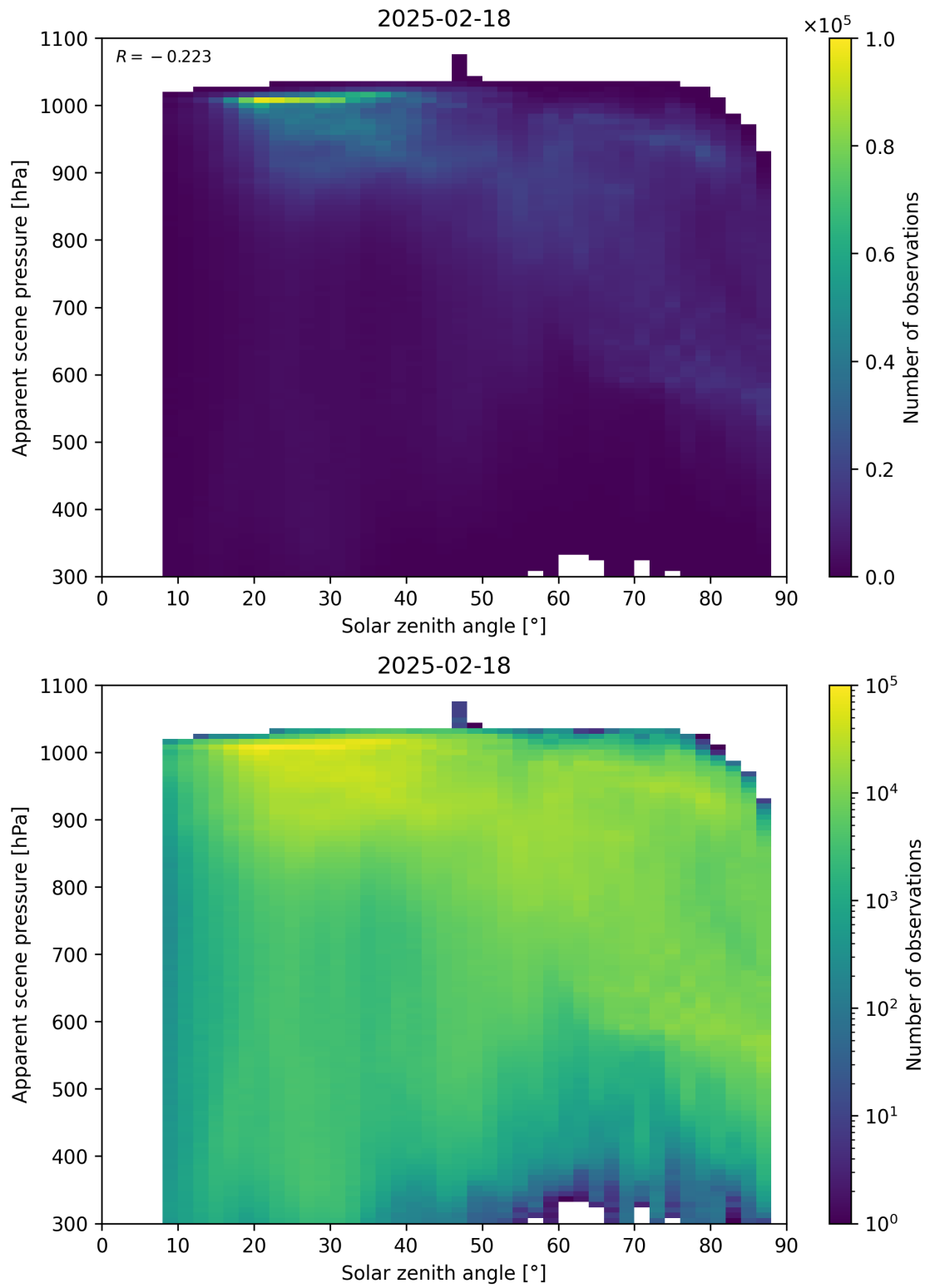
Figure 108: Scatter density plot of “Solar zenith angle” against “Apparent scene pressure” for 2025-02-18 to 2025-02-19.
