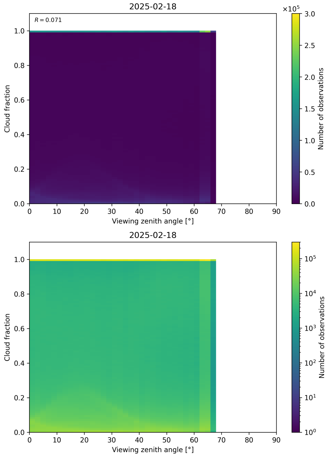
Figure 120: Scatter density plot of “Viewing zenith angle” against “Cloud fraction” for 2025-02-18 to 2025-02-19.
