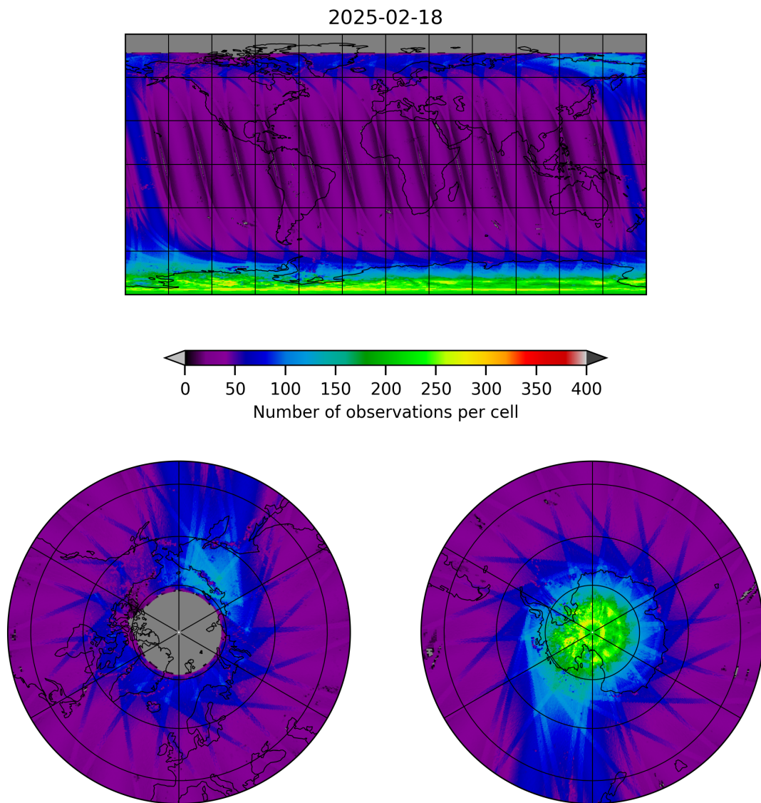
Figure 11: Map of the number of observations for 2025-02-18 to 2025-02-19
