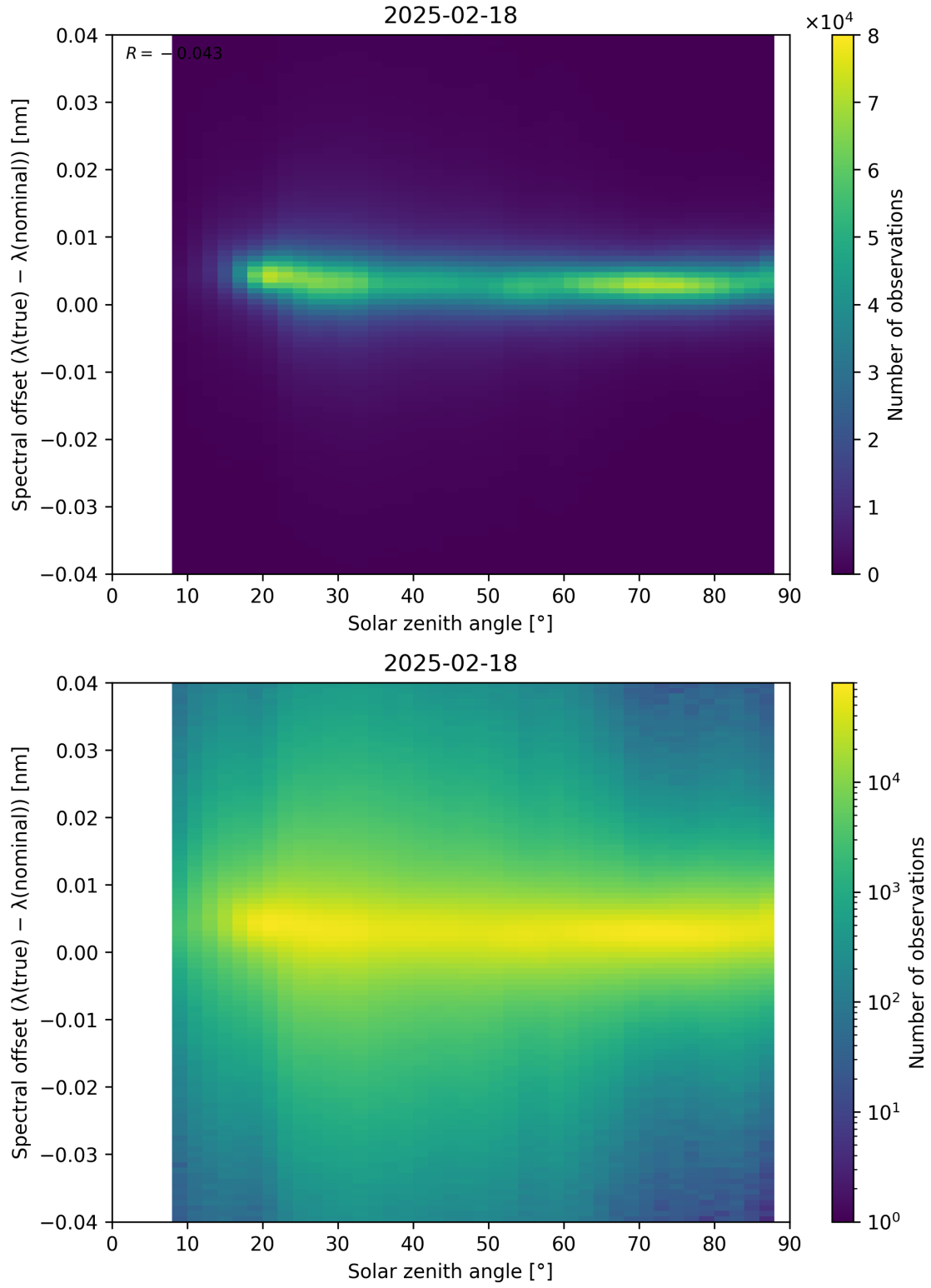
Figure 117: Scatter density plot of “Solar zenith angle” against “Spectral offset ( \lambda_{\text{true}} - \lambda_{\text{nominal}} )” for 2025-02-18 to 2025-02-19.
