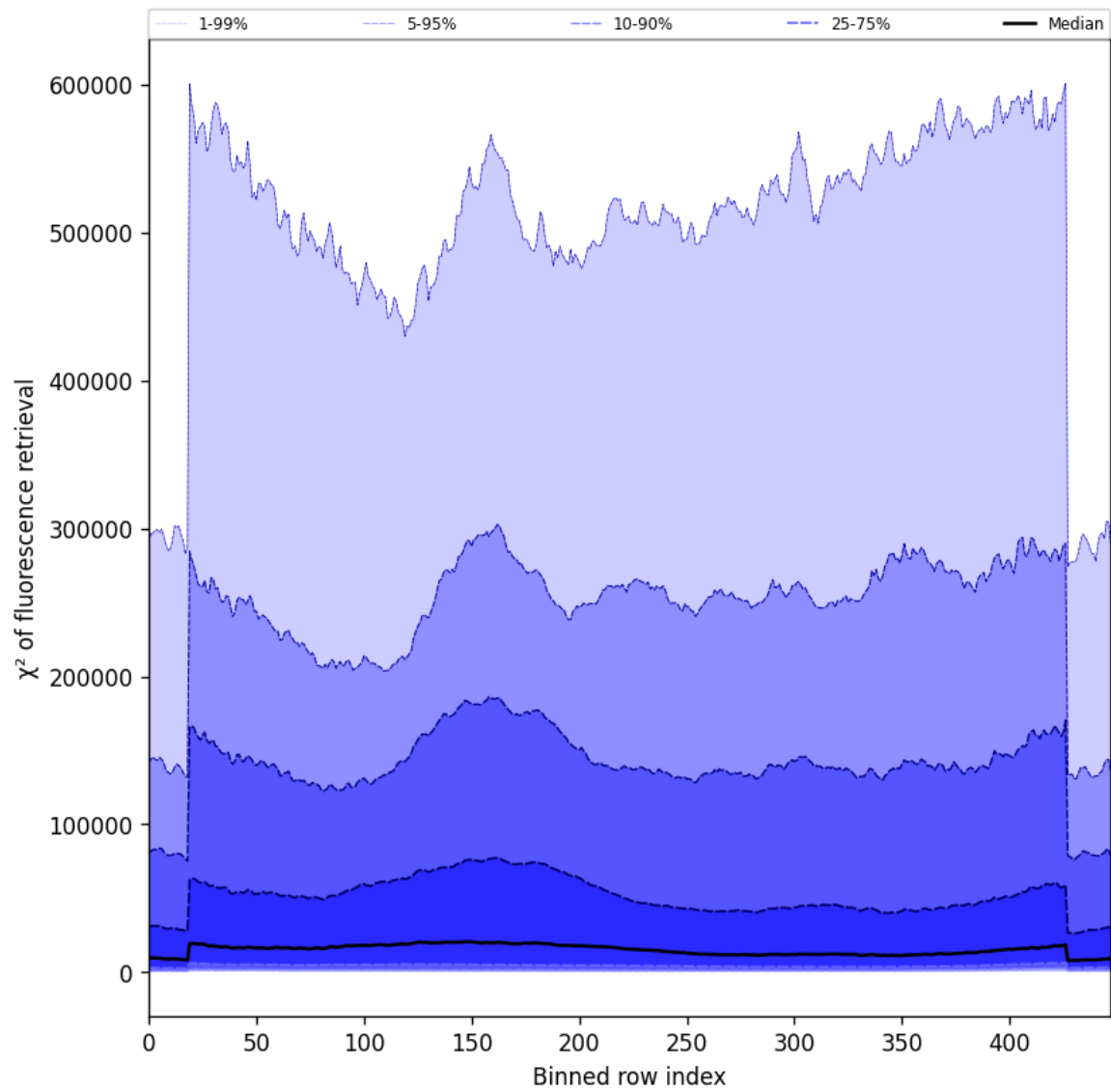
Figure 59: Along track statistics of “ \chi^2 of fluorescence retrieval” for 2025-02-18 to 2025-02-19
