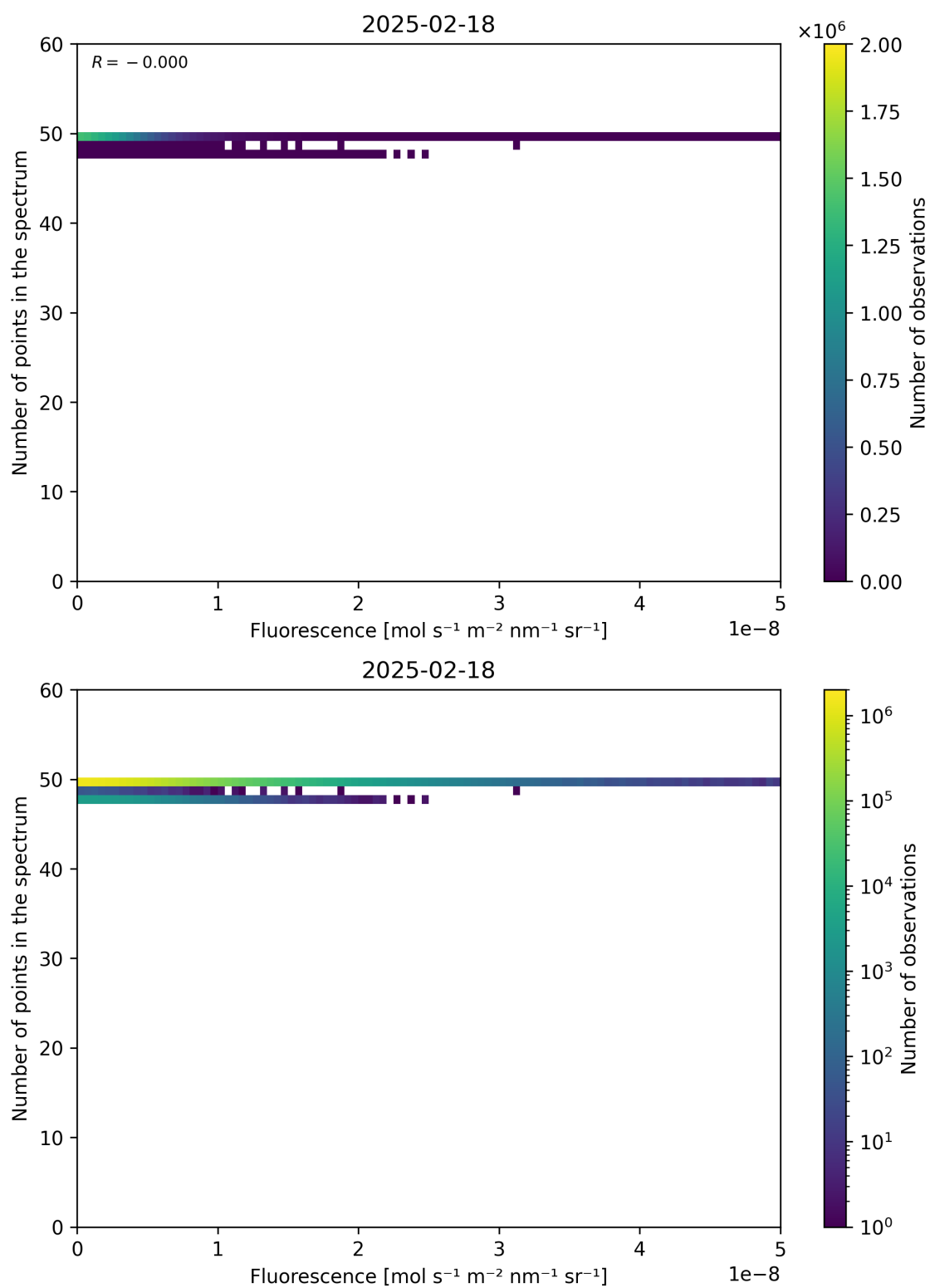
Figure 86: Scatter density plot of “Fluorescence” against “Number of points in the spectrum” for 2025-02-18 to 2025-02-19.
