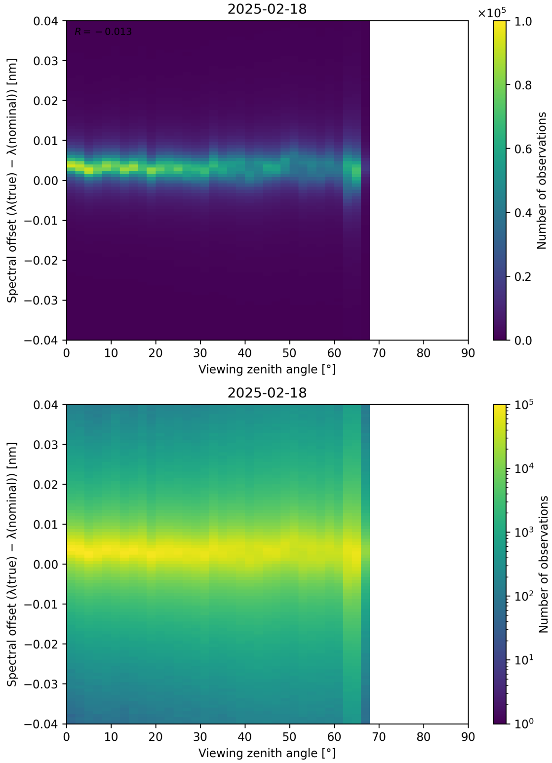
Figure 128: Scatter density plot of “Viewing zenith angle” against “Spectral offset ( \lambda_{\text{true}} - \lambda_{\text{nominal}} )” for 2025-02-18 to 2025-02-19.
