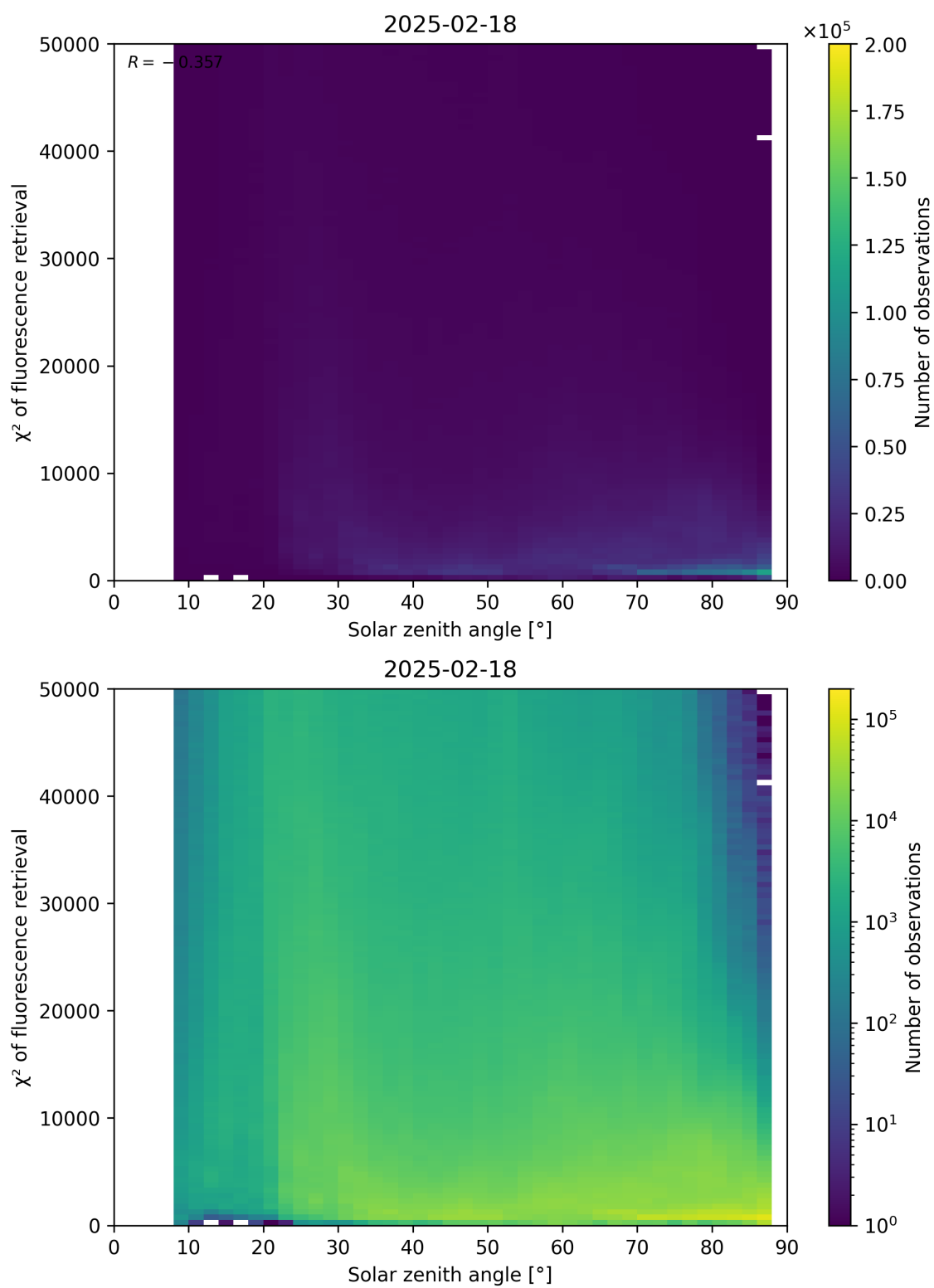
Figure 109: Scatter density plot of “Solar zenith angle” against “ \chi^2 of fluorescence retrieval” for 2025-02-18 to 2025-02-19.
