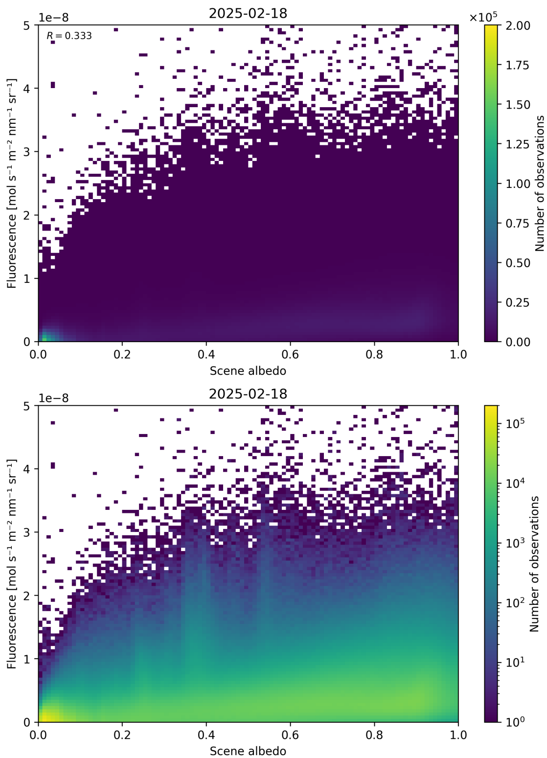
Figure 104: Scatter density plot of “Scene albedo” against “Fluorescence” for 2025-02-18 to 2025-02-19.
