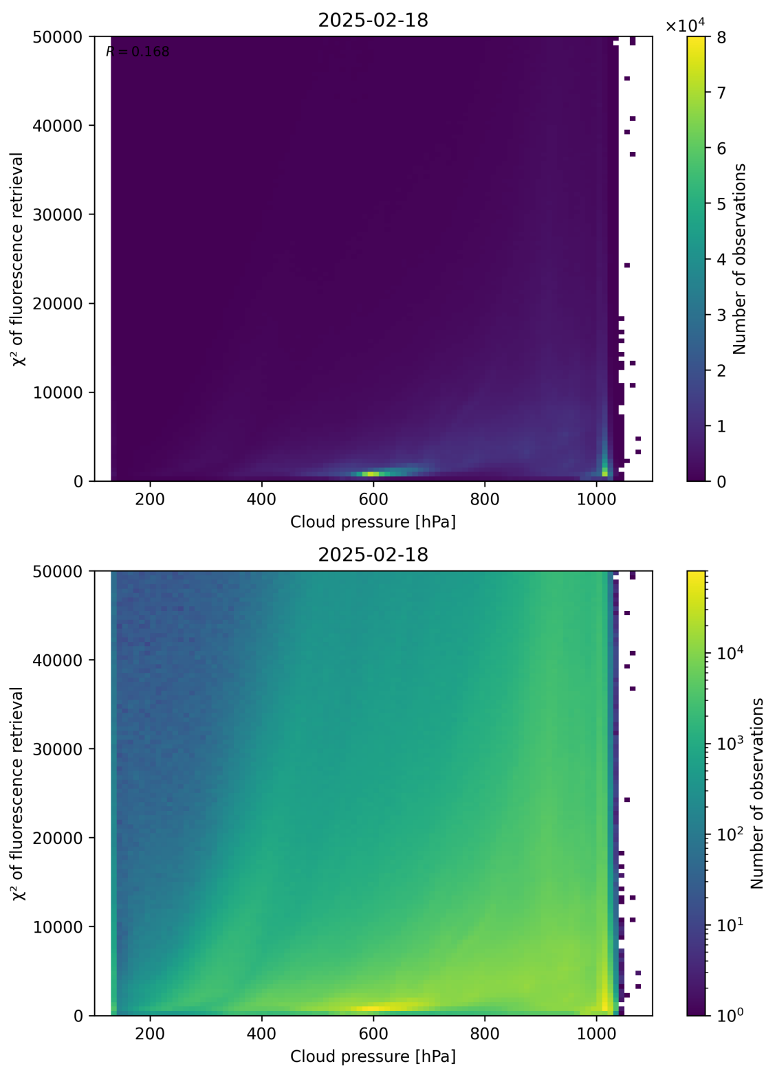
Figure 78: Scatter density plot of “Cloud pressure” against “ \chi^2 of fluorescence retrieval” for 2025-02-18 to 2025-02-19.
