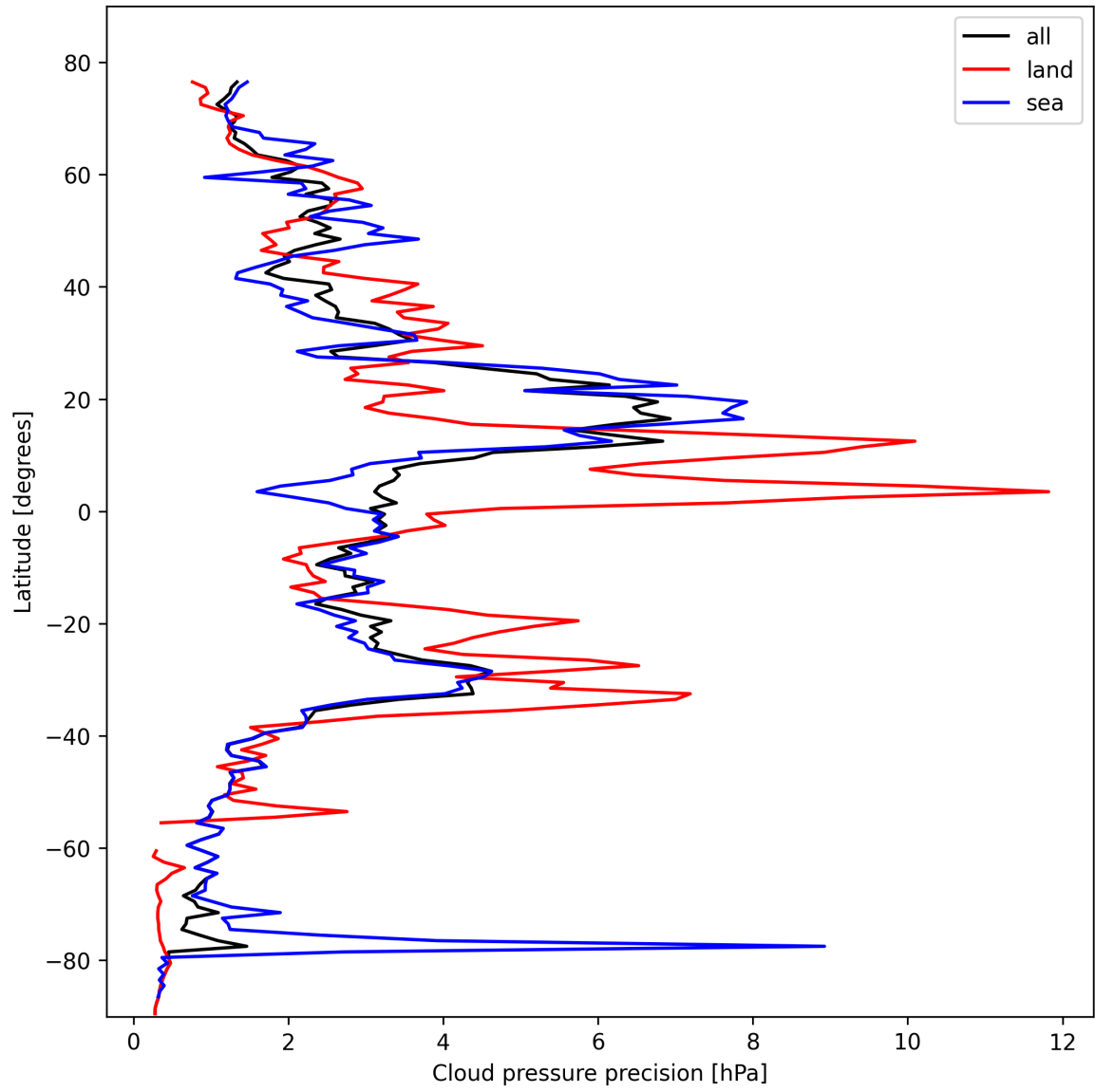
Figure 14: Zonal average of “Cloud pressure precision” for 2025-02-18 to 2025-02-19.
