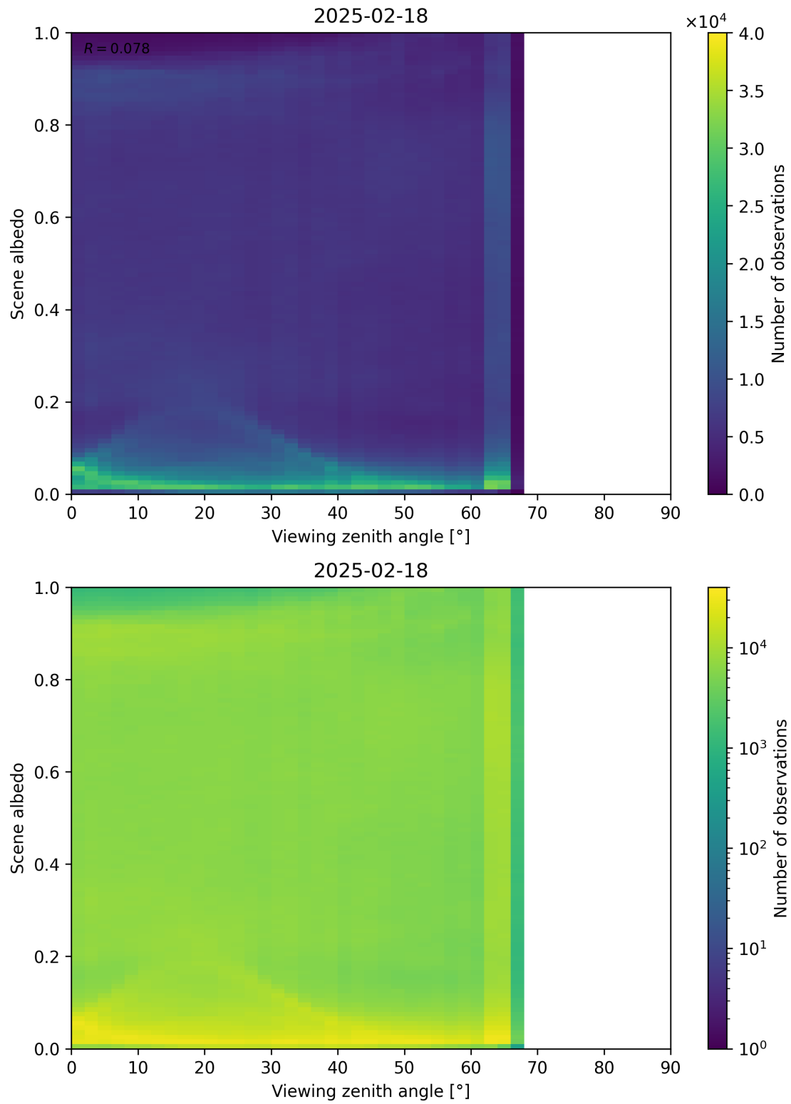
Figure 126: Scatter density plot of “Viewing zenith angle” against “Scene albedo” for 2025-02-18 to 2025-02-19.
