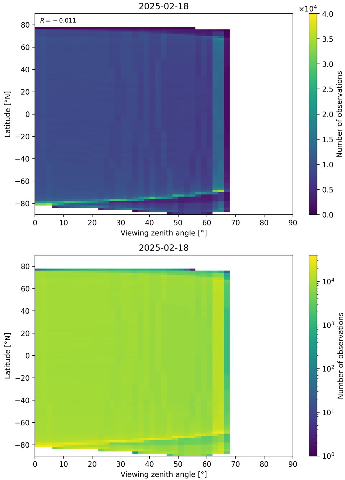
Figure 123: Scatter density plot of “Viewing zenith angle” against “Latitude” for 2025-02-18 to 2025-02-19.
