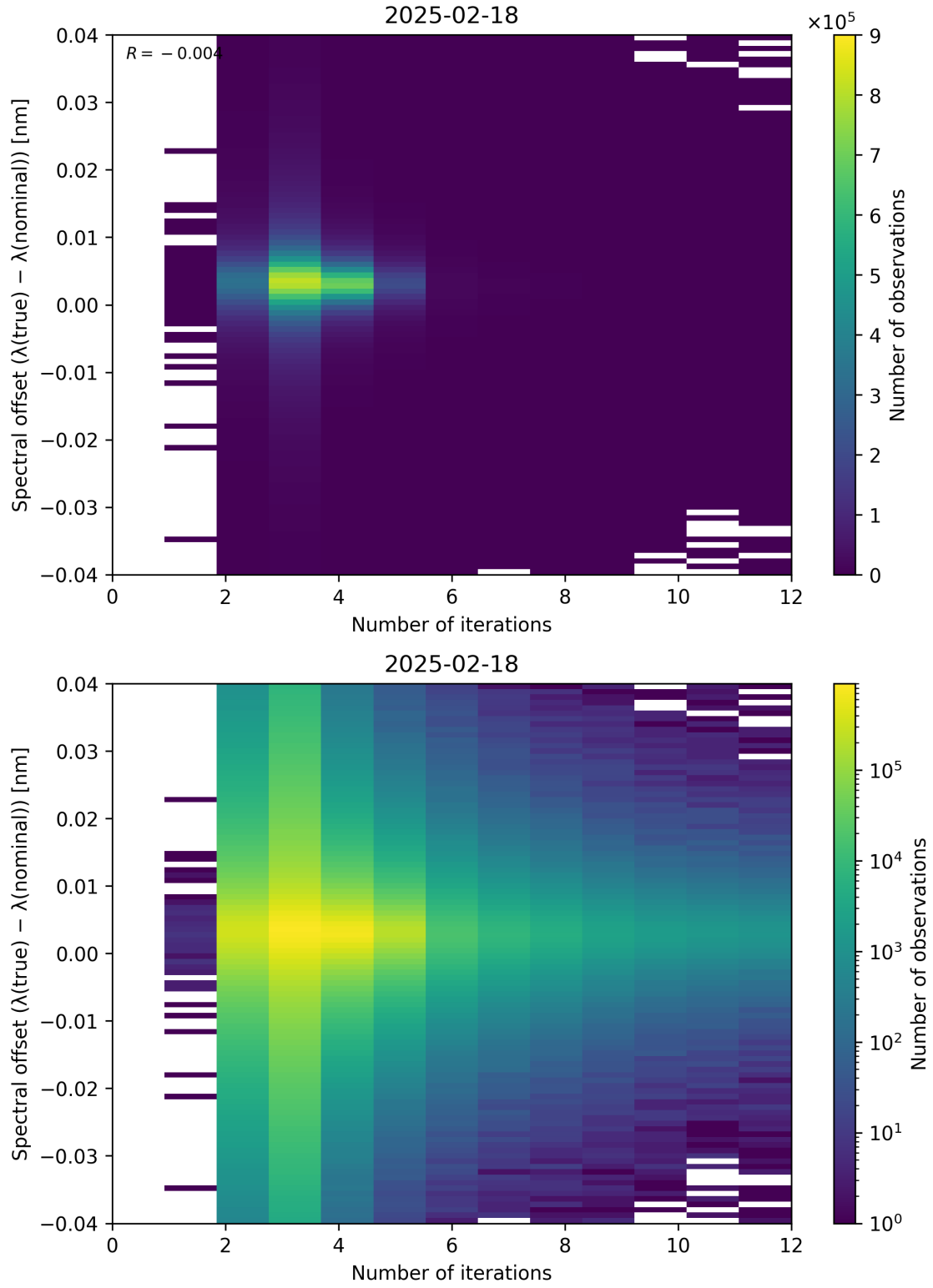
Figure 100: Scatter density plot of “Number of iterations” against “Spectral offset ( \lambda_{\text{true}} - \lambda_{\text{nominal}} )” for 2025-02-18 to 2025-02-19.
