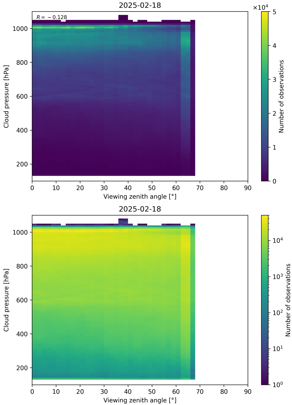
Figure 121: Scatter density plot of “Viewing zenith angle” against “Cloud pressure” for 2025-02-18 to 2025-02-19.
