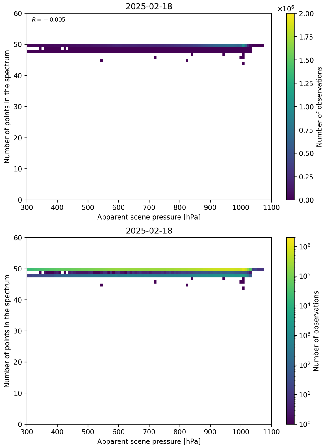
Figure 66: Scatter density plot of “Apparent scene pressure” against “Number of points in the spectrum” for 2025-02-18 to 2025-02-19.
