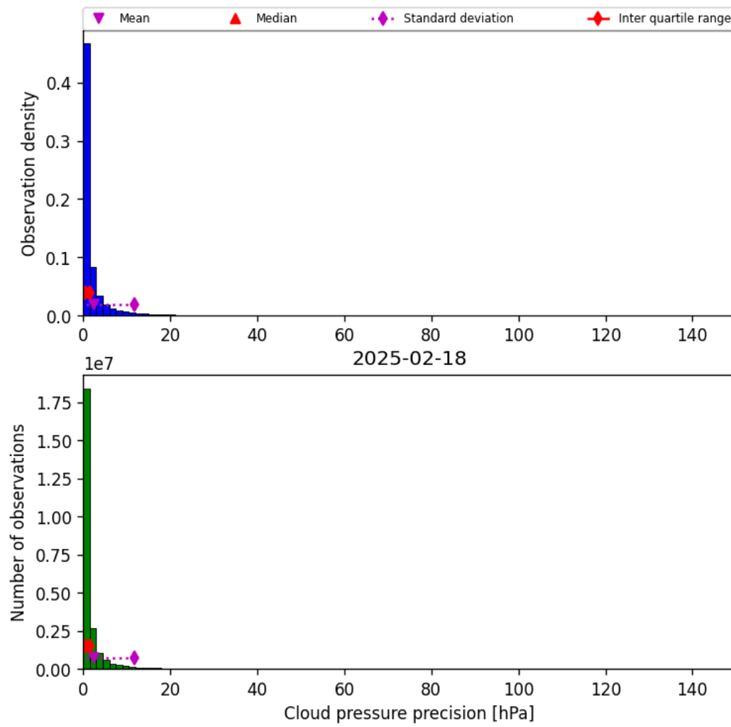
Figure 31: Histogram of “Cloud pressure precision” for 2025-02-18 to 2025-02-19
