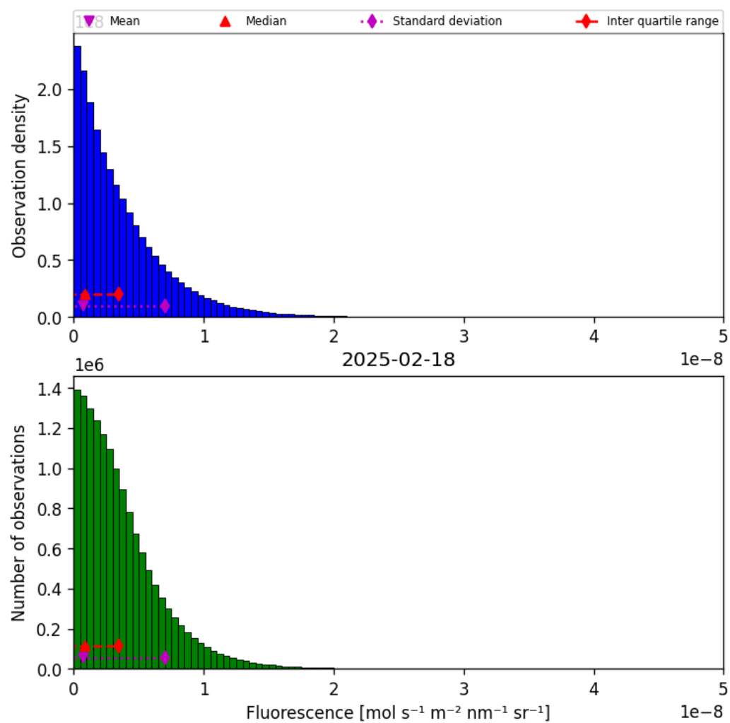
Figure 40: Histogram of “Fluorescence” for 2025-02-18 to 2025-02-19
