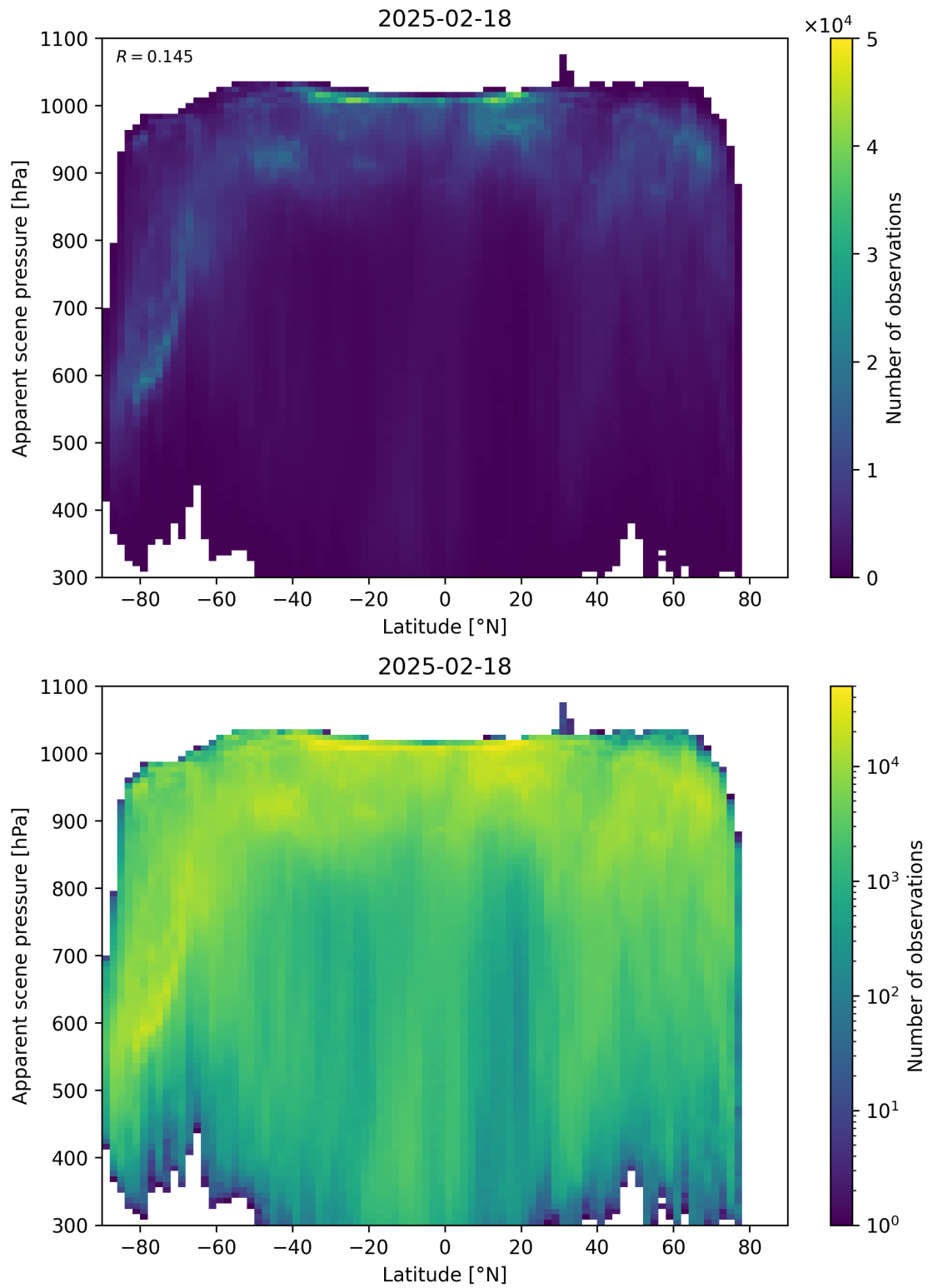
Figure 88: Scatter density plot of “Latitude” against “Apparent scene pressure” for 2025-02-18 to 2025-02-19.
