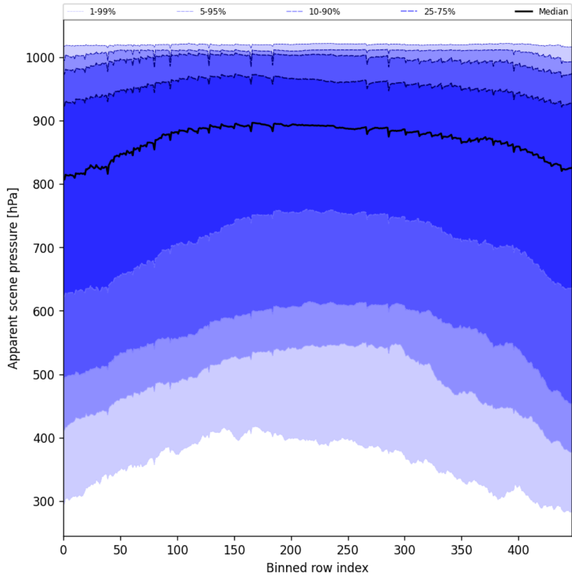
Figure 53: Along track statistics of “Apparent scene pressure” for 2025-02-18 to 2025-02-19
