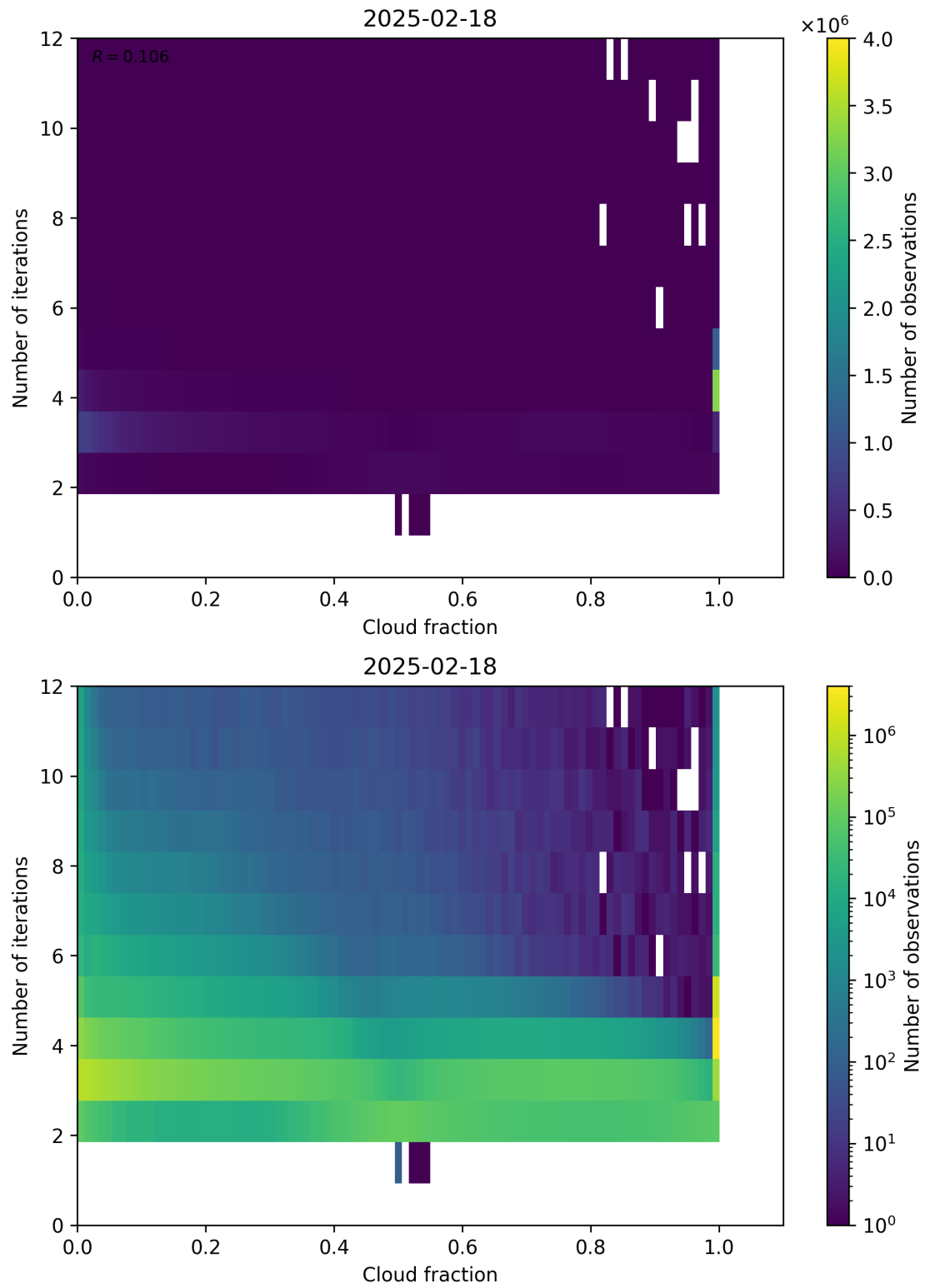
Figure 73: Scatter density plot of “Cloud fraction” against “Number of iterations” for 2025-02-18 to 2025-02-19.
