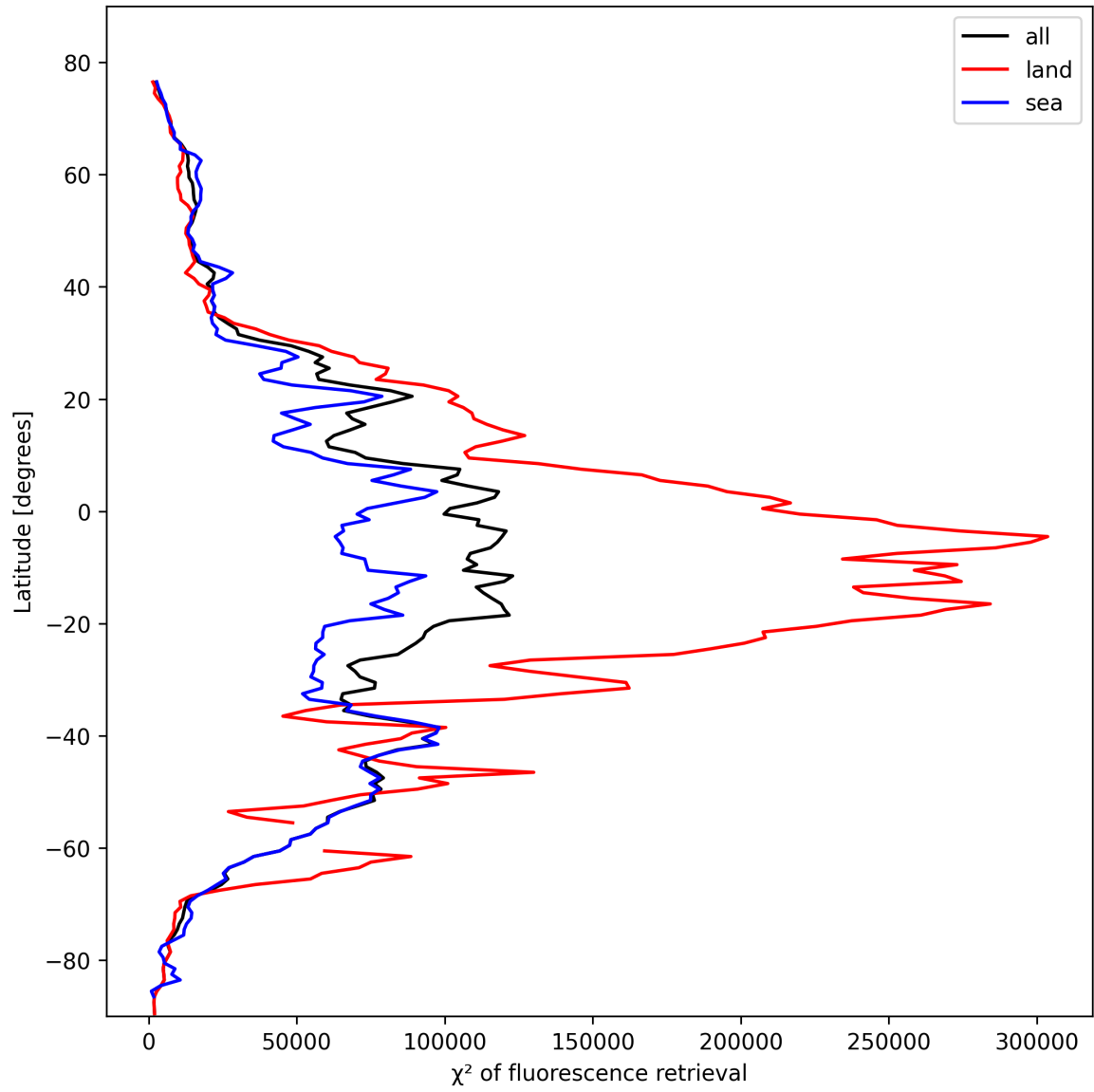
Figure 25: Zonal average of “ \chi^2 of fluorescence retrieval” for 2025-02-18 to 2025-02-19.
