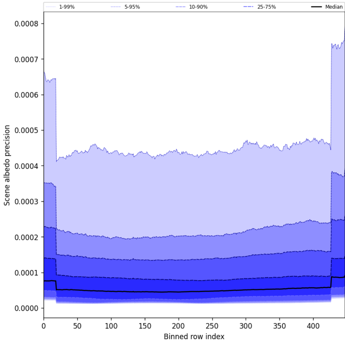
Figure 52: Along track statistics of “Scene albedo precision” for 2025-02-18 to 2025-02-19
