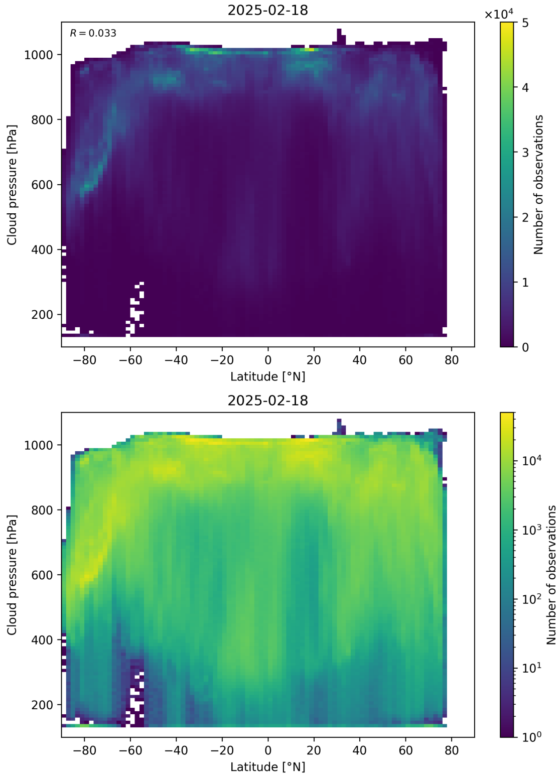
Figure 91: Scatter density plot of “Latitude” against “Cloud pressure” for 2025-02-18 to 2025-02-19.
