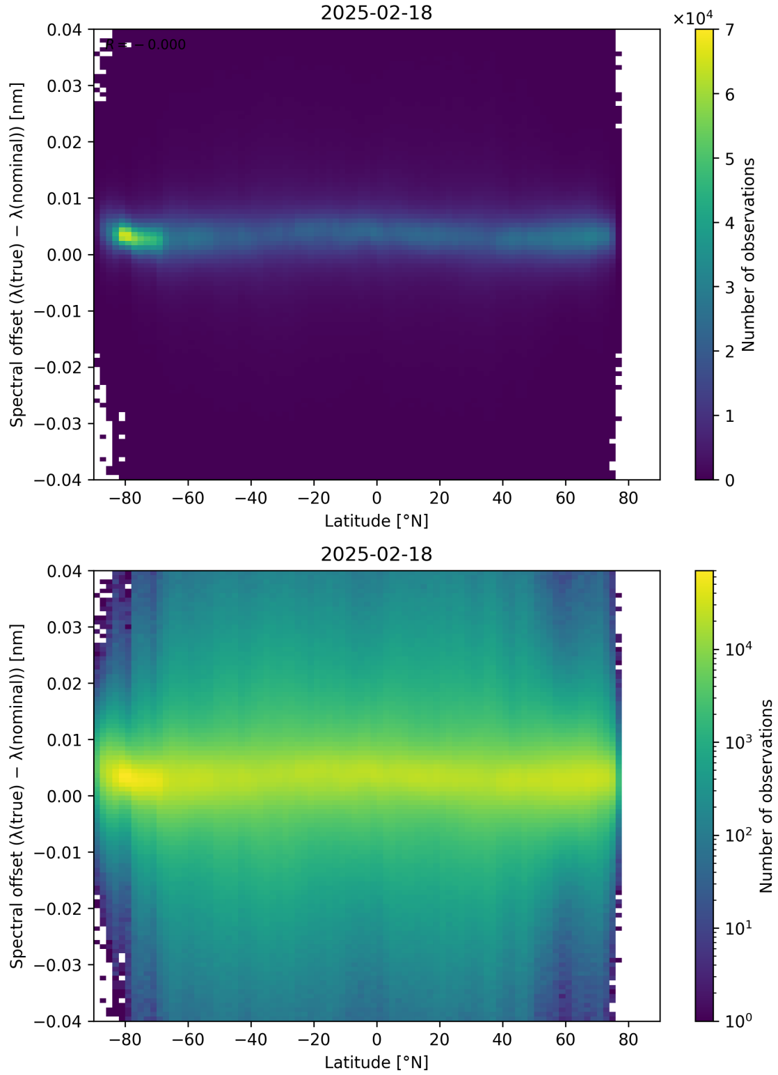
Figure 96: Scatter density plot of “Latitude” against “Spectral offset ( \lambda_{\text{true}} - \lambda_{\text{nominal}} )” for 2025-02-18 to 2025-02-19.
