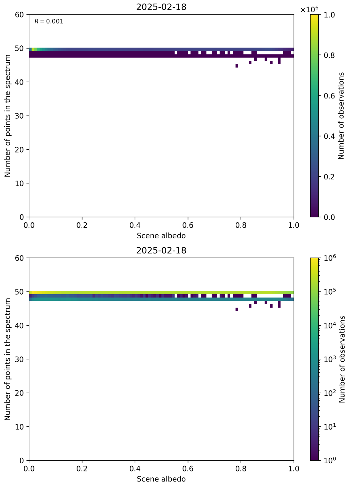
Figure 106: Scatter density plot of “Scene albedo” against “Number of points in the spectrum” for 2025-02-18 to 2025-02-19.
