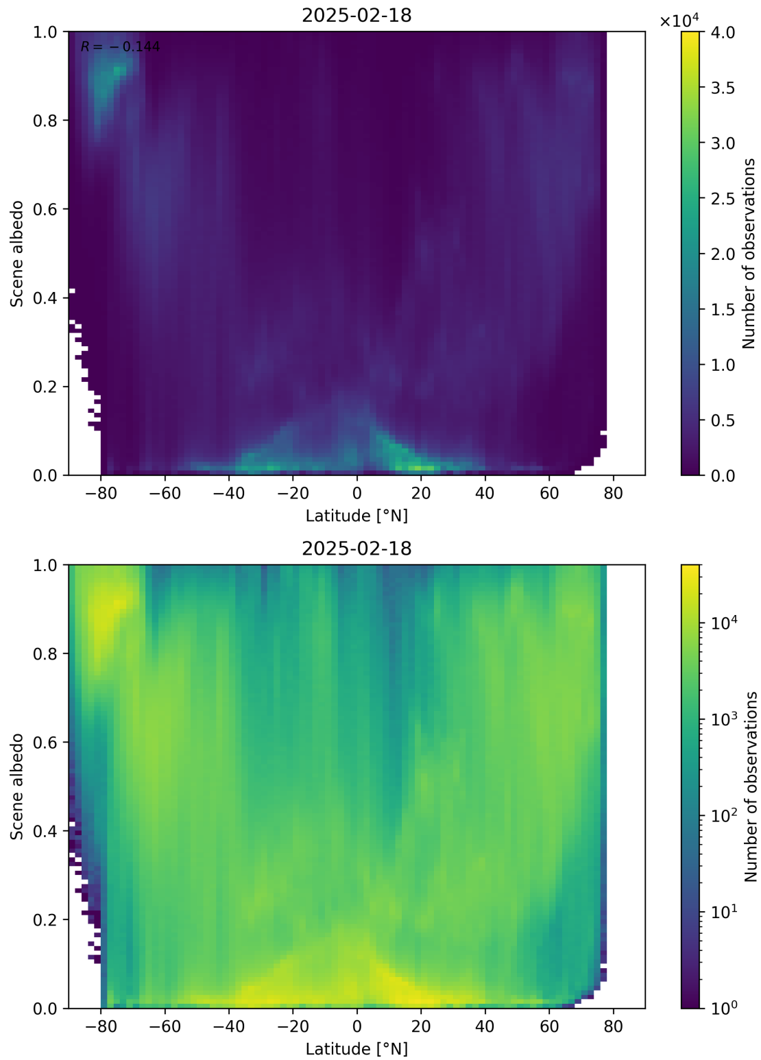
Figure 95: Scatter density plot of “Latitude” against “Scene albedo” for 2025-02-18 to 2025-02-19.
