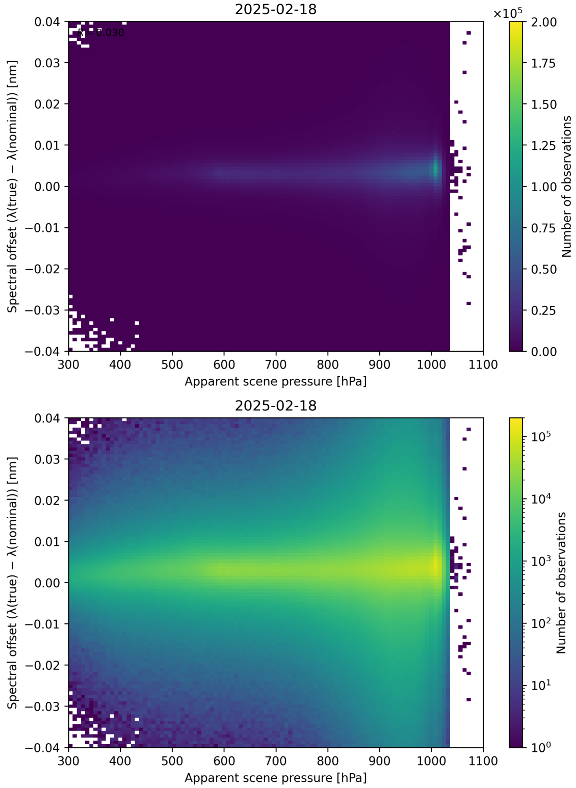
Figure 67: Scatter density plot of “Apparent scene pressure” against “Spectral offset ( \lambda_{\text{true}} - \lambda_{\text{nominal}} )” for 2025-02-18 to 2025-02-19.
