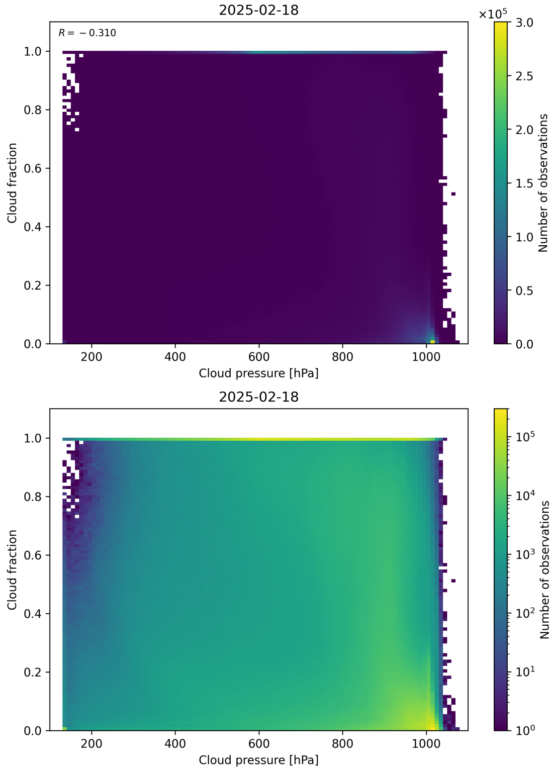
Figure 79: Scatter density plot of “Cloud pressure” against “Cloud fraction” for 2025-02-18 to 2025-02-19.
