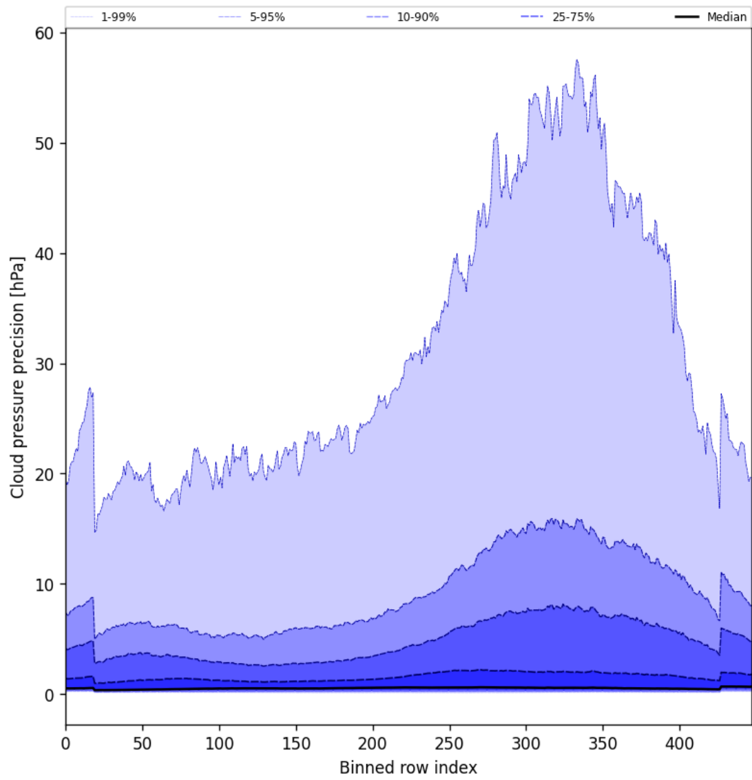
Figure 48: Along track statistics of “Cloud pressure precision” for 2025-02-18 to 2025-02-19
