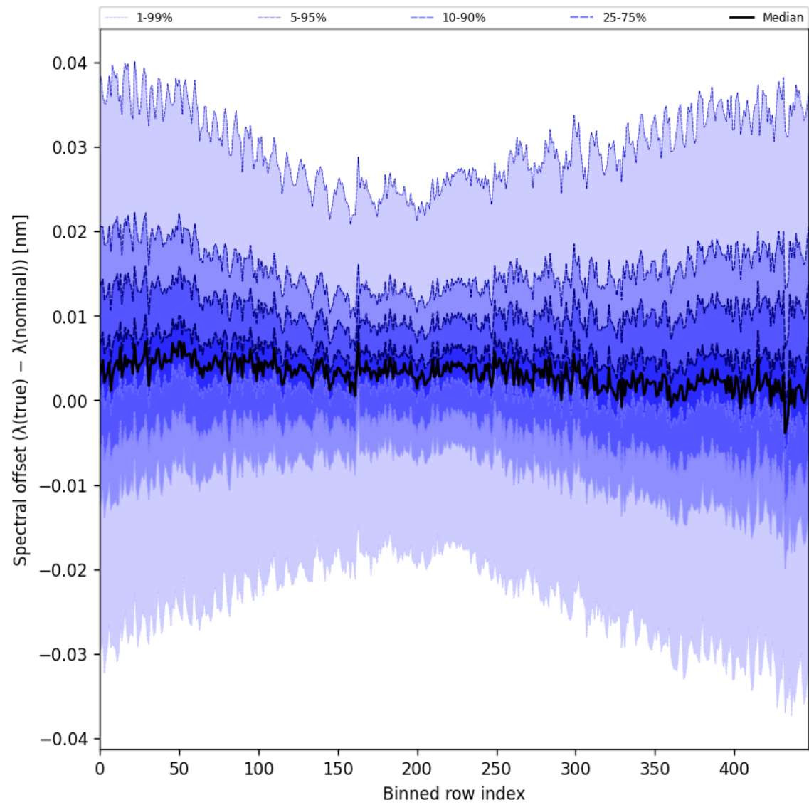
Figure 62: Along track statistics of “Spectral offset ( \lambda_{\text{true}} - \lambda_{\text{nominal}} )” for 2025-02-18 to 2025-02-19
