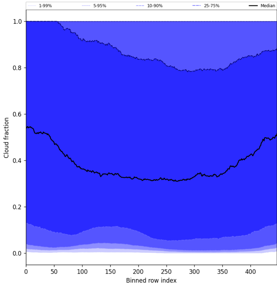
Figure 49: Along track statistics of “Cloud fraction” for 2025-02-18 to 2025-02-19
