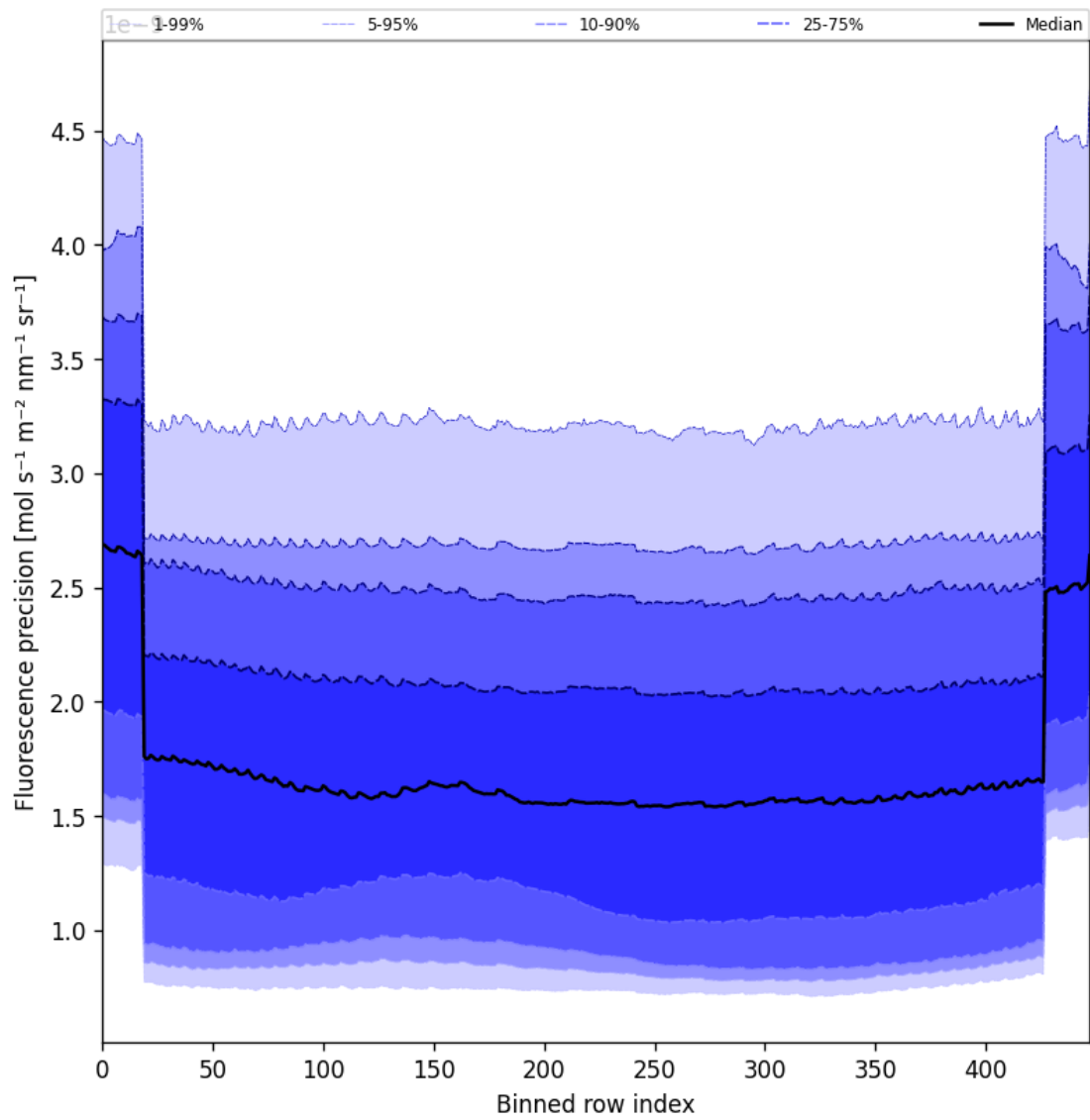
Figure 58: Along track statistics of “Fluorescence precision” for 2025-02-18 to 2025-02-19
