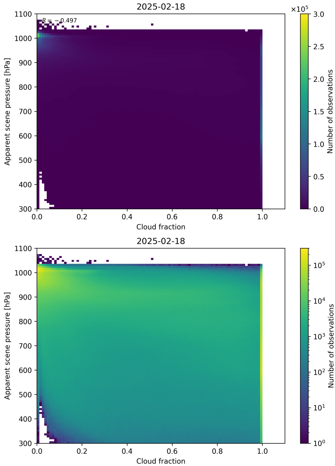
Figure 70: Scatter density plot of “Cloud fraction” against “Apparent scene pressure” for 2025-02-18 to 2025-02-19.
