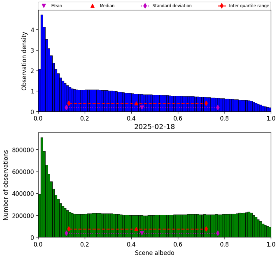
Figure 34: Histogram of “Scene albedo” for 2025-02-18 to 2025-02-19
