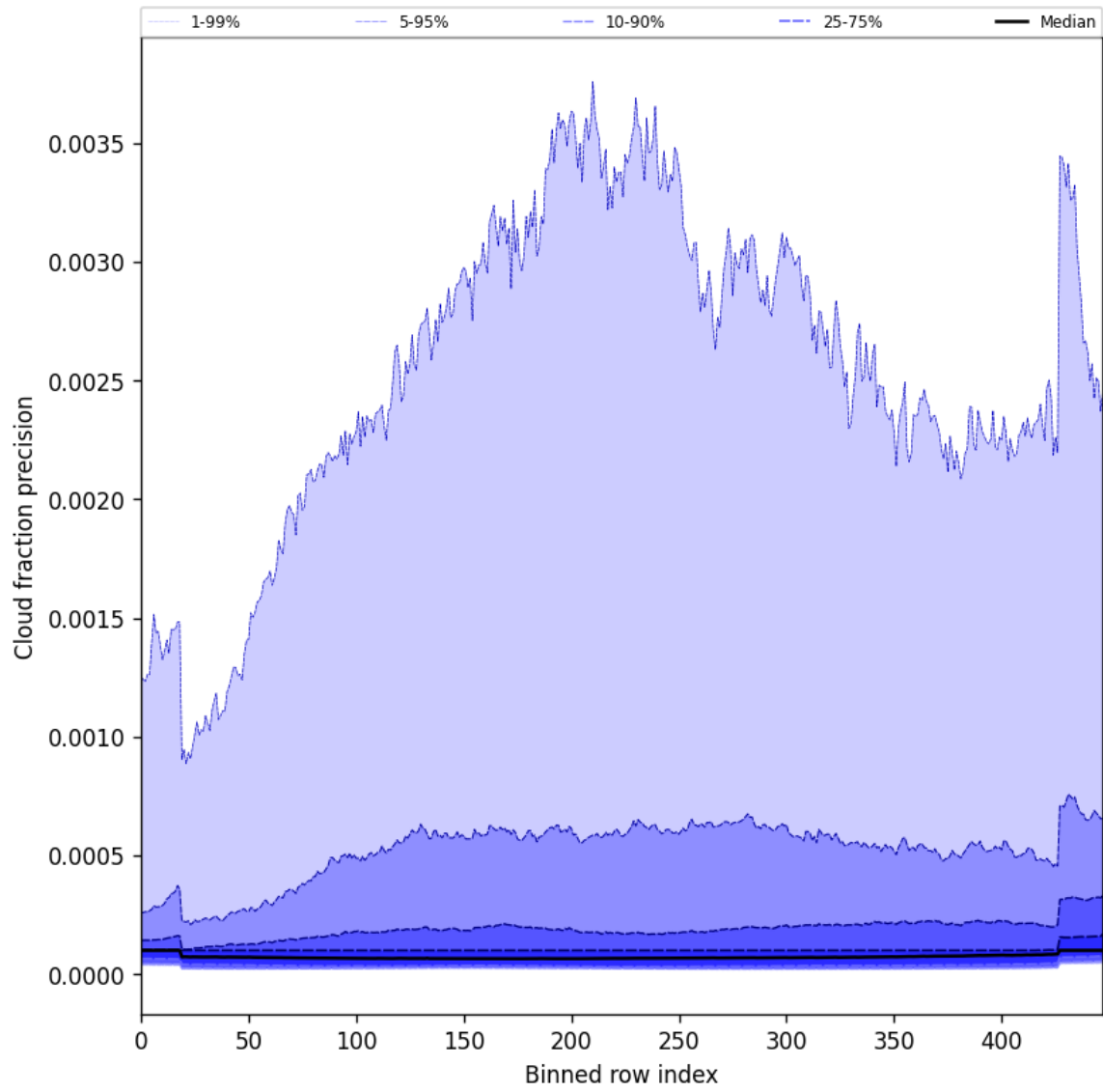
Figure 50: Along track statistics of “Cloud fraction precision” for 2025-02-18 to 2025-02-19
