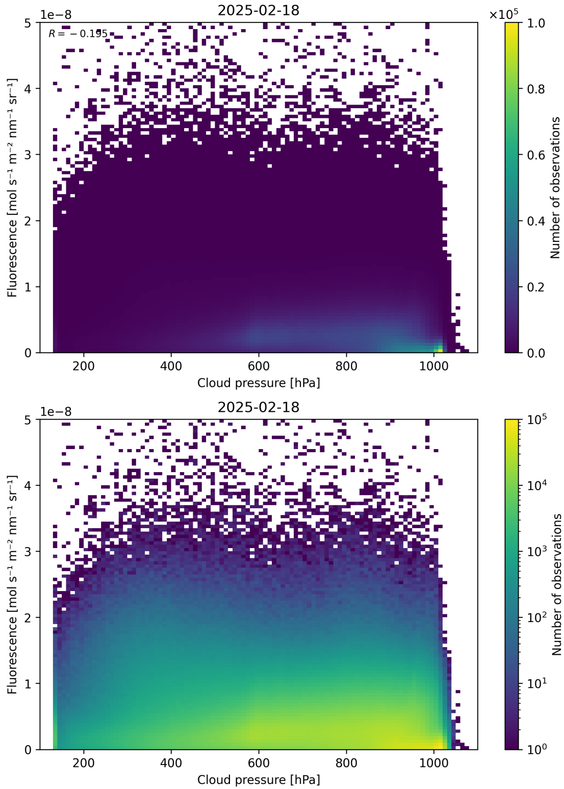
Figure 80: Scatter density plot of “Cloud pressure” against “Fluorescence” for 2025-02-18 to 2025-02-19.
