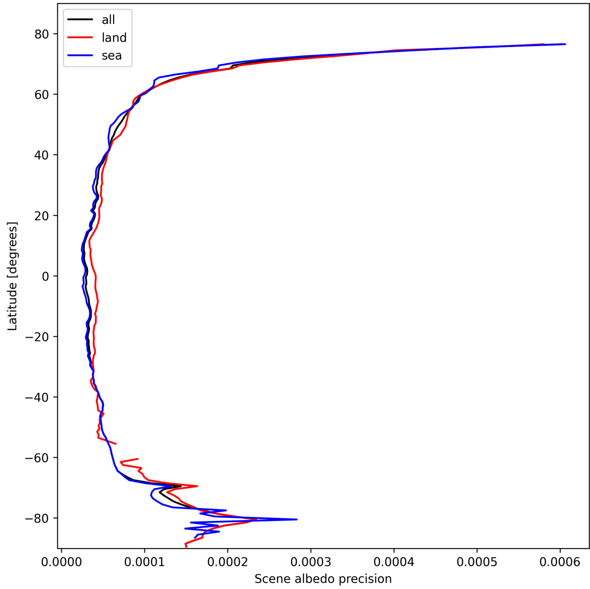
Figure 18: Zonal average of “Scene albedo precision” for 2025-02-18 to 2025-02-19.
