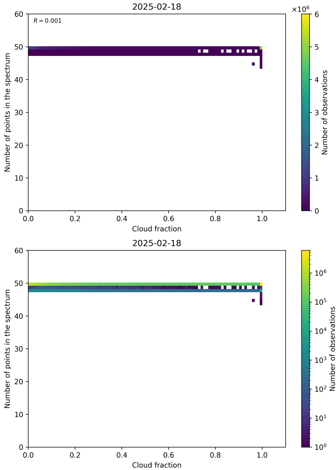
Figure 74: Scatter density plot of “Cloud fraction” against “Number of points in the spectrum” for 2025-02-18 to 2025-02-19.
