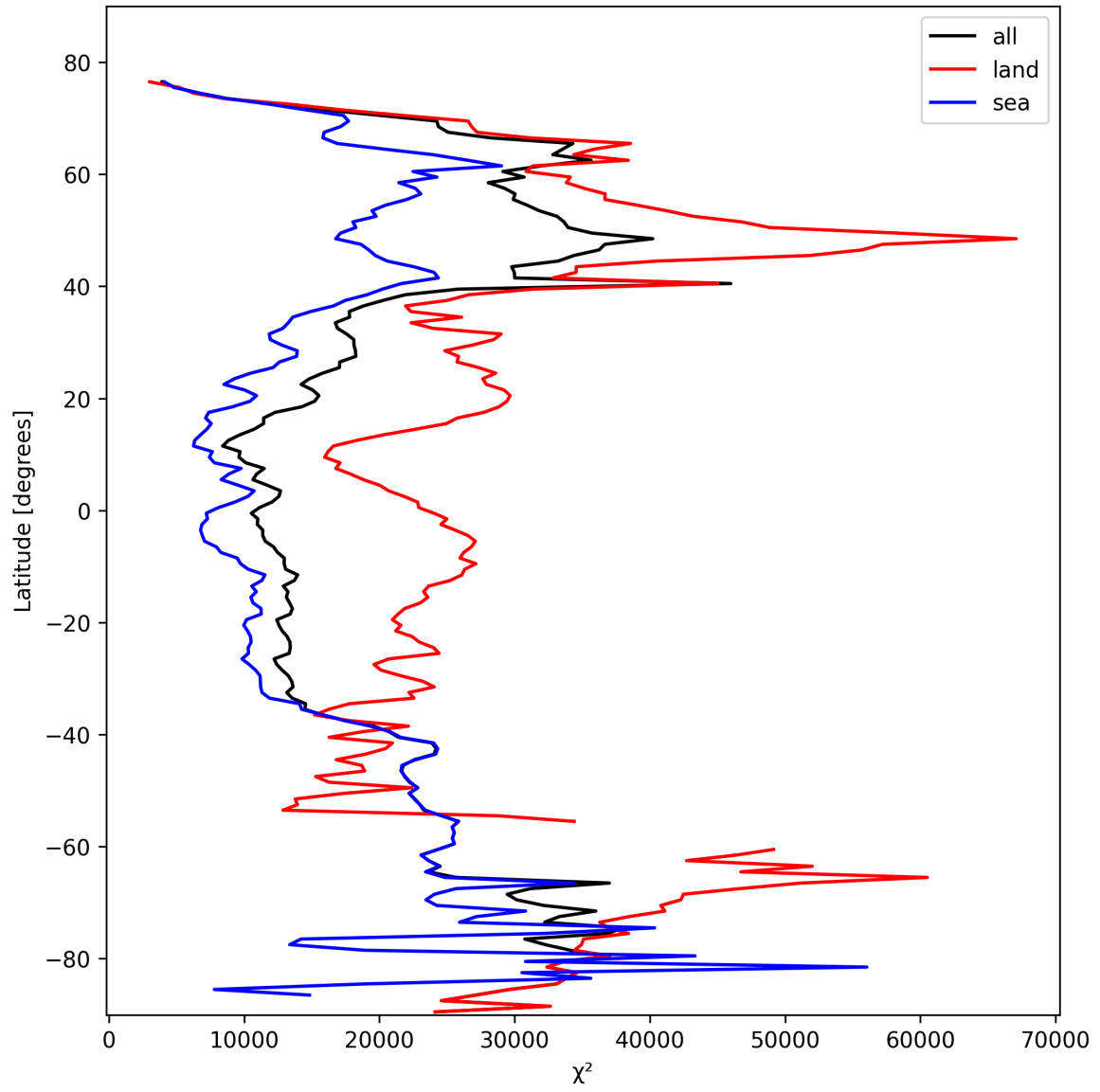
Figure 21: Zonal average of “ \chi^2 ” for 2025-02-18 to 2025-02-19.
