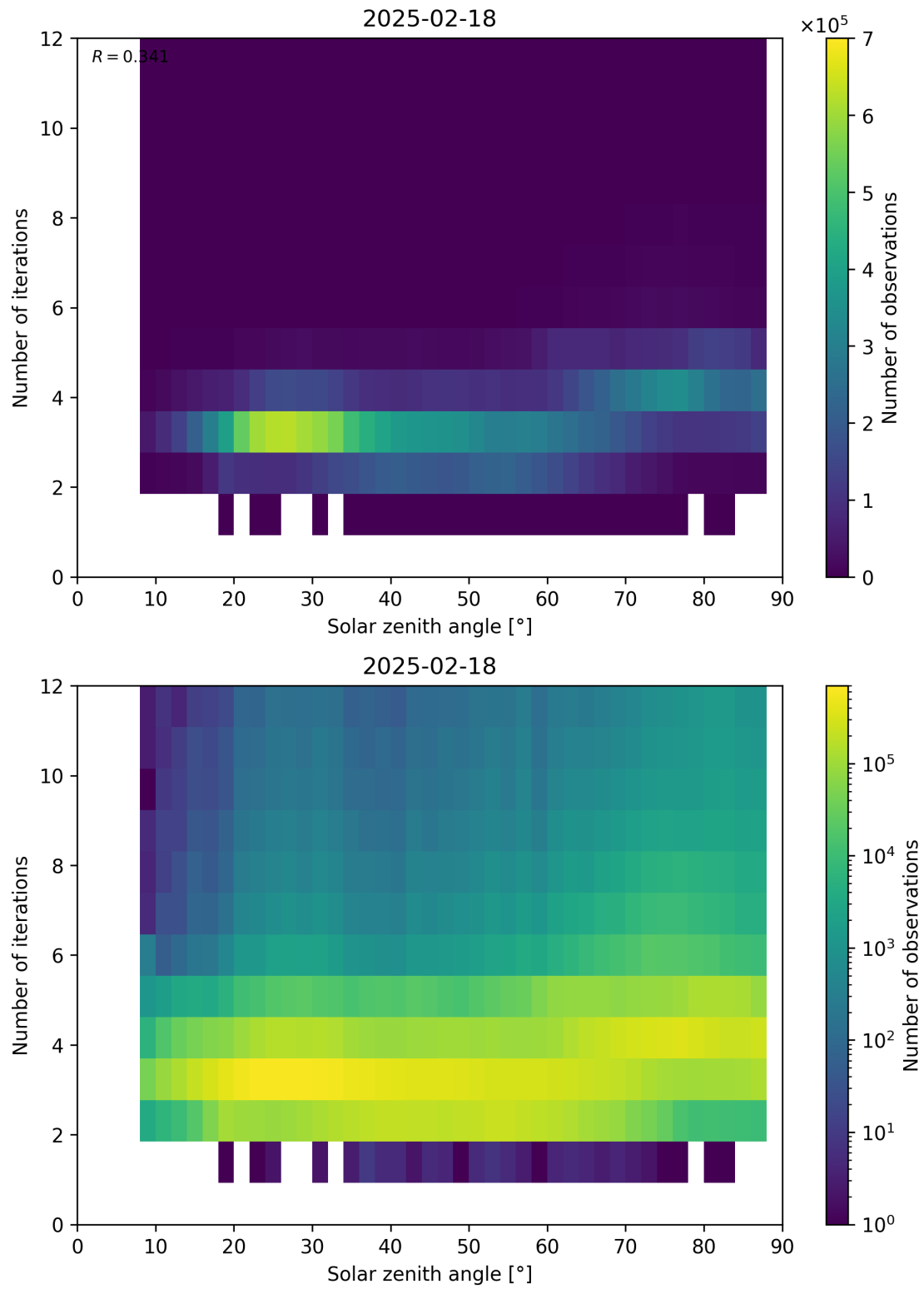
Figure 114: Scatter density plot of “Solar zenith angle” against “Number of iterations” for 2025-02-18 to 2025-02-19.
