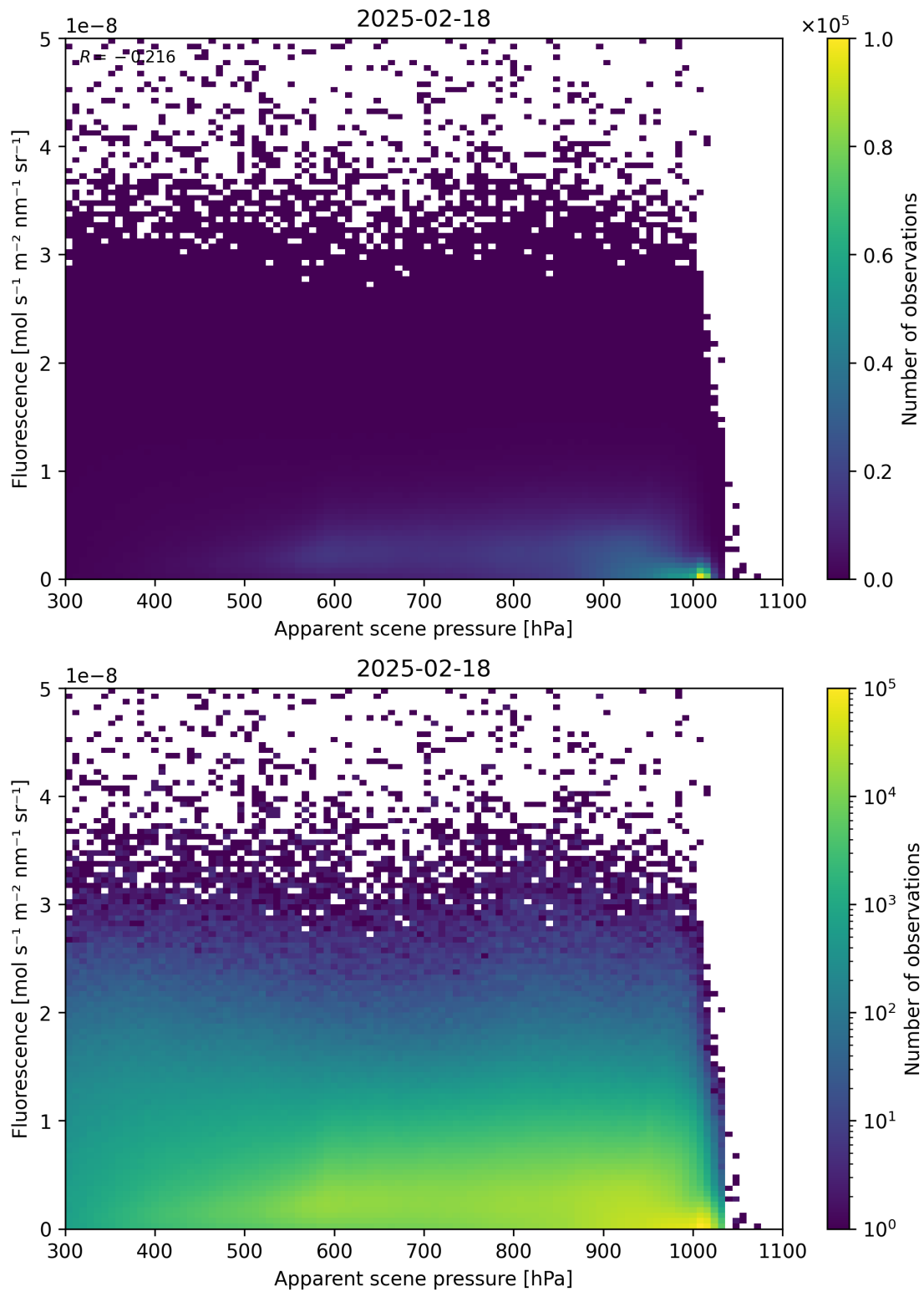
Figure 64: Scatter density plot of “Apparent scene pressure” against “Fluorescence” for 2025-02-18 to 2025-02-19.
