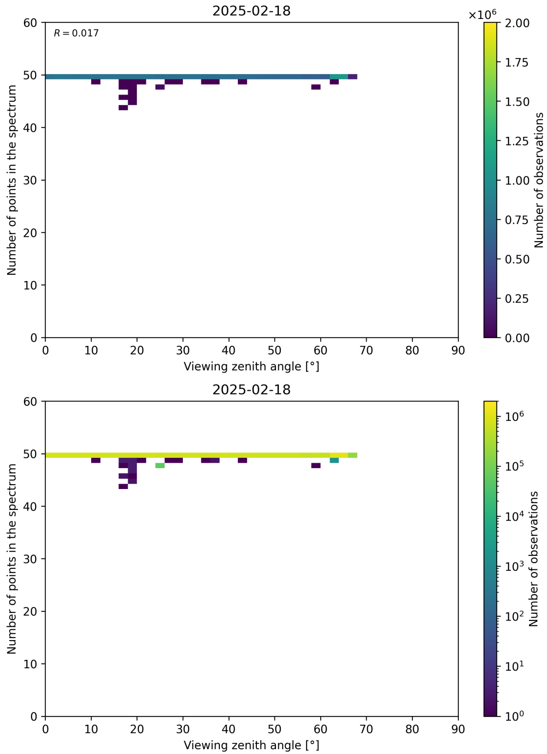
Figure 125: Scatter density plot of “Viewing zenith angle” against “Number of points in the spectrum” for 2025-02-18 to 2025-02-19.
