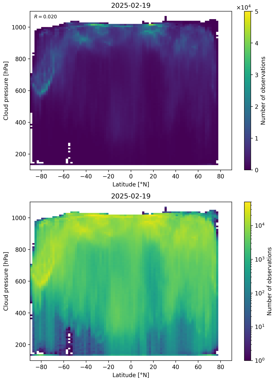
Figure 91: Scatter density plot of “Latitude” against “Cloud pressure” for 2025-02-19 to 2025-02-20.
