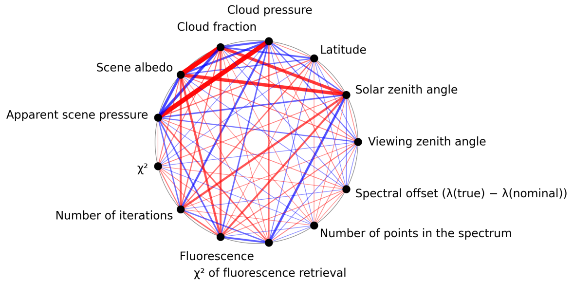
Figure 1: Map of correlation graph for 2025-02-19 to 2025-02-20.
