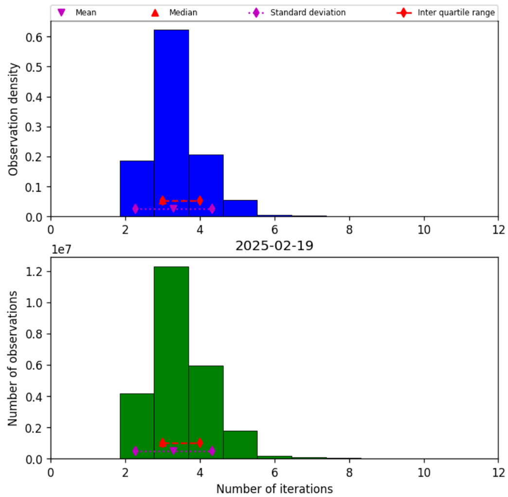
Figure 39: Histogram of “Number of iterations” for 2025-02-19 to 2025-02-20
