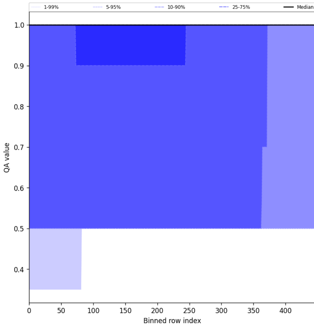
Figure 46: Along track statistics of “QA value” for 2025-02-19 to 2025-02-20
