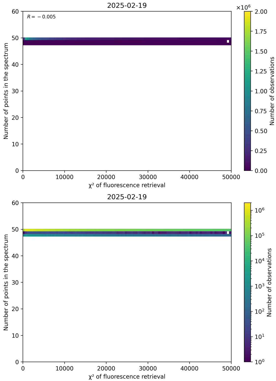
Figure 68: Scatter density plot of “ \chi^2 of fluorescence retrieval” against “Number of points in the spectrum” for 2025-02-19 to 2025-02-20.
