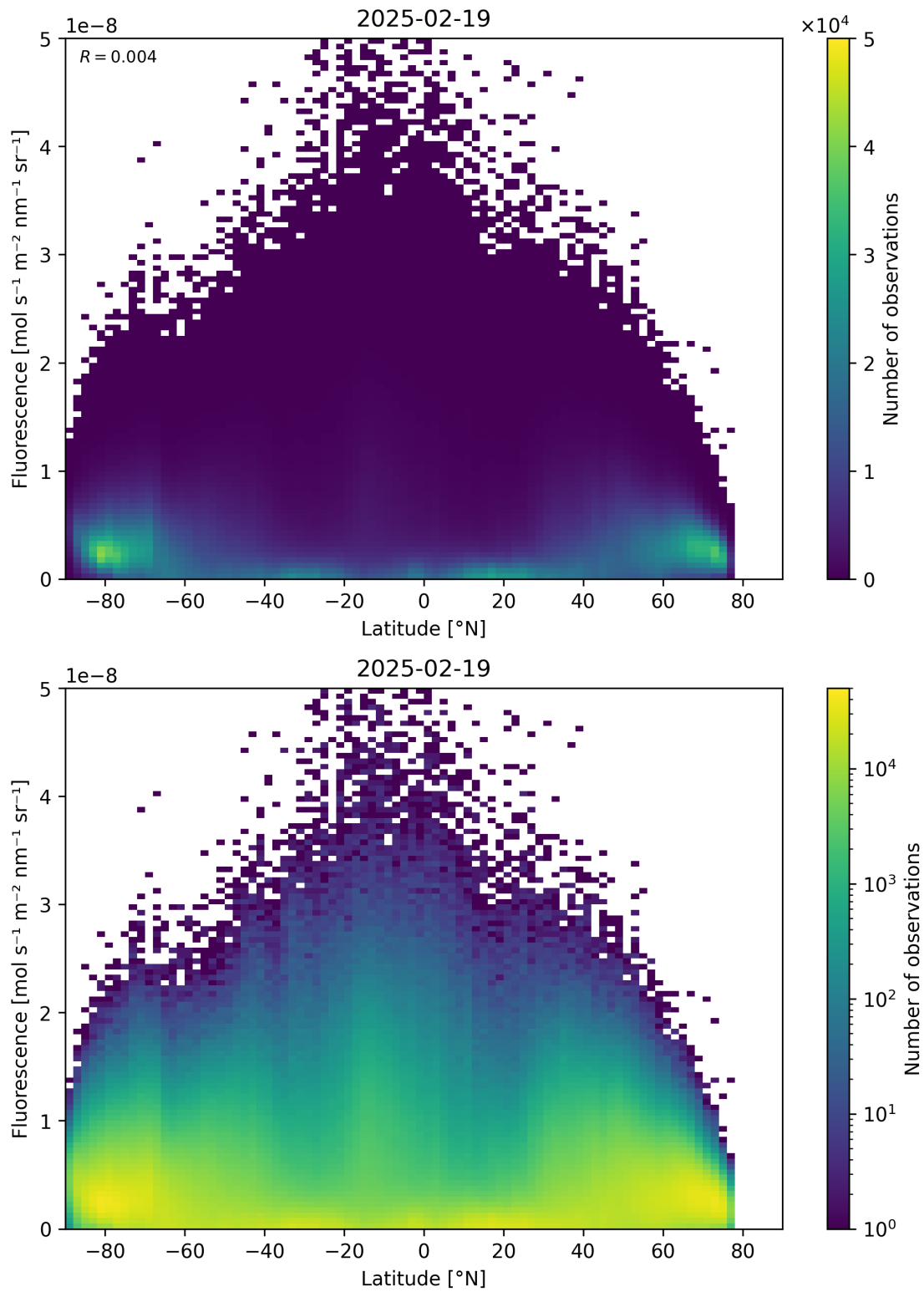
Figure 92: Scatter density plot of “Latitude” against “Fluorescence” for 2025-02-19 to 2025-02-20.
