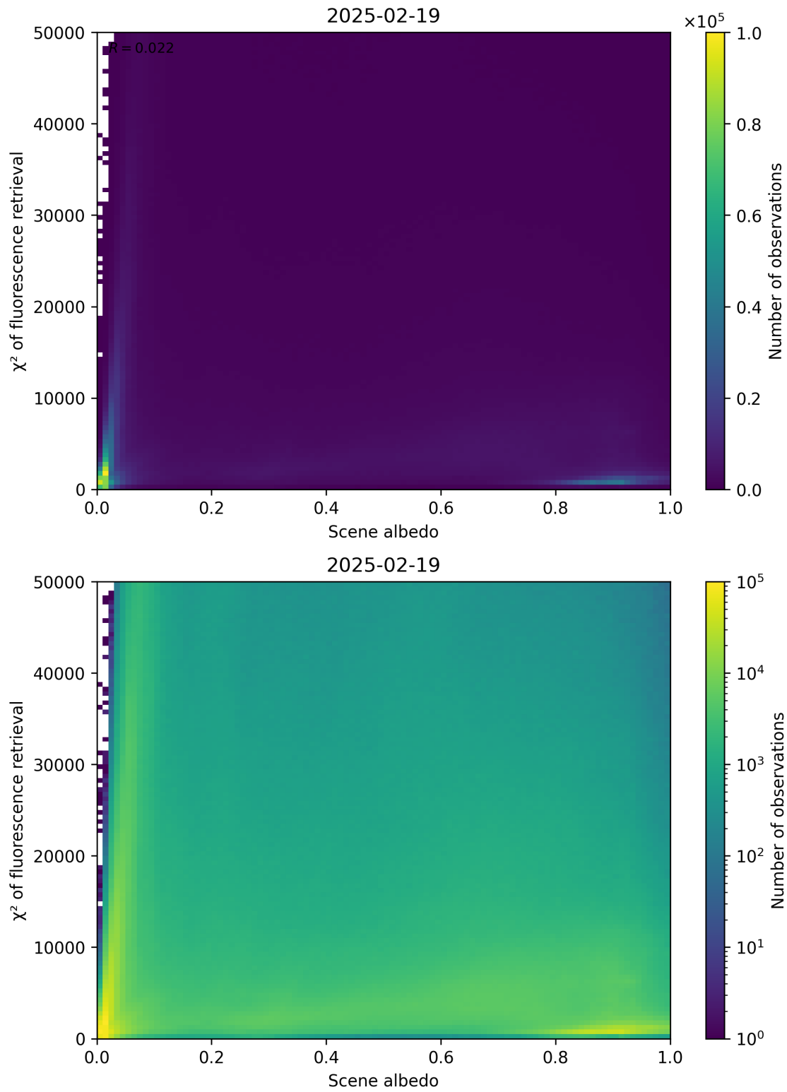
Figure 103: Scatter density plot of “Scene albedo” against “ \chi^2 of fluorescence retrieval” for 2025-02-19 to 2025-02-20.
