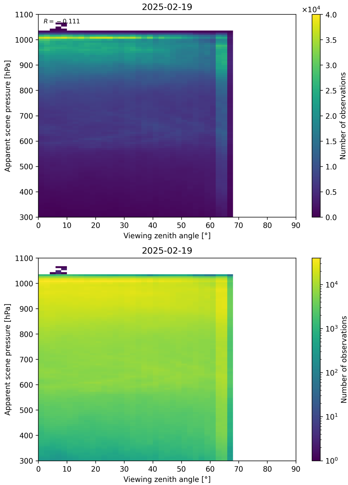
Figure 118: Scatter density plot of “Viewing zenith angle” against “Apparent scene pressure” for 2025-02-19 to 2025-02-20.
