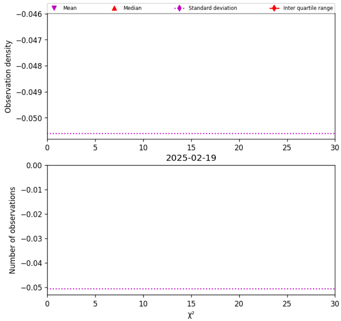
Figure 38: Histogram of " \chi^2 " for 2025-02-19 to 2025-02-20
