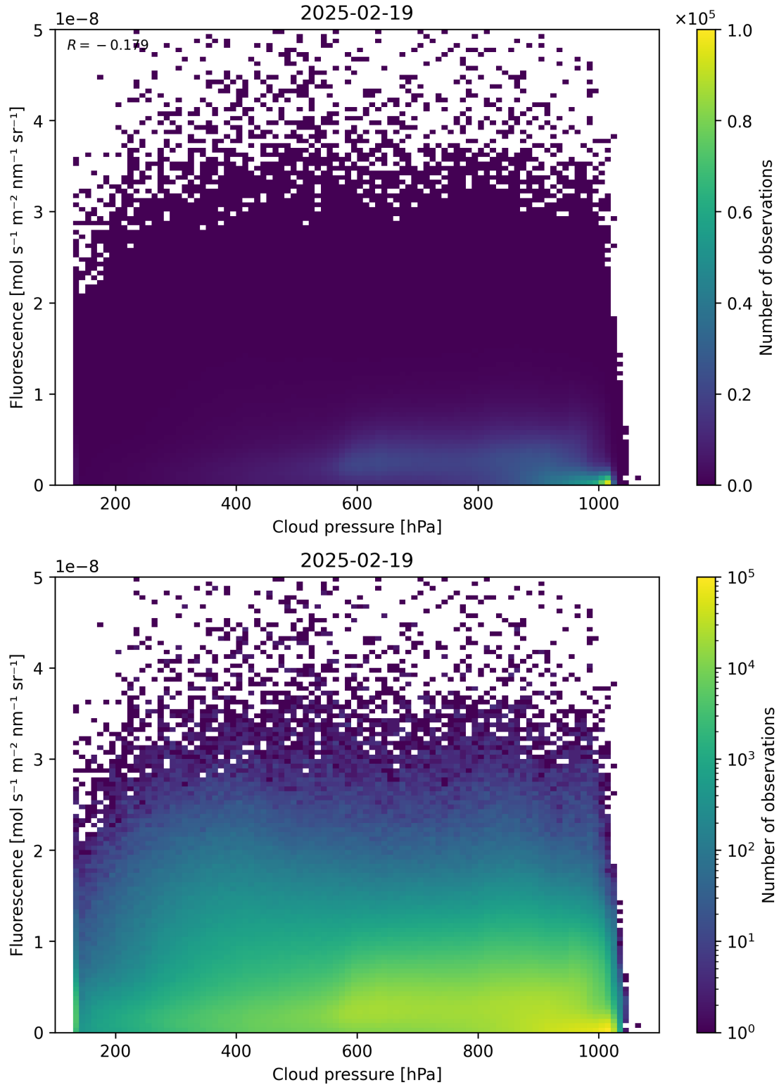
Figure 80: Scatter density plot of “Cloud pressure” against “Fluorescence” for 2025-02-19 to 2025-02-20.
