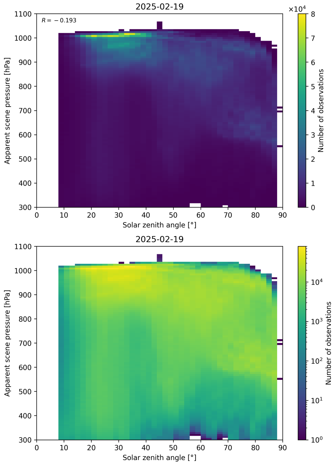
Figure 108: Scatter density plot of “Solar zenith angle” against “Apparent scene pressure” for 2025-02-19 to 2025-02-20.
