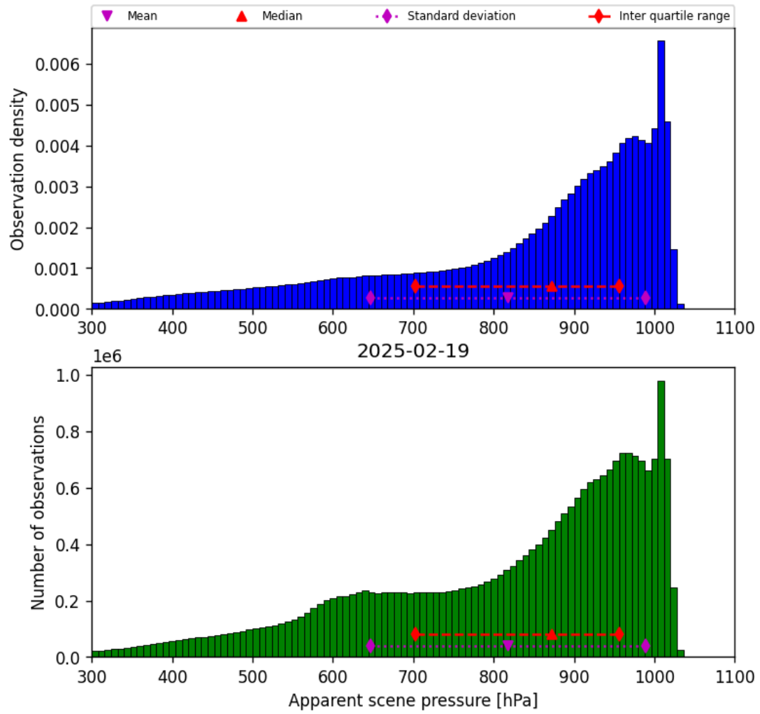
Figure 36: Histogram of “Apparent scene pressure” for 2025-02-19 to 2025-02-20
