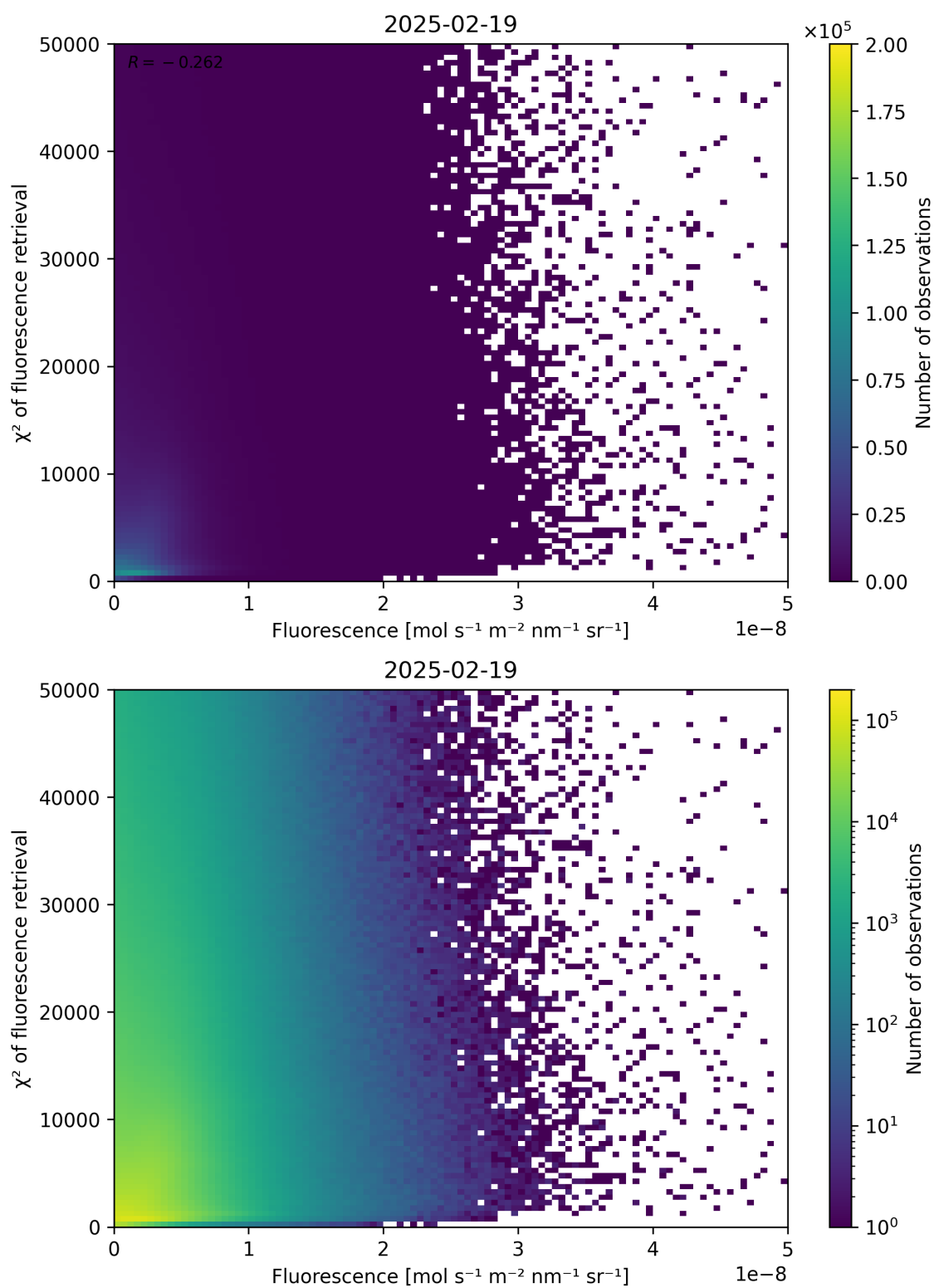
Figure 85: Scatter density plot of “Fluorescence” against “ \chi^2 of fluorescence retrieval” for 2025-02-19 to 2025-02-20.
