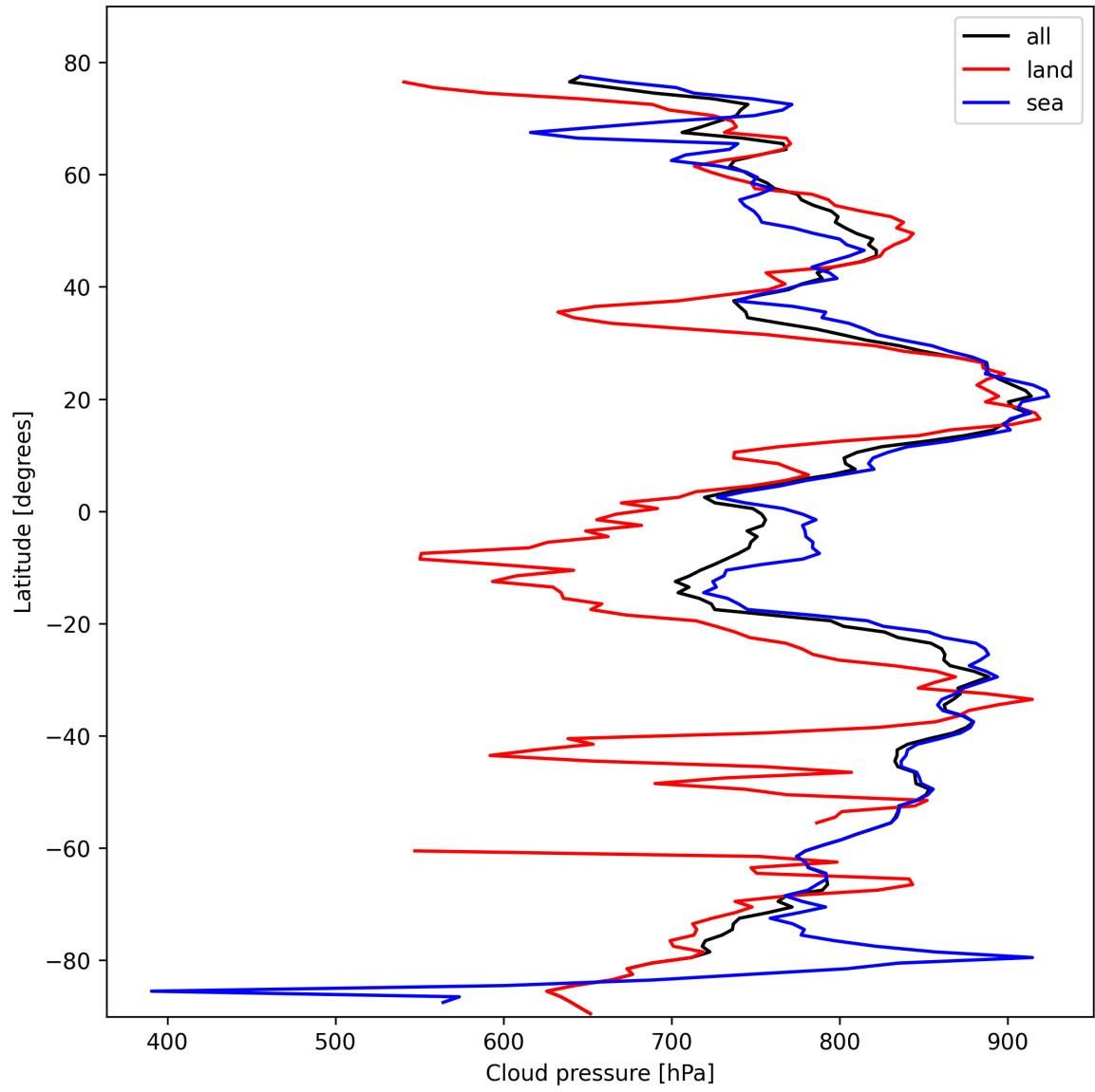
Figure 13: Zonal average of “Cloud pressure” for 2025-02-19 to 2025-02-20.
