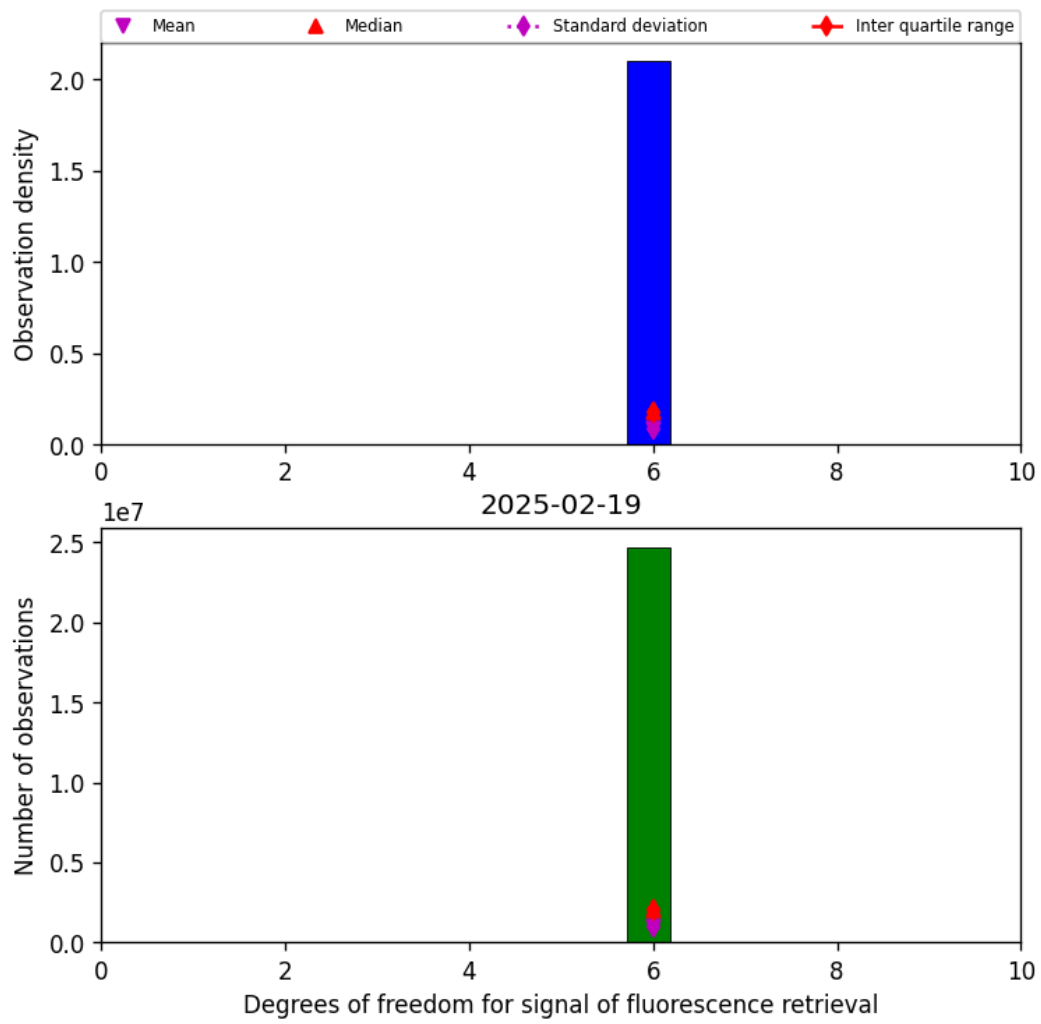
Figure 43: Histogram of “Degrees of freedom for signal of fluorescence retrieval” for 2025-02-19 to 2025-02-20
