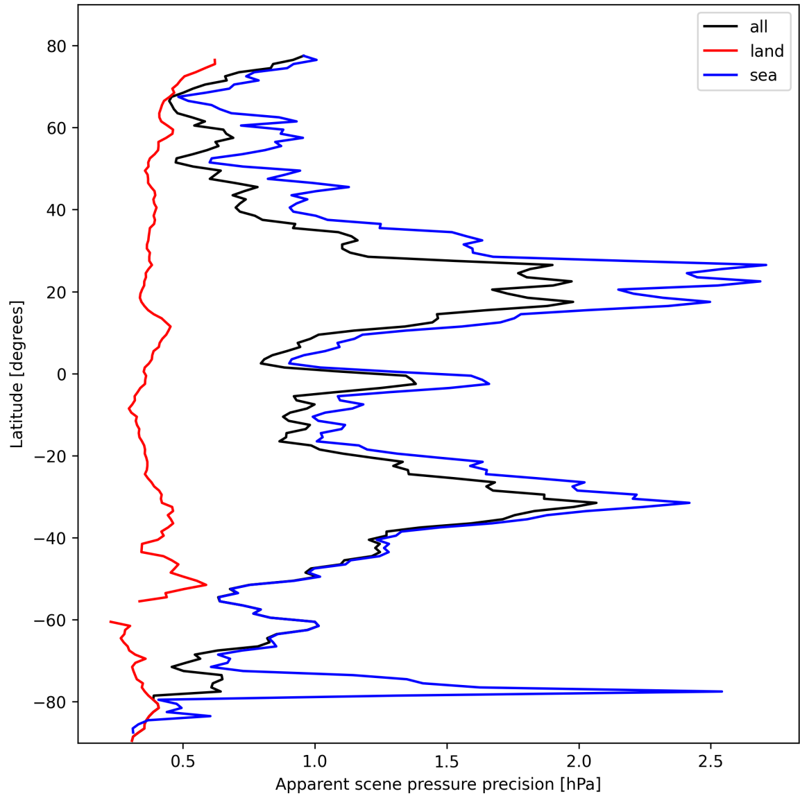
Figure 20: Zonal average of “Apparent scene pressure precision” for 2025-02-19 to 2025-02-20.
