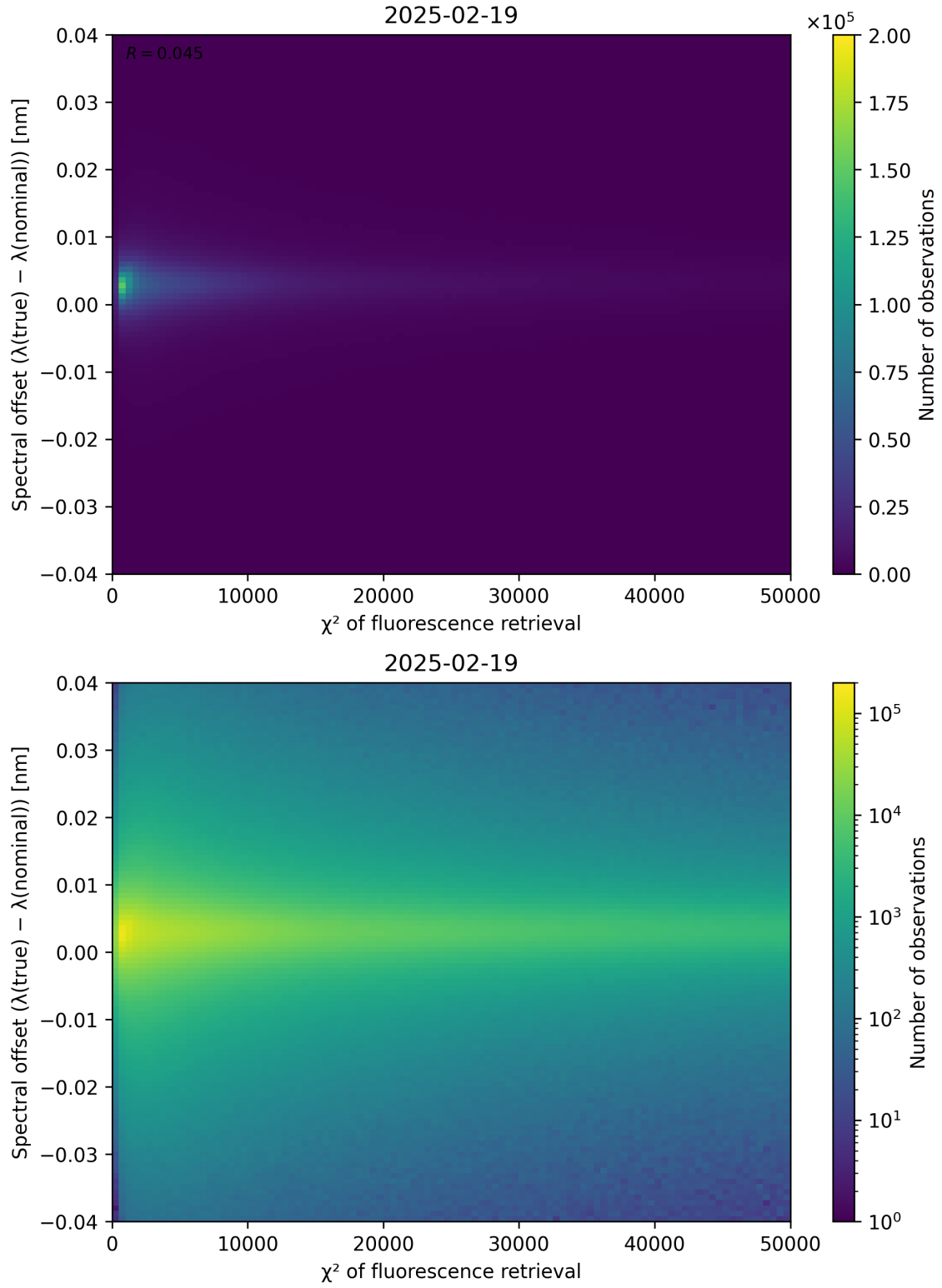
Figure 69: Scatter density plot of “ \chi^2 of fluorescence retrieval” against “Spectral offset ( \lambda_{\text{true}} - \lambda_{\text{nominal}} )” for 2025-02-19 to 2025-02-20.
