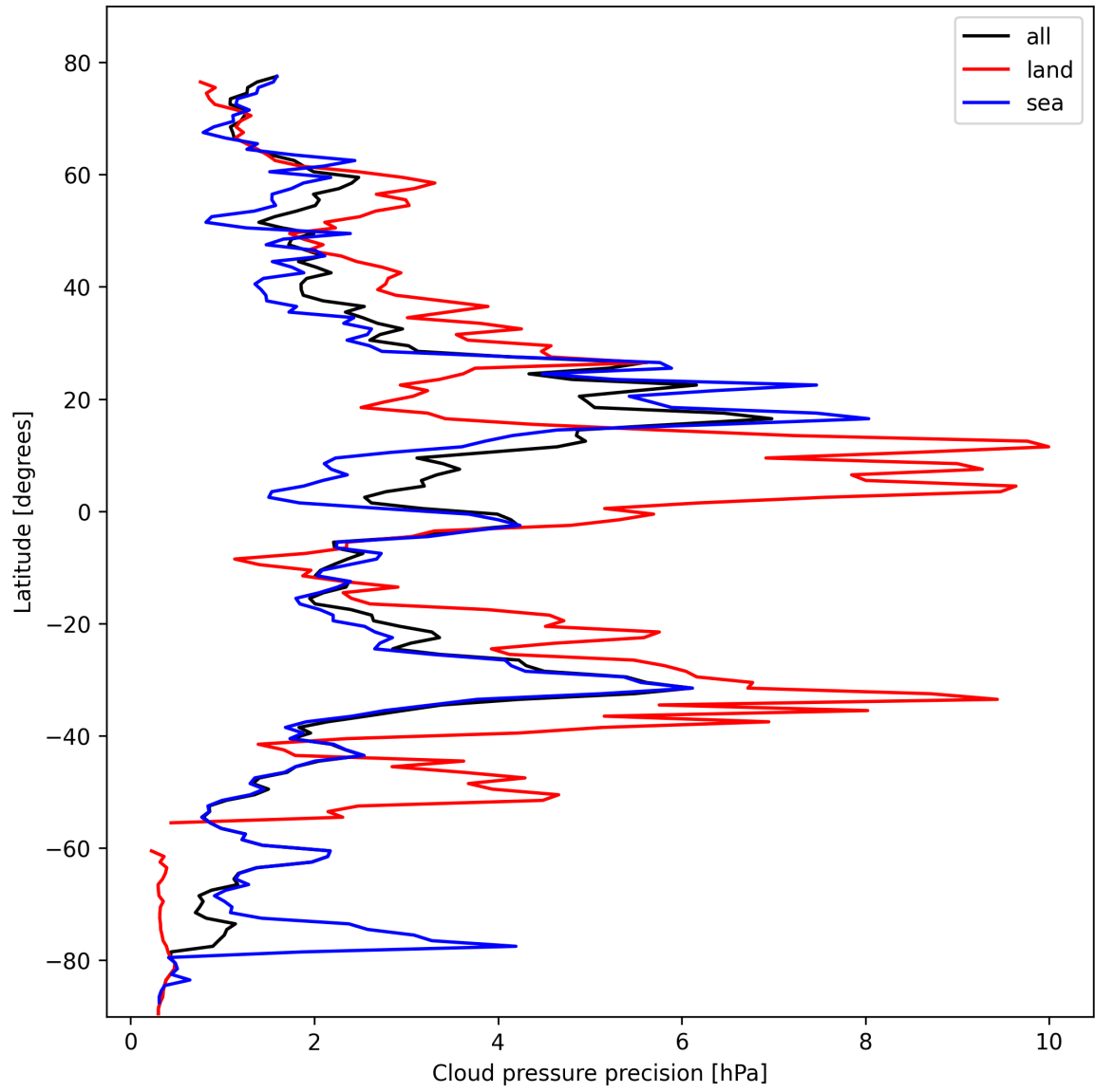
Figure 14: Zonal average of “Cloud pressure precision” for 2025-02-19 to 2025-02-20.
