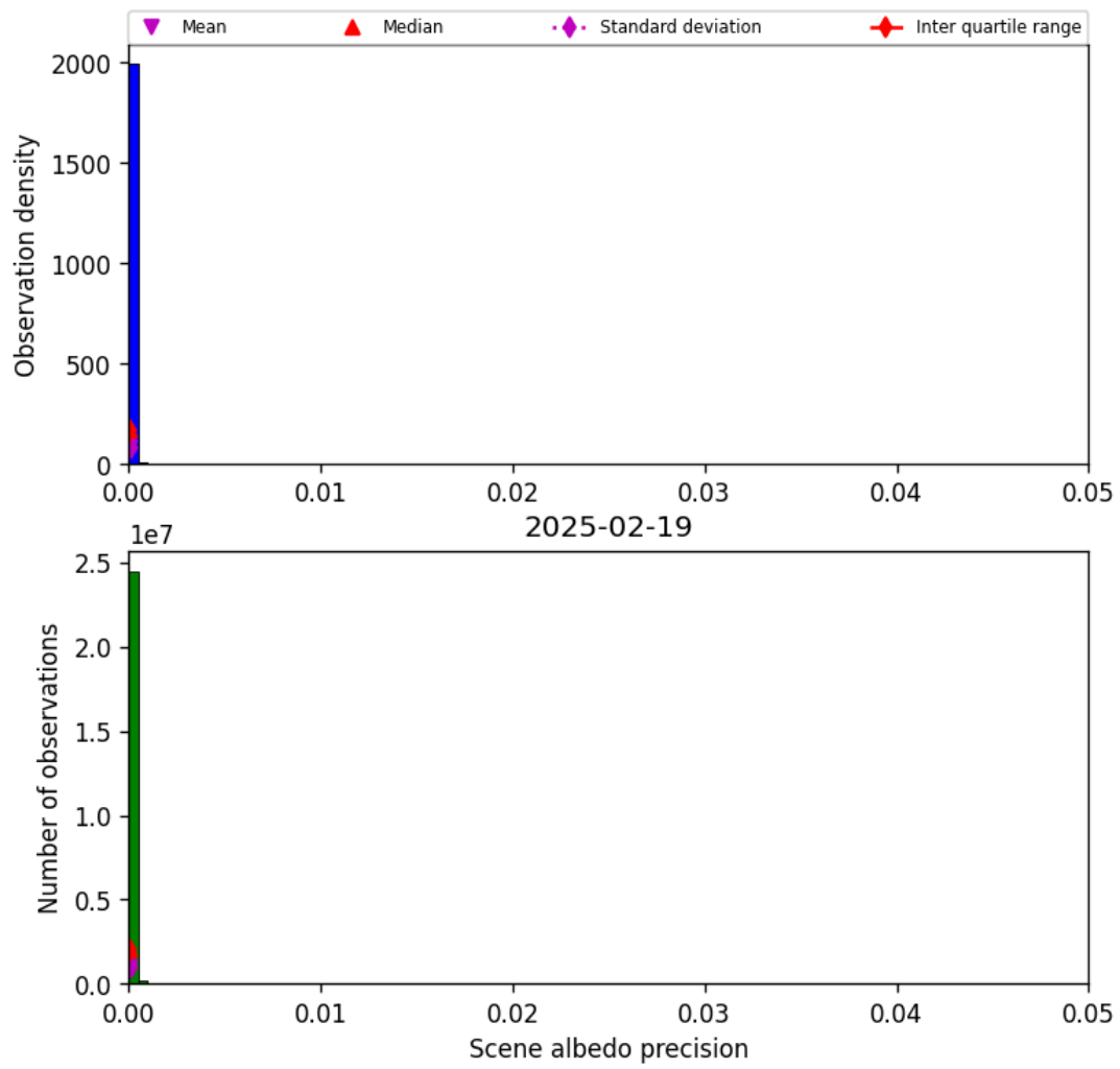
Figure 35: Histogram of “Scene albedo precision” for 2025-02-19 to 2025-02-20
