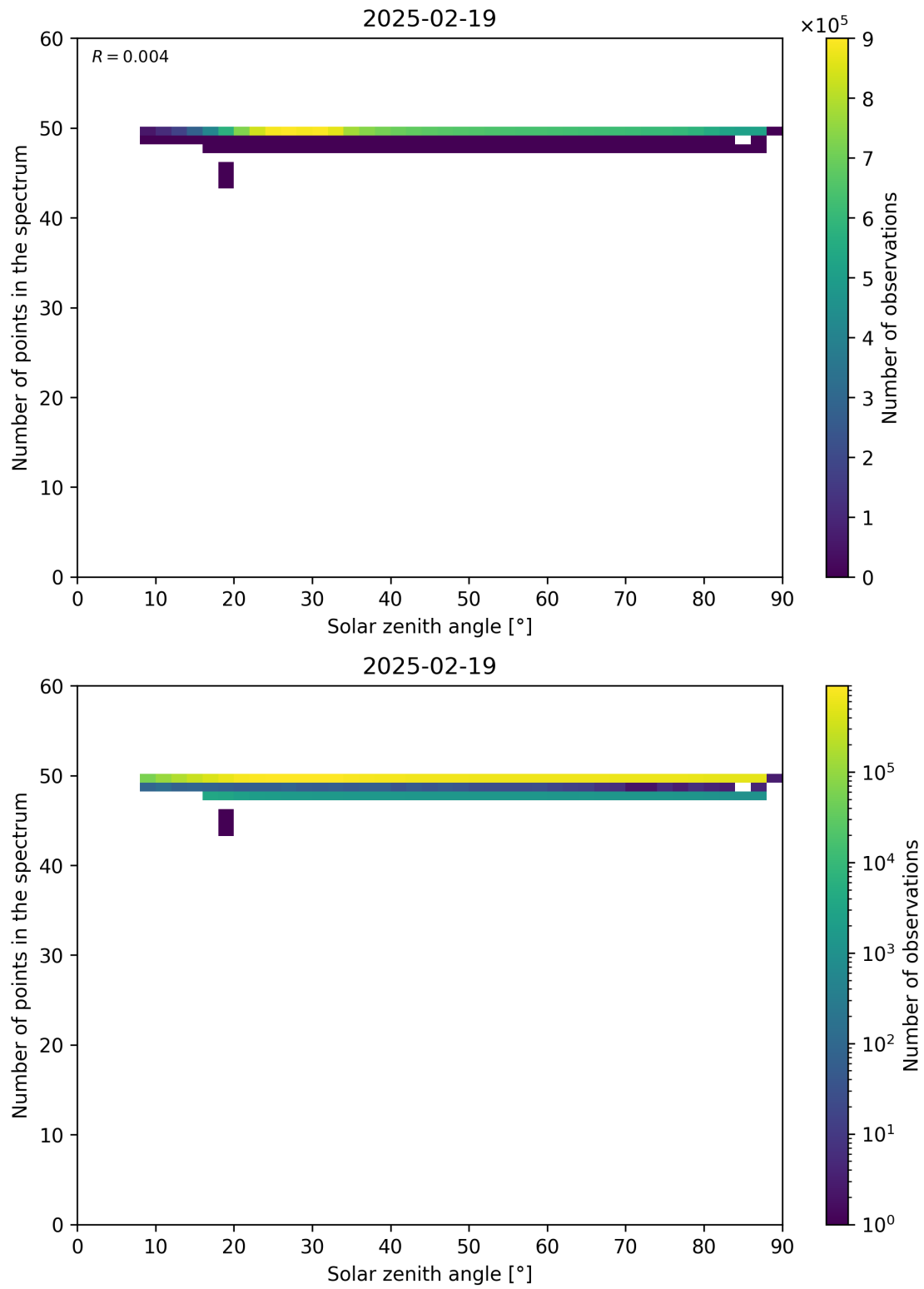
Figure 115: Scatter density plot of “Solar zenith angle” against “Number of points in the spectrum” for 2025-02-19 to 2025-02-20.
