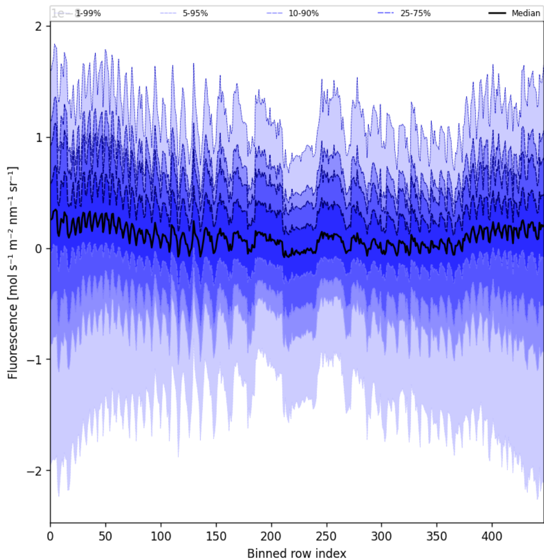
Figure 57: Along track statistics of “Fluorescence” for 2025-02-19 to 2025-02-20
