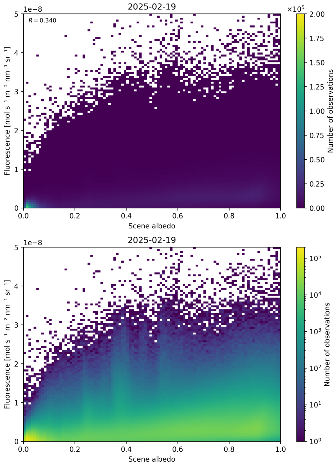
Figure 104: Scatter density plot of “Scene albedo” against “Fluorescence” for 2025-02-19 to 2025-02-20.
