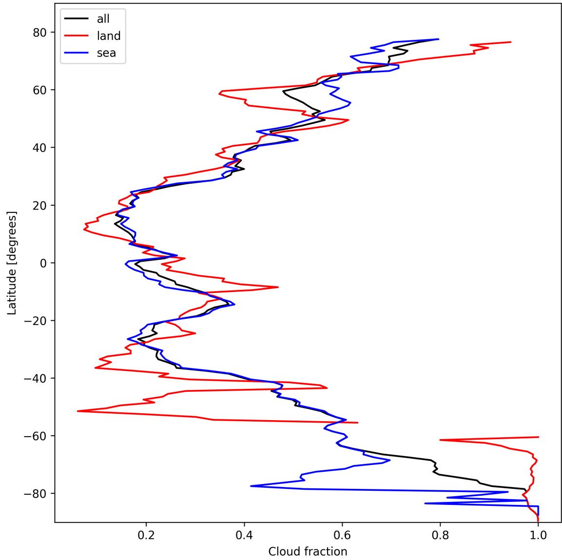
Figure 15: Zonal average of “Cloud fraction” for 2025-02-19 to 2025-02-20.
