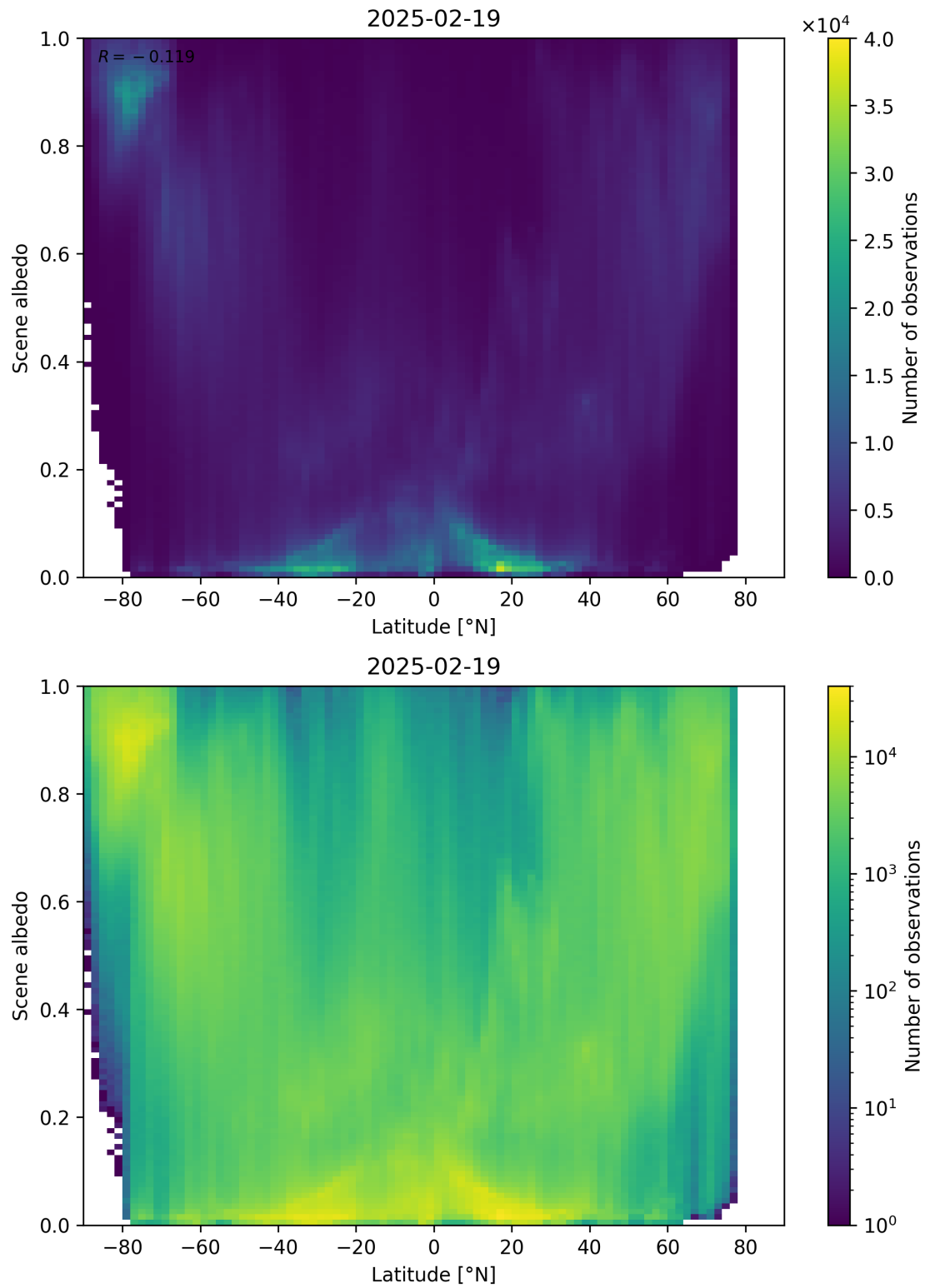
Figure 95: Scatter density plot of “Latitude” against “Scene albedo” for 2025-02-19 to 2025-02-20.
