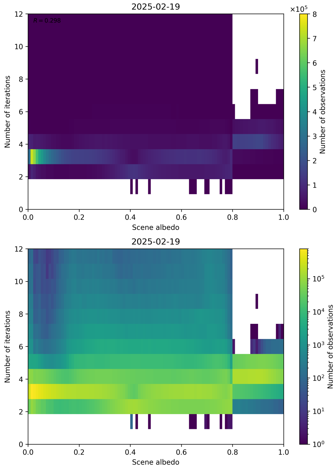
Figure 105: Scatter density plot of “Scene albedo” against “Number of iterations” for 2025-02-19 to 2025-02-20.
