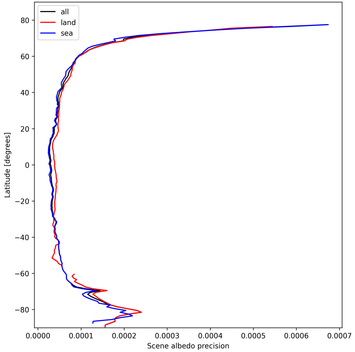
Figure 18: Zonal average of “Scene albedo precision” for 2025-02-19 to 2025-02-20.
