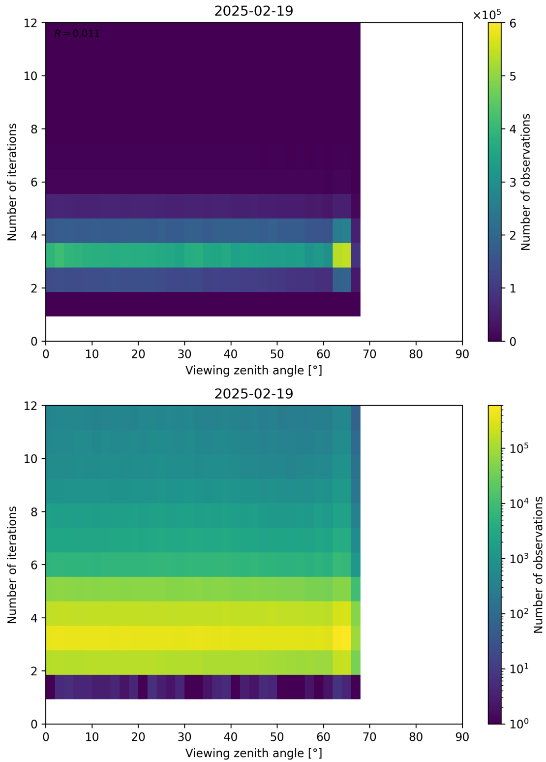
Figure 124: Scatter density plot of “Viewing zenith angle” against “Number of iterations” for 2025-02-19 to 2025-02-20.
