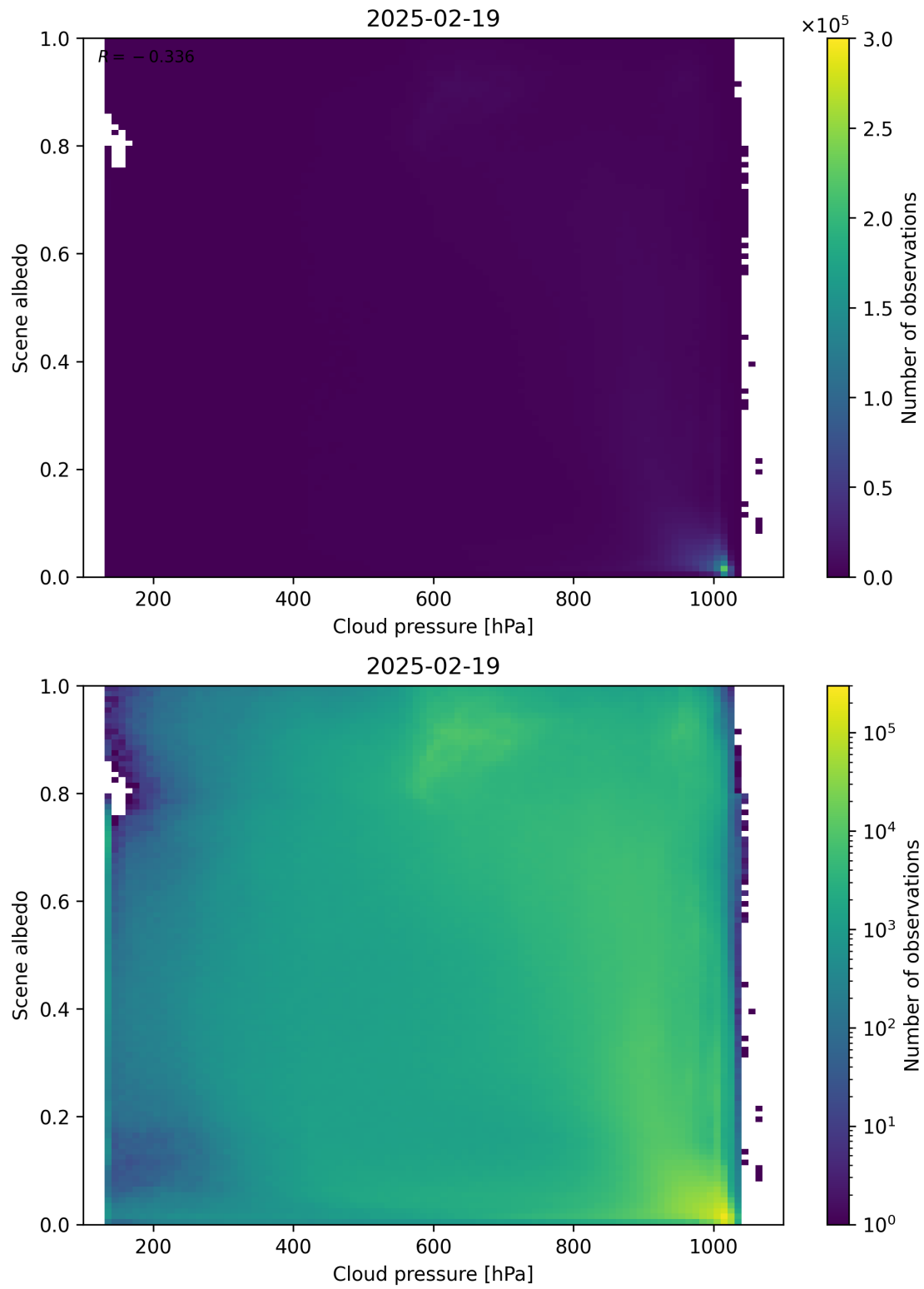
Figure 83: Scatter density plot of “Cloud pressure” against “Scene albedo” for 2025-02-19 to 2025-02-20.
