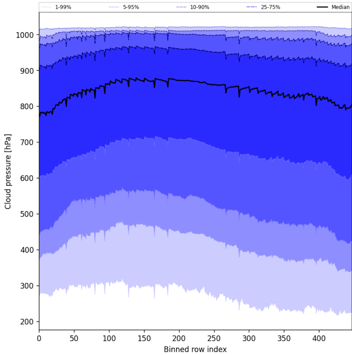
Figure 47: Along track statistics of “Cloud pressure” for 2025-02-19 to 2025-02-20
