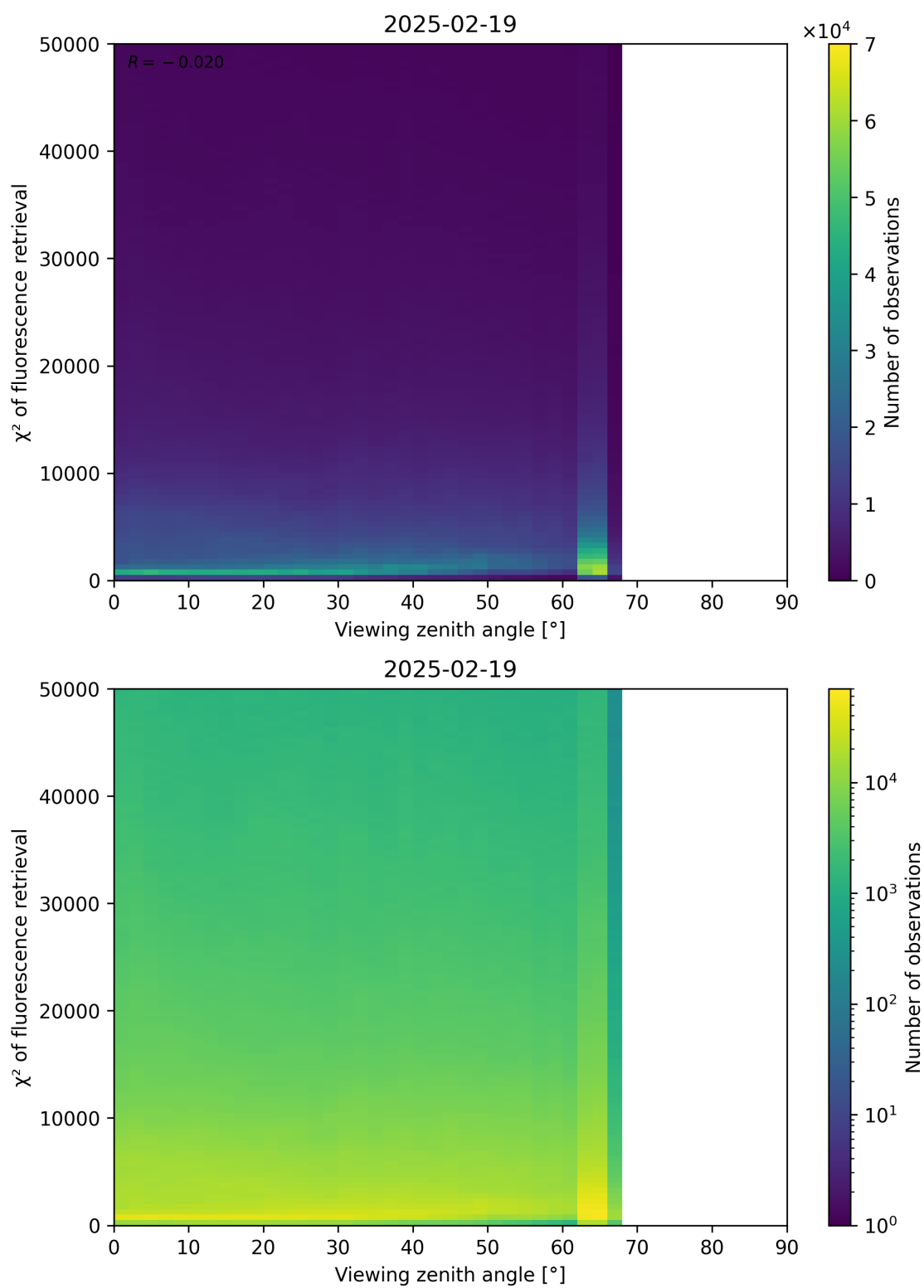
Figure 119: Scatter density plot of “Viewing zenith angle” against “ \chi^2 of fluorescence retrieval” for 2025-02-19 to 2025-02-20.
