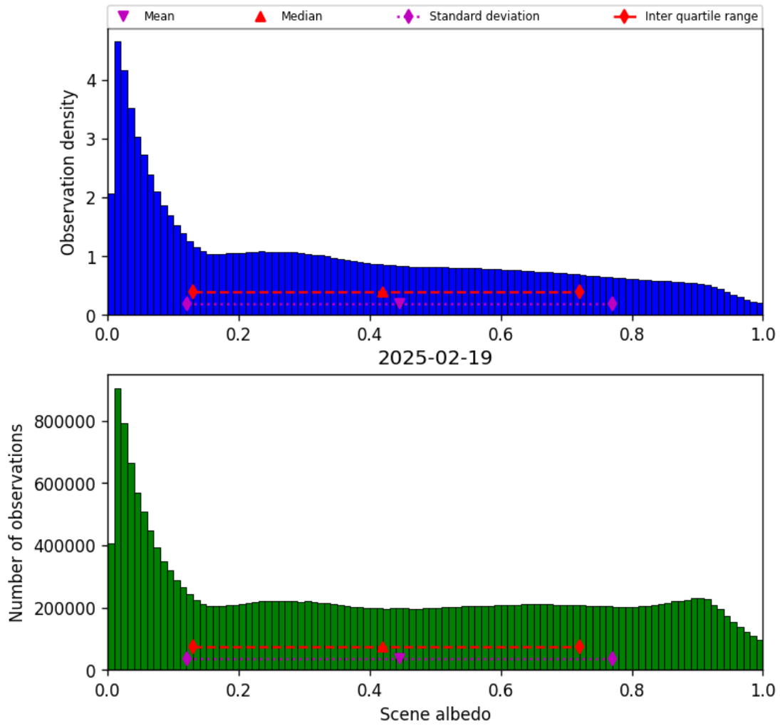
Figure 34: Histogram of “Scene albedo” for 2025-02-19 to 2025-02-20
