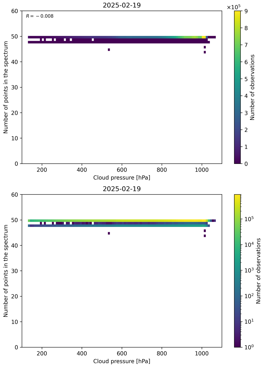
Figure 82: Scatter density plot of “Cloud pressure” against “Number of points in the spectrum” for 2025-02-19 to 2025-02-20.
