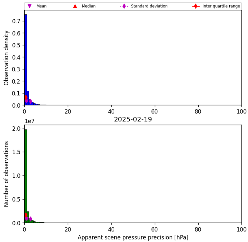
Figure 37: Histogram of “Apparent scene pressure precision” for 2025-02-19 to 2025-02-20
