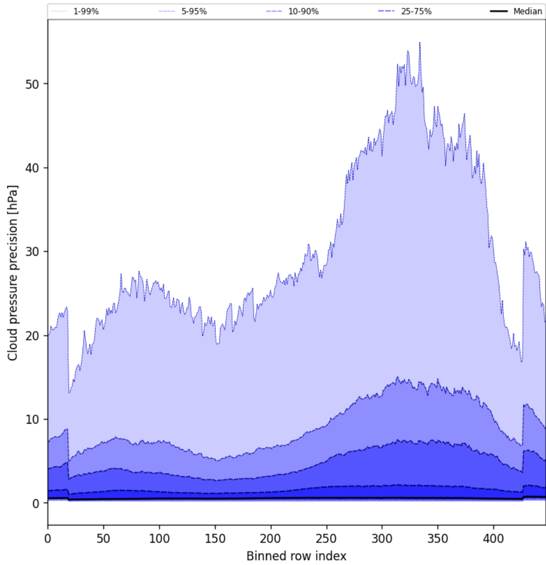
Figure 48: Along track statistics of “Cloud pressure precision” for 2025-02-19 to 2025-02-20
