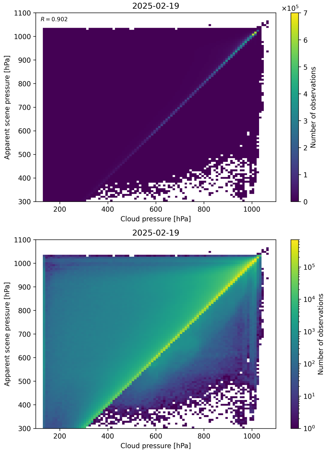
Figure 77: Scatter density plot of “Cloud pressure” against “Apparent scene pressure” for 2025-02-19 to 2025-02-20.
