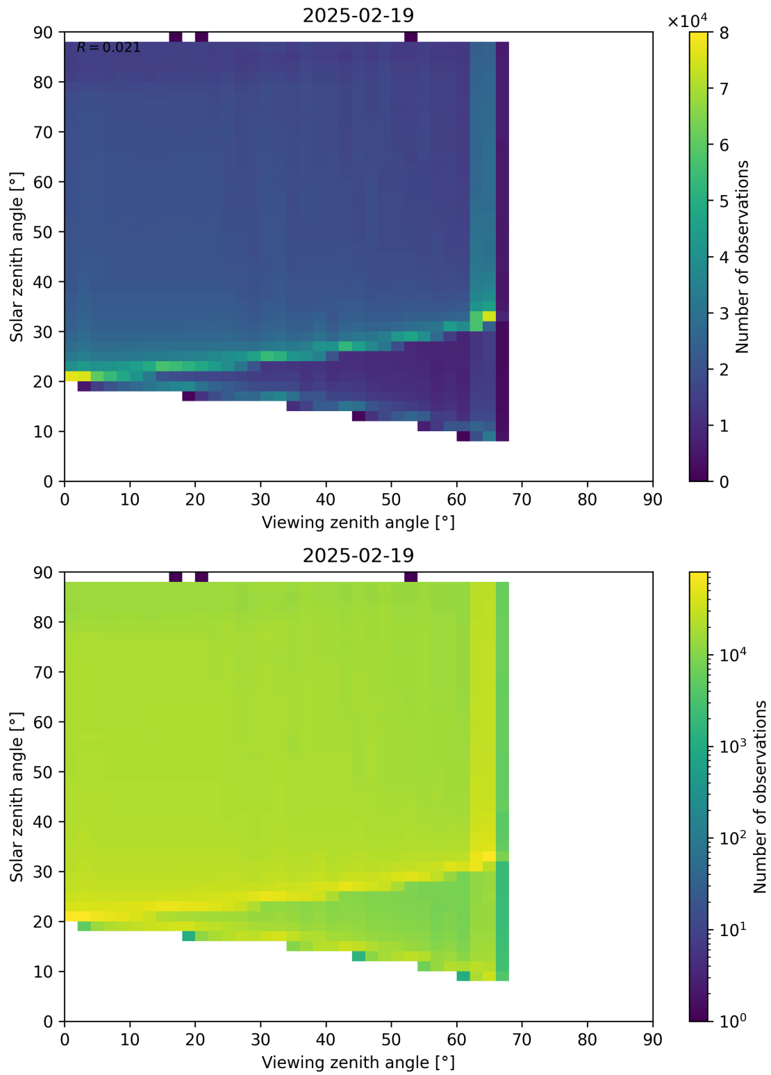
Figure 127: Scatter density plot of “Viewing zenith angle” against “Solar zenith angle” for 2025-02-19 to 2025-02-20.
