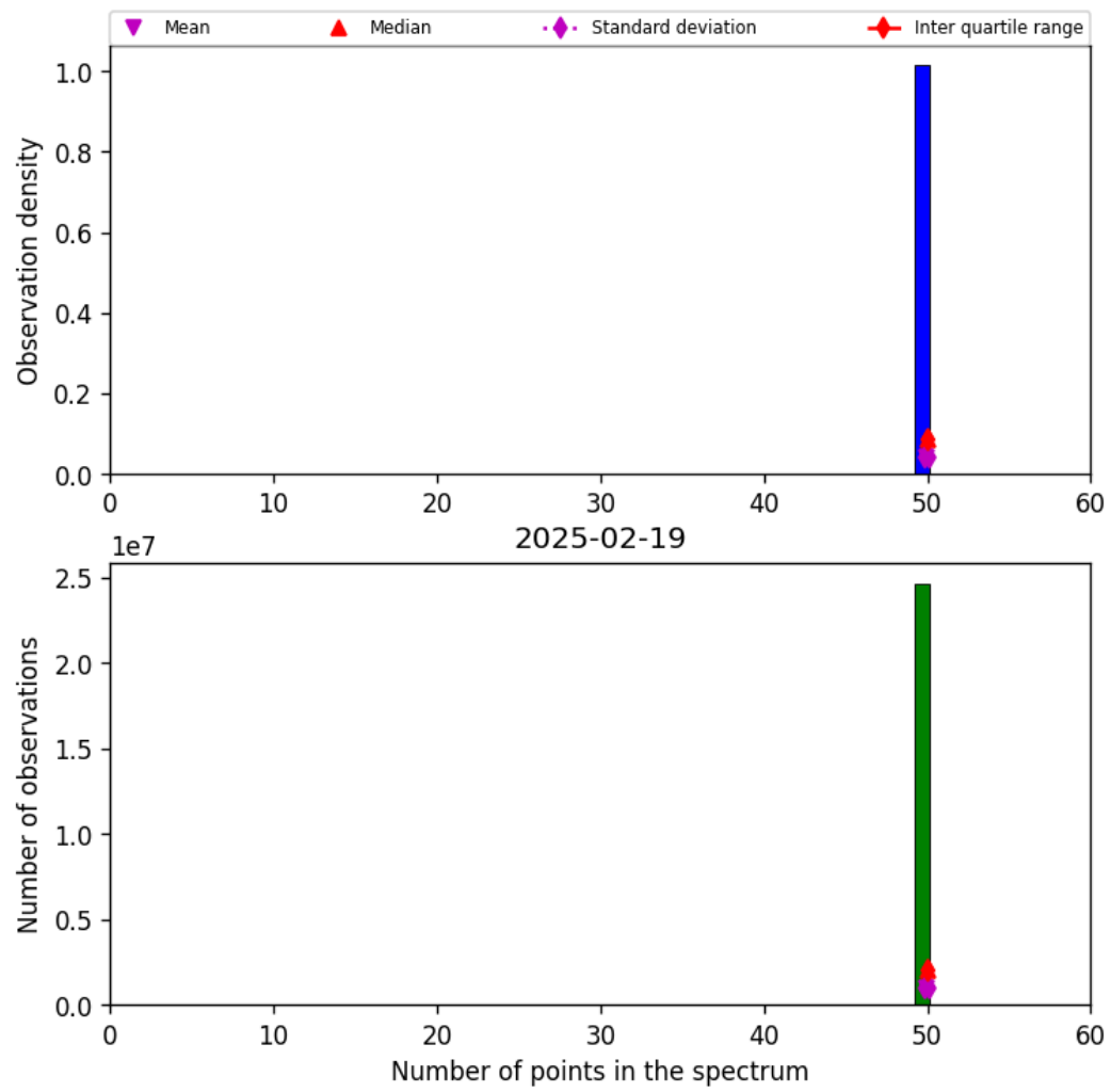
Figure 44: Histogram of “Number of points in the spectrum” for 2025-02-19 to 2025-02-20
