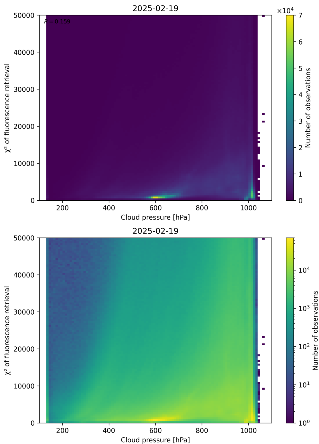
Figure 78: Scatter density plot of “Cloud pressure” against “ \chi^2 of fluorescence retrieval” for 2025-02-19 to 2025-02-20.
