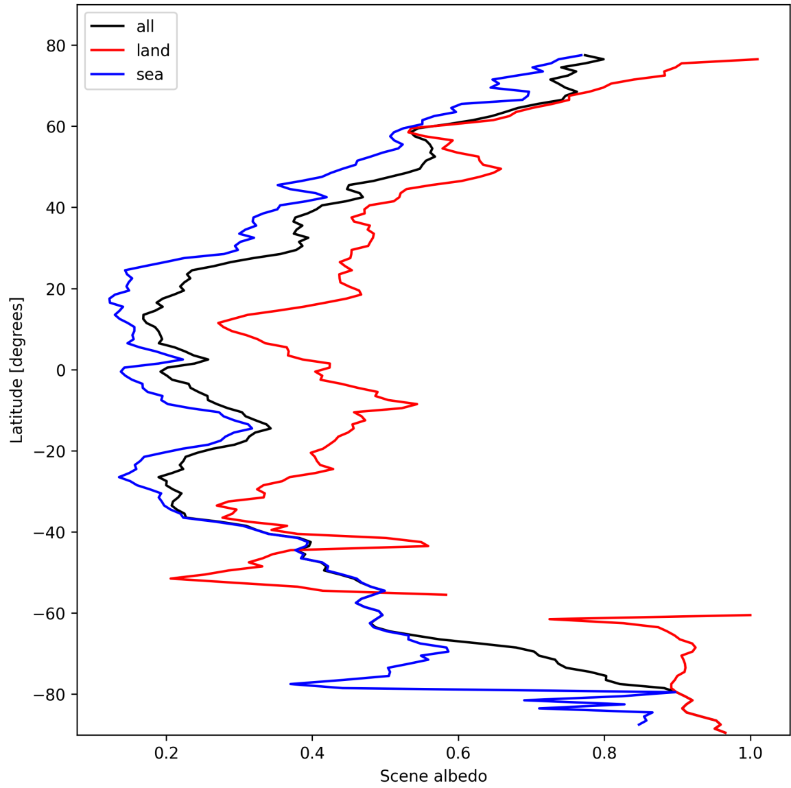
Figure 17: Zonal average of “Scene albedo” for 2025-02-19 to 2025-02-20.
