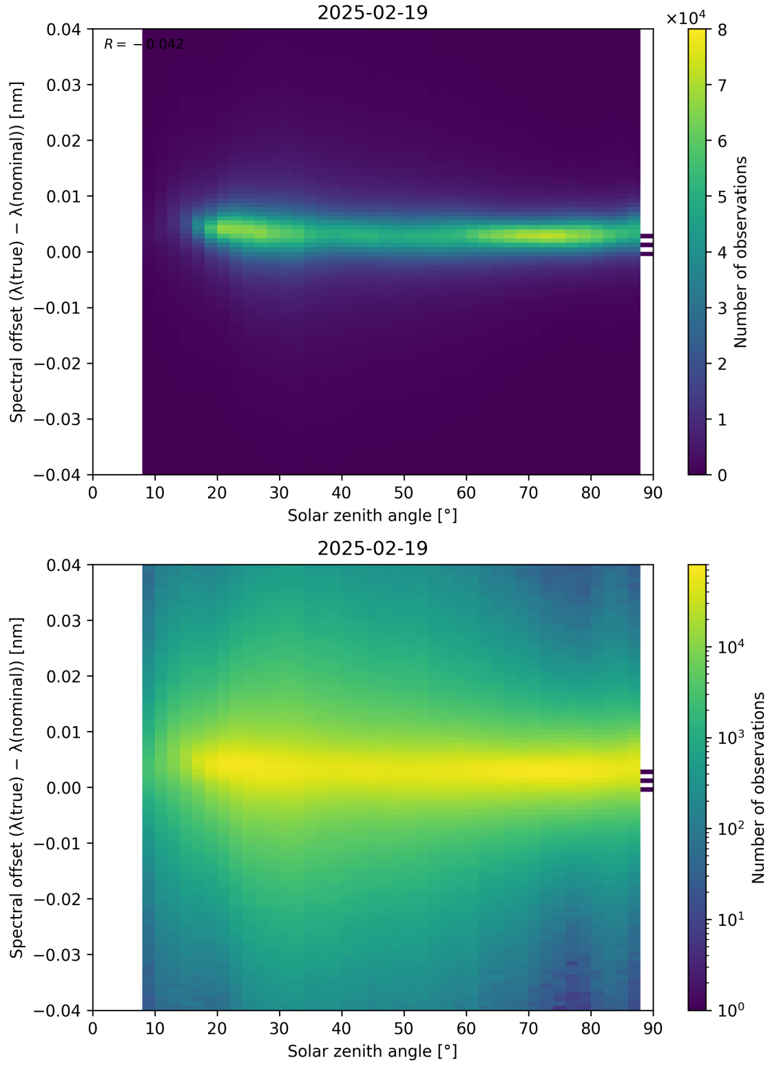
Figure 117: Scatter density plot of “Solar zenith angle” against “Spectral offset ( \lambda_{\text{true}} - \lambda_{\text{nominal}} )” for 2025-02-19 to 2025-02-20.
