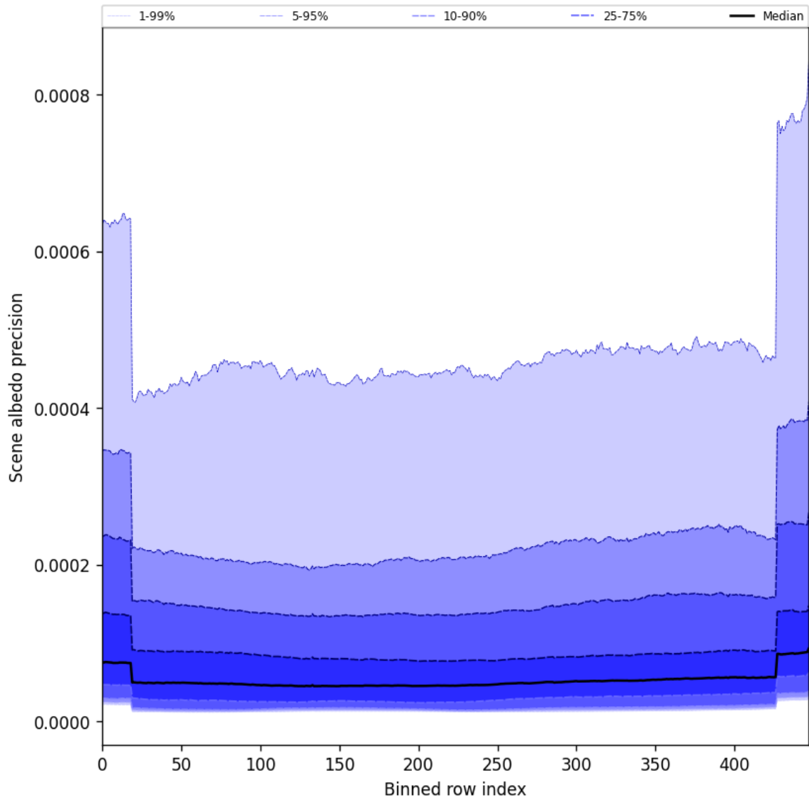
Figure 52: Along track statistics of “Scene albedo precision” for 2025-02-19 to 2025-02-20
