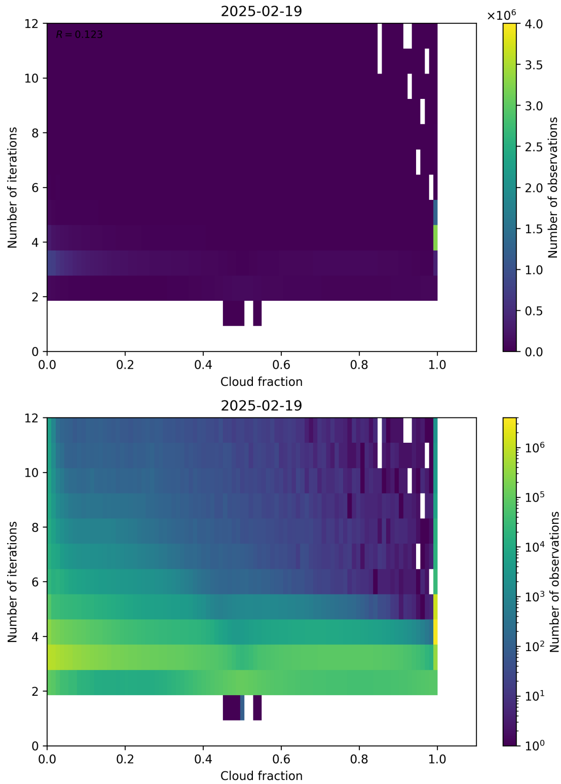
Figure 73: Scatter density plot of “Cloud fraction” against “Number of iterations” for 2025-02-19 to 2025-02-20.
