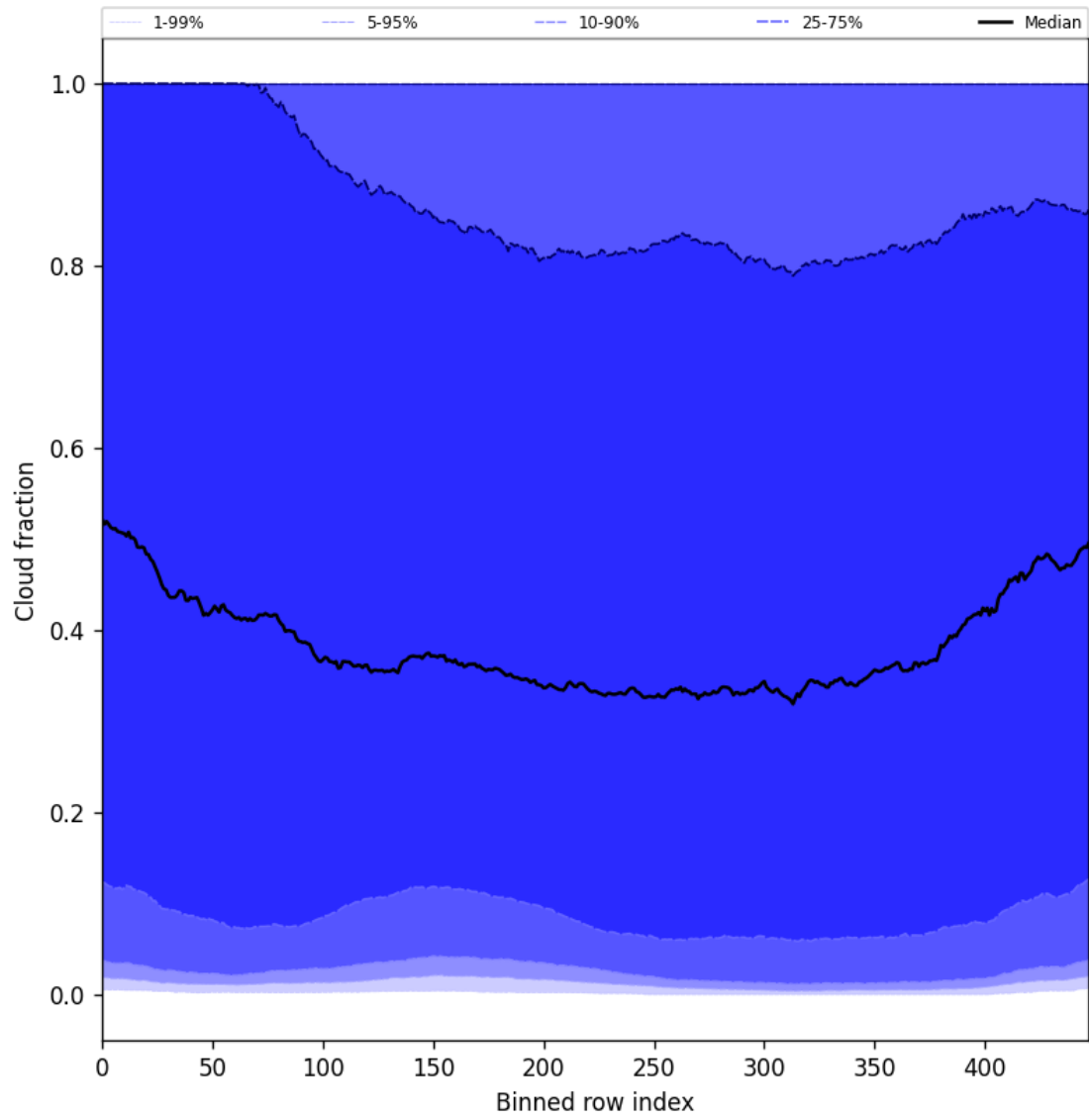
Figure 49: Along track statistics of “Cloud fraction” for 2025-02-19 to 2025-02-20
