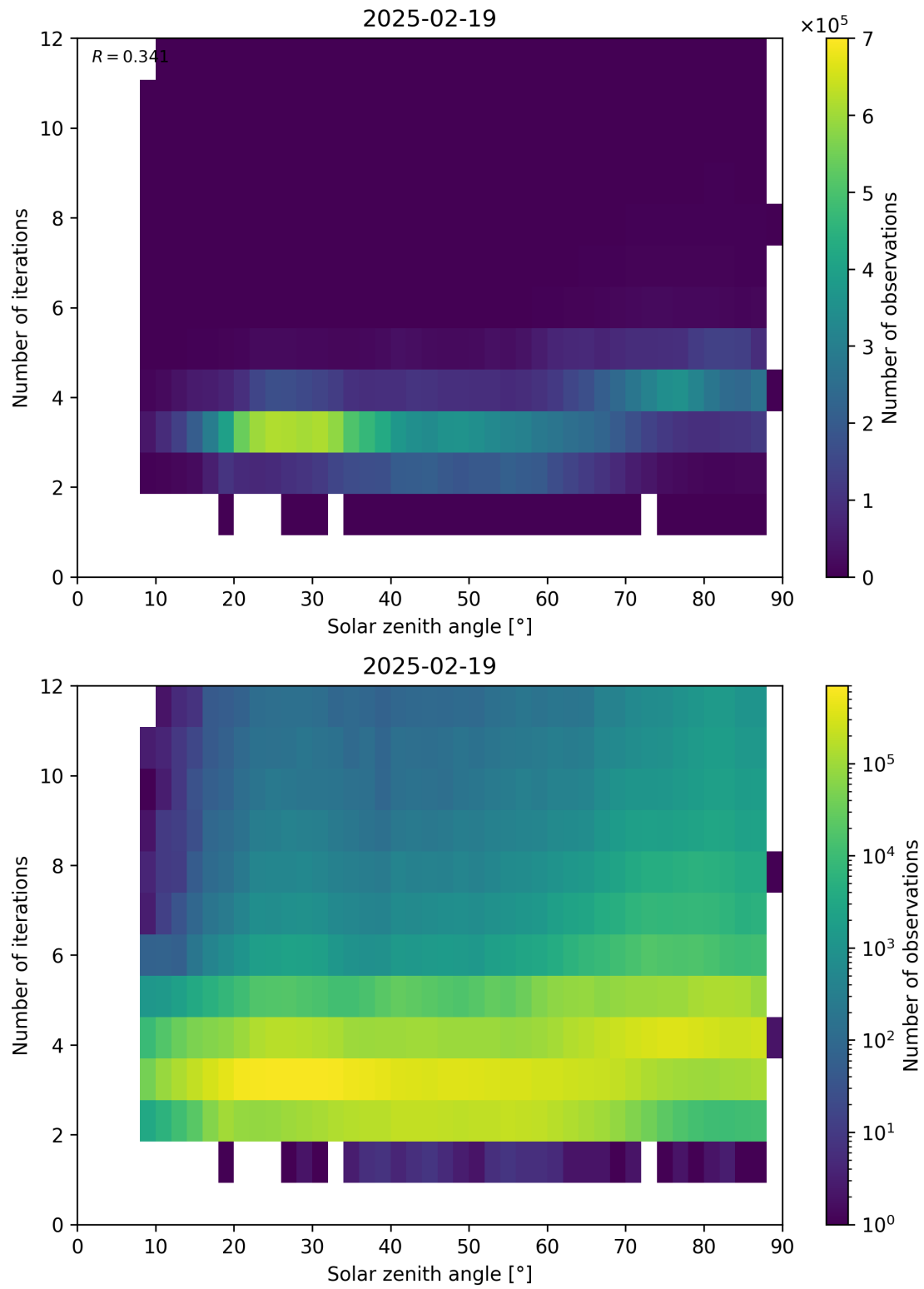
Figure 114: Scatter density plot of “Solar zenith angle” against “Number of iterations” for 2025-02-19 to 2025-02-20.
