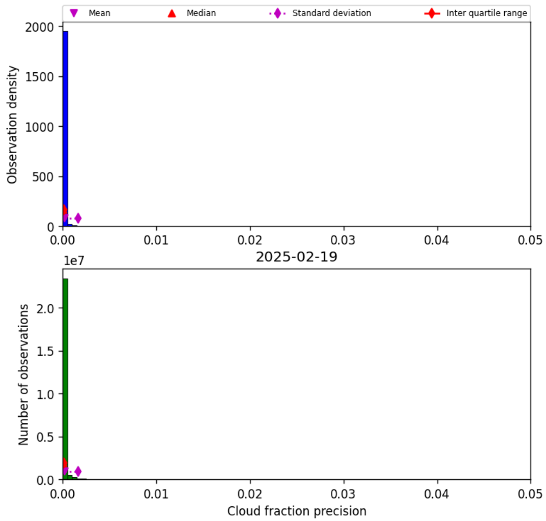
Figure 33: Histogram of “Cloud fraction precision” for 2025-02-19 to 2025-02-20
