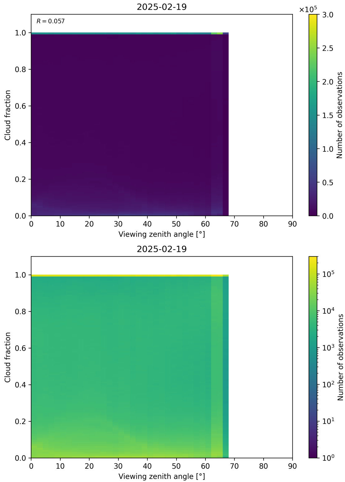
Figure 120: Scatter density plot of “Viewing zenith angle” against “Cloud fraction” for 2025-02-19 to 2025-02-20.
