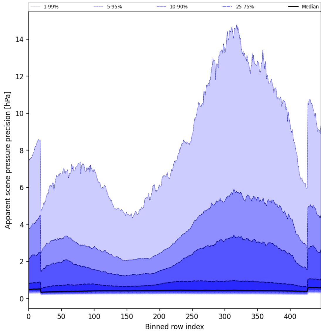
Figure 54: Along track statistics of “Apparent scene pressure precision” for 2025-02-19 to 2025-02-20
