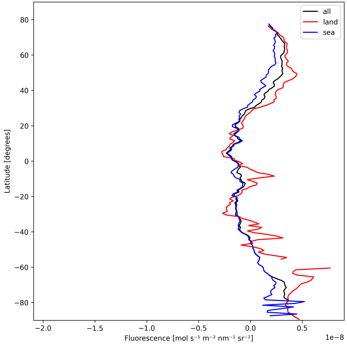
Figure 23: Zonal average of “Fluorescence” for 2025-02-19 to 2025-02-20.
