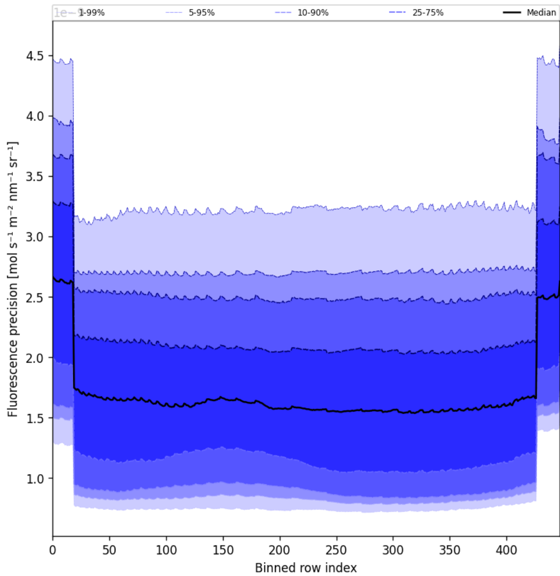
Figure 58: Along track statistics of “Fluorescence precision” for 2025-02-19 to 2025-02-20
