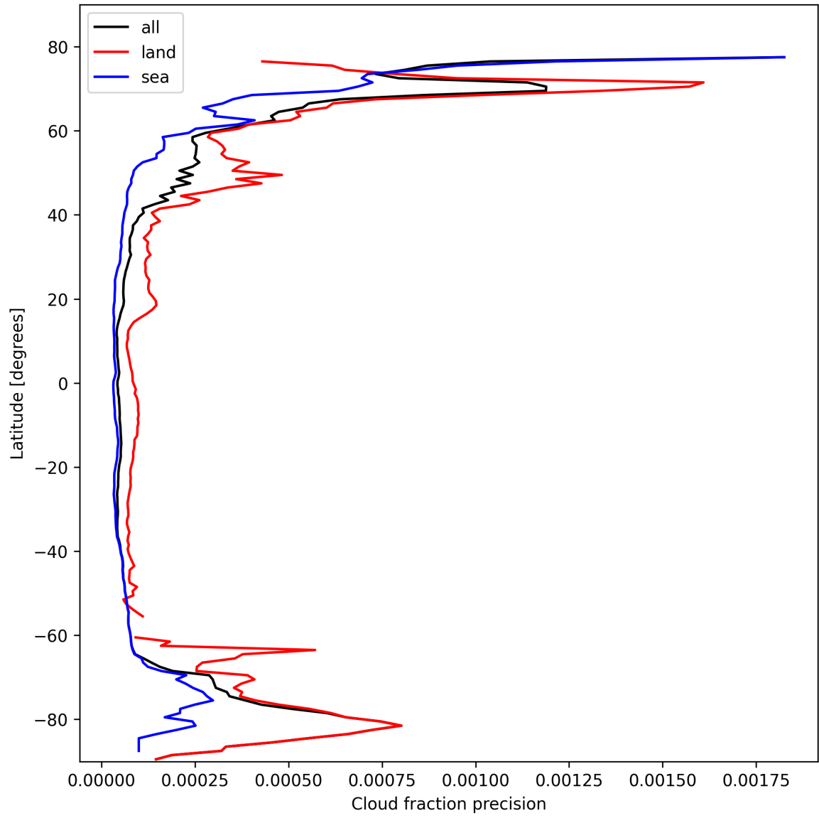
Figure 16: Zonal average of “Cloud fraction precision” for 2025-02-19 to 2025-02-20.
