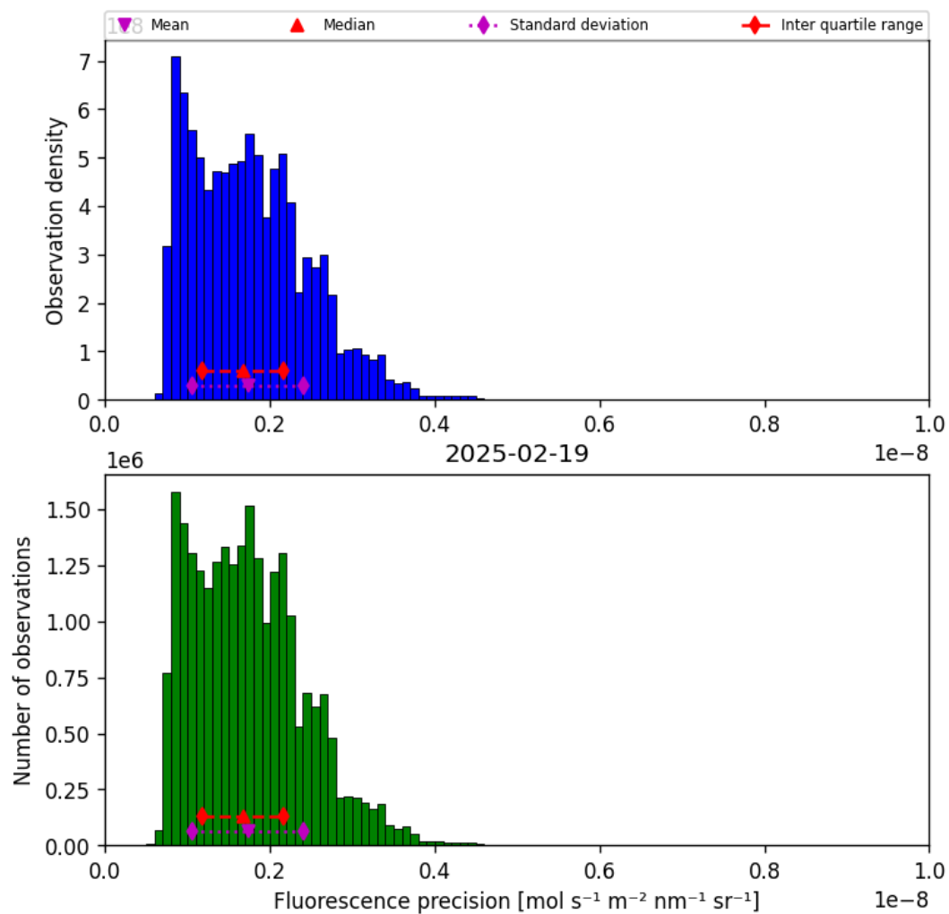
Figure 41: Histogram of “Fluorescence precision” for 2025-02-19 to 2025-02-20
