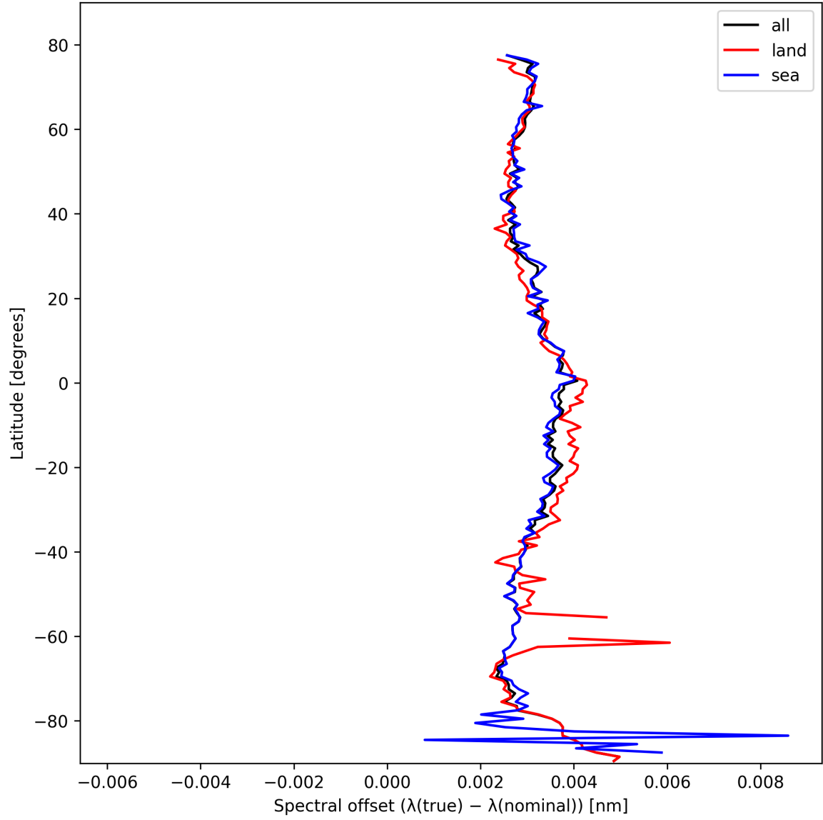
Figure 28: Zonal average of “Spectral offset ( \lambda_{\text{true}} - \lambda_{\text{nominal}} )” for 2025-02-19 to 2025-02-20.
