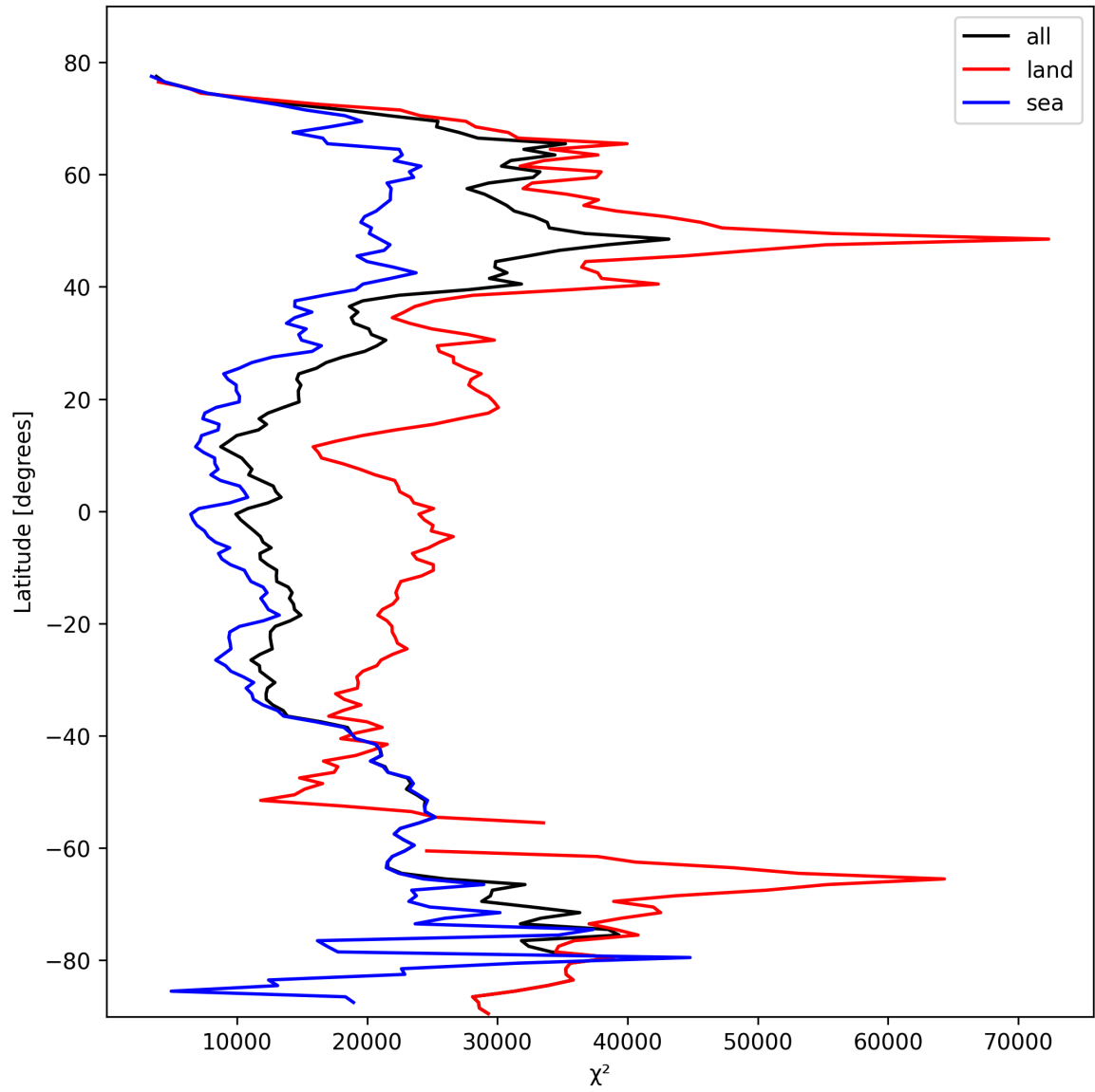
Figure 21: Zonal average of “ \chi^2 ” for 2025-02-19 to 2025-02-20.
