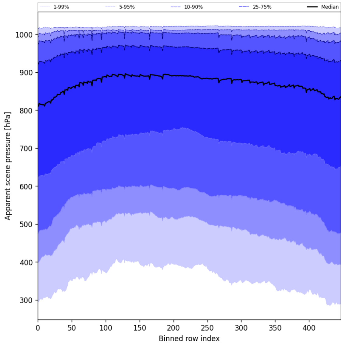
Figure 53: Along track statistics of “Apparent scene pressure” for 2025-02-19 to 2025-02-20
