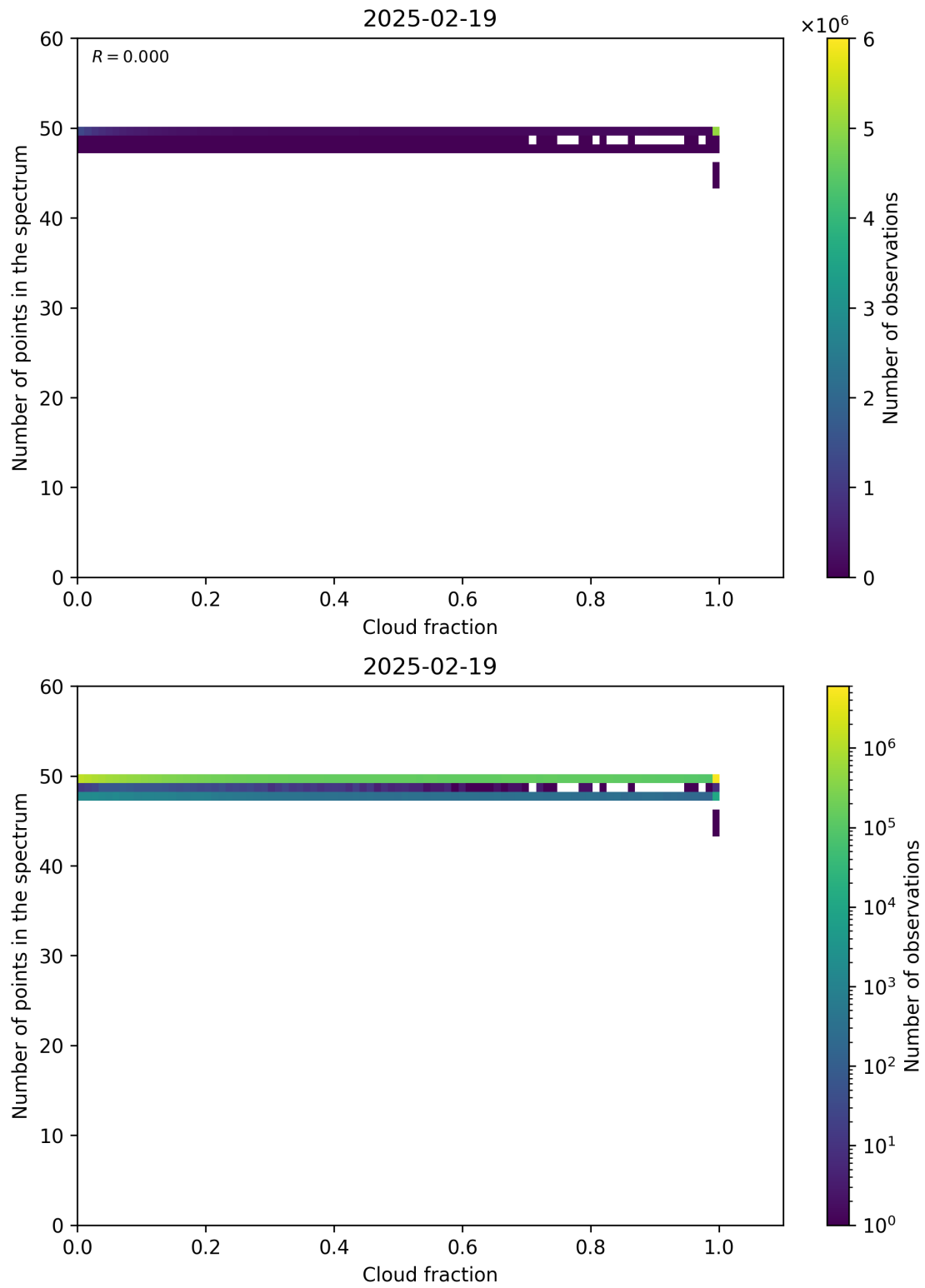
Figure 74: Scatter density plot of “Cloud fraction” against “Number of points in the spectrum” for 2025-02-19 to 2025-02-20.
