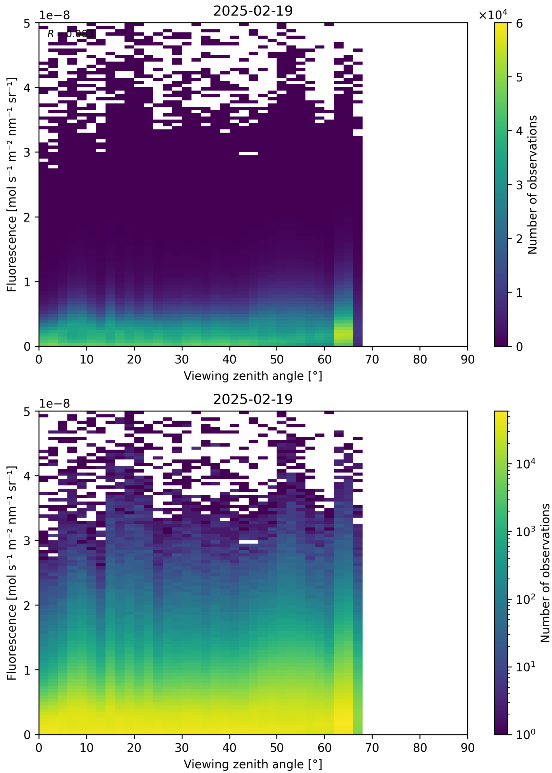
Figure 122: Scatter density plot of “Viewing zenith angle” against “Fluorescence” for 2025-02-19 to 2025-02-20.
