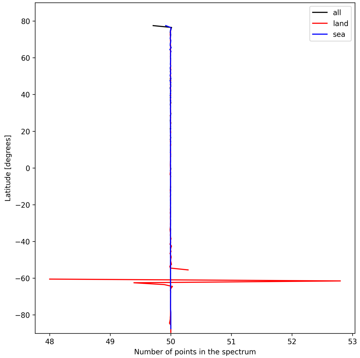
Figure 27: Zonal average of “Number of points in the spectrum” for 2025-02-19 to 2025-02-20.
