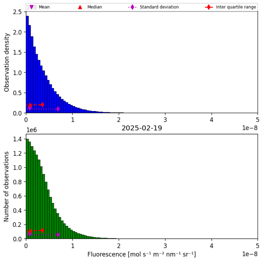
Figure 40: Histogram of “Fluorescence” for 2025-02-19 to 2025-02-20
