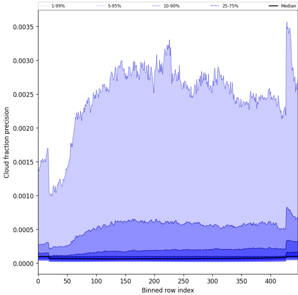
Figure 50: Along track statistics of “Cloud fraction precision” for 2025-02-19 to 2025-02-20
