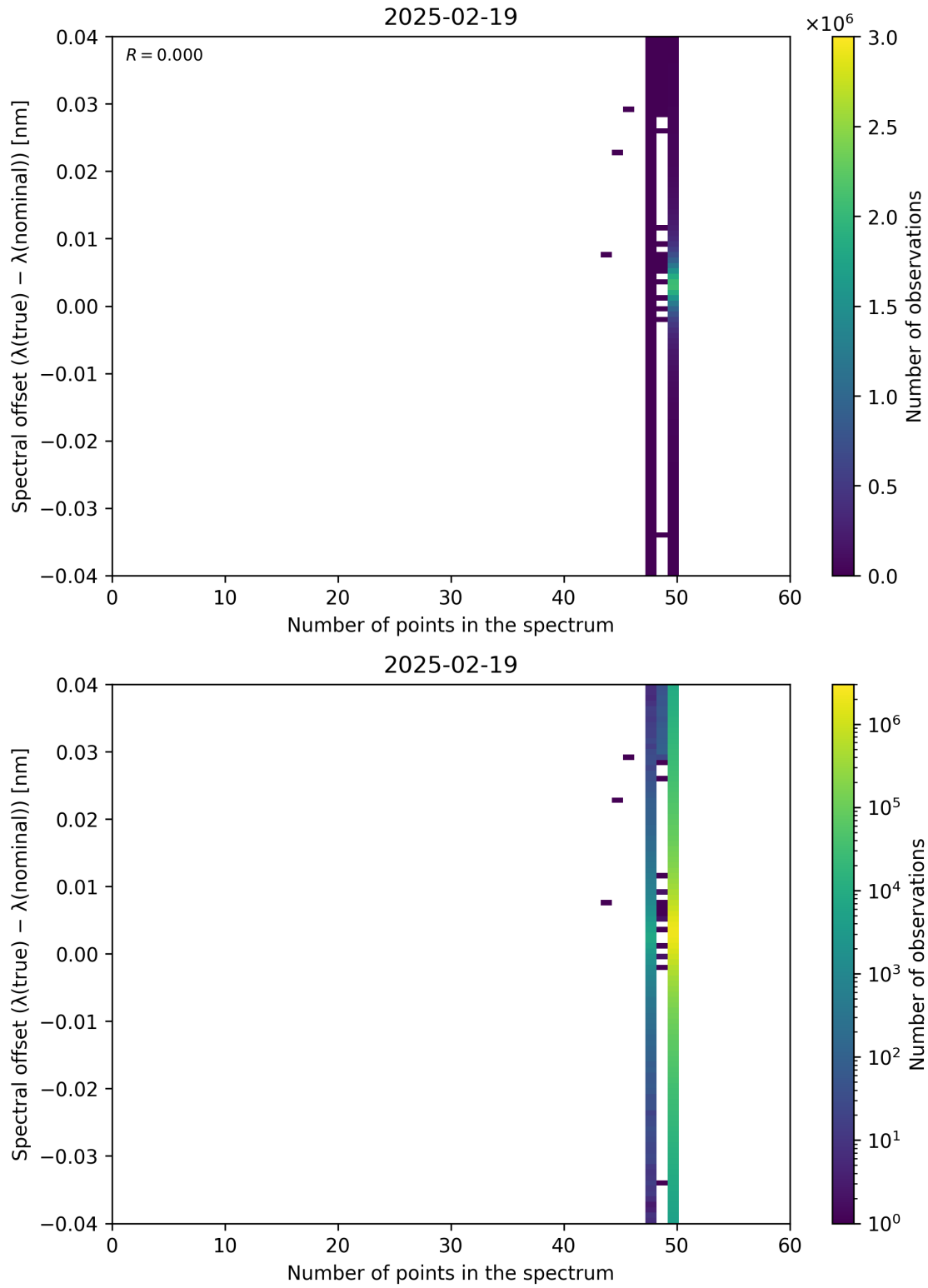
Figure 101: Scatter density plot of “Number of points in the spectrum” against “Spectral offset ( \lambda_{\text{true}} - \lambda_{\text{nominal}} )” for 2025-02-19 to 2025-02-20.
