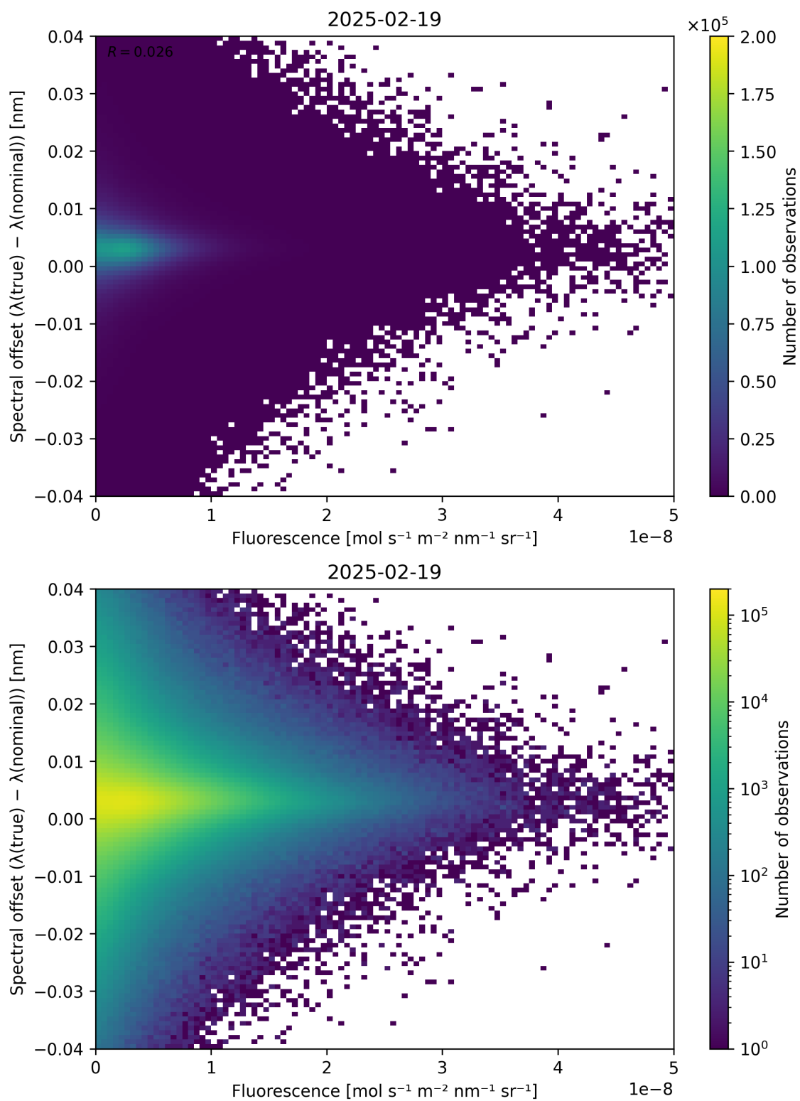
Figure 87: Scatter density plot of “Fluorescence” against “Spectral offset ( \lambda_{\text{true}} - \lambda_{\text{nominal}} )” for 2025-02-19 to 2025-02-20.
