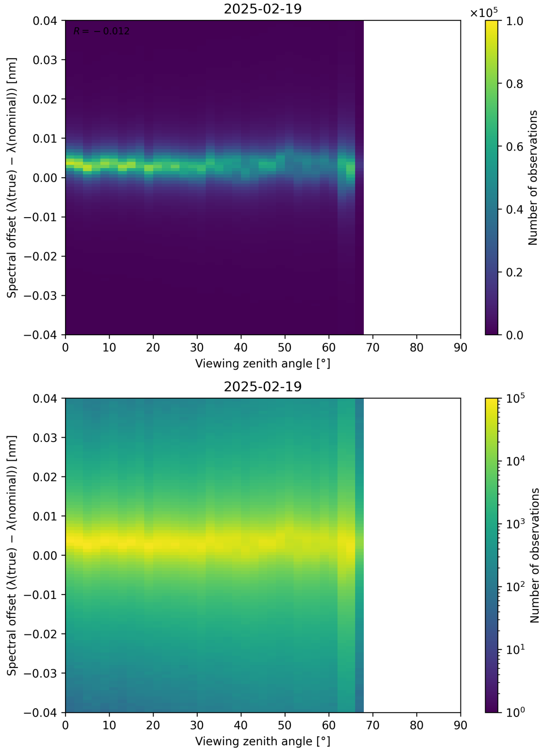
Figure 128: Scatter density plot of “Viewing zenith angle” against “Spectral offset ( \lambda_{\text{true}} - \lambda_{\text{nominal}} )” for 2025-02-19 to 2025-02-20.
