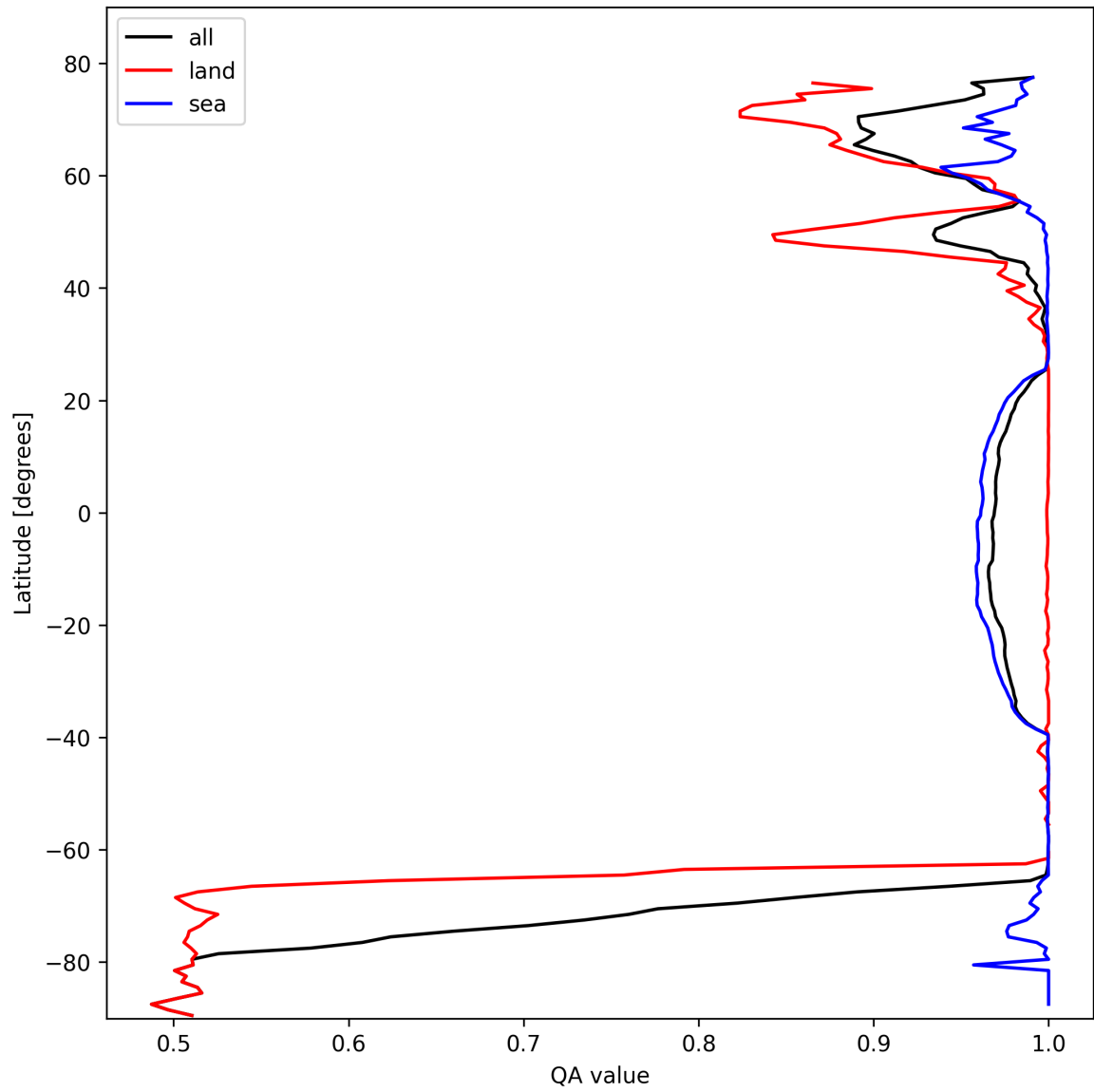
Figure 12: Zonal average of “QA value” for 2025-02-19 to 2025-02-20.
