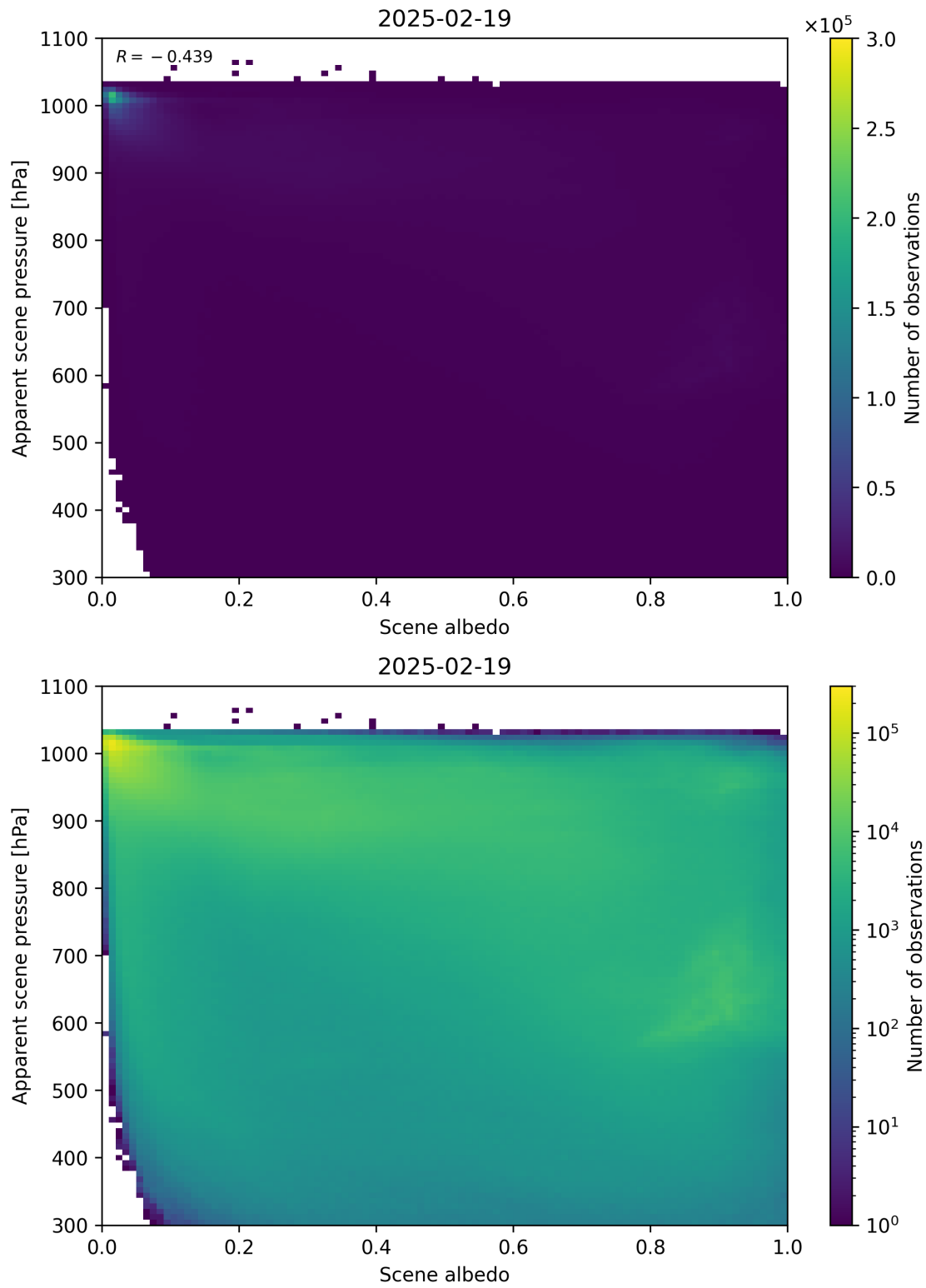
Figure 102: Scatter density plot of “Scene albedo” against “Apparent scene pressure” for 2025-02-19 to 2025-02-20.
