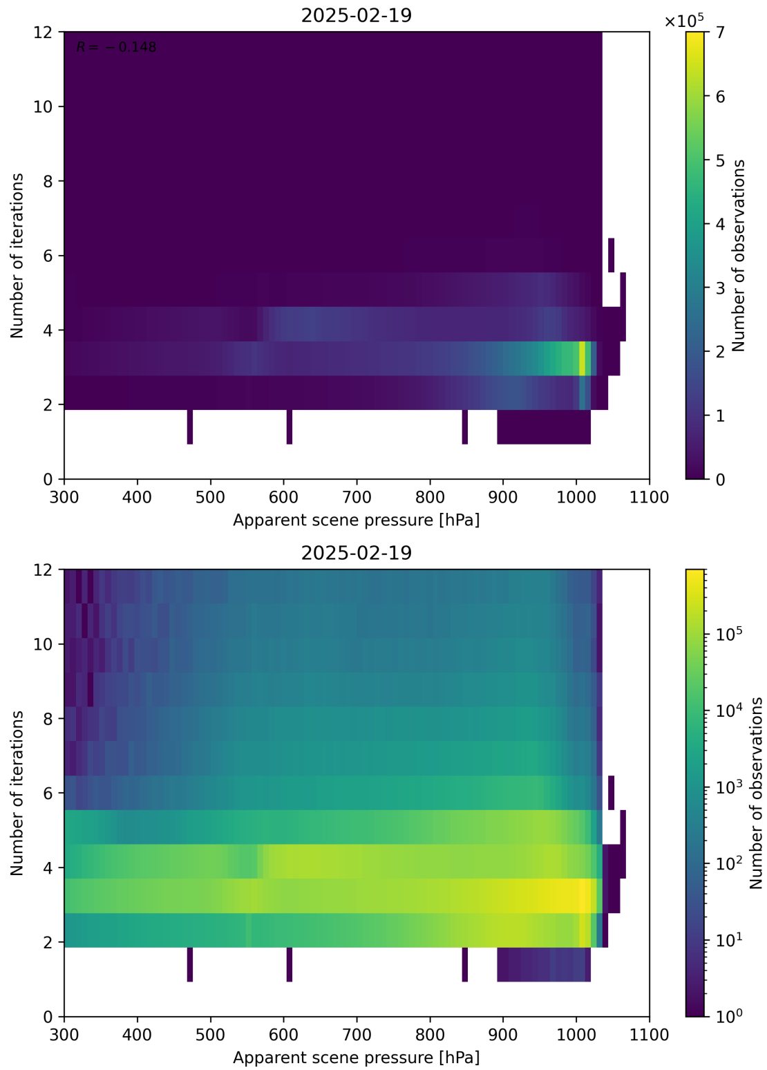
Figure 65: Scatter density plot of “Apparent scene pressure” against “Number of iterations” for 2025-02-19 to 2025-02-20.
