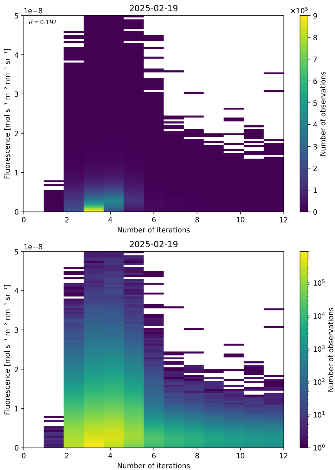
Figure 98: Scatter density plot of “Number of iterations” against “Fluorescence” for 2025-02-19 to 2025-02-20.
