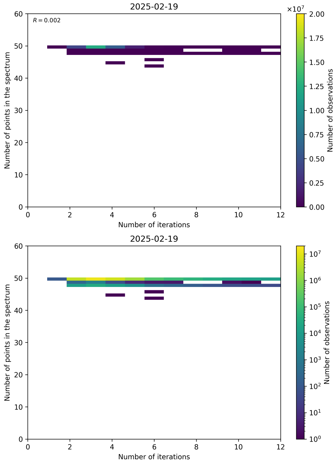
Figure 99: Scatter density plot of “Number of iterations” against “Number of points in the spectrum” for 2025-02-19 to 2025-02-20.
