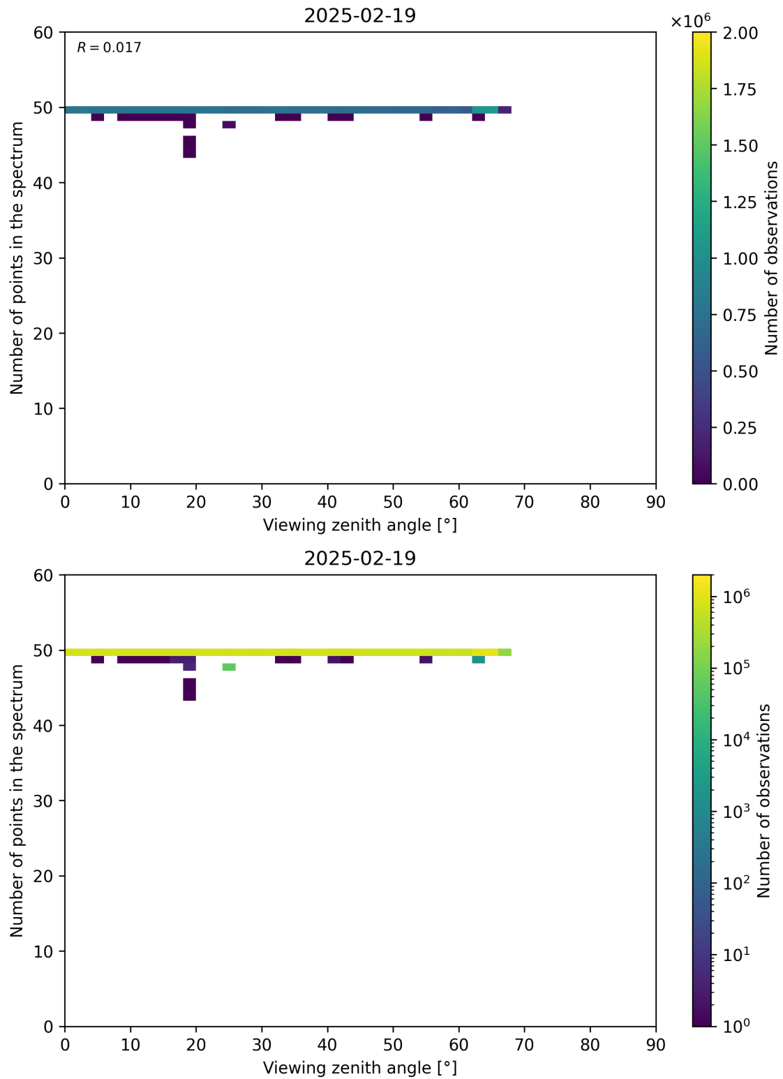
Figure 125: Scatter density plot of “Viewing zenith angle” against “Number of points in the spectrum” for 2025-02-19 to 2025-02-20.
