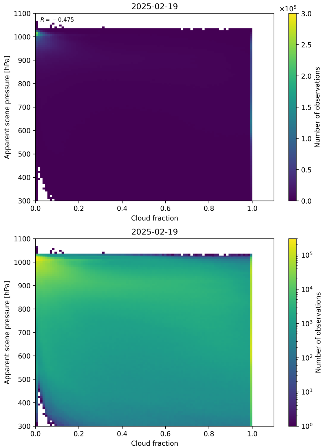
Figure 70: Scatter density plot of “Cloud fraction” against “Apparent scene pressure” for 2025-02-19 to 2025-02-20.
