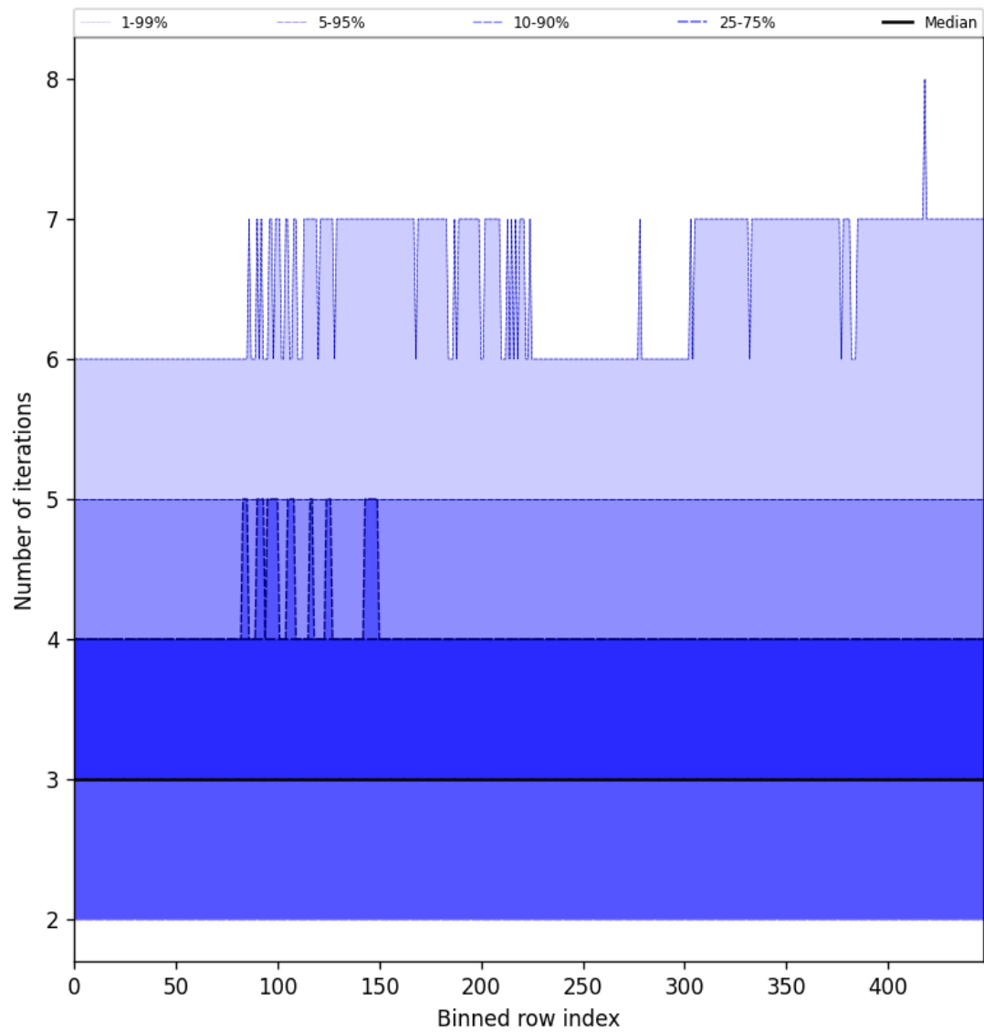
Figure 56: Along track statistics of “Number of iterations” for 2025-02-19 to 2025-02-20
