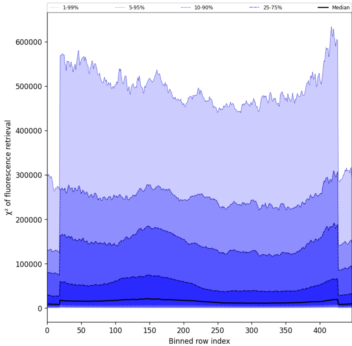
Figure 59: Along track statistics of “ \chi^2 of fluorescence retrieval” for 2025-02-19 to 2025-02-20
