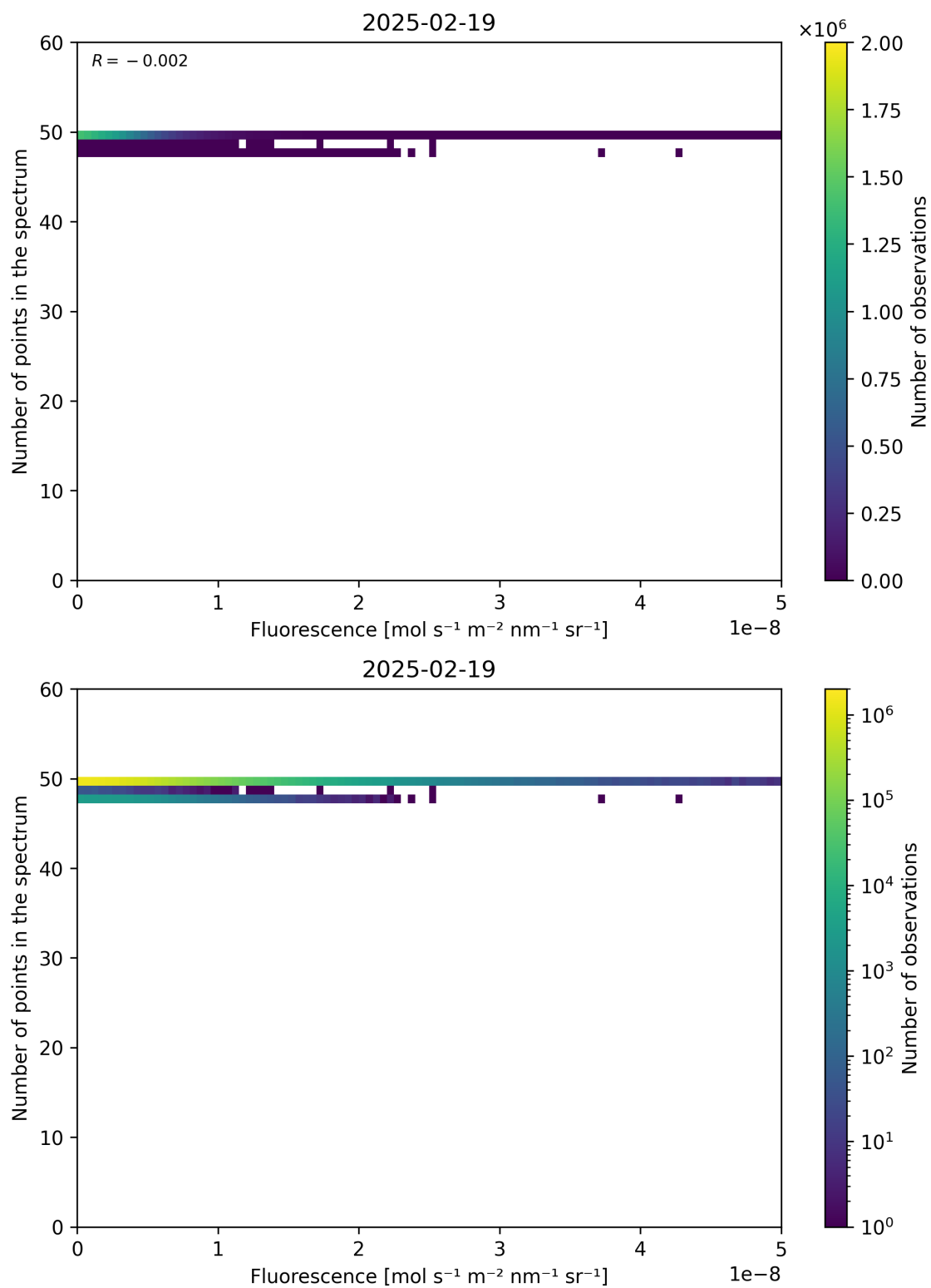
Figure 86: Scatter density plot of “Fluorescence” against “Number of points in the spectrum” for 2025-02-19 to 2025-02-20.
