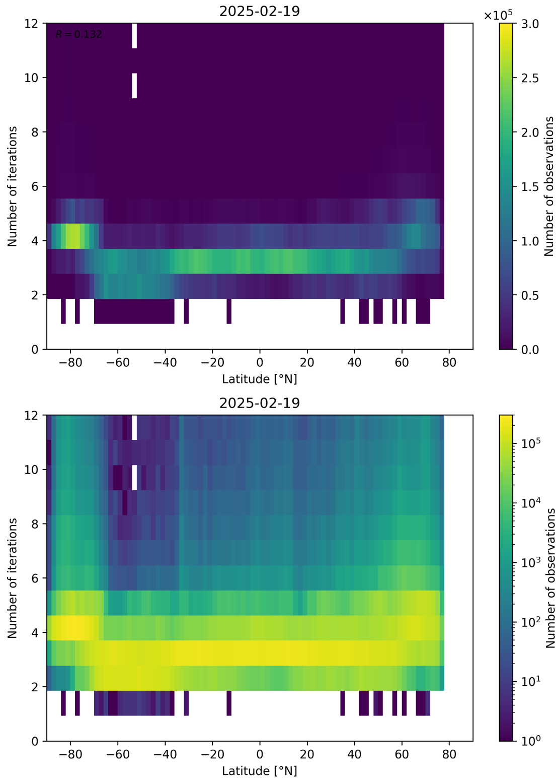
Figure 93: Scatter density plot of “Latitude” against “Number of iterations” for 2025-02-19 to 2025-02-20.
