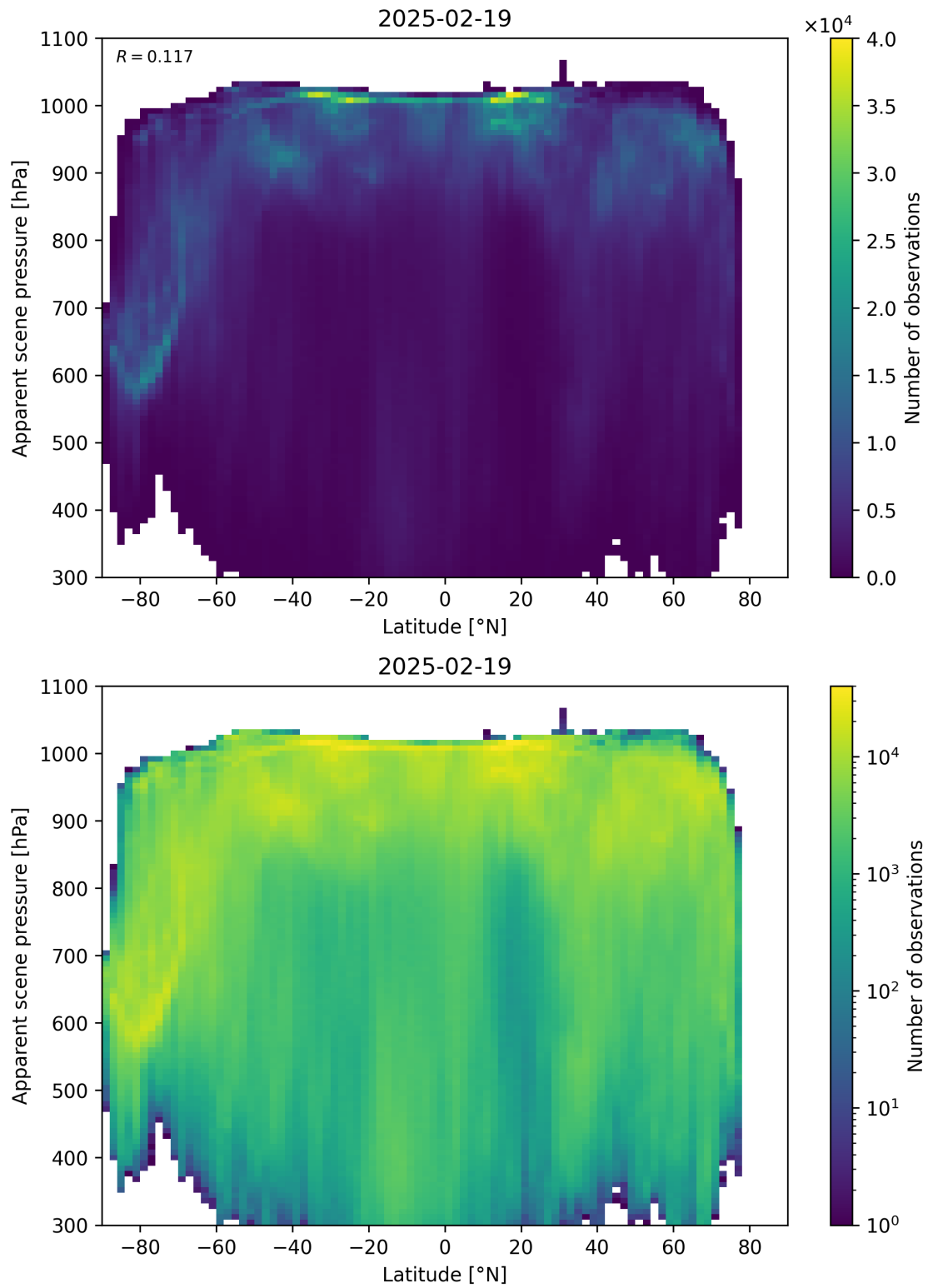
Figure 88: Scatter density plot of “Latitude” against “Apparent scene pressure” for 2025-02-19 to 2025-02-20.
