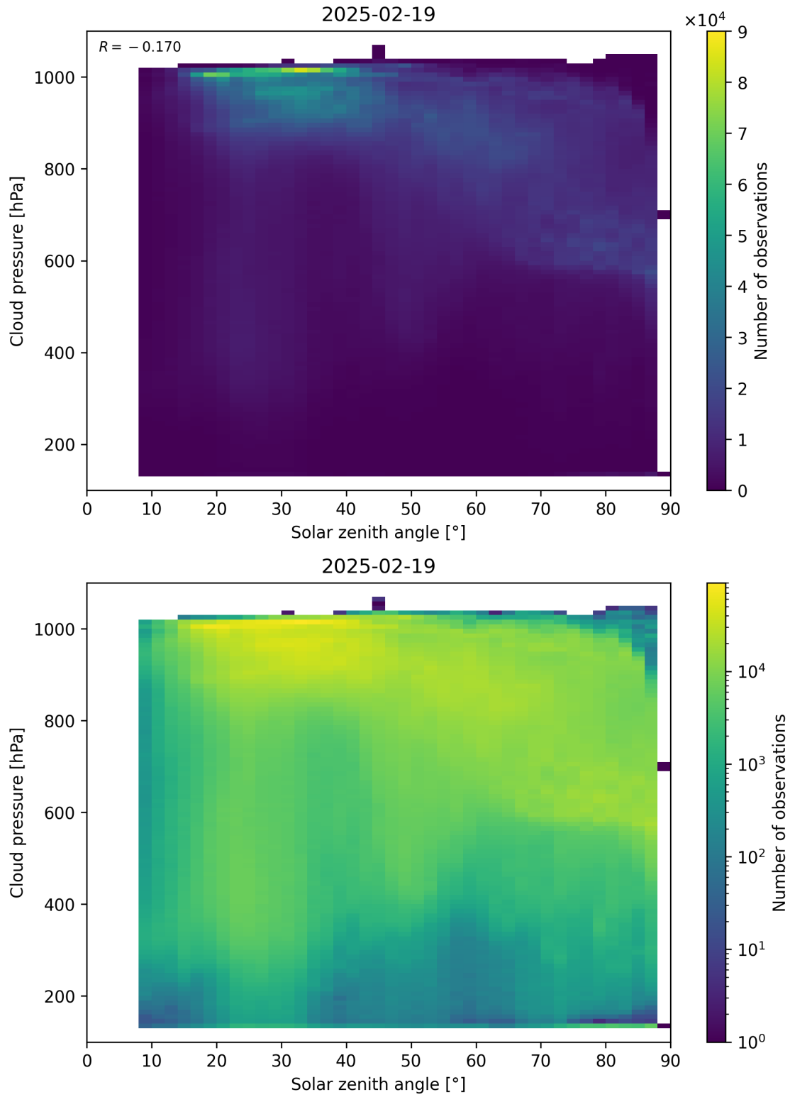
Figure 111: Scatter density plot of “Solar zenith angle” against “Cloud pressure” for 2025-02-19 to 2025-02-20.
