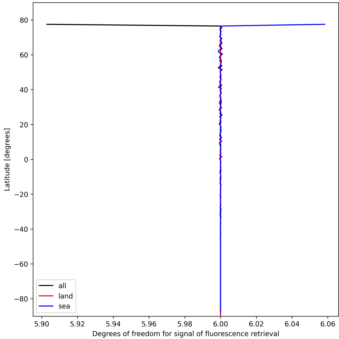
Figure 26: Zonal average of “Degrees of freedom for signal of fluorescence retrieval” for 2025-02-19 to 2025-02-20.
