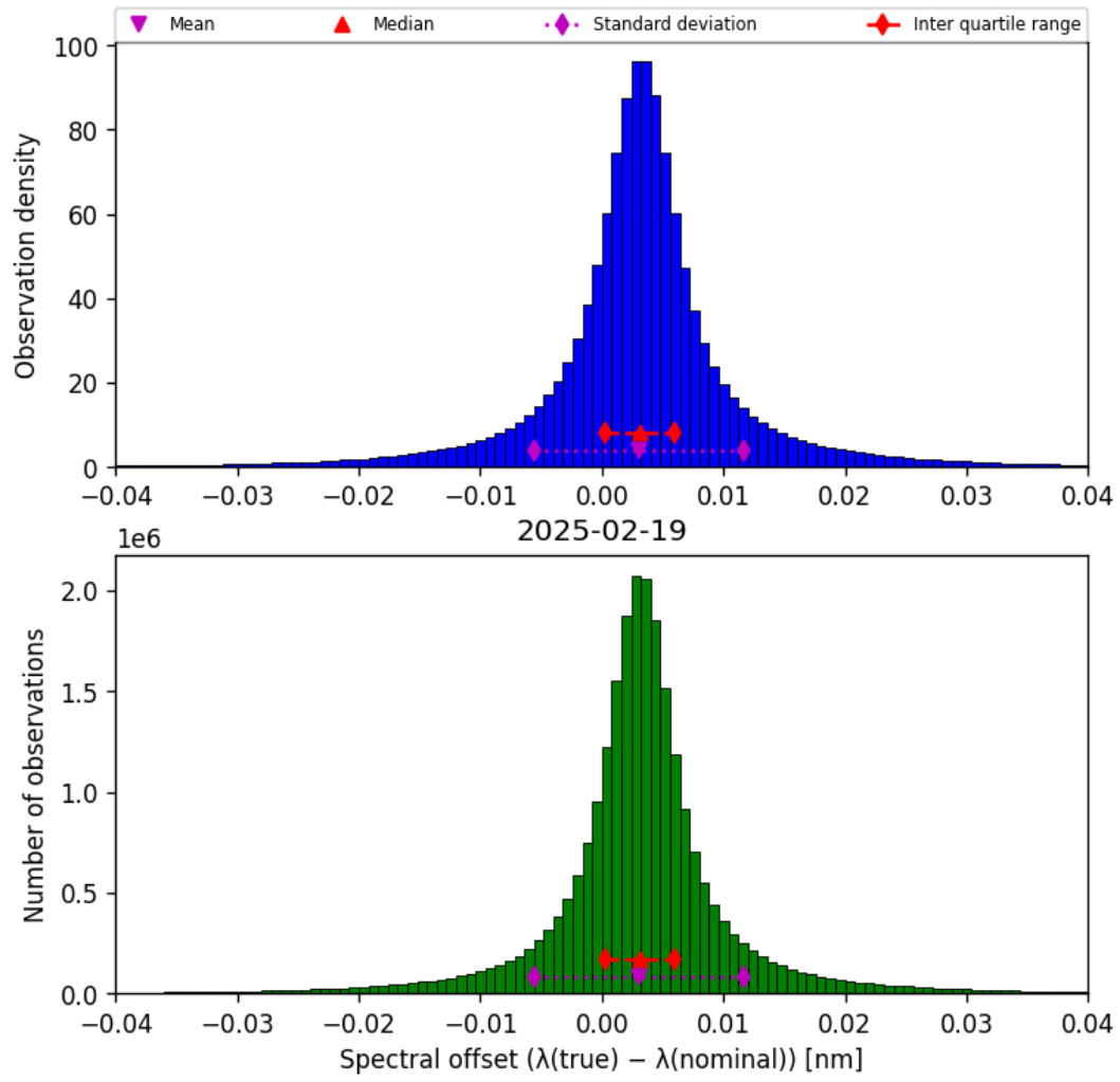
Figure 45: Histogram of “Spectral offset ( \lambda_{\text{true}} - \lambda_{\text{nominal}} )” for 2025-02-19 to 2025-02-20
