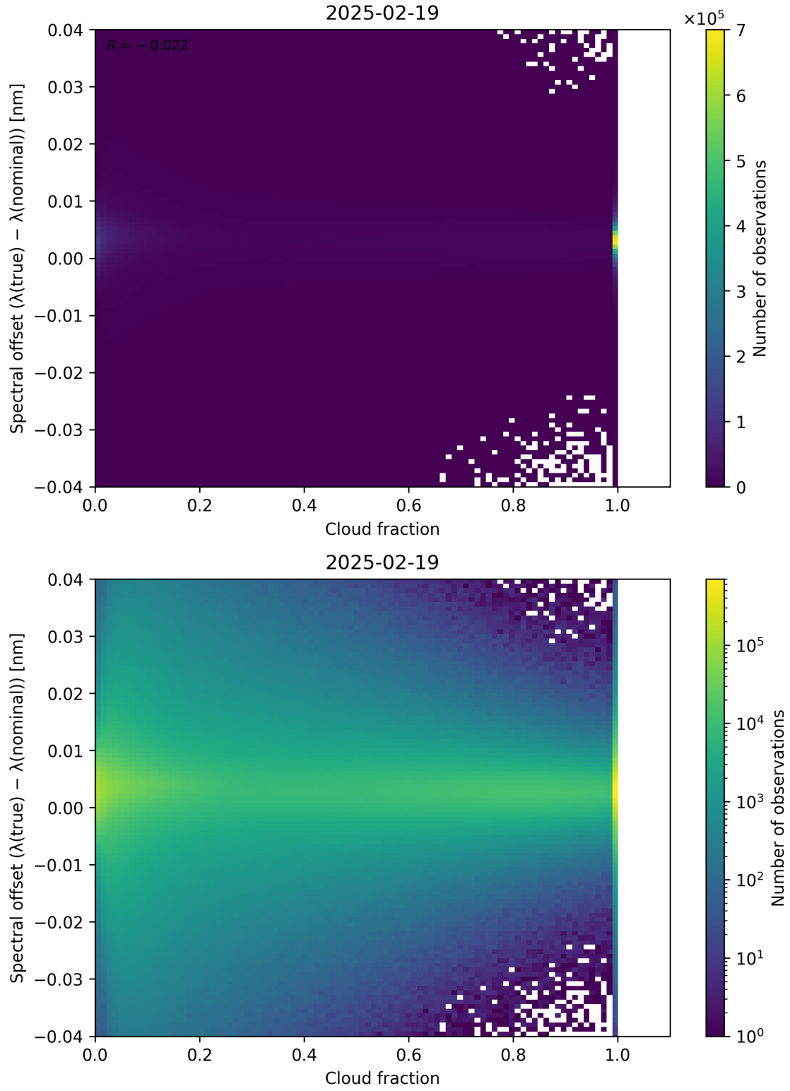
Figure 76: Scatter density plot of “Cloud fraction” against “Spectral offset ( \lambda_{\text{true}} - \lambda_{\text{nominal}} )” for 2025-02-19 to 2025-02-20.
