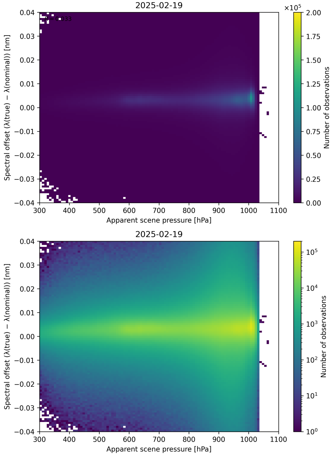
Figure 67: Scatter density plot of “Apparent scene pressure” against “Spectral offset ( \lambda_{\text{true}} - \lambda_{\text{nominal}} )” for 2025-02-19 to 2025-02-20.
