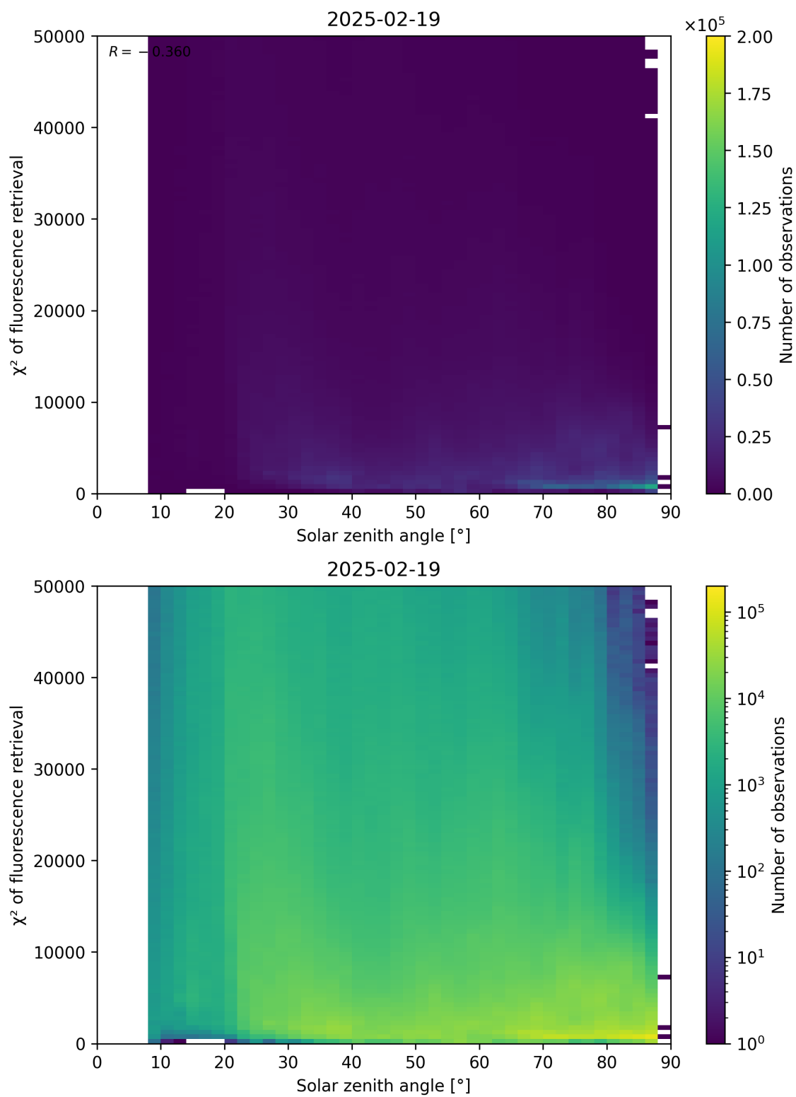
Figure 109: Scatter density plot of “Solar zenith angle” against “ \chi^2 of fluorescence retrieval” for 2025-02-19 to 2025-02-20.
