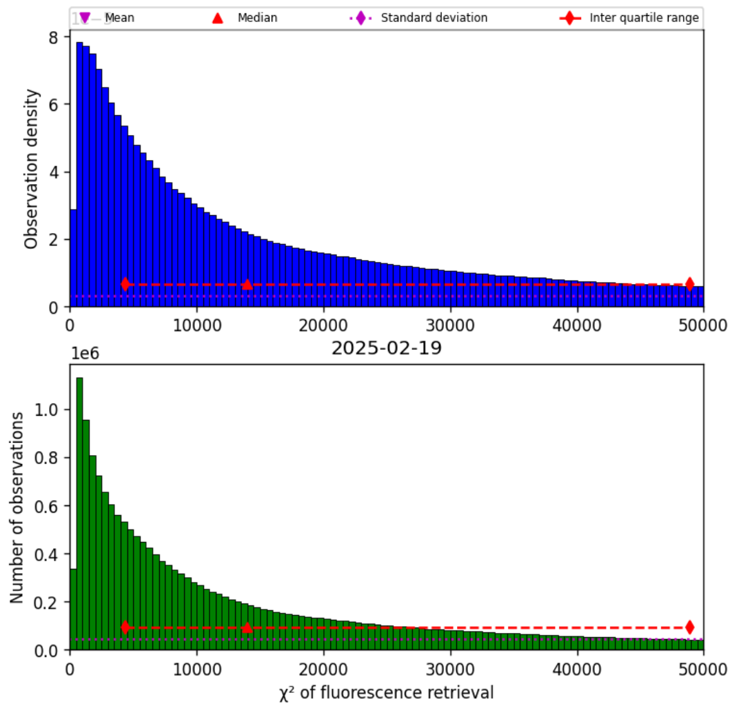
Figure 42: Histogram of “ \chi^2 of fluorescence retrieval” for 2025-02-19 to 2025-02-20
