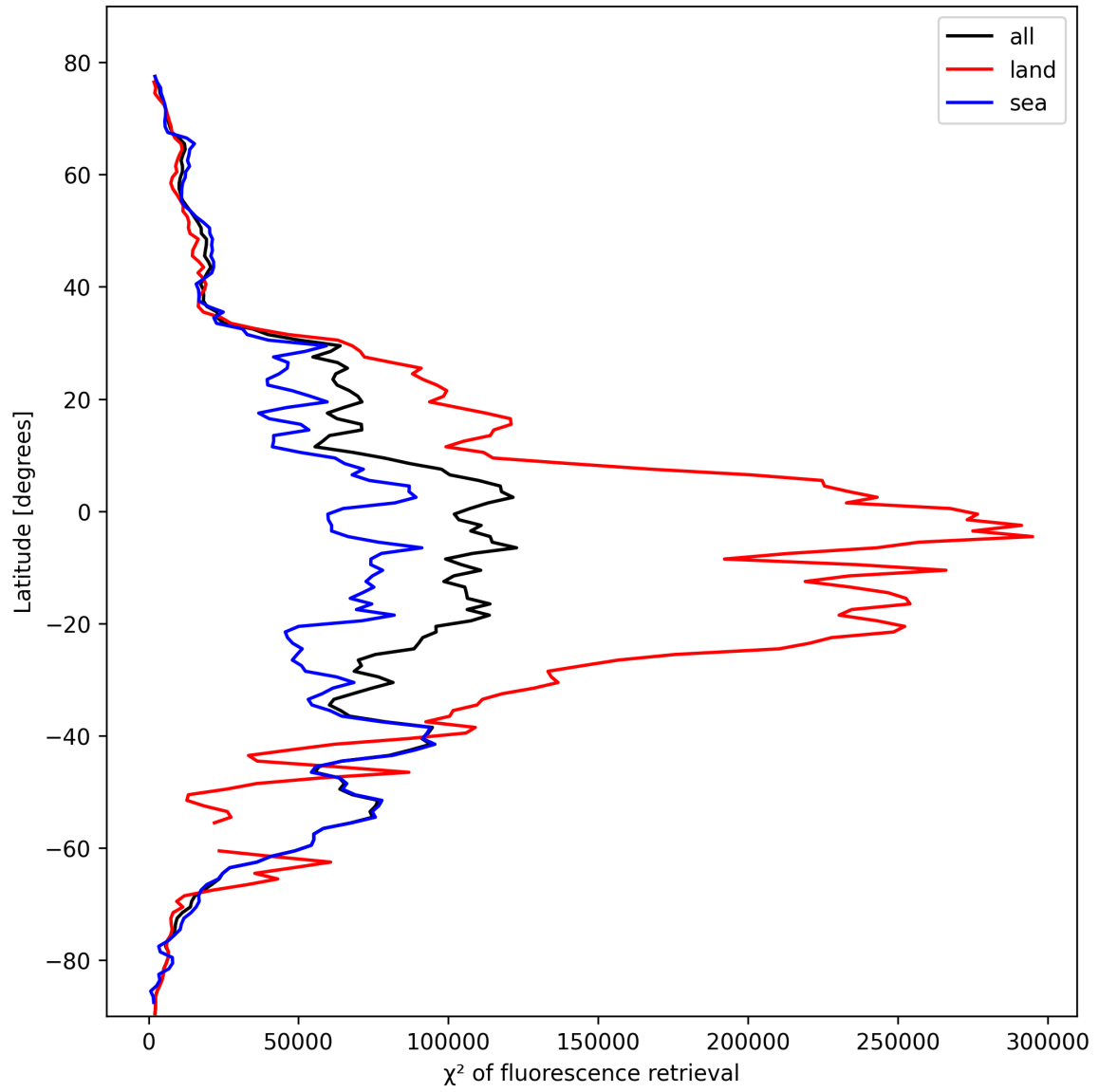
Figure 25: Zonal average of “ \chi^2 of fluorescence retrieval” for 2025-02-19 to 2025-02-20.
