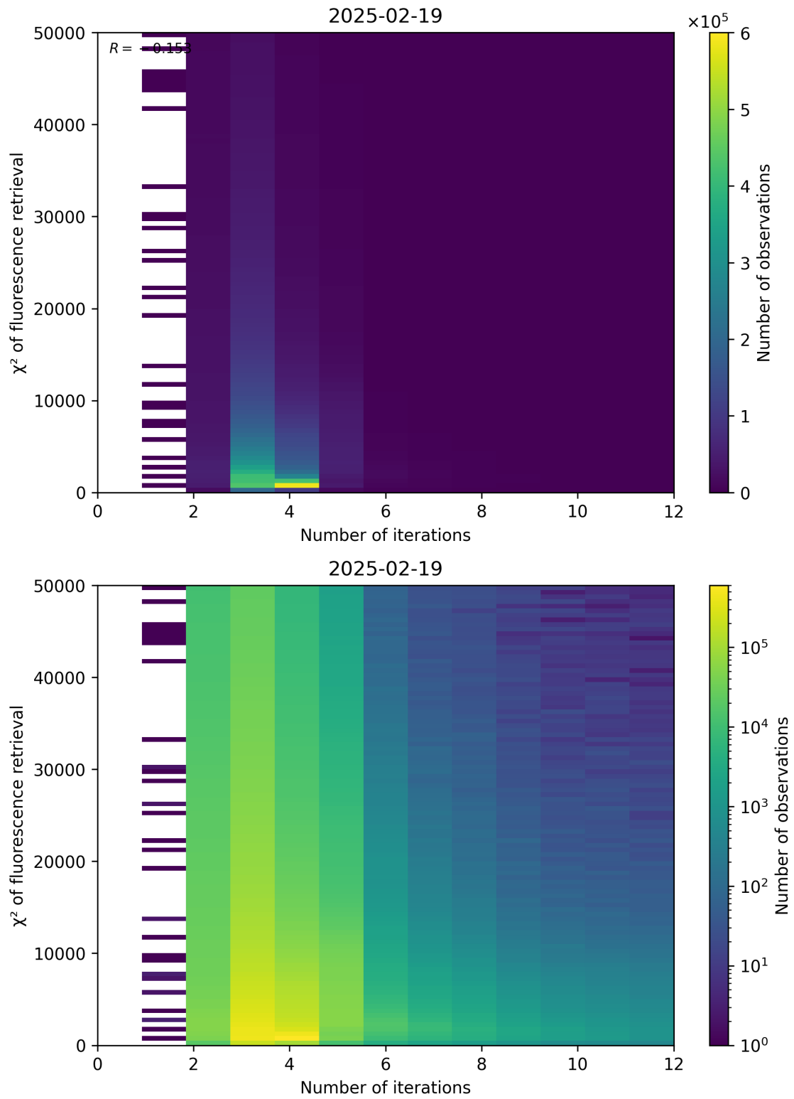
Figure 97: Scatter density plot of “Number of iterations” against “ \chi^2 of fluorescence retrieval” for 2025-02-19 to 2025-02-20.
