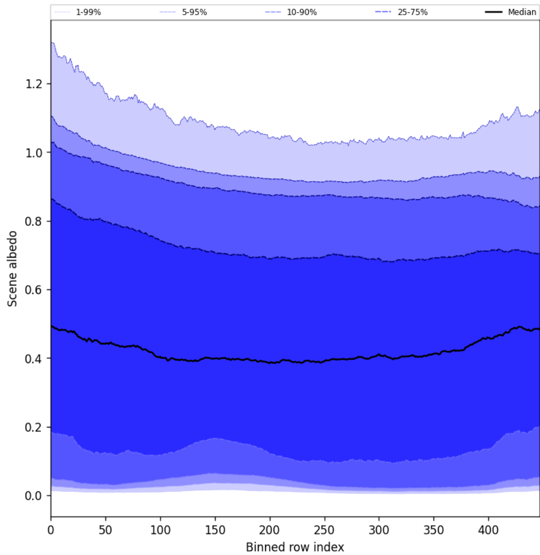
Figure 51: Along track statistics of “Scene albedo” for 2025-02-19 to 2025-02-20
