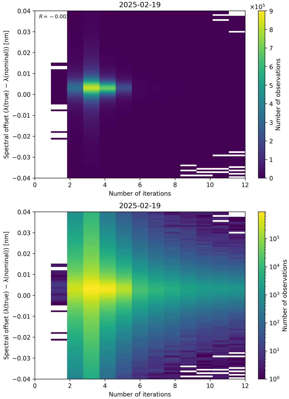
Figure 100: Scatter density plot of “Number of iterations” against “Spectral offset ( \lambda_{\text{true}} - \lambda_{\text{nominal}} )” for 2025-02-19 to 2025-02-20.
