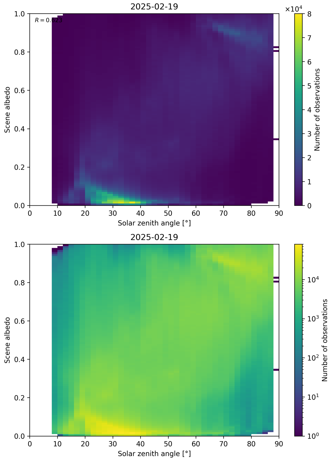
Figure 116: Scatter density plot of “Solar zenith angle” against “Scene albedo” for 2025-02-19 to 2025-02-20.
