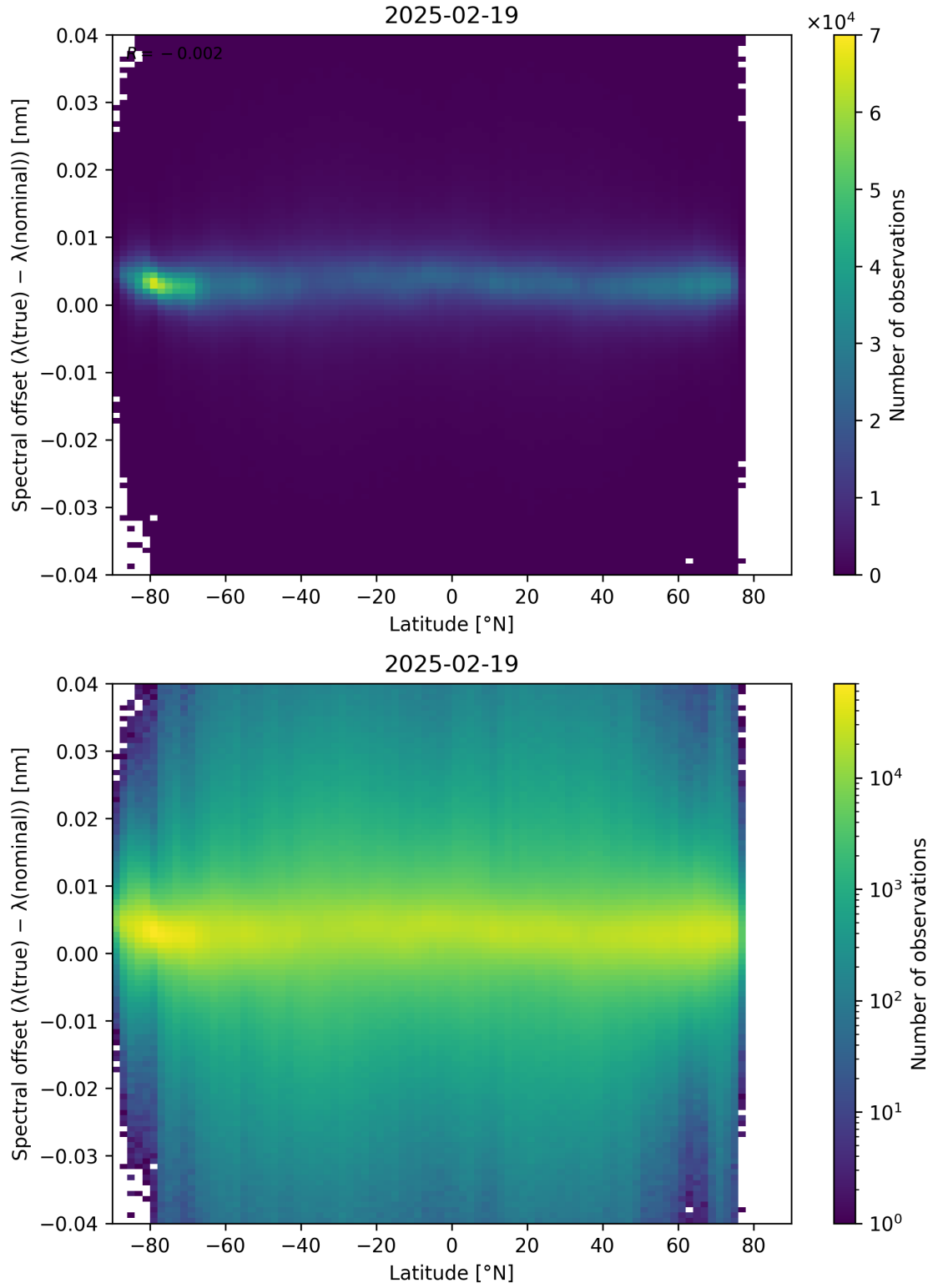
Figure 96: Scatter density plot of “Latitude” against “Spectral offset ( \lambda_{\text{true}} - \lambda_{\text{nominal}} )” for 2025-02-19 to 2025-02-20.
