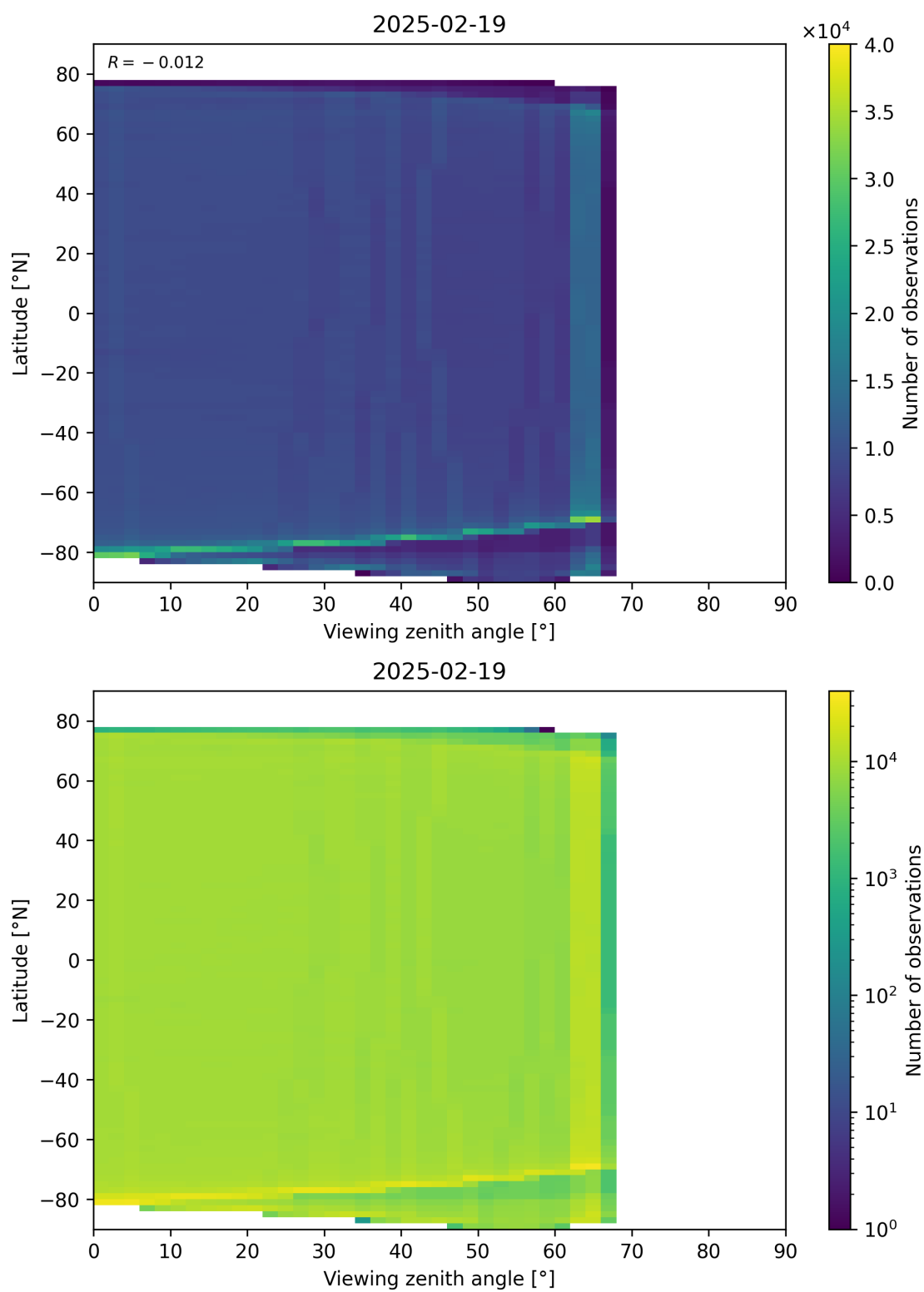
Figure 123: Scatter density plot of “Viewing zenith angle” against “Latitude” for 2025-02-19 to 2025-02-20.
