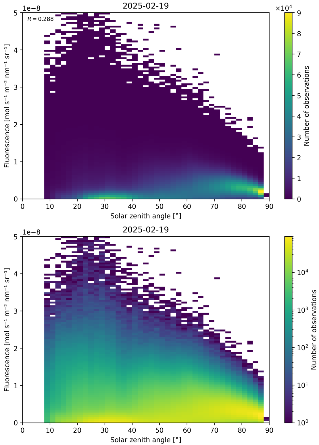
Figure 112: Scatter density plot of “Solar zenith angle” against “Fluorescence” for 2025-02-19 to 2025-02-20.
