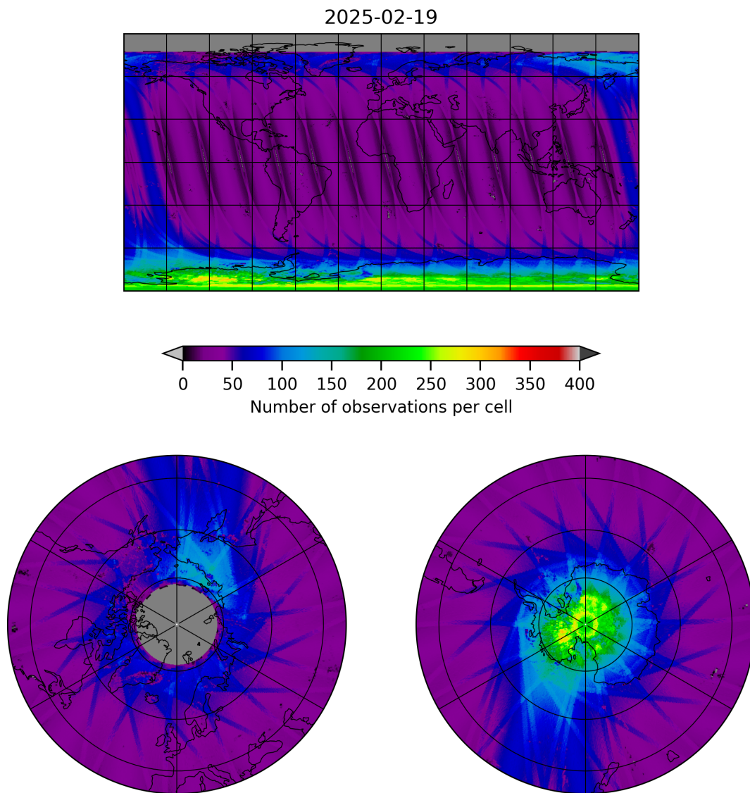
Figure 11: Map of the number of observations for 2025-02-19 to 2025-02-20
