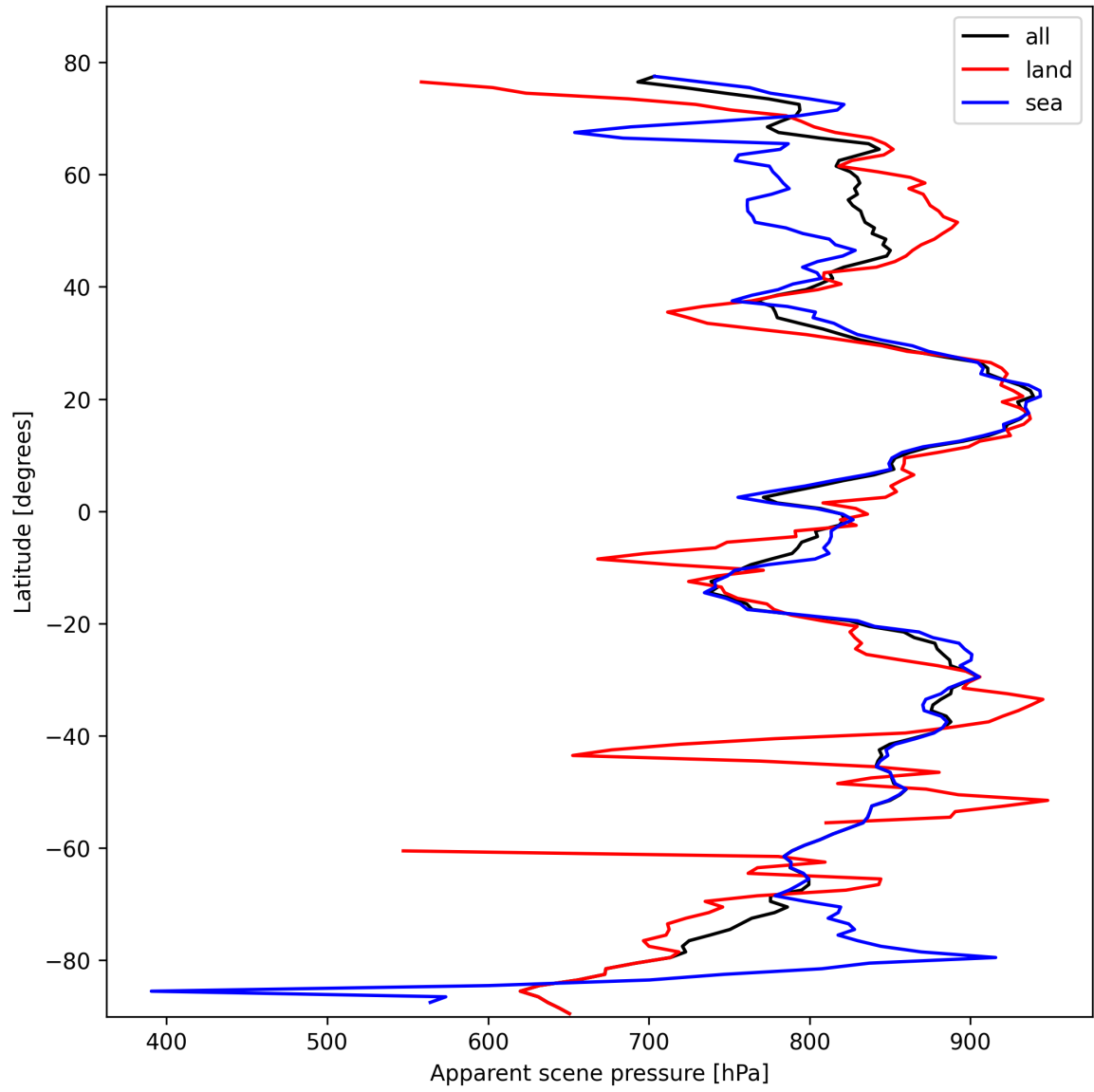
Figure 19: Zonal average of “Apparent scene pressure” for 2025-02-19 to 2025-02-20.
