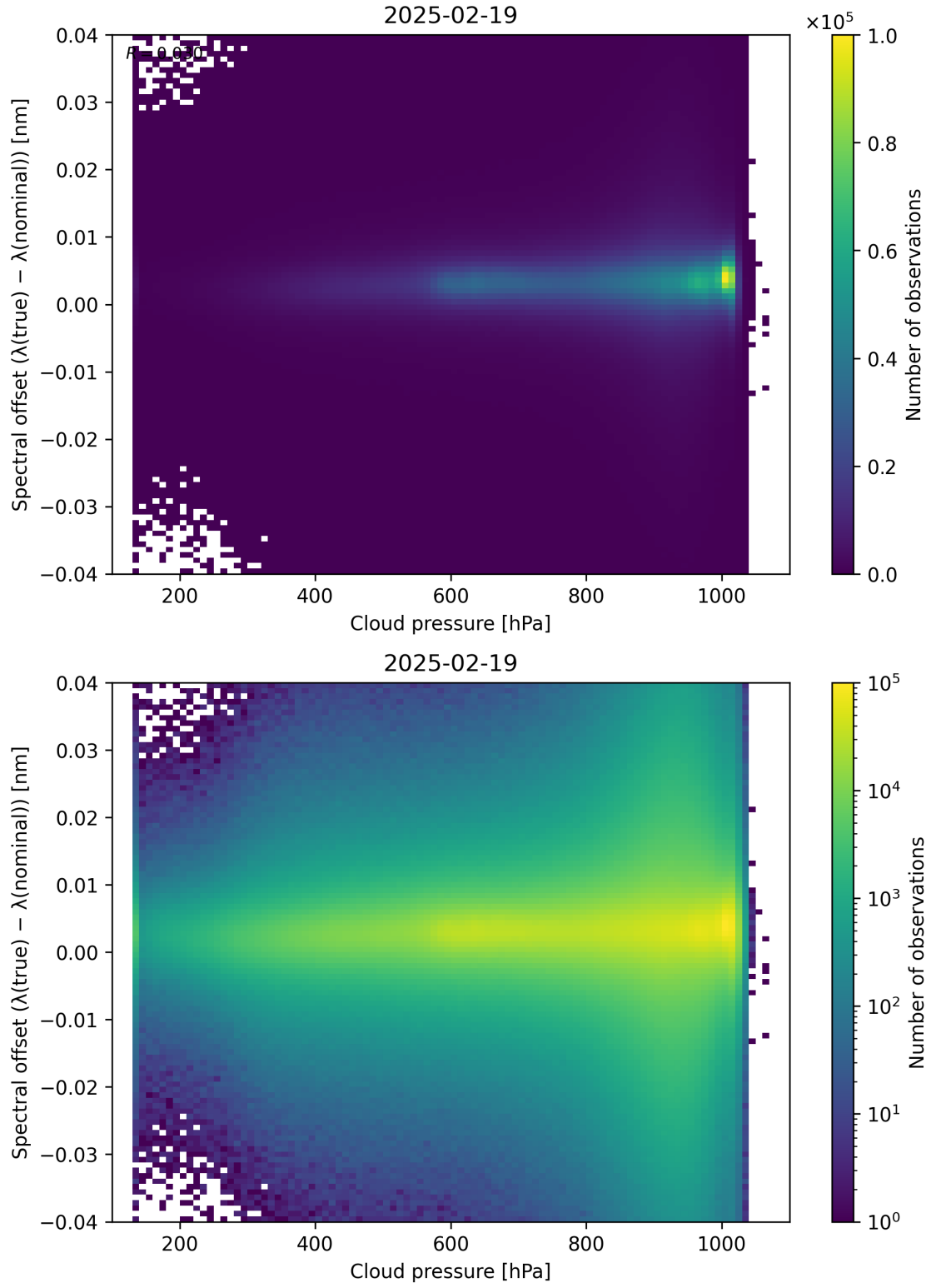
Figure 84: Scatter density plot of “Cloud pressure” against “Spectral offset ( \lambda_{\text{true}} - \lambda_{\text{nominal}} )” for 2025-02-19 to 2025-02-20.
