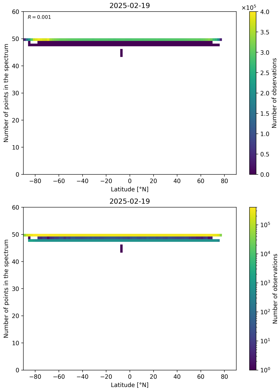
Figure 94: Scatter density plot of “Latitude” against “Number of points in the spectrum” for 2025-02-19 to 2025-02-20.
