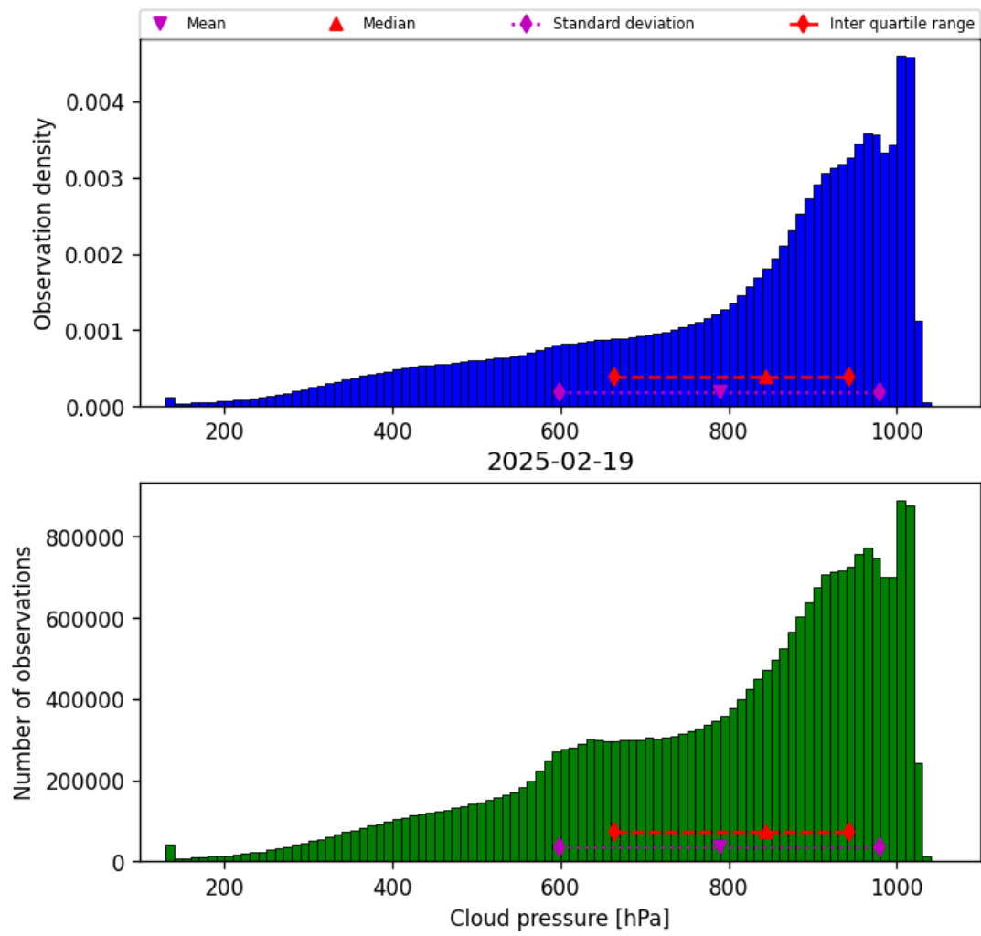
Figure 30: Histogram of “Cloud pressure” for 2025-02-19 to 2025-02-20
