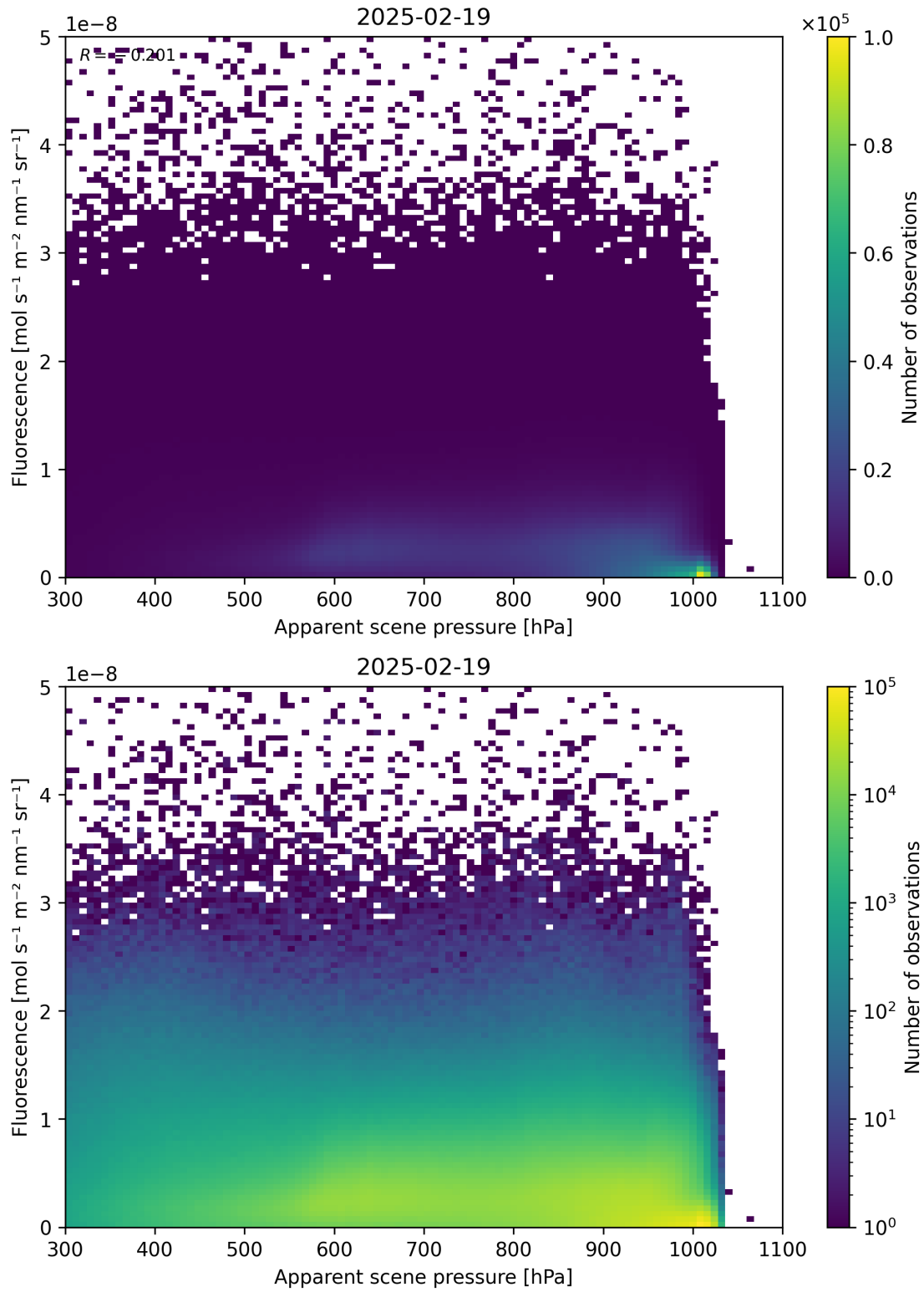
Figure 64: Scatter density plot of “Apparent scene pressure” against “Fluorescence” for 2025-02-19 to 2025-02-20.
