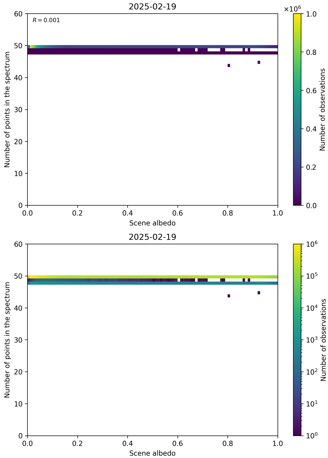
Figure 106: Scatter density plot of “Scene albedo” against “Number of points in the spectrum” for 2025-02-19 to 2025-02-20.
