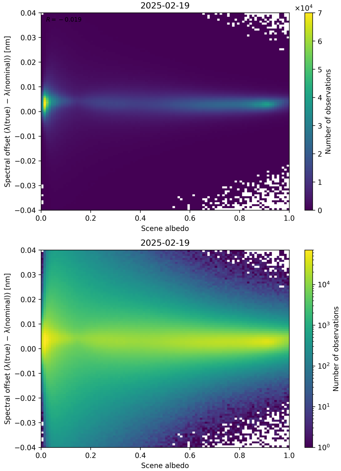
Figure 107: Scatter density plot of “Scene albedo” against “Spectral offset ( \lambda_{\text{true}} - \lambda_{\text{nominal}} )” for 2025-02-19 to 2025-02-20.
