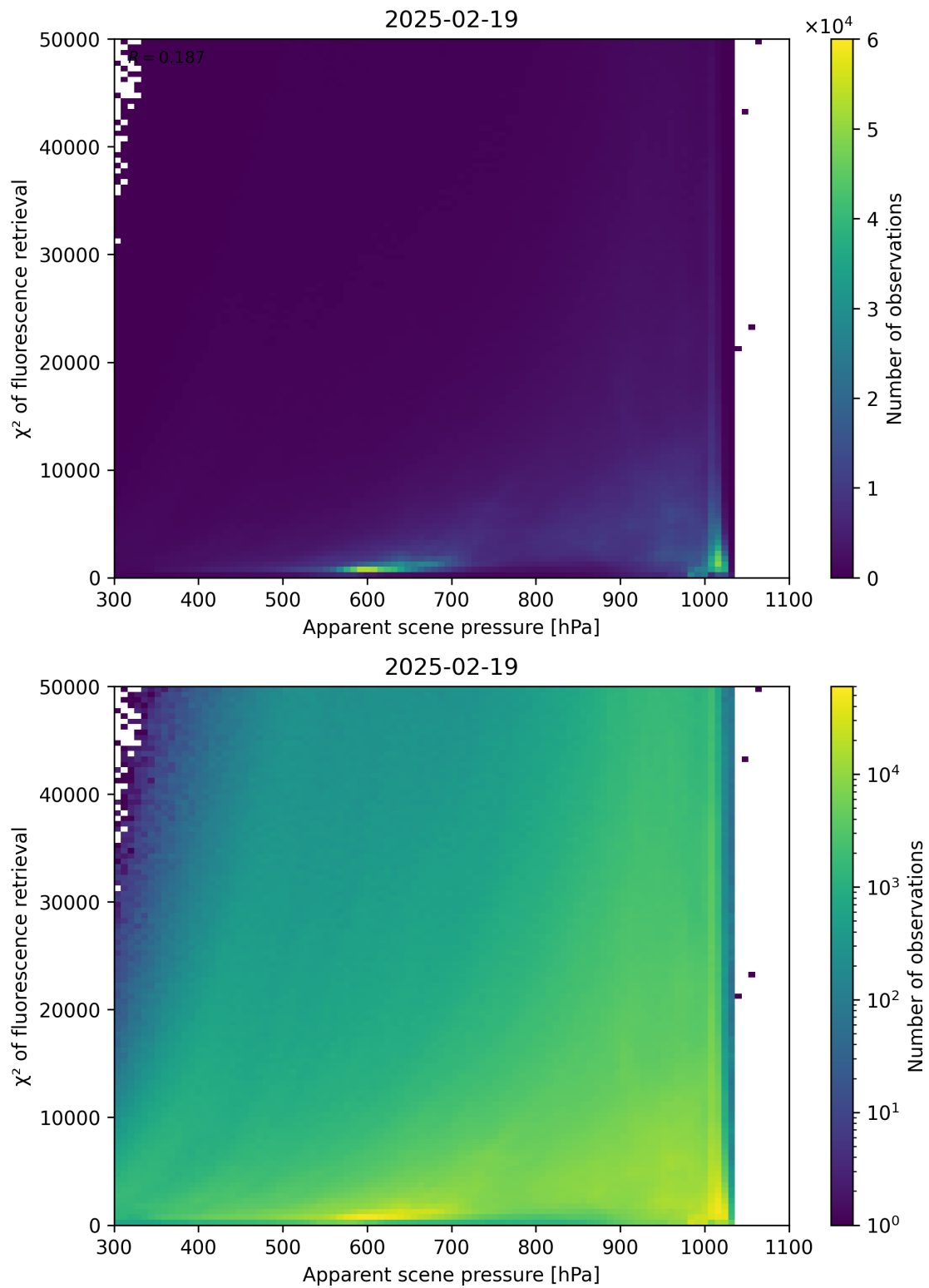
Figure 63: Scatter density plot of “Apparent scene pressure” against “ \chi^2 of fluorescence retrieval” for 2025-02-19 to 2025-02-20.
