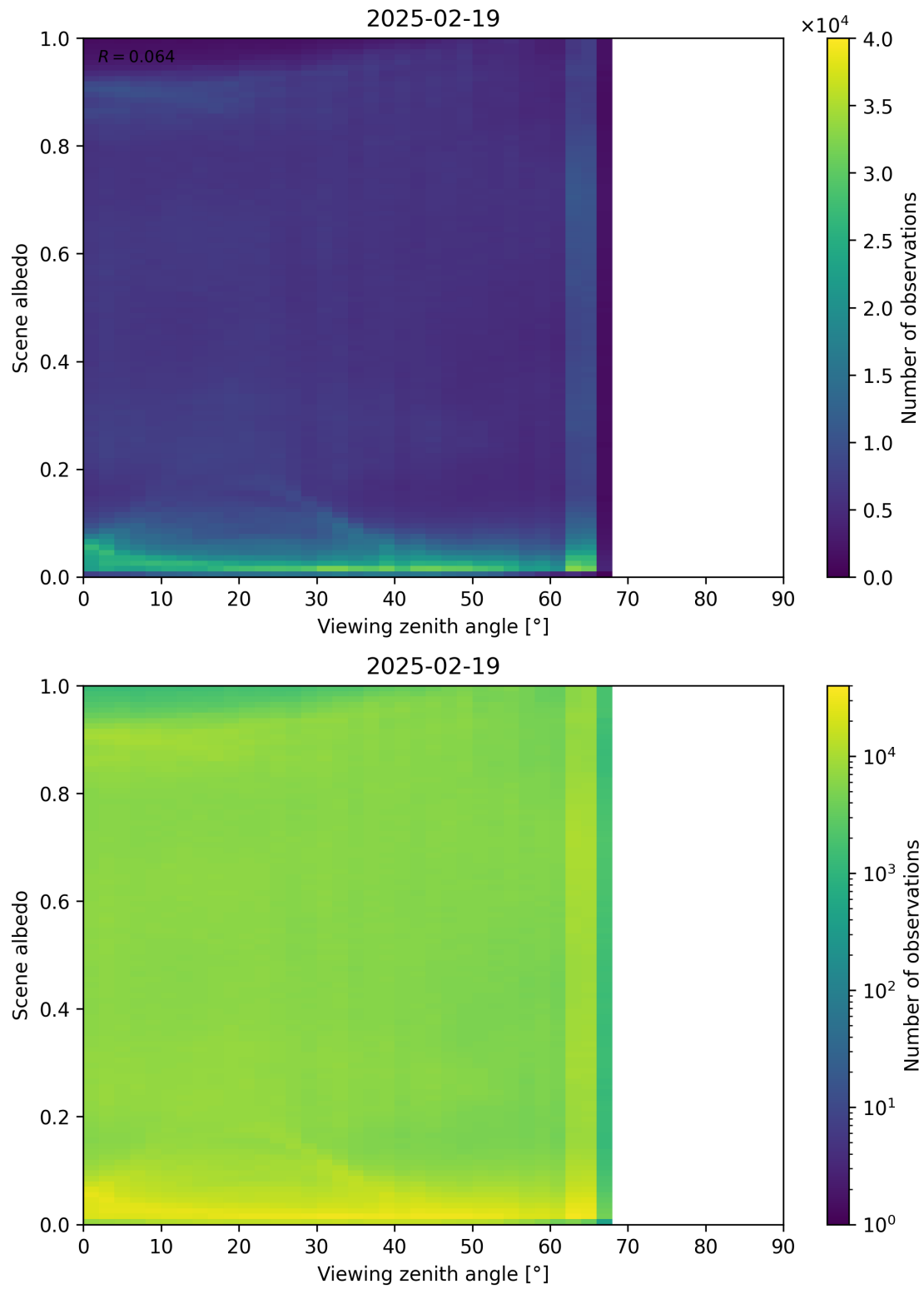
Figure 126: Scatter density plot of “Viewing zenith angle” against “Scene albedo” for 2025-02-19 to 2025-02-20.
