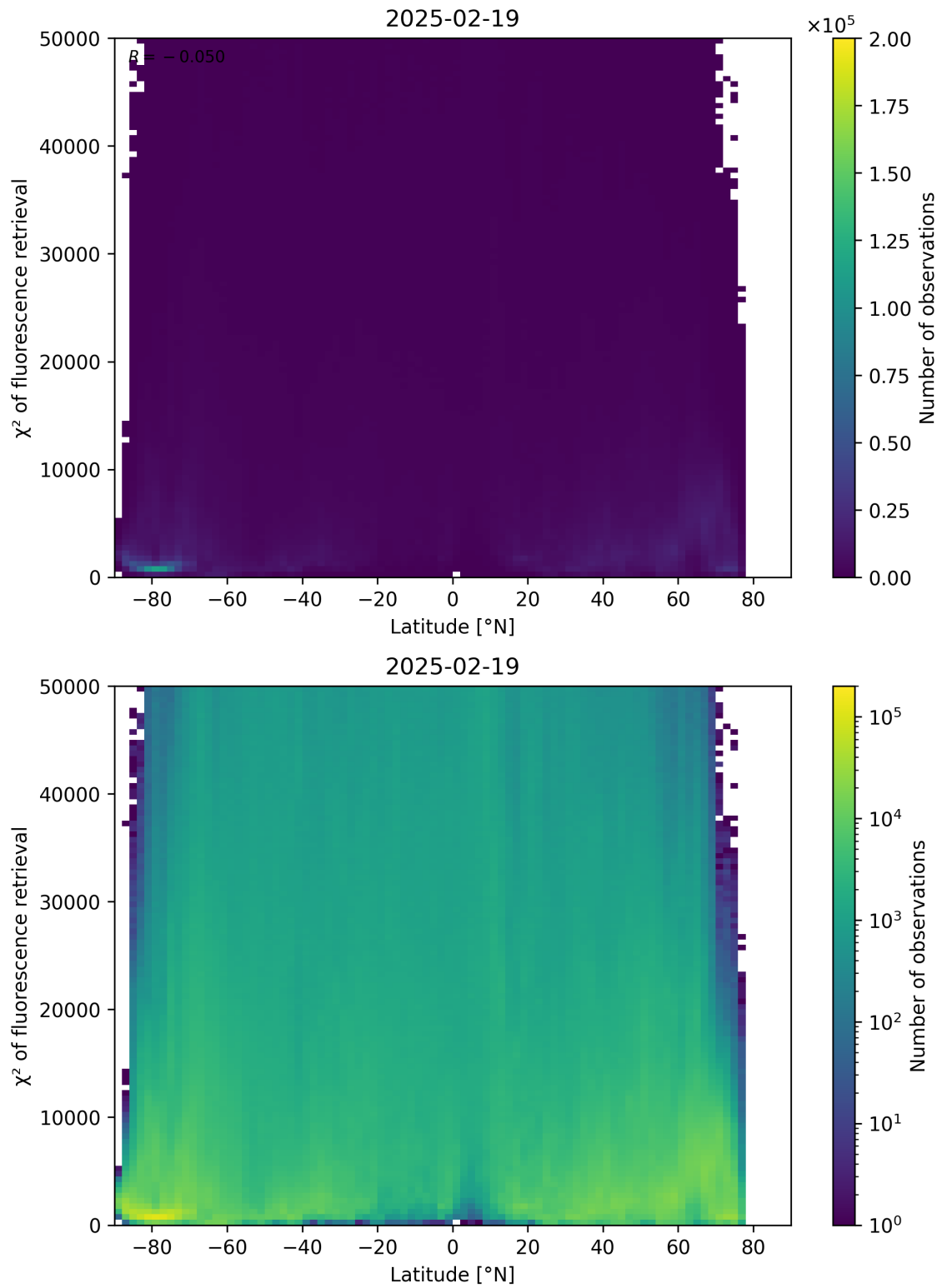
Figure 89: Scatter density plot of “Latitude” against “ \chi^2 of fluorescence retrieval” for 2025-02-19 to 2025-02-20.
