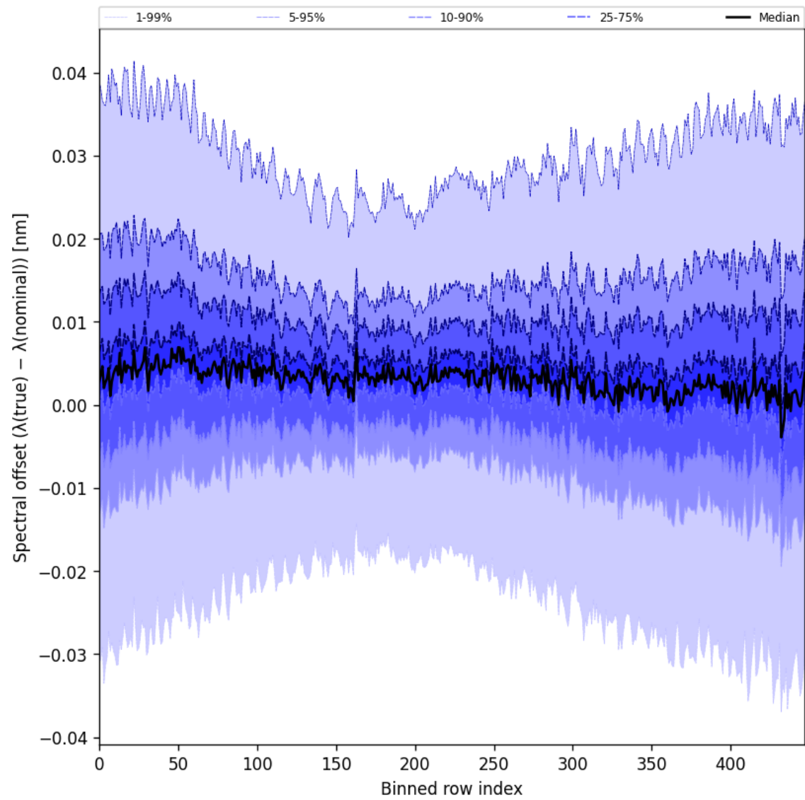
Figure 62: Along track statistics of “Spectral offset ( \lambda_{\text{true}} - \lambda_{\text{nominal}} )” for 2025-02-19 to 2025-02-20
