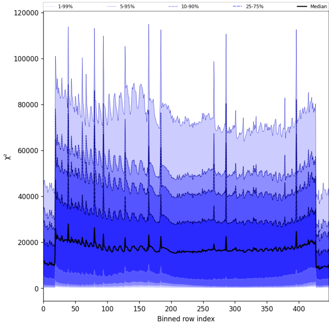
Figure 55: Along track statistics of “ \chi^2 ” for 2025-02-19 to 2025-02-20
