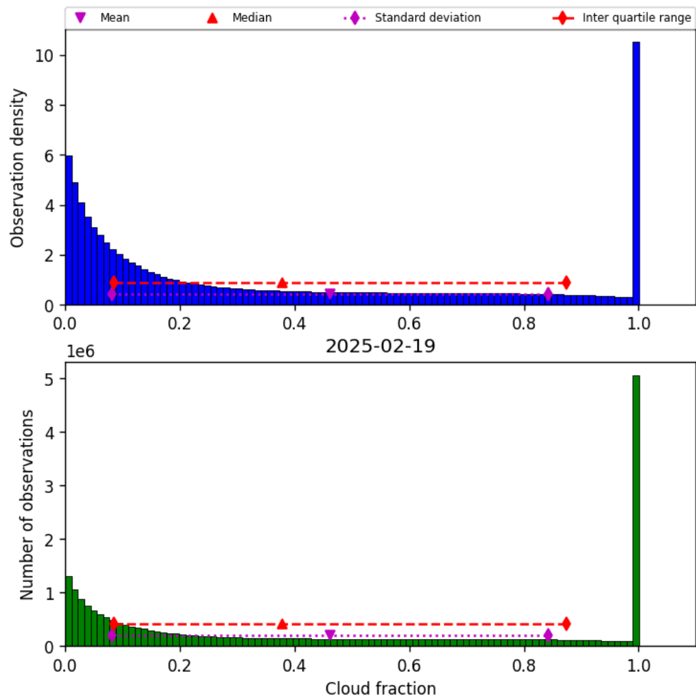
Figure 32: Histogram of “Cloud fraction” for 2025-02-19 to 2025-02-20
