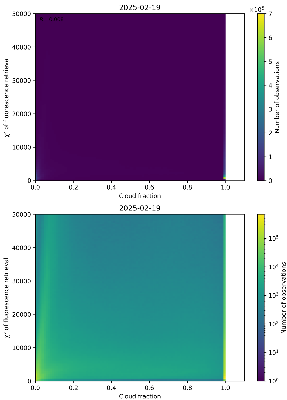
Figure 71: Scatter density plot of “Cloud fraction” against “ \chi^2 of fluorescence retrieval” for 2025-02-19 to 2025-02-20.
