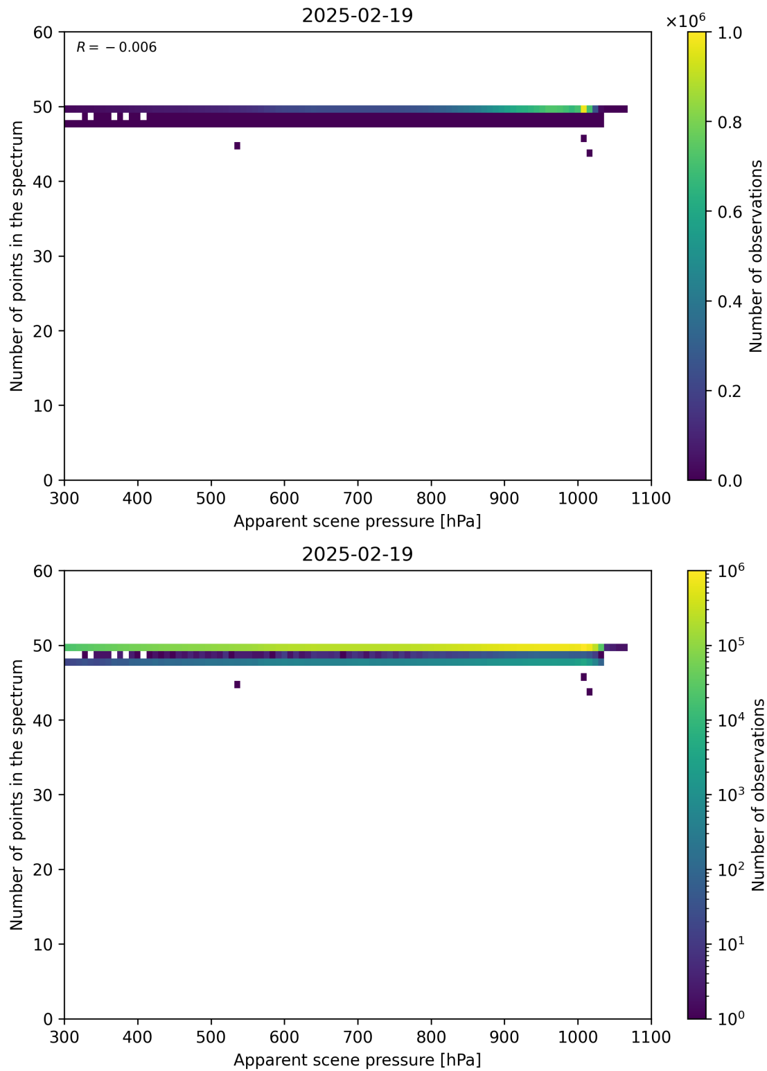
Figure 66: Scatter density plot of “Apparent scene pressure” against “Number of points in the spectrum” for 2025-02-19 to 2025-02-20.
