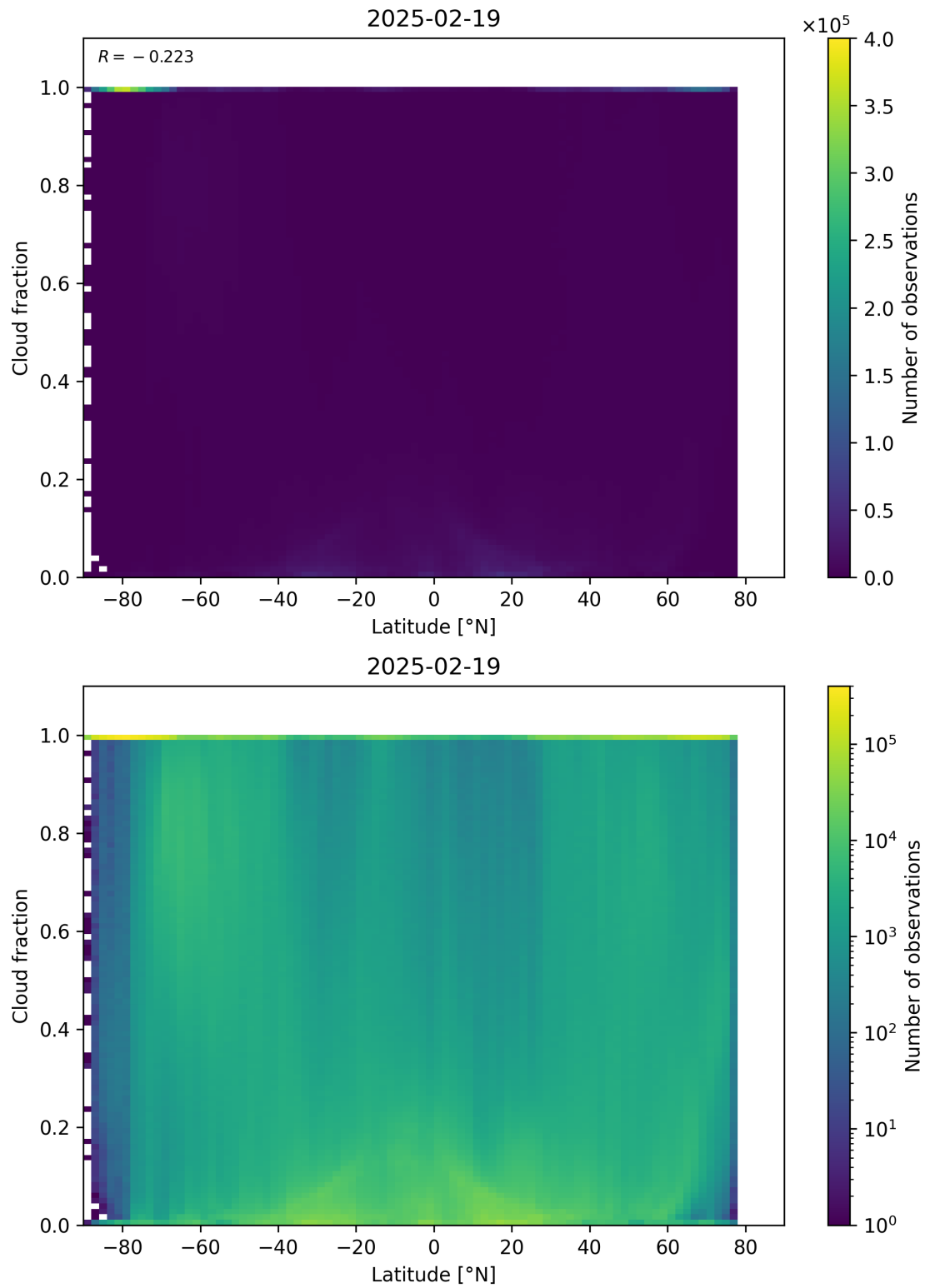
Figure 90: Scatter density plot of “Latitude” against “Cloud fraction” for 2025-02-19 to 2025-02-20.
