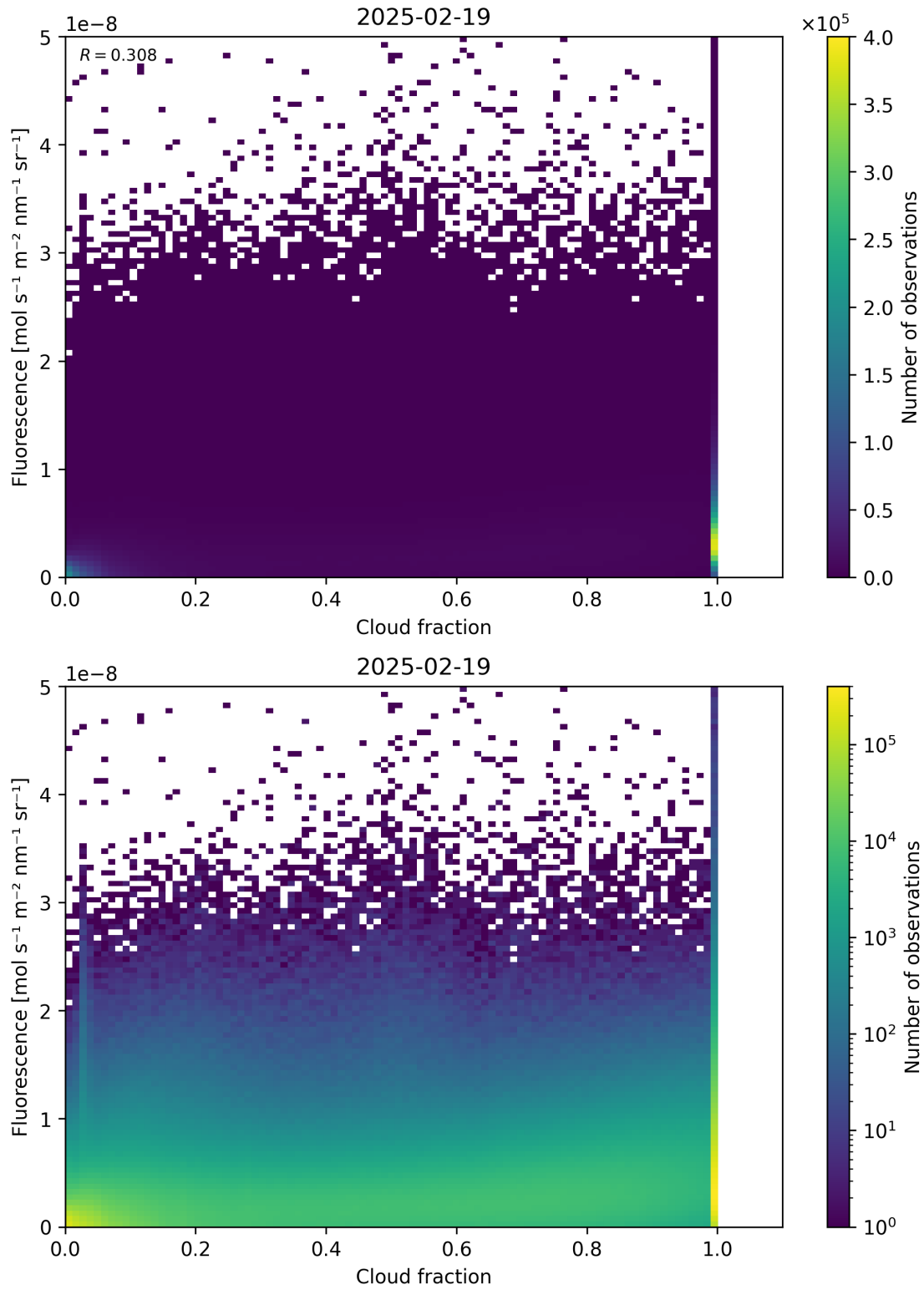
Figure 72: Scatter density plot of “Cloud fraction” against “Fluorescence” for 2025-02-19 to 2025-02-20.
