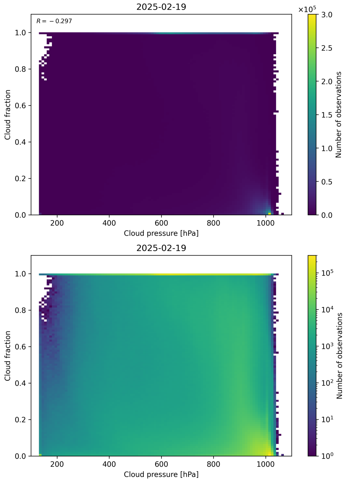
Figure 79: Scatter density plot of “Cloud pressure” against “Cloud fraction” for 2025-02-19 to 2025-02-20.
