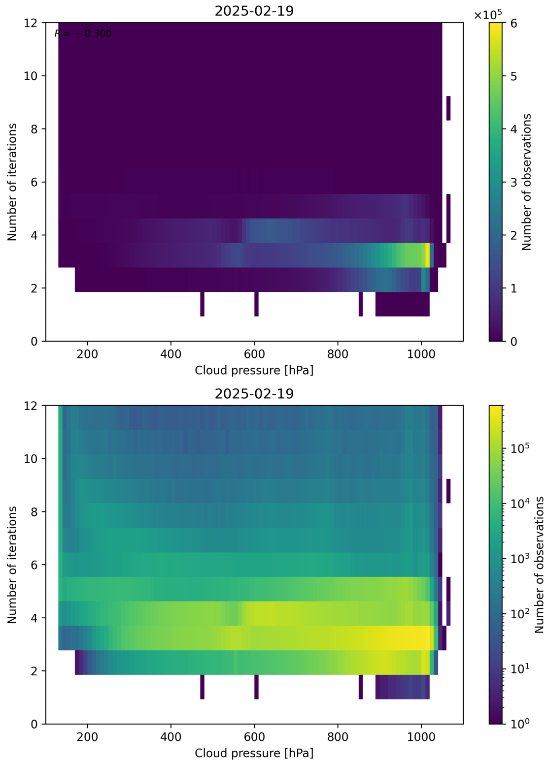
Figure 81: Scatter density plot of “Cloud pressure” against “Number of iterations” for 2025-02-19 to 2025-02-20.
