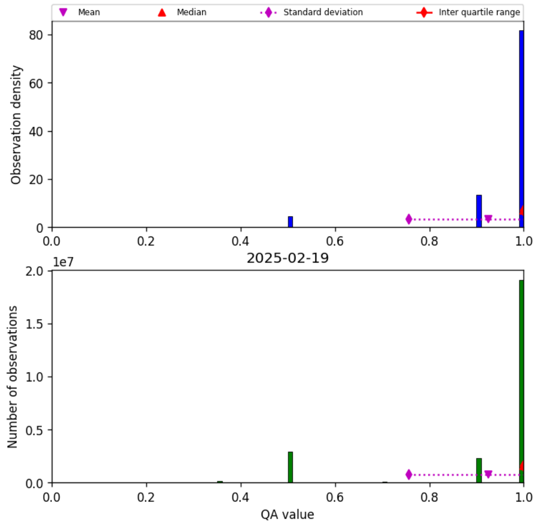
Figure 29: Histogram of “QA value” for 2025-02-19 to 2025-02-20
