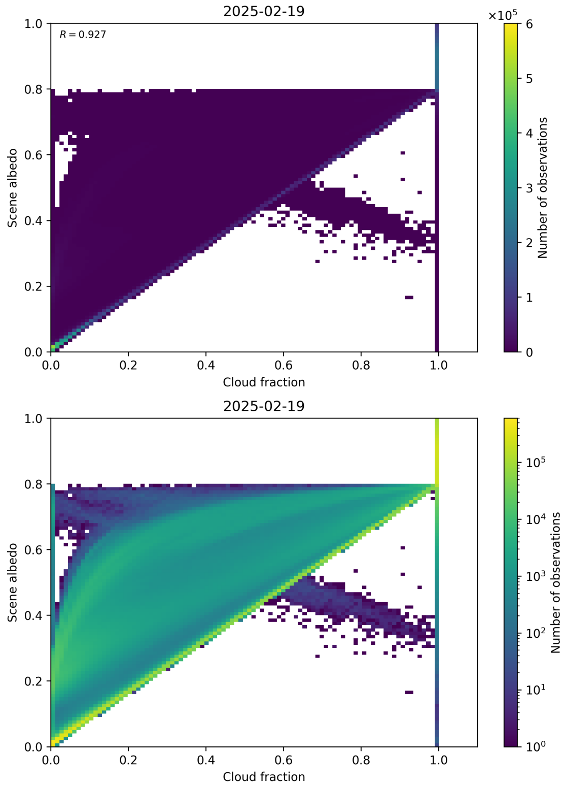
Figure 75: Scatter density plot of “Cloud fraction” against “Scene albedo” for 2025-02-19 to 2025-02-20.
