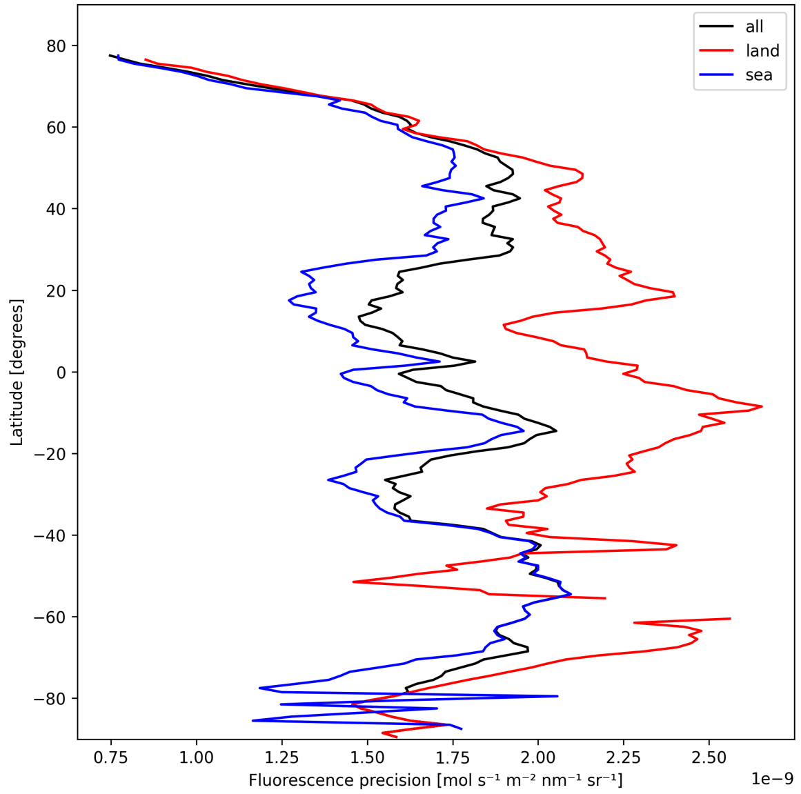
Figure 24: Zonal average of “Fluorescence precision” for 2025-02-19 to 2025-02-20.
