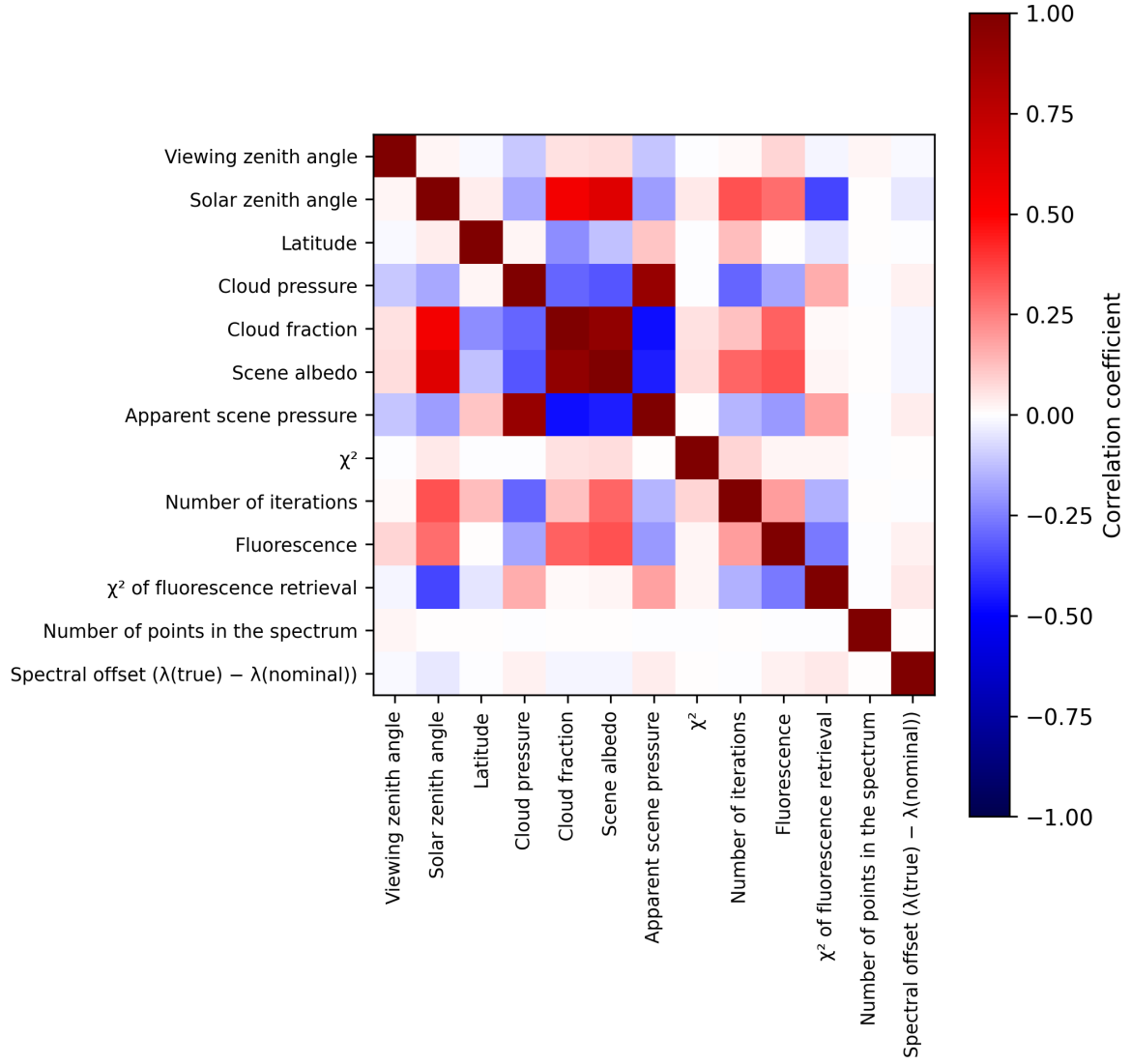
Figure 2: Map of correlation matrix for 2025-02-19 to 2025-02-20.
