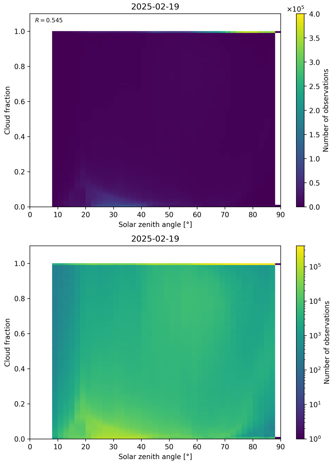
Figure 110: Scatter density plot of “Solar zenith angle” against “Cloud fraction” for 2025-02-19 to 2025-02-20.
