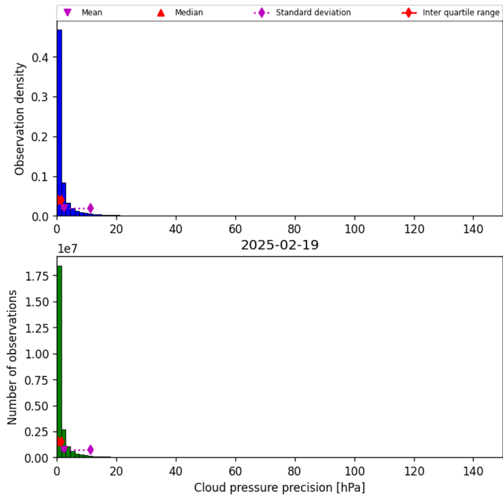
Figure 31: Histogram of “Cloud pressure precision” for 2025-02-19 to 2025-02-20
