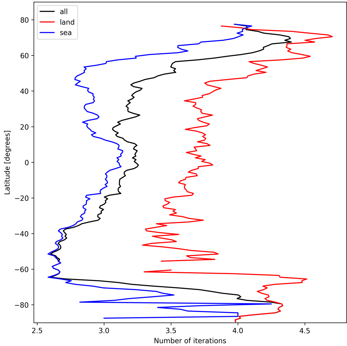
Figure 22: Zonal average of “Number of iterations” for 2025-02-19 to 2025-02-20.
