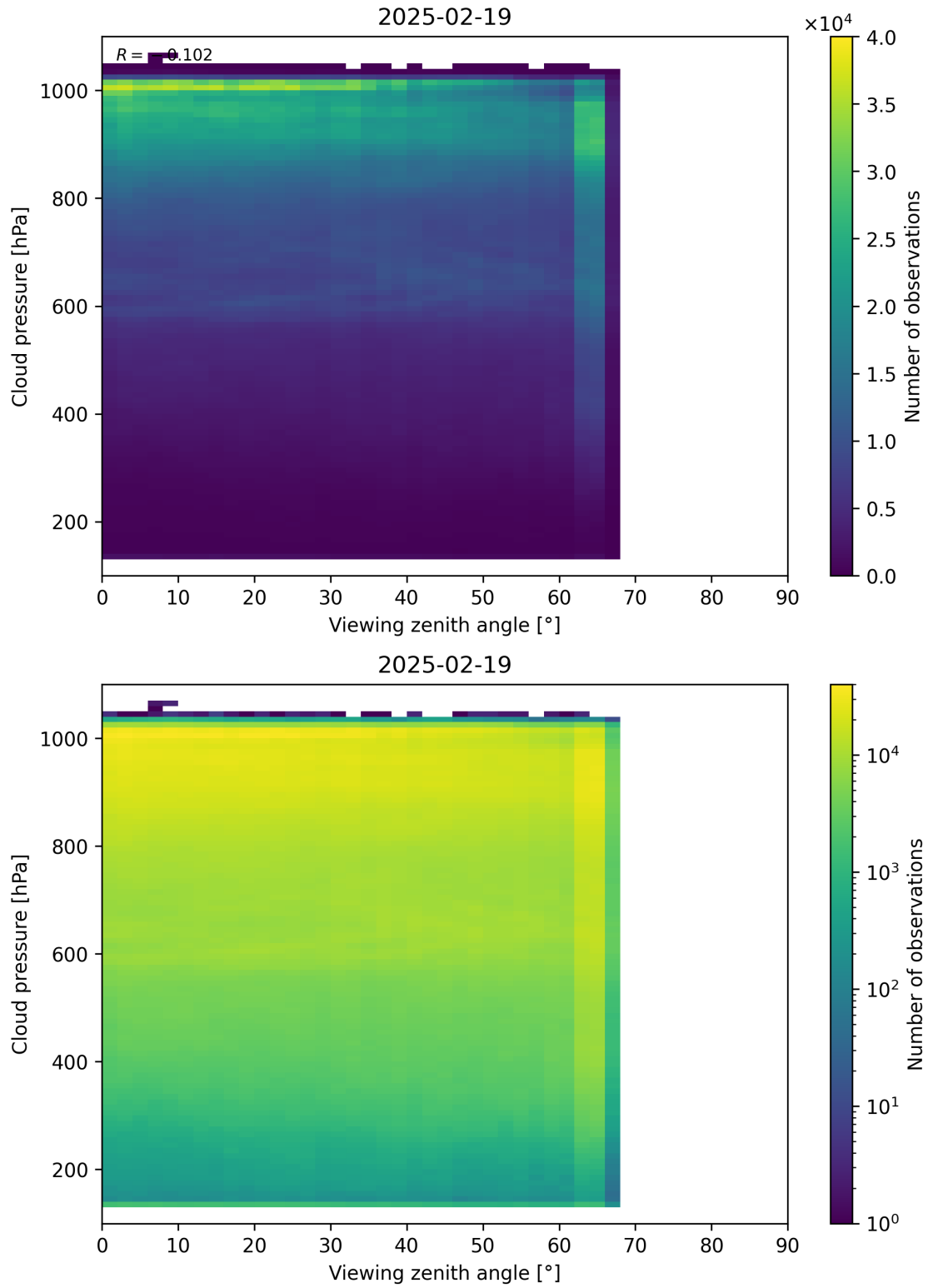
Figure 121: Scatter density plot of “Viewing zenith angle” against “Cloud pressure” for 2025-02-19 to 2025-02-20.
