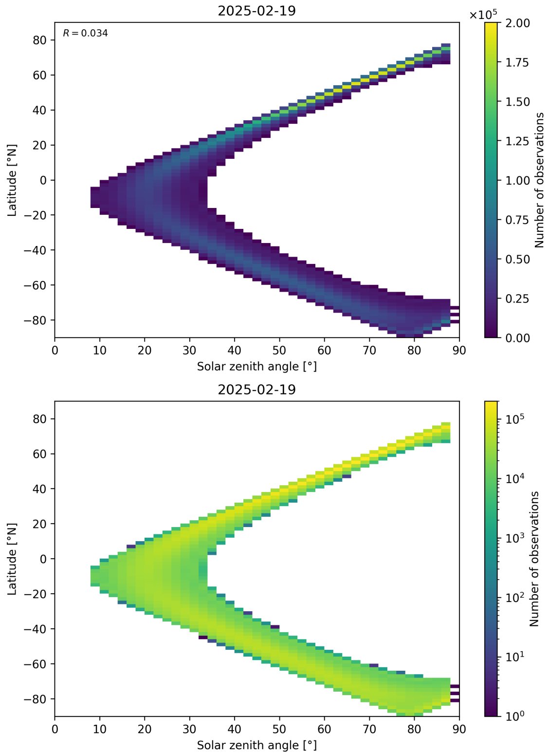
Figure 113: Scatter density plot of “Solar zenith angle” against “Latitude” for 2025-02-19 to 2025-02-20.
