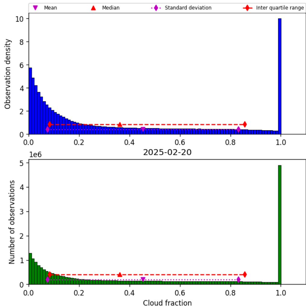
Figure 32: Histogram of “Cloud fraction” for 2025-02-19 to 2025-02-21
