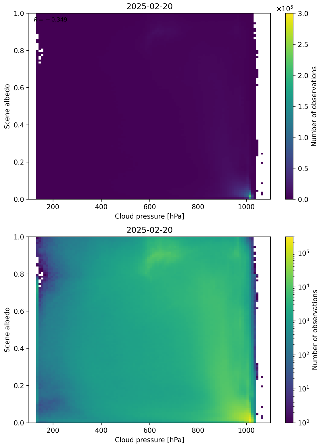
Figure 83: Scatter density plot of “Cloud pressure” against “Scene albedo” for 2025-02-19 to 2025-02-21.
