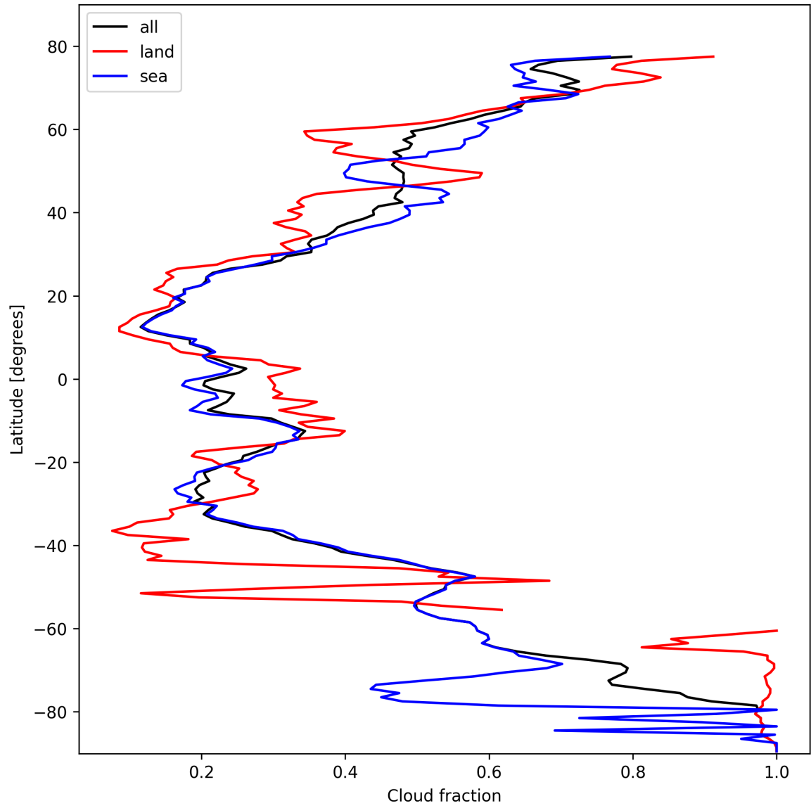
Figure 15: Zonal average of “Cloud fraction” for 2025-02-19 to 2025-02-21.
