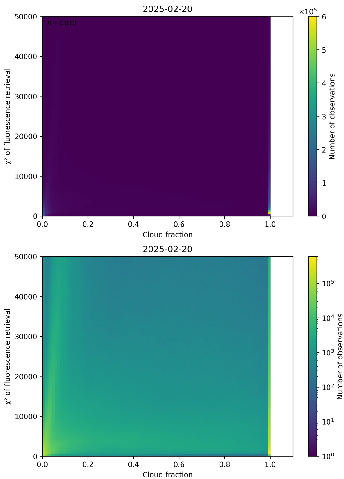
Figure 71: Scatter density plot of “Cloud fraction” against “ \chi^2 of fluorescence retrieval” for 2025-02-19 to 2025-02-21.
