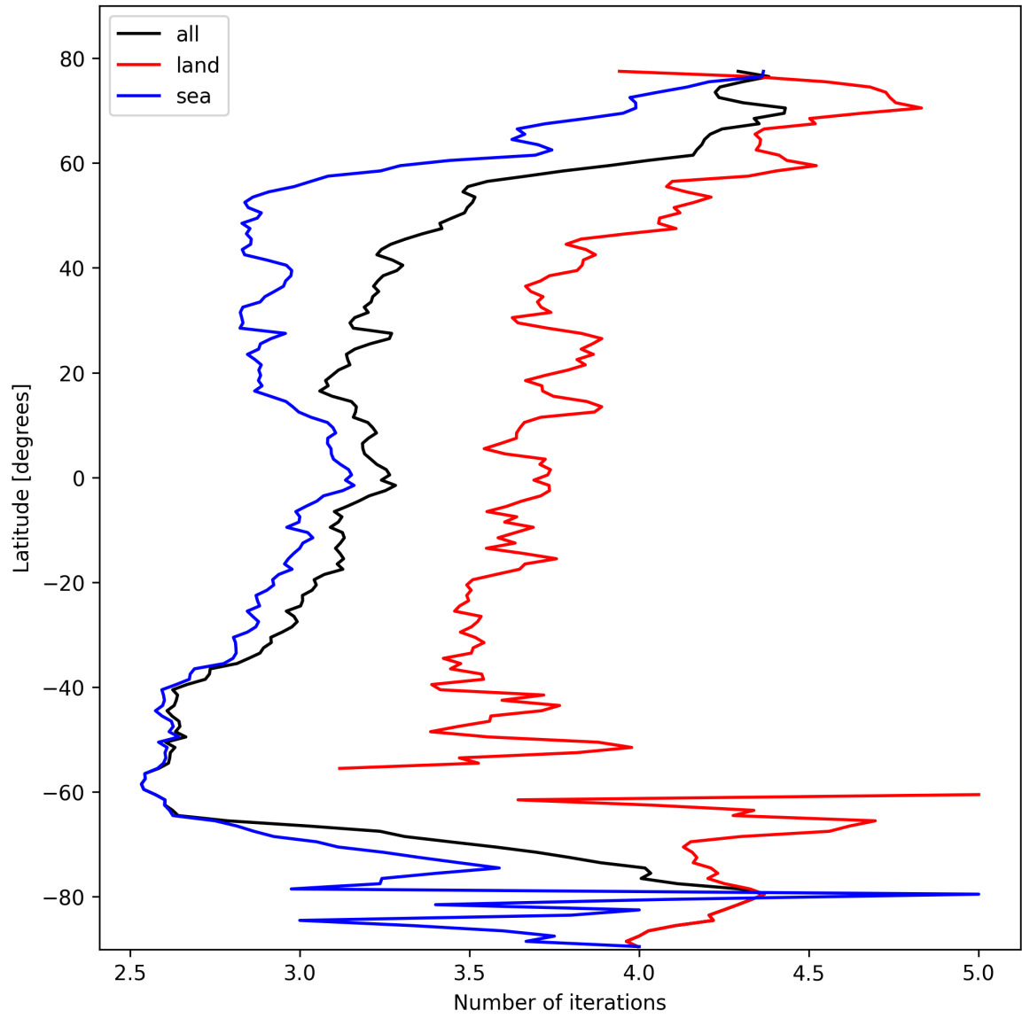
Figure 22: Zonal average of “Number of iterations” for 2025-02-19 to 2025-02-21.
