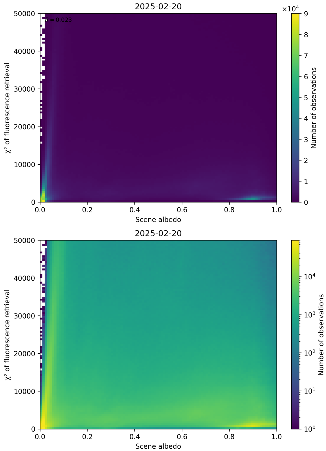
Figure 103: Scatter density plot of “Scene albedo” against “ \chi^2 of fluorescence retrieval” for 2025-02-19 to 2025-02-21.
