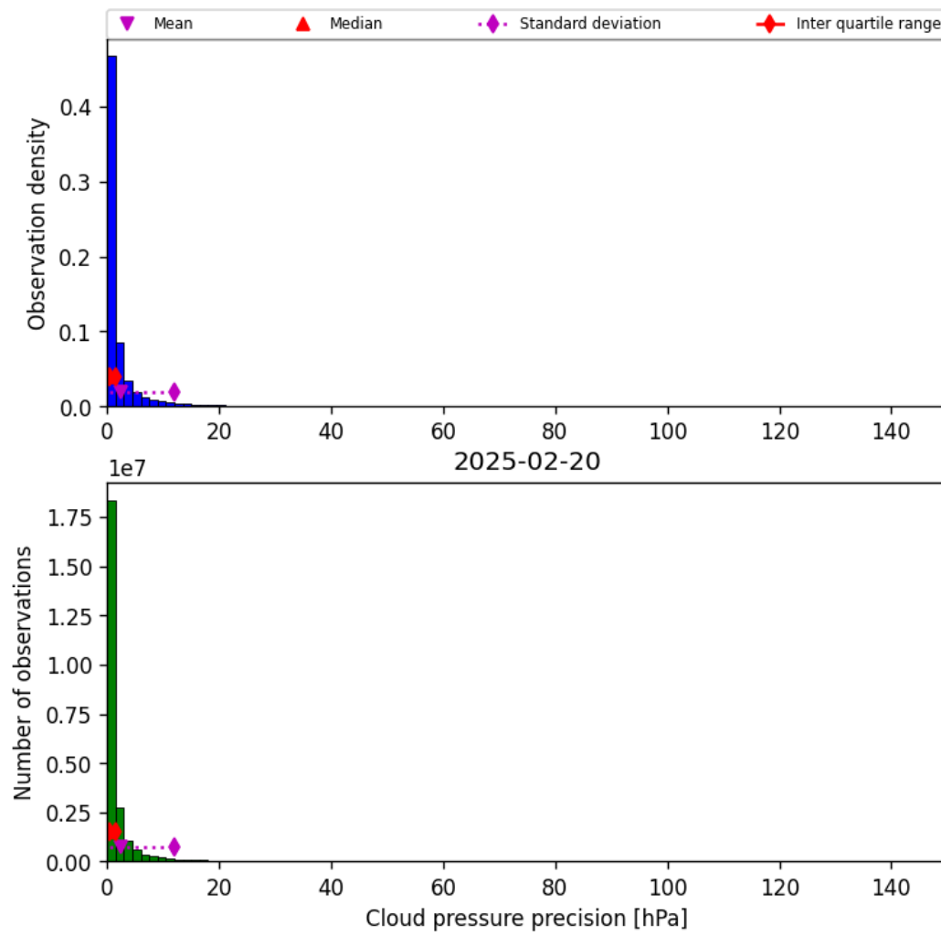
Figure 31: Histogram of “Cloud pressure precision” for 2025-02-19 to 2025-02-21
