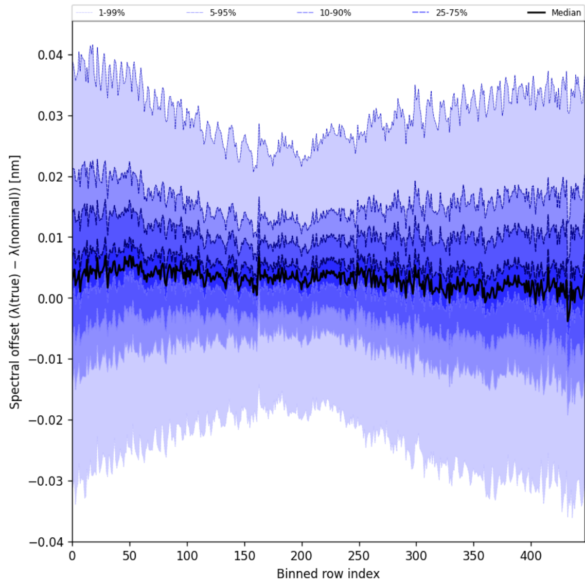
Figure 62: Along track statistics of “Spectral offset ( \lambda_{\text{true}} - \lambda_{\text{nominal}} )” for 2025-02-19 to 2025-02-21
