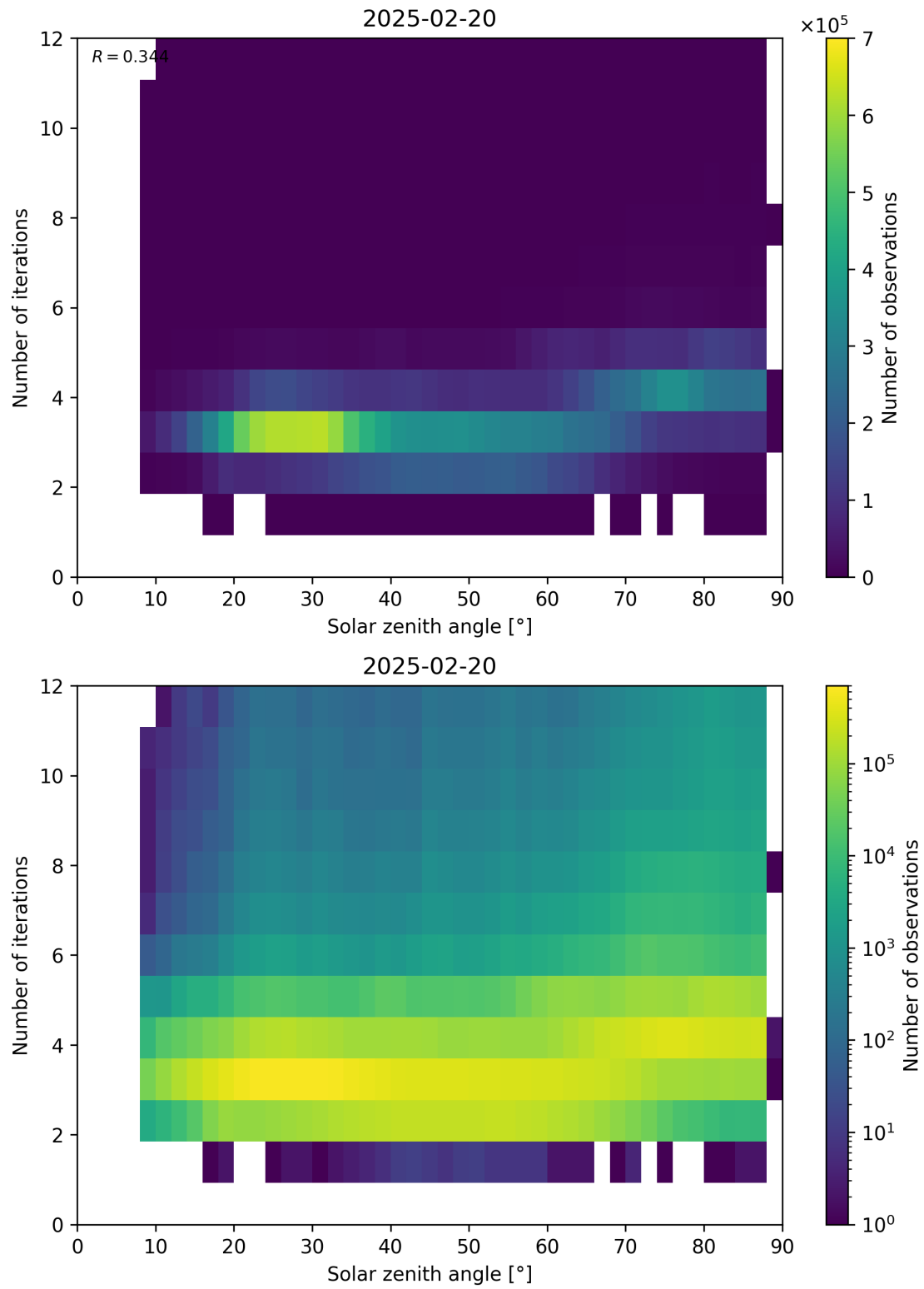
Figure 114: Scatter density plot of “Solar zenith angle” against “Number of iterations” for 2025-02-19 to 2025-02-21.
