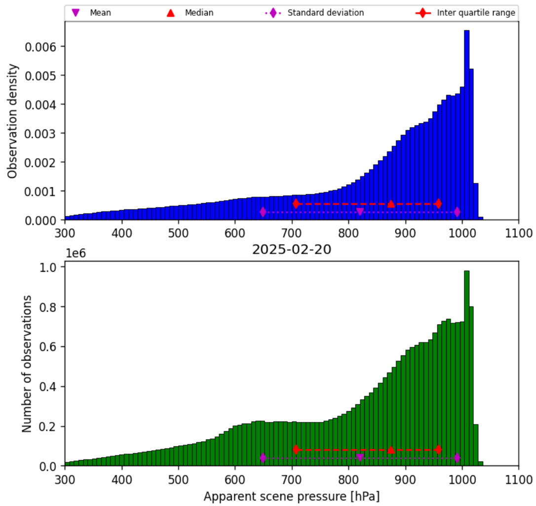
Figure 36: Histogram of “Apparent scene pressure” for 2025-02-19 to 2025-02-21
