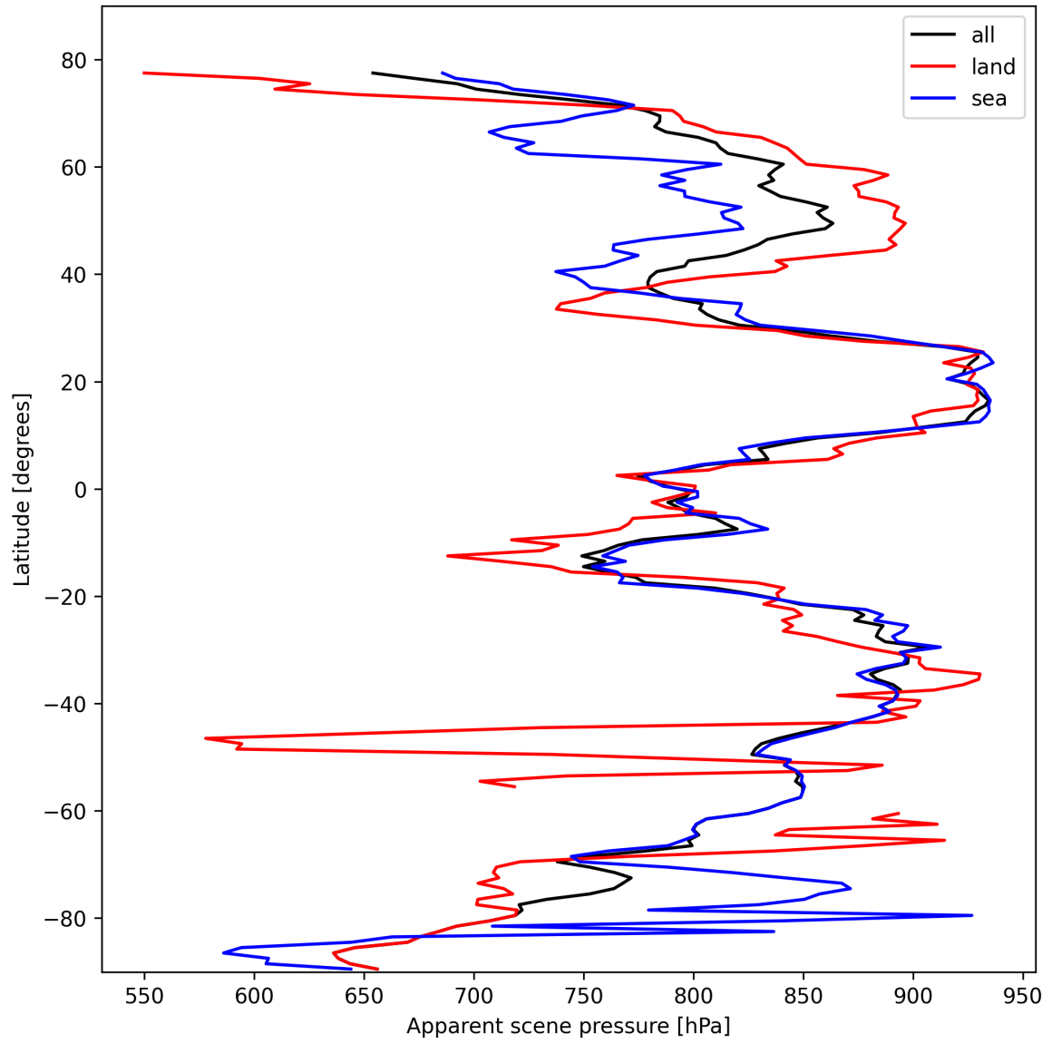
Figure 19: Zonal average of “Apparent scene pressure” for 2025-02-19 to 2025-02-21.
