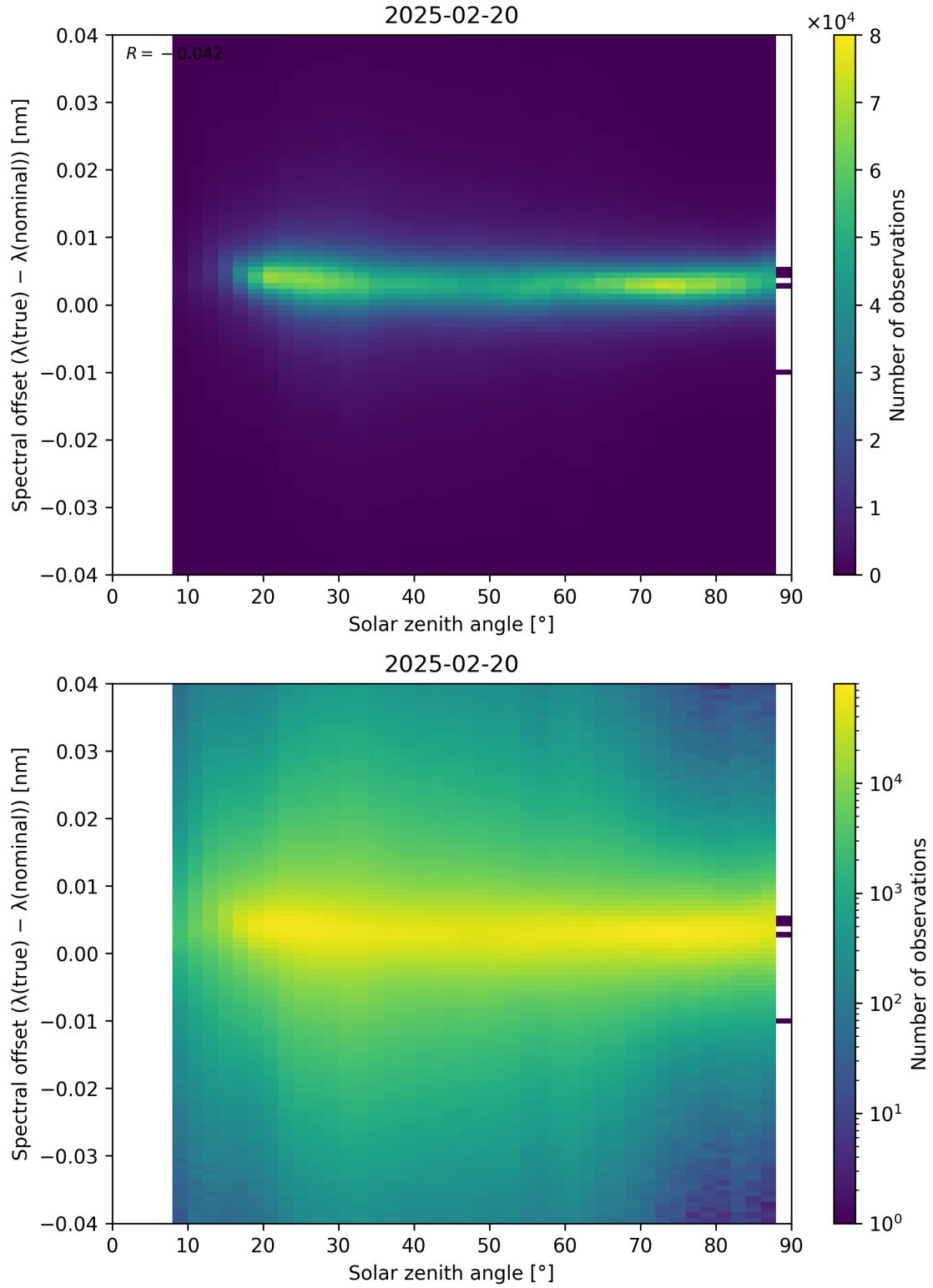
Figure 117: Scatter density plot of “Solar zenith angle” against “Spectral offset ( \lambda_{\text{true}} - \lambda_{\text{nominal}} )” for 2025-02-19 to 2025-02-21.
