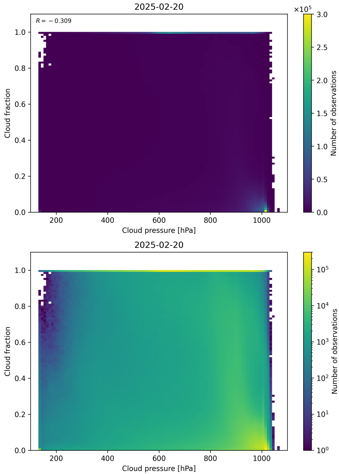
Figure 79: Scatter density plot of “Cloud pressure” against “Cloud fraction” for 2025-02-19 to 2025-02-21.
