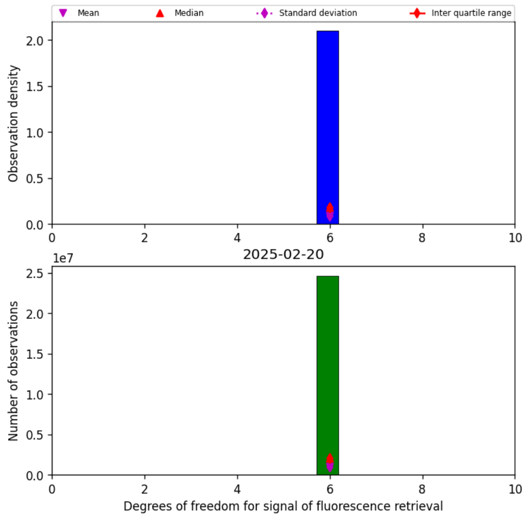
Figure 43: Histogram of “Degrees of freedom for signal of fluorescence retrieval” for 2025-02-19 to 2025-02-21
