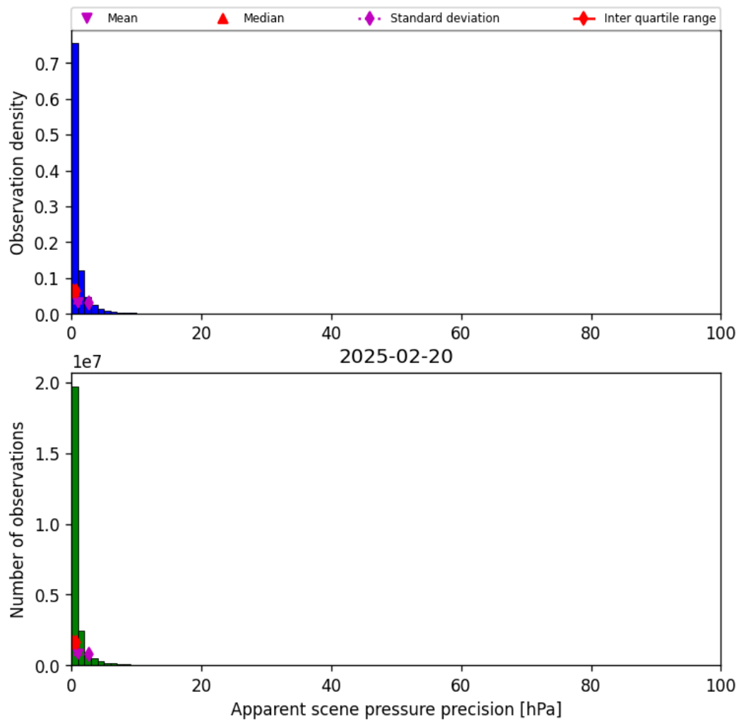
Figure 37: Histogram of “Apparent scene pressure precision” for 2025-02-19 to 2025-02-21
