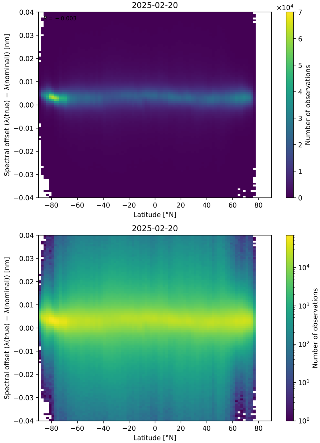
Figure 96: Scatter density plot of “Latitude” against “Spectral offset ( \lambda_{\text{true}} - \lambda_{\text{nominal}} )” for 2025-02-19 to 2025-02-21.
