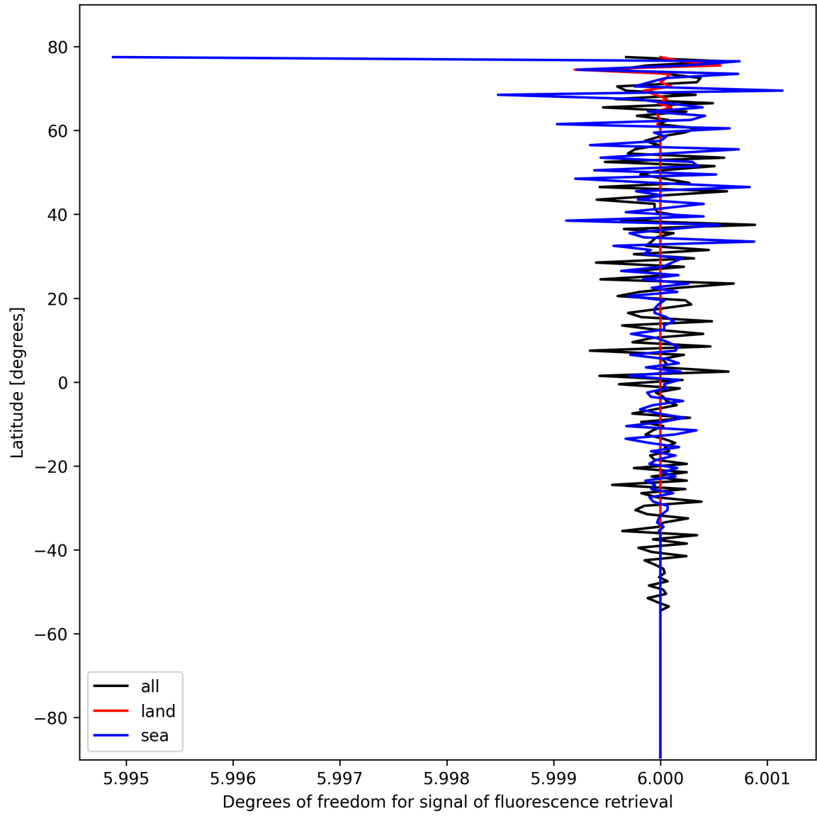
Figure 26: Zonal average of “Degrees of freedom for signal of fluorescence retrieval” for 2025-02-19 to 2025-02-21.
