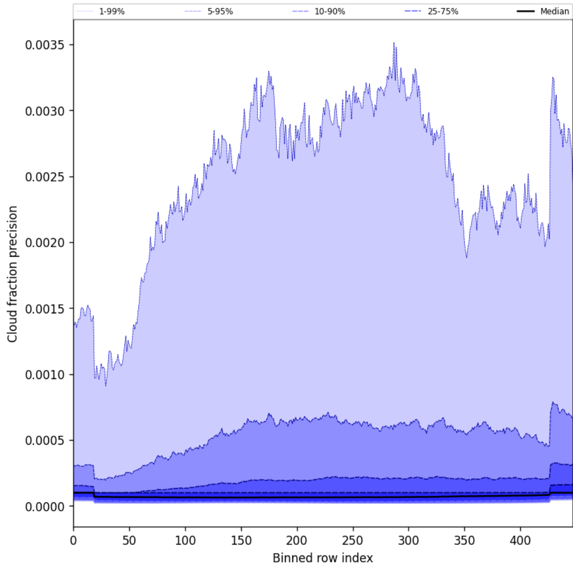
Figure 50: Along track statistics of “Cloud fraction precision” for 2025-02-19 to 2025-02-21
