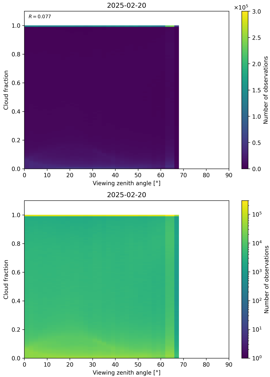
Figure 120: Scatter density plot of “Viewing zenith angle” against “Cloud fraction” for 2025-02-19 to 2025-02-21.
