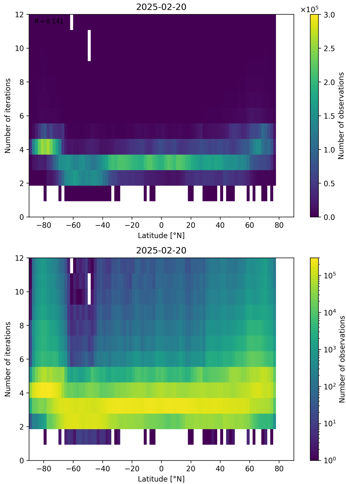
Figure 93: Scatter density plot of “Latitude” against “Number of iterations” for 2025-02-19 to 2025-02-21.
