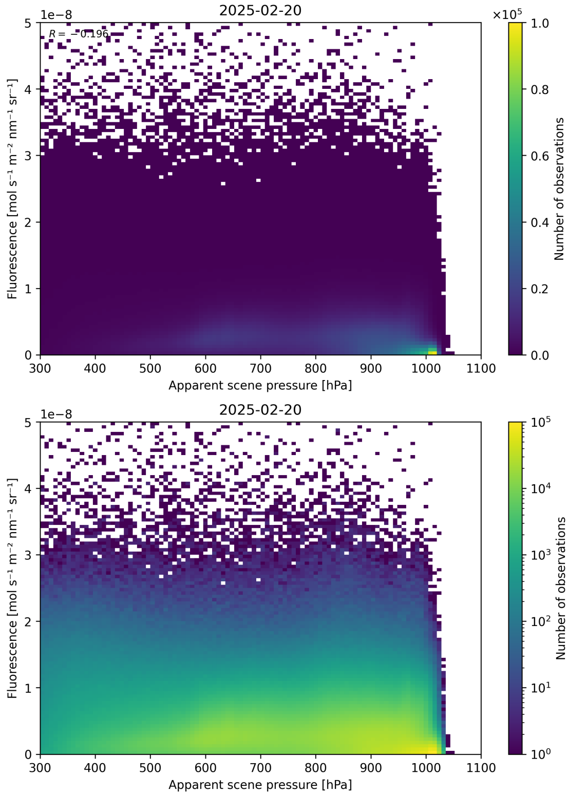
Figure 64: Scatter density plot of “Apparent scene pressure” against “Fluorescence” for 2025-02-19 to 2025-02-21.
