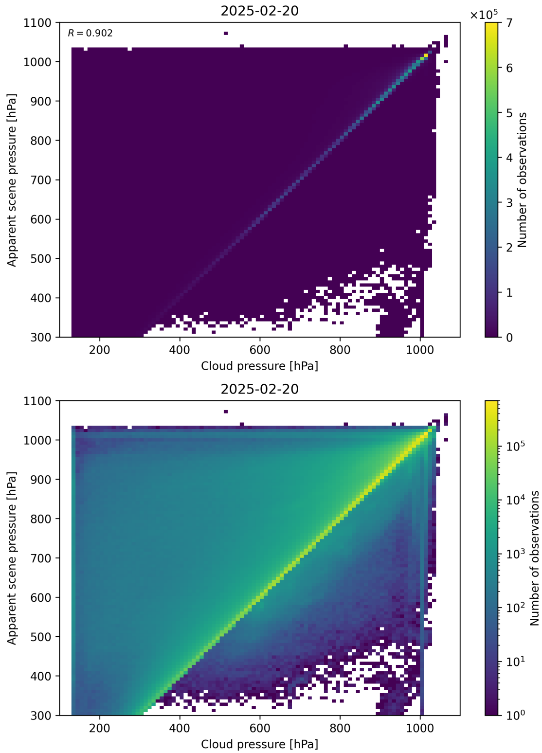
Figure 77: Scatter density plot of “Cloud pressure” against “Apparent scene pressure” for 2025-02-19 to 2025-02-21.
