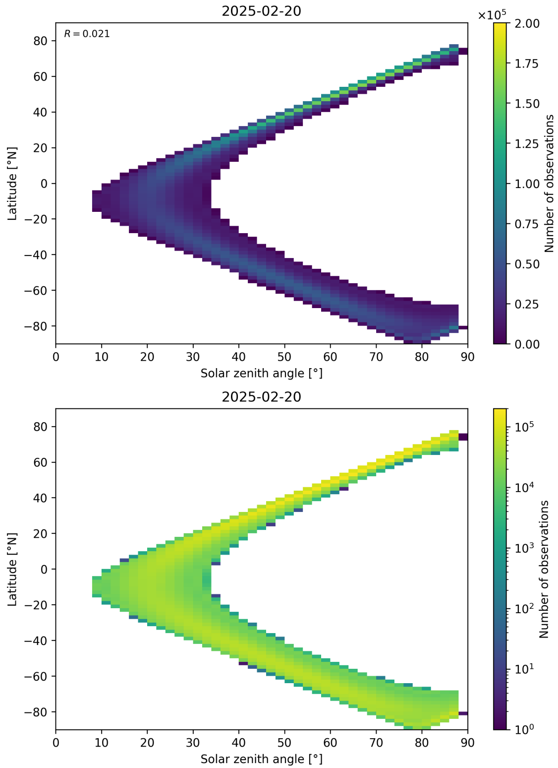
Figure 113: Scatter density plot of “Solar zenith angle” against “Latitude” for 2025-02-19 to 2025-02-21.
