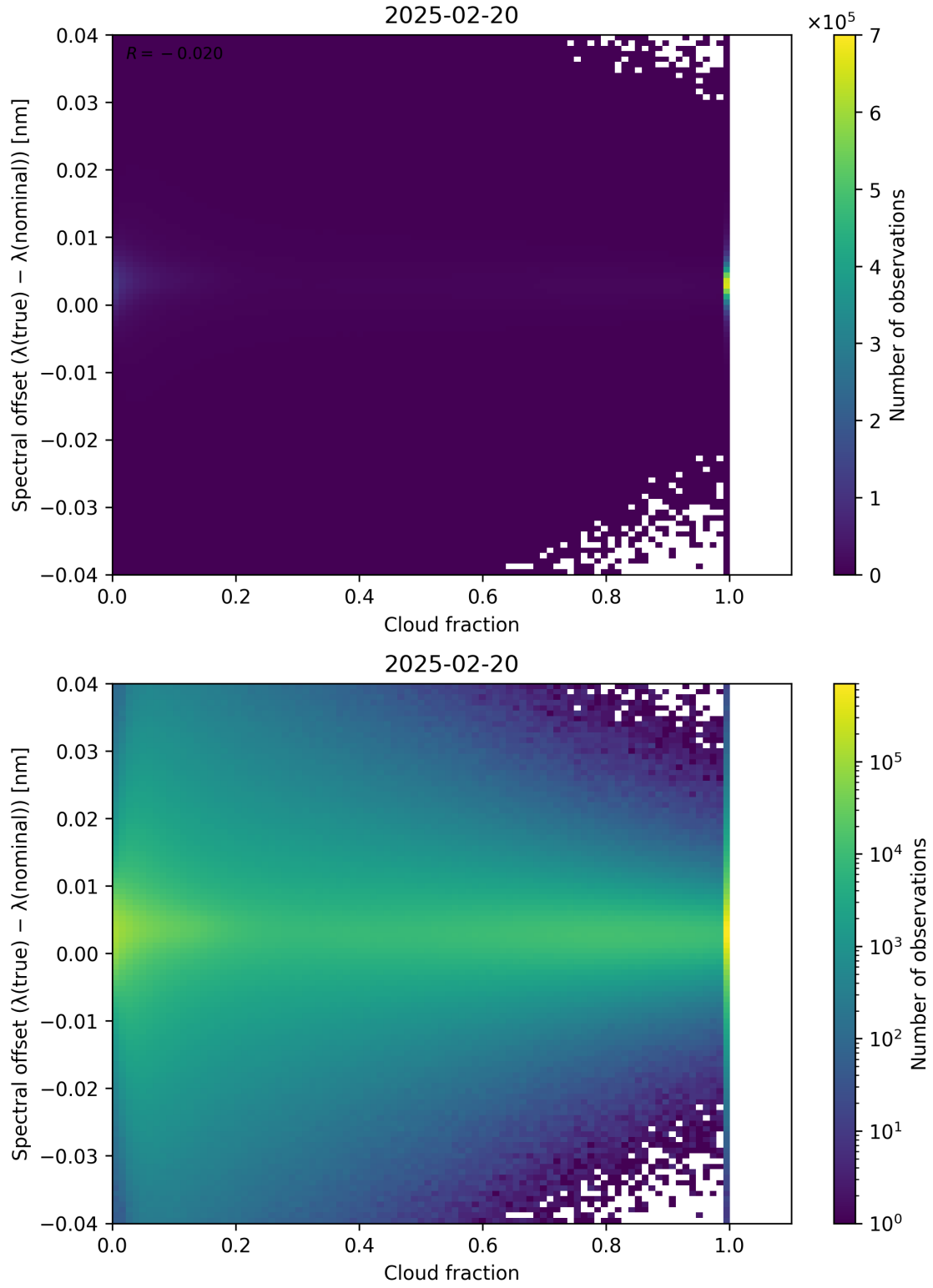
Figure 76: Scatter density plot of “Cloud fraction” against “Spectral offset ( \lambda_{\text{true}} - \lambda_{\text{nominal}} )” for 2025-02-19 to 2025-02-21.
