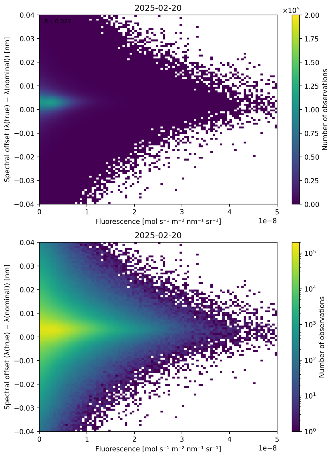
Figure 87: Scatter density plot of “Fluorescence” against “Spectral offset ( \lambda_{\text{true}} - \lambda_{\text{nominal}} )” for 2025-02-19 to 2025-02-21.
