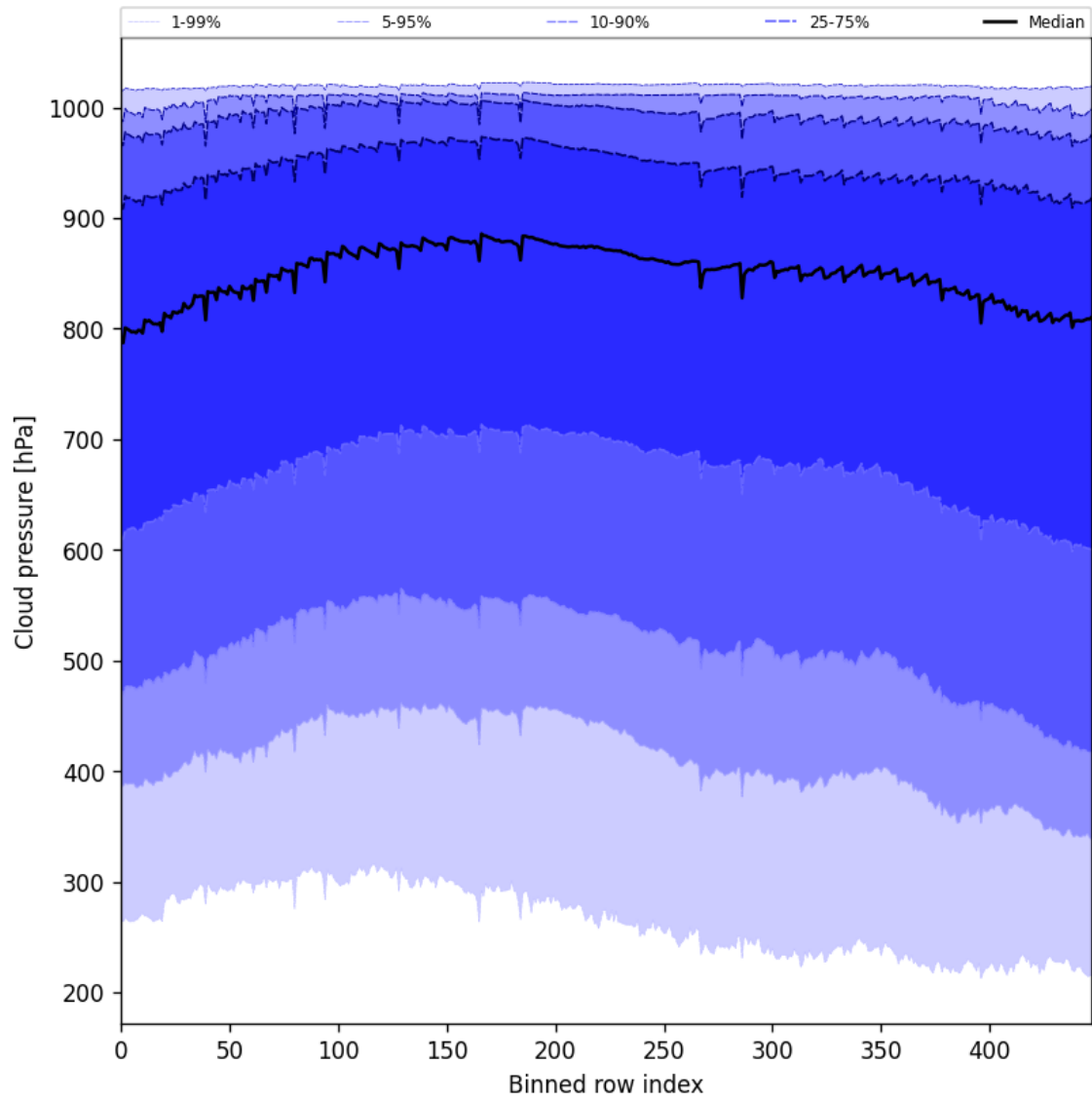
Figure 47: Along track statistics of “Cloud pressure” for 2025-02-19 to 2025-02-21
