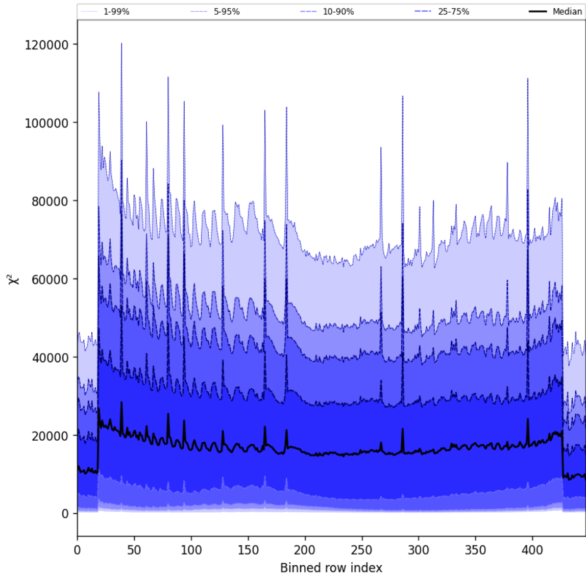
Figure 55: Along track statistics of “ \chi^2 ” for 2025-02-19 to 2025-02-21
