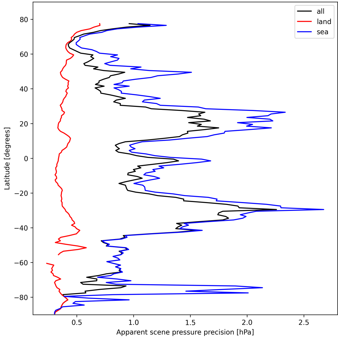
Figure 20: Zonal average of “Apparent scene pressure precision” for 2025-02-19 to 2025-02-21.
