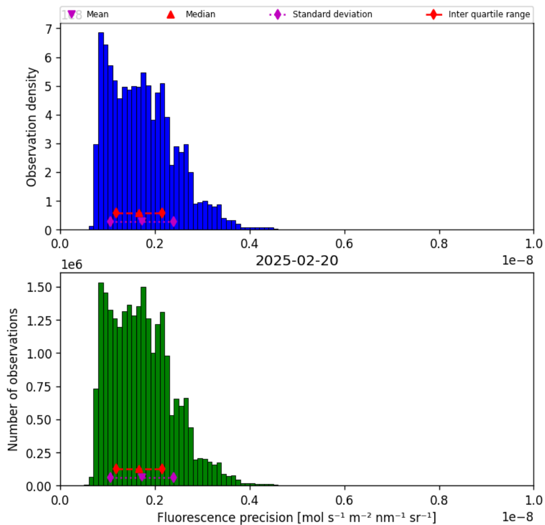
Figure 41: Histogram of “Fluorescence precision” for 2025-02-19 to 2025-02-21
