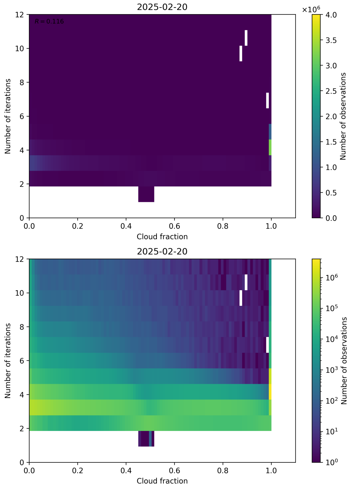
Figure 73: Scatter density plot of “Cloud fraction” against “Number of iterations” for 2025-02-19 to 2025-02-21.
