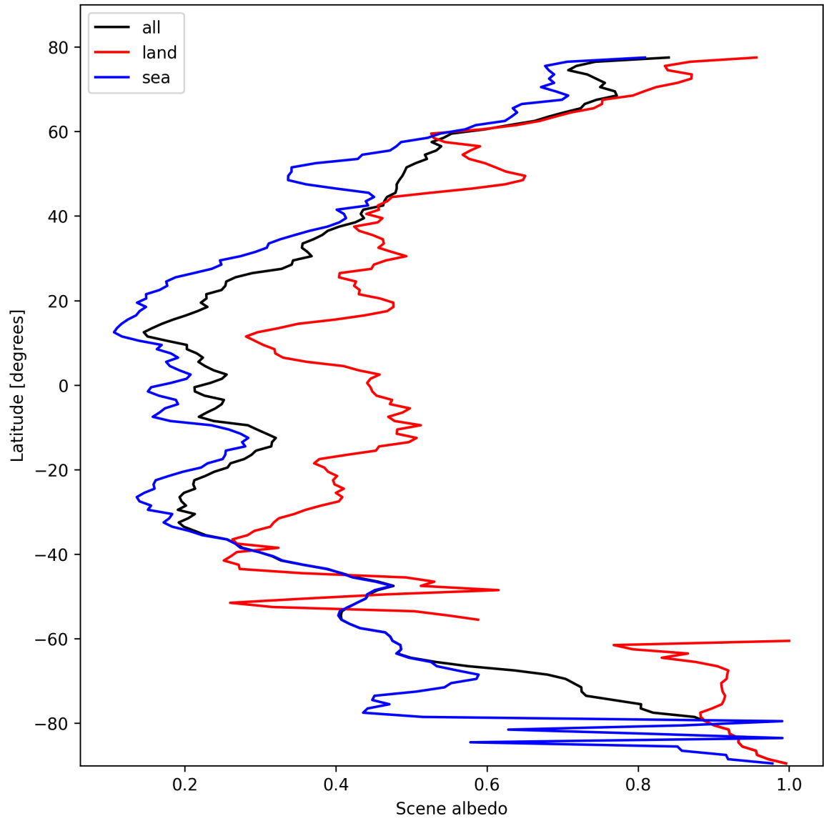
Figure 17: Zonal average of “Scene albedo” for 2025-02-19 to 2025-02-21.
