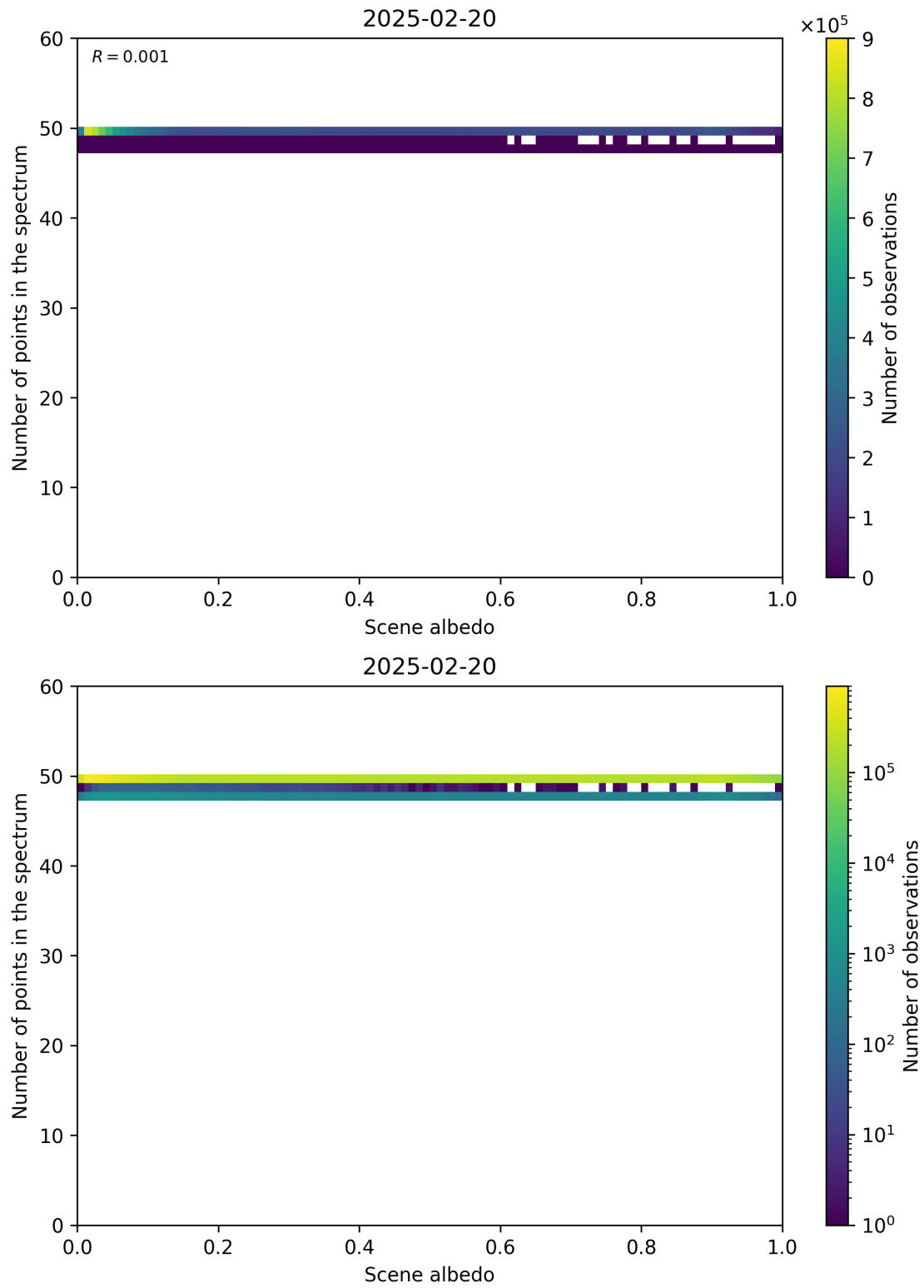
Figure 106: Scatter density plot of “Scene albedo” against “Number of points in the spectrum” for 2025-02-19 to 2025-02-21.
