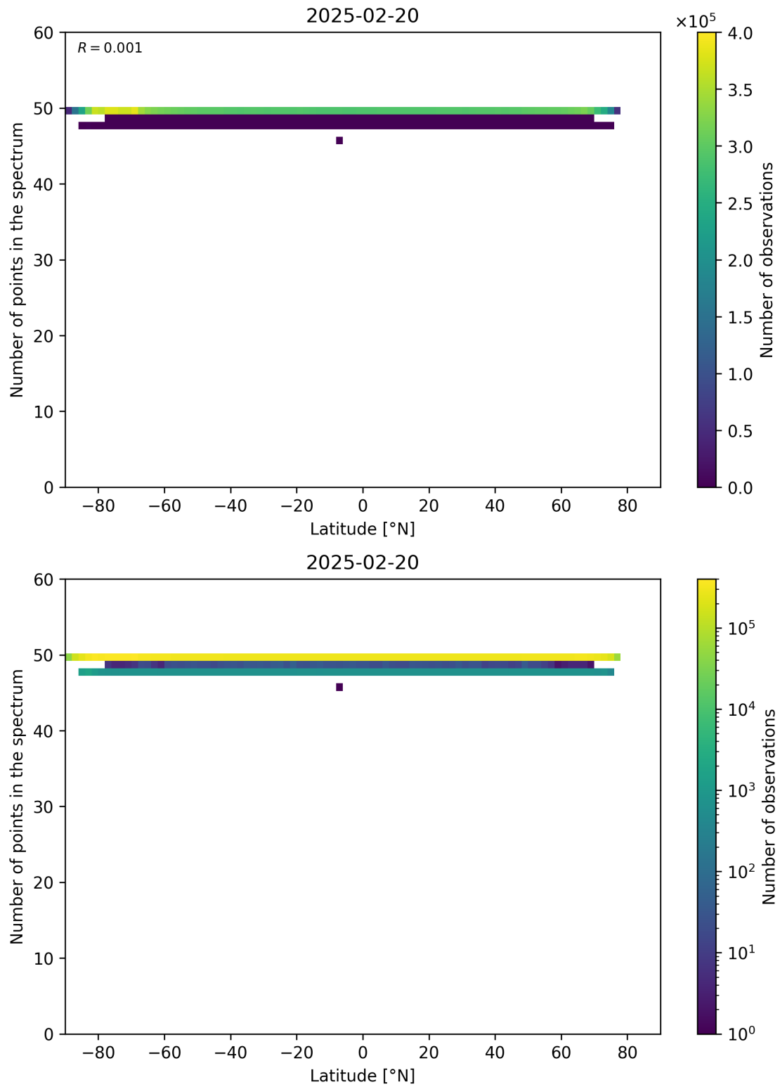
Figure 94: Scatter density plot of “Latitude” against “Number of points in the spectrum” for 2025-02-19 to 2025-02-21.
