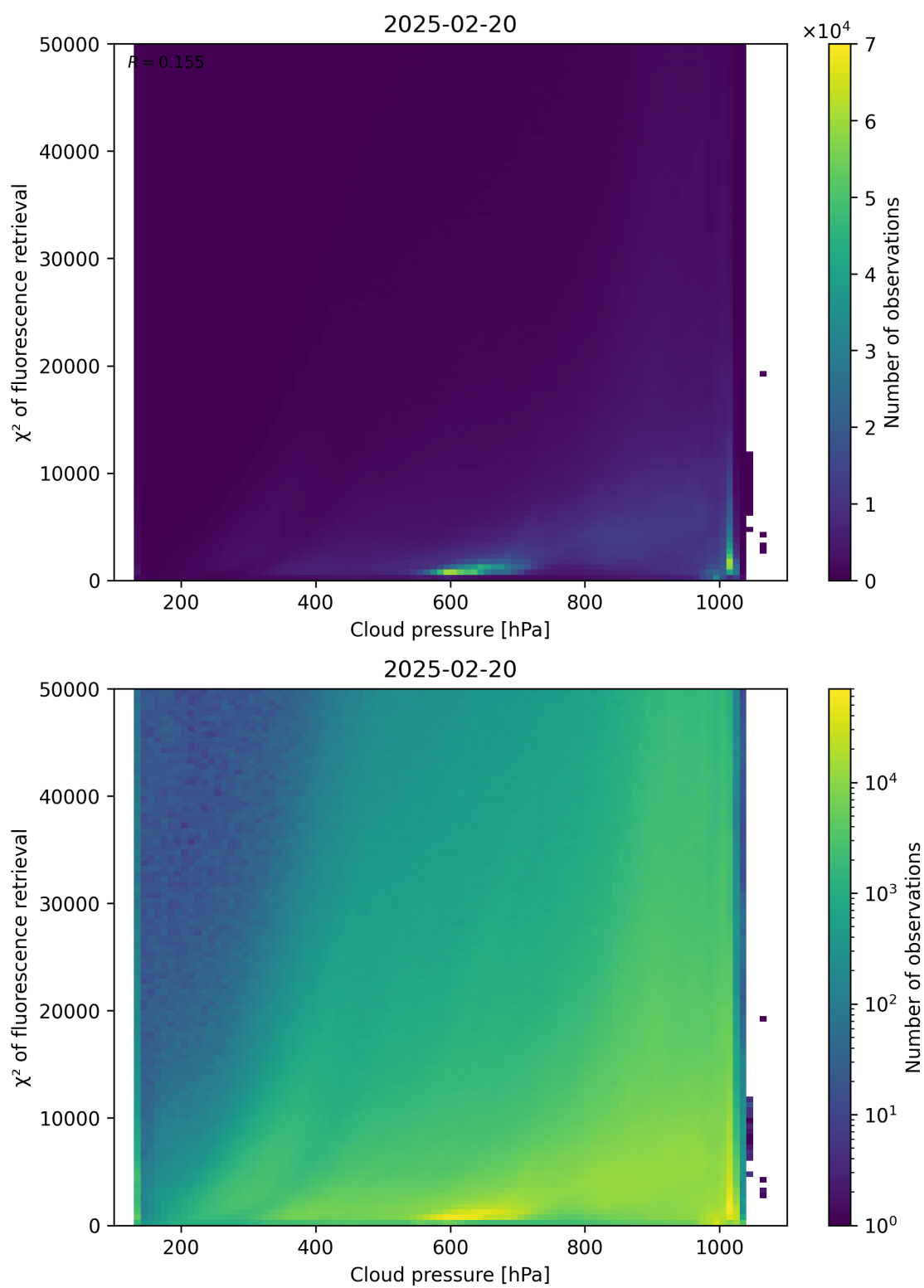
Figure 78: Scatter density plot of “Cloud pressure” against “ \chi^2 of fluorescence retrieval” for 2025-02-19 to 2025-02-21.
