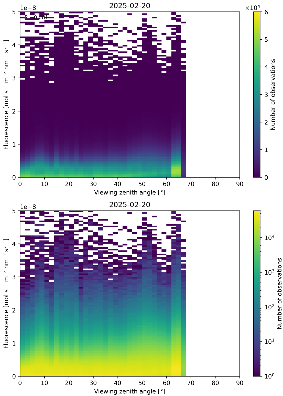
Figure 122: Scatter density plot of “Viewing zenith angle” against “Fluorescence” for 2025-02-19 to 2025-02-21.
