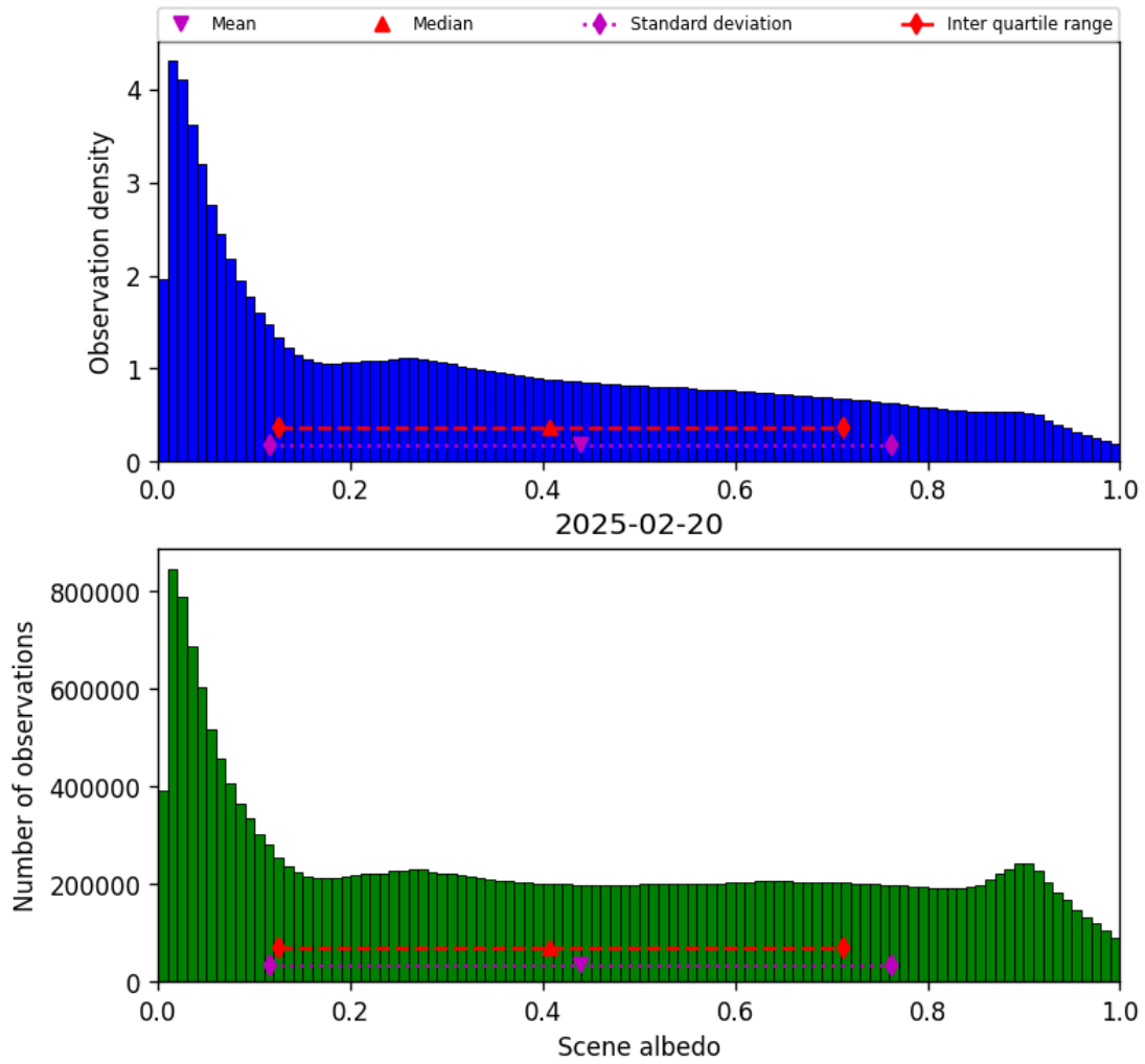
Figure 34: Histogram of “Scene albedo” for 2025-02-19 to 2025-02-21
