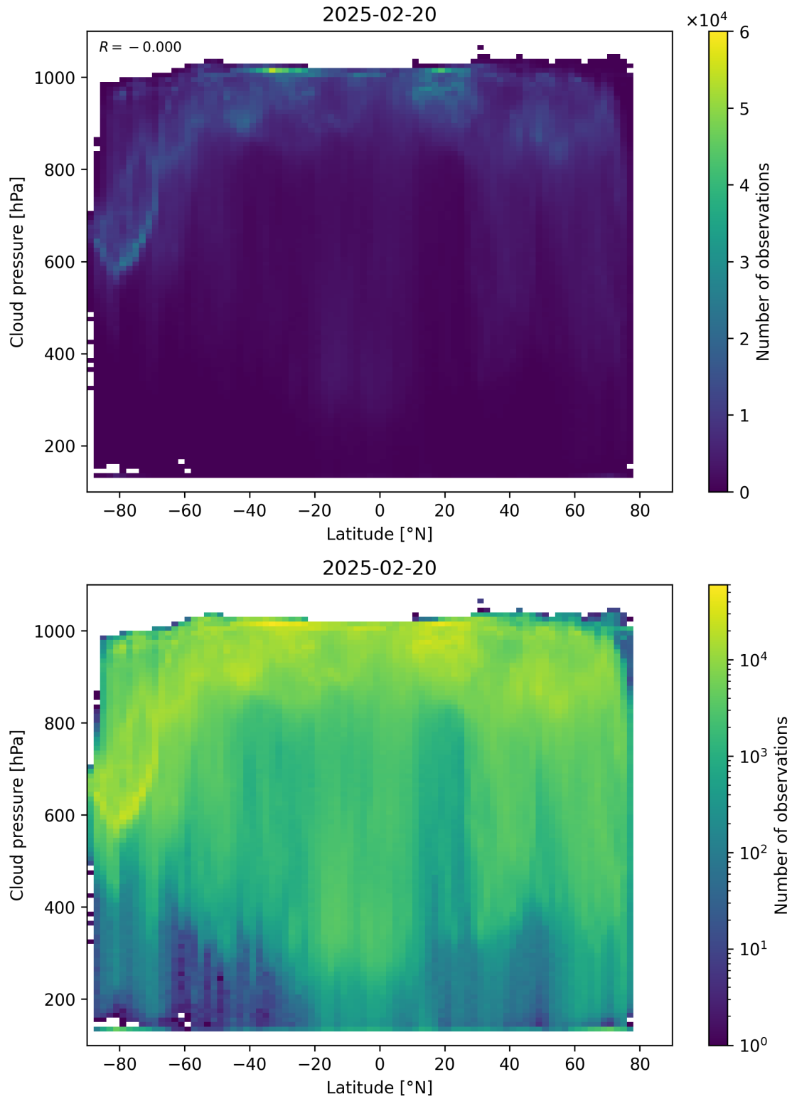
Figure 91: Scatter density plot of “Latitude” against “Cloud pressure” for 2025-02-19 to 2025-02-21.
