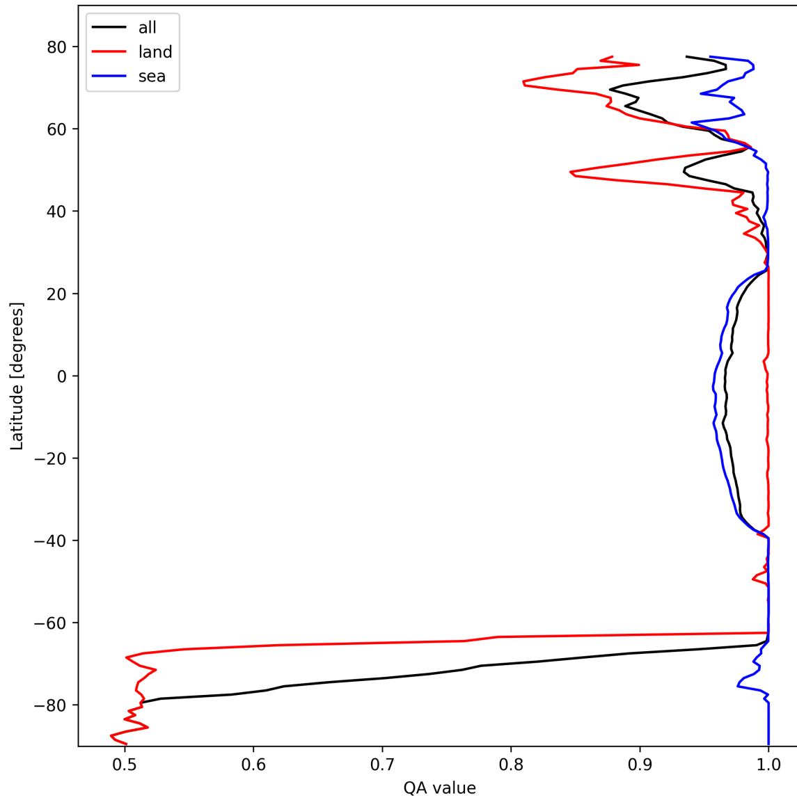
Figure 12: Zonal average of “QA value” for 2025-02-19 to 2025-02-21.
