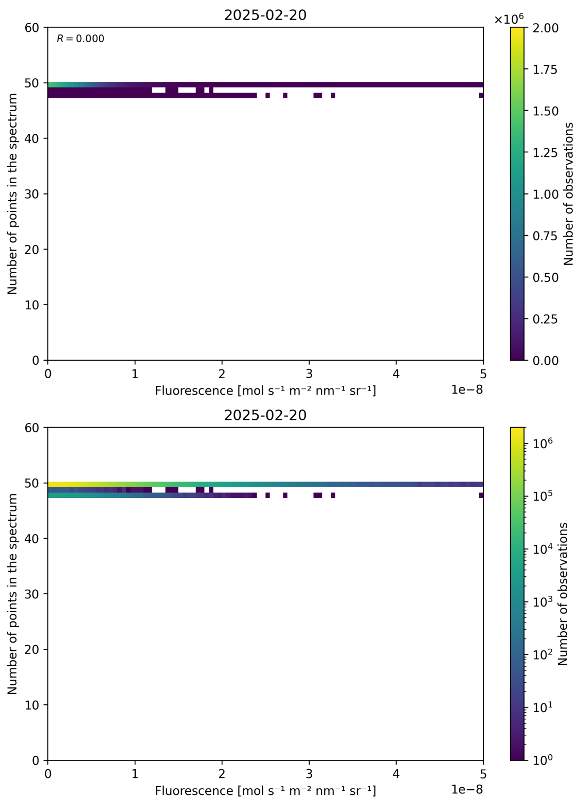
Figure 86: Scatter density plot of “Fluorescence” against “Number of points in the spectrum” for 2025-02-19 to 2025-02-21.
