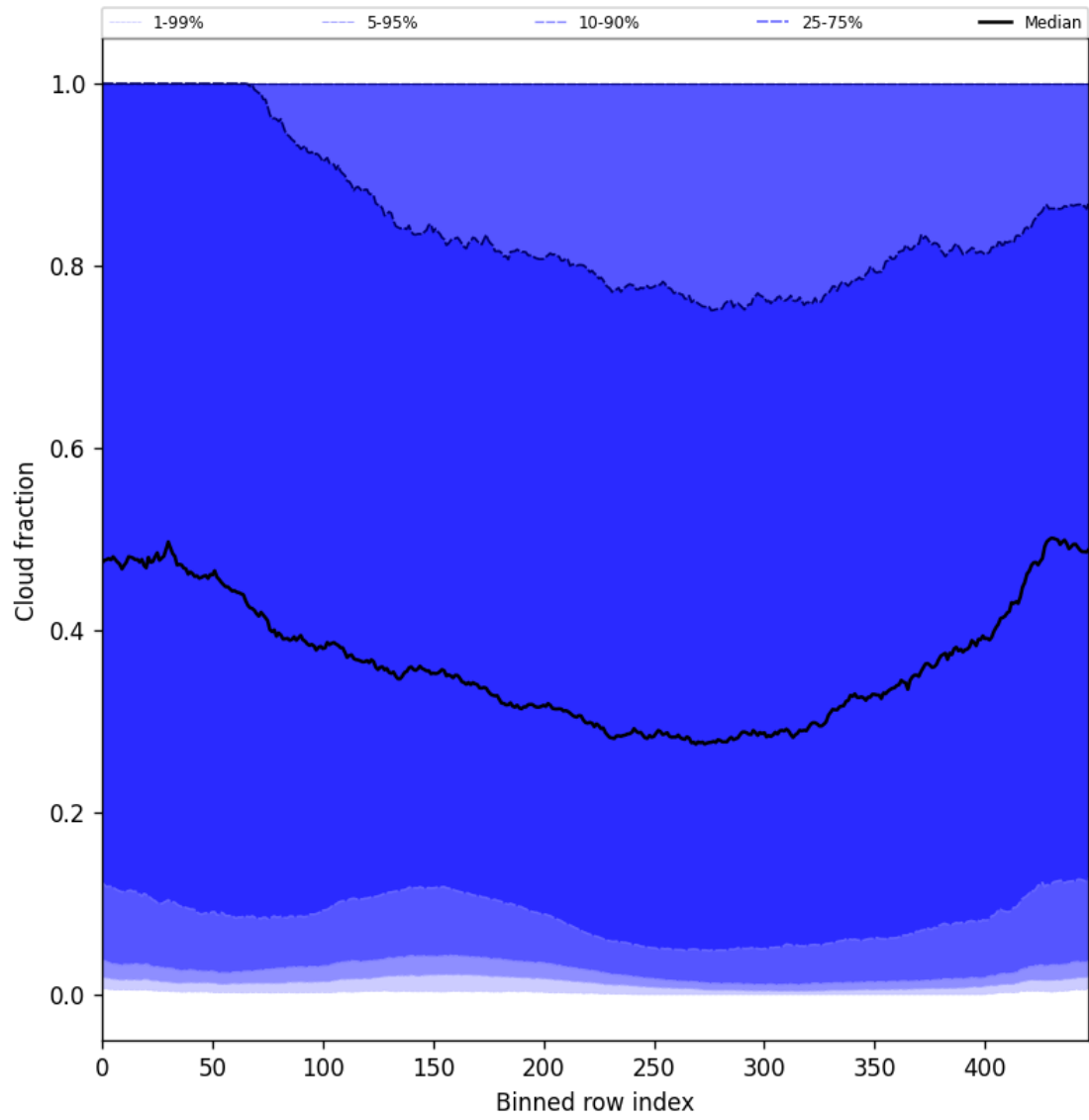
Figure 49: Along track statistics of “Cloud fraction” for 2025-02-19 to 2025-02-21
