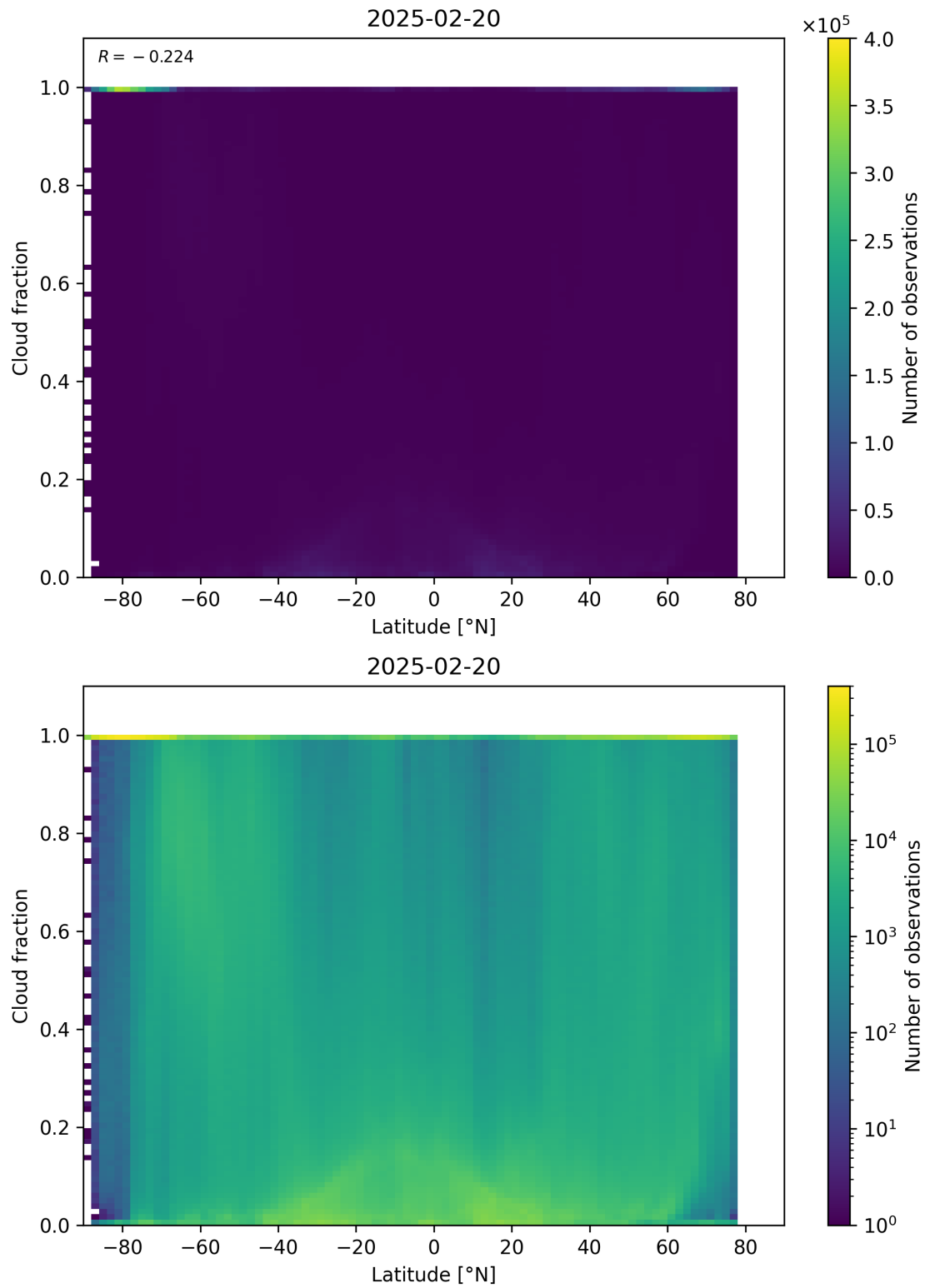
Figure 90: Scatter density plot of “Latitude” against “Cloud fraction” for 2025-02-19 to 2025-02-21.
