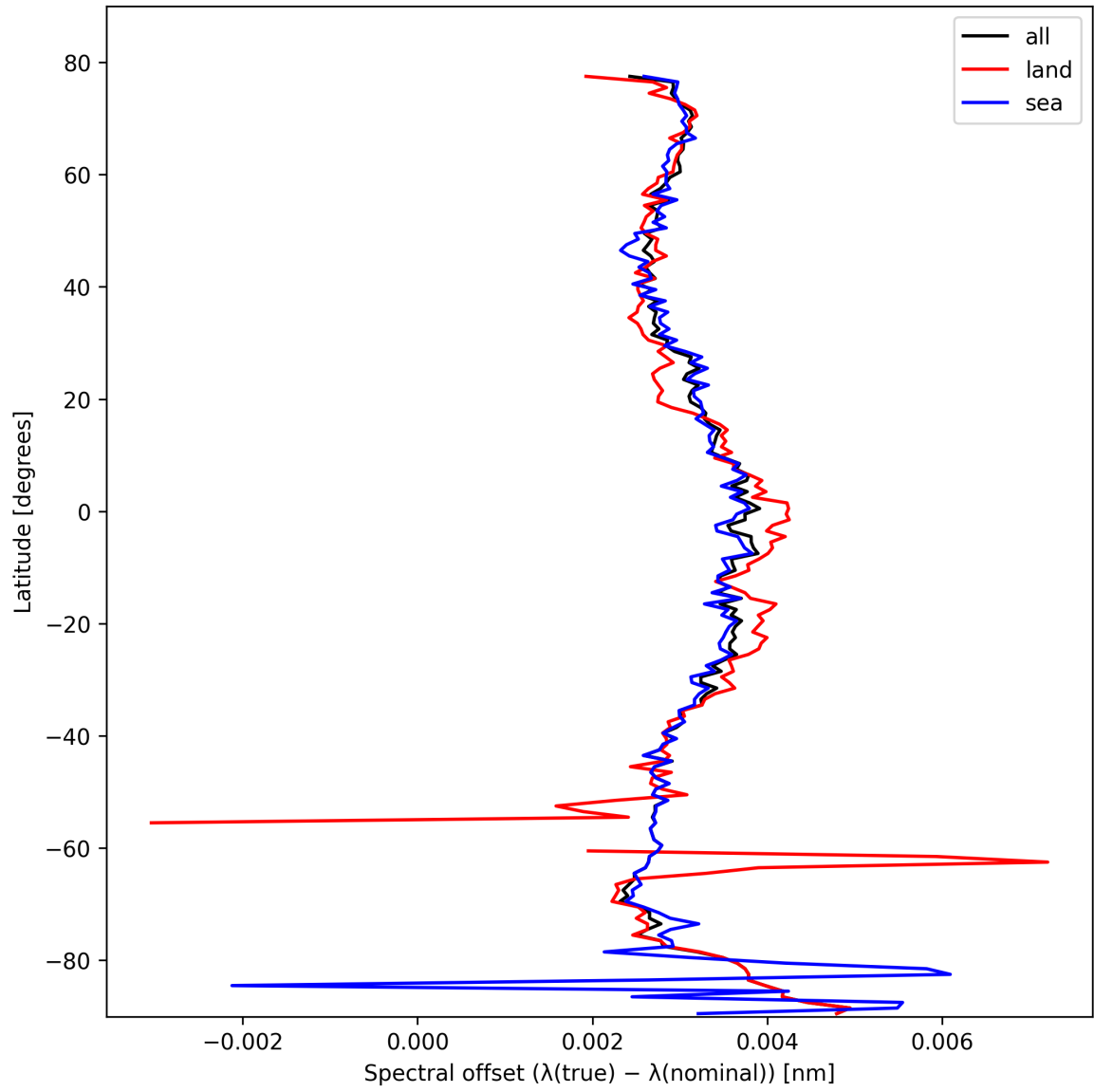
Figure 28: Zonal average of “Spectral offset ( \lambda_{\text{true}} - \lambda_{\text{nominal}} )” for 2025-02-19 to 2025-02-21.
