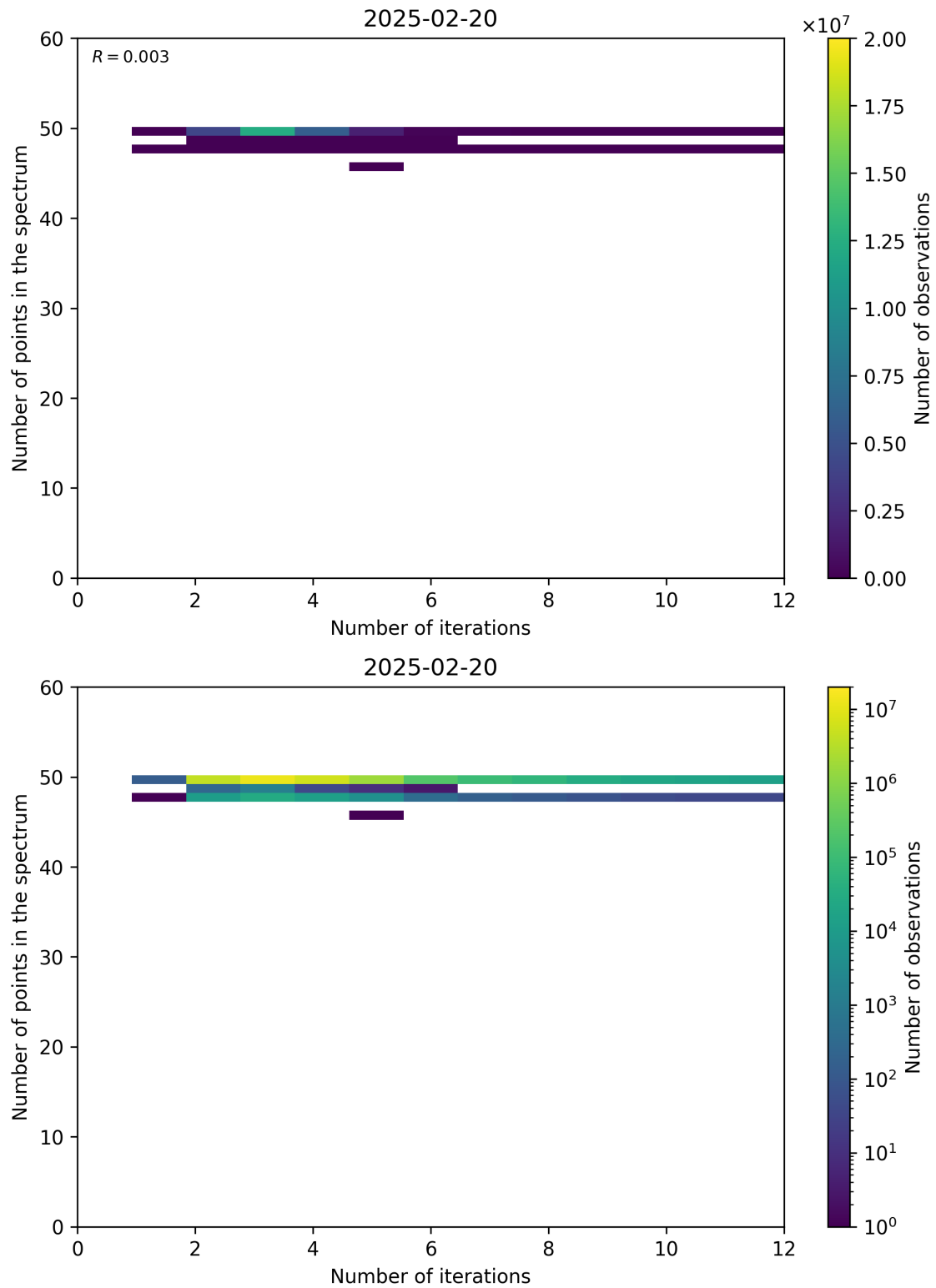
Figure 99: Scatter density plot of “Number of iterations” against “Number of points in the spectrum” for 2025-02-19 to 2025-02-21.
