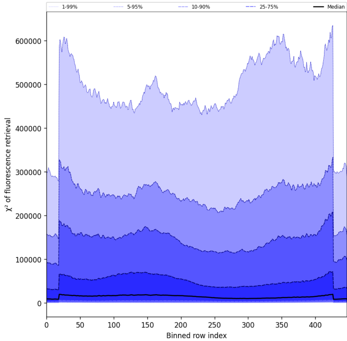
Figure 59: Along track statistics of “ \chi^2 of fluorescence retrieval” for 2025-02-19 to 2025-02-21
