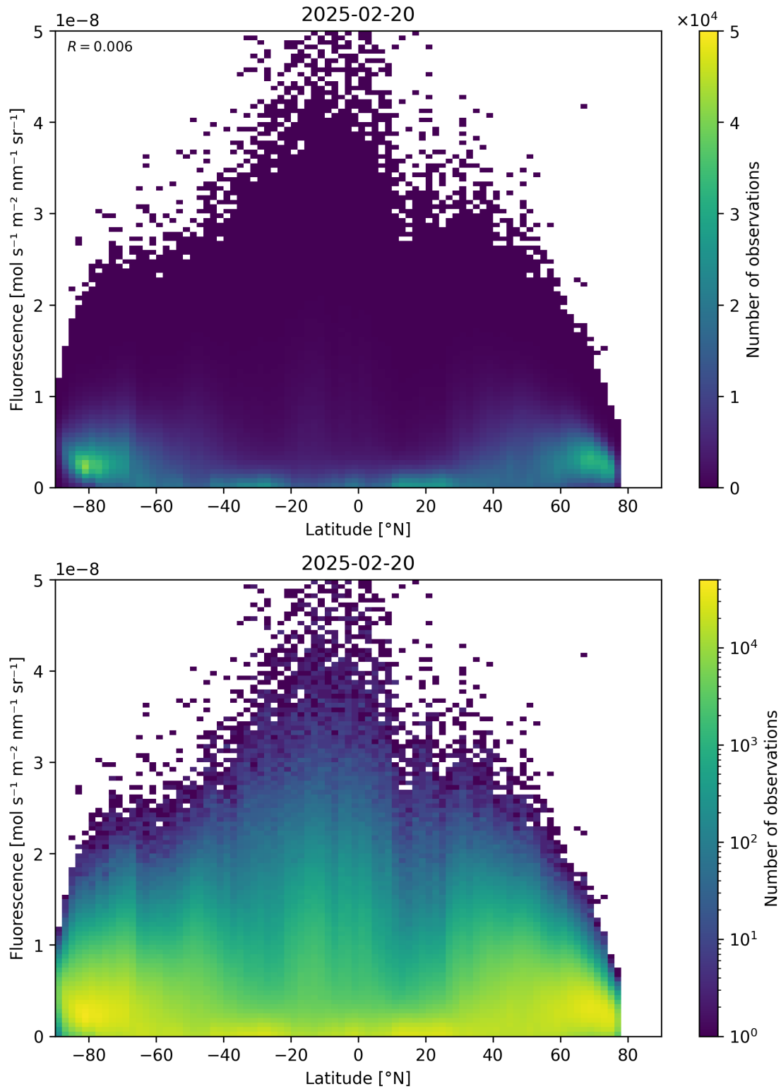
Figure 92: Scatter density plot of “Latitude” against “Fluorescence” for 2025-02-19 to 2025-02-21.
