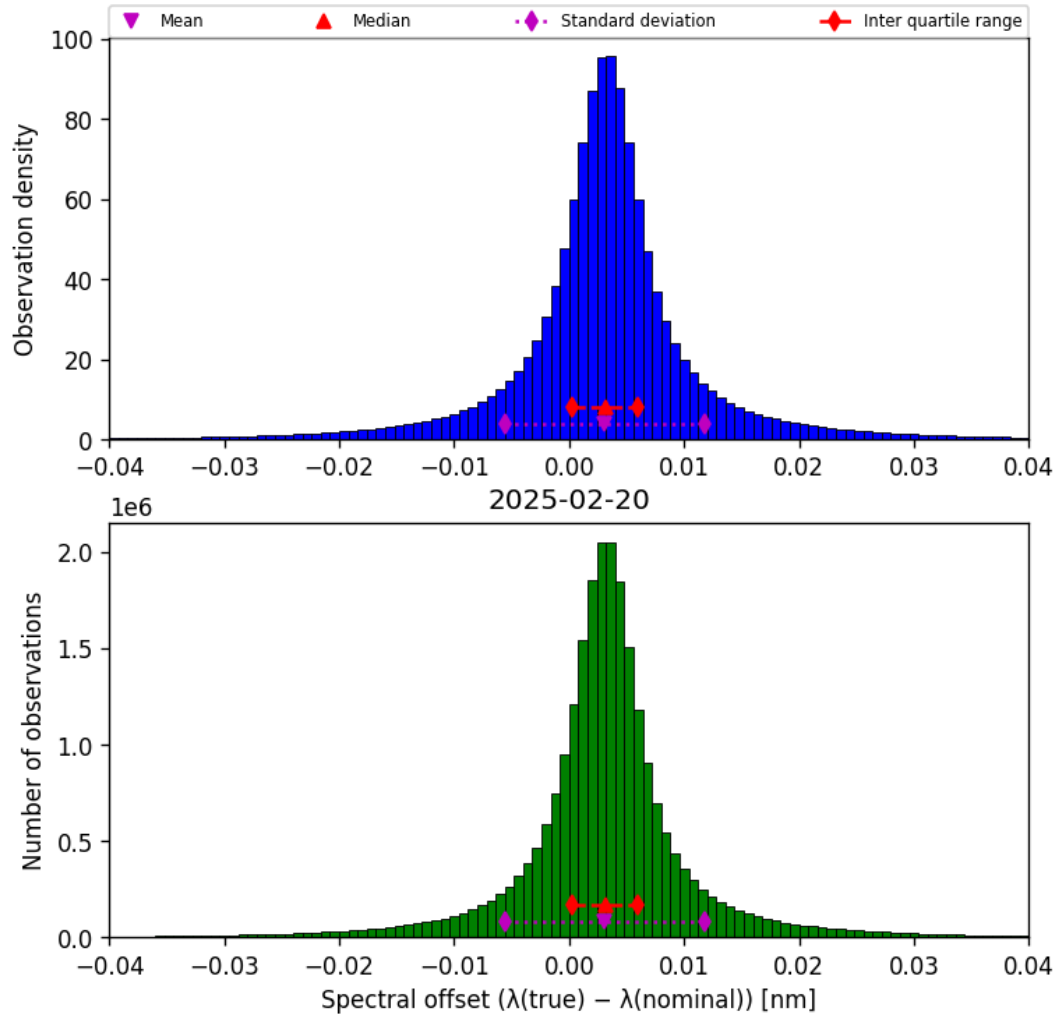
Figure 45: Histogram of “Spectral offset ( \lambda_{\text{true}} - \lambda_{\text{nominal}} )” for 2025-02-19 to 2025-02-21
