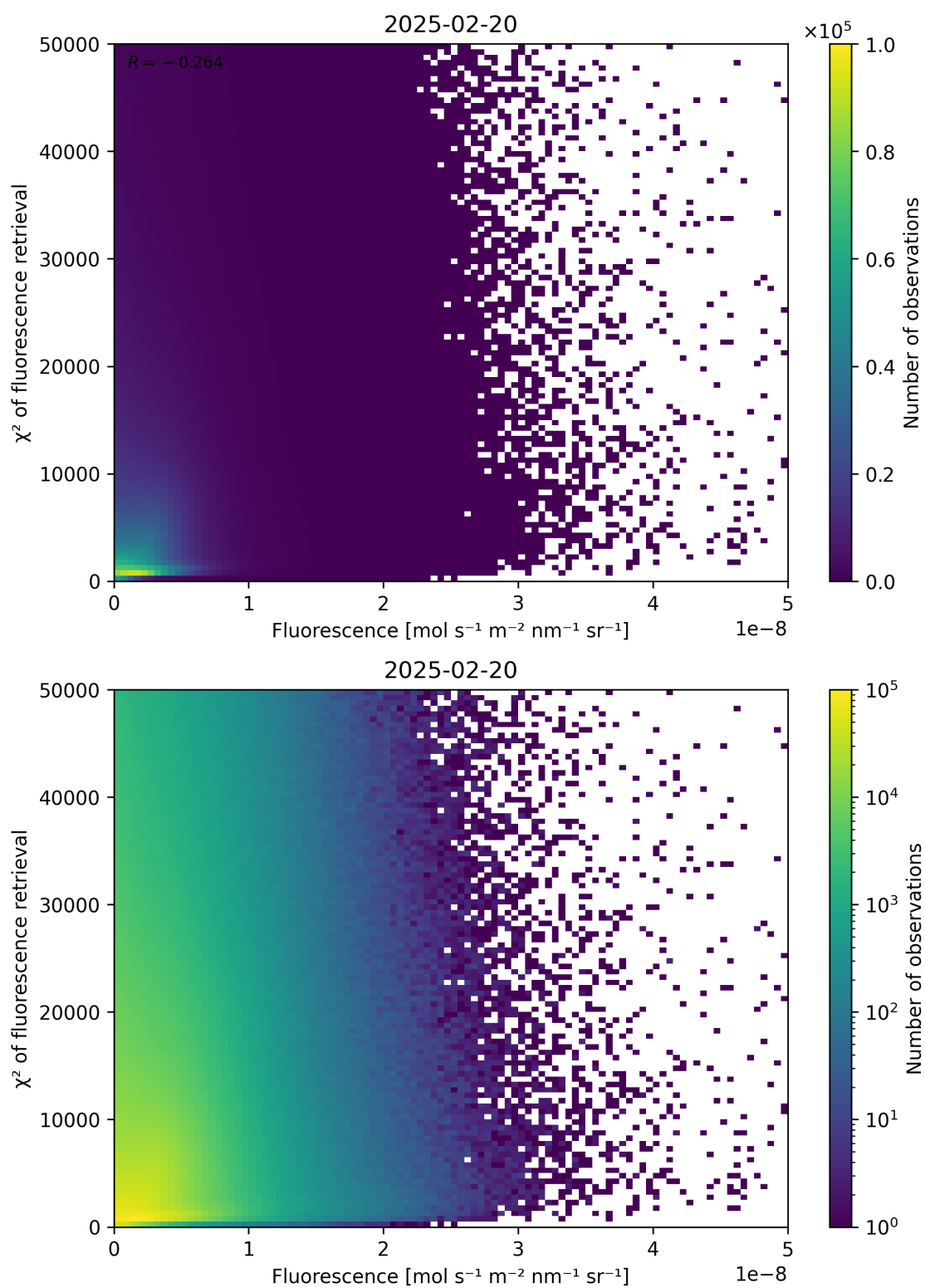
Figure 85: Scatter density plot of “Fluorescence” against “ \chi^2 of fluorescence retrieval” for 2025-02-19 to 2025-02-21.
