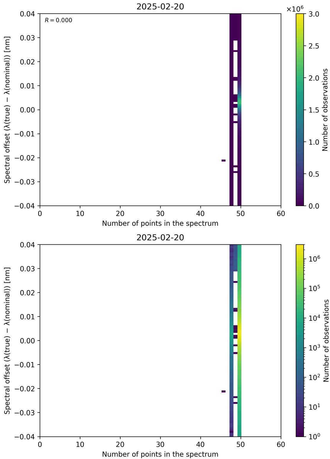
Figure 101: Scatter density plot of “Number of points in the spectrum” against “Spectral offset ( \lambda_{\text{true}} - \lambda_{\text{nominal}} )” for 2025-02-19 to 2025-02-21.
