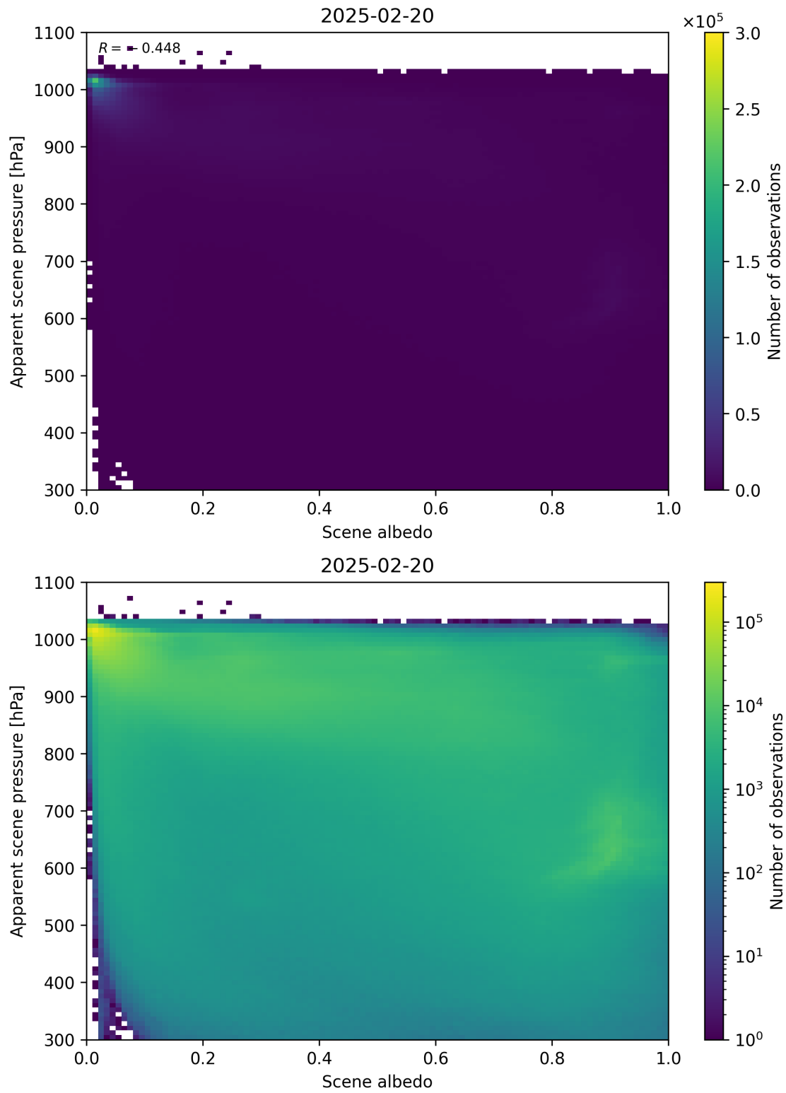
Figure 102: Scatter density plot of “Scene albedo” against “Apparent scene pressure” for 2025-02-19 to 2025-02-21.
