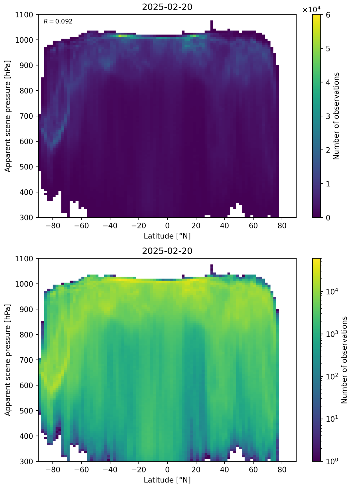
Figure 88: Scatter density plot of “Latitude” against “Apparent scene pressure” for 2025-02-19 to 2025-02-21.
