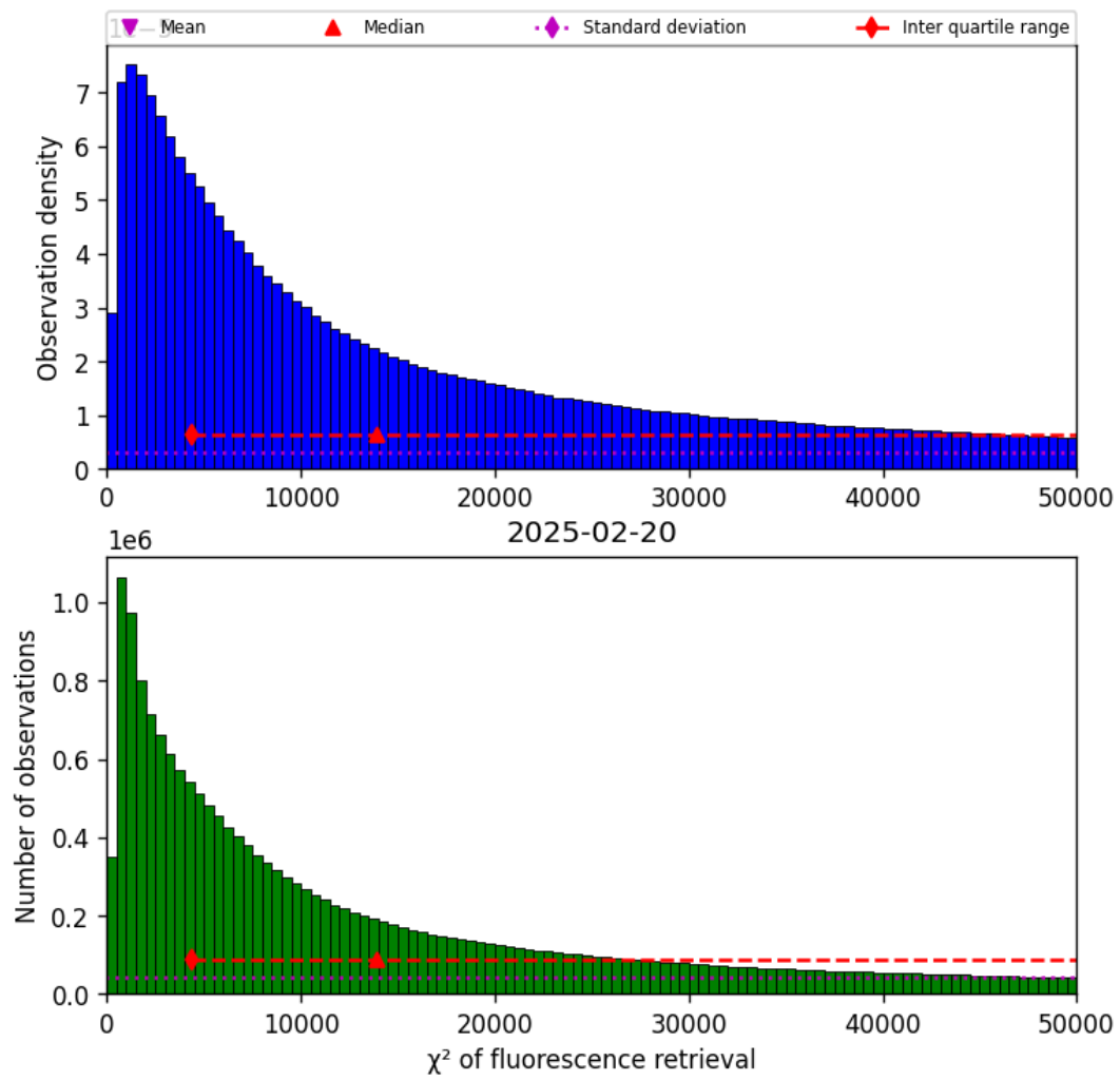
Figure 42: Histogram of “ \chi^2 of fluorescence retrieval” for 2025-02-19 to 2025-02-21
