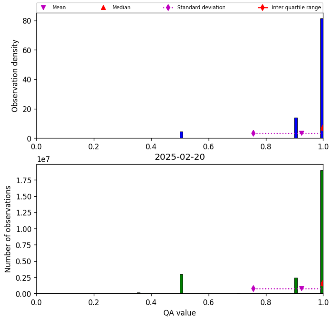
Figure 29: Histogram of “QA value” for 2025-02-19 to 2025-02-21
