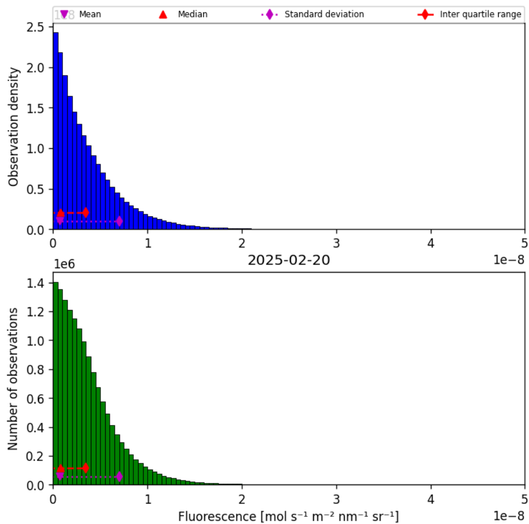
Figure 40: Histogram of “Fluorescence” for 2025-02-19 to 2025-02-21
