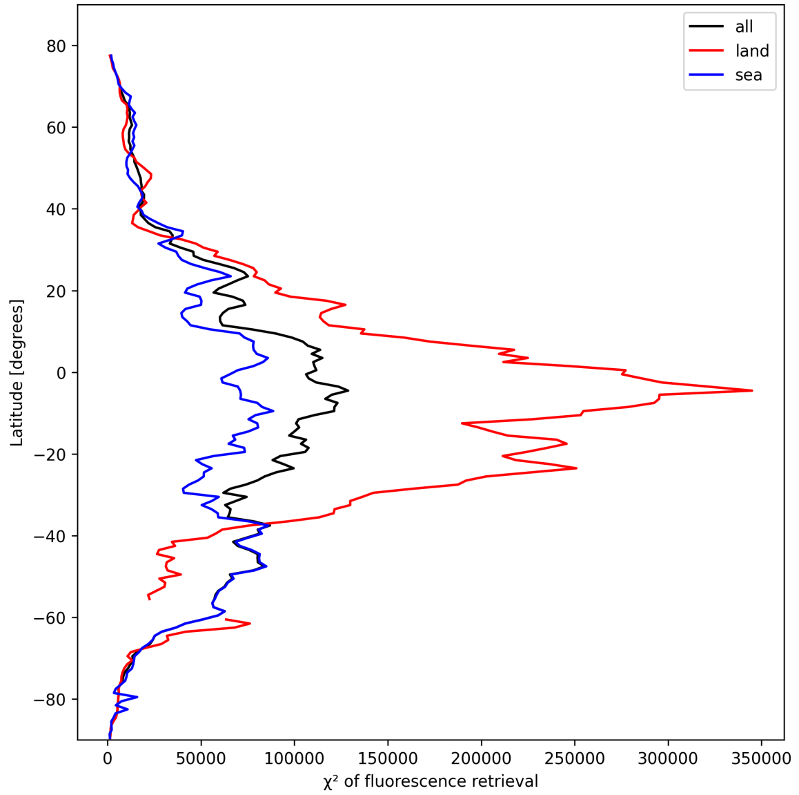
Figure 25: Zonal average of “ \chi^2 of fluorescence retrieval” for 2025-02-19 to 2025-02-21.
