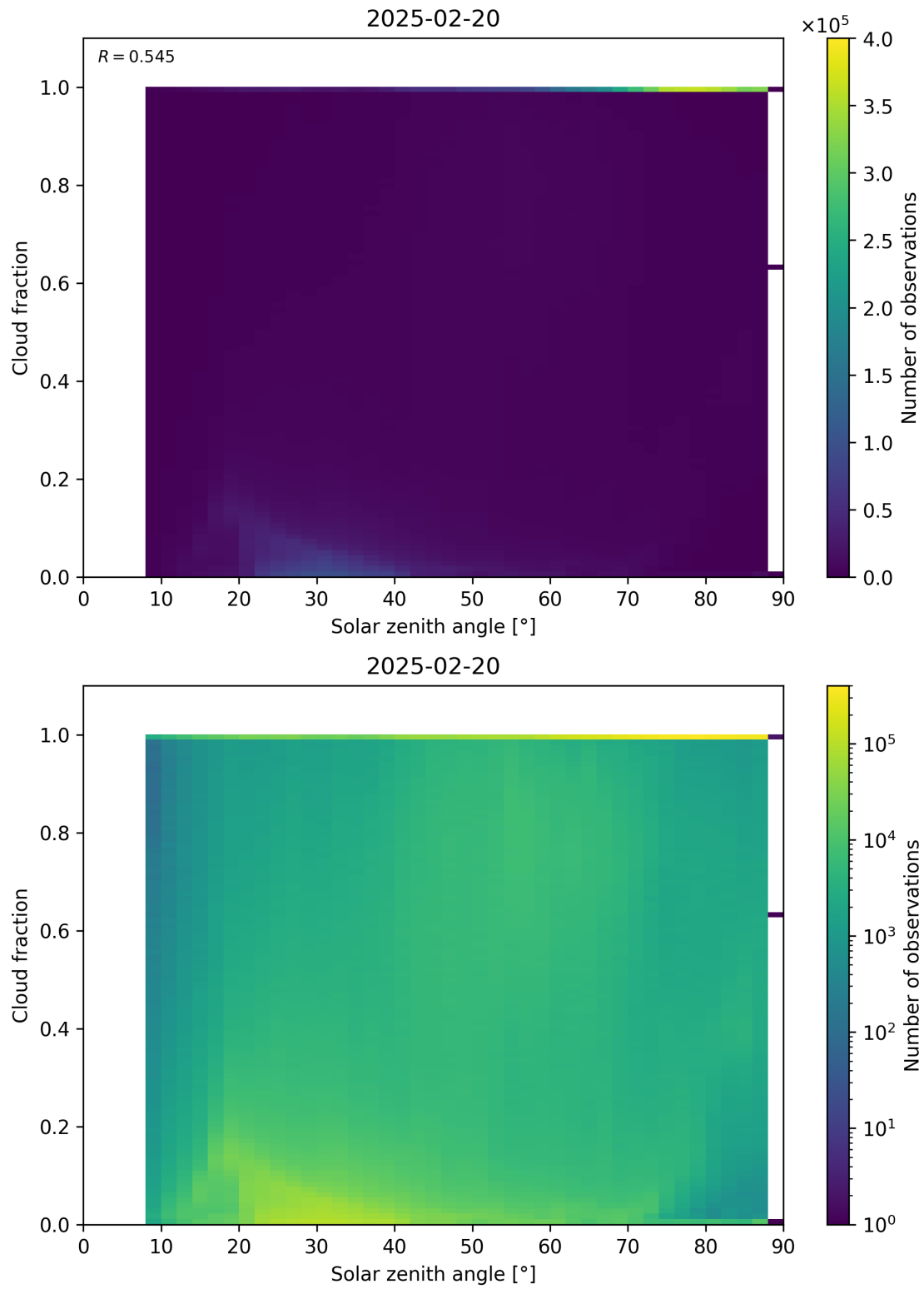
Figure 110: Scatter density plot of “Solar zenith angle” against “Cloud fraction” for 2025-02-19 to 2025-02-21.
