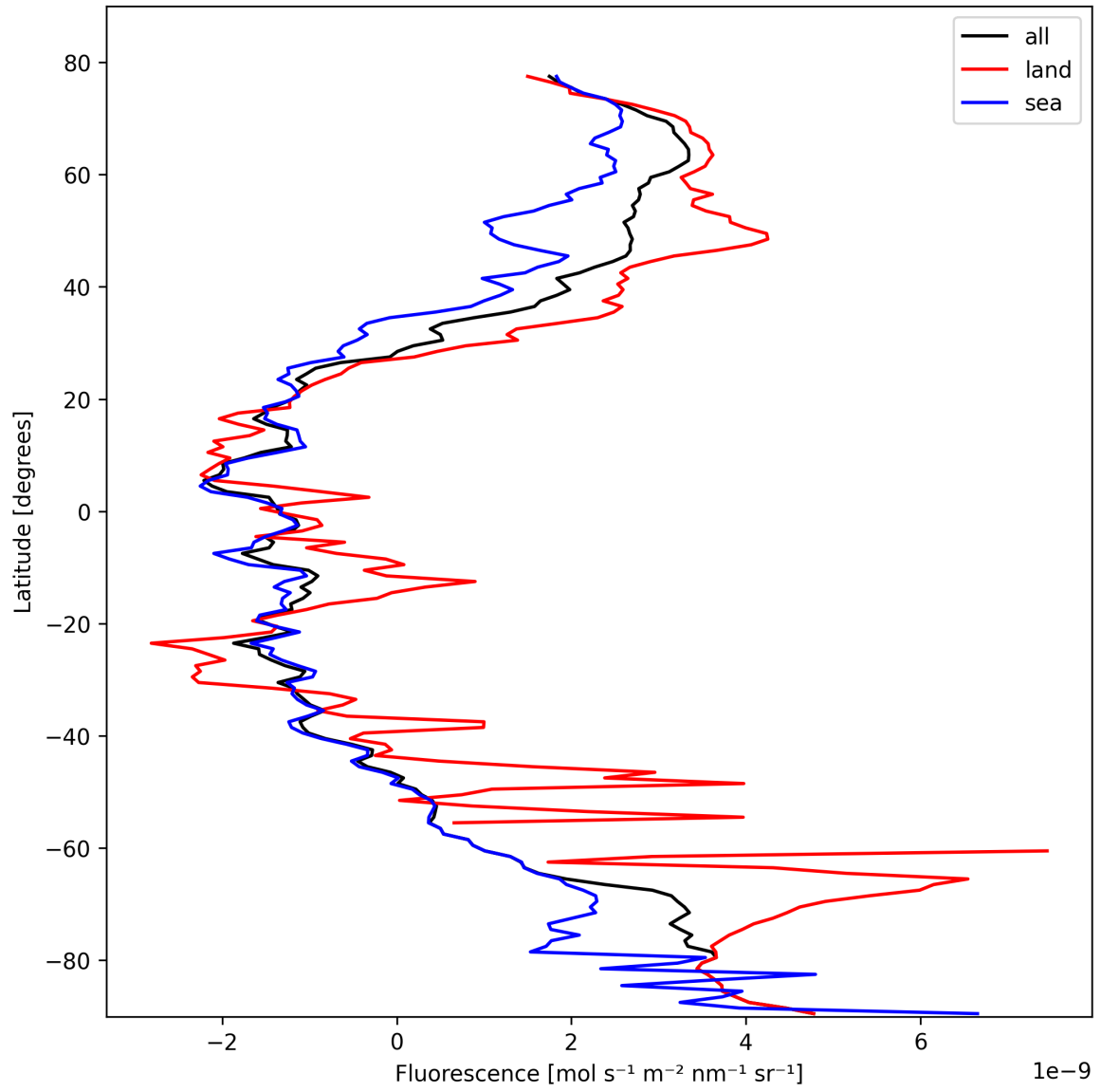
Figure 23: Zonal average of “Fluorescence” for 2025-02-19 to 2025-02-21.
