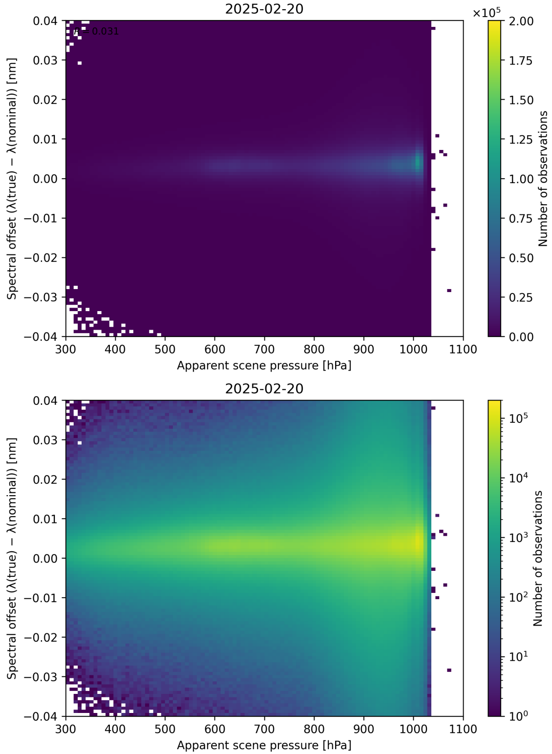
Figure 67: Scatter density plot of “Apparent scene pressure” against “Spectral offset ( \lambda_{\text{true}} - \lambda_{\text{nominal}} )” for 2025-02-19 to 2025-02-21.
