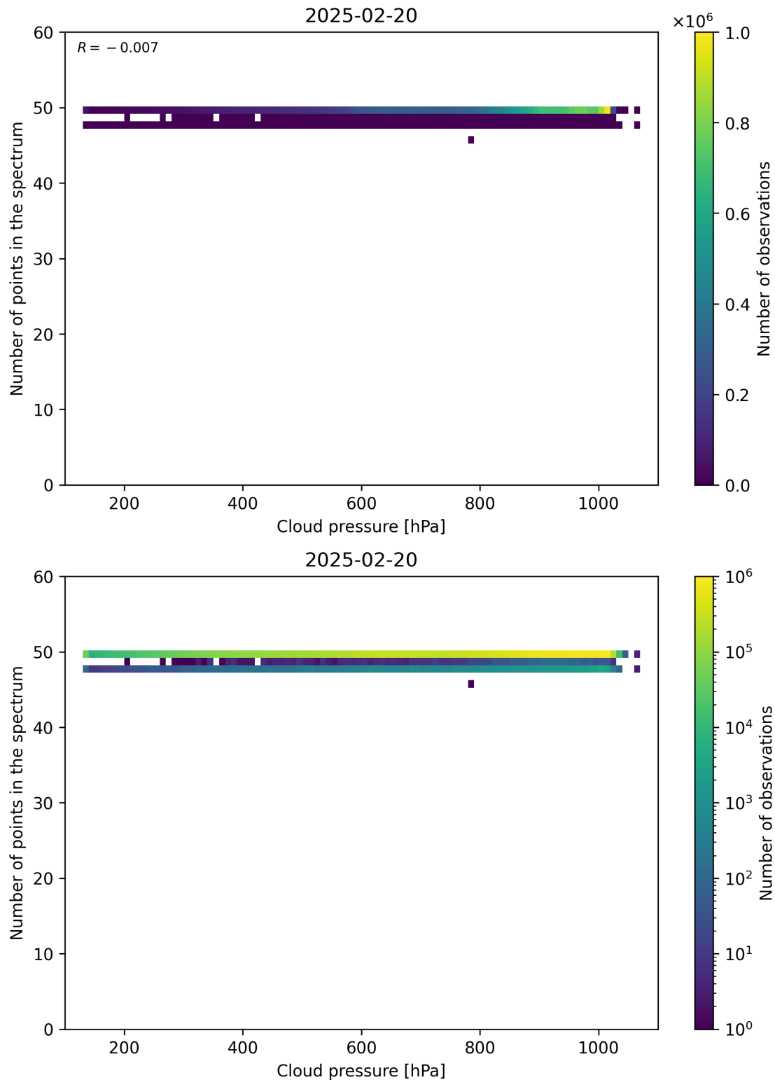
Figure 82: Scatter density plot of “Cloud pressure” against “Number of points in the spectrum” for 2025-02-19 to 2025-02-21.
