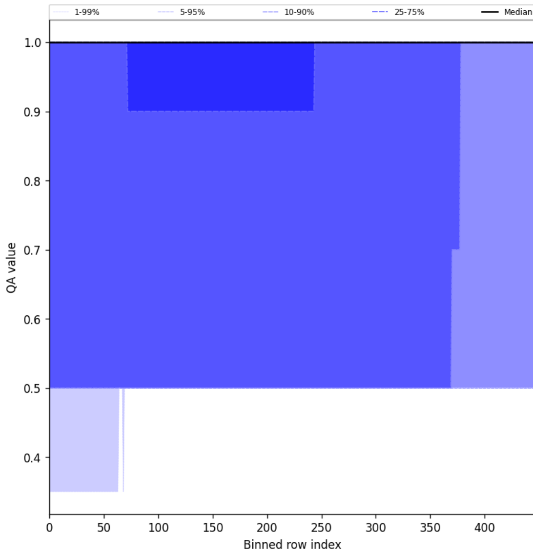
Figure 46: Along track statistics of “QA value” for 2025-02-19 to 2025-02-21
