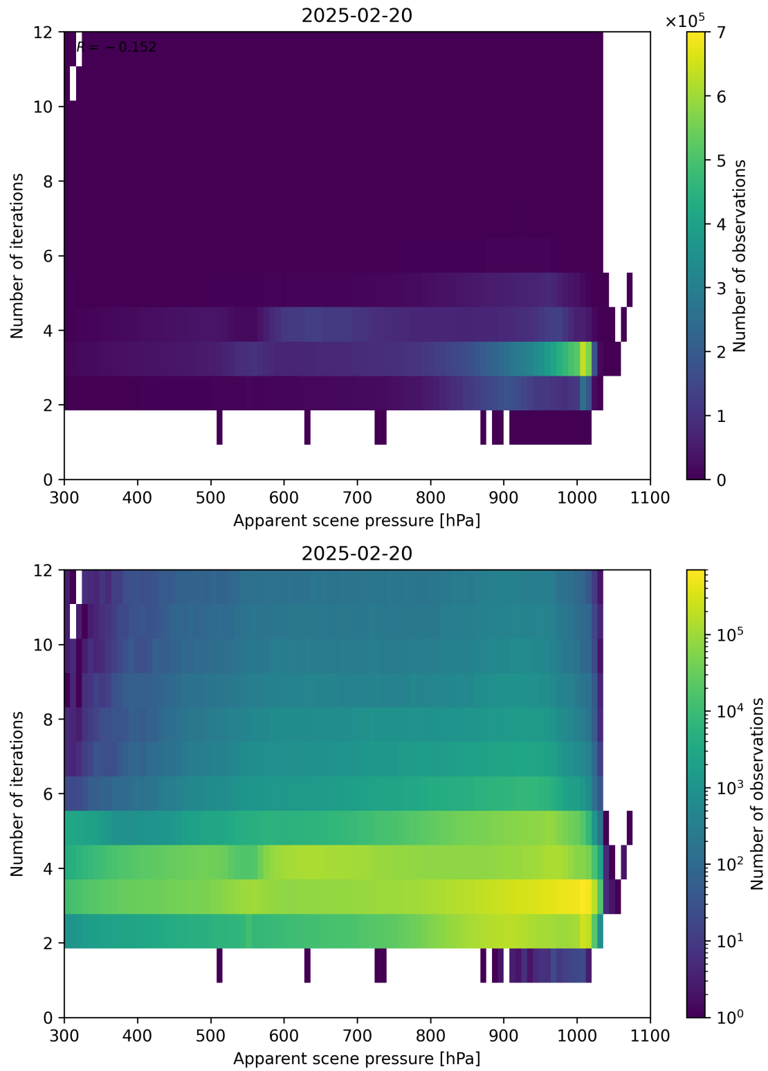
Figure 65: Scatter density plot of “Apparent scene pressure” against “Number of iterations” for 2025-02-19 to 2025-02-21.
