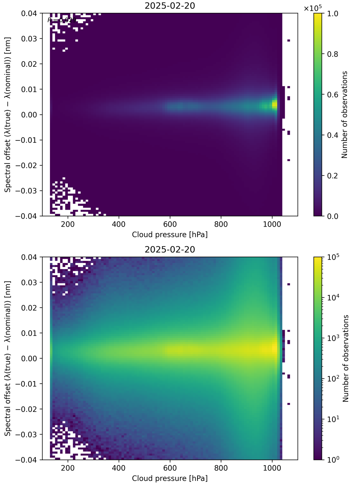
Figure 84: Scatter density plot of “Cloud pressure” against “Spectral offset ( \lambda_{\text{true}} - \lambda_{\text{nominal}} )” for 2025-02-19 to 2025-02-21.
