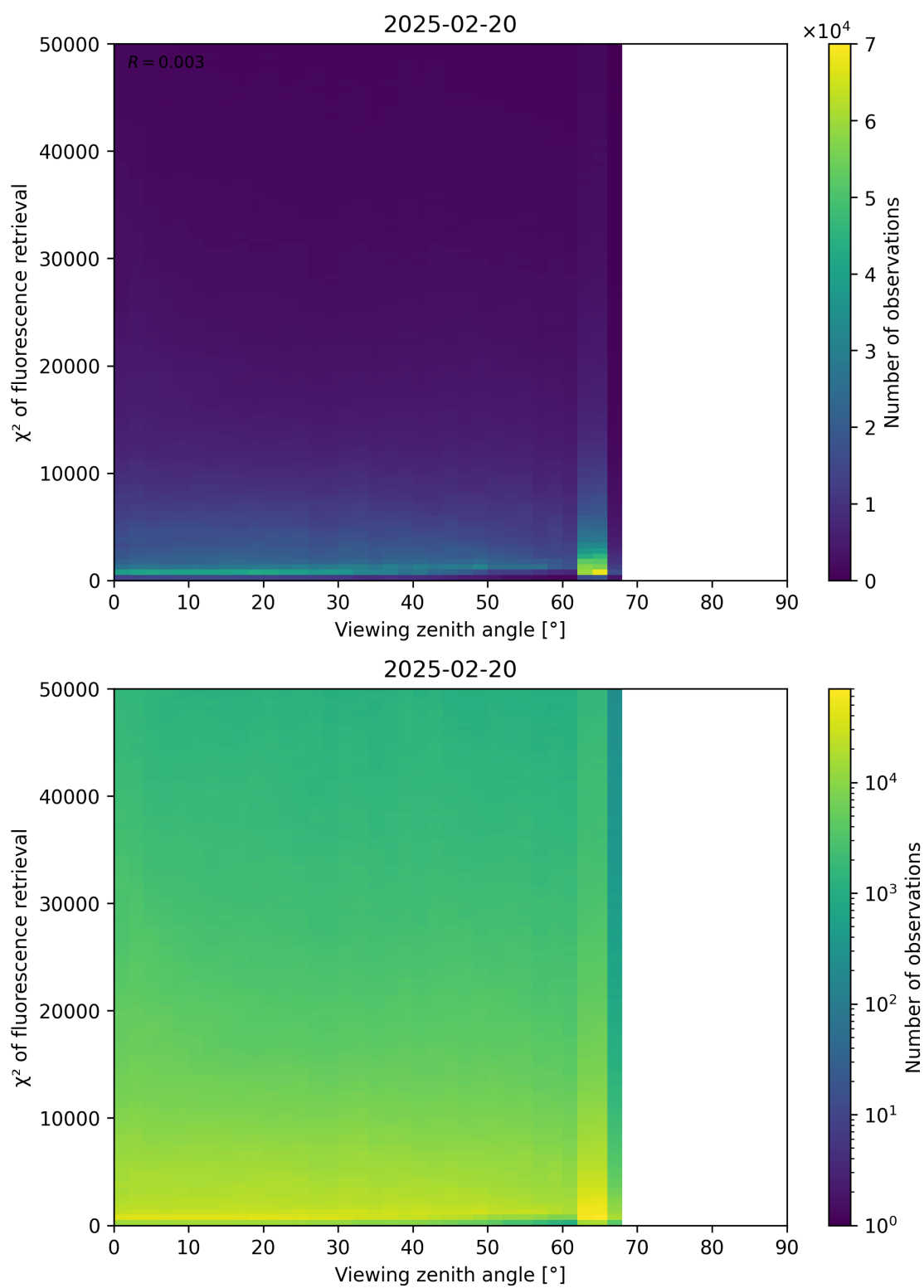
Figure 119: Scatter density plot of “Viewing zenith angle” against “ \chi^2 of fluorescence retrieval” for 2025-02-19 to 2025-02-21.
