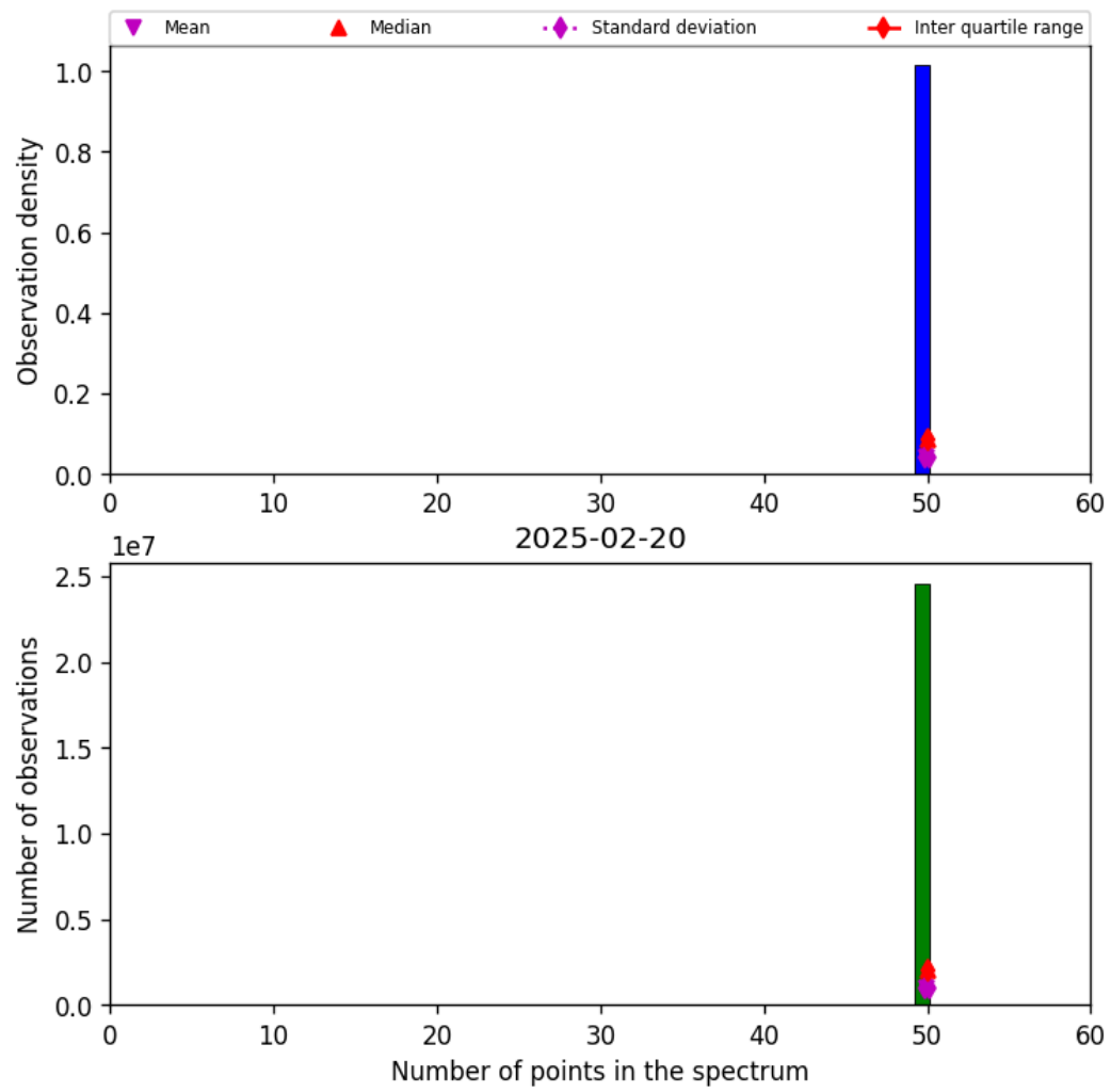
Figure 44: Histogram of "Number of points in the spectrum" for 2025-02-19 to 2025-02-21
