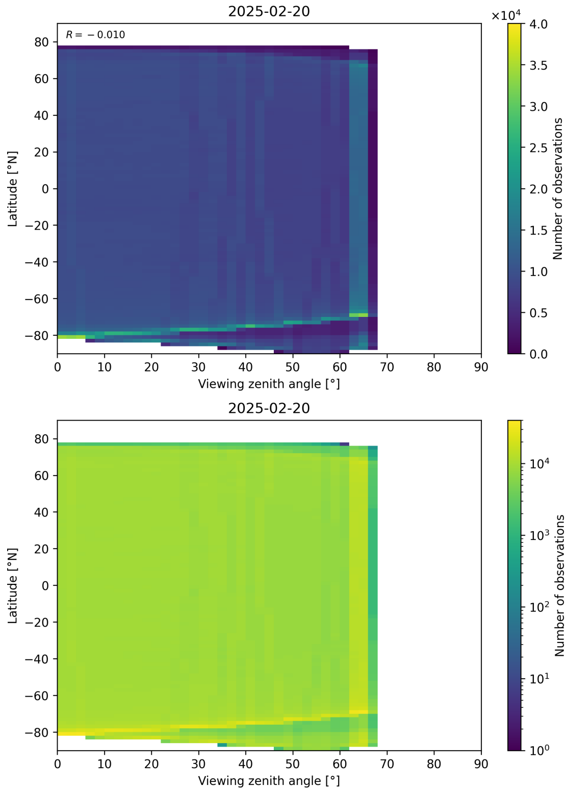
Figure 123: Scatter density plot of “Viewing zenith angle” against “Latitude” for 2025-02-19 to 2025-02-21.
