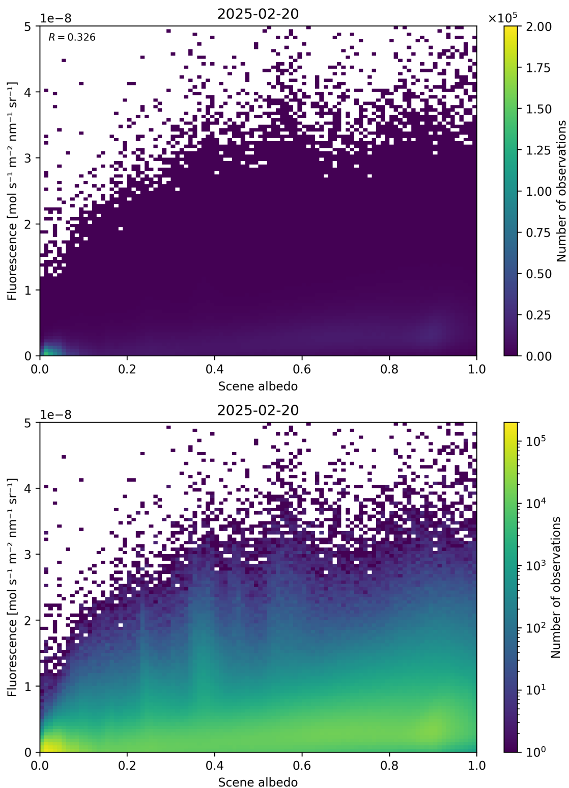
Figure 104: Scatter density plot of “Scene albedo” against “Fluorescence” for 2025-02-19 to 2025-02-21.
