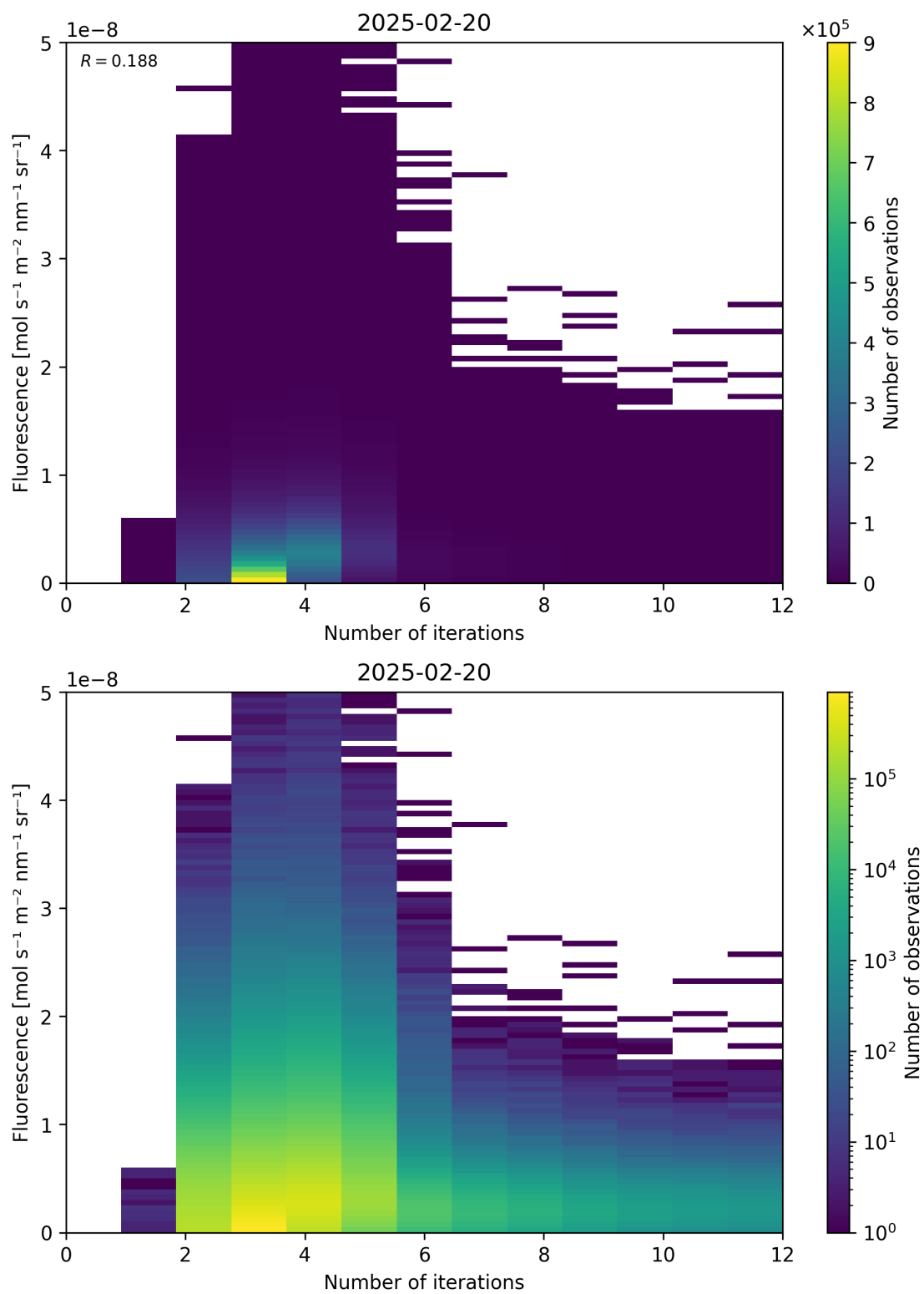
Figure 98: Scatter density plot of “Number of iterations” against “Fluorescence” for 2025-02-19 to 2025-02-21.
