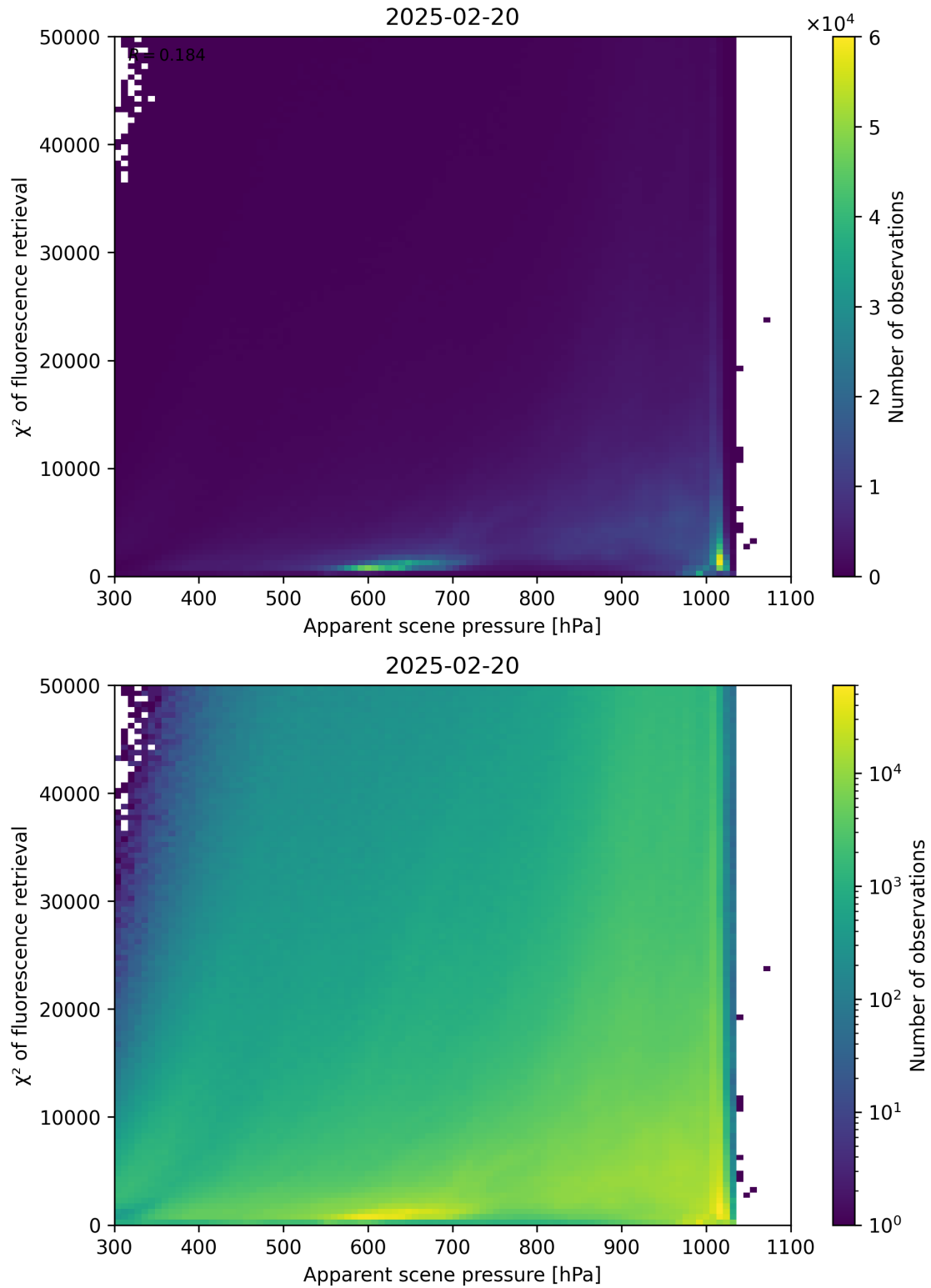
Figure 63: Scatter density plot of “Apparent scene pressure” against “ \chi^2 of fluorescence retrieval” for 2025-02-19 to 2025-02-21.
