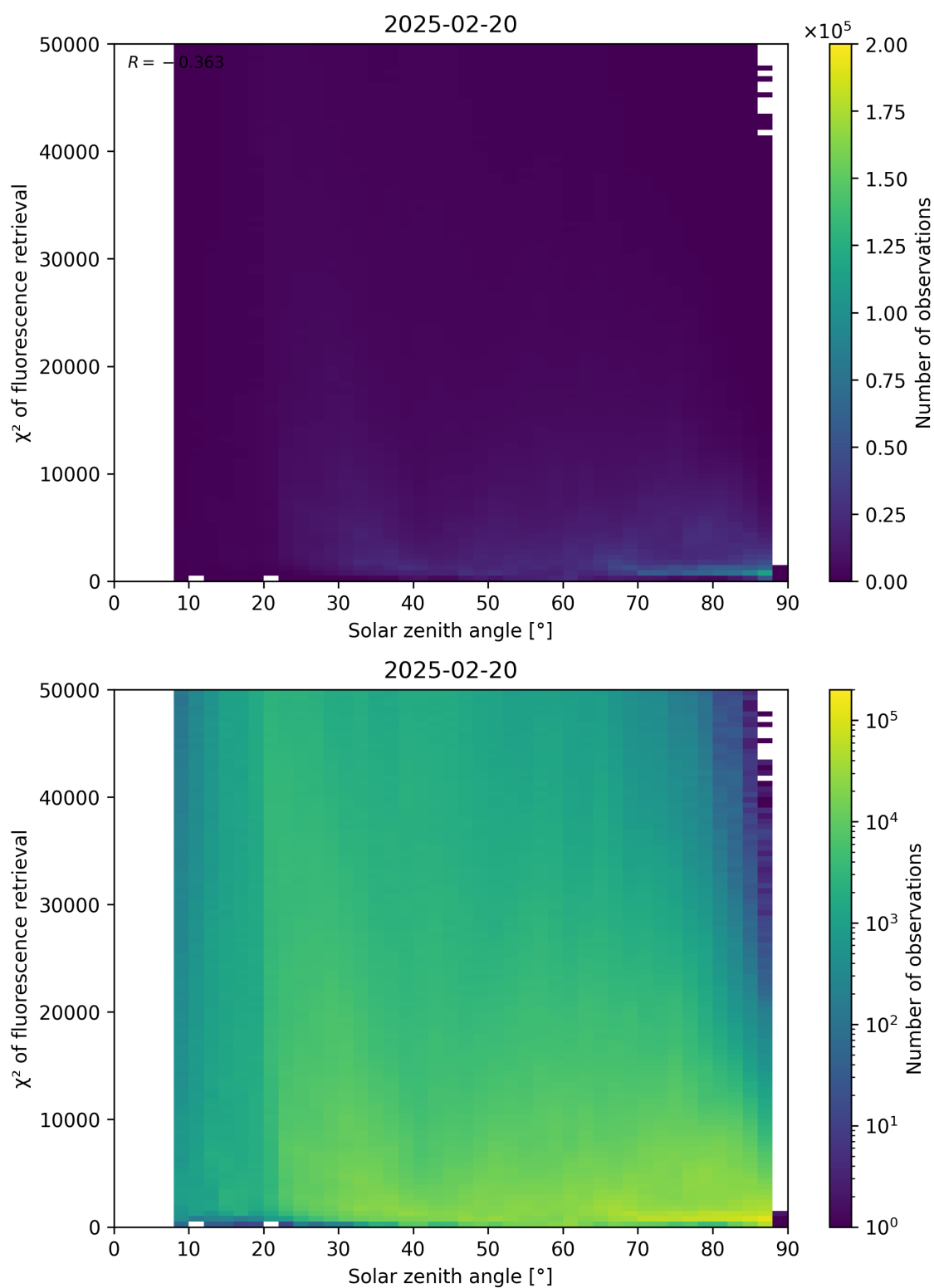
Figure 109: Scatter density plot of “Solar zenith angle” against “ \chi^2 of fluorescence retrieval” for 2025-02-19 to 2025-02-21.
