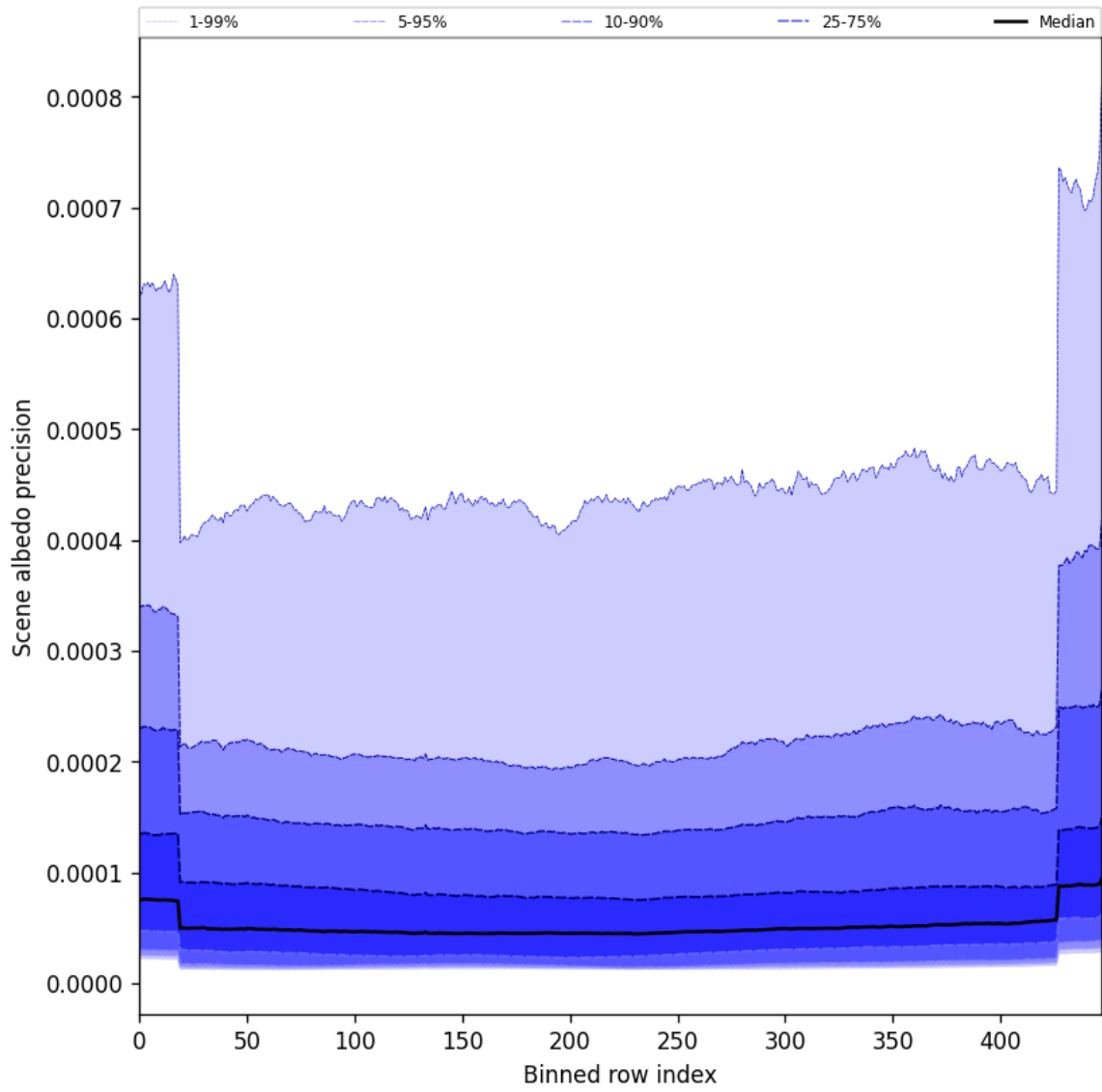
Figure 52: Along track statistics of “Scene albedo precision” for 2025-02-19 to 2025-02-21
