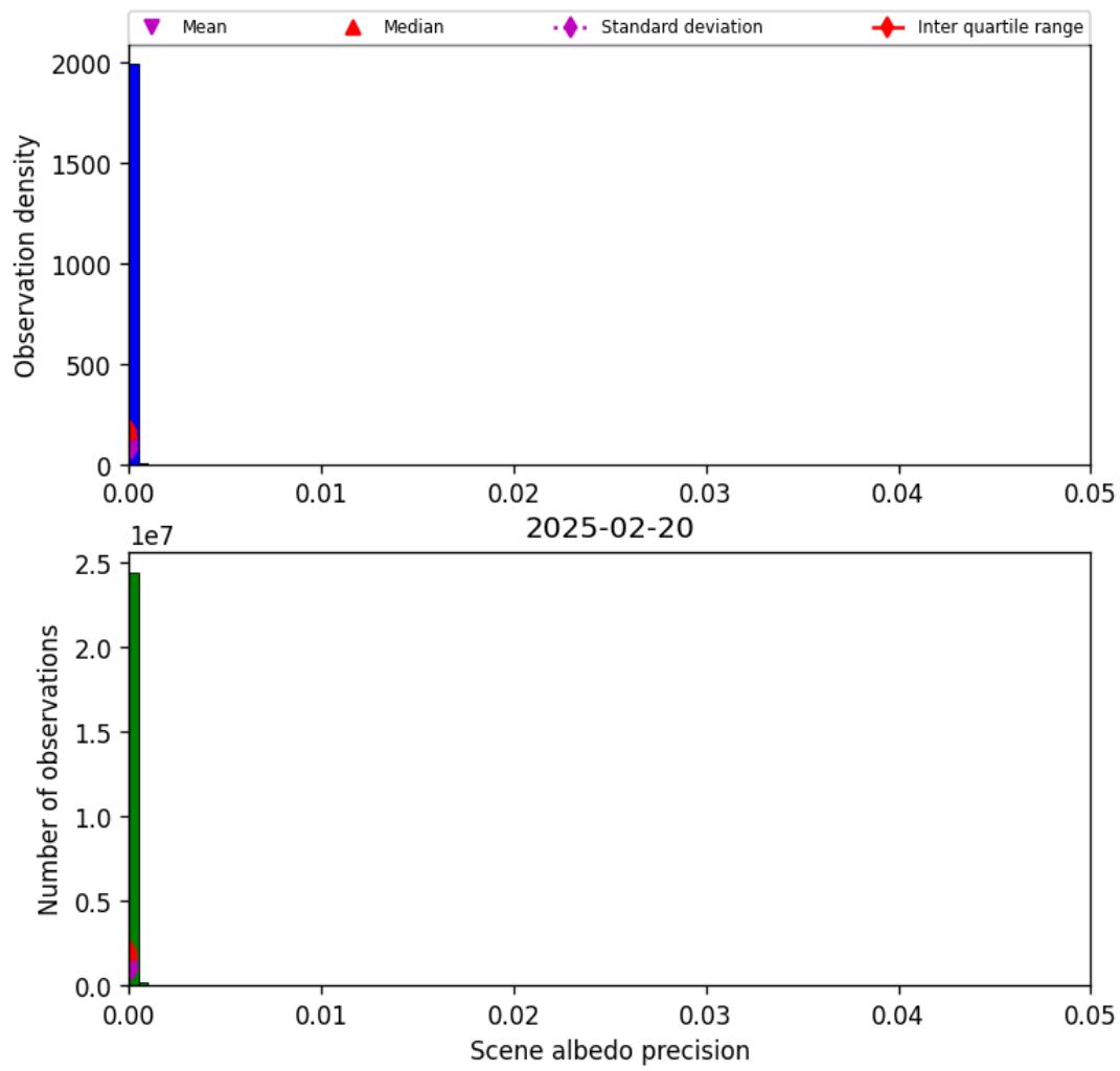
Figure 35: Histogram of “Scene albedo precision” for 2025-02-19 to 2025-02-21
