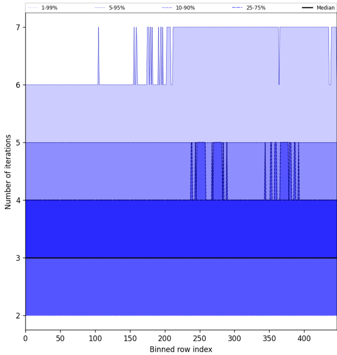
Figure 56: Along track statistics of “Number of iterations” for 2025-02-19 to 2025-02-21
