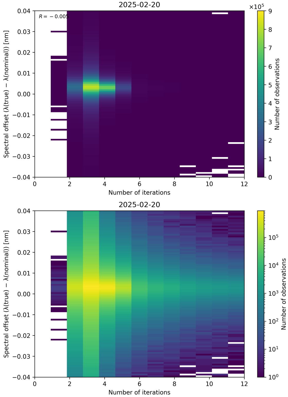
Figure 100: Scatter density plot of “Number of iterations” against “Spectral offset ( \lambda_{\text{true}} - \lambda_{\text{nominal}} )” for 2025-02-19 to 2025-02-21.
