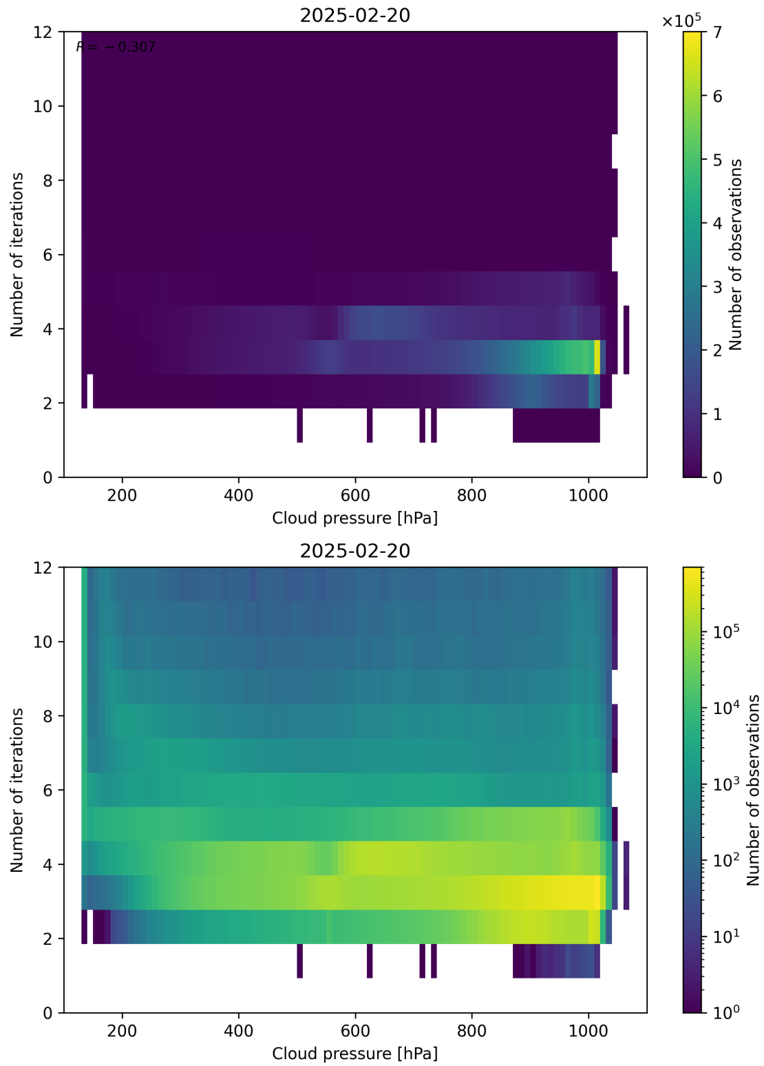
Figure 81: Scatter density plot of “Cloud pressure” against “Number of iterations” for 2025-02-19 to 2025-02-21.
