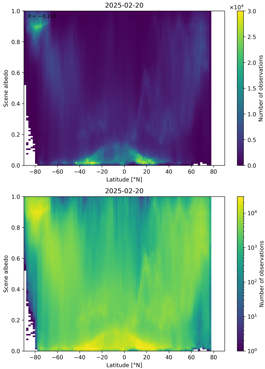
Figure 95: Scatter density plot of “Latitude” against “Scene albedo” for 2025-02-19 to 2025-02-21.
