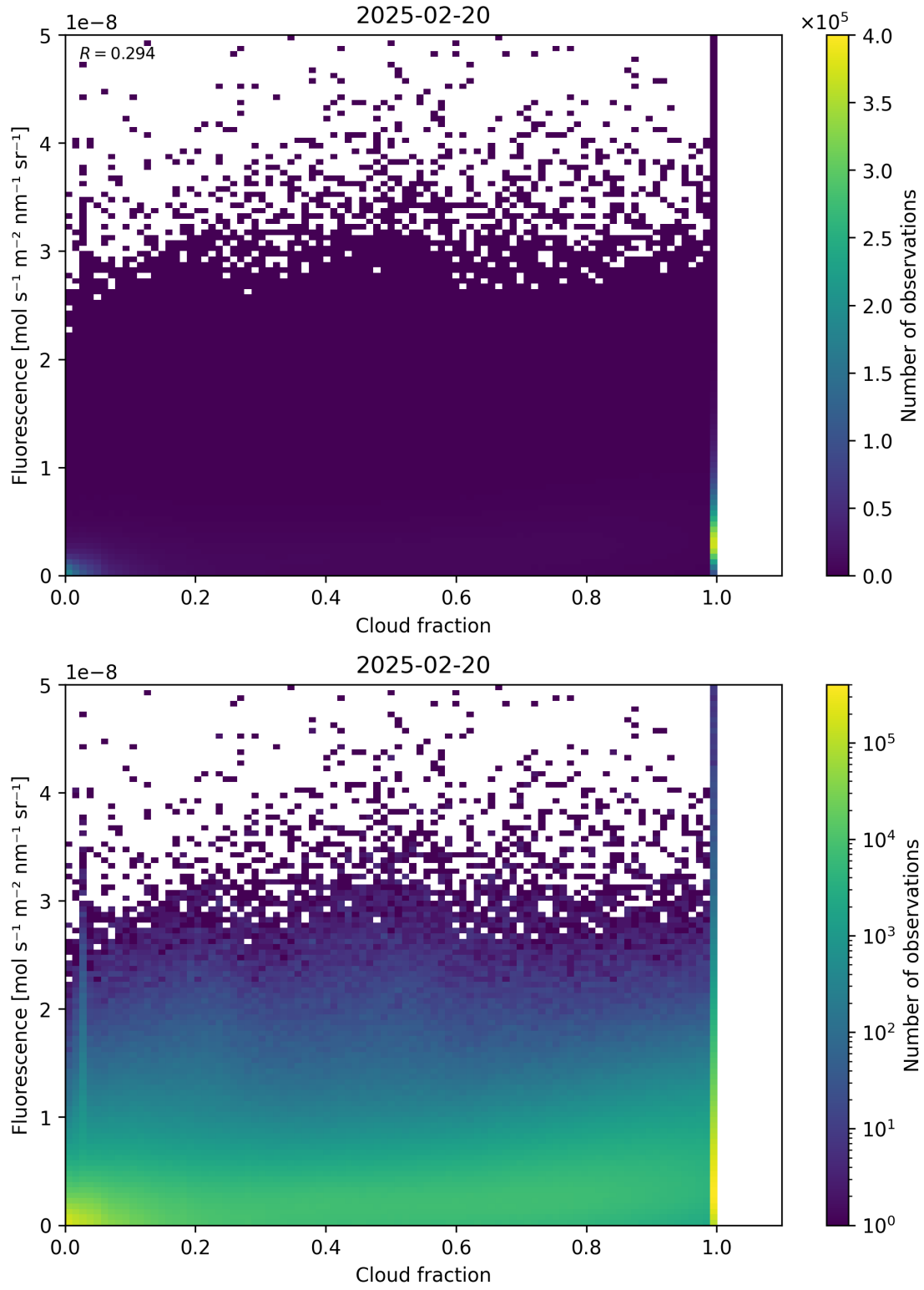
Figure 72: Scatter density plot of “Cloud fraction” against “Fluorescence” for 2025-02-19 to 2025-02-21.
