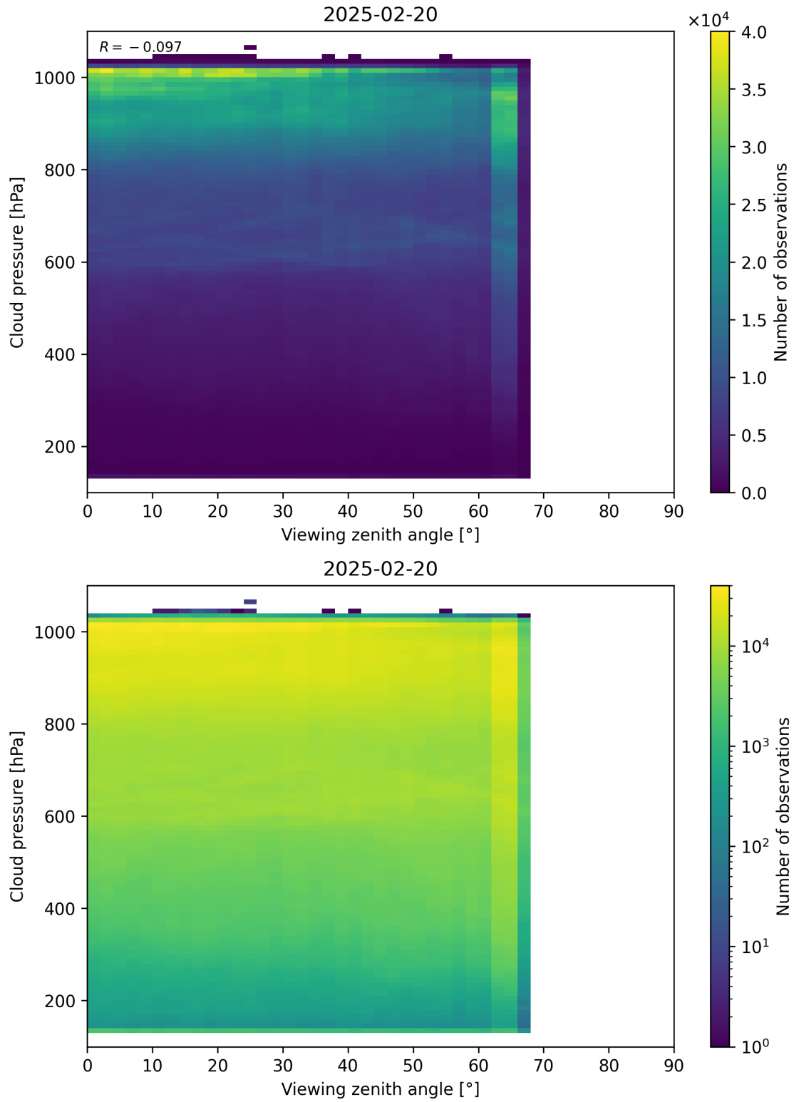
Figure 121: Scatter density plot of “Viewing zenith angle” against “Cloud pressure” for 2025-02-19 to 2025-02-21.
