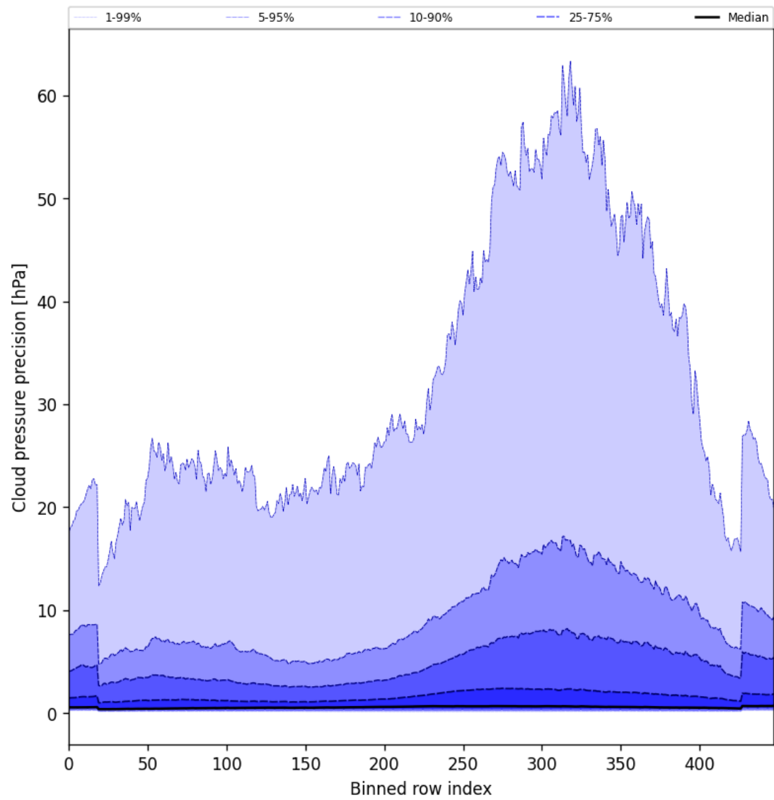
Figure 48: Along track statistics of “Cloud pressure precision” for 2025-02-19 to 2025-02-21
