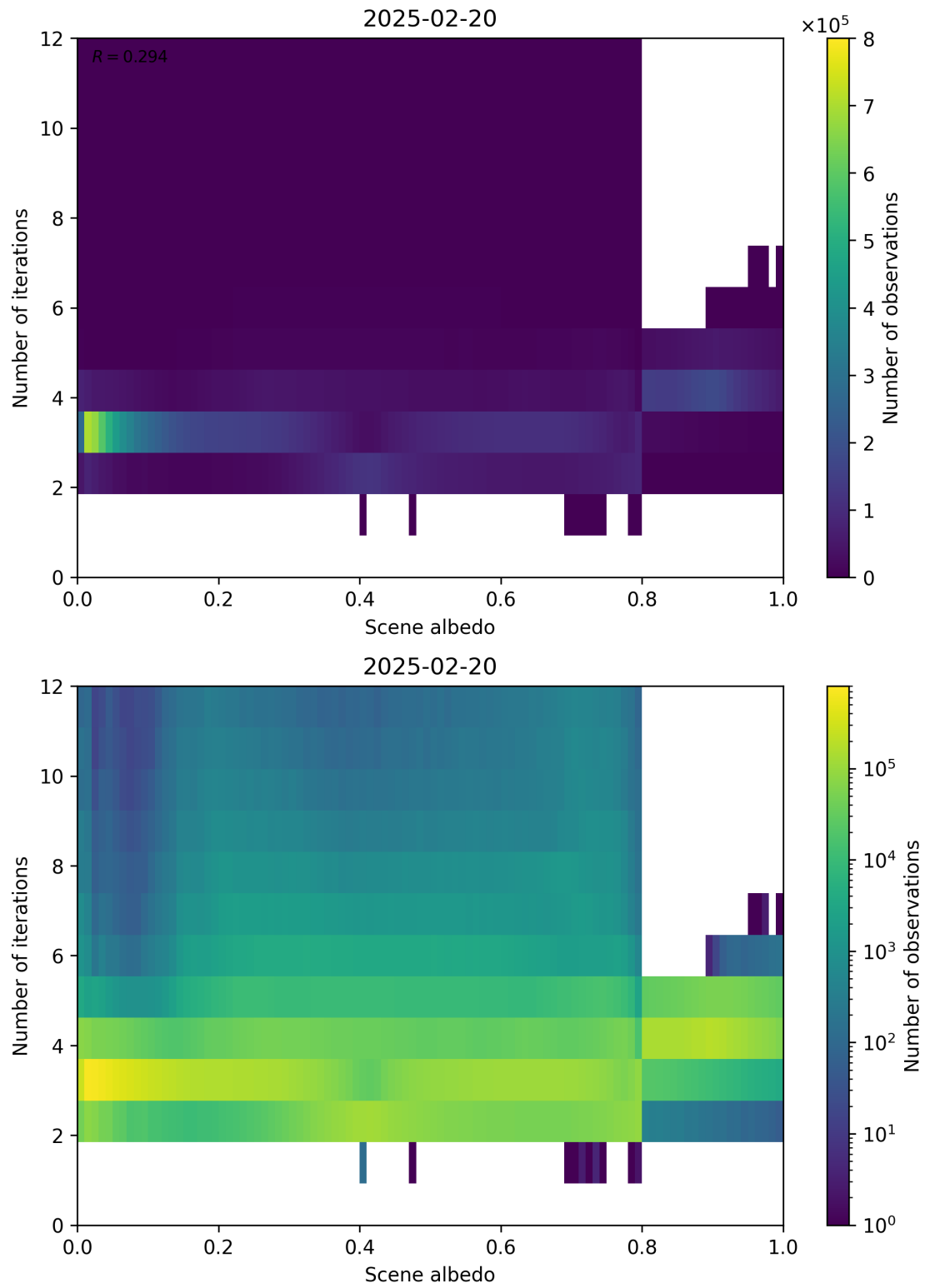
Figure 105: Scatter density plot of “Scene albedo” against “Number of iterations” for 2025-02-19 to 2025-02-21.
