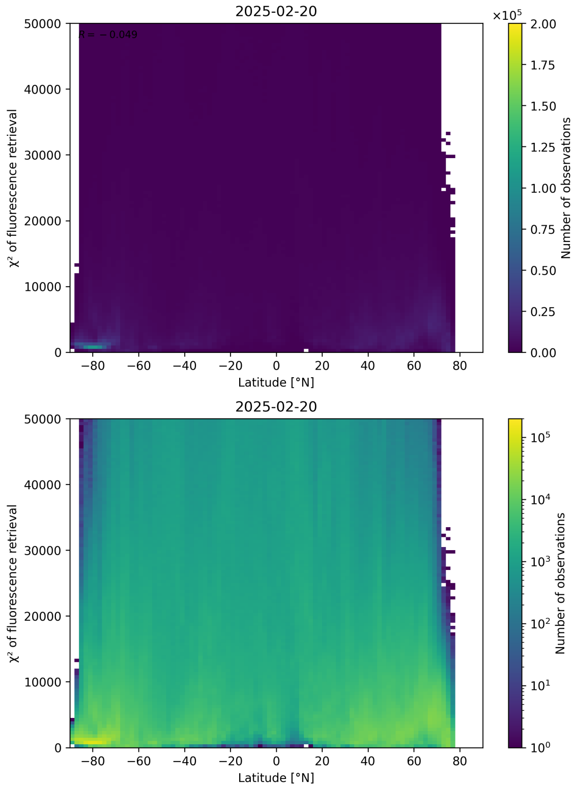
Figure 89: Scatter density plot of “Latitude” against “ \chi^2 of fluorescence retrieval” for 2025-02-19 to 2025-02-21.
