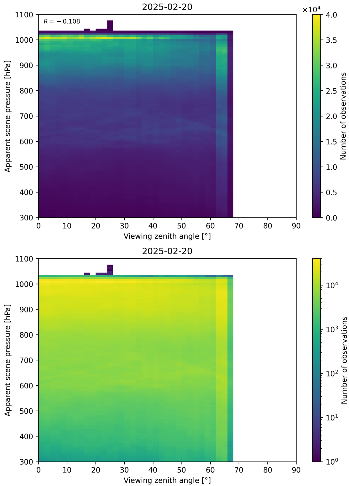
Figure 118: Scatter density plot of “Viewing zenith angle” against “Apparent scene pressure” for 2025-02-19 to 2025-02-21.
