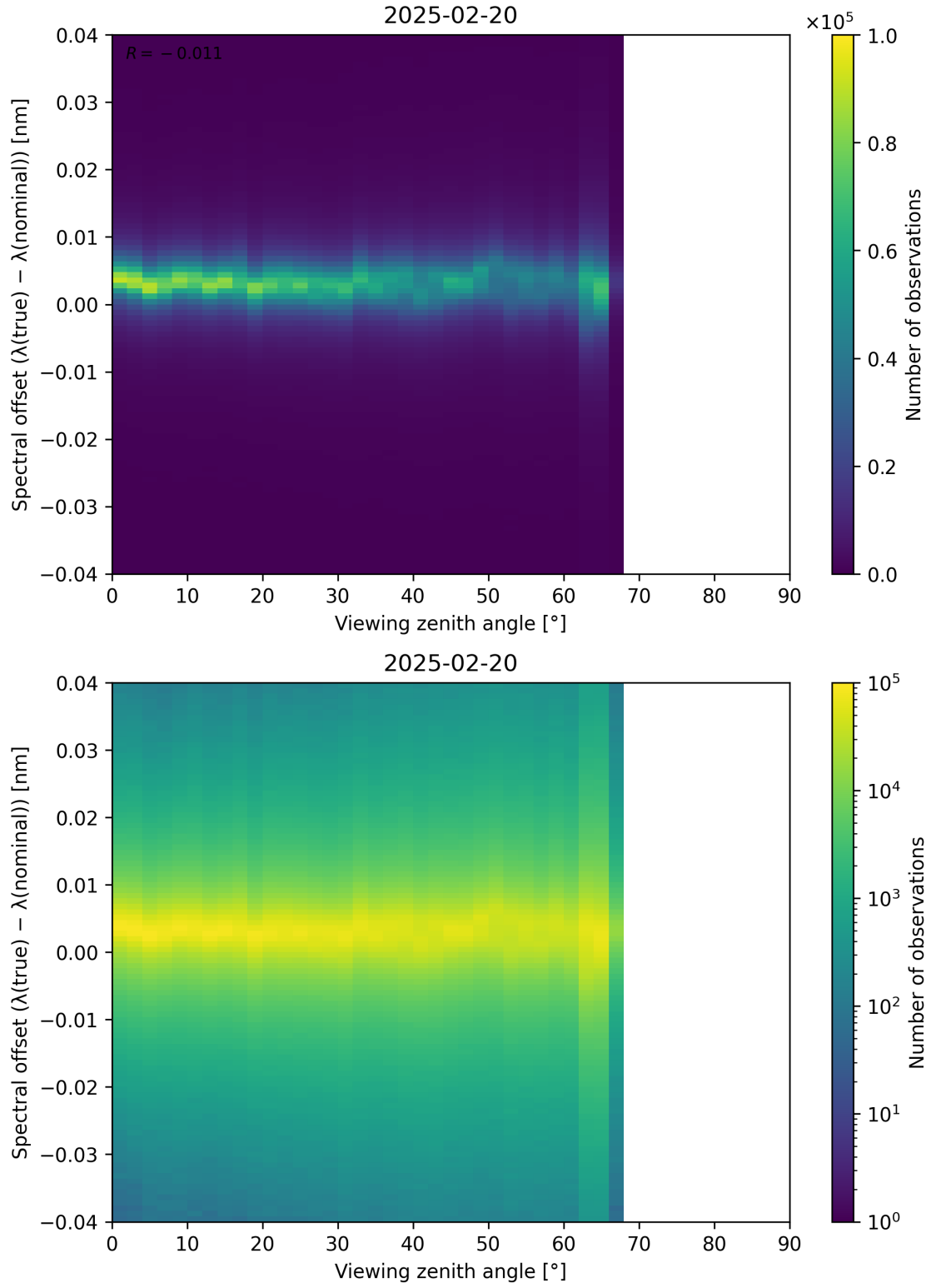
Figure 128: Scatter density plot of “Viewing zenith angle” against “Spectral offset ( \lambda_{\text{true}} - \lambda_{\text{nominal}} )” for 2025-02-19 to 2025-02-21.
