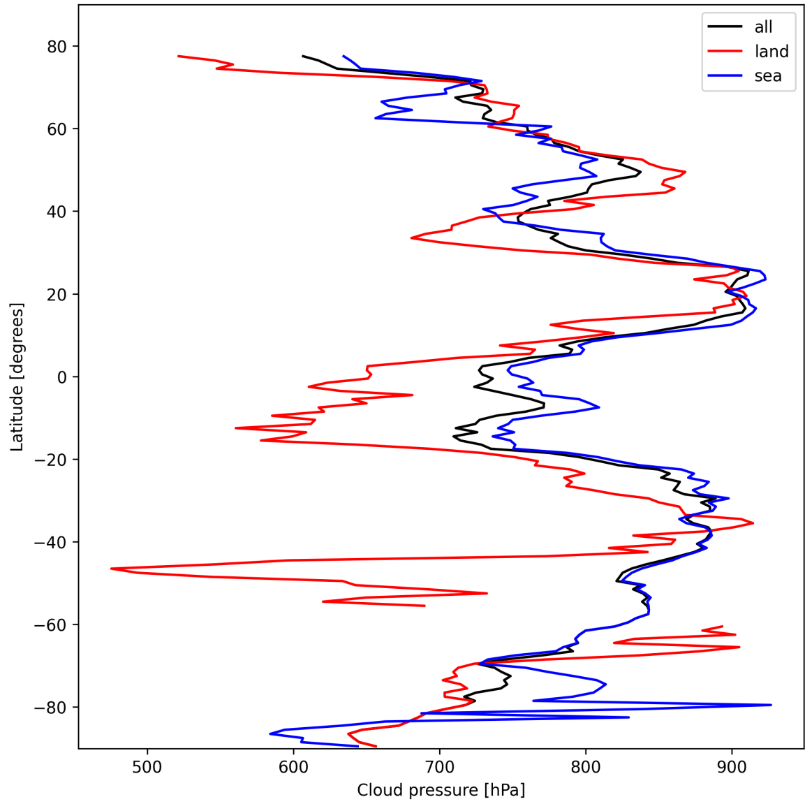
Figure 13: Zonal average of “Cloud pressure” for 2025-02-19 to 2025-02-21.
