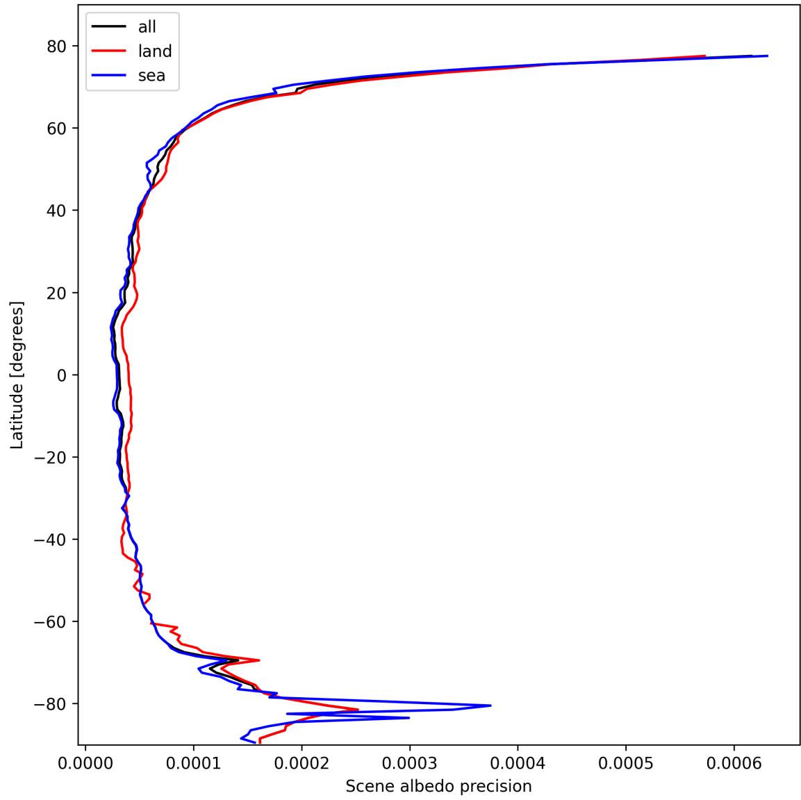
Figure 18: Zonal average of “Scene albedo precision” for 2025-02-19 to 2025-02-21.
