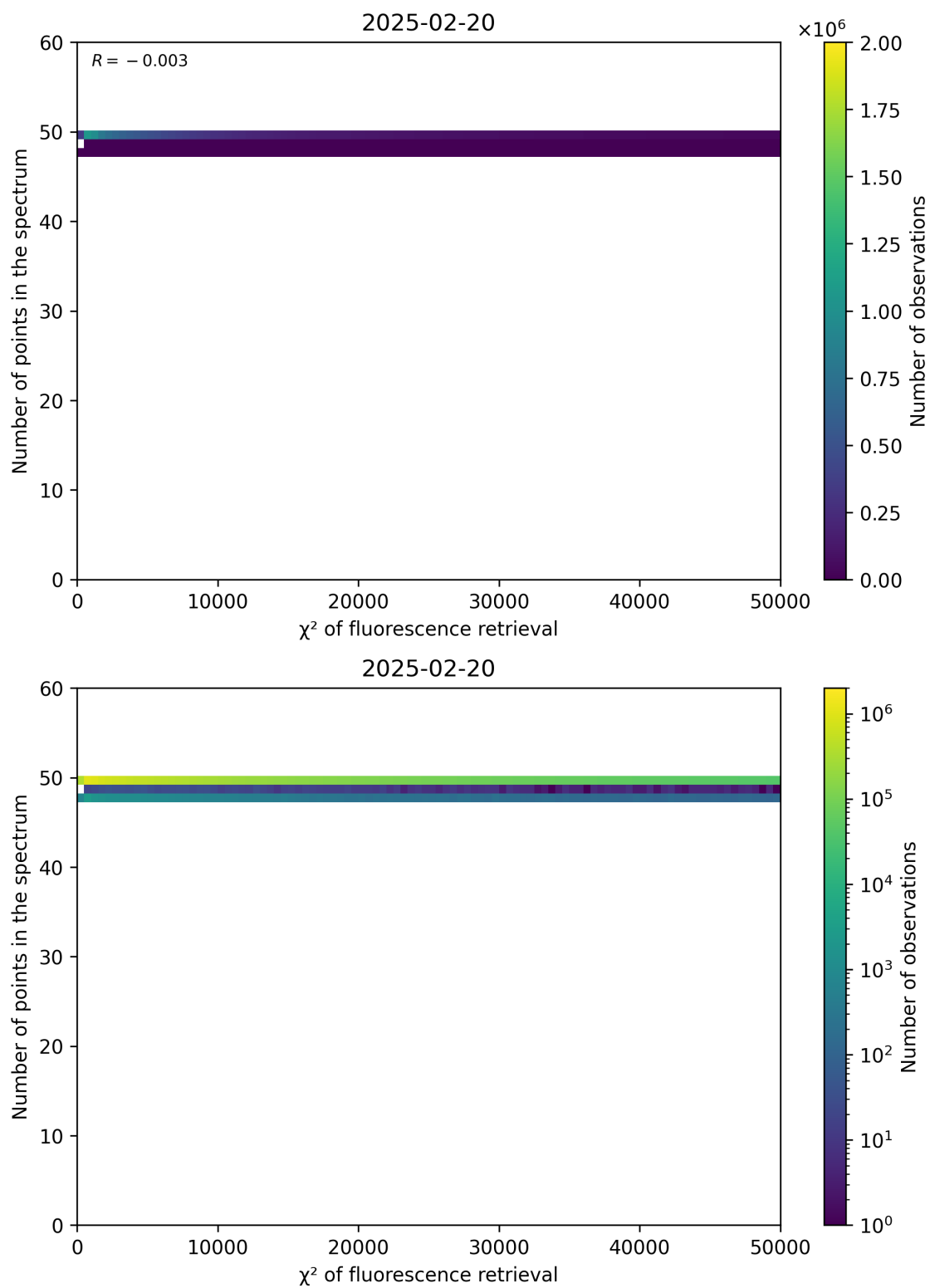
Figure 68: Scatter density plot of “ \chi^2 of fluorescence retrieval” against “Number of points in the spectrum” for 2025-02-19 to 2025-02-21.
