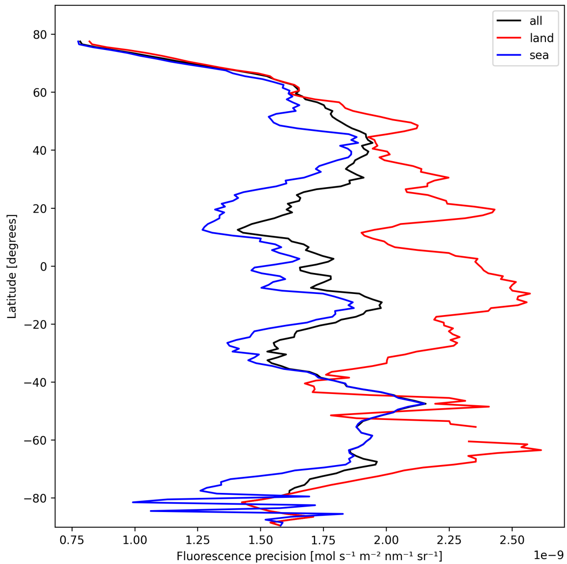
Figure 24: Zonal average of “Fluorescence precision” for 2025-02-19 to 2025-02-21.
