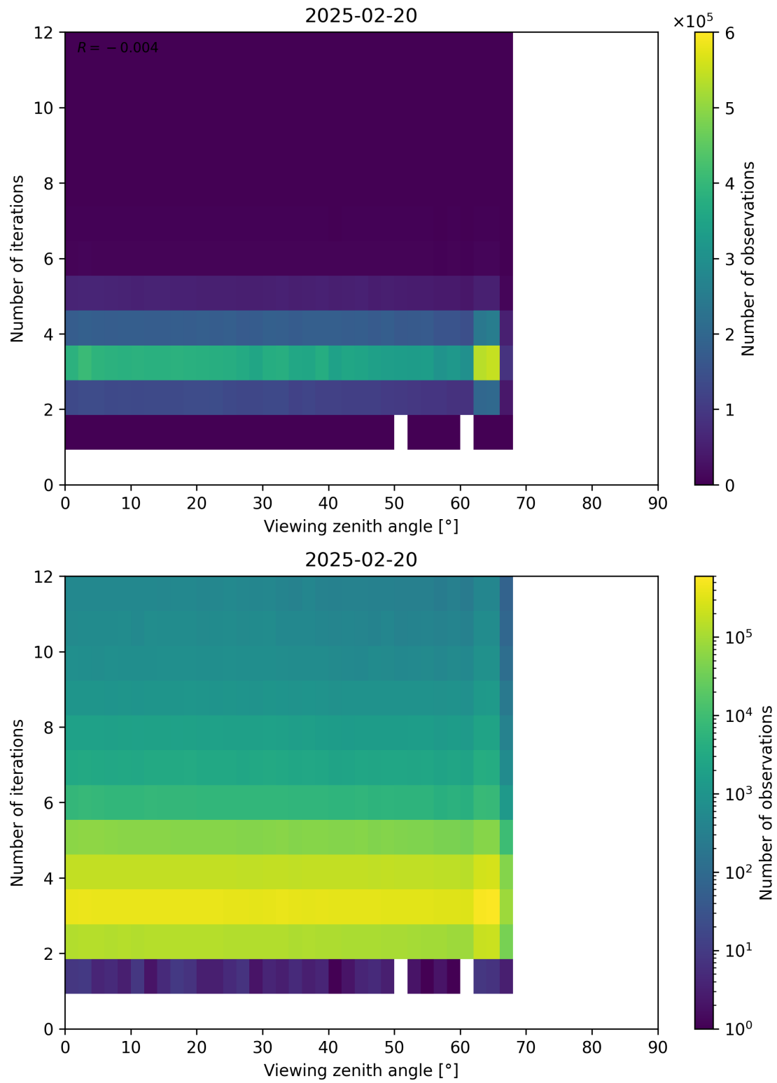
Figure 124: Scatter density plot of “Viewing zenith angle” against “Number of iterations” for 2025-02-19 to 2025-02-21.
