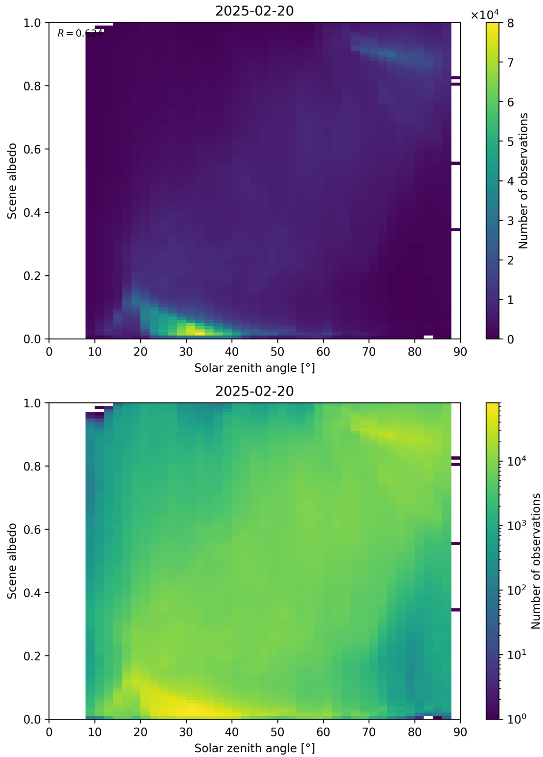
Figure 116: Scatter density plot of “Solar zenith angle” against “Scene albedo” for 2025-02-19 to 2025-02-21.
