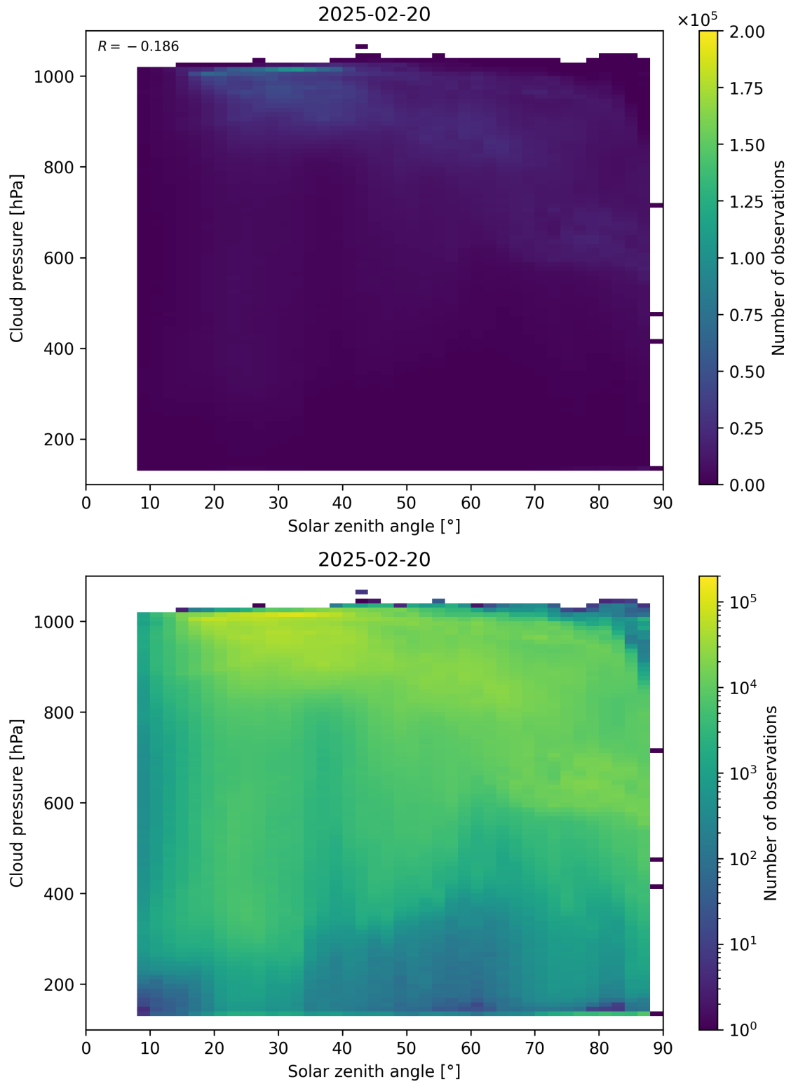
Figure 111: Scatter density plot of “Solar zenith angle” against “Cloud pressure” for 2025-02-19 to 2025-02-21.
