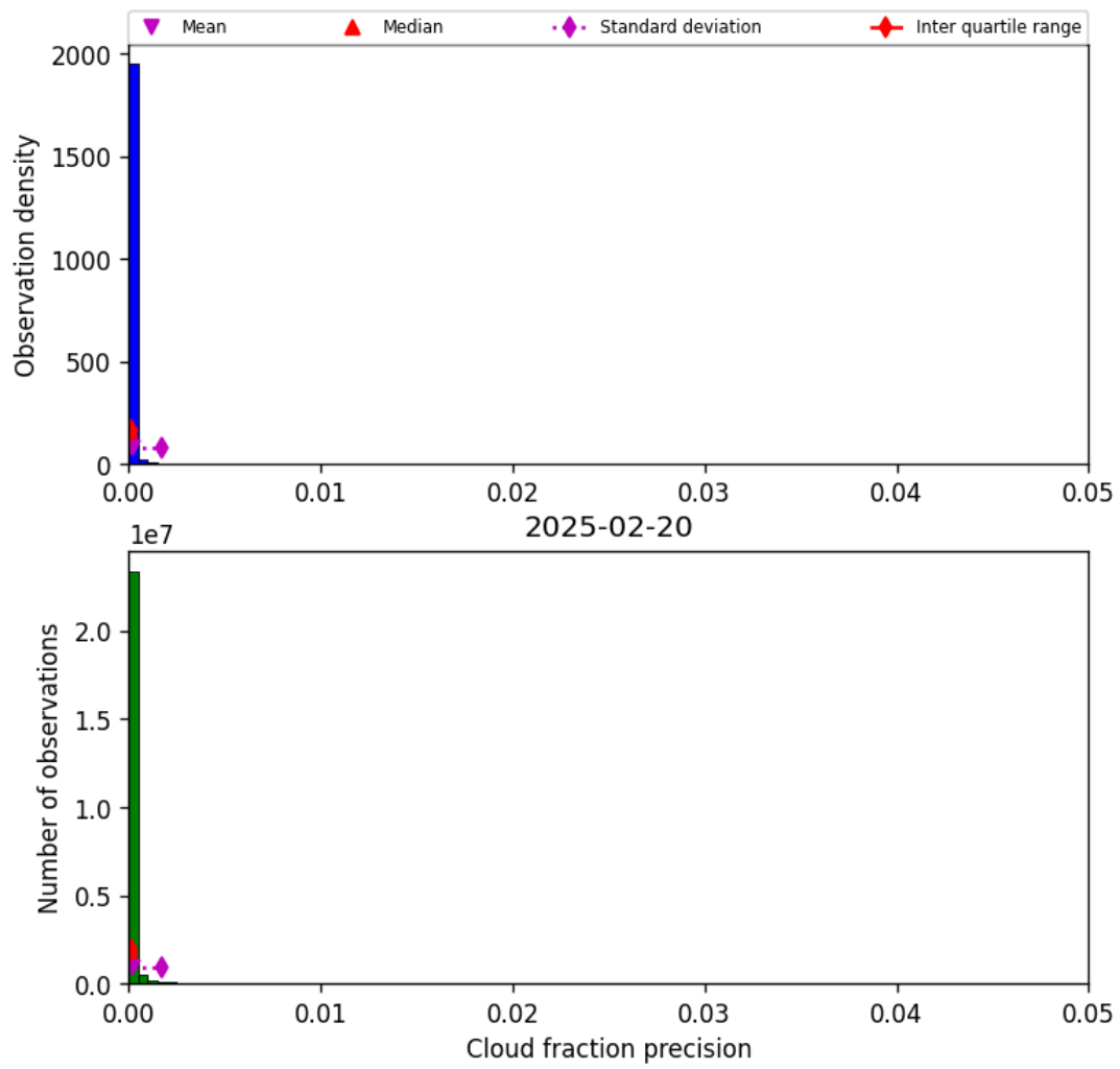
Figure 33: Histogram of “Cloud fraction precision” for 2025-02-19 to 2025-02-21
