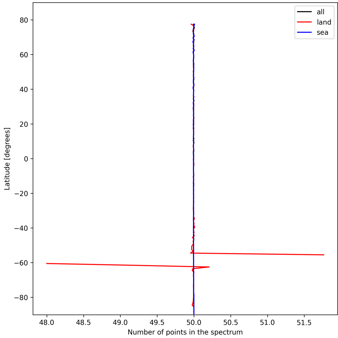
Figure 27: Zonal average of “Number of points in the spectrum” for 2025-02-19 to 2025-02-21.
