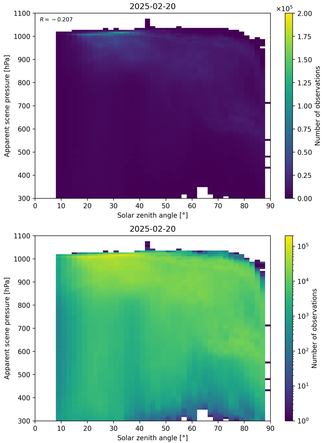
Figure 108: Scatter density plot of “Solar zenith angle” against “Apparent scene pressure” for 2025-02-19 to 2025-02-21.
