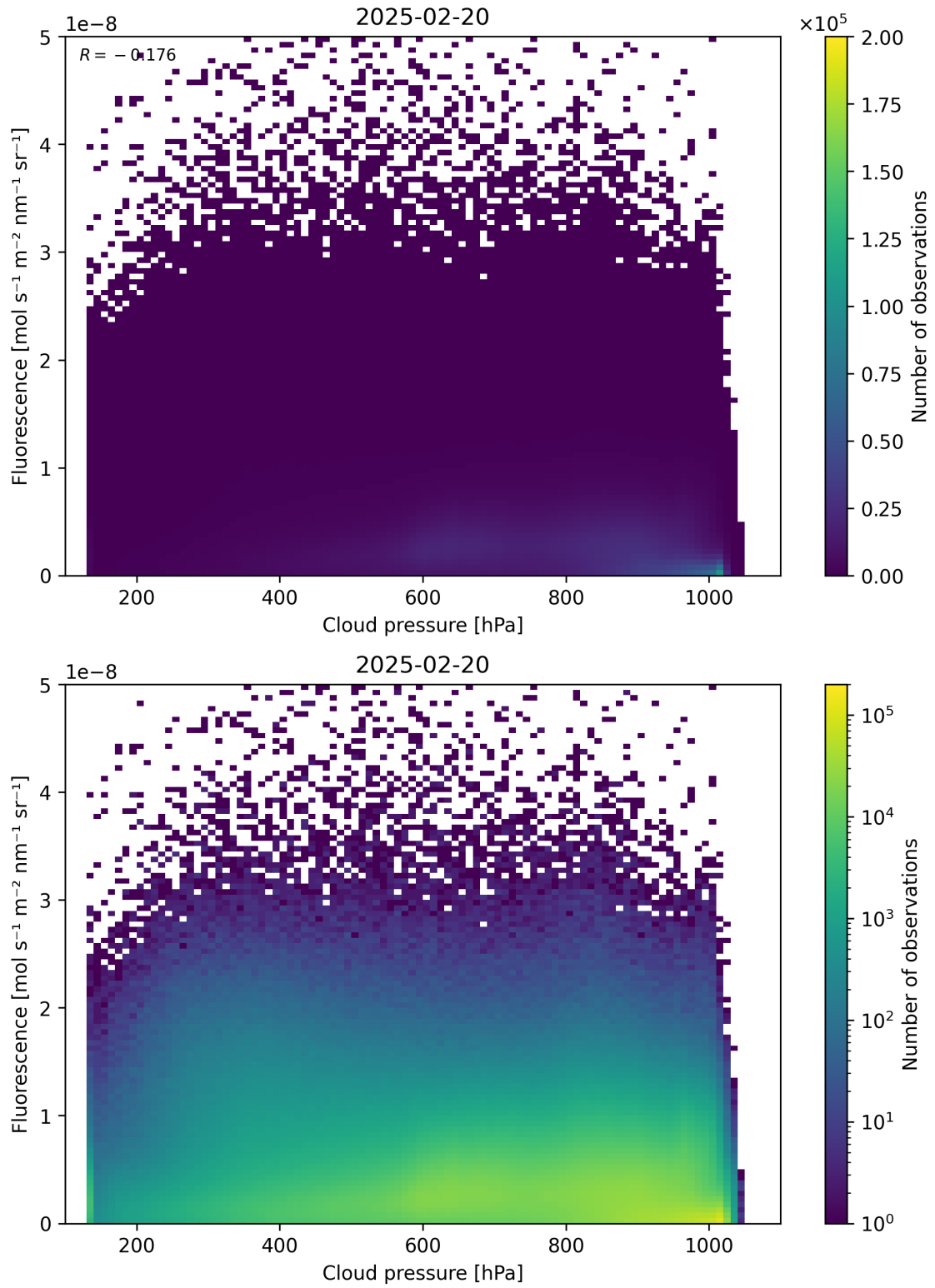
Figure 80: Scatter density plot of “Cloud pressure” against “Fluorescence” for 2025-02-19 to 2025-02-21.
