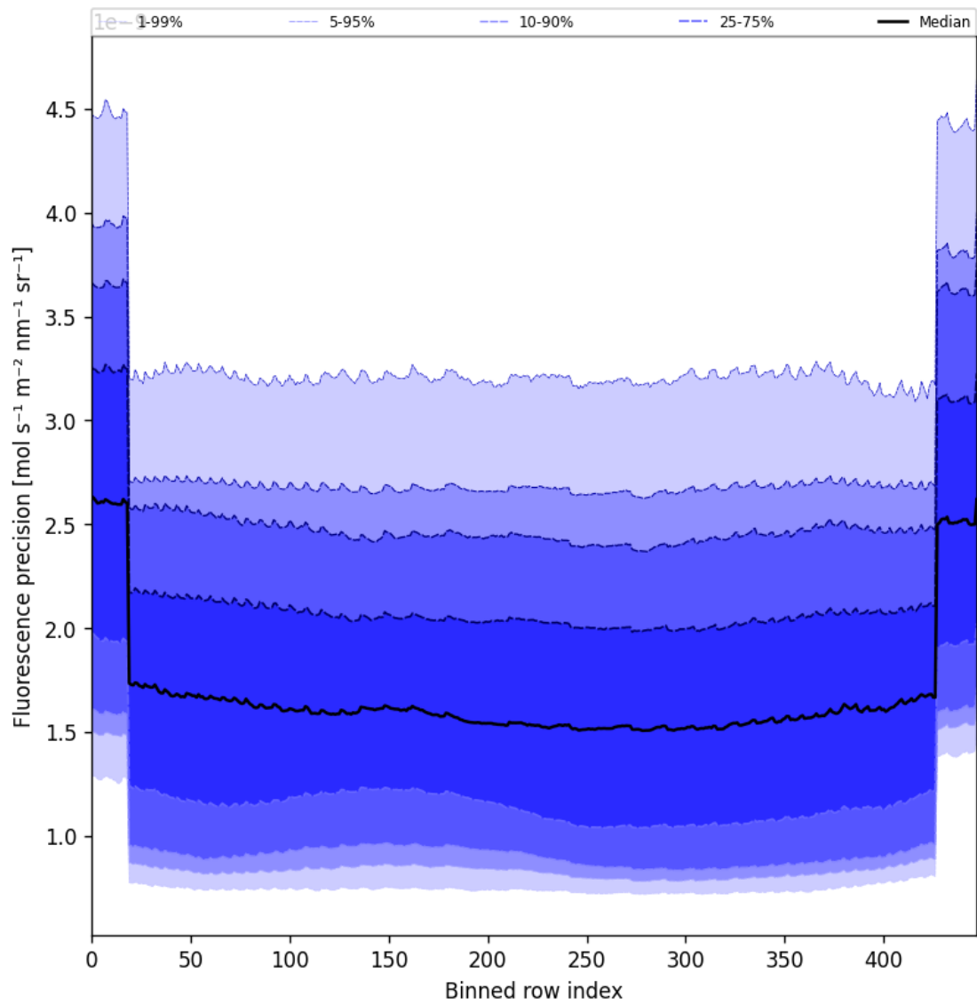
Figure 58: Along track statistics of “Fluorescence precision” for 2025-02-19 to 2025-02-21
