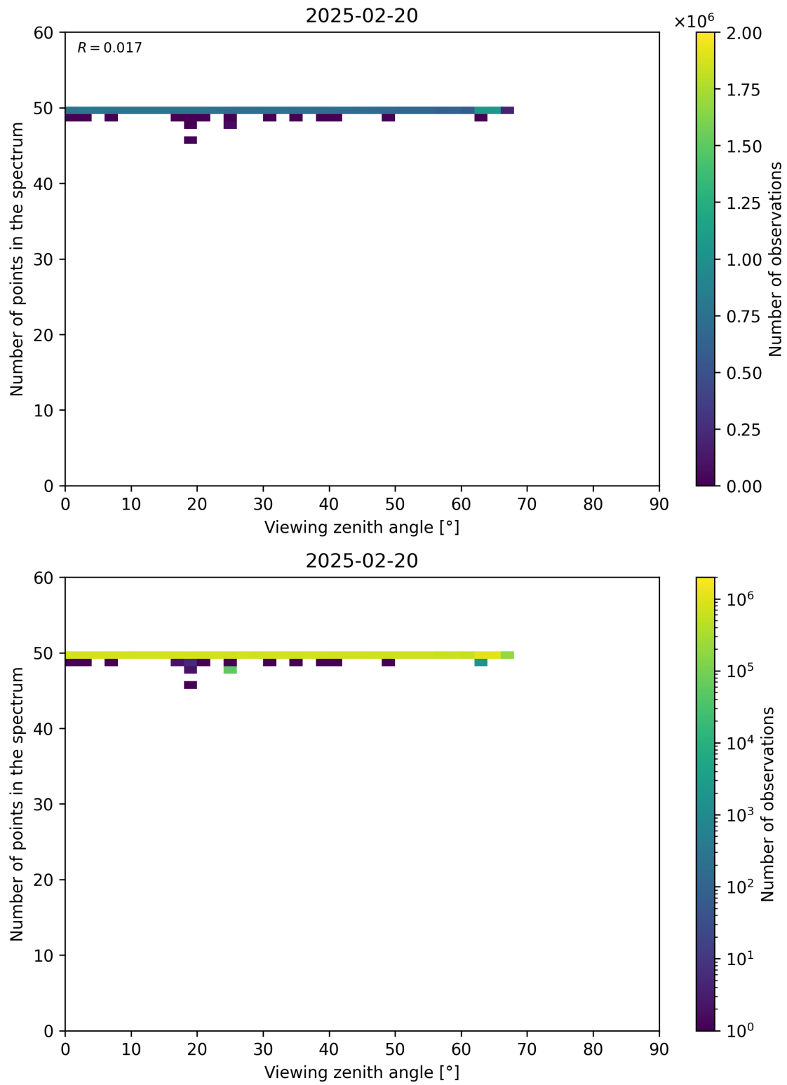
Figure 125: Scatter density plot of “Viewing zenith angle” against “Number of points in the spectrum” for 2025-02-19 to 2025-02-21.
