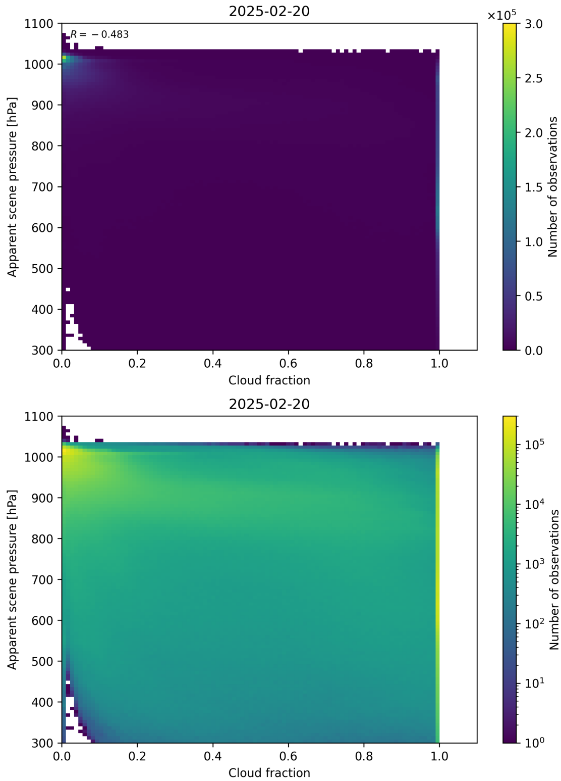
Figure 70: Scatter density plot of “Cloud fraction” against “Apparent scene pressure” for 2025-02-19 to 2025-02-21.
