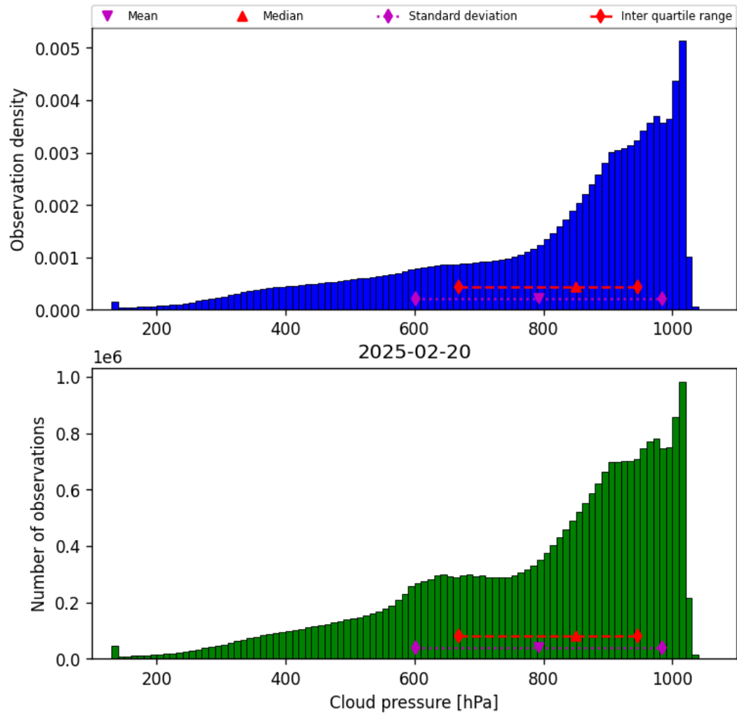
Figure 30: Histogram of “Cloud pressure” for 2025-02-19 to 2025-02-21
