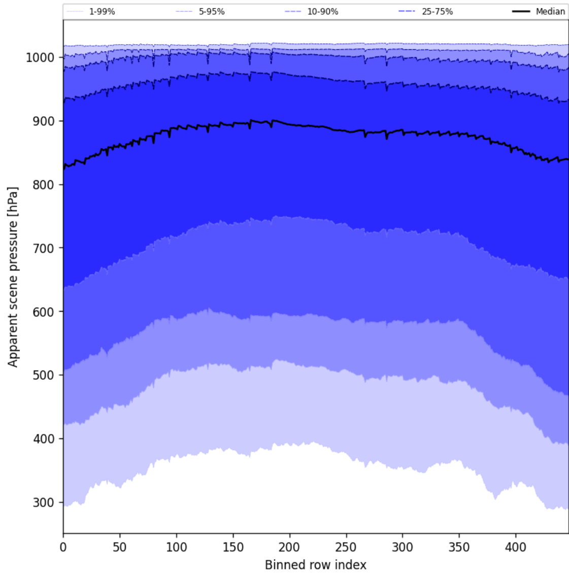
Figure 53: Along track statistics of “Apparent scene pressure” for 2025-02-19 to 2025-02-21
