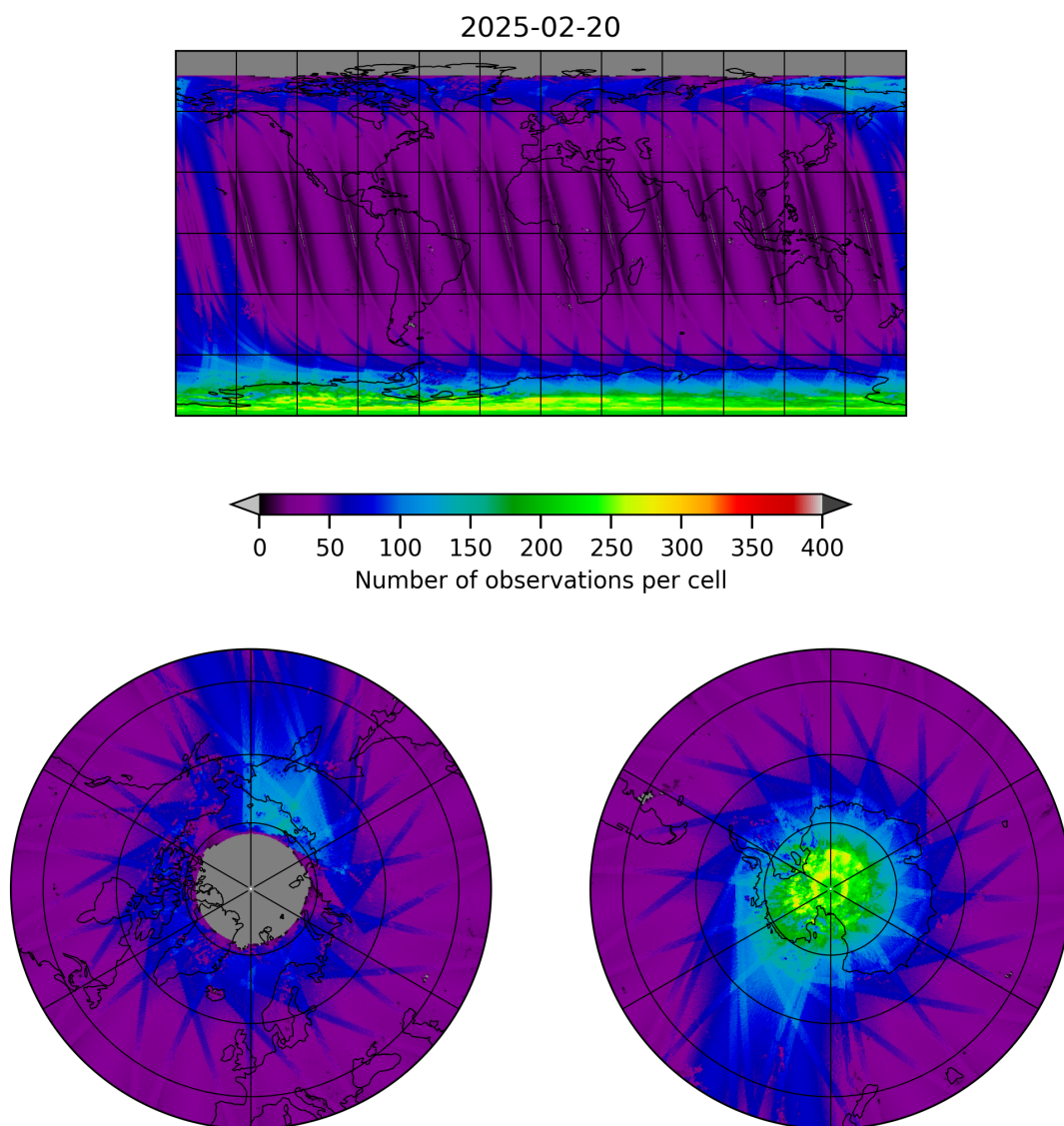
Figure 11: Map of the number of observations for 2025-02-19 to 2025-02-21
