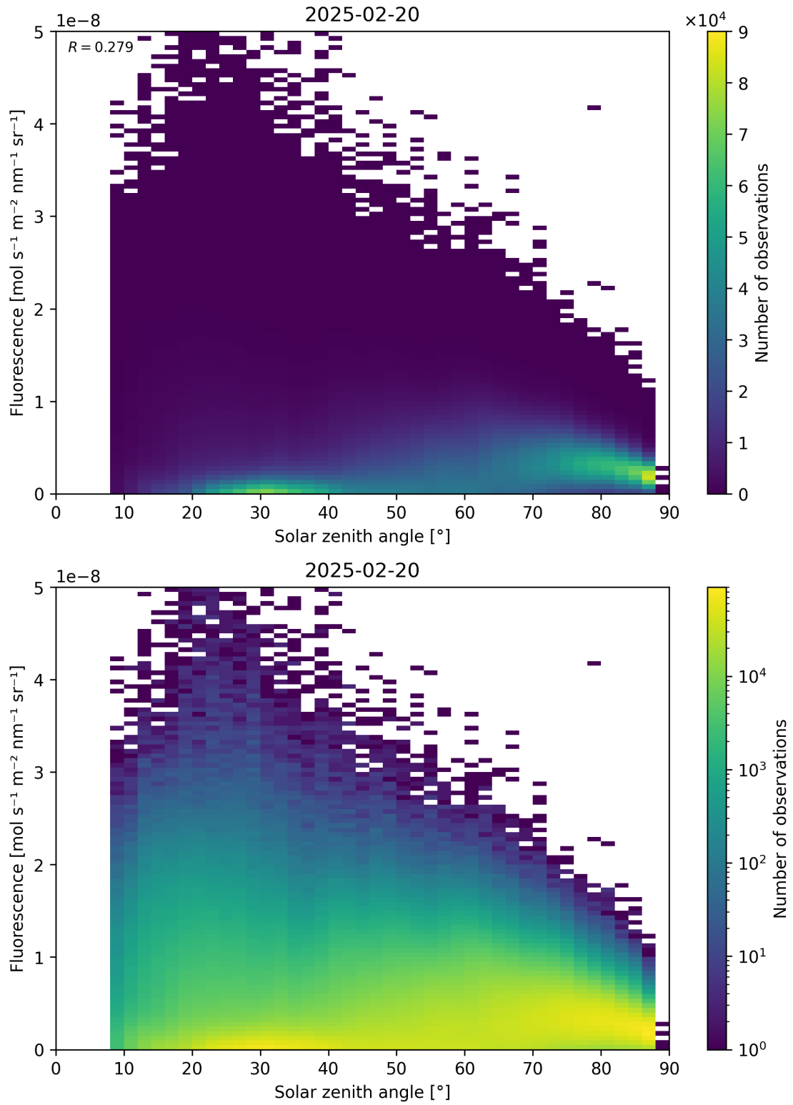
Figure 112: Scatter density plot of “Solar zenith angle” against “Fluorescence” for 2025-02-19 to 2025-02-21.
