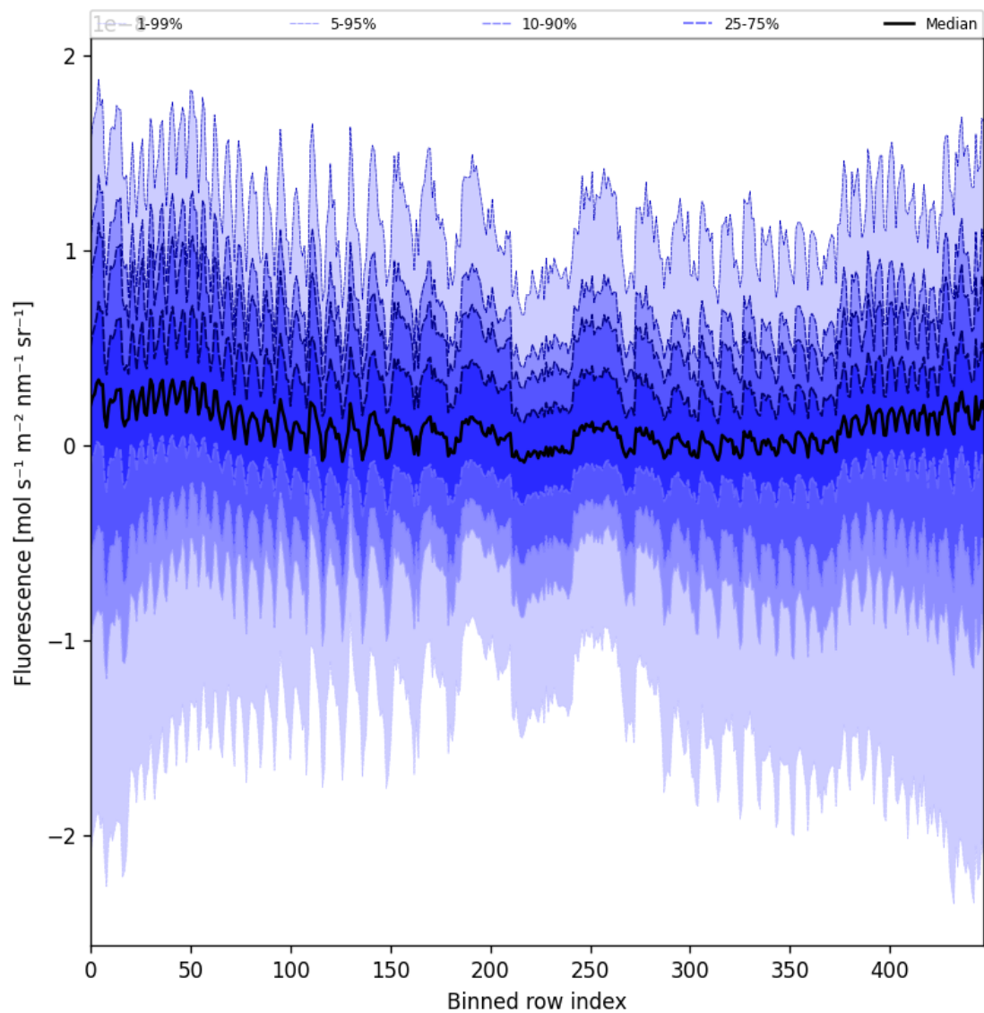
Figure 57: Along track statistics of “Fluorescence” for 2025-02-19 to 2025-02-21
