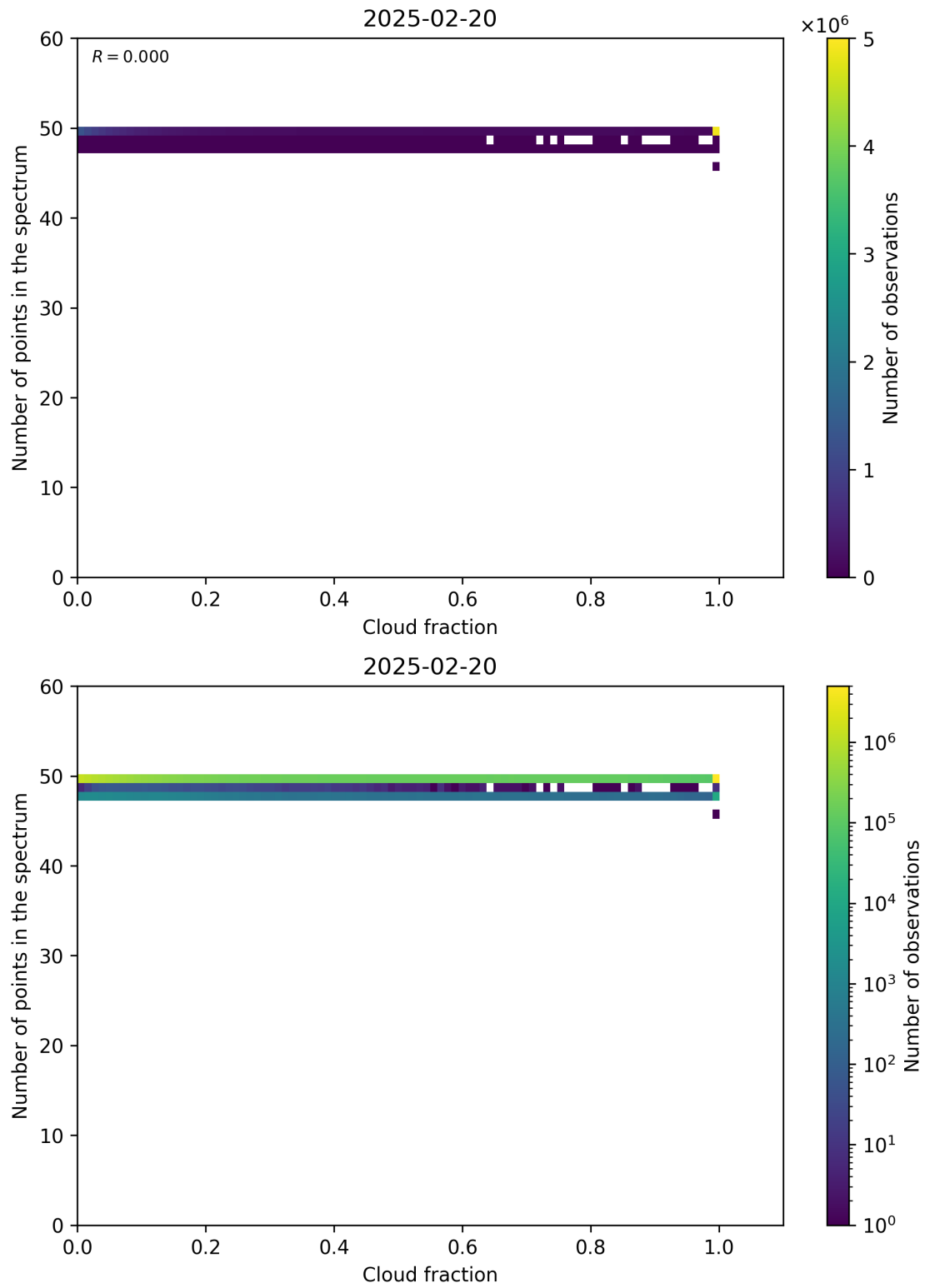
Figure 74: Scatter density plot of “Cloud fraction” against “Number of points in the spectrum” for 2025-02-19 to 2025-02-21.
