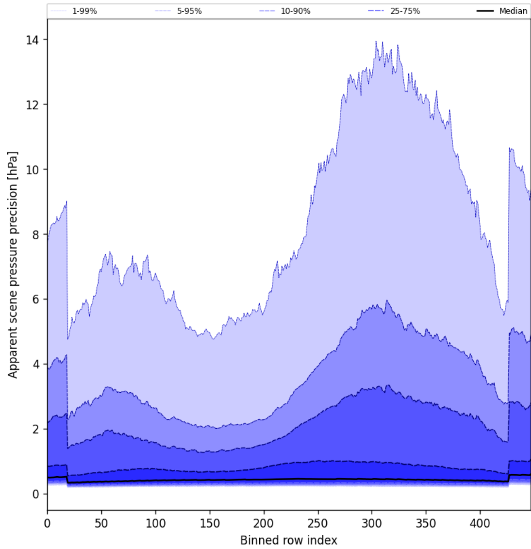
Figure 54: Along track statistics of “Apparent scene pressure precision” for 2025-02-19 to 2025-02-21
