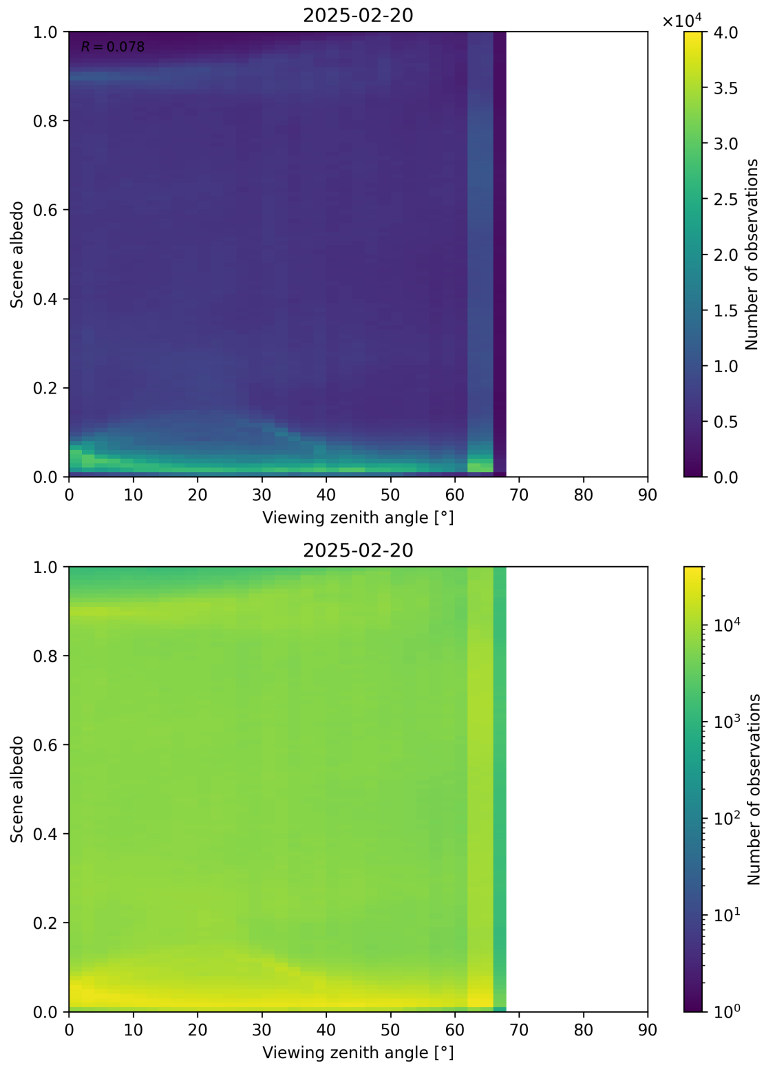
Figure 126: Scatter density plot of “Viewing zenith angle” against “Scene albedo” for 2025-02-19 to 2025-02-21.
