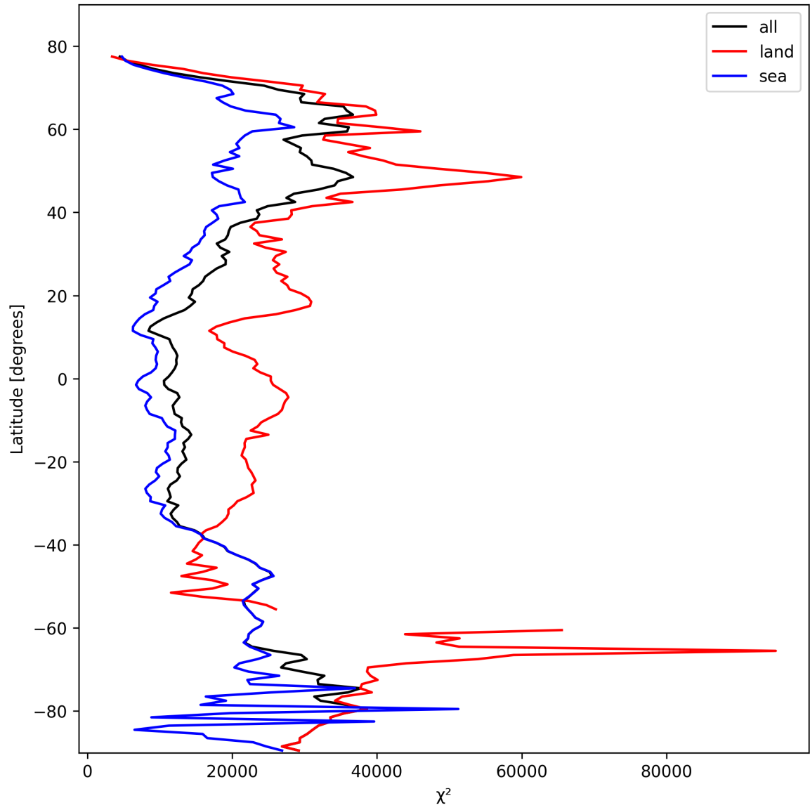
Figure 21: Zonal average of “ \chi^2 ” for 2025-02-19 to 2025-02-21.
