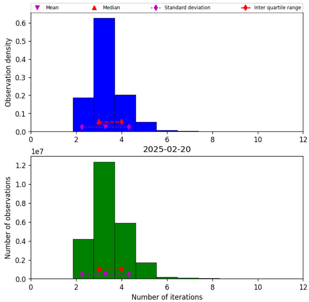
Figure 39: Histogram of “Number of iterations” for 2025-02-19 to 2025-02-21
