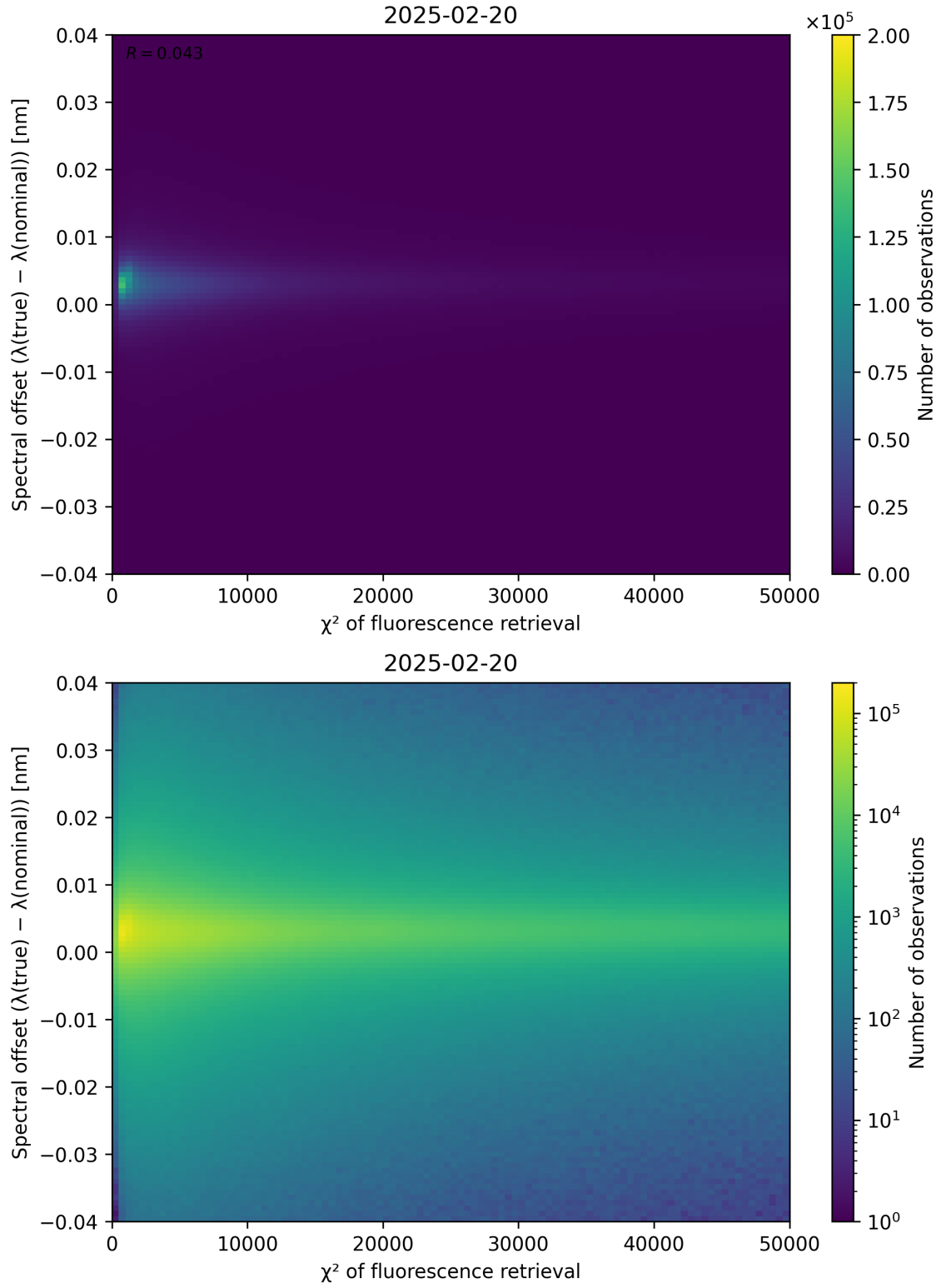
Figure 69: Scatter density plot of “ \chi^2 of fluorescence retrieval” against “Spectral offset ( \lambda_{\text{true}} - \lambda_{\text{nominal}} )” for 2025-02-19 to 2025-02-21.
