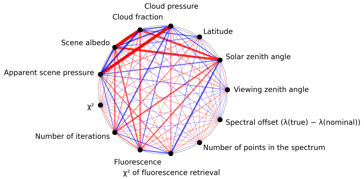
Figure 1: Map of correlation graph for 2025-02-19 to 2025-02-21.
