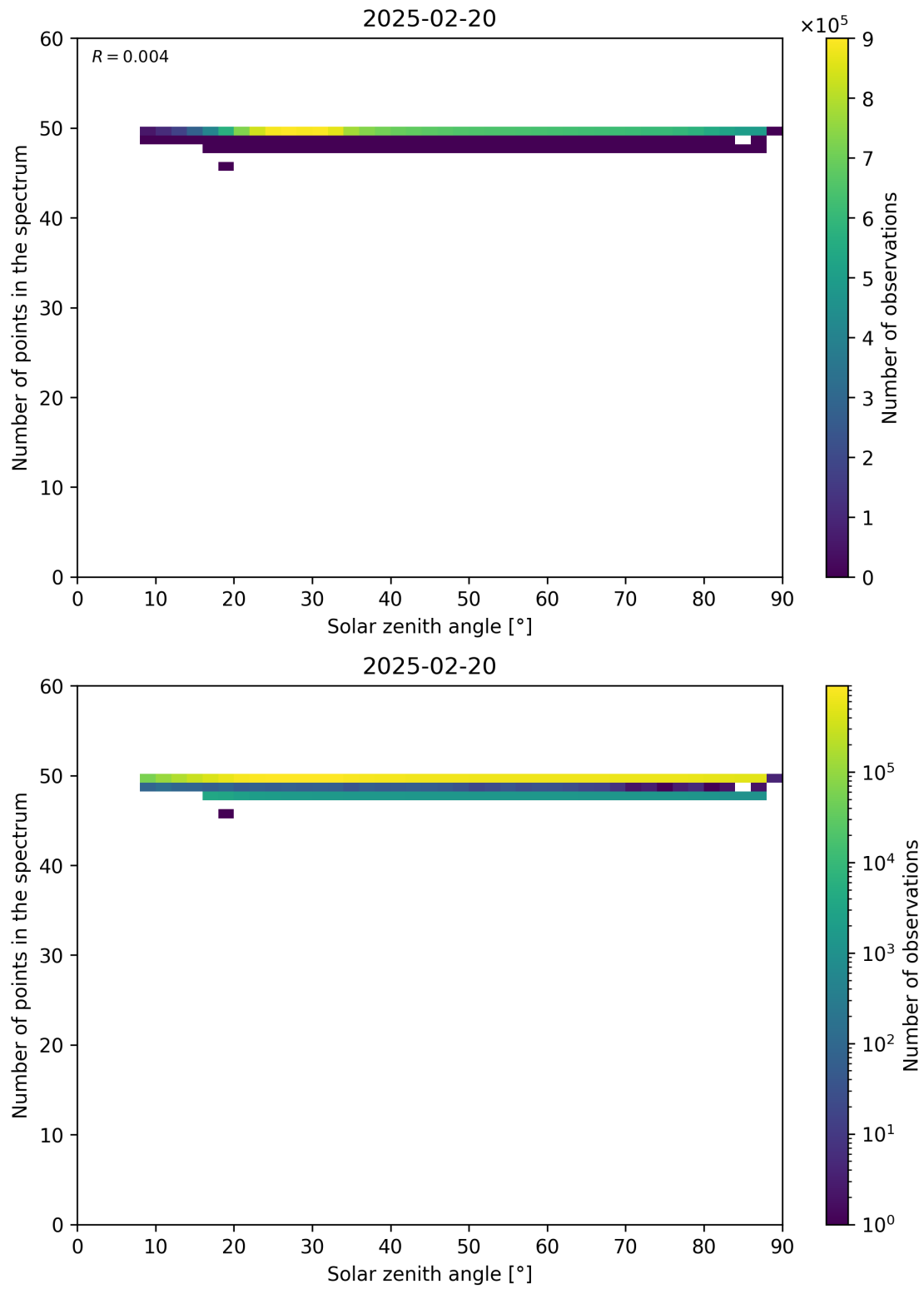
Figure 115: Scatter density plot of “Solar zenith angle” against “Number of points in the spectrum” for 2025-02-19 to 2025-02-21.
