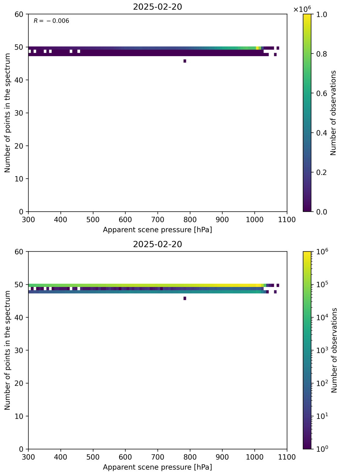
Figure 66: Scatter density plot of “Apparent scene pressure” against “Number of points in the spectrum” for 2025-02-19 to 2025-02-21.
