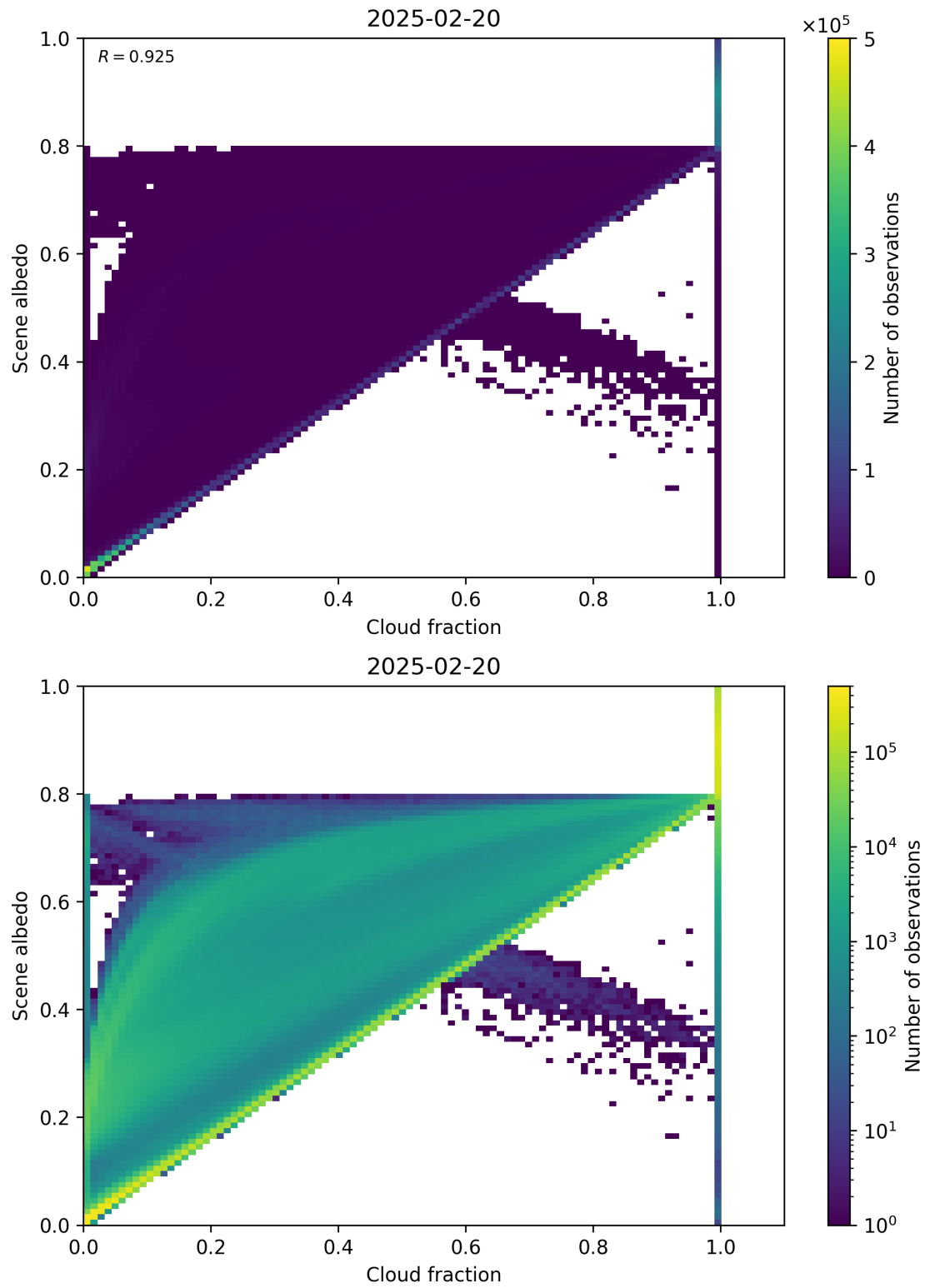
Figure 75: Scatter density plot of “Cloud fraction” against “Scene albedo” for 2025-02-19 to 2025-02-21.
