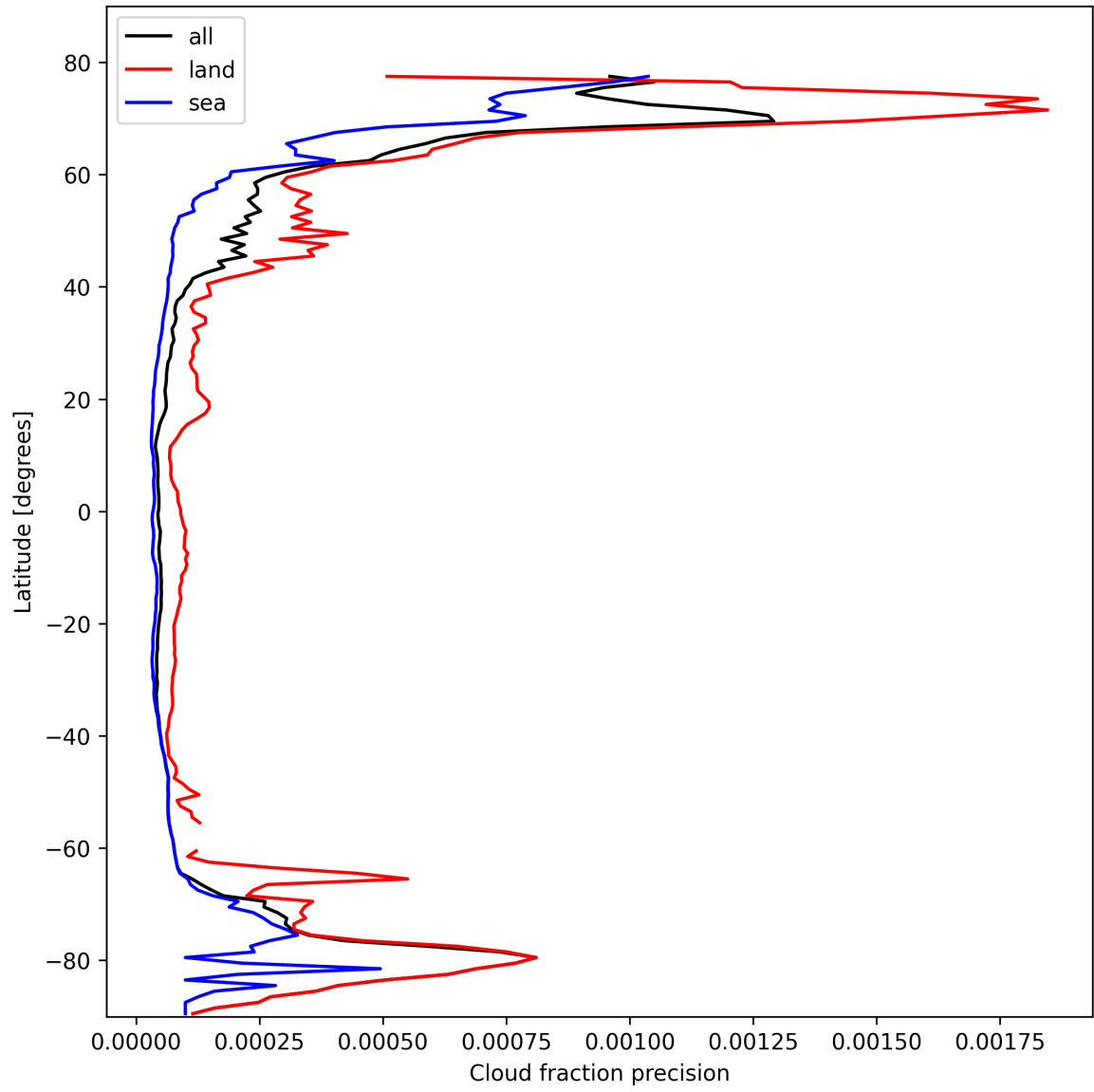
Figure 16: Zonal average of “Cloud fraction precision” for 2025-02-19 to 2025-02-21.
