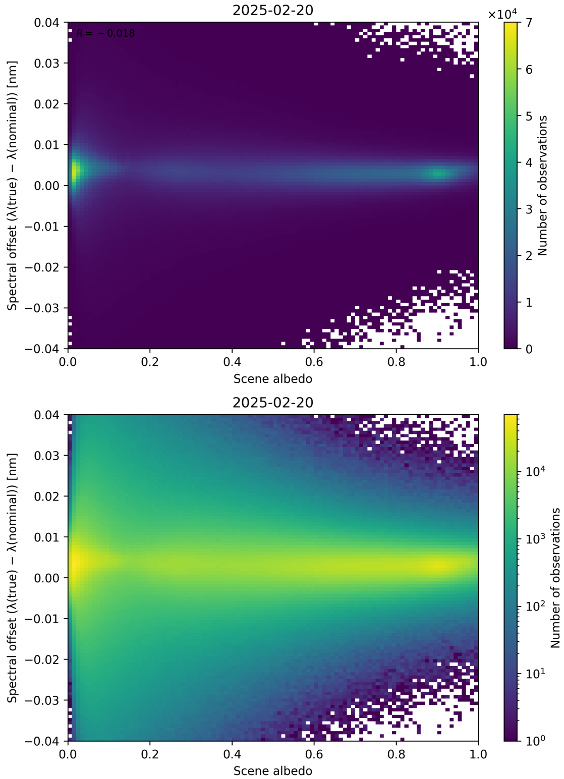
Figure 107: Scatter density plot of “Scene albedo” against “Spectral offset ( \lambda_{\text{true}} - \lambda_{\text{nominal}} )” for 2025-02-19 to 2025-02-21.
