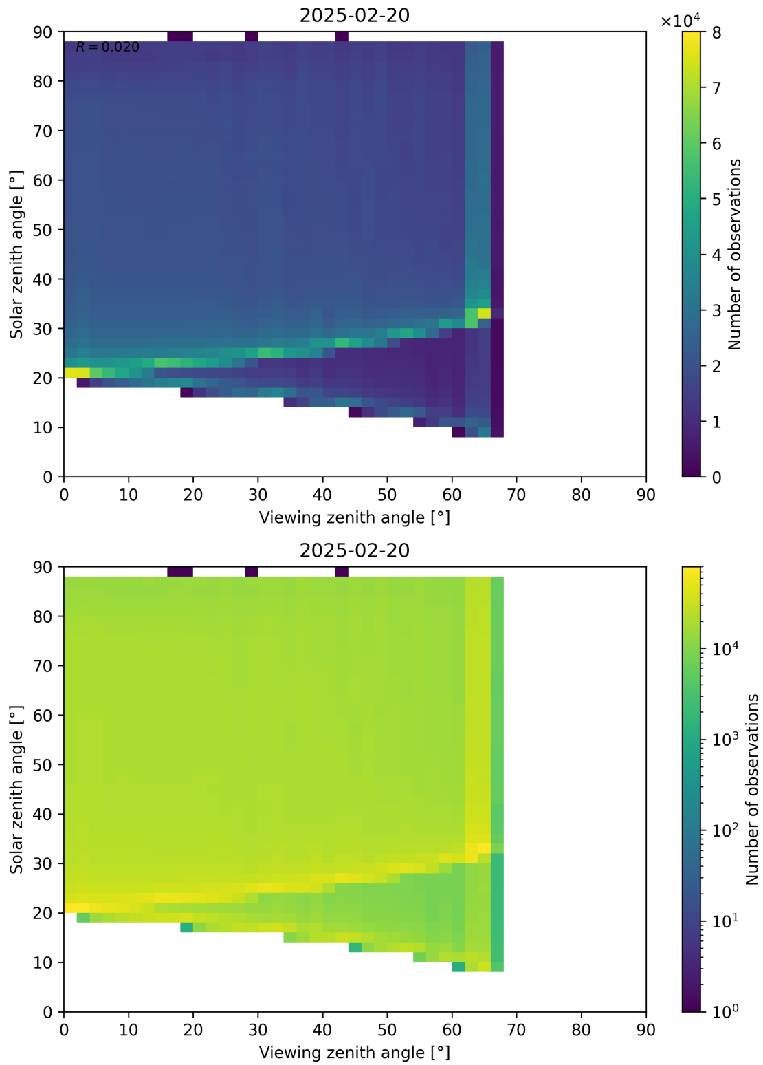
Figure 127: Scatter density plot of “Viewing zenith angle” against “Solar zenith angle” for 2025-02-19 to 2025-02-21.
