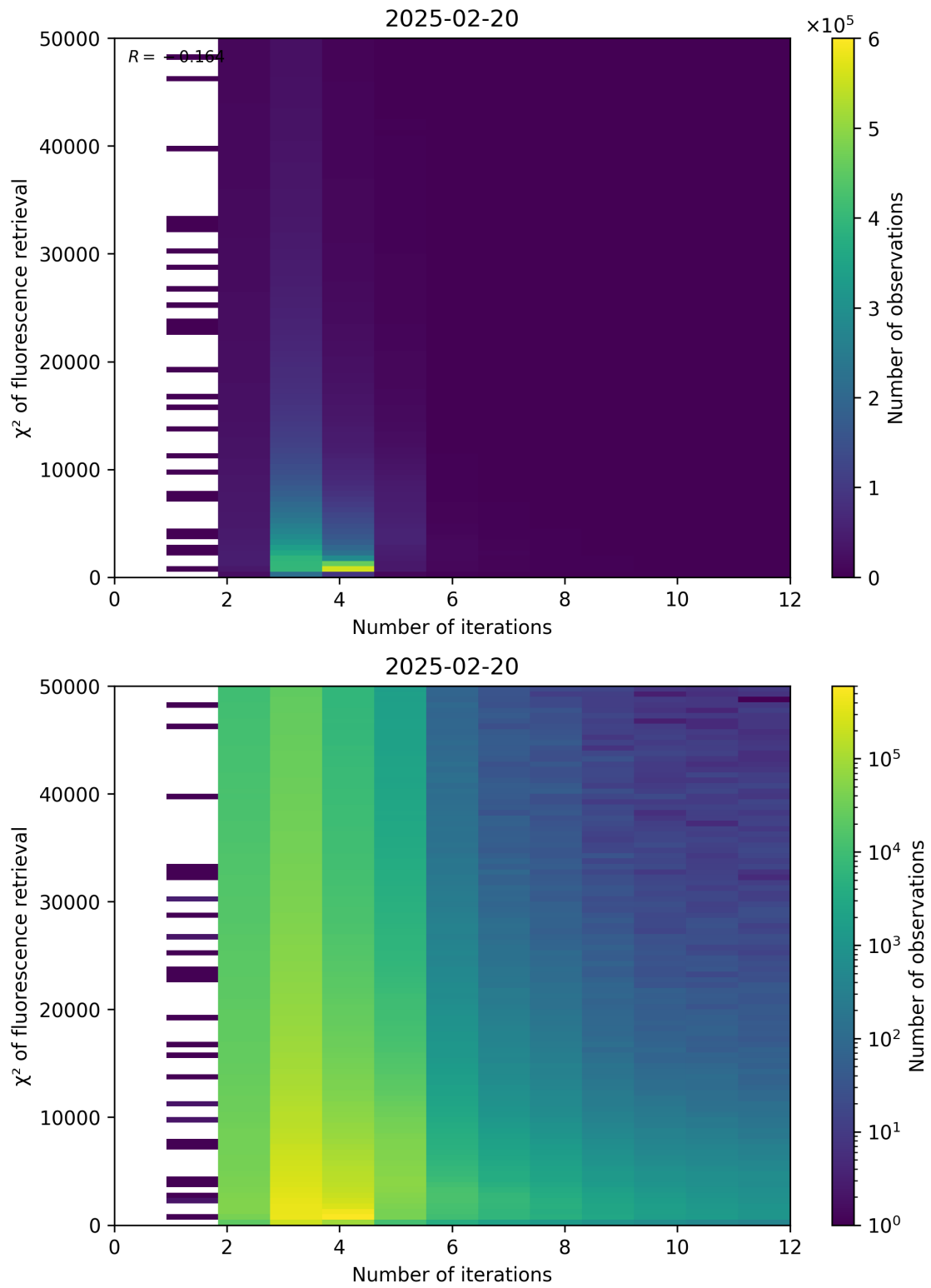
Figure 97: Scatter density plot of “Number of iterations” against “ \chi^2 of fluorescence retrieval” for 2025-02-19 to 2025-02-21.
