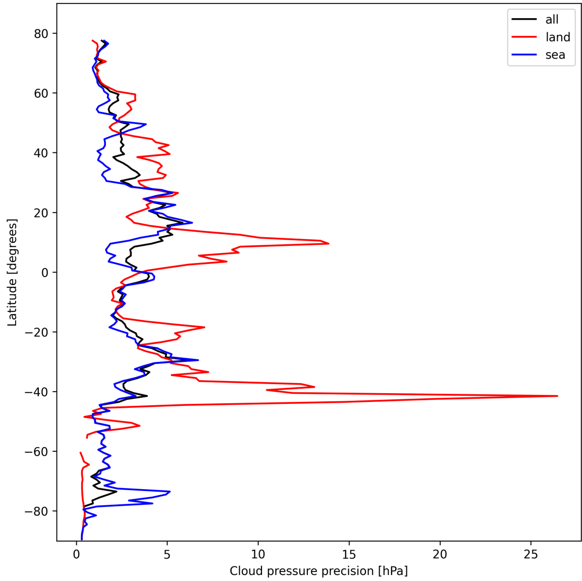
Figure 14: Zonal average of "Cloud pressure precision" for 2025-02-19 to 2025-02-21.
