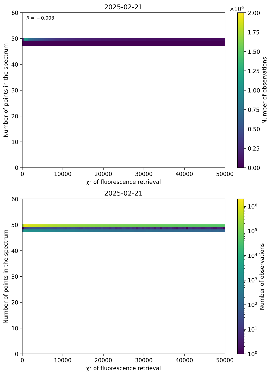
Figure 68: Scatter density plot of " \chi^2 of fluorescence retrieval" against "Number of points in the spectrum" for 2025-02-20 to 2025-02-22.
