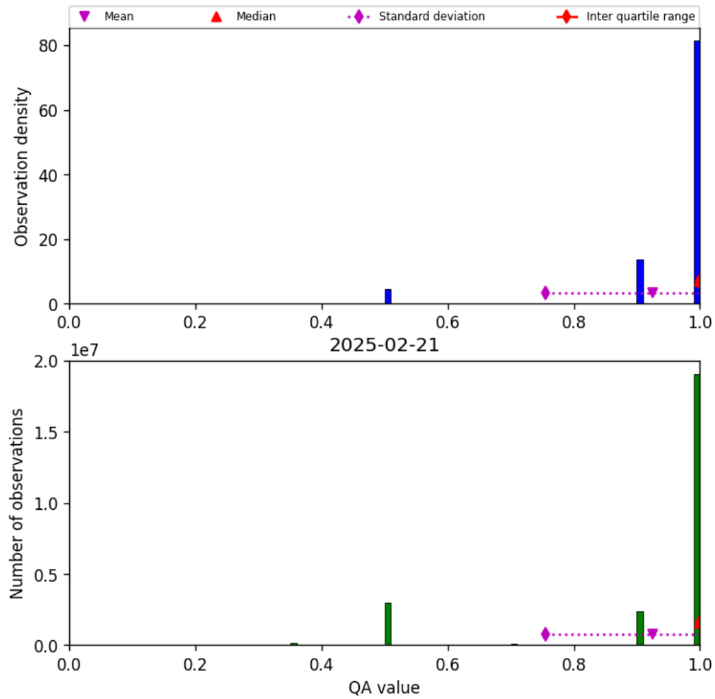
Figure 29: Histogram of “QA value” for 2025-02-20 to 2025-02-22
