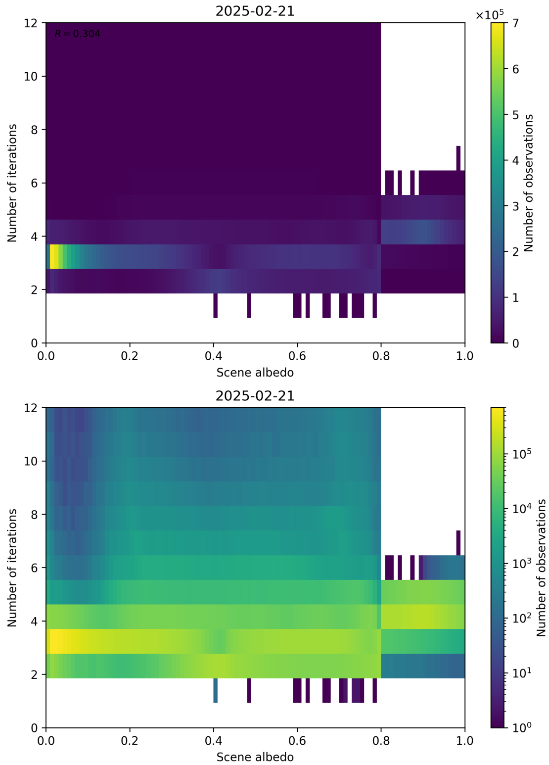
Figure 105: Scatter density plot of “Scene albedo” against “Number of iterations” for 2025-02-20 to 2025-02-22.
