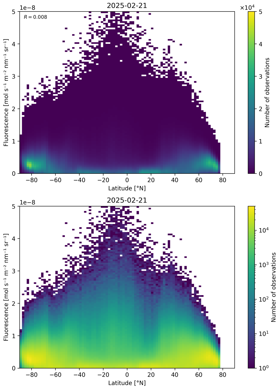
Figure 92: Scatter density plot of “Latitude” against “Fluorescence” for 2025-02-20 to 2025-02-22.
