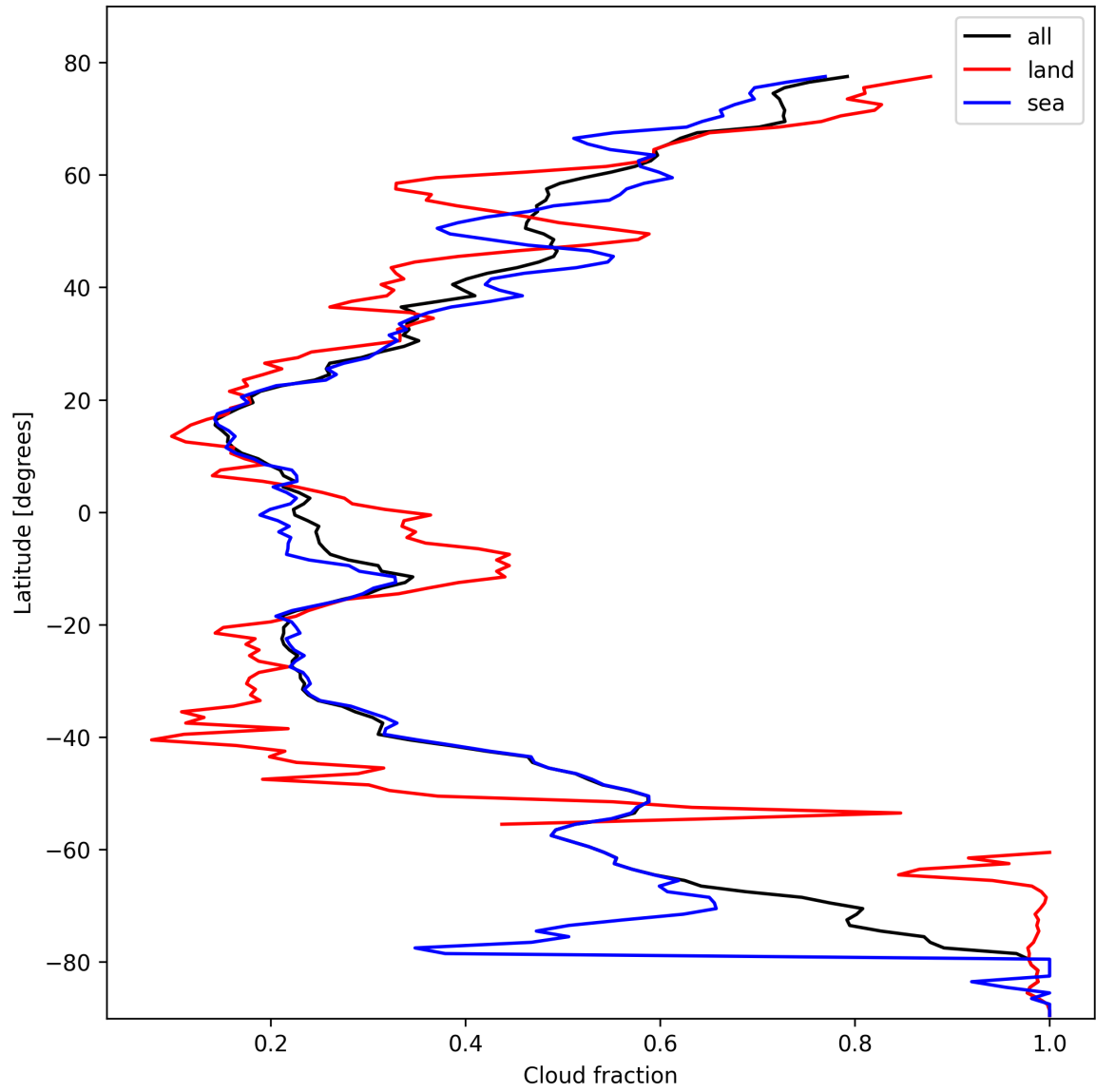
Figure 15: Zonal average of “Cloud fraction” for 2025-02-20 to 2025-02-22.
