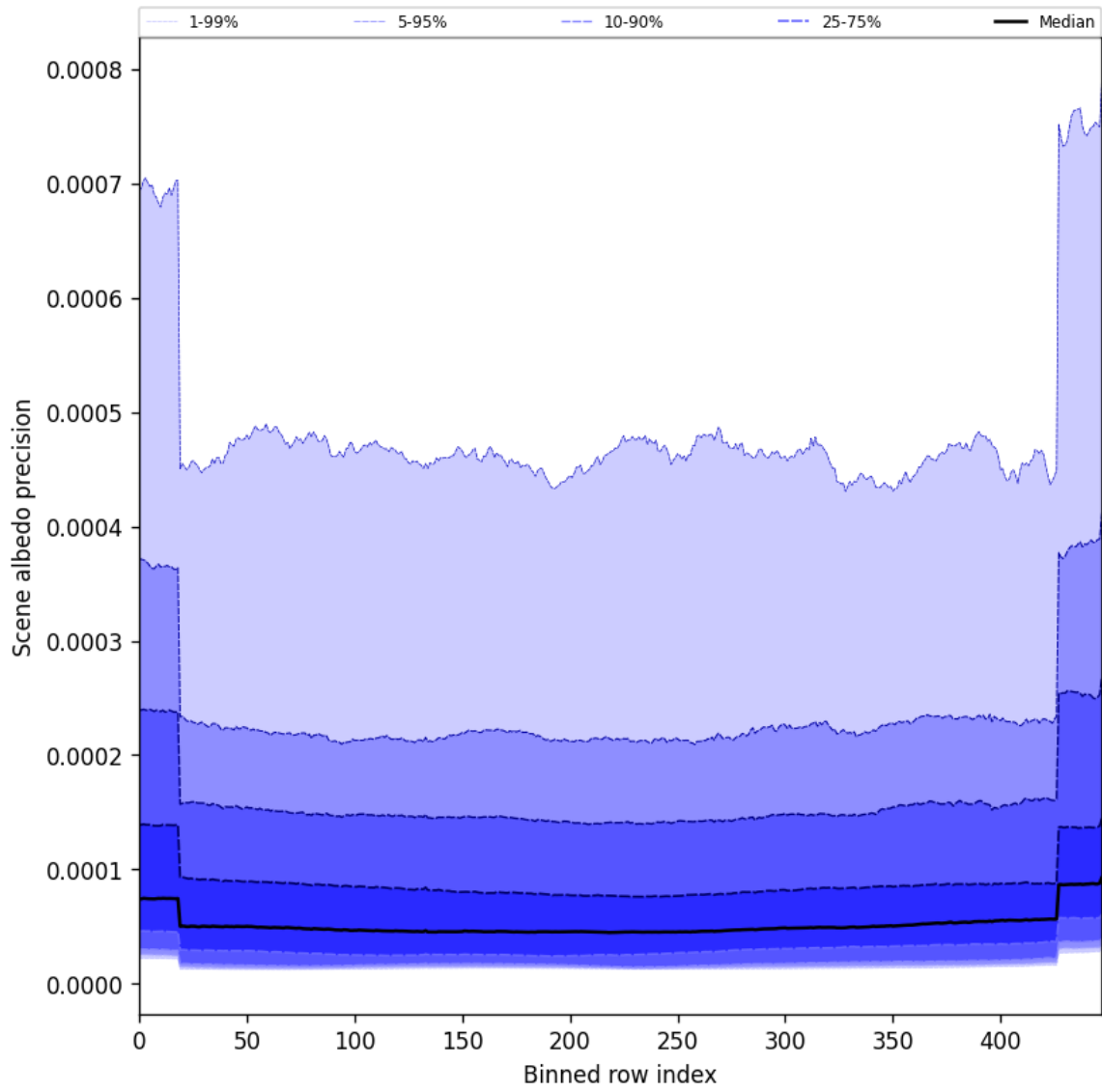
Figure 52: Along track statistics of “Scene albedo precision” for 2025-02-20 to 2025-02-22
