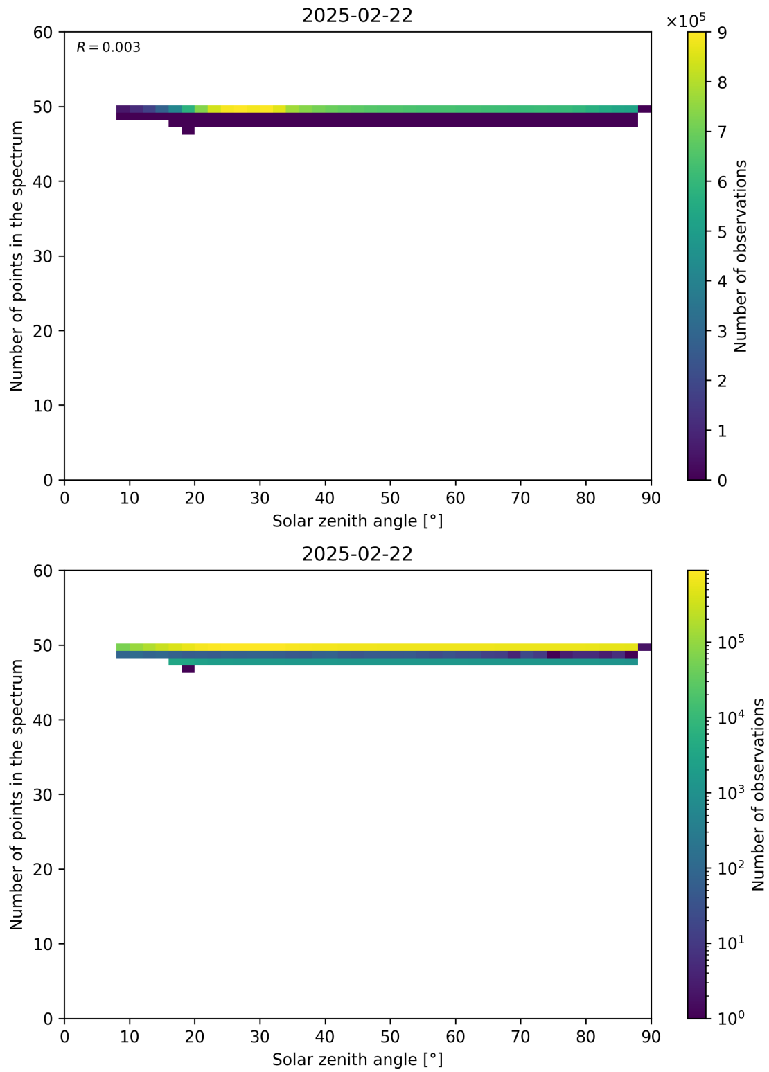
Figure 115: Scatter density plot of “Solar zenith angle” against “Number of points in the spectrum” for 2025-02-21 to 2025-02-23.
