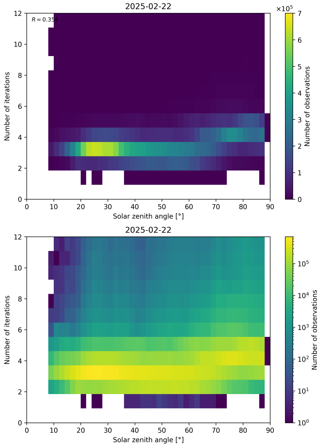
Figure 114: Scatter density plot of “Solar zenith angle” against “Number of iterations” for 2025-02-21 to 2025-02-23.
