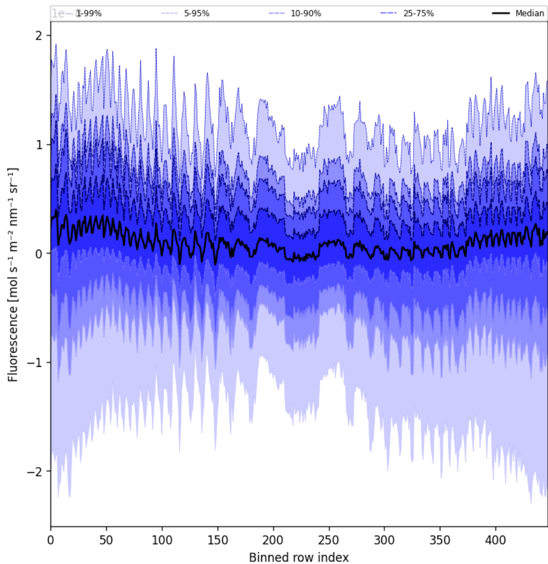
Figure 57: Along track statistics of “Fluorescence” for 2025-02-21 to 2025-02-23
