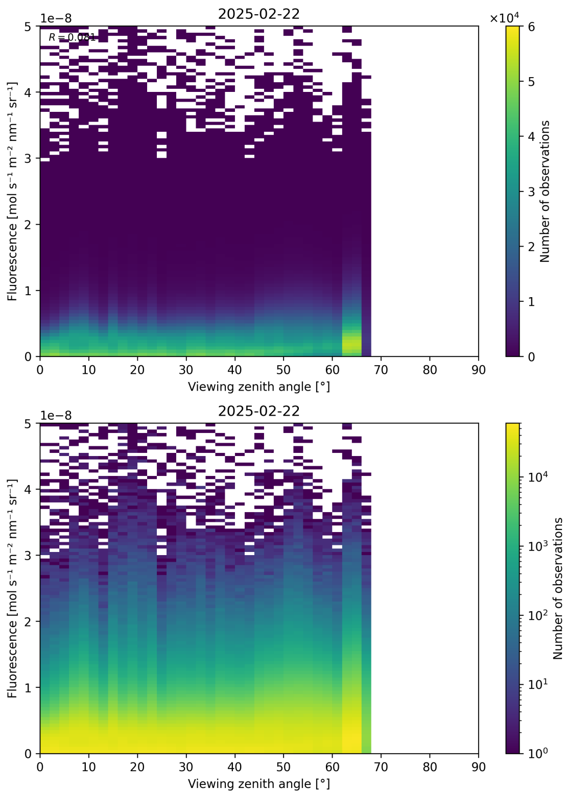
Figure 122: Scatter density plot of “Viewing zenith angle” against “Fluorescence” for 2025-02-21 to 2025-02-23.
