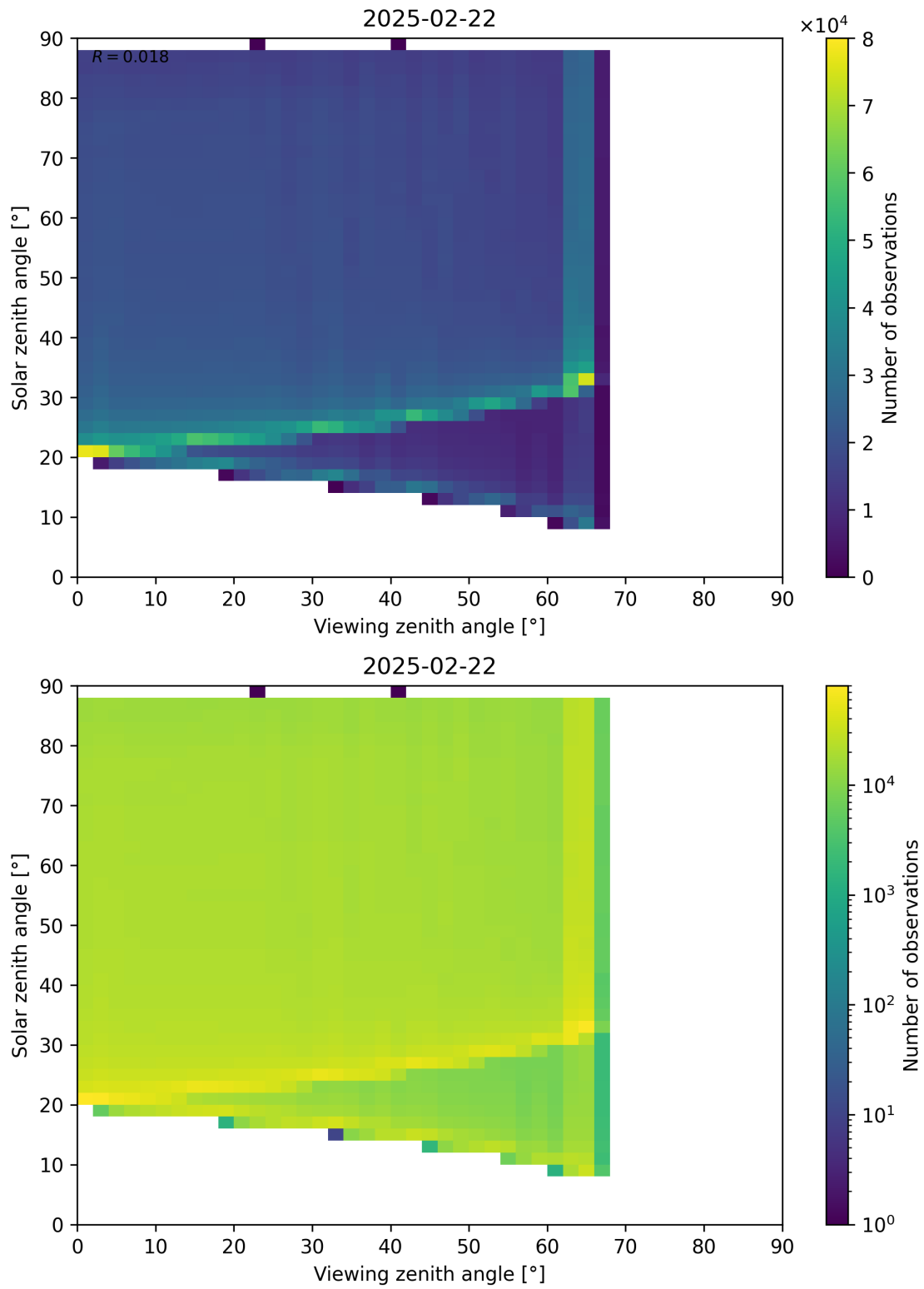
Figure 127: Scatter density plot of “Viewing zenith angle” against “Solar zenith angle” for 2025-02-21 to 2025-02-23.
