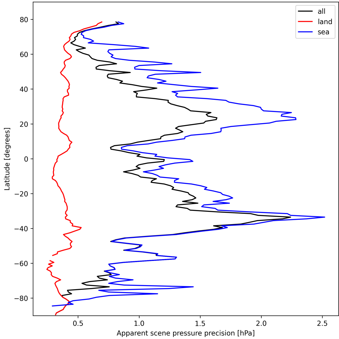
Figure 20: Zonal average of “Apparent scene pressure precision” for 2025-02-21 to 2025-02-23.
