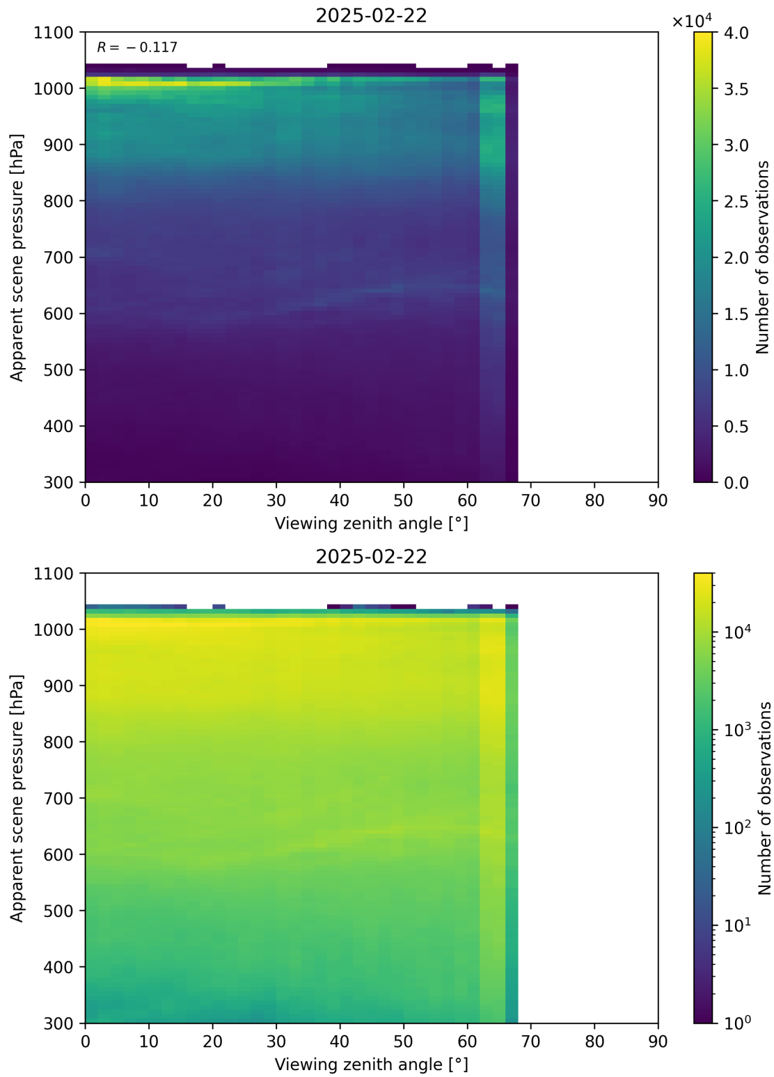
Figure 118: Scatter density plot of “Viewing zenith angle” against “Apparent scene pressure” for 2025-02-21 to 2025-02-23.
