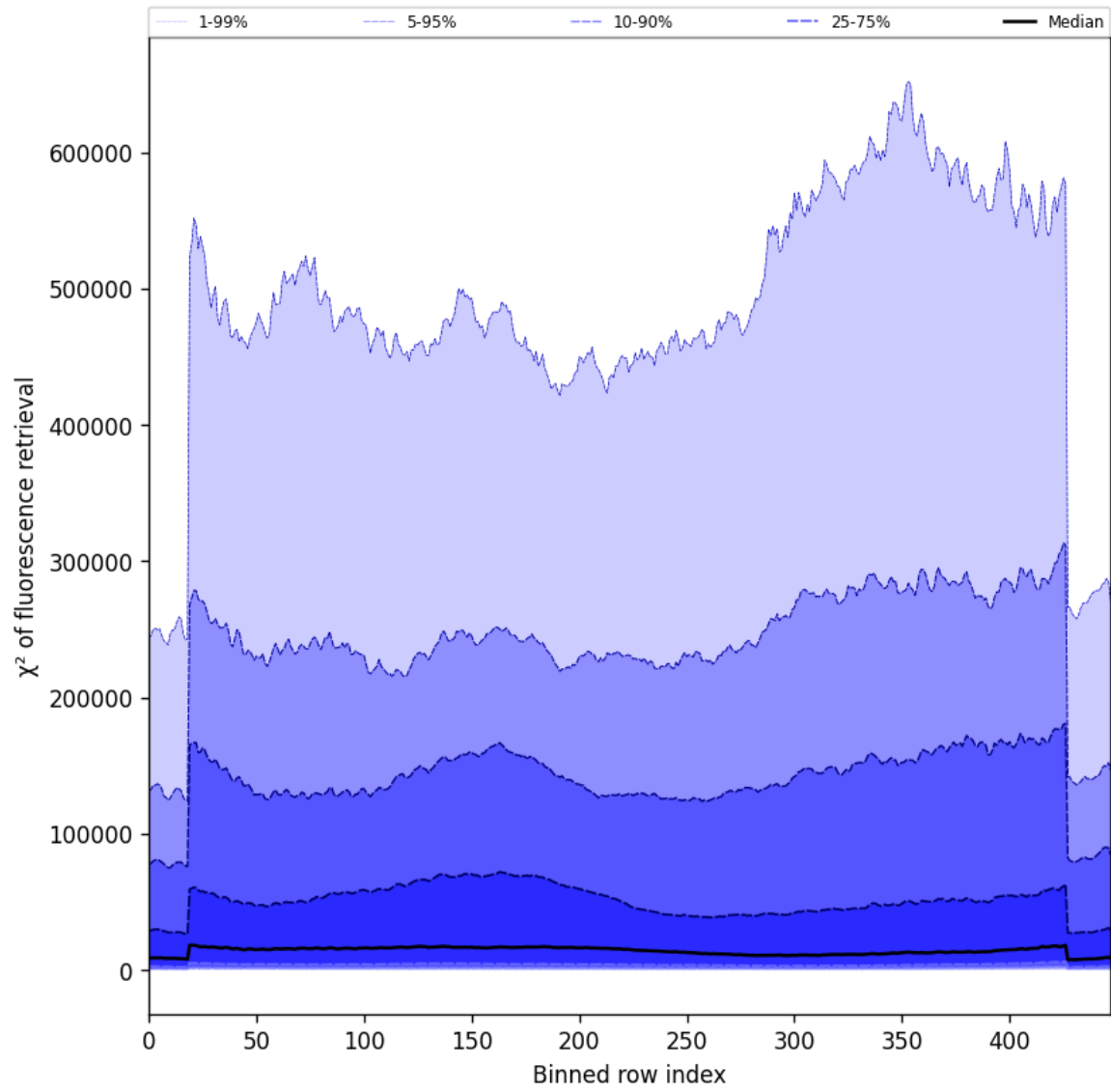
Figure 59: Along track statistics of “ \chi^2 of fluorescence retrieval” for 2025-02-21 to 2025-02-23
