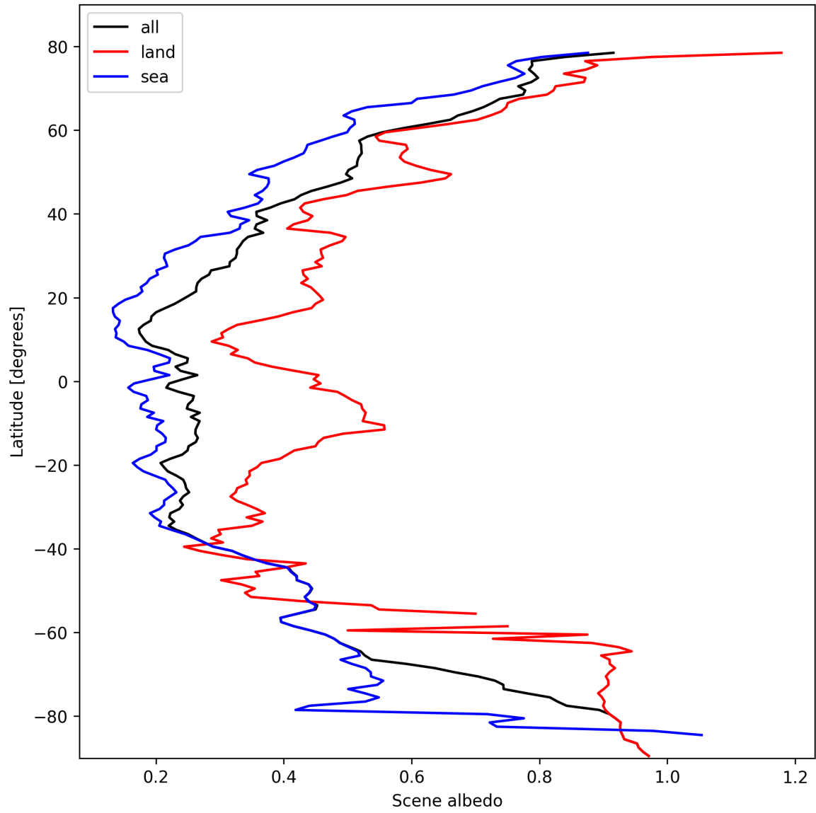
Figure 17: Zonal average of “Scene albedo” for 2025-02-21 to 2025-02-23.
