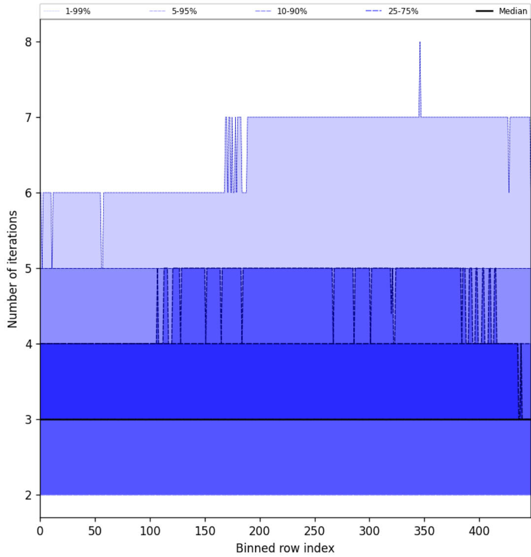
Figure 56: Along track statistics of “Number of iterations” for 2025-02-21 to 2025-02-23
