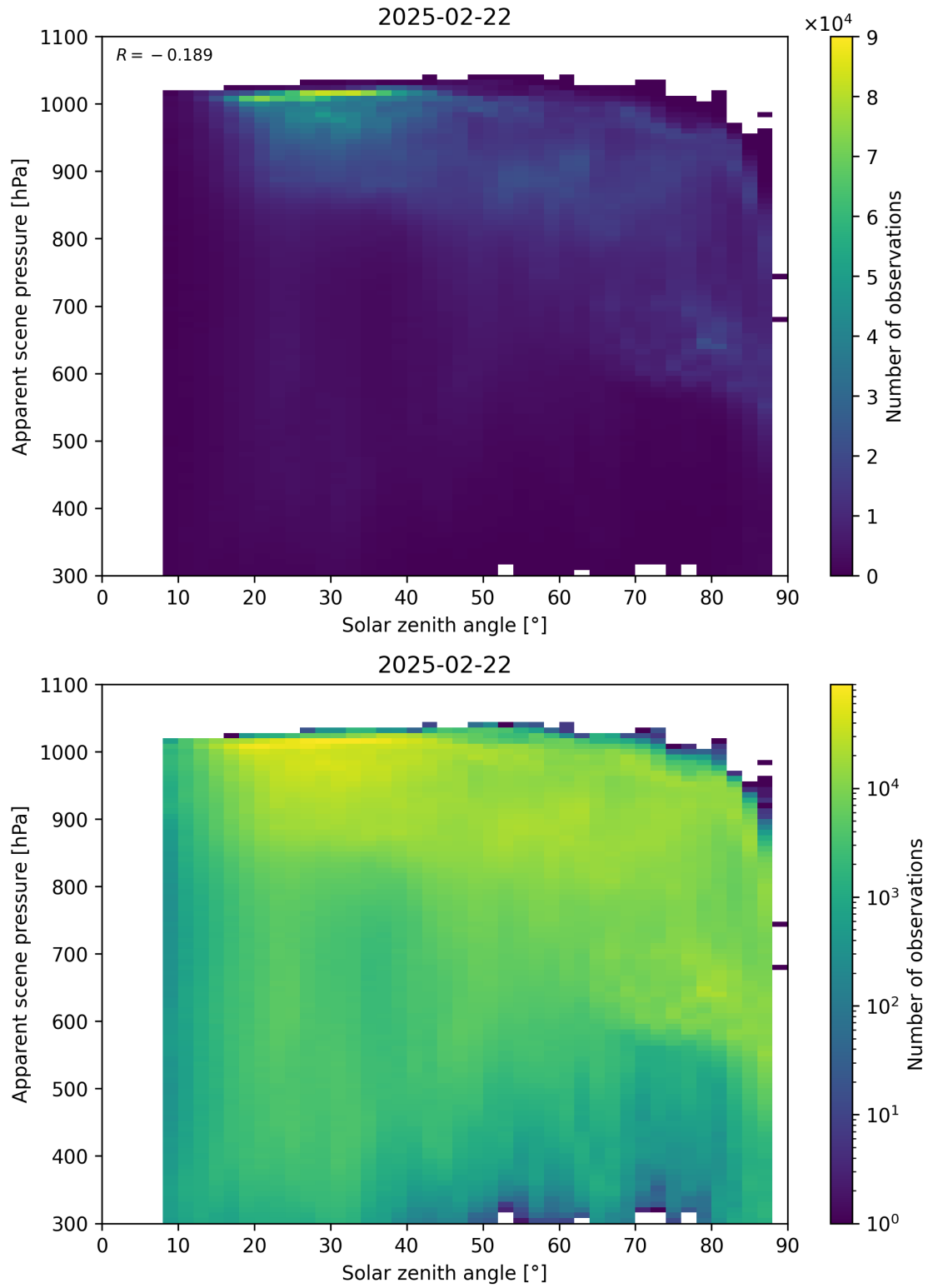
Figure 108: Scatter density plot of “Solar zenith angle” against “Apparent scene pressure” for 2025-02-21 to 2025-02-23.
