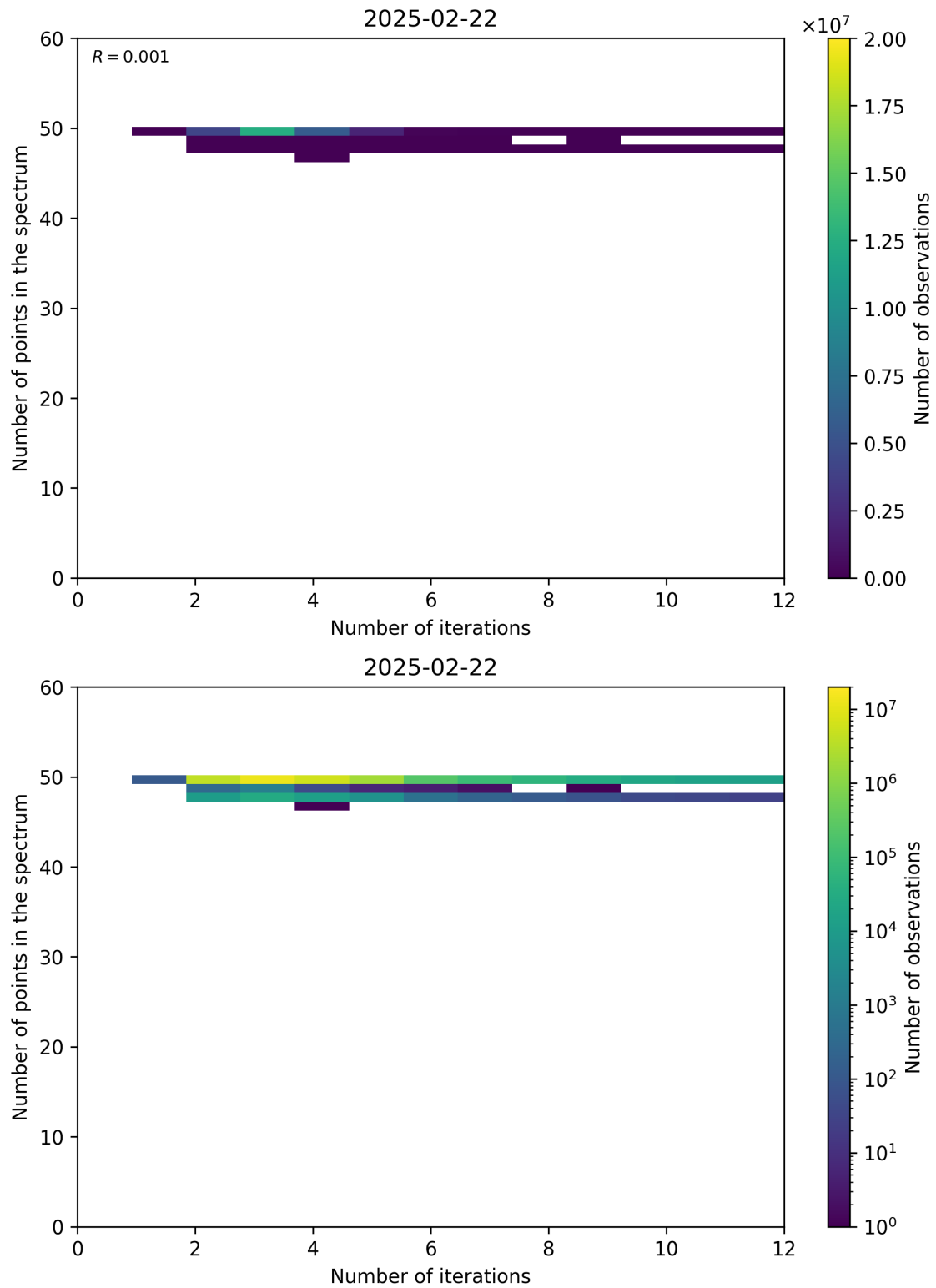
Figure 99: Scatter density plot of “Number of iterations” against “Number of points in the spectrum” for 2025-02-21 to 2025-02-23.
