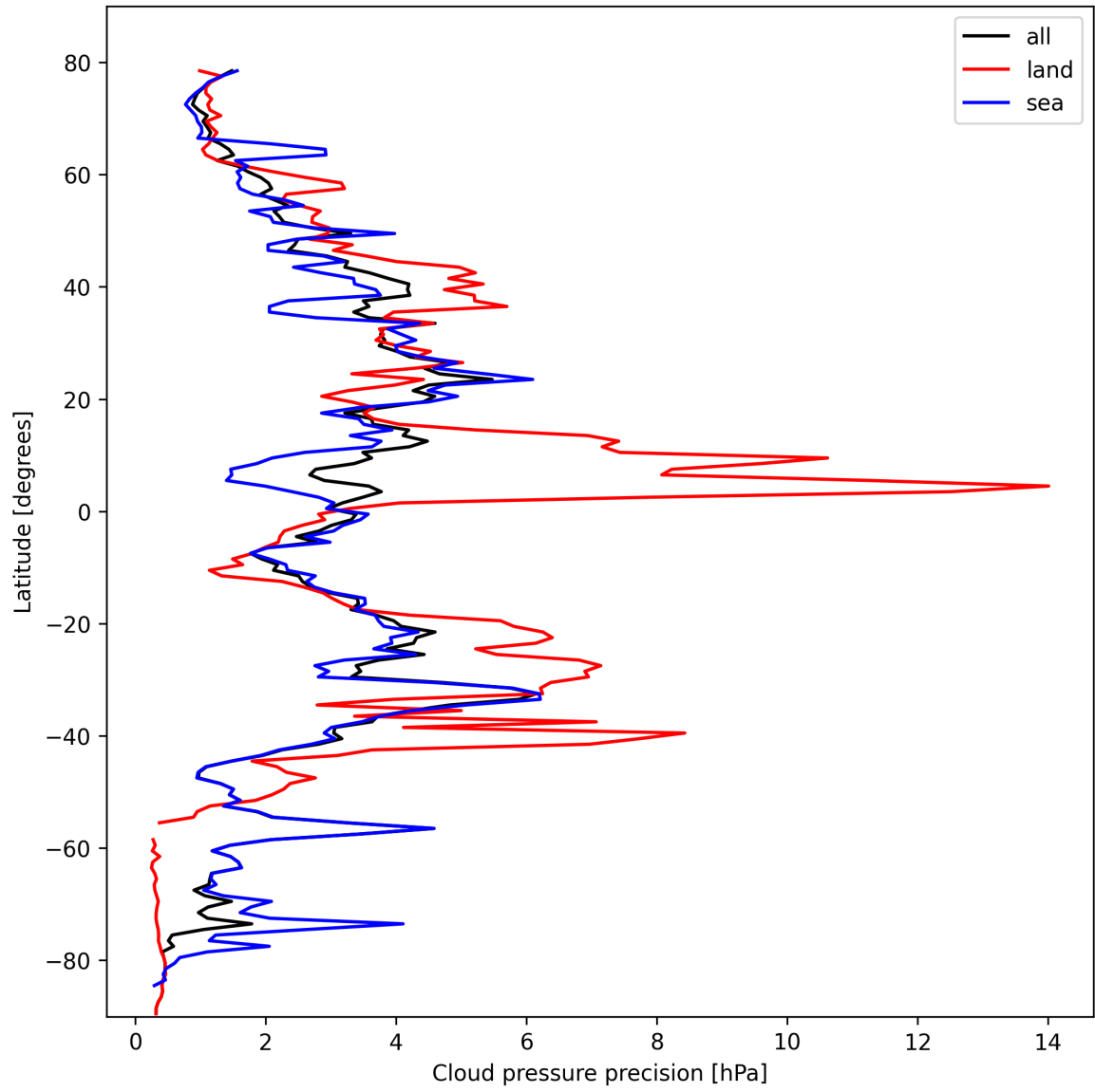
Figure 14: Zonal average of “Cloud pressure precision” for 2025-02-21 to 2025-02-23.
