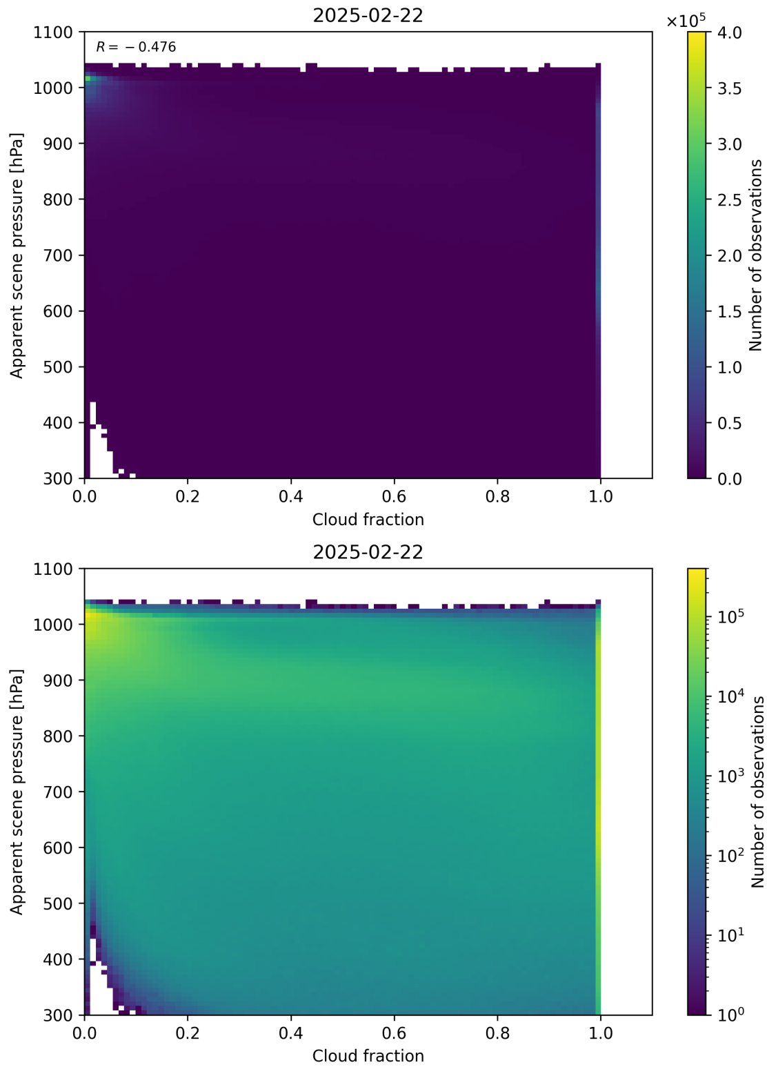
Figure 70: Scatter density plot of “Cloud fraction” against “Apparent scene pressure” for 2025-02-21 to 2025-02-23.
