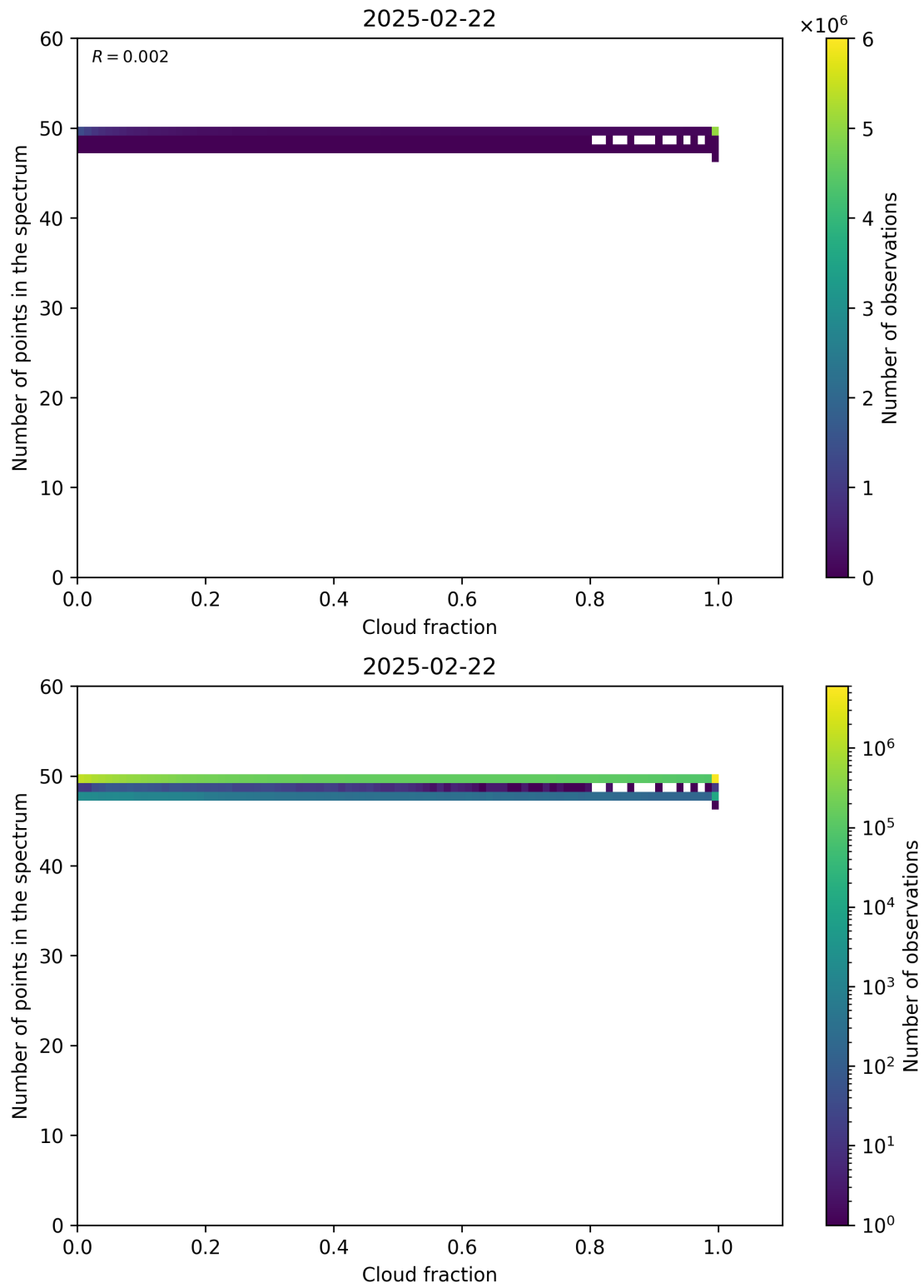
Figure 74: Scatter density plot of “Cloud fraction” against “Number of points in the spectrum” for 2025-02-21 to 2025-02-23.
