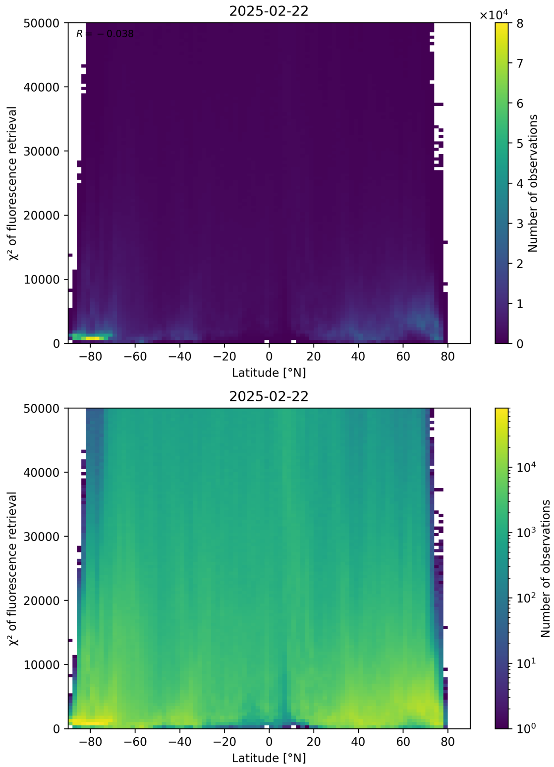
Figure 89: Scatter density plot of “Latitude” against “ \chi^2 of fluorescence retrieval” for 2025-02-21 to 2025-02-23.
