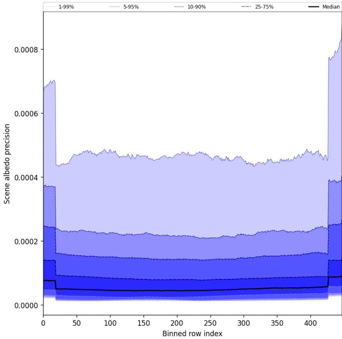
Figure 52: Along track statistics of “Scene albedo precision” for 2025-02-21 to 2025-02-23
