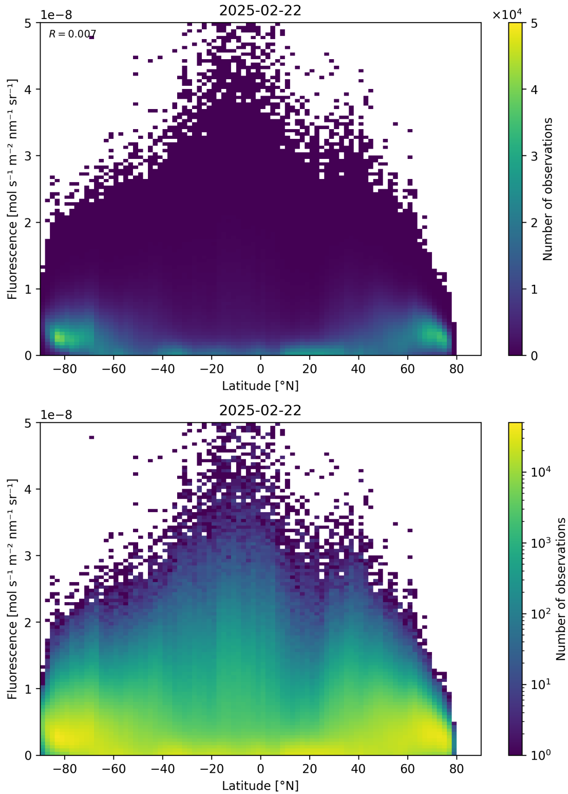
Figure 92: Scatter density plot of “Latitude” against “Fluorescence” for 2025-02-21 to 2025-02-23.
