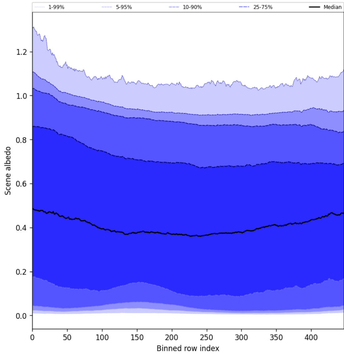
Figure 51: Along track statistics of “Scene albedo” for 2025-02-21 to 2025-02-23
