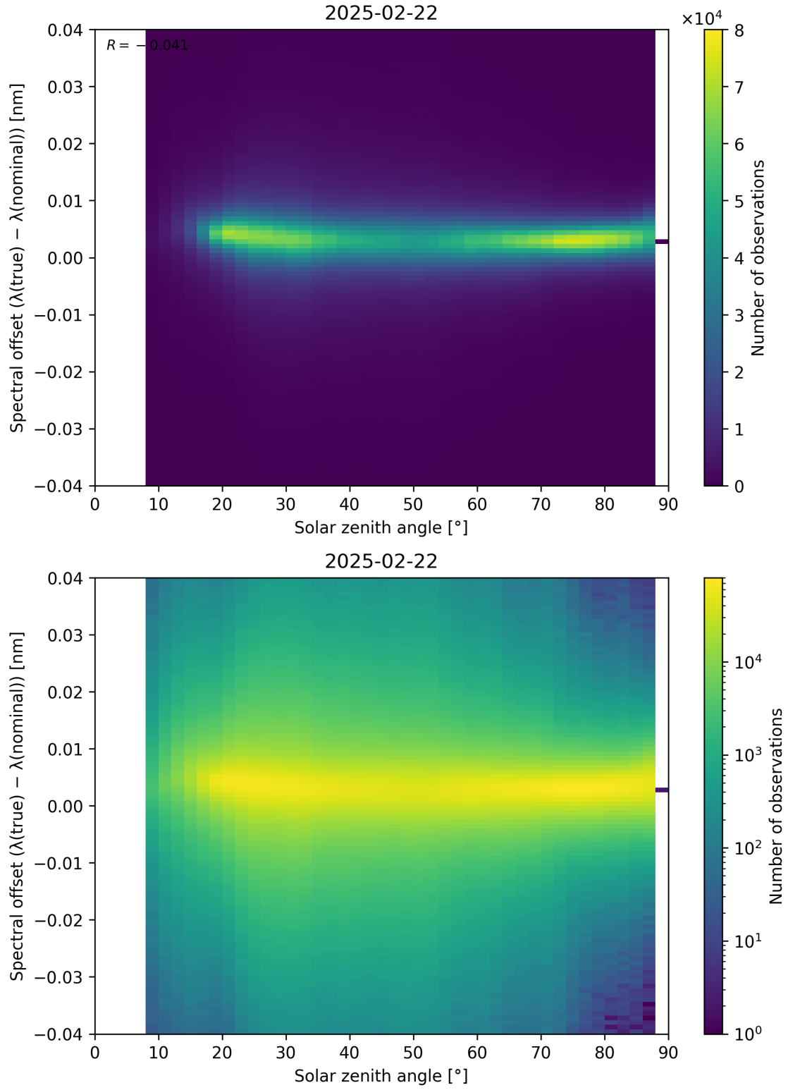
Figure 117: Scatter density plot of “Solar zenith angle” against “Spectral offset ( \lambda_{\text{true}} - \lambda_{\text{nominal}} )” for 2025-02-21 to 2025-02-23.
