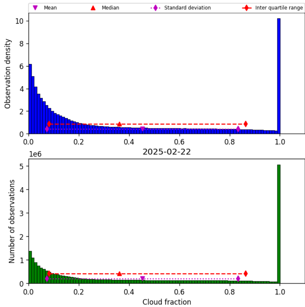
Figure 32: Histogram of “Cloud fraction” for 2025-02-21 to 2025-02-23
