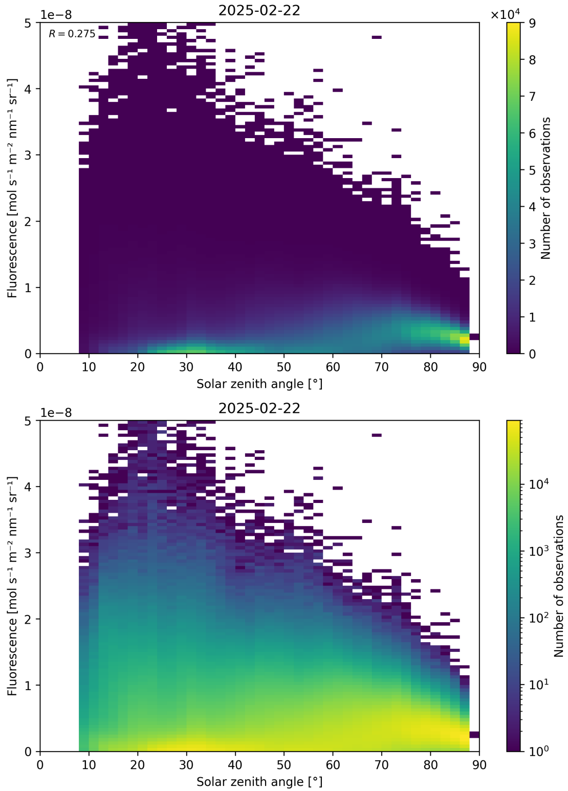
Figure 112: Scatter density plot of “Solar zenith angle” against “Fluorescence” for 2025-02-21 to 2025-02-23.
