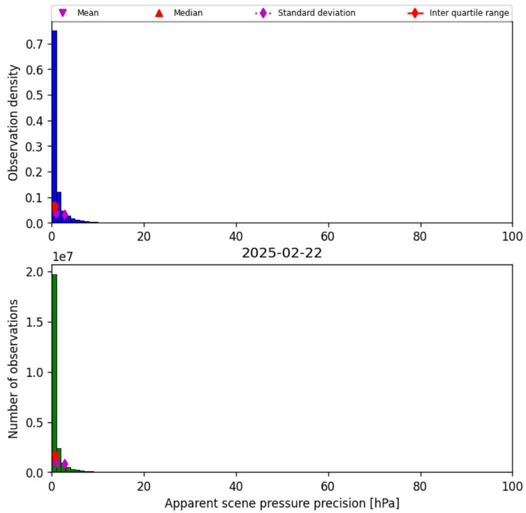
Figure 37: Histogram of “Apparent scene pressure precision” for 2025-02-21 to 2025-02-23
