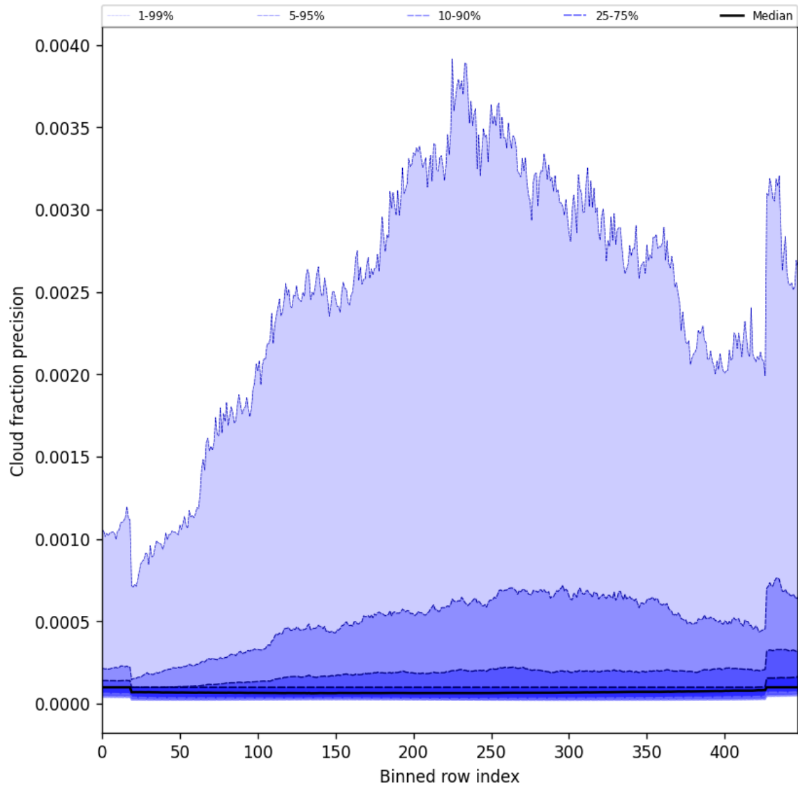
Figure 50: Along track statistics of “Cloud fraction precision” for 2025-02-21 to 2025-02-23
