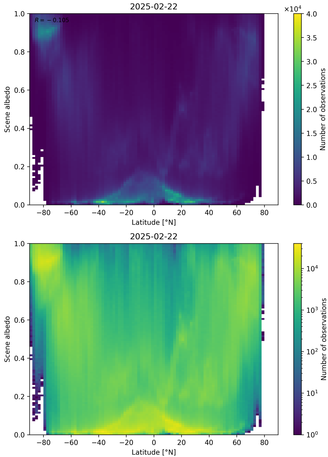
Figure 95: Scatter density plot of “Latitude” against “Scene albedo” for 2025-02-21 to 2025-02-23.
