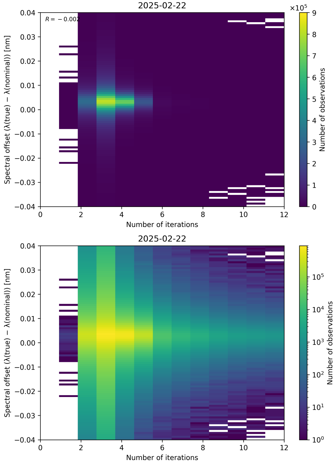
Figure 100: Scatter density plot of “Number of iterations” against “Spectral offset ( \lambda_{\text{true}} - \lambda_{\text{nominal}} )” for 2025-02-21 to 2025-02-23.
