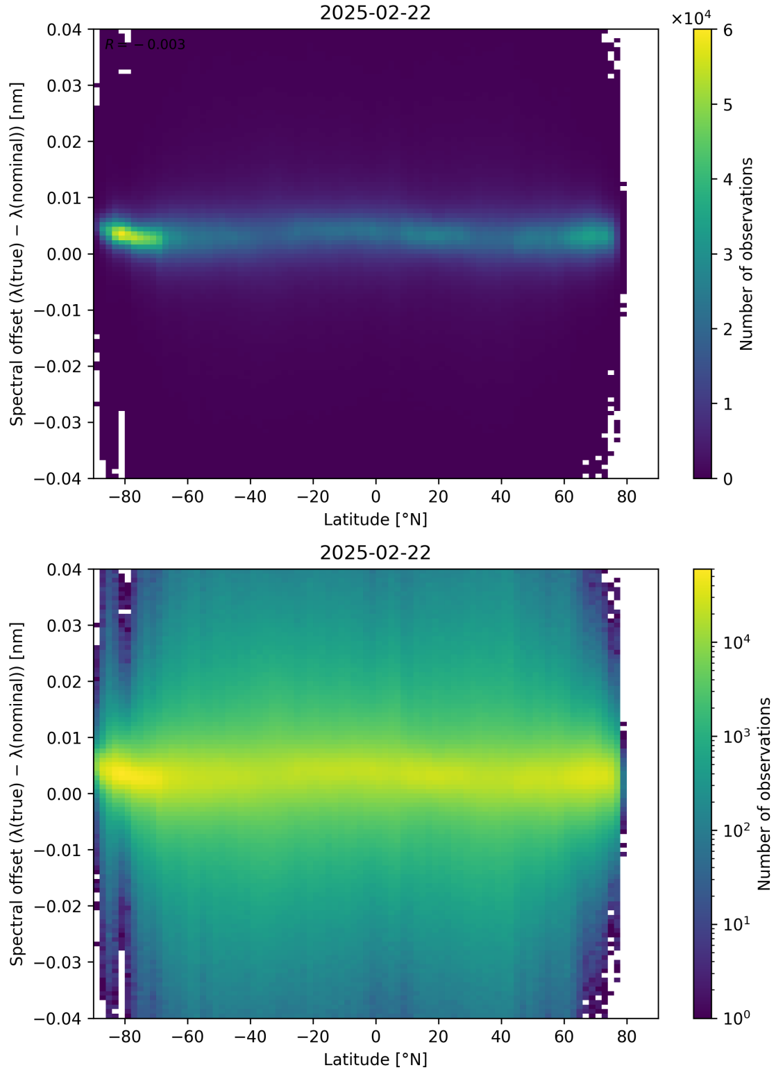
Figure 96: Scatter density plot of “Latitude” against “Spectral offset ( \lambda_{\text{true}} - \lambda_{\text{nominal}} )” for 2025-02-21 to 2025-02-23.
