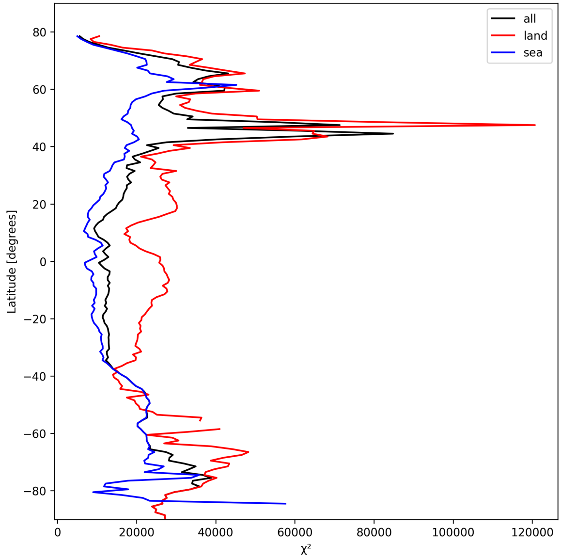
Figure 21: Zonal average of “ \chi^2 ” for 2025-02-21 to 2025-02-23.
