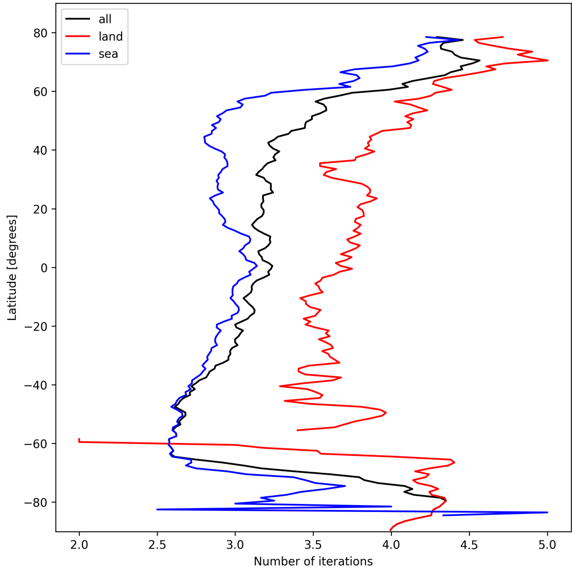
Figure 22: Zonal average of “Number of iterations” for 2025-02-21 to 2025-02-23.
