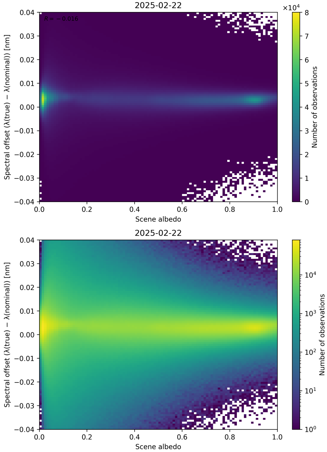
Figure 107: Scatter density plot of “Scene albedo” against “Spectral offset ( \lambda_{\text{true}} - \lambda_{\text{nominal}} )” for 2025-02-21 to 2025-02-23.
