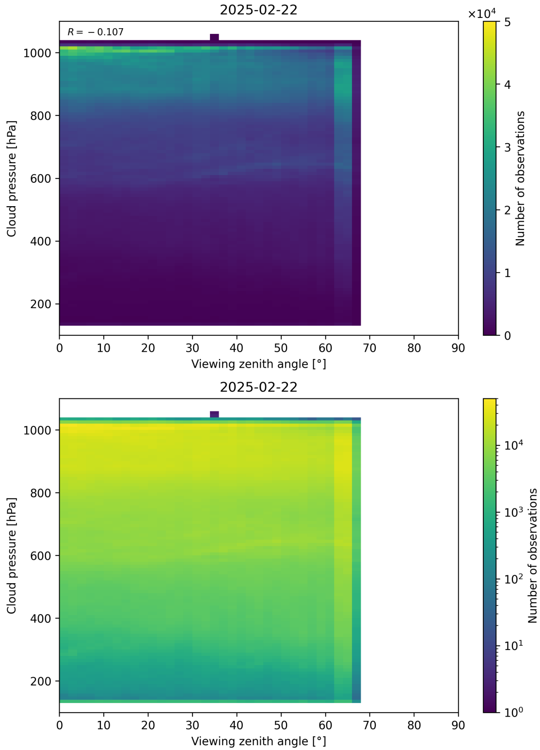
Figure 121: Scatter density plot of “Viewing zenith angle” against “Cloud pressure” for 2025-02-21 to 2025-02-23.
