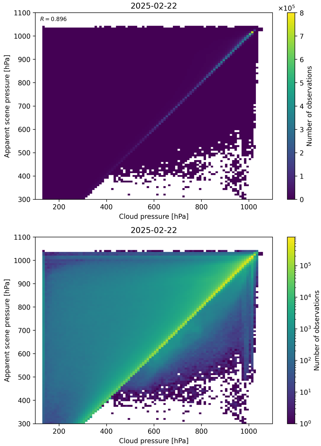
Figure 77: Scatter density plot of “Cloud pressure” against “Apparent scene pressure” for 2025-02-21 to 2025-02-23.
