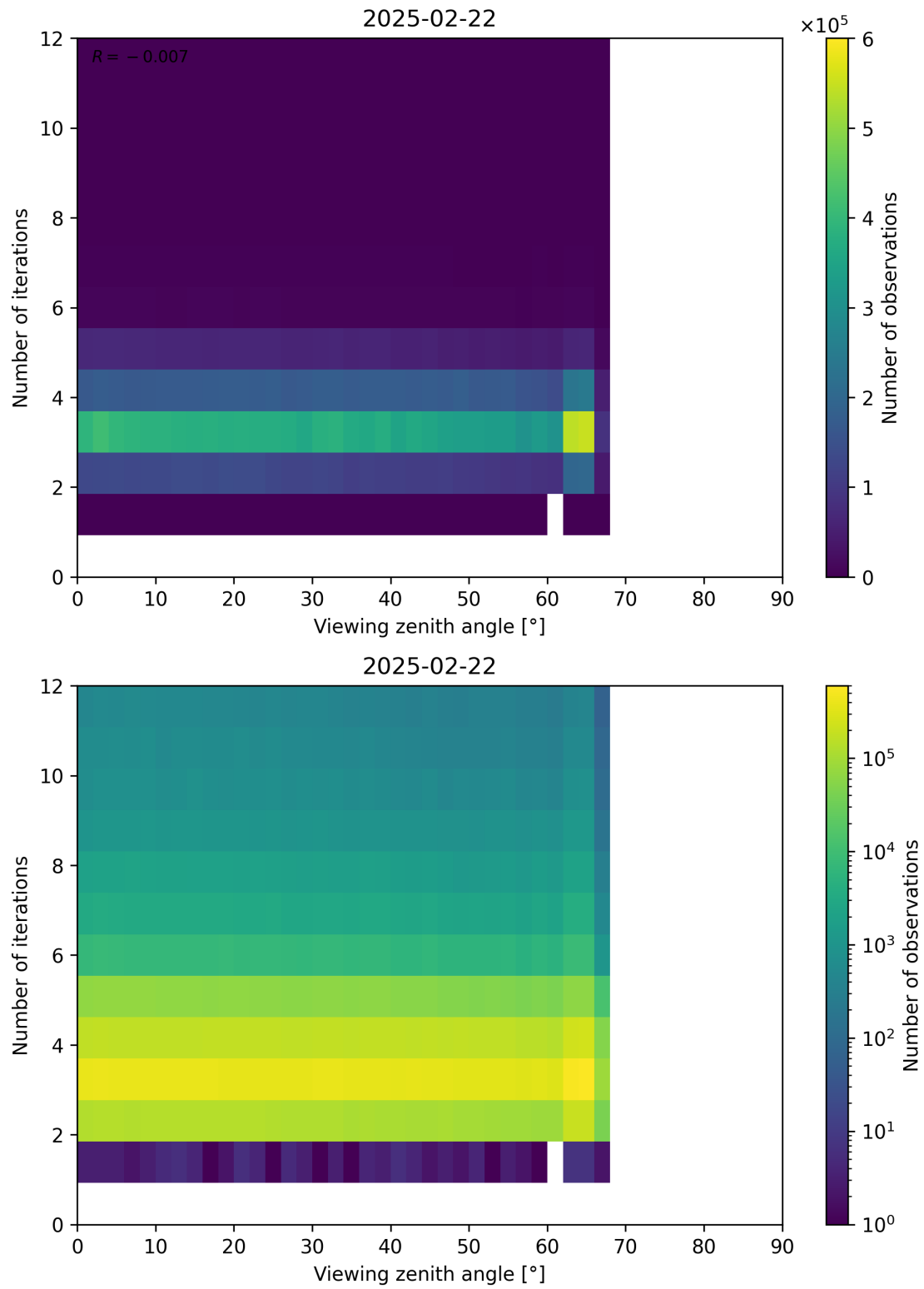
Figure 124: Scatter density plot of “Viewing zenith angle” against “Number of iterations” for 2025-02-21 to 2025-02-23.
