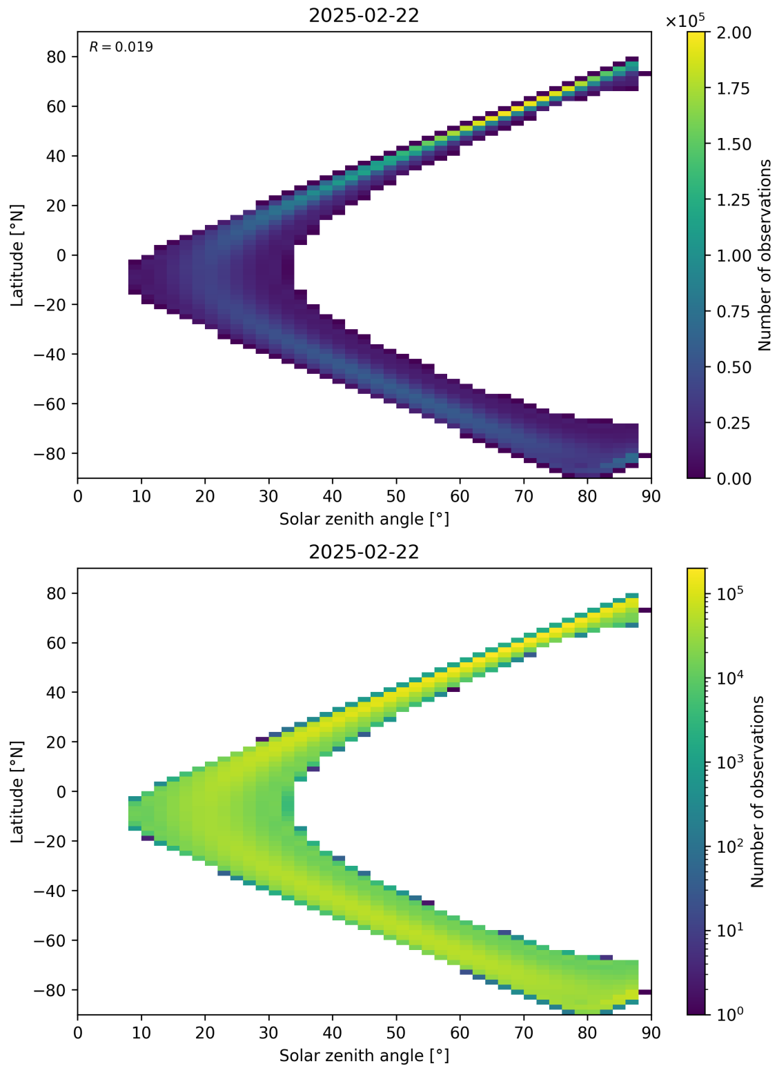
Figure 113: Scatter density plot of “Solar zenith angle” against “Latitude” for 2025-02-21 to 2025-02-23.
