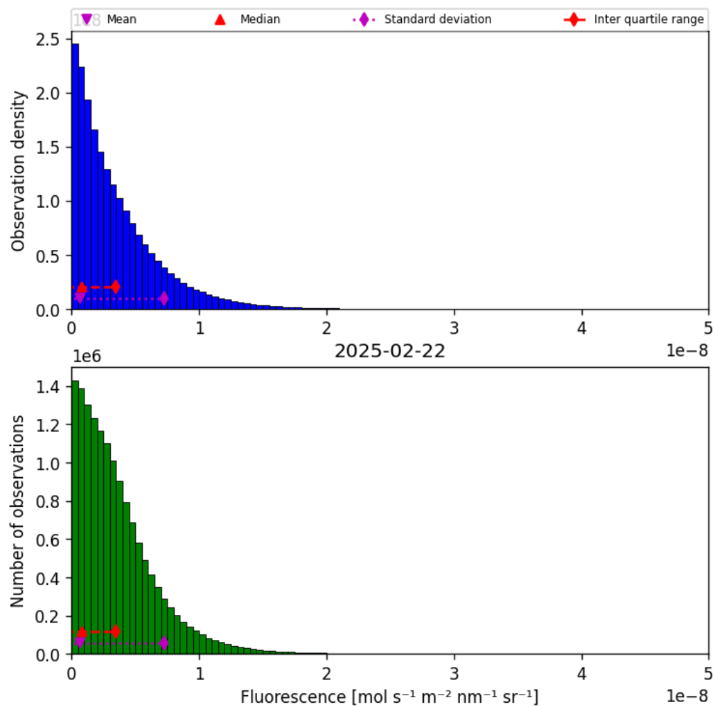
Figure 40: Histogram of “Fluorescence” for 2025-02-21 to 2025-02-23
