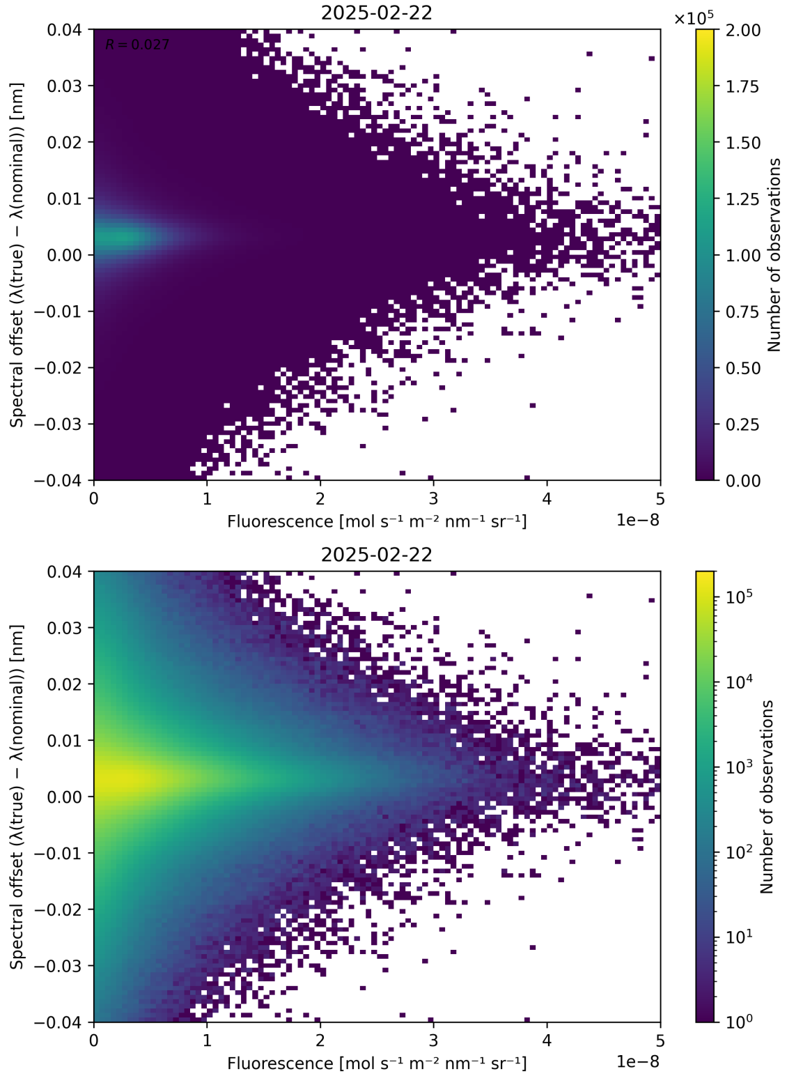
Figure 87: Scatter density plot of “Fluorescence” against “Spectral offset ( \lambda_{\text{true}} - \lambda_{\text{nominal}} )” for 2025-02-21 to 2025-02-23.
