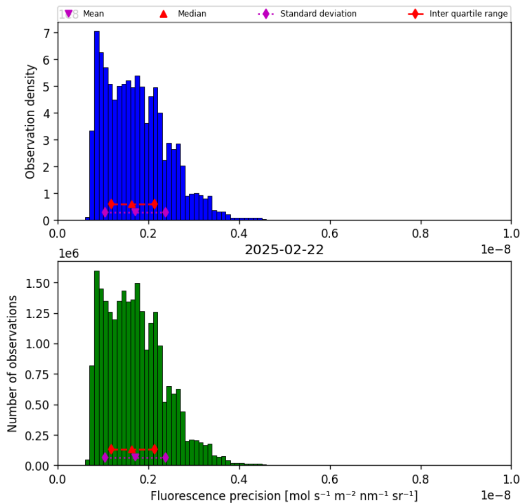
Figure 41: Histogram of “Fluorescence precision” for 2025-02-21 to 2025-02-23
