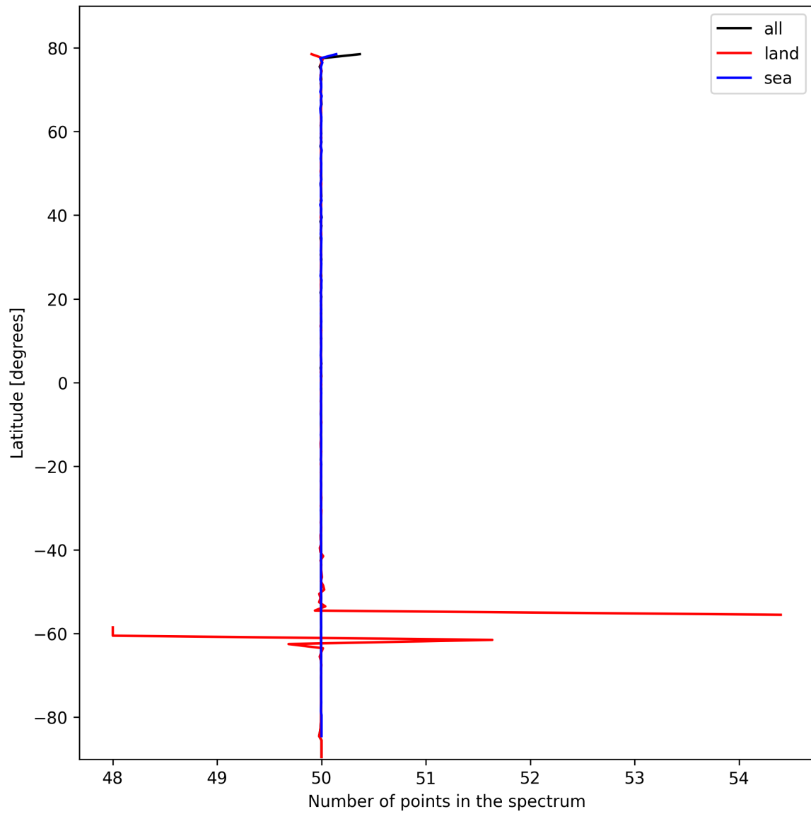
Figure 27: Zonal average of “Number of points in the spectrum” for 2025-02-21 to 2025-02-23.
