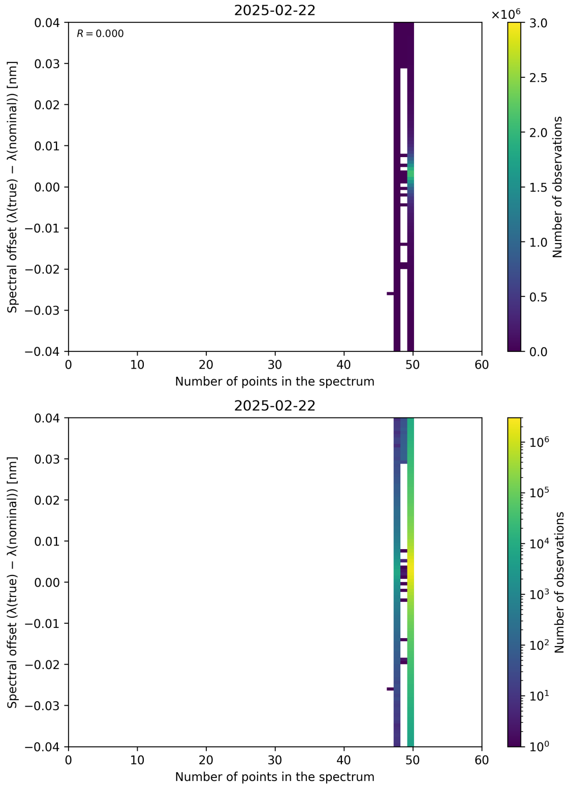
Figure 101: Scatter density plot of “Number of points in the spectrum” against “Spectral offset ( \lambda_{\text{true}} - \lambda_{\text{nominal}} )” for 2025-02-21 to 2025-02-23.
