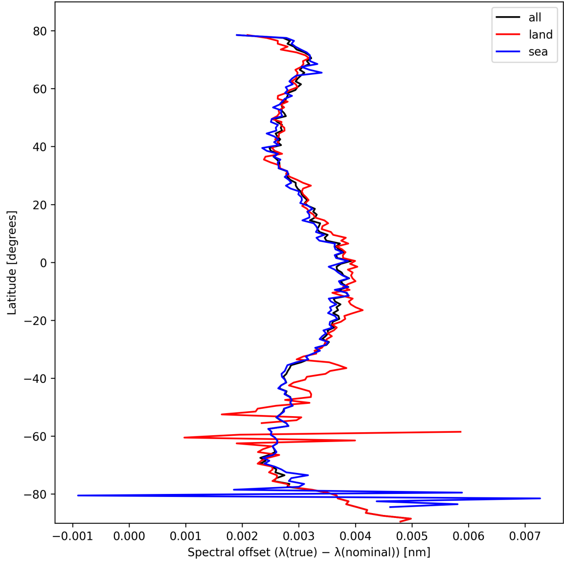
Figure 28: Zonal average of “Spectral offset ( \lambda_{\text{true}} - \lambda_{\text{nominal}} )” for 2025-02-21 to 2025-02-23.
