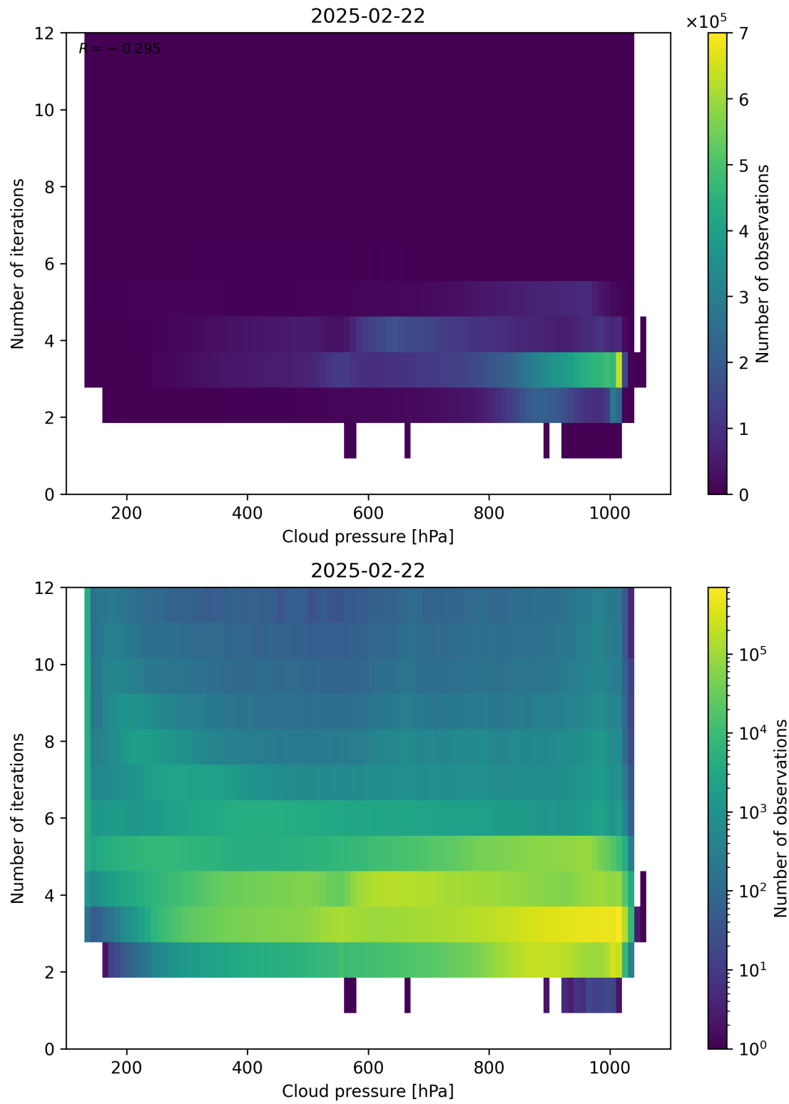
Figure 81: Scatter density plot of “Cloud pressure” against “Number of iterations” for 2025-02-21 to 2025-02-23.
