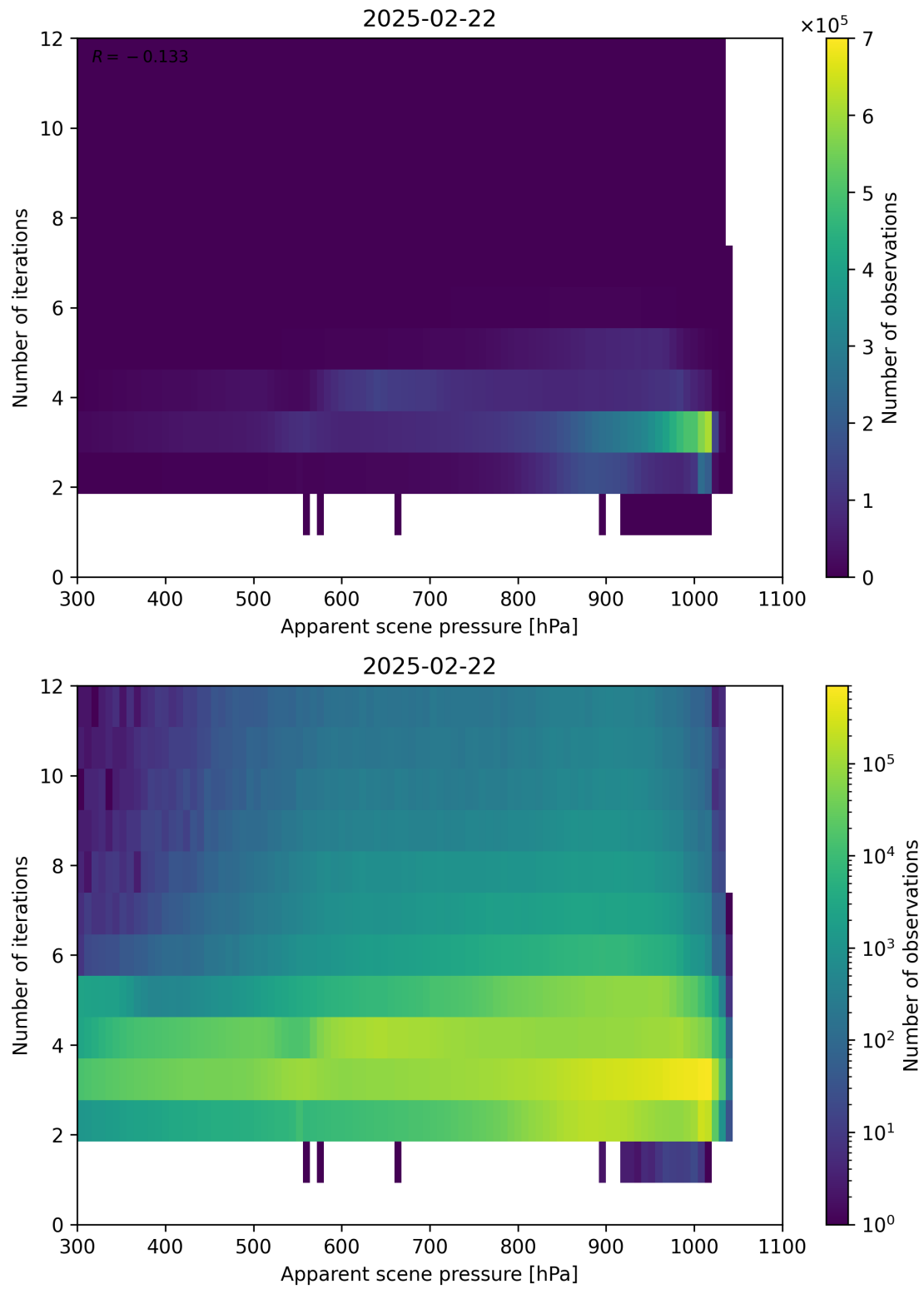
Figure 65: Scatter density plot of “Apparent scene pressure” against “Number of iterations” for 2025-02-21 to 2025-02-23.
