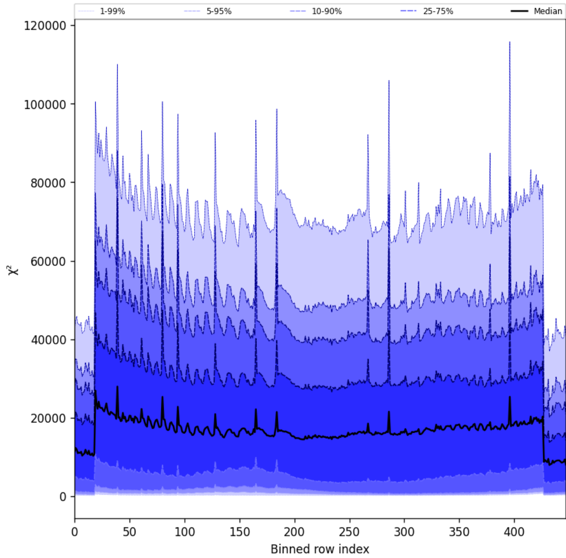
Figure 55: Along track statistics of “ \chi^2 ” for 2025-02-21 to 2025-02-23
