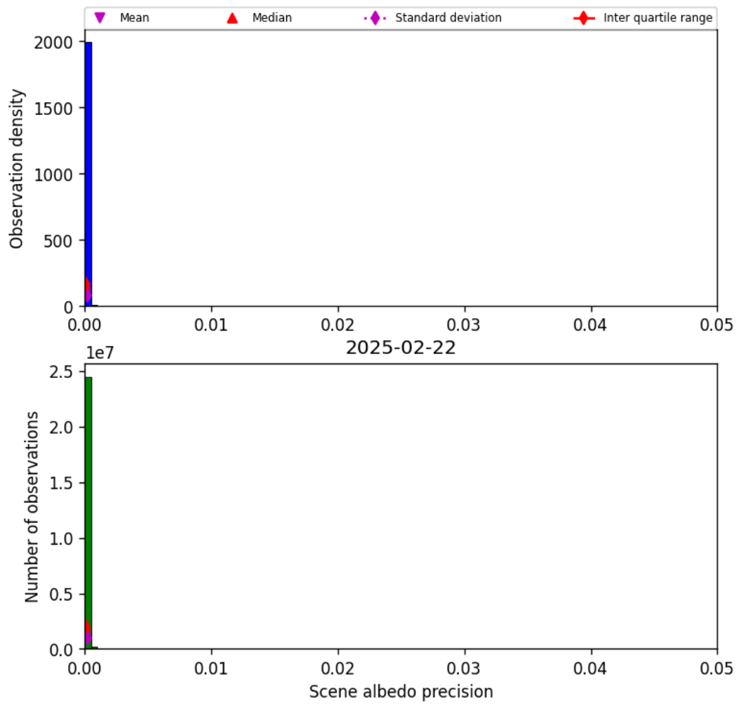
Figure 35: Histogram of “Scene albedo precision” for 2025-02-21 to 2025-02-23
