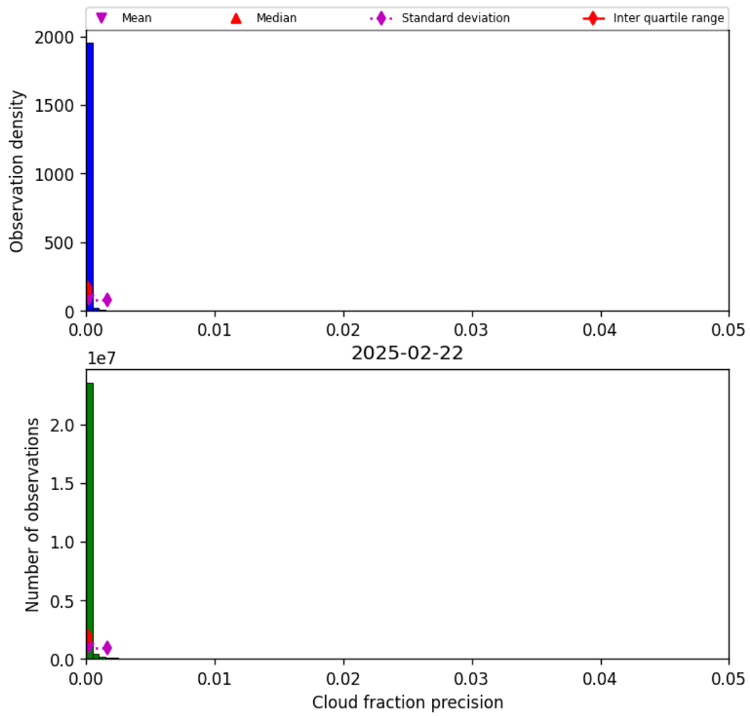
Figure 33: Histogram of “Cloud fraction precision” for 2025-02-21 to 2025-02-23
