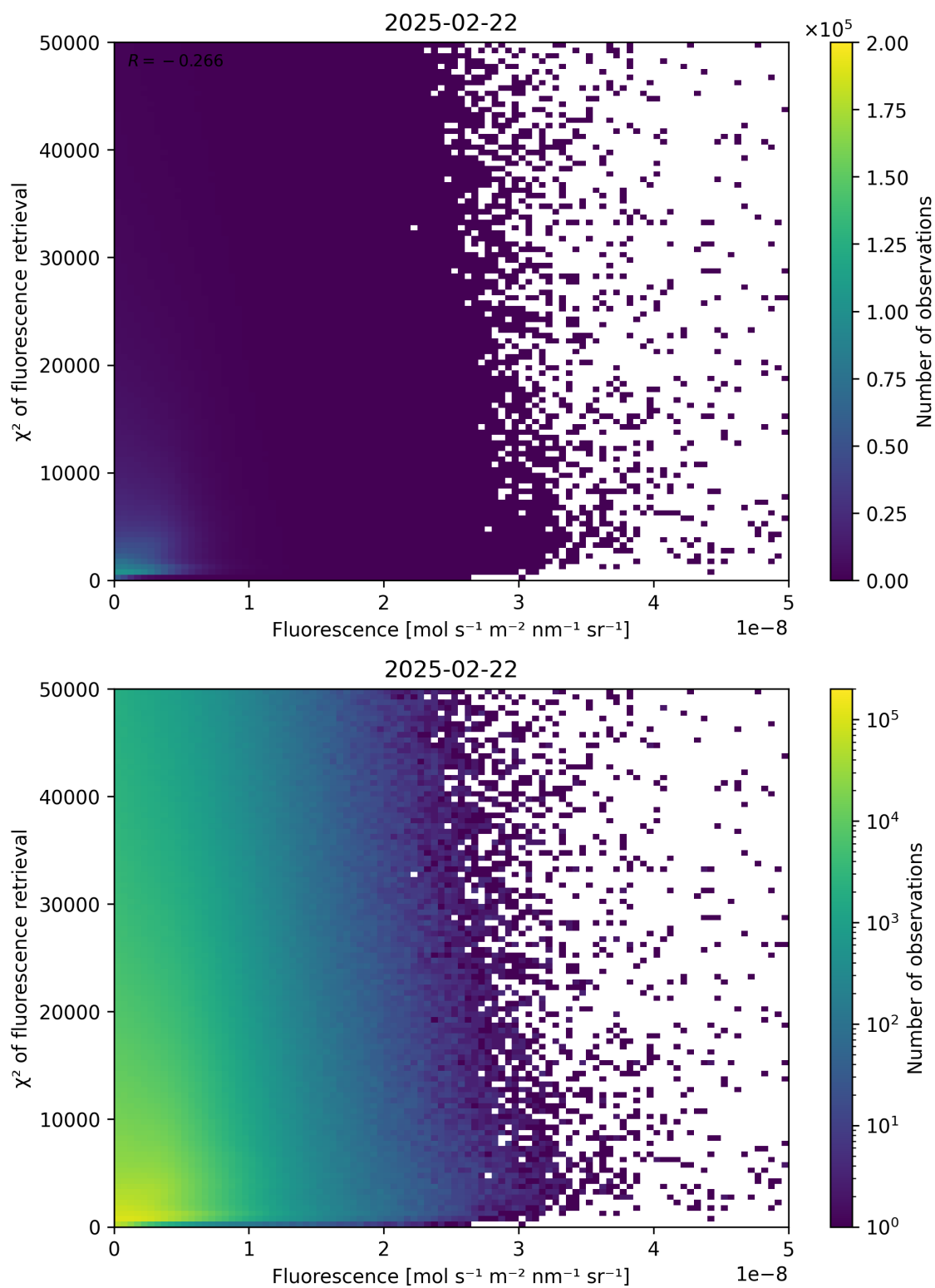
Figure 85: Scatter density plot of “Fluorescence” against “ \chi^2 of fluorescence retrieval” for 2025-02-21 to 2025-02-23.
