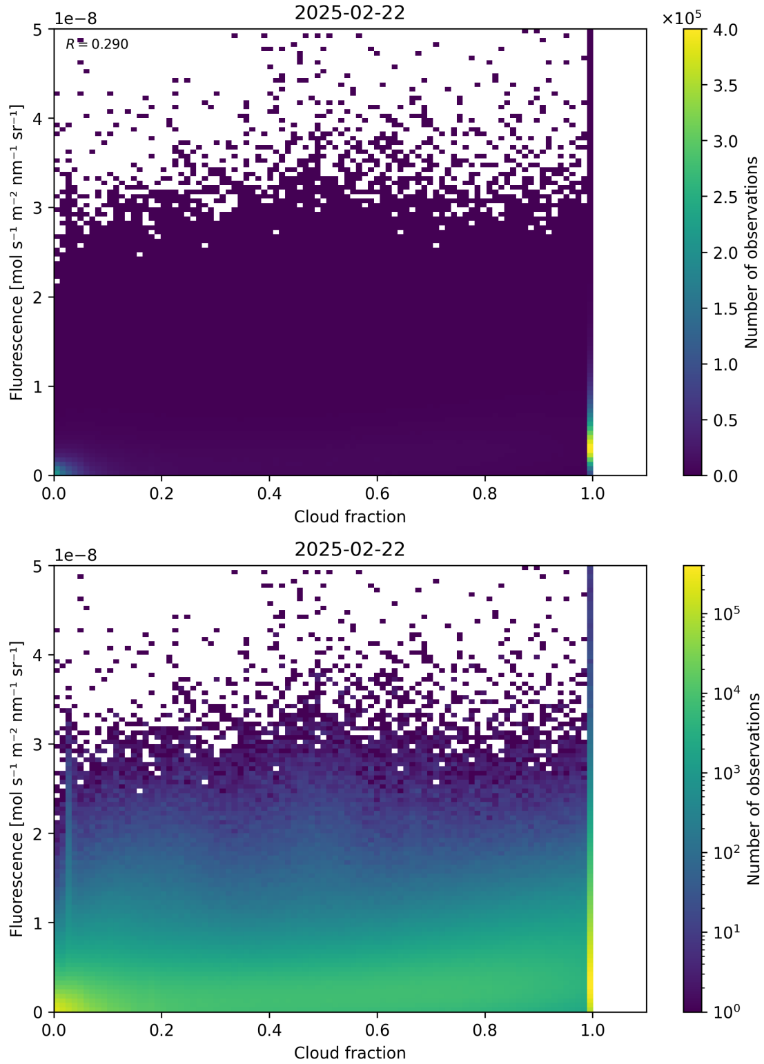
Figure 72: Scatter density plot of “Cloud fraction” against “Fluorescence” for 2025-02-21 to 2025-02-23.
