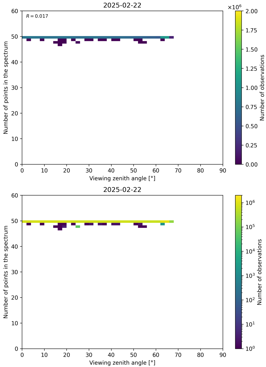
Figure 125: Scatter density plot of “Viewing zenith angle” against “Number of points in the spectrum” for 2025-02-21 to 2025-02-23.
