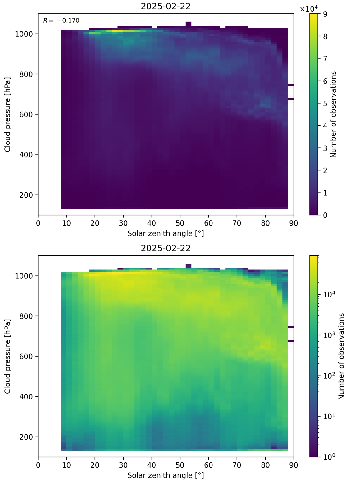
Figure 111: Scatter density plot of “Solar zenith angle” against “Cloud pressure” for 2025-02-21 to 2025-02-23.
