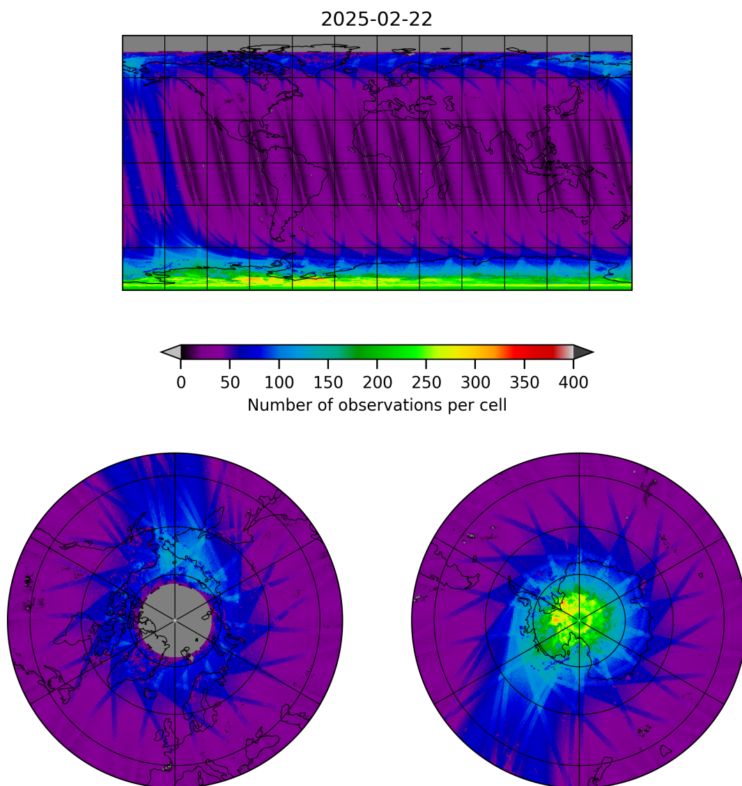
Figure 11: Map of the number of observations for 2025-02-21 to 2025-02-23
