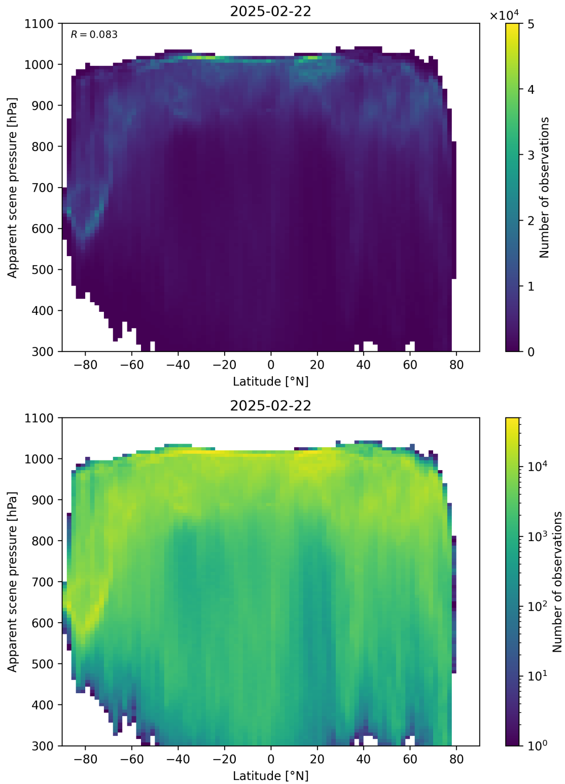
Figure 88: Scatter density plot of “Latitude” against “Apparent scene pressure” for 2025-02-21 to 2025-02-23.
