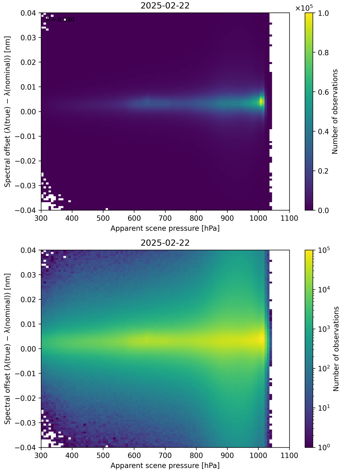
Figure 67: Scatter density plot of “Apparent scene pressure” against “Spectral offset ( \lambda_{\text{true}} - \lambda_{\text{nominal}} )” for 2025-02-21 to 2025-02-23.
