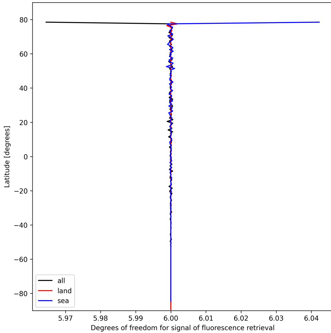
Figure 26: Zonal average of “Degrees of freedom for signal of fluorescence retrieval” for 2025-02-21 to 2025-02-23.
