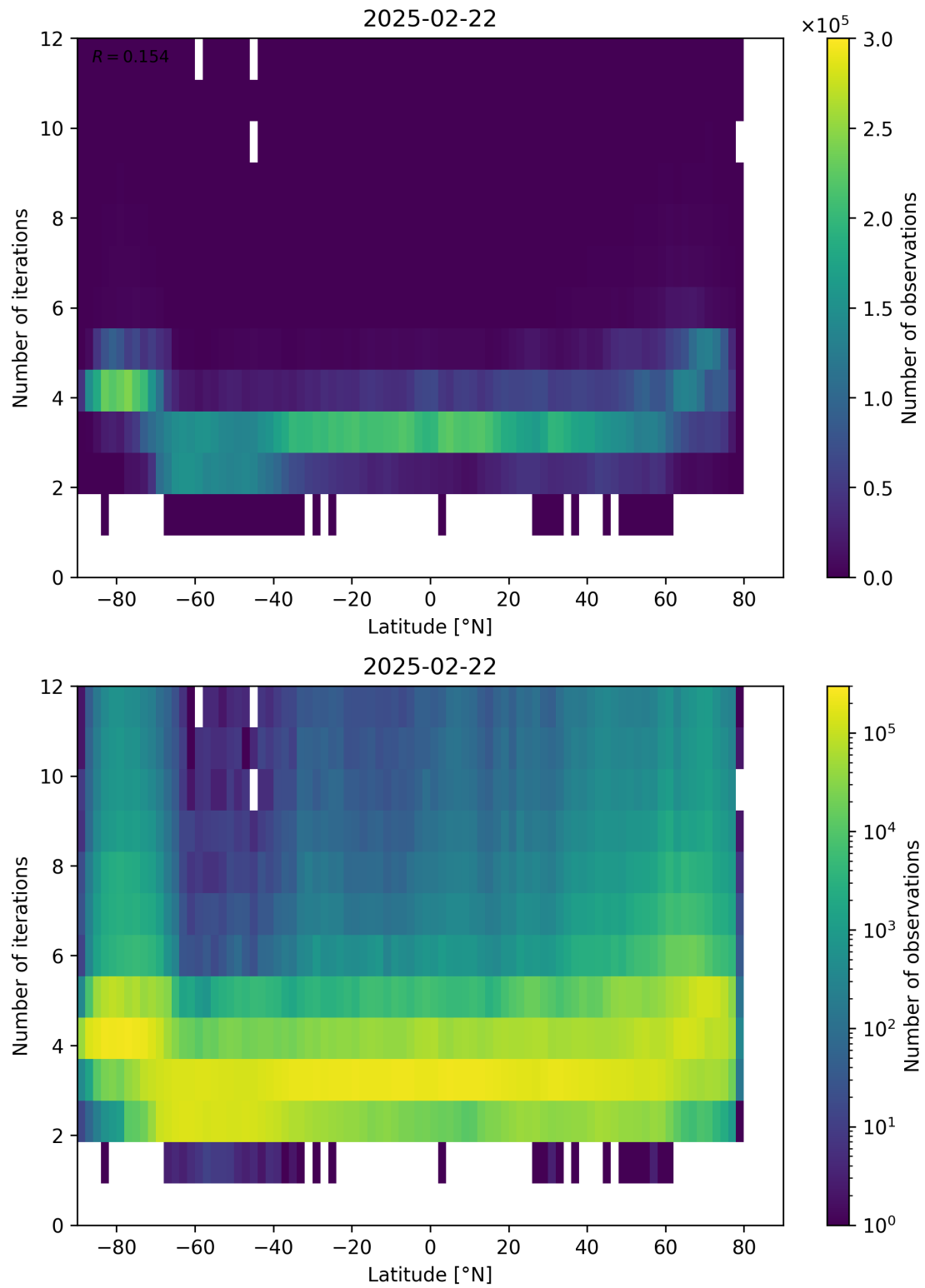
Figure 93: Scatter density plot of “Latitude” against “Number of iterations” for 2025-02-21 to 2025-02-23.
