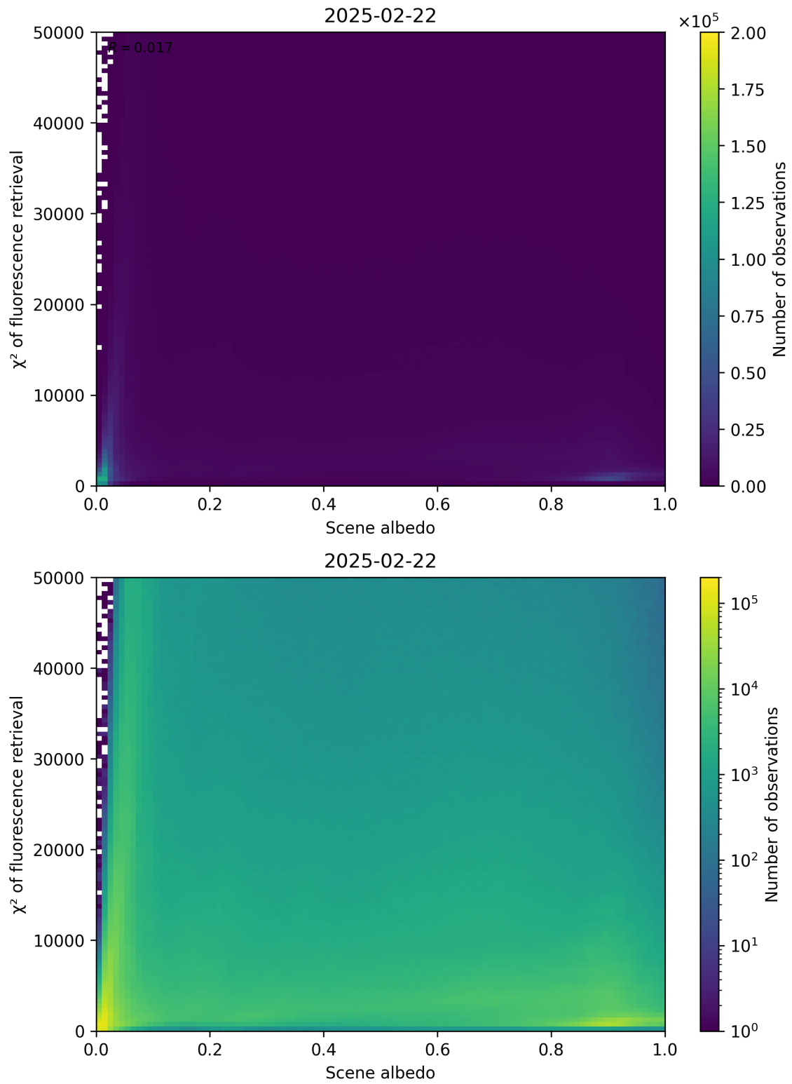
Figure 103: Scatter density plot of “Scene albedo” against “ \chi^2 of fluorescence retrieval” for 2025-02-21 to 2025-02-23.
