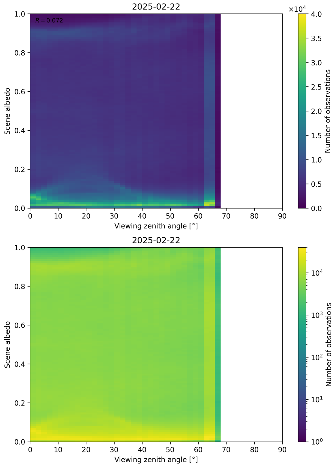
Figure 126: Scatter density plot of “Viewing zenith angle” against “Scene albedo” for 2025-02-21 to 2025-02-23.
