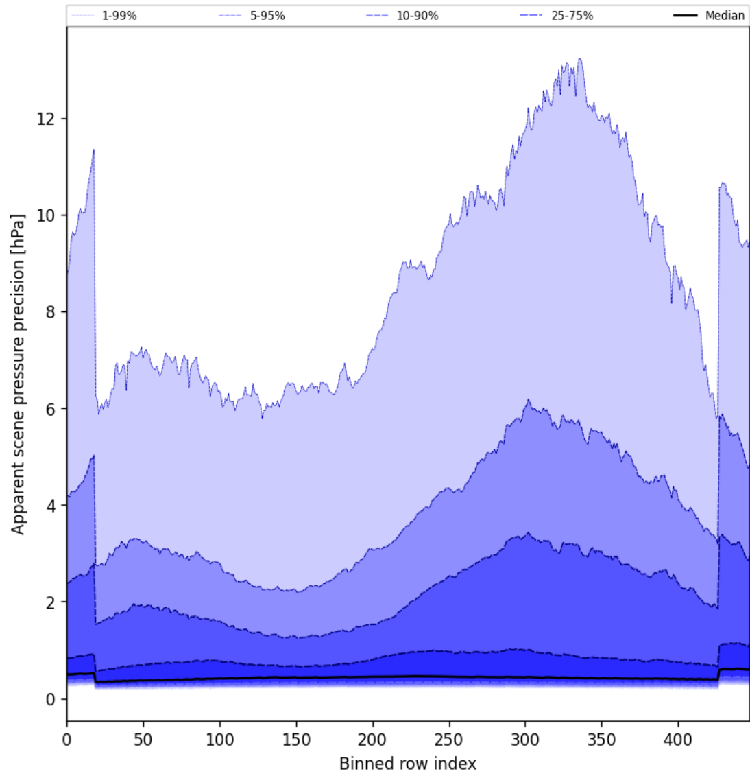
Figure 54: Along track statistics of “Apparent scene pressure precision” for 2025-02-21 to 2025-02-23
