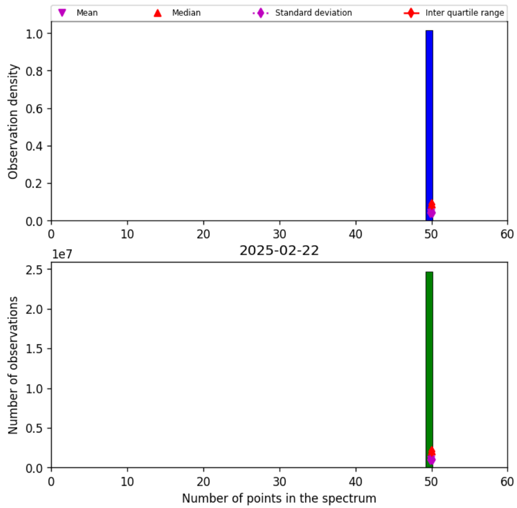
Figure 44: Histogram of “Number of points in the spectrum” for 2025-02-21 to 2025-02-23
