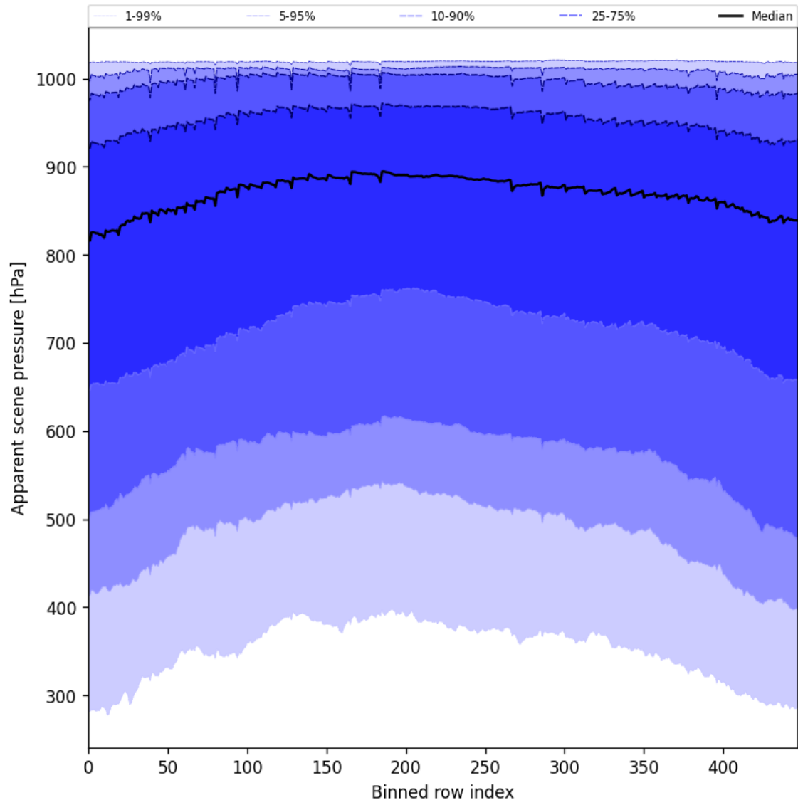
Figure 53: Along track statistics of “Apparent scene pressure” for 2025-02-21 to 2025-02-23
