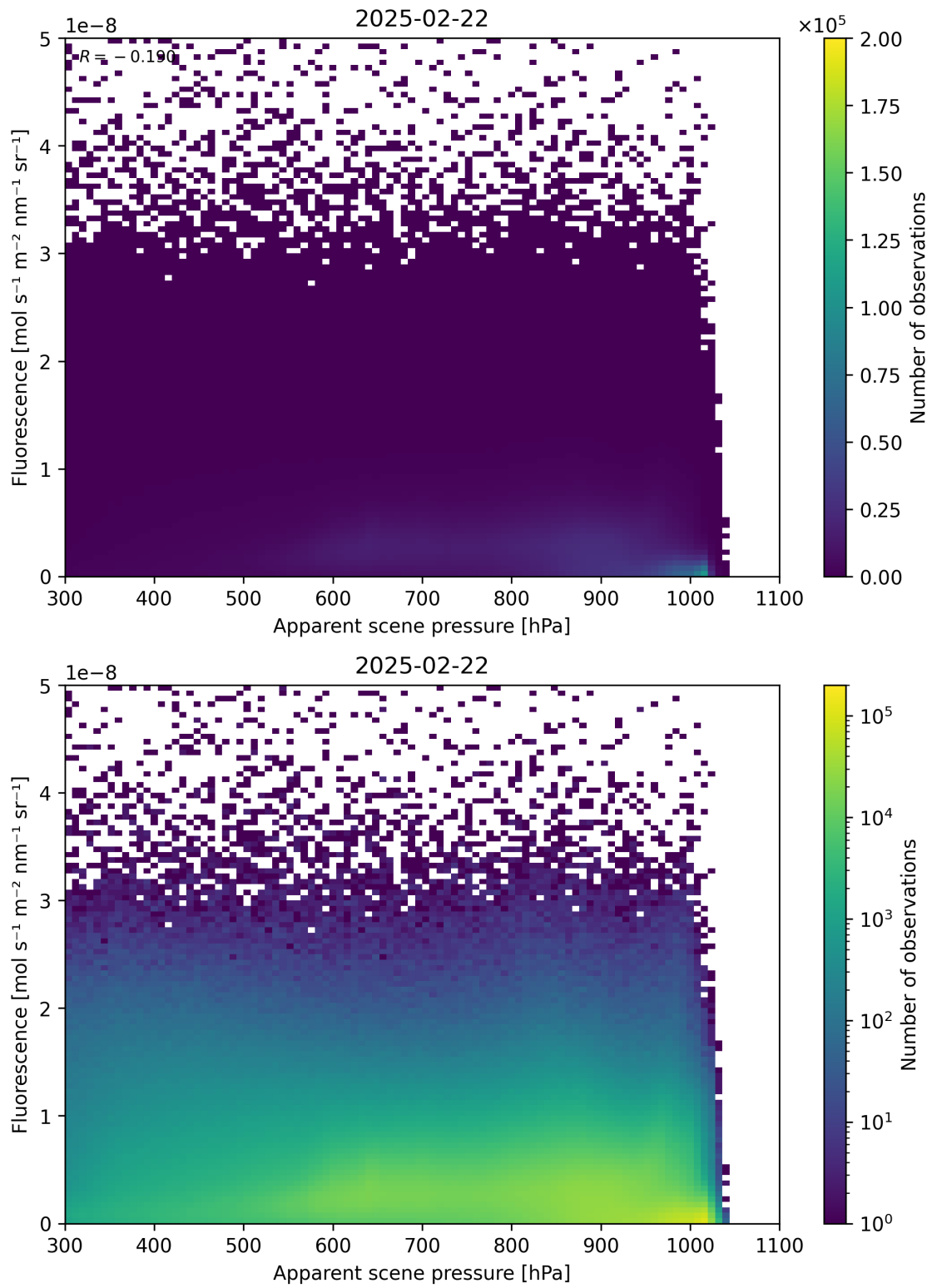
Figure 64: Scatter density plot of “Apparent scene pressure” against “Fluorescence” for 2025-02-21 to 2025-02-23.
