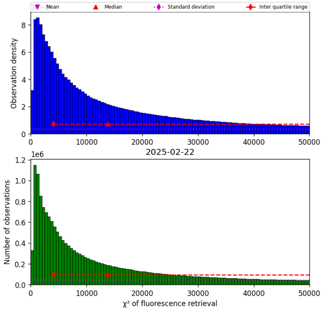
Figure 42: Histogram of “ \chi^2 of fluorescence retrieval” for 2025-02-21 to 2025-02-23
