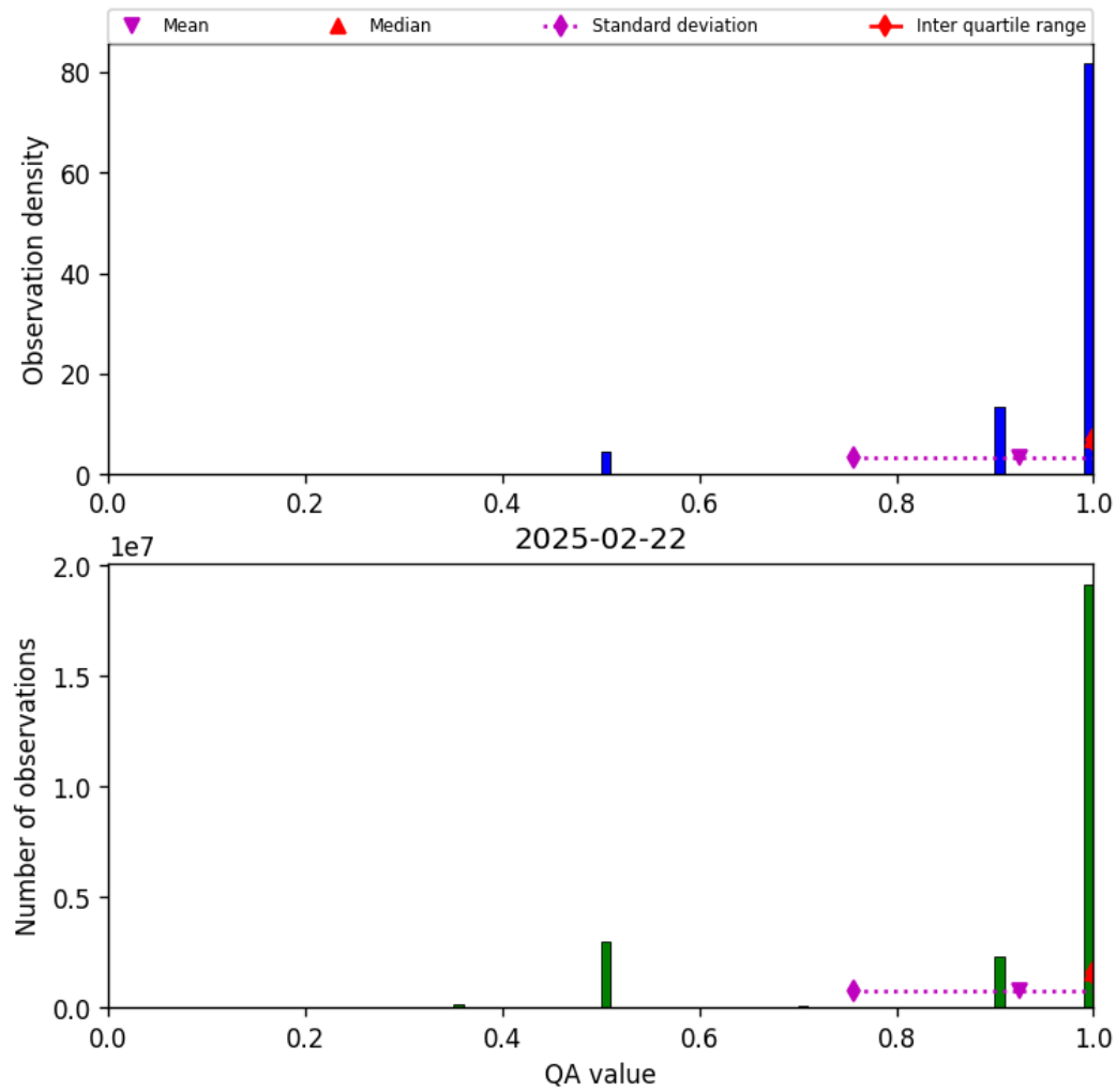
Figure 29: Histogram of “QA value” for 2025-02-21 to 2025-02-23
