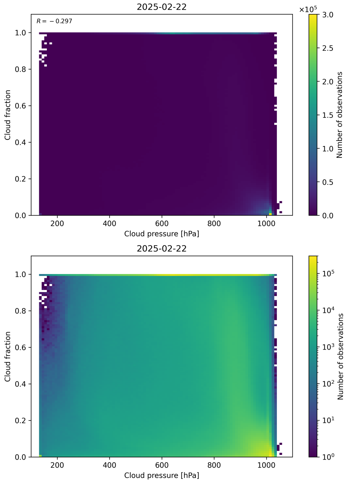
Figure 79: Scatter density plot of “Cloud pressure” against “Cloud fraction” for 2025-02-21 to 2025-02-23.
