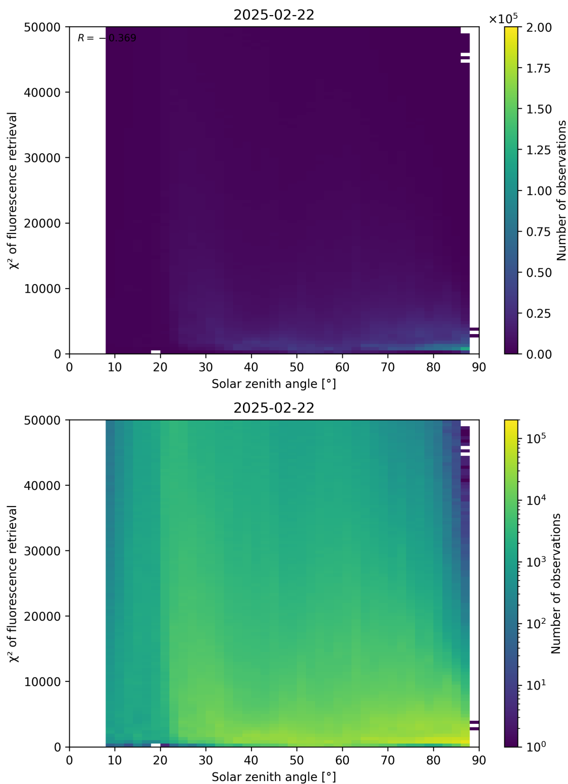
Figure 109: Scatter density plot of “Solar zenith angle” against “ \chi^2 of fluorescence retrieval” for 2025-02-21 to 2025-02-23.
