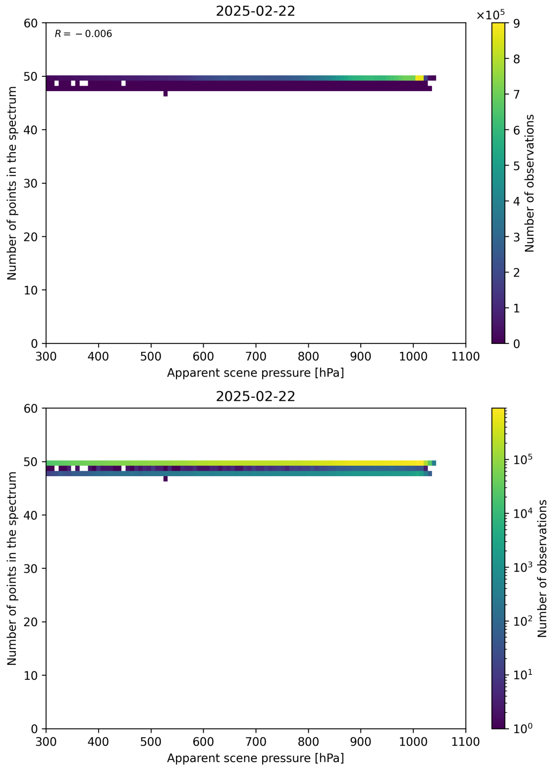
Figure 66: Scatter density plot of “Apparent scene pressure” against “Number of points in the spectrum” for 2025-02-21 to 2025-02-23.
