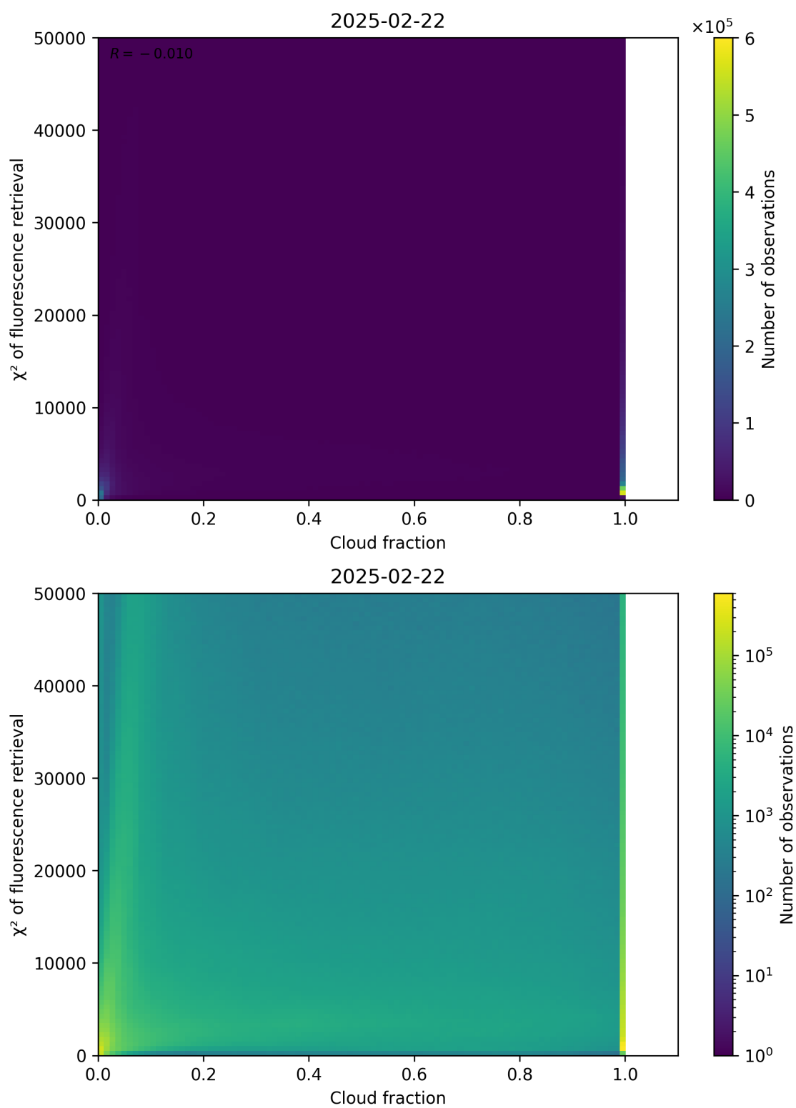
Figure 71: Scatter density plot of “Cloud fraction” against “ \chi^2 of fluorescence retrieval” for 2025-02-21 to 2025-02-23.
