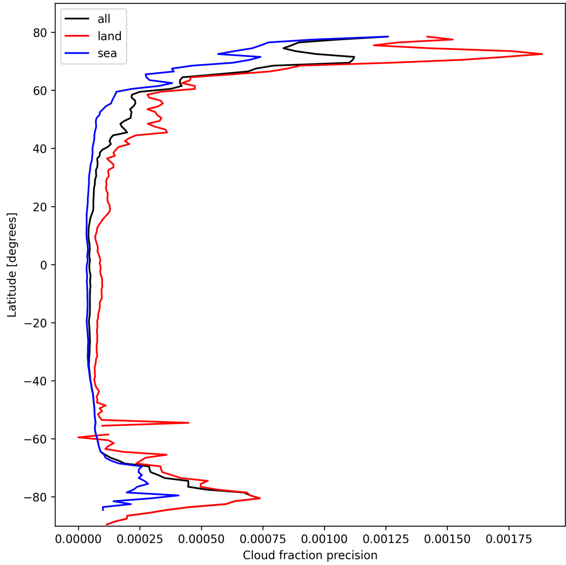
Figure 16: Zonal average of “Cloud fraction precision” for 2025-02-21 to 2025-02-23.
