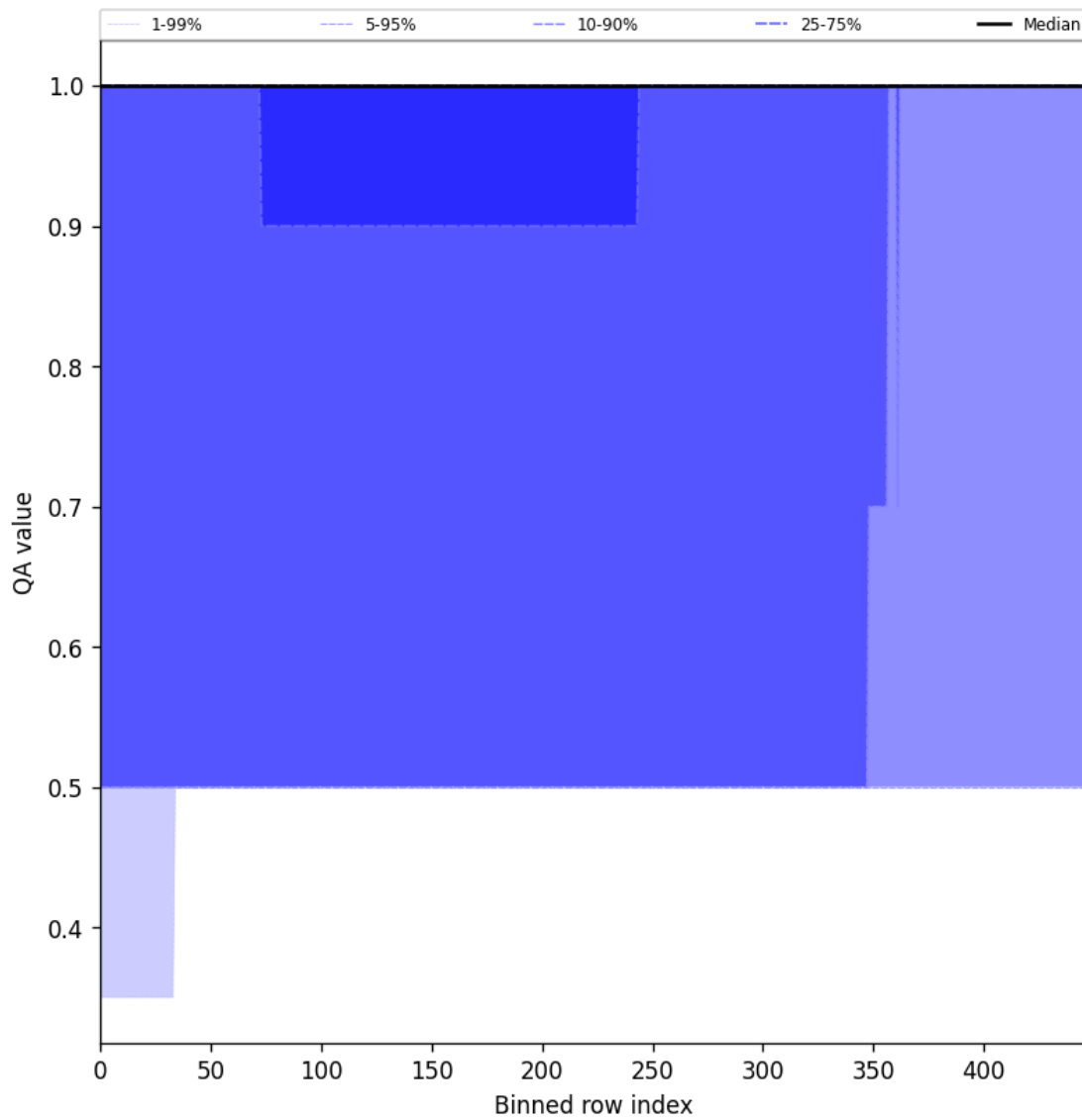
Figure 46: Along track statistics of “QA value” for 2025-02-21 to 2025-02-23
