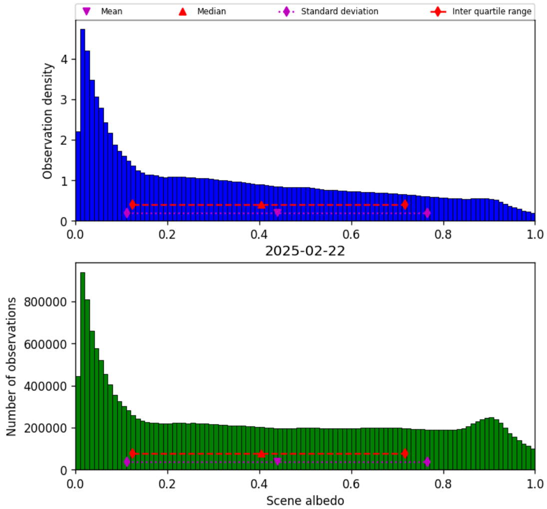
Figure 34: Histogram of “Scene albedo” for 2025-02-21 to 2025-02-23
