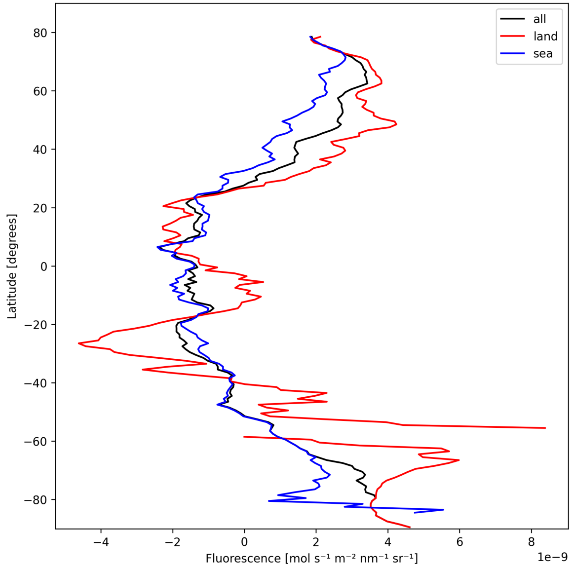
Figure 23: Zonal average of “Fluorescence” for 2025-02-21 to 2025-02-23.
