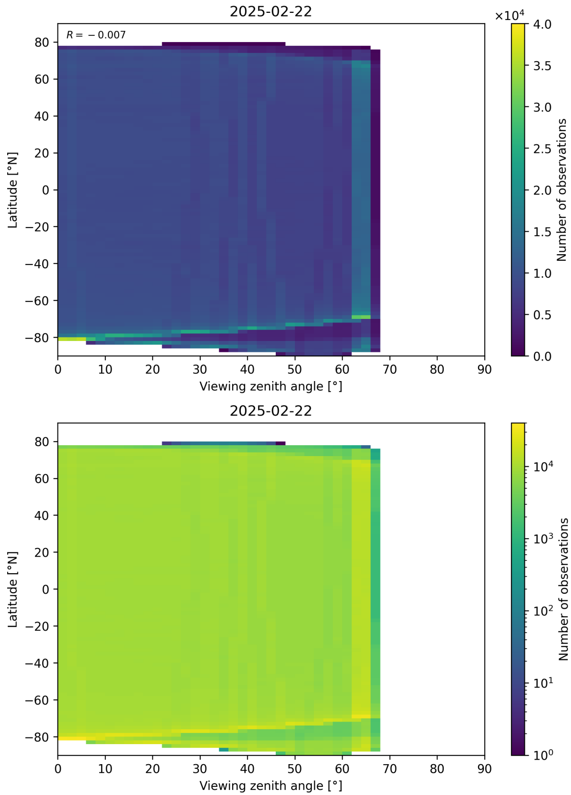
Figure 123: Scatter density plot of “Viewing zenith angle” against “Latitude” for 2025-02-21 to 2025-02-23.
