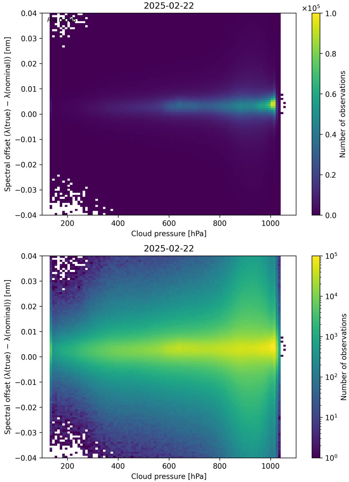
Figure 84: Scatter density plot of “Cloud pressure” against “Spectral offset ( \lambda_{\text{true}} - \lambda_{\text{nominal}} )” for 2025-02-21 to 2025-02-23.
