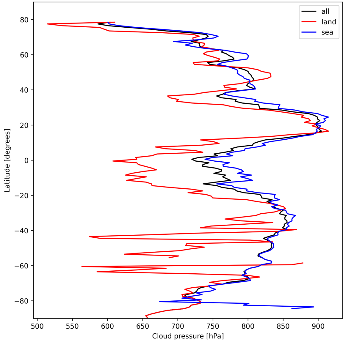
Figure 13: Zonal average of “Cloud pressure” for 2025-02-21 to 2025-02-23.
