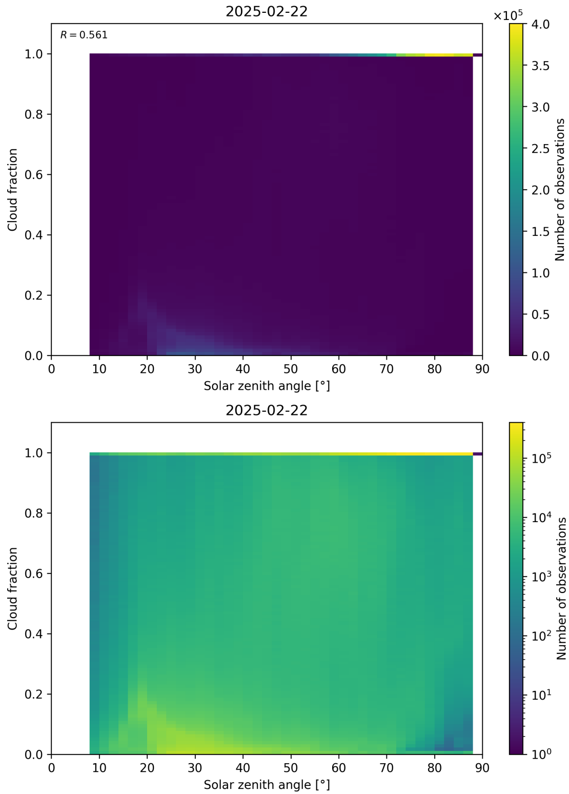
Figure 110: Scatter density plot of “Solar zenith angle” against “Cloud fraction” for 2025-02-21 to 2025-02-23.
