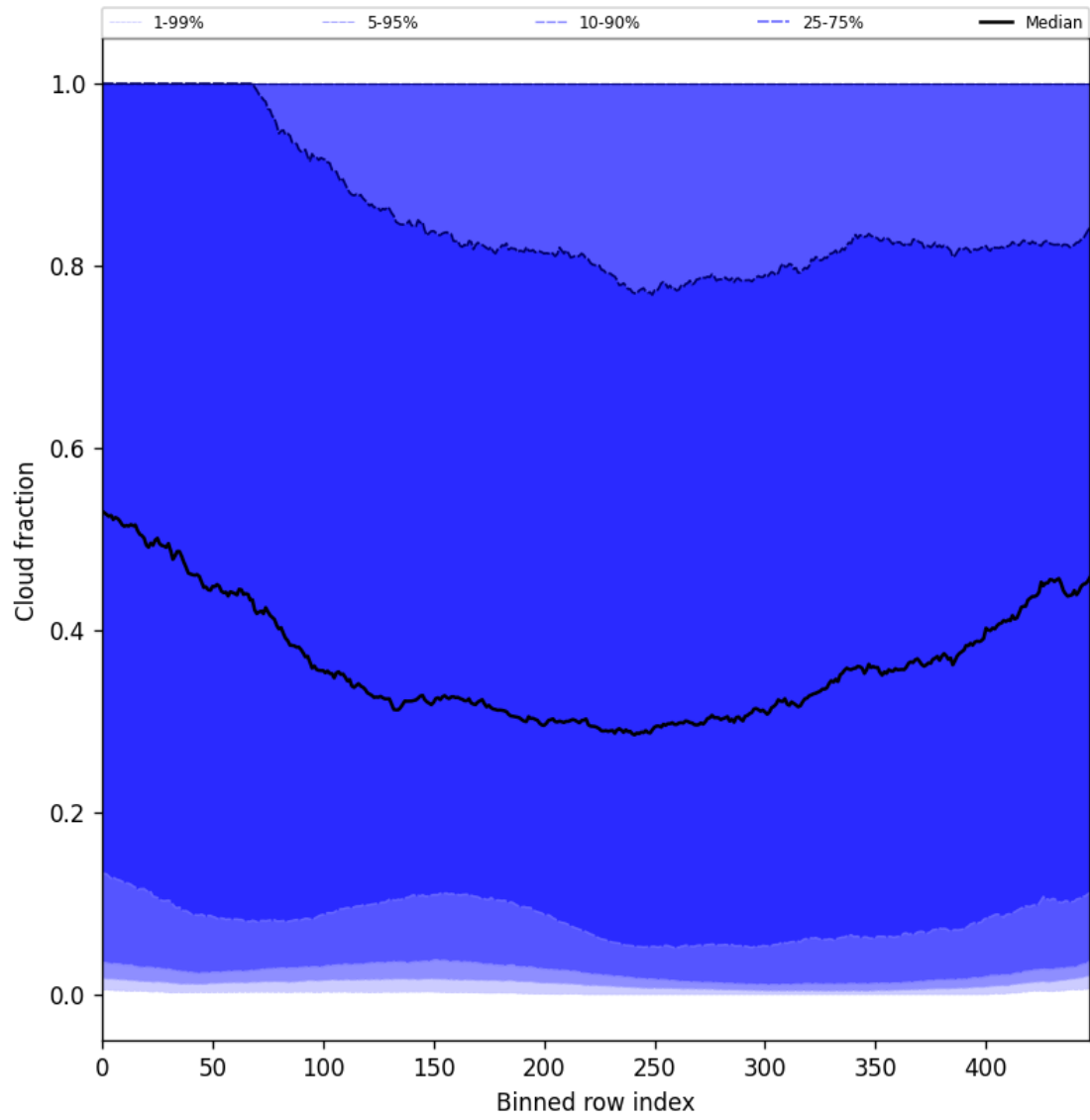
Figure 49: Along track statistics of “Cloud fraction” for 2025-02-21 to 2025-02-23
