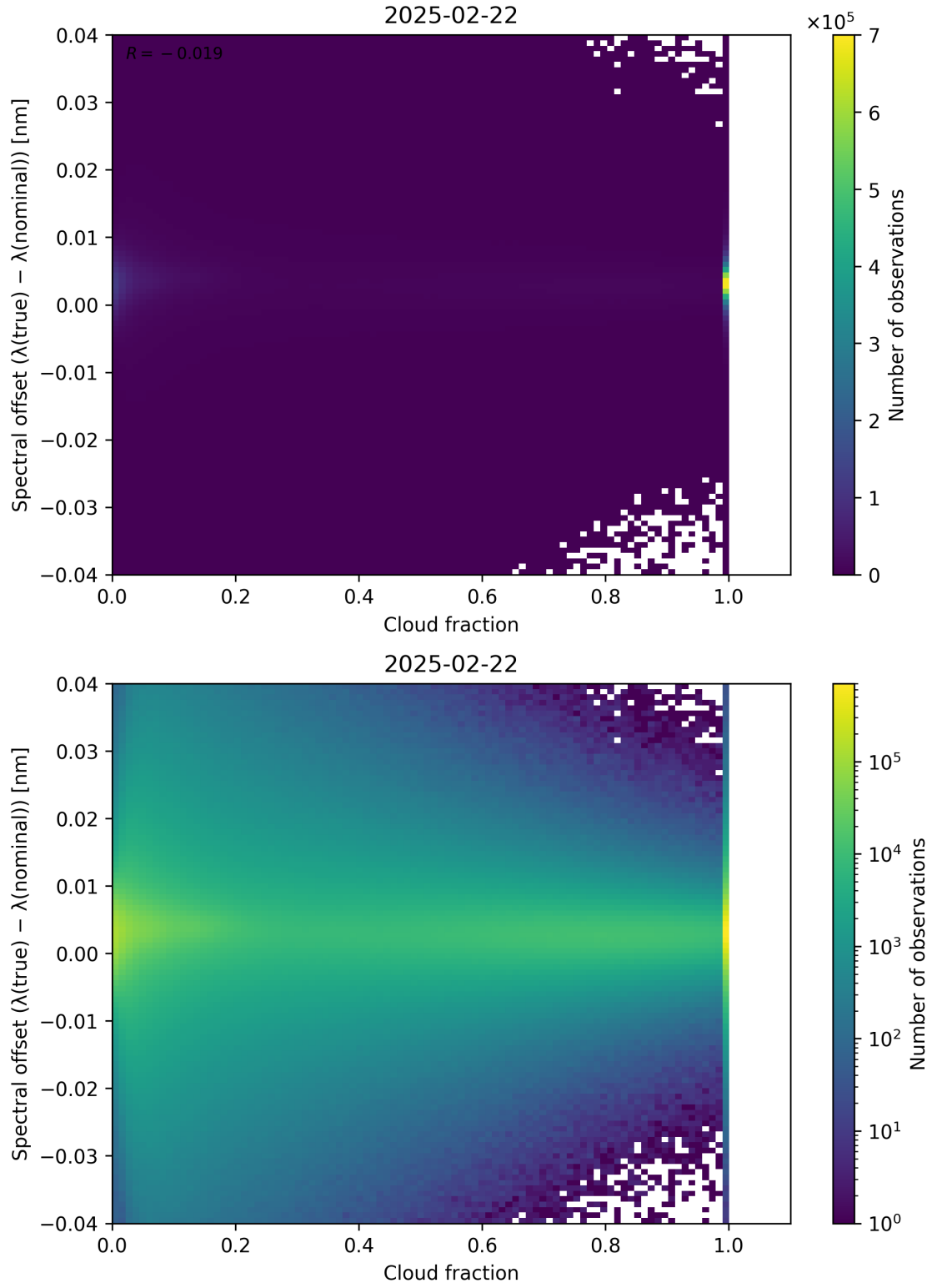
Figure 76: Scatter density plot of “Cloud fraction” against “Spectral offset ( \lambda_{\text{true}} - \lambda_{\text{nominal}} )” for 2025-02-21 to 2025-02-23.
