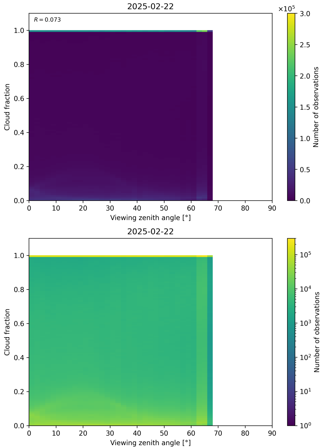
Figure 120: Scatter density plot of “Viewing zenith angle” against “Cloud fraction” for 2025-02-21 to 2025-02-23.
