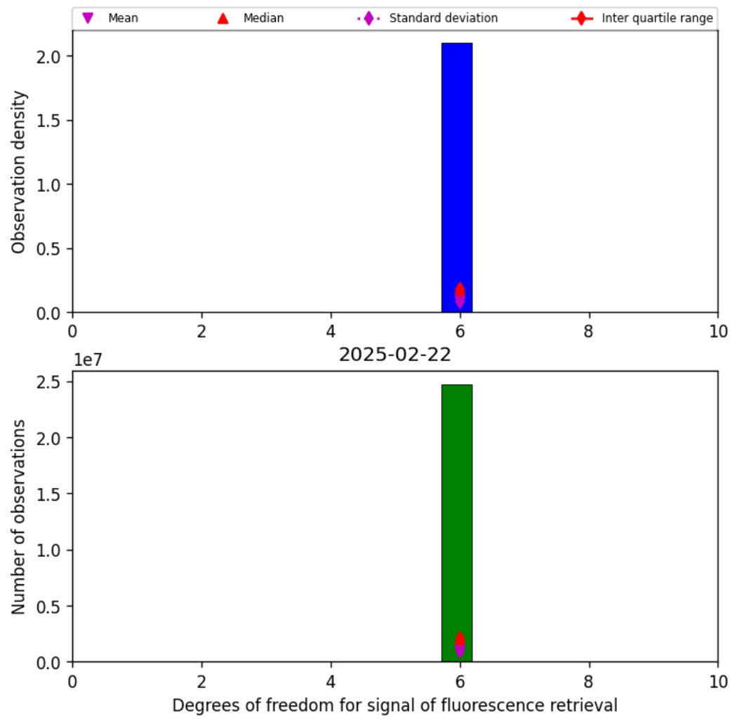
Figure 43: Histogram of "Degrees of freedom for signal of fluorescence retrieval" for 2025-02-21 to 2025-02-23
