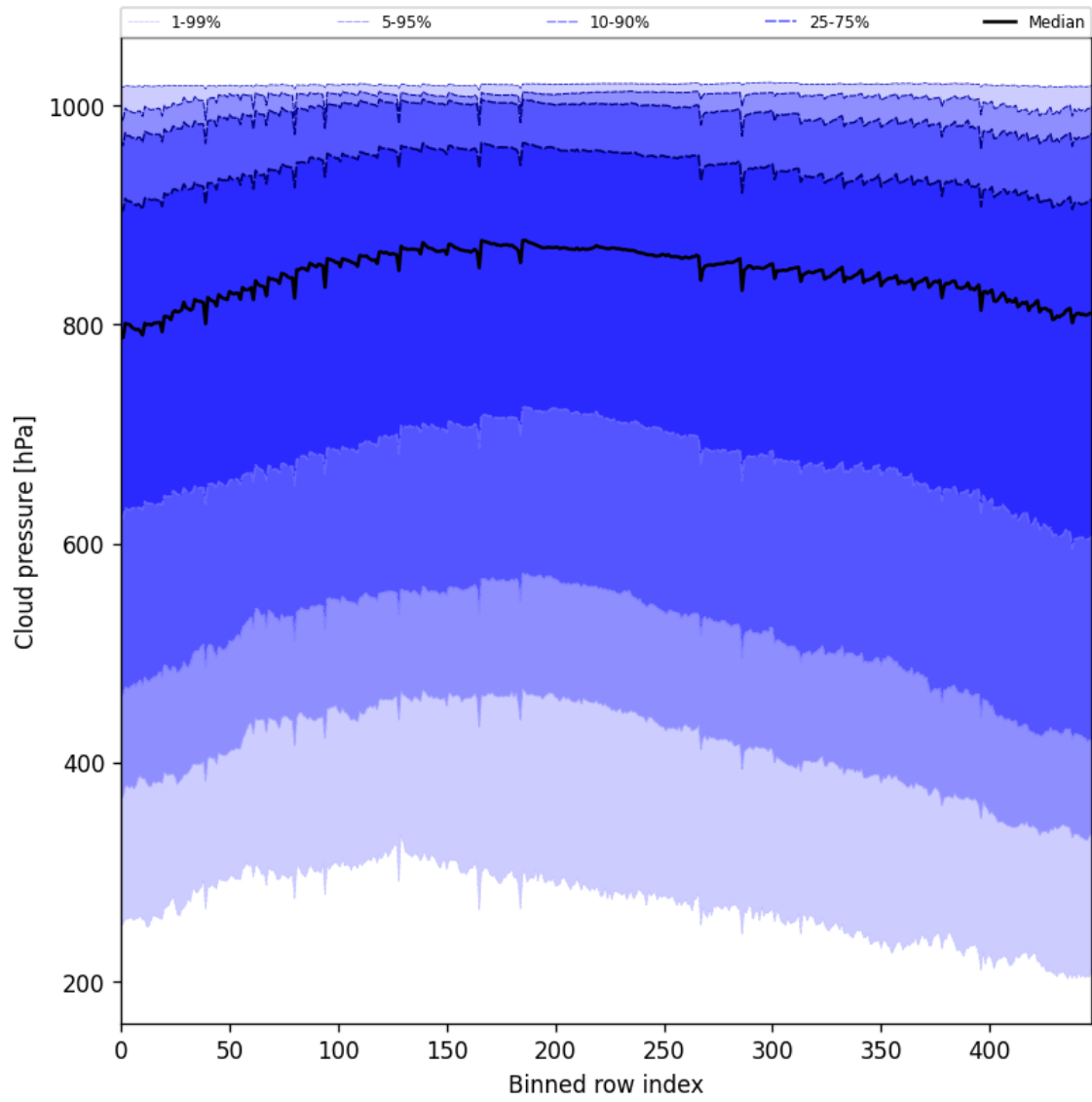
Figure 47: Along track statistics of “Cloud pressure” for 2025-02-21 to 2025-02-23
