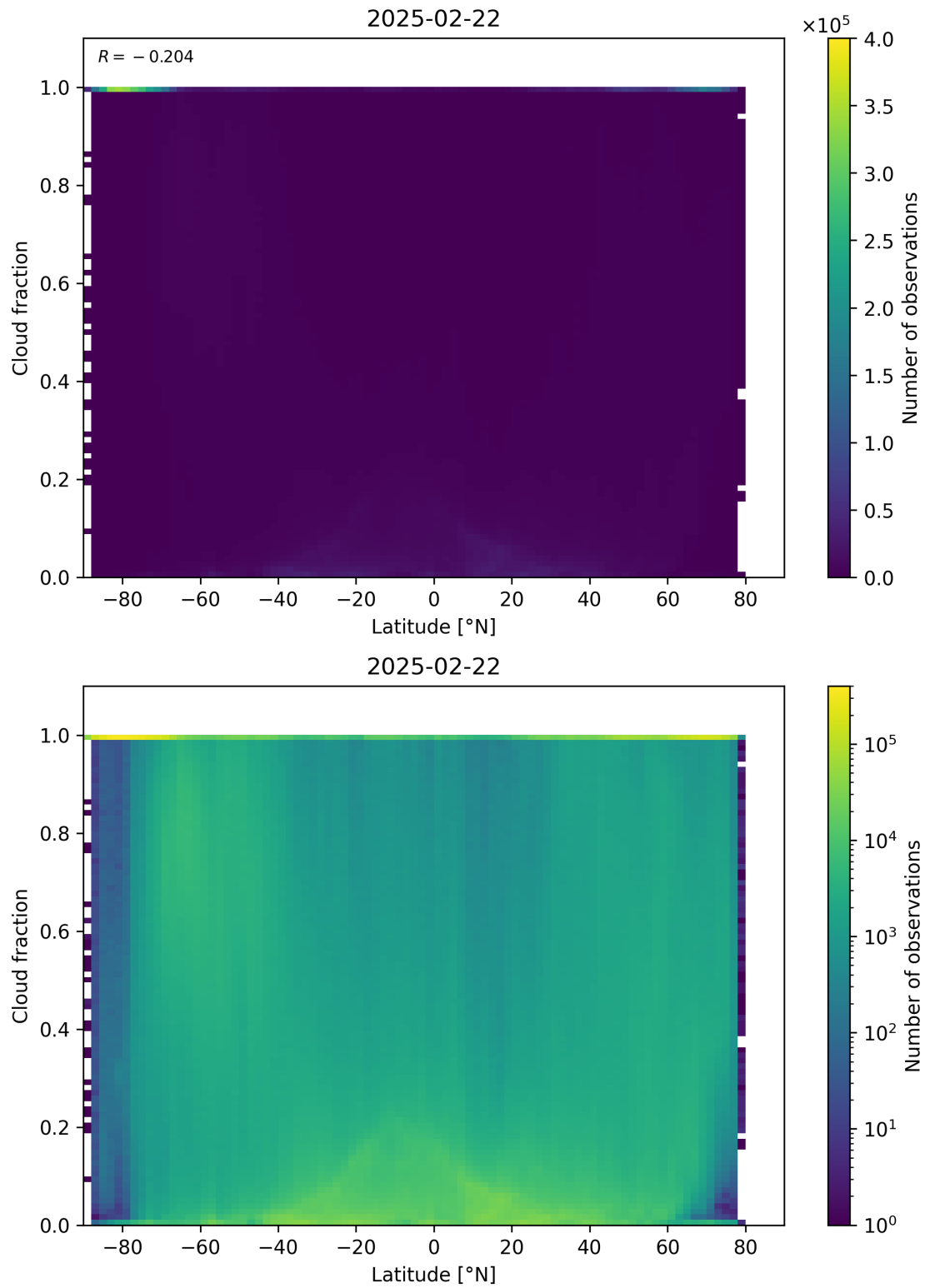
Figure 90: Scatter density plot of “Latitude” against “Cloud fraction” for 2025-02-21 to 2025-02-23.
