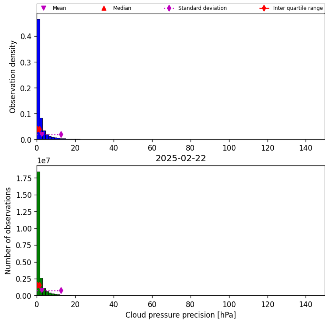
Figure 31: Histogram of “Cloud pressure precision” for 2025-02-21 to 2025-02-23
