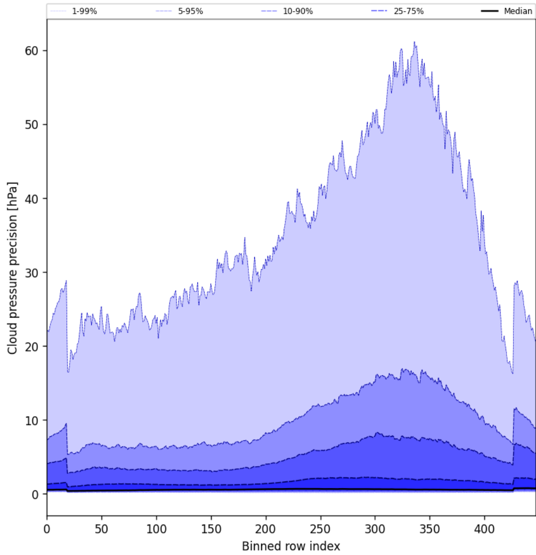
Figure 48: Along track statistics of “Cloud pressure precision” for 2025-02-21 to 2025-02-23
