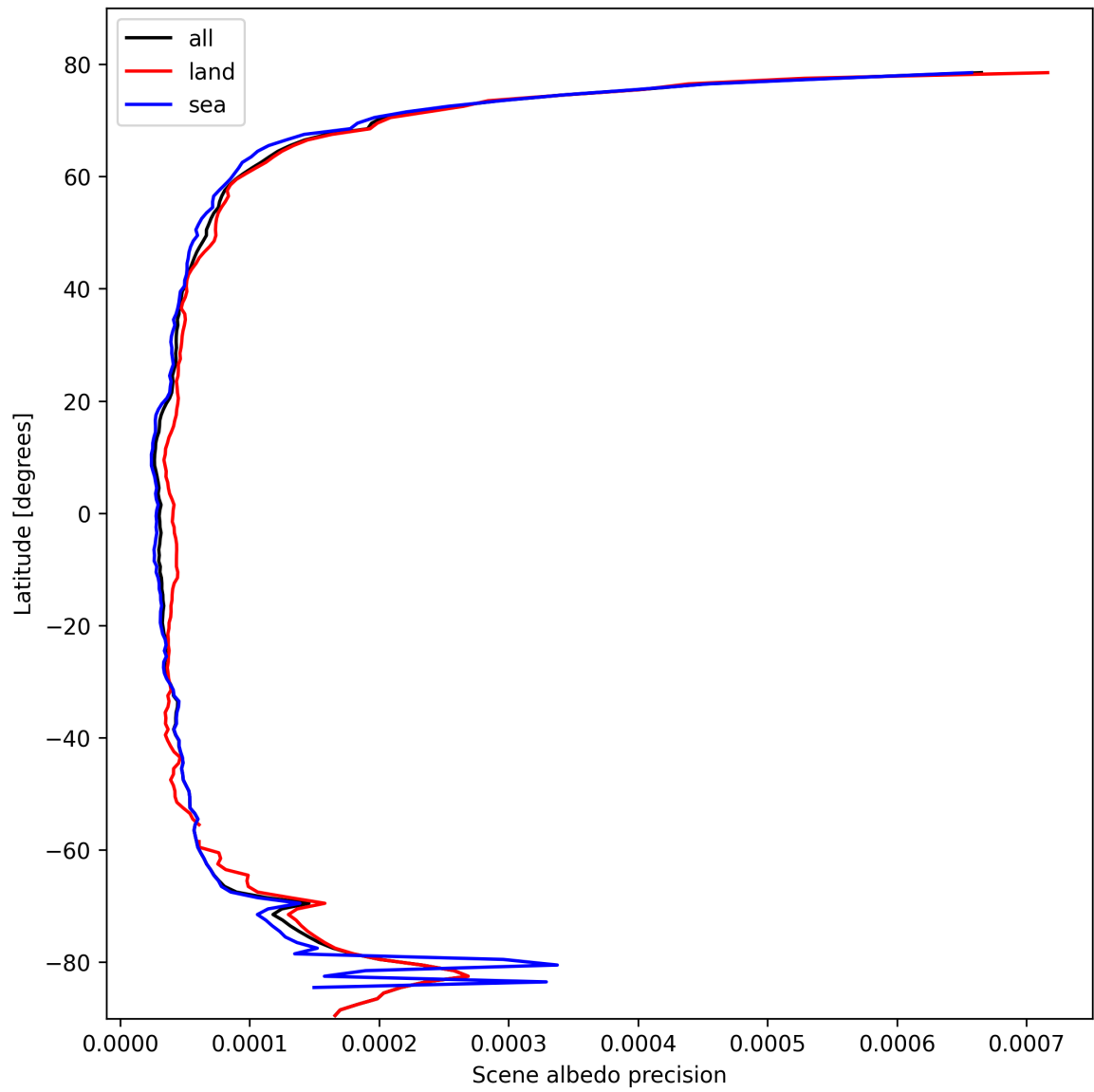
Figure 18: Zonal average of “Scene albedo precision” for 2025-02-21 to 2025-02-23.
