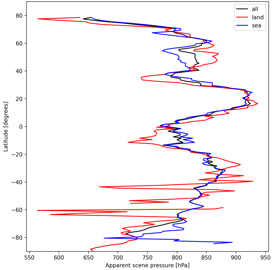
Figure 19: Zonal average of “Apparent scene pressure” for 2025-02-21 to 2025-02-23.
