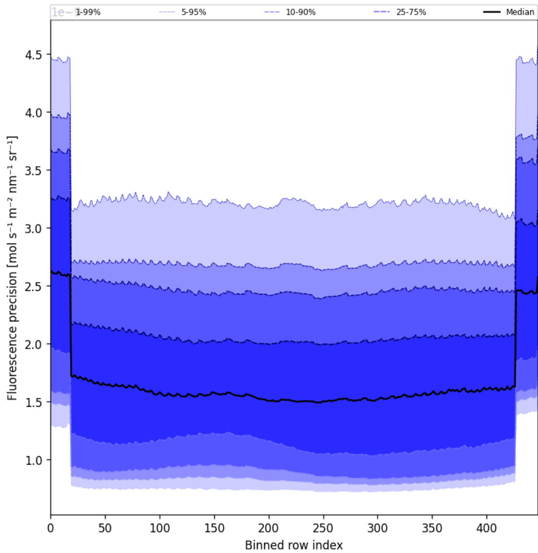
Figure 58: Along track statistics of "Fluorescence precision" for 2025-02-21 to 2025-02-23
