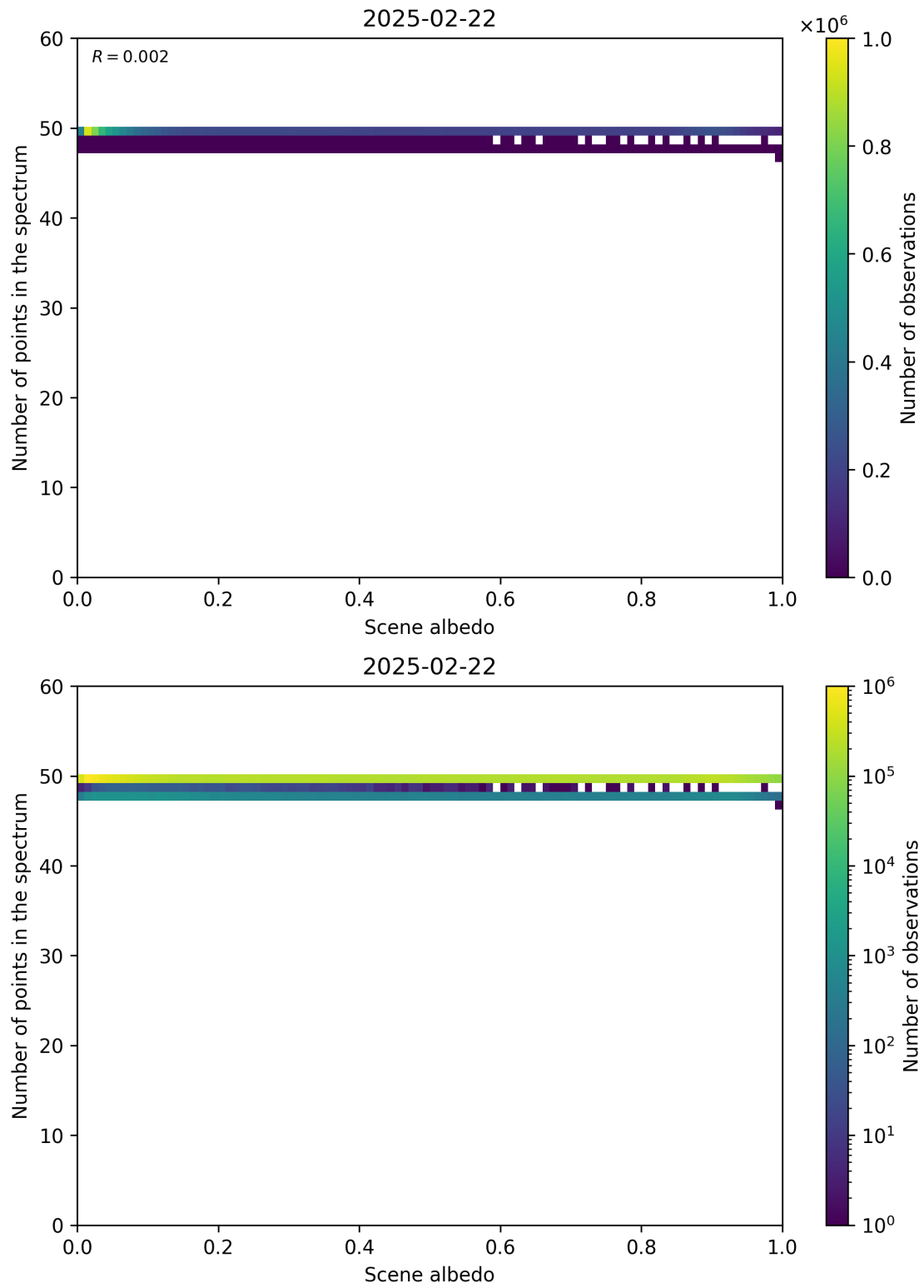
Figure 106: Scatter density plot of “Scene albedo” against “Number of points in the spectrum” for 2025-02-21 to 2025-02-23.
