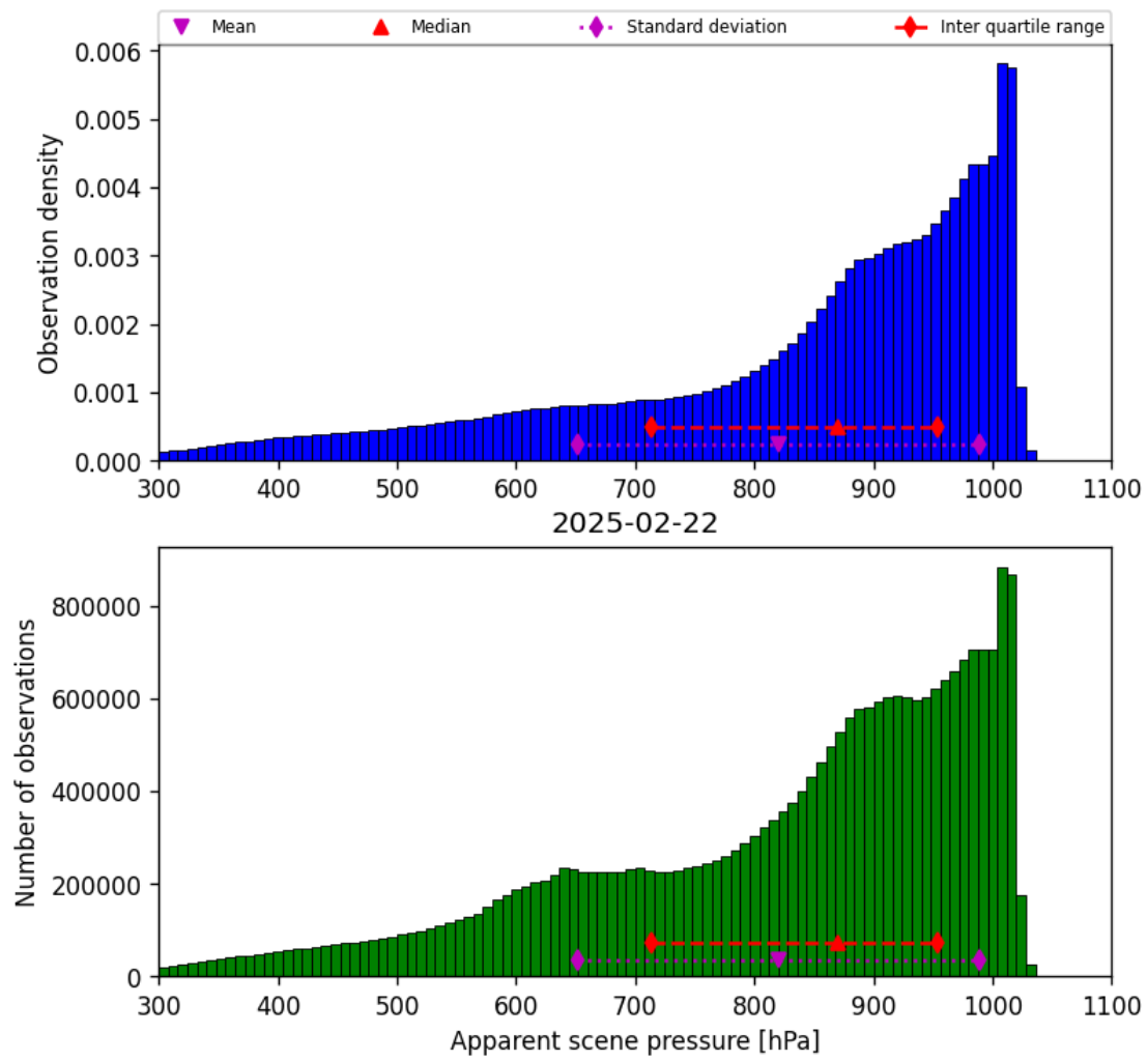
Figure 36: Histogram of “Apparent scene pressure” for 2025-02-21 to 2025-02-23
