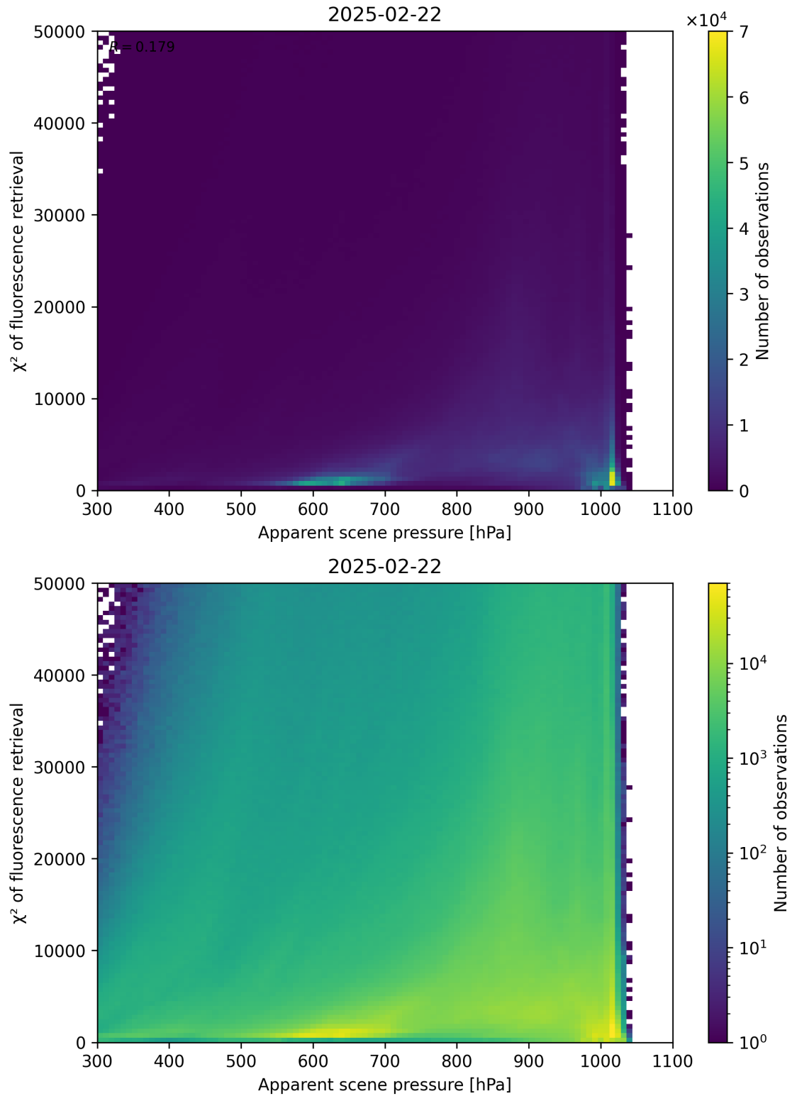
Figure 63: Scatter density plot of “Apparent scene pressure” against “ \chi^2 of fluorescence retrieval” for 2025-02-21 to 2025-02-23.
