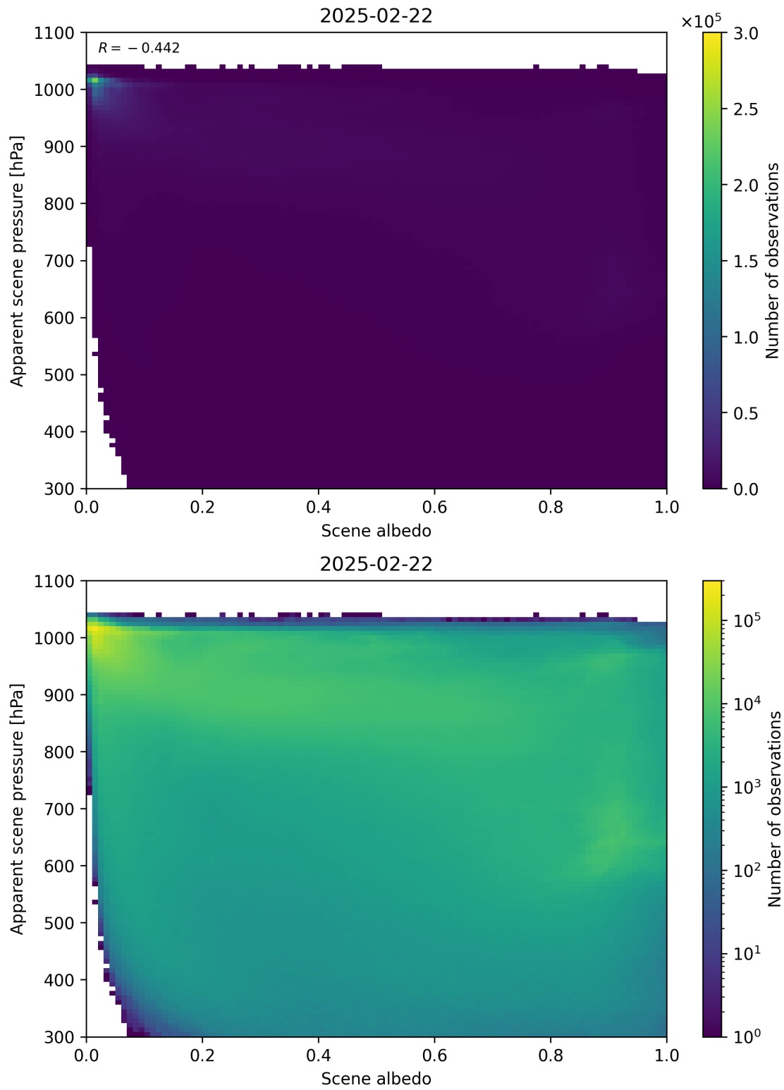
Figure 102: Scatter density plot of “Scene albedo” against “Apparent scene pressure” for 2025-02-21 to 2025-02-23.
