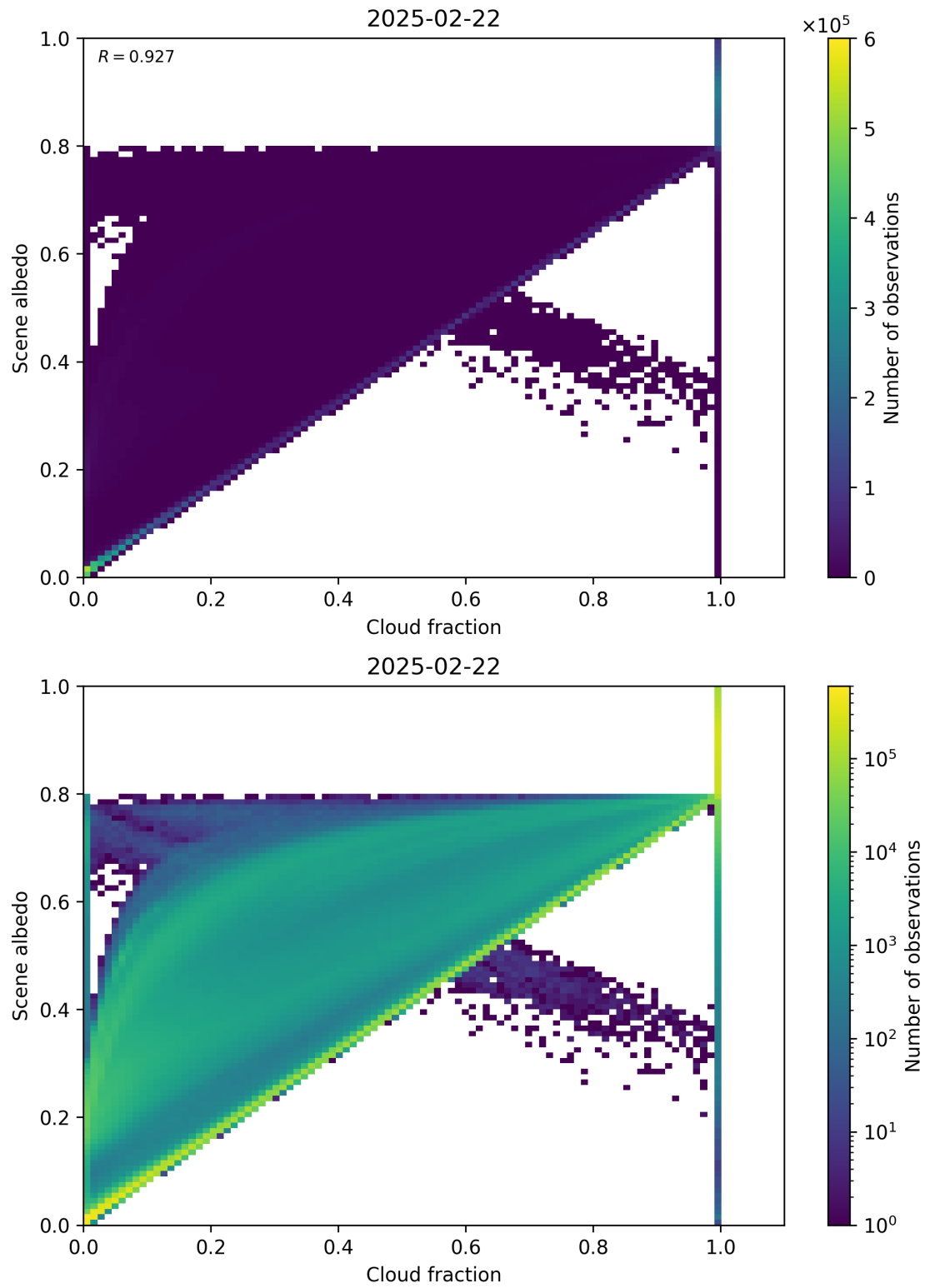
Figure 75: Scatter density plot of “Cloud fraction” against “Scene albedo” for 2025-02-21 to 2025-02-23.
