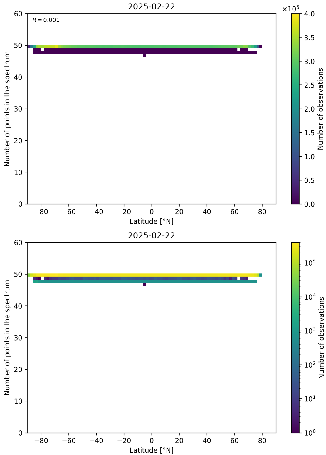
Figure 94: Scatter density plot of “Latitude” against “Number of points in the spectrum” for 2025-02-21 to 2025-02-23.
