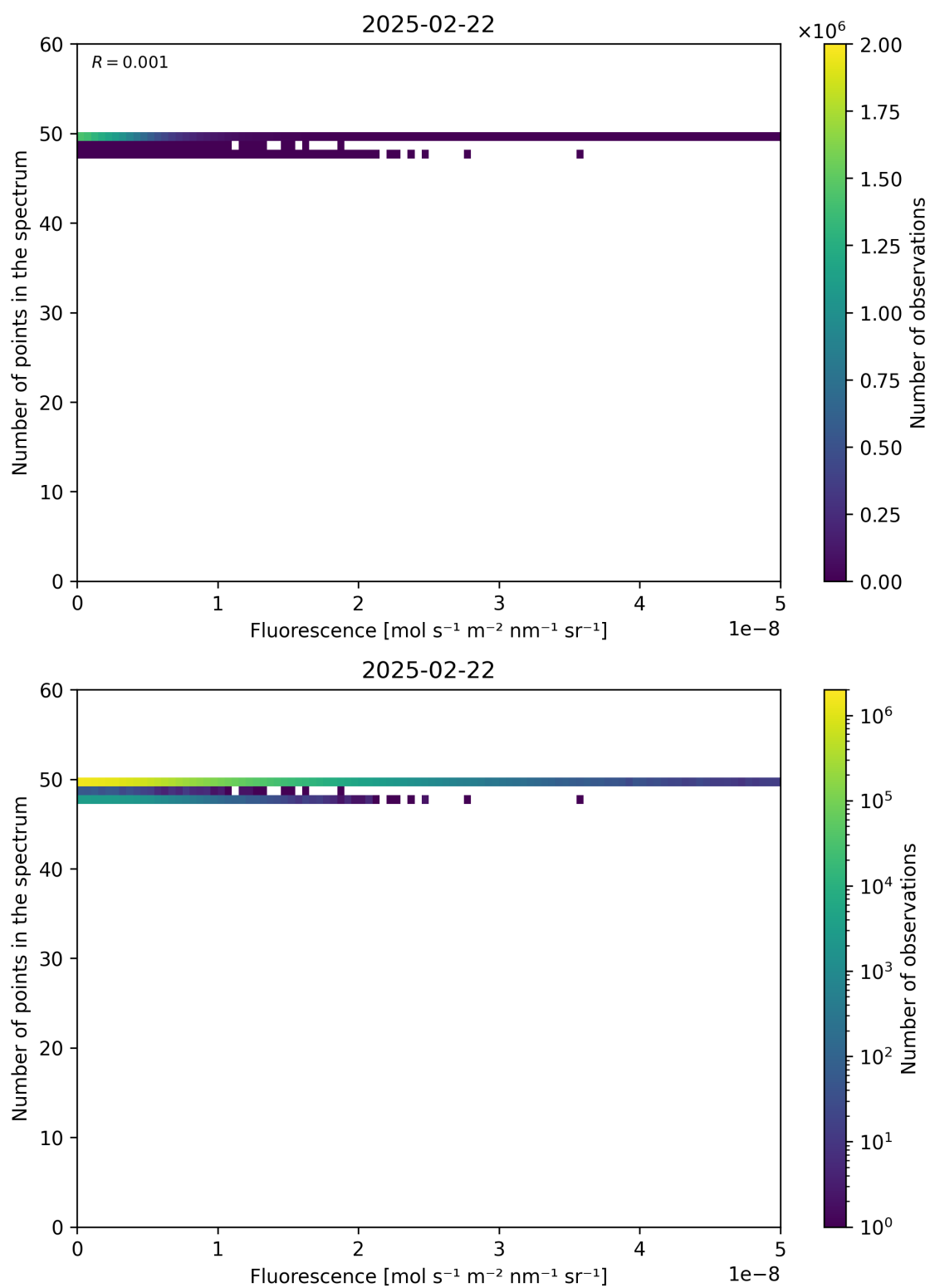
Figure 86: Scatter density plot of “Fluorescence” against “Number of points in the spectrum” for 2025-02-21 to 2025-02-23.
