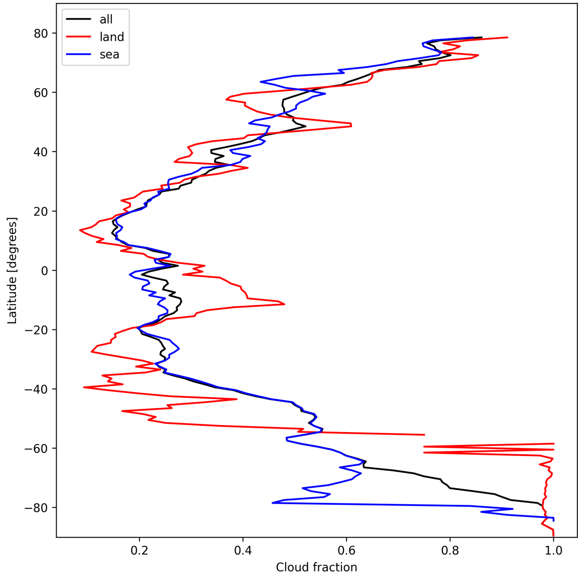
Figure 15: Zonal average of “Cloud fraction” for 2025-02-21 to 2025-02-23.
