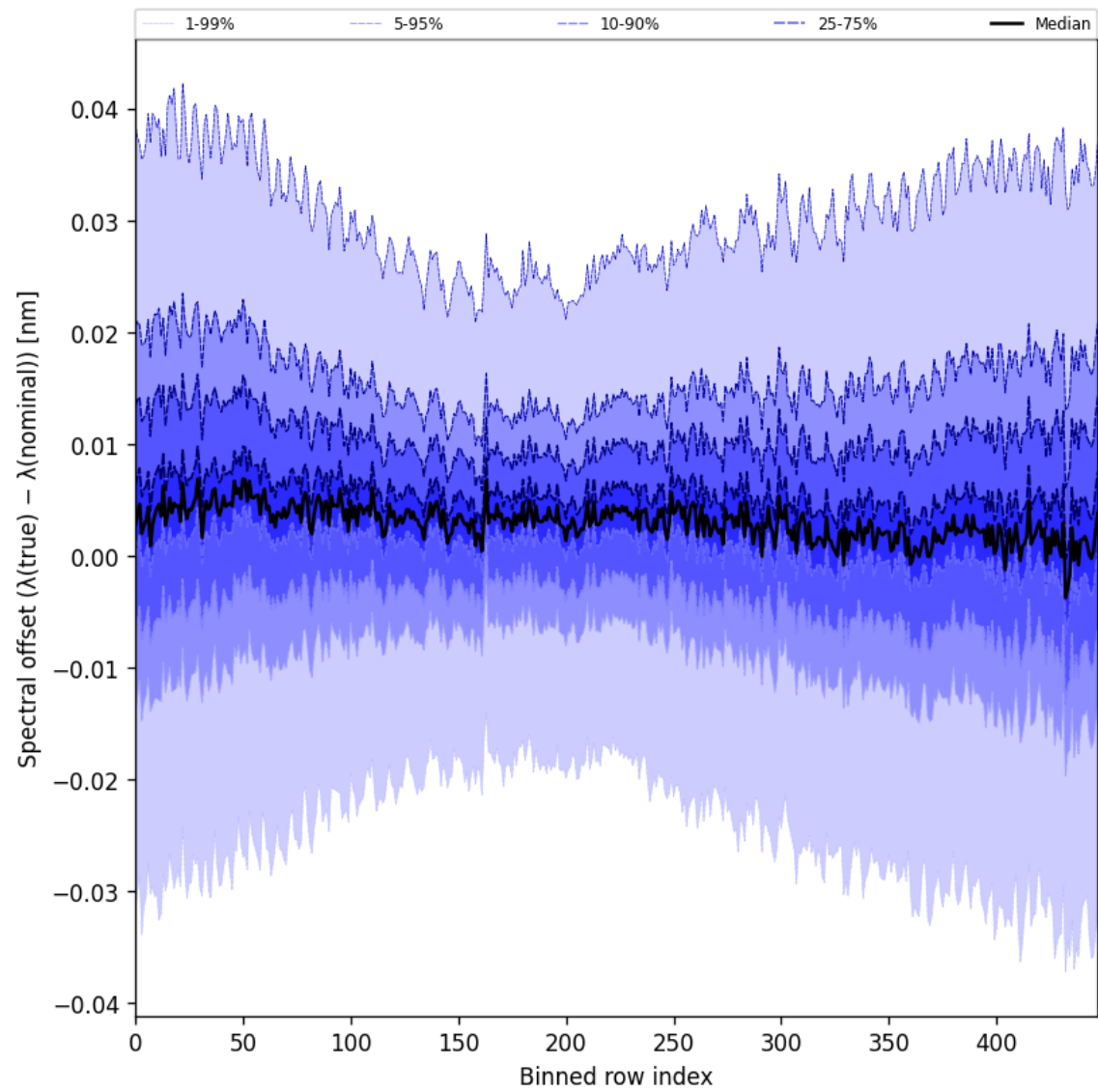
Figure 62: Along track statistics of “Spectral offset ( \lambda_{\text{true}} - \lambda_{\text{nominal}} )” for 2025-02-21 to 2025-02-23
