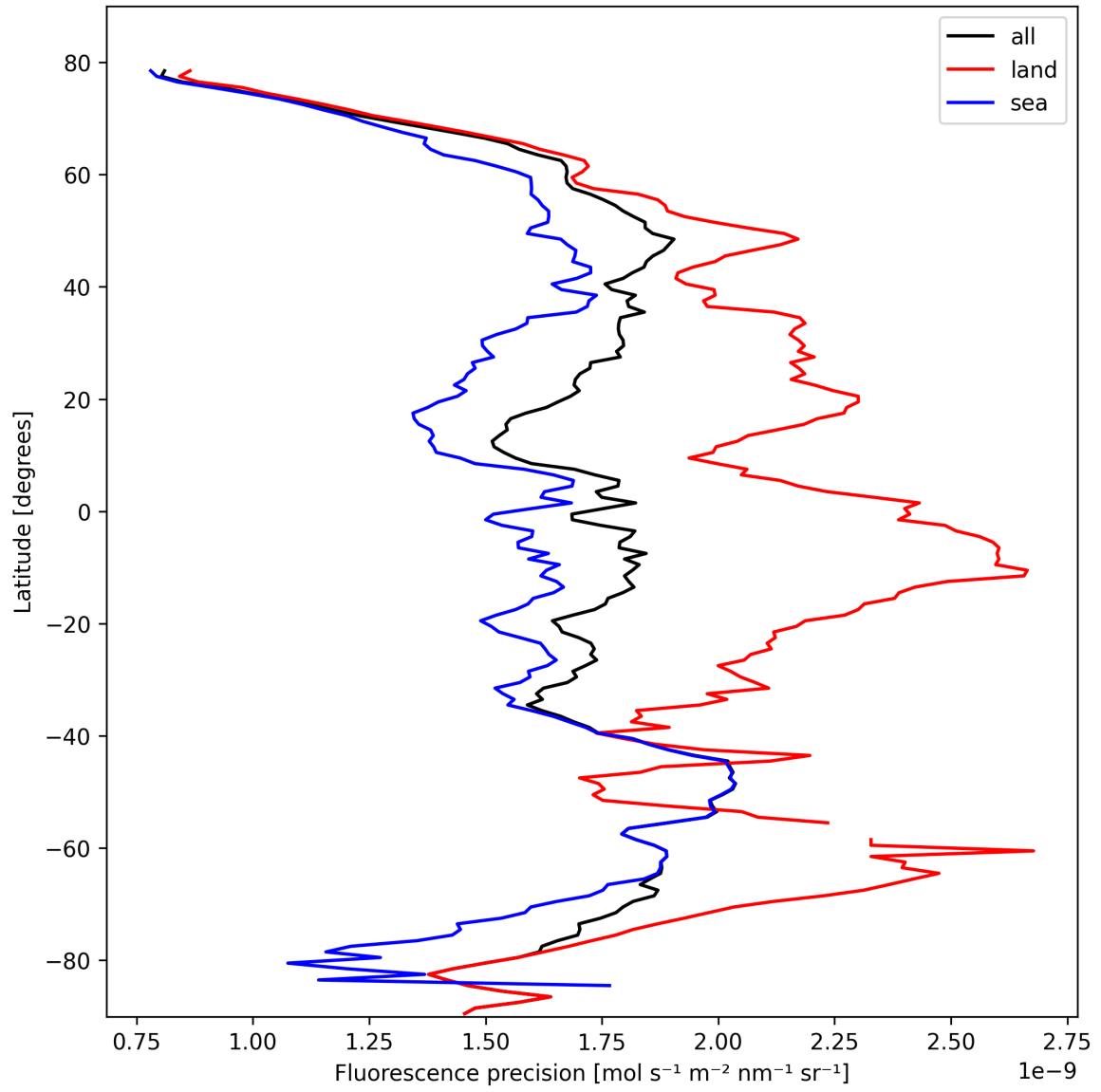
Figure 24: Zonal average of “Fluorescence precision” for 2025-02-21 to 2025-02-23.
