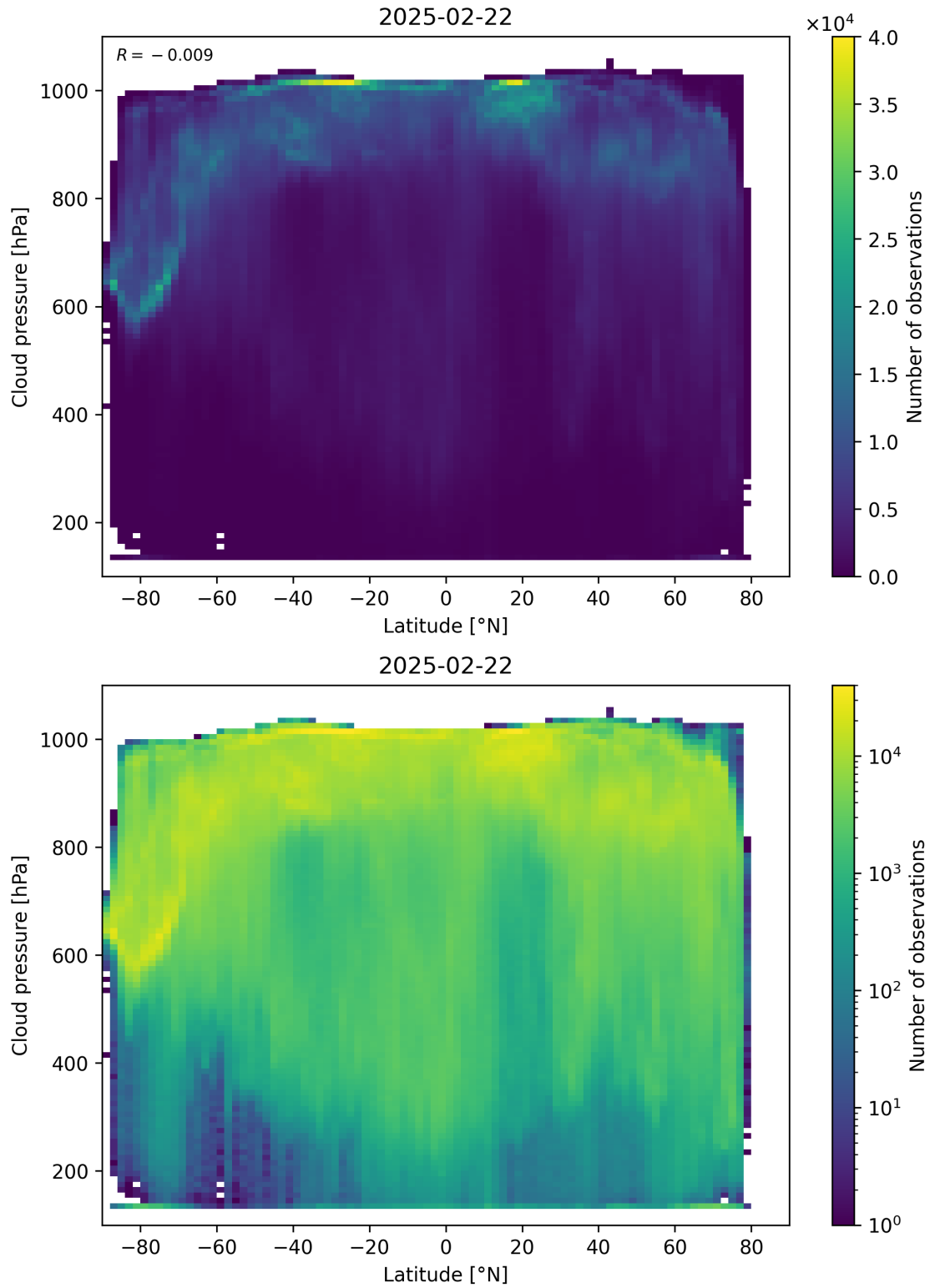
Figure 91: Scatter density plot of “Latitude” against “Cloud pressure” for 2025-02-21 to 2025-02-23.
