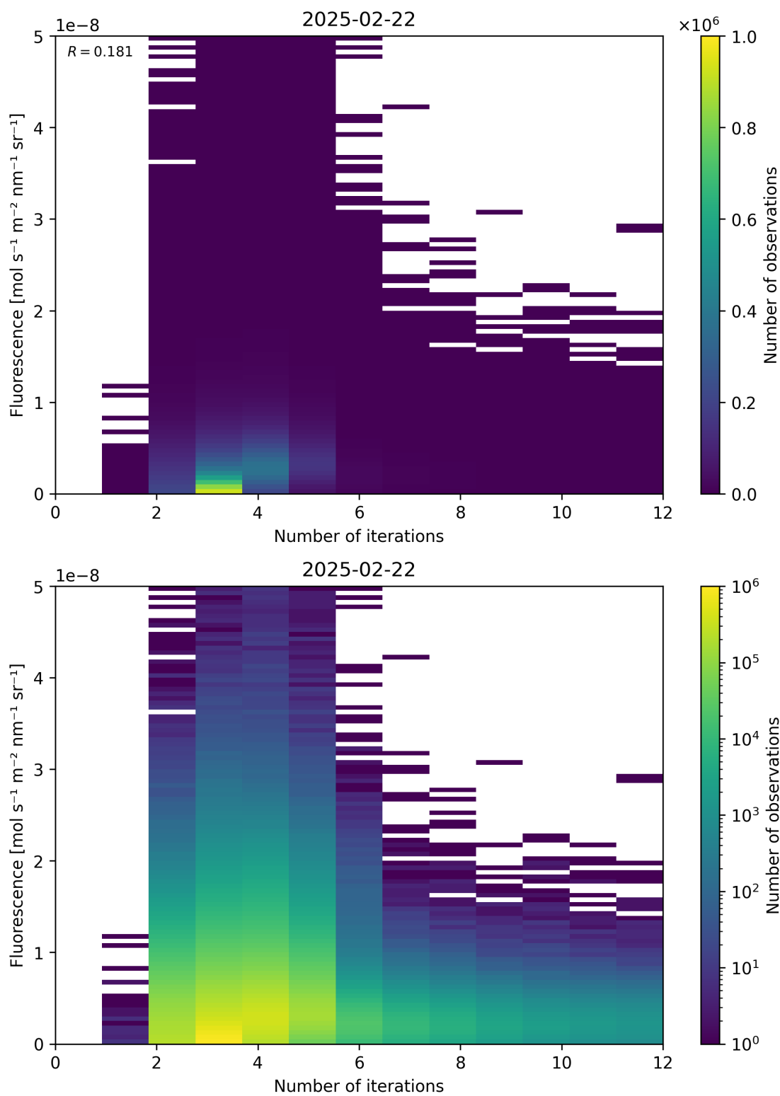
Figure 98: Scatter density plot of “Number of iterations” against “Fluorescence” for 2025-02-21 to 2025-02-23.
