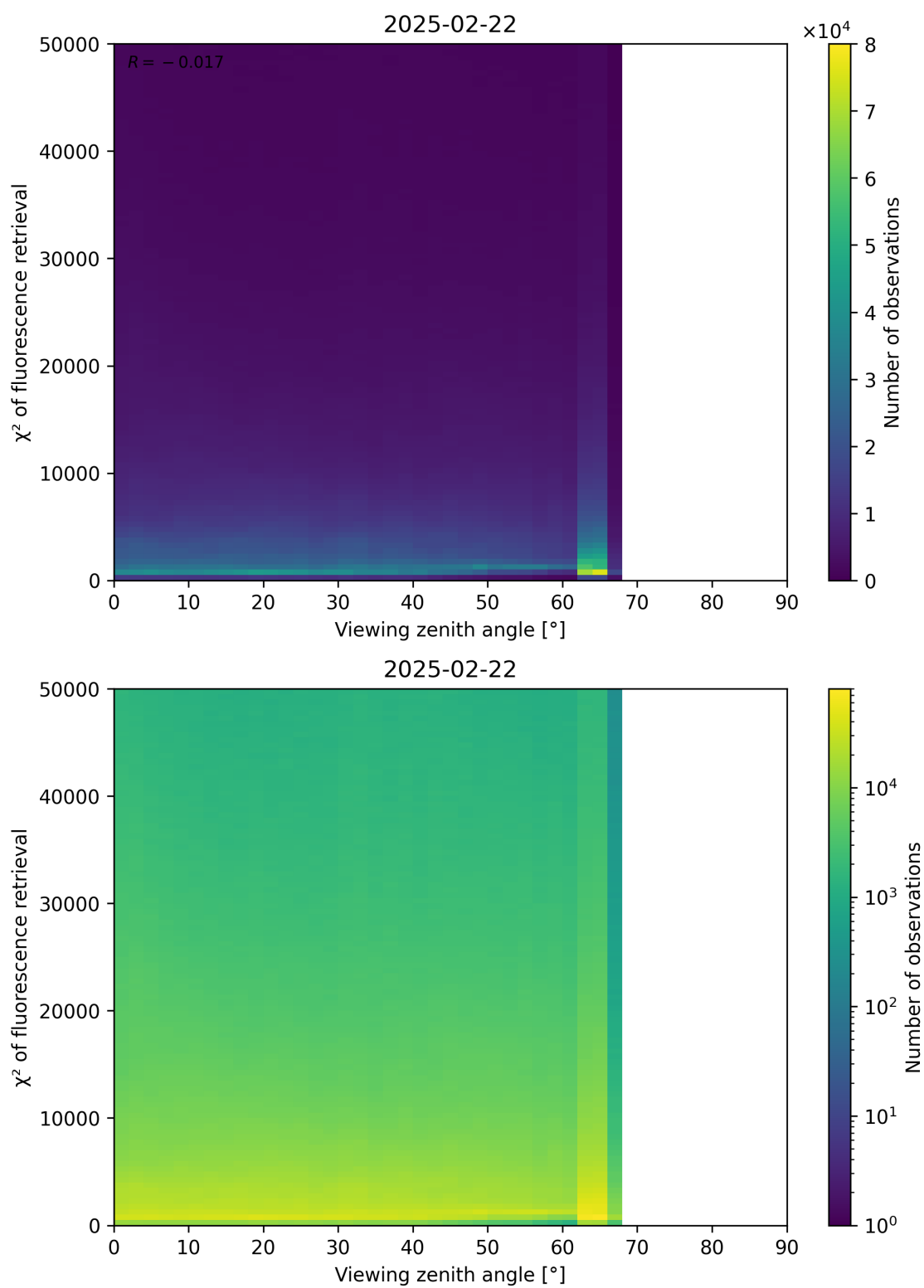
Figure 119: Scatter density plot of “Viewing zenith angle” against “ \chi^2 of fluorescence retrieval” for 2025-02-21 to 2025-02-23.
