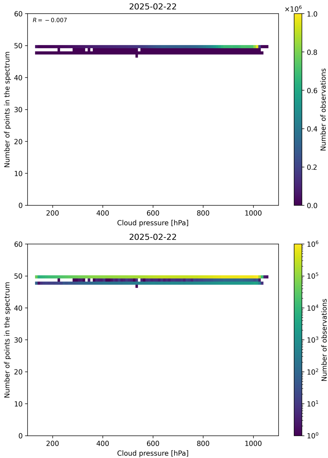
Figure 82: Scatter density plot of “Cloud pressure” against “Number of points in the spectrum” for 2025-02-21 to 2025-02-23.
