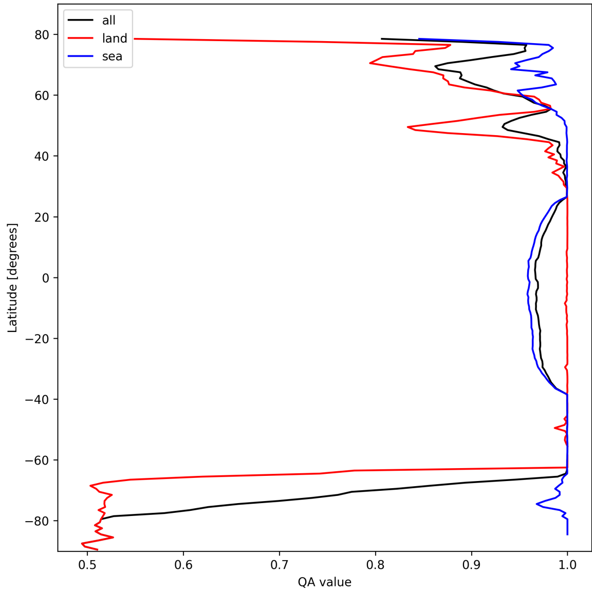
Figure 12: Zonal average of “QA value” for 2025-02-21 to 2025-02-23.
