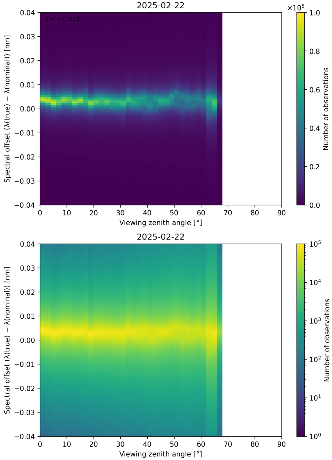
Figure 128: Scatter density plot of “Viewing zenith angle” against “Spectral offset ( \lambda_{\text{true}} - \lambda_{\text{nominal}} )” for 2025-02-21 to 2025-02-23.
