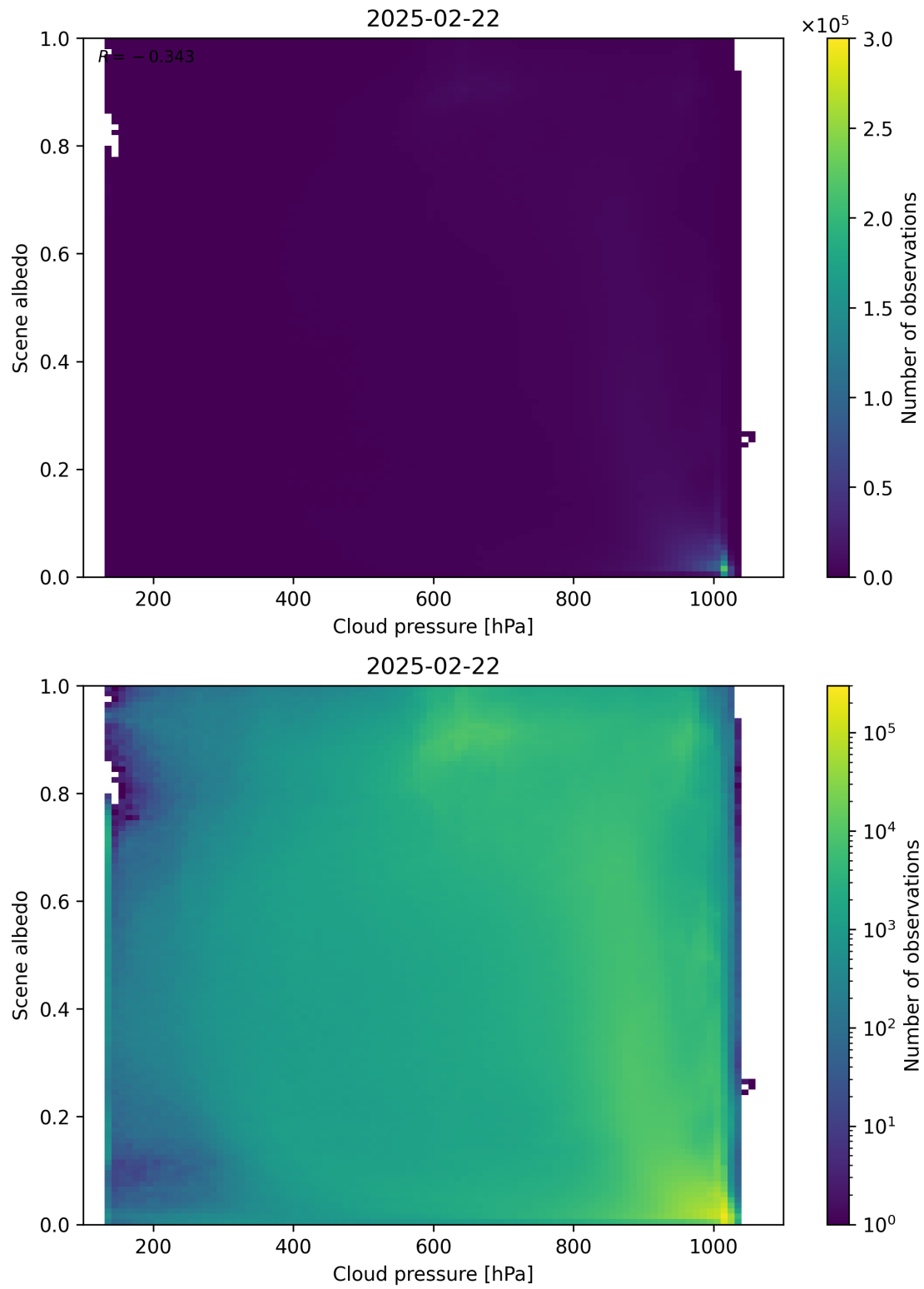
Figure 83: Scatter density plot of “Cloud pressure” against “Scene albedo” for 2025-02-21 to 2025-02-23.
