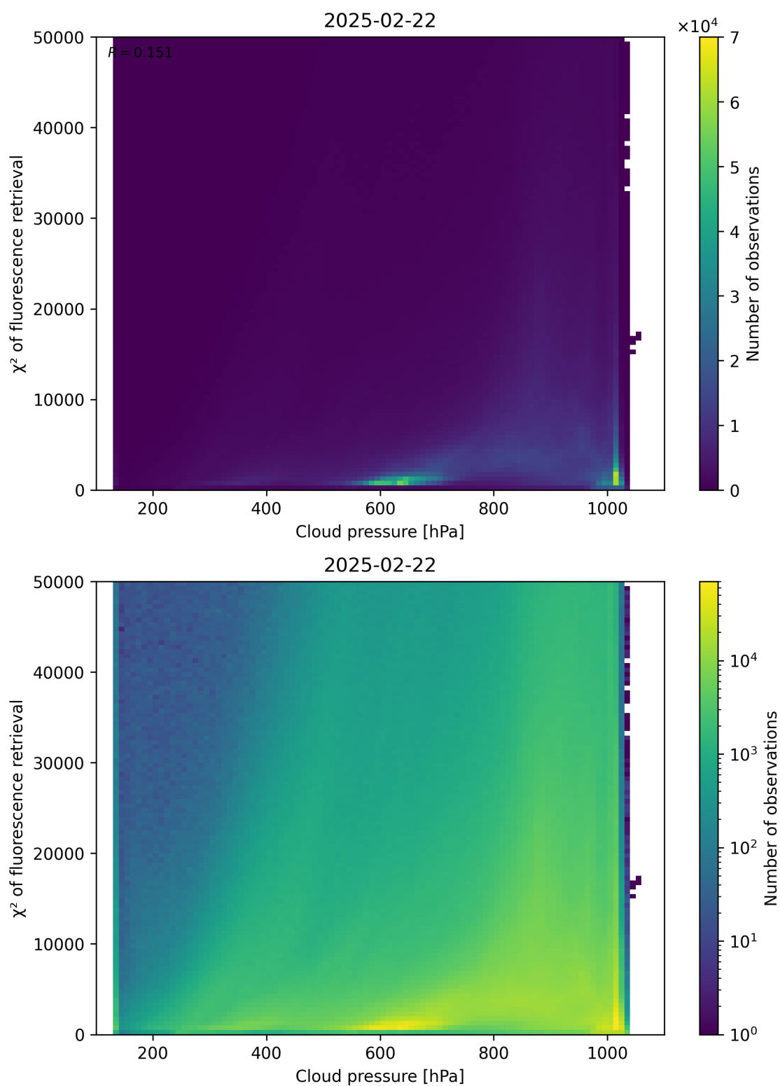
Figure 78: Scatter density plot of “Cloud pressure” against “ \chi^2 of fluorescence retrieval” for 2025-02-21 to 2025-02-23.
