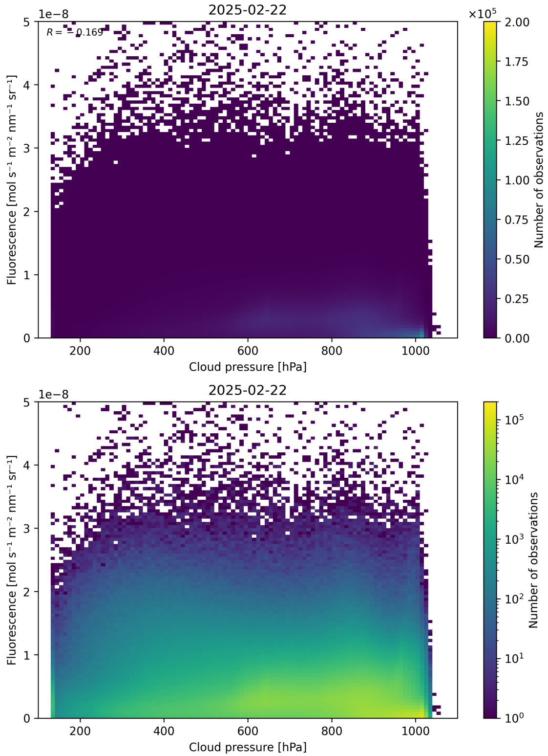
Figure 80: Scatter density plot of “Cloud pressure” against “Fluorescence” for 2025-02-21 to 2025-02-23.
