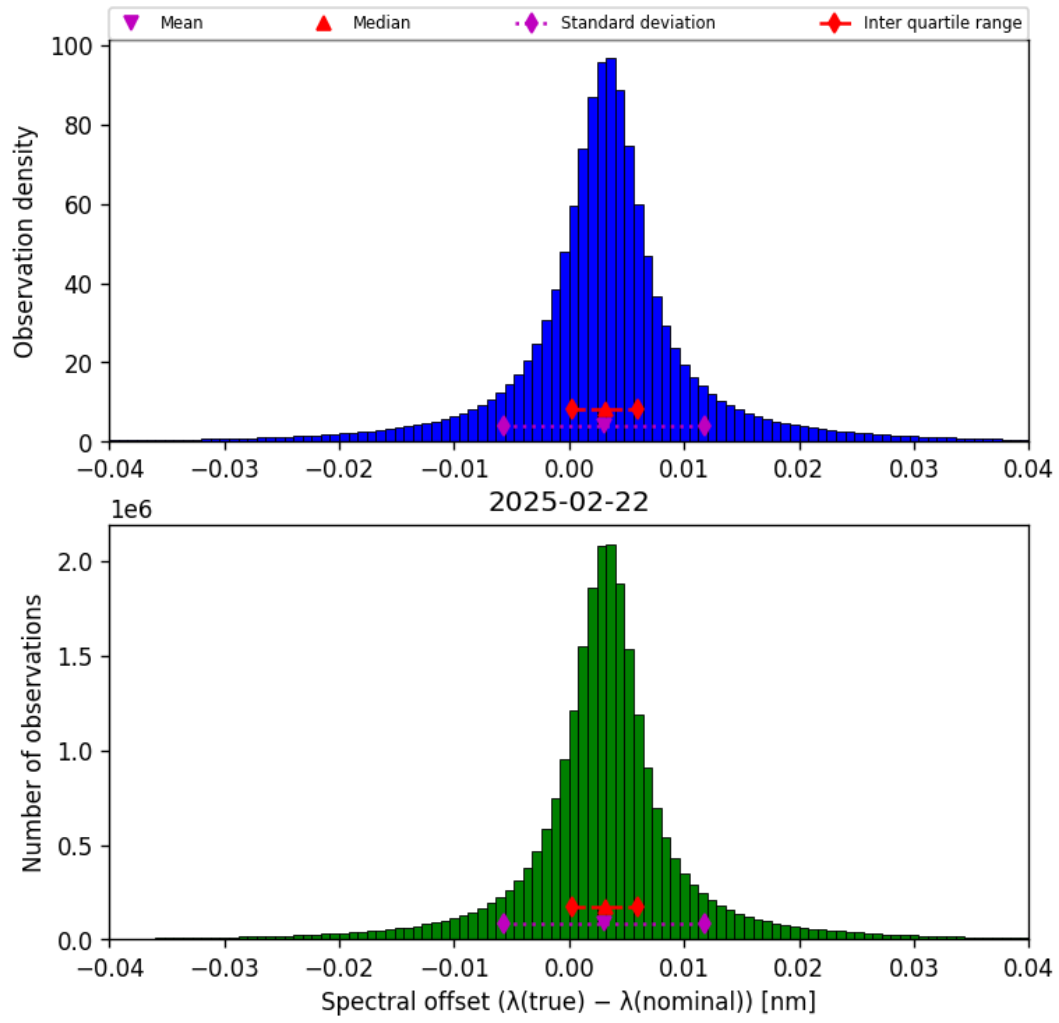
Figure 45: Histogram of “Spectral offset ( \lambda_{\text{true}} - \lambda_{\text{nominal}} )” for 2025-02-21 to 2025-02-23
