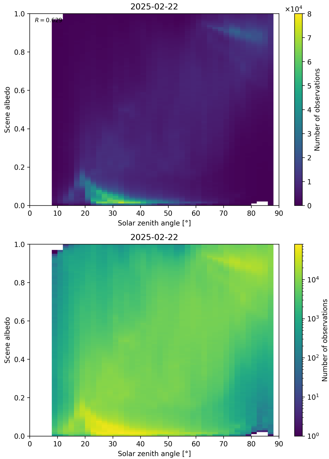
Figure 116: Scatter density plot of “Solar zenith angle” against “Scene albedo” for 2025-02-21 to 2025-02-23.
