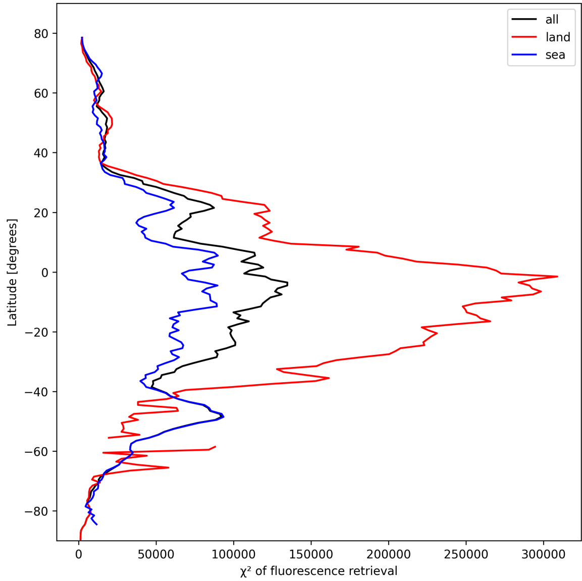
Figure 25: Zonal average of “ \chi^2 of fluorescence retrieval” for 2025-02-21 to 2025-02-23.
