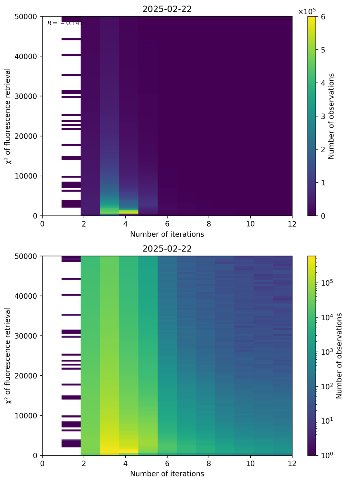
Figure 97: Scatter density plot of “Number of iterations” against “ \chi^2 of fluorescence retrieval” for 2025-02-21 to 2025-02-23.
