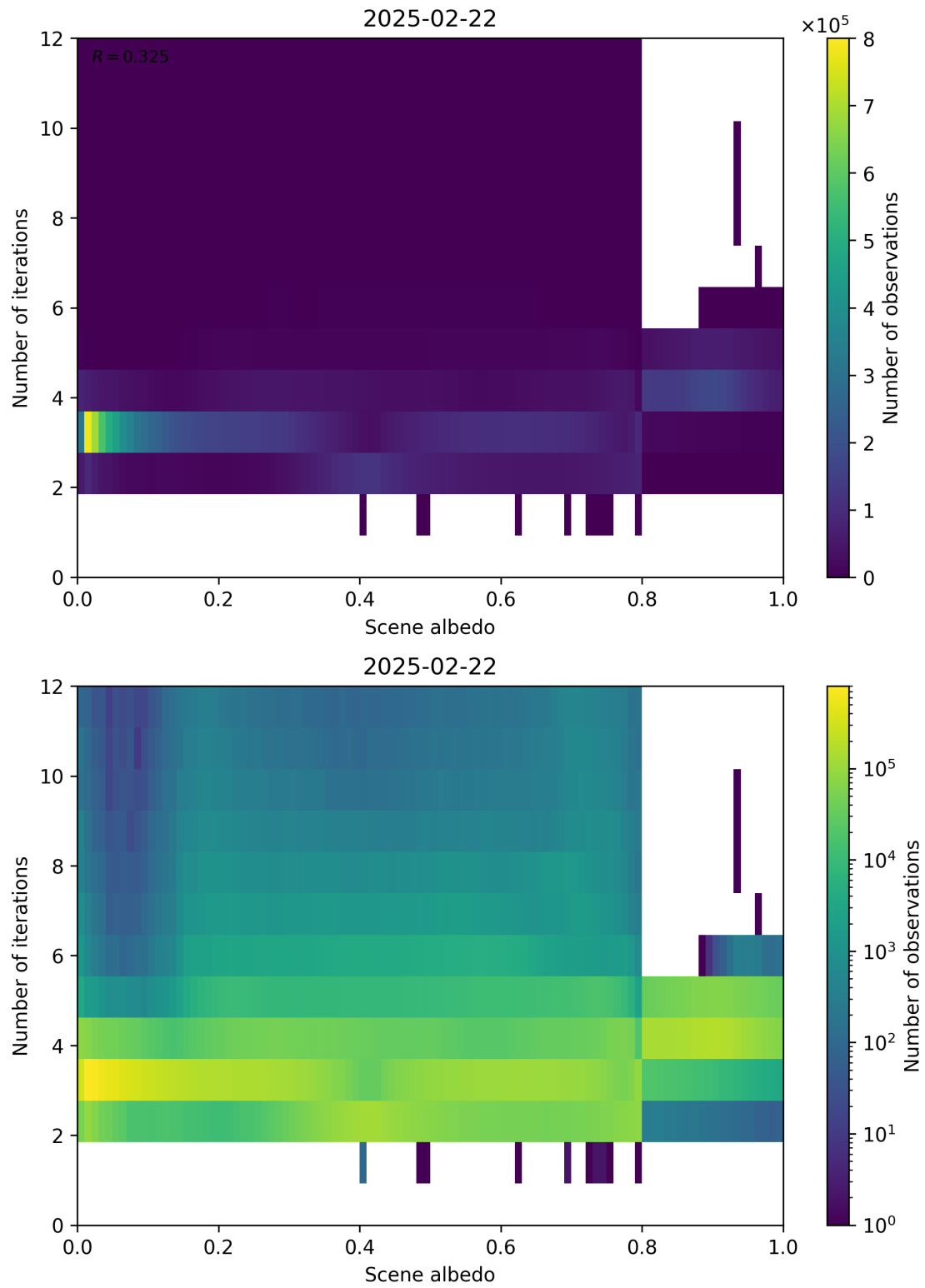
Figure 105: Scatter density plot of “Scene albedo” against “Number of iterations” for 2025-02-21 to 2025-02-23.
