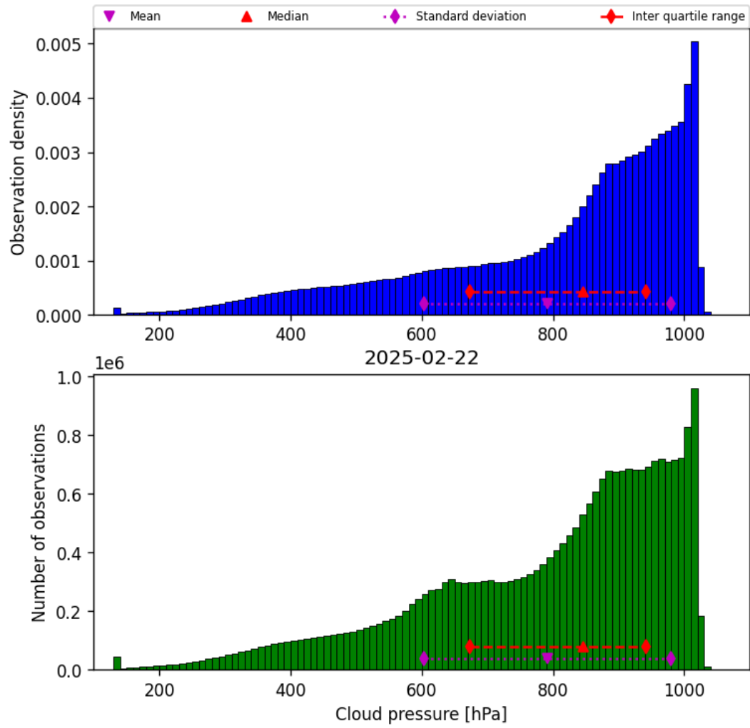
Figure 30: Histogram of “Cloud pressure” for 2025-02-21 to 2025-02-23
