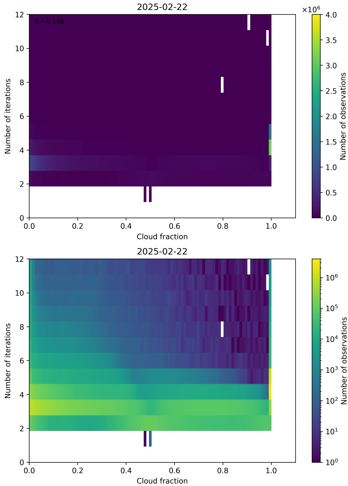
Figure 73: Scatter density plot of “Cloud fraction” against “Number of iterations” for 2025-02-21 to 2025-02-23.
