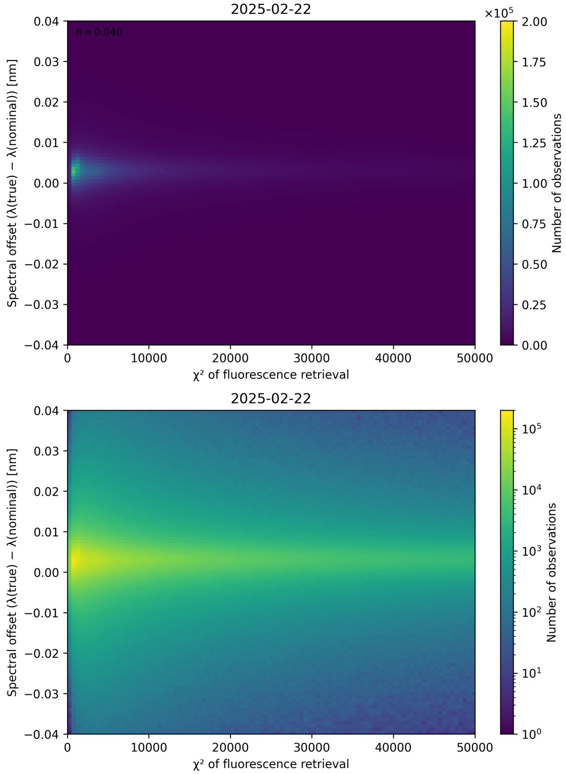
Figure 69: Scatter density plot of “ \chi^2 of fluorescence retrieval” against “Spectral offset ( \lambda_{\text{true}} - \lambda_{\text{nominal}} )” for 2025-02-21 to 2025-02-23.
