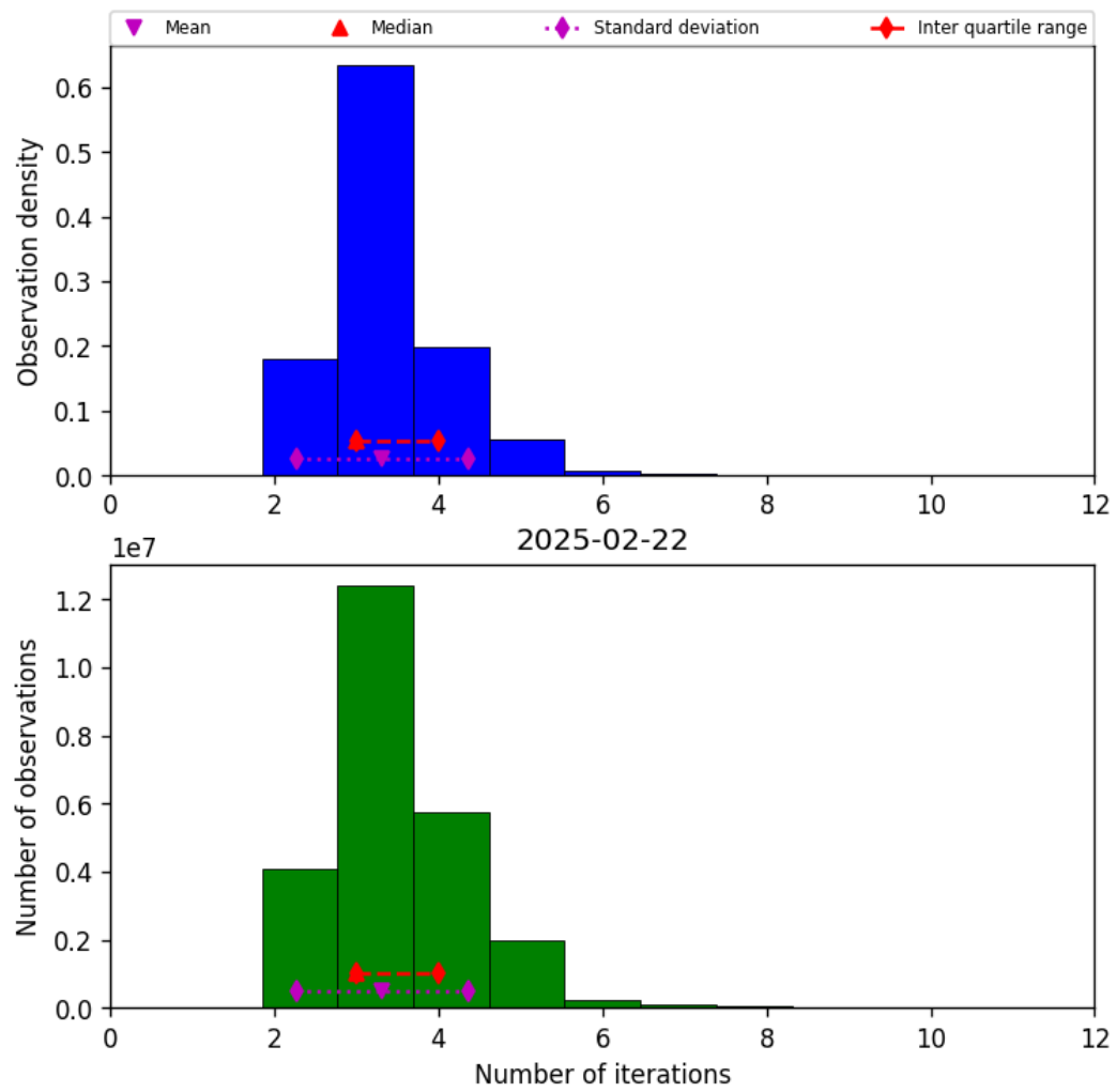
Figure 39: Histogram of “Number of iterations” for 2025-02-21 to 2025-02-23
