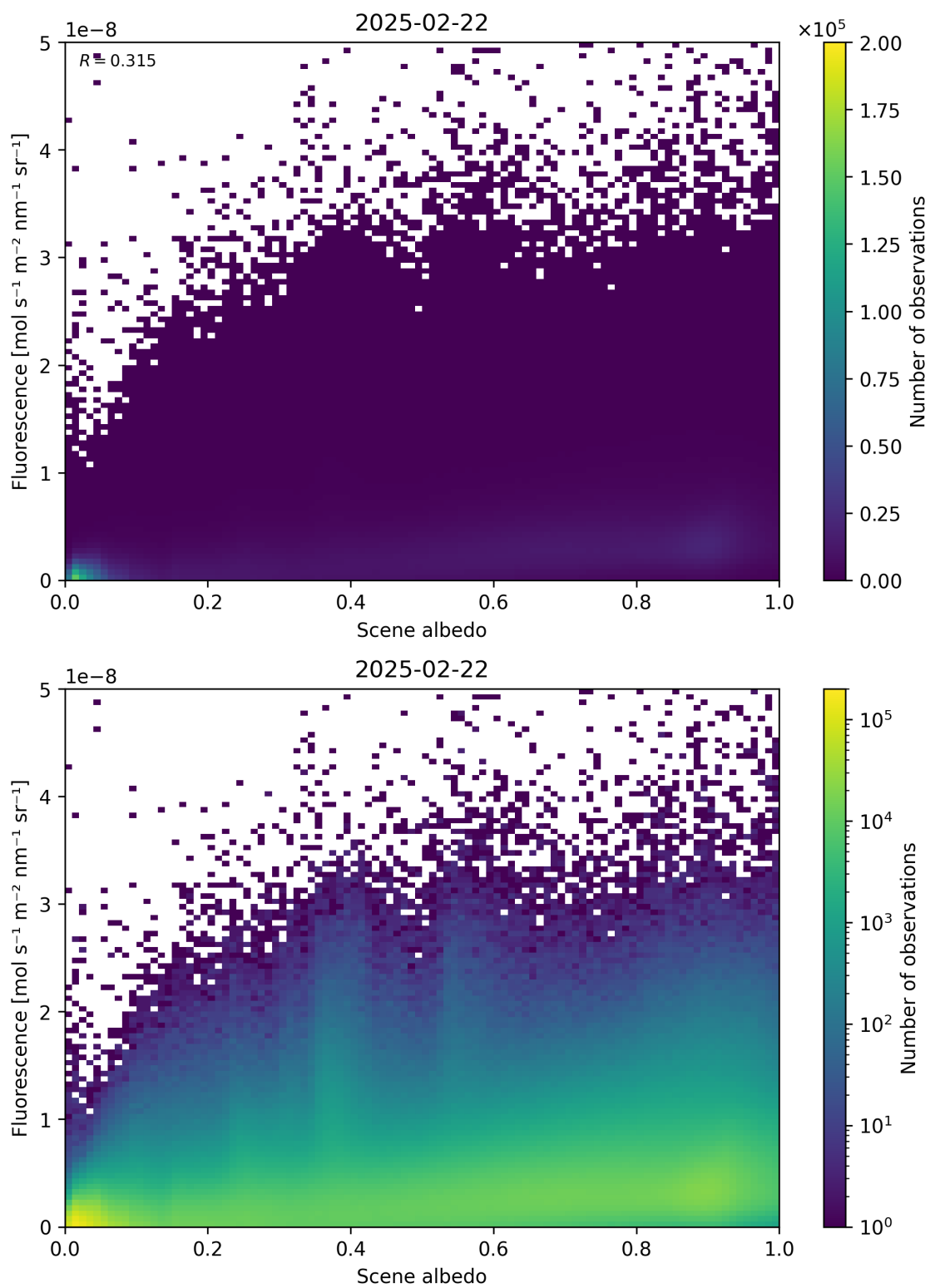
Figure 104: Scatter density plot of “Scene albedo” against “Fluorescence” for 2025-02-21 to 2025-02-23.
