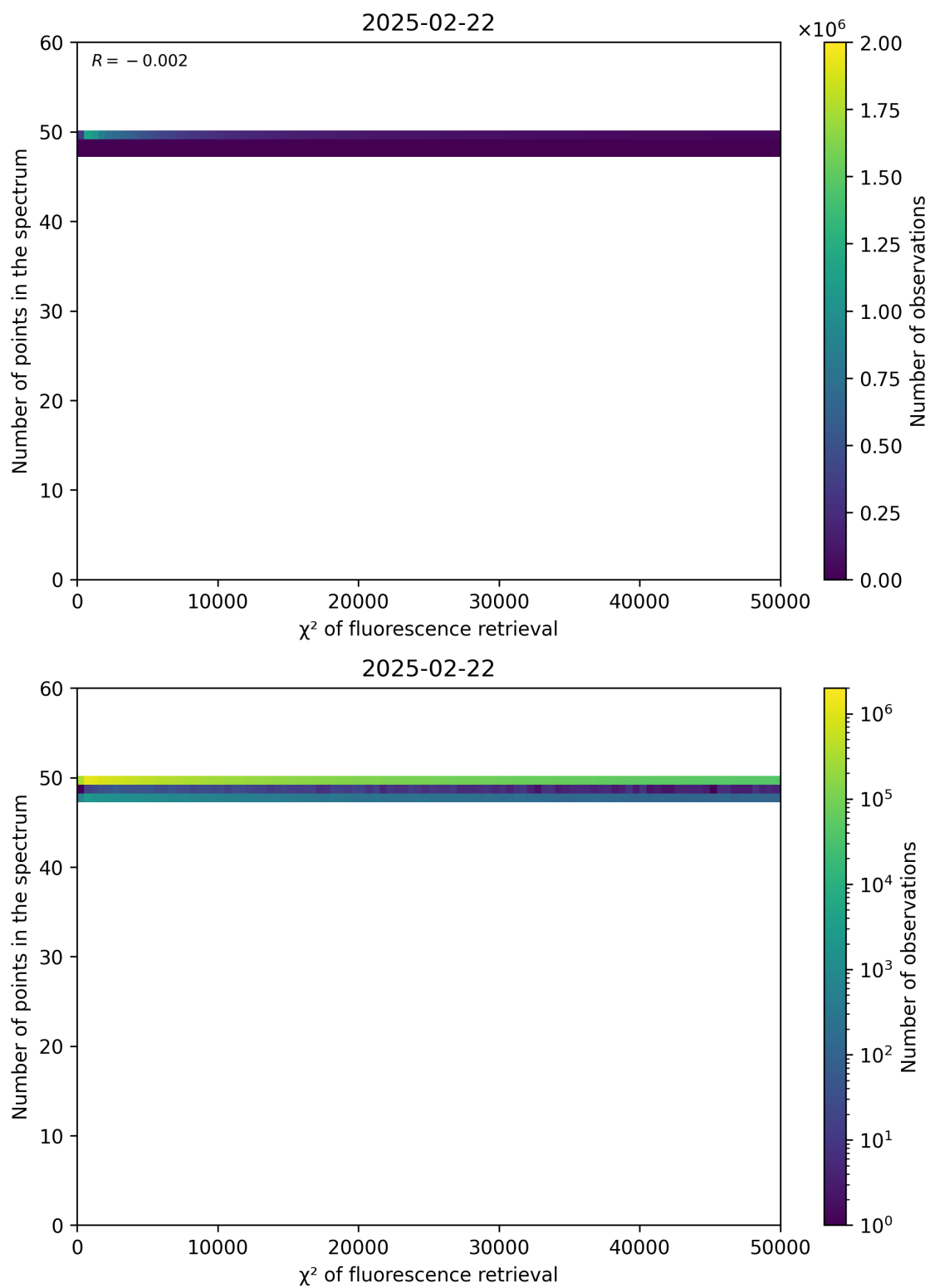
Figure 68: Scatter density plot of “ \chi^2 of fluorescence retrieval” against “Number of points in the spectrum” for 2025-02-21 to 2025-02-23.
