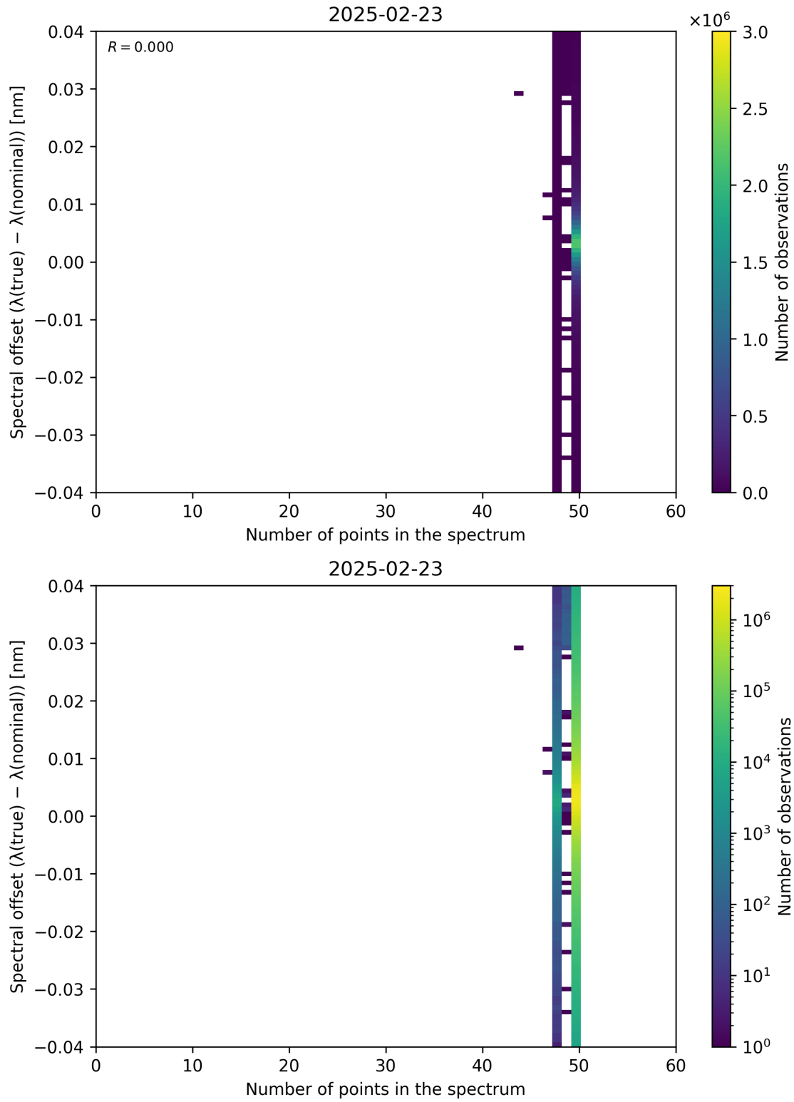
Figure 101: Scatter density plot of “Number of points in the spectrum” against “Spectral offset ( \lambda_{\text{true}} - \lambda_{\text{nominal}} )” for 2025-02-22 to 2025-02-24.
