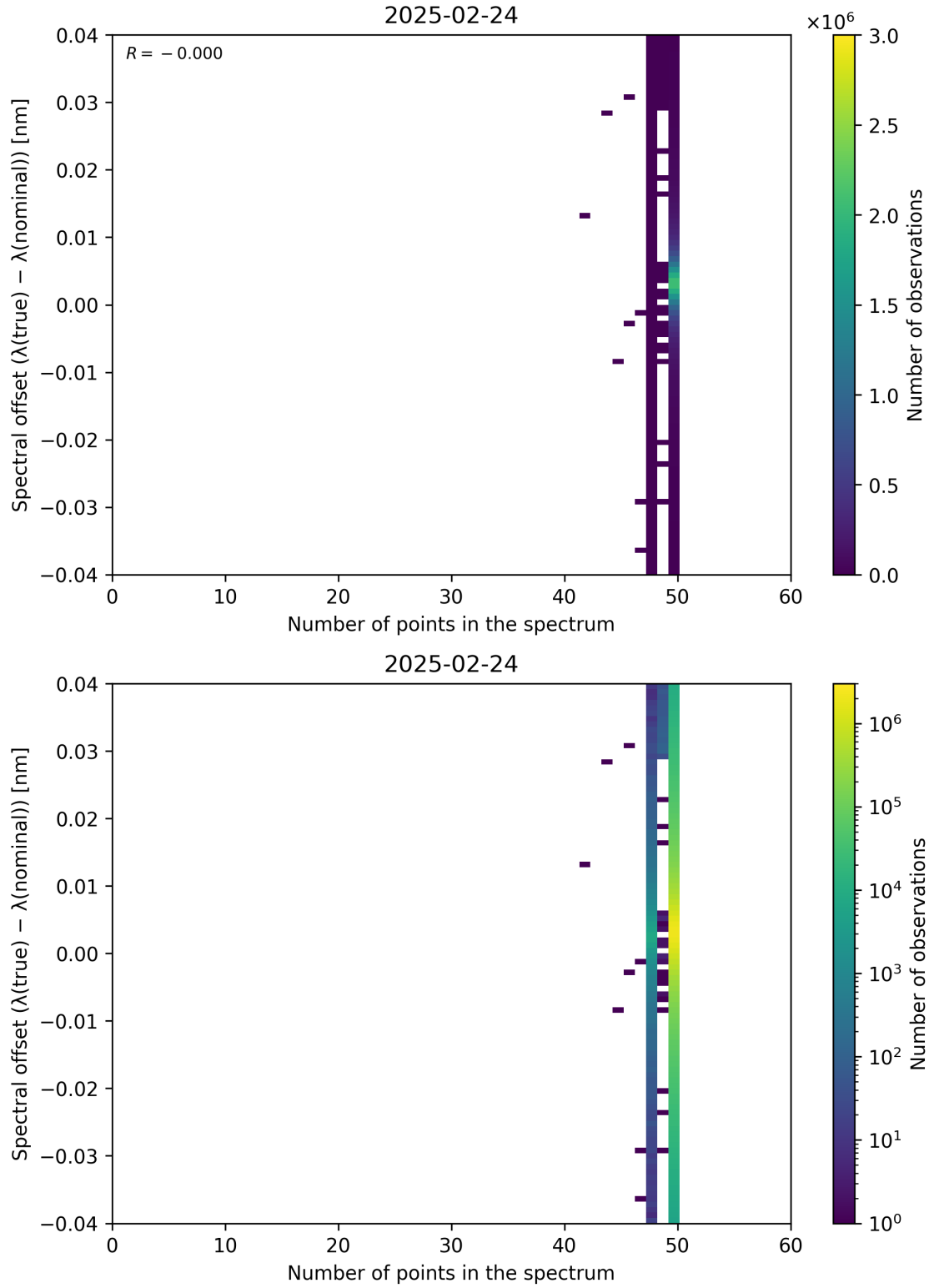
Figure 101: Scatter density plot of “Number of points in the spectrum” against “Spectral offset ( \lambda_{\text{true}} - \lambda_{\text{nominal}} )” for 2025-02-24 to 2025-02-25.
