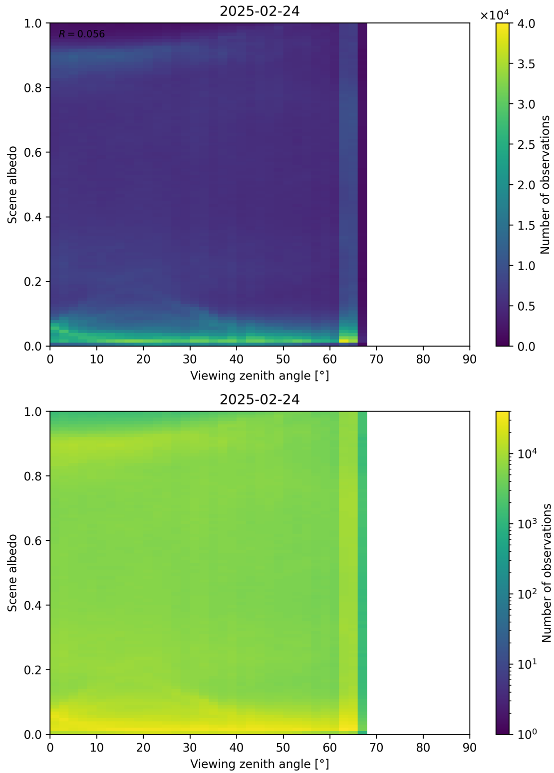
Figure 126: Scatter density plot of “Viewing zenith angle” against “Scene albedo” for 2025-02-24 to 2025-02-25.
