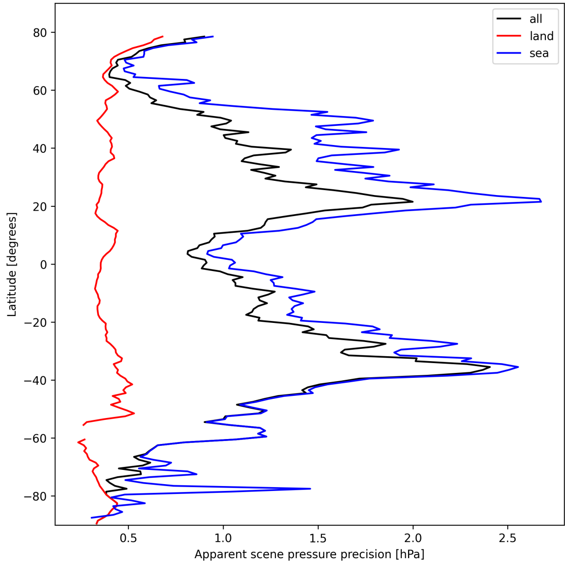
Figure 20: Zonal average of “Apparent scene pressure precision” for 2025-02-24 to 2025-02-25.
