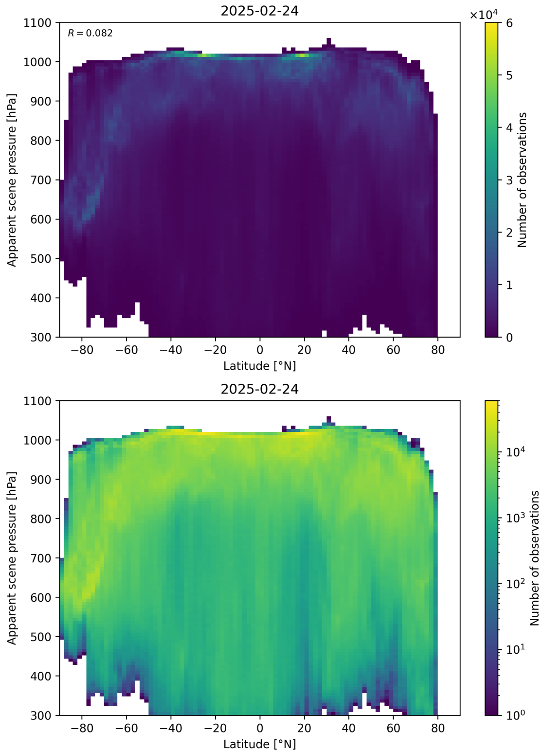
Figure 88: Scatter density plot of “Latitude” against “Apparent scene pressure” for 2025-02-24 to 2025-02-25.
