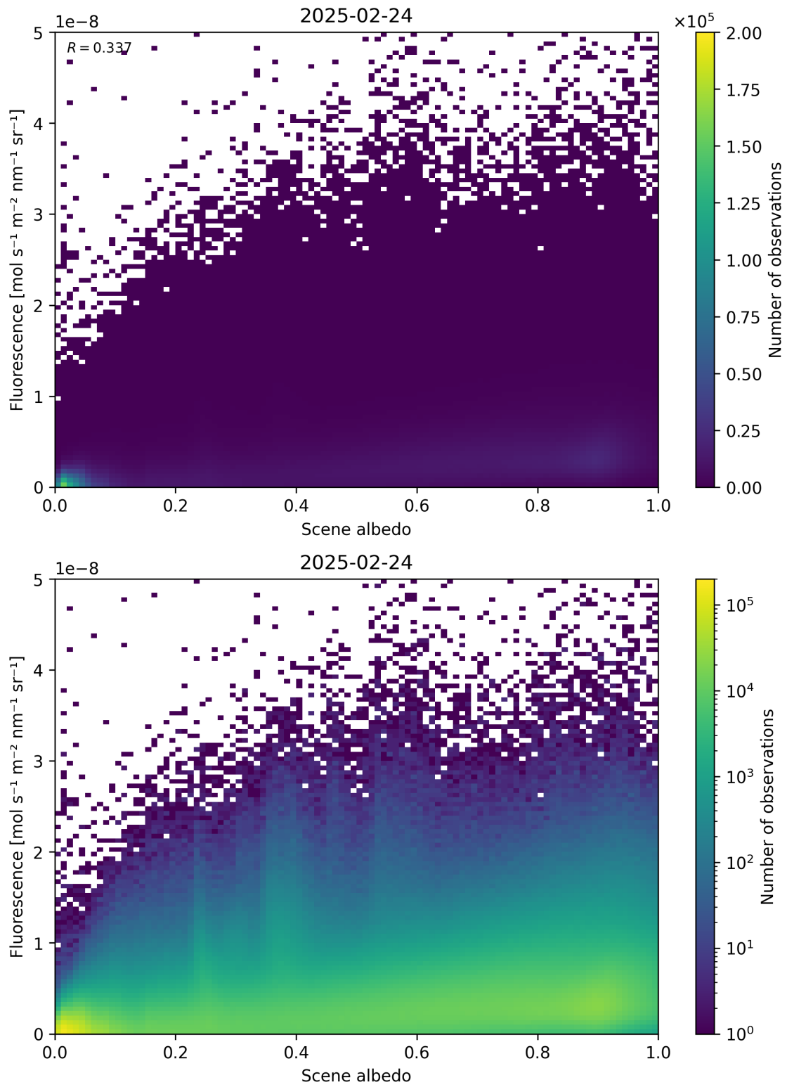
Figure 104: Scatter density plot of “Scene albedo” against “Fluorescence” for 2025-02-24 to 2025-02-25.
