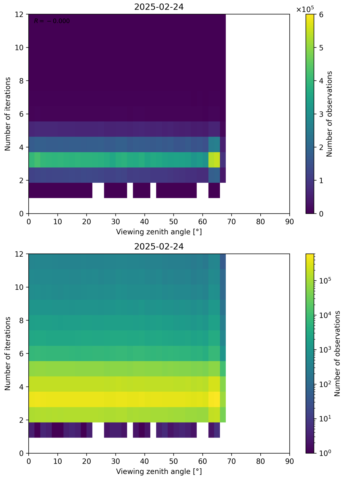
Figure 124: Scatter density plot of “Viewing zenith angle” against “Number of iterations” for 2025-02-24 to 2025-02-25.
