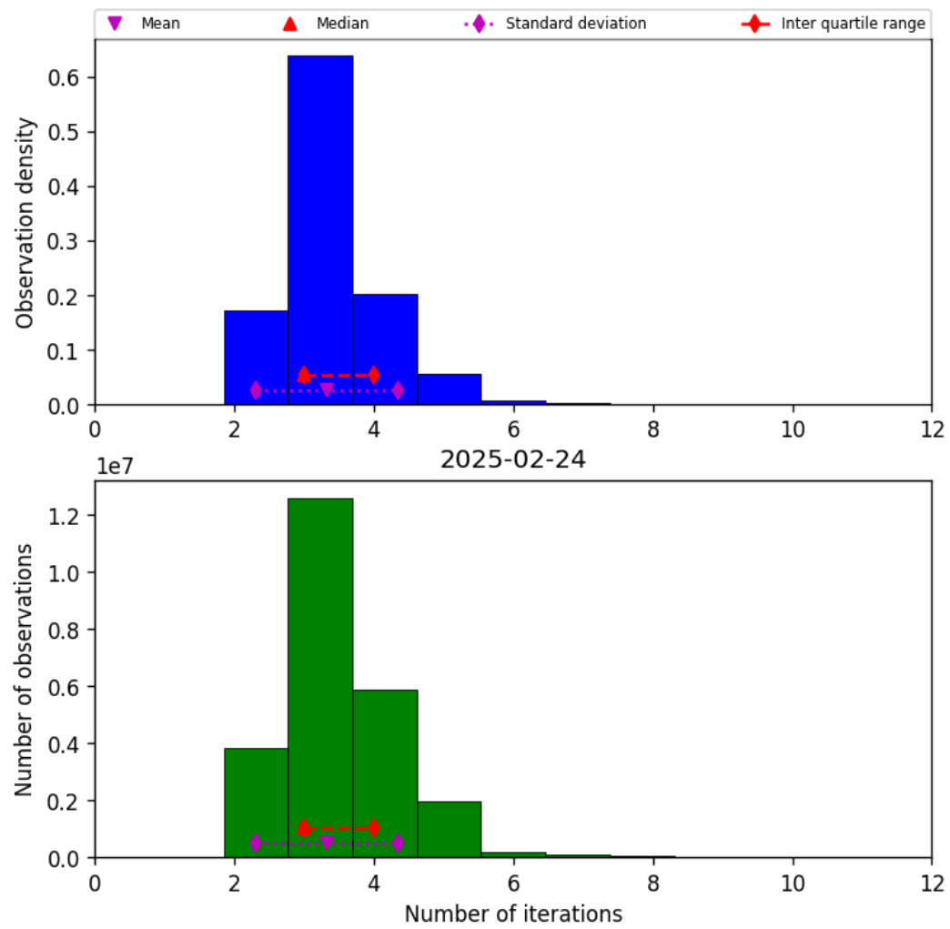
Figure 39: Histogram of “Number of iterations” for 2025-02-24 to 2025-02-25
