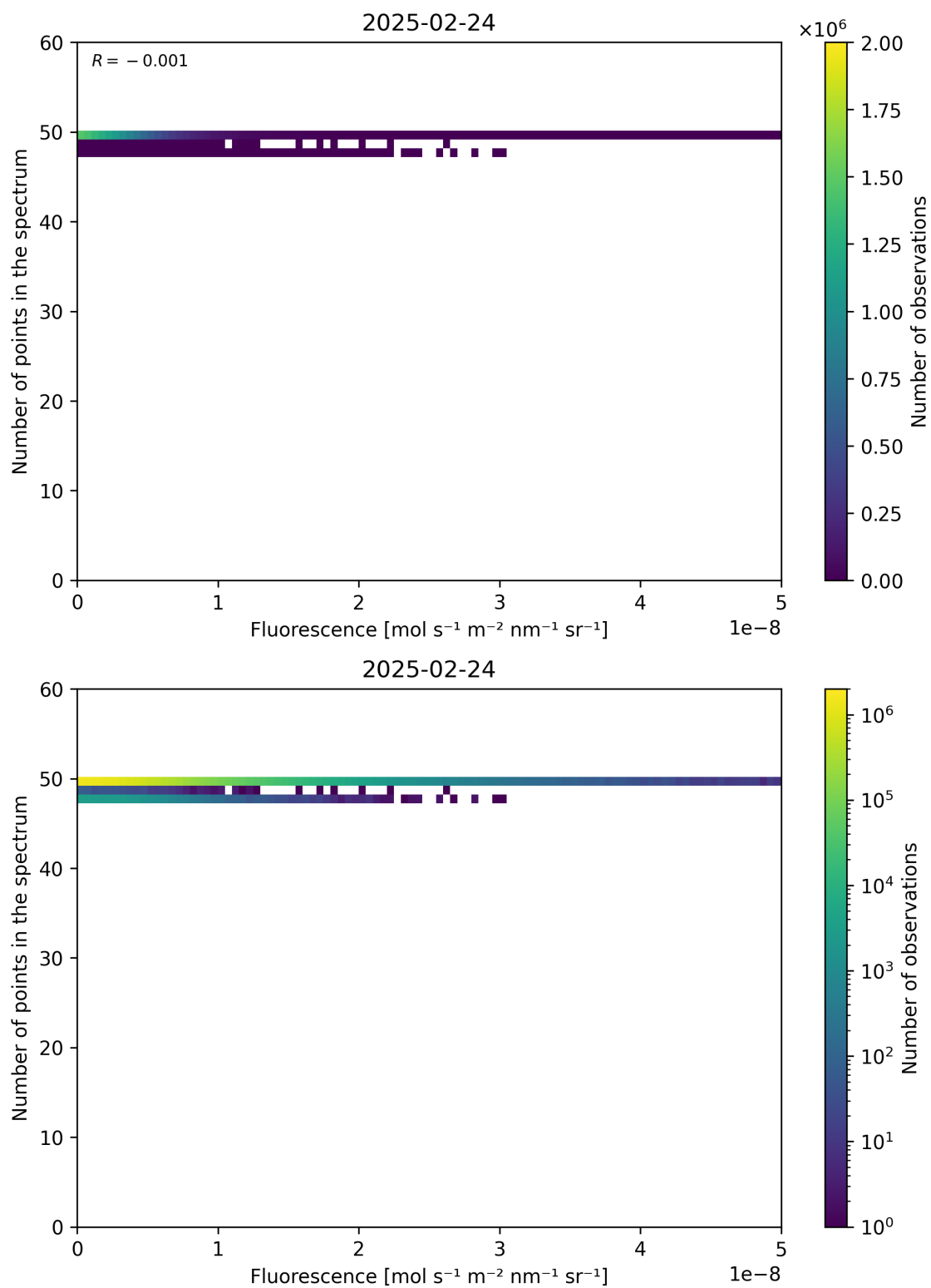
Figure 86: Scatter density plot of “Fluorescence” against “Number of points in the spectrum” for 2025-02-24 to 2025-02-25.
