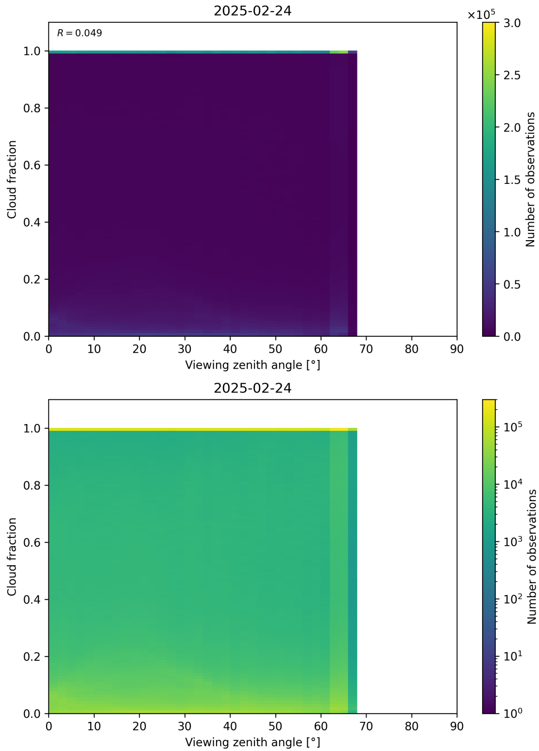
Figure 120: Scatter density plot of “Viewing zenith angle” against “Cloud fraction” for 2025-02-24 to 2025-02-25.
