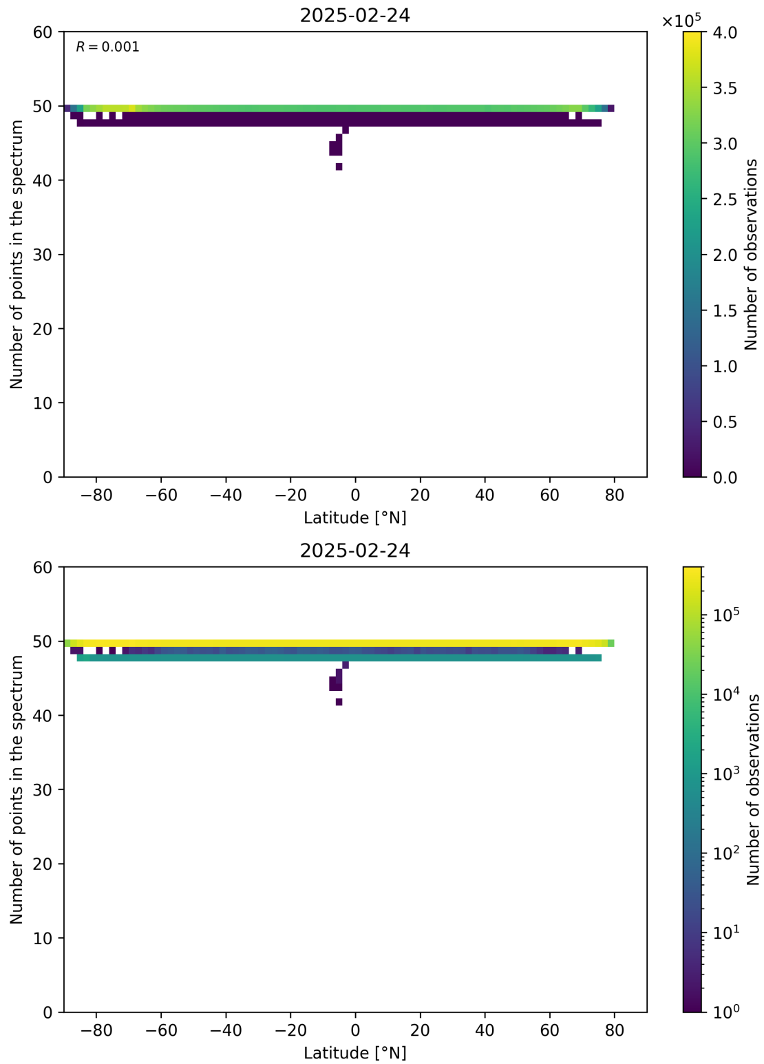
Figure 94: Scatter density plot of “Latitude” against “Number of points in the spectrum” for 2025-02-24 to 2025-02-25.
