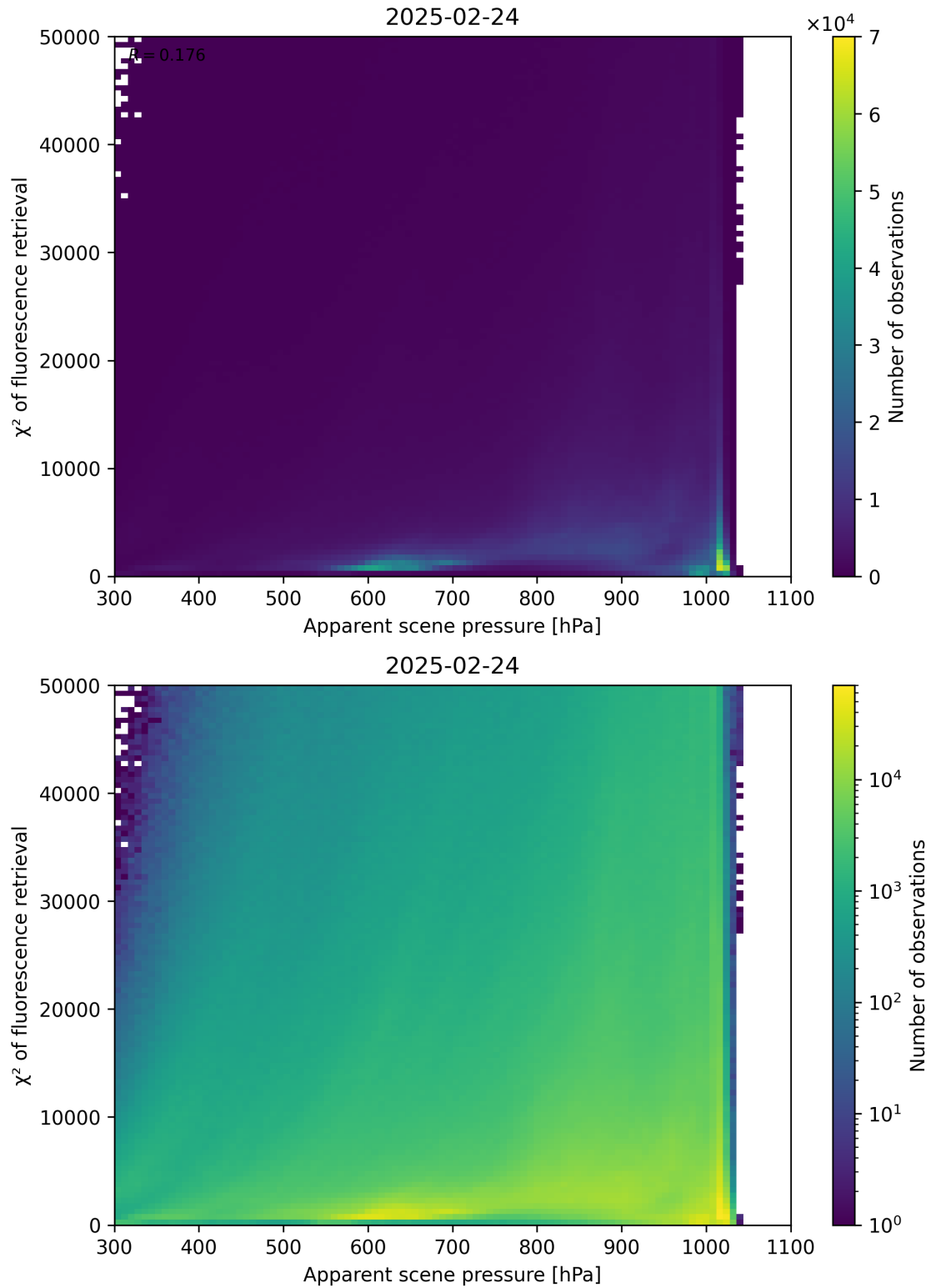
Figure 63: Scatter density plot of “Apparent scene pressure” against “ \chi^2 of fluorescence retrieval” for 2025-02-24 to 2025-02-25.
