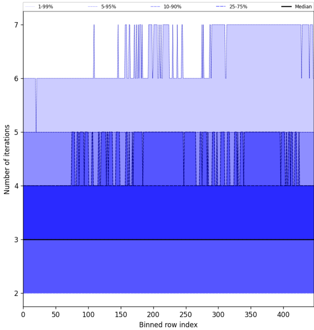
Figure 56: Along track statistics of “Number of iterations” for 2025-02-24 to 2025-02-25
