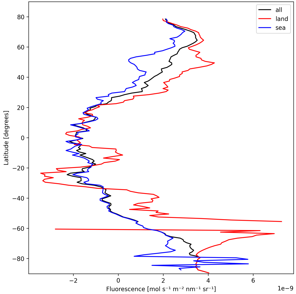
Figure 23: Zonal average of “Fluorescence” for 2025-02-24 to 2025-02-25.
