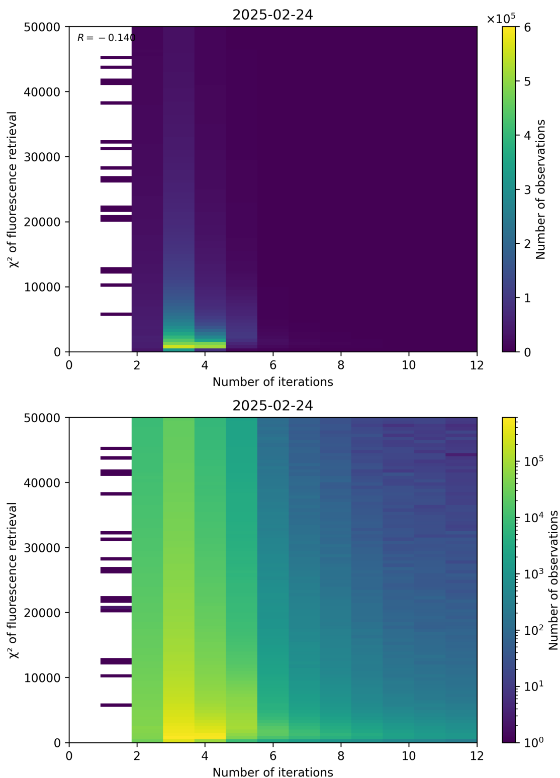
Figure 97: Scatter density plot of “Number of iterations” against “ \chi^2 of fluorescence retrieval” for 2025-02-24 to 2025-02-25.
