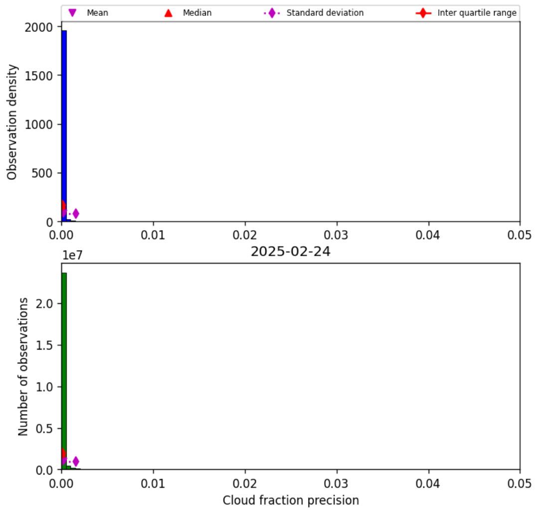
Figure 33: Histogram of “Cloud fraction precision” for 2025-02-24 to 2025-02-25
