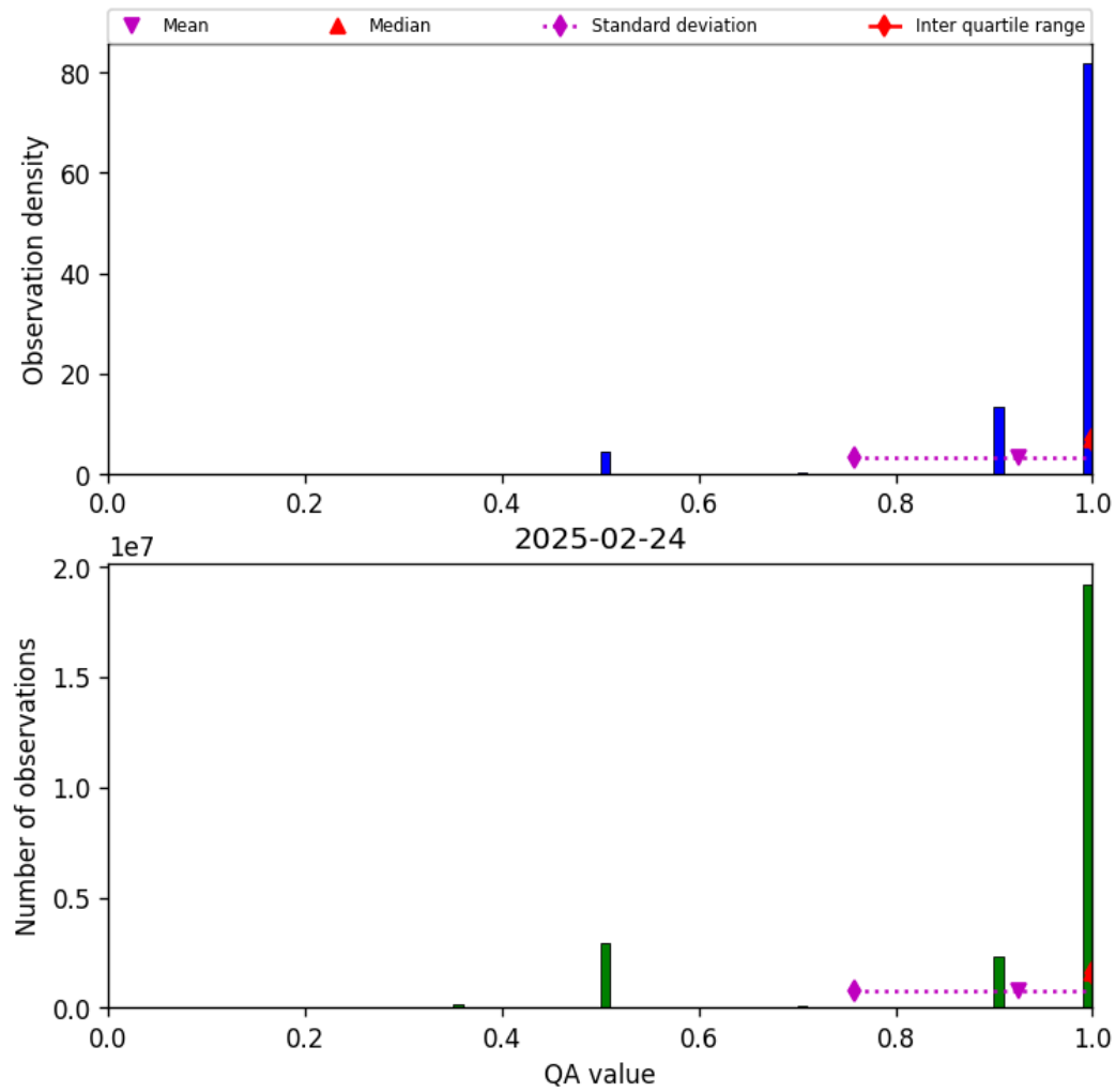
Figure 29: Histogram of “QA value” for 2025-02-24 to 2025-02-25
