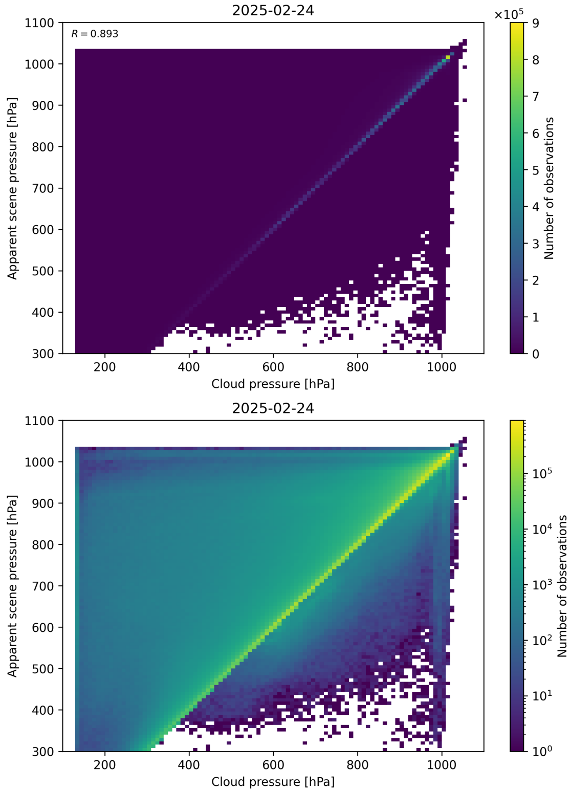
Figure 77: Scatter density plot of “Cloud pressure” against “Apparent scene pressure” for 2025-02-24 to 2025-02-25.
