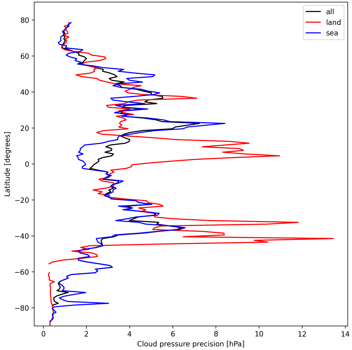
Figure 14: Zonal average of “Cloud pressure precision” for 2025-02-24 to 2025-02-25.
