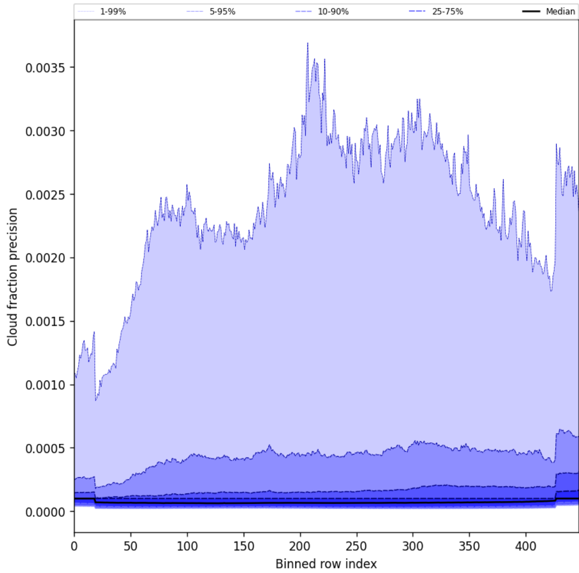
Figure 50: Along track statistics of “Cloud fraction precision” for 2025-02-24 to 2025-02-25
