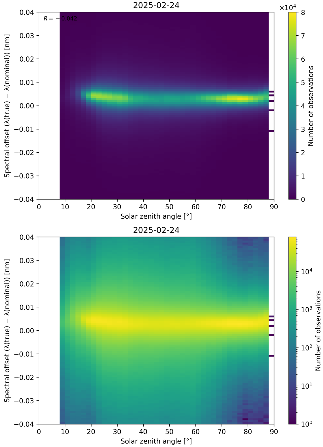
Figure 117: Scatter density plot of “Solar zenith angle” against “Spectral offset ( \lambda_{\text{true}} - \lambda_{\text{nominal}} )” for 2025-02-24 to 2025-02-25.
