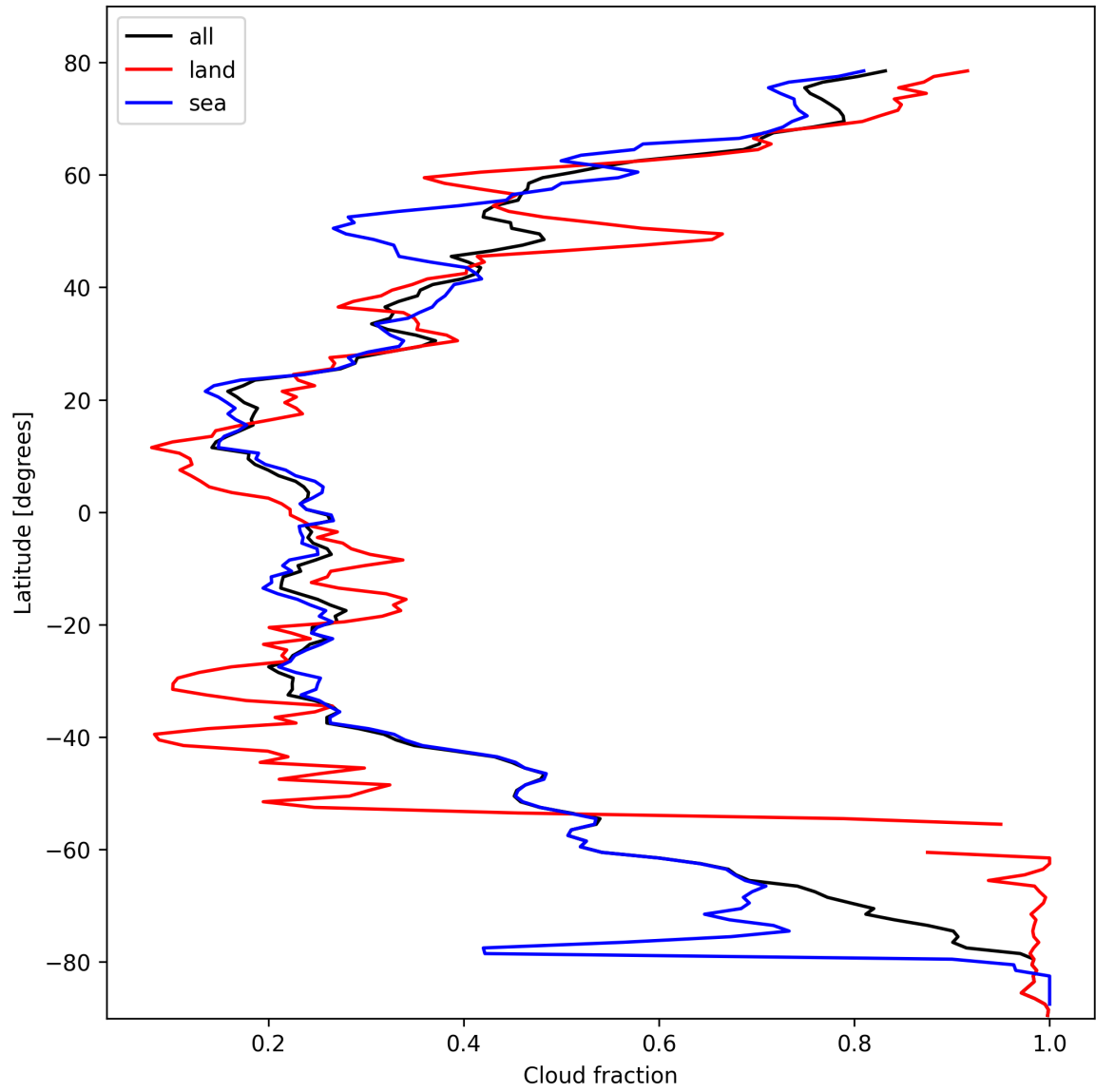
Figure 15: Zonal average of “Cloud fraction” for 2025-02-24 to 2025-02-25.
