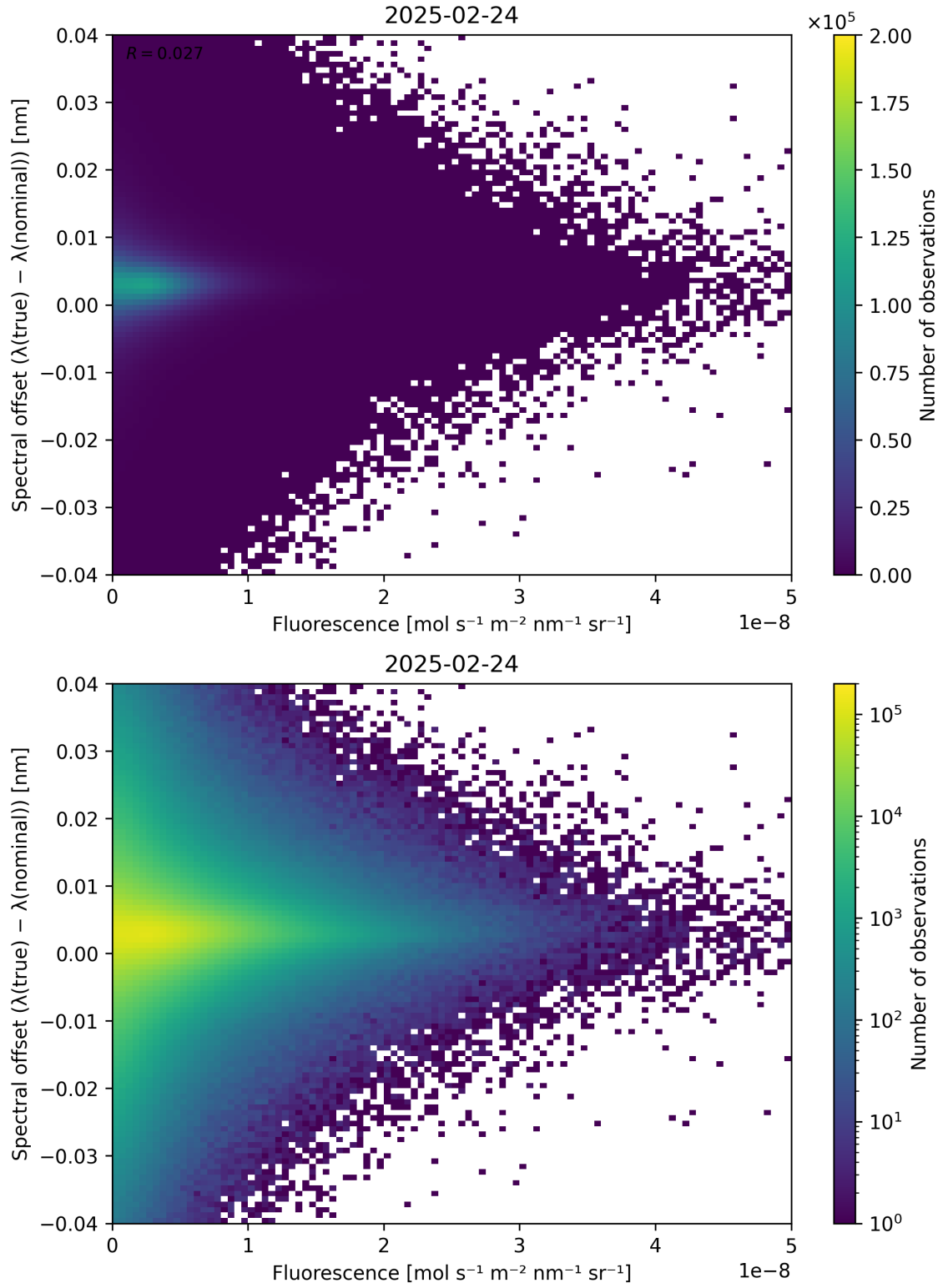
Figure 87: Scatter density plot of “Fluorescence” against “Spectral offset ( \lambda_{\text{true}} - \lambda_{\text{nominal}} )” for 2025-02-24 to 2025-02-25.
