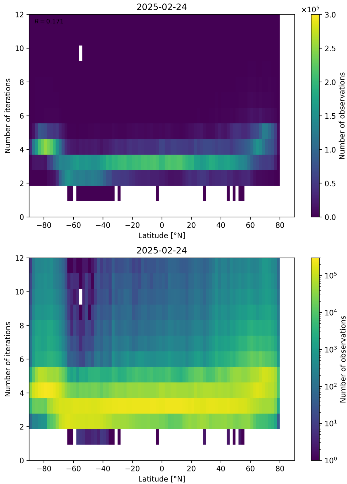
Figure 93: Scatter density plot of “Latitude” against “Number of iterations” for 2025-02-24 to 2025-02-25.
