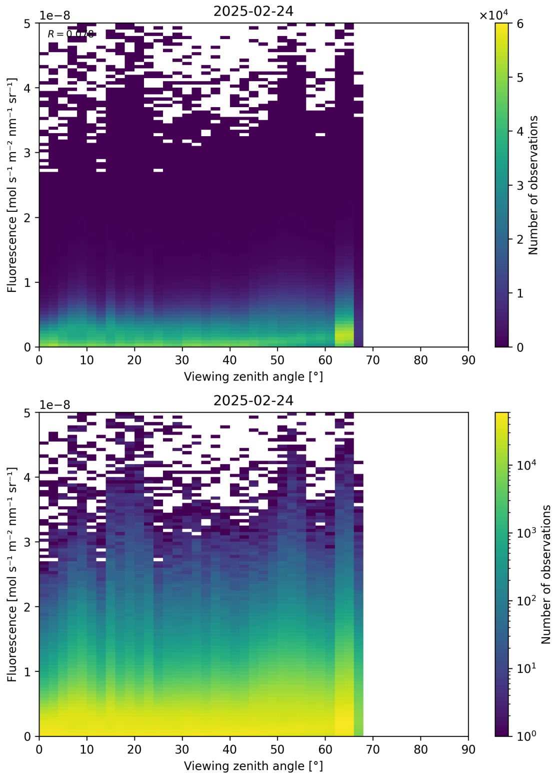
Figure 122: Scatter density plot of “Viewing zenith angle” against “Fluorescence” for 2025-02-24 to 2025-02-25.
