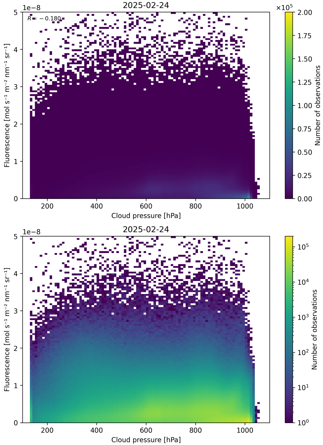
Figure 80: Scatter density plot of “Cloud pressure” against “Fluorescence” for 2025-02-24 to 2025-02-25.
