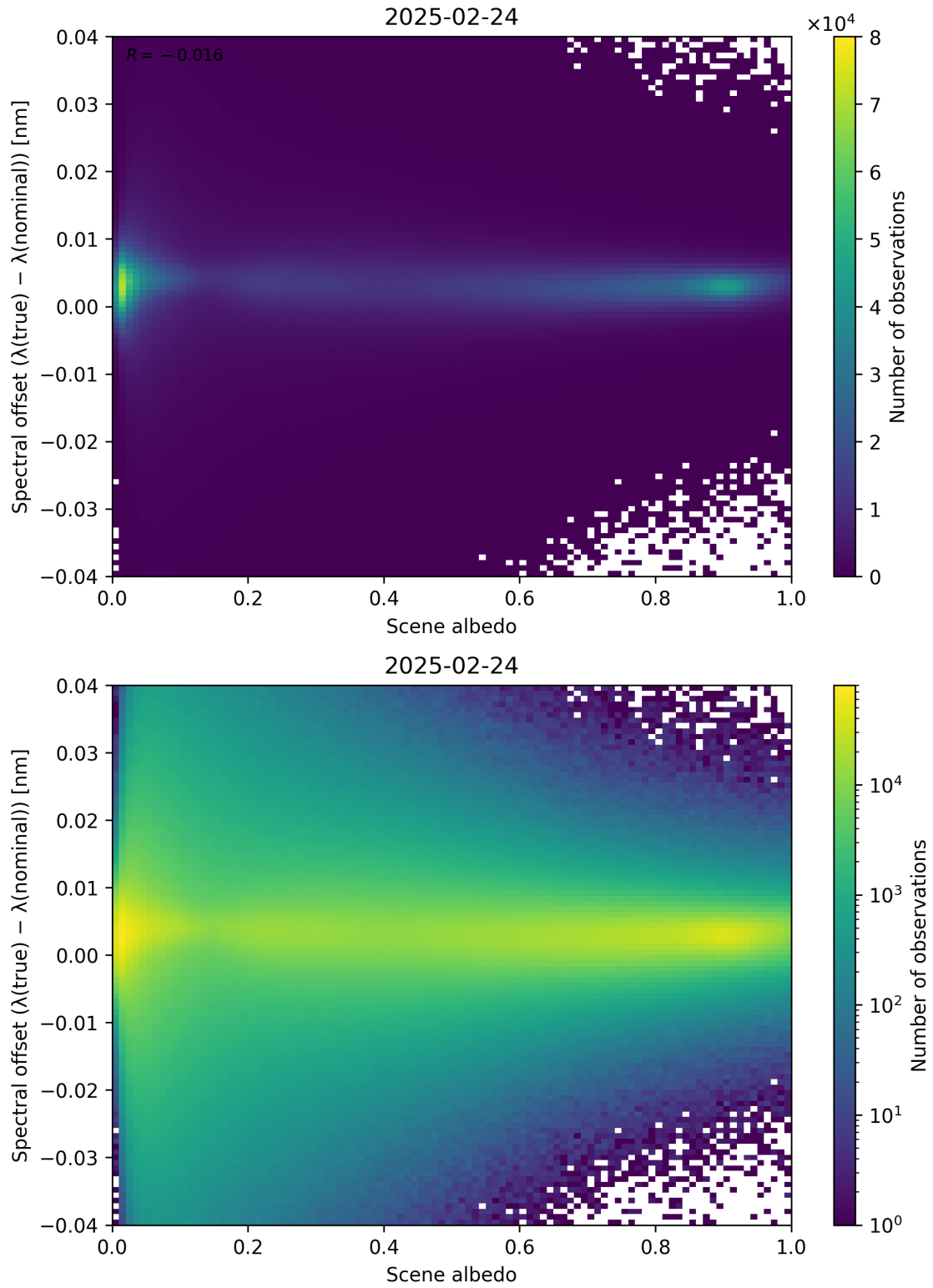
Figure 107: Scatter density plot of “Scene albedo” against “Spectral offset ( \lambda_{\text{true}} - \lambda_{\text{nominal}} )” for 2025-02-24 to 2025-02-25.
