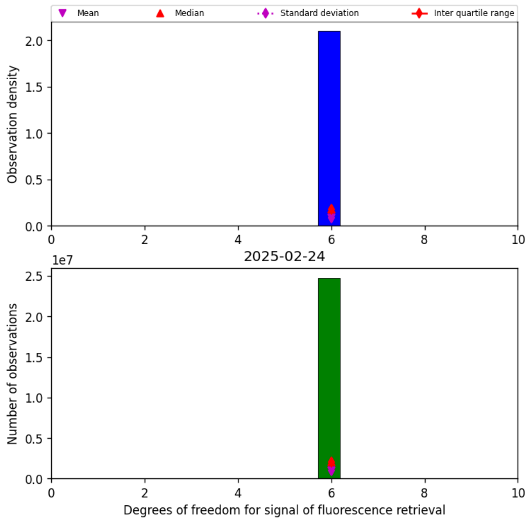
Figure 43: Histogram of “Degrees of freedom for signal of fluorescence retrieval” for 2025-02-24 to 2025-02-25
