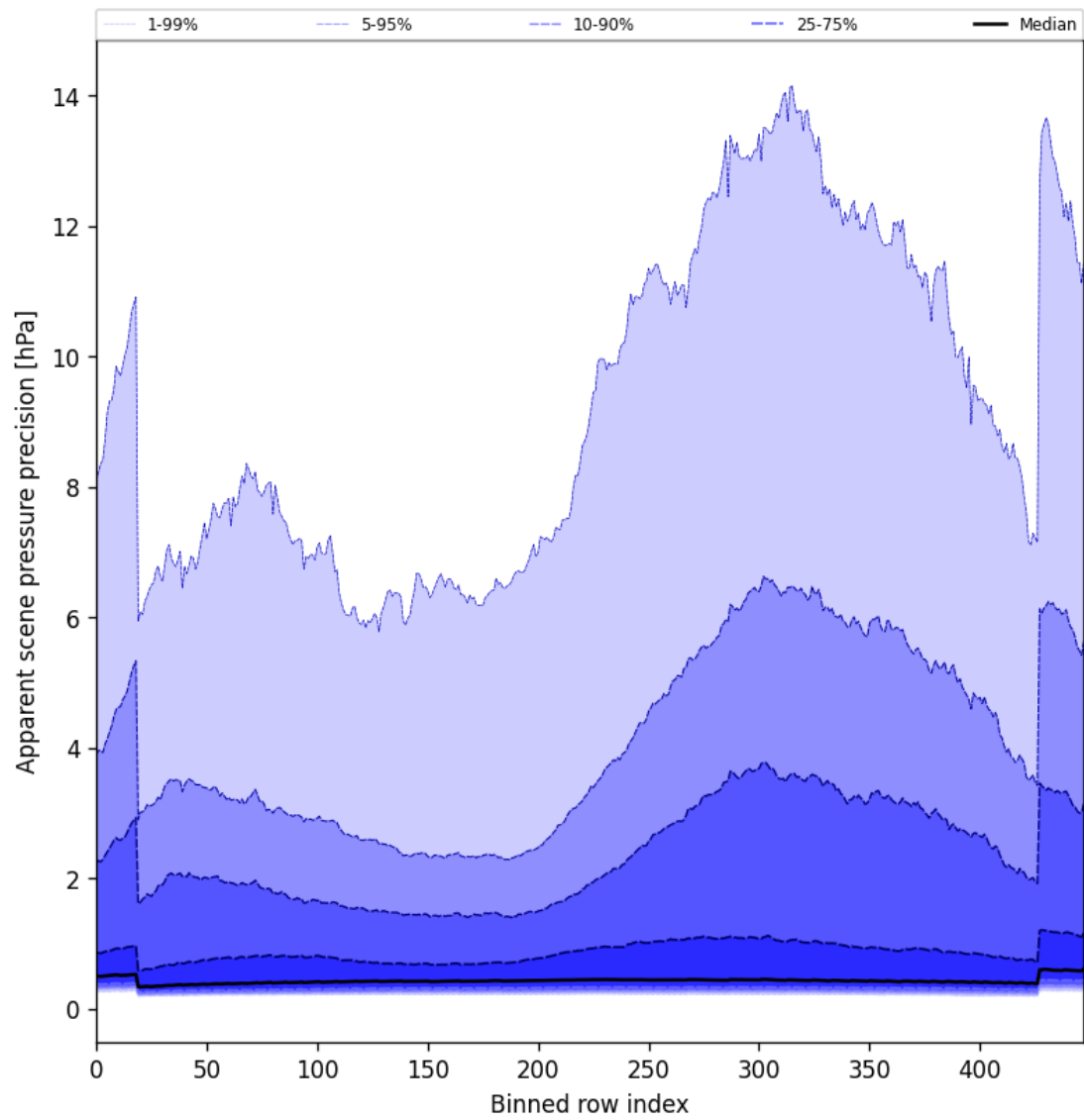
Figure 54: Along track statistics of “Apparent scene pressure precision” for 2025-02-24 to 2025-02-25
