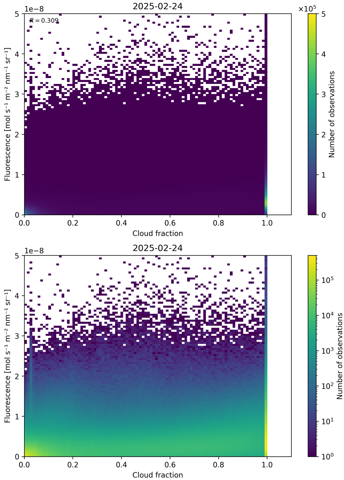
Figure 72: Scatter density plot of “Cloud fraction” against “Fluorescence” for 2025-02-24 to 2025-02-25.
