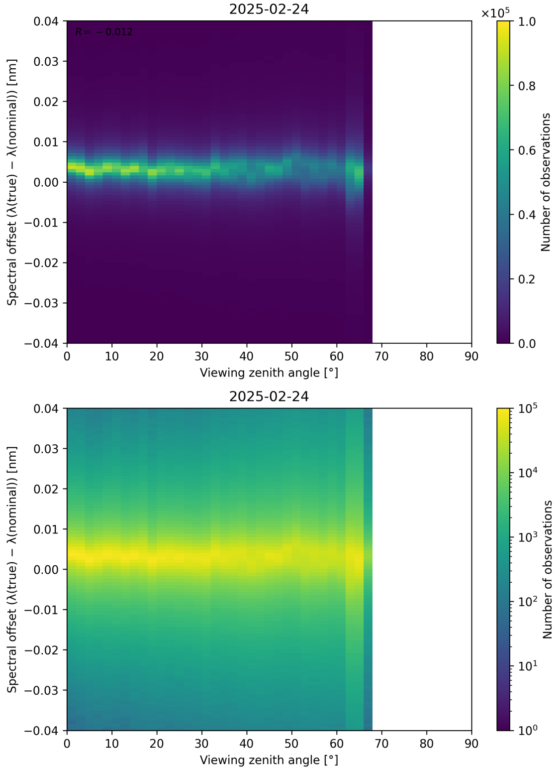
Figure 128: Scatter density plot of “Viewing zenith angle” against “Spectral offset ( \lambda_{\text{true}} - \lambda_{\text{nominal}} )” for 2025-02-24 to 2025-02-25.
