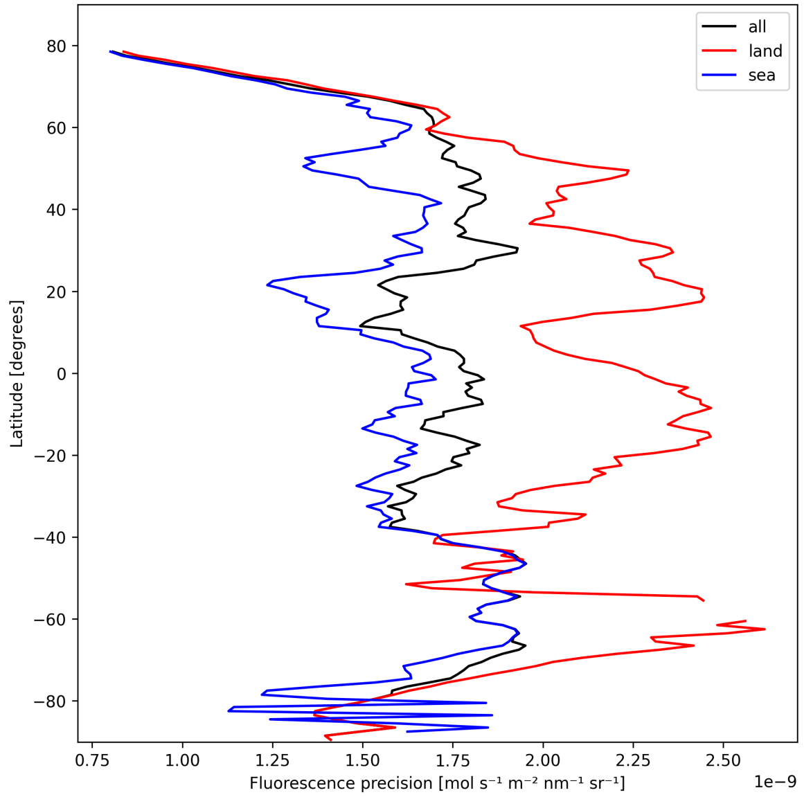
Figure 24: Zonal average of “Fluorescence precision” for 2025-02-24 to 2025-02-25.
