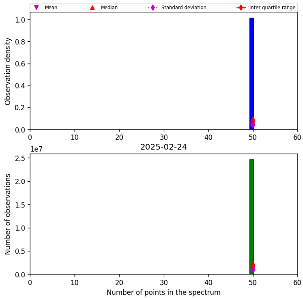
Figure 44: Histogram of “Number of points in the spectrum” for 2025-02-24 to 2025-02-25
