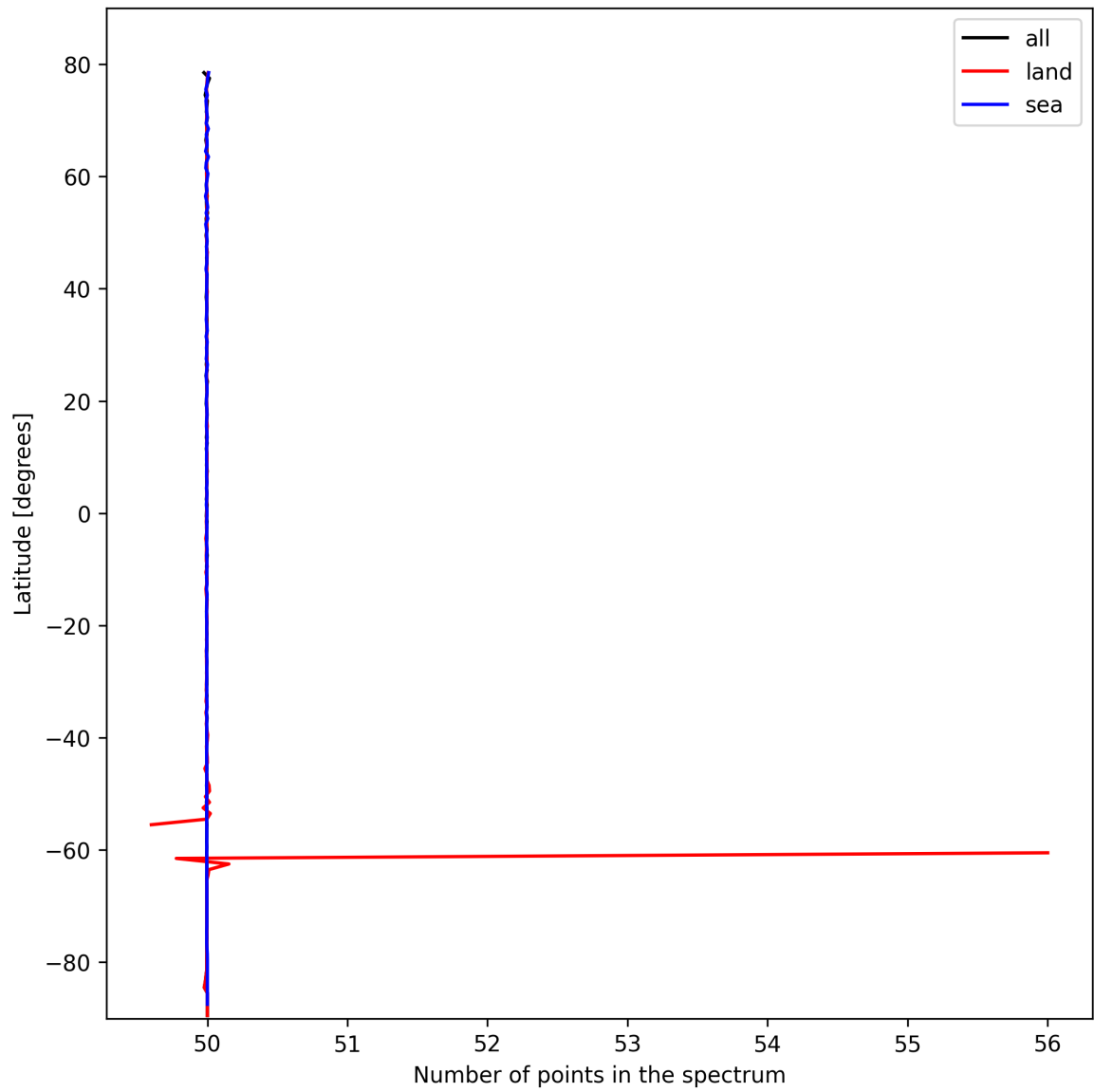
Figure 27: Zonal average of “Number of points in the spectrum” for 2025-02-24 to 2025-02-25.
