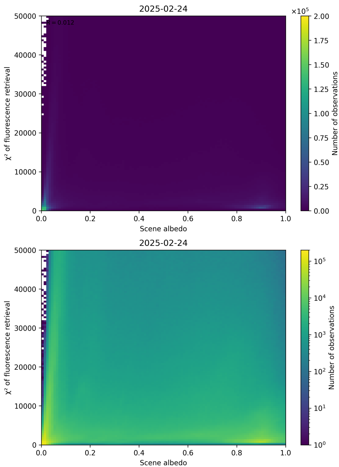
Figure 103: Scatter density plot of “Scene albedo” against “ \chi^2 of fluorescence retrieval” for 2025-02-24 to 2025-02-25.
