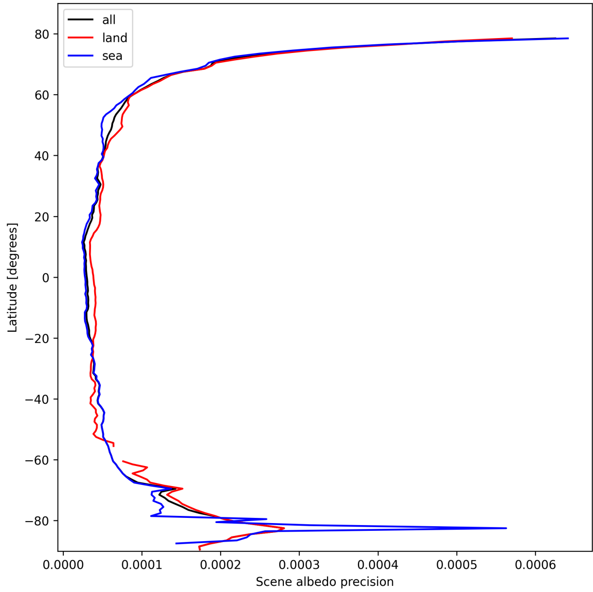
Figure 18: Zonal average of “Scene albedo precision” for 2025-02-24 to 2025-02-25.
