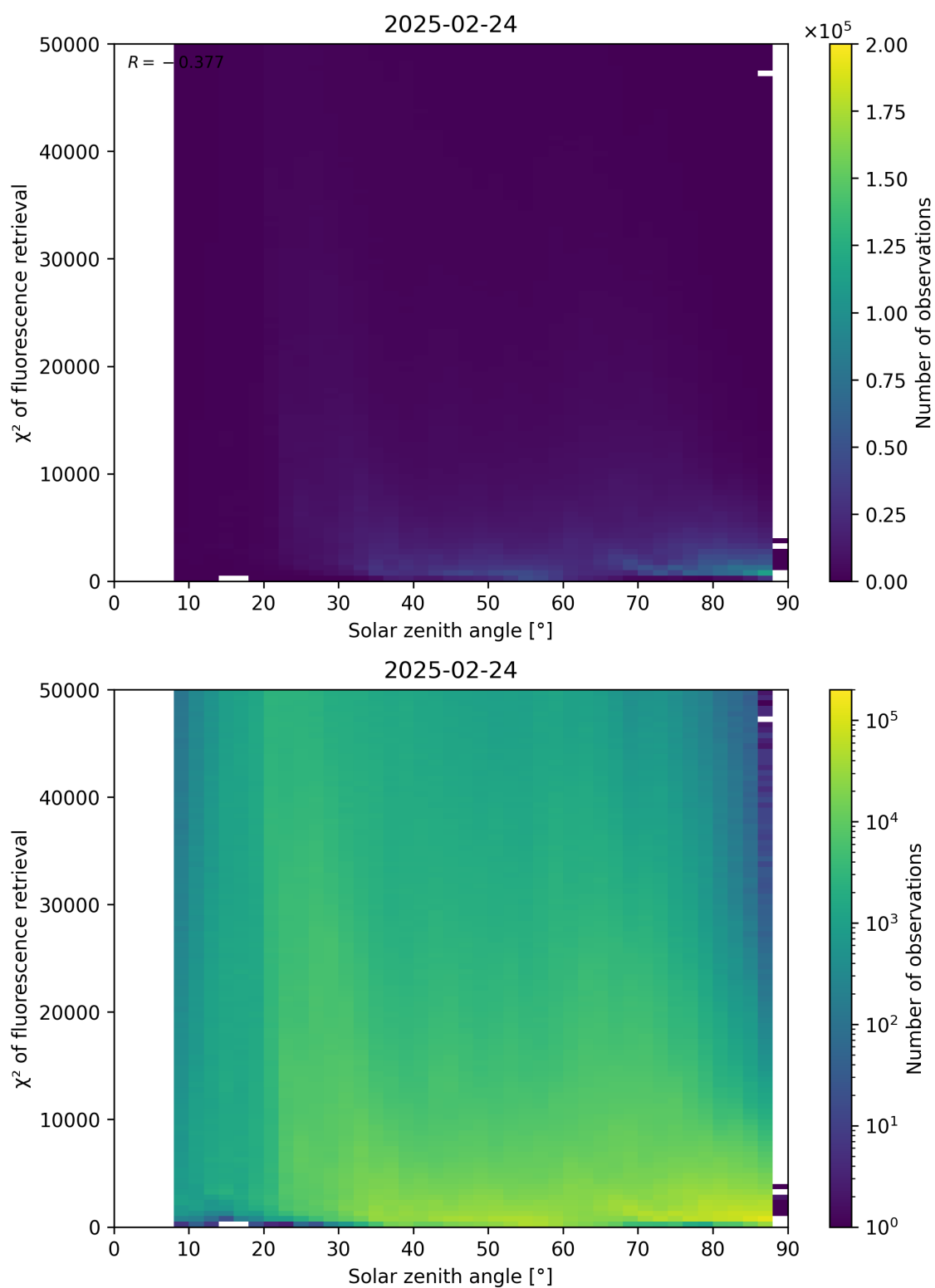
Figure 109: Scatter density plot of “Solar zenith angle” against “ \chi^2 of fluorescence retrieval” for 2025-02-24 to 2025-02-25.
