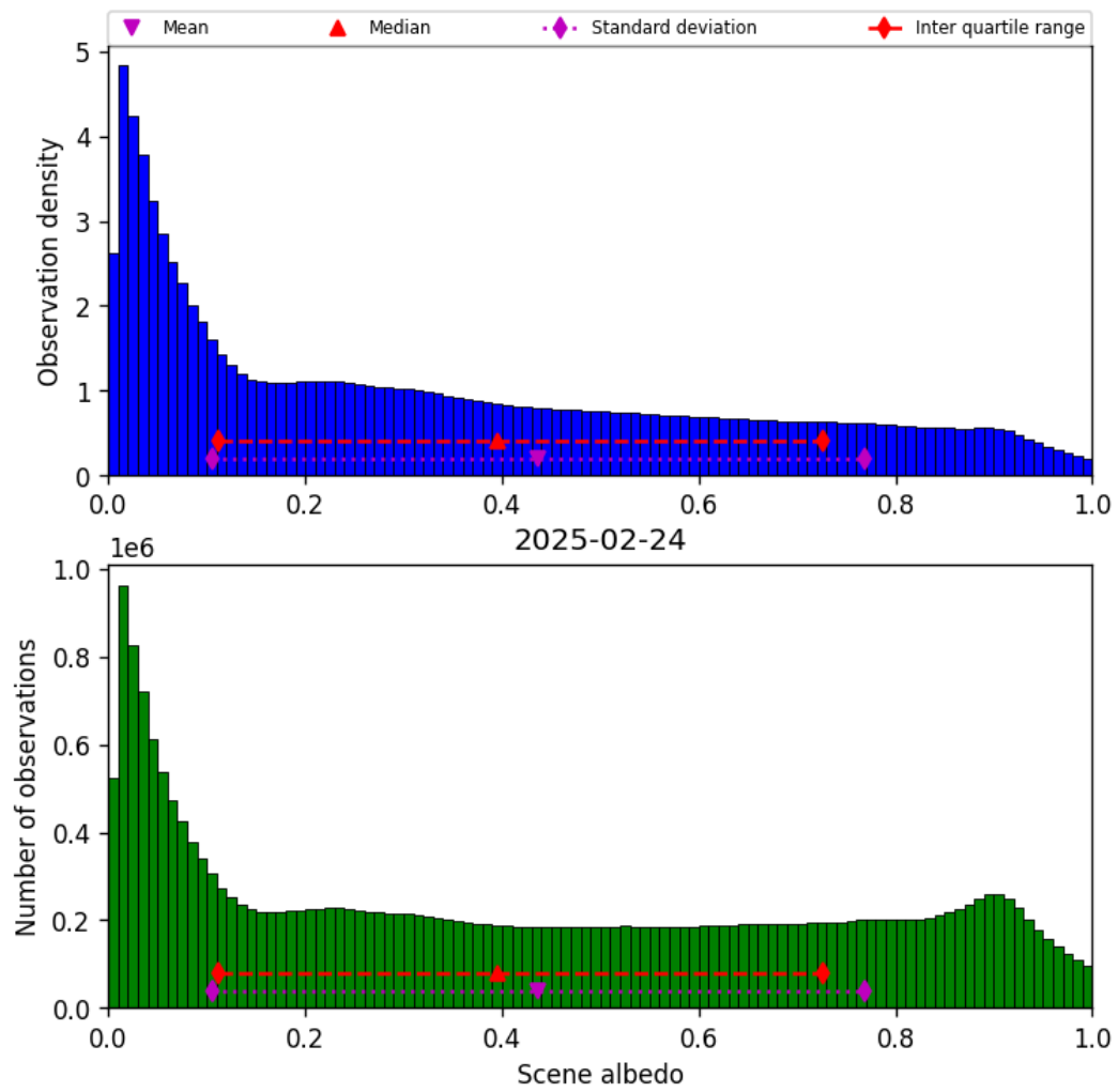
Figure 34: Histogram of “Scene albedo” for 2025-02-24 to 2025-02-25
