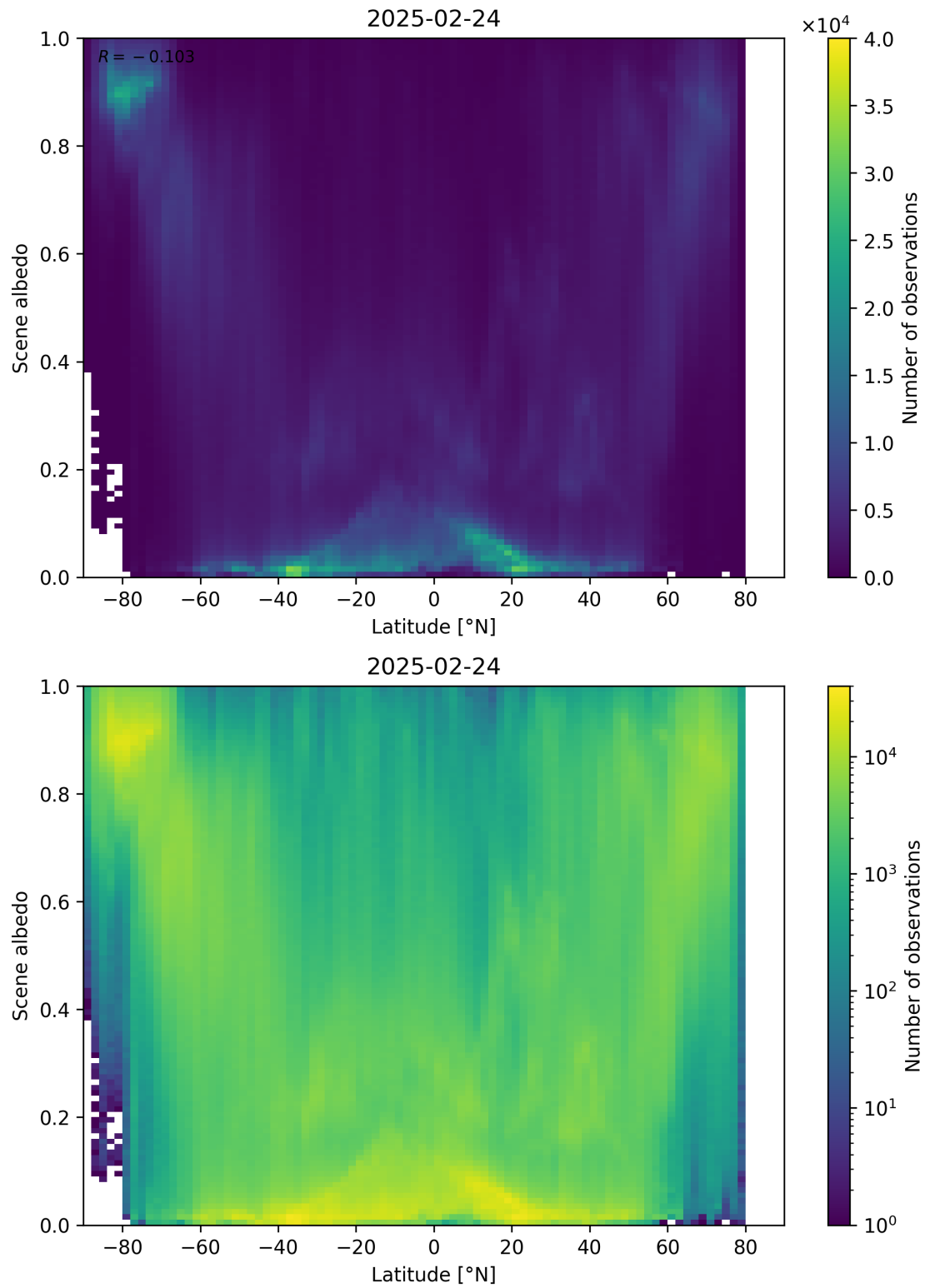
Figure 95: Scatter density plot of “Latitude” against “Scene albedo” for 2025-02-24 to 2025-02-25.
