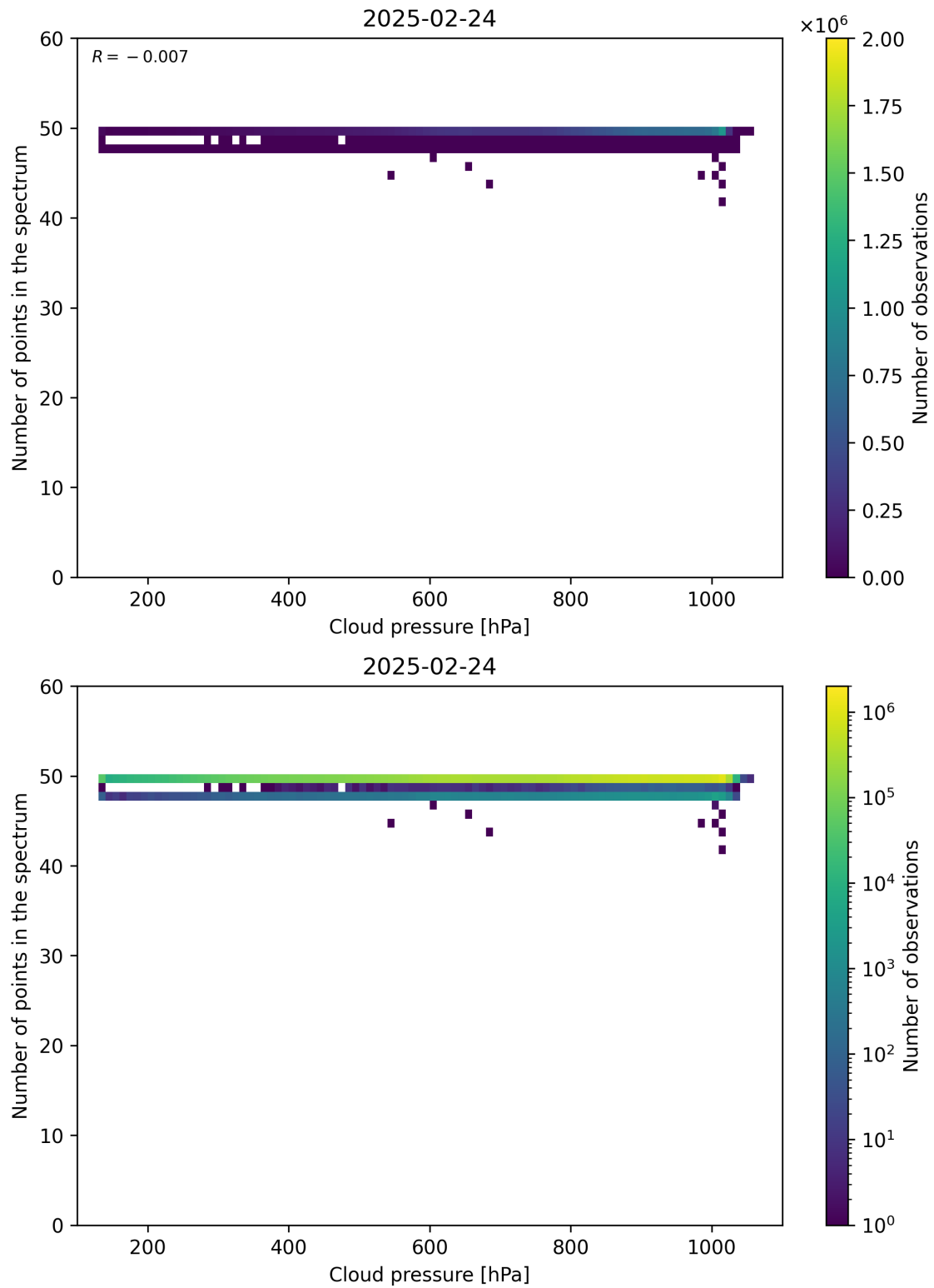
Figure 82: Scatter density plot of “Cloud pressure” against “Number of points in the spectrum” for 2025-02-24 to 2025-02-25.
