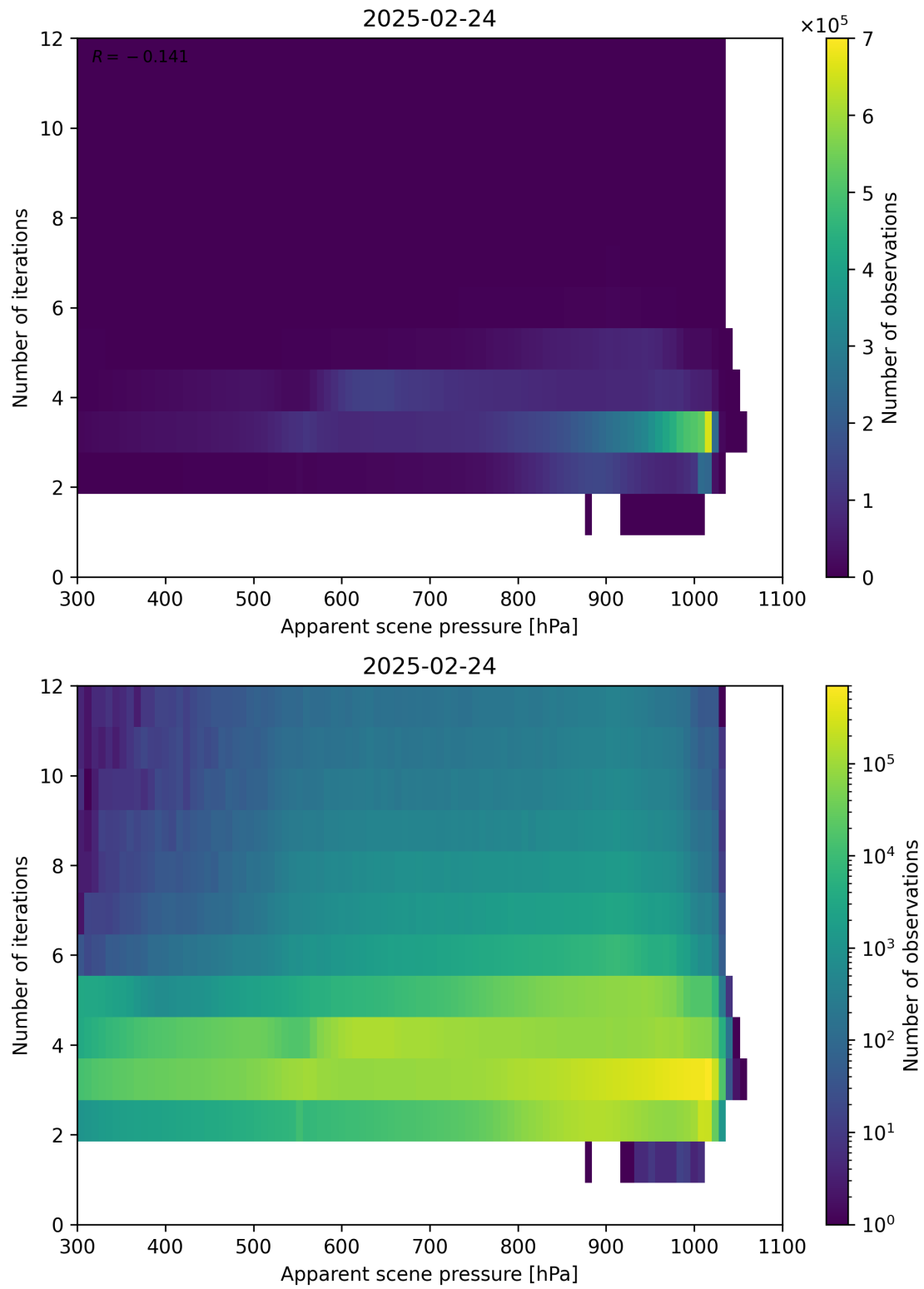
Figure 65: Scatter density plot of “Apparent scene pressure” against “Number of iterations” for 2025-02-24 to 2025-02-25.
