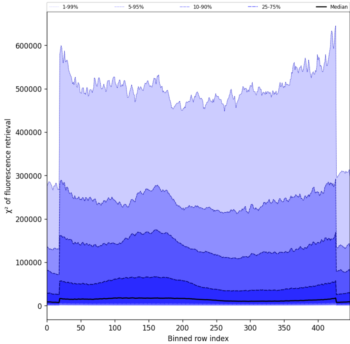
Figure 59: Along track statistics of “ \chi^2 of fluorescence retrieval” for 2025-02-24 to 2025-02-25
