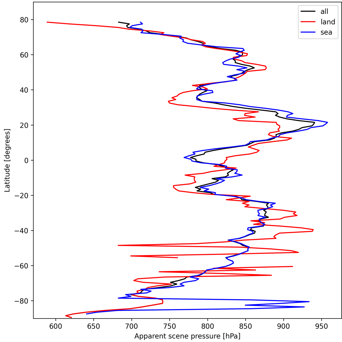
Figure 19: Zonal average of “Apparent scene pressure” for 2025-02-24 to 2025-02-25.
