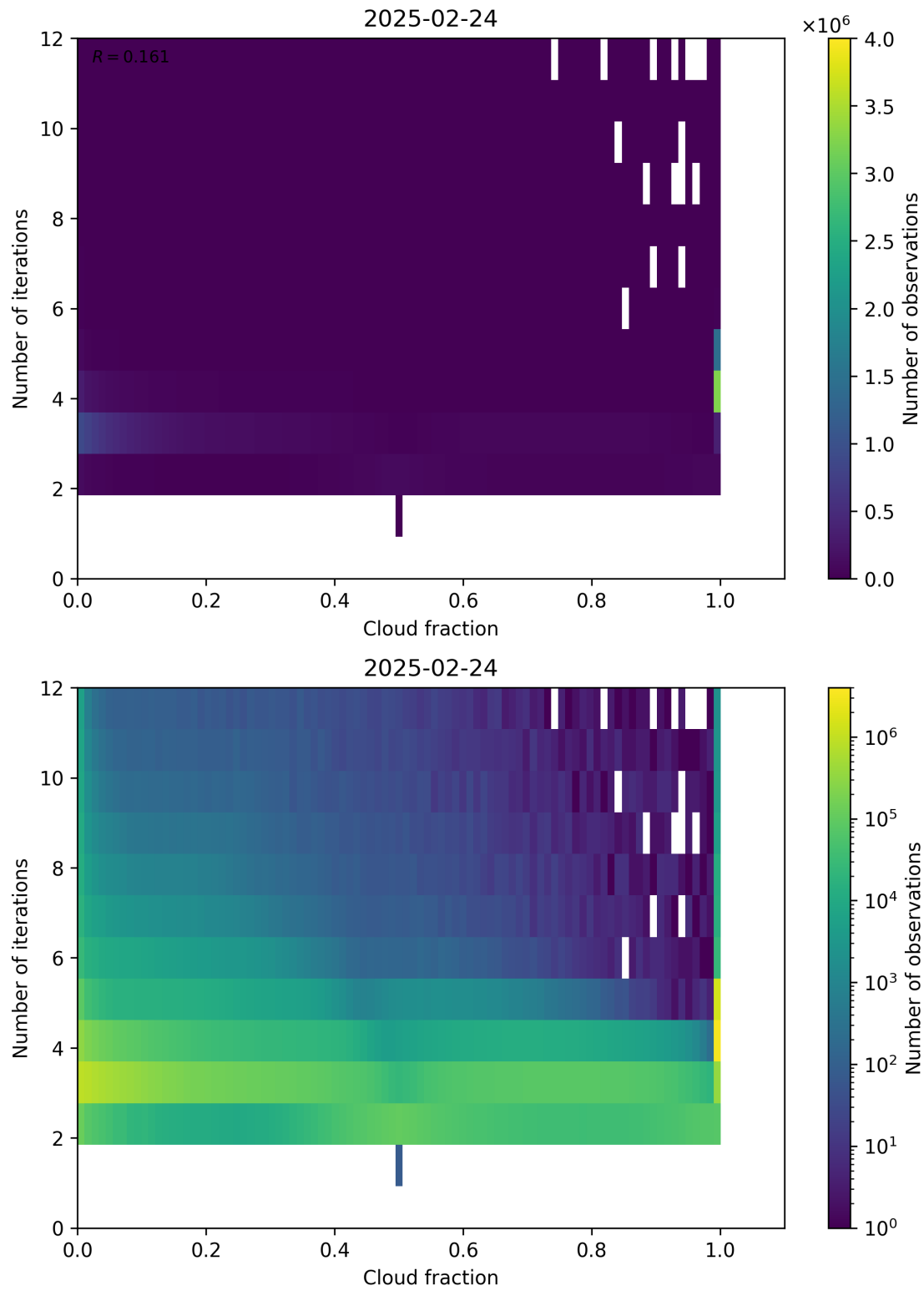
Figure 73: Scatter density plot of “Cloud fraction” against “Number of iterations” for 2025-02-24 to 2025-02-25.
