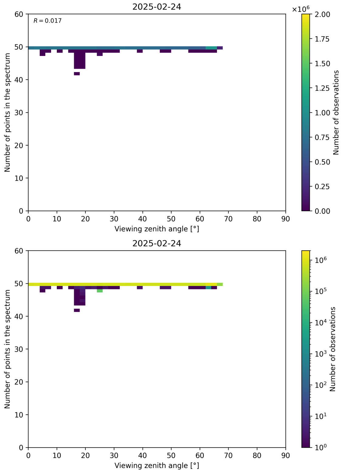
Figure 125: Scatter density plot of “Viewing zenith angle” against “Number of points in the spectrum” for 2025-02-24 to 2025-02-25.
