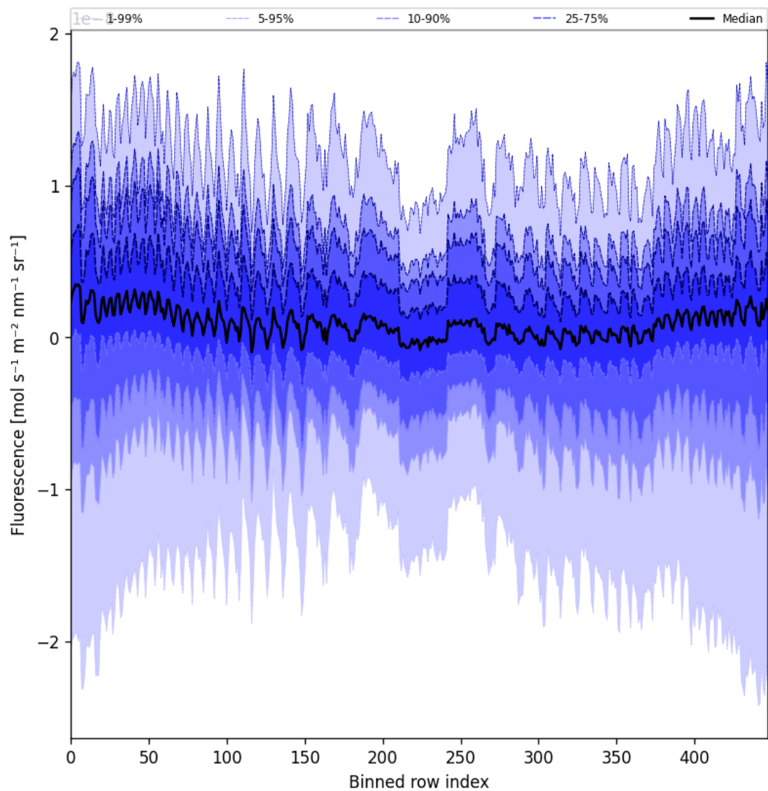
Figure 57: Along track statistics of “Fluorescence” for 2025-02-24 to 2025-02-25
