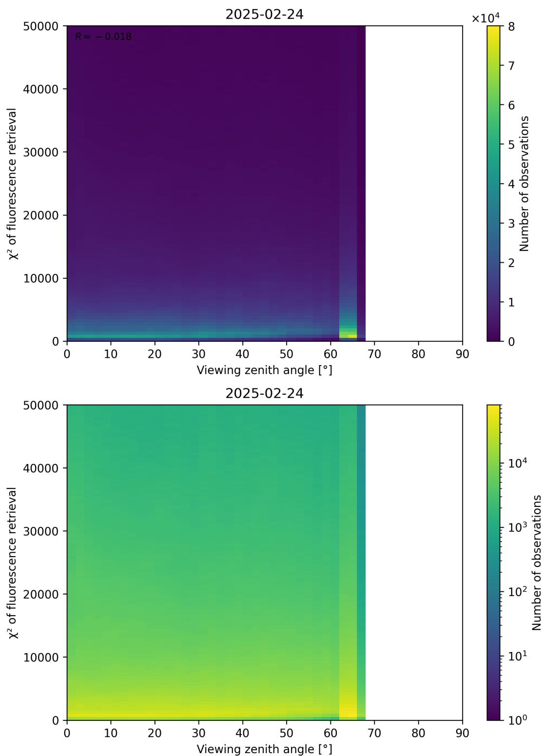
Figure 119: Scatter density plot of “Viewing zenith angle” against “ \chi^2 of fluorescence retrieval” for 2025-02-24 to 2025-02-25.
