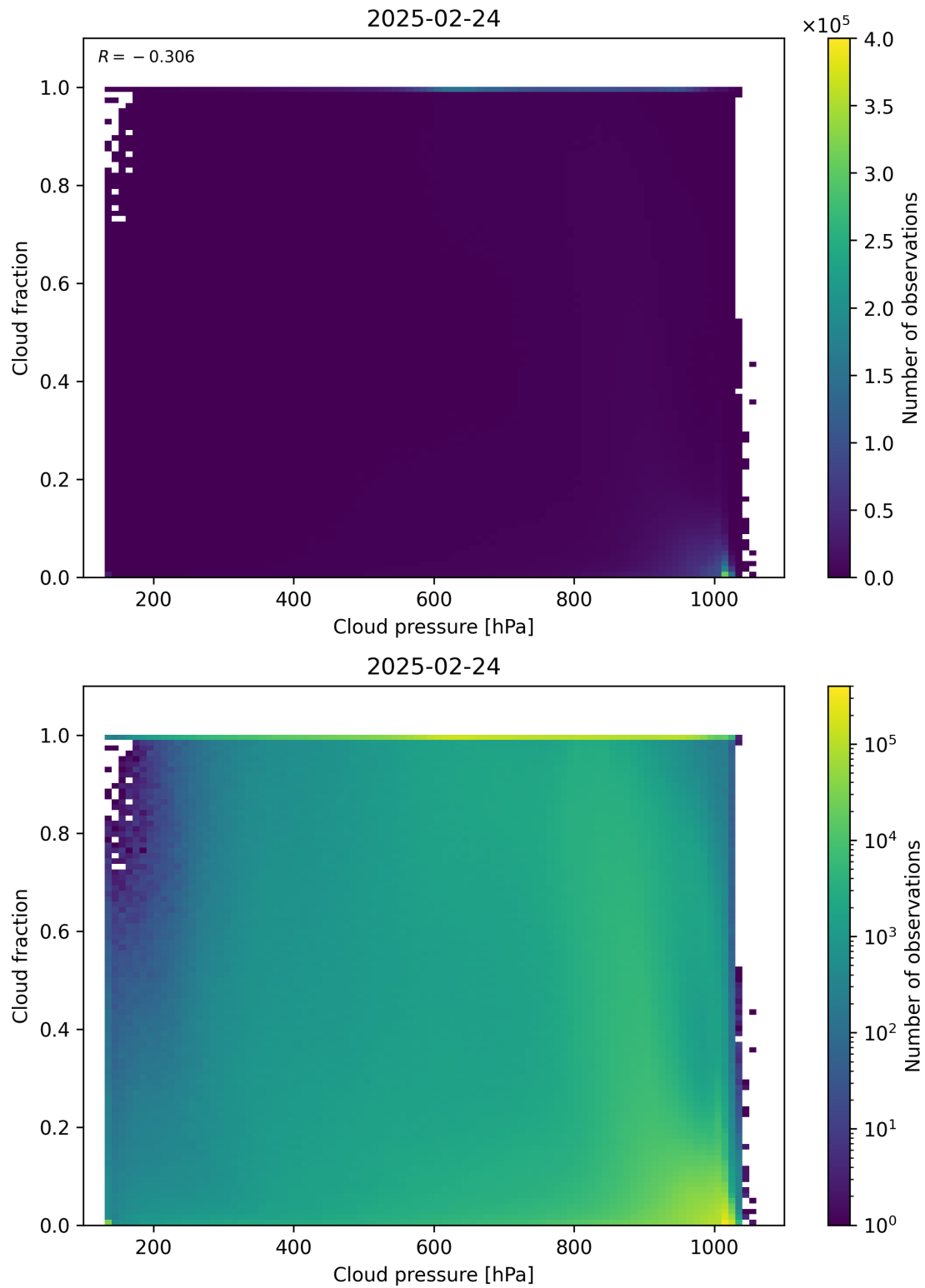
Figure 79: Scatter density plot of “Cloud pressure” against “Cloud fraction” for 2025-02-24 to 2025-02-25.
