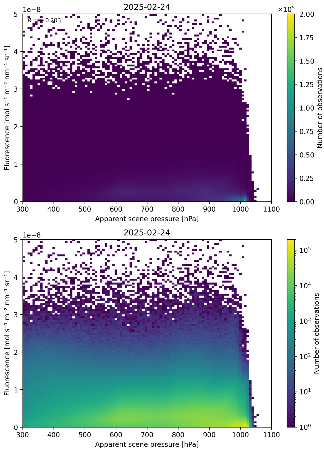
Figure 64: Scatter density plot of “Apparent scene pressure” against “Fluorescence” for 2025-02-24 to 2025-02-25.
