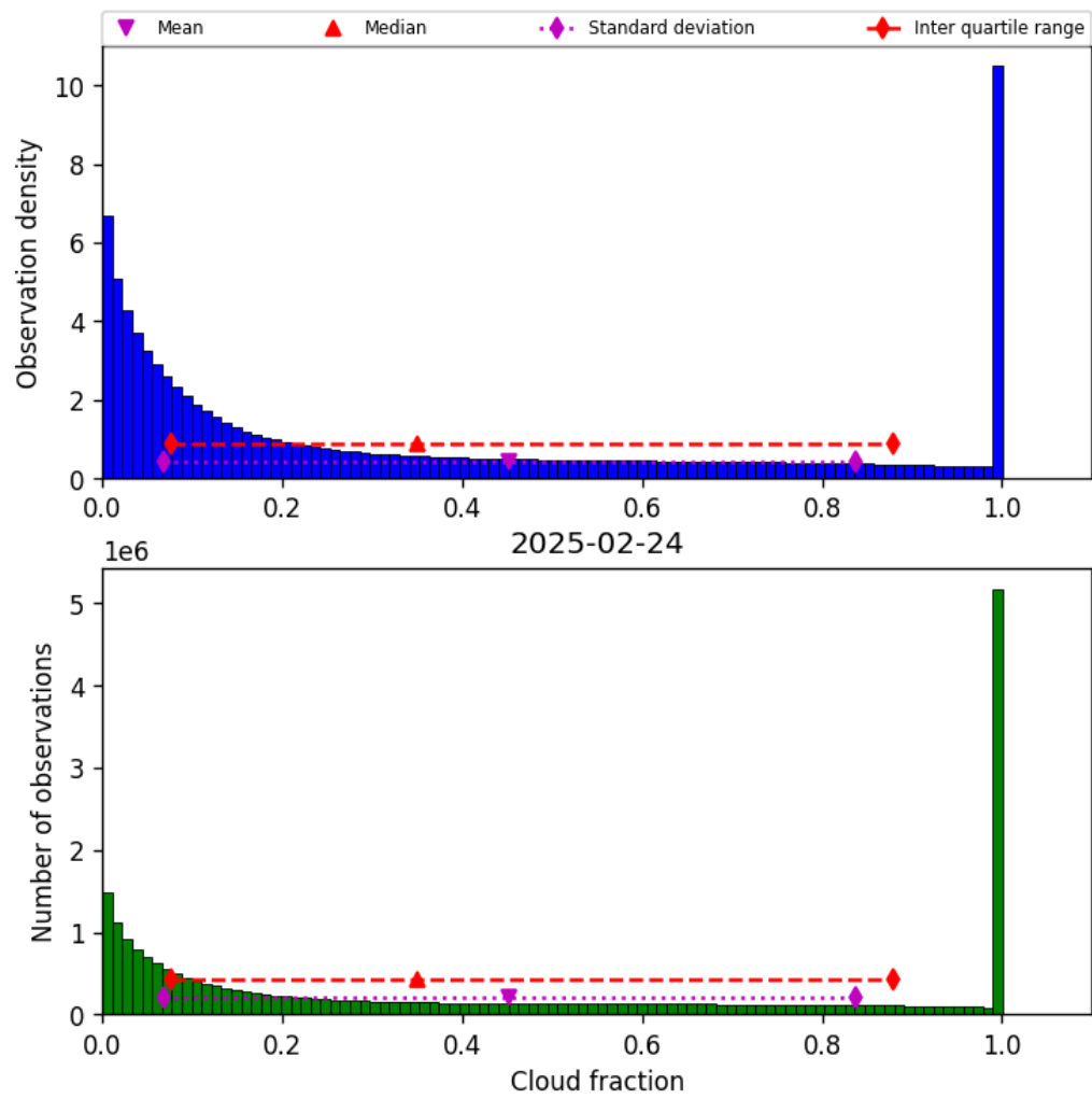
Figure 32: Histogram of “Cloud fraction” for 2025-02-24 to 2025-02-25
