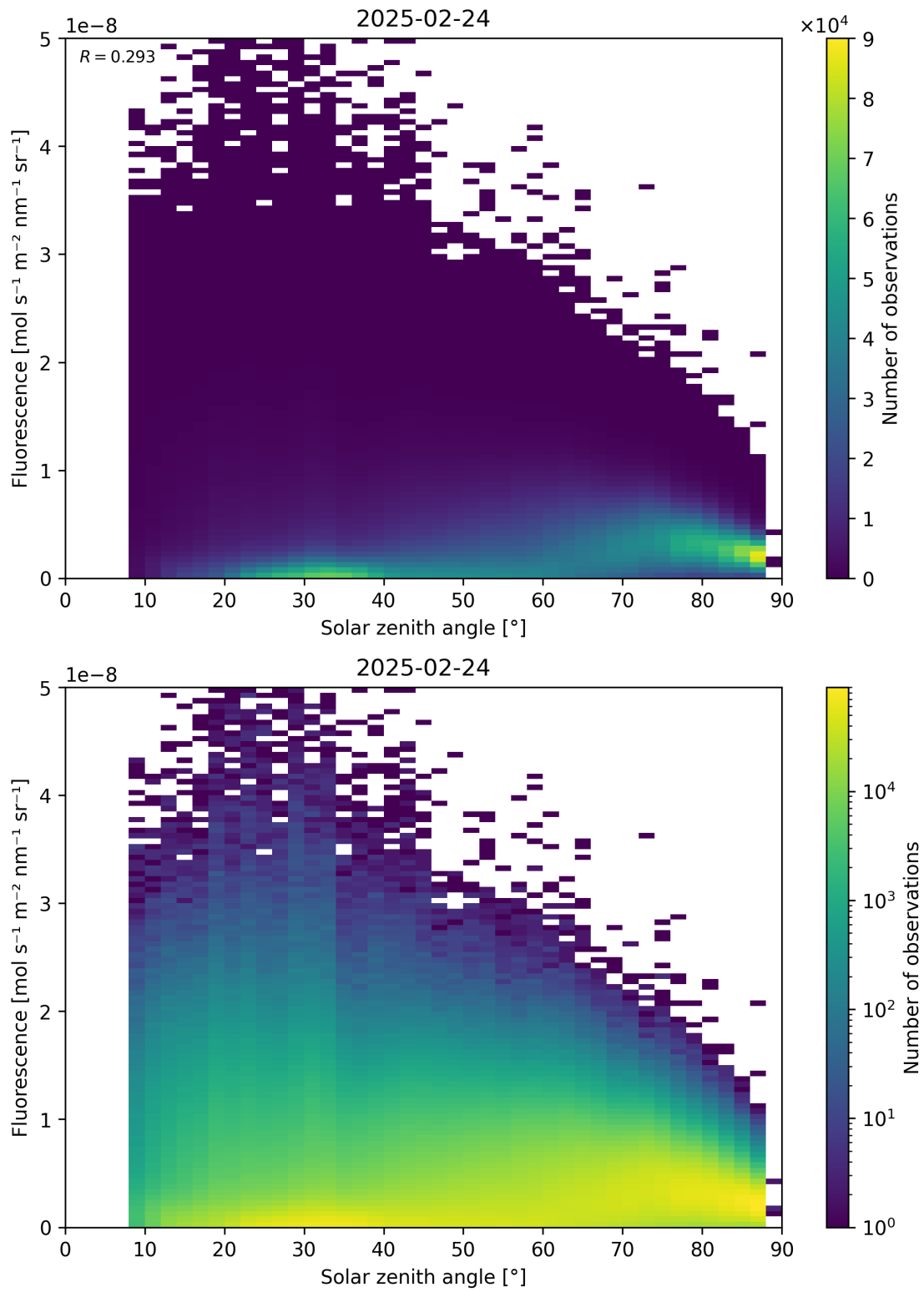
Figure 112: Scatter density plot of “Solar zenith angle” against “Fluorescence” for 2025-02-24 to 2025-02-25.
