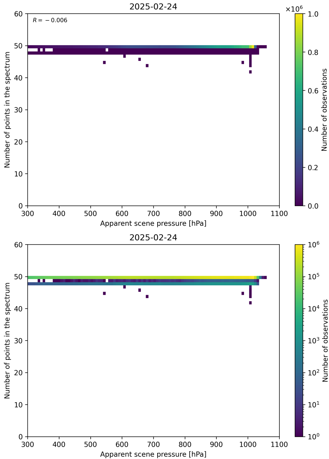
Figure 66: Scatter density plot of “Apparent scene pressure” against “Number of points in the spectrum” for 2025-02-24 to 2025-02-25.
