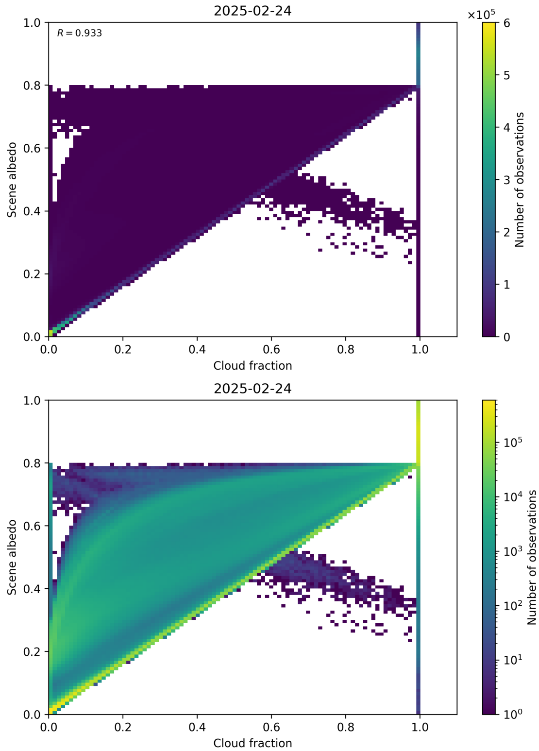
Figure 75: Scatter density plot of “Cloud fraction” against “Scene albedo” for 2025-02-24 to 2025-02-25.
