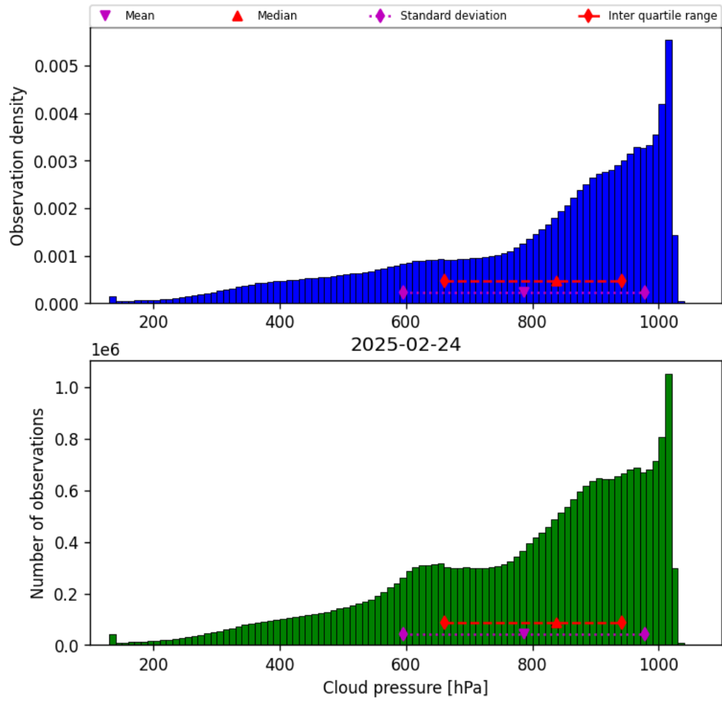
Figure 30: Histogram of “Cloud pressure” for 2025-02-24 to 2025-02-25
