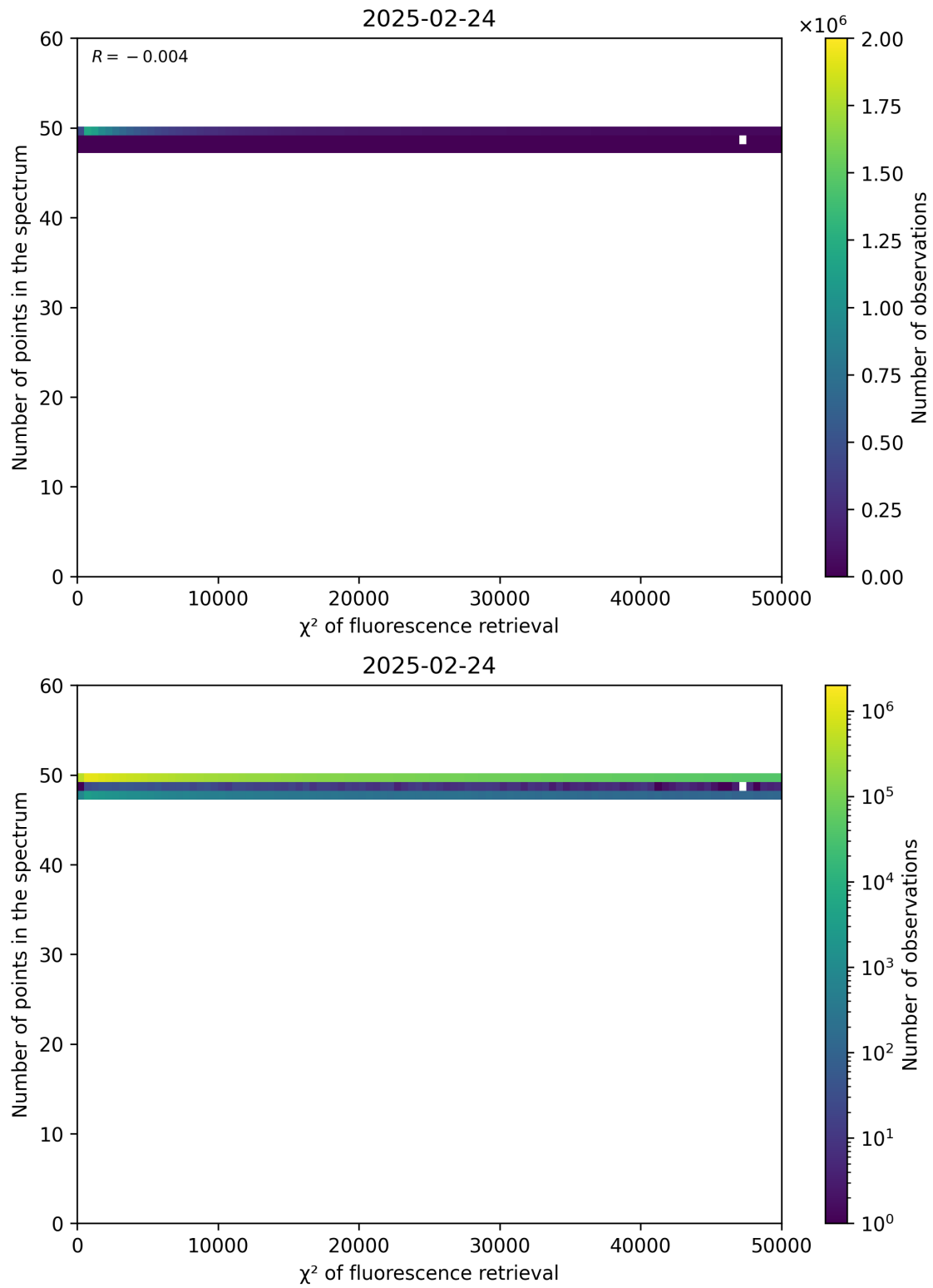
Figure 68: Scatter density plot of “ \chi^2 of fluorescence retrieval” against “Number of points in the spectrum” for 2025-02-24 to 2025-02-25.
