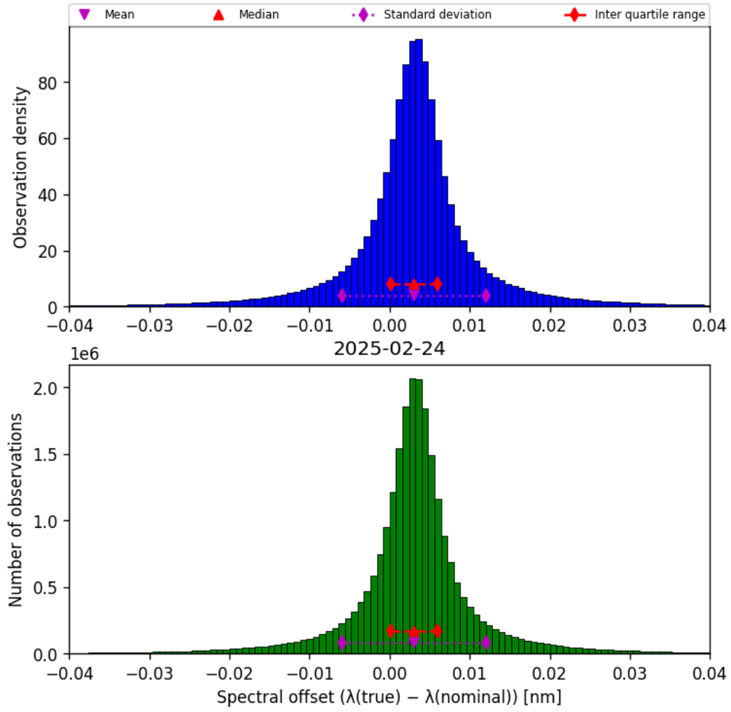
Figure 45: Histogram of “Spectral offset ( \lambda_{\text{true}} - \lambda_{\text{nominal}} )” for 2025-02-24 to 2025-02-25
