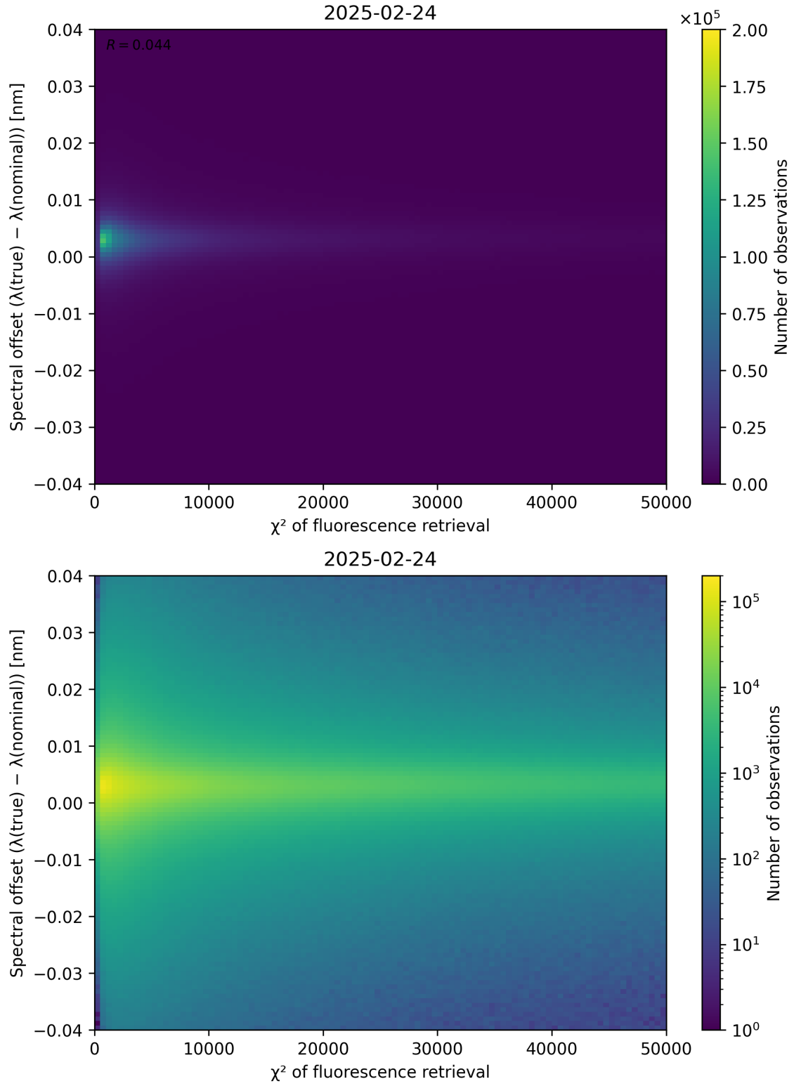
Figure 69: Scatter density plot of “ \chi^2 of fluorescence retrieval” against “Spectral offset ( \lambda_{\text{true}} - \lambda_{\text{nominal}} )” for 2025-02-24 to 2025-02-25.
