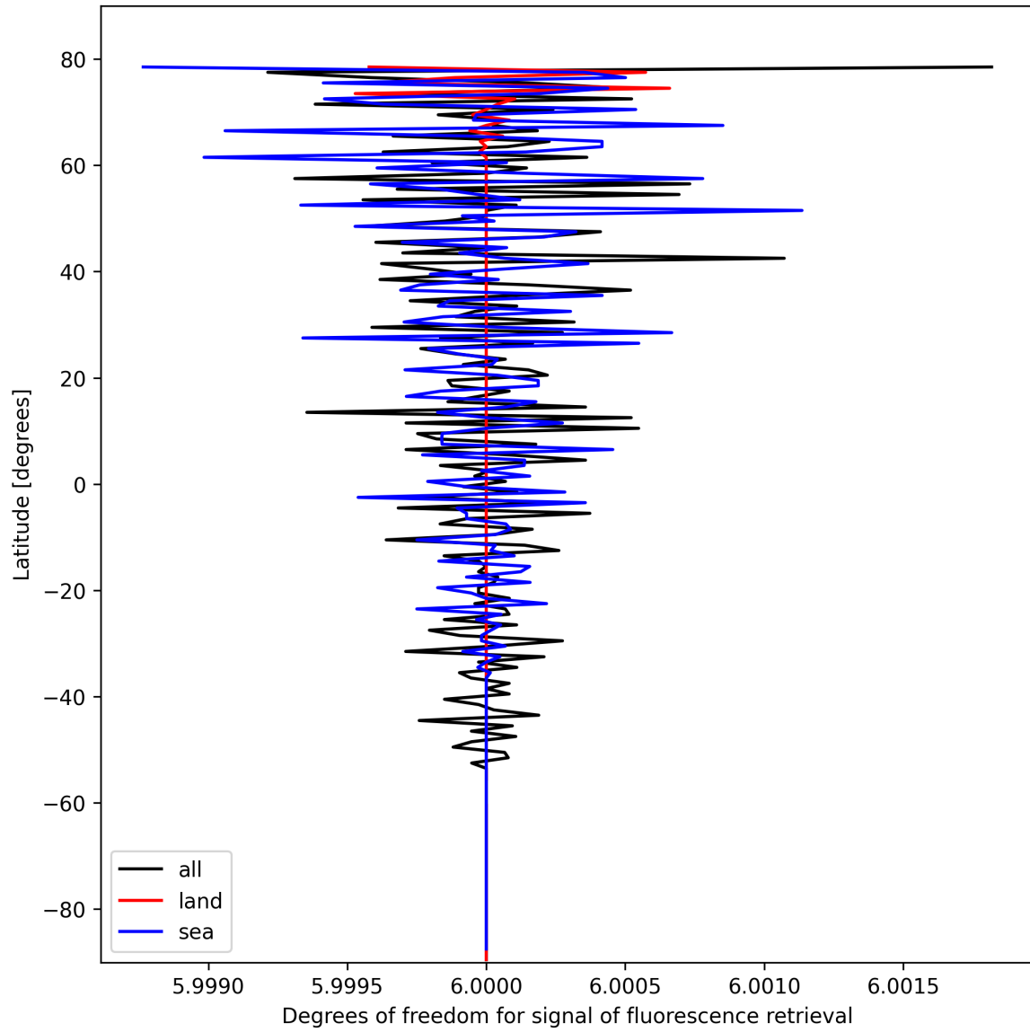
Figure 26: Zonal average of “Degrees of freedom for signal of fluorescence retrieval” for 2025-02-24 to 2025-02-25.
