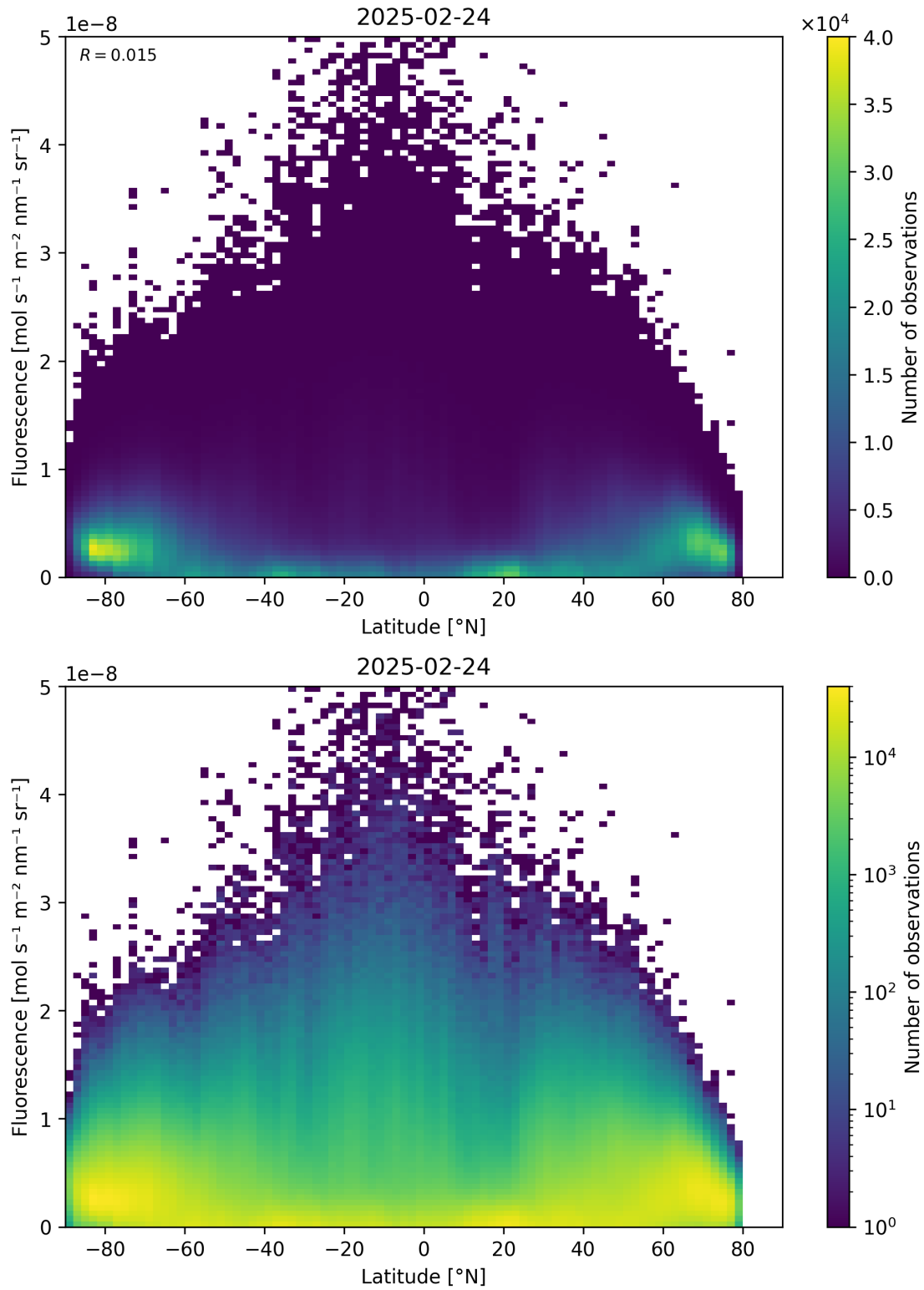
Figure 92: Scatter density plot of “Latitude” against “Fluorescence” for 2025-02-24 to 2025-02-25.
