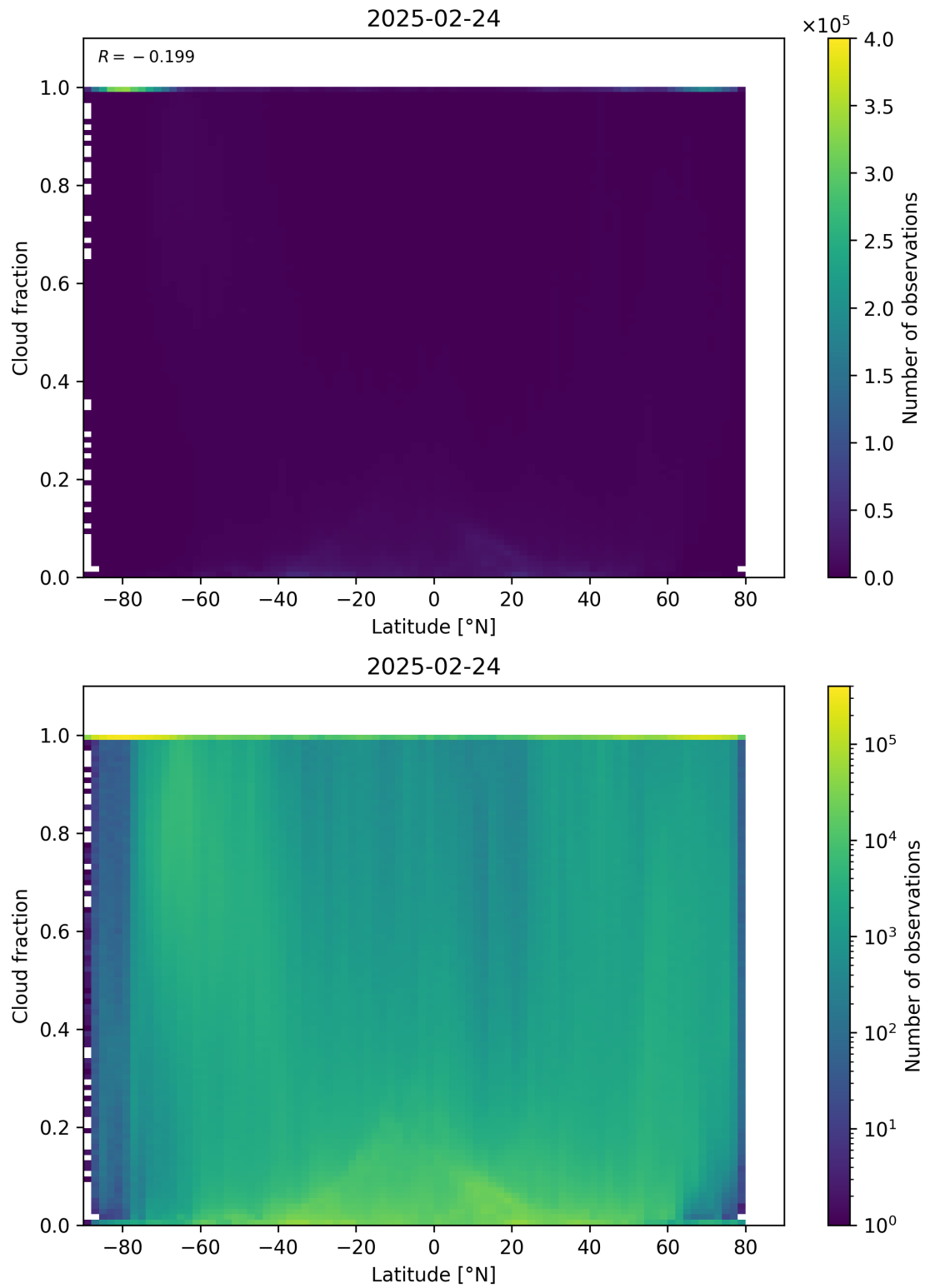
Figure 90: Scatter density plot of “Latitude” against “Cloud fraction” for 2025-02-24 to 2025-02-25.
