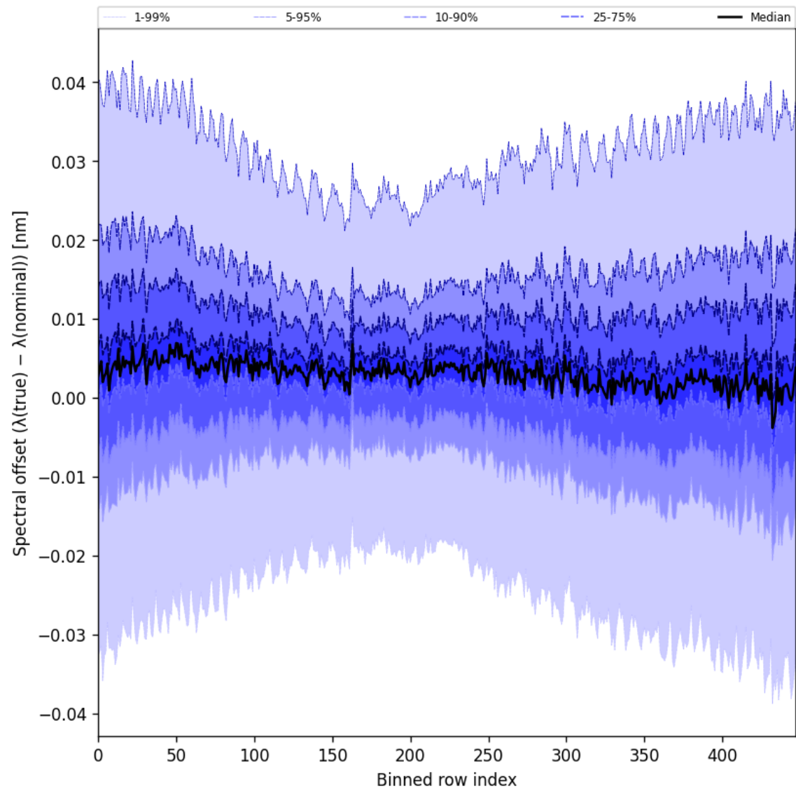
Figure 62: Along track statistics of “Spectral offset ( \lambda_{\text{true}} - \lambda_{\text{nominal}} )” for 2025-02-24 to 2025-02-25
