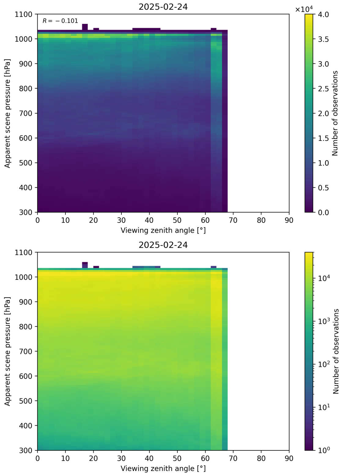
Figure 118: Scatter density plot of “Viewing zenith angle” against “Apparent scene pressure” for 2025-02-24 to 2025-02-25.
