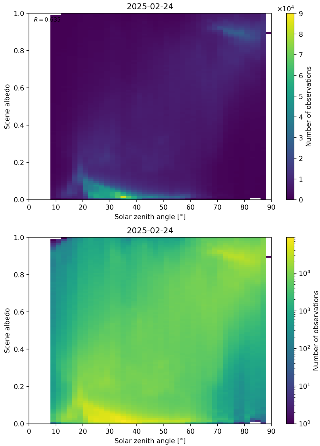
Figure 116: Scatter density plot of “Solar zenith angle” against “Scene albedo” for 2025-02-24 to 2025-02-25.
