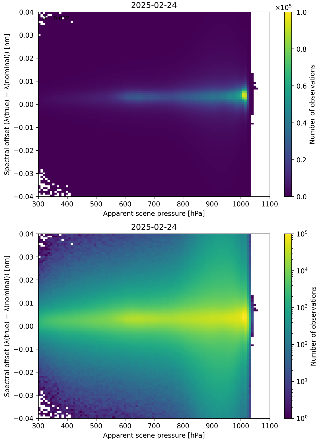
Figure 67: Scatter density plot of “Apparent scene pressure” against “Spectral offset ( \lambda_{\text{true}} - \lambda_{\text{nominal}} )” for 2025-02-24 to 2025-02-25.
