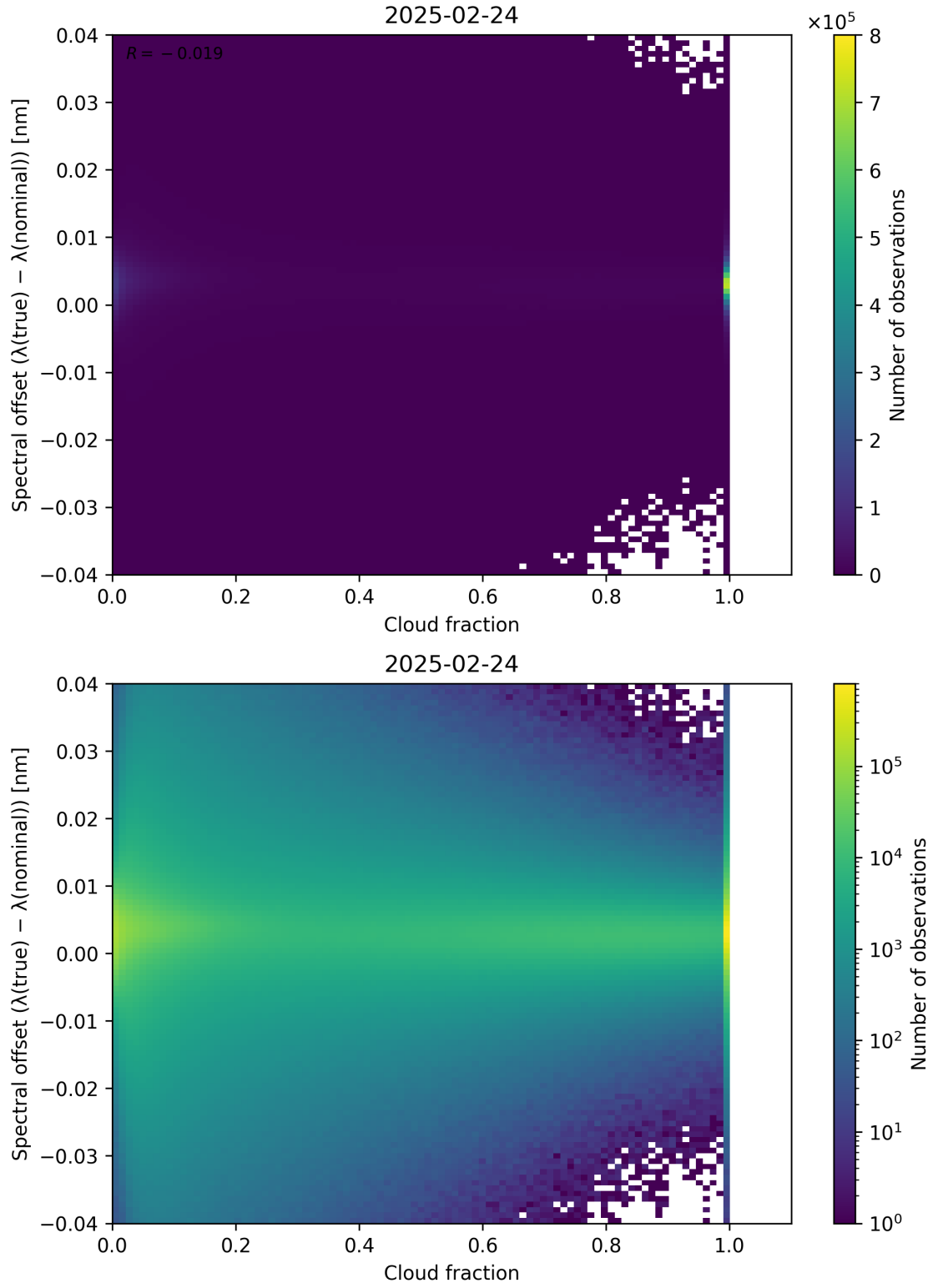
Figure 76: Scatter density plot of “Cloud fraction” against “Spectral offset ( \lambda_{\text{true}} - \lambda_{\text{nominal}} )” for 2025-02-24 to 2025-02-25.
