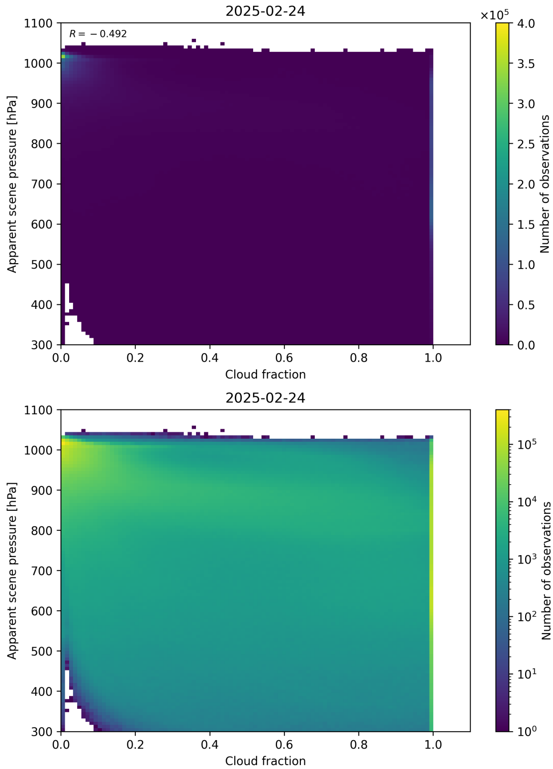
Figure 70: Scatter density plot of “Cloud fraction” against “Apparent scene pressure” for 2025-02-24 to 2025-02-25.
