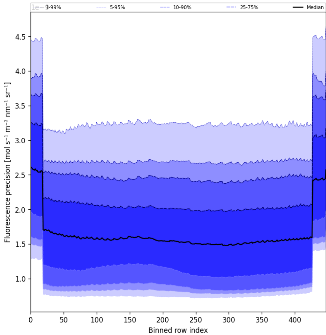
Figure 58: Along track statistics of “Fluorescence precision” for 2025-02-24 to 2025-02-25
