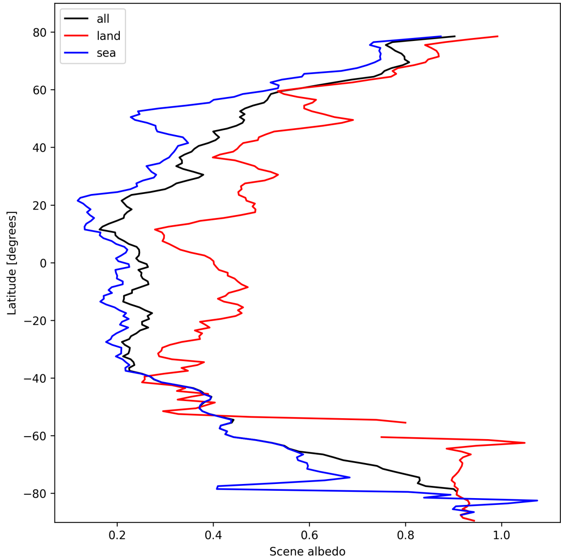
Figure 17: Zonal average of “Scene albedo” for 2025-02-24 to 2025-02-25.
