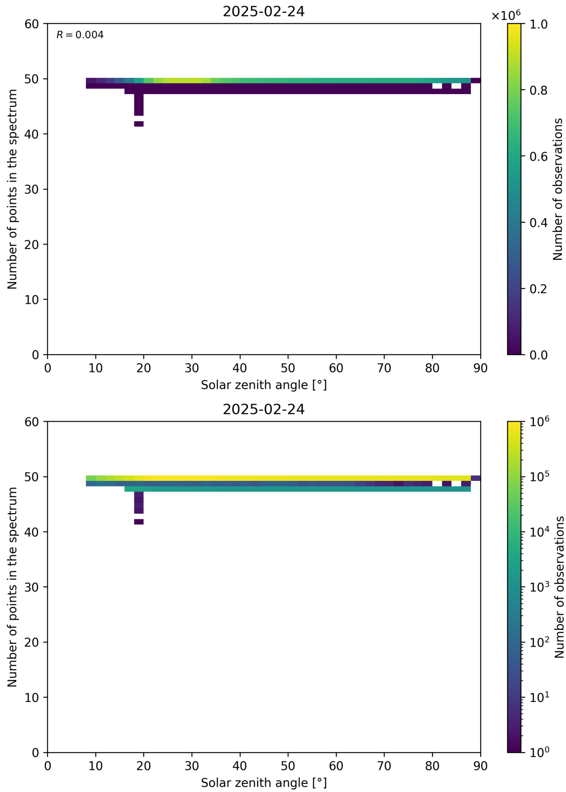
Figure 115: Scatter density plot of “Solar zenith angle” against “Number of points in the spectrum” for 2025-02-24 to 2025-02-25.
