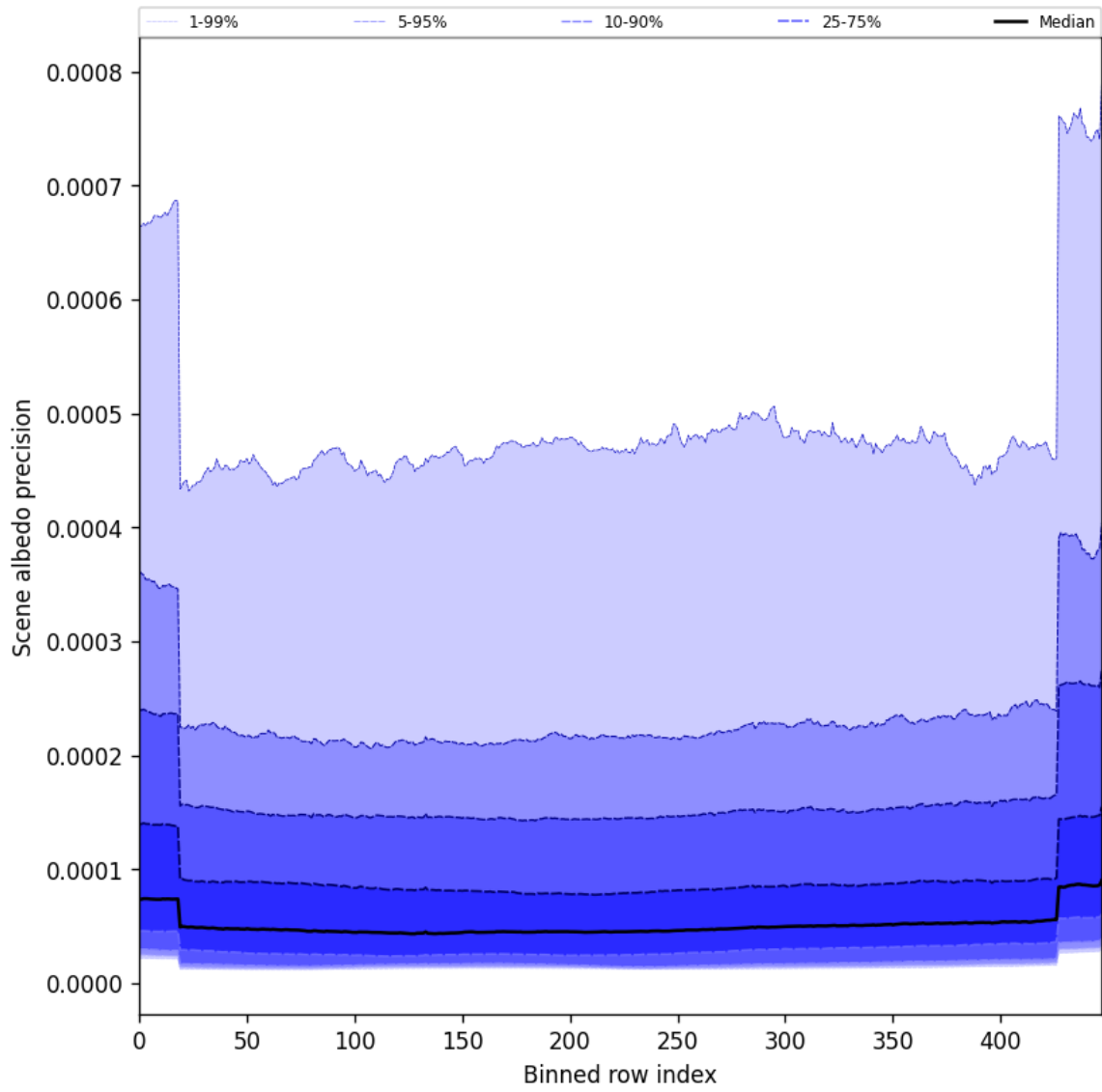
Figure 52: Along track statistics of “Scene albedo precision” for 2025-02-24 to 2025-02-25
