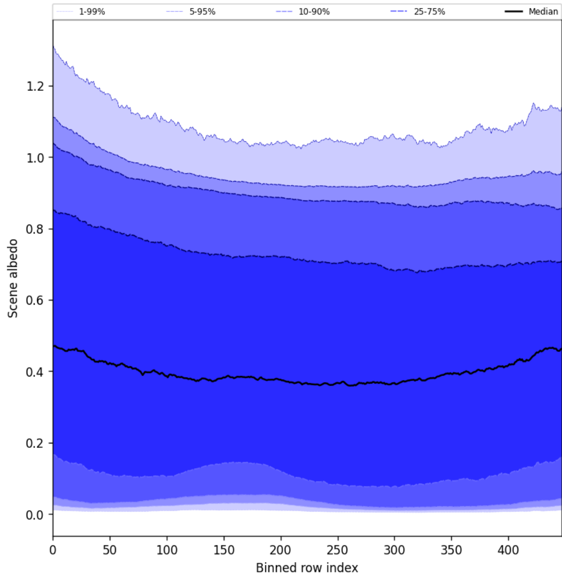
Figure 51: Along track statistics of “Scene albedo” for 2025-02-24 to 2025-02-25
