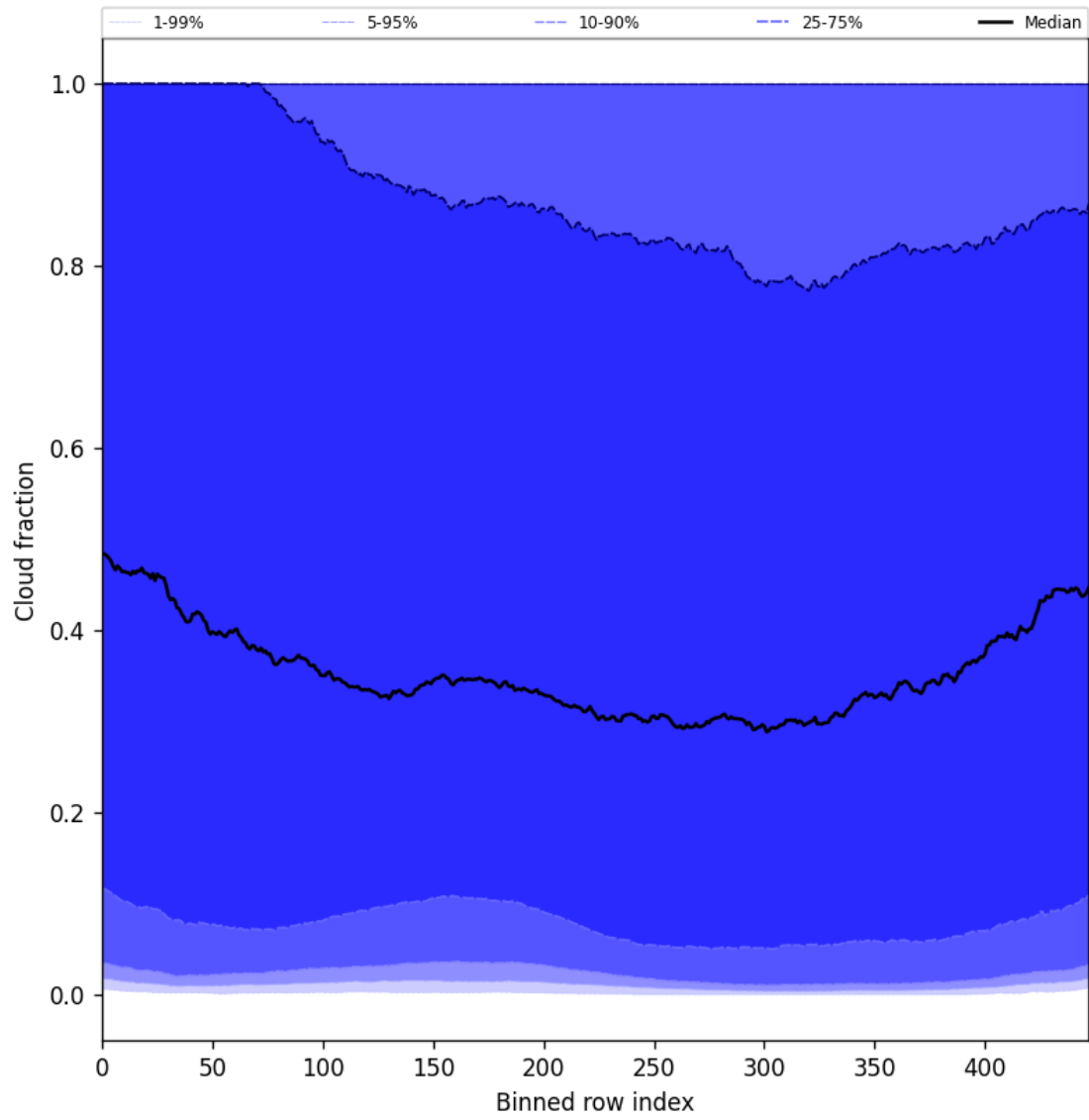
Figure 49: Along track statistics of “Cloud fraction” for 2025-02-24 to 2025-02-25
