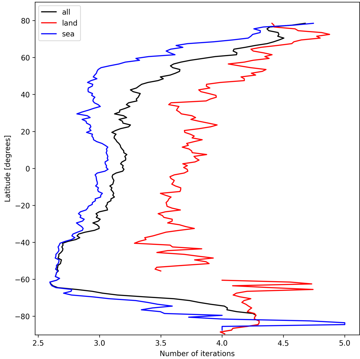
Figure 22: Zonal average of “Number of iterations” for 2025-02-24 to 2025-02-25.
