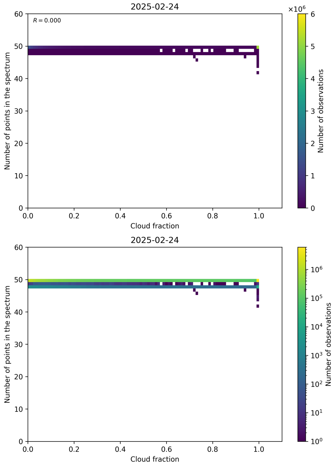
Figure 74: Scatter density plot of “Cloud fraction” against “Number of points in the spectrum” for 2025-02-24 to 2025-02-25.
