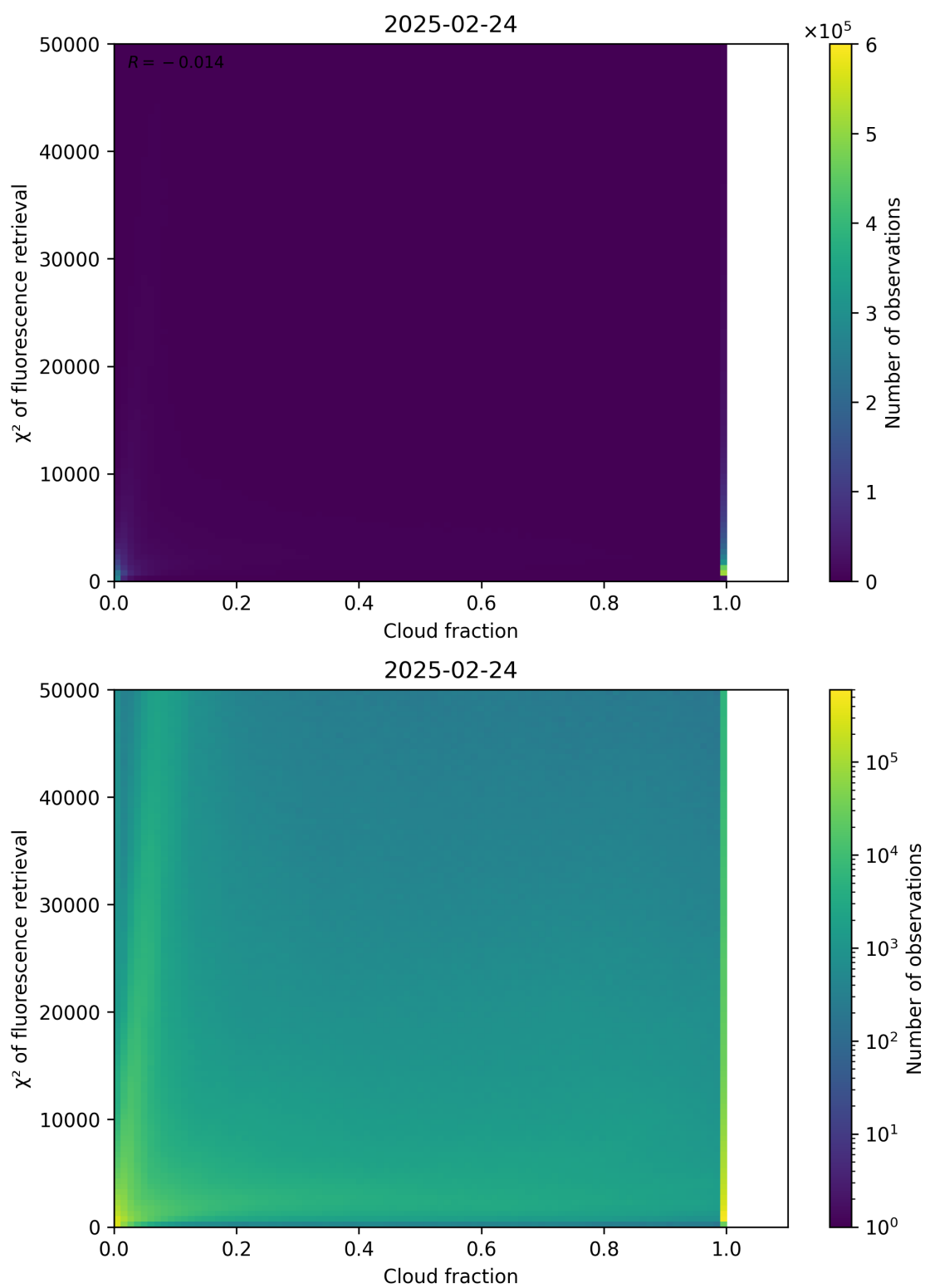
Figure 71: Scatter density plot of “Cloud fraction” against “ \chi^2 of fluorescence retrieval” for 2025-02-24 to 2025-02-25.
