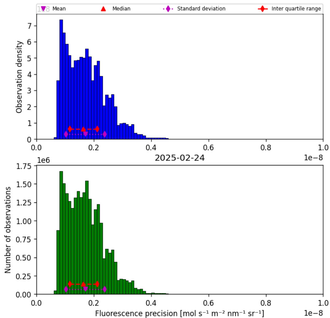
Figure 41: Histogram of “Fluorescence precision” for 2025-02-24 to 2025-02-25
