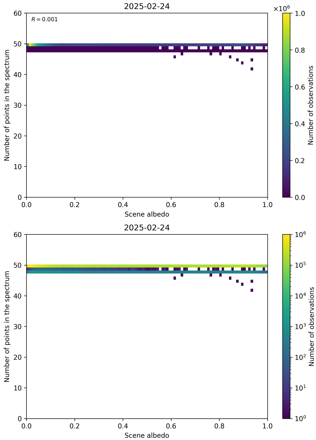
Figure 106: Scatter density plot of “Scene albedo” against “Number of points in the spectrum” for 2025-02-24 to 2025-02-25.
