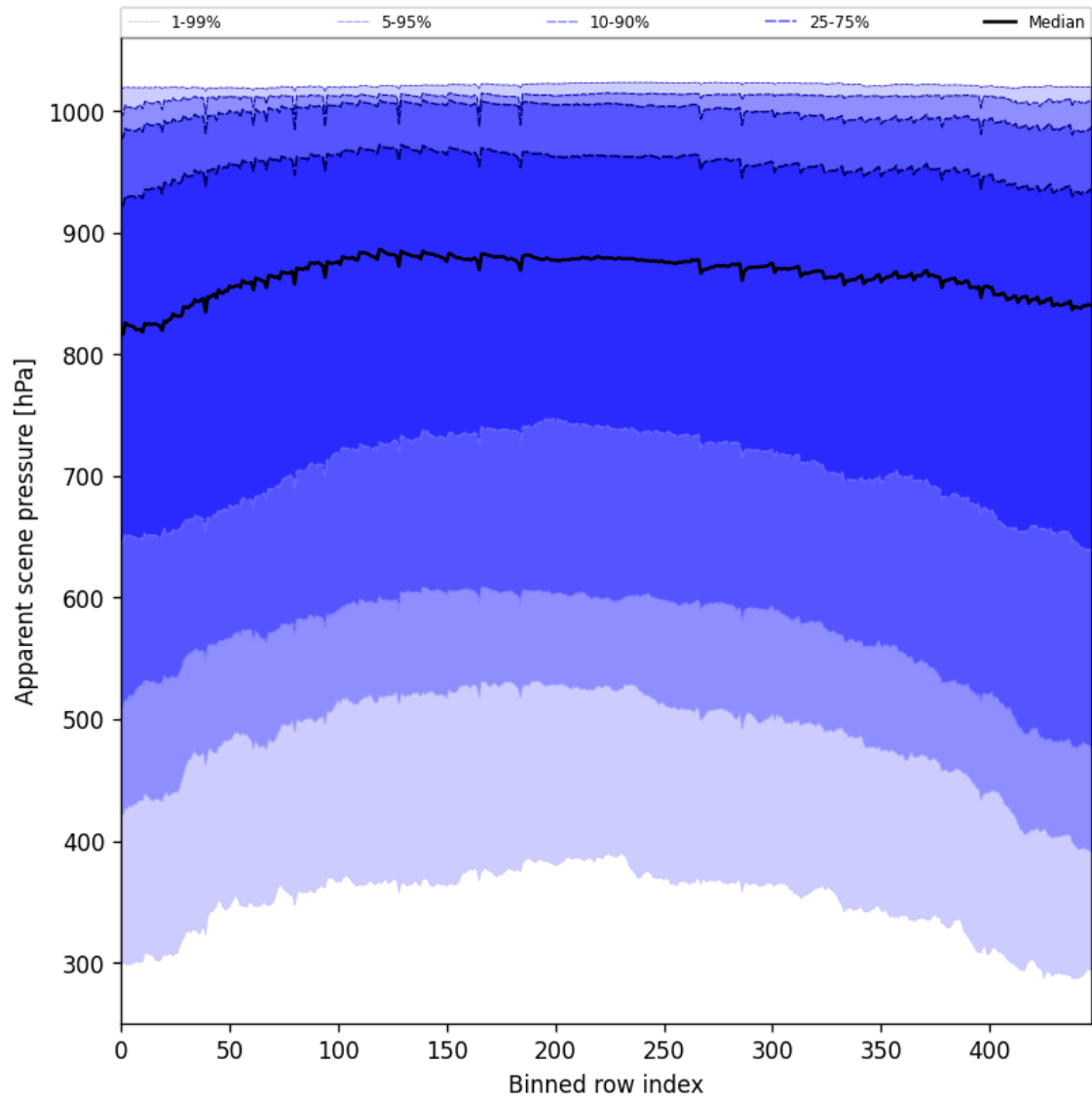
Figure 53: Along track statistics of “Apparent scene pressure” for 2025-02-24 to 2025-02-25
