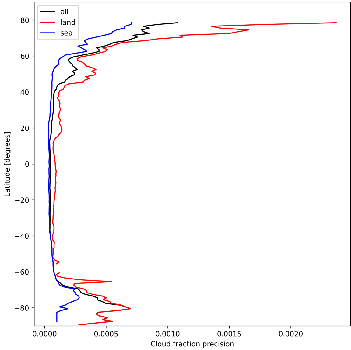
Figure 16: Zonal average of “Cloud fraction precision” for 2025-02-24 to 2025-02-25.
