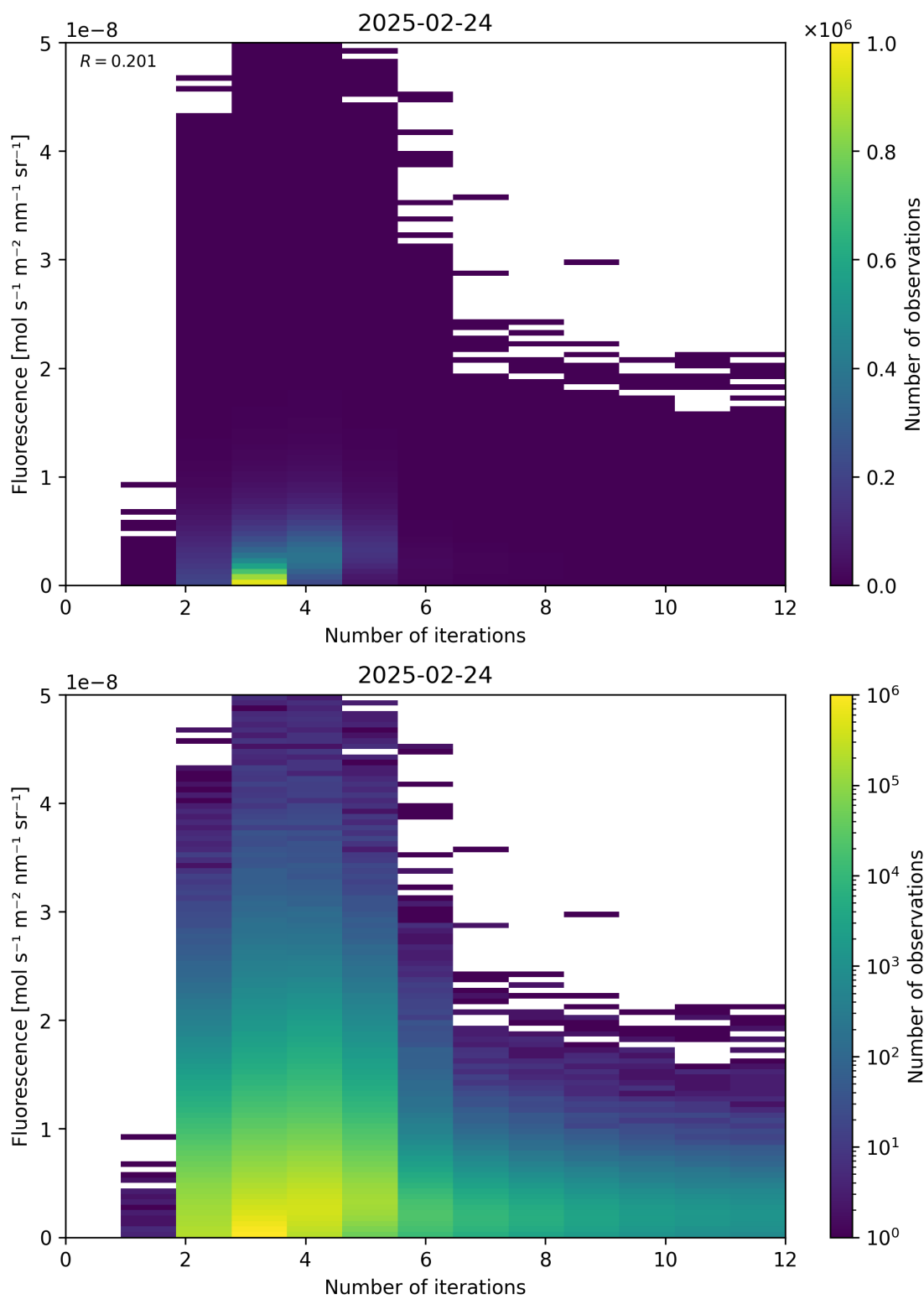
Figure 98: Scatter density plot of “Number of iterations” against “Fluorescence” for 2025-02-24 to 2025-02-25.
