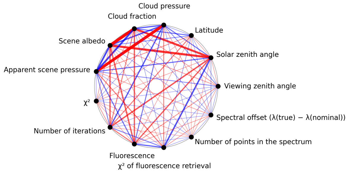
Figure 1: Map of correlation graph for 2025-02-24 to 2025-02-25.
