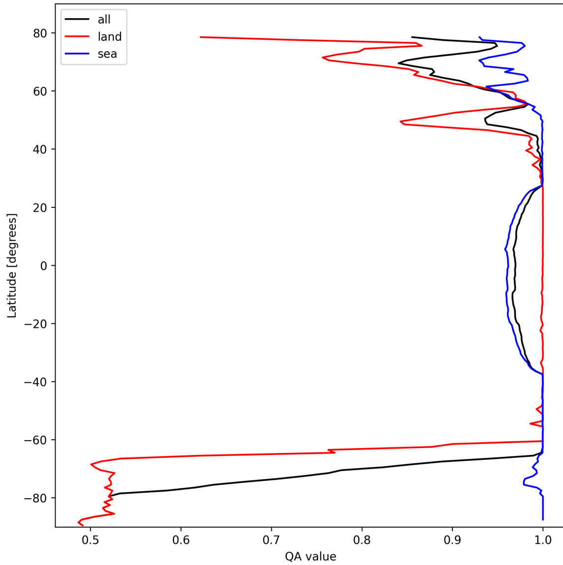
Figure 12: Zonal average of “QA value” for 2025-02-24 to 2025-02-25.
