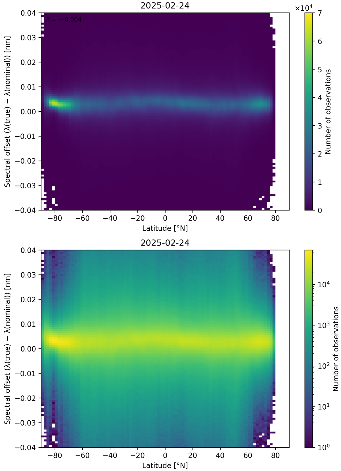
Figure 96: Scatter density plot of “Latitude” against “Spectral offset ( \lambda_{\text{true}} - \lambda_{\text{nominal}} )” for 2025-02-24 to 2025-02-25.
