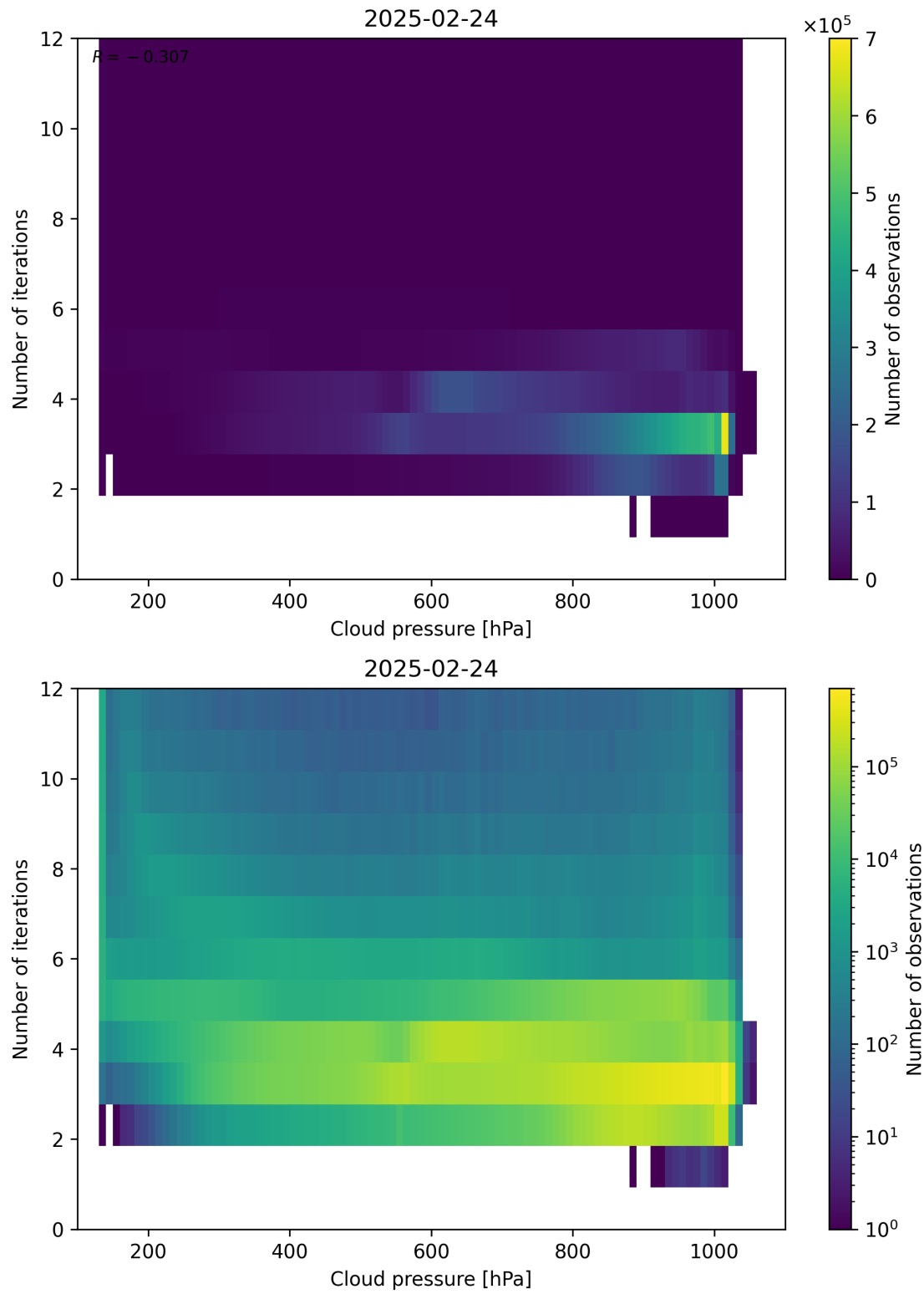
Figure 81: Scatter density plot of “Cloud pressure” against “Number of iterations” for 2025-02-24 to 2025-02-25.
