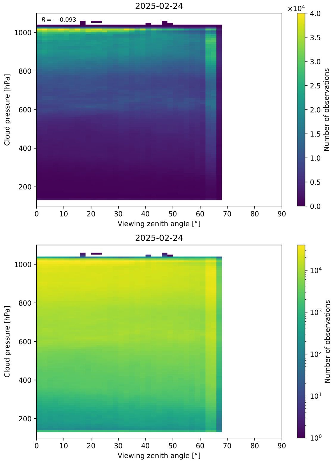
Figure 121: Scatter density plot of “Viewing zenith angle” against “Cloud pressure” for 2025-02-24 to 2025-02-25.
