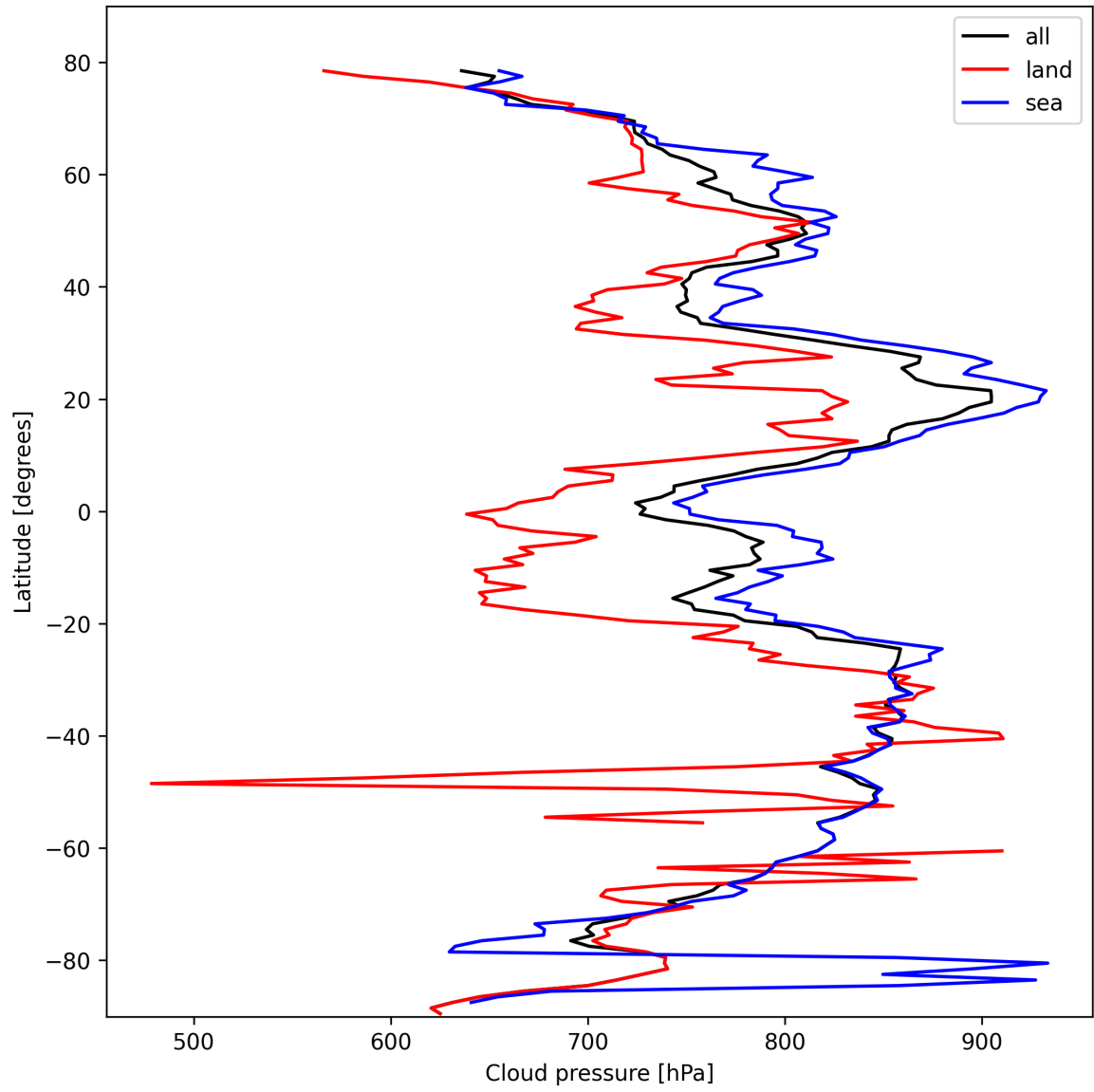
Figure 13: Zonal average of “Cloud pressure” for 2025-02-24 to 2025-02-25.
