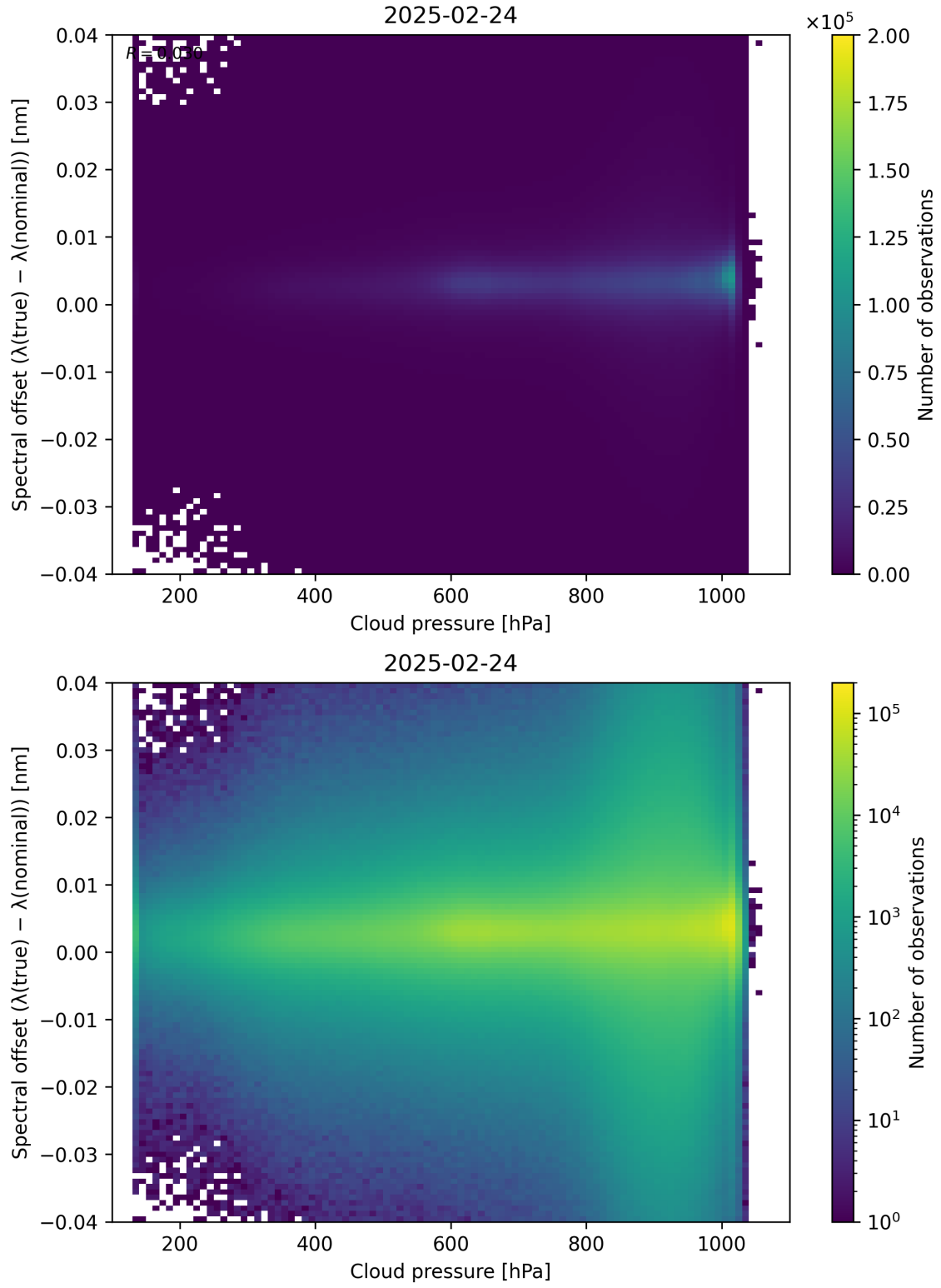
Figure 84: Scatter density plot of “Cloud pressure” against “Spectral offset ( \lambda_{\text{true}} - \lambda_{\text{nominal}} )” for 2025-02-24 to 2025-02-25.
