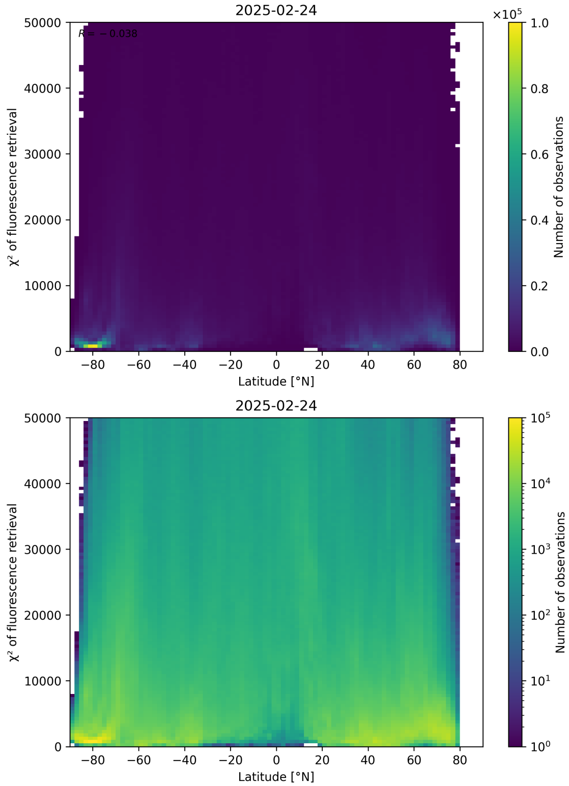
Figure 89: Scatter density plot of “Latitude” against “ \chi^2 of fluorescence retrieval” for 2025-02-24 to 2025-02-25.
