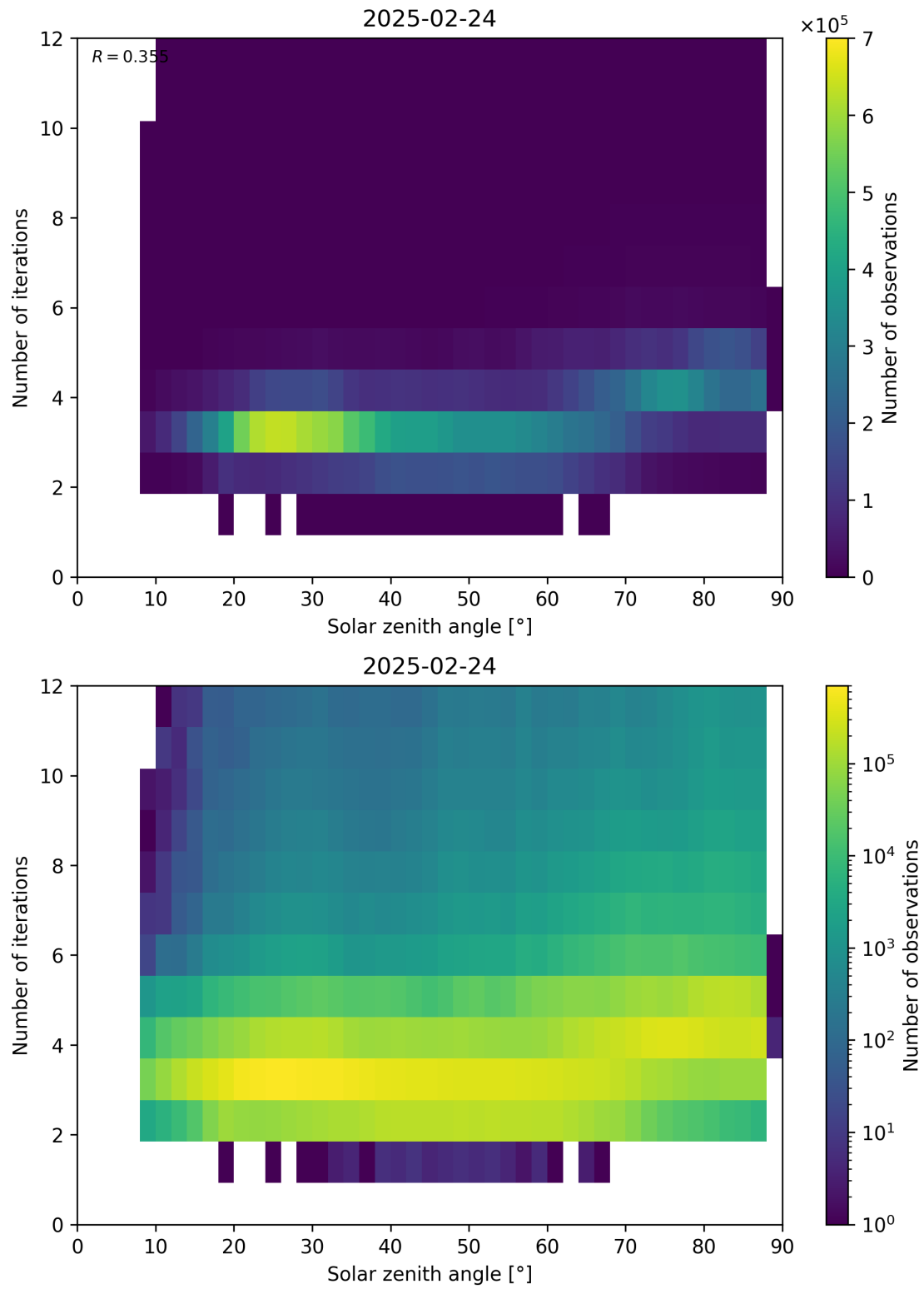
Figure 114: Scatter density plot of “Solar zenith angle” against “Number of iterations” for 2025-02-24 to 2025-02-25.
