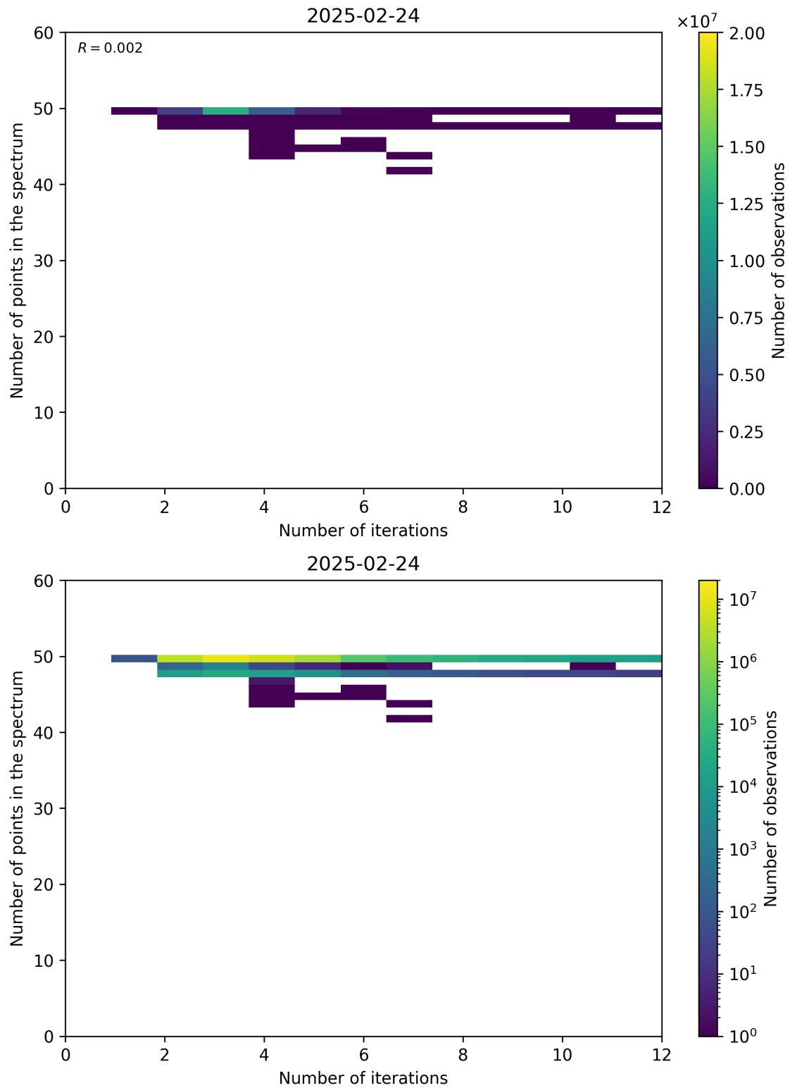
Figure 99: Scatter density plot of “Number of iterations” against “Number of points in the spectrum” for 2025-02-24 to 2025-02-25.
