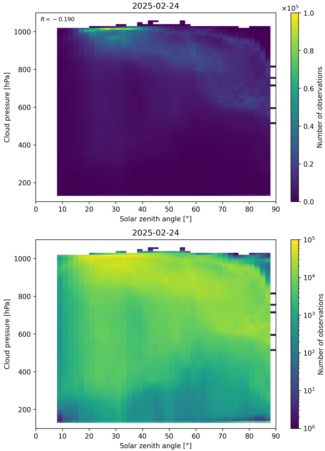
Figure 111: Scatter density plot of “Solar zenith angle” against “Cloud pressure” for 2025-02-24 to 2025-02-25.
