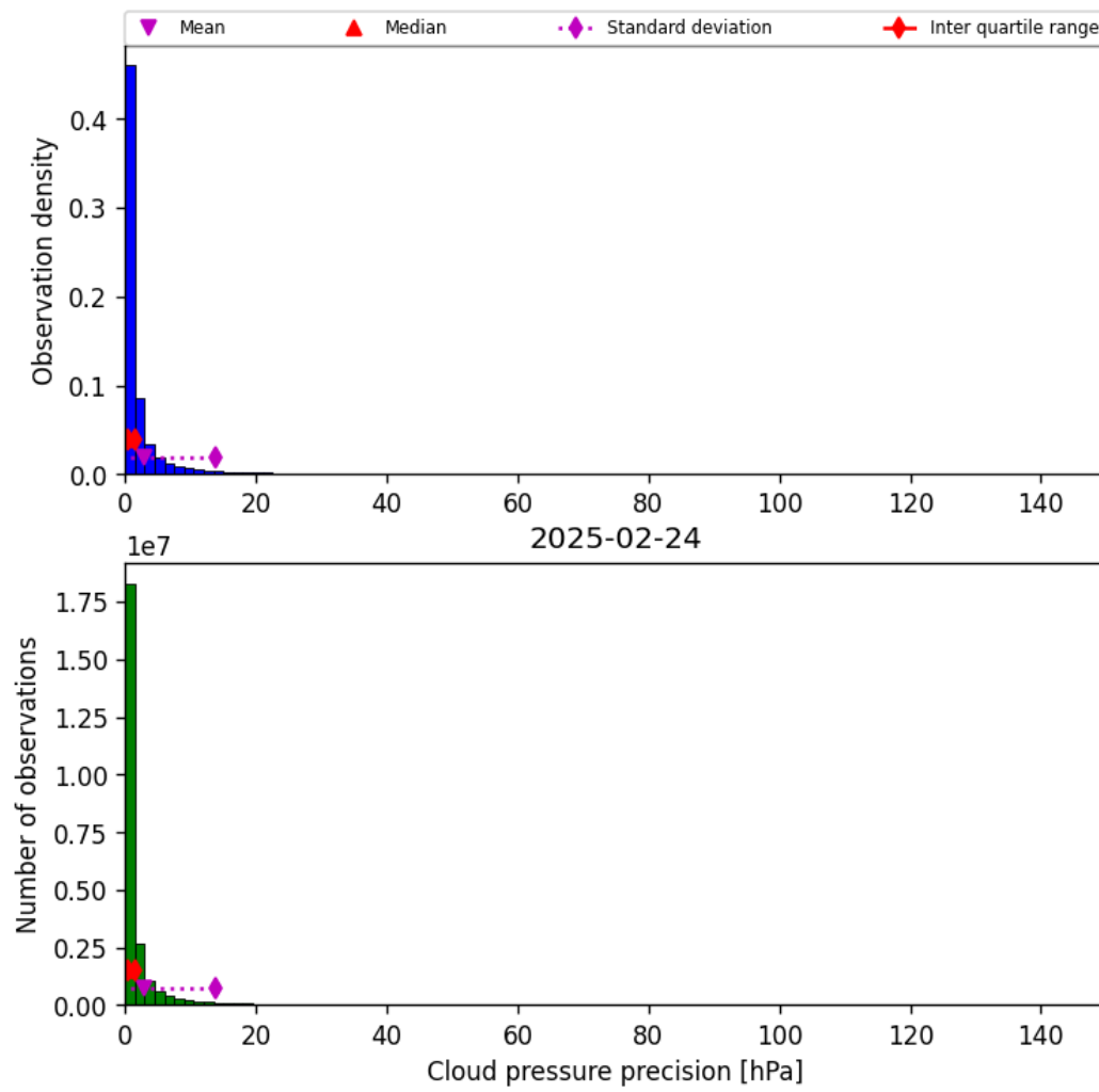
Figure 31: Histogram of “Cloud pressure precision” for 2025-02-24 to 2025-02-25
