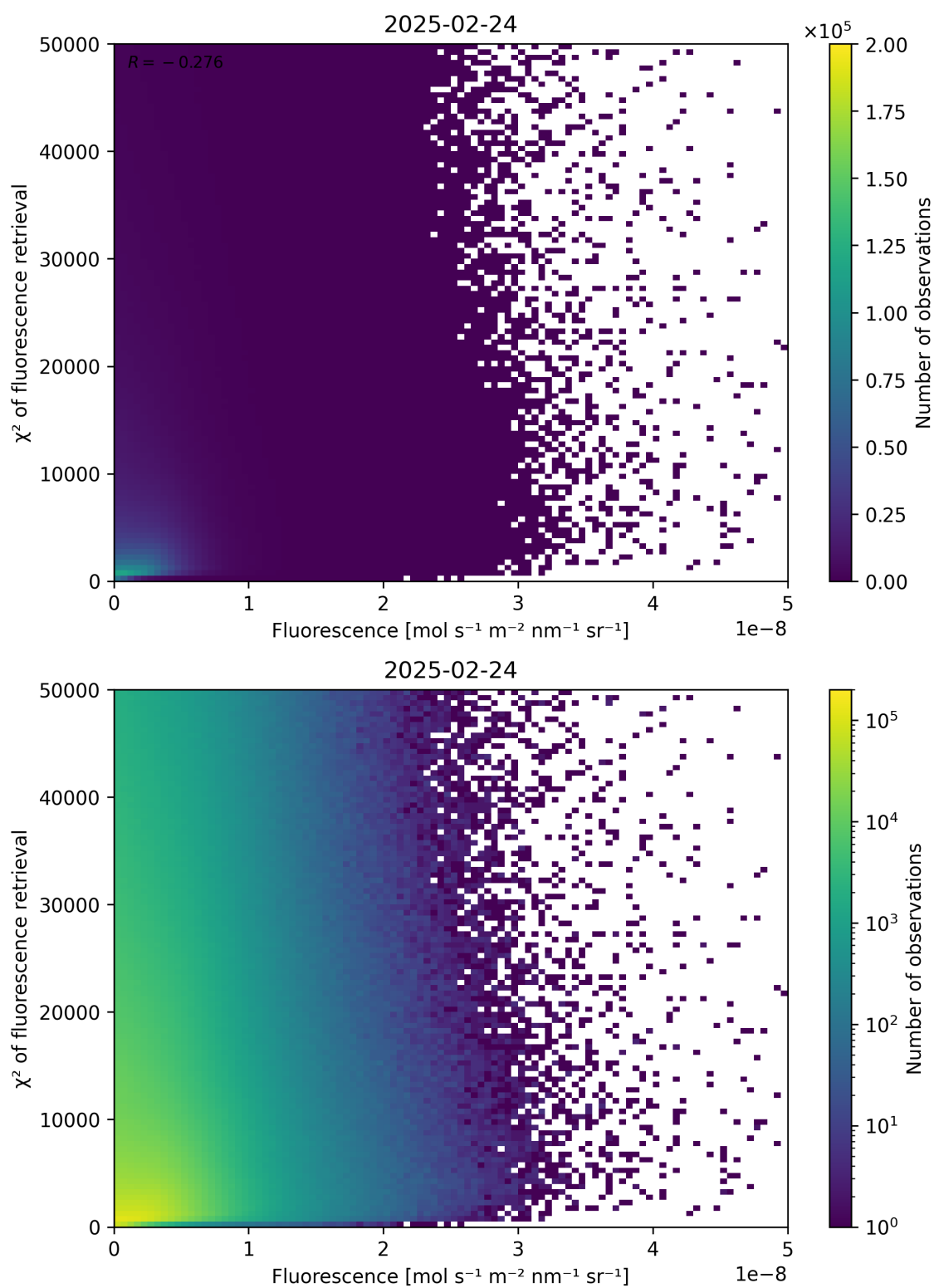
Figure 85: Scatter density plot of “Fluorescence” against “ \chi^2 of fluorescence retrieval” for 2025-02-24 to 2025-02-25.
