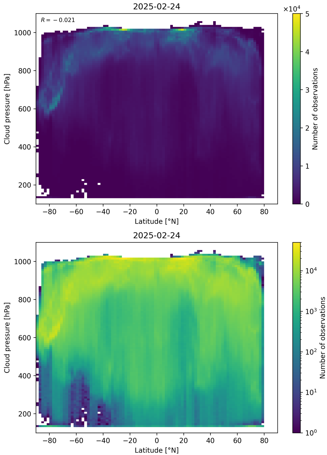
Figure 91: Scatter density plot of “Latitude” against “Cloud pressure” for 2025-02-24 to 2025-02-25.
