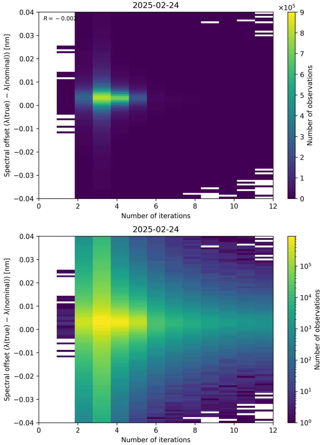
Figure 100: Scatter density plot of “Number of iterations” against “Spectral offset ( \lambda_{\text{true}} - \lambda_{\text{nominal}} )” for 2025-02-24 to 2025-02-25.
