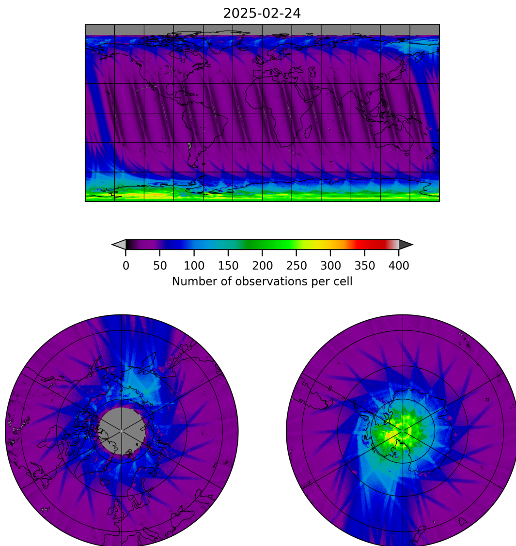
Figure 11: Map of the number of observations for 2025-02-24 to 2025-02-25
