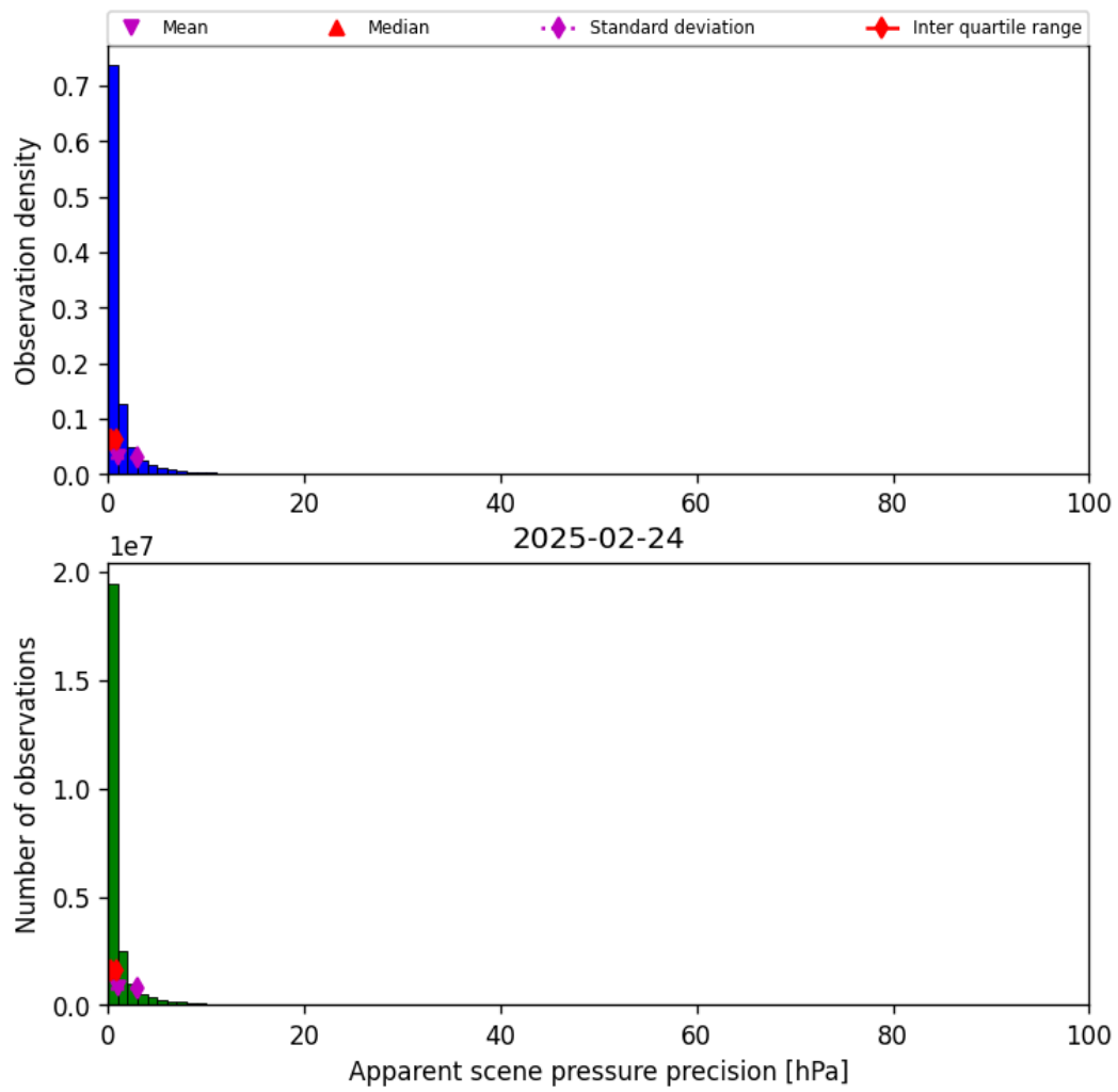
Figure 37: Histogram of “Apparent scene pressure precision” for 2025-02-24 to 2025-02-25
