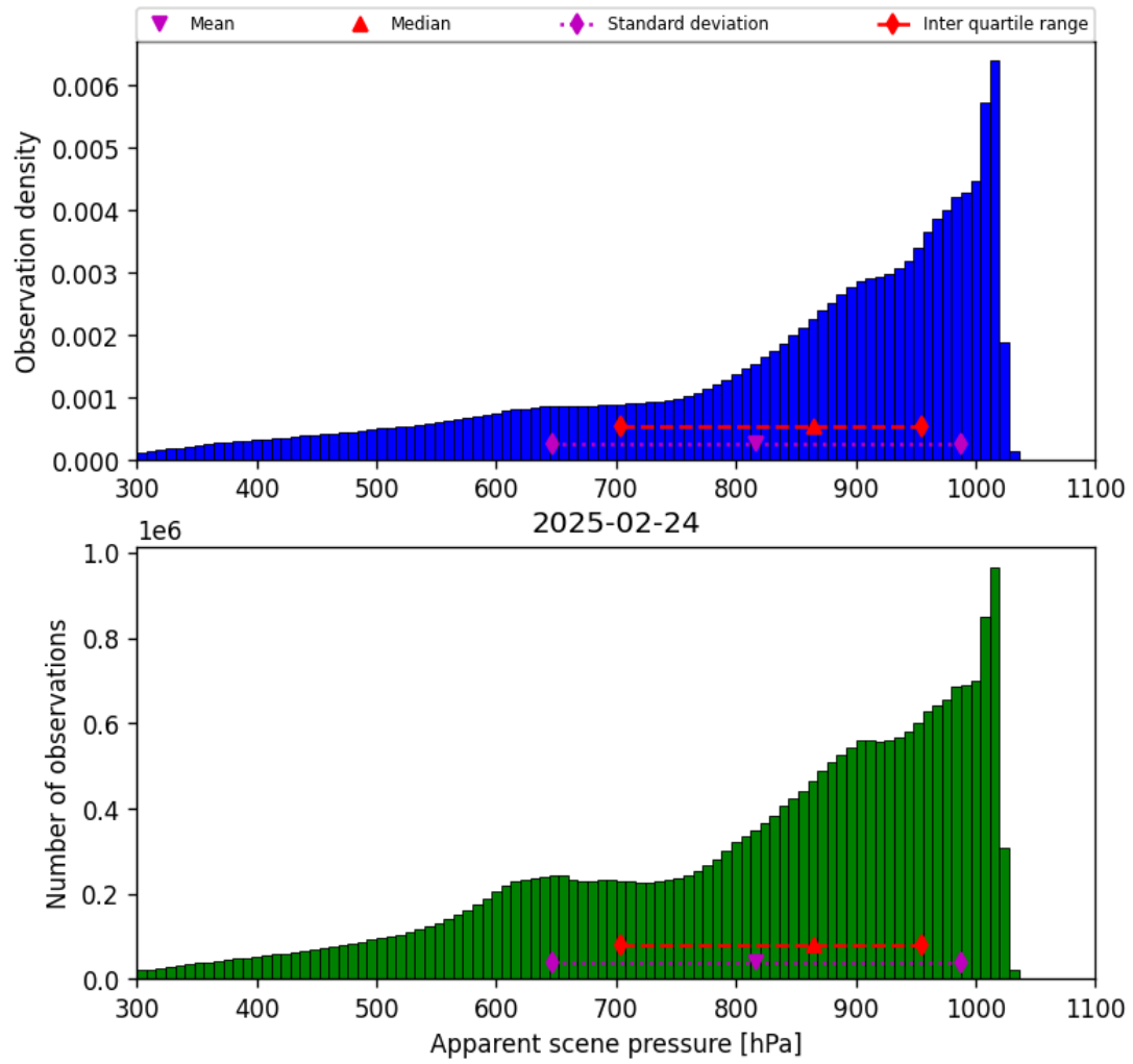
Figure 36: Histogram of “Apparent scene pressure” for 2025-02-24 to 2025-02-25
