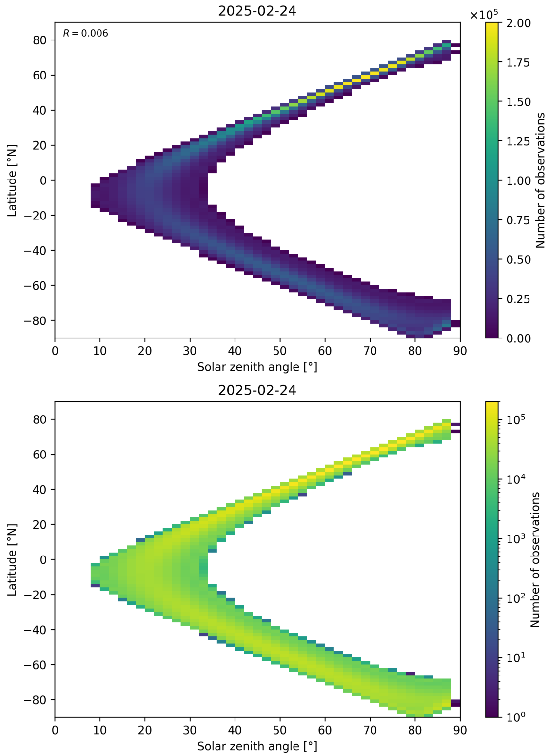
Figure 113: Scatter density plot of “Solar zenith angle” against “Latitude” for 2025-02-24 to 2025-02-25.
