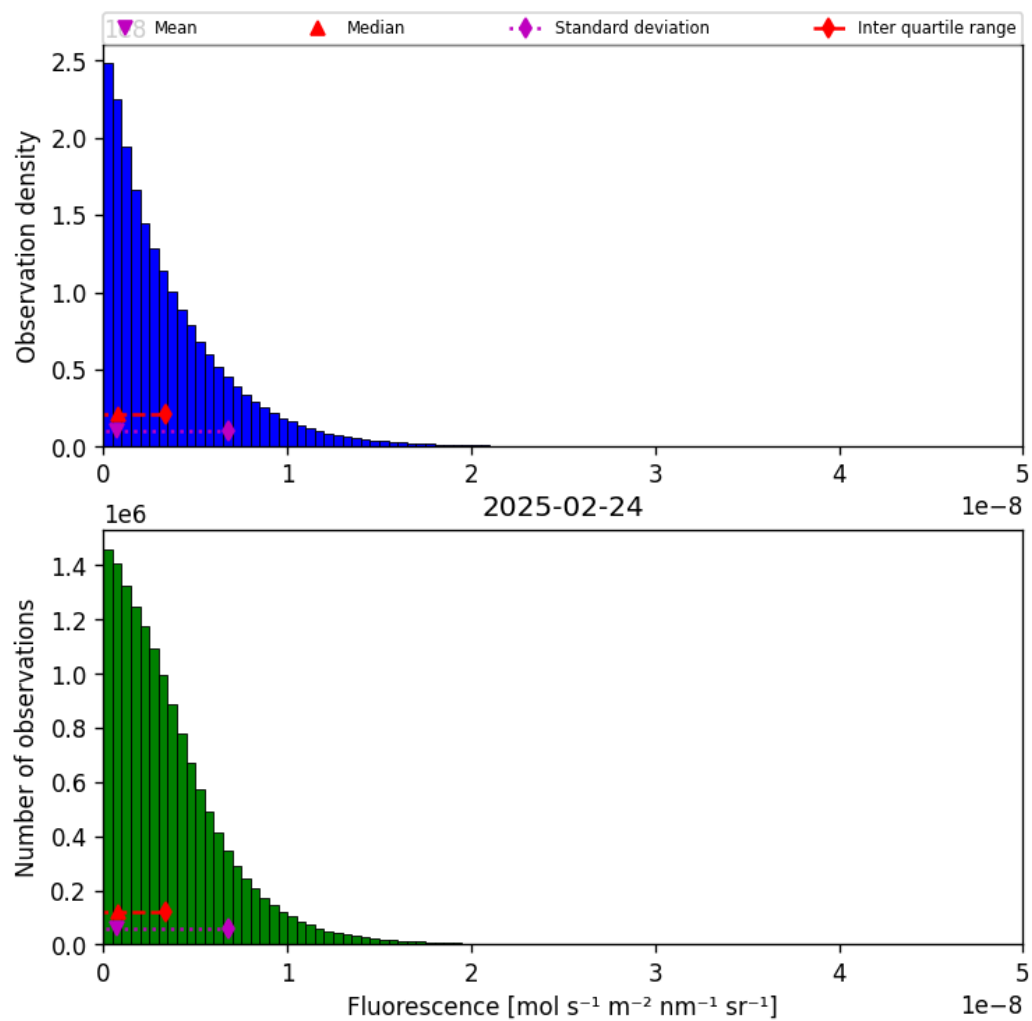
Figure 40: Histogram of “Fluorescence” for 2025-02-24 to 2025-02-25
