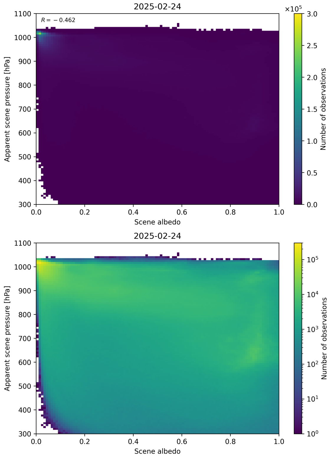
Figure 102: Scatter density plot of “Scene albedo” against “Apparent scene pressure” for 2025-02-24 to 2025-02-25.
