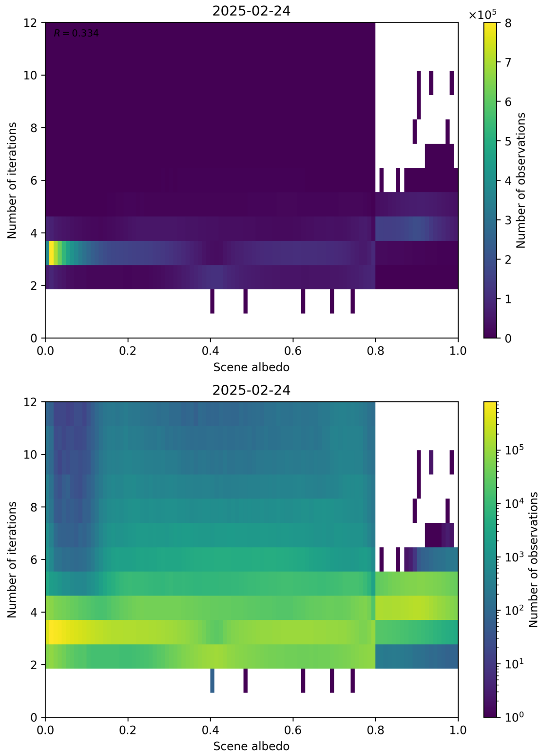
Figure 105: Scatter density plot of “Scene albedo” against “Number of iterations” for 2025-02-24 to 2025-02-25.
