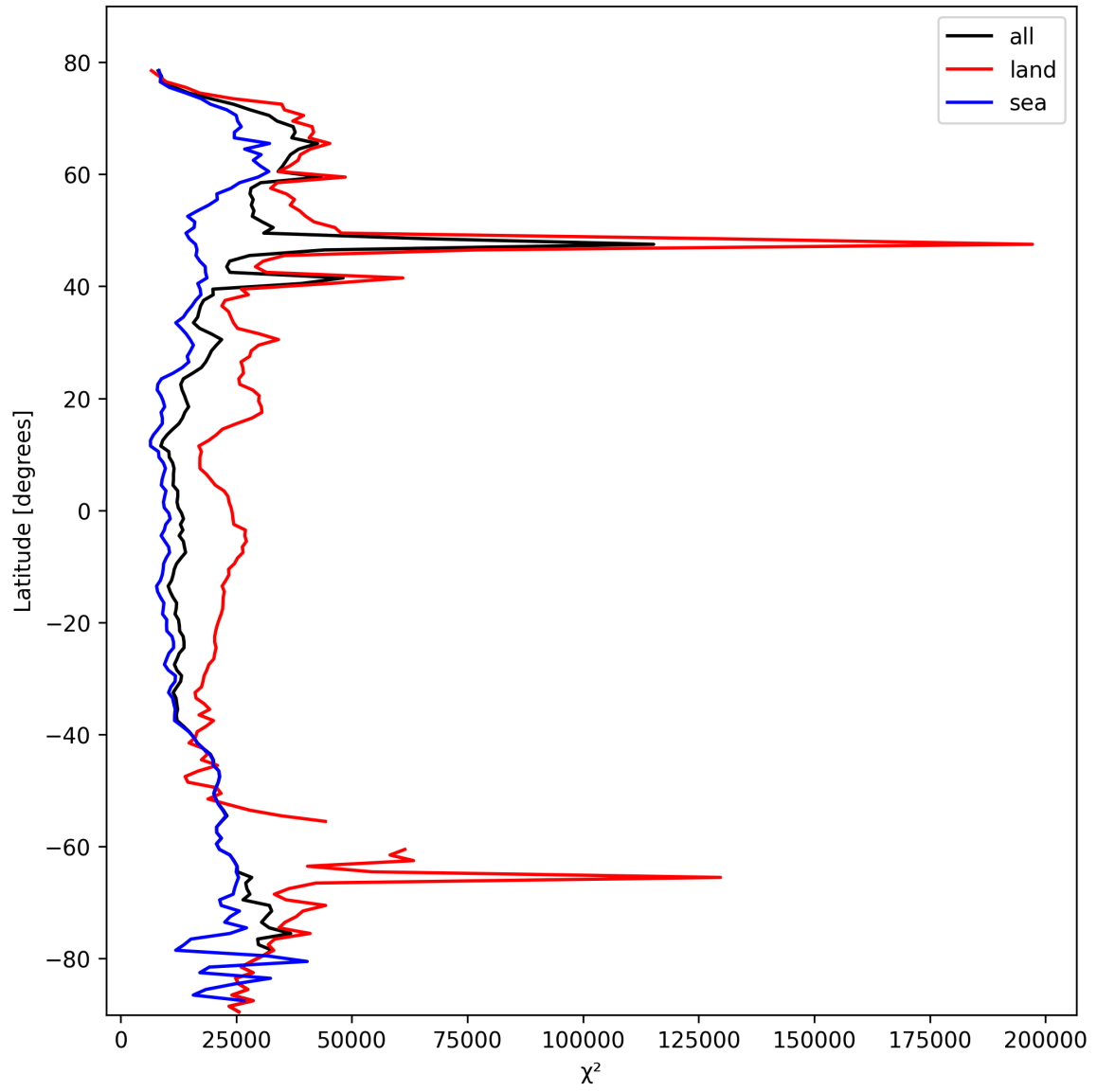
Figure 21: Zonal average of “ \chi^2 ” for 2025-02-24 to 2025-02-25.
