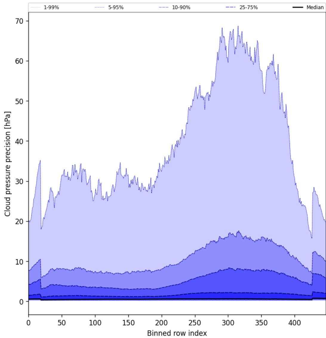
Figure 48: Along track statistics of “Cloud pressure precision” for 2025-02-24 to 2025-02-25
