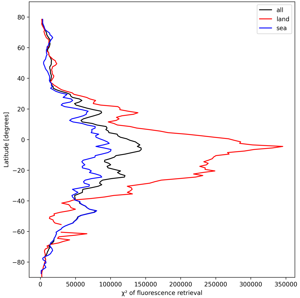
Figure 25: Zonal average of “ \chi^2 of fluorescence retrieval” for 2025-02-24 to 2025-02-25.
