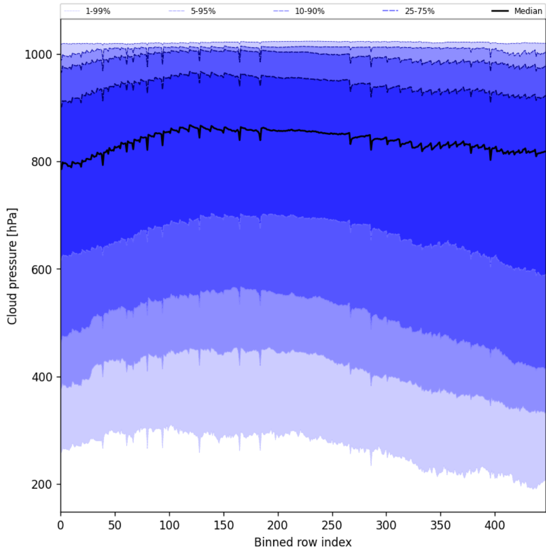
Figure 47: Along track statistics of “Cloud pressure” for 2025-02-24 to 2025-02-25
