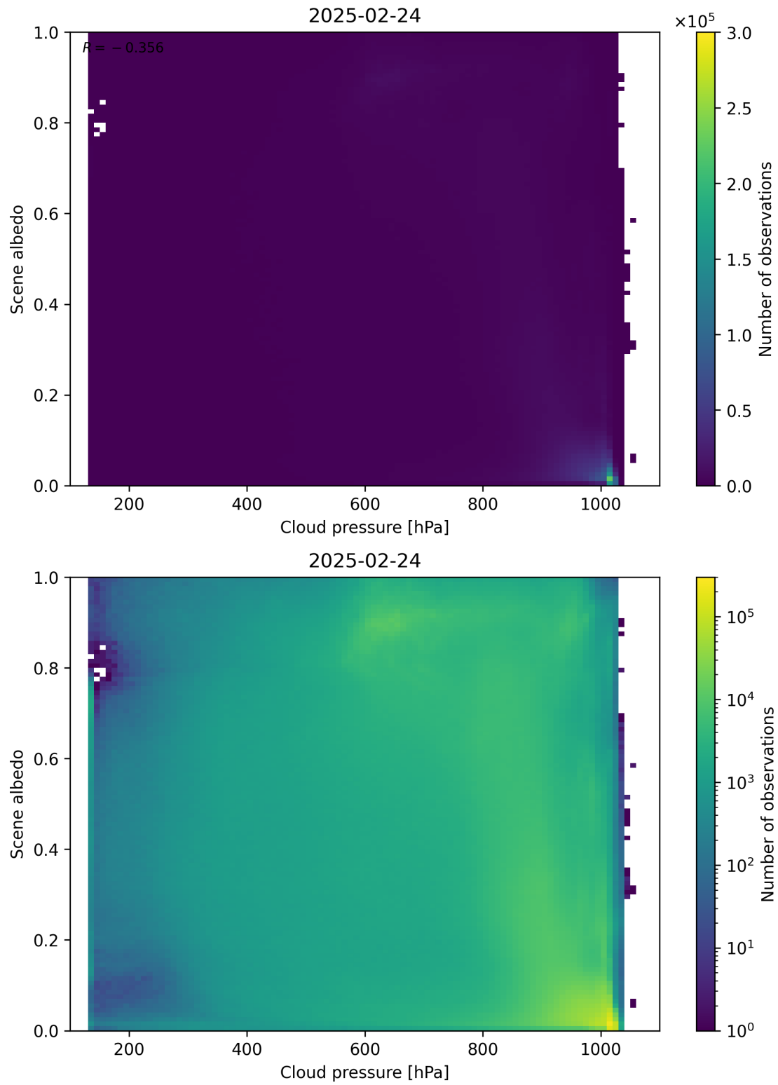
Figure 83: Scatter density plot of “Cloud pressure” against “Scene albedo” for 2025-02-24 to 2025-02-25.
