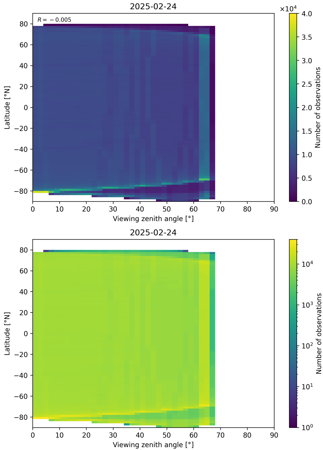
Figure 123: Scatter density plot of “Viewing zenith angle” against “Latitude” for 2025-02-24 to 2025-02-25.
