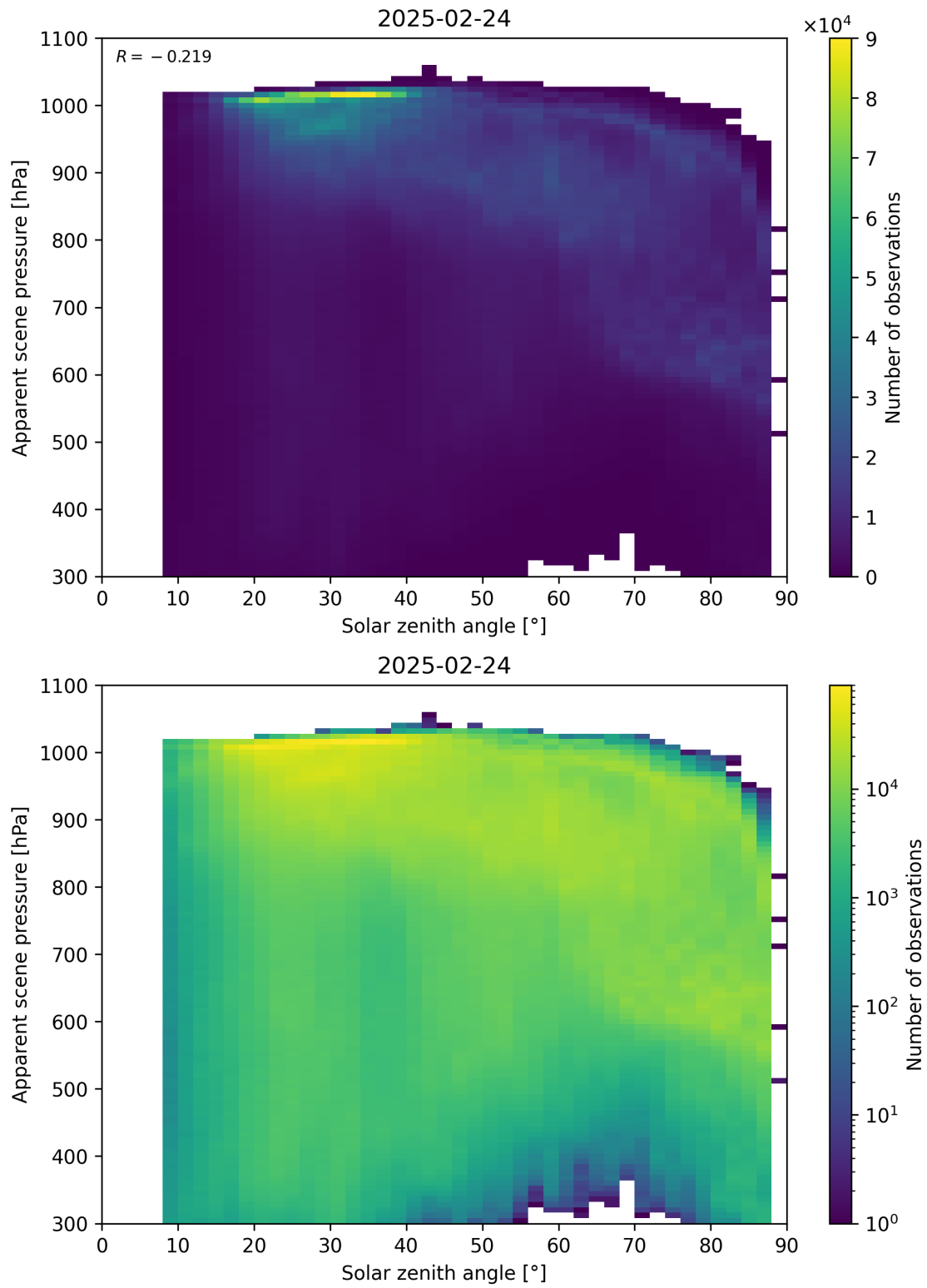
Figure 108: Scatter density plot of “Solar zenith angle” against “Apparent scene pressure” for 2025-02-24 to 2025-02-25.
