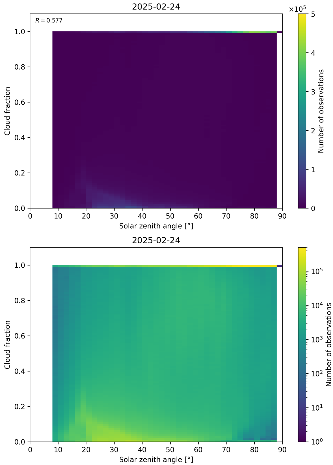
Figure 110: Scatter density plot of “Solar zenith angle” against “Cloud fraction” for 2025-02-24 to 2025-02-25.
