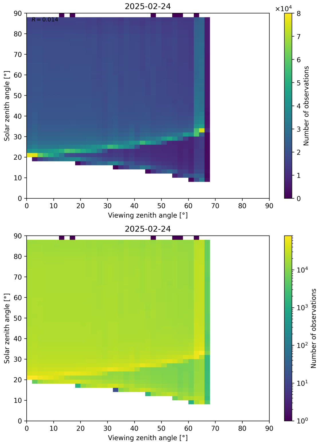
Figure 127: Scatter density plot of “Viewing zenith angle” against “Solar zenith angle” for 2025-02-24 to 2025-02-25.
