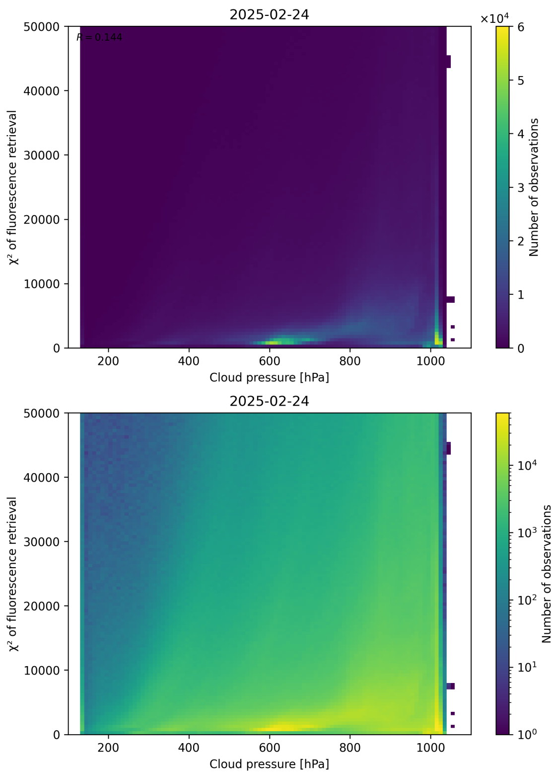
Figure 78: Scatter density plot of “Cloud pressure” against “ \chi^2 of fluorescence retrieval” for 2025-02-24 to 2025-02-25.
