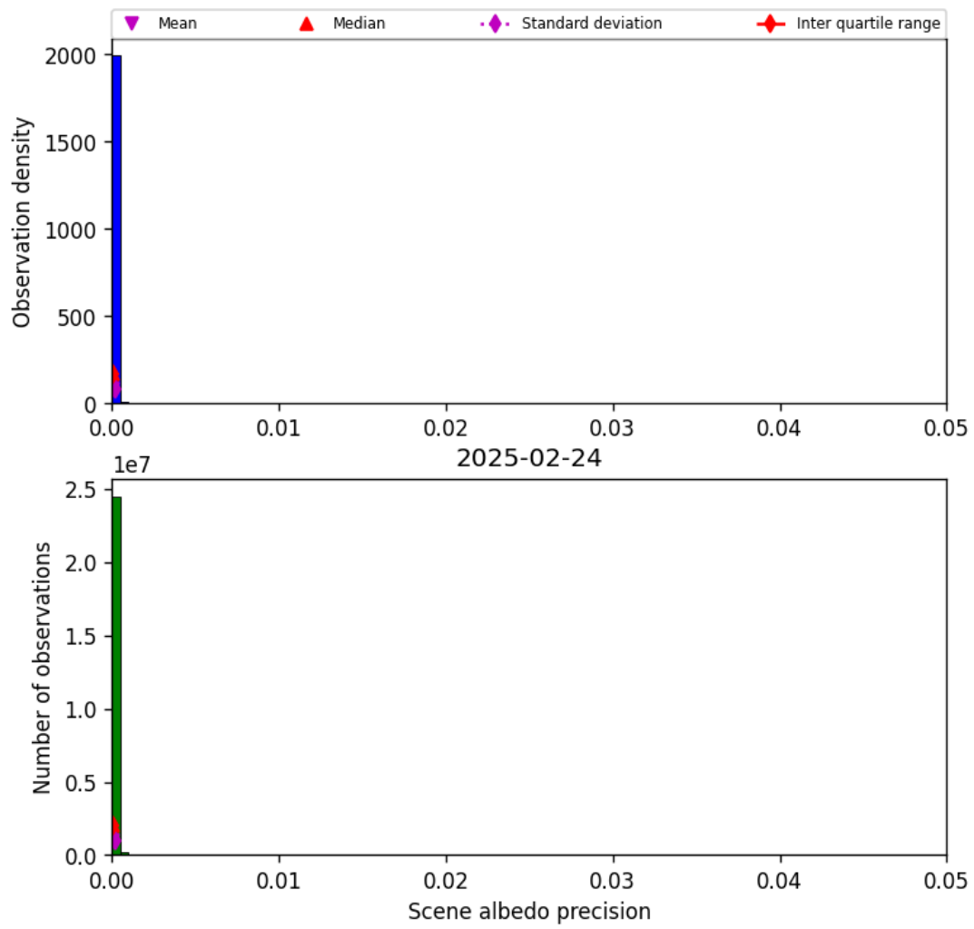
Figure 35: Histogram of “Scene albedo precision” for 2025-02-24 to 2025-02-25
