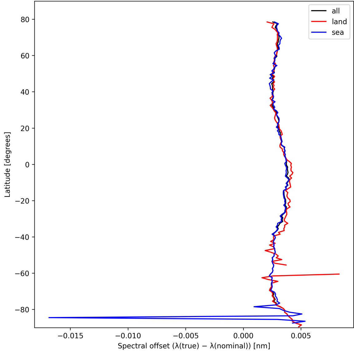
Figure 28: Zonal average of “Spectral offset ( \lambda_{\text{true}} - \lambda_{\text{nominal}} )” for 2025-02-24 to 2025-02-25.
