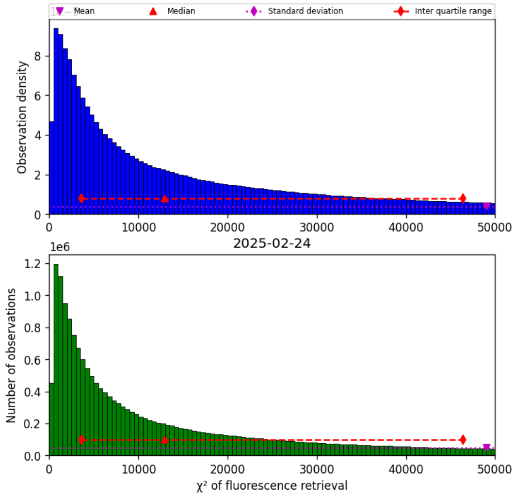
Figure 42: Histogram of “ \chi^2 of fluorescence retrieval” for 2025-02-24 to 2025-02-25
