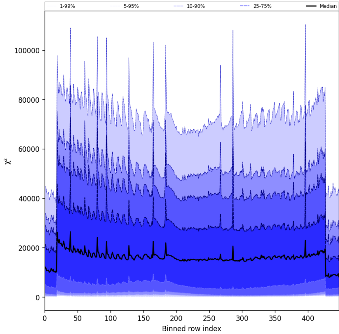
Figure 55: Along track statistics of “ \chi^2 ” for 2025-02-24 to 2025-02-25
