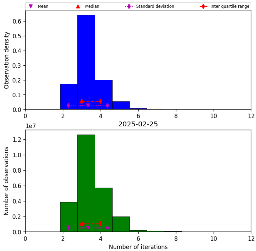
Figure 39: Histogram of “Number of iterations” for 2025-02-24 to 2025-02-26
