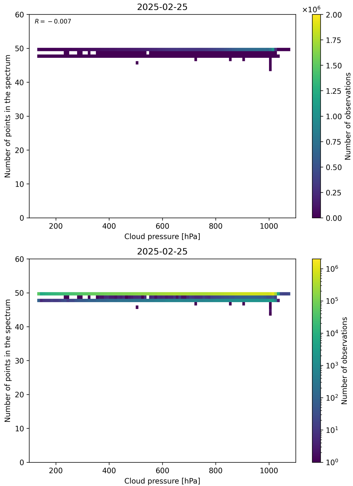
Figure 82: Scatter density plot of “Cloud pressure” against “Number of points in the spectrum” for 2025-02-24 to 2025-02-26.
