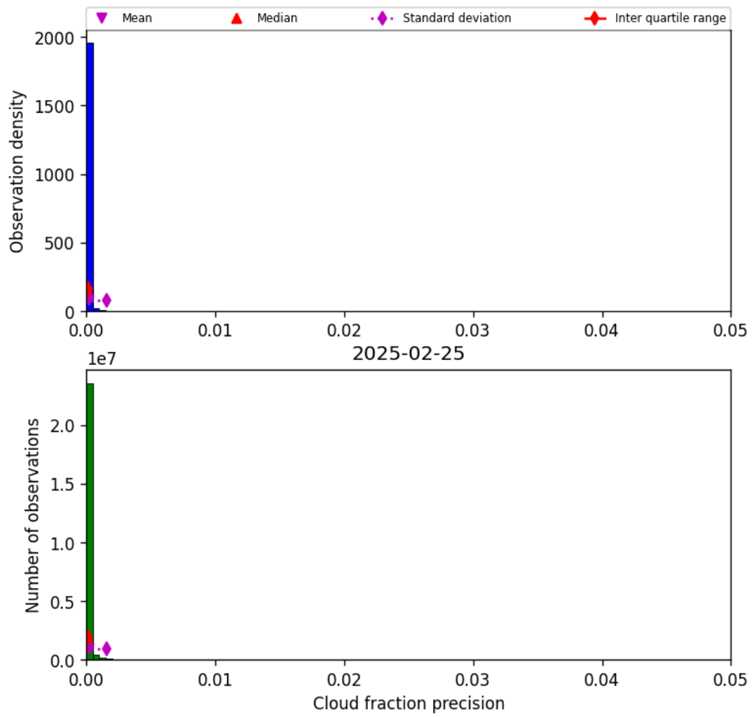
Figure 33: Histogram of “Cloud fraction precision” for 2025-02-24 to 2025-02-26
