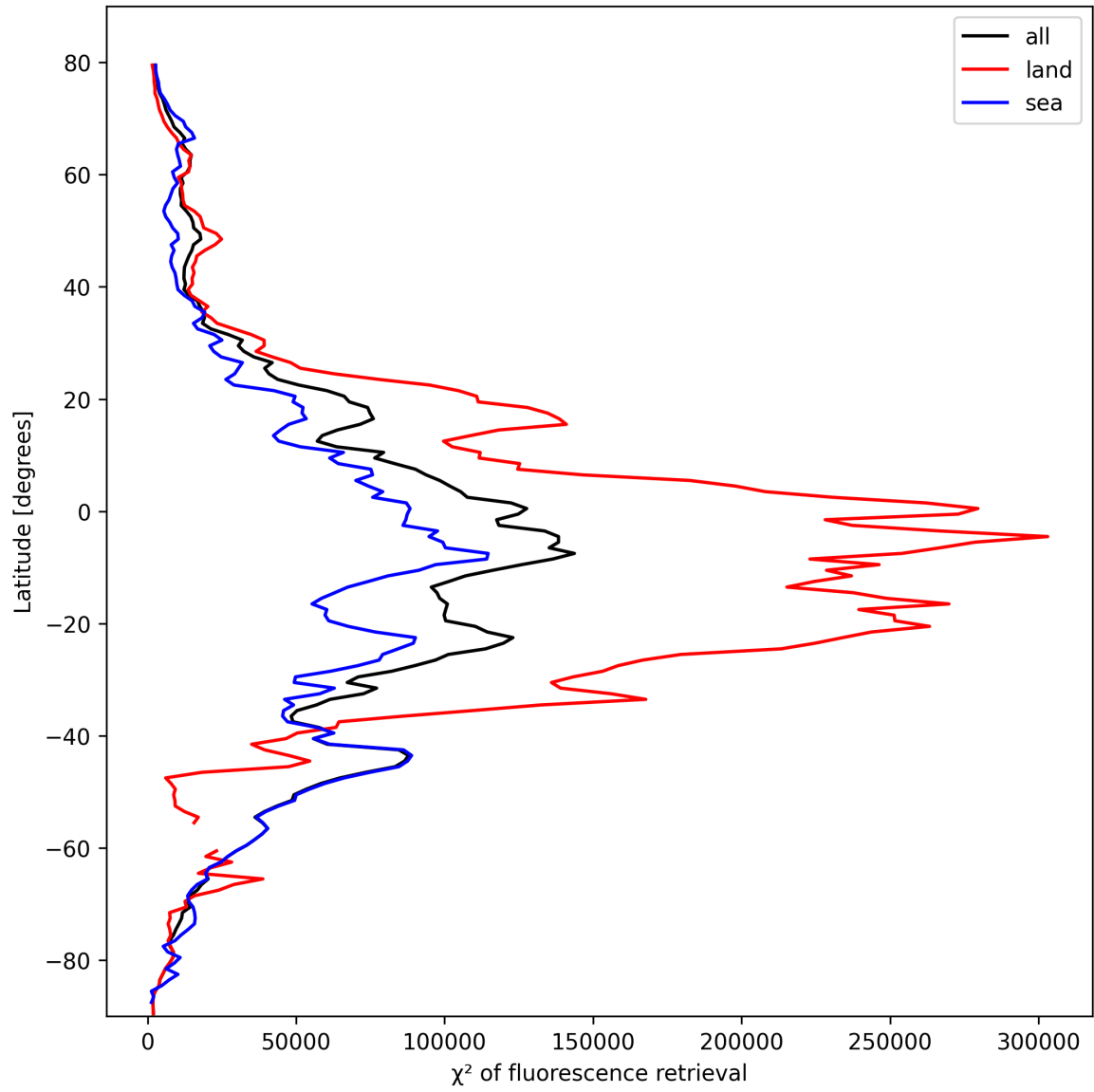
Figure 25: Zonal average of “ \chi^2 of fluorescence retrieval” for 2025-02-24 to 2025-02-26.
