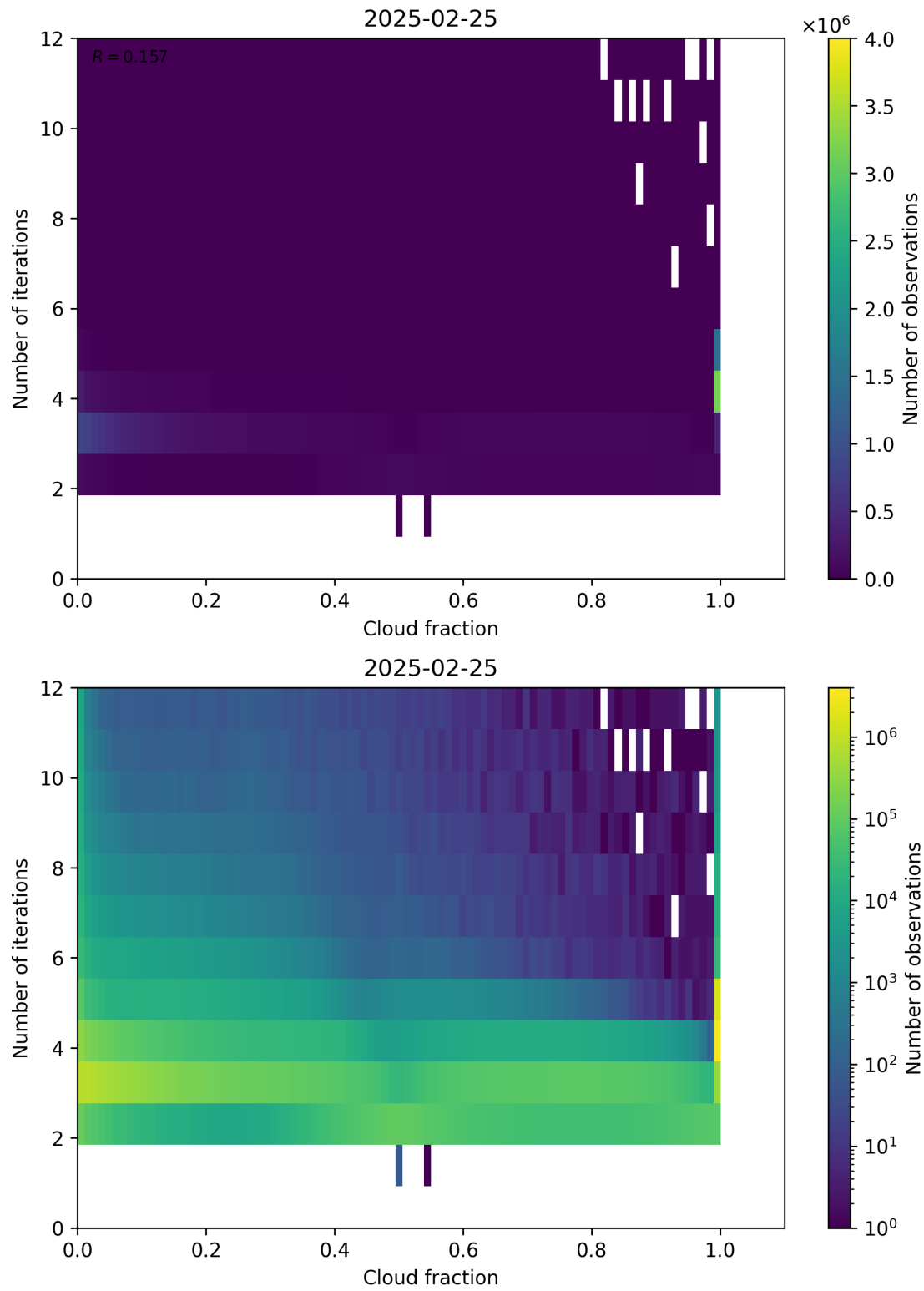
Figure 73: Scatter density plot of “Cloud fraction” against “Number of iterations” for 2025-02-24 to 2025-02-26.
