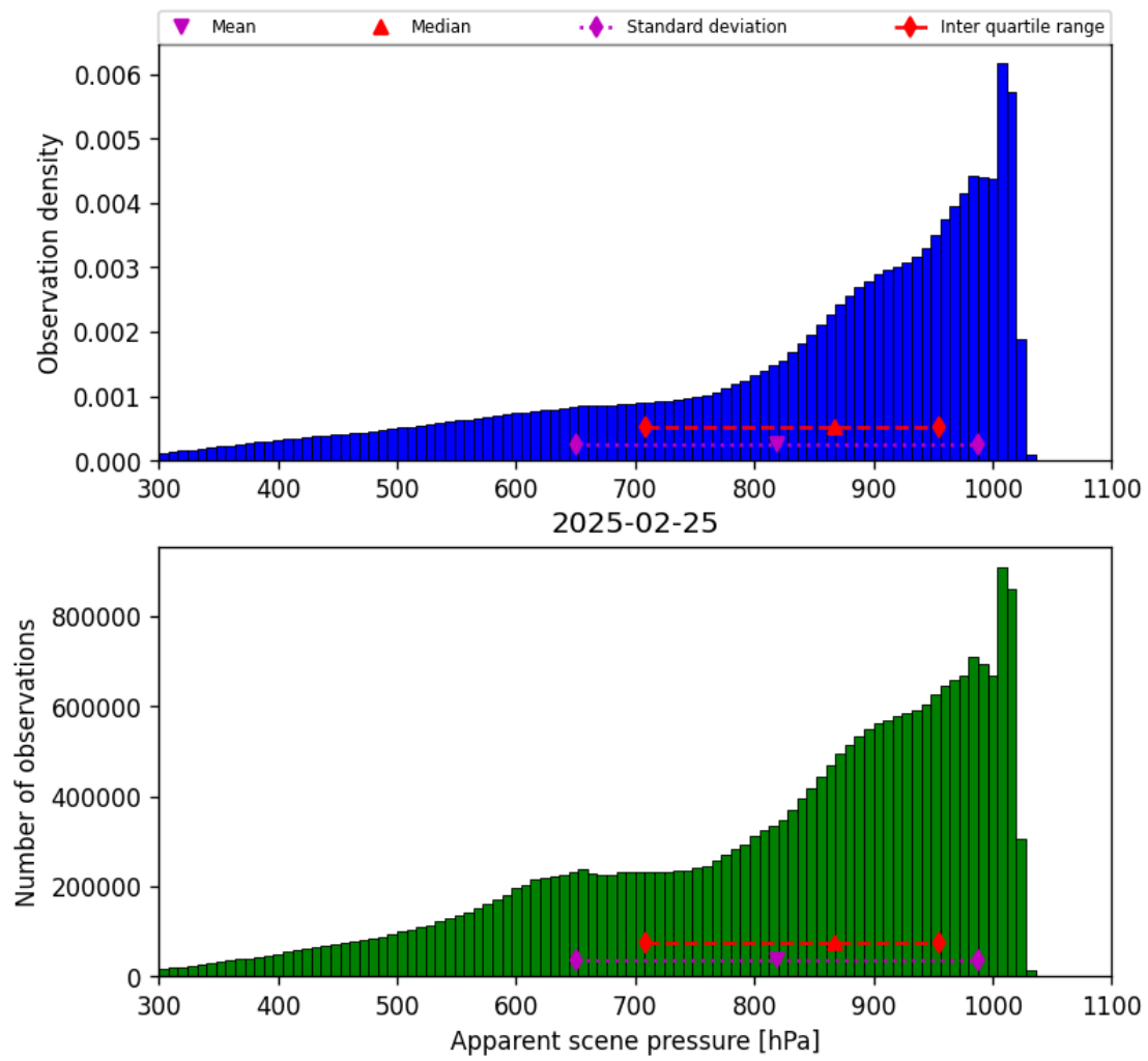
Figure 36: Histogram of “Apparent scene pressure” for 2025-02-24 to 2025-02-26
