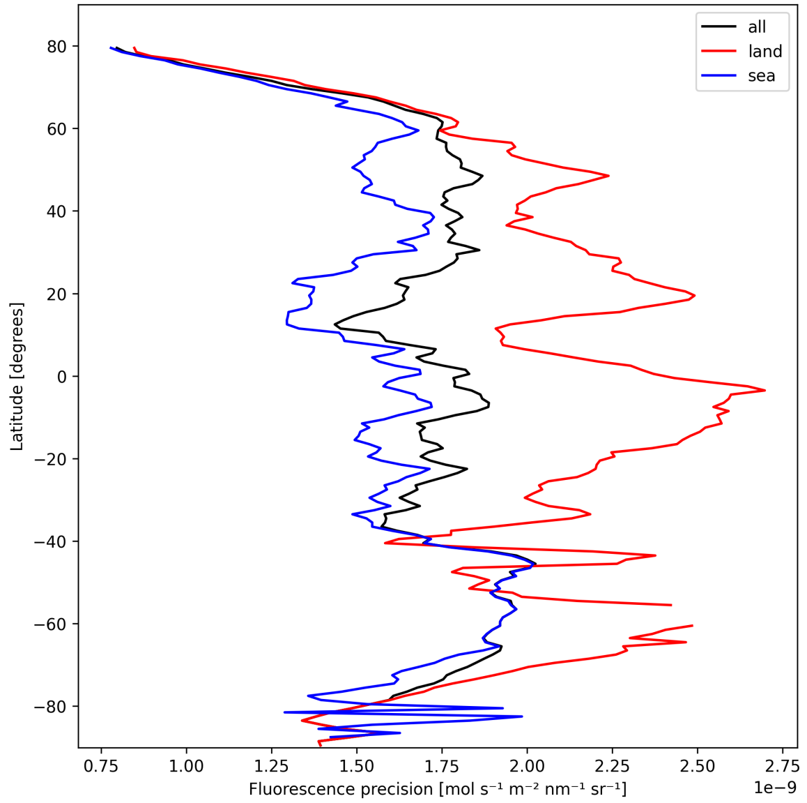
Figure 24: Zonal average of “Fluorescence precision” for 2025-02-24 to 2025-02-26.
