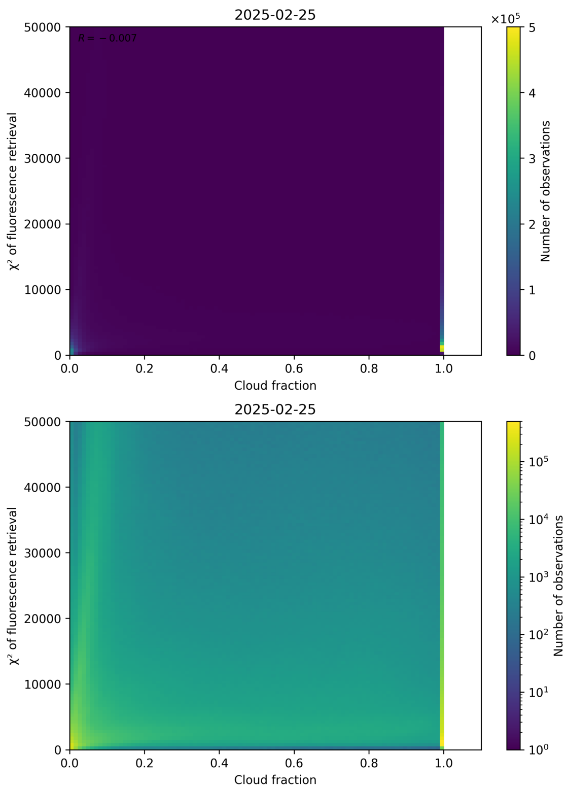
Figure 71: Scatter density plot of “Cloud fraction” against “ \chi^2 of fluorescence retrieval” for 2025-02-24 to 2025-02-26.
