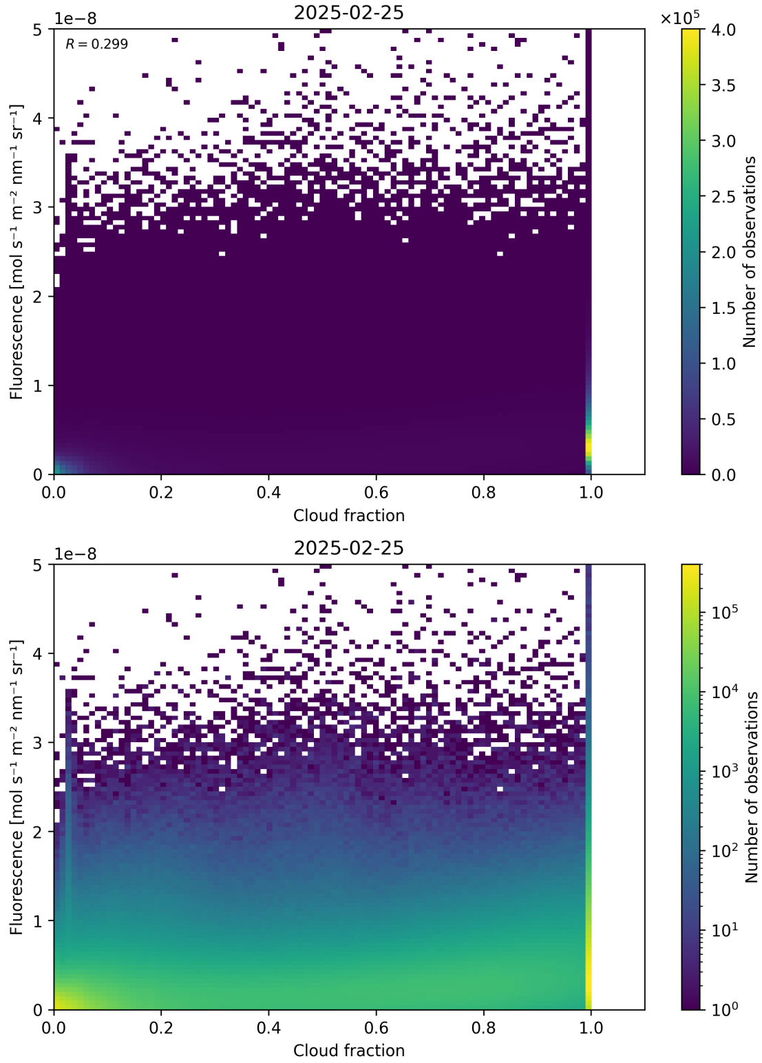
Figure 72: Scatter density plot of “Cloud fraction” against “Fluorescence” for 2025-02-24 to 2025-02-26.
