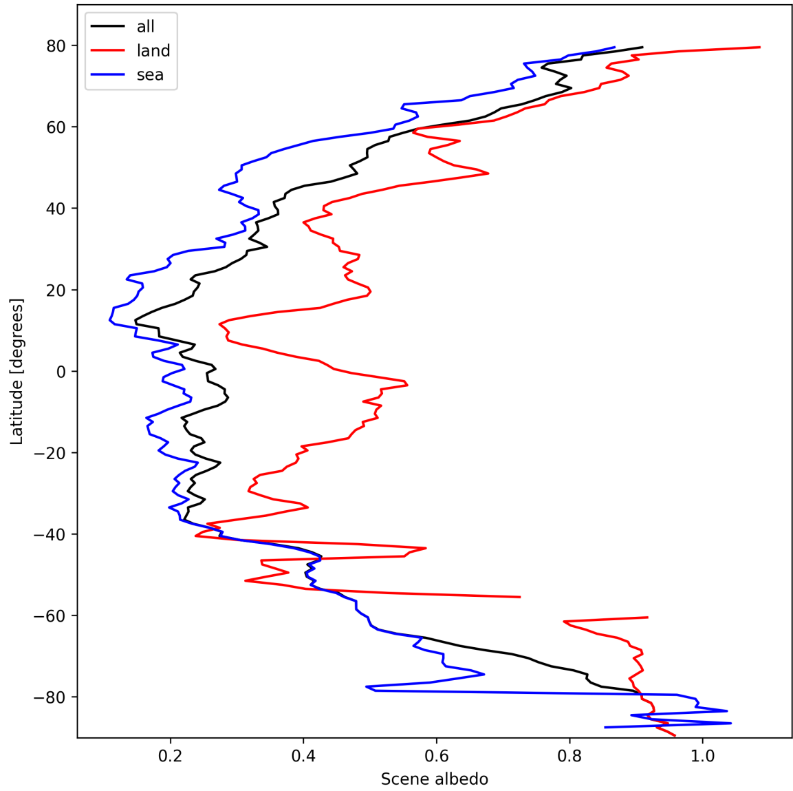
Figure 17: Zonal average of “Scene albedo” for 2025-02-24 to 2025-02-26.
