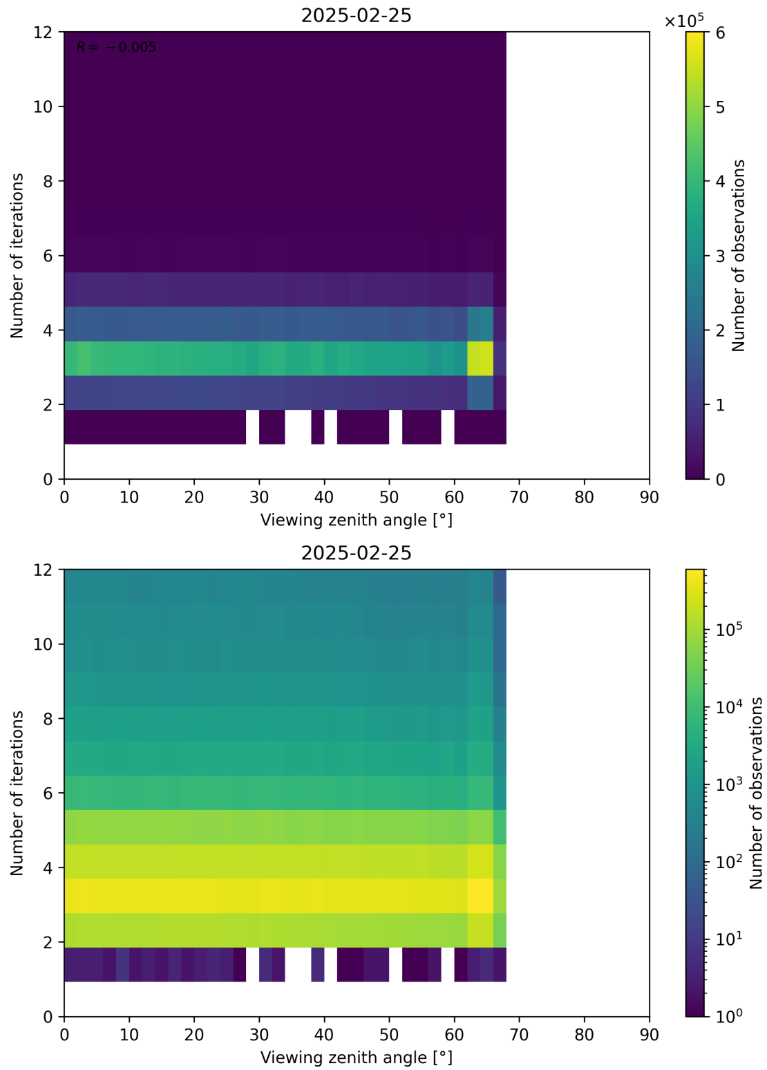
Figure 124: Scatter density plot of “Viewing zenith angle” against “Number of iterations” for 2025-02-24 to 2025-02-26.
