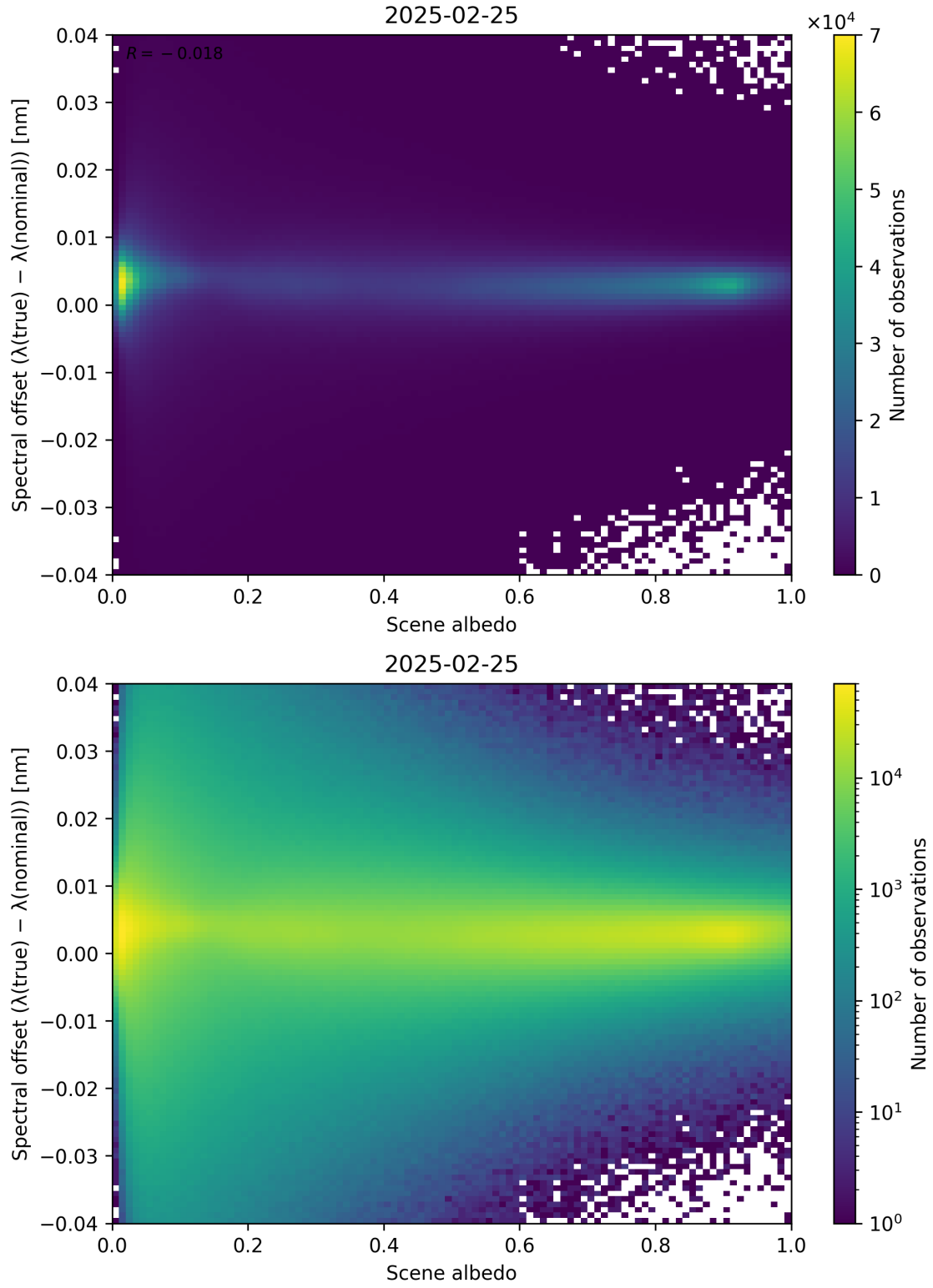
Figure 107: Scatter density plot of “Scene albedo” against “Spectral offset ( \lambda_{\text{true}} - \lambda_{\text{nominal}} )” for 2025-02-24 to 2025-02-26.
