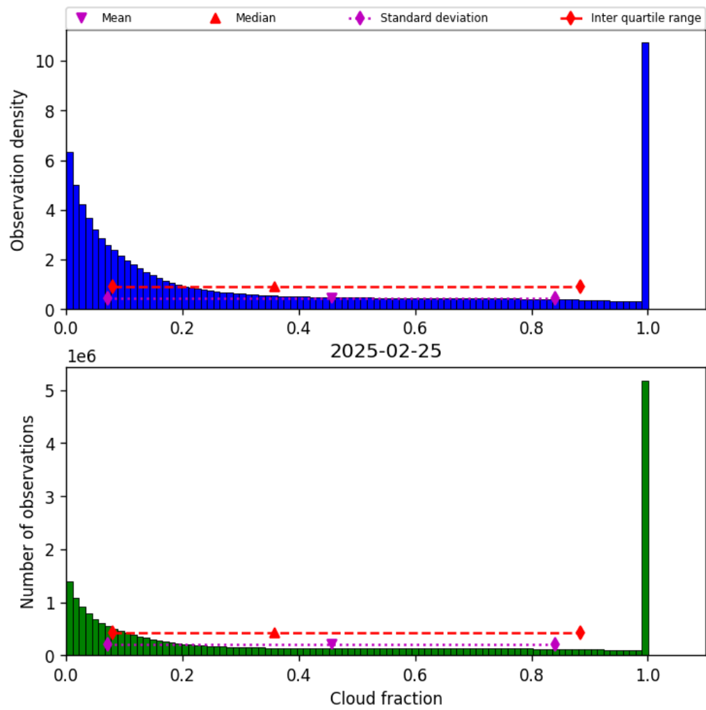
Figure 32: Histogram of “Cloud fraction” for 2025-02-24 to 2025-02-26
