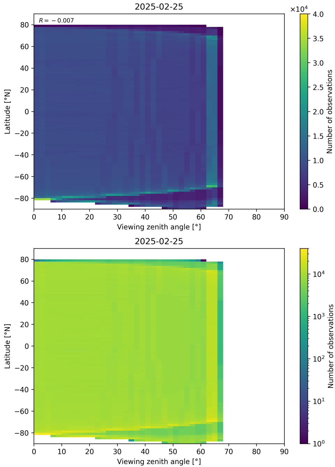
Figure 123: Scatter density plot of “Viewing zenith angle” against “Latitude” for 2025-02-24 to 2025-02-26.
