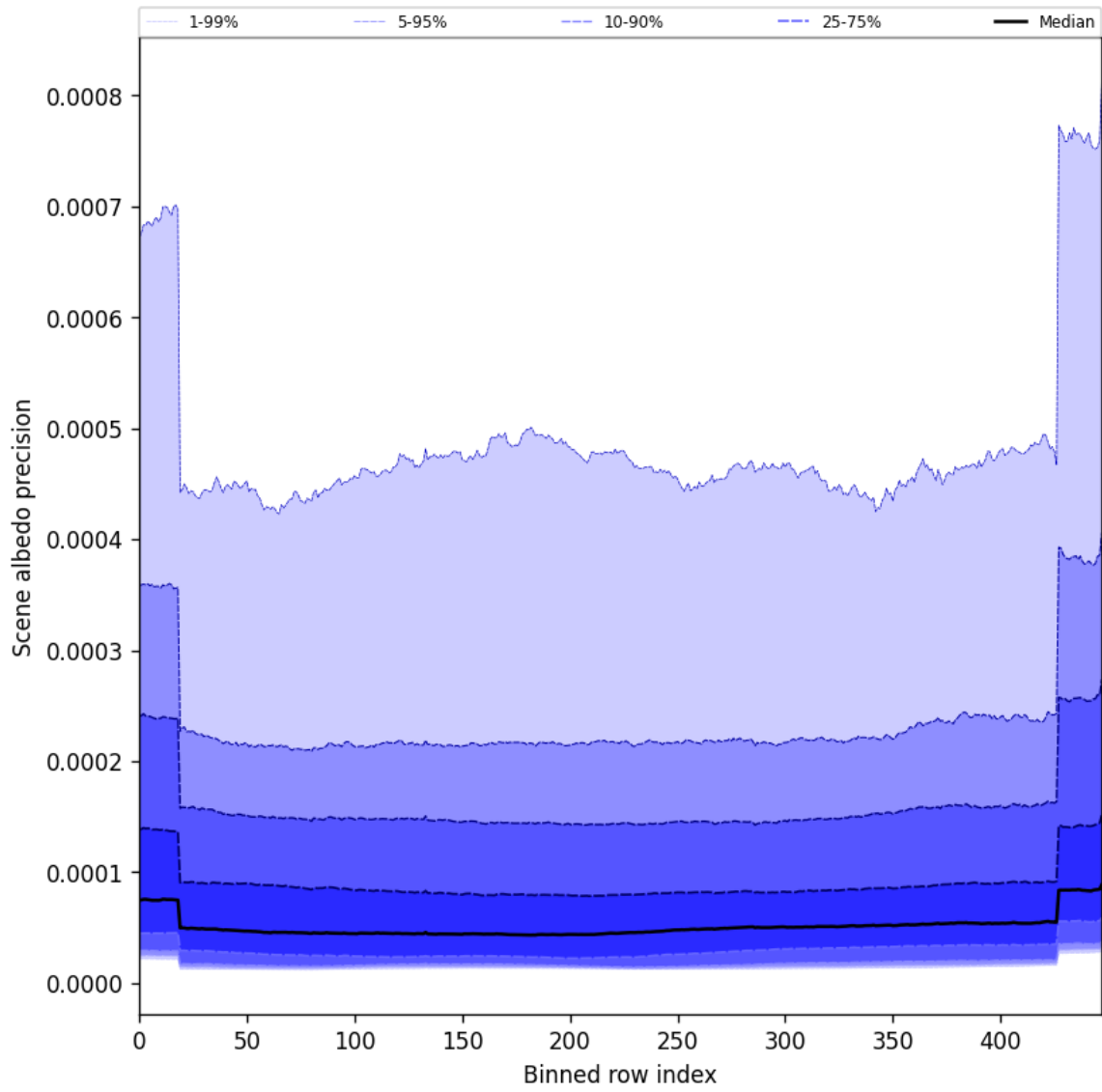
Figure 52: Along track statistics of “Scene albedo precision” for 2025-02-24 to 2025-02-26
