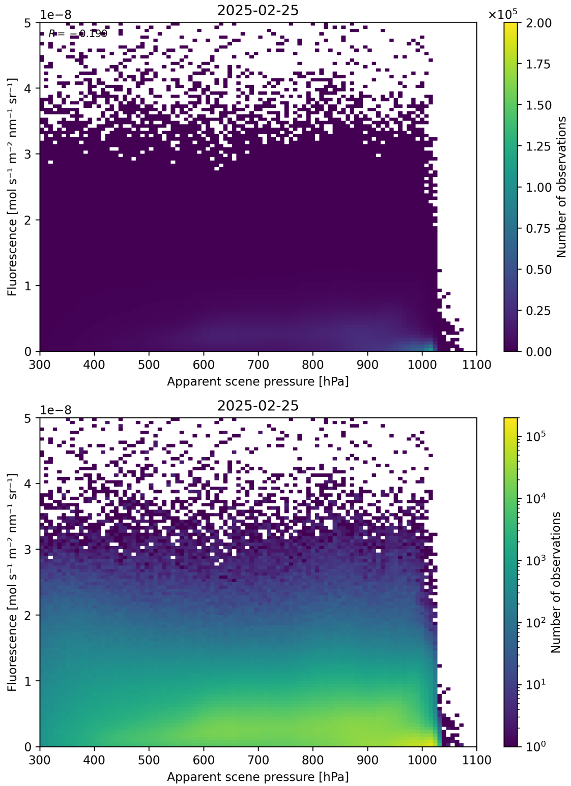
Figure 64: Scatter density plot of “Apparent scene pressure” against “Fluorescence” for 2025-02-24 to 2025-02-26.
