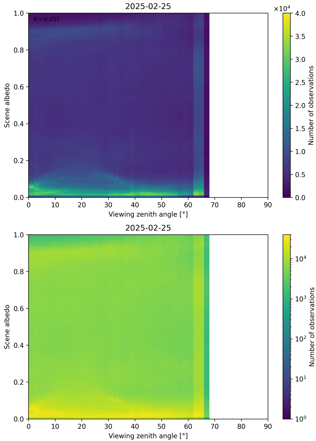
Figure 126: Scatter density plot of “Viewing zenith angle” against “Scene albedo” for 2025-02-24 to 2025-02-26.
