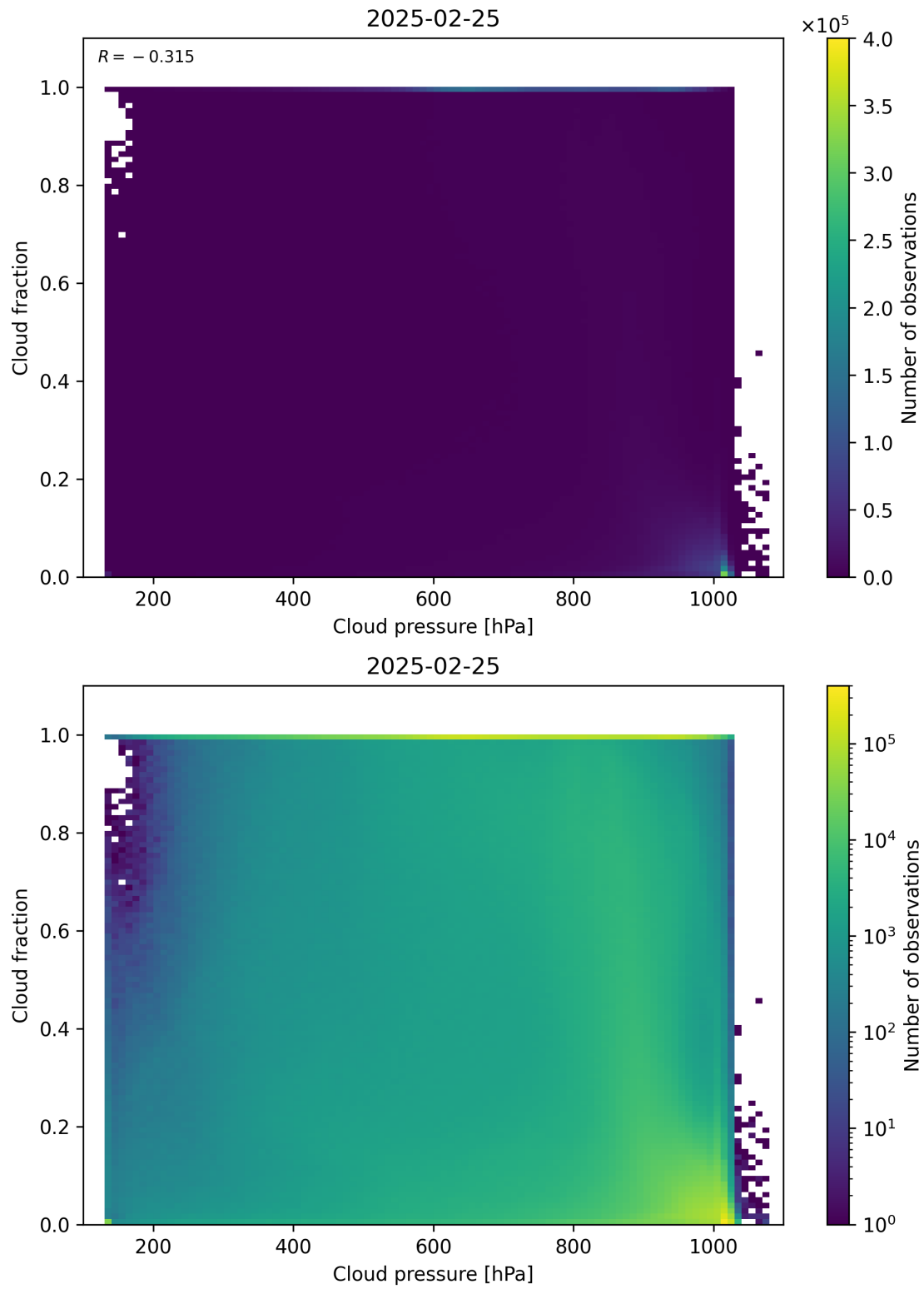
Figure 79: Scatter density plot of “Cloud pressure” against “Cloud fraction” for 2025-02-24 to 2025-02-26.
