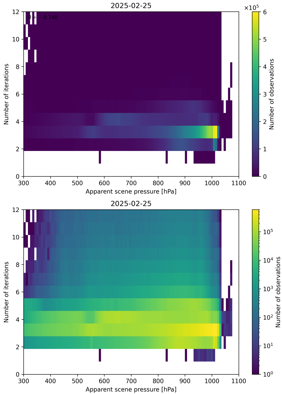
Figure 65: Scatter density plot of “Apparent scene pressure” against “Number of iterations” for 2025-02-24 to 2025-02-26.
