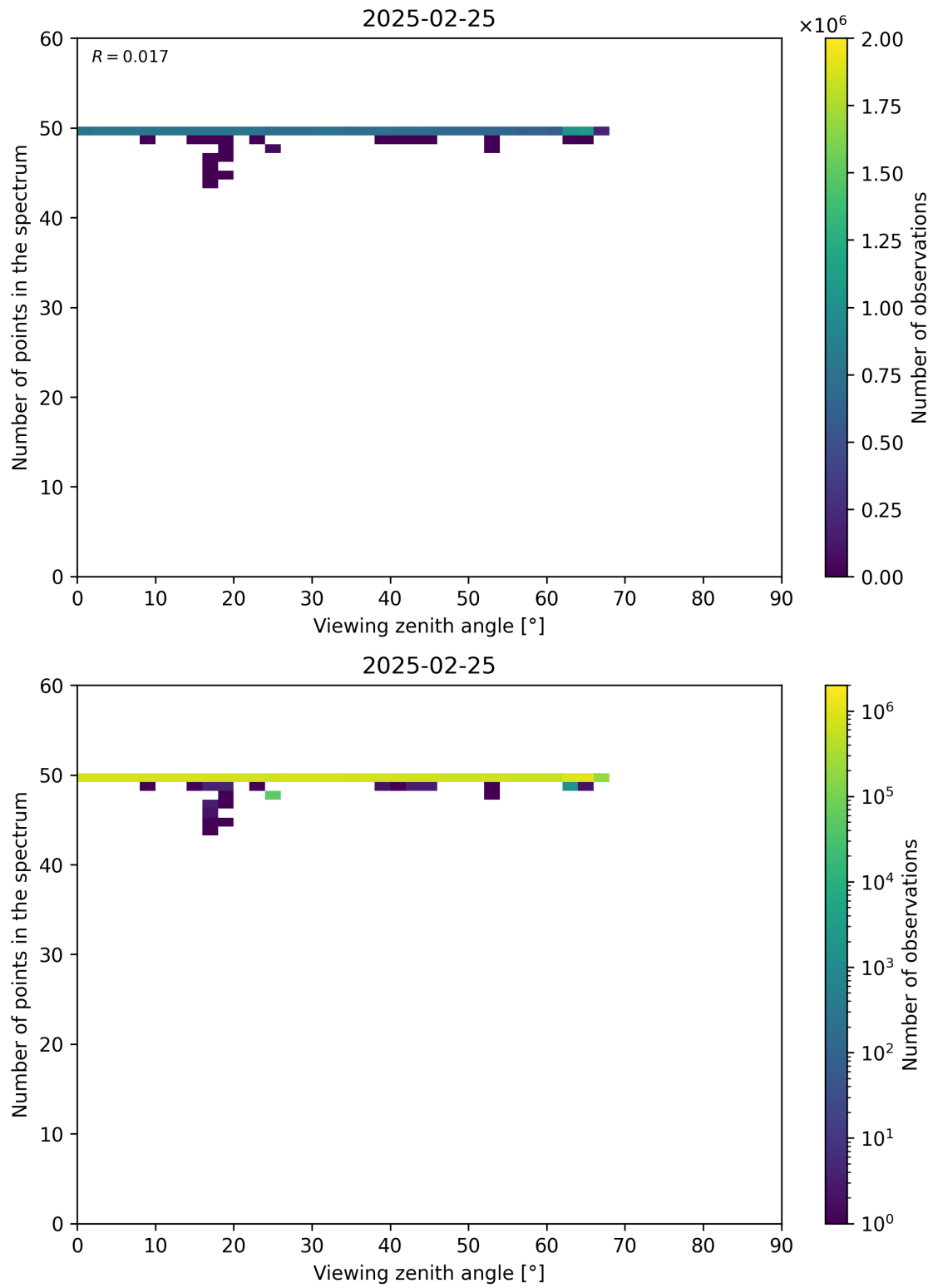
Figure 125: Scatter density plot of “Viewing zenith angle” against “Number of points in the spectrum” for 2025-02-24 to 2025-02-26.
