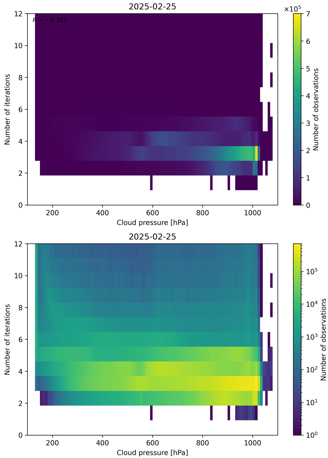
Figure 81: Scatter density plot of “Cloud pressure” against “Number of iterations” for 2025-02-24 to 2025-02-26.
