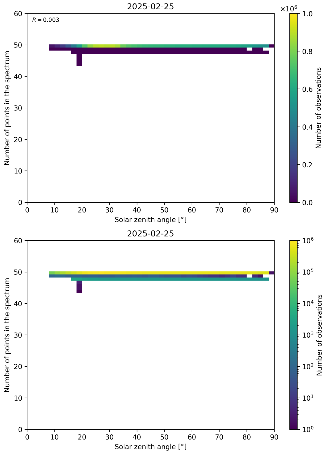
Figure 115: Scatter density plot of “Solar zenith angle” against “Number of points in the spectrum” for 2025-02-24 to 2025-02-26.
