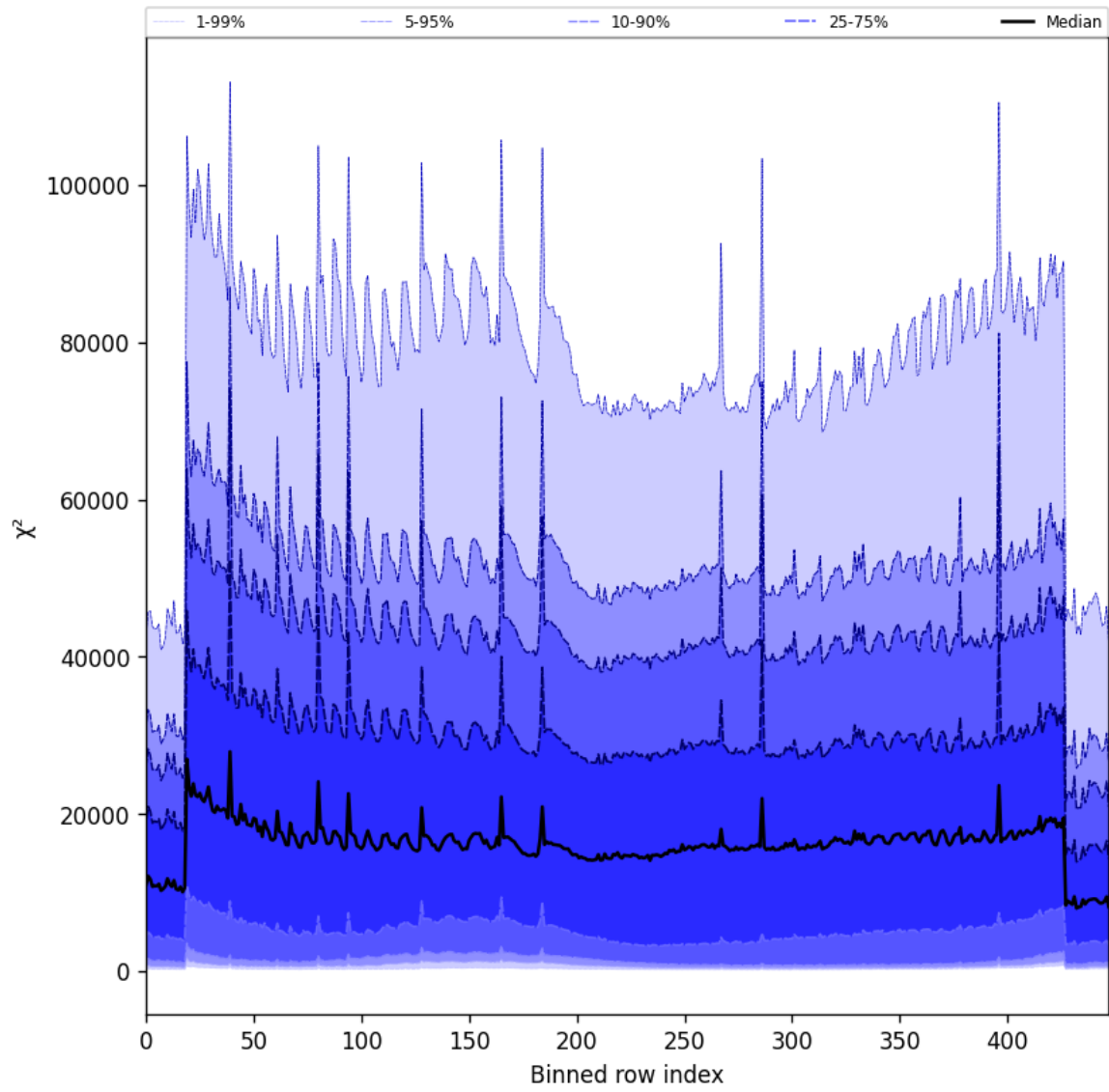
Figure 55: Along track statistics of “ \chi^2 ” for 2025-02-24 to 2025-02-26
