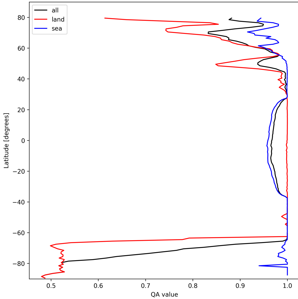
Figure 12: Zonal average of “QA value” for 2025-02-24 to 2025-02-26.
