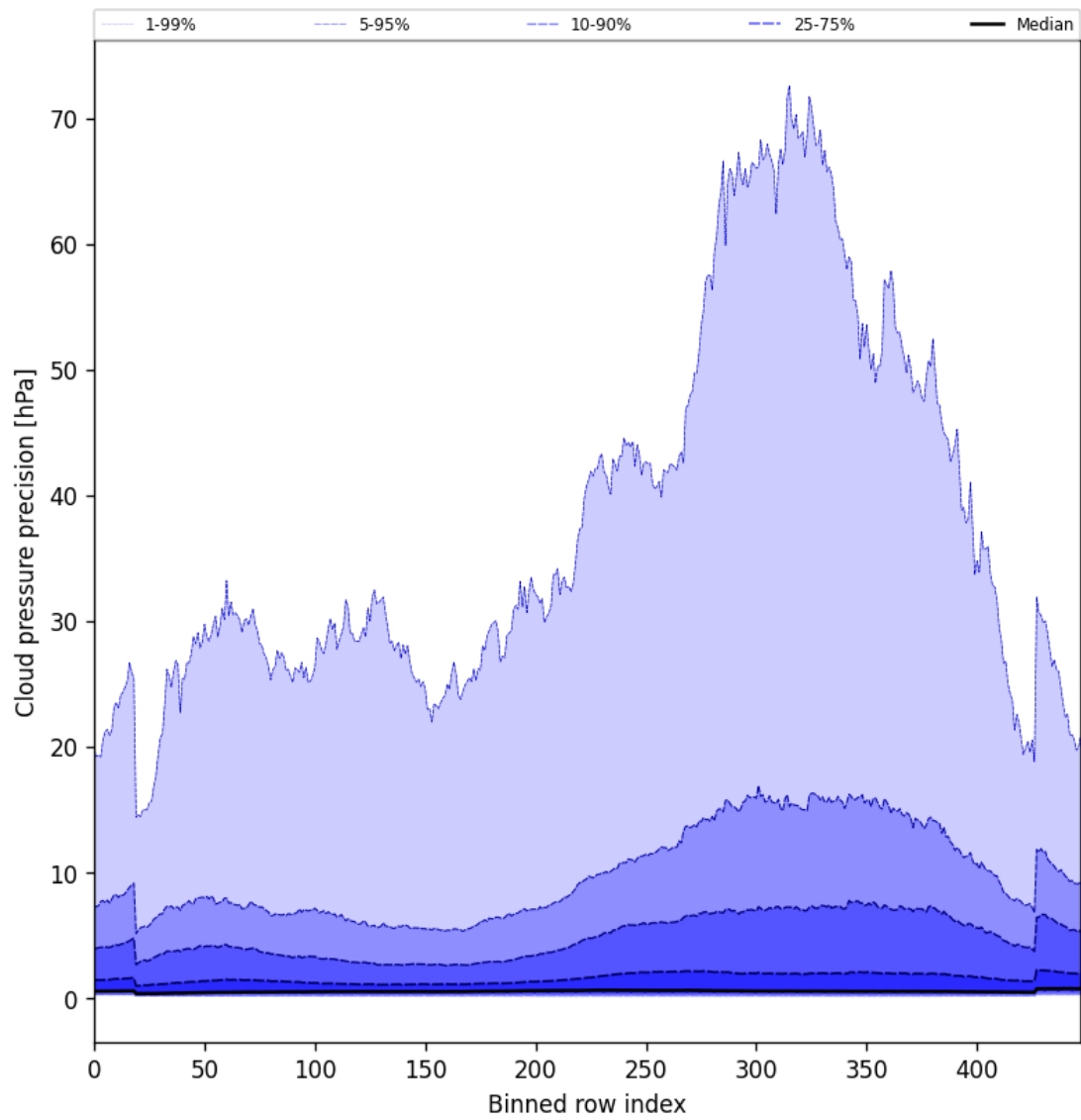
Figure 48: Along track statistics of “Cloud pressure precision” for 2025-02-24 to 2025-02-26
