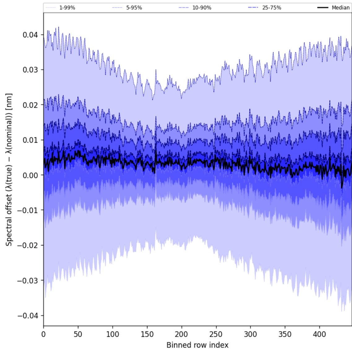
Figure 62: Along track statistics of “Spectral offset ( \lambda_{\text{true}} - \lambda_{\text{nominal}} )” for 2025-02-24 to 2025-02-26
