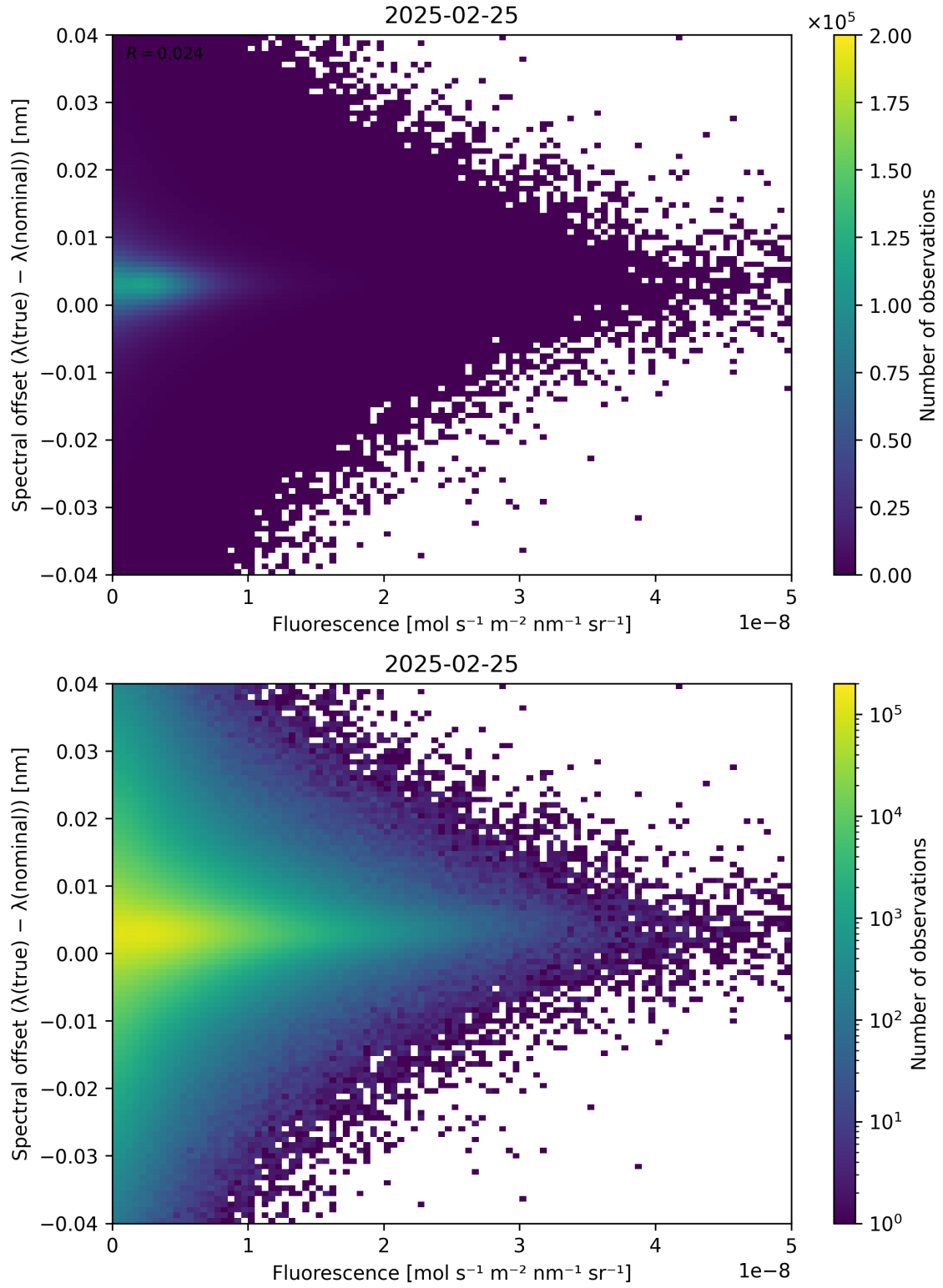
Figure 87: Scatter density plot of “Fluorescence” against “Spectral offset ( \lambda_{\text{true}} - \lambda_{\text{nominal}} )” for 2025-02-24 to 2025-02-26.
