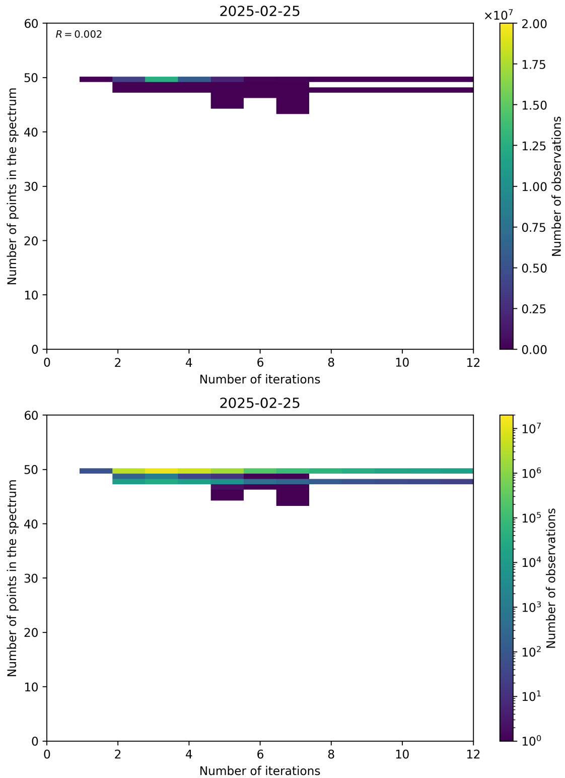
Figure 99: Scatter density plot of “Number of iterations” against “Number of points in the spectrum” for 2025-02-24 to 2025-02-26.
