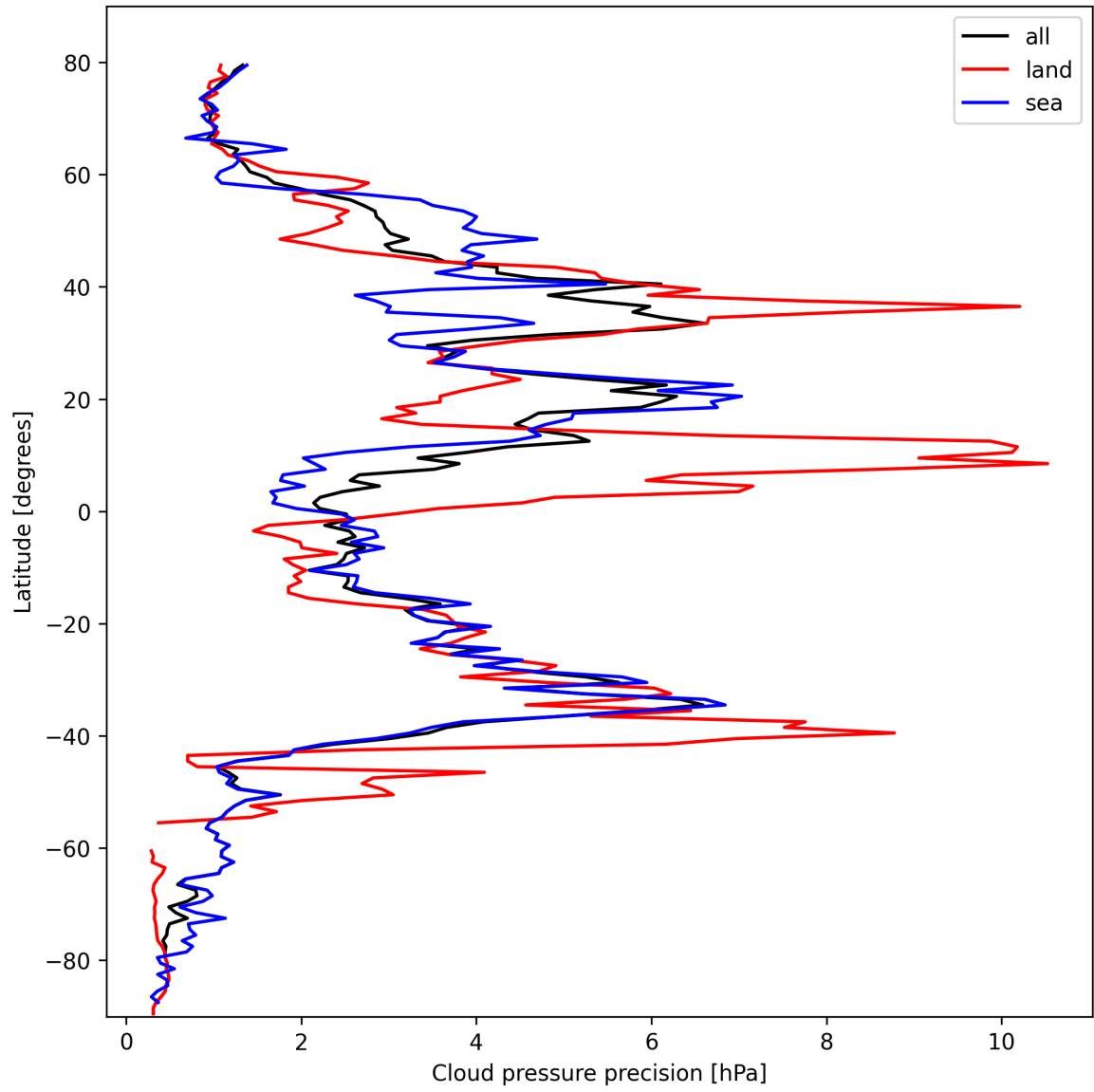
Figure 14: Zonal average of “Cloud pressure precision” for 2025-02-24 to 2025-02-26.
