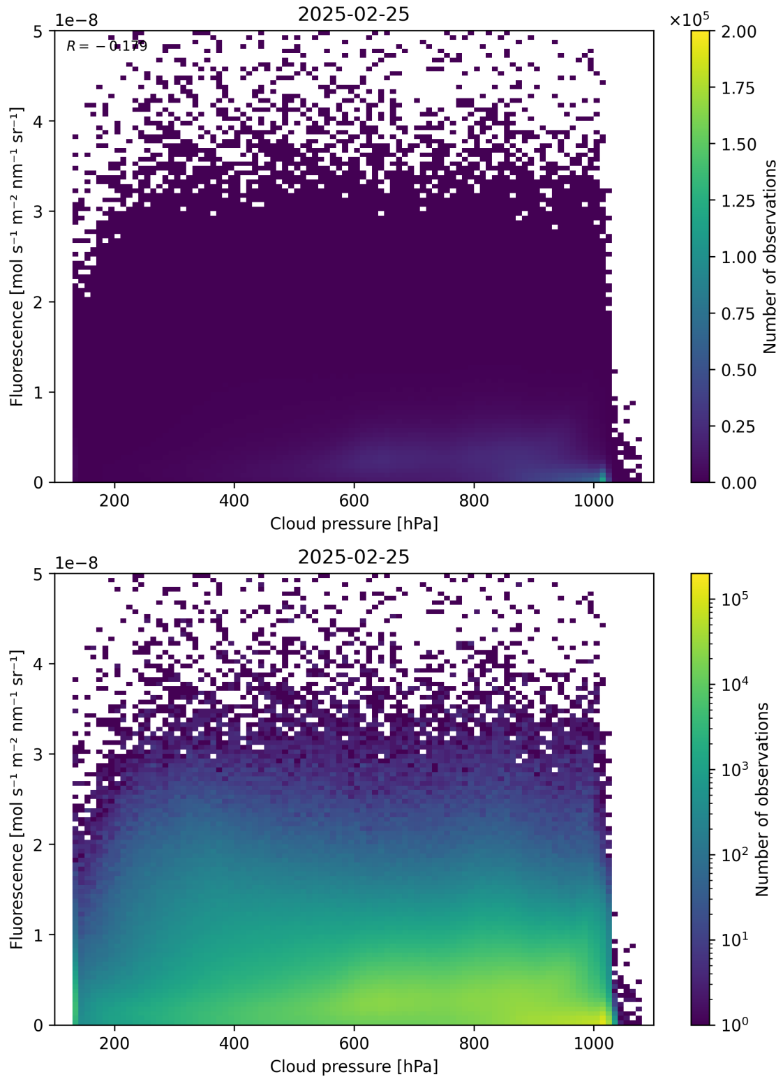
Figure 80: Scatter density plot of “Cloud pressure” against “Fluorescence” for 2025-02-24 to 2025-02-26.
