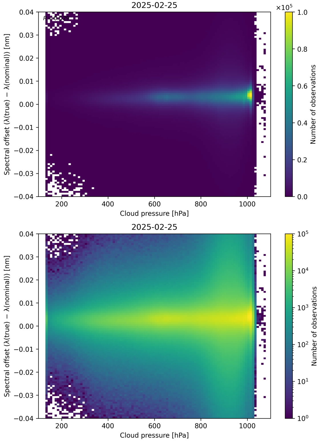
Figure 84: Scatter density plot of “Cloud pressure” against “Spectral offset ( \lambda_{\text{true}} - \lambda_{\text{nominal}} )” for 2025-02-24 to 2025-02-26.
