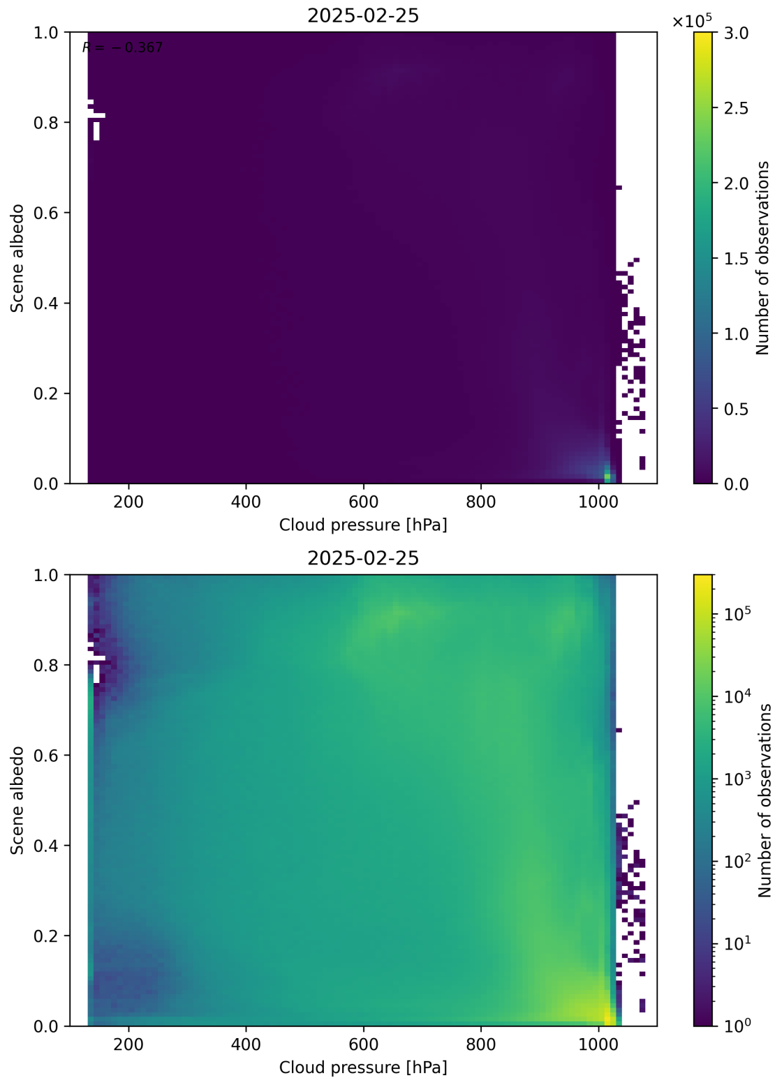
Figure 83: Scatter density plot of “Cloud pressure” against “Scene albedo” for 2025-02-24 to 2025-02-26.
