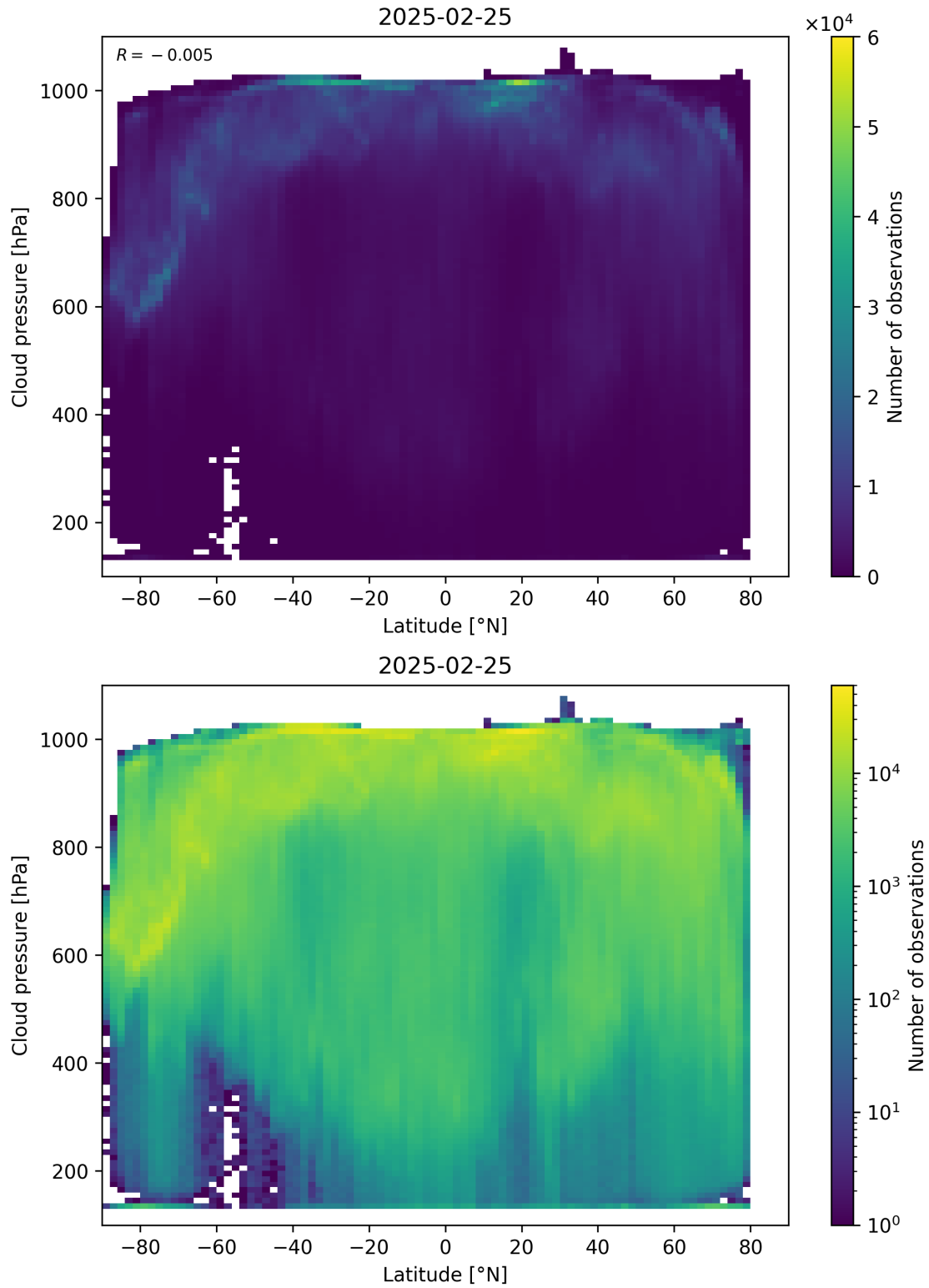
Figure 91: Scatter density plot of “Latitude” against “Cloud pressure” for 2025-02-24 to 2025-02-26.
