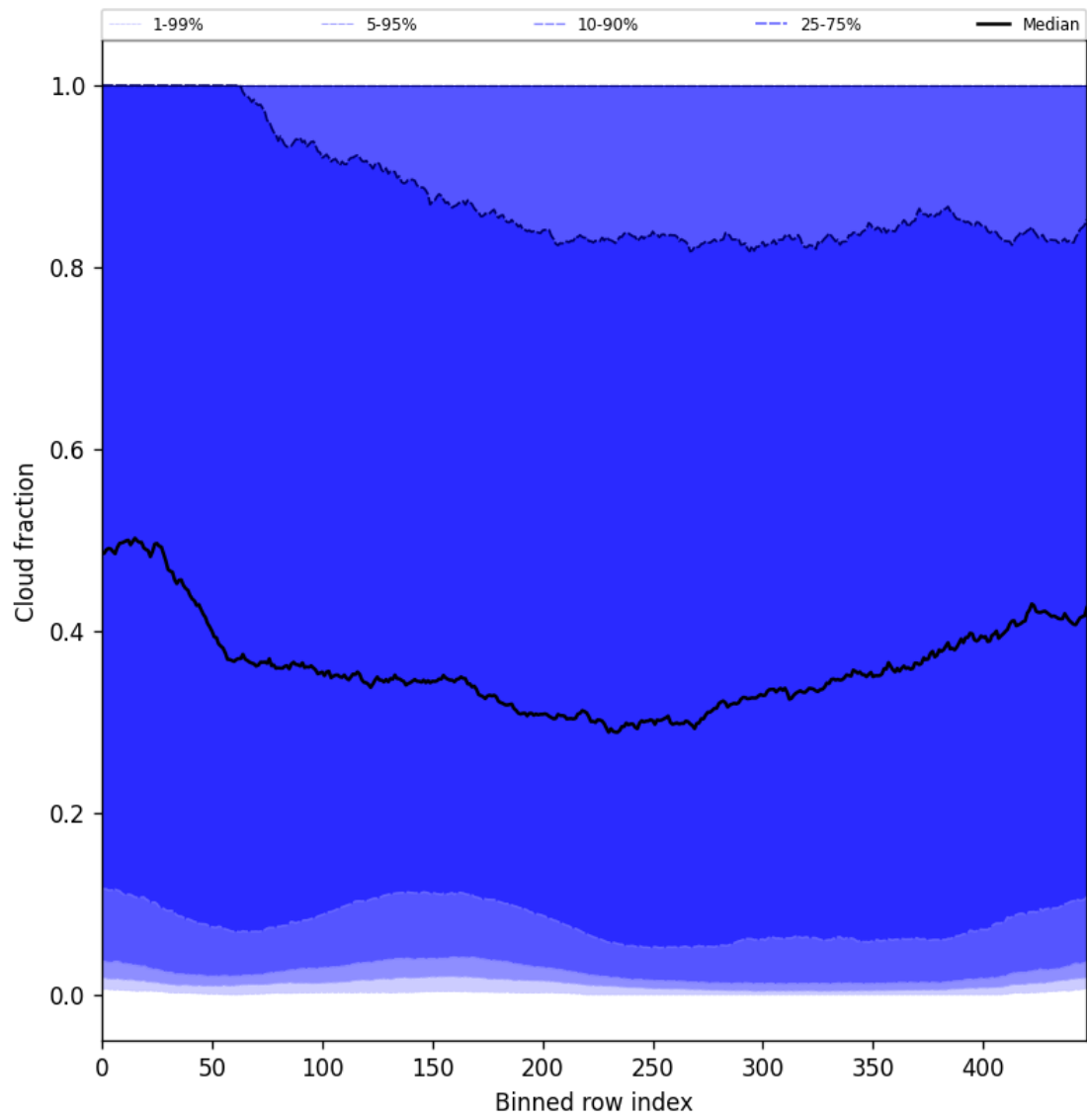
Figure 49: Along track statistics of “Cloud fraction” for 2025-02-24 to 2025-02-26
