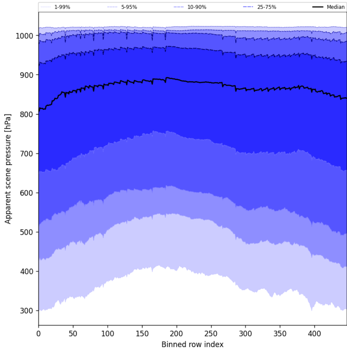
Figure 53: Along track statistics of “Apparent scene pressure” for 2025-02-24 to 2025-02-26
