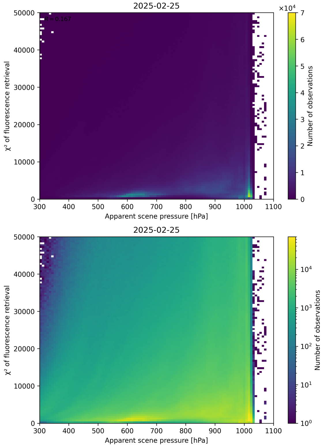
Figure 63: Scatter density plot of “Apparent scene pressure” against “ \chi^2 of fluorescence retrieval” for 2025-02-24 to 2025-02-26.
