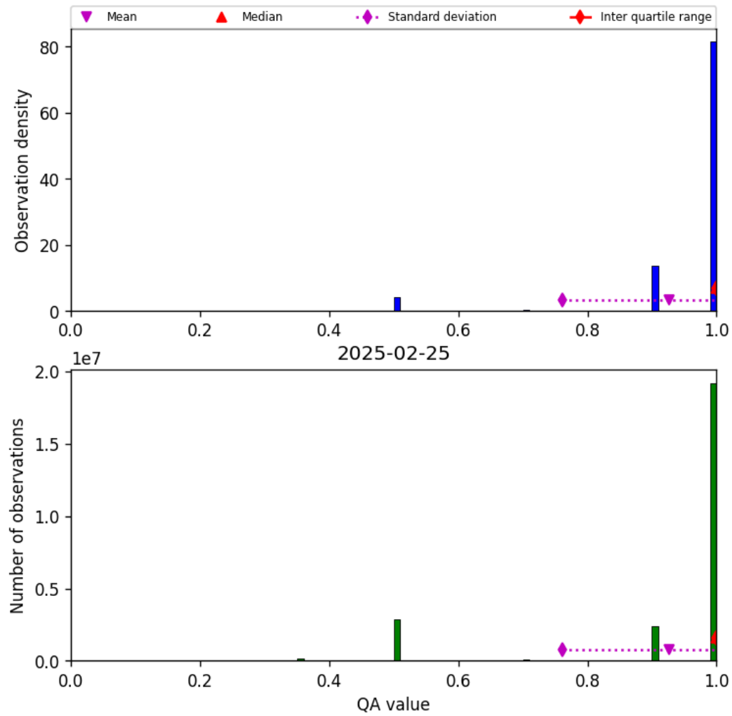
Figure 29: Histogram of “QA value” for 2025-02-24 to 2025-02-26
