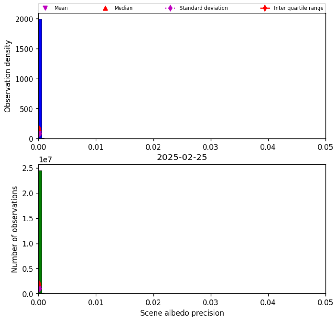
Figure 35: Histogram of “Scene albedo precision” for 2025-02-24 to 2025-02-26
