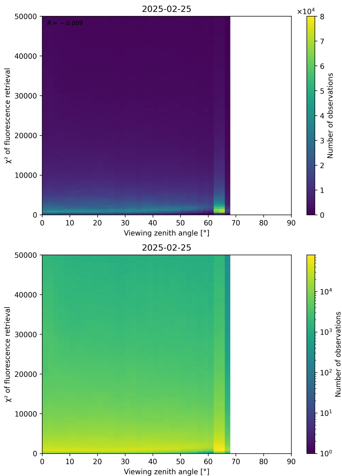
Figure 119: Scatter density plot of “Viewing zenith angle” against “ \chi^2 of fluorescence retrieval” for 2025-02-24 to 2025-02-26.
