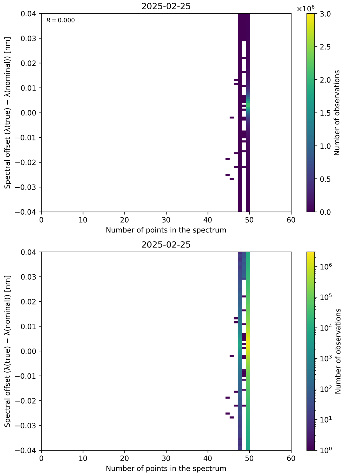
Figure 101: Scatter density plot of “Number of points in the spectrum” against “Spectral offset ( \lambda_{\text{true}} - \lambda_{\text{nominal}} )” for 2025-02-24 to 2025-02-26.
