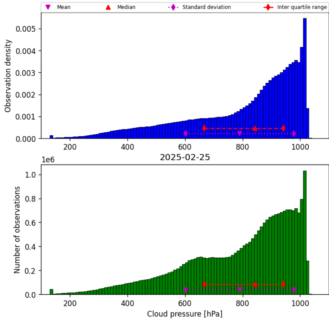
Figure 30: Histogram of “Cloud pressure” for 2025-02-24 to 2025-02-26
