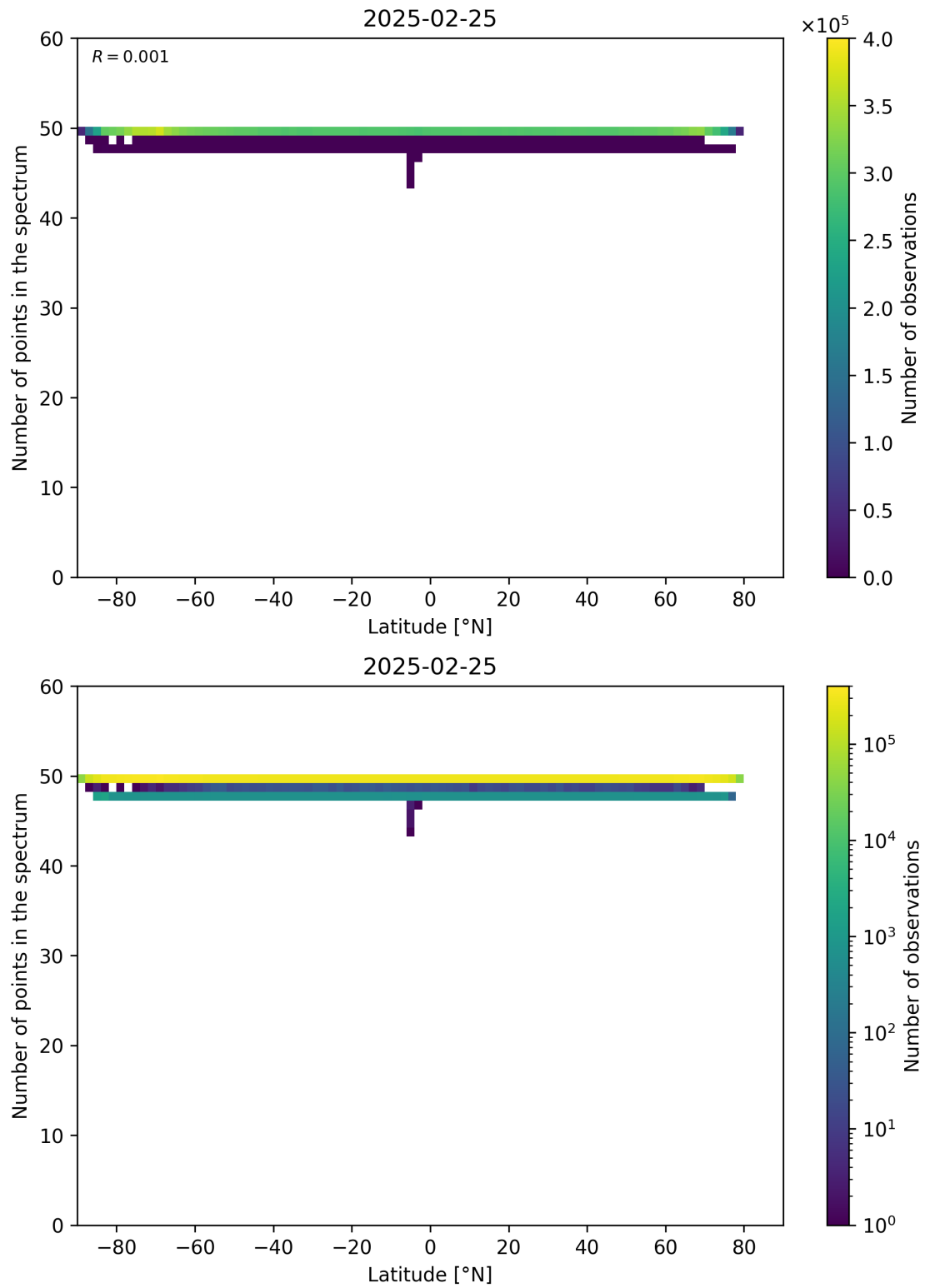
Figure 94: Scatter density plot of “Latitude” against “Number of points in the spectrum” for 2025-02-24 to 2025-02-26.
