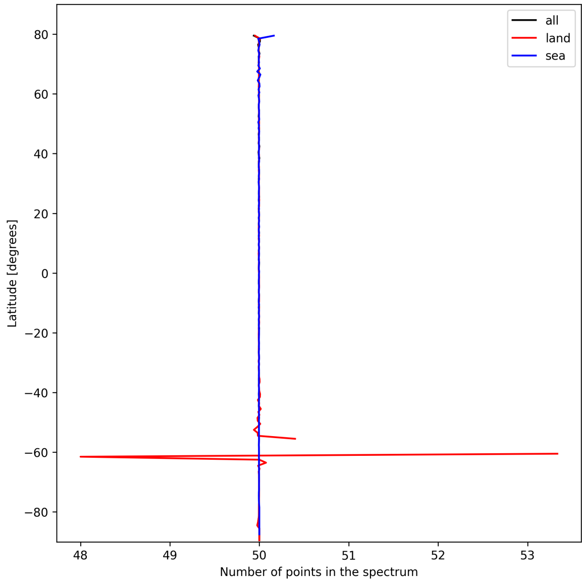
Figure 27: Zonal average of “Number of points in the spectrum” for 2025-02-24 to 2025-02-26.
