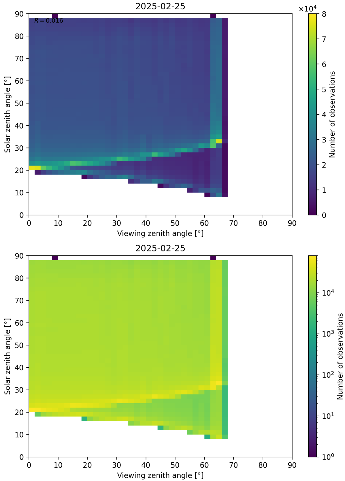
Figure 127: Scatter density plot of “Viewing zenith angle” against “Solar zenith angle” for 2025-02-24 to 2025-02-26.
