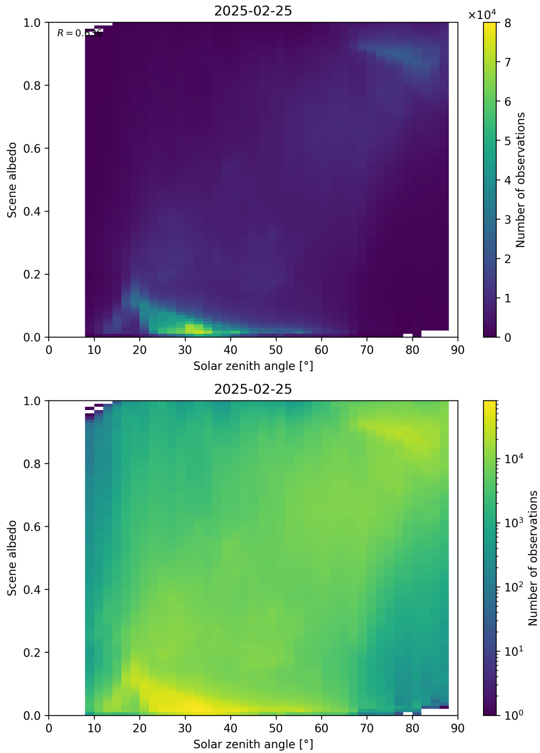
Figure 116: Scatter density plot of “Solar zenith angle” against “Scene albedo” for 2025-02-24 to 2025-02-26.
