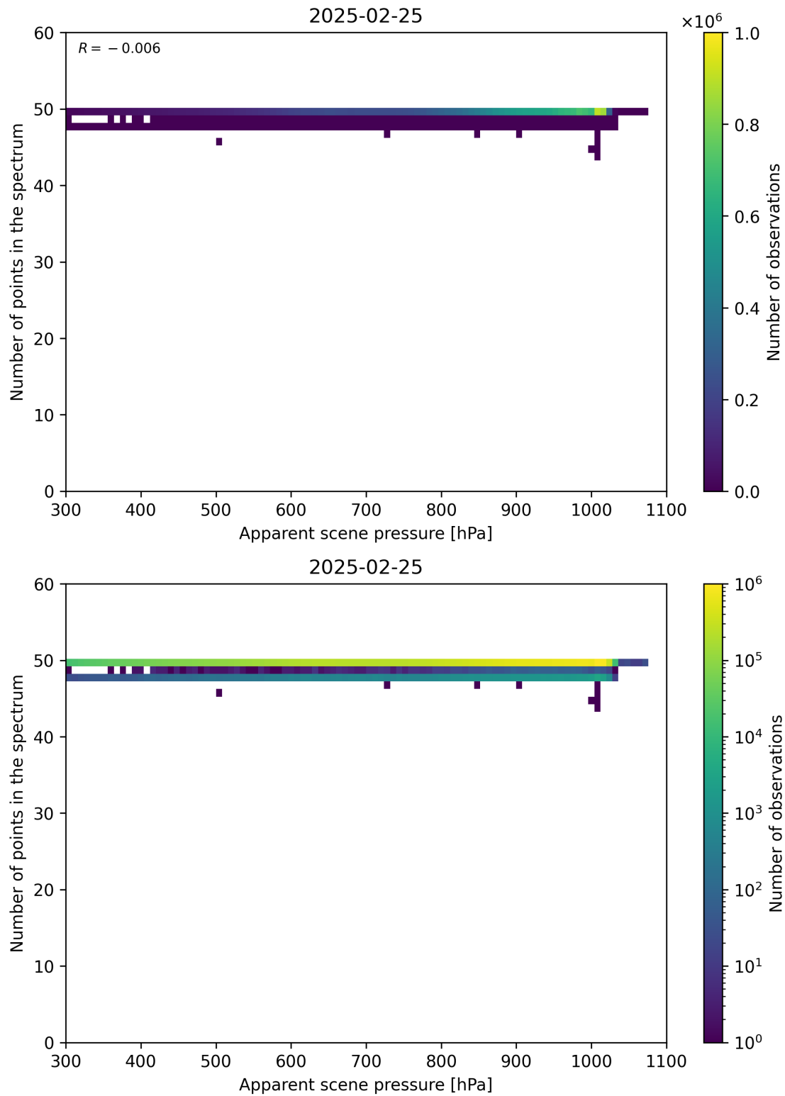
Figure 66: Scatter density plot of “Apparent scene pressure” against “Number of points in the spectrum” for 2025-02-24 to 2025-02-26.
