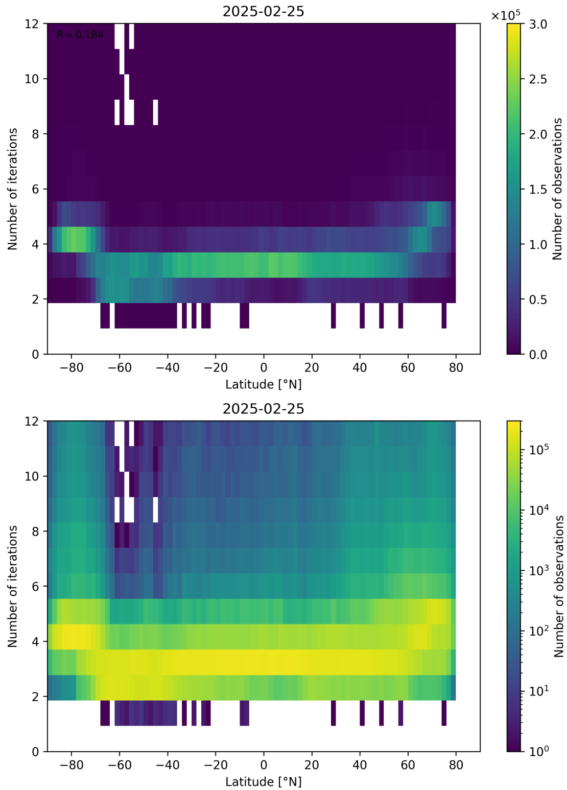
Figure 93: Scatter density plot of “Latitude” against “Number of iterations” for 2025-02-24 to 2025-02-26.
