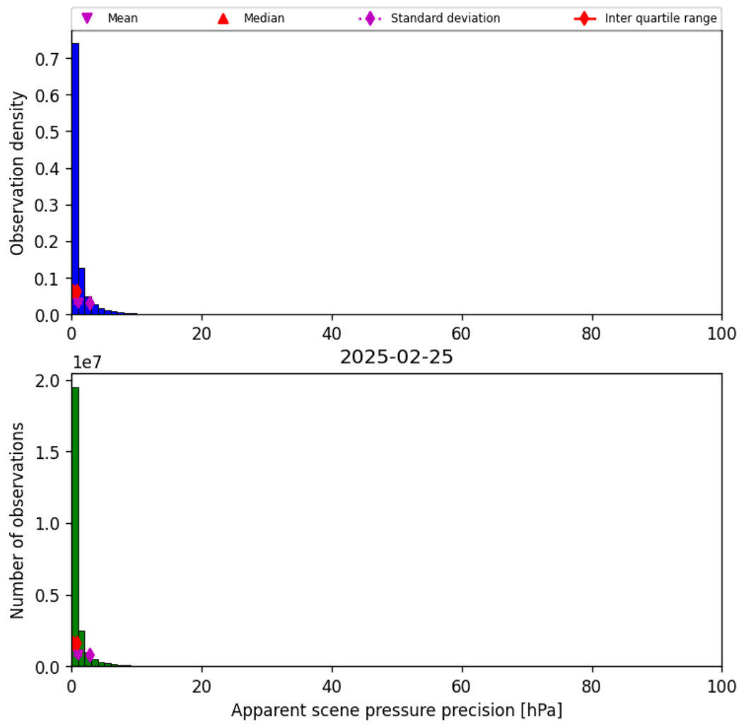
Figure 37: Histogram of “Apparent scene pressure precision” for 2025-02-24 to 2025-02-26
