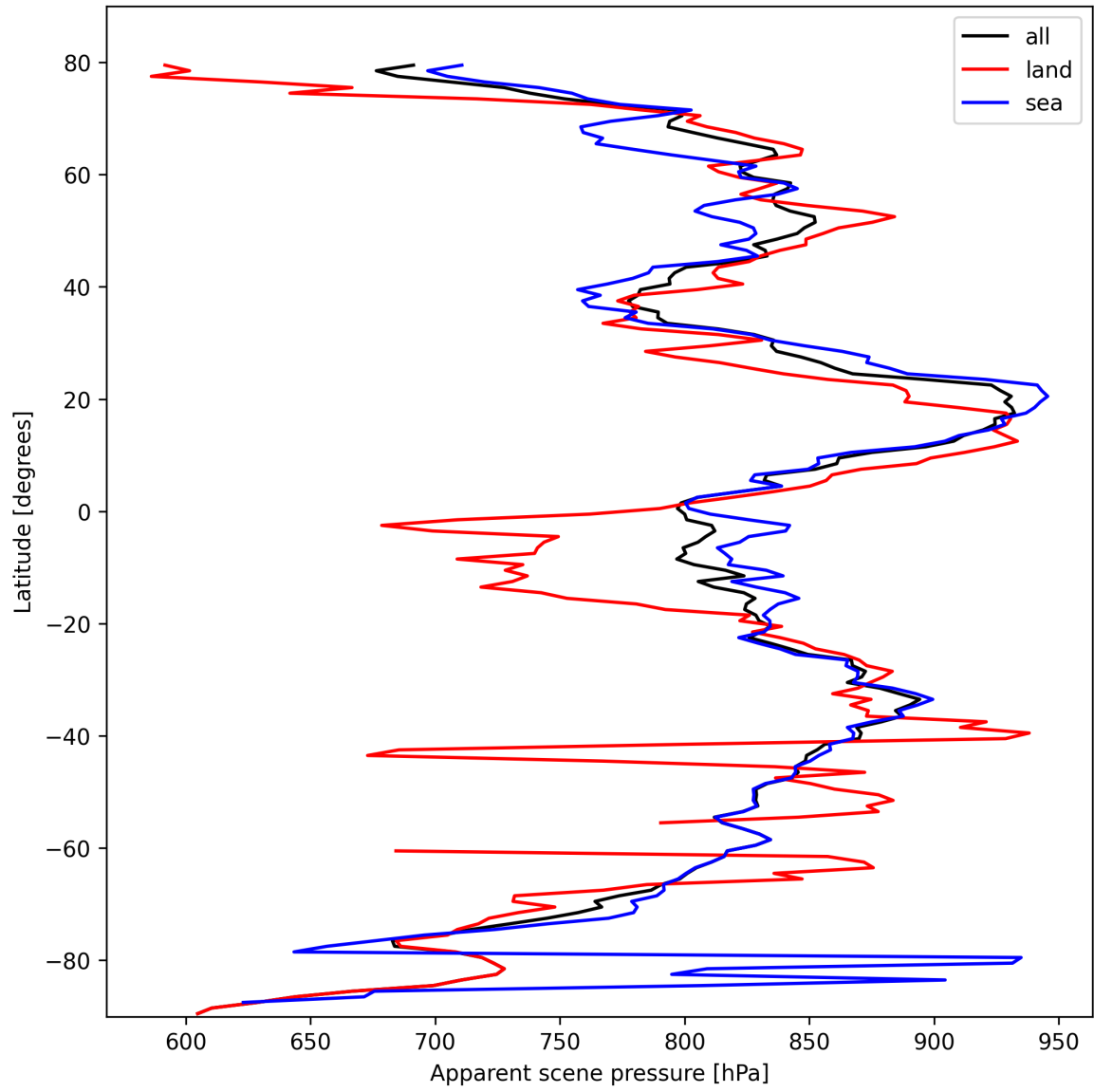
Figure 19: Zonal average of “Apparent scene pressure” for 2025-02-24 to 2025-02-26.
