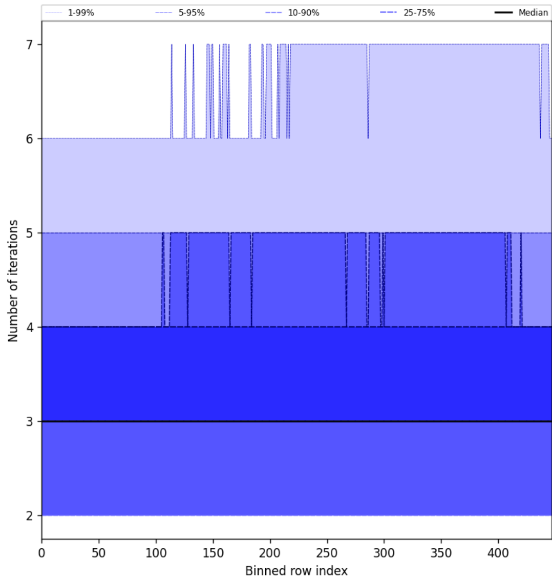
Figure 56: Along track statistics of “Number of iterations” for 2025-02-24 to 2025-02-26
