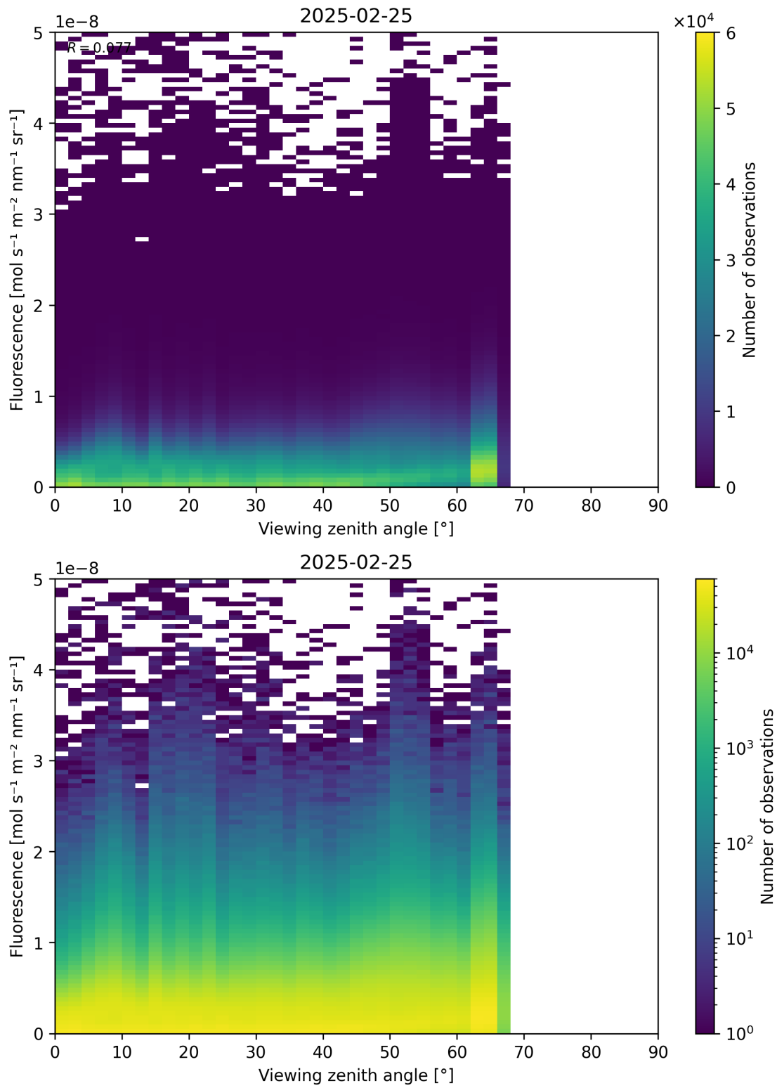
Figure 122: Scatter density plot of “Viewing zenith angle” against “Fluorescence” for 2025-02-24 to 2025-02-26.
