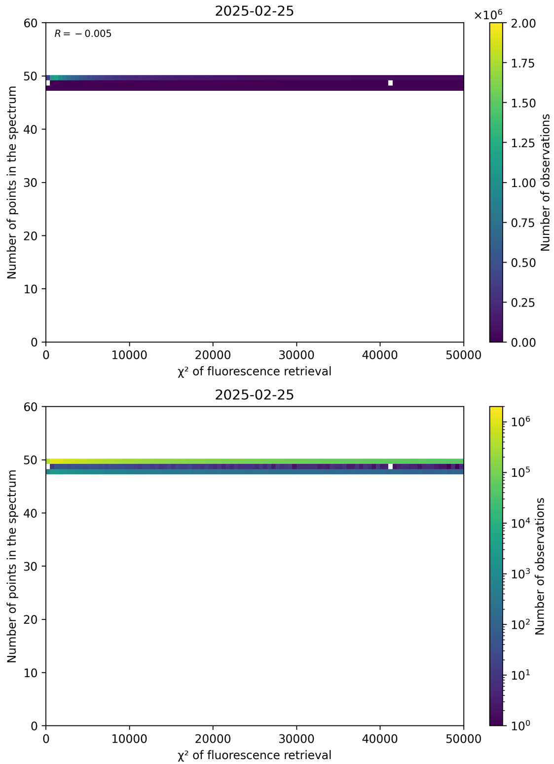
Figure 68: Scatter density plot of “ \chi^2 of fluorescence retrieval” against “Number of points in the spectrum” for 2025-02-24 to 2025-02-26.
