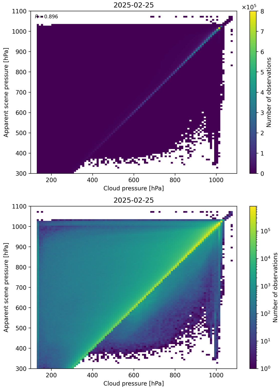
Figure 77: Scatter density plot of “Cloud pressure” against “Apparent scene pressure” for 2025-02-24 to 2025-02-26.
