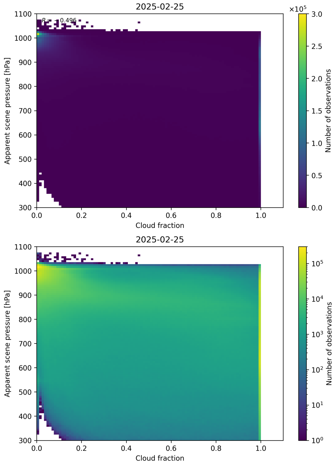
Figure 70: Scatter density plot of “Cloud fraction” against “Apparent scene pressure” for 2025-02-24 to 2025-02-26.
