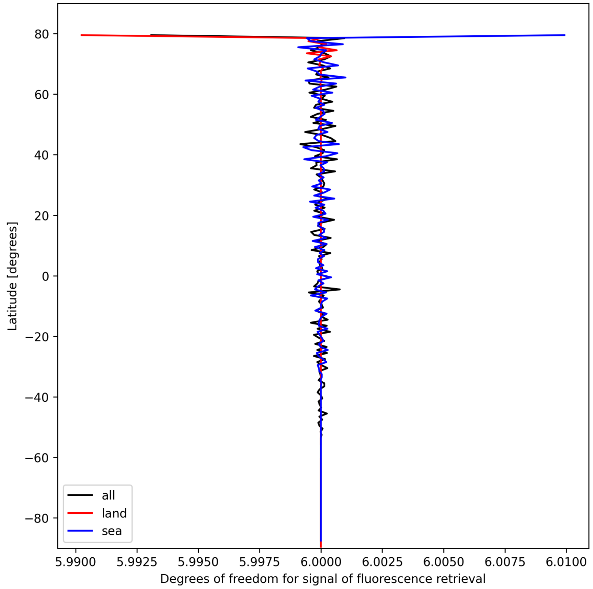
Figure 26: Zonal average of “Degrees of freedom for signal of fluorescence retrieval” for 2025-02-24 to 2025-02-26.
