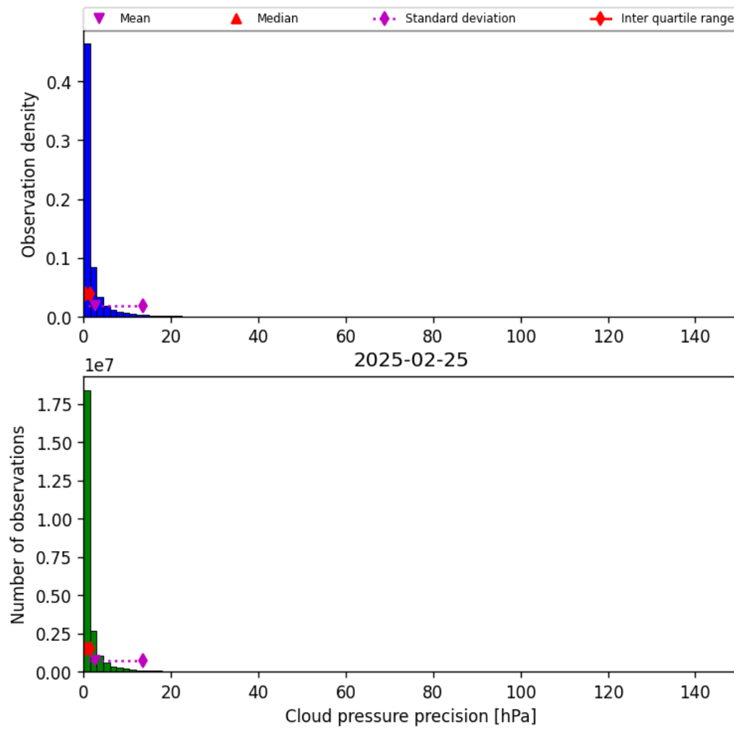
Figure 31: Histogram of “Cloud pressure precision” for 2025-02-24 to 2025-02-26
