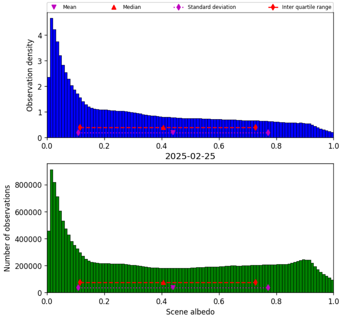
Figure 34: Histogram of “Scene albedo” for 2025-02-24 to 2025-02-26
