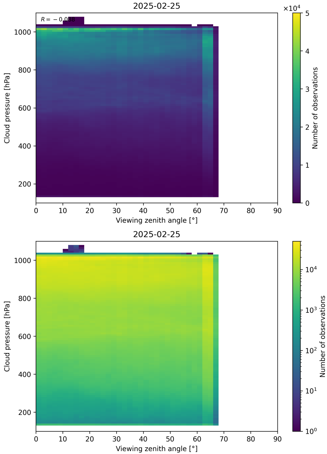
Figure 121: Scatter density plot of “Viewing zenith angle” against “Cloud pressure” for 2025-02-24 to 2025-02-26.
