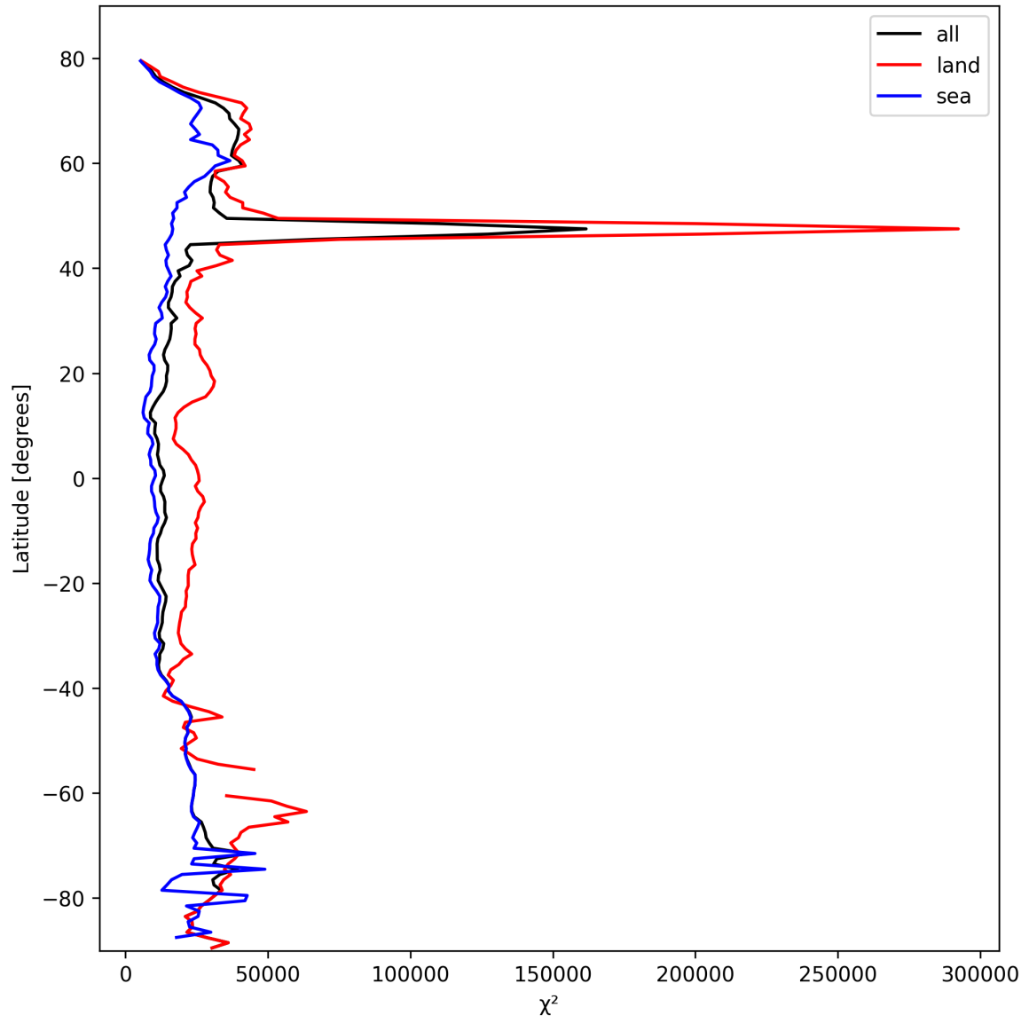
Figure 21: Zonal average of “ \chi^2 ” for 2025-02-24 to 2025-02-26.
