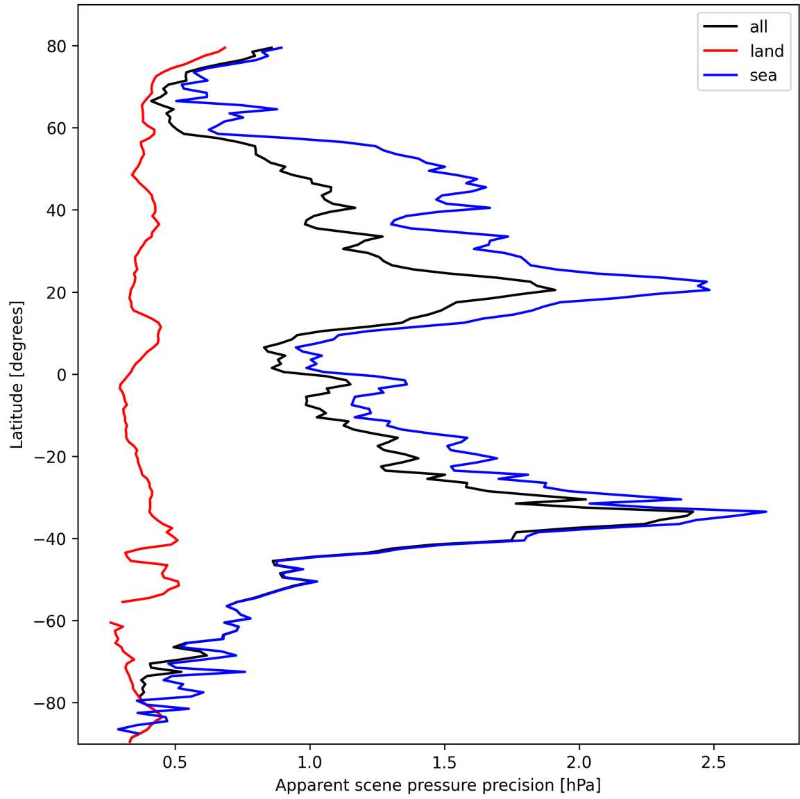
Figure 20: Zonal average of “Apparent scene pressure precision” for 2025-02-24 to 2025-02-26.
