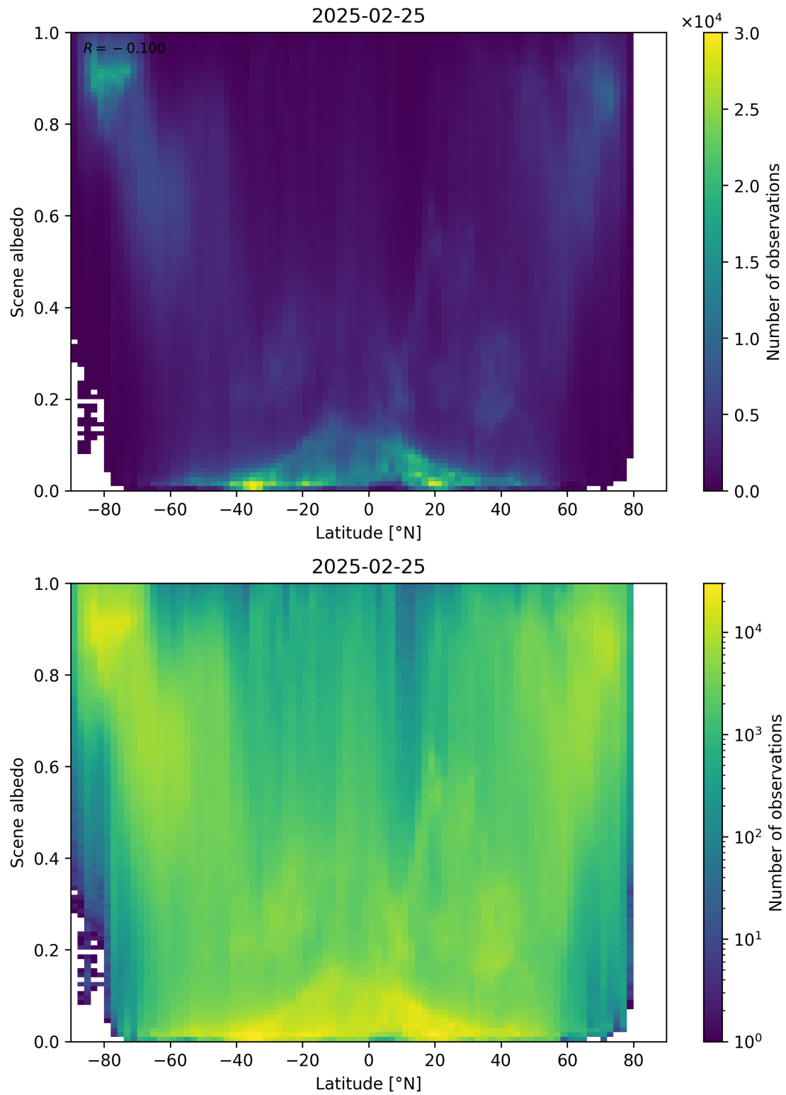
Figure 95: Scatter density plot of “Latitude” against “Scene albedo” for 2025-02-24 to 2025-02-26.
