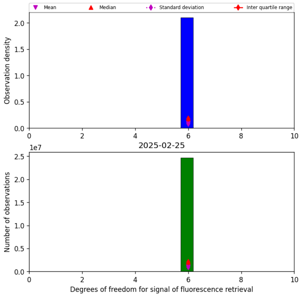
Figure 43: Histogram of "Degrees of freedom for signal of fluorescence retrieval" for 2025-02-24 to 2025-02-26
