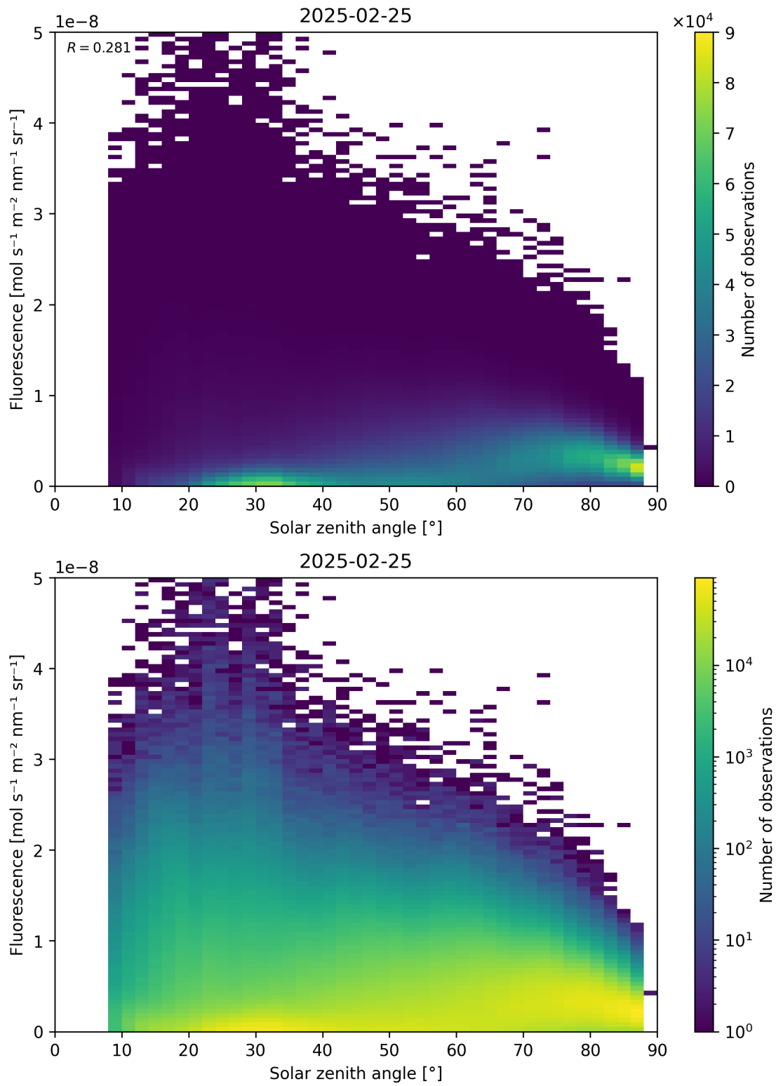
Figure 112: Scatter density plot of “Solar zenith angle” against “Fluorescence” for 2025-02-24 to 2025-02-26.
