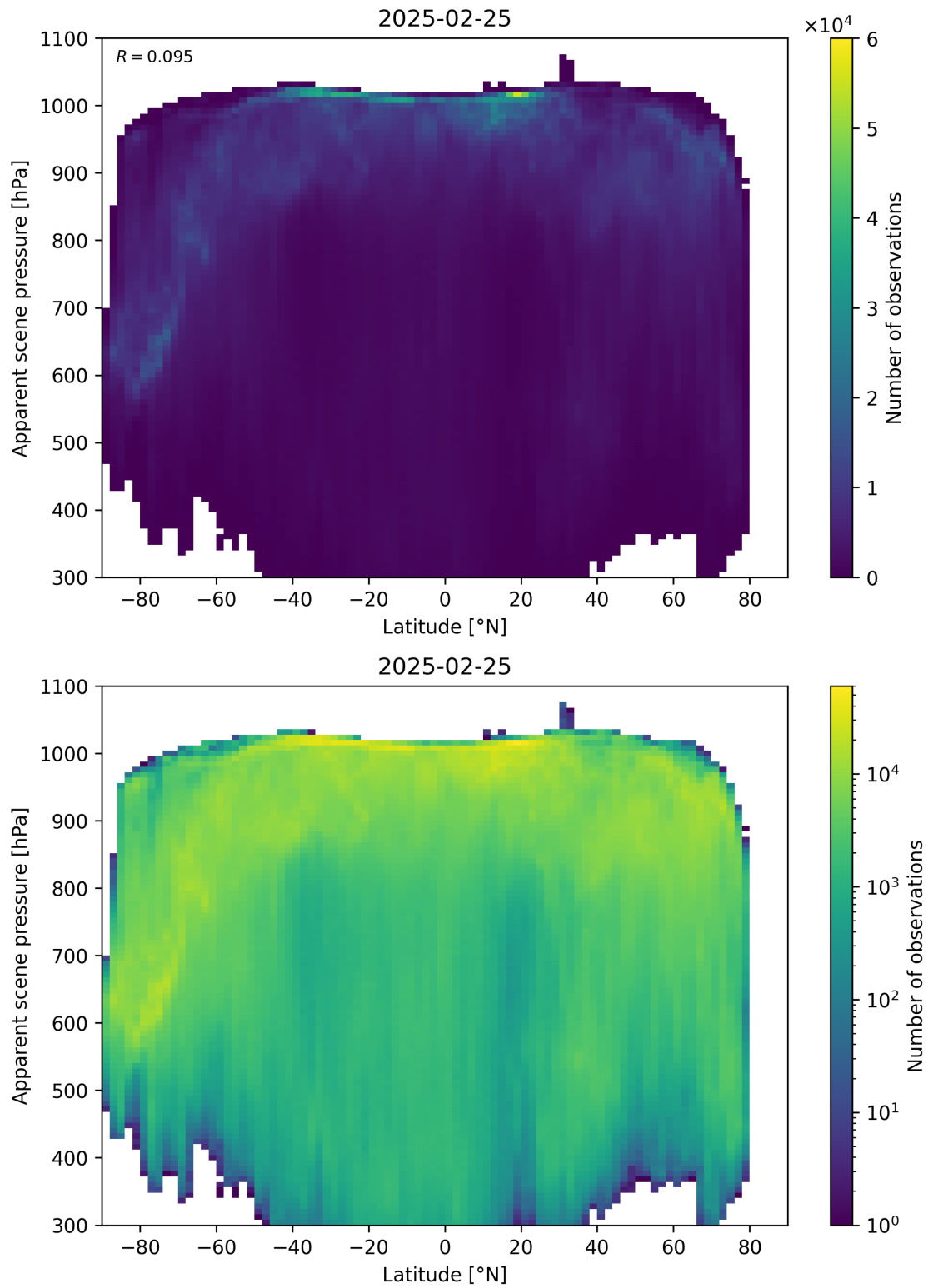
Figure 88: Scatter density plot of “Latitude” against “Apparent scene pressure” for 2025-02-24 to 2025-02-26.
