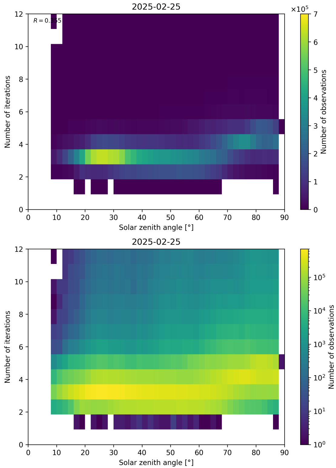
Figure 114: Scatter density plot of “Solar zenith angle” against “Number of iterations” for 2025-02-24 to 2025-02-26.
