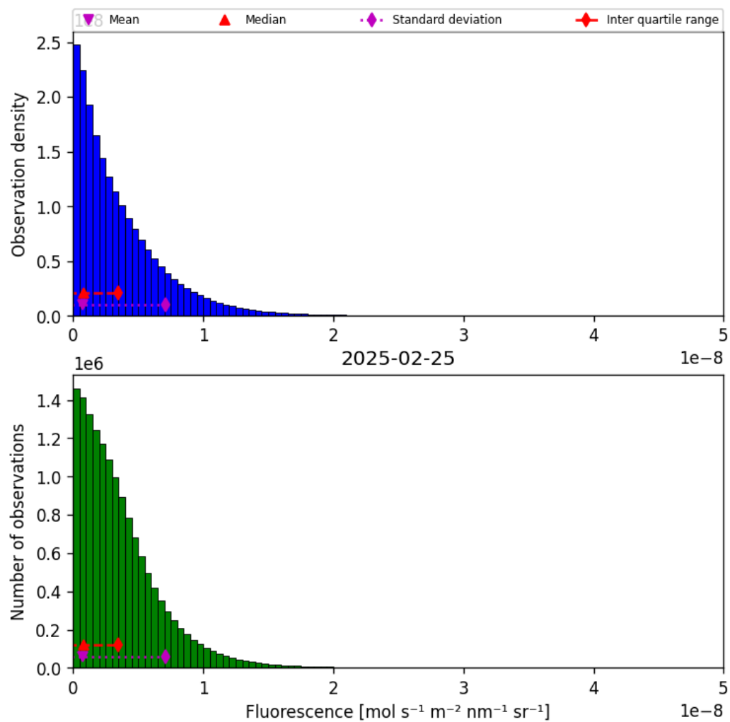
Figure 40: Histogram of “Fluorescence” for 2025-02-24 to 2025-02-26
