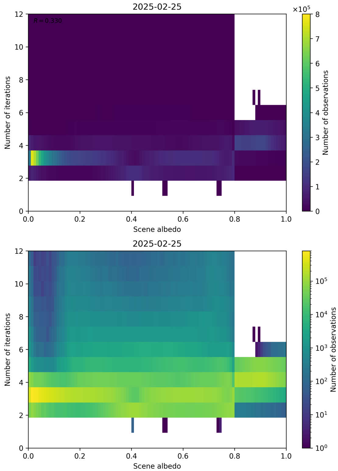
Figure 105: Scatter density plot of “Scene albedo” against “Number of iterations” for 2025-02-24 to 2025-02-26.
