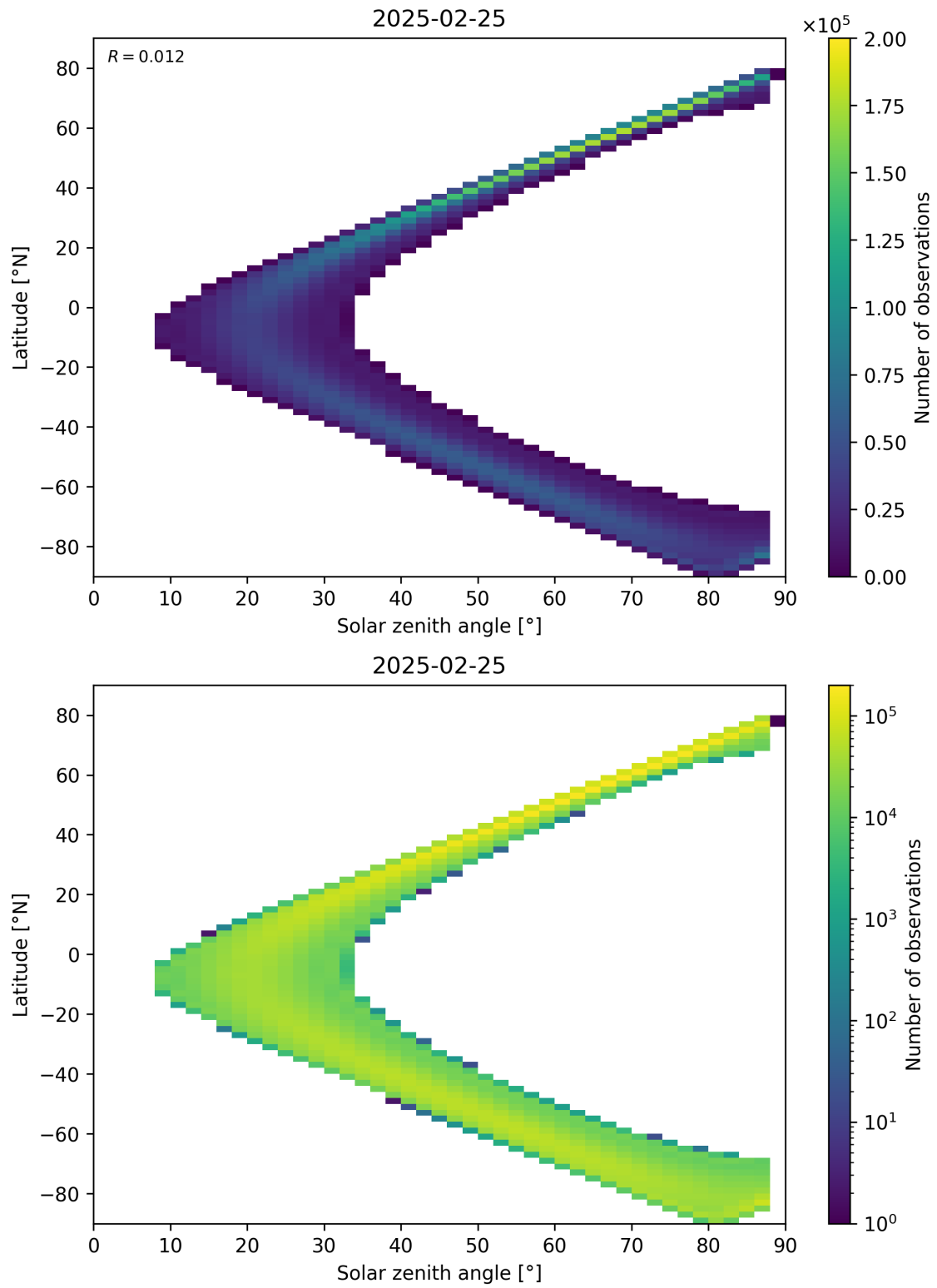
Figure 113: Scatter density plot of “Solar zenith angle” against “Latitude” for 2025-02-24 to 2025-02-26.
