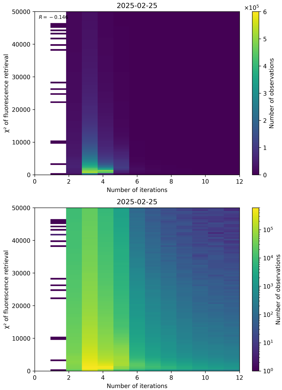
Figure 97: Scatter density plot of “Number of iterations” against “ \chi^2 of fluorescence retrieval” for 2025-02-24 to 2025-02-26.
