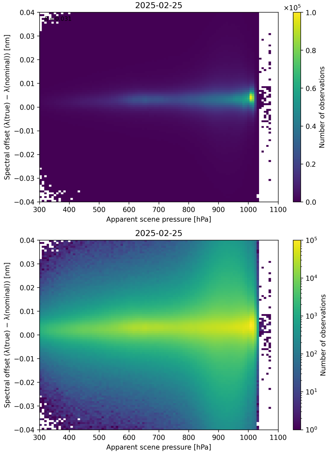
Figure 67: Scatter density plot of “Apparent scene pressure” against “Spectral offset ( \lambda_{\text{true}} - \lambda_{\text{nominal}} )” for 2025-02-24 to 2025-02-26.
