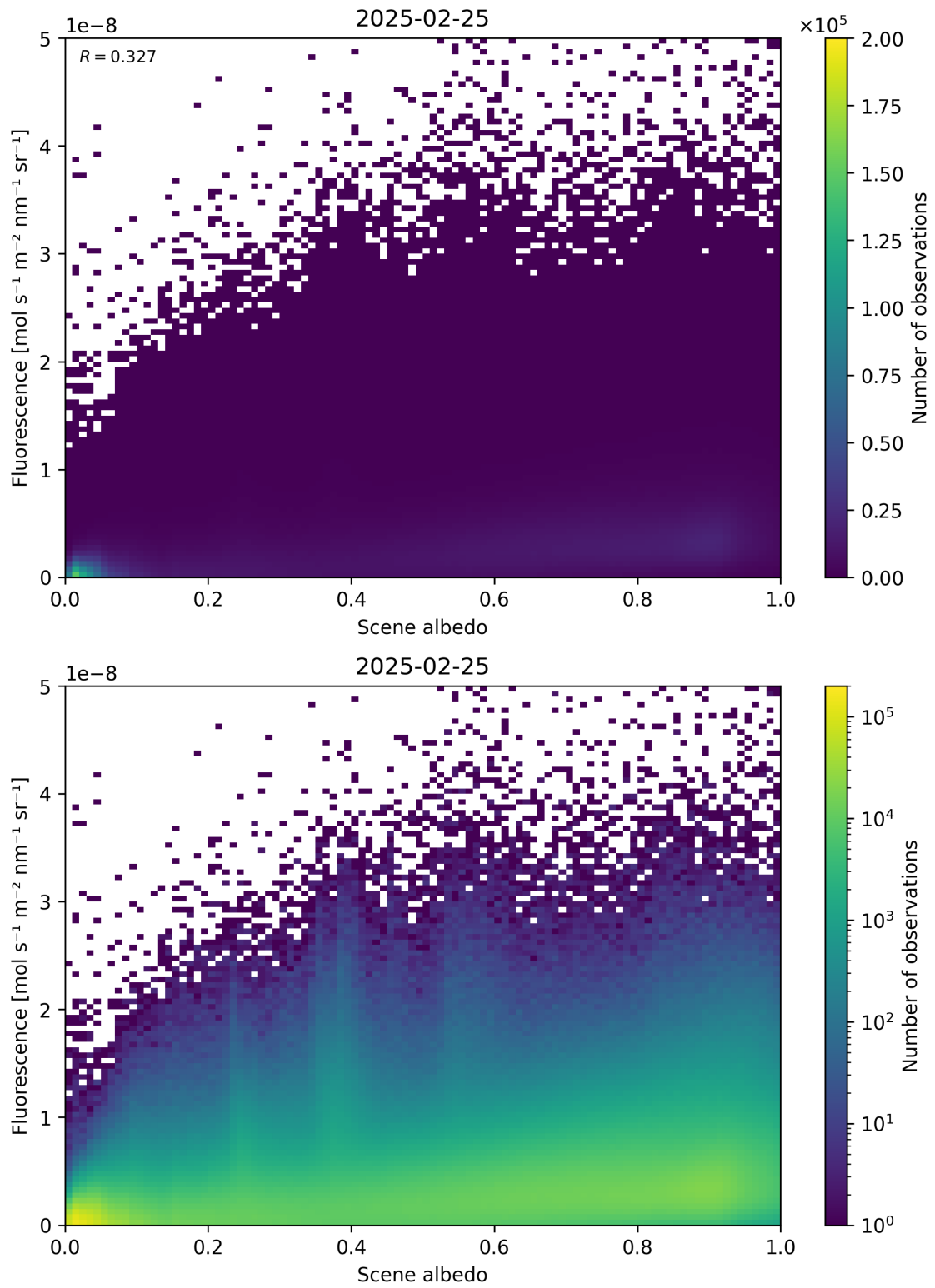
Figure 104: Scatter density plot of “Scene albedo” against “Fluorescence” for 2025-02-24 to 2025-02-26.
