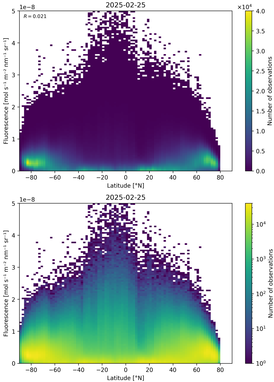
Figure 92: Scatter density plot of “Latitude” against “Fluorescence” for 2025-02-24 to 2025-02-26.
