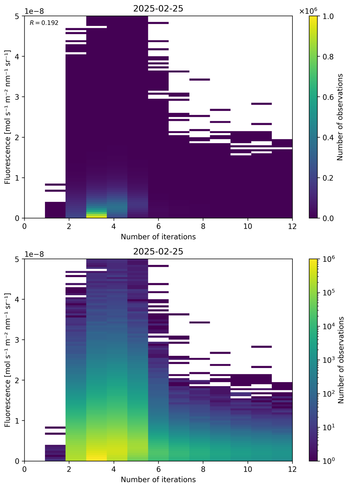
Figure 98: Scatter density plot of “Number of iterations” against “Fluorescence” for 2025-02-24 to 2025-02-26.
