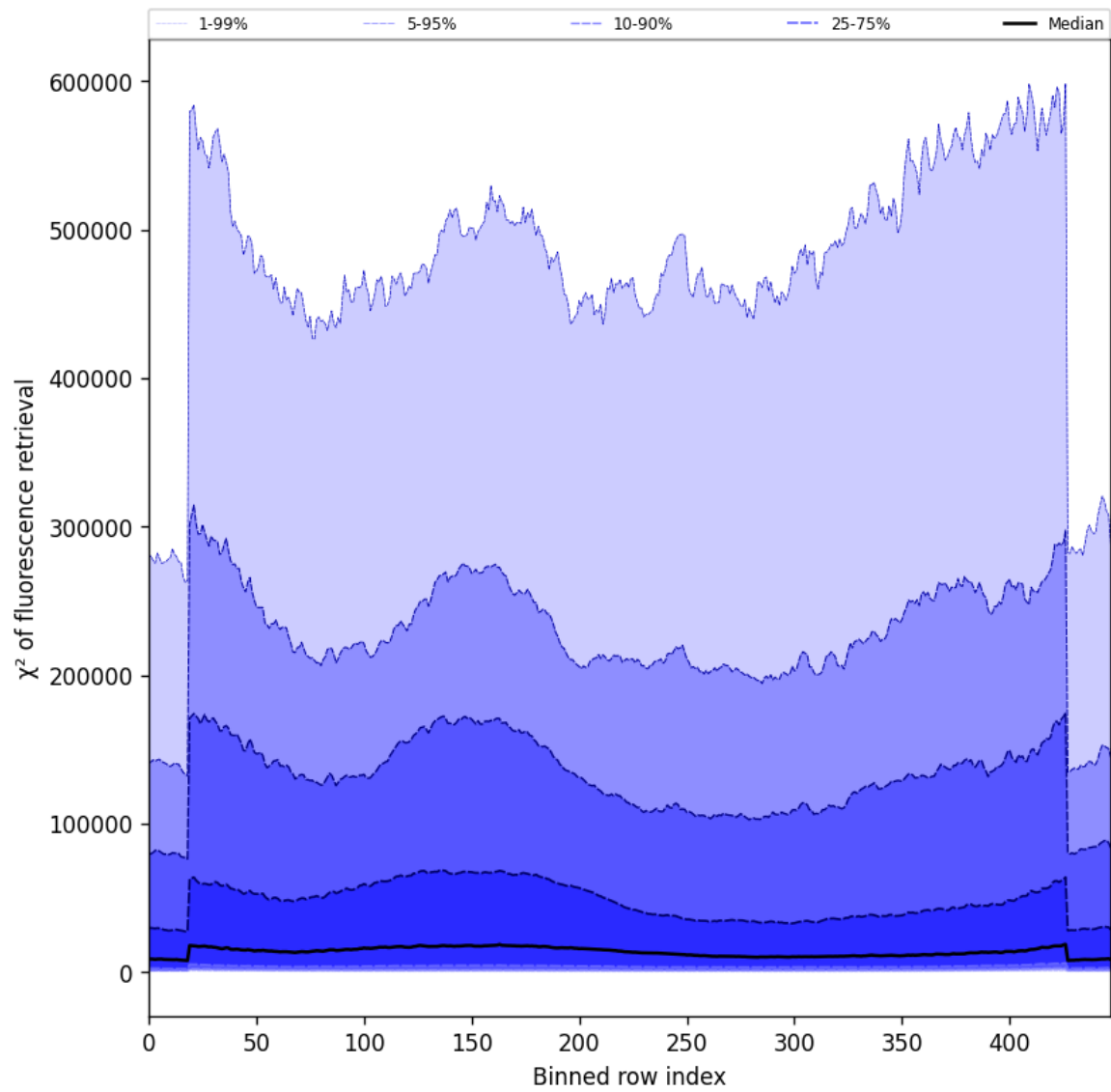
Figure 59: Along track statistics of “ \chi^2 of fluorescence retrieval” for 2025-02-24 to 2025-02-26
