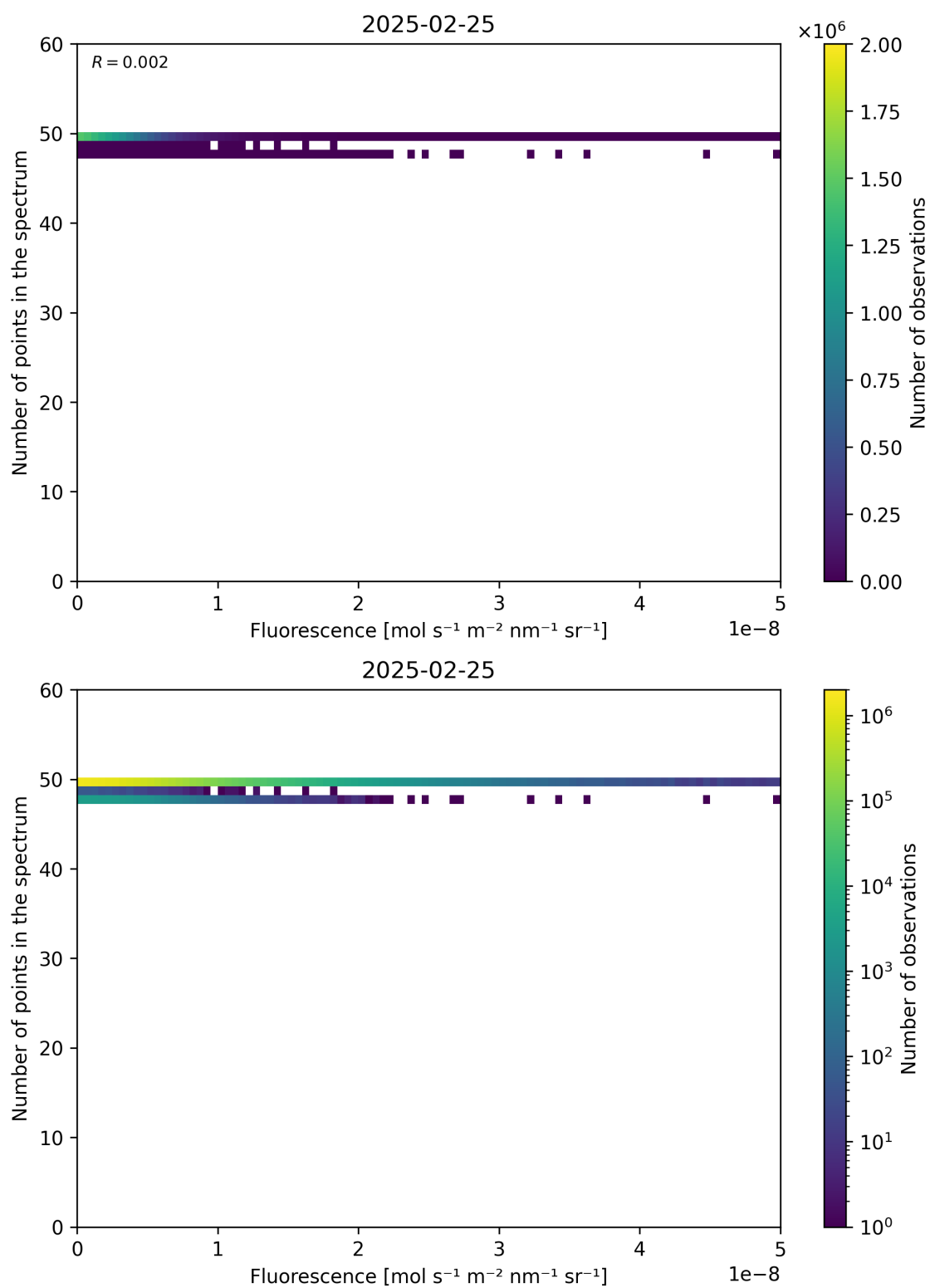
Figure 86: Scatter density plot of “Fluorescence” against “Number of points in the spectrum” for 2025-02-24 to 2025-02-26.
