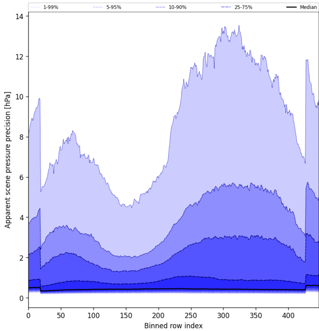
Figure 54: Along track statistics of “Apparent scene pressure precision” for 2025-02-24 to 2025-02-26
