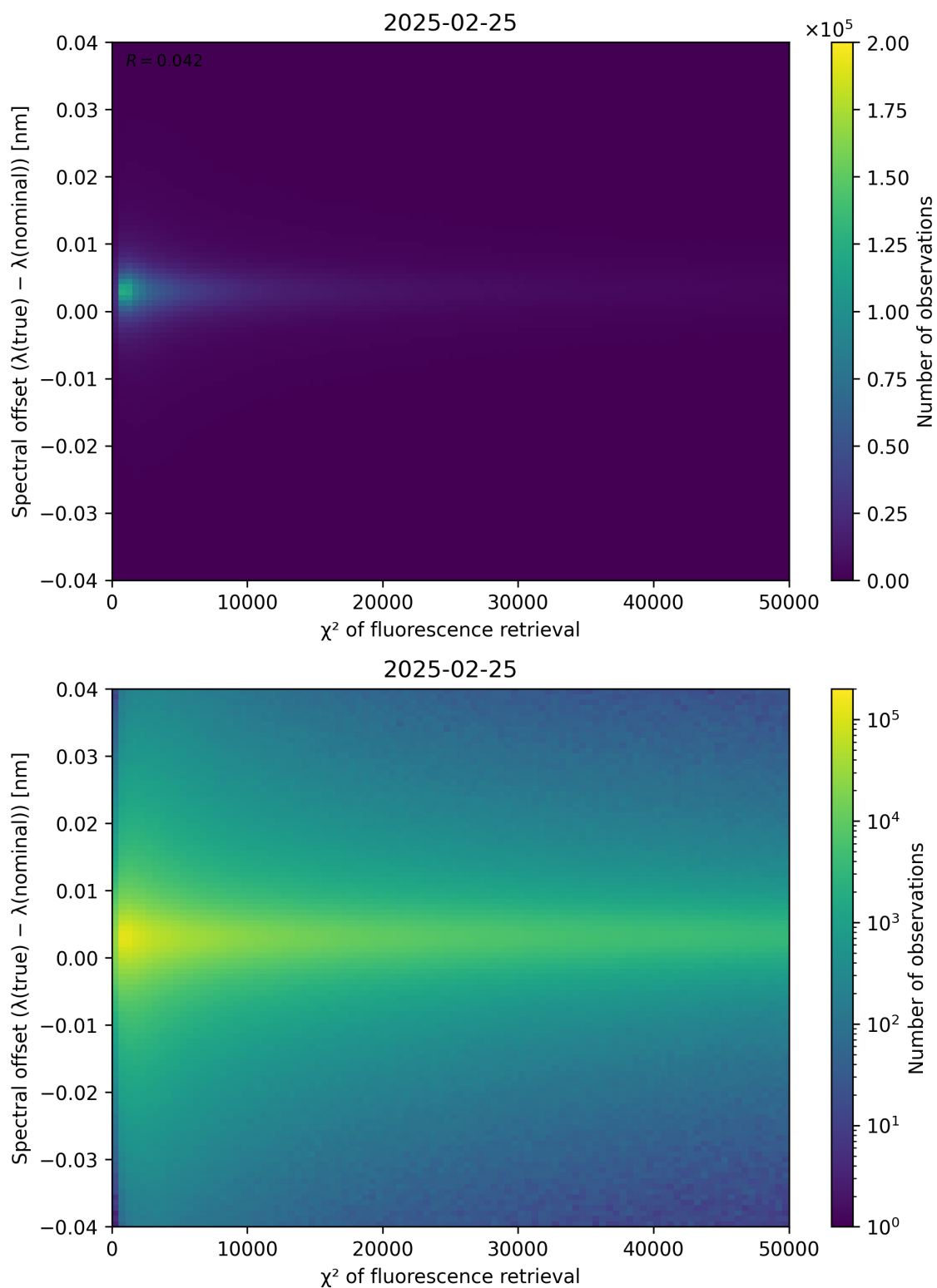
Figure 69: Scatter density plot of “ \chi^2 of fluorescence retrieval” against “Spectral offset ( \lambda_{\text{true}} - \lambda_{\text{nominal}} )” for 2025-02-24 to 2025-02-26.
