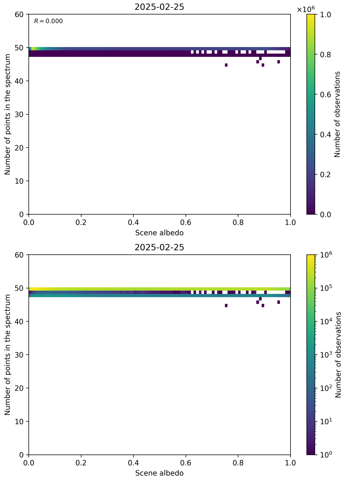
Figure 106: Scatter density plot of “Scene albedo” against “Number of points in the spectrum” for 2025-02-24 to 2025-02-26.
