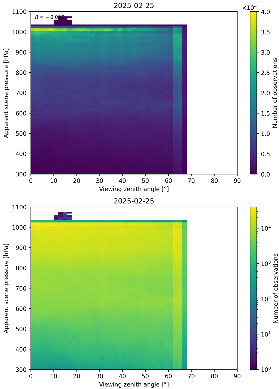
Figure 118: Scatter density plot of “Viewing zenith angle” against “Apparent scene pressure” for 2025-02-24 to 2025-02-26.
