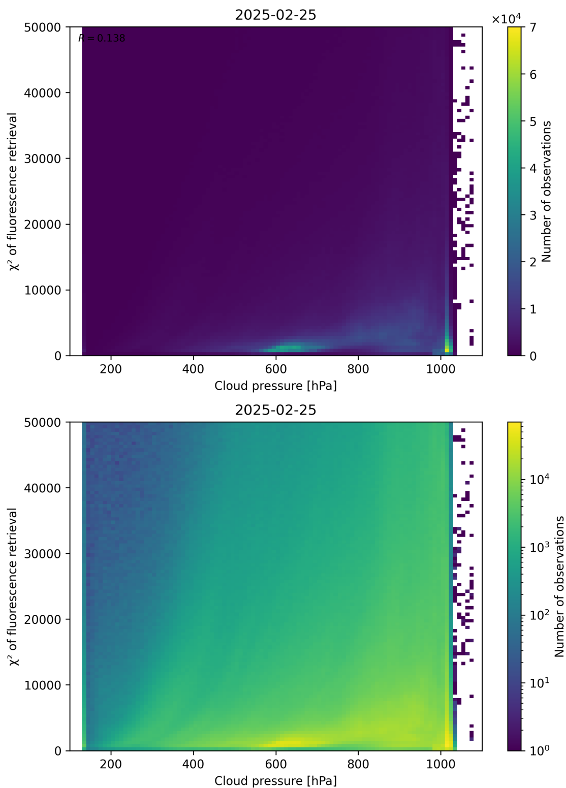
Figure 78: Scatter density plot of “Cloud pressure” against “ \chi^2 of fluorescence retrieval” for 2025-02-24 to 2025-02-26.
