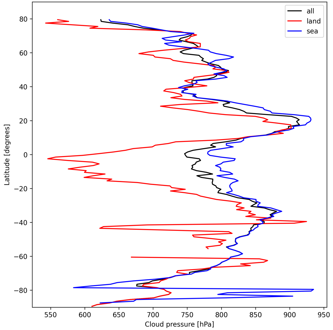
Figure 13: Zonal average of “Cloud pressure” for 2025-02-24 to 2025-02-26.
