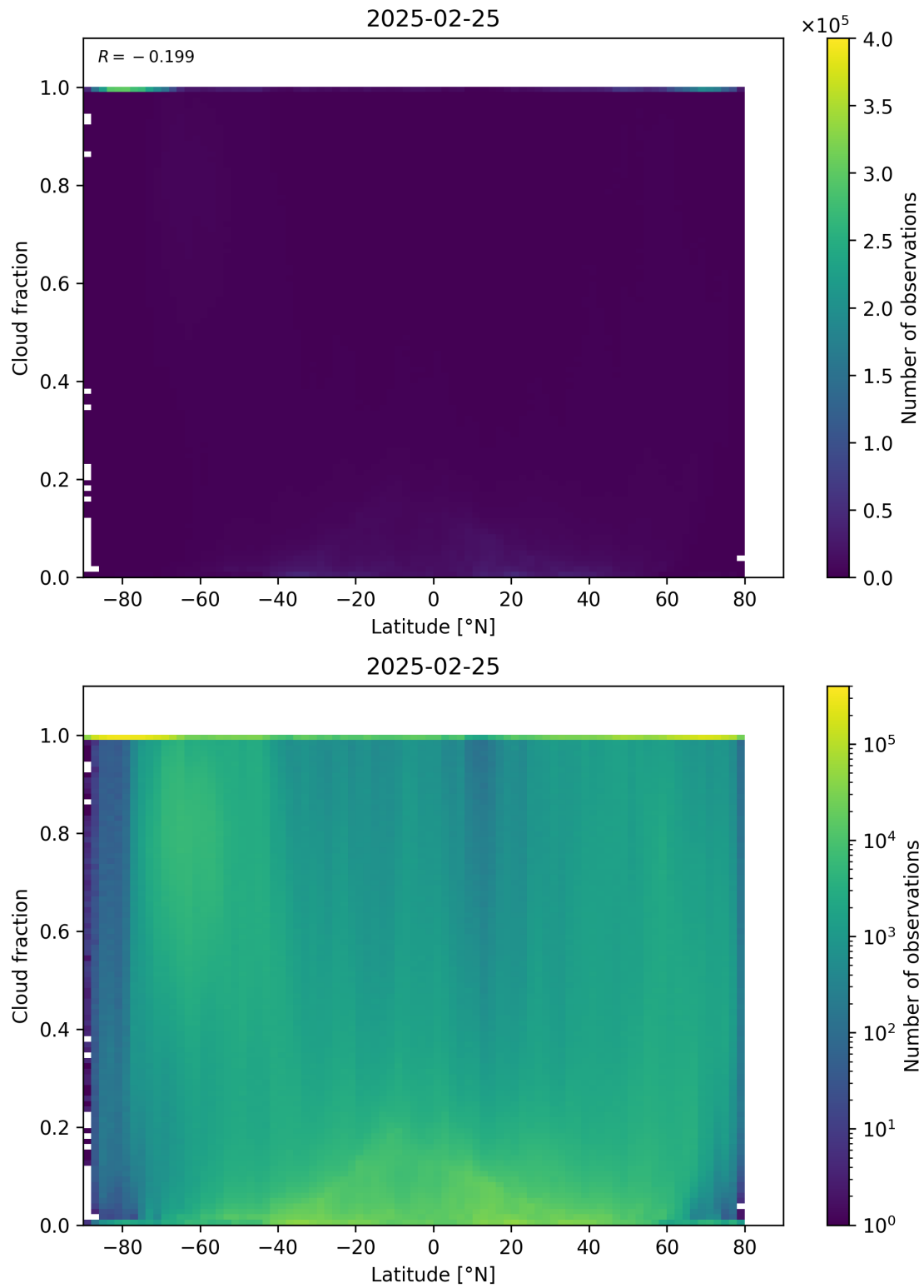
Figure 90: Scatter density plot of “Latitude” against “Cloud fraction” for 2025-02-24 to 2025-02-26.
