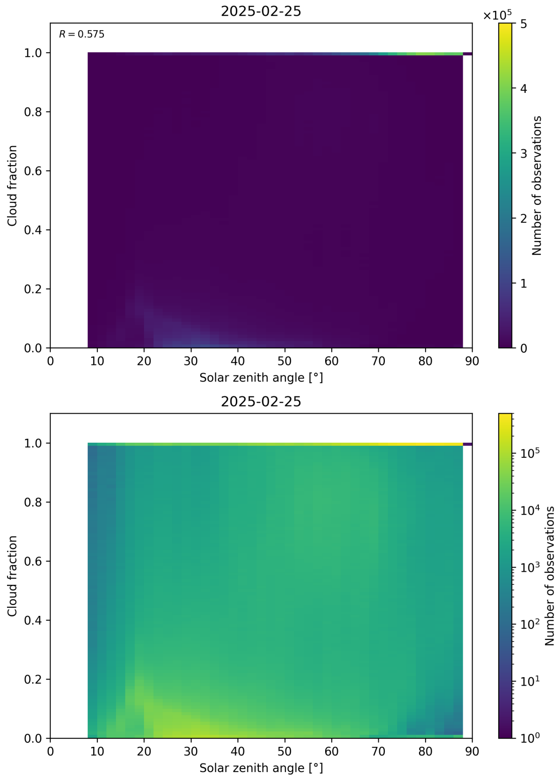
Figure 110: Scatter density plot of “Solar zenith angle” against “Cloud fraction” for 2025-02-24 to 2025-02-26.
