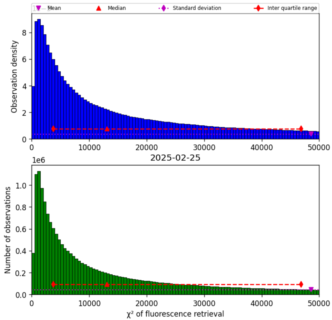
Figure 42: Histogram of “ \chi^2 of fluorescence retrieval” for 2025-02-24 to 2025-02-26
