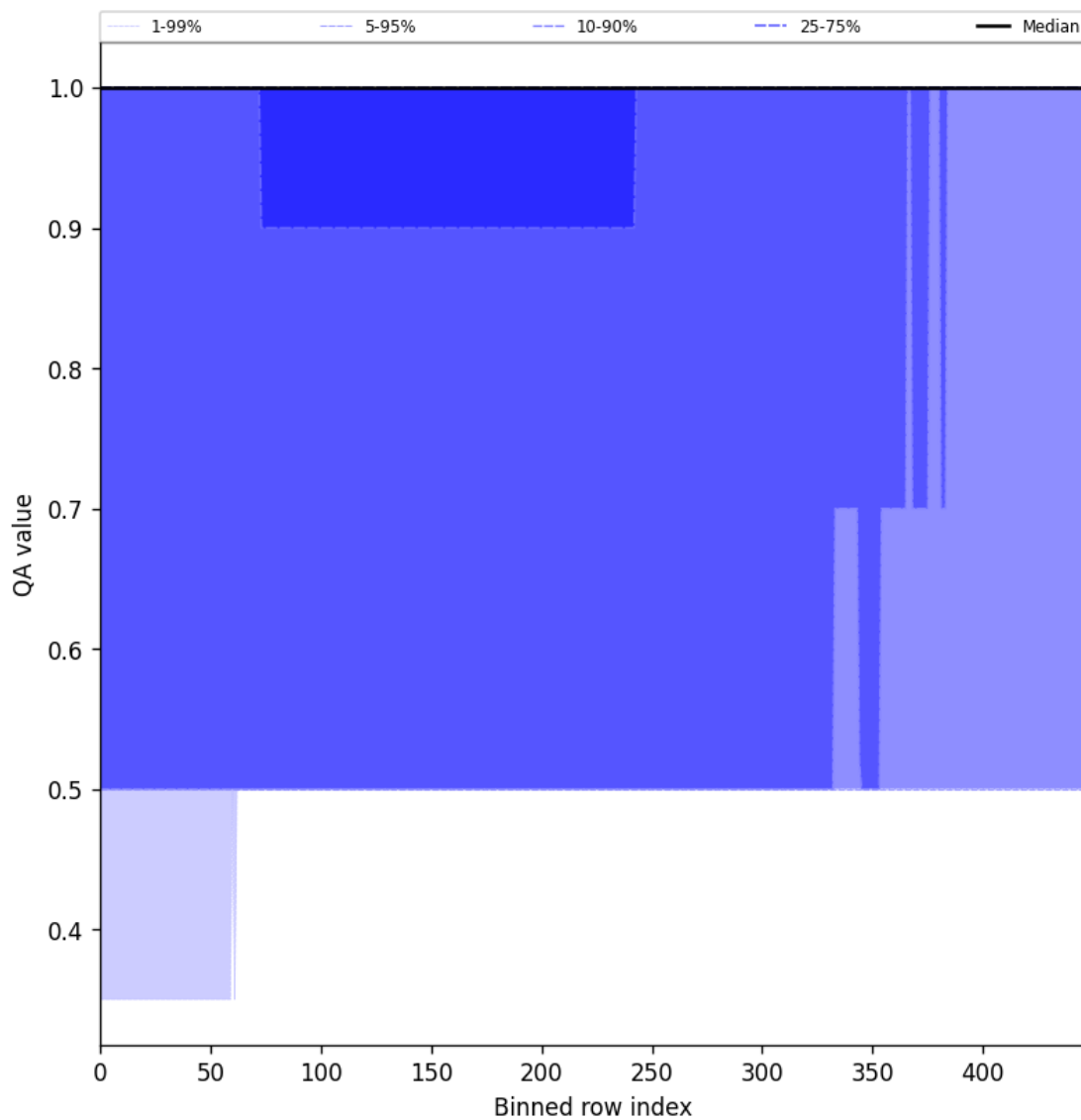
Figure 46: Along track statistics of “QA value” for 2025-02-24 to 2025-02-26
