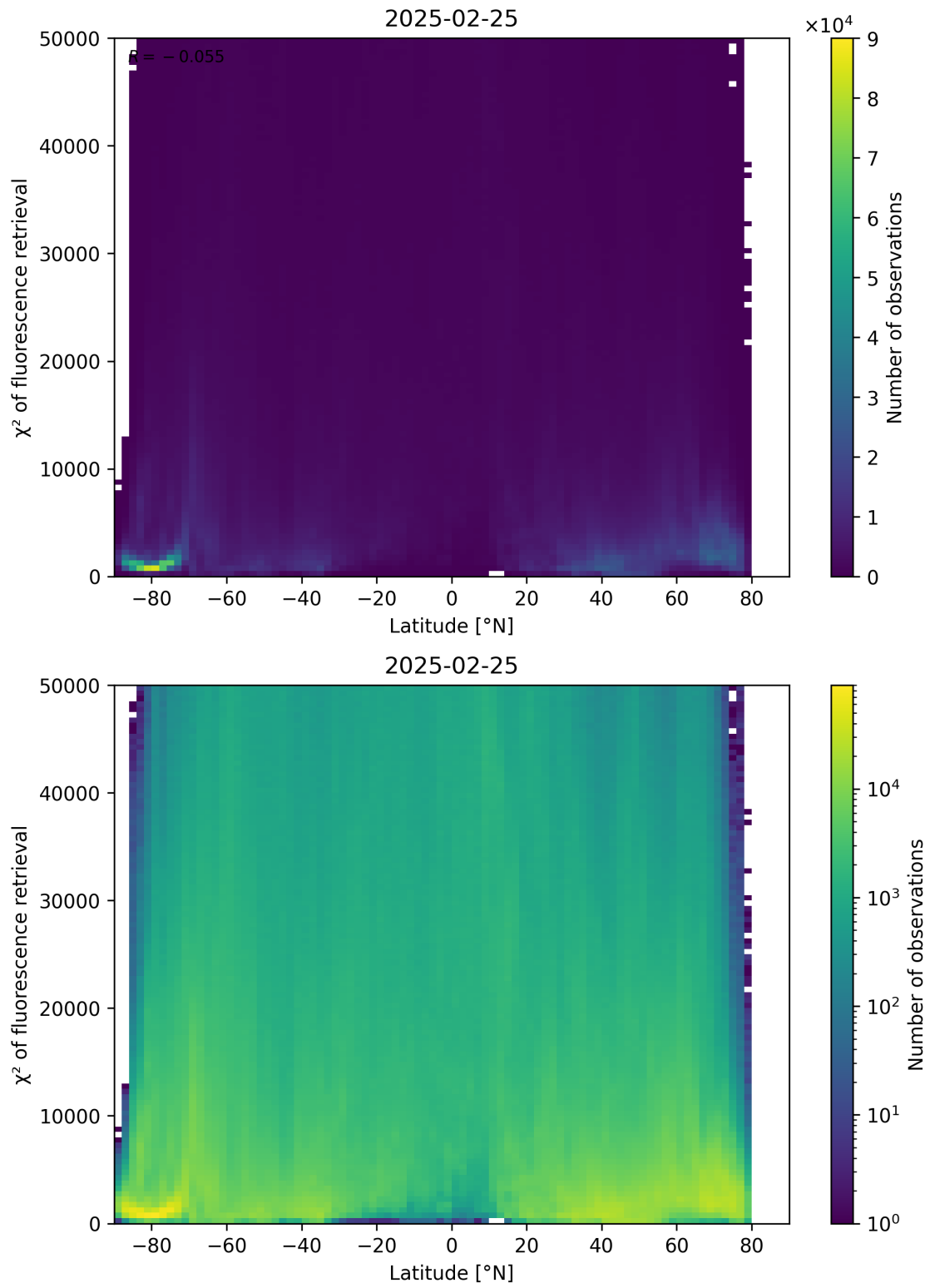
Figure 89: Scatter density plot of “Latitude” against “ \chi^2 of fluorescence retrieval” for 2025-02-24 to 2025-02-26.
