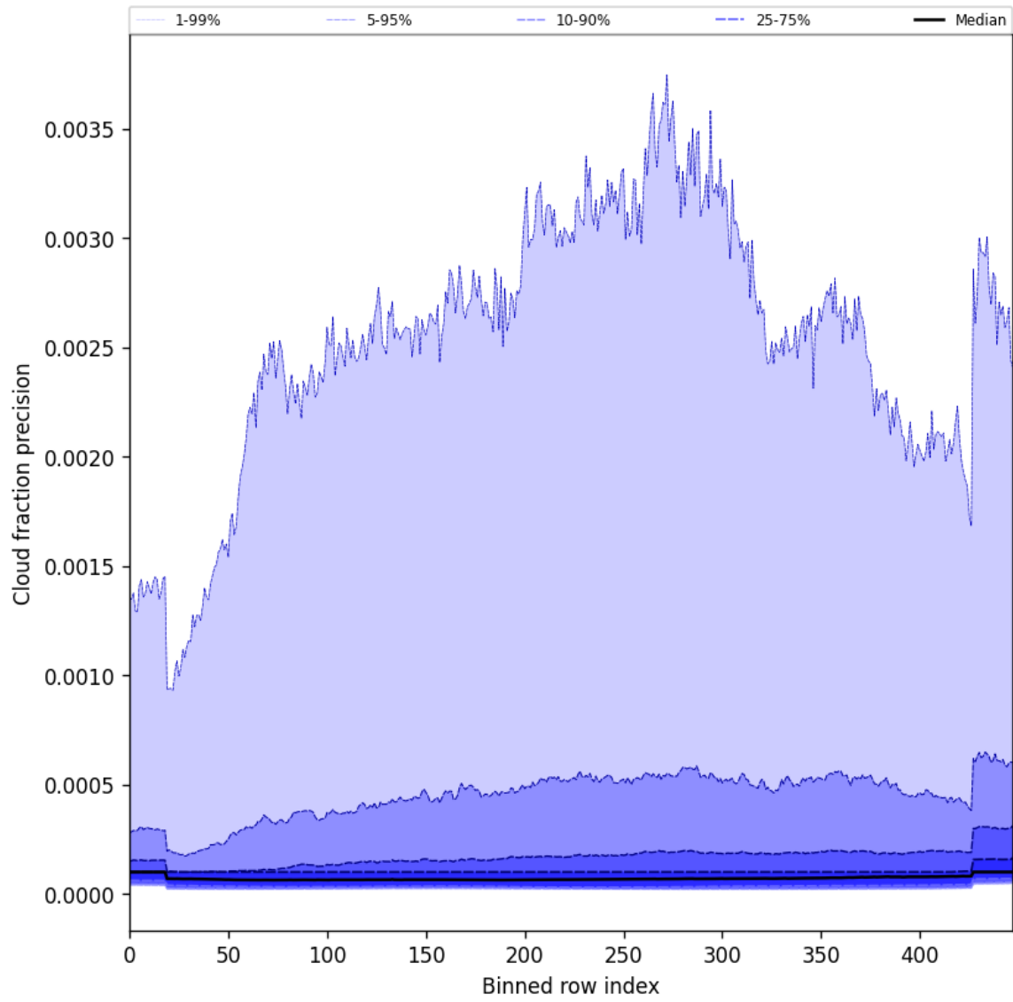
Figure 50: Along track statistics of “Cloud fraction precision” for 2025-02-24 to 2025-02-26
