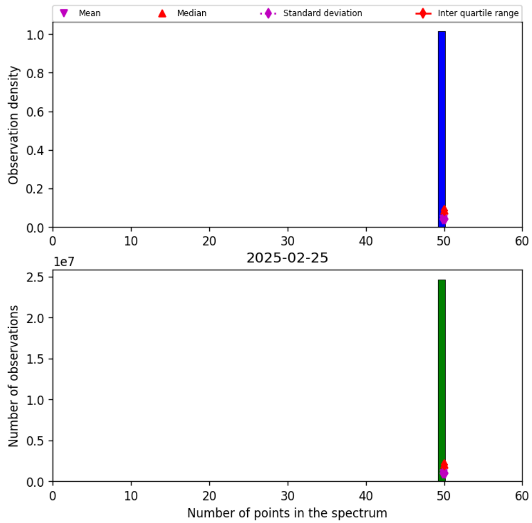
Figure 44: Histogram of "Number of points in the spectrum" for 2025-02-24 to 2025-02-26
