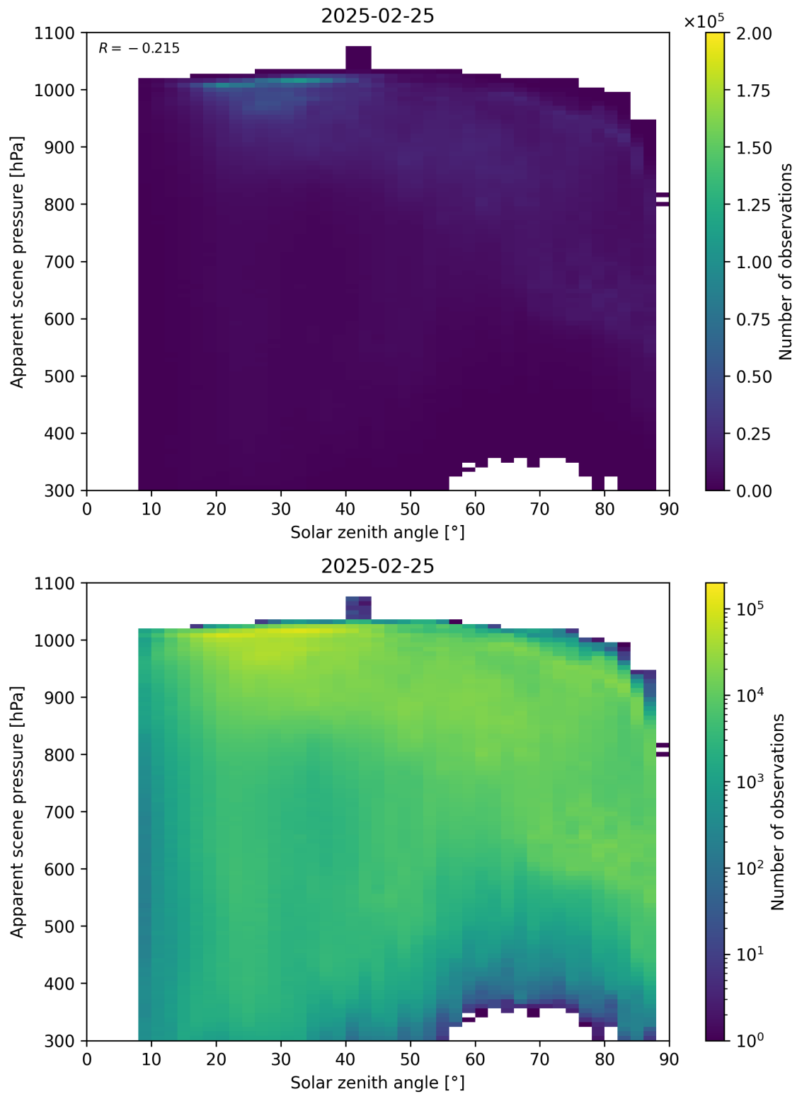
Figure 108: Scatter density plot of “Solar zenith angle” against “Apparent scene pressure” for 2025-02-24 to 2025-02-26.
