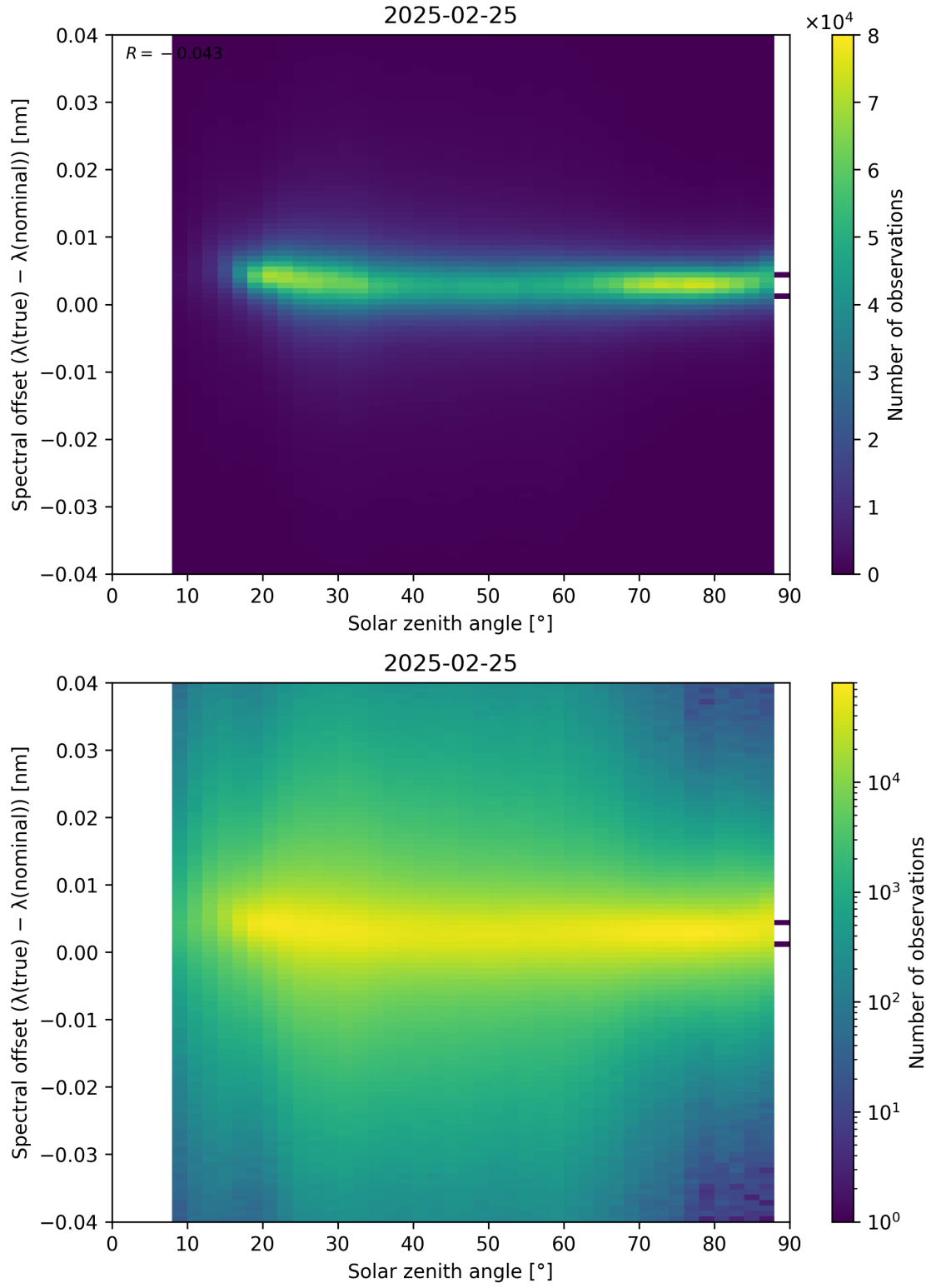
Figure 117: Scatter density plot of “Solar zenith angle” against “Spectral offset ( \lambda_{\text{true}} - \lambda_{\text{nominal}} )” for 2025-02-24 to 2025-02-26.
