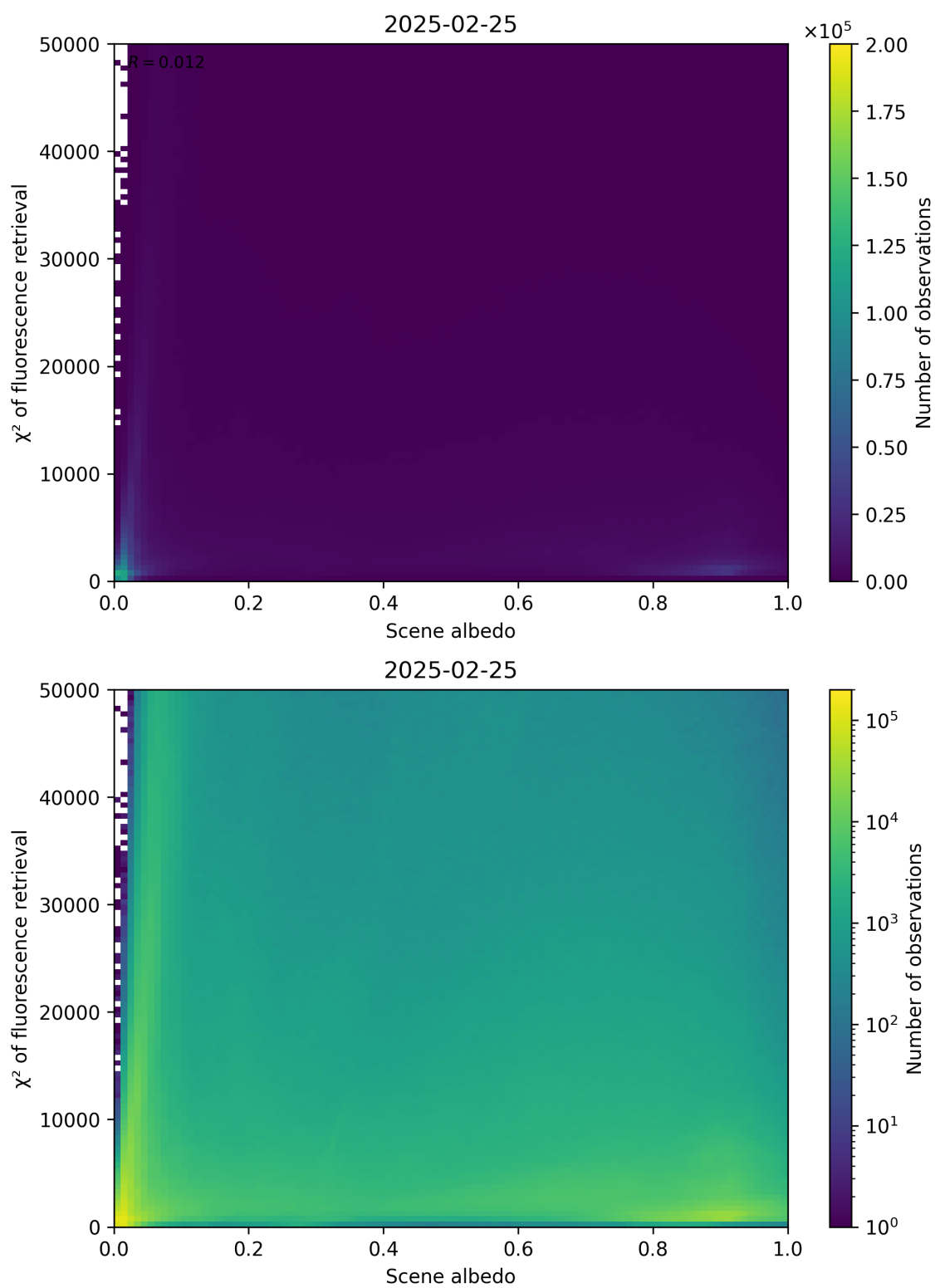
Figure 103: Scatter density plot of “Scene albedo” against “ \chi^2 of fluorescence retrieval” for 2025-02-24 to 2025-02-26.
