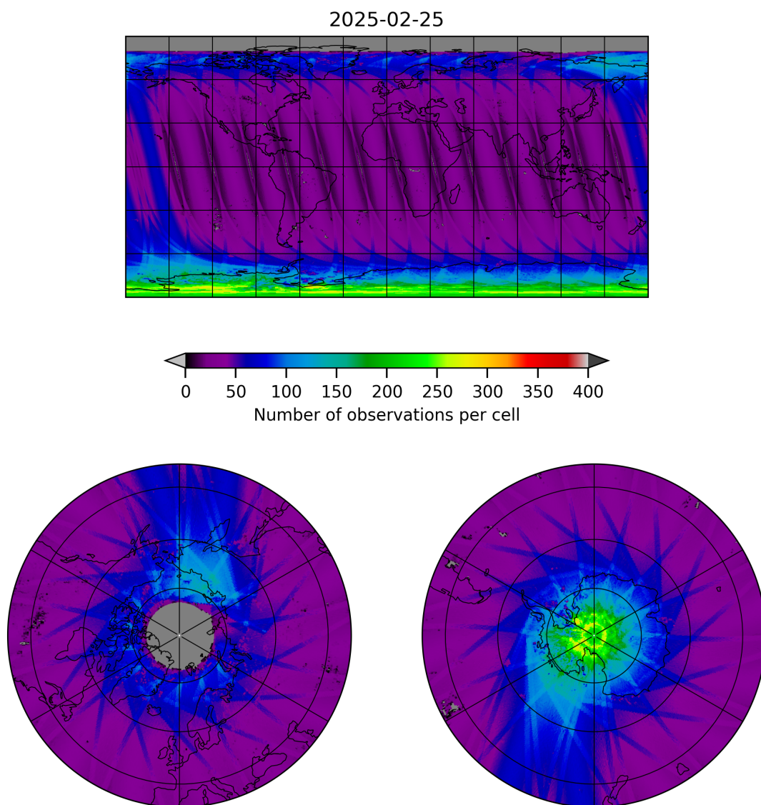
Figure 11: Map of the number of observations for 2025-02-24 to 2025-02-26
