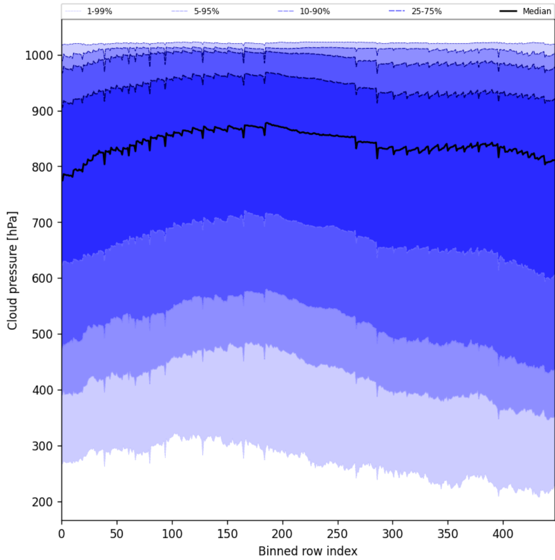
Figure 47: Along track statistics of “Cloud pressure” for 2025-02-24 to 2025-02-26
