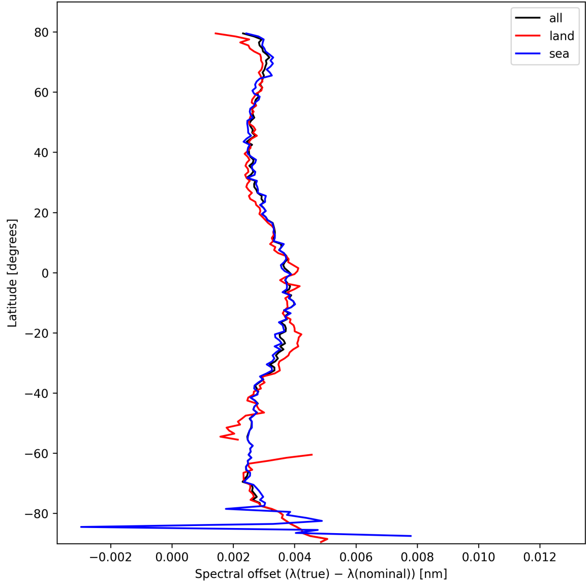
Figure 28: Zonal average of “Spectral offset ( \lambda_{\text{true}} - \lambda_{\text{nominal}} )” for 2025-02-24 to 2025-02-26.
