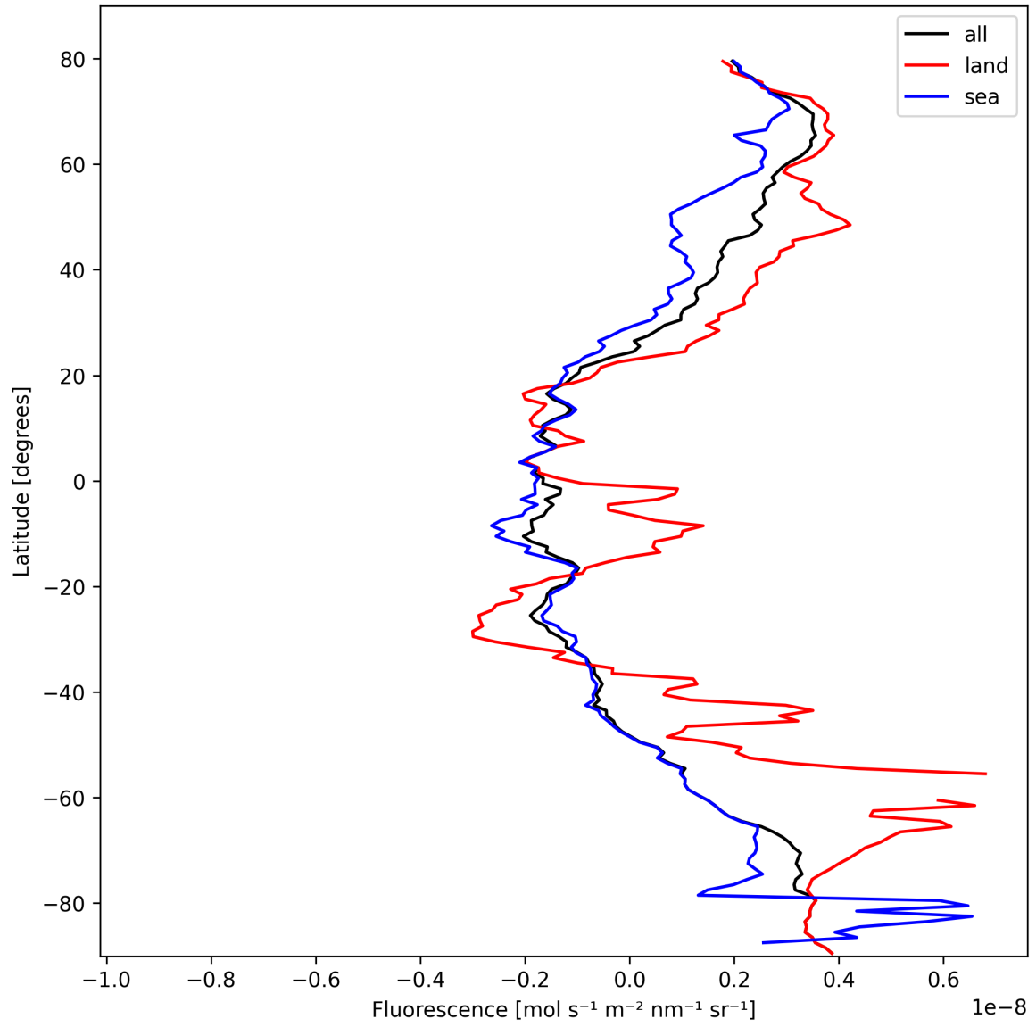
Figure 23: Zonal average of “Fluorescence” for 2025-02-24 to 2025-02-26.
