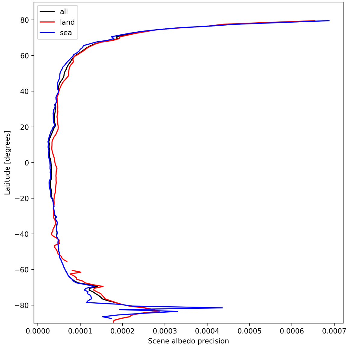
Figure 18: Zonal average of “Scene albedo precision” for 2025-02-24 to 2025-02-26.
