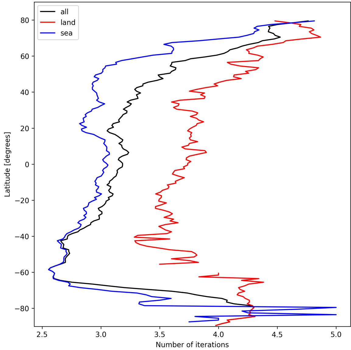
Figure 22: Zonal average of “Number of iterations” for 2025-02-24 to 2025-02-26.
