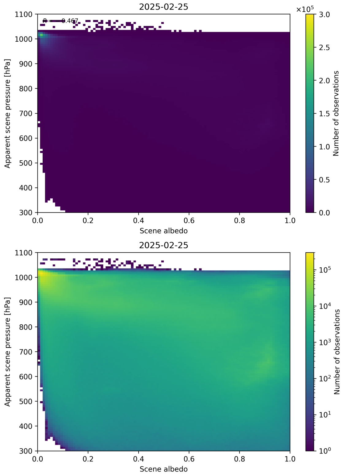
Figure 102: Scatter density plot of “Scene albedo” against “Apparent scene pressure” for 2025-02-24 to 2025-02-26.
