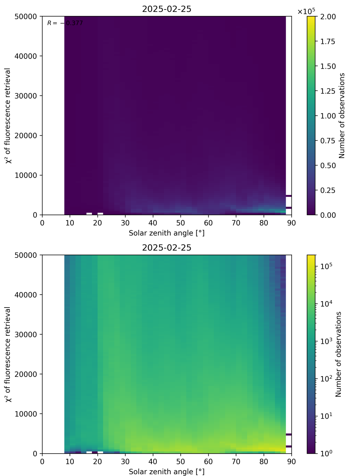
Figure 109: Scatter density plot of “Solar zenith angle” against “ \chi^2 of fluorescence retrieval” for 2025-02-24 to 2025-02-26.
