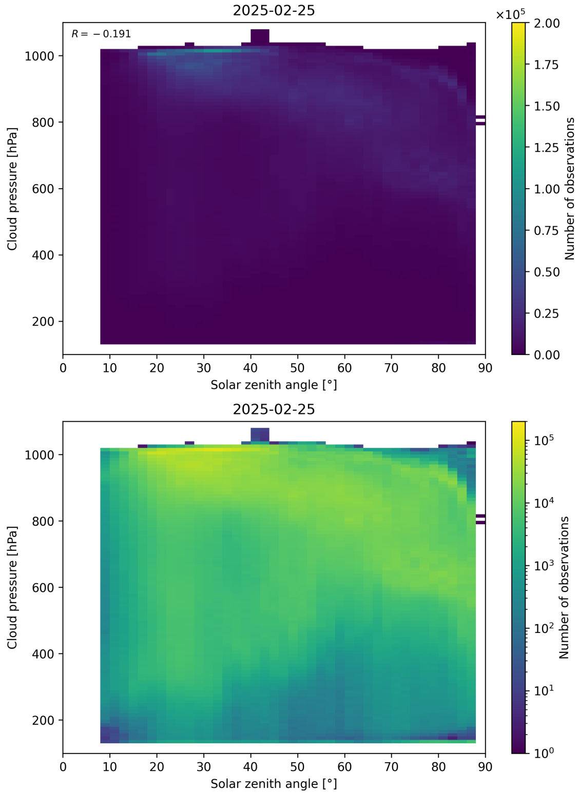
Figure 111: Scatter density plot of “Solar zenith angle” against “Cloud pressure” for 2025-02-24 to 2025-02-26.
