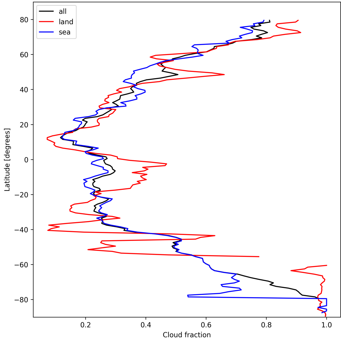
Figure 15: Zonal average of “Cloud fraction” for 2025-02-24 to 2025-02-26.
