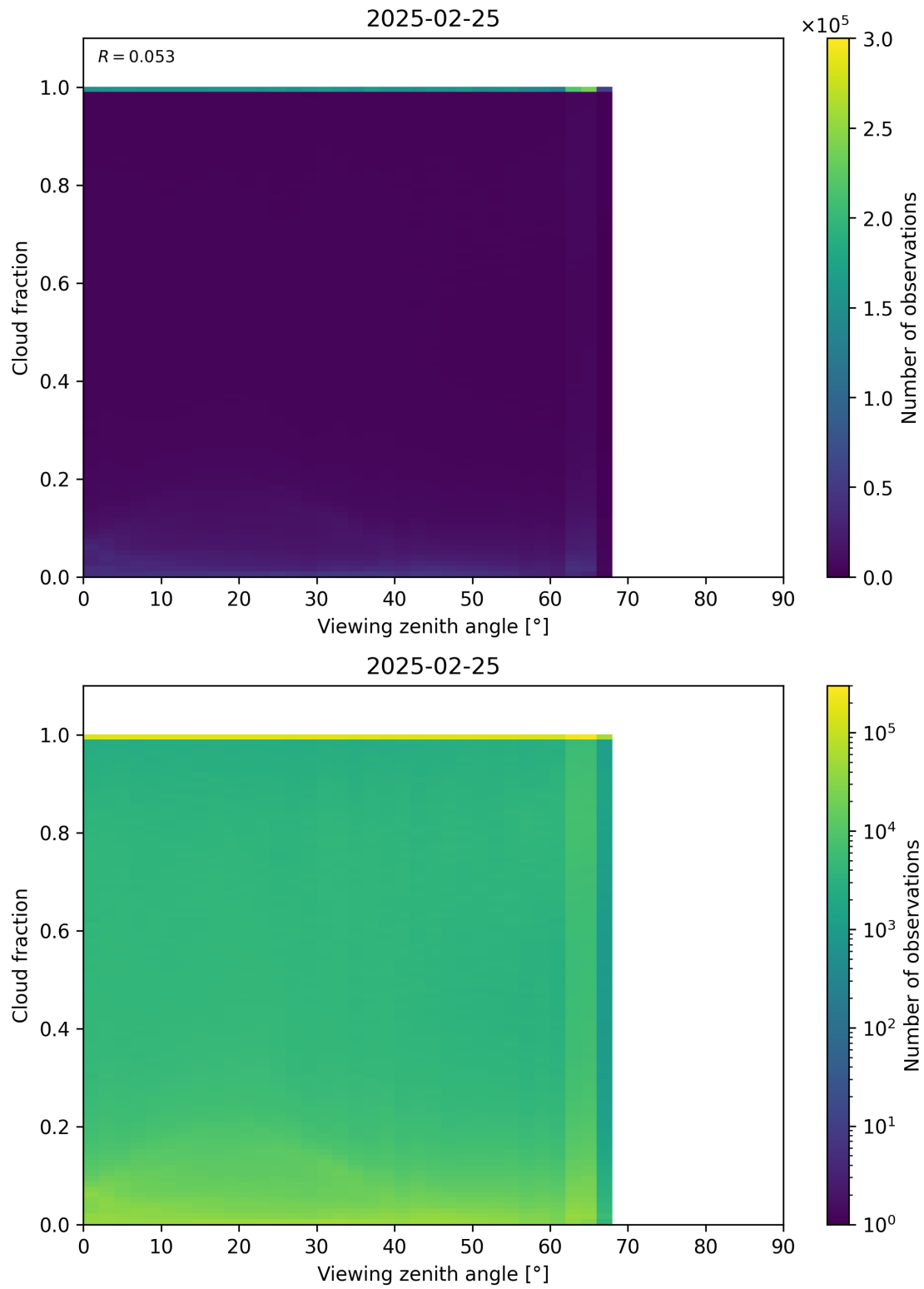
Figure 120: Scatter density plot of “Viewing zenith angle” against “Cloud fraction” for 2025-02-24 to 2025-02-26.
