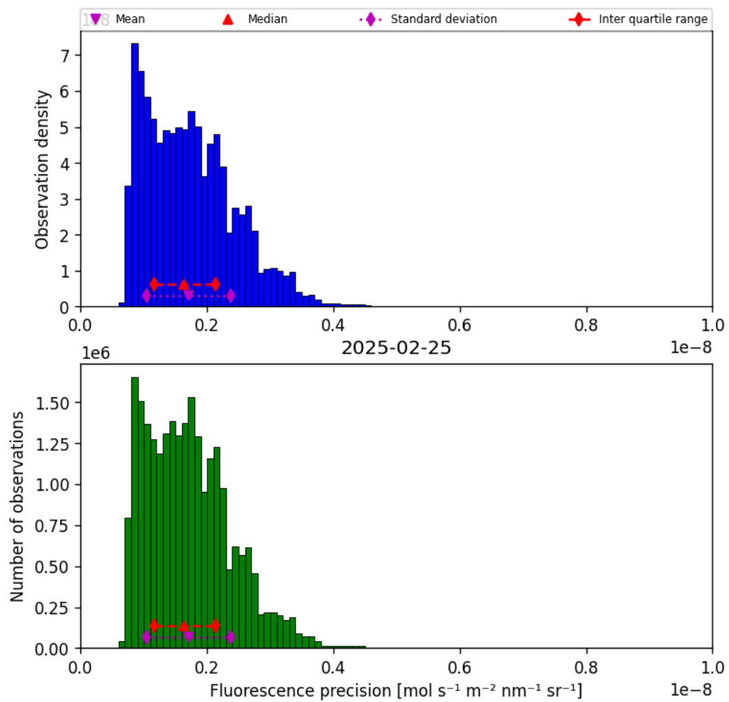
Figure 41: Histogram of “Fluorescence precision” for 2025-02-24 to 2025-02-26
