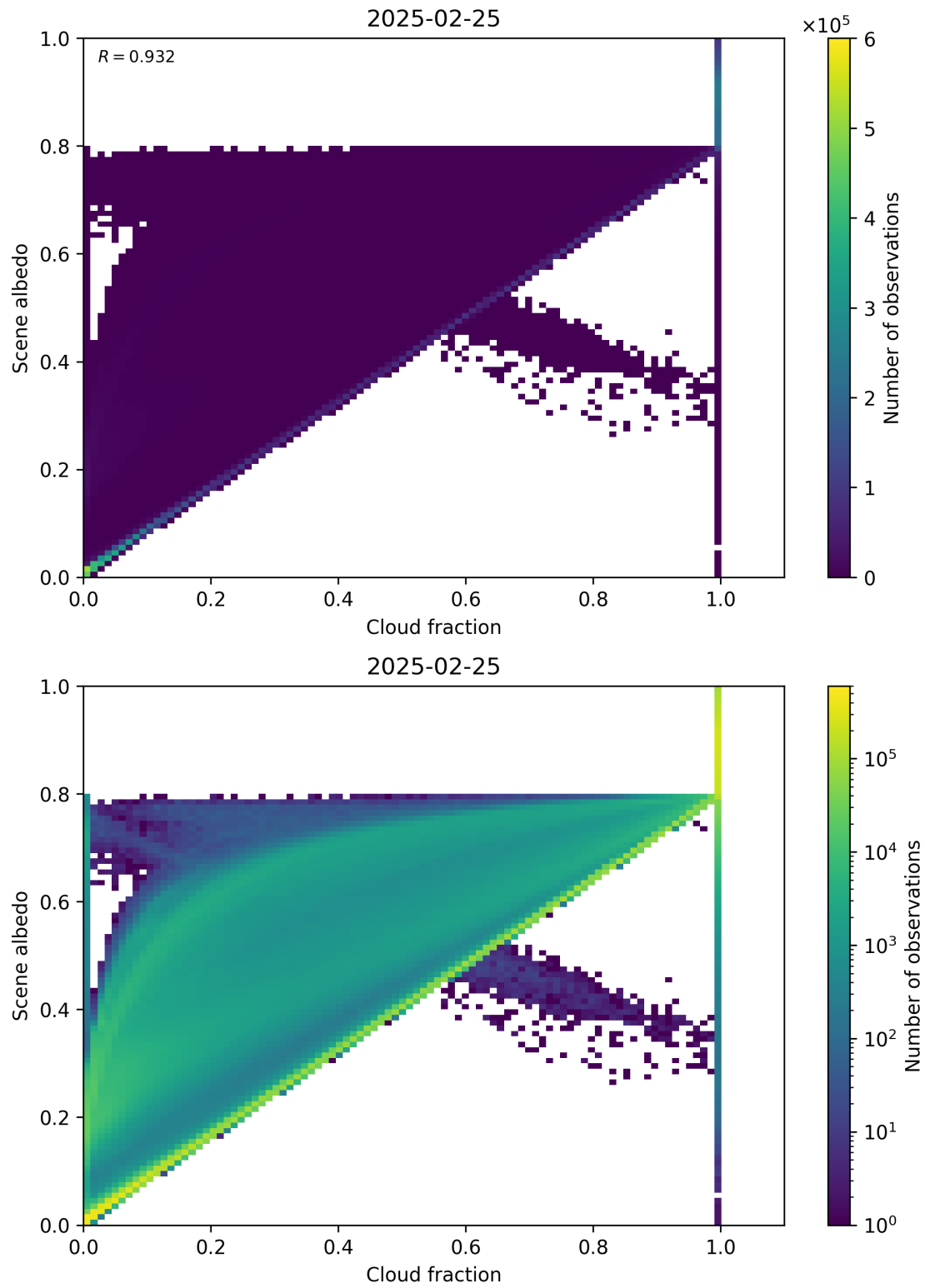
Figure 75: Scatter density plot of “Cloud fraction” against “Scene albedo” for 2025-02-24 to 2025-02-26.
