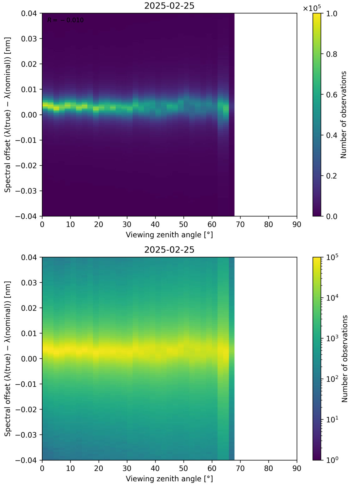
Figure 128: Scatter density plot of “Viewing zenith angle” against “Spectral offset ( \lambda_{\text{true}} - \lambda_{\text{nominal}} )” for 2025-02-24 to 2025-02-26.
