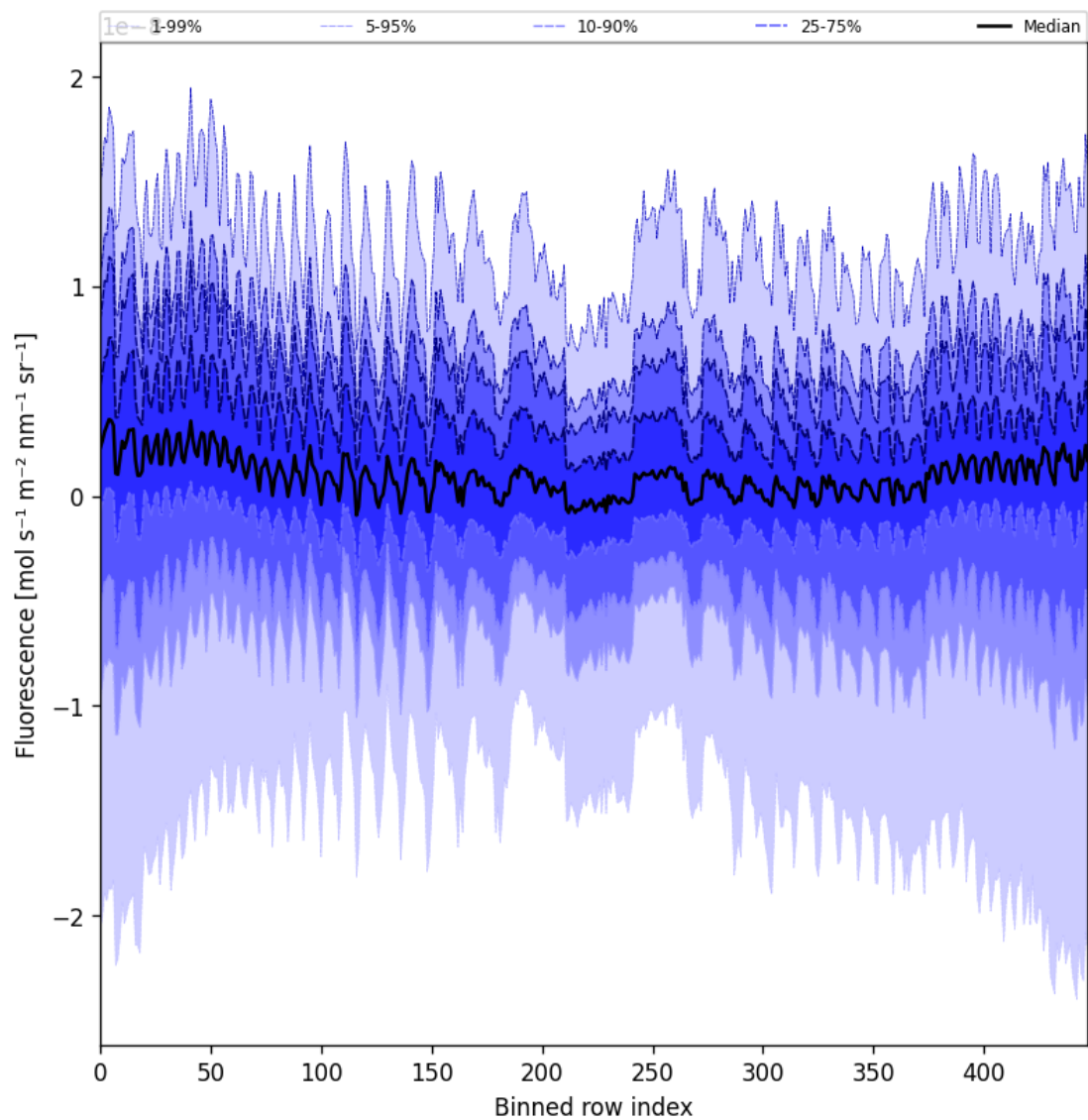
Figure 57: Along track statistics of “Fluorescence” for 2025-02-24 to 2025-02-26
