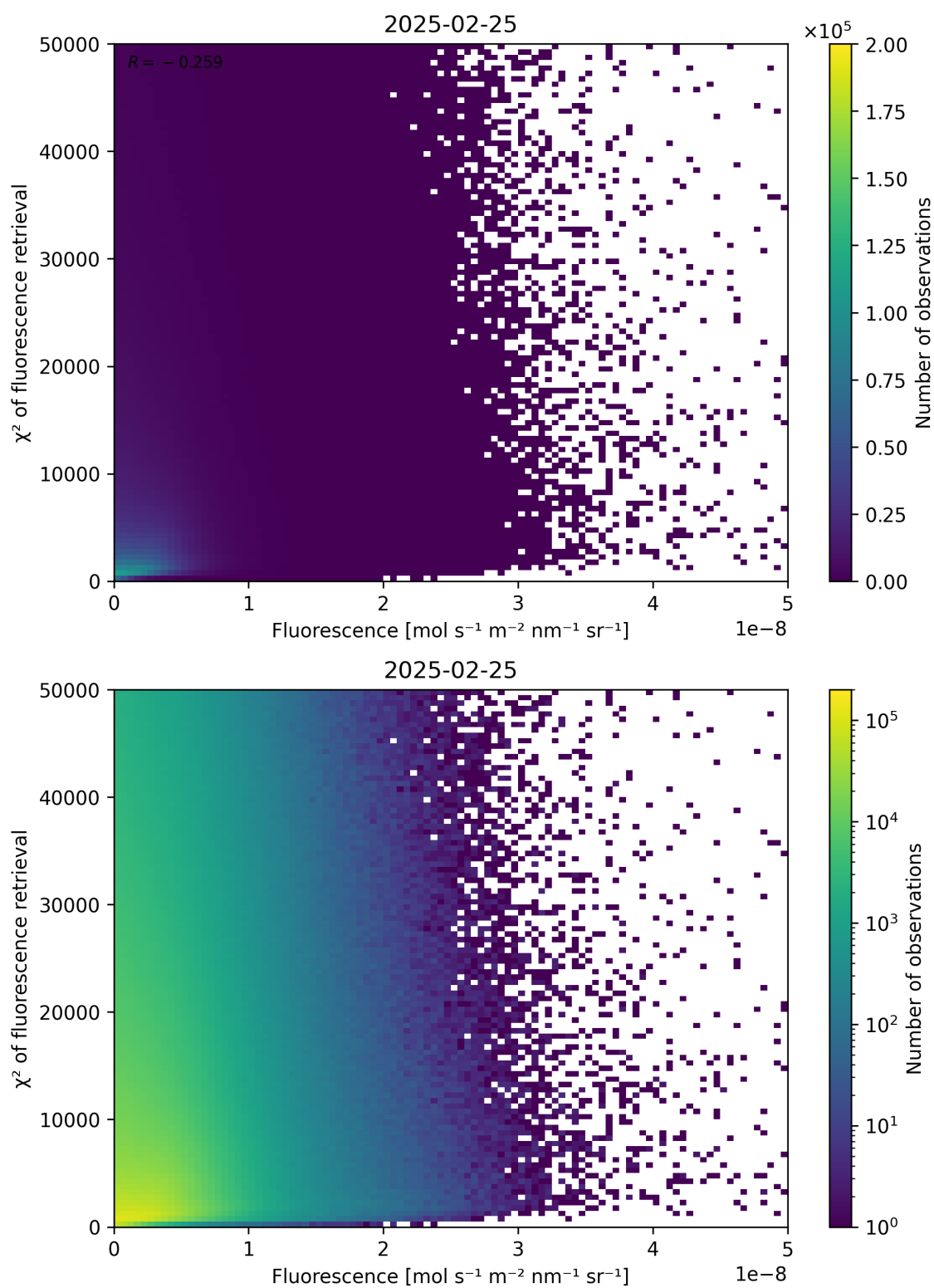
Figure 85: Scatter density plot of “Fluorescence” against “ \chi^2 of fluorescence retrieval” for 2025-02-24 to 2025-02-26.
