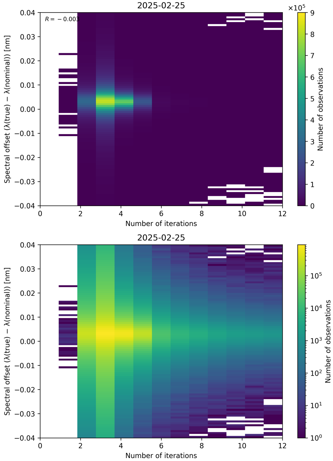
Figure 100: Scatter density plot of “Number of iterations” against “Spectral offset ( \lambda_{\text{true}} - \lambda_{\text{nominal}} )” for 2025-02-24 to 2025-02-26.
