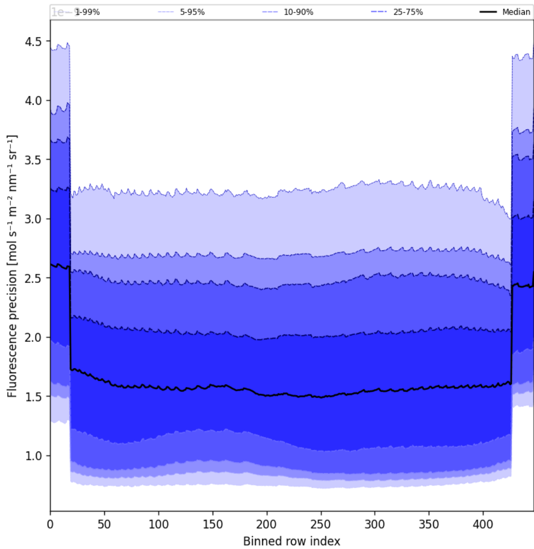
Figure 58: Along track statistics of “Fluorescence precision” for 2025-02-24 to 2025-02-26
