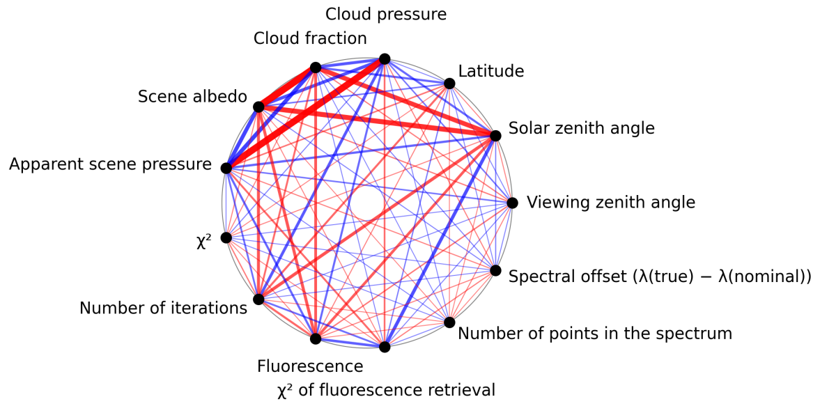
Figure 1: Map of correlation graph for 2025-02-24 to 2025-02-26.
