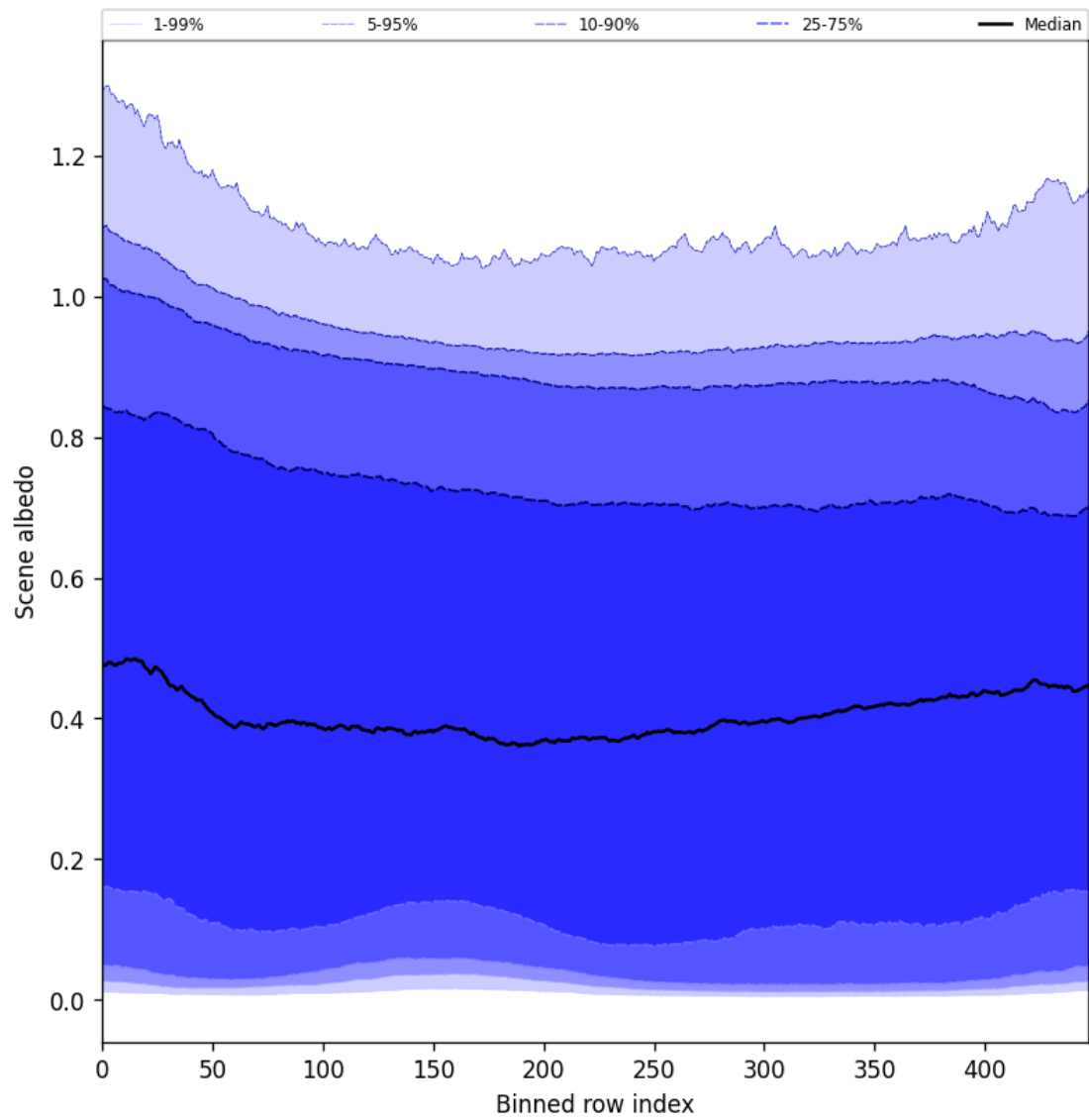
Figure 51: Along track statistics of “Scene albedo” for 2025-02-24 to 2025-02-26
