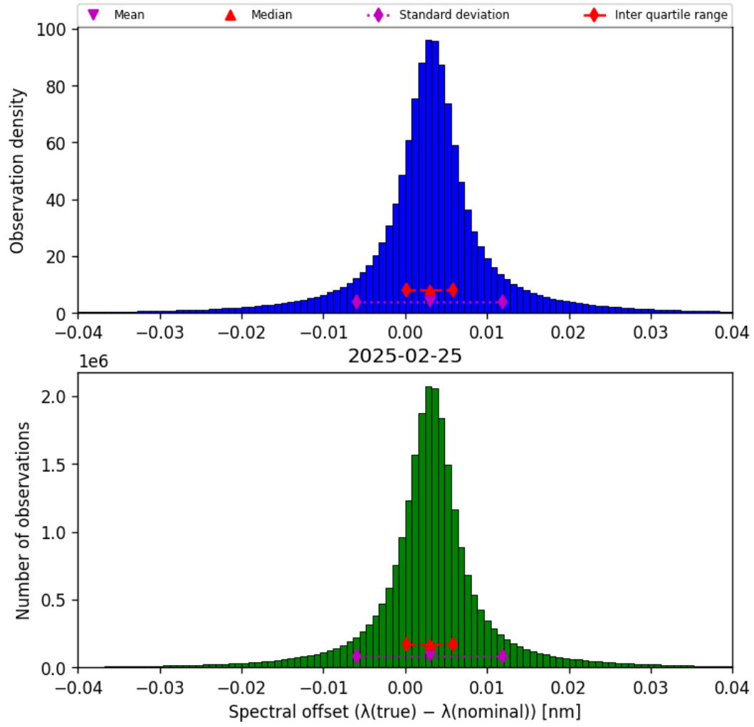
Figure 45: Histogram of “Spectral offset ( \lambda_{\text{true}} - \lambda_{\text{nominal}} )” for 2025-02-24 to 2025-02-26
