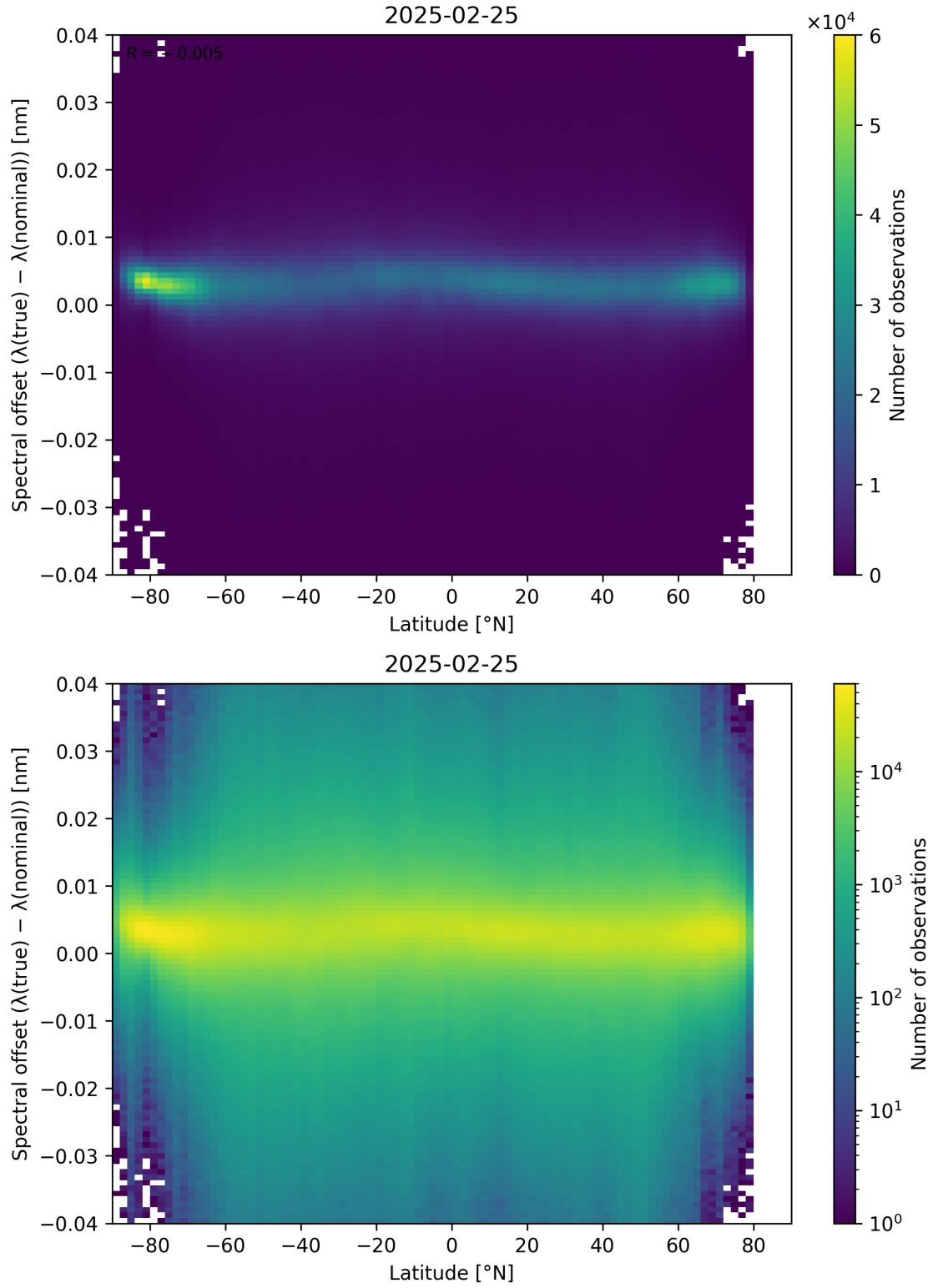
Figure 96: Scatter density plot of “Latitude” against “Spectral offset ( \lambda_{\text{true}} - \lambda_{\text{nominal}} )” for 2025-02-24 to 2025-02-26.
