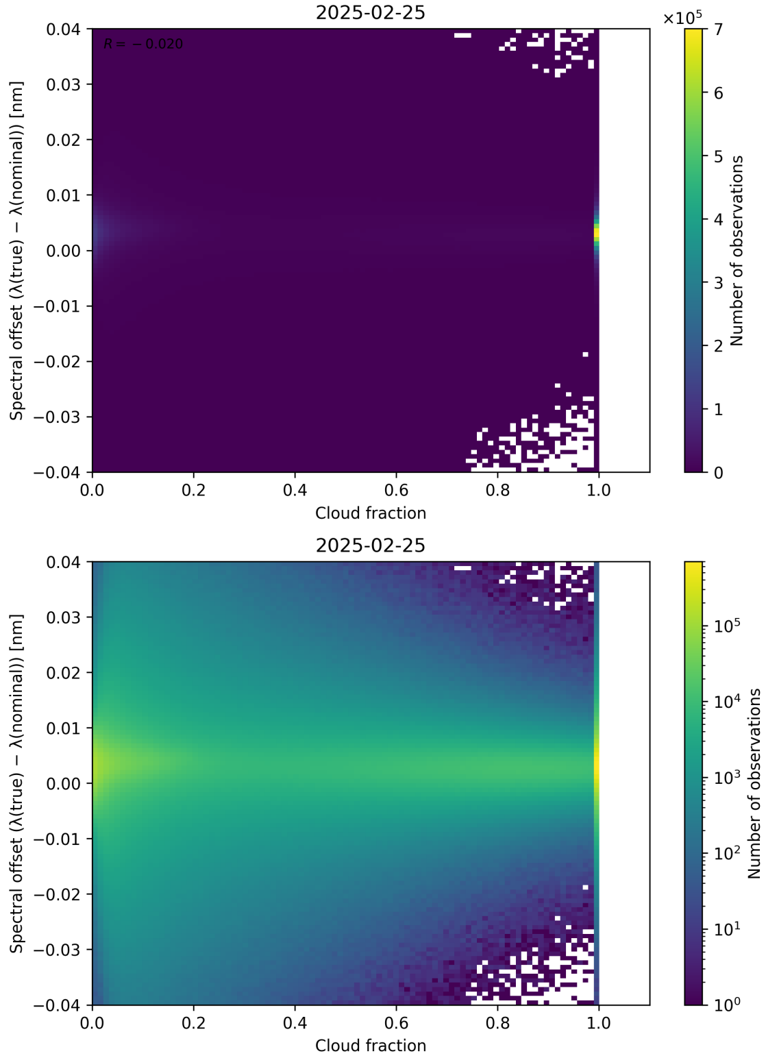
Figure 76: Scatter density plot of “Cloud fraction” against “Spectral offset ( \lambda_{\text{true}} - \lambda_{\text{nominal}} )” for 2025-02-24 to 2025-02-26.
