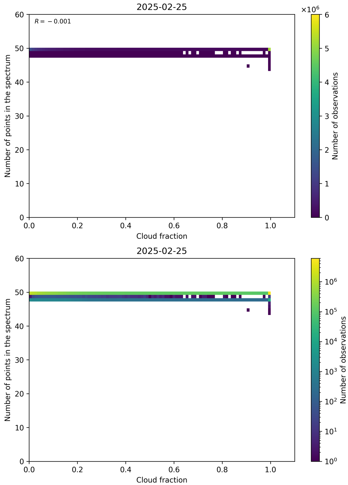
Figure 74: Scatter density plot of “Cloud fraction” against “Number of points in the spectrum” for 2025-02-24 to 2025-02-26.
