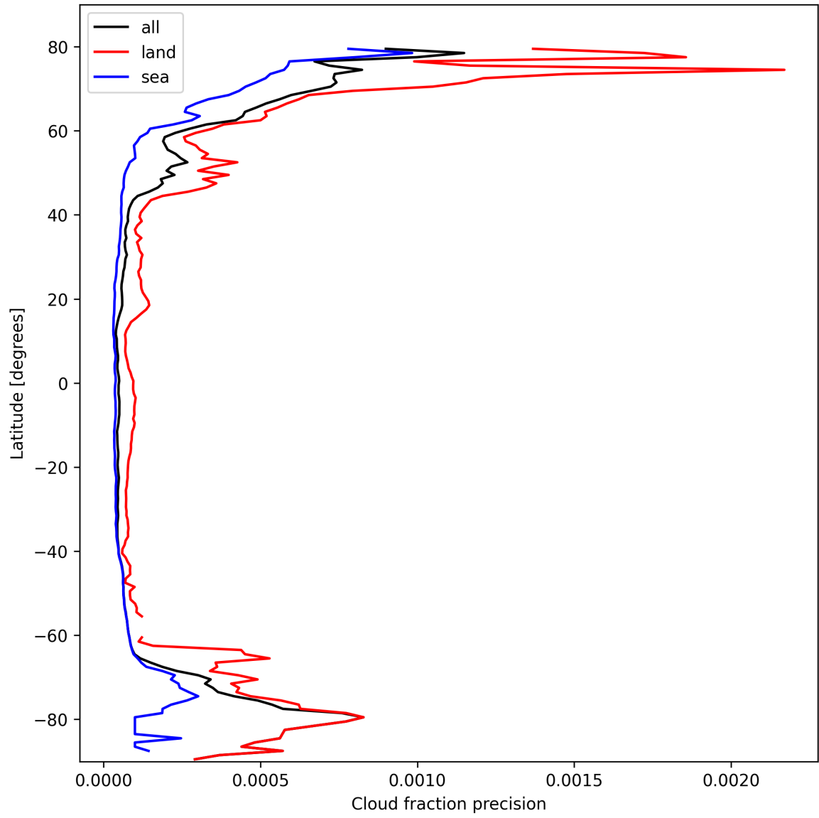
Figure 16: Zonal average of “Cloud fraction precision” for 2025-02-24 to 2025-02-26.
