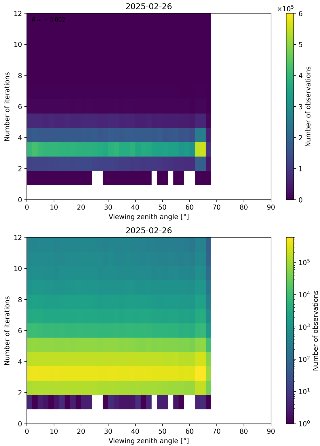
Figure 124: Scatter density plot of “Viewing zenith angle” against “Number of iterations” for 2025-02-25 to 2025-02-27.
