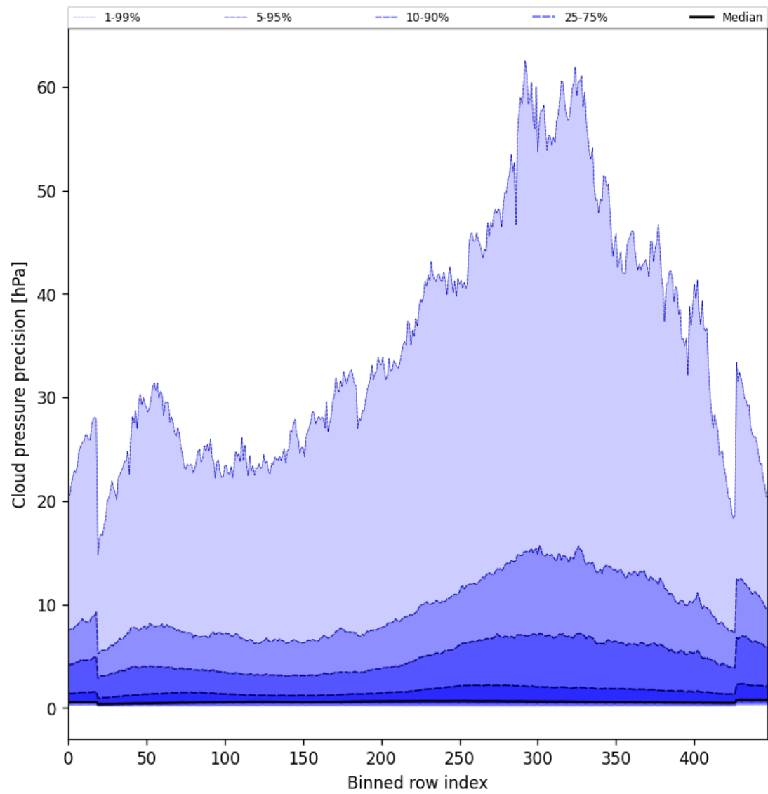
Figure 48: Along track statistics of “Cloud pressure precision” for 2025-02-25 to 2025-02-27
