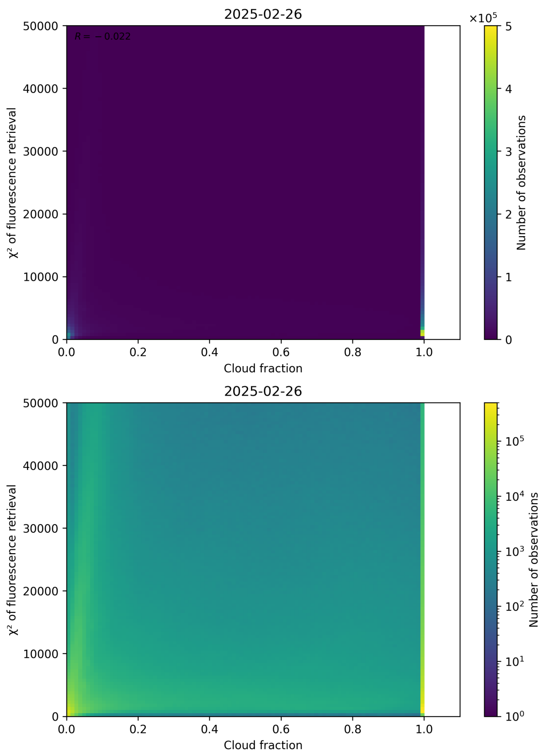
Figure 71: Scatter density plot of “Cloud fraction” against “ \chi^2 of fluorescence retrieval” for 2025-02-25 to 2025-02-27.
