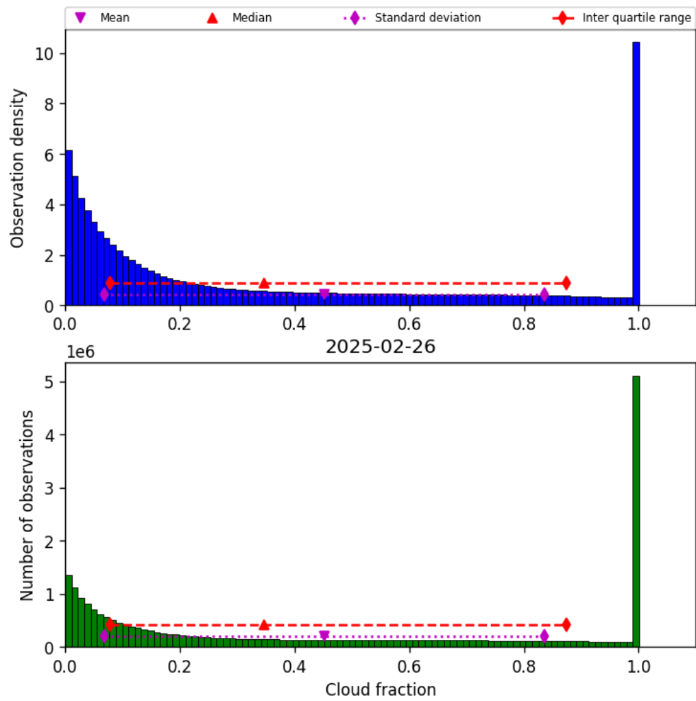
Figure 32: Histogram of “Cloud fraction” for 2025-02-25 to 2025-02-27
