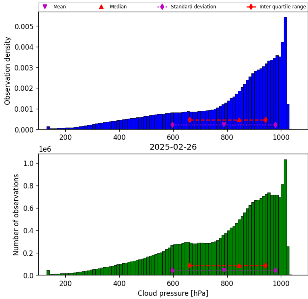
Figure 30: Histogram of “Cloud pressure” for 2025-02-25 to 2025-02-27
