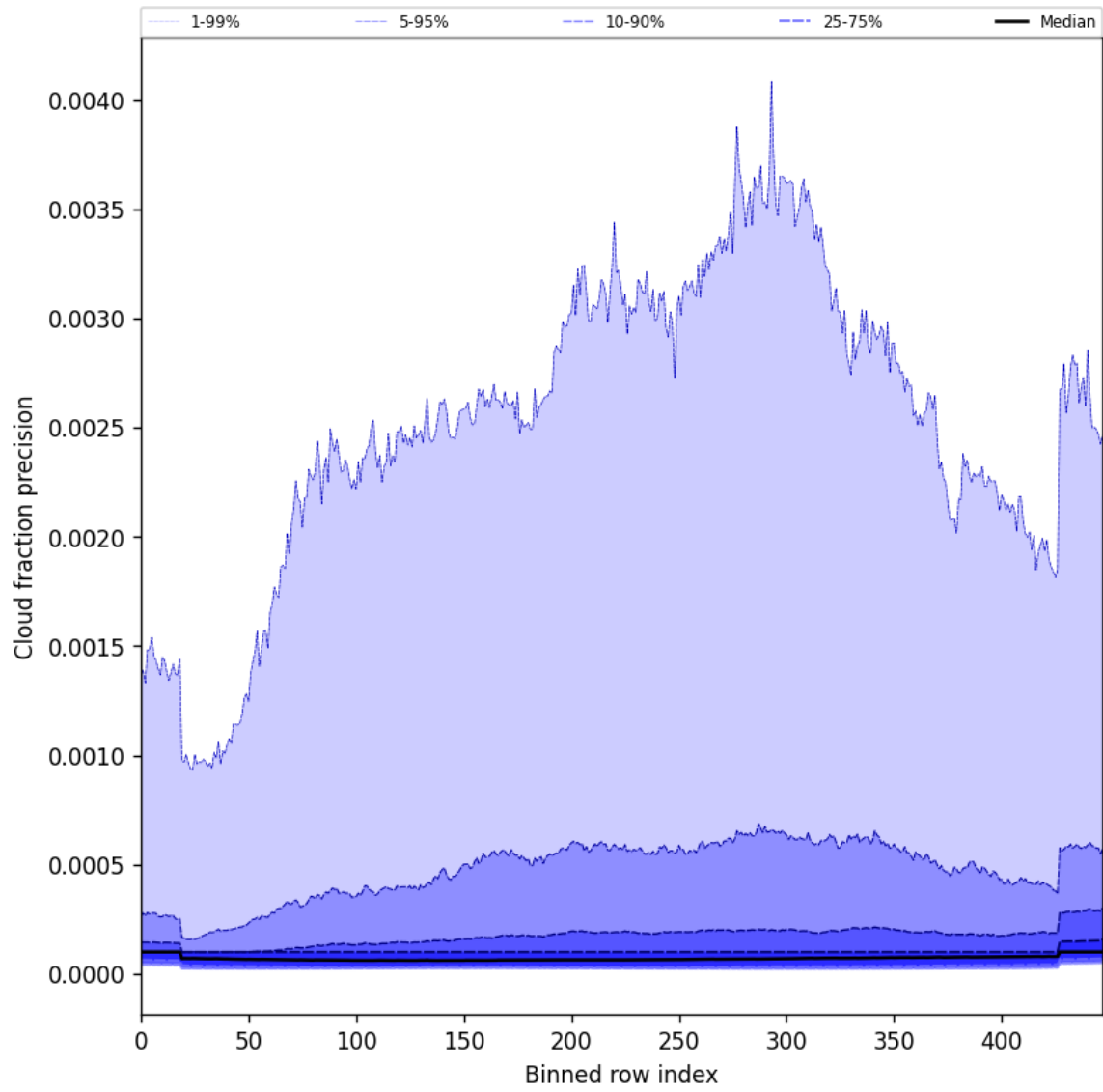
Figure 50: Along track statistics of “Cloud fraction precision” for 2025-02-25 to 2025-02-27
