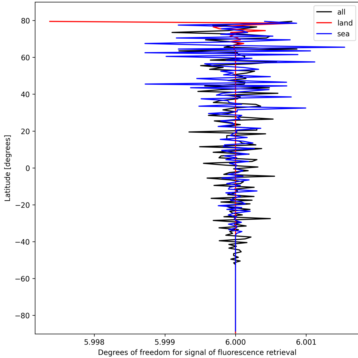
Figure 26: Zonal average of “Degrees of freedom for signal of fluorescence retrieval” for 2025-02-25 to 2025-02-27.
