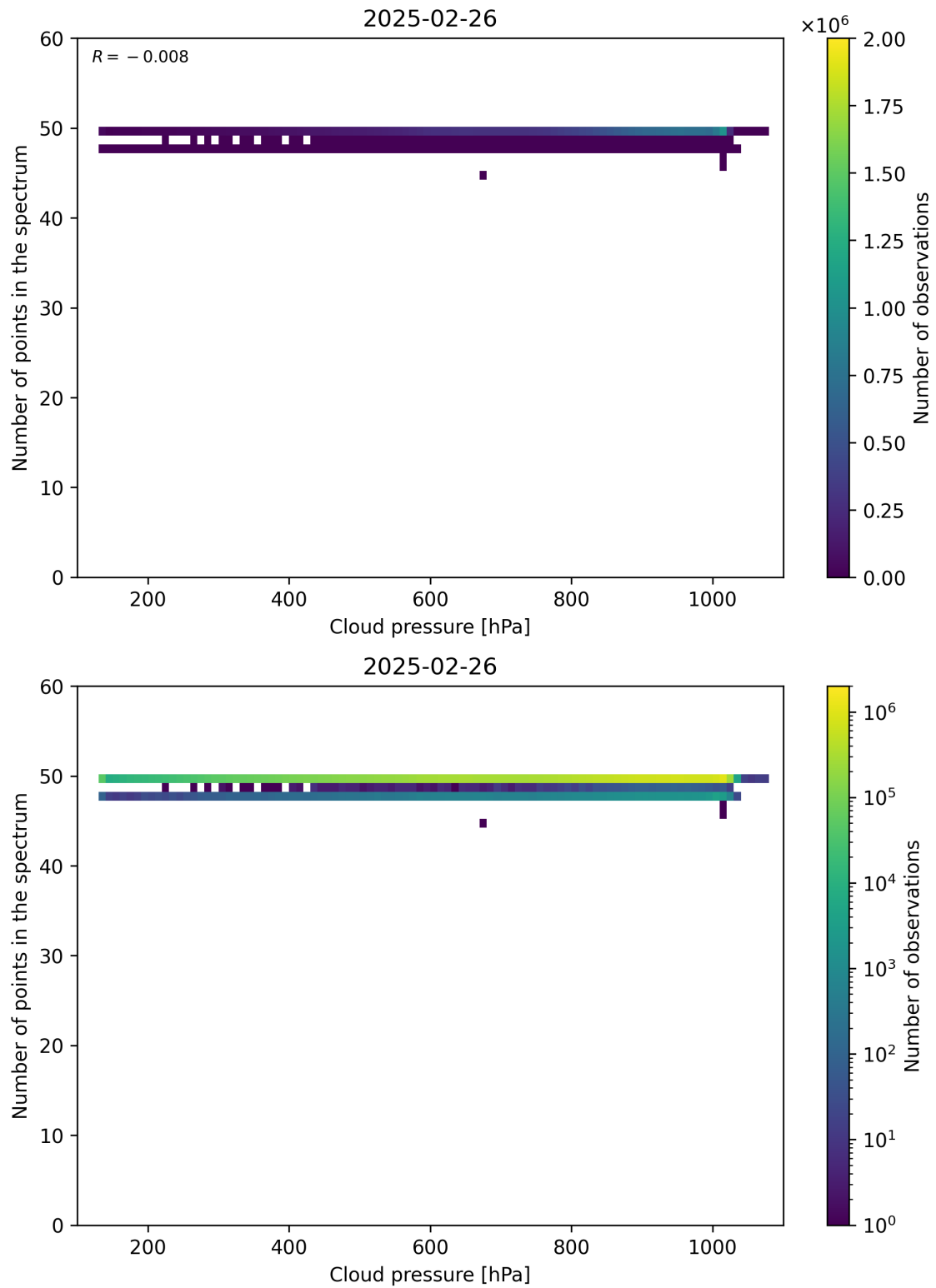
Figure 82: Scatter density plot of “Cloud pressure” against “Number of points in the spectrum” for 2025-02-25 to 2025-02-27.
