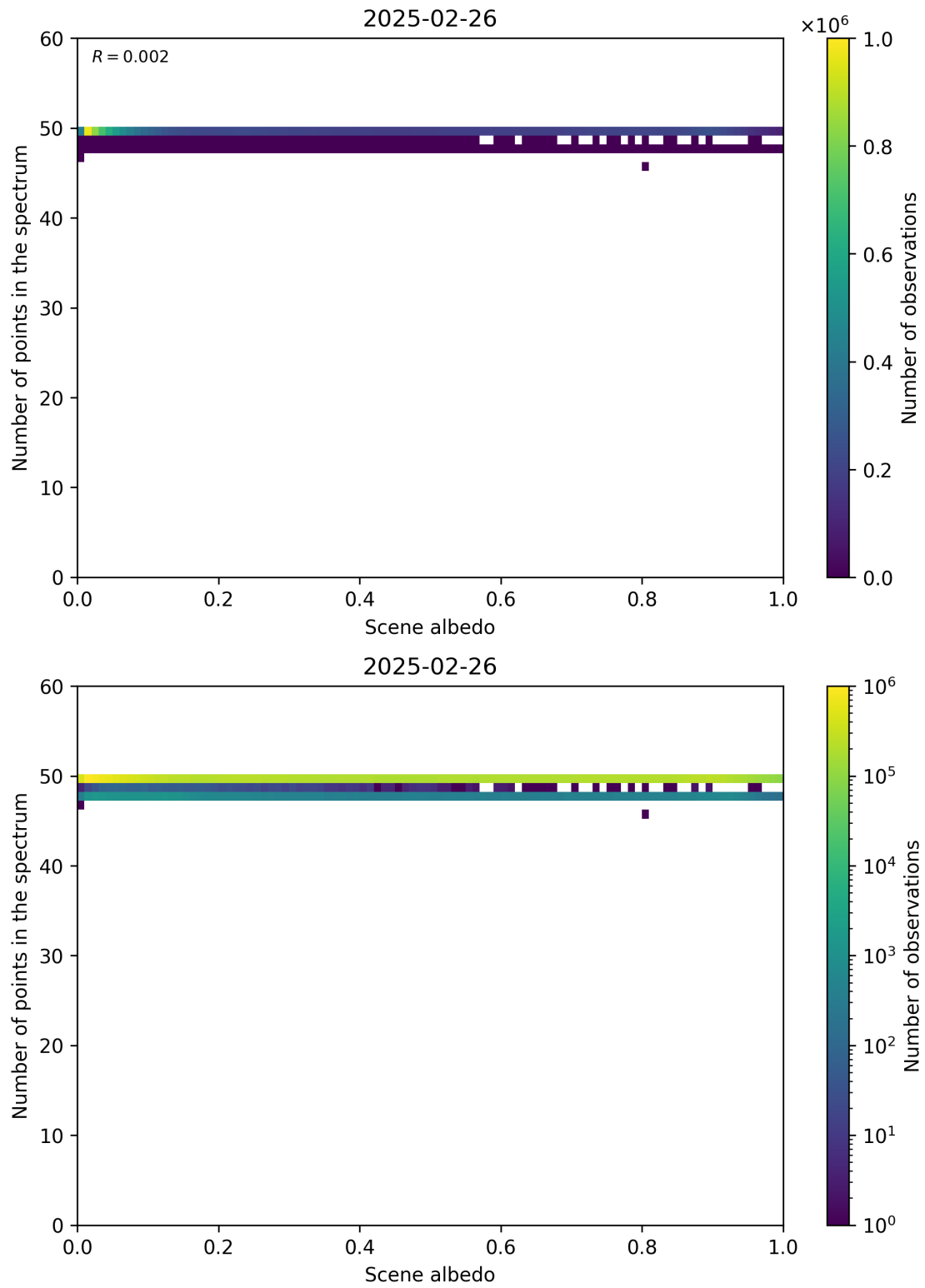
Figure 106: Scatter density plot of “Scene albedo” against “Number of points in the spectrum” for 2025-02-25 to 2025-02-27.
