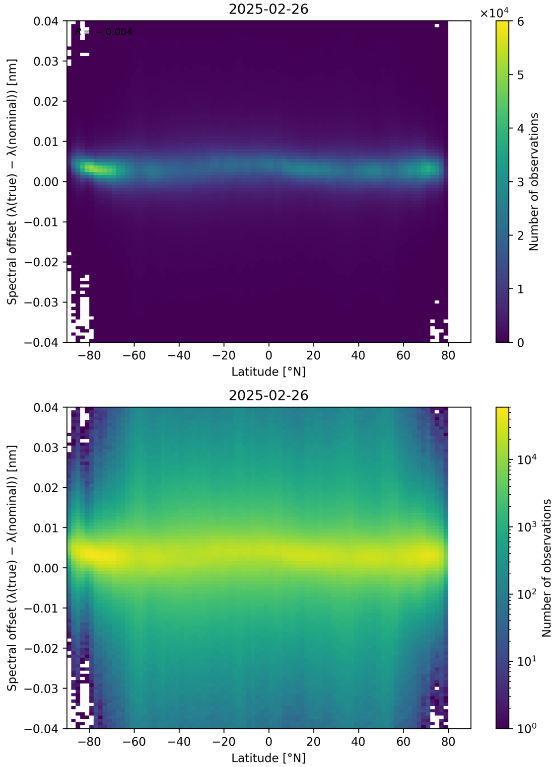
Figure 96: Scatter density plot of “Latitude” against “Spectral offset ( \lambda_{\text{true}} - \lambda_{\text{nominal}} )” for 2025-02-25 to 2025-02-27.
