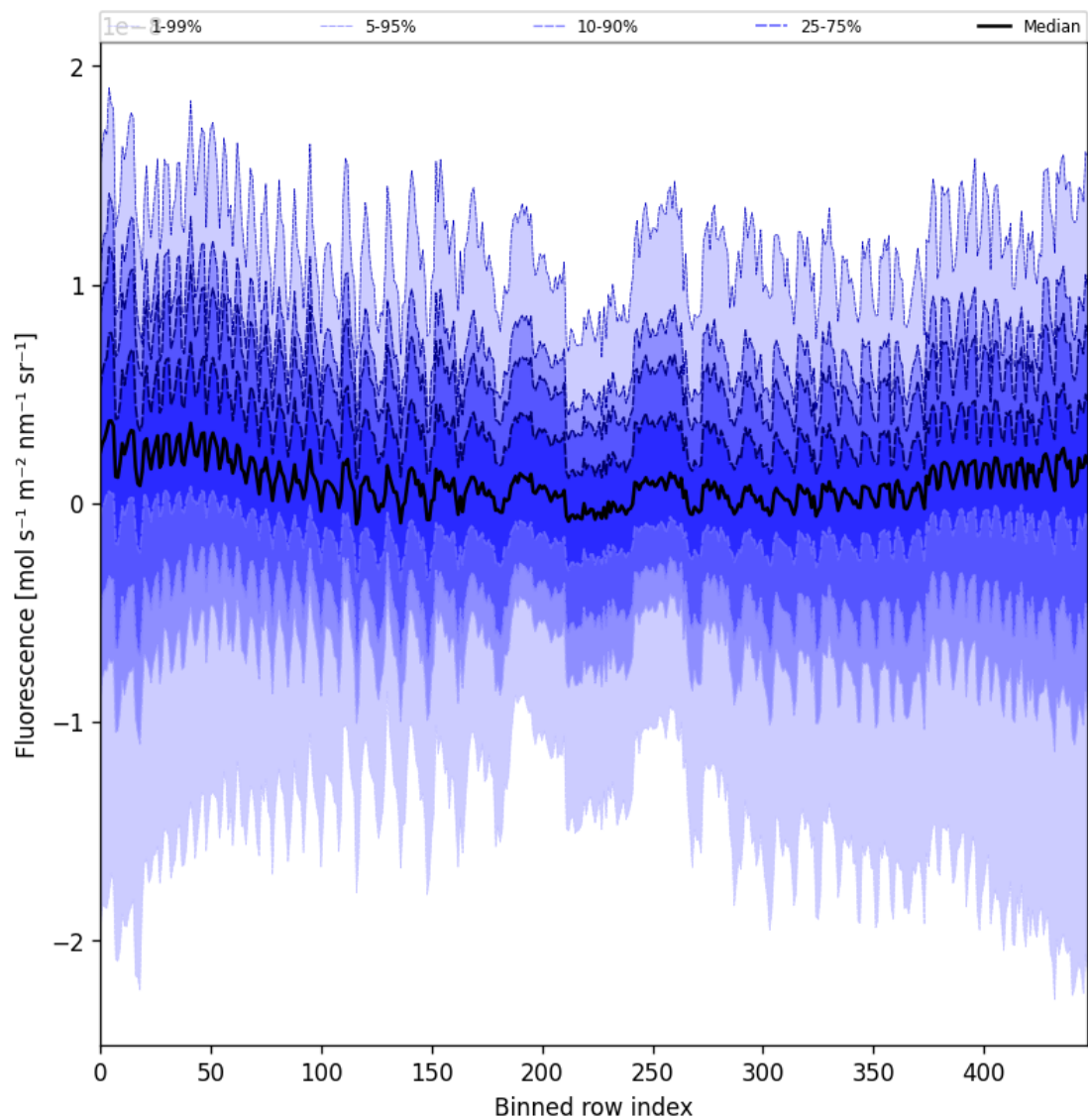
Figure 57: Along track statistics of “Fluorescence” for 2025-02-25 to 2025-02-27
