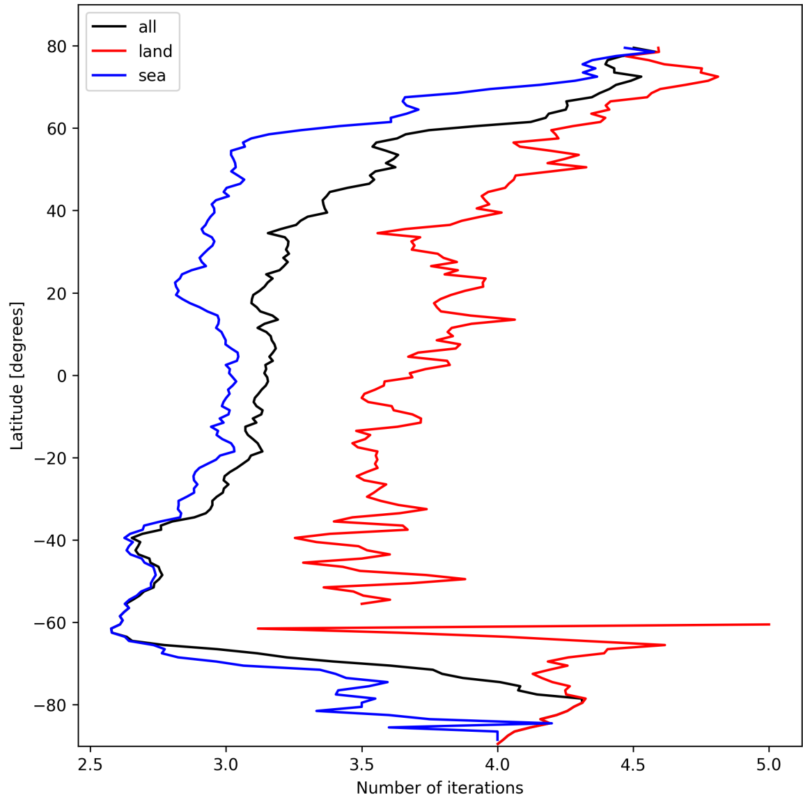
Figure 22: Zonal average of “Number of iterations” for 2025-02-25 to 2025-02-27.
