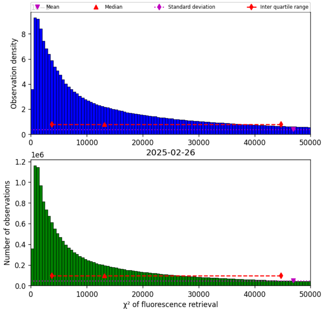
Figure 42: Histogram of “ \chi^2 of fluorescence retrieval” for 2025-02-25 to 2025-02-27
