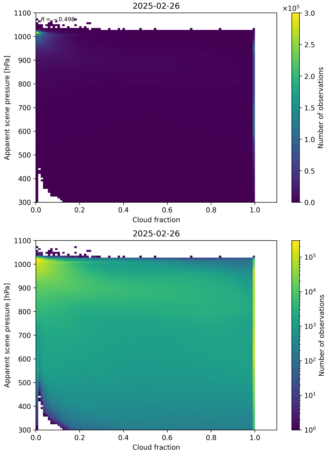
Figure 70: Scatter density plot of “Cloud fraction” against “Apparent scene pressure” for 2025-02-25 to 2025-02-27.
