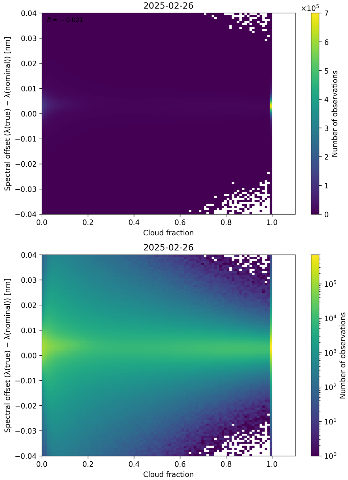
Figure 76: Scatter density plot of “Cloud fraction” against “Spectral offset ( \lambda_{\text{true}} - \lambda_{\text{nominal}} )” for 2025-02-25 to 2025-02-27.
