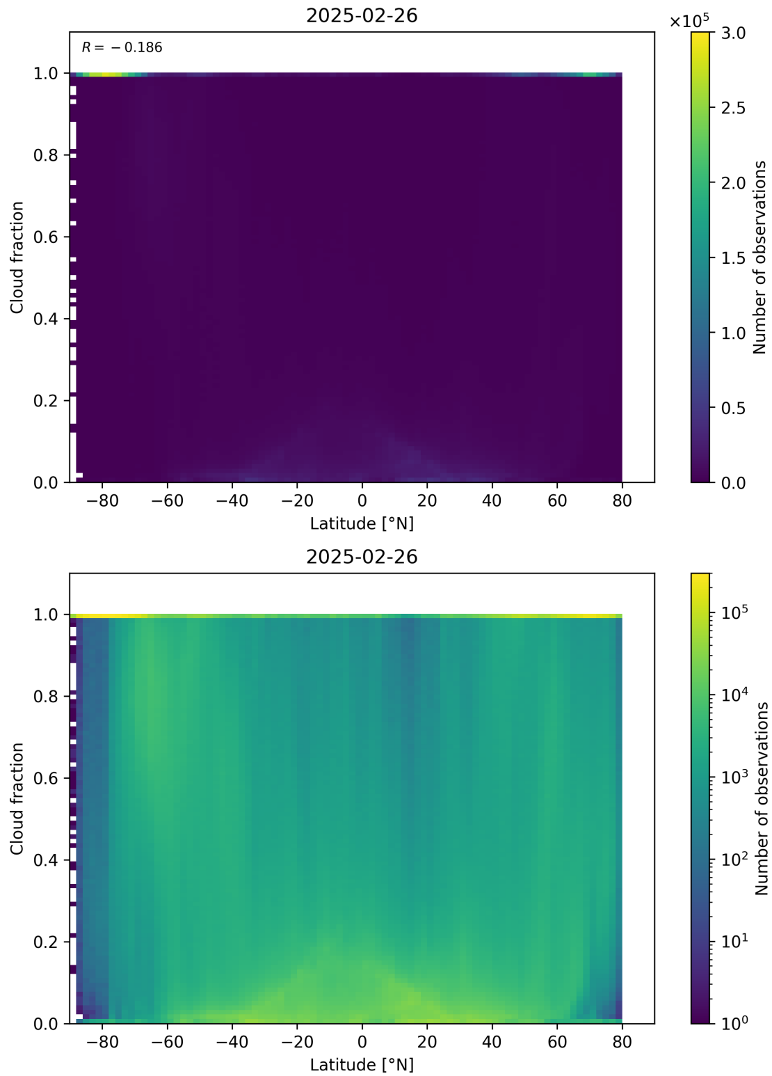
Figure 90: Scatter density plot of “Latitude” against “Cloud fraction” for 2025-02-25 to 2025-02-27.
