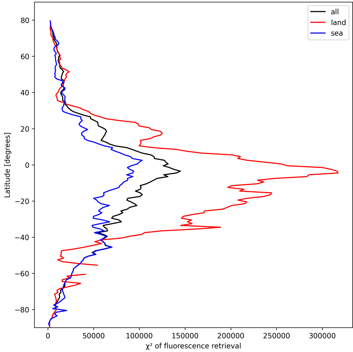
Figure 25: Zonal average of “ \chi^2 of fluorescence retrieval” for 2025-02-25 to 2025-02-27.
