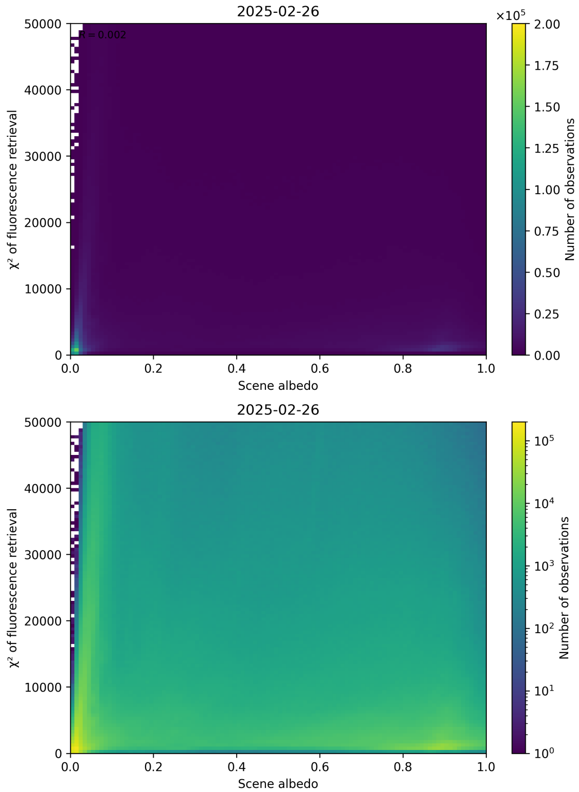
Figure 103: Scatter density plot of “Scene albedo” against “ \chi^2 of fluorescence retrieval” for 2025-02-25 to 2025-02-27.
