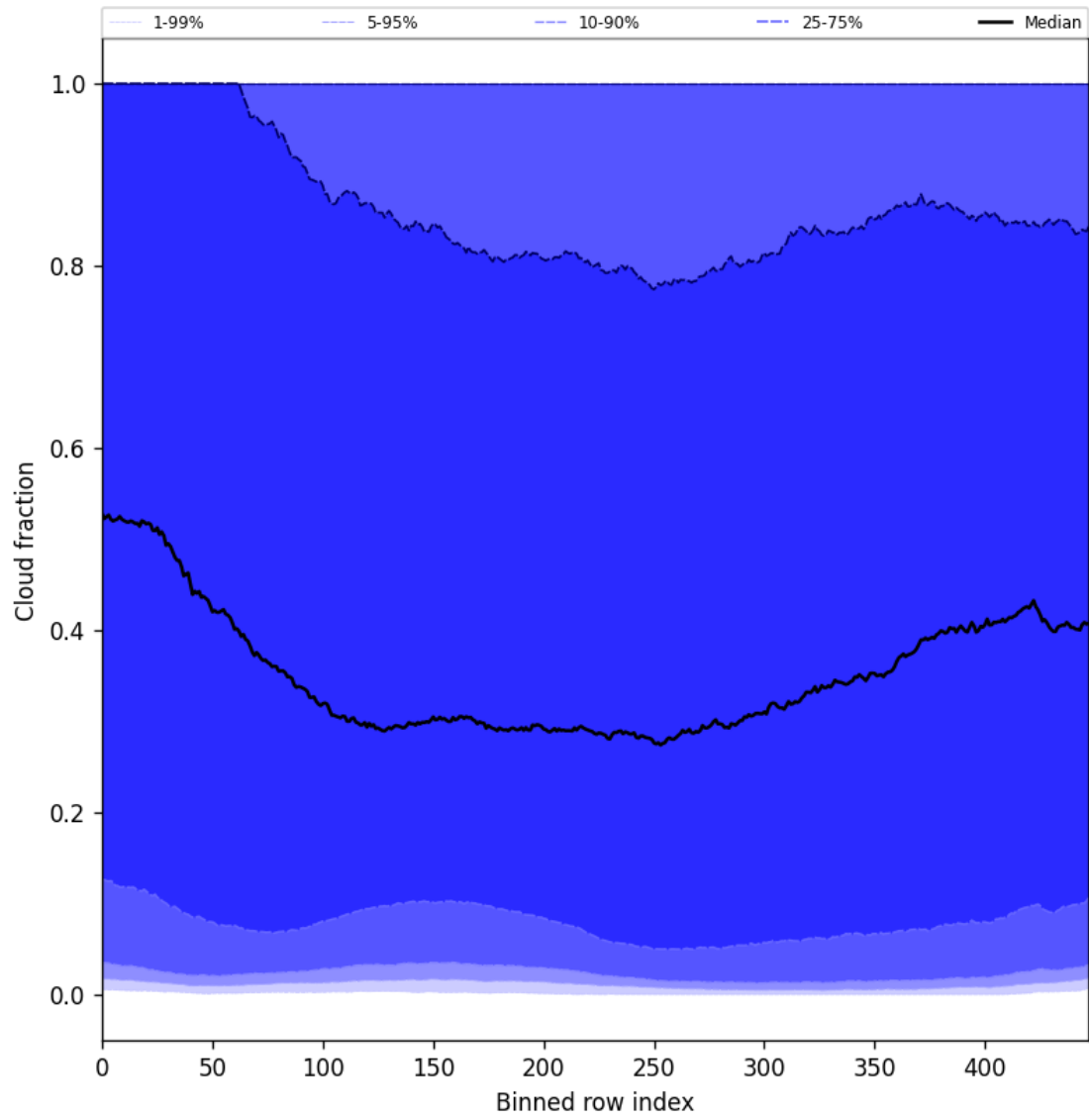
Figure 49: Along track statistics of “Cloud fraction” for 2025-02-25 to 2025-02-27
