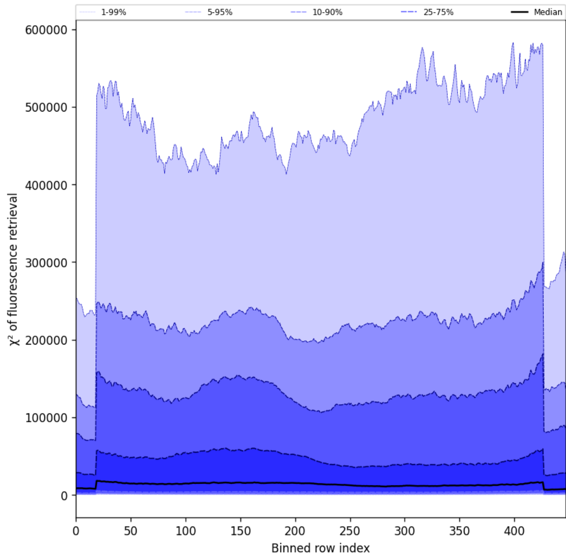
Figure 59: Along track statistics of “ \chi^2 of fluorescence retrieval” for 2025-02-25 to 2025-02-27
