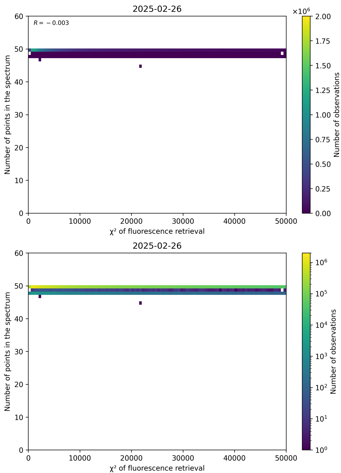
Figure 68: Scatter density plot of “ \chi^2 of fluorescence retrieval” against “Number of points in the spectrum” for 2025-02-25 to 2025-02-27.
