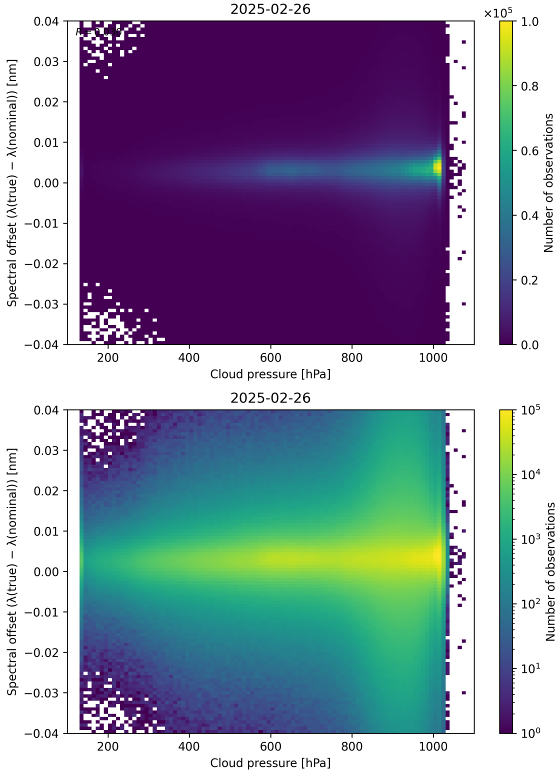
Figure 84: Scatter density plot of “Cloud pressure” against “Spectral offset ( \lambda_{\text{true}} - \lambda_{\text{nominal}} )” for 2025-02-25 to 2025-02-27.
