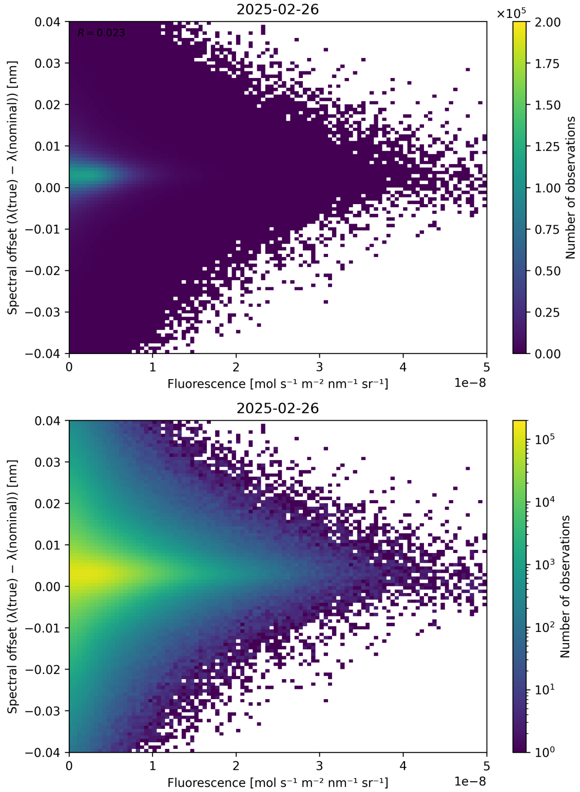
Figure 87: Scatter density plot of “Fluorescence” against “Spectral offset ( \lambda_{\text{true}} - \lambda_{\text{nominal}} )” for 2025-02-25 to 2025-02-27.
