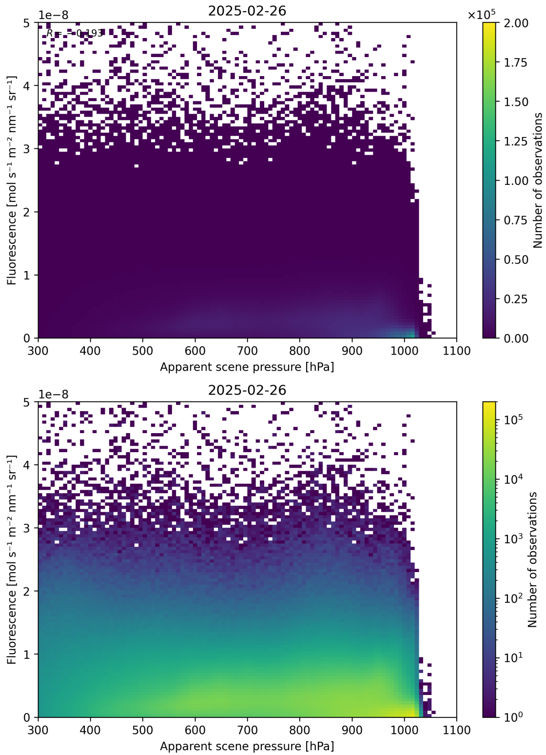
Figure 64: Scatter density plot of “Apparent scene pressure” against “Fluorescence” for 2025-02-25 to 2025-02-27.
