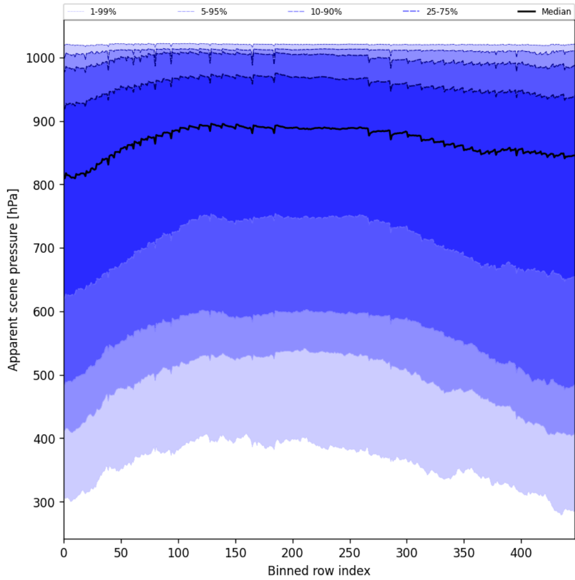
Figure 53: Along track statistics of “Apparent scene pressure” for 2025-02-25 to 2025-02-27
