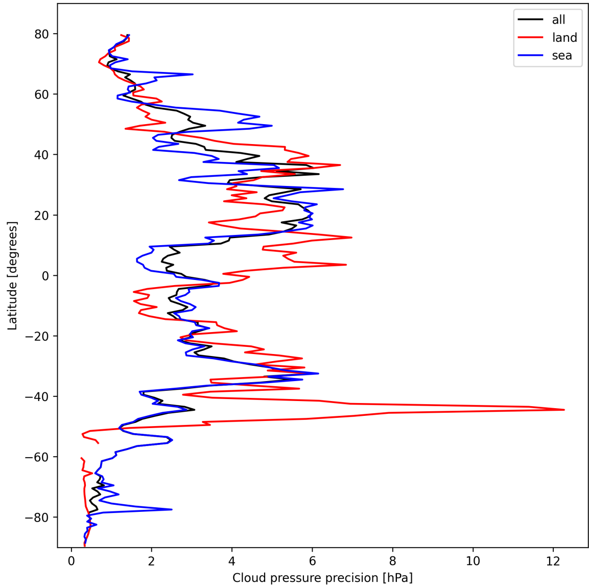
Figure 14: Zonal average of “Cloud pressure precision” for 2025-02-25 to 2025-02-27.
