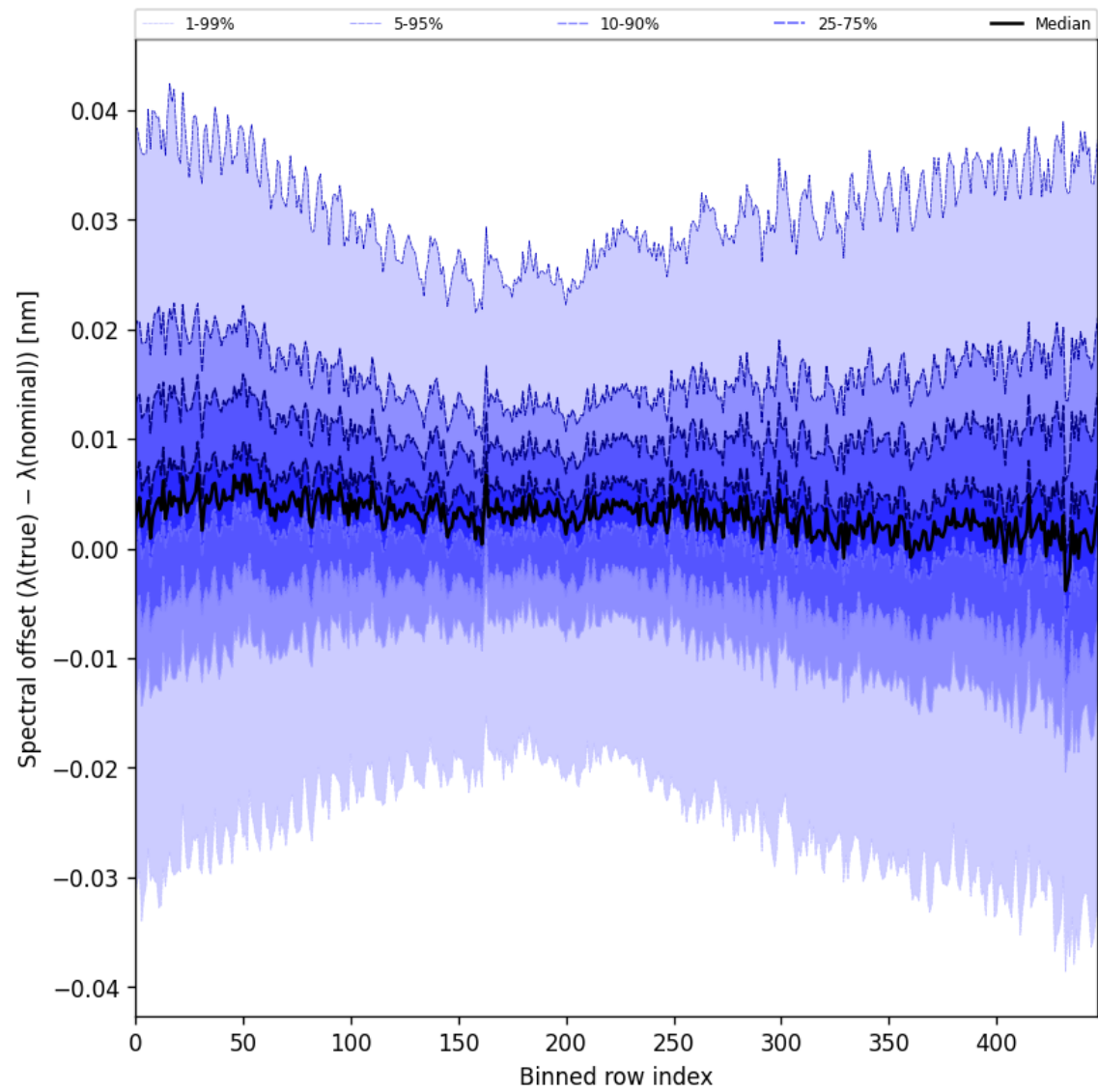
Figure 62: Along track statistics of “Spectral offset ( \lambda_{\text{true}} - \lambda_{\text{nominal}} )” for 2025-02-25 to 2025-02-27
