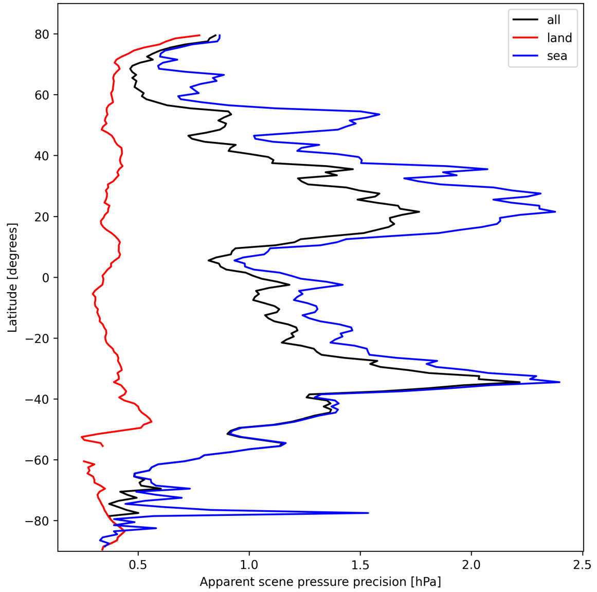
Figure 20: Zonal average of “Apparent scene pressure precision” for 2025-02-25 to 2025-02-27.
