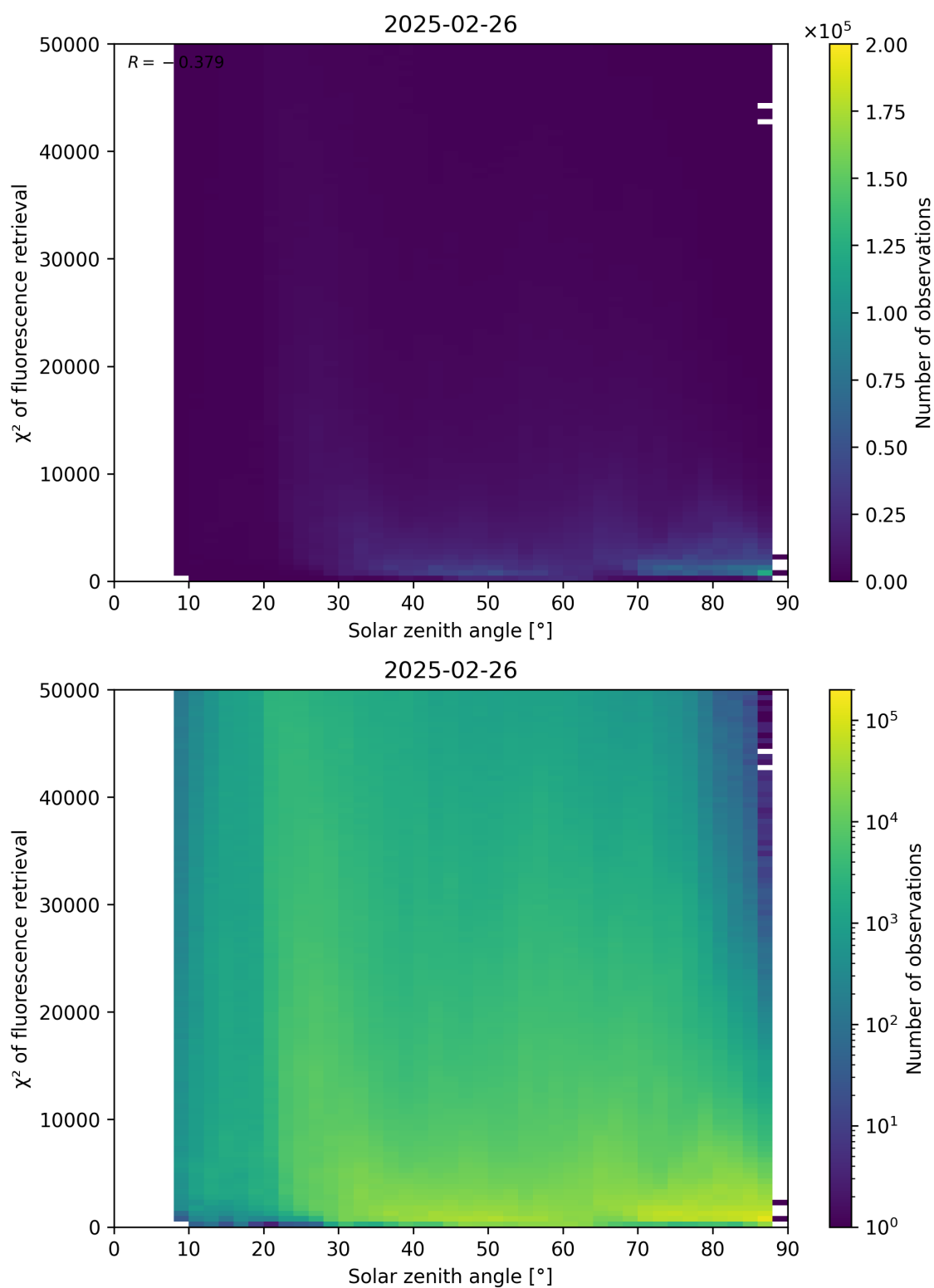
Figure 109: Scatter density plot of “Solar zenith angle” against “ \chi^2 of fluorescence retrieval” for 2025-02-25 to 2025-02-27.
