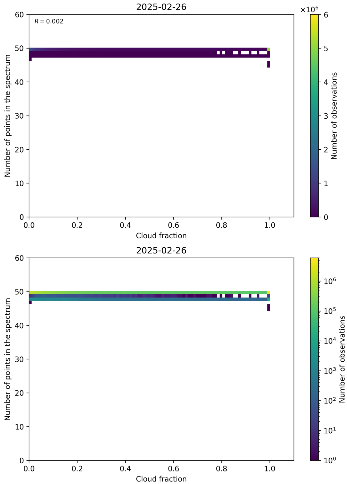
Figure 74: Scatter density plot of “Cloud fraction” against “Number of points in the spectrum” for 2025-02-25 to 2025-02-27.
