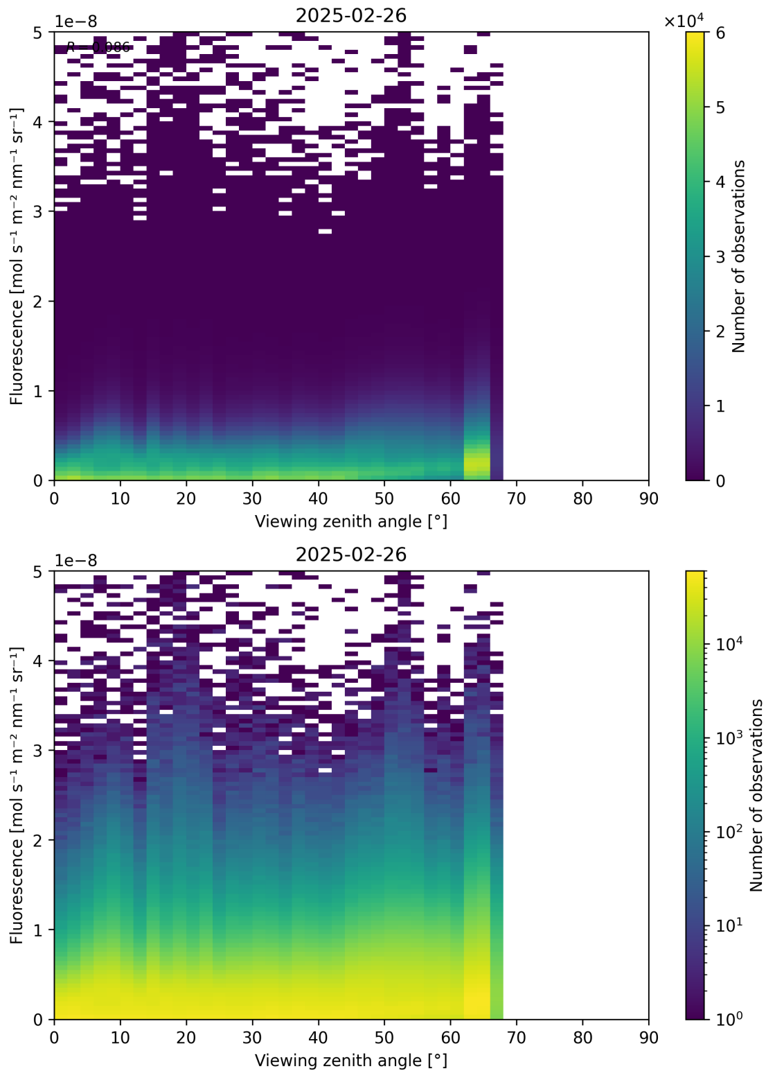
Figure 122: Scatter density plot of “Viewing zenith angle” against “Fluorescence” for 2025-02-25 to 2025-02-27.
