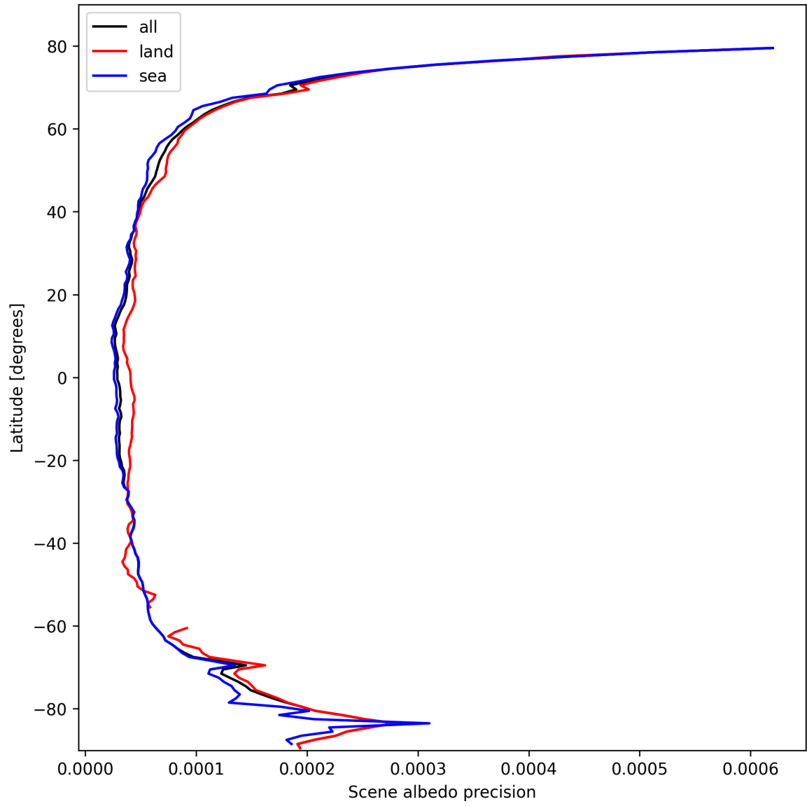
Figure 18: Zonal average of “Scene albedo precision” for 2025-02-25 to 2025-02-27.
