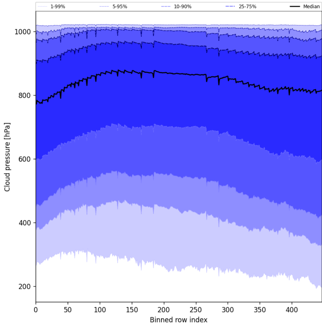
Figure 47: Along track statistics of “Cloud pressure” for 2025-02-25 to 2025-02-27
