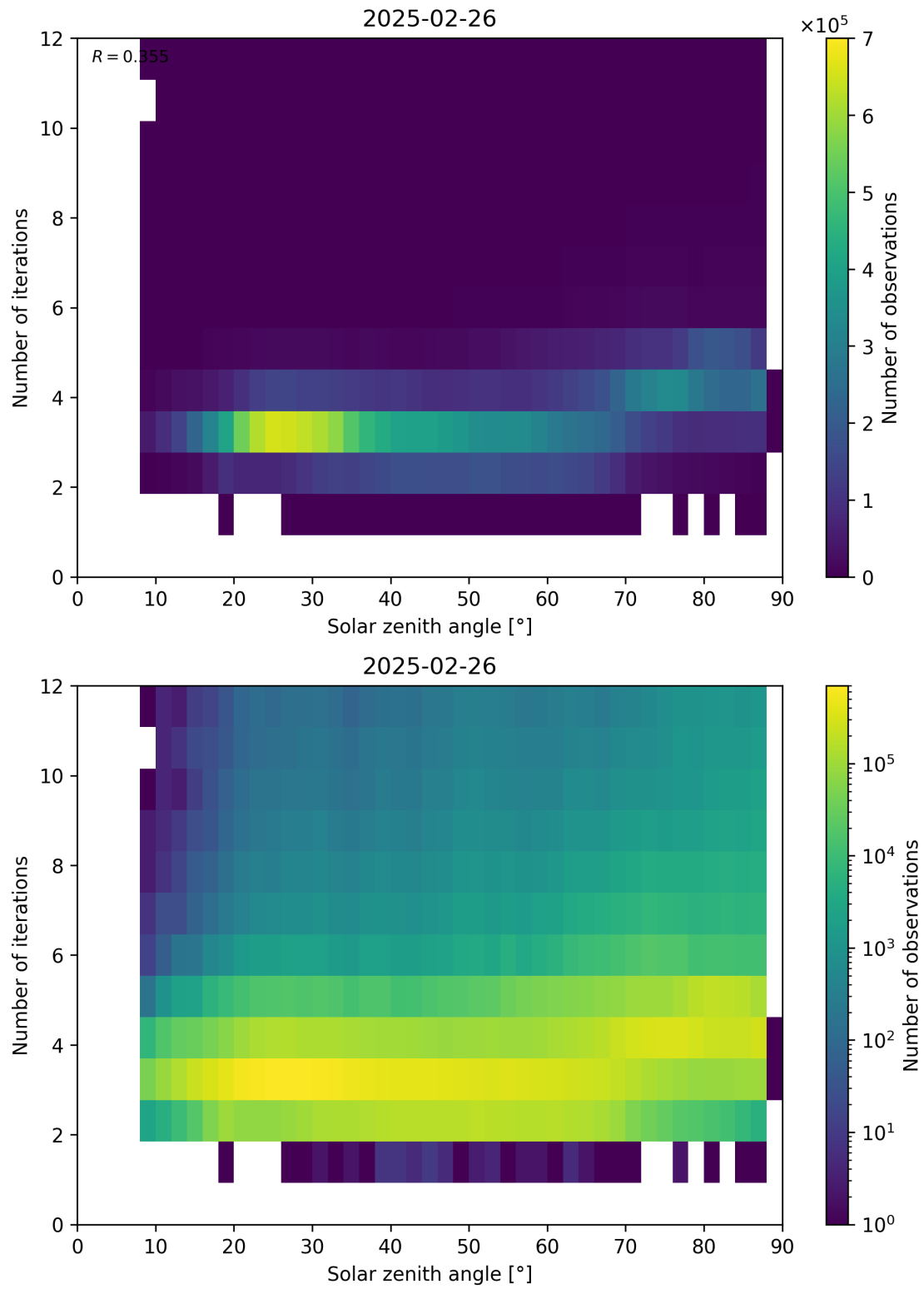
Figure 114: Scatter density plot of “Solar zenith angle” against “Number of iterations” for 2025-02-25 to 2025-02-27.
