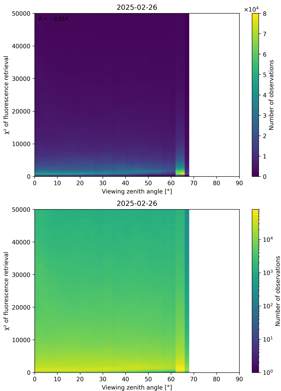
Figure 119: Scatter density plot of “Viewing zenith angle” against “ \chi^2 of fluorescence retrieval” for 2025-02-25 to 2025-02-27.
