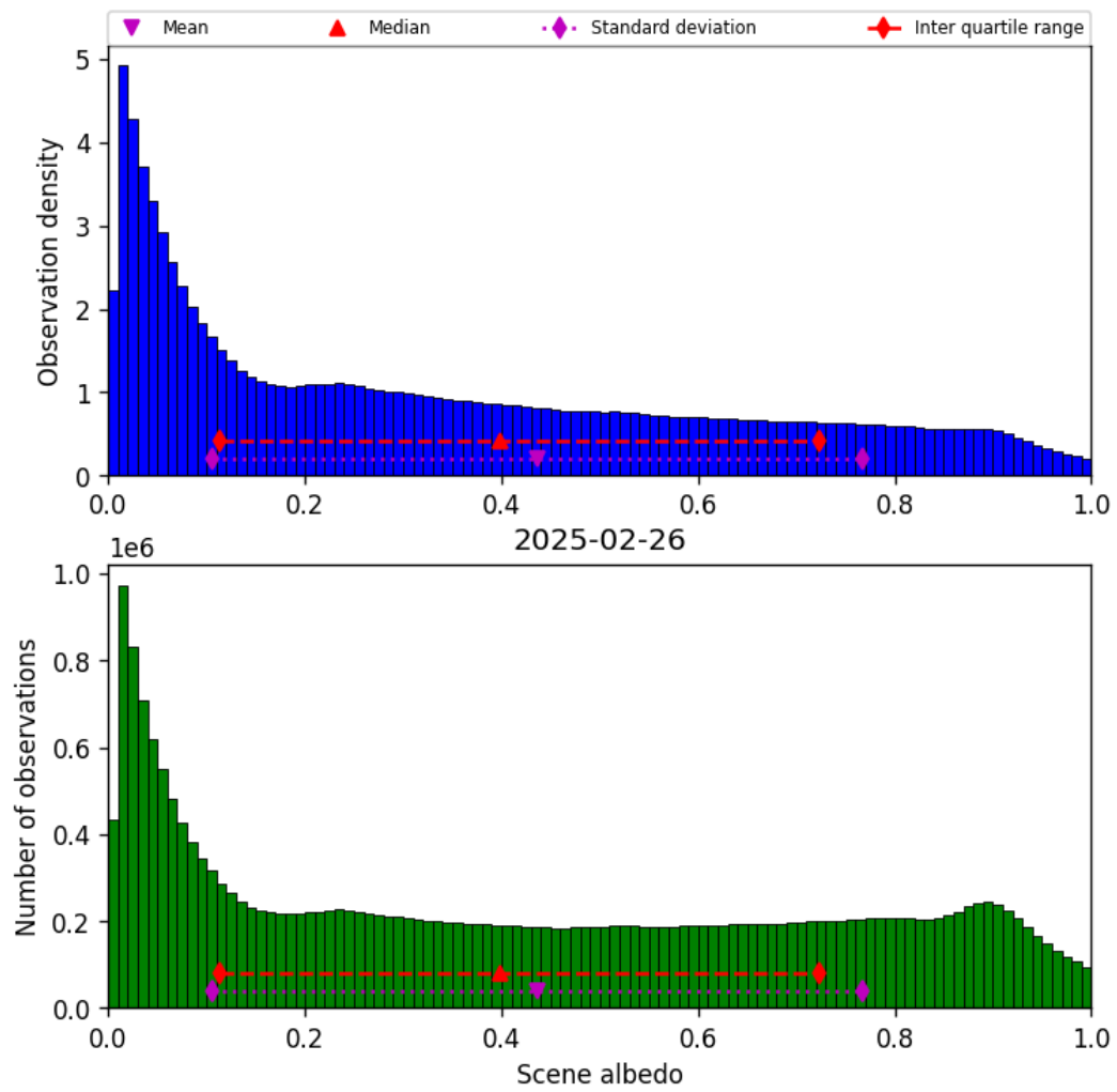
Figure 34: Histogram of “Scene albedo” for 2025-02-25 to 2025-02-27
