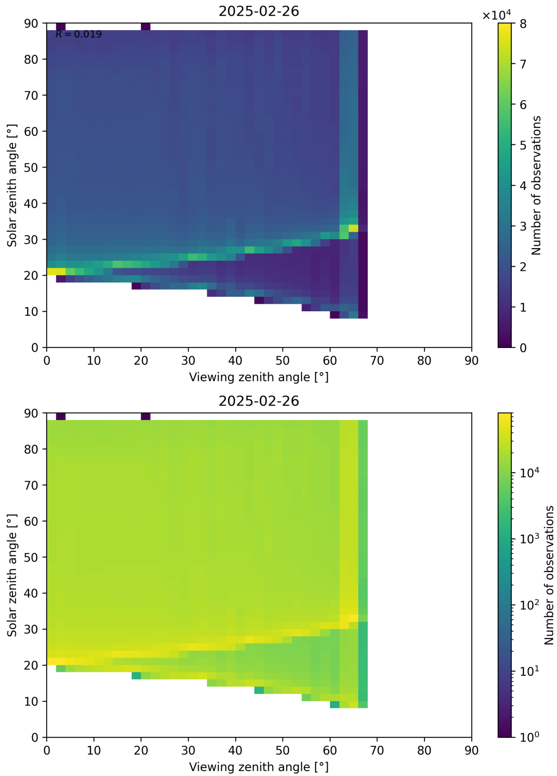
Figure 127: Scatter density plot of “Viewing zenith angle” against “Solar zenith angle” for 2025-02-25 to 2025-02-27.
