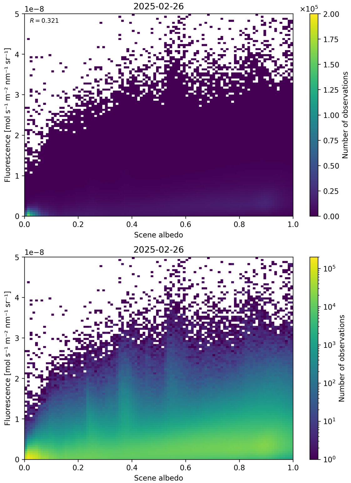
Figure 104: Scatter density plot of “Scene albedo” against “Fluorescence” for 2025-02-25 to 2025-02-27.
