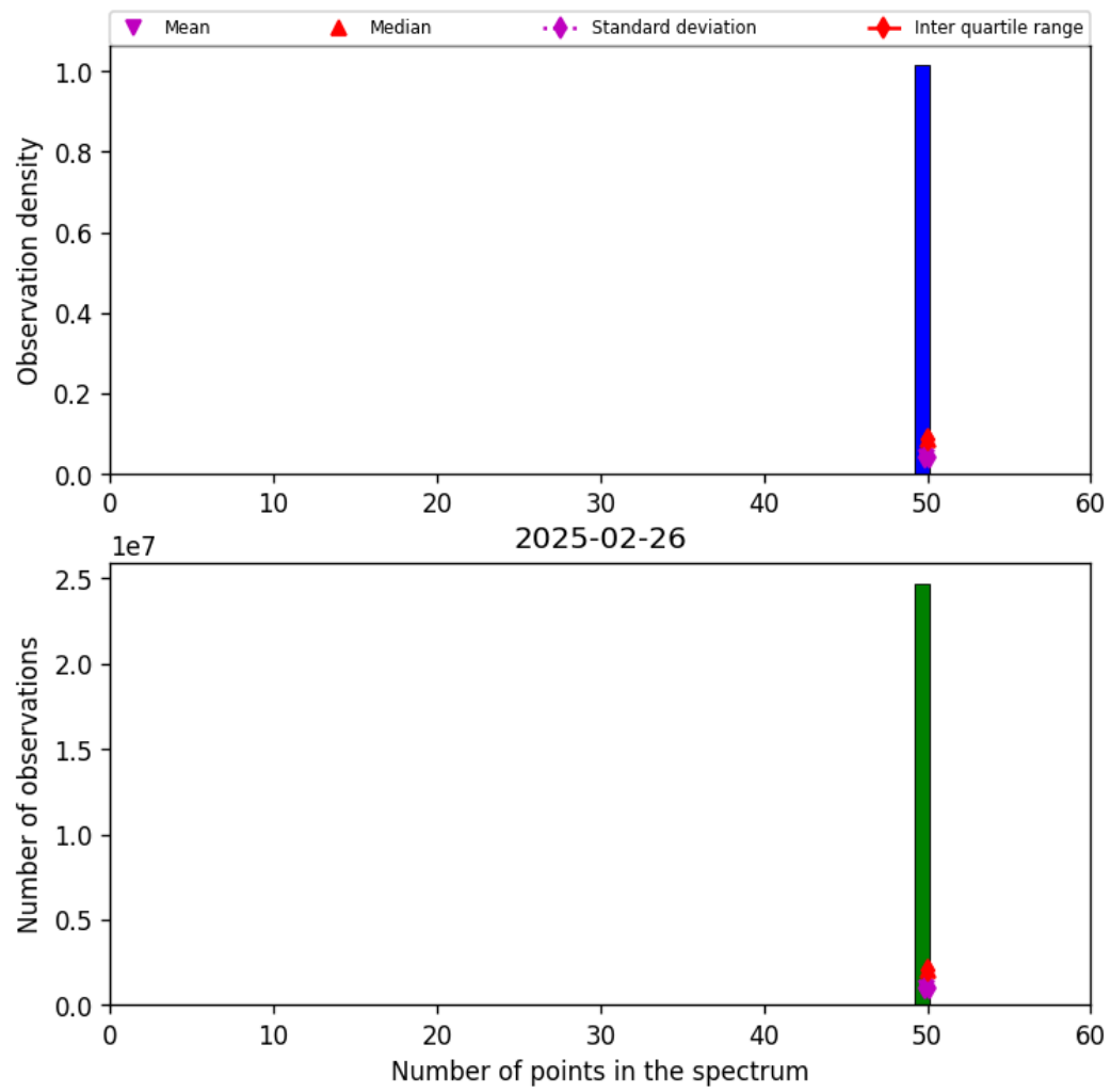
Figure 44: Histogram of “Number of points in the spectrum” for 2025-02-25 to 2025-02-27
