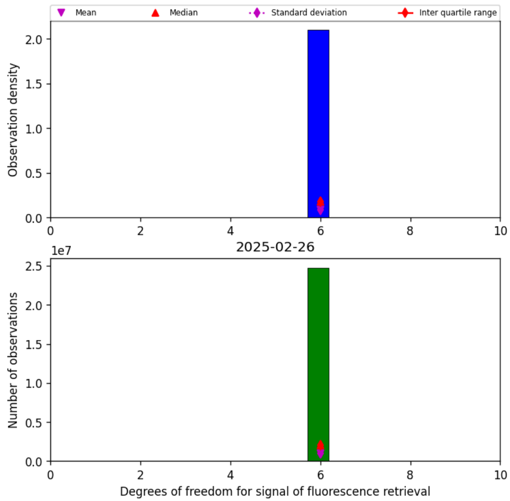
Figure 43: Histogram of “Degrees of freedom for signal of fluorescence retrieval” for 2025-02-25 to 2025-02-27
