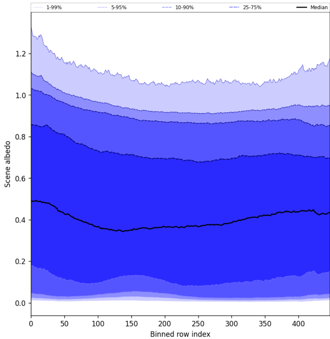
Figure 51: Along track statistics of “Scene albedo” for 2025-02-25 to 2025-02-27
