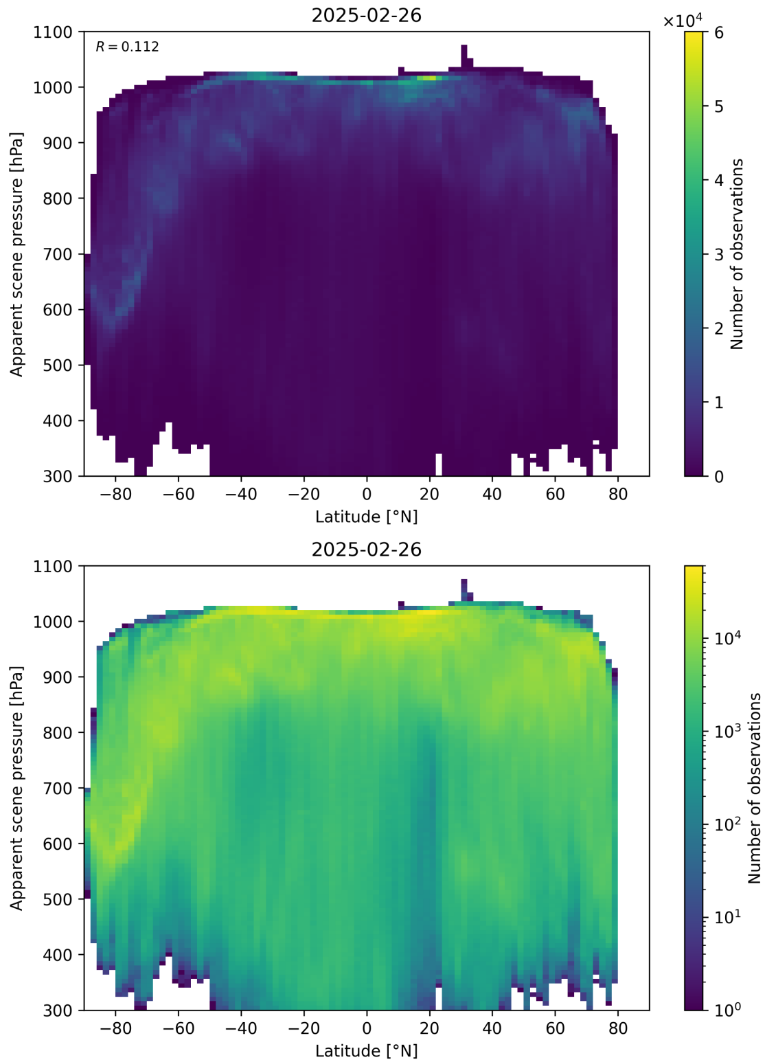
Figure 88: Scatter density plot of “Latitude” against “Apparent scene pressure” for 2025-02-25 to 2025-02-27.
