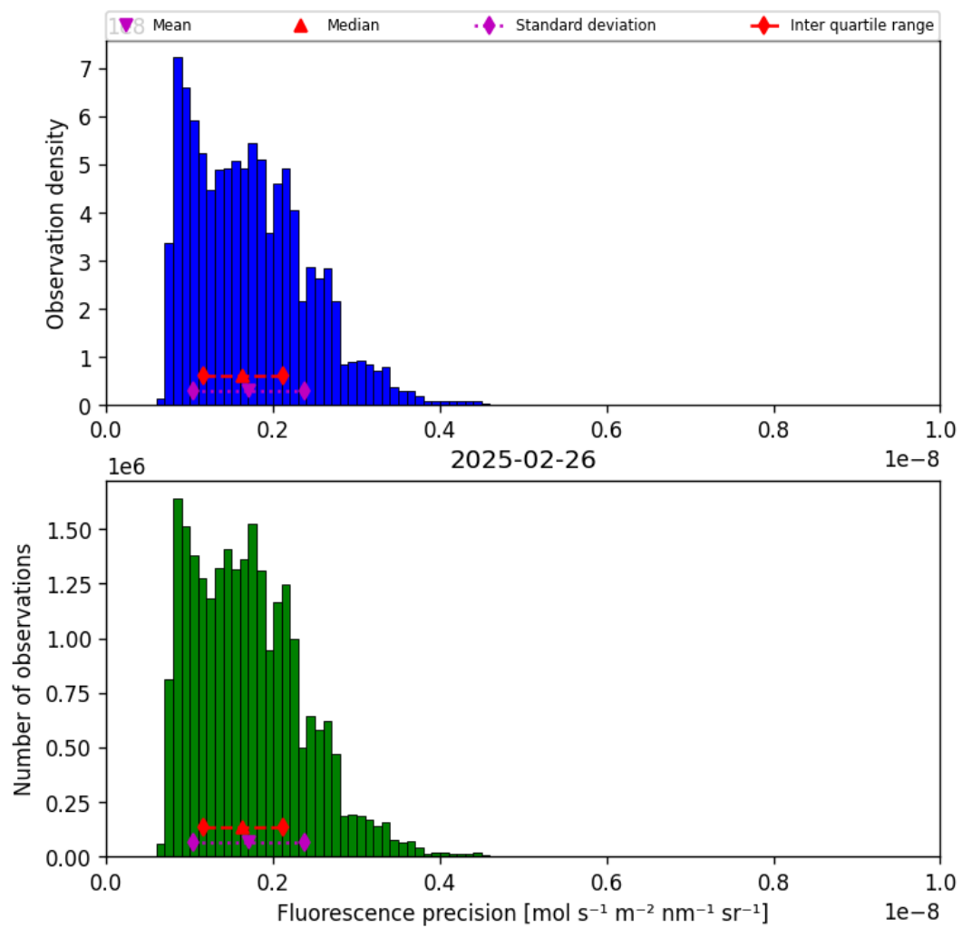
Figure 41: Histogram of “Fluorescence precision” for 2025-02-25 to 2025-02-27
