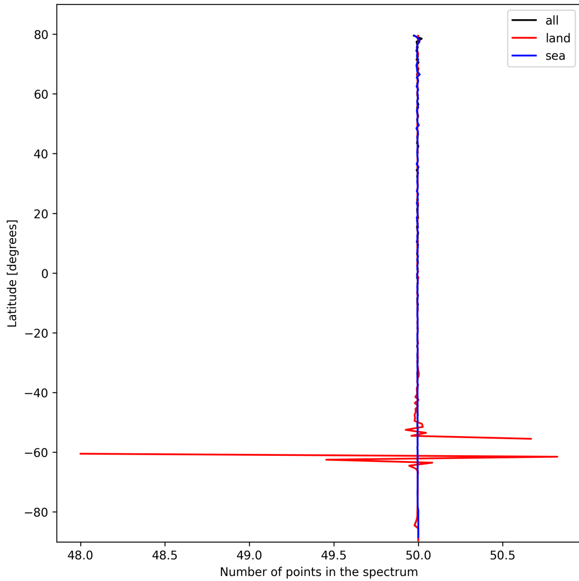
Figure 27: Zonal average of “Number of points in the spectrum” for 2025-02-25 to 2025-02-27.
