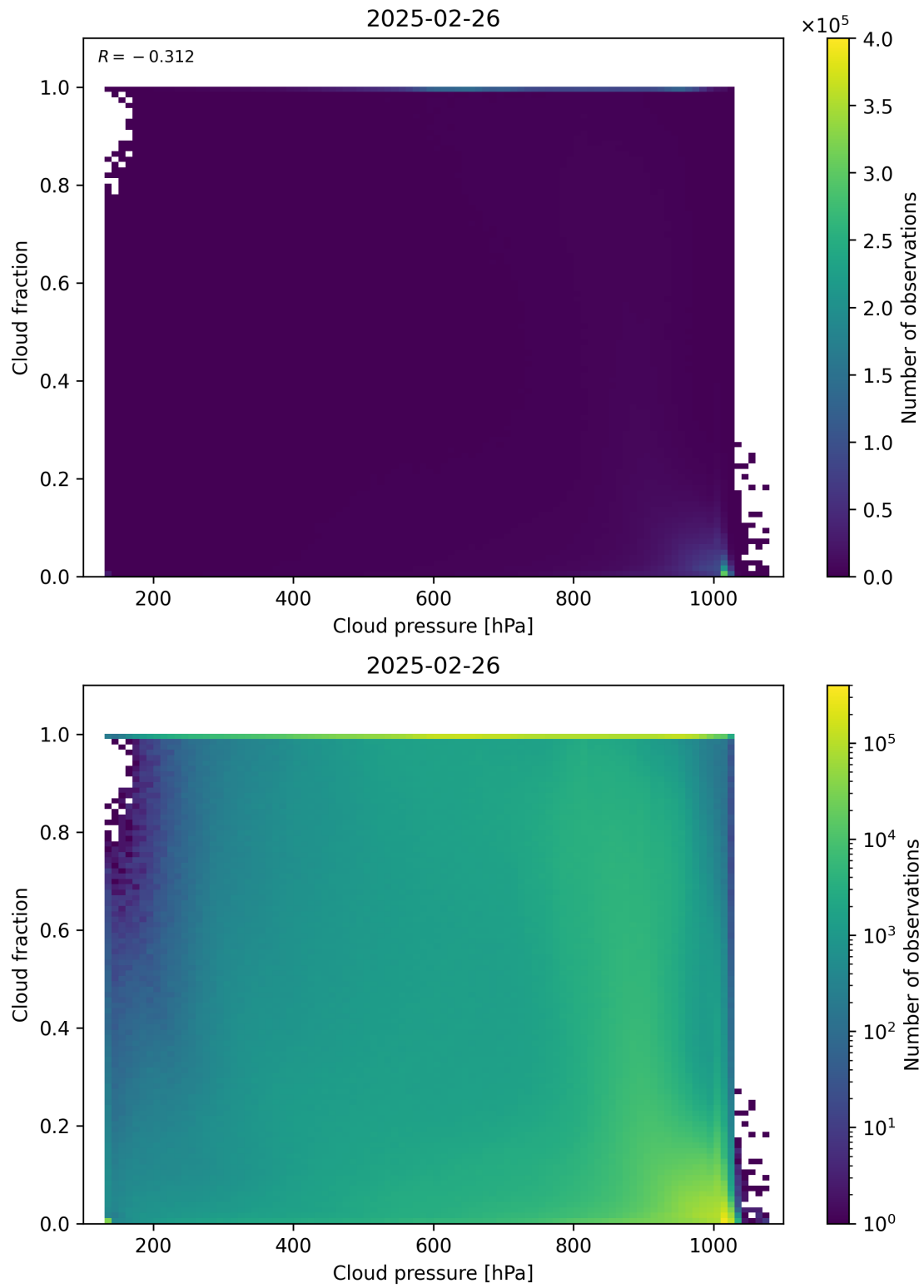
Figure 79: Scatter density plot of “Cloud pressure” against “Cloud fraction” for 2025-02-25 to 2025-02-27.
