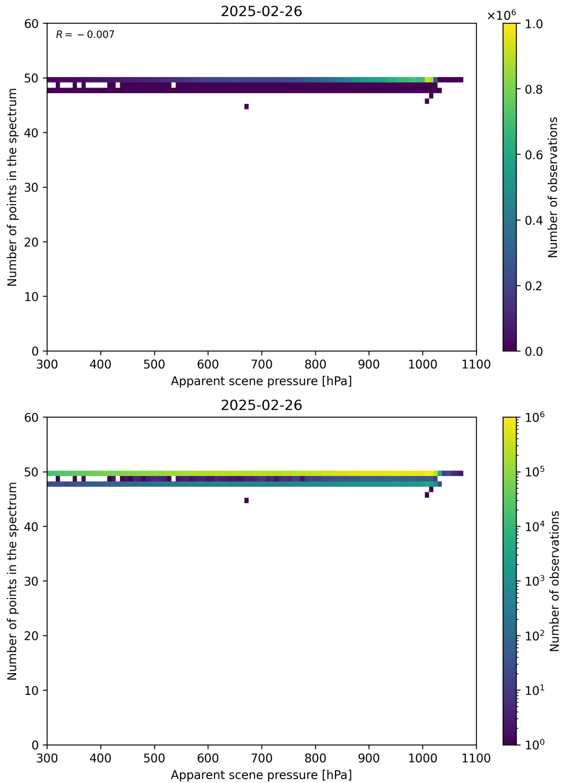
Figure 66: Scatter density plot of “Apparent scene pressure” against “Number of points in the spectrum” for 2025-02-25 to 2025-02-27.
