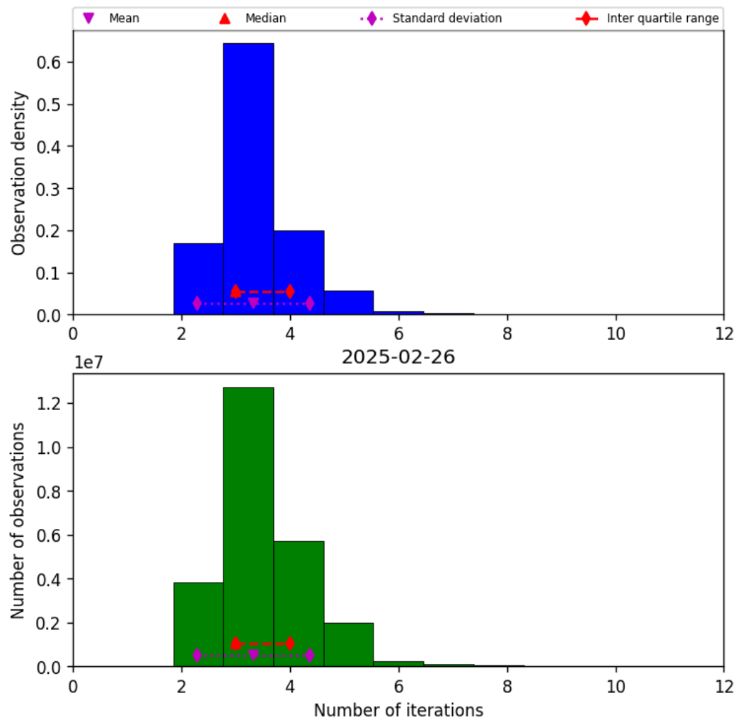
Figure 39: Histogram of “Number of iterations” for 2025-02-25 to 2025-02-27
