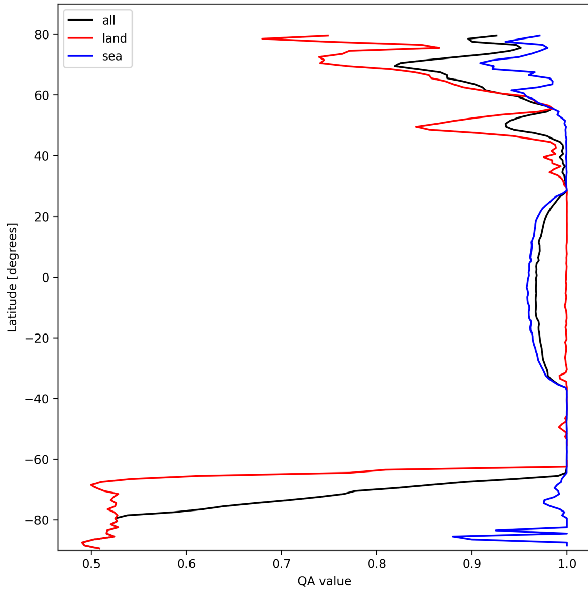
Figure 12: Zonal average of “QA value” for 2025-02-25 to 2025-02-27.
