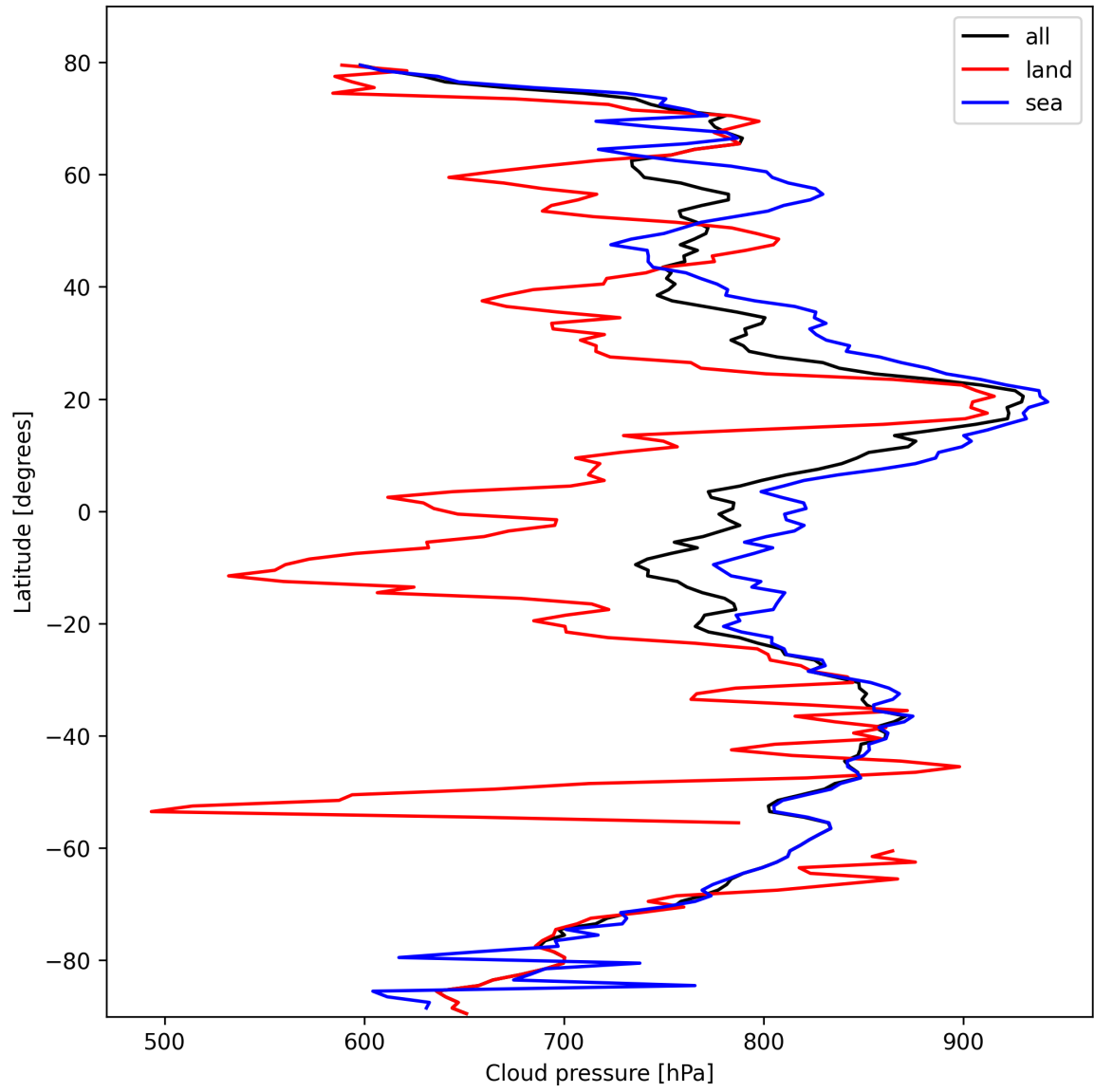
Figure 13: Zonal average of “Cloud pressure” for 2025-02-25 to 2025-02-27.
