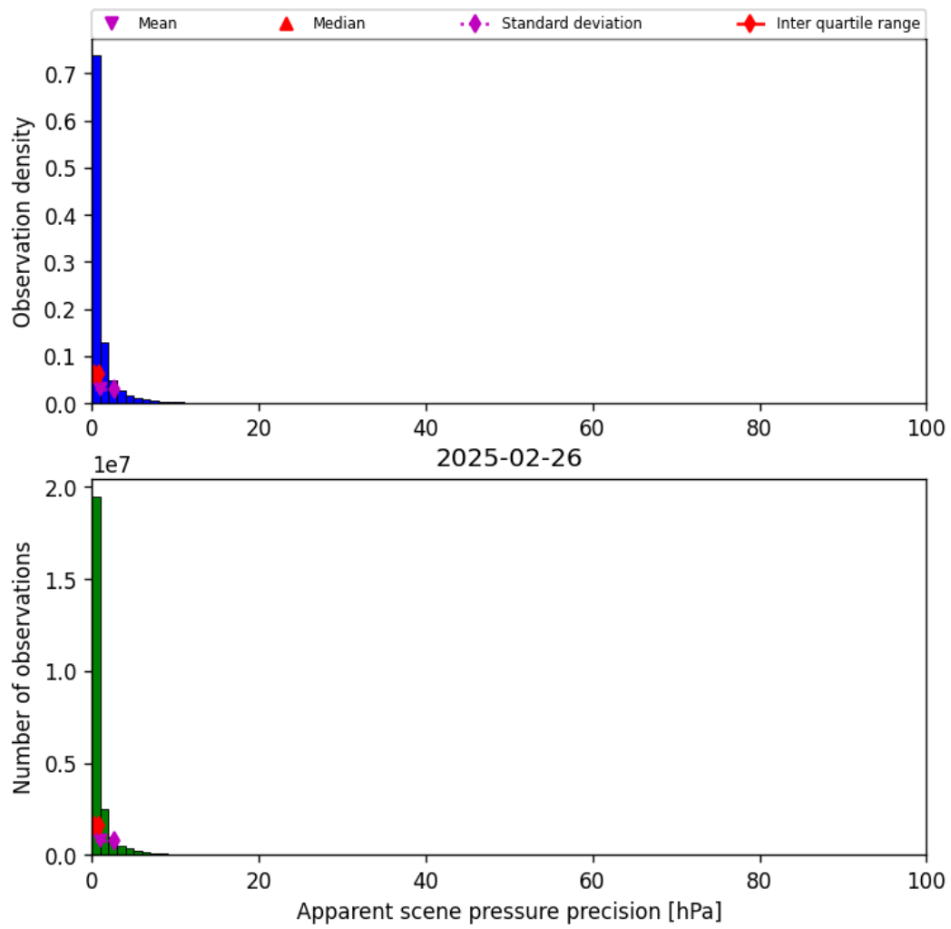
Figure 37: Histogram of “Apparent scene pressure precision” for 2025-02-25 to 2025-02-27
