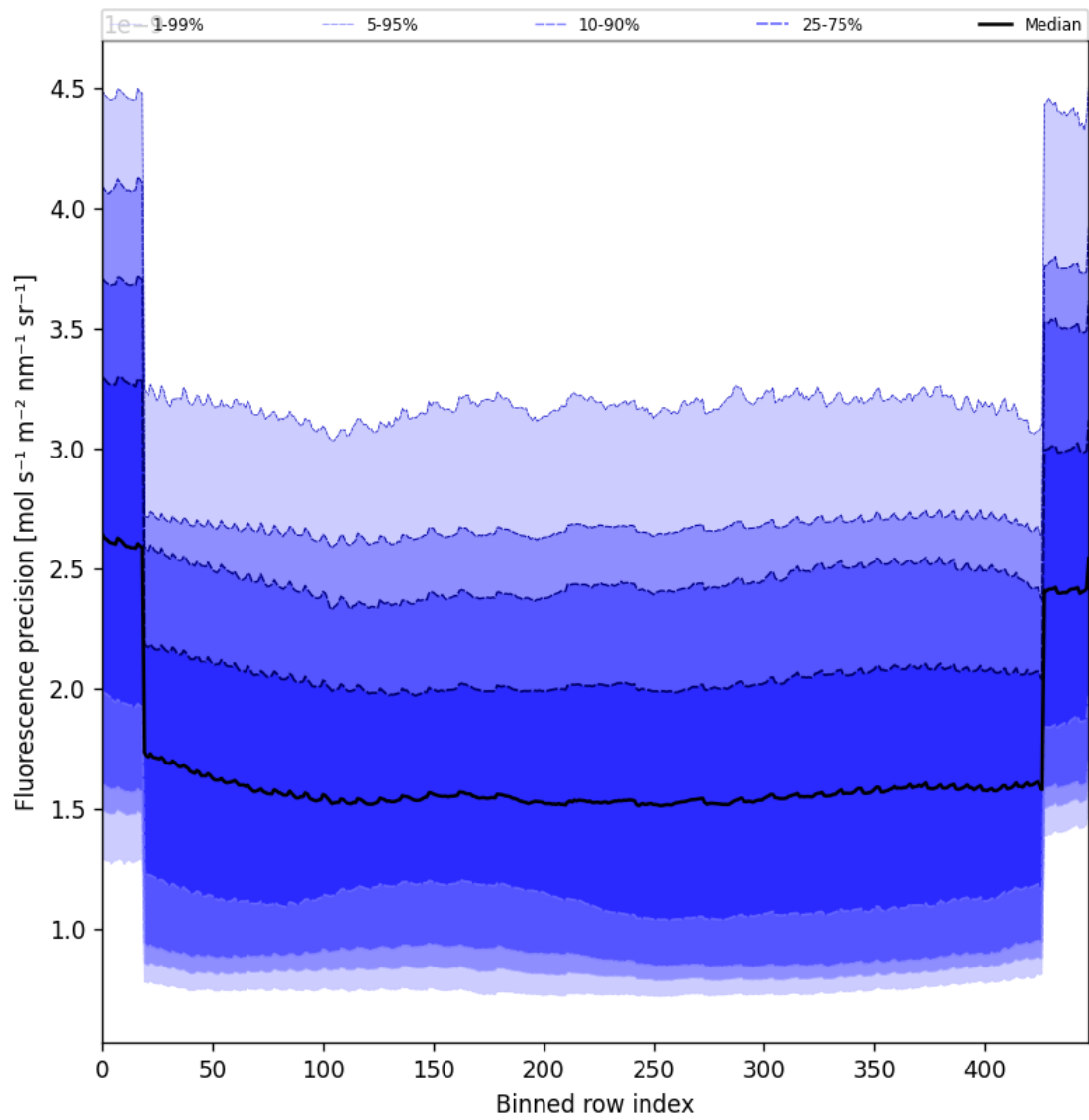
Figure 58: Along track statistics of “Fluorescence precision” for 2025-02-25 to 2025-02-27
