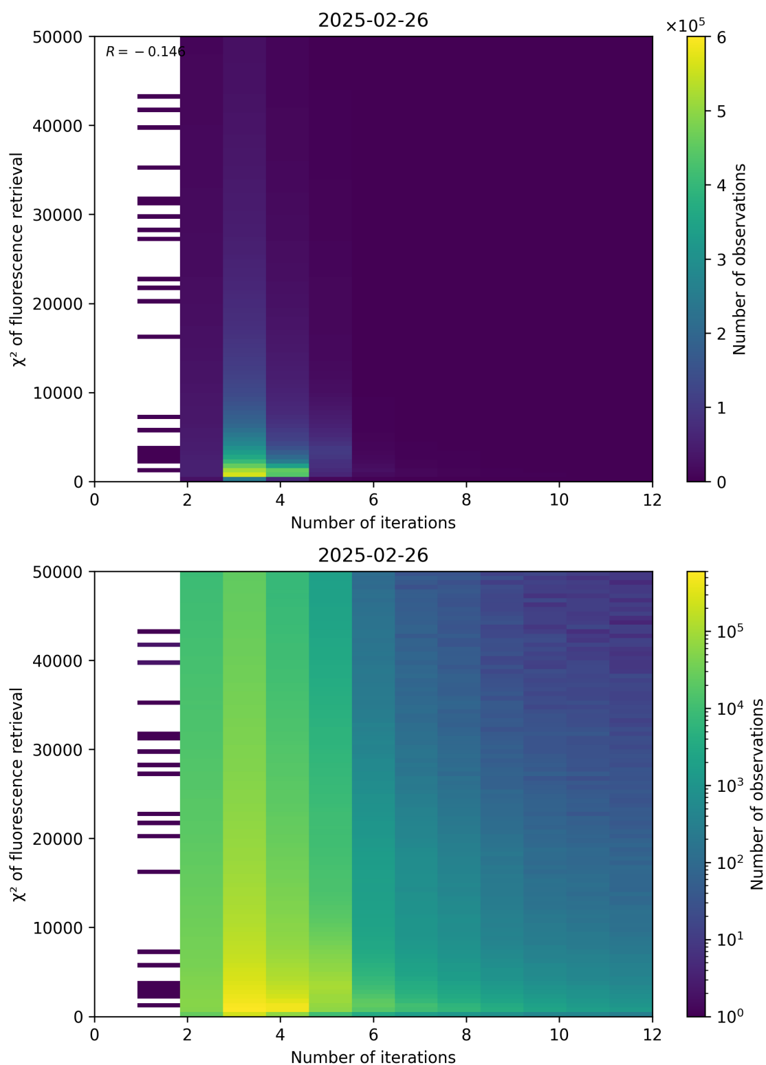
Figure 97: Scatter density plot of “Number of iterations” against “ \chi^2 of fluorescence retrieval” for 2025-02-25 to 2025-02-27.
