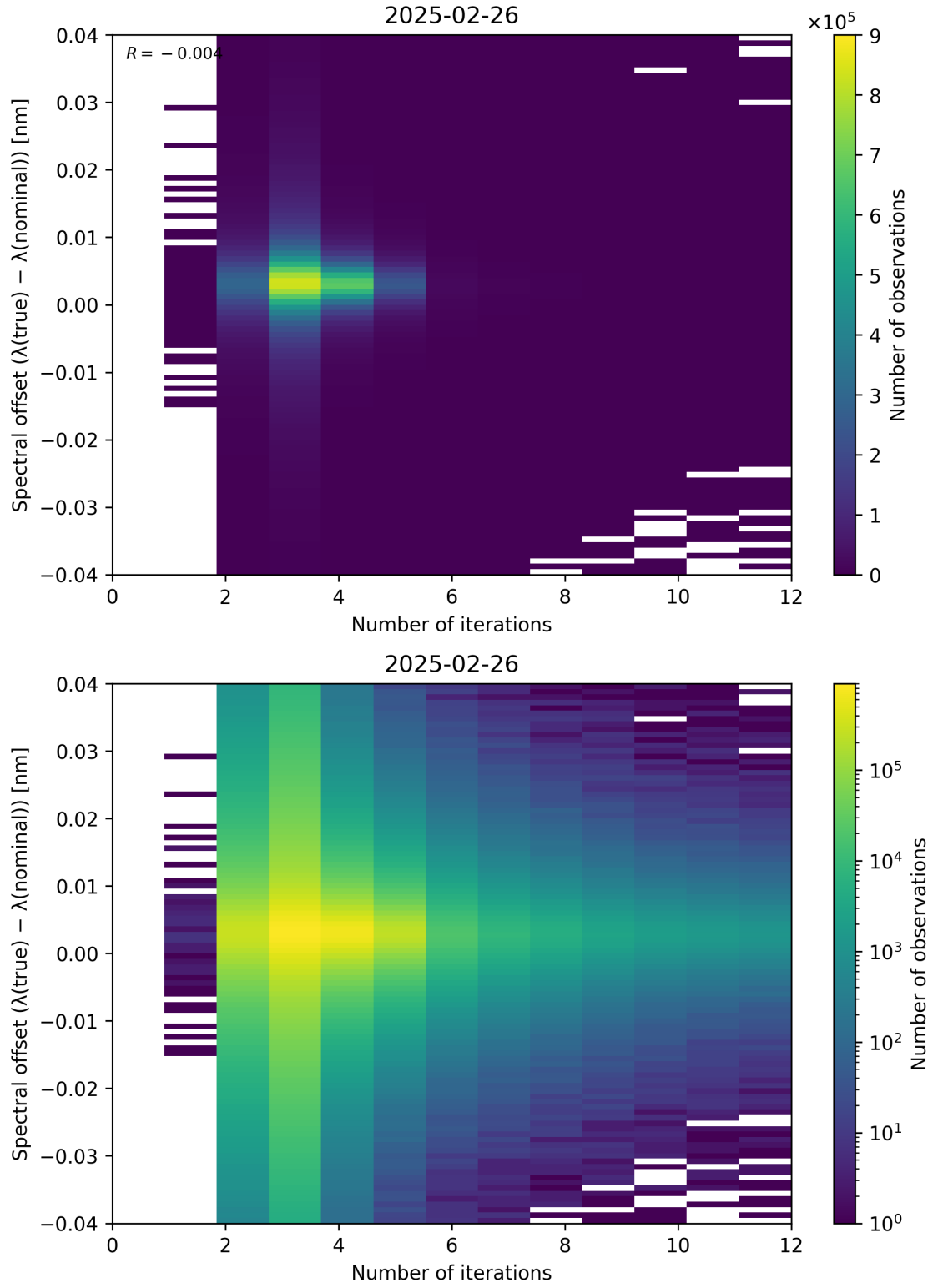
Figure 100: Scatter density plot of “Number of iterations” against “Spectral offset ( \lambda_{\text{true}} - \lambda_{\text{nominal}} )” for 2025-02-25 to 2025-02-27.
