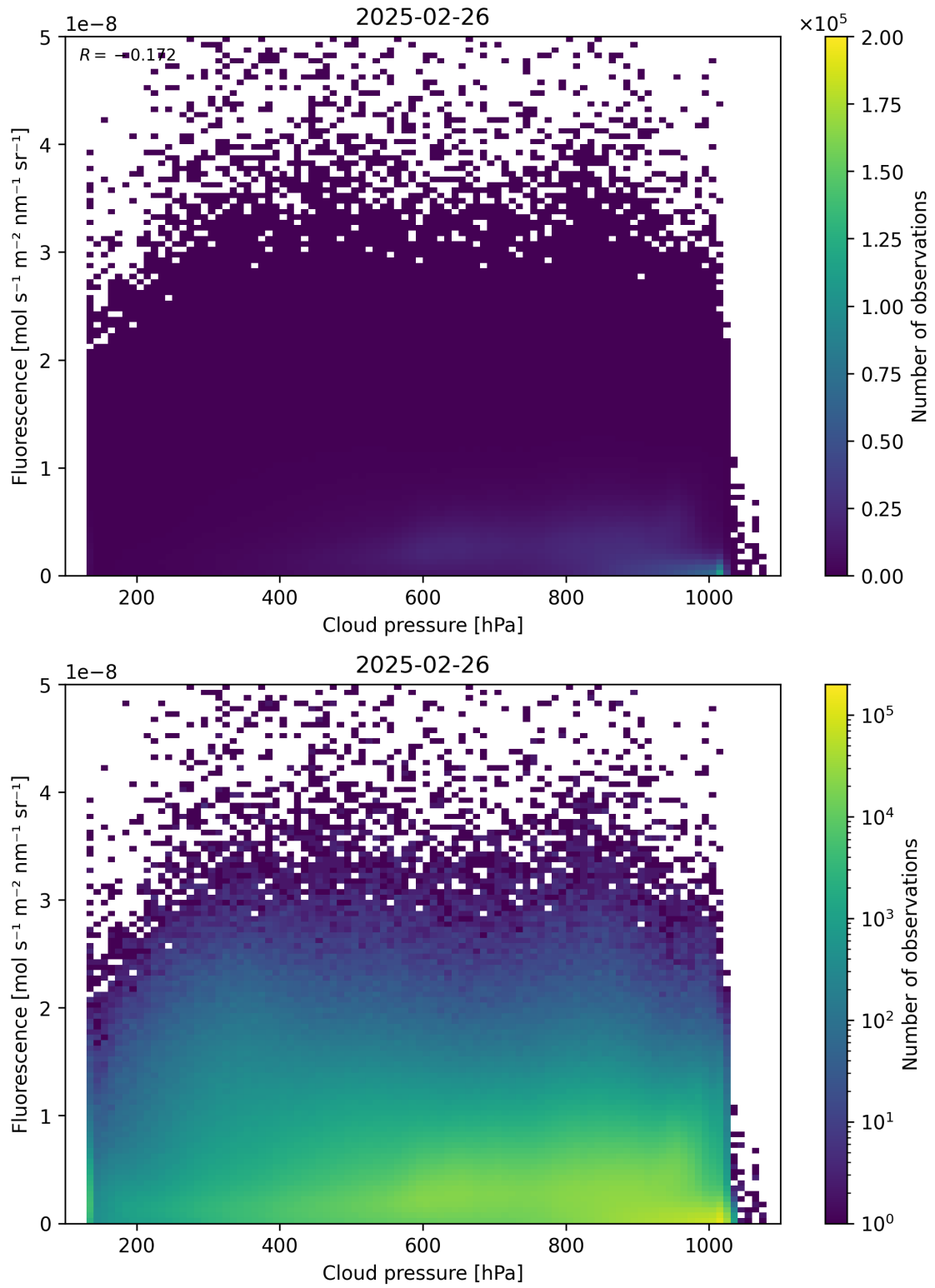
Figure 80: Scatter density plot of “Cloud pressure” against “Fluorescence” for 2025-02-25 to 2025-02-27.
