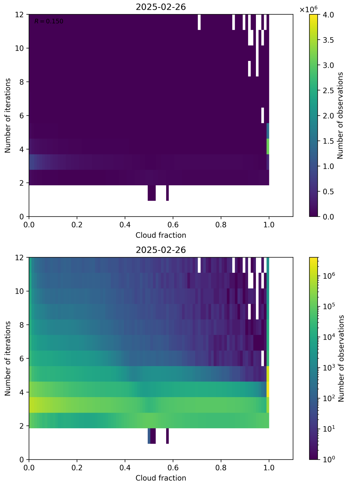
Figure 73: Scatter density plot of “Cloud fraction” against “Number of iterations” for 2025-02-25 to 2025-02-27.
