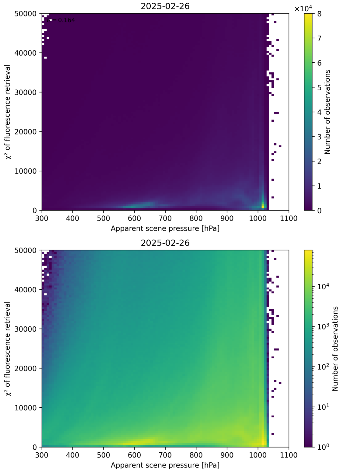
Figure 63: Scatter density plot of “Apparent scene pressure” against “ \chi^2 of fluorescence retrieval” for 2025-02-25 to 2025-02-27.
