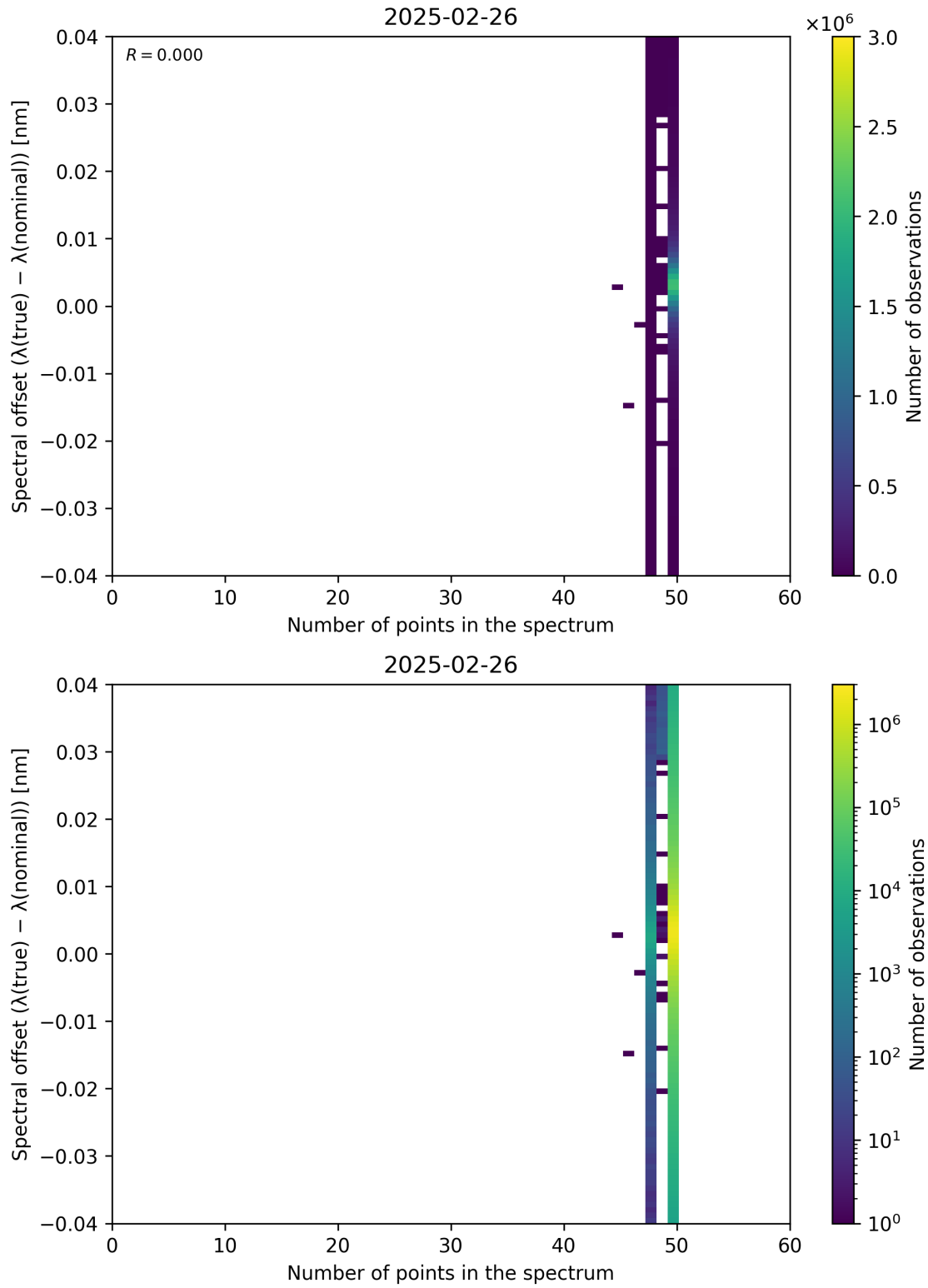
Figure 101: Scatter density plot of “Number of points in the spectrum” against “Spectral offset ( \lambda_{\text{true}} - \lambda_{\text{nominal}} )” for 2025-02-25 to 2025-02-27.
