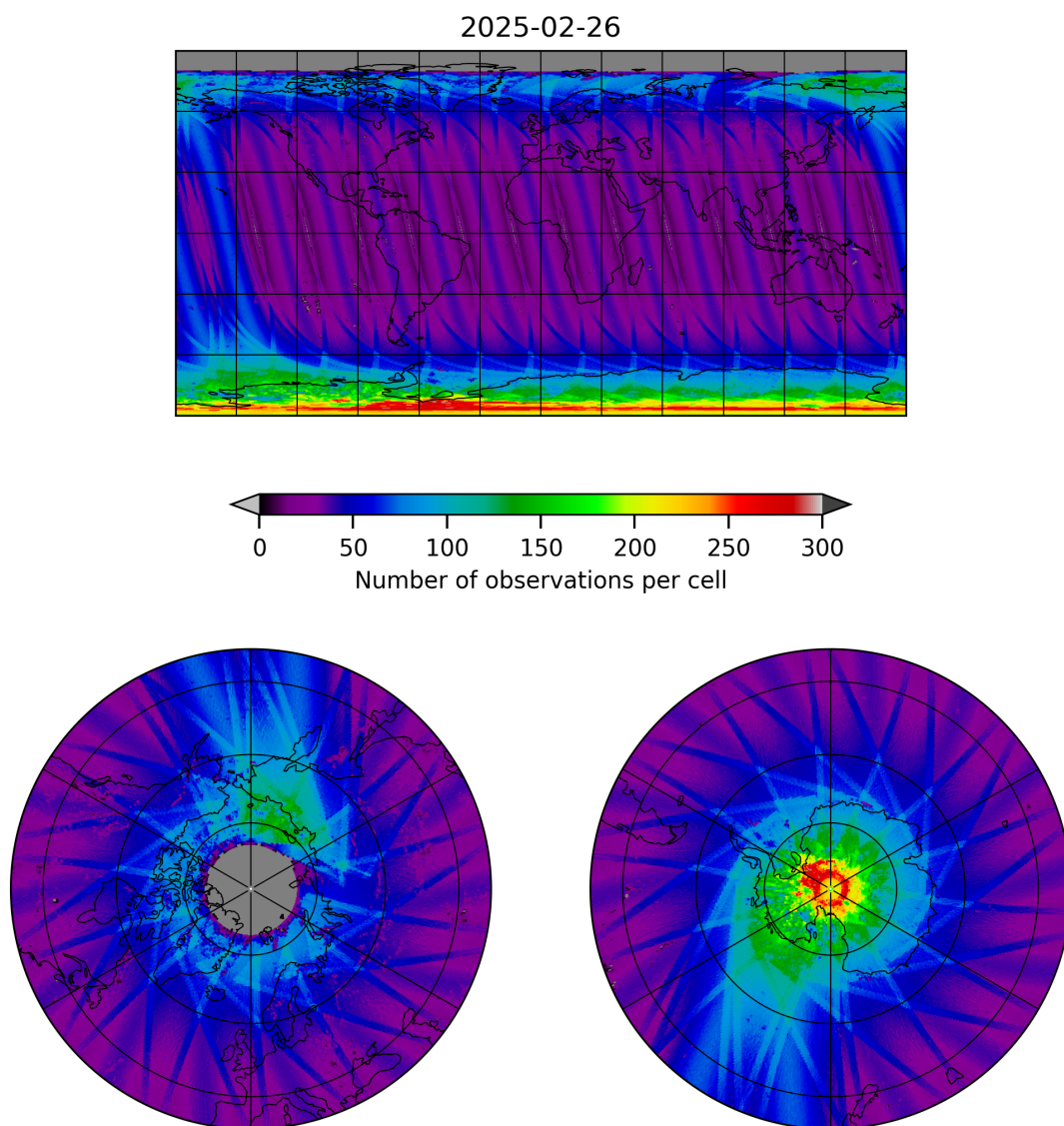
Figure 11: Map of the number of observations for 2025-02-25 to 2025-02-27
