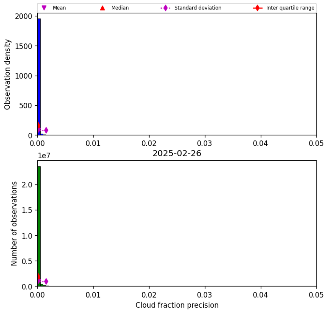
Figure 33: Histogram of “Cloud fraction precision” for 2025-02-25 to 2025-02-27
