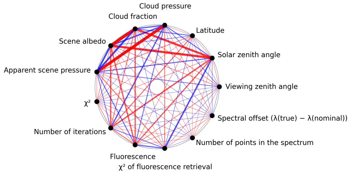
Figure 1: Map of correlation graph for 2025-02-25 to 2025-02-27.
