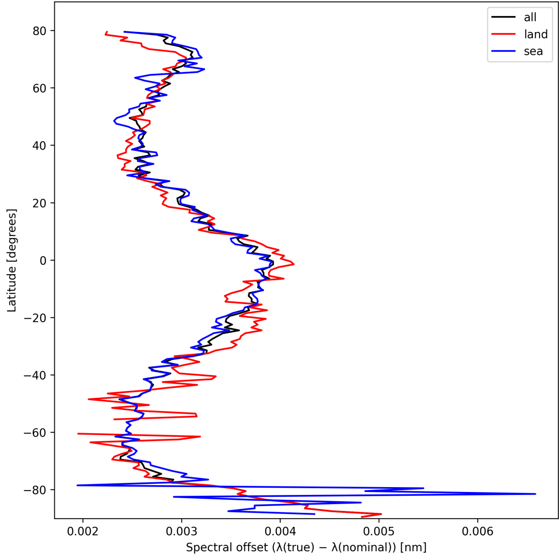
Figure 28: Zonal average of “Spectral offset ( \lambda_{\text{true}} - \lambda_{\text{nominal}} )” for 2025-02-25 to 2025-02-27.
