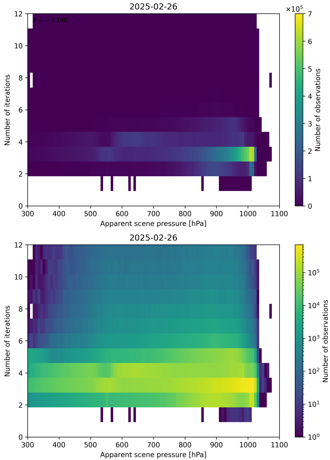
Figure 65: Scatter density plot of “Apparent scene pressure” against “Number of iterations” for 2025-02-25 to 2025-02-27.
