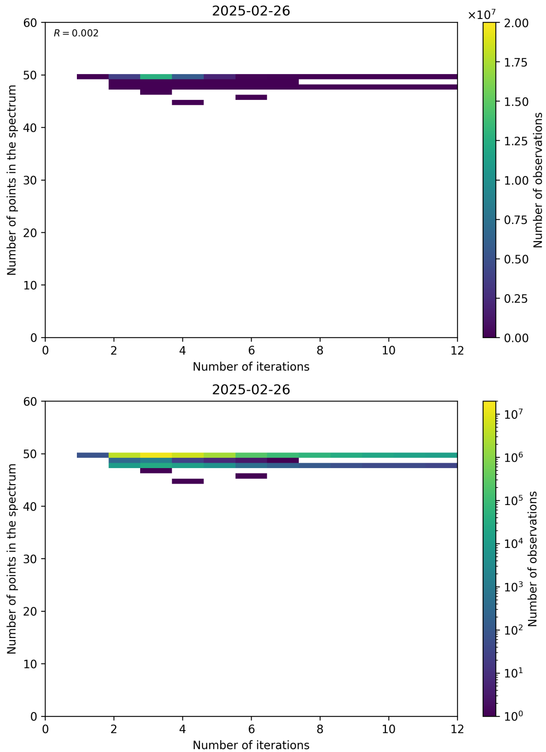
Figure 99: Scatter density plot of “Number of iterations” against “Number of points in the spectrum” for 2025-02-25 to 2025-02-27.
