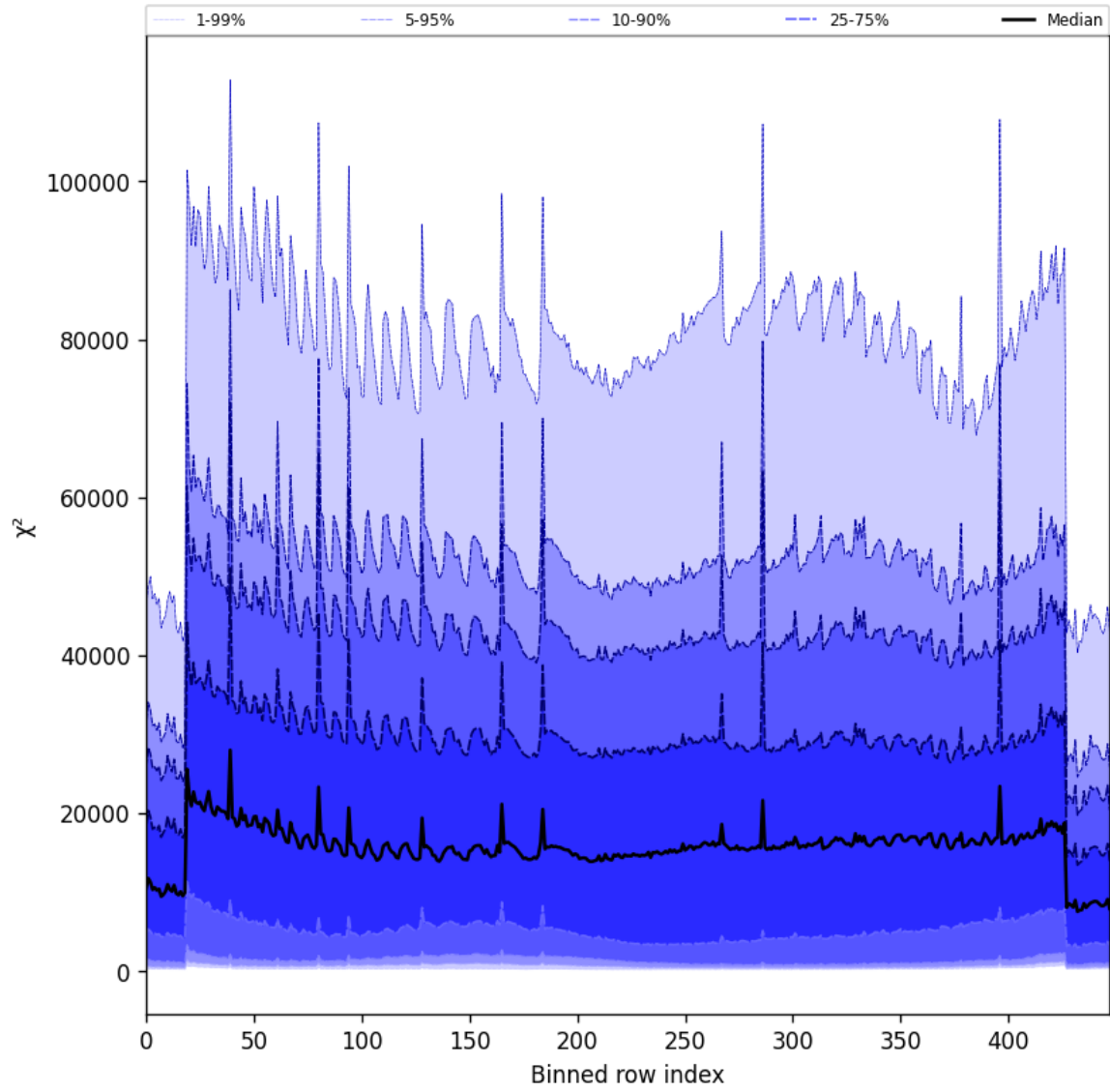
Figure 55: Along track statistics of “ \chi^2 ” for 2025-02-25 to 2025-02-27
