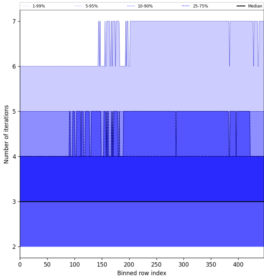
Figure 56: Along track statistics of “Number of iterations” for 2025-02-25 to 2025-02-27
