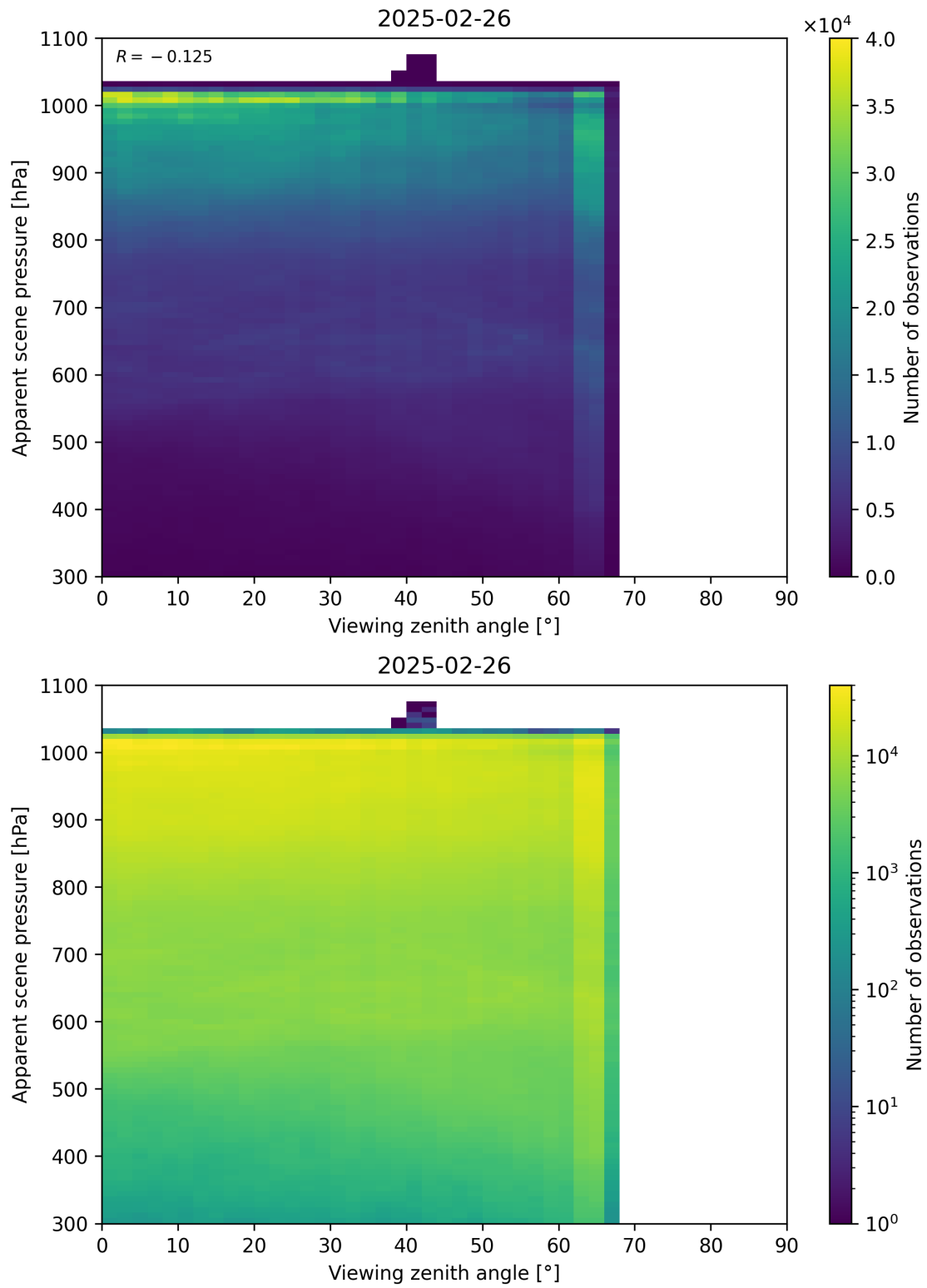
Figure 118: Scatter density plot of “Viewing zenith angle” against “Apparent scene pressure” for 2025-02-25 to 2025-02-27.
