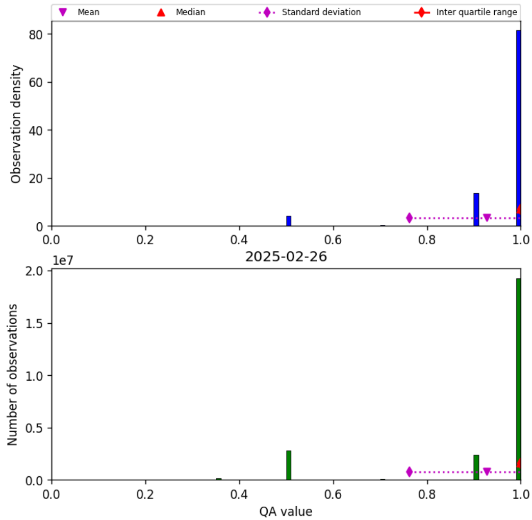
Figure 29: Histogram of "QA value" for 2025-02-25 to 2025-02-27
