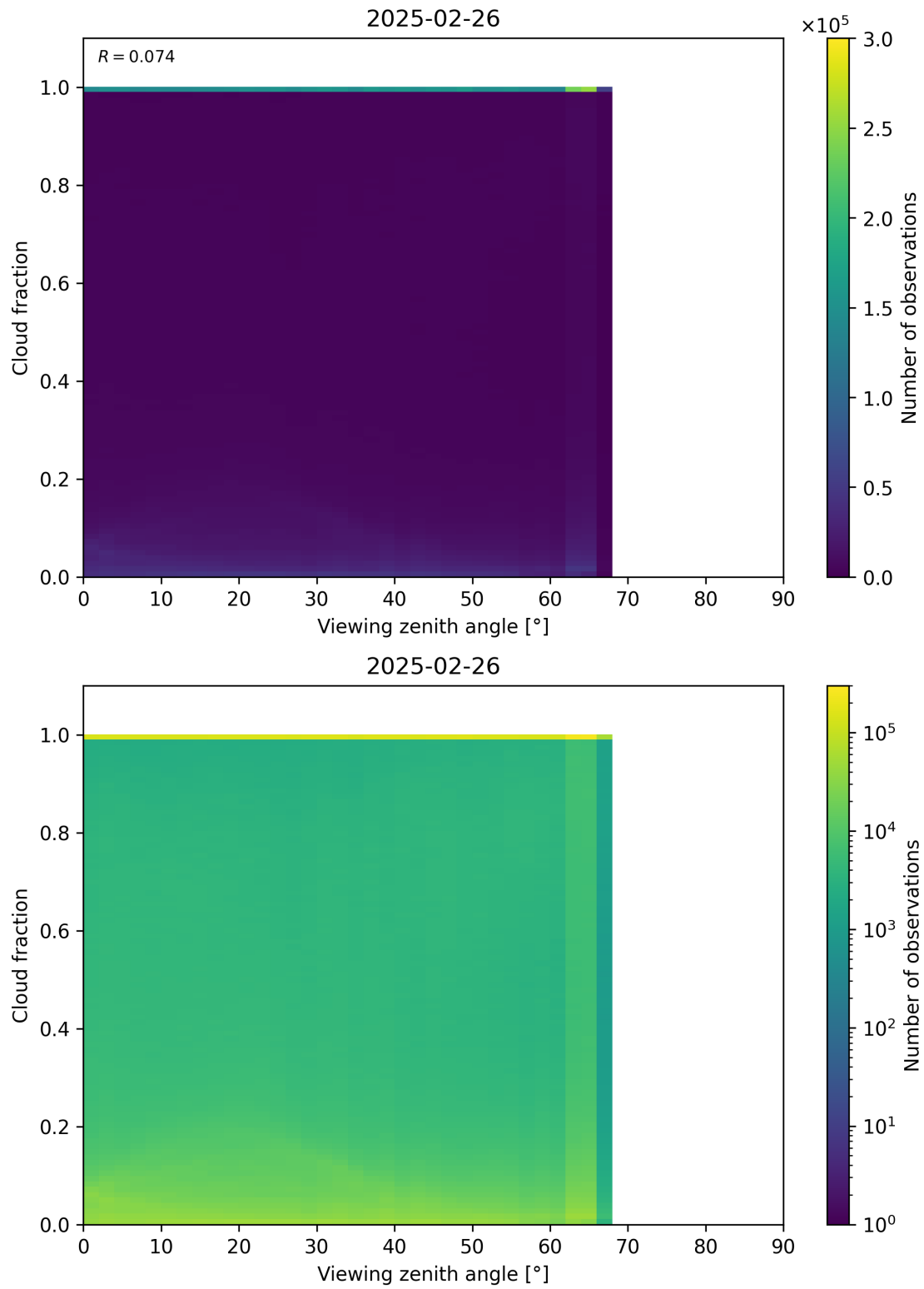
Figure 120: Scatter density plot of “Viewing zenith angle” against “Cloud fraction” for 2025-02-25 to 2025-02-27.
