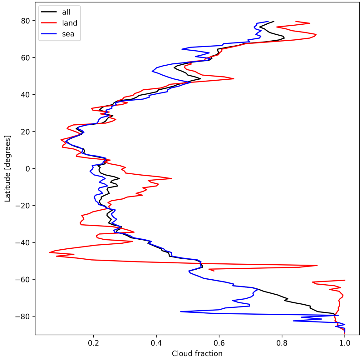
Figure 15: Zonal average of “Cloud fraction” for 2025-02-25 to 2025-02-27.
