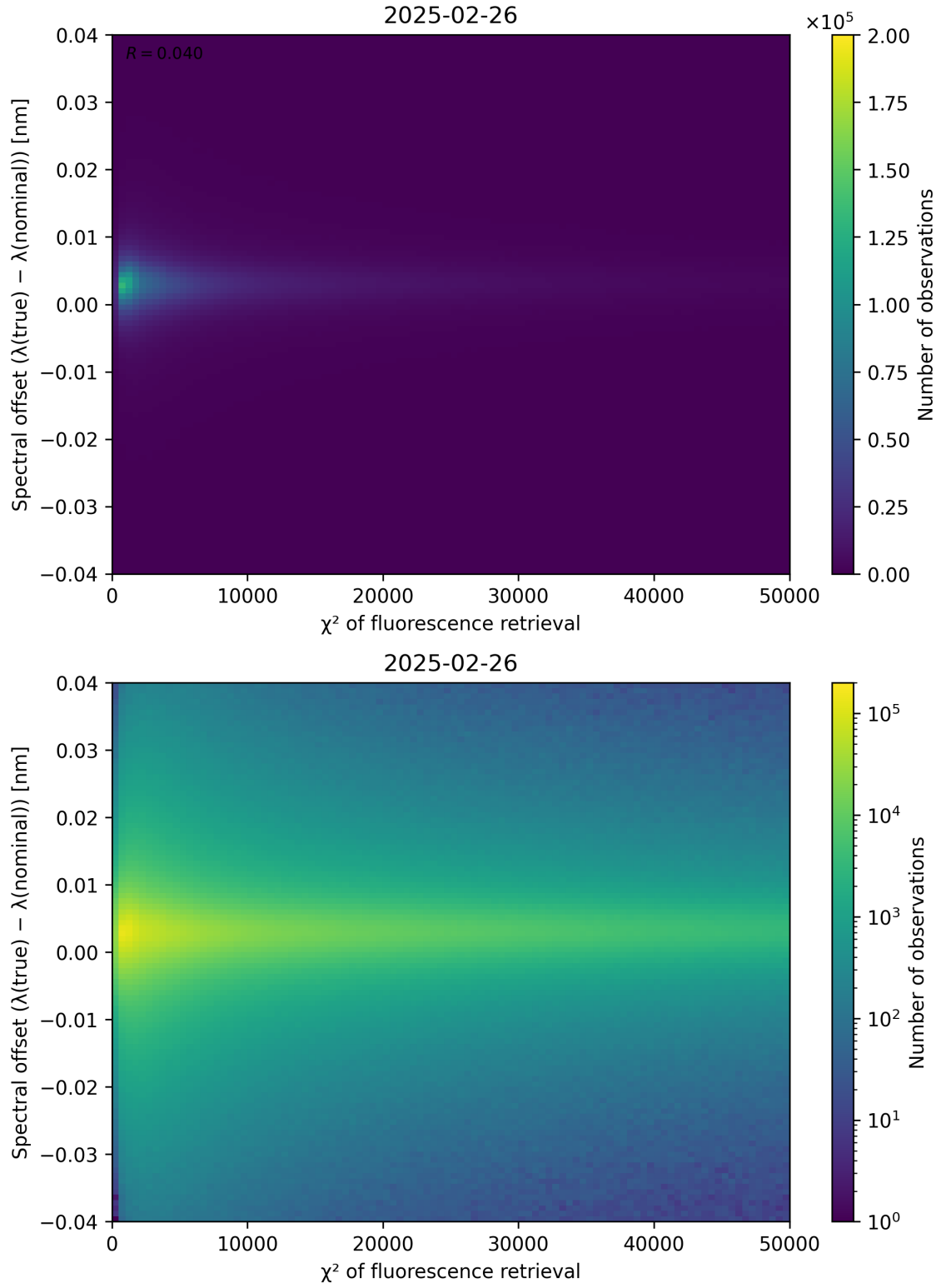
Figure 69: Scatter density plot of “ \chi^2 of fluorescence retrieval” against “Spectral offset ( \lambda_{\text{true}} - \lambda_{\text{nominal}} )” for 2025-02-25 to 2025-02-27.
