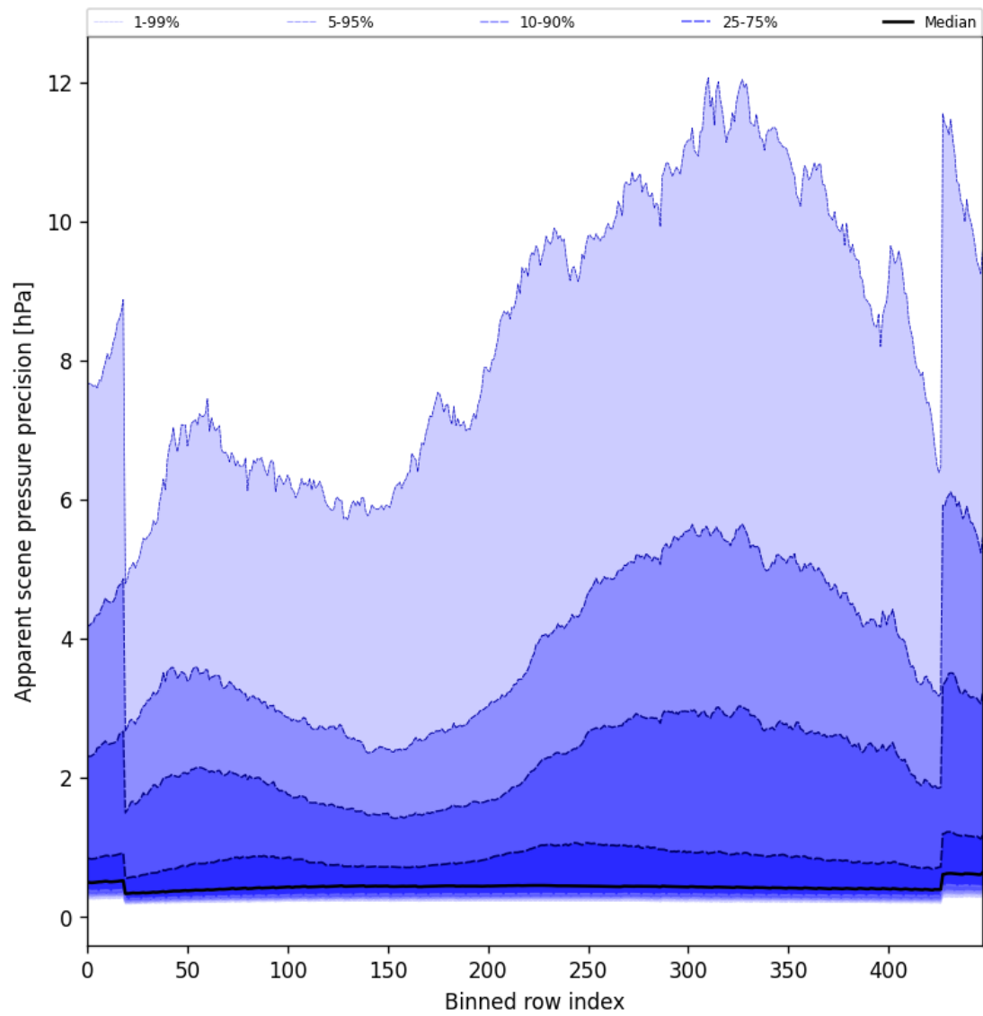
Figure 54: Along track statistics of “Apparent scene pressure precision” for 2025-02-25 to 2025-02-27
