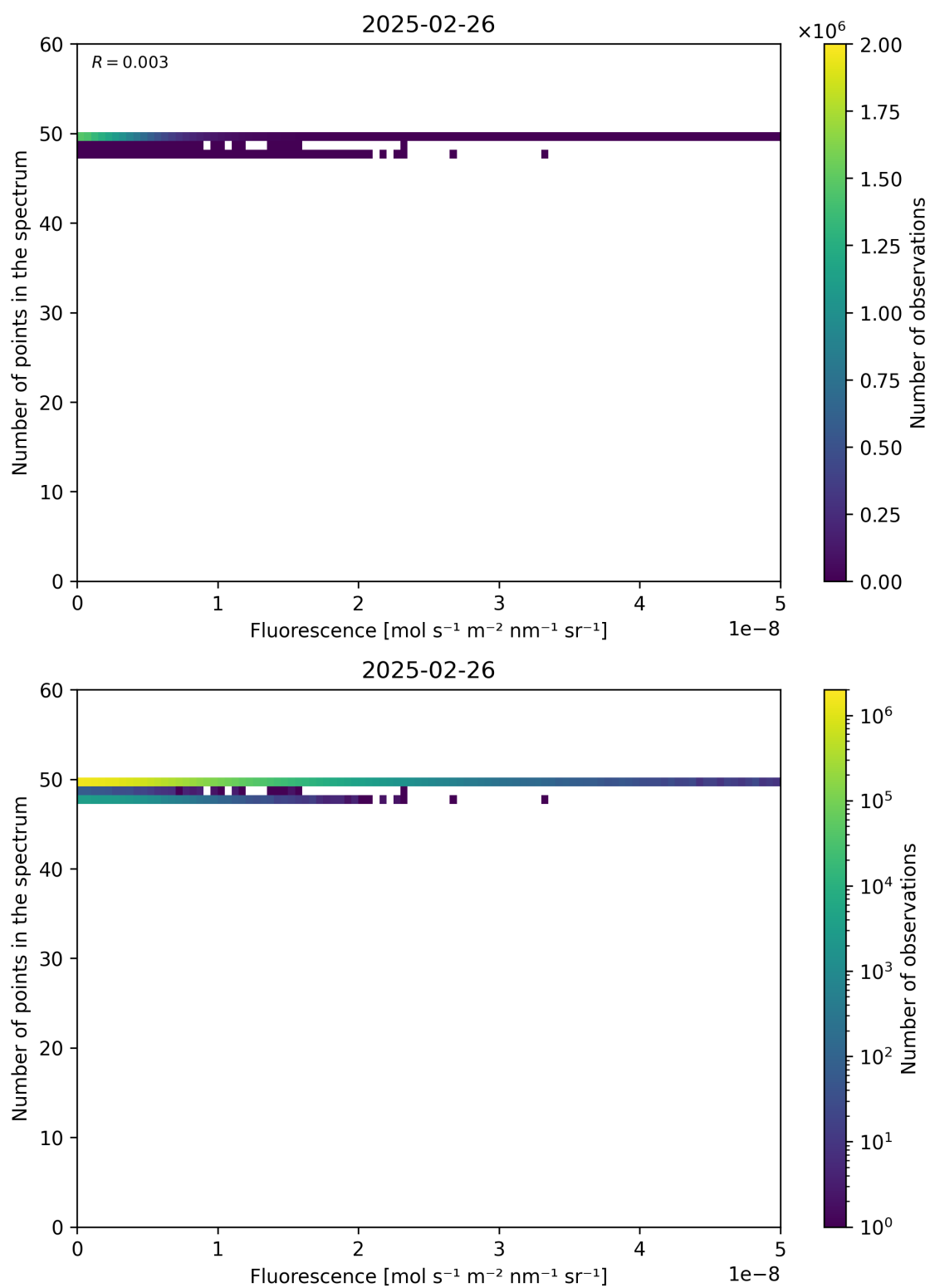
Figure 86: Scatter density plot of “Fluorescence” against “Number of points in the spectrum” for 2025-02-25 to 2025-02-27.
