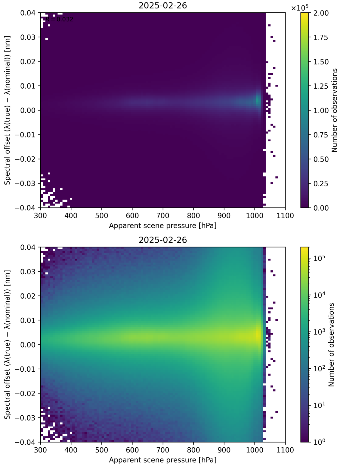
Figure 67: Scatter density plot of “Apparent scene pressure” against “Spectral offset ( \lambda_{\text{true}} - \lambda_{\text{nominal}} )” for 2025-02-25 to 2025-02-27.
