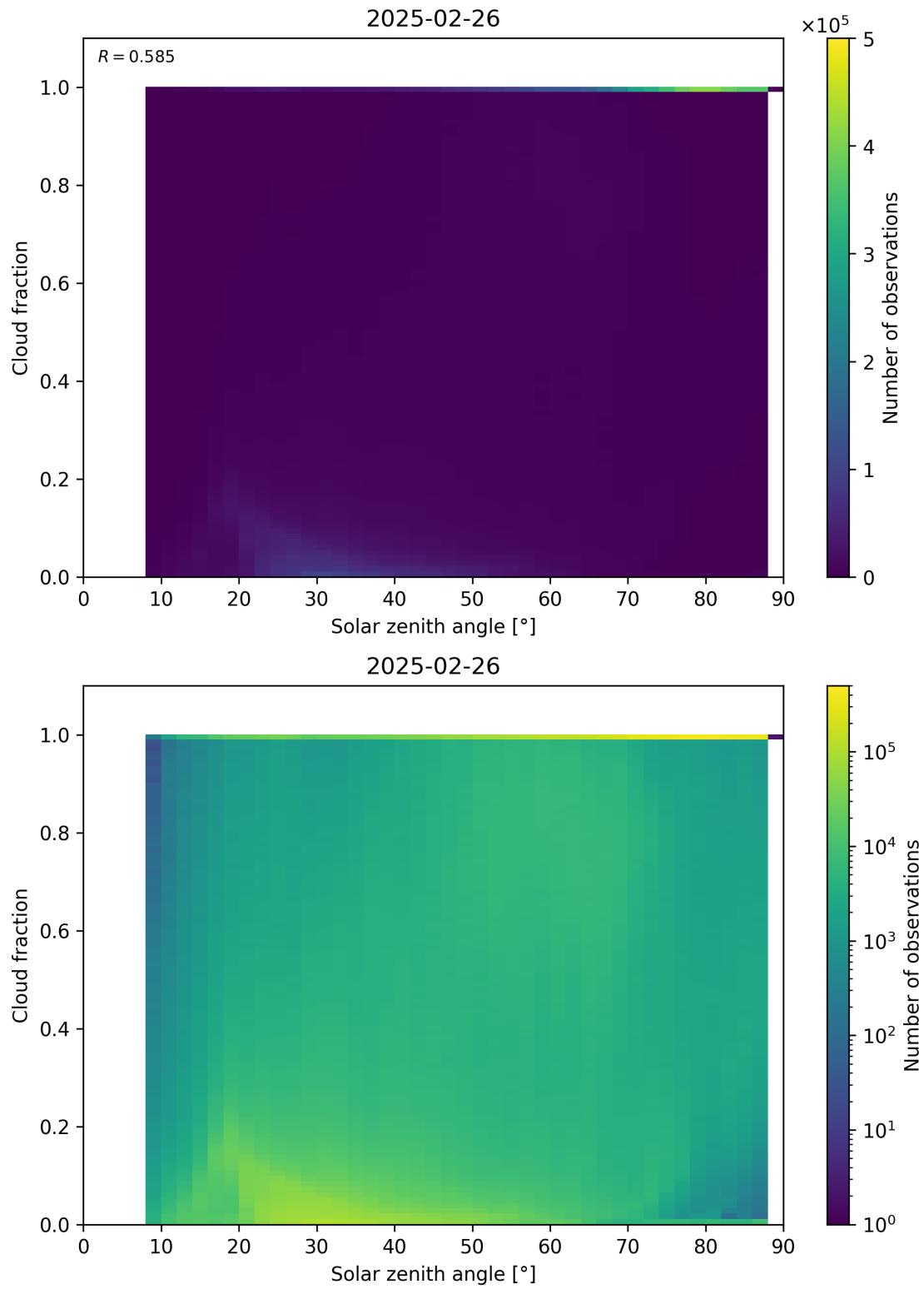
Figure 110: Scatter density plot of “Solar zenith angle” against “Cloud fraction” for 2025-02-25 to 2025-02-27.
