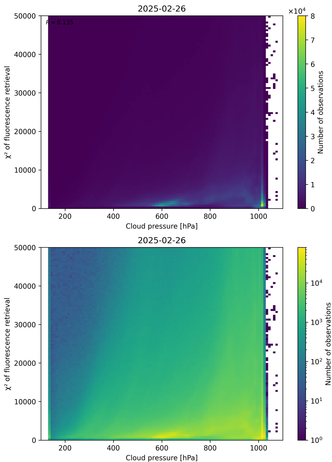
Figure 78: Scatter density plot of “Cloud pressure” against “ \chi^2 of fluorescence retrieval” for 2025-02-25 to 2025-02-27.
