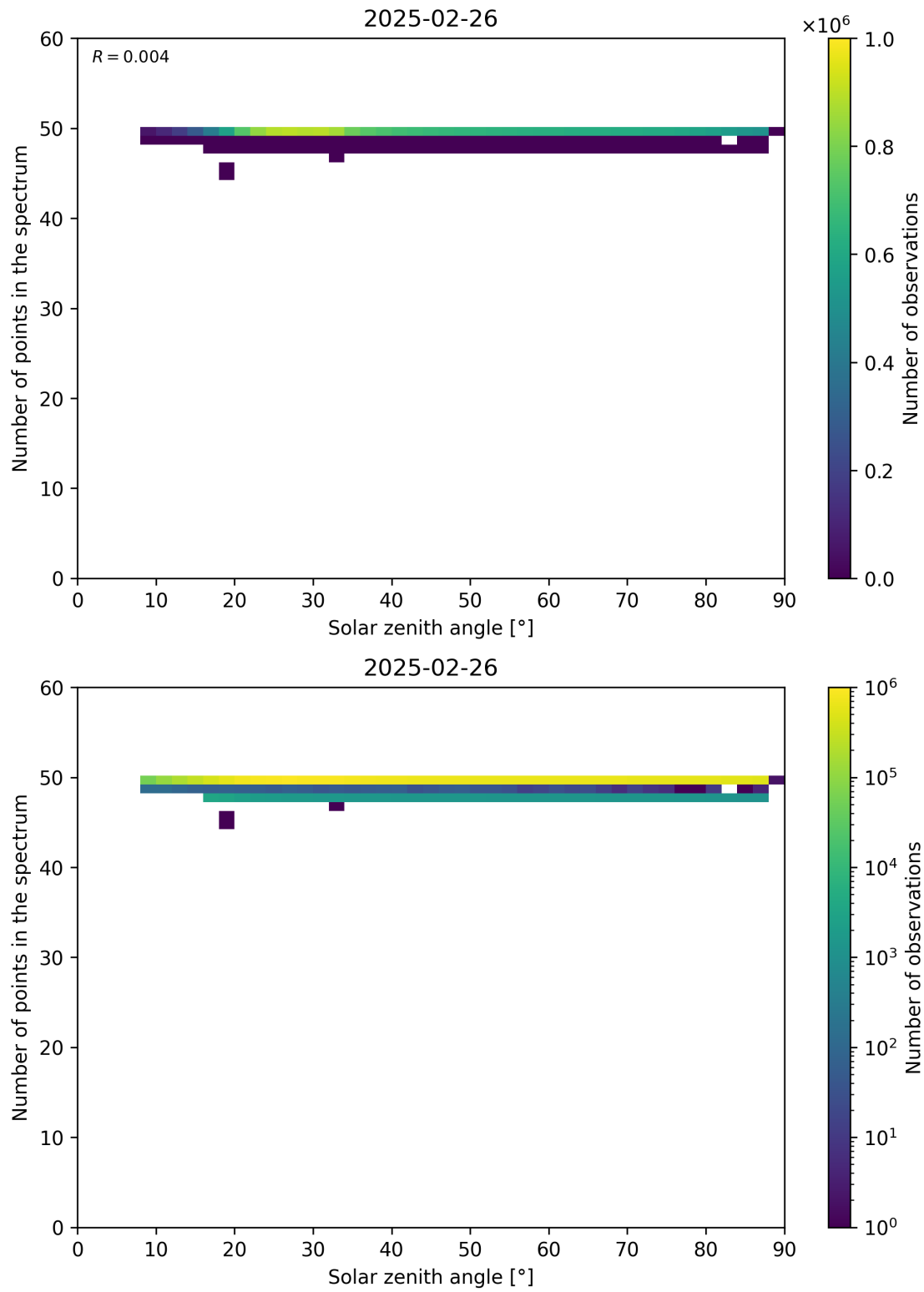
Figure 115: Scatter density plot of “Solar zenith angle” against “Number of points in the spectrum” for 2025-02-25 to 2025-02-27.
