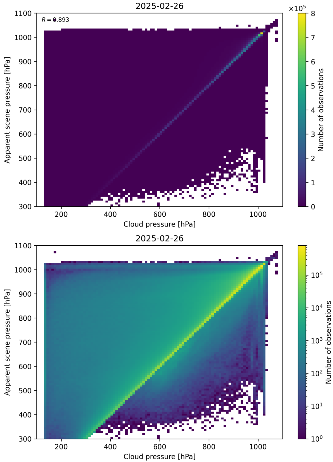
Figure 77: Scatter density plot of “Cloud pressure” against “Apparent scene pressure” for 2025-02-25 to 2025-02-27.
