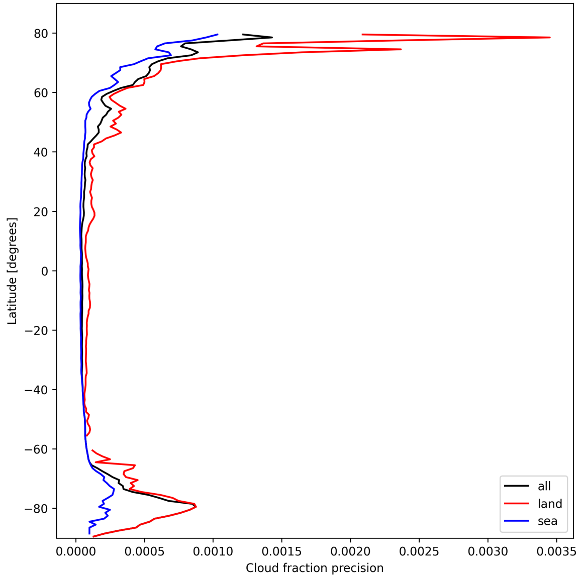
Figure 16: Zonal average of “Cloud fraction precision” for 2025-02-25 to 2025-02-27.
