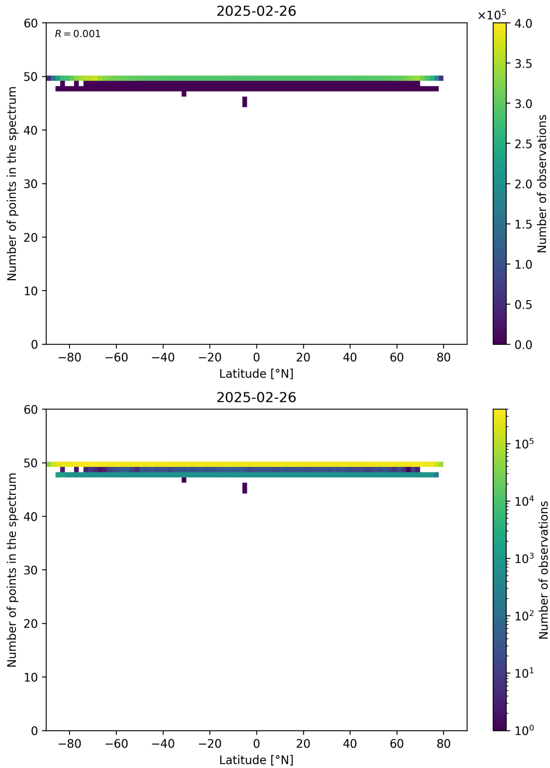
Figure 94: Scatter density plot of “Latitude” against “Number of points in the spectrum” for 2025-02-25 to 2025-02-27.
