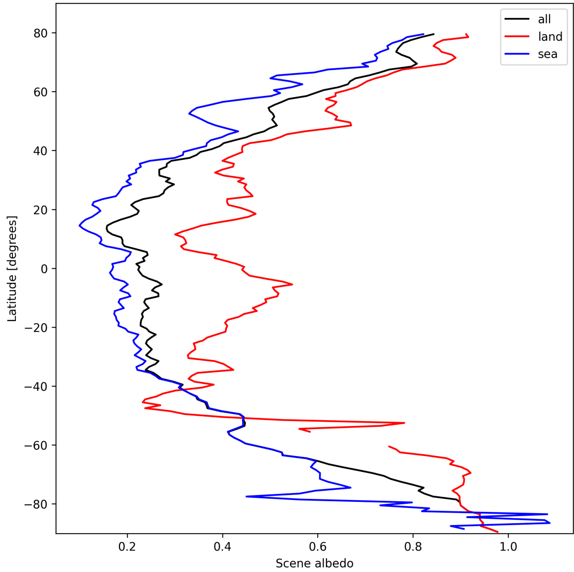
Figure 17: Zonal average of “Scene albedo” for 2025-02-25 to 2025-02-27.
