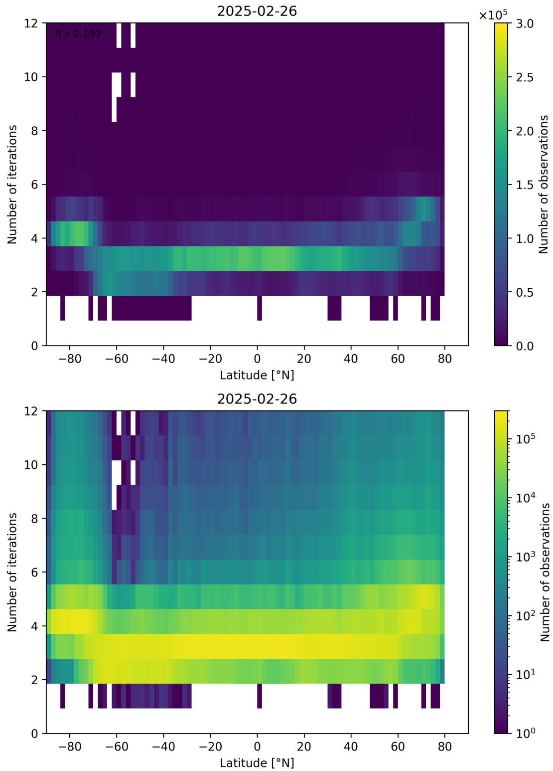
Figure 93: Scatter density plot of “Latitude” against “Number of iterations” for 2025-02-25 to 2025-02-27.
