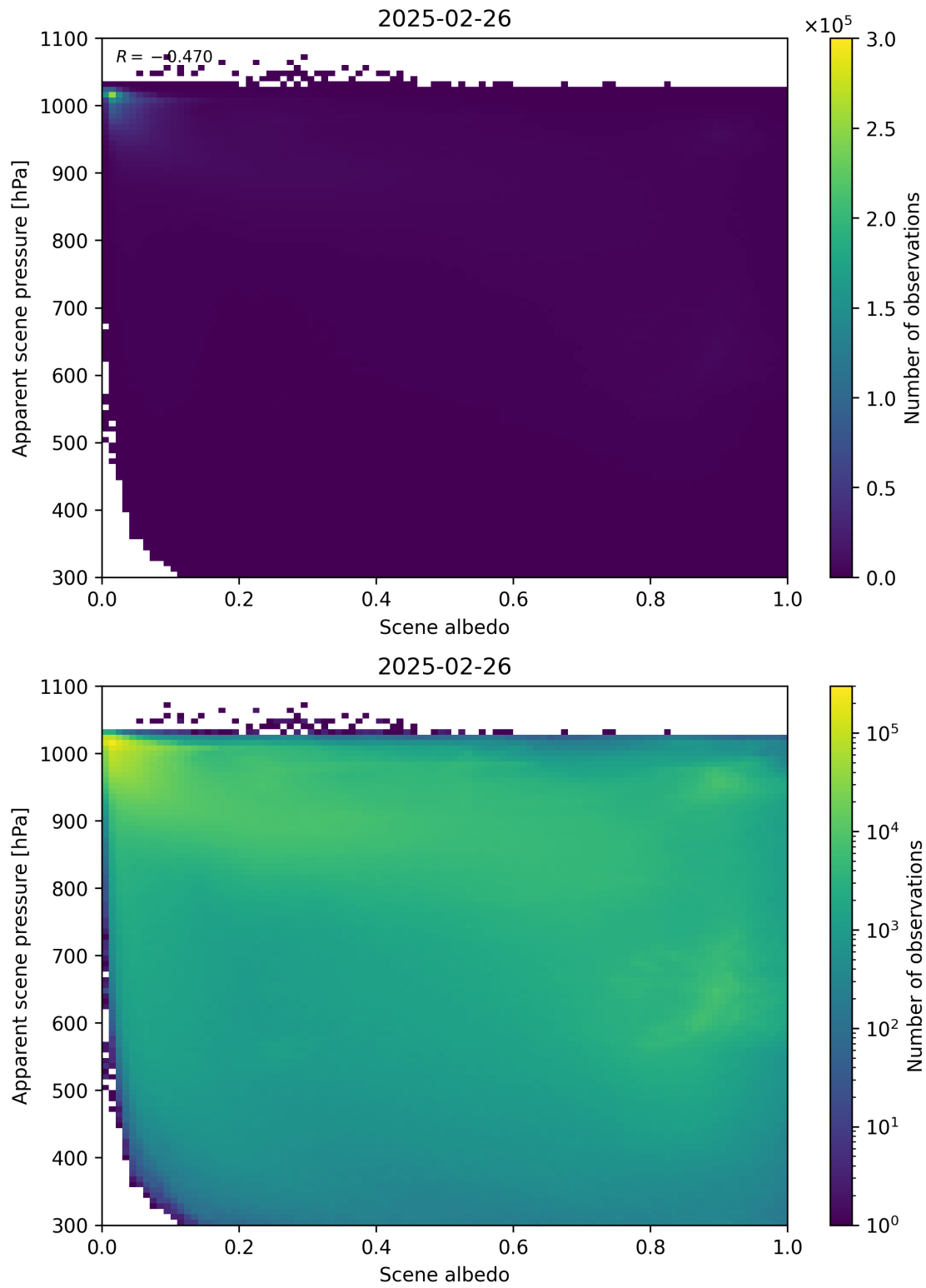
Figure 102: Scatter density plot of “Scene albedo” against “Apparent scene pressure” for 2025-02-25 to 2025-02-27.
