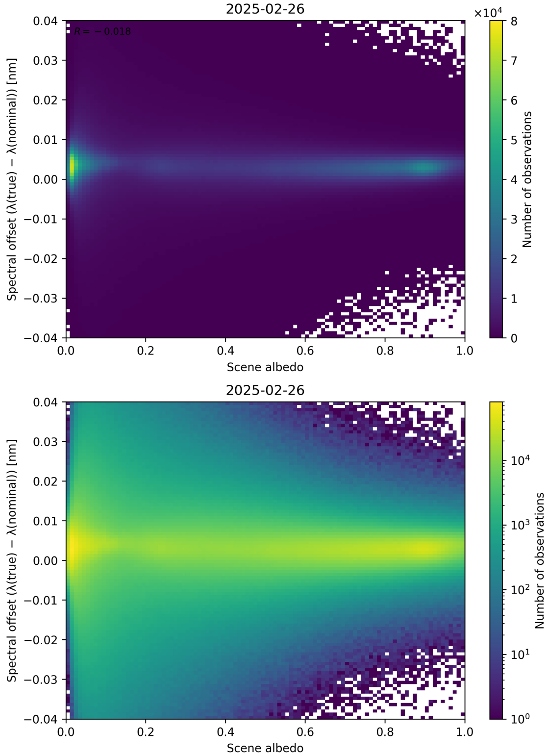
Figure 107: Scatter density plot of “Scene albedo” against “Spectral offset ( \lambda_{\text{true}} - \lambda_{\text{nominal}} )” for 2025-02-25 to 2025-02-27.
