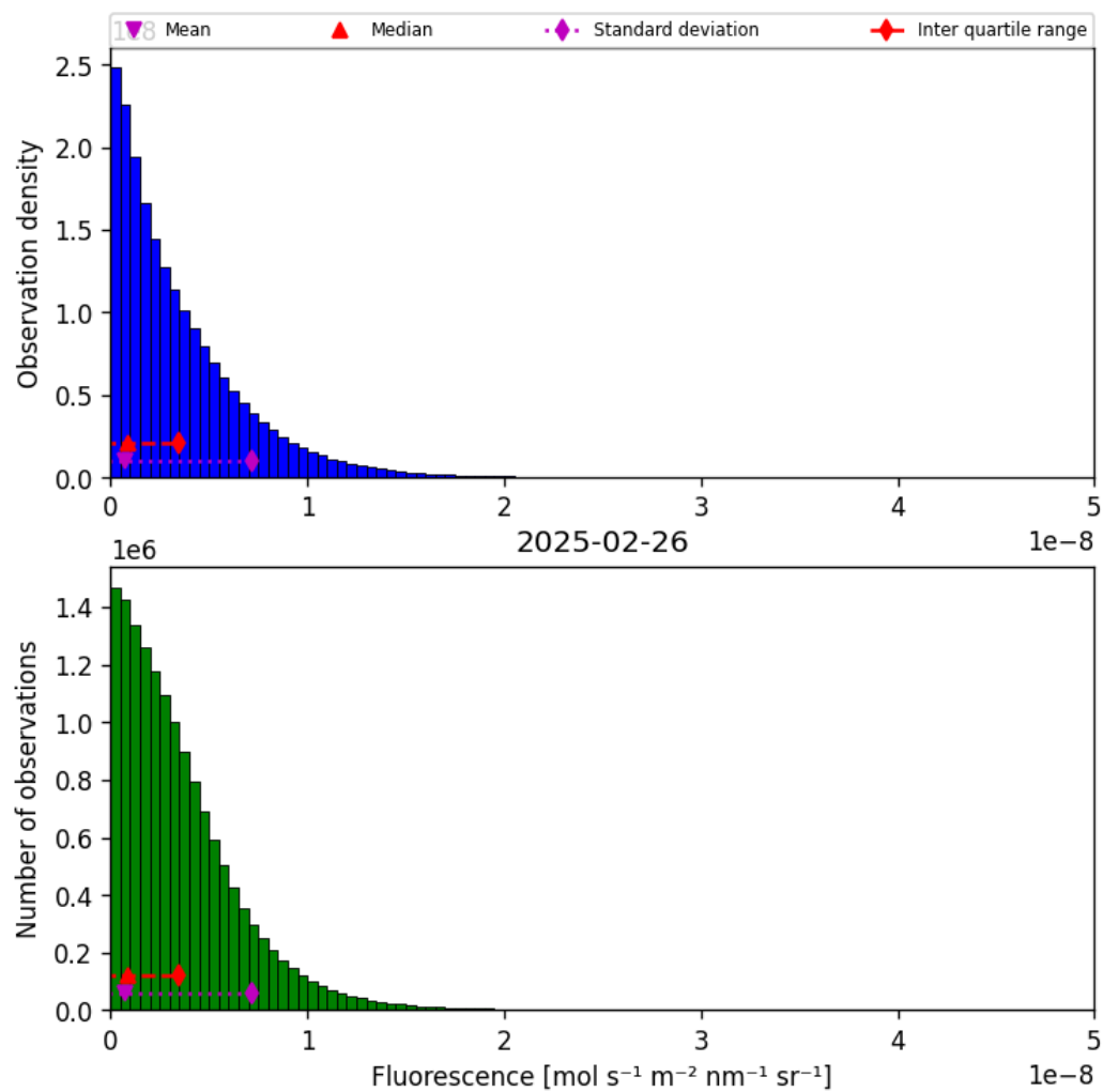
Figure 40: Histogram of “Fluorescence” for 2025-02-25 to 2025-02-27
