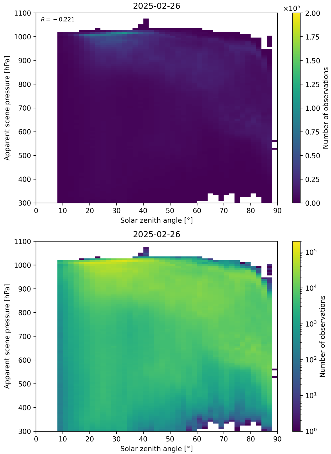
Figure 108: Scatter density plot of “Solar zenith angle” against “Apparent scene pressure” for 2025-02-25 to 2025-02-27.
