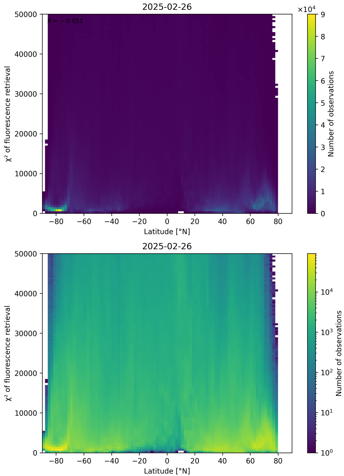
Figure 89: Scatter density plot of “Latitude” against “ \chi^2 of fluorescence retrieval” for 2025-02-25 to 2025-02-27.
