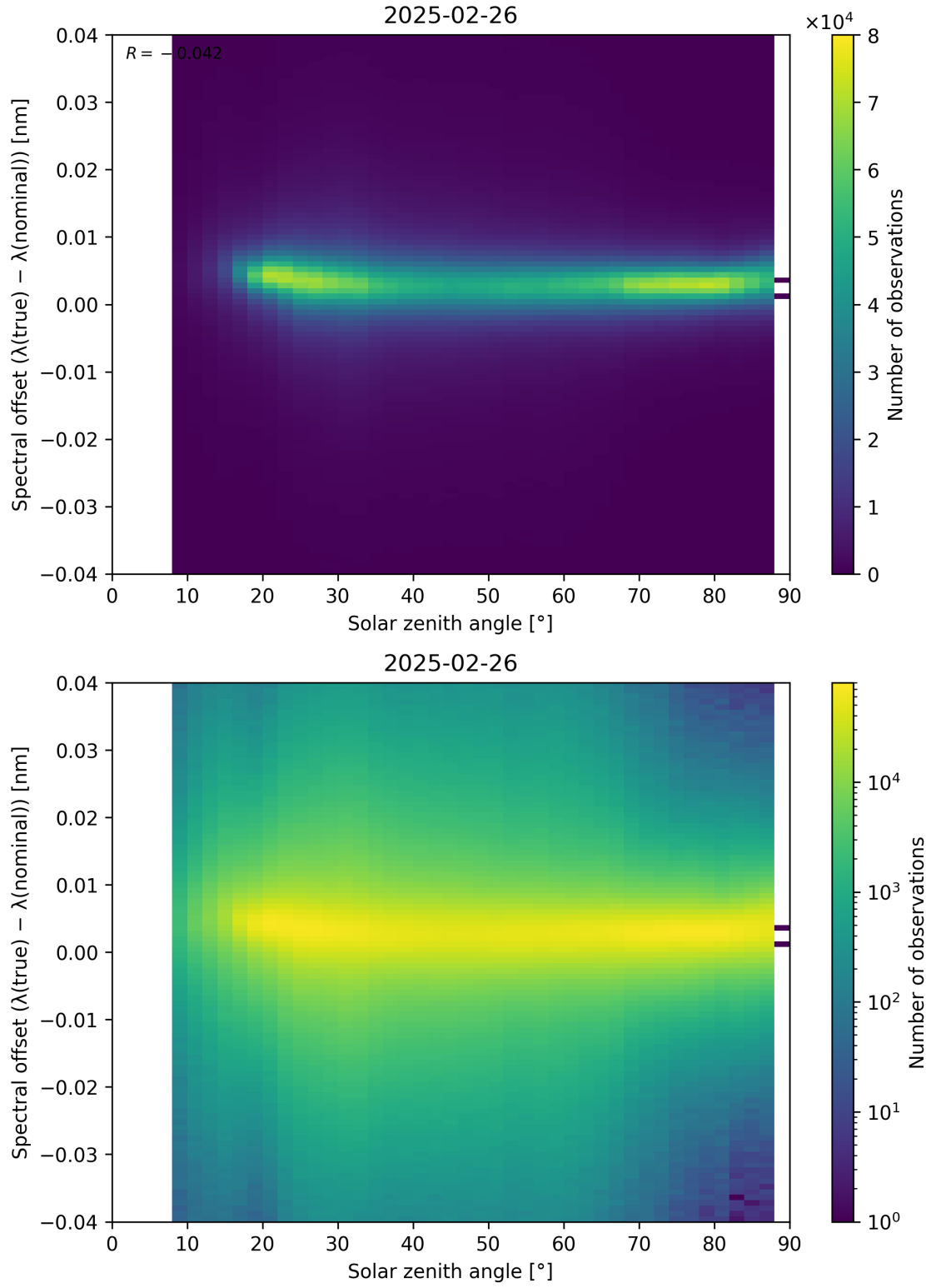
Figure 117: Scatter density plot of “Solar zenith angle” against “Spectral offset ( \lambda_{\text{true}} - \lambda_{\text{nominal}} )” for 2025-02-25 to 2025-02-27.
