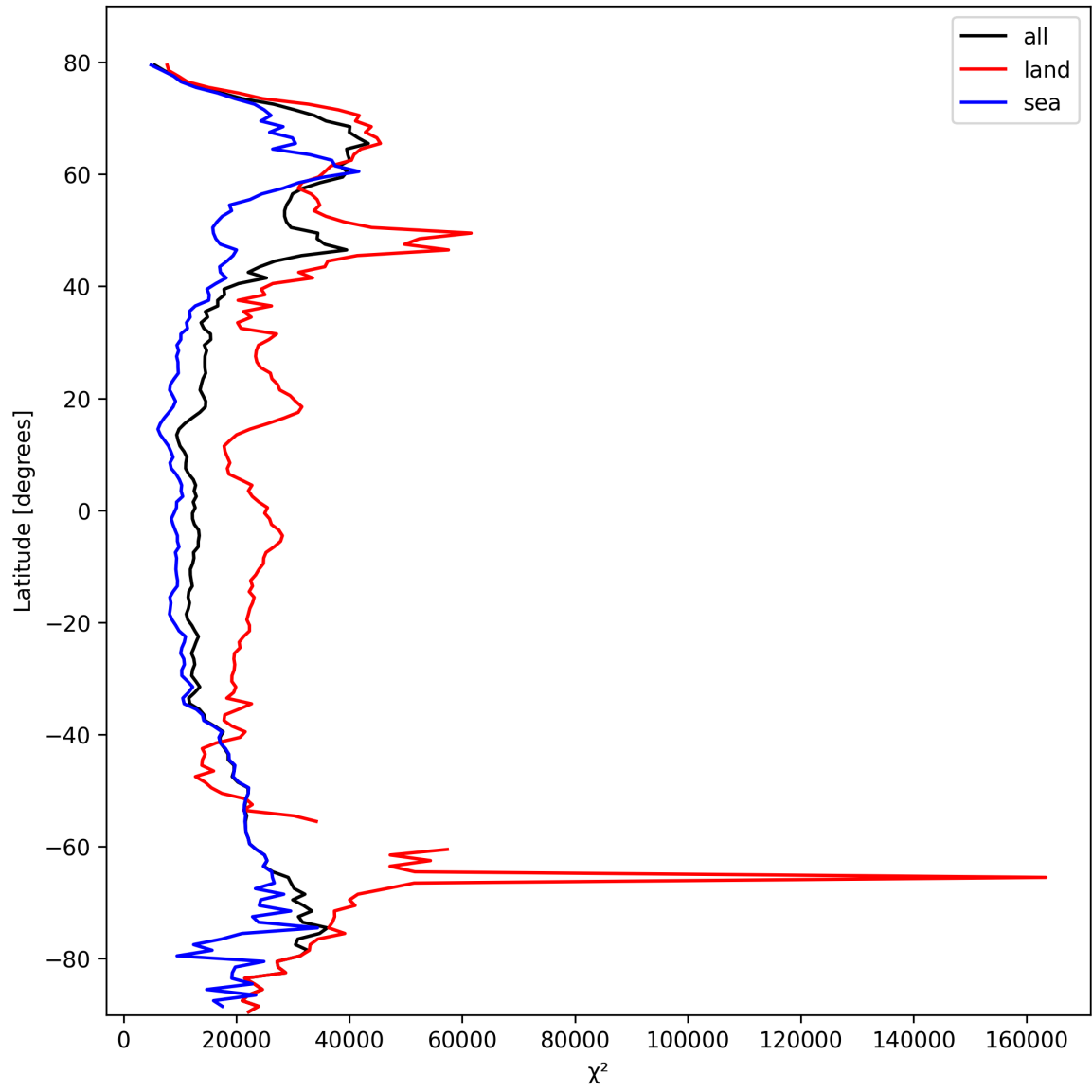
Figure 21: Zonal average of “ \chi^2 ” for 2025-02-25 to 2025-02-27.
