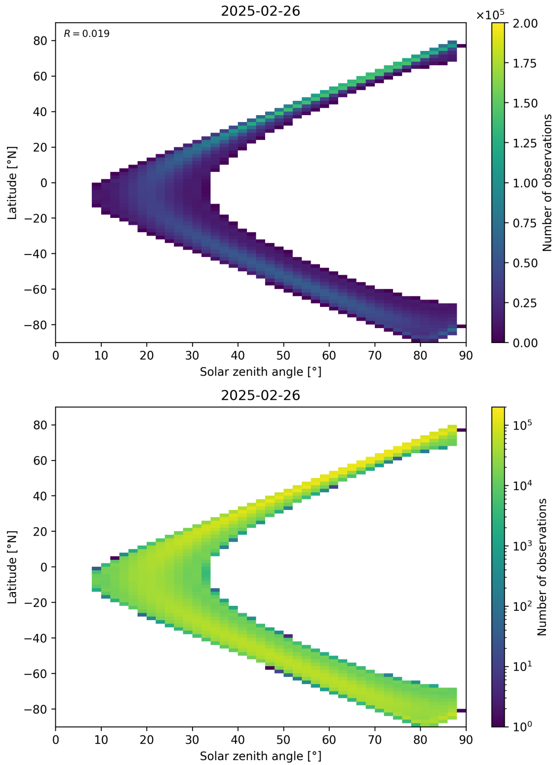
Figure 113: Scatter density plot of “Solar zenith angle” against “Latitude” for 2025-02-25 to 2025-02-27.
