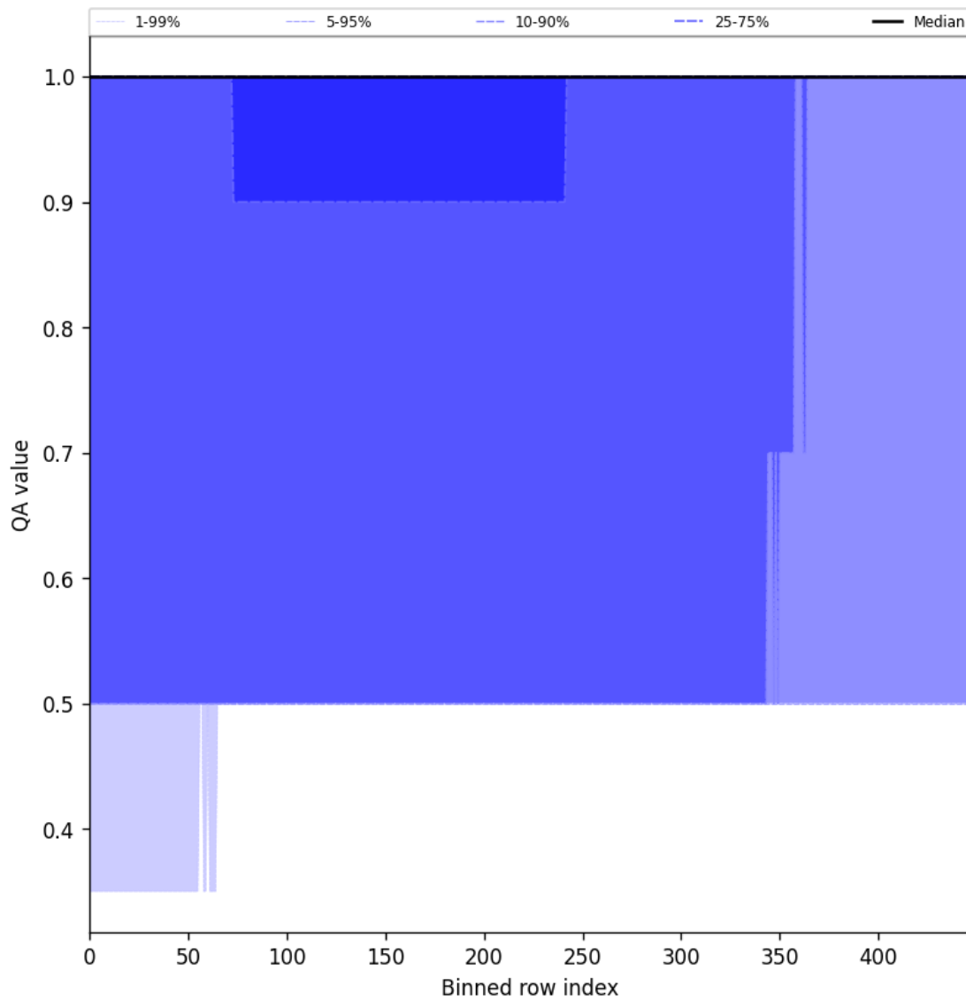
Figure 46: Along track statistics of “QA value” for 2025-02-25 to 2025-02-27
