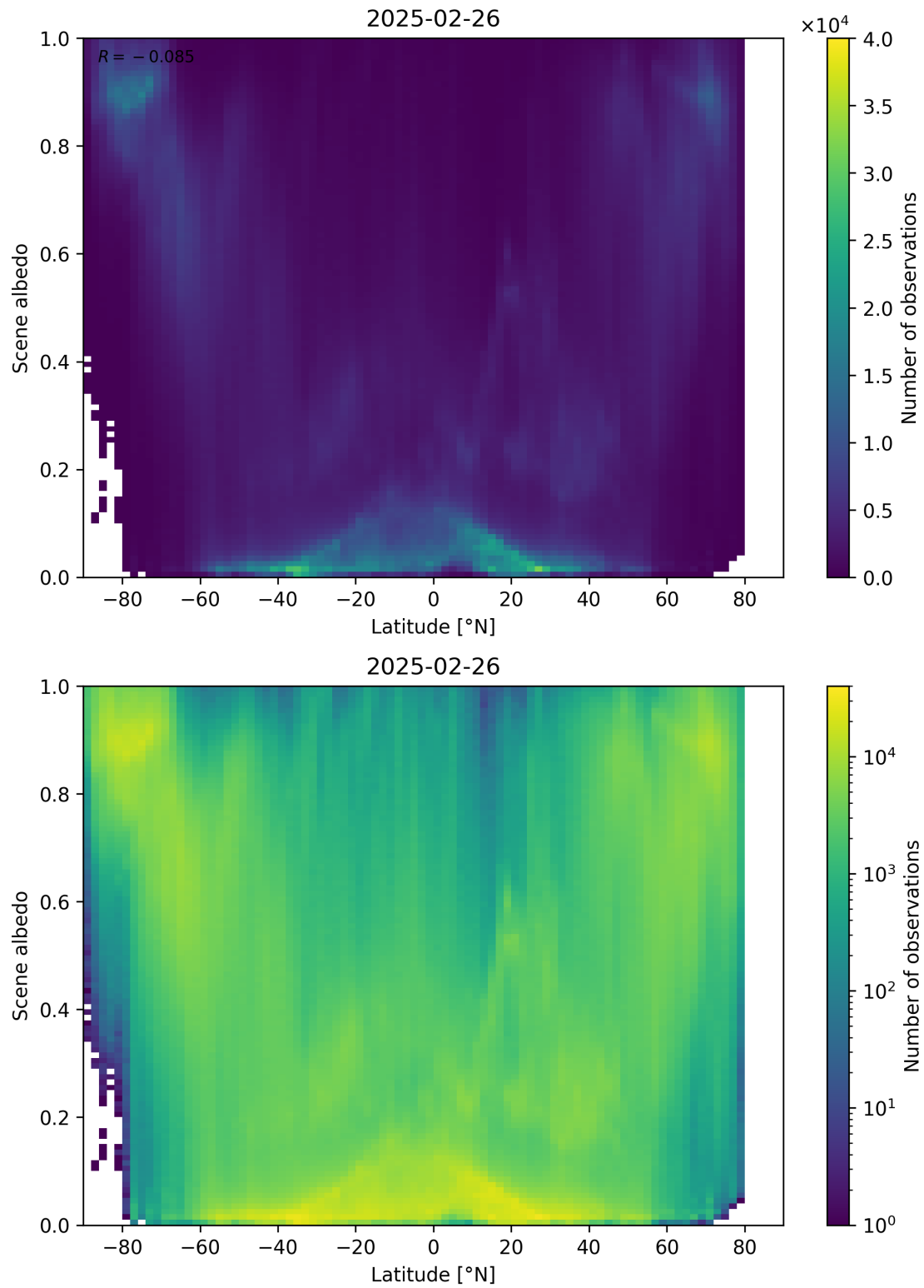
Figure 95: Scatter density plot of “Latitude” against “Scene albedo” for 2025-02-25 to 2025-02-27.
