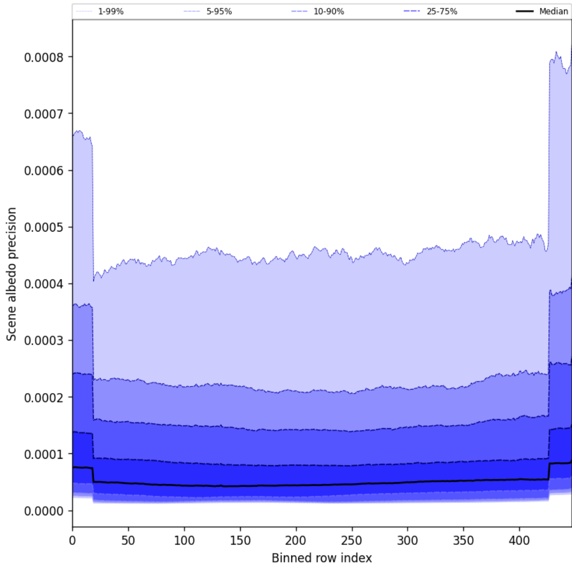
Figure 52: Along track statistics of “Scene albedo precision” for 2025-02-25 to 2025-02-27
