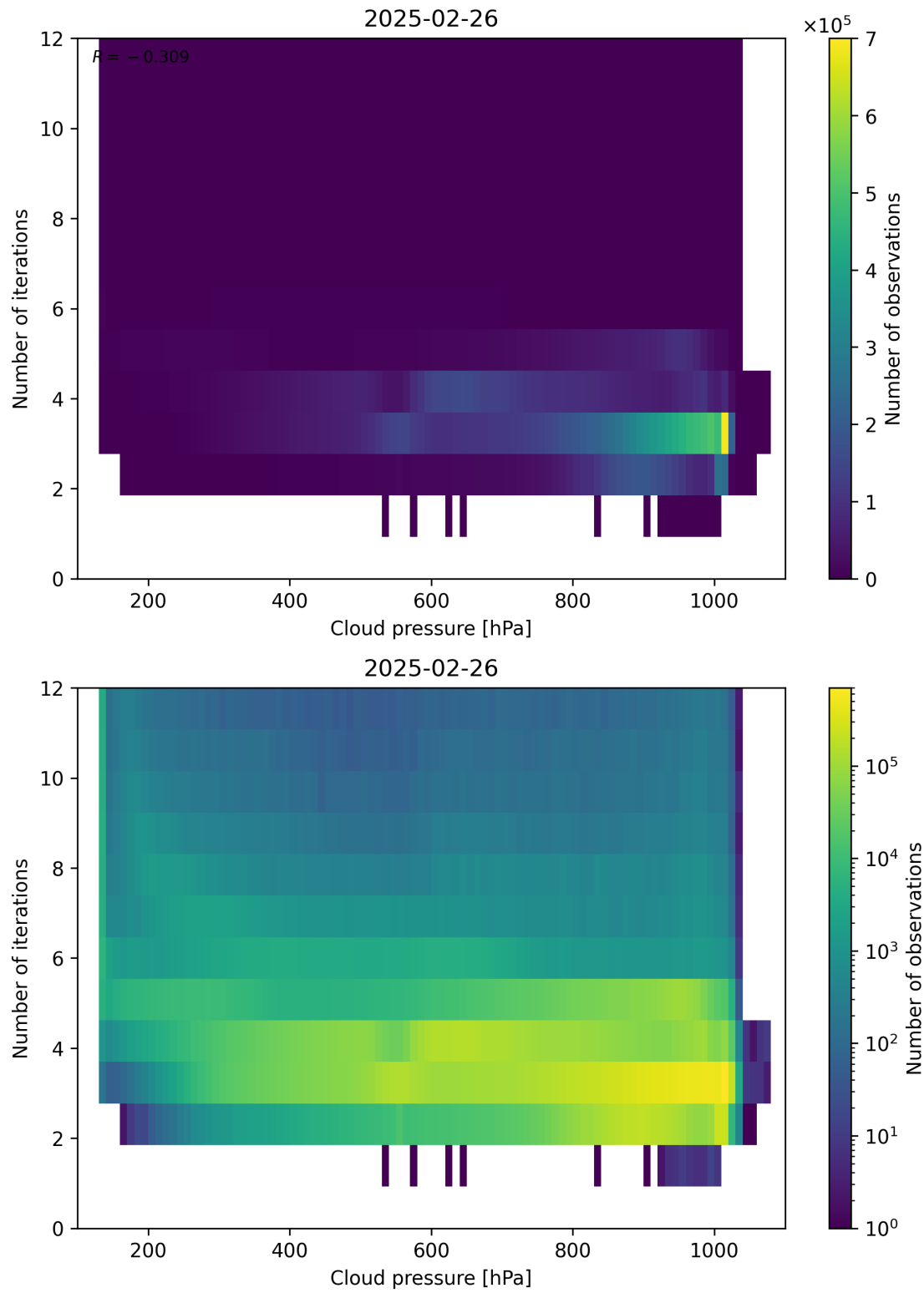
Figure 81: Scatter density plot of “Cloud pressure” against “Number of iterations” for 2025-02-25 to 2025-02-27.
