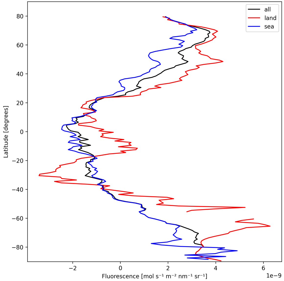
Figure 23: Zonal average of “Fluorescence” for 2025-02-25 to 2025-02-27.
