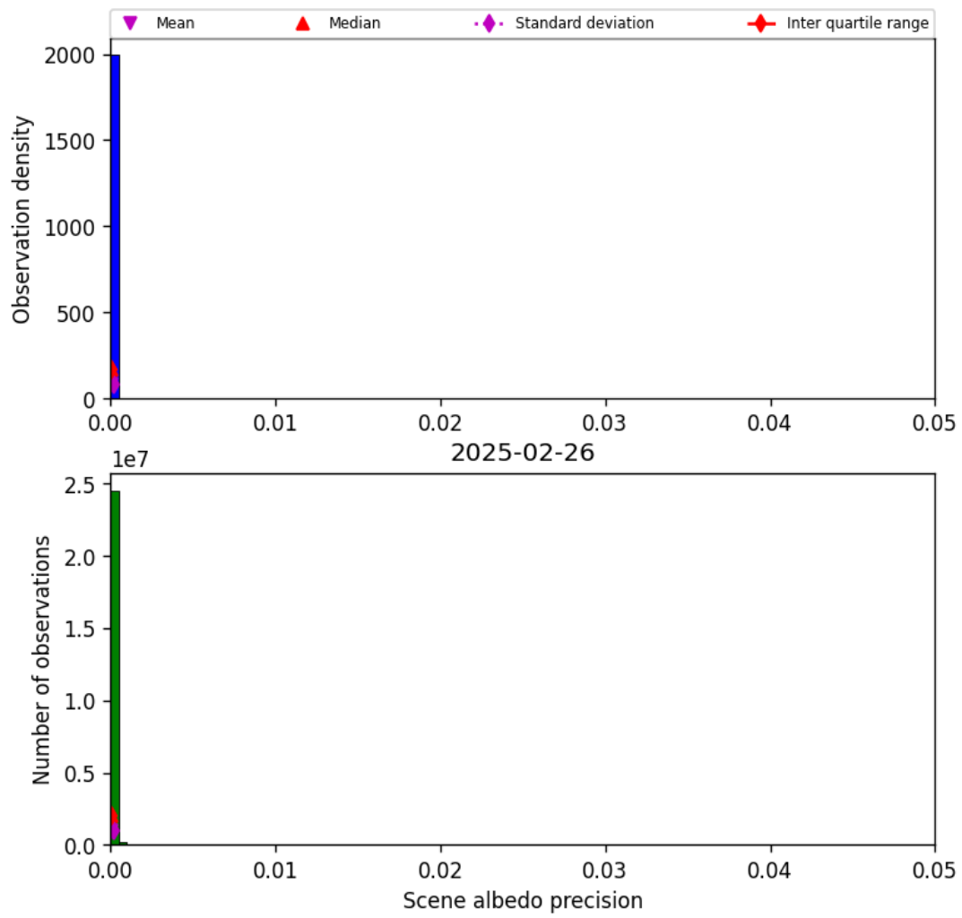
Figure 35: Histogram of “Scene albedo precision” for 2025-02-25 to 2025-02-27
