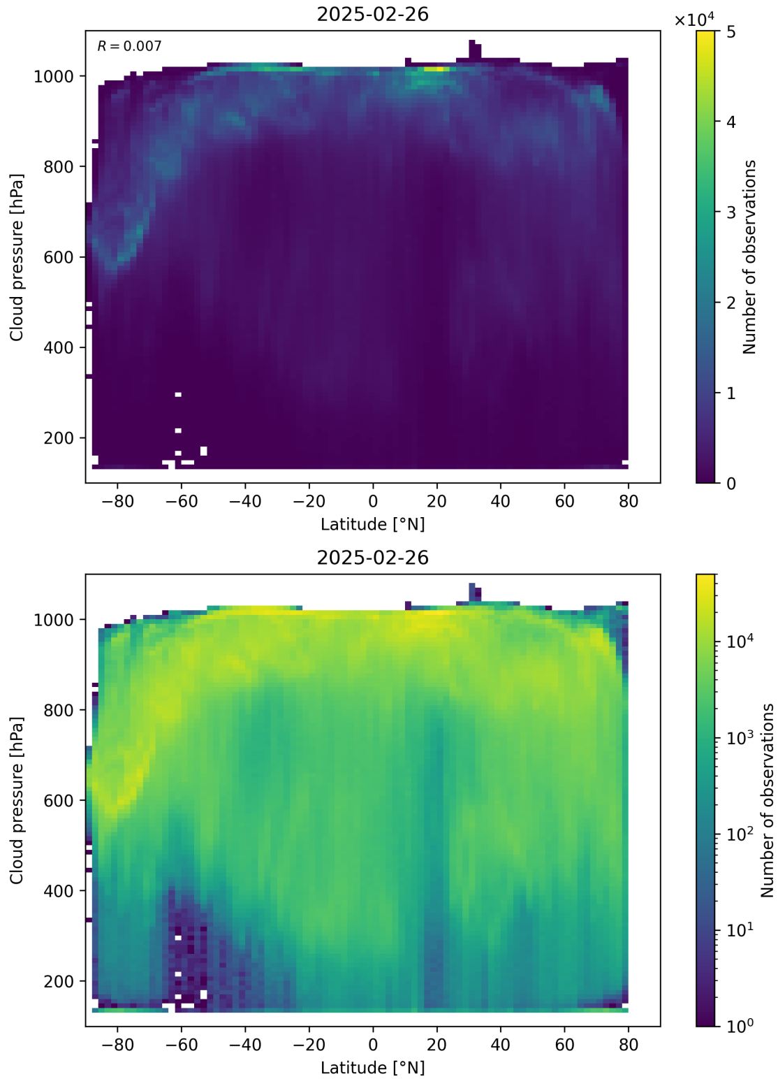
Figure 91: Scatter density plot of “Latitude” against “Cloud pressure” for 2025-02-25 to 2025-02-27.
