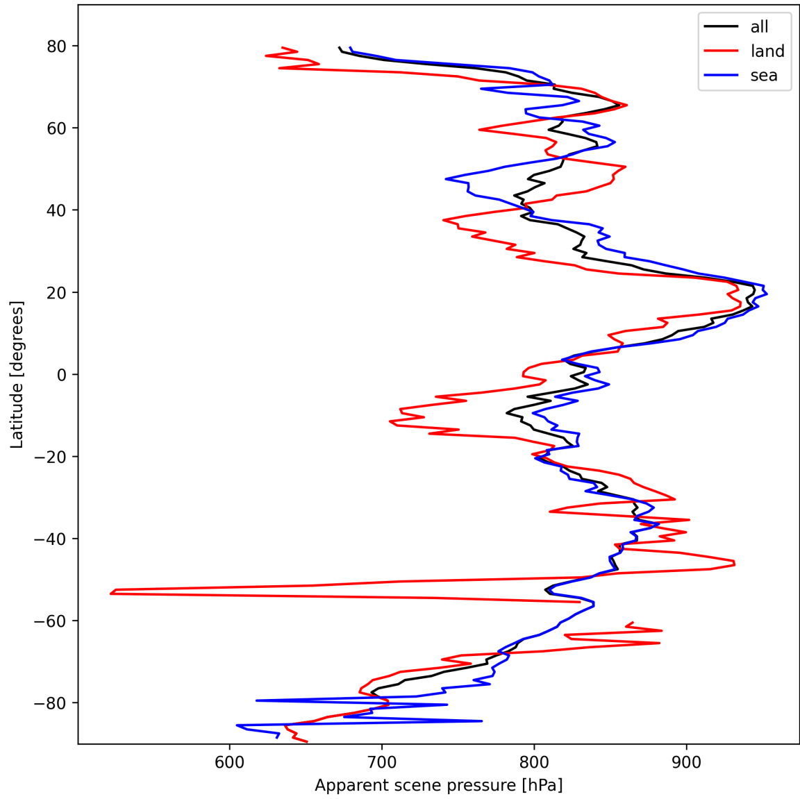
Figure 19: Zonal average of “Apparent scene pressure” for 2025-02-25 to 2025-02-27.
