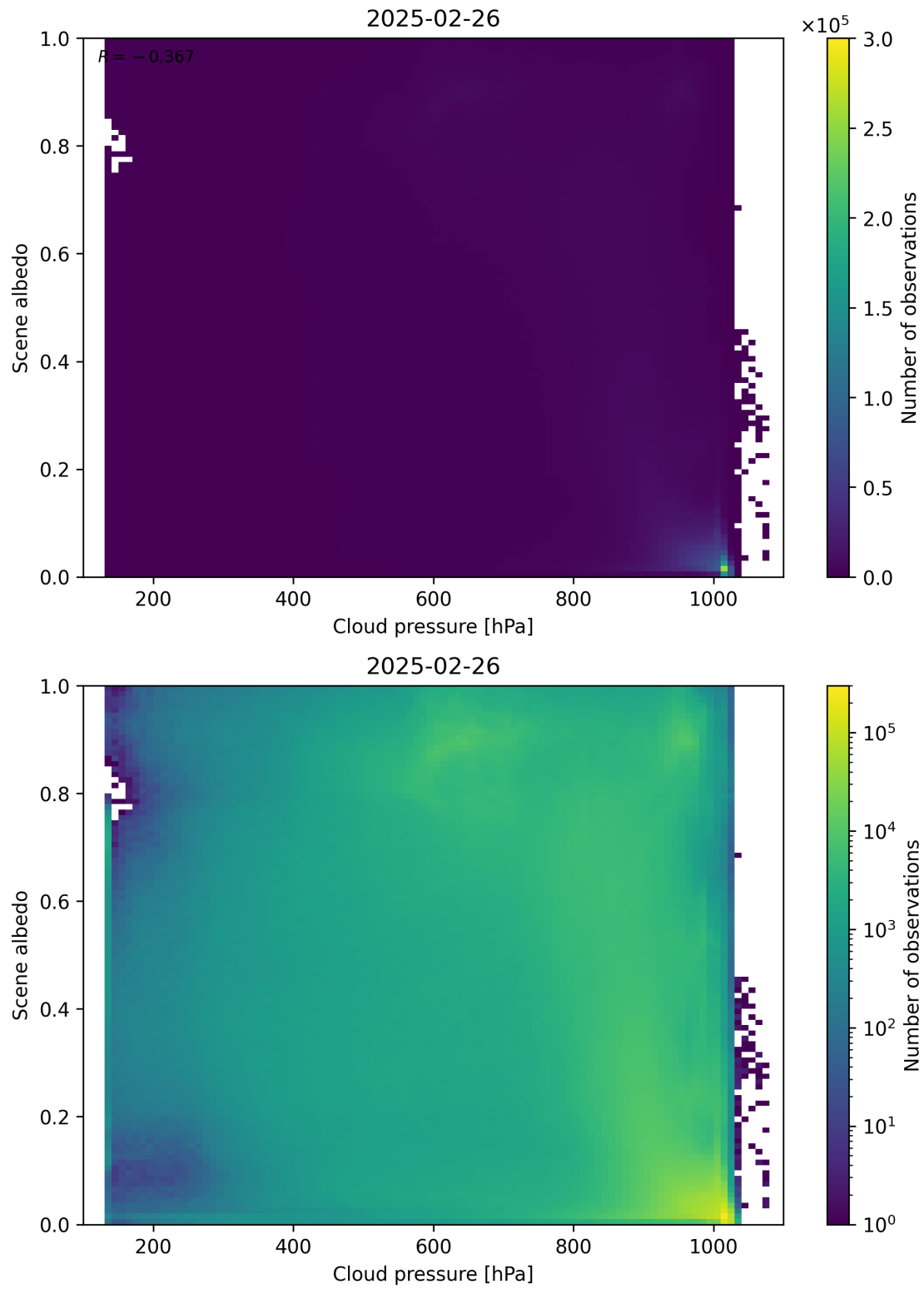
Figure 83: Scatter density plot of “Cloud pressure” against “Scene albedo” for 2025-02-25 to 2025-02-27.
