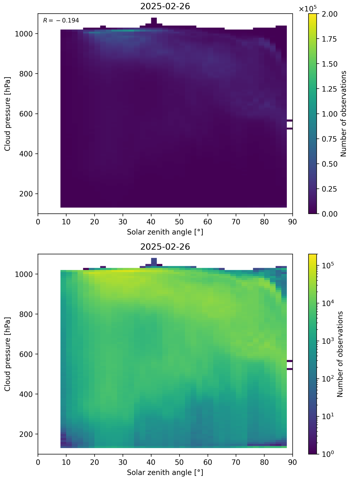
Figure 111: Scatter density plot of “Solar zenith angle” against “Cloud pressure” for 2025-02-25 to 2025-02-27.
