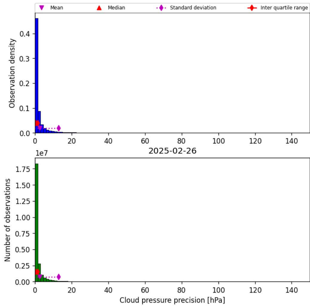
Figure 31: Histogram of “Cloud pressure precision” for 2025-02-25 to 2025-02-27
