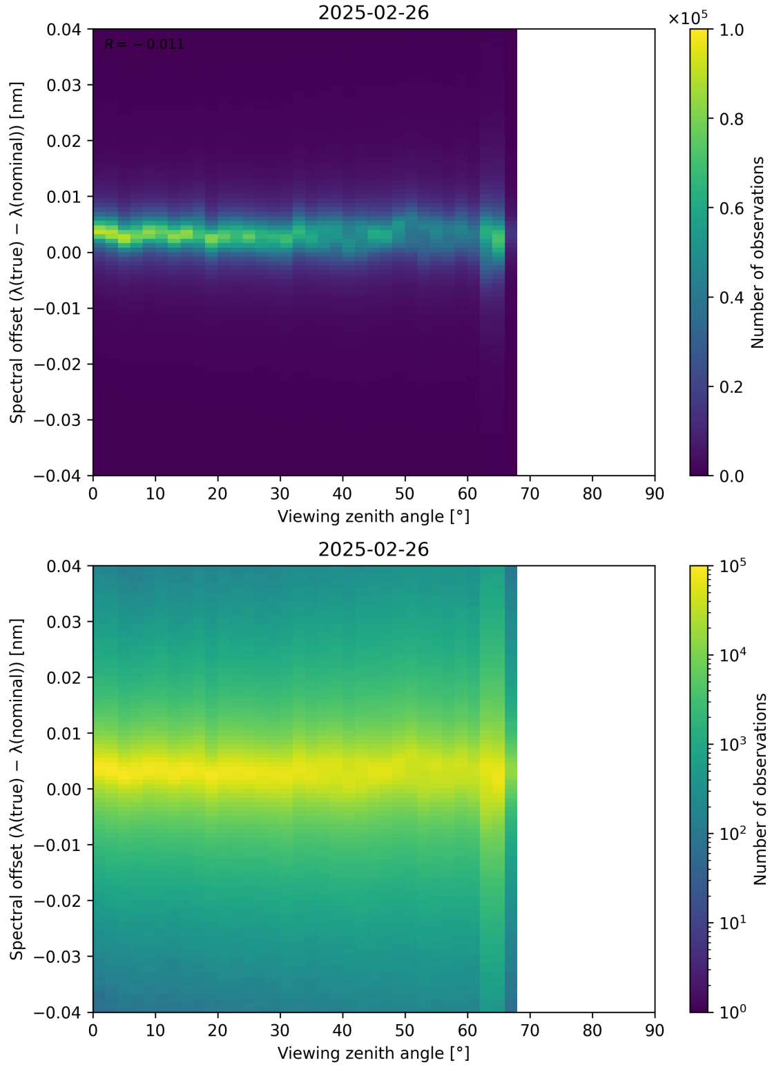
Figure 128: Scatter density plot of “Viewing zenith angle” against “Spectral offset ( \lambda_{\text{true}} - \lambda_{\text{nominal}} )” for 2025-02-25 to 2025-02-27.
