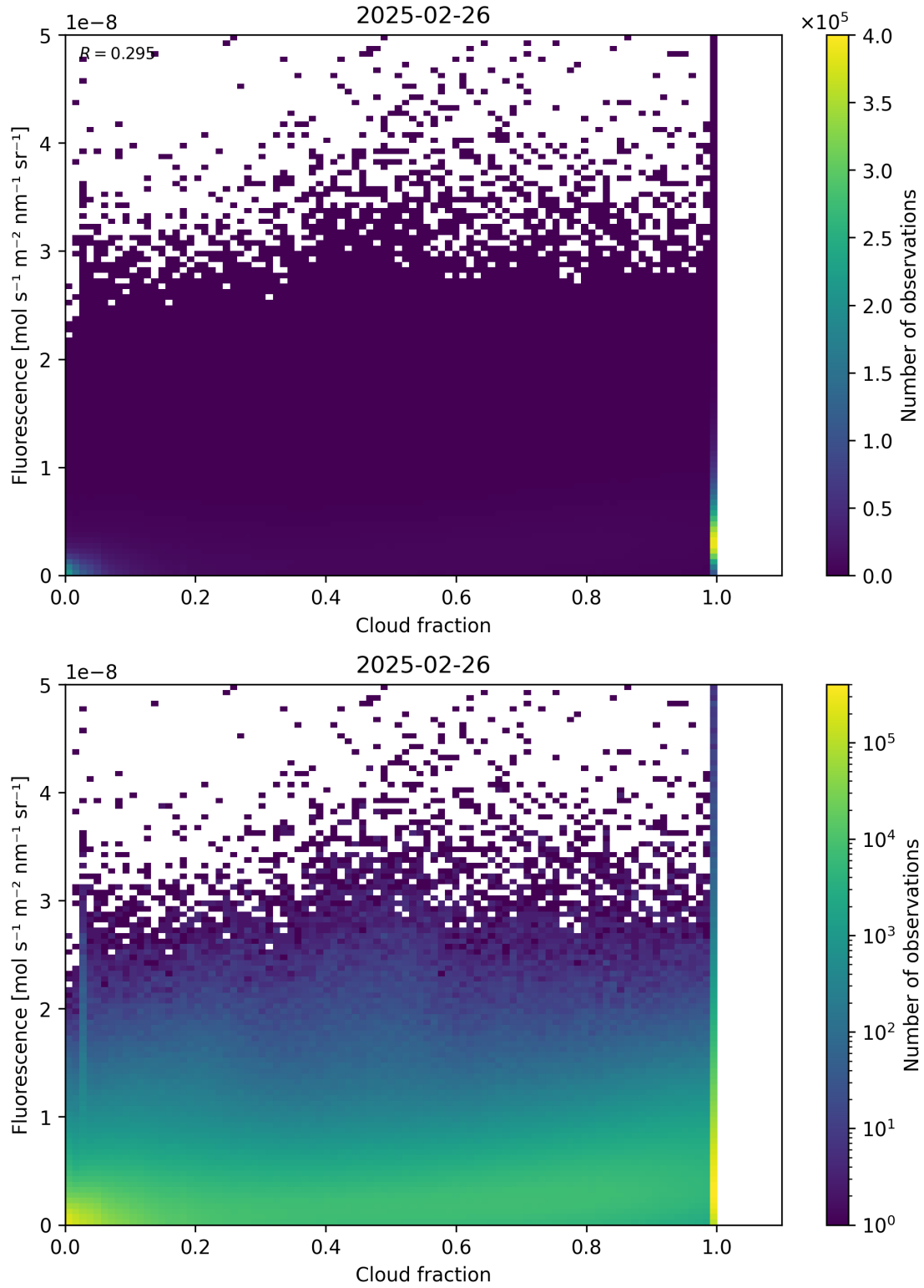
Figure 72: Scatter density plot of “Cloud fraction” against “Fluorescence” for 2025-02-25 to 2025-02-27.
