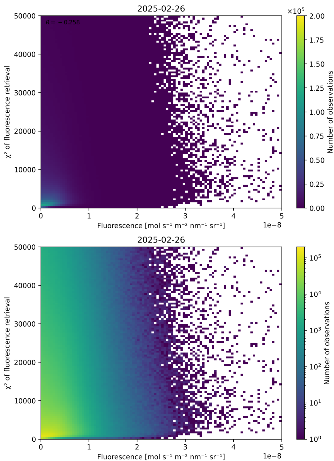
Figure 85: Scatter density plot of “Fluorescence” against “ \chi^2 of fluorescence retrieval” for 2025-02-25 to 2025-02-27.
