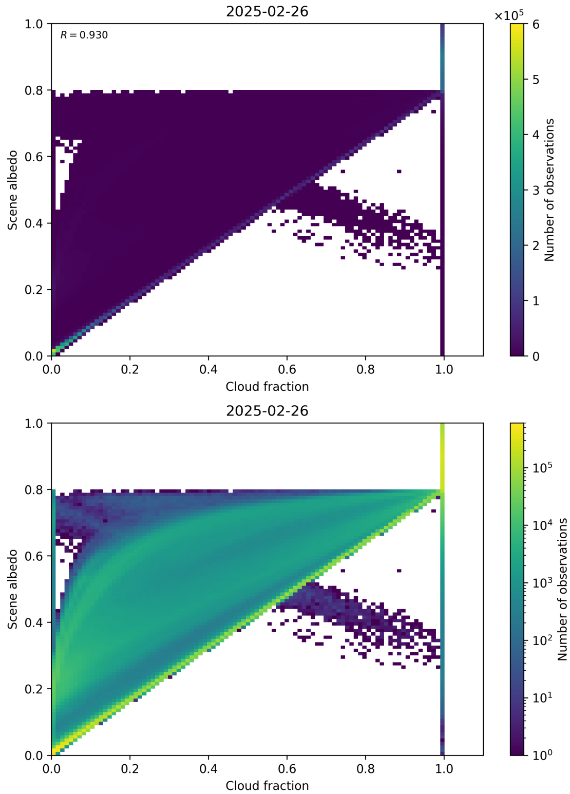
Figure 75: Scatter density plot of “Cloud fraction” against “Scene albedo” for 2025-02-25 to 2025-02-27.
