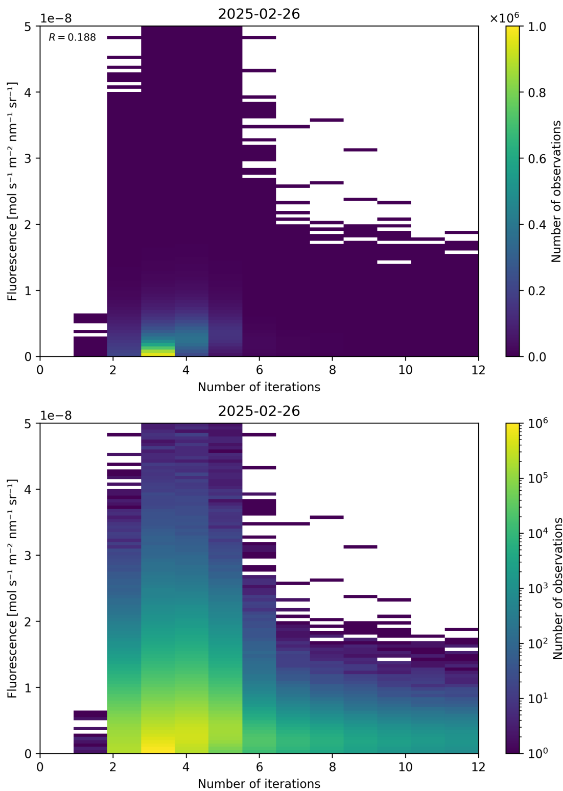
Figure 98: Scatter density plot of “Number of iterations” against “Fluorescence” for 2025-02-25 to 2025-02-27.
