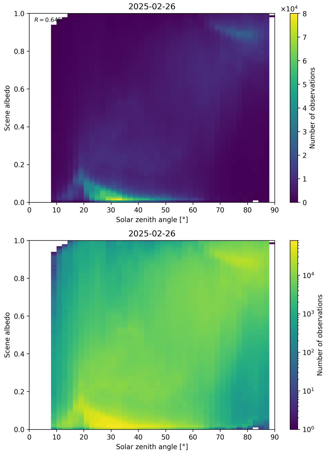
Figure 116: Scatter density plot of “Solar zenith angle” against “Scene albedo” for 2025-02-25 to 2025-02-27.
