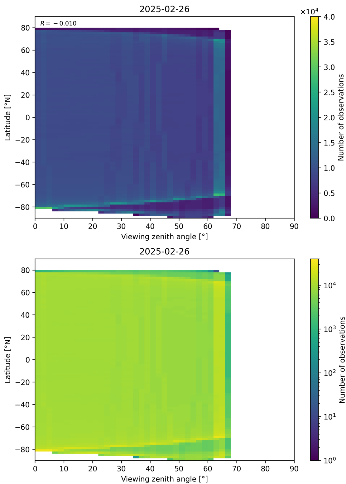
Figure 123: Scatter density plot of “Viewing zenith angle” against “Latitude” for 2025-02-25 to 2025-02-27.
