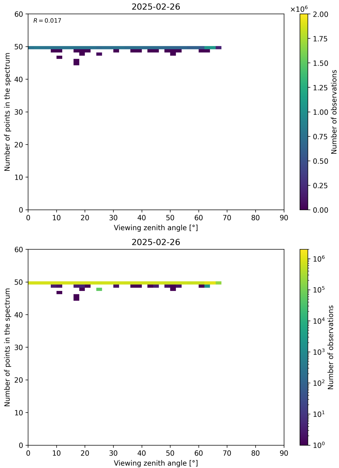
Figure 125: Scatter density plot of “Viewing zenith angle” against “Number of points in the spectrum” for 2025-02-25 to 2025-02-27.
