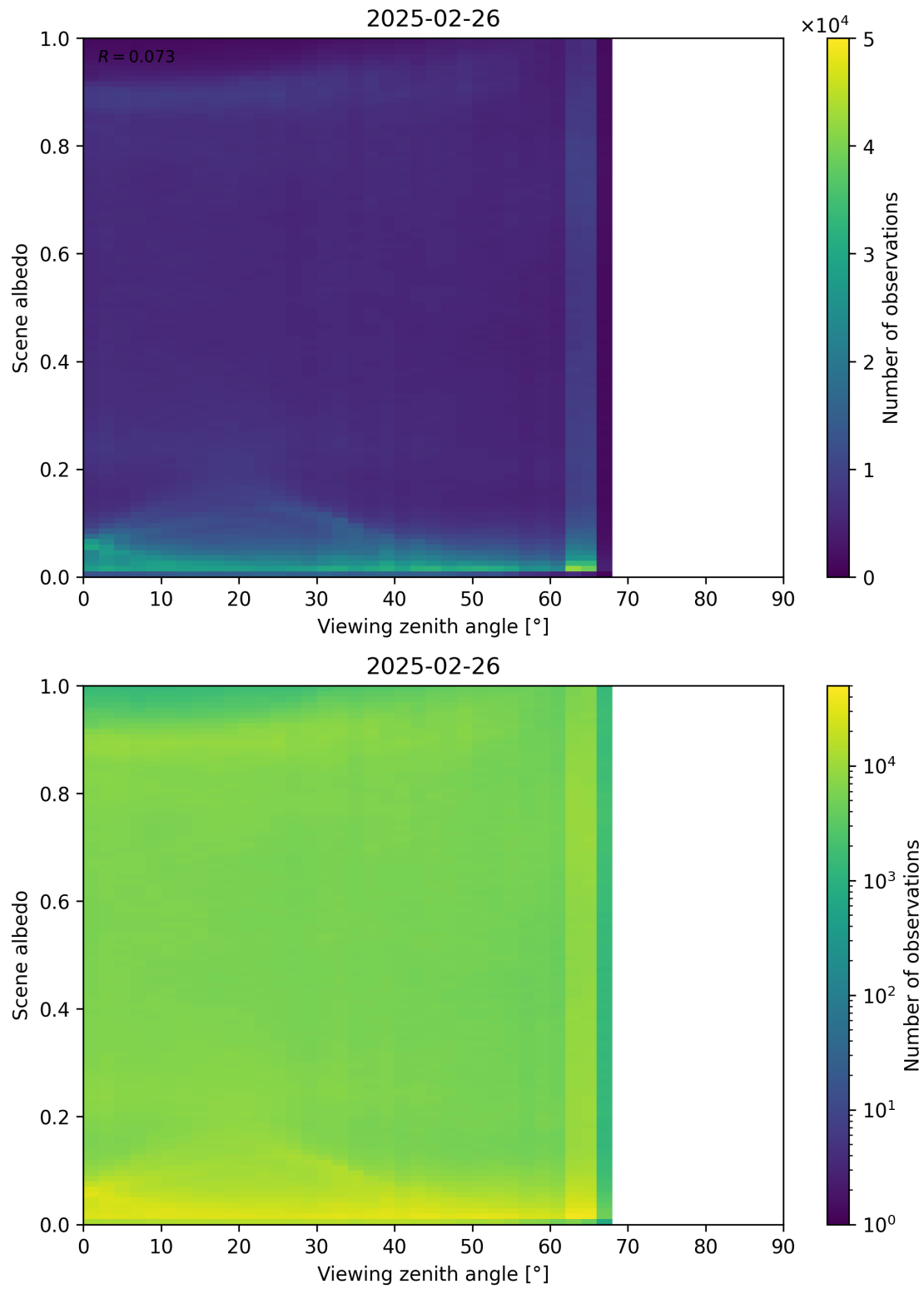
Figure 126: Scatter density plot of “Viewing zenith angle” against “Scene albedo” for 2025-02-25 to 2025-02-27.
