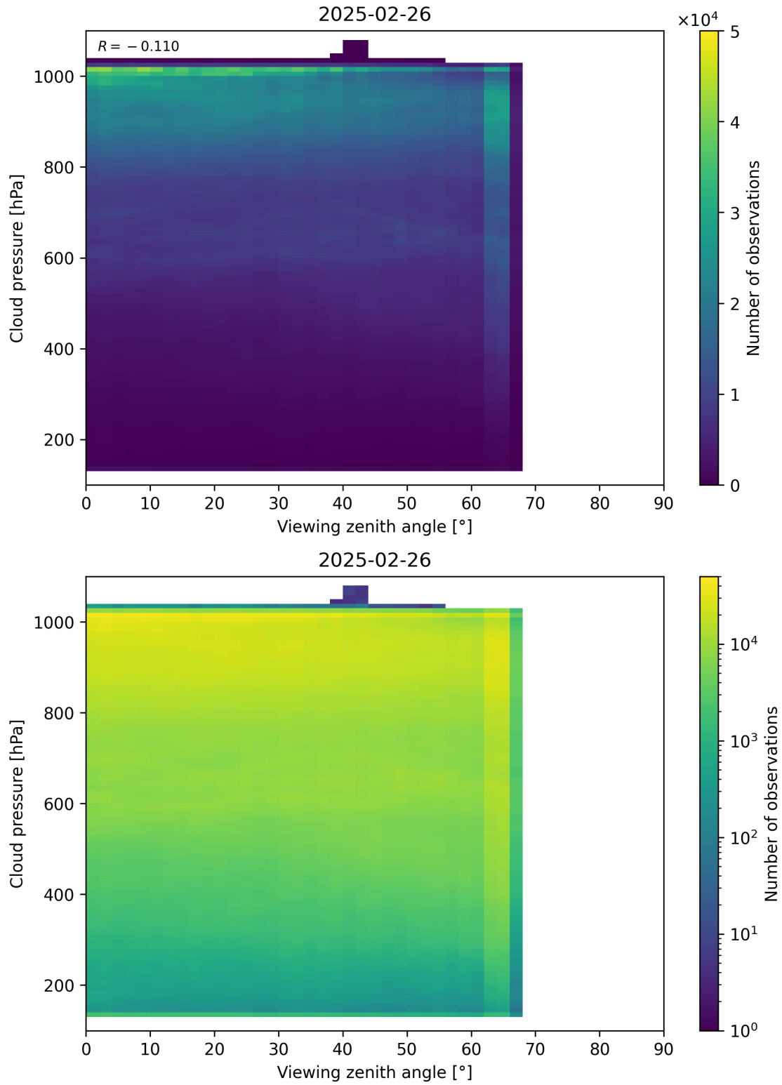
Figure 121: Scatter density plot of “Viewing zenith angle” against “Cloud pressure” for 2025-02-25 to 2025-02-27.
