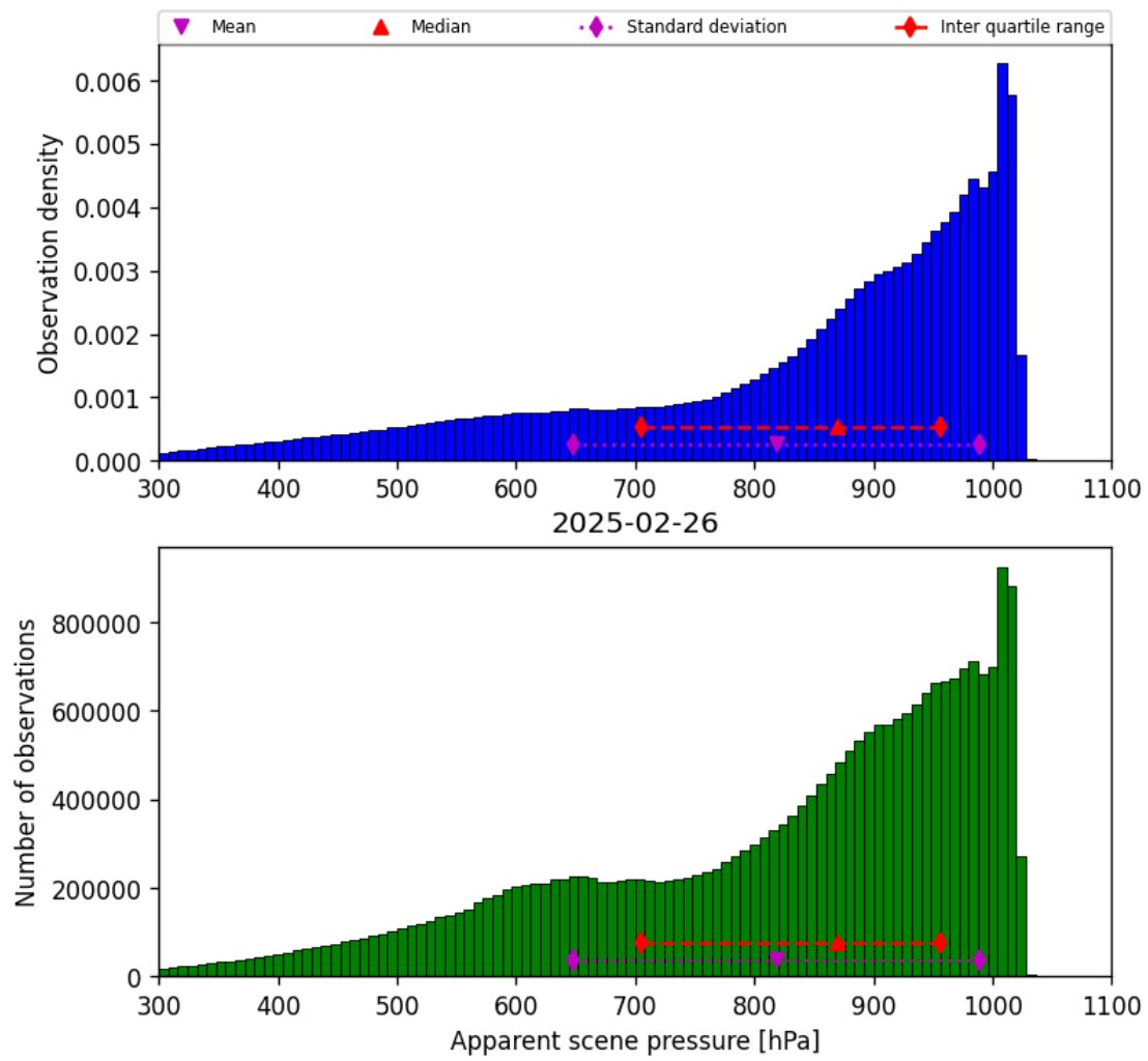
Figure 36: Histogram of “Apparent scene pressure” for 2025-02-25 to 2025-02-27
