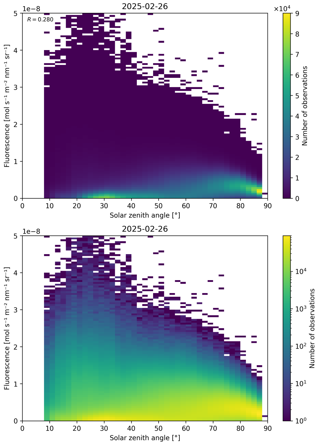
Figure 112: Scatter density plot of “Solar zenith angle” against “Fluorescence” for 2025-02-25 to 2025-02-27.
