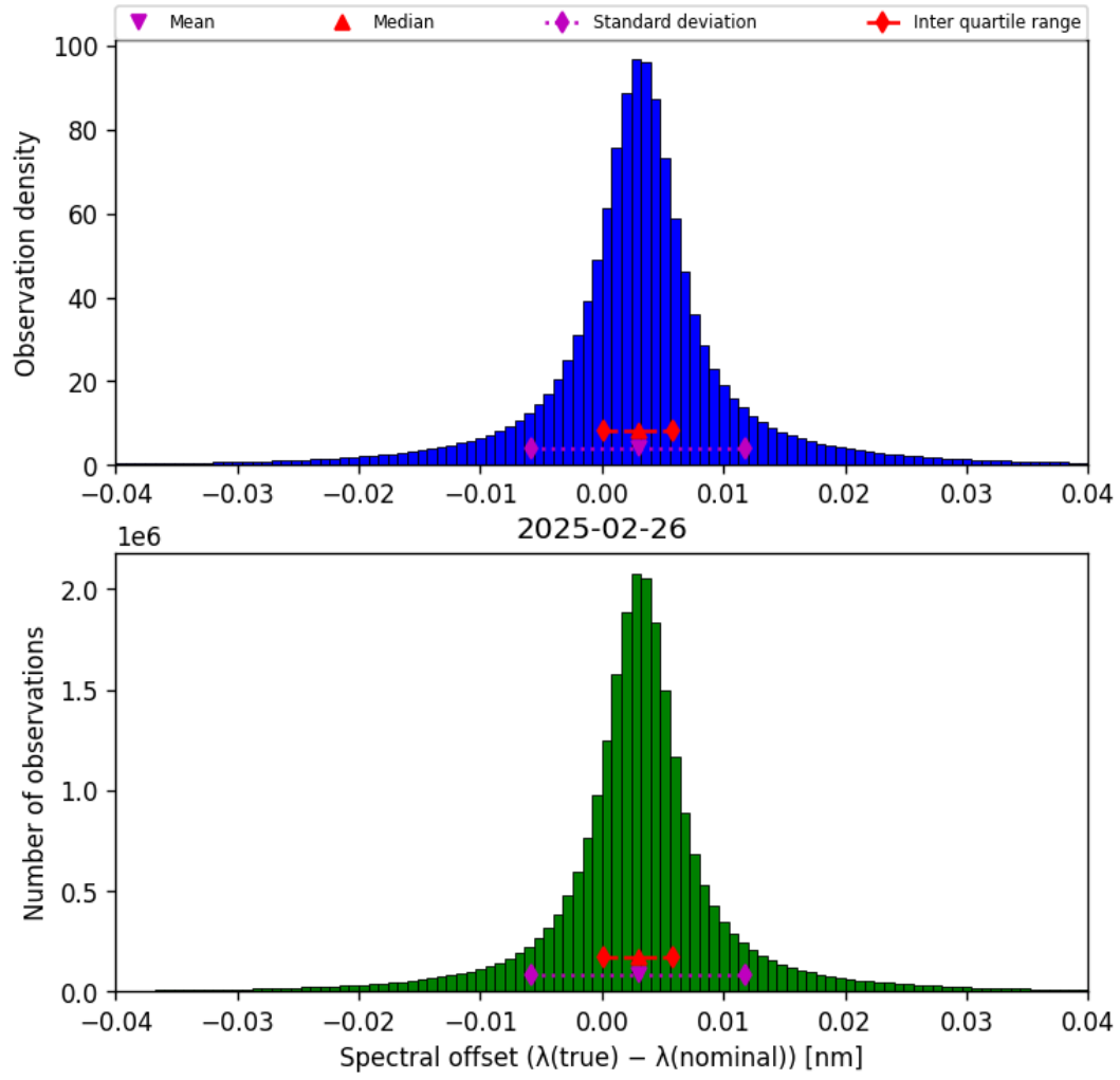
Figure 45: Histogram of “Spectral offset ( \lambda_{\text{true}} - \lambda_{\text{nominal}} )” for 2025-02-25 to 2025-02-27
