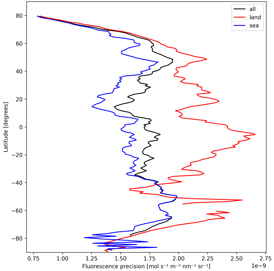
Figure 24: Zonal average of “Fluorescence precision” for 2025-02-25 to 2025-02-27.
