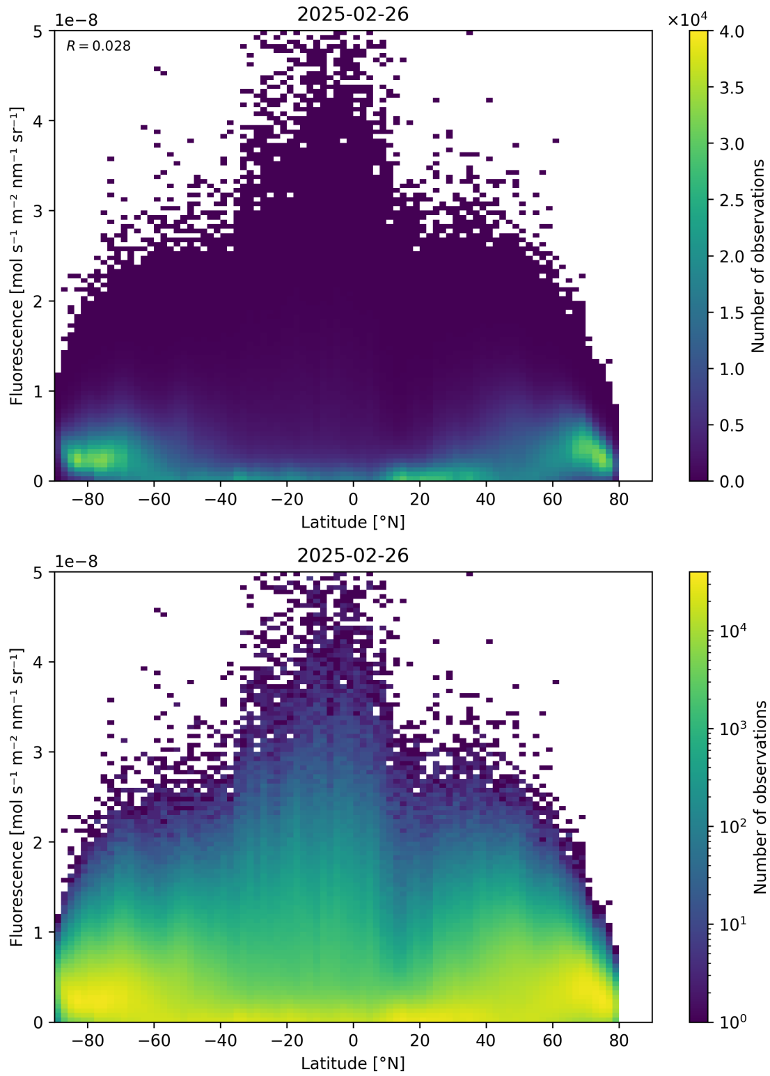
Figure 92: Scatter density plot of “Latitude” against “Fluorescence” for 2025-02-25 to 2025-02-27.
