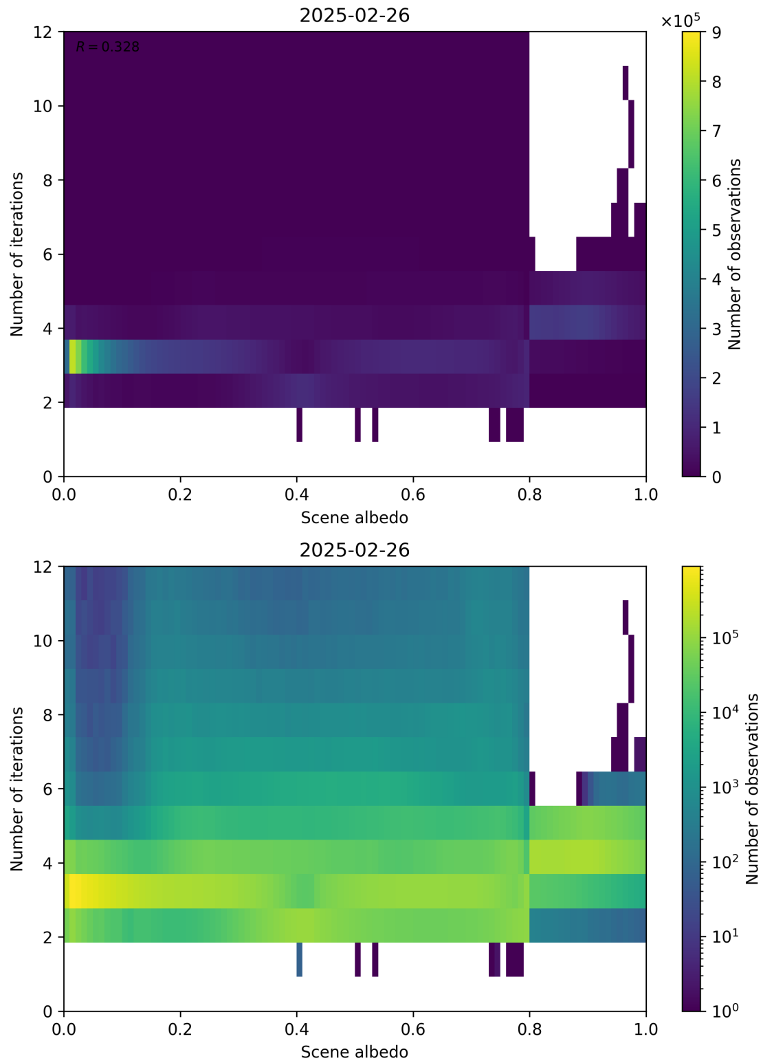
Figure 105: Scatter density plot of “Scene albedo” against “Number of iterations” for 2025-02-25 to 2025-02-27.
