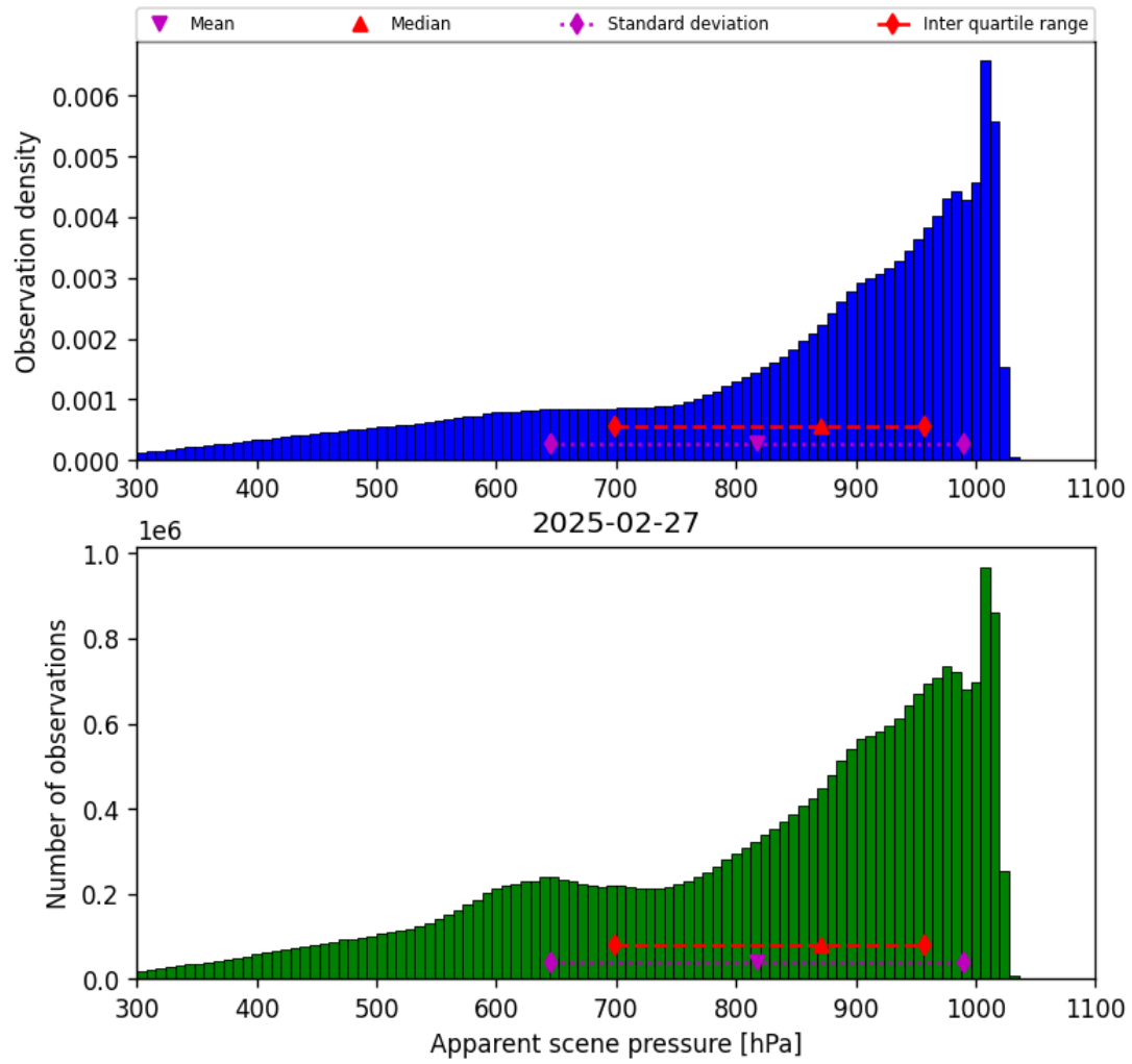
Figure 36: Histogram of “Apparent scene pressure” for 2025-02-26 to 2025-02-28
