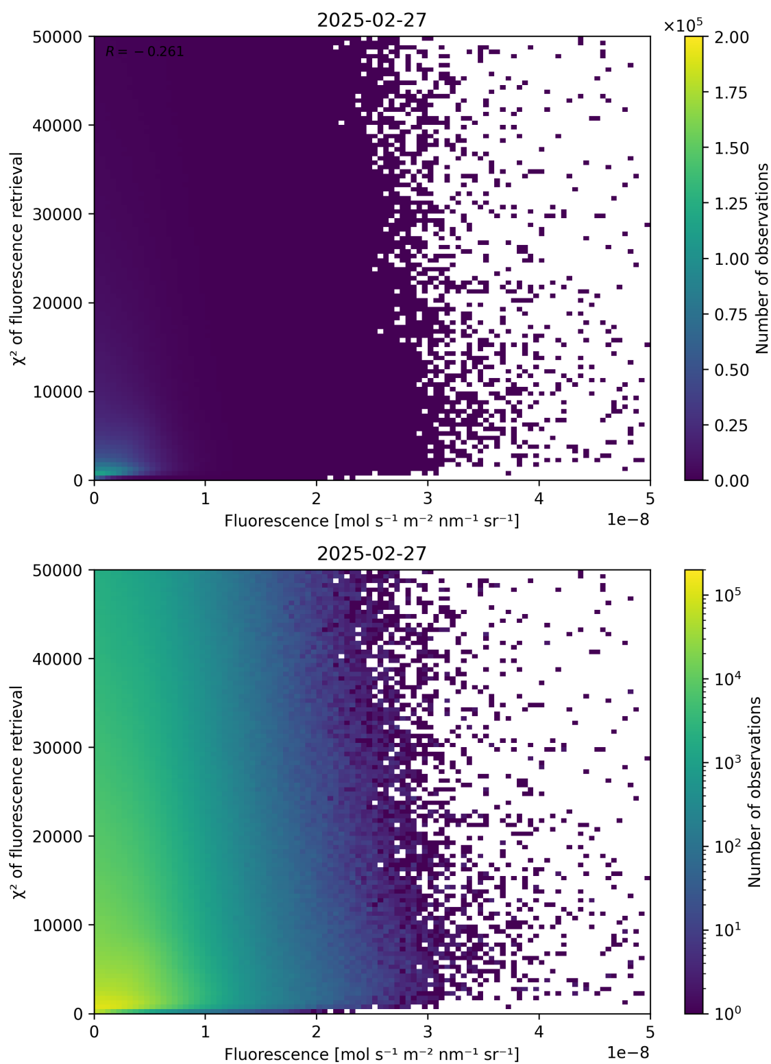
Figure 85: Scatter density plot of “Fluorescence” against “ \chi^2 of fluorescence retrieval” for 2025-02-26 to 2025-02-28.
