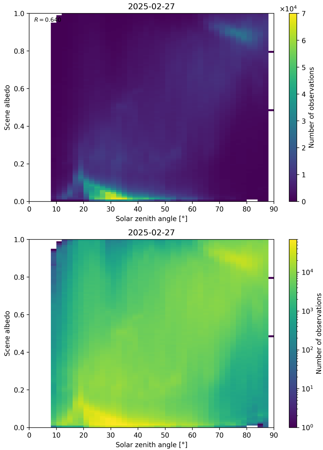
Figure 116: Scatter density plot of “Solar zenith angle” against “Scene albedo” for 2025-02-26 to 2025-02-28.
