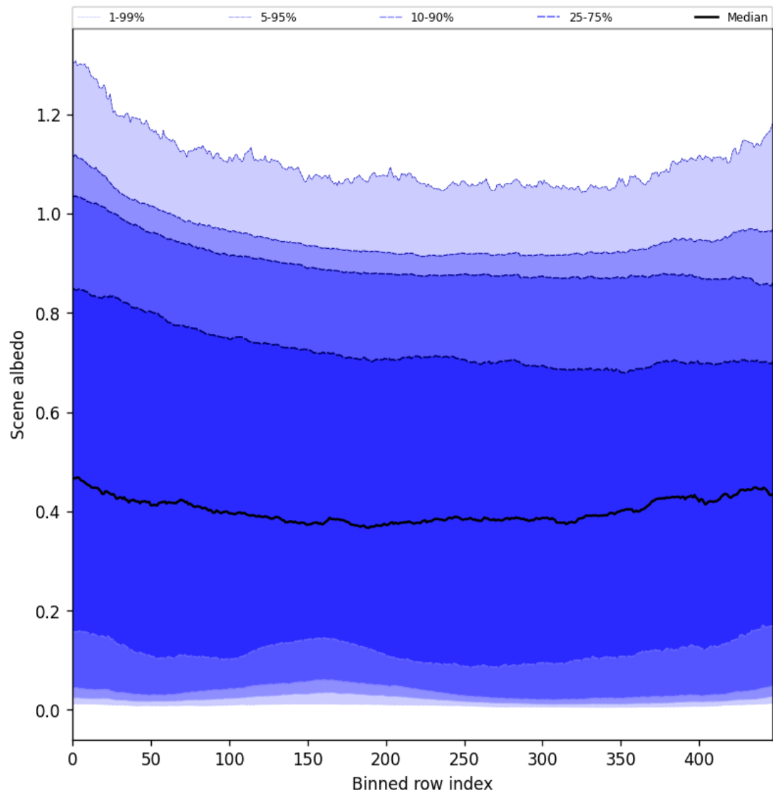
Figure 51: Along track statistics of “Scene albedo” for 2025-02-26 to 2025-02-28
