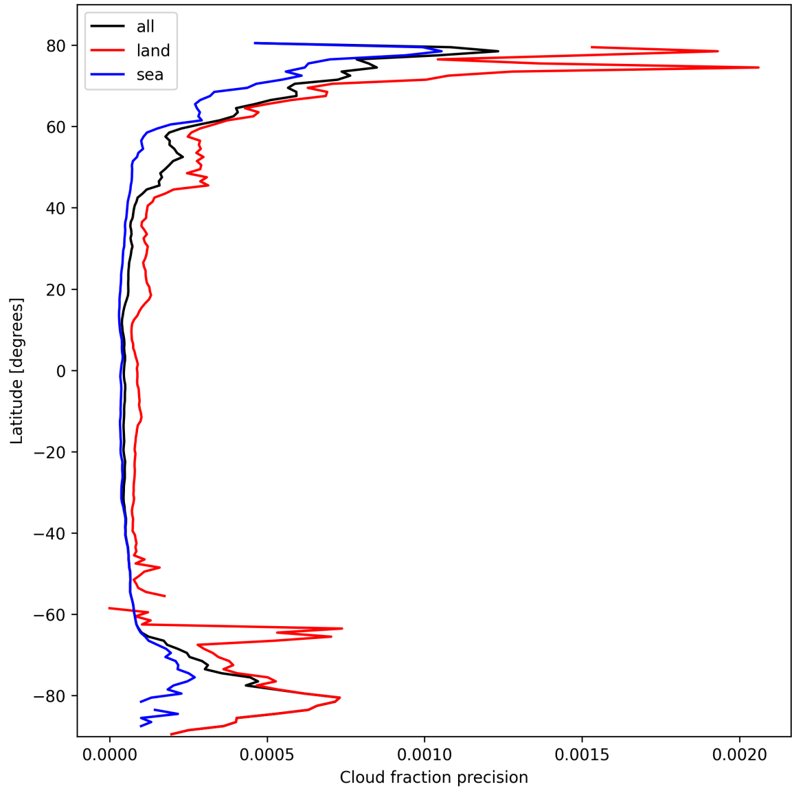
Figure 16: Zonal average of “Cloud fraction precision” for 2025-02-26 to 2025-02-28.
