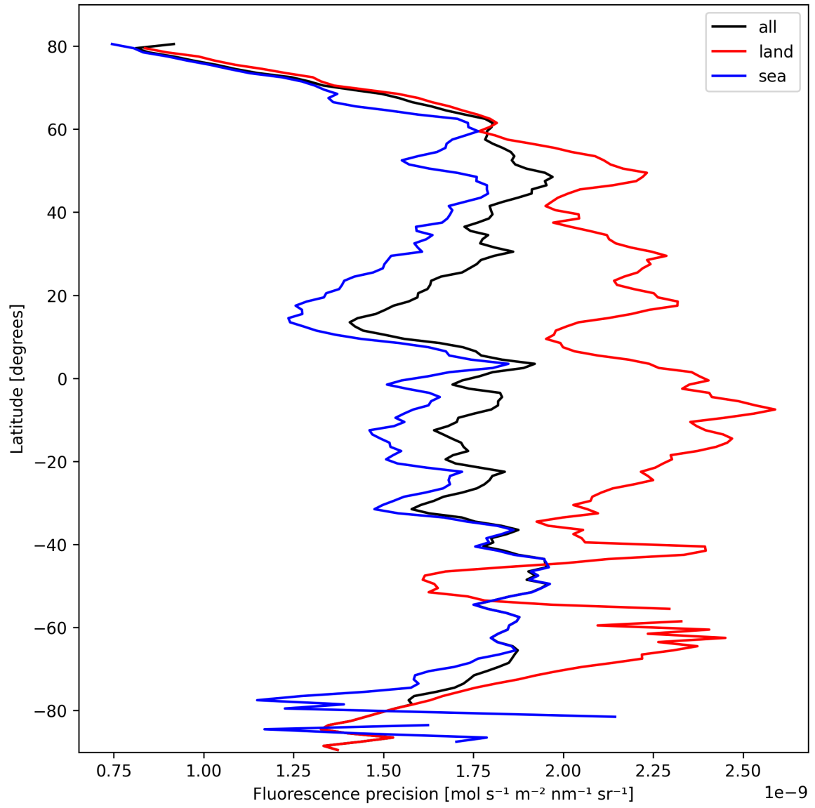
Figure 24: Zonal average of “Fluorescence precision” for 2025-02-26 to 2025-02-28.
