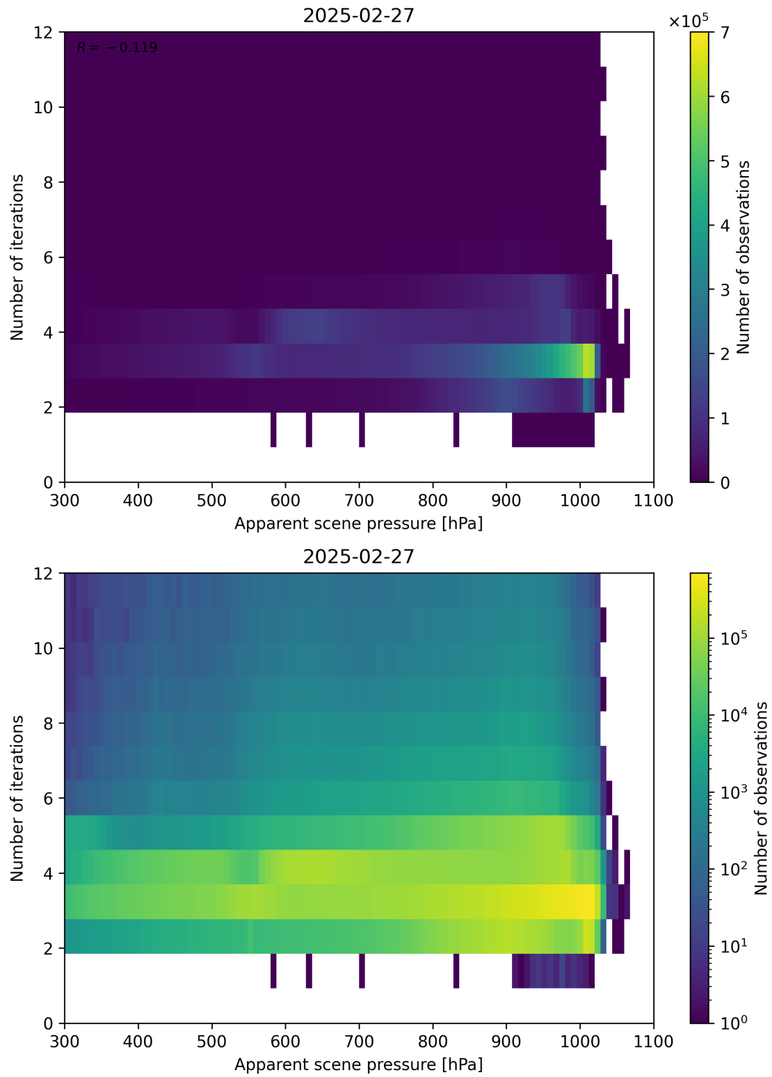
Figure 65: Scatter density plot of “Apparent scene pressure” against “Number of iterations” for 2025-02-26 to 2025-02-28.
