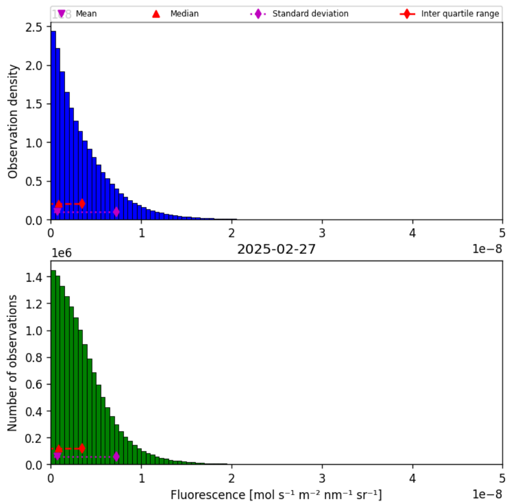
Figure 40: Histogram of “Fluorescence” for 2025-02-26 to 2025-02-28
