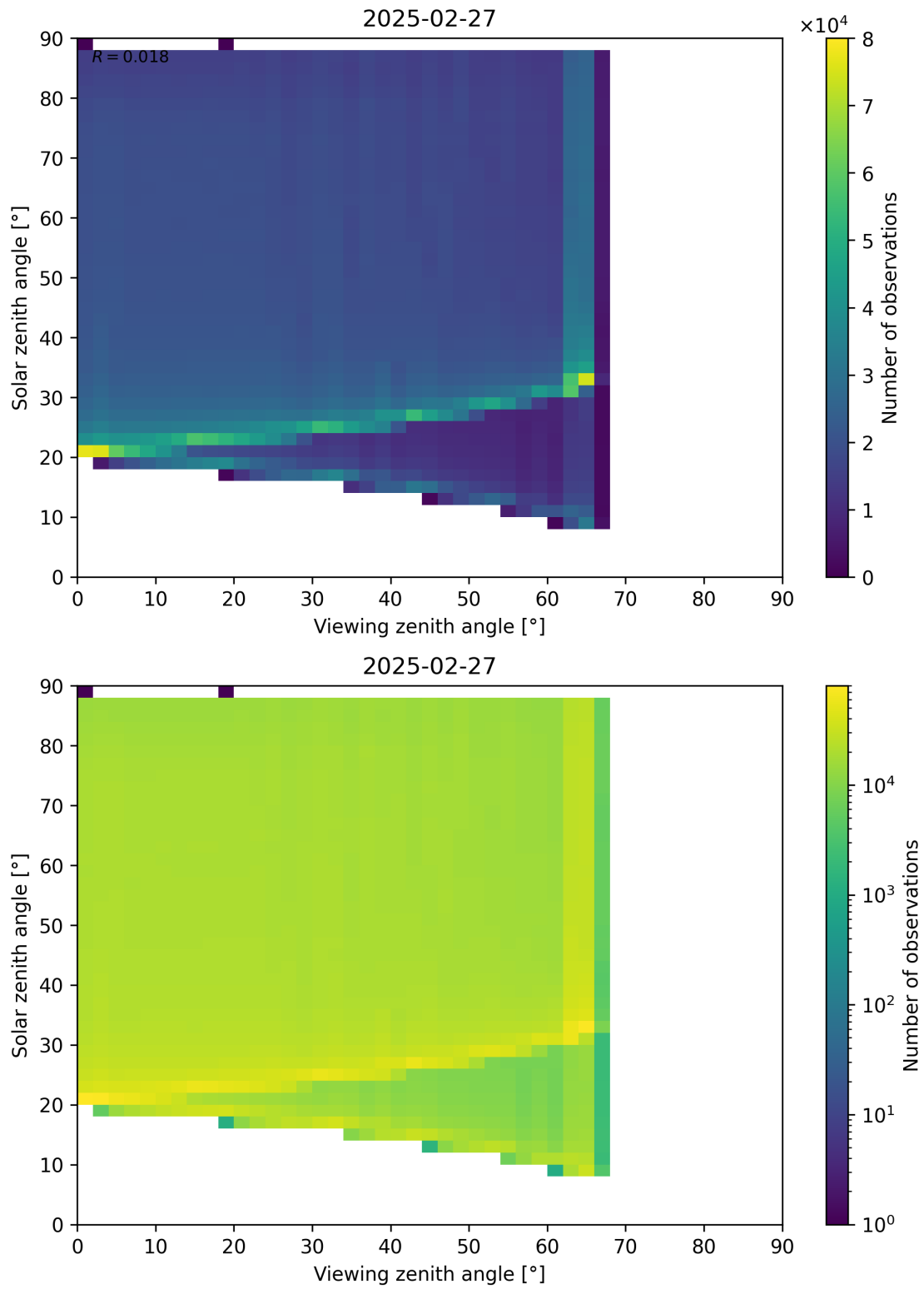
Figure 127: Scatter density plot of “Viewing zenith angle” against “Solar zenith angle” for 2025-02-26 to 2025-02-28.
