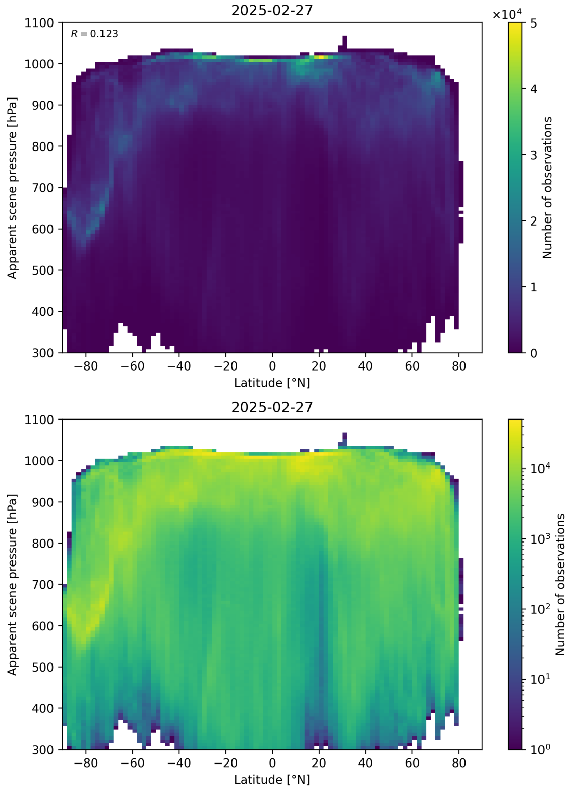
Figure 88: Scatter density plot of “Latitude” against “Apparent scene pressure” for 2025-02-26 to 2025-02-28.
