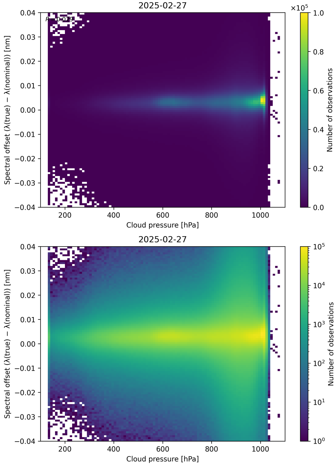
Figure 84: Scatter density plot of “Cloud pressure” against “Spectral offset ( \lambda_{\text{true}} - \lambda_{\text{nominal}} )” for 2025-02-26 to 2025-02-28.
