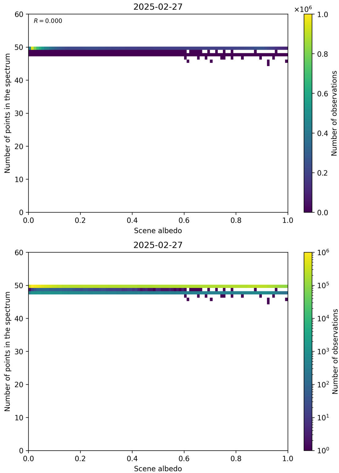
Figure 106: Scatter density plot of “Scene albedo” against “Number of points in the spectrum” for 2025-02-26 to 2025-02-28.
