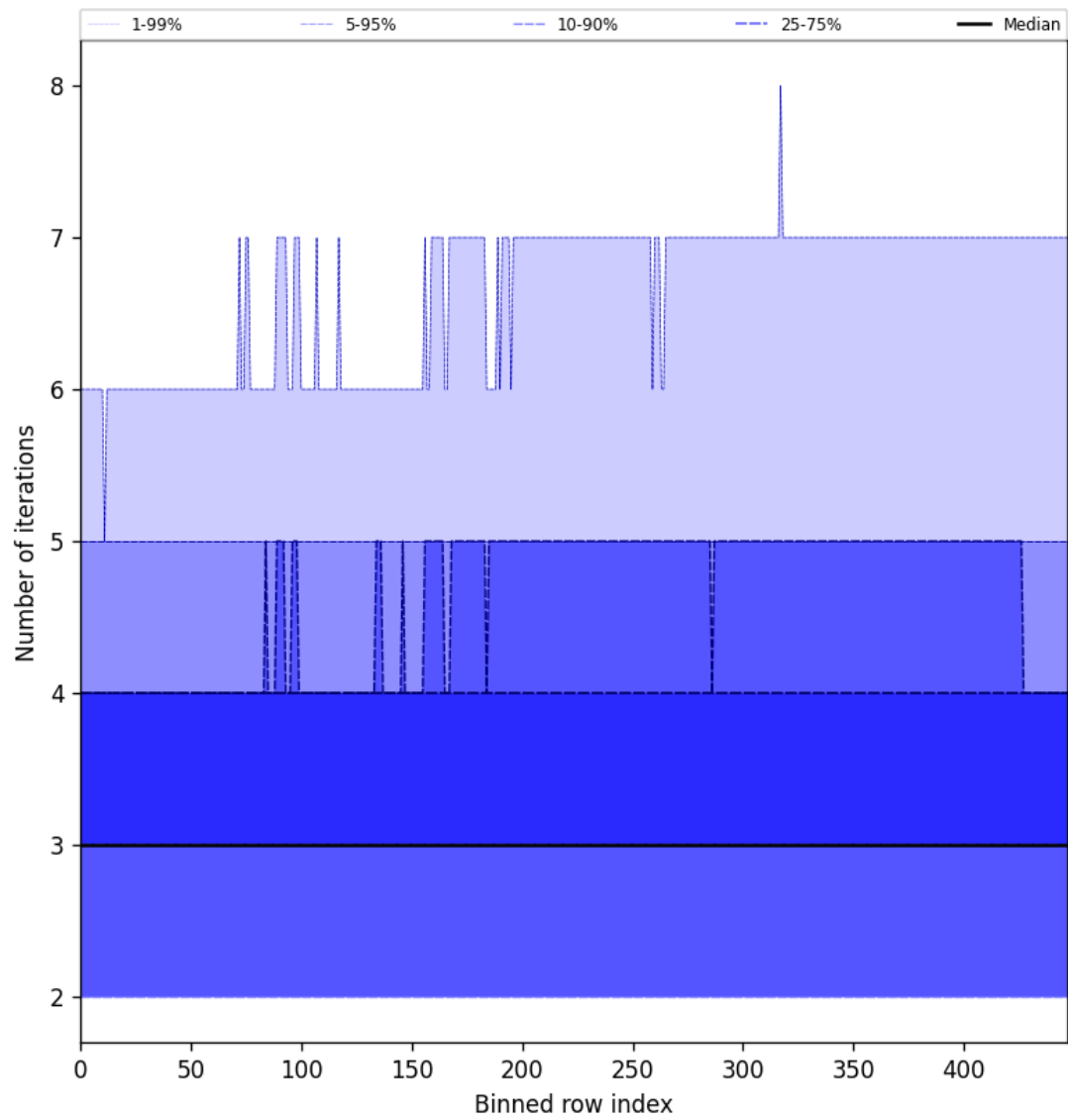
Figure 56: Along track statistics of “Number of iterations” for 2025-02-26 to 2025-02-28
