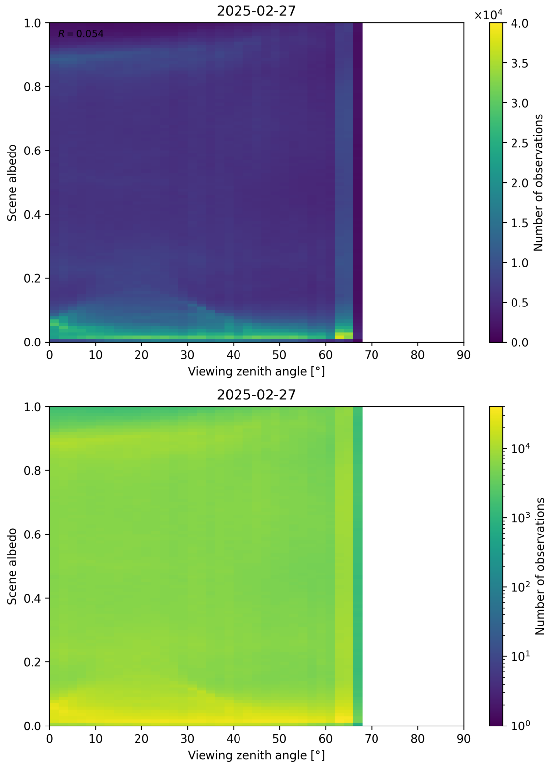
Figure 126: Scatter density plot of “Viewing zenith angle” against “Scene albedo” for 2025-02-26 to 2025-02-28.
