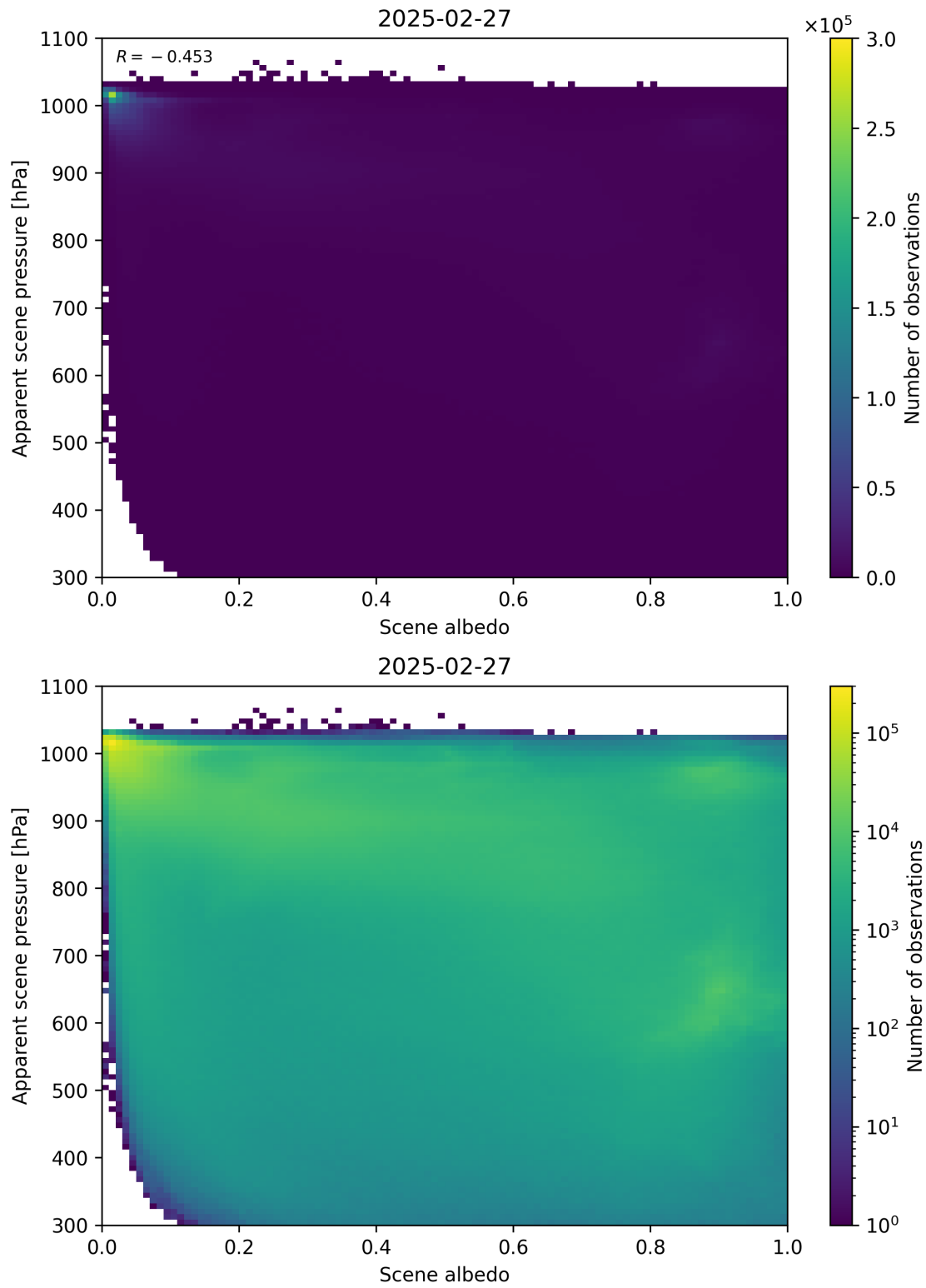
Figure 102: Scatter density plot of “Scene albedo” against “Apparent scene pressure” for 2025-02-26 to 2025-02-28.
