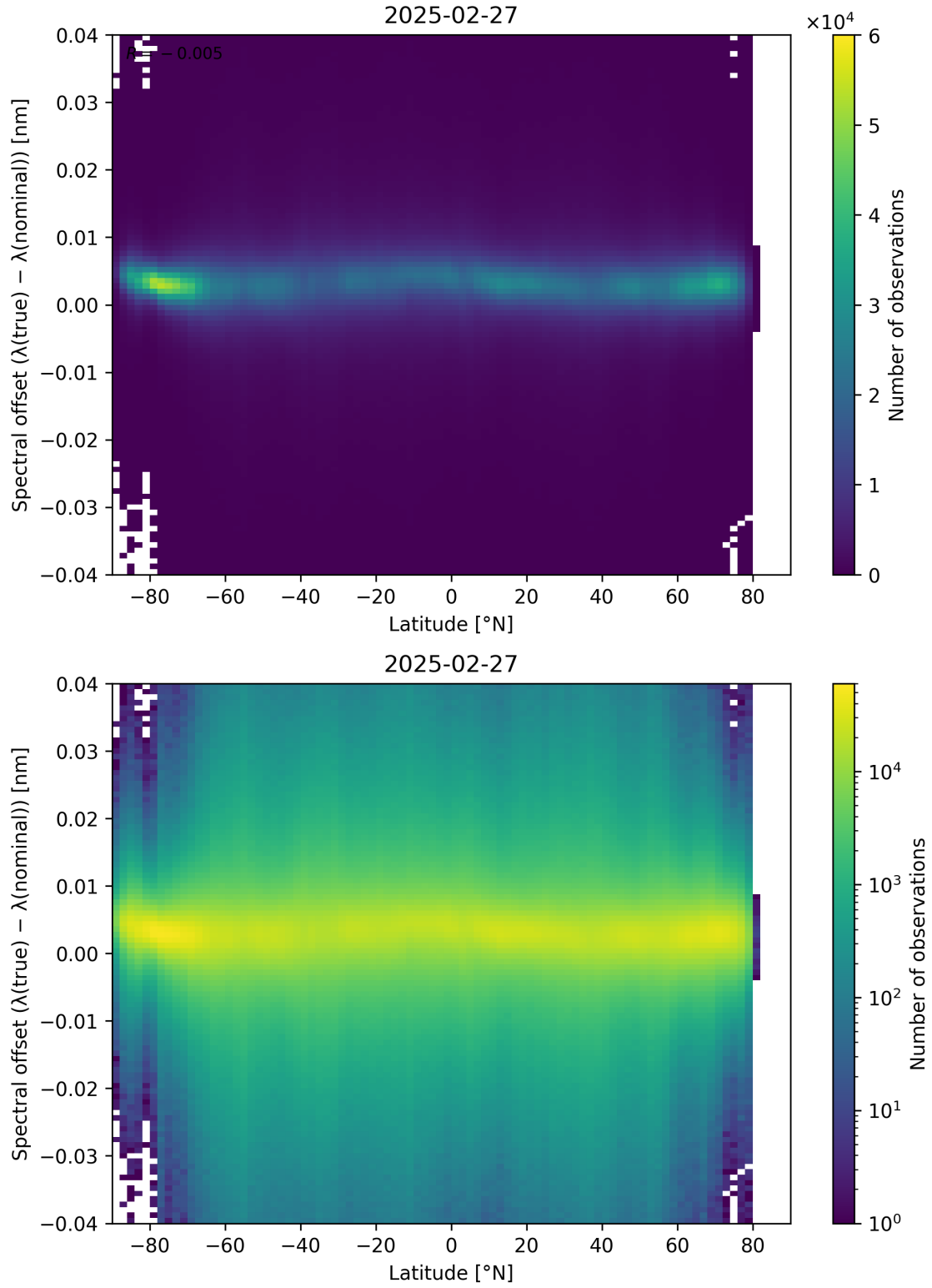
Figure 96: Scatter density plot of “Latitude” against “Spectral offset ( \lambda_{\text{true}} - \lambda_{\text{nominal}} )” for 2025-02-26 to 2025-02-28.
