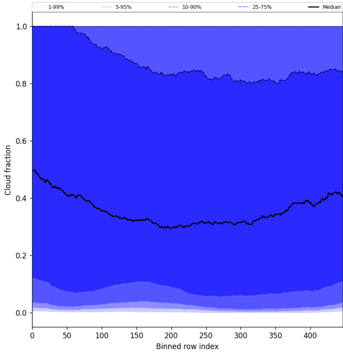
Figure 49: Along track statistics of “Cloud fraction” for 2025-02-26 to 2025-02-28
