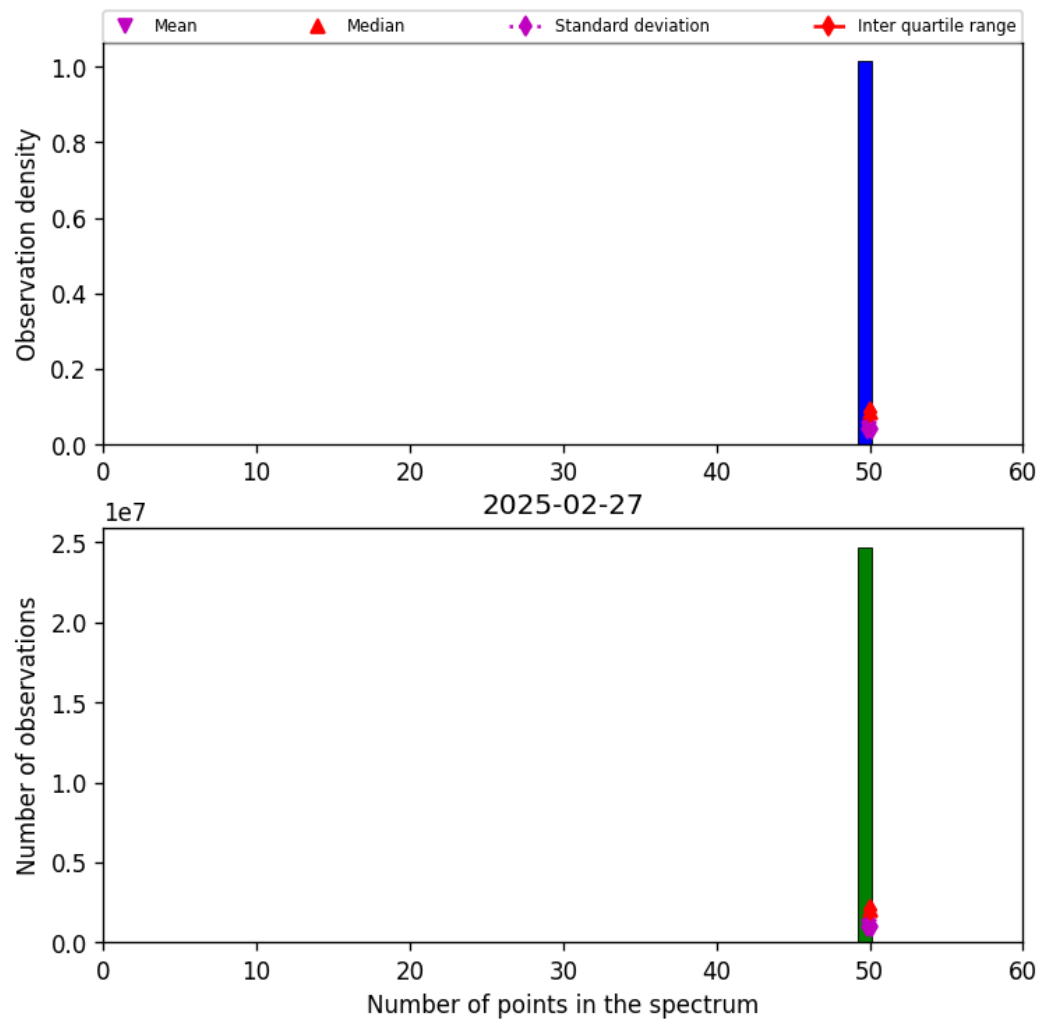
Figure 44: Histogram of “Number of points in the spectrum” for 2025-02-26 to 2025-02-28
