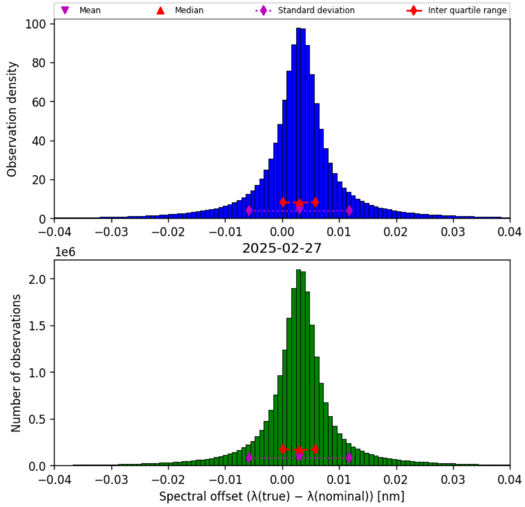
Figure 45: Histogram of “Spectral offset ( \lambda_{\text{true}} - \lambda_{\text{nominal}} )” for 2025-02-26 to 2025-02-28
