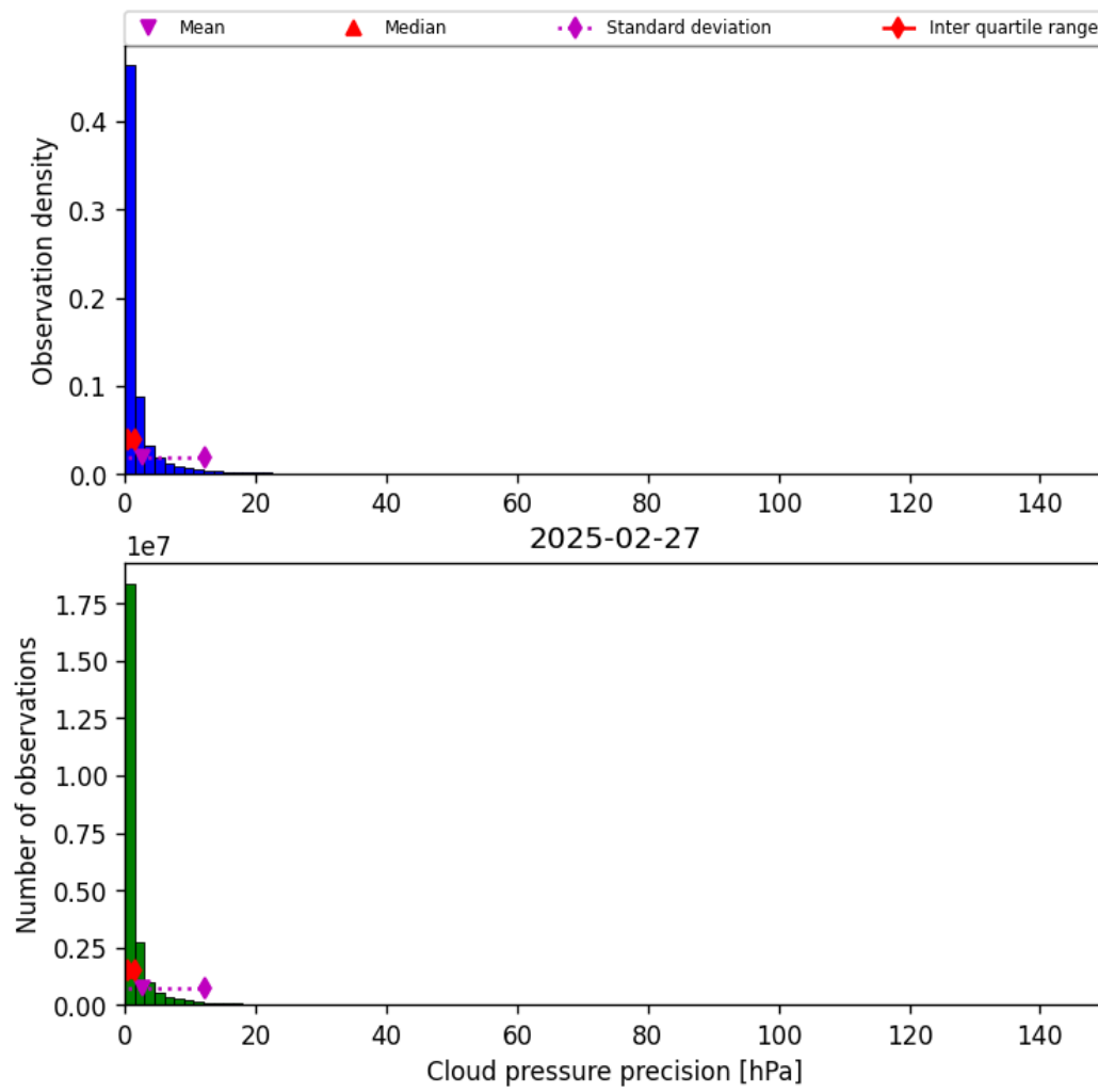
Figure 31: Histogram of “Cloud pressure precision” for 2025-02-26 to 2025-02-28
