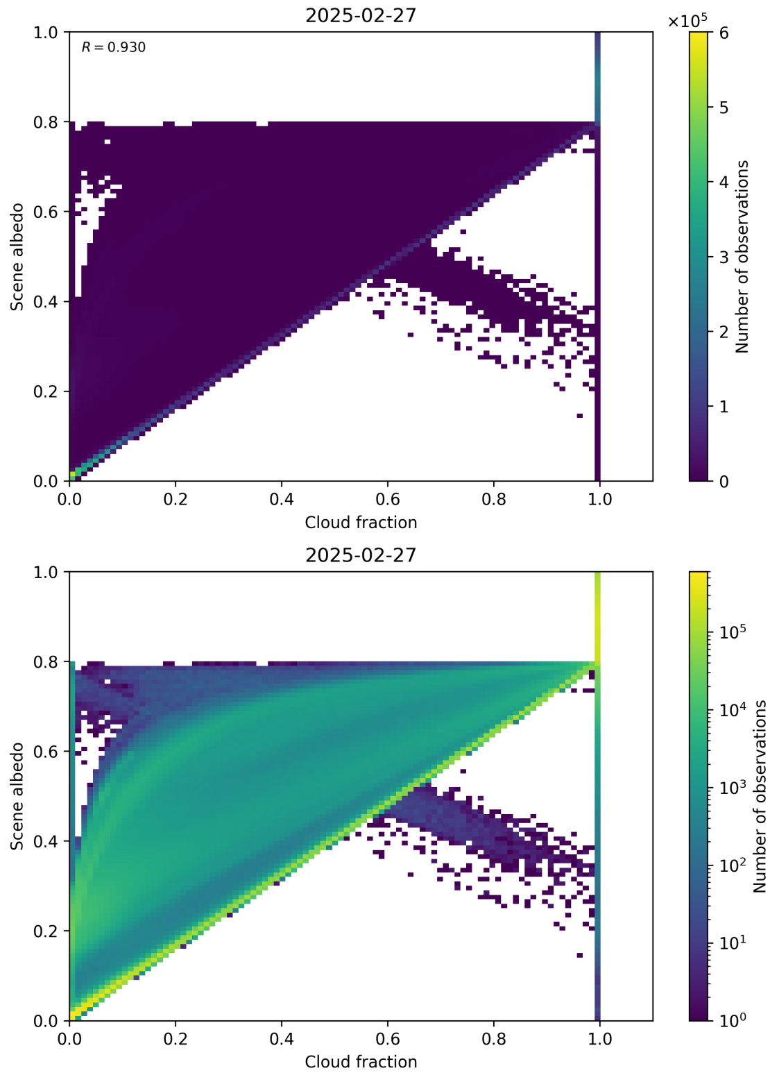
Figure 75: Scatter density plot of “Cloud fraction” against “Scene albedo” for 2025-02-26 to 2025-02-28.
