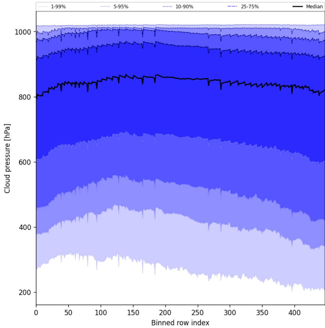
Figure 47: Along track statistics of “Cloud pressure” for 2025-02-26 to 2025-02-28
