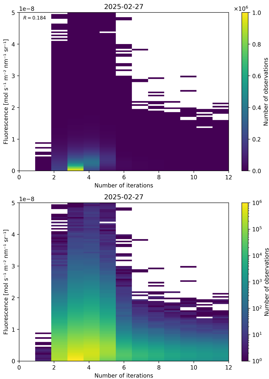
Figure 98: Scatter density plot of “Number of iterations” against “Fluorescence” for 2025-02-26 to 2025-02-28.
