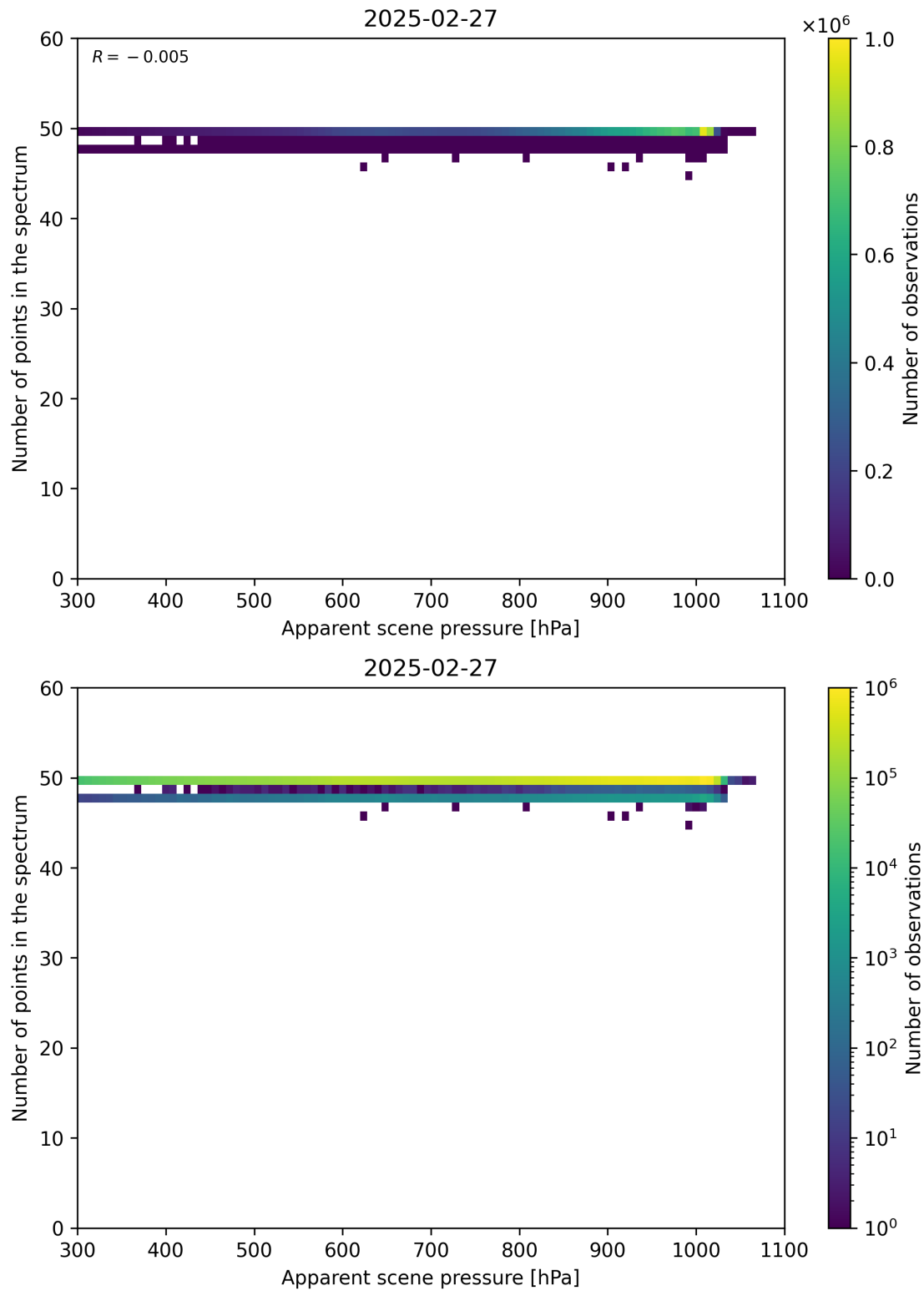
Figure 66: Scatter density plot of “Apparent scene pressure” against “Number of points in the spectrum” for 2025-02-26 to 2025-02-28.
