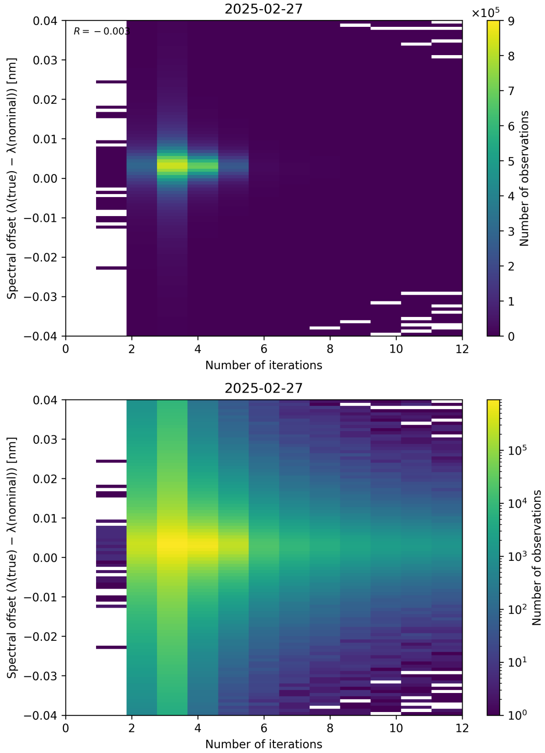
Figure 100: Scatter density plot of “Number of iterations” against “Spectral offset ( \lambda_{\text{true}} - \lambda_{\text{nominal}} )” for 2025-02-26 to 2025-02-28.
