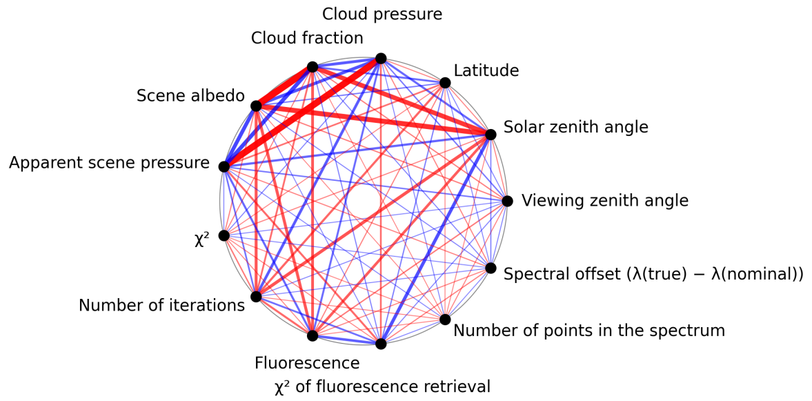
Figure 1: Map of correlation graph for 2025-02-26 to 2025-02-28.
