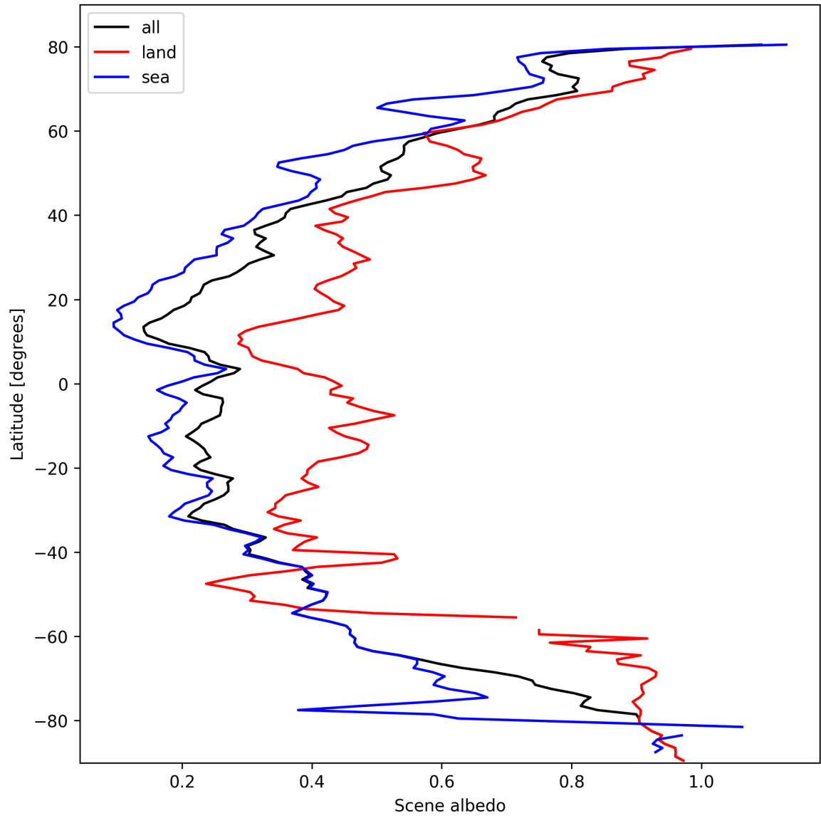
Figure 17: Zonal average of “Scene albedo” for 2025-02-26 to 2025-02-28.
