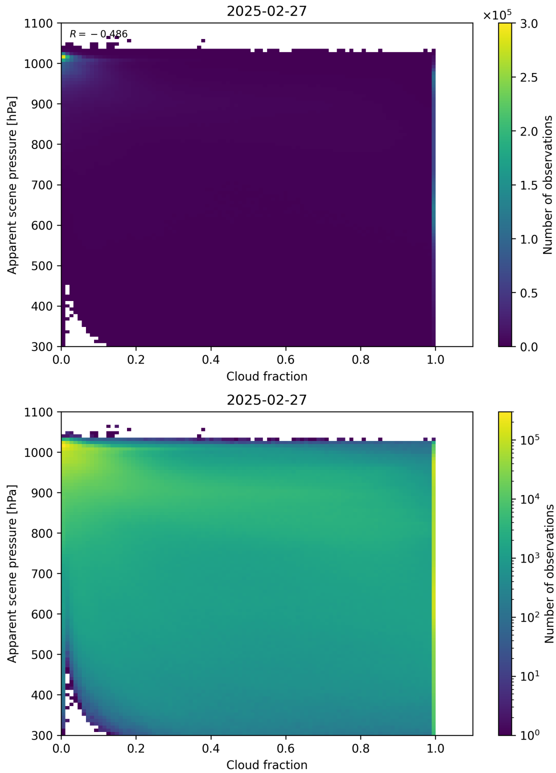
Figure 70: Scatter density plot of “Cloud fraction” against “Apparent scene pressure” for 2025-02-26 to 2025-02-28.
