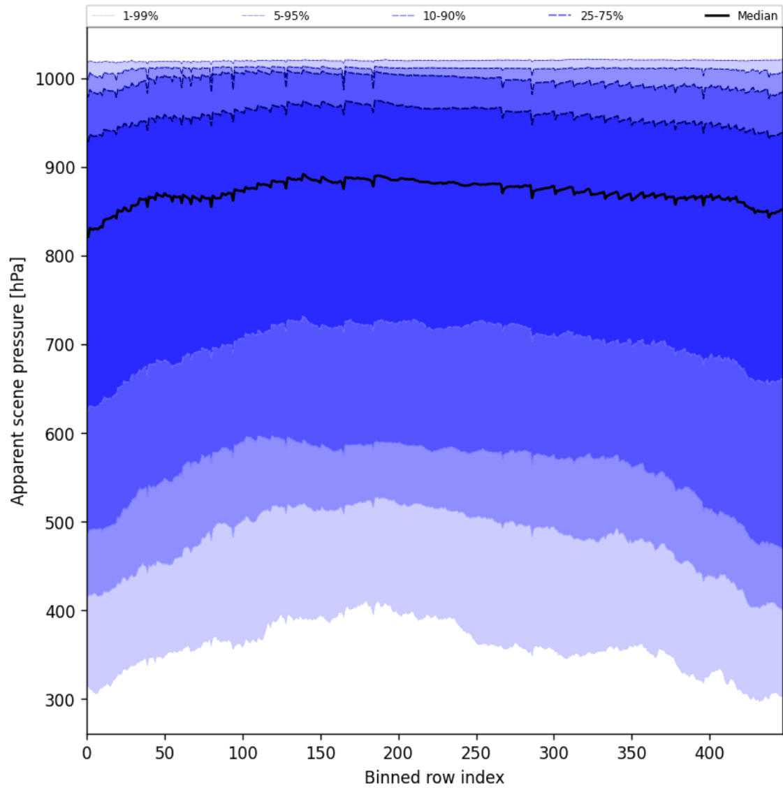
Figure 53: Along track statistics of “Apparent scene pressure” for 2025-02-26 to 2025-02-28
