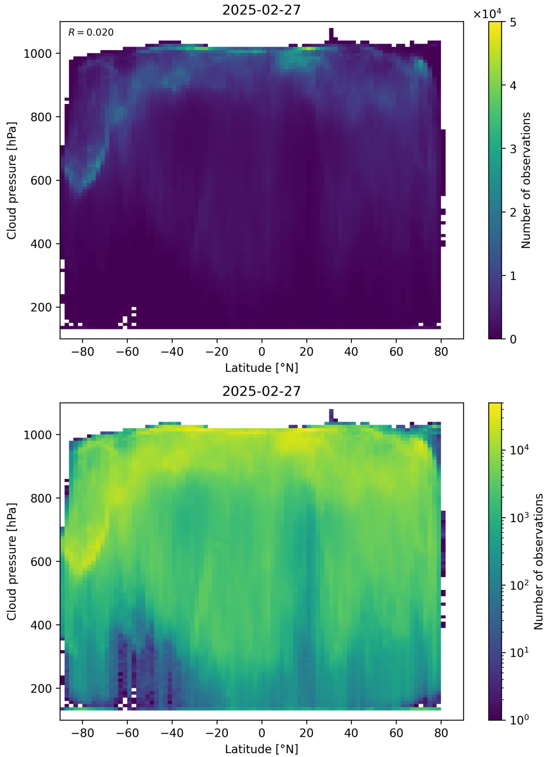
Figure 91: Scatter density plot of “Latitude” against “Cloud pressure” for 2025-02-26 to 2025-02-28.
