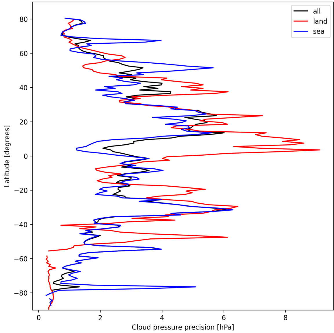
Figure 14: Zonal average of “Cloud pressure precision” for 2025-02-26 to 2025-02-28.
