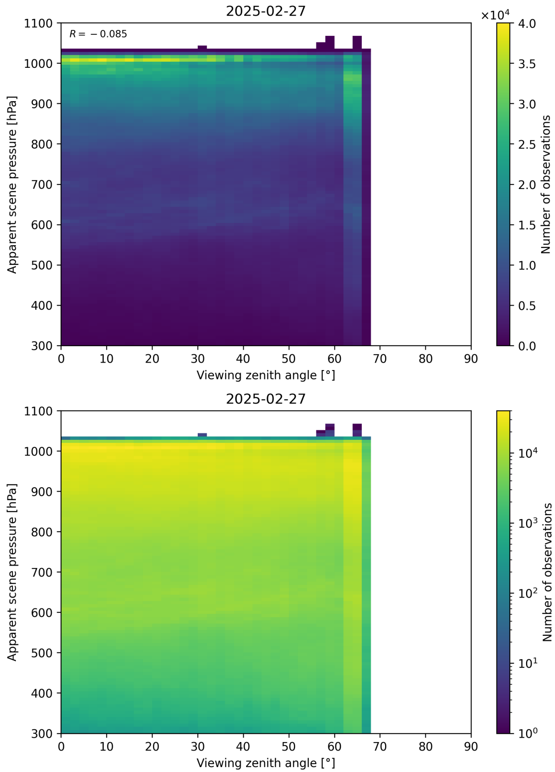
Figure 118: Scatter density plot of “Viewing zenith angle” against “Apparent scene pressure” for 2025-02-26 to 2025-02-28.
