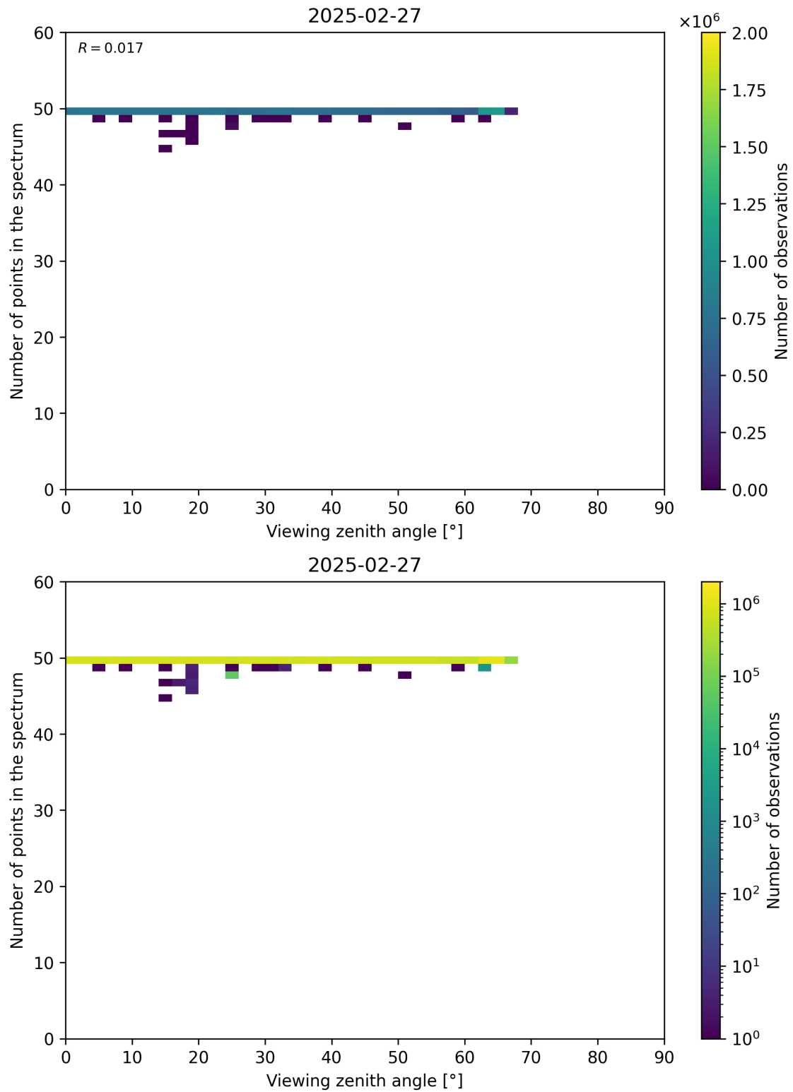
Figure 125: Scatter density plot of “Viewing zenith angle” against “Number of points in the spectrum” for 2025-02-26 to 2025-02-28.
