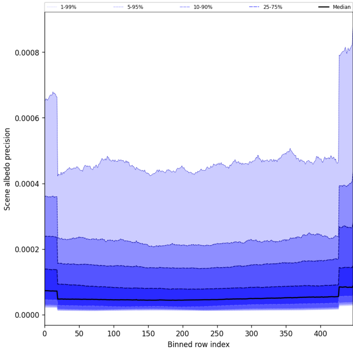
Figure 52: Along track statistics of “Scene albedo precision” for 2025-02-26 to 2025-02-28
