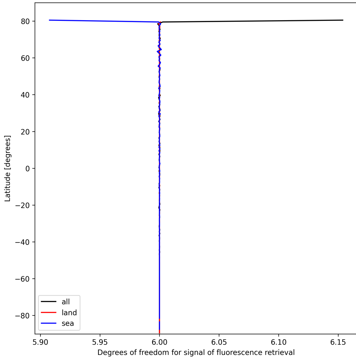
Figure 26: Zonal average of “Degrees of freedom for signal of fluorescence retrieval” for 2025-02-26 to 2025-02-28.
