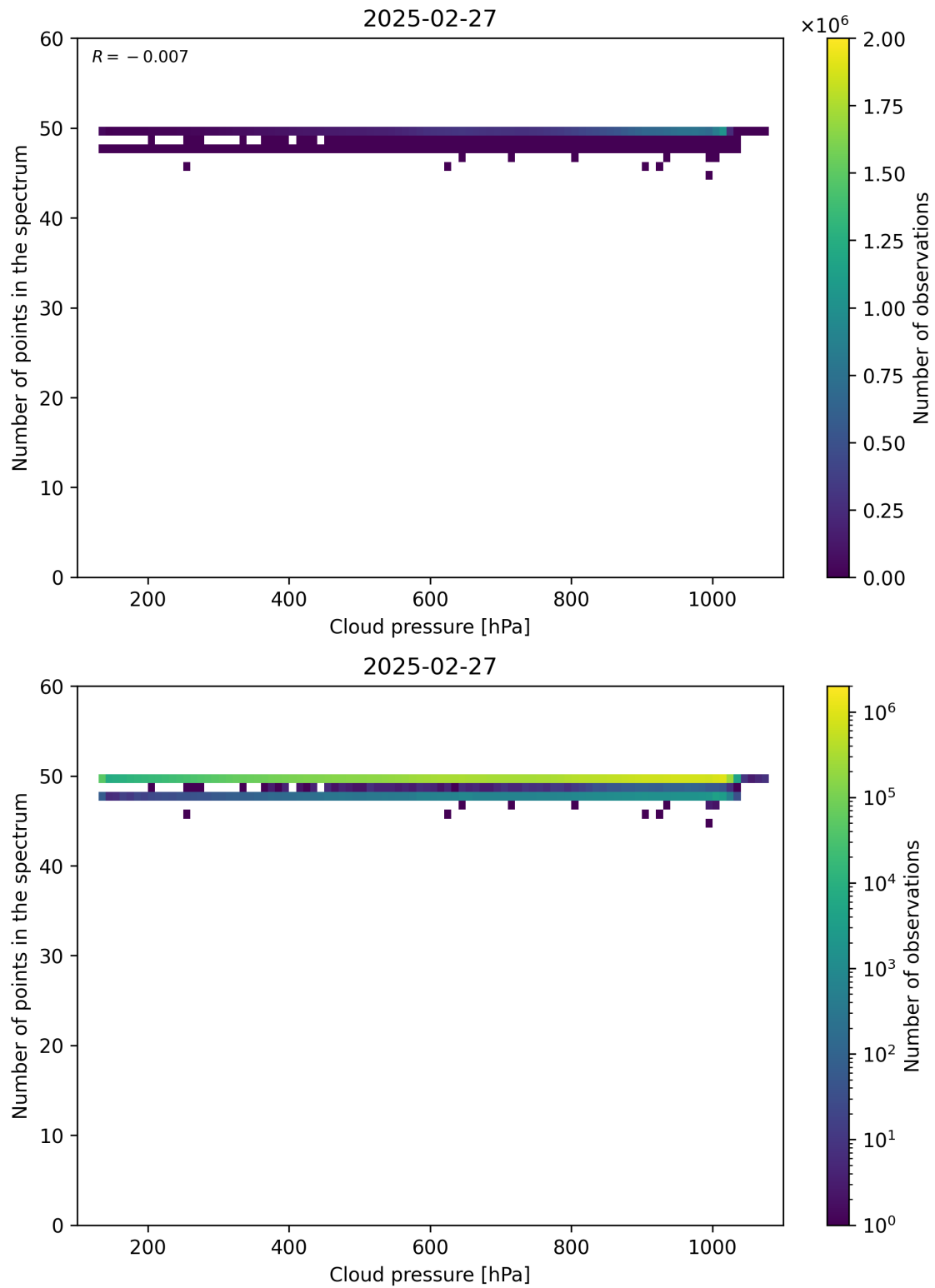
Figure 82: Scatter density plot of “Cloud pressure” against “Number of points in the spectrum” for 2025-02-26 to 2025-02-28.
