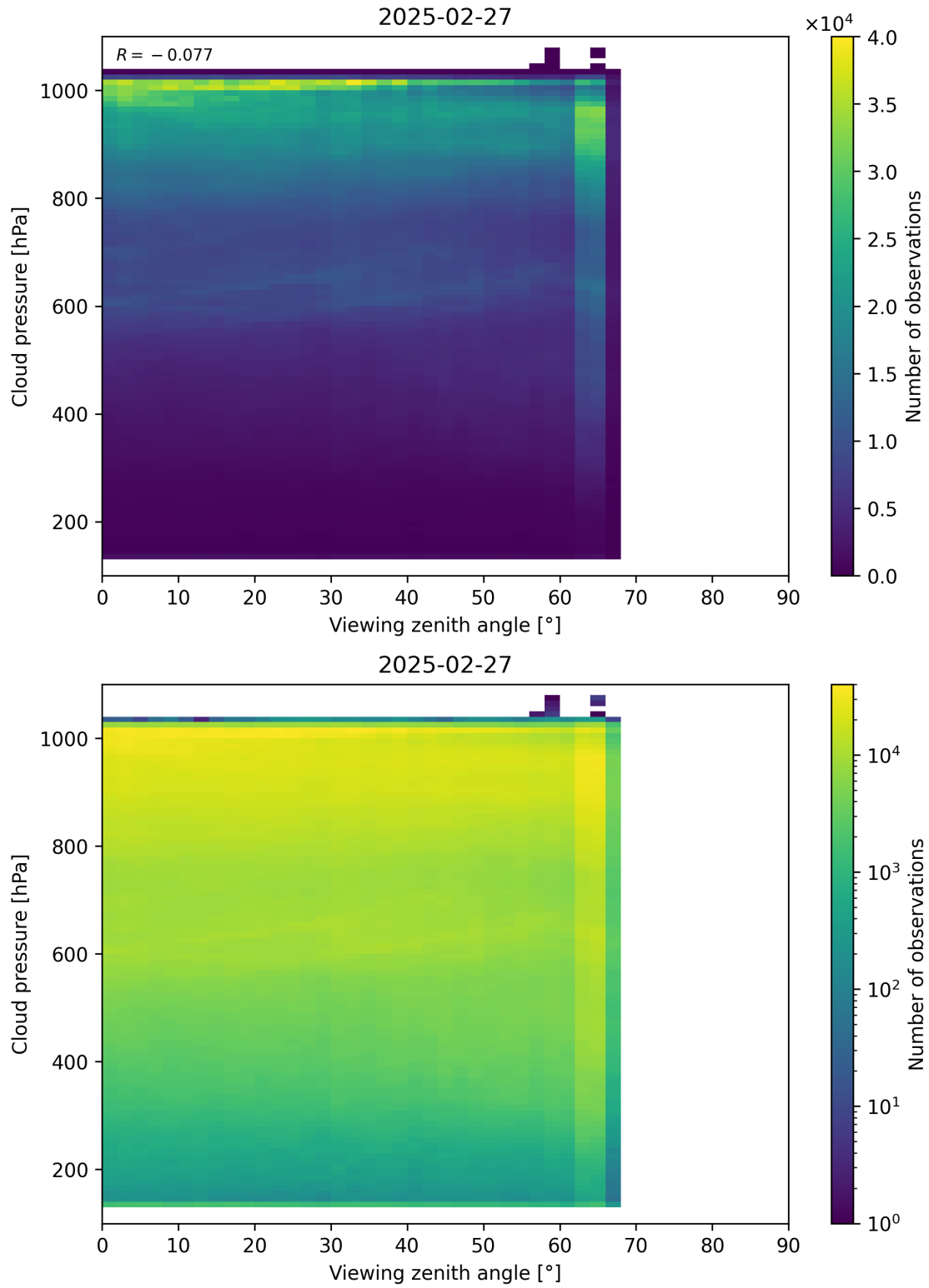
Figure 121: Scatter density plot of “Viewing zenith angle” against “Cloud pressure” for 2025-02-26 to 2025-02-28.
