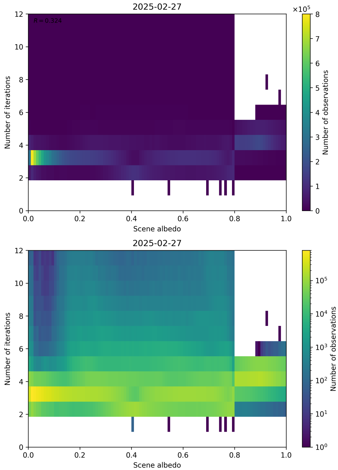
Figure 105: Scatter density plot of “Scene albedo” against “Number of iterations” for 2025-02-26 to 2025-02-28.
