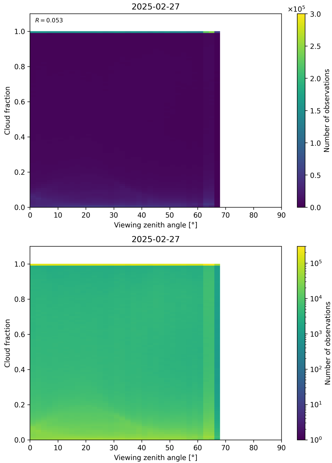
Figure 120: Scatter density plot of “Viewing zenith angle” against “Cloud fraction” for 2025-02-26 to 2025-02-28.
