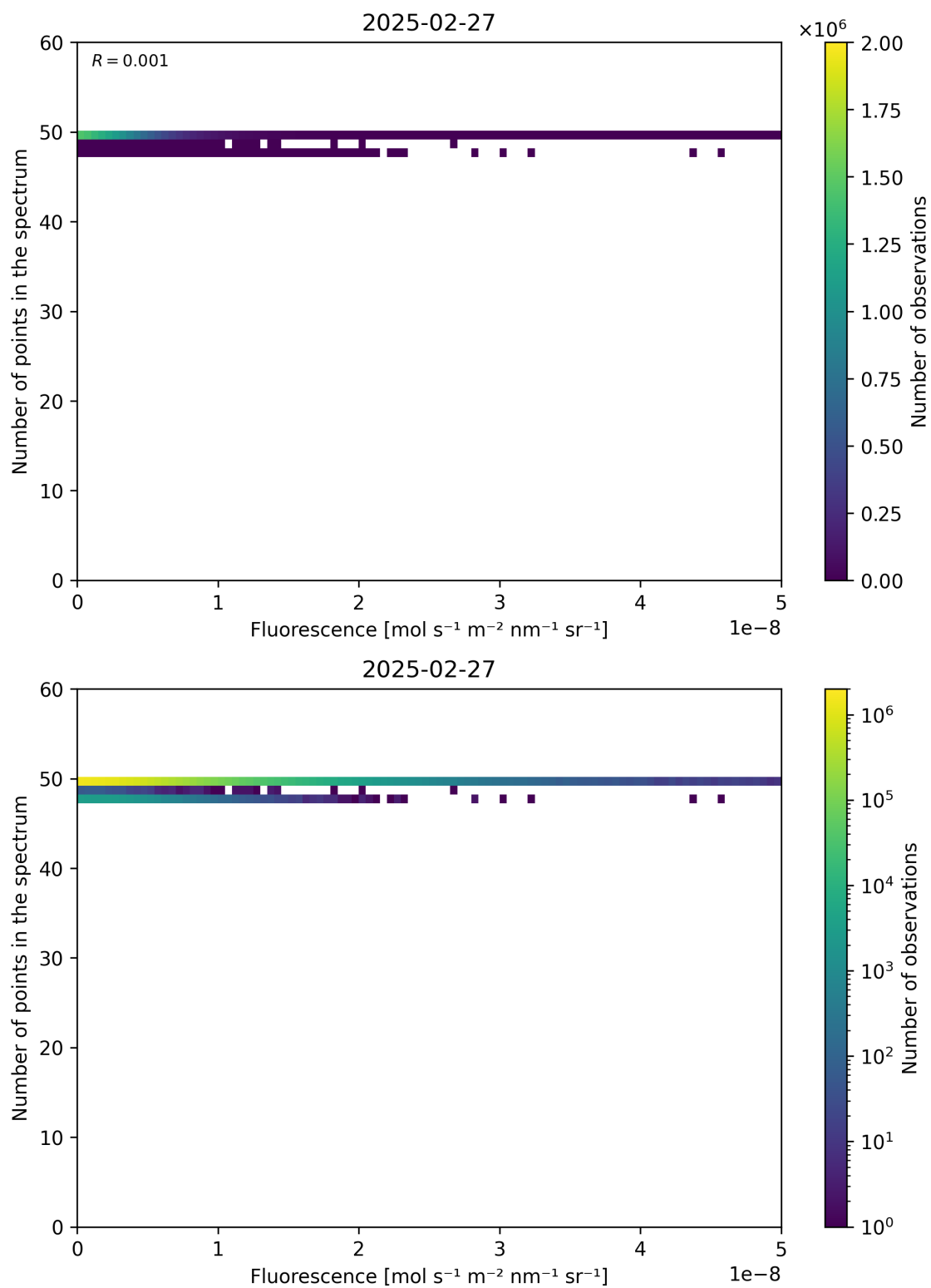
Figure 86: Scatter density plot of “Fluorescence” against “Number of points in the spectrum” for 2025-02-26 to 2025-02-28.
