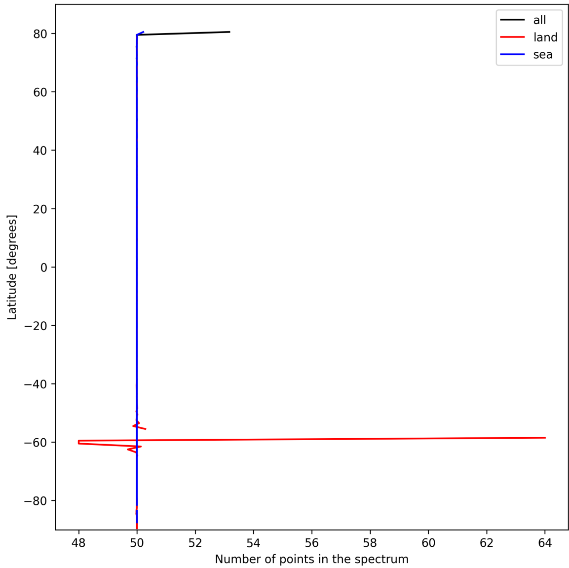
Figure 27: Zonal average of “Number of points in the spectrum” for 2025-02-26 to 2025-02-28.
