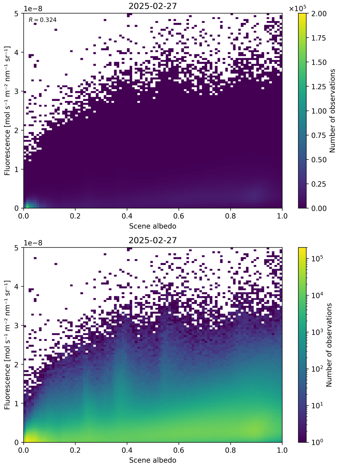
Figure 104: Scatter density plot of “Scene albedo” against “Fluorescence” for 2025-02-26 to 2025-02-28.
