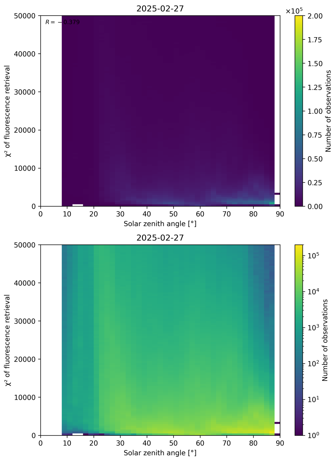
Figure 109: Scatter density plot of “Solar zenith angle” against “ \chi^2 of fluorescence retrieval” for 2025-02-26 to 2025-02-28.
