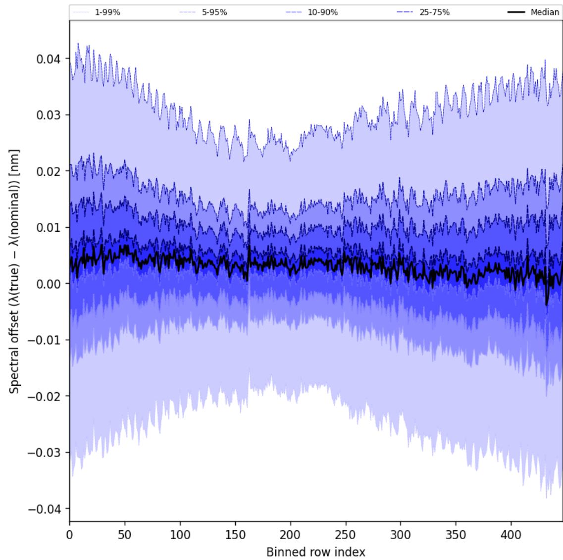
Figure 62: Along track statistics of “Spectral offset ( \lambda_{\text{true}} - \lambda_{\text{nominal}} )” for 2025-02-26 to 2025-02-28
