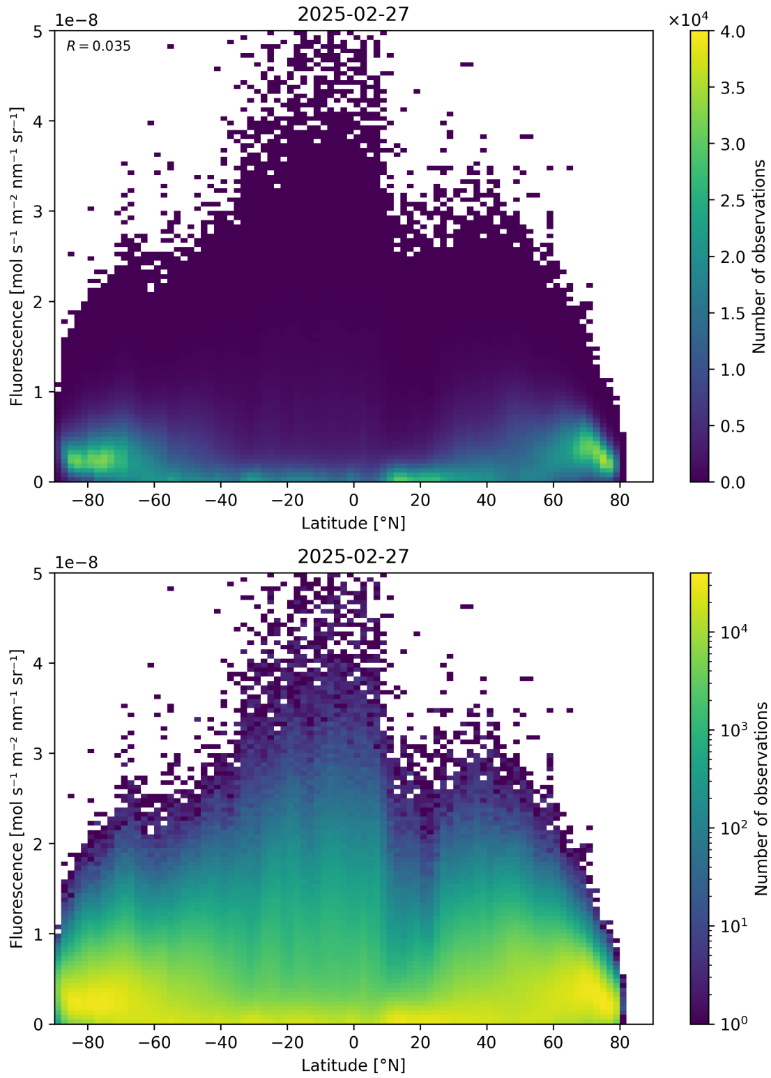
Figure 92: Scatter density plot of “Latitude” against “Fluorescence” for 2025-02-26 to 2025-02-28.
