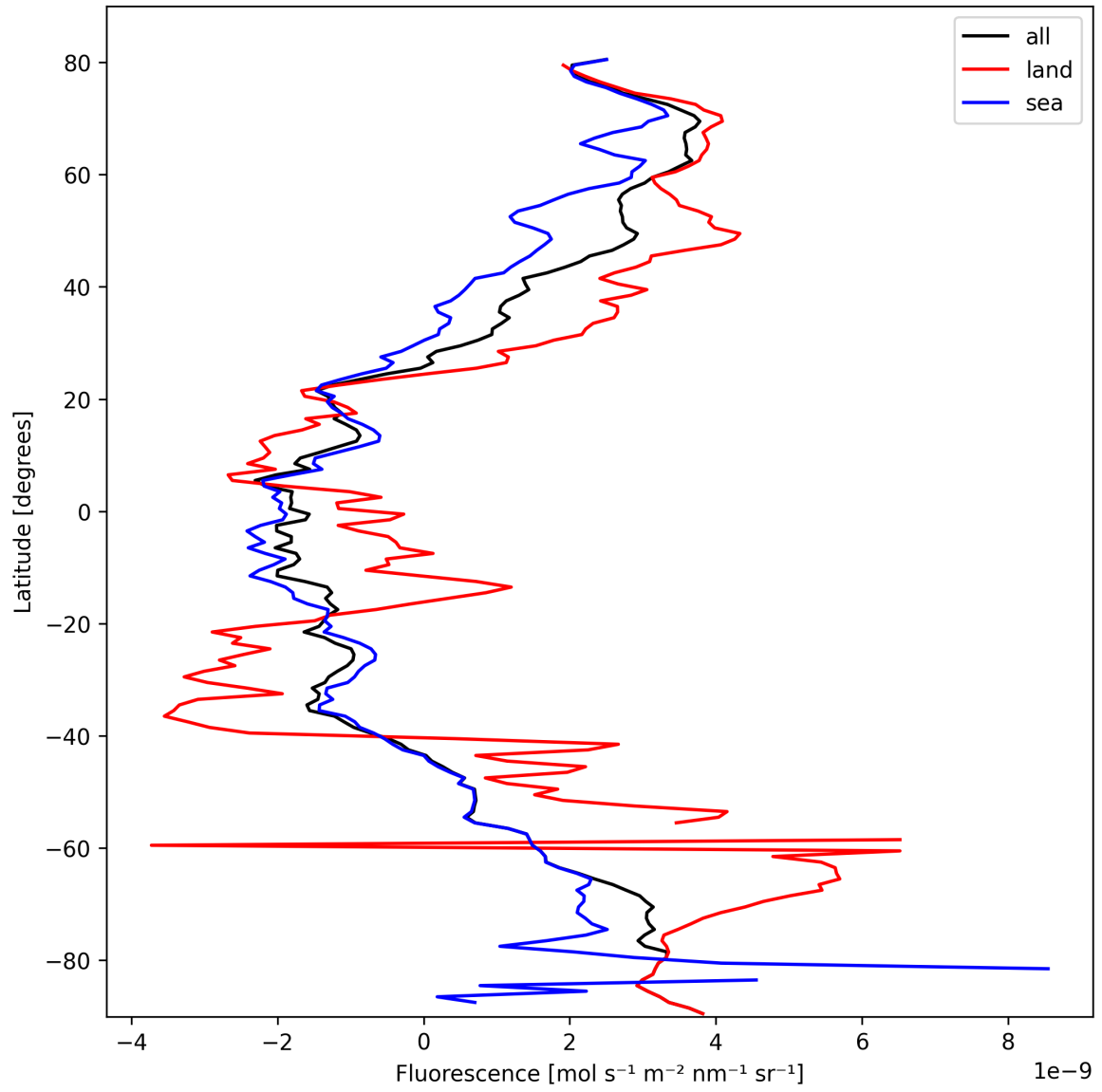
Figure 23: Zonal average of “Fluorescence” for 2025-02-26 to 2025-02-28.
