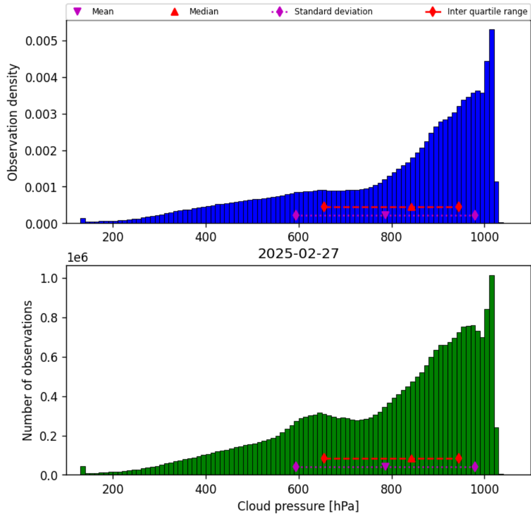
Figure 30: Histogram of “Cloud pressure” for 2025-02-26 to 2025-02-28
