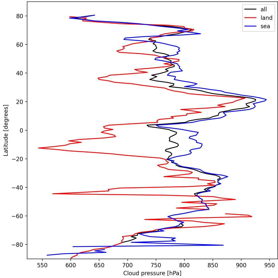
Figure 13: Zonal average of “Cloud pressure” for 2025-02-26 to 2025-02-28.
