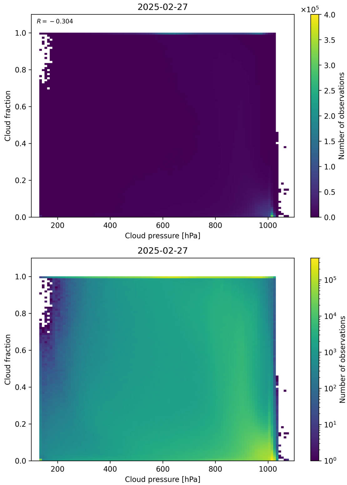
Figure 79: Scatter density plot of “Cloud pressure” against “Cloud fraction” for 2025-02-26 to 2025-02-28.
