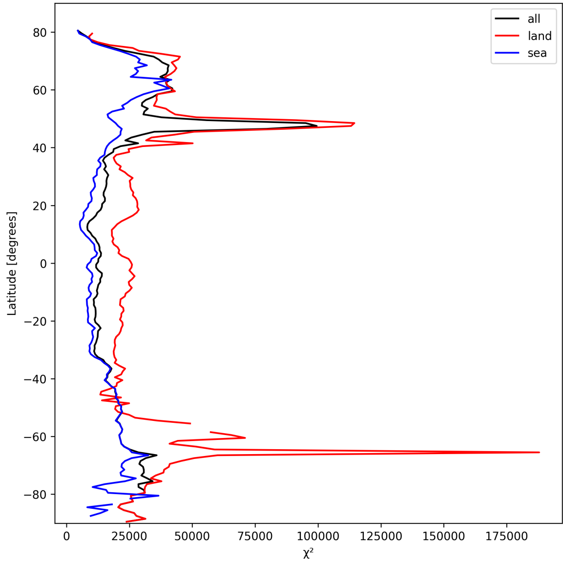
Figure 21: Zonal average of “ \chi^2 ” for 2025-02-26 to 2025-02-28.
