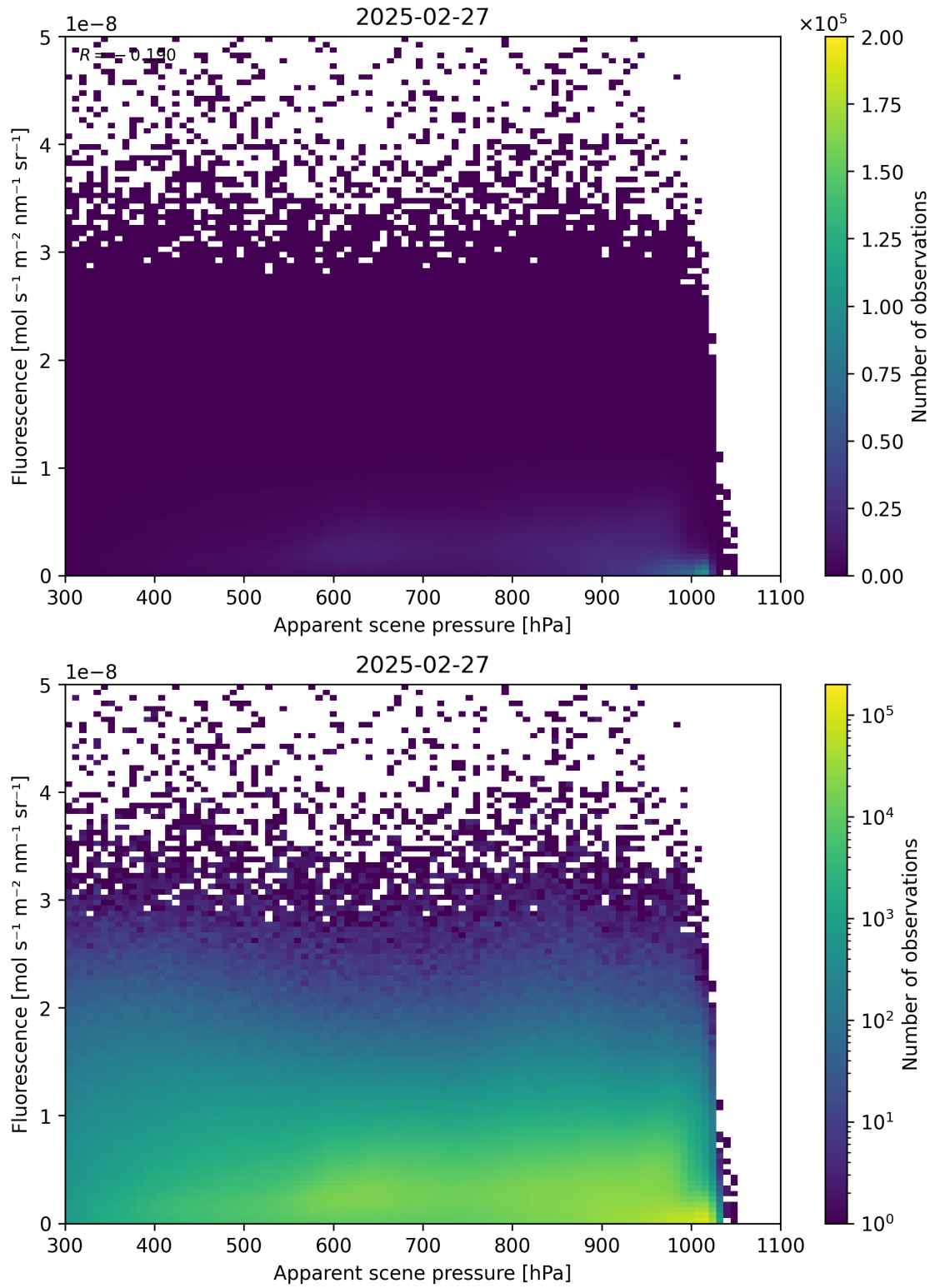
Figure 64: Scatter density plot of “Apparent scene pressure” against “Fluorescence” for 2025-02-26 to 2025-02-28.
