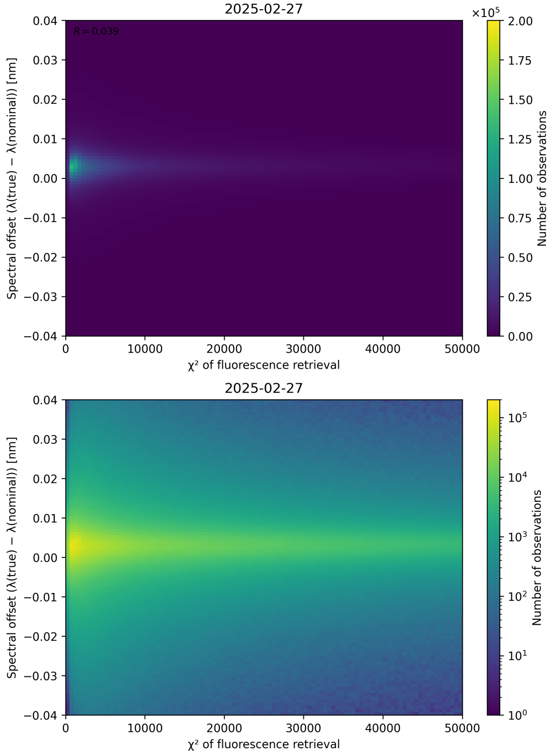
Figure 69: Scatter density plot of “ \chi^2 of fluorescence retrieval” against “Spectral offset ( \lambda_{\text{true}} - \lambda_{\text{nominal}} )” for 2025-02-26 to 2025-02-28.
