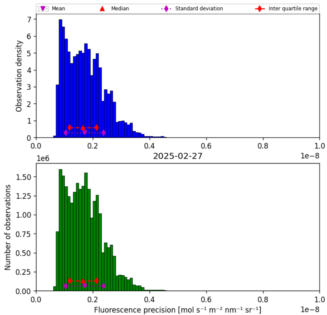
Figure 41: Histogram of “Fluorescence precision” for 2025-02-26 to 2025-02-28
