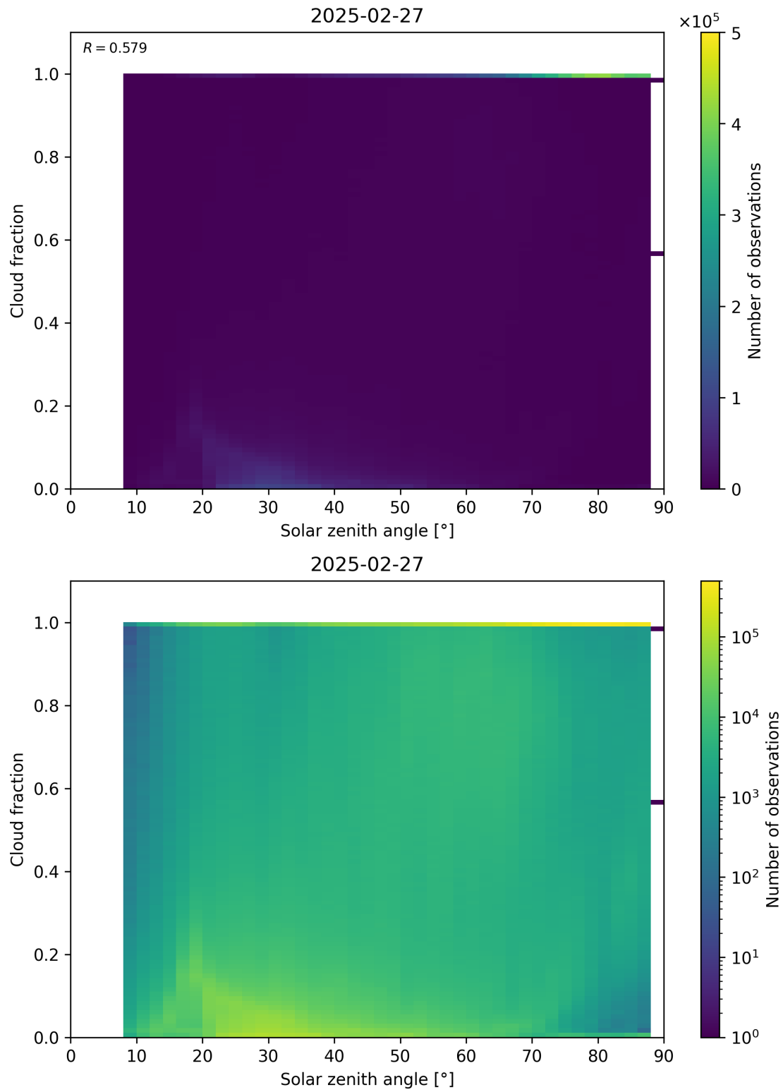
Figure 110: Scatter density plot of “Solar zenith angle” against “Cloud fraction” for 2025-02-26 to 2025-02-28.
