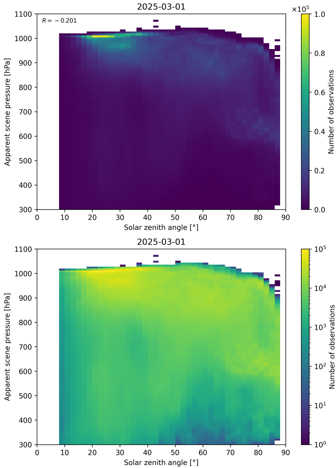
Figure 108: Scatter density plot of “Solar zenith angle” against “Apparent scene pressure” for 2025-03-01 to 2025-03-02.
