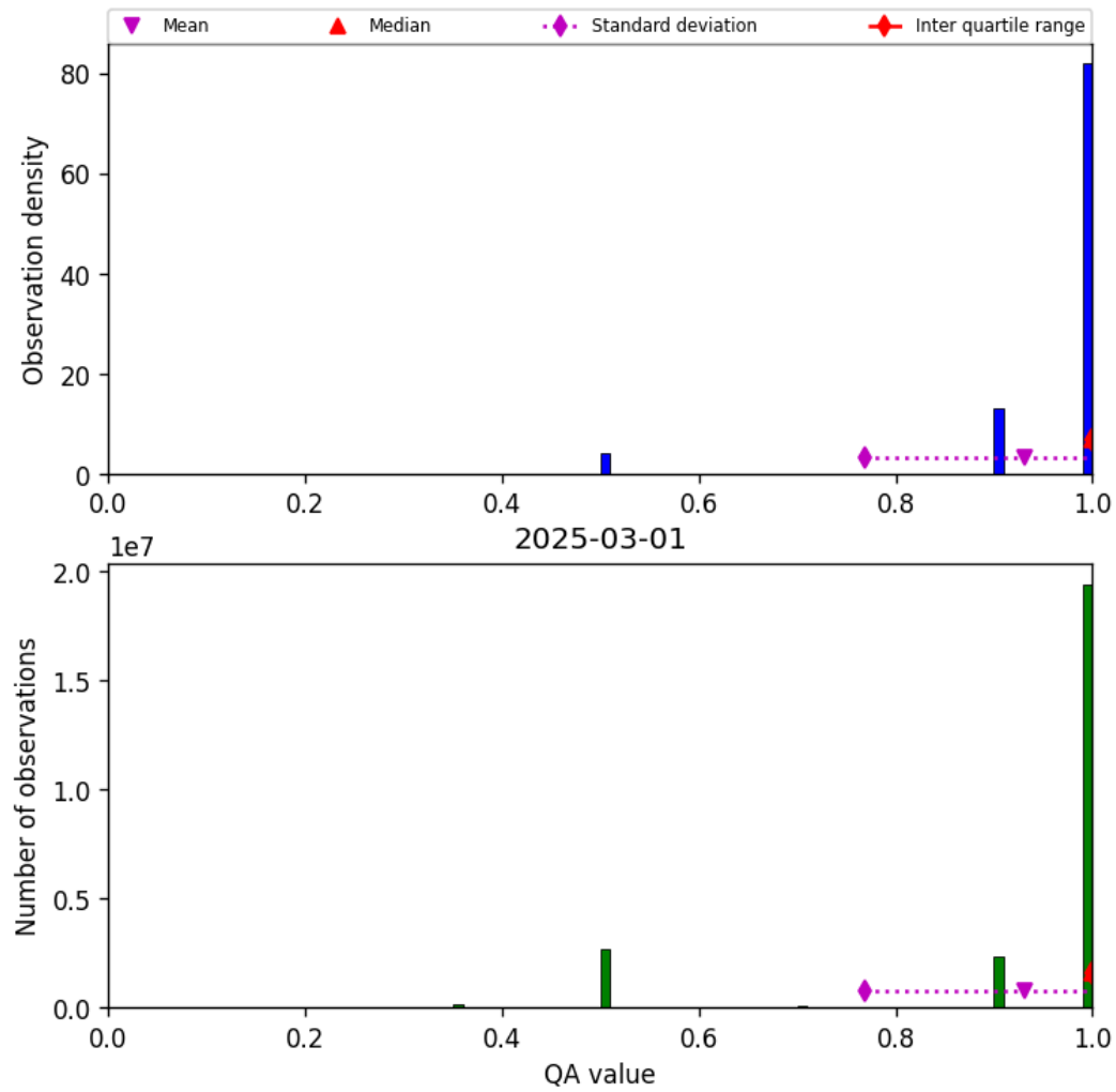
Figure 29: Histogram of “QA value” for 2025-03-01 to 2025-03-02
