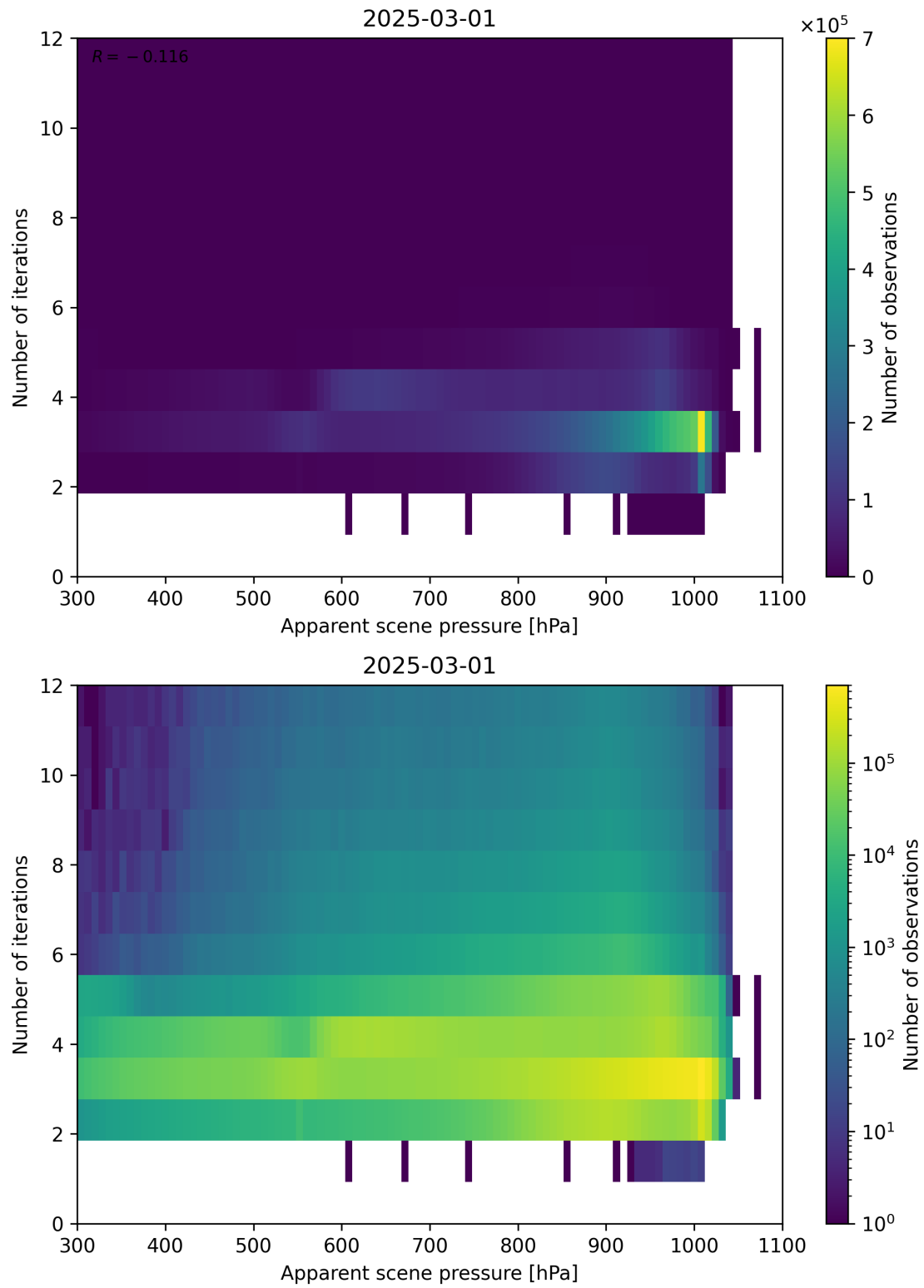
Figure 65: Scatter density plot of “Apparent scene pressure” against “Number of iterations” for 2025-03-01 to 2025-03-02.
