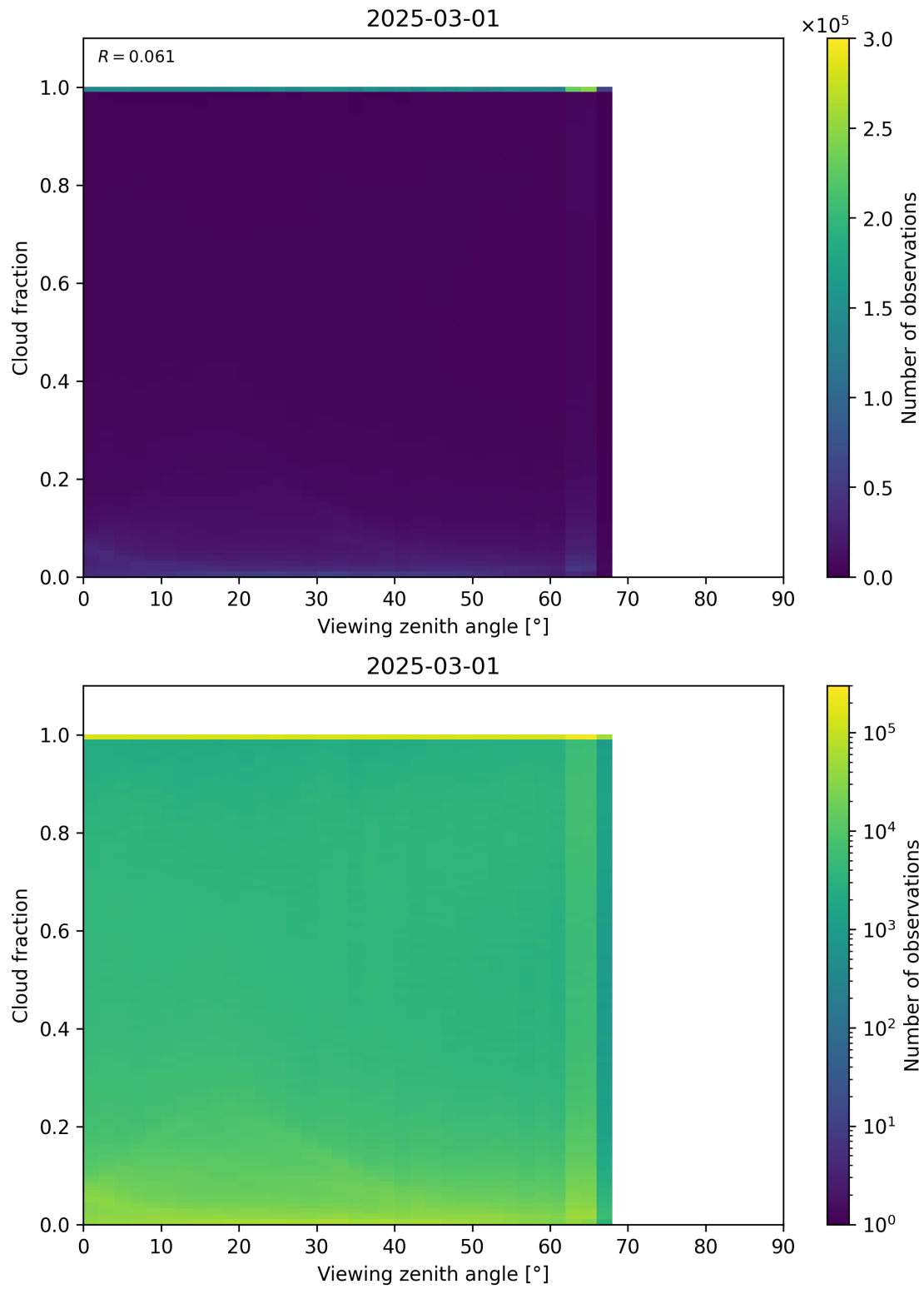
Figure 120: Scatter density plot of “Viewing zenith angle” against “Cloud fraction” for 2025-03-01 to 2025-03-02.
