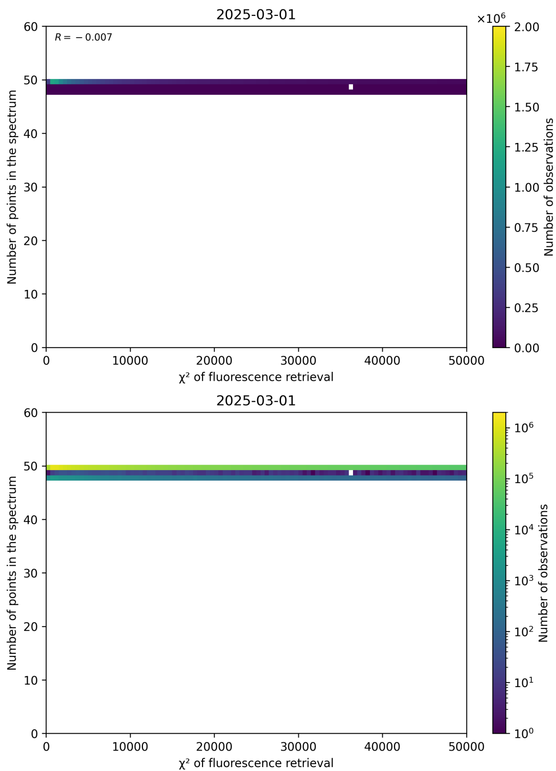
Figure 68: Scatter density plot of “ \chi^2 of fluorescence retrieval” against “Number of points in the spectrum” for 2025-03-01 to 2025-03-02.
