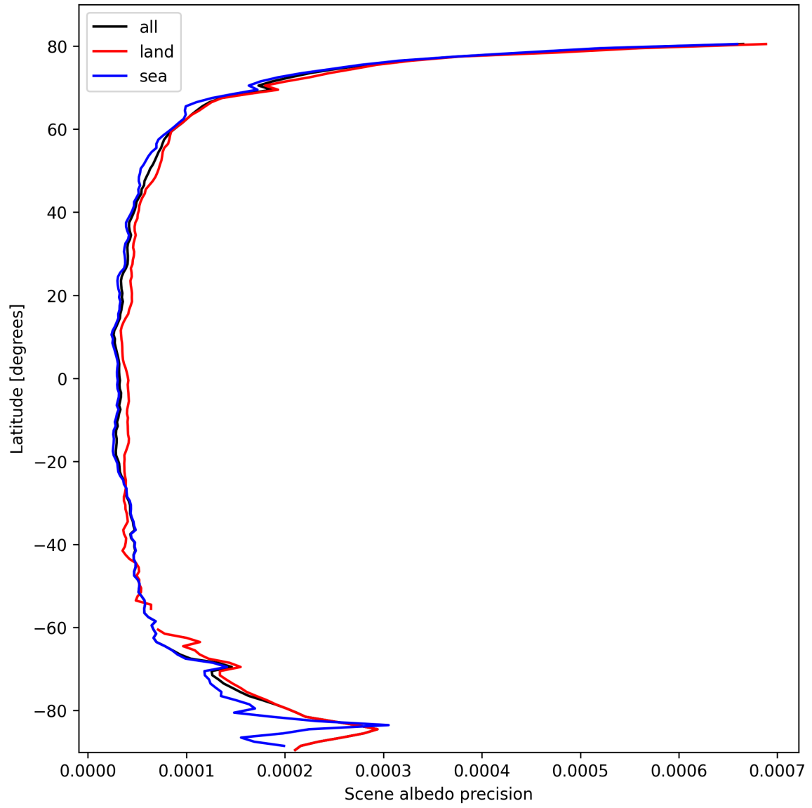
Figure 18: Zonal average of “Scene albedo precision” for 2025-03-01 to 2025-03-02.
