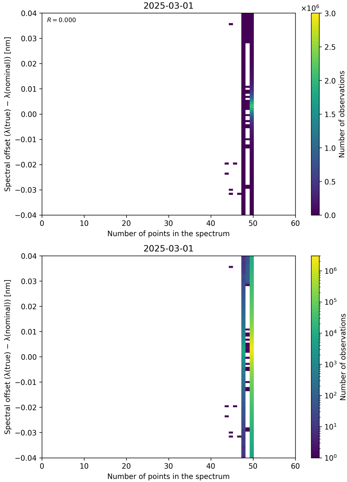
Figure 101: Scatter density plot of “Number of points in the spectrum” against “Spectral offset ( \lambda_{\text{true}} - \lambda_{\text{nominal}} )” for 2025-03-01 to 2025-03-02.
