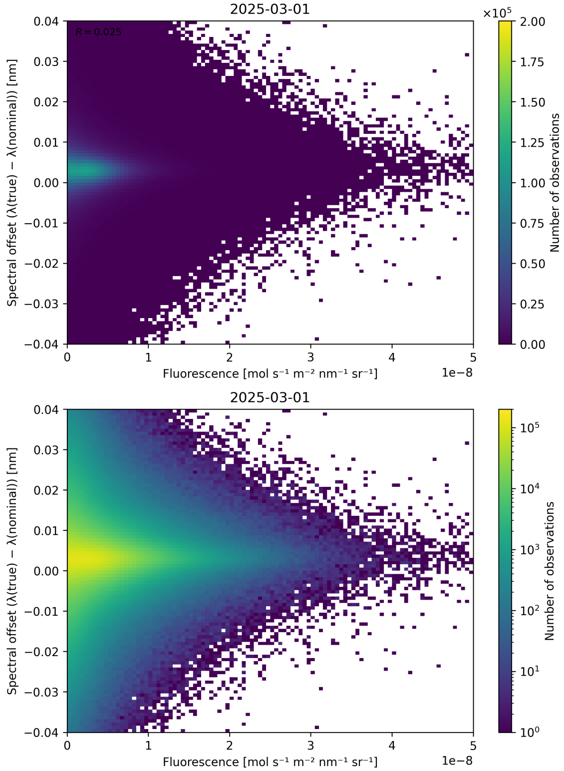
Figure 87: Scatter density plot of “Fluorescence” against “Spectral offset ( \lambda_{\text{true}} - \lambda_{\text{nominal}} )” for 2025-03-01 to 2025-03-02.
