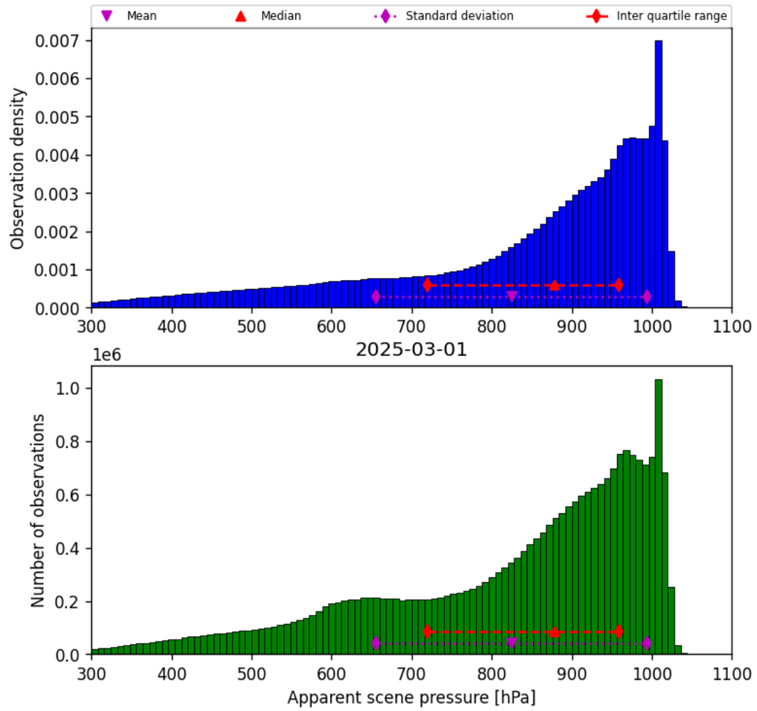
Figure 36: Histogram of “Apparent scene pressure” for 2025-03-01 to 2025-03-02
