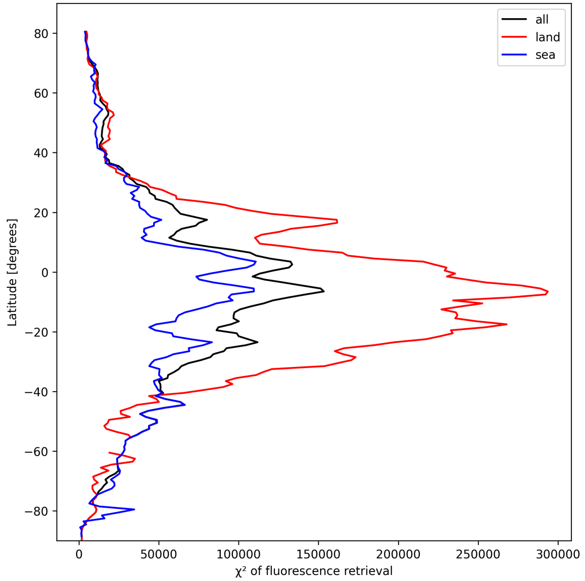
Figure 25: Zonal average of “ \chi^2 of fluorescence retrieval” for 2025-03-01 to 2025-03-02.
