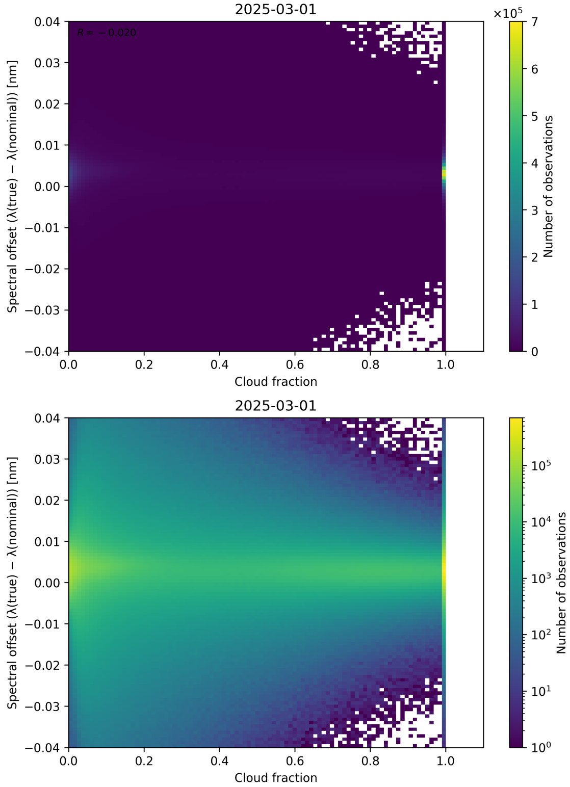
Figure 76: Scatter density plot of “Cloud fraction” against “Spectral offset ( \lambda_{\text{true}} - \lambda_{\text{nominal}} )” for 2025-03-01 to 2025-03-02.
