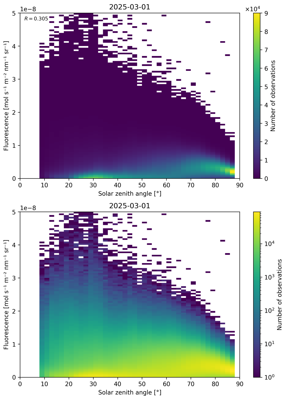
Figure 112: Scatter density plot of “Solar zenith angle” against “Fluorescence” for 2025-03-01 to 2025-03-02.
