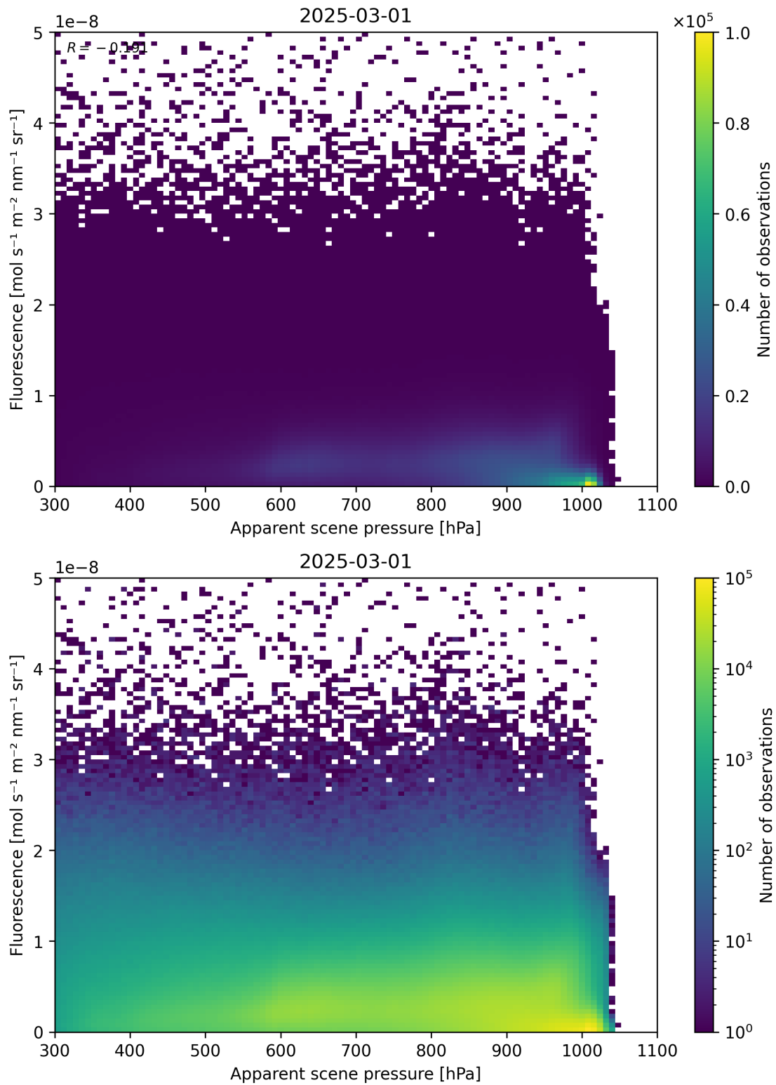
Figure 64: Scatter density plot of “Apparent scene pressure” against “Fluorescence” for 2025-03-01 to 2025-03-02.
