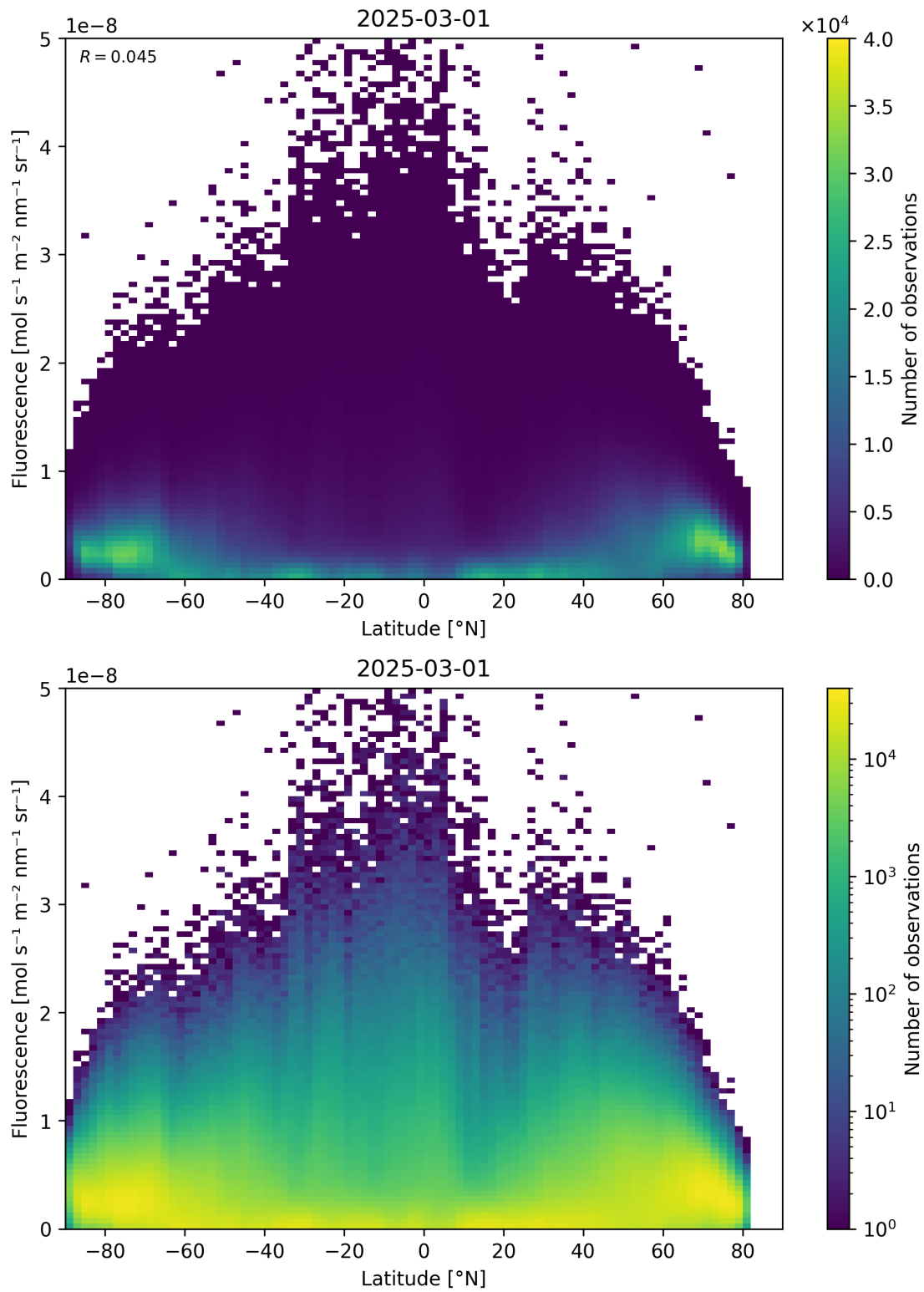
Figure 92: Scatter density plot of “Latitude” against “Fluorescence” for 2025-03-01 to 2025-03-02.
