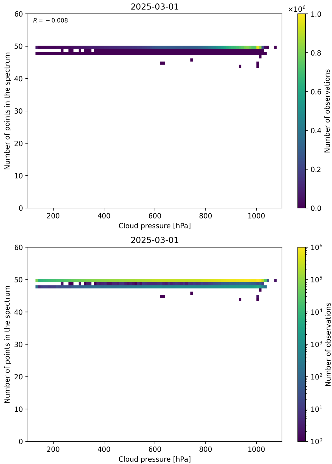
Figure 82: Scatter density plot of “Cloud pressure” against “Number of points in the spectrum” for 2025-03-01 to 2025-03-02.
