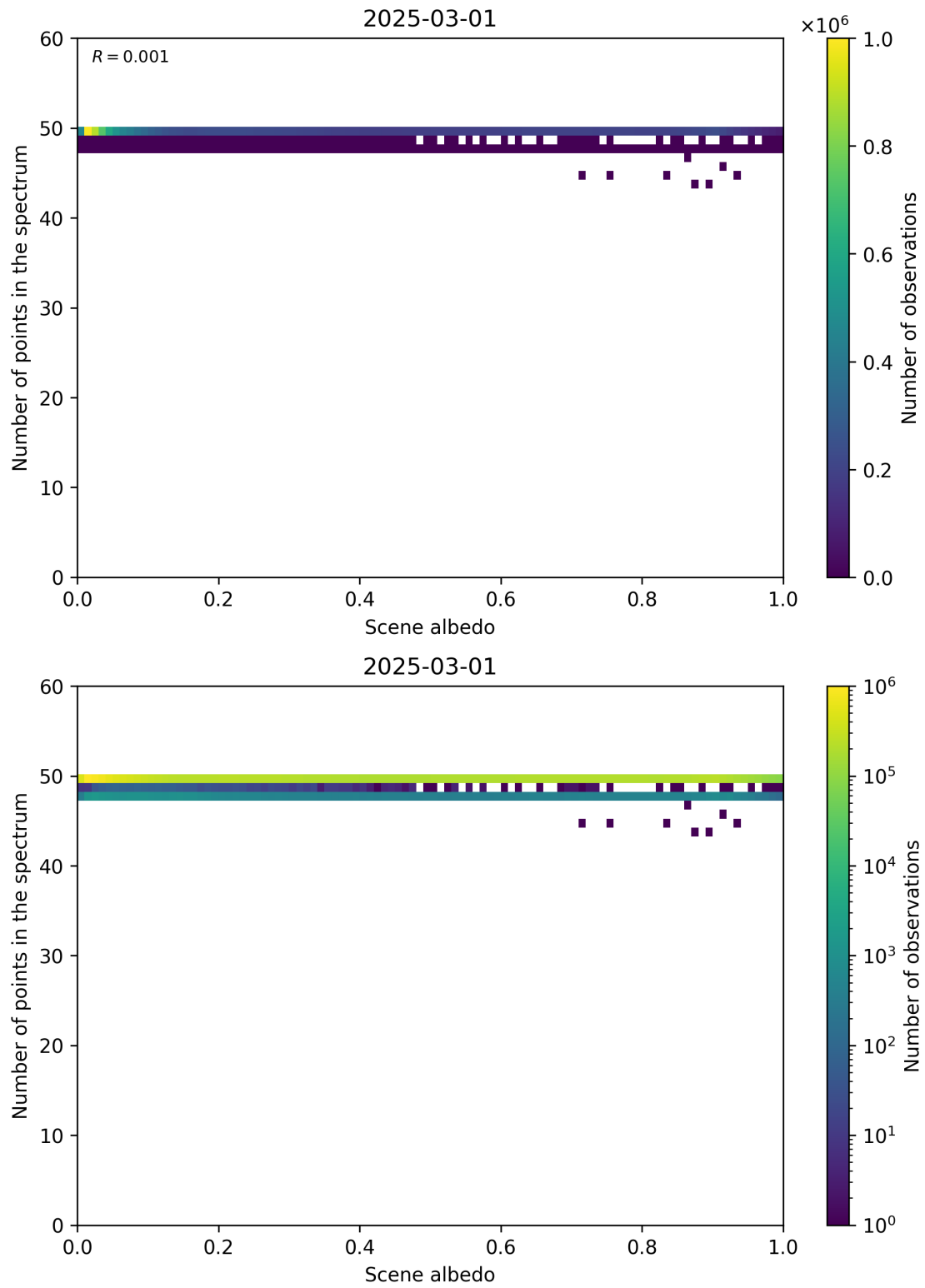
Figure 106: Scatter density plot of “Scene albedo” against “Number of points in the spectrum” for 2025-03-01 to 2025-03-02.
