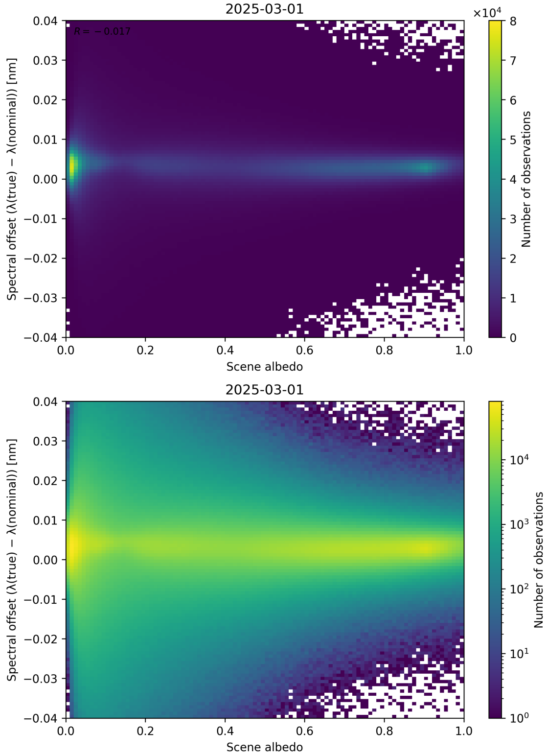
Figure 107: Scatter density plot of “Scene albedo” against “Spectral offset ( \lambda_{\text{true}} - \lambda_{\text{nominal}} )” for 2025-03-01 to 2025-03-02.
