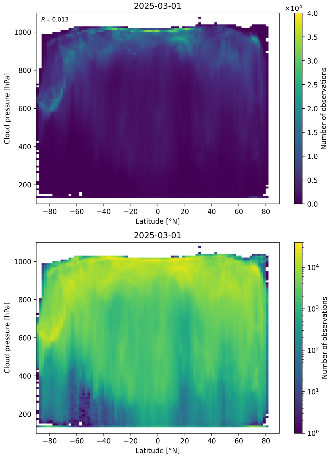
Figure 91: Scatter density plot of “Latitude” against “Cloud pressure” for 2025-03-01 to 2025-03-02.
