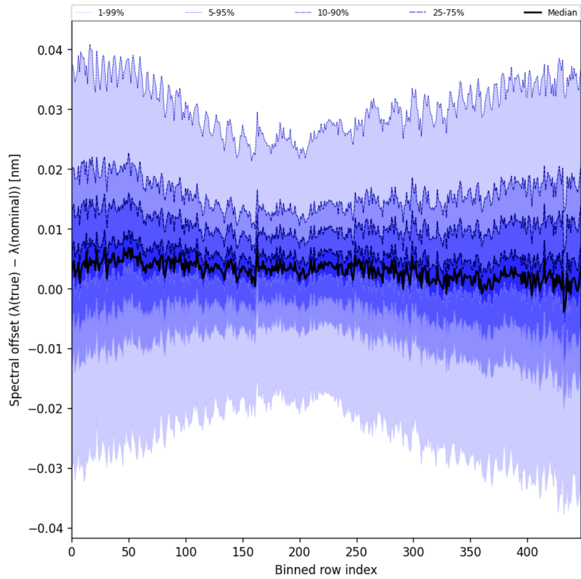
Figure 62: Along track statistics of “Spectral offset ( \lambda_{\text{true}} - \lambda_{\text{nominal}} )” for 2025-03-01 to 2025-03-02
