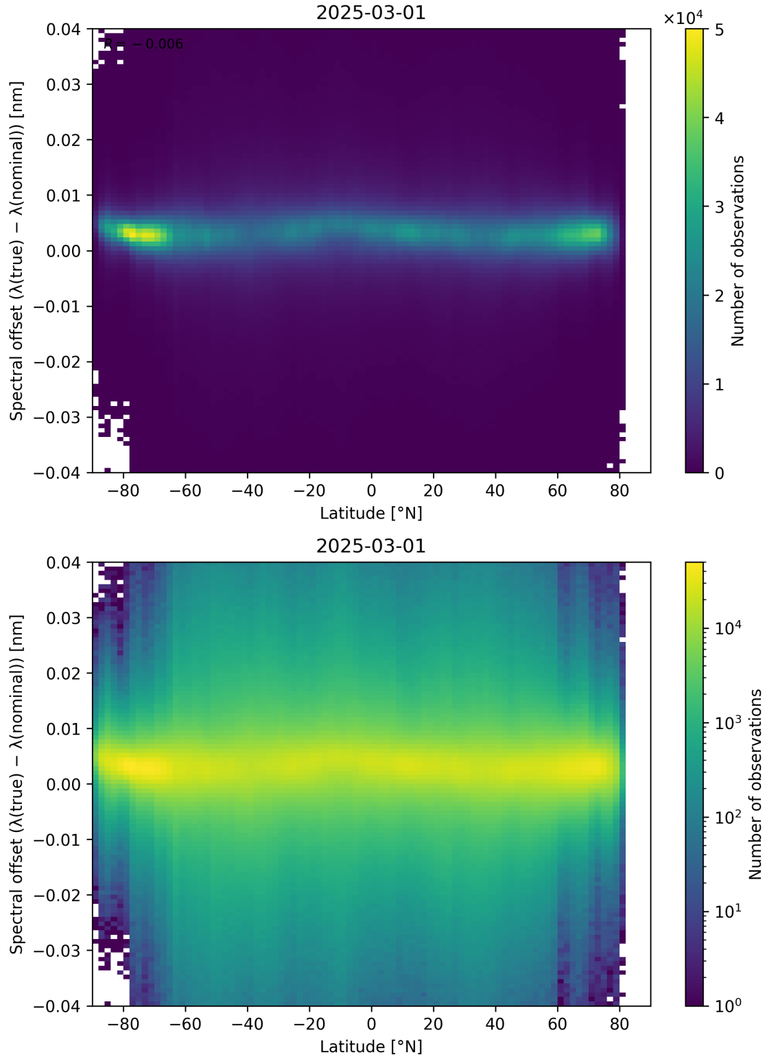
Figure 96: Scatter density plot of “Latitude” against “Spectral offset ( \lambda_{\text{true}} - \lambda_{\text{nominal}} )” for 2025-03-01 to 2025-03-02.
