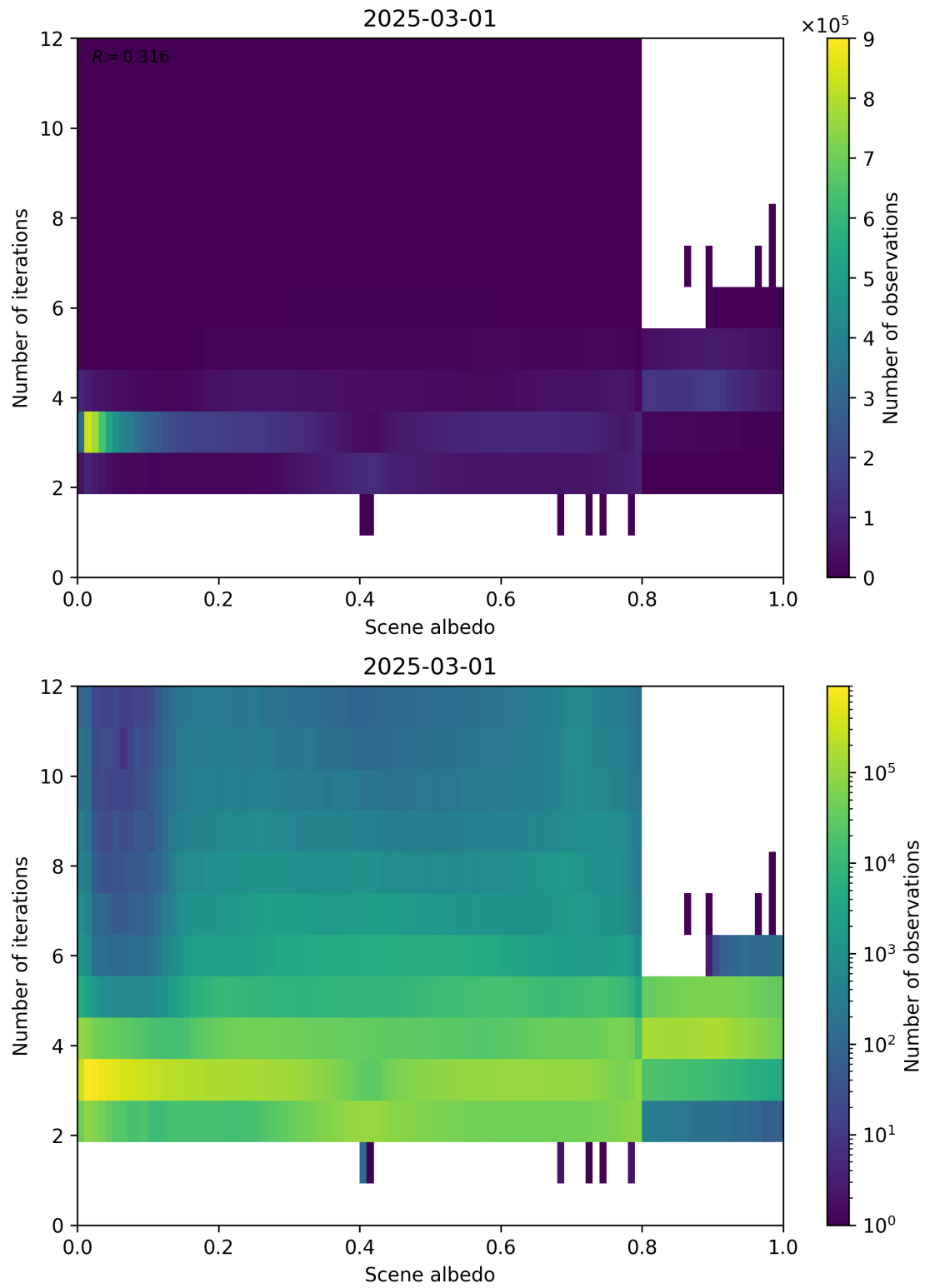
Figure 105: Scatter density plot of “Scene albedo” against “Number of iterations” for 2025-03-01 to 2025-03-02.
