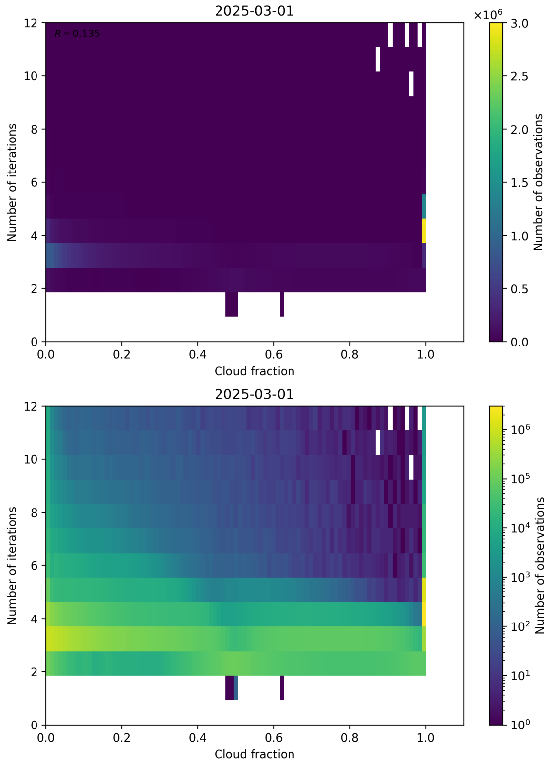
Figure 73: Scatter density plot of “Cloud fraction” against “Number of iterations” for 2025-03-01 to 2025-03-02.
