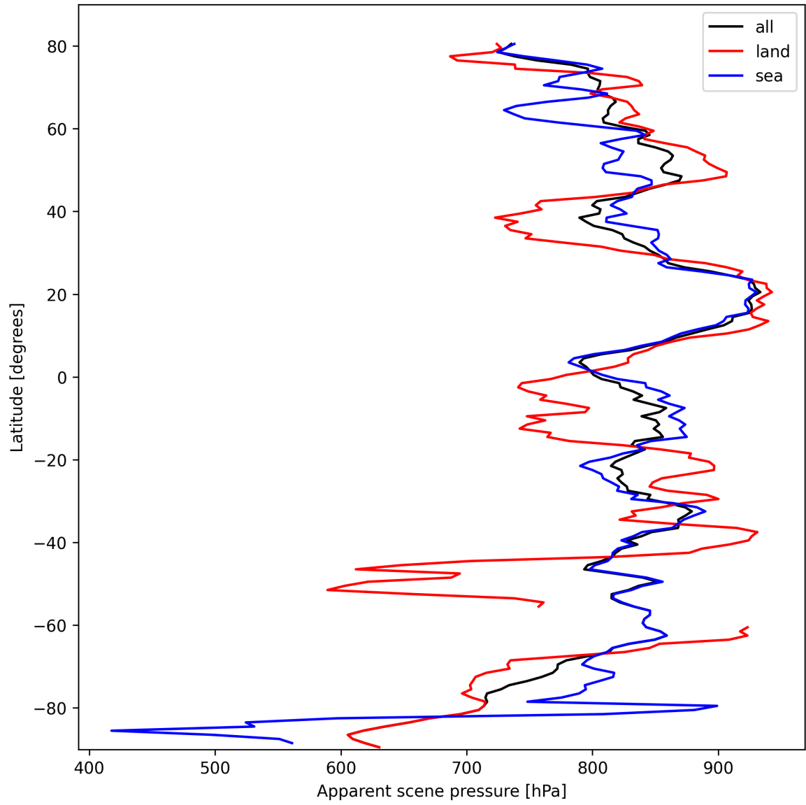
Figure 19: Zonal average of “Apparent scene pressure” for 2025-03-01 to 2025-03-02.
