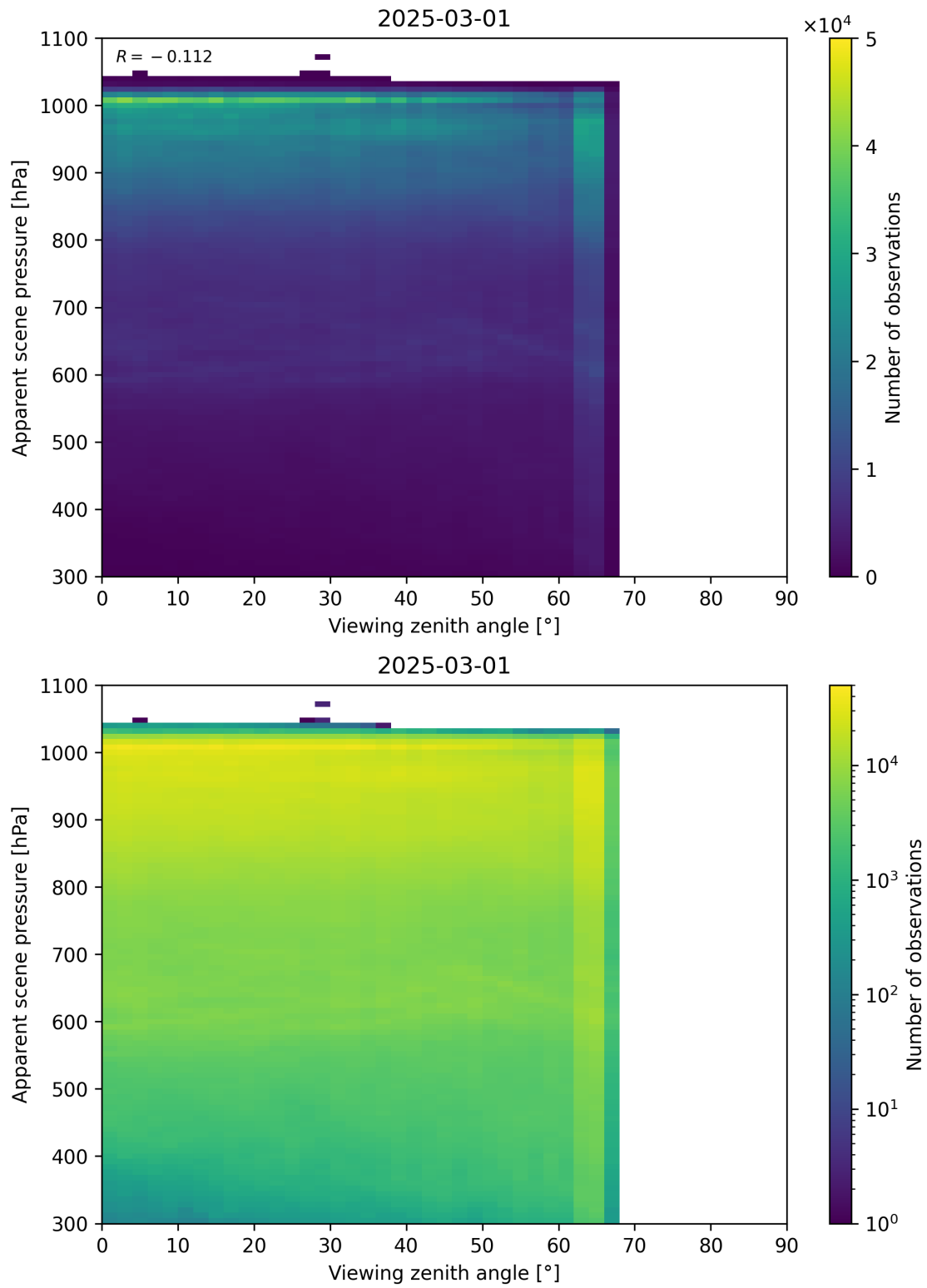
Figure 118: Scatter density plot of “Viewing zenith angle” against “Apparent scene pressure” for 2025-03-01 to 2025-03-02.
