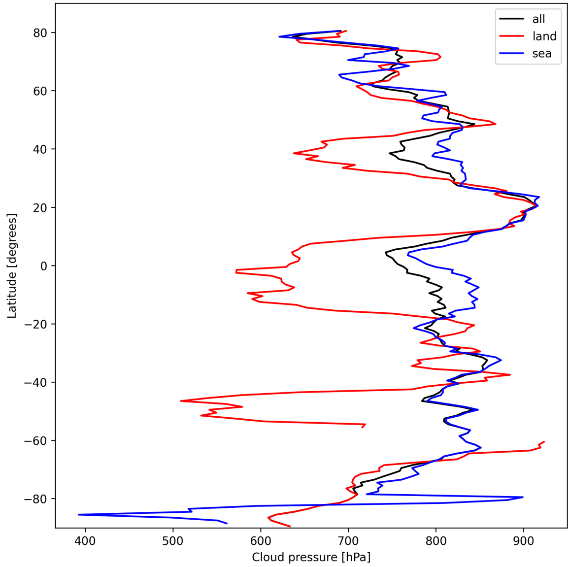
Figure 13: Zonal average of “Cloud pressure” for 2025-03-01 to 2025-03-02.
