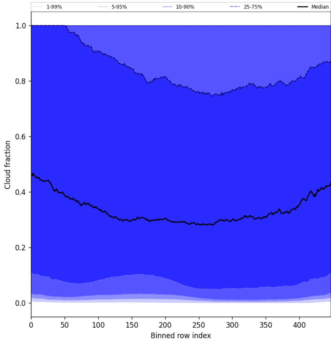
Figure 49: Along track statistics of “Cloud fraction” for 2025-03-01 to 2025-03-02
