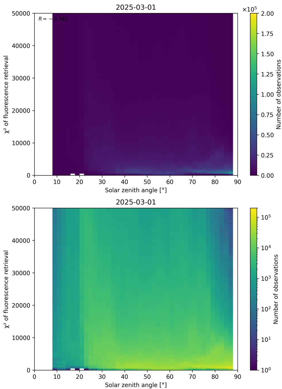
Figure 109: Scatter density plot of “Solar zenith angle” against “ \chi^2 of fluorescence retrieval” for 2025-03-01 to 2025-03-02.
