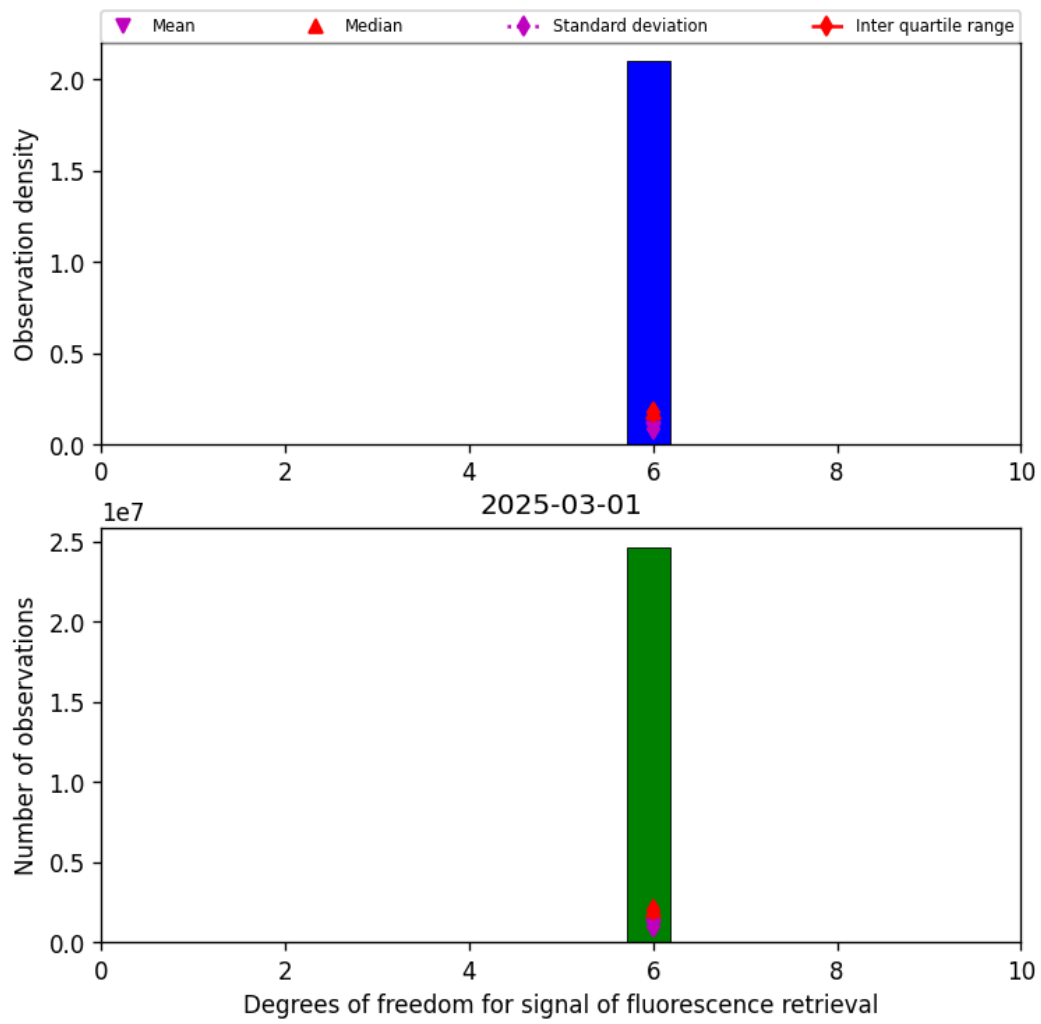
Figure 43: Histogram of “Degrees of freedom for signal of fluorescence retrieval” for 2025-03-01 to 2025-03-02
