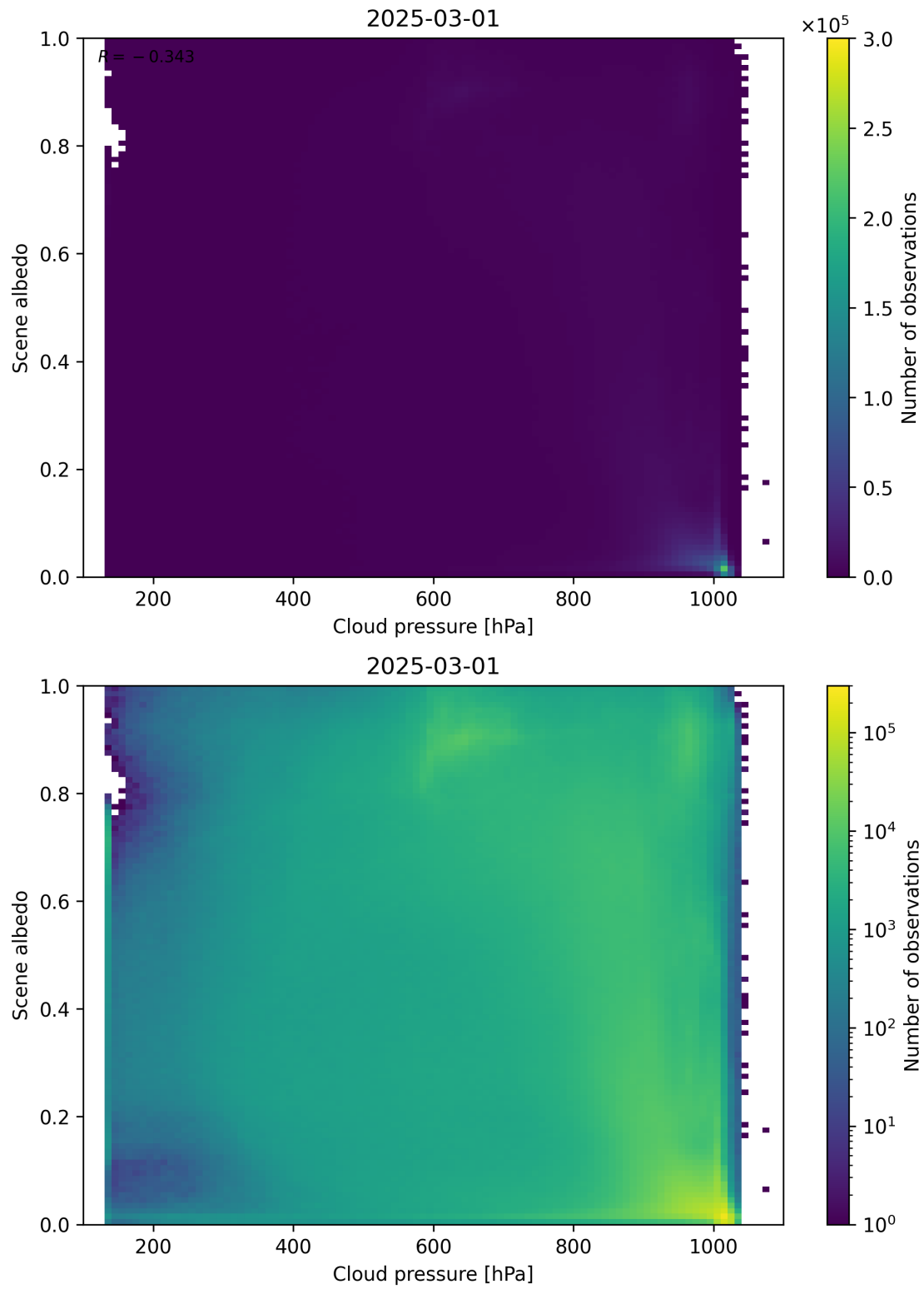
Figure 83: Scatter density plot of “Cloud pressure” against “Scene albedo” for 2025-03-01 to 2025-03-02.
