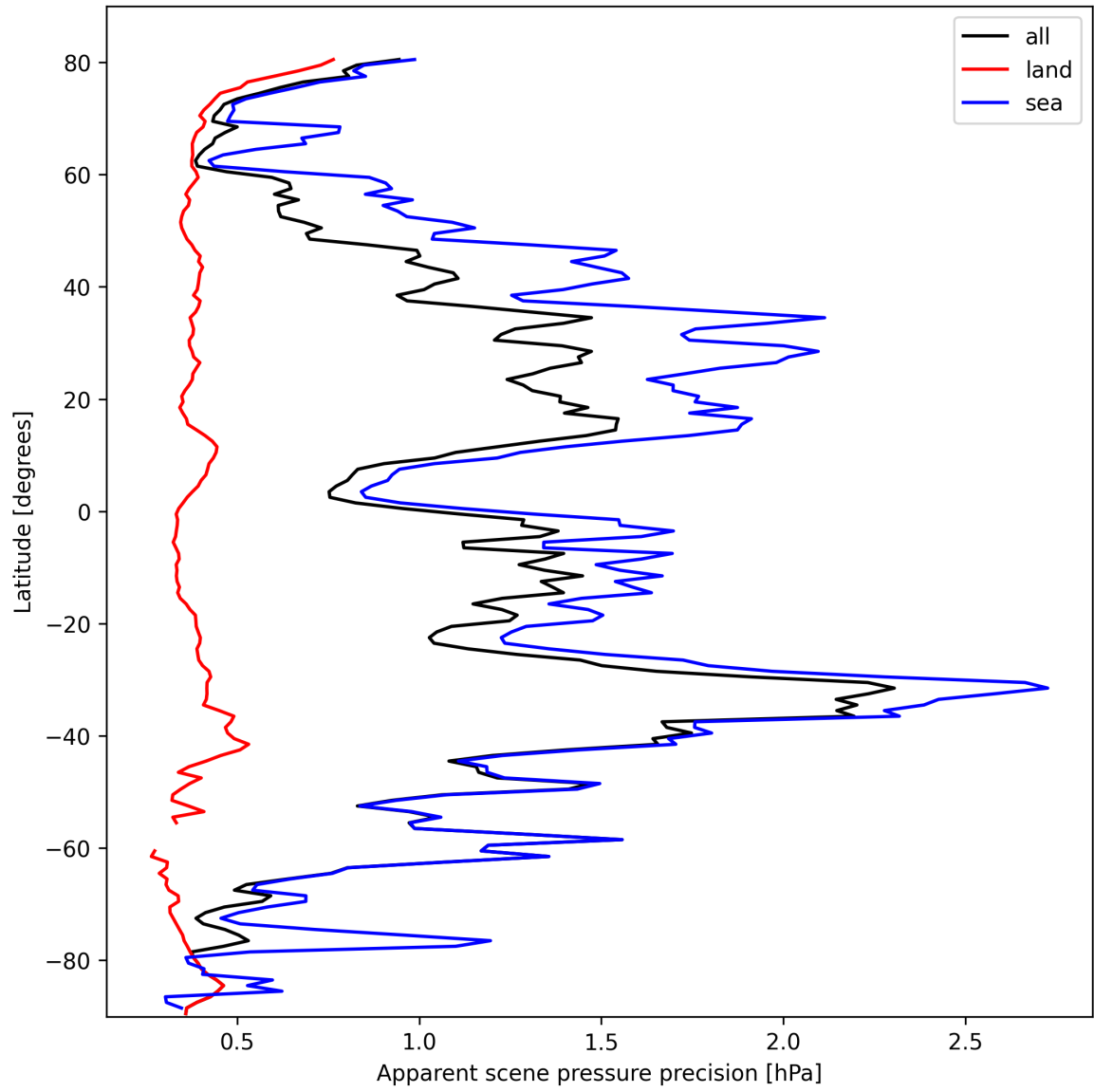
Figure 20: Zonal average of “Apparent scene pressure precision” for 2025-03-01 to 2025-03-02.
