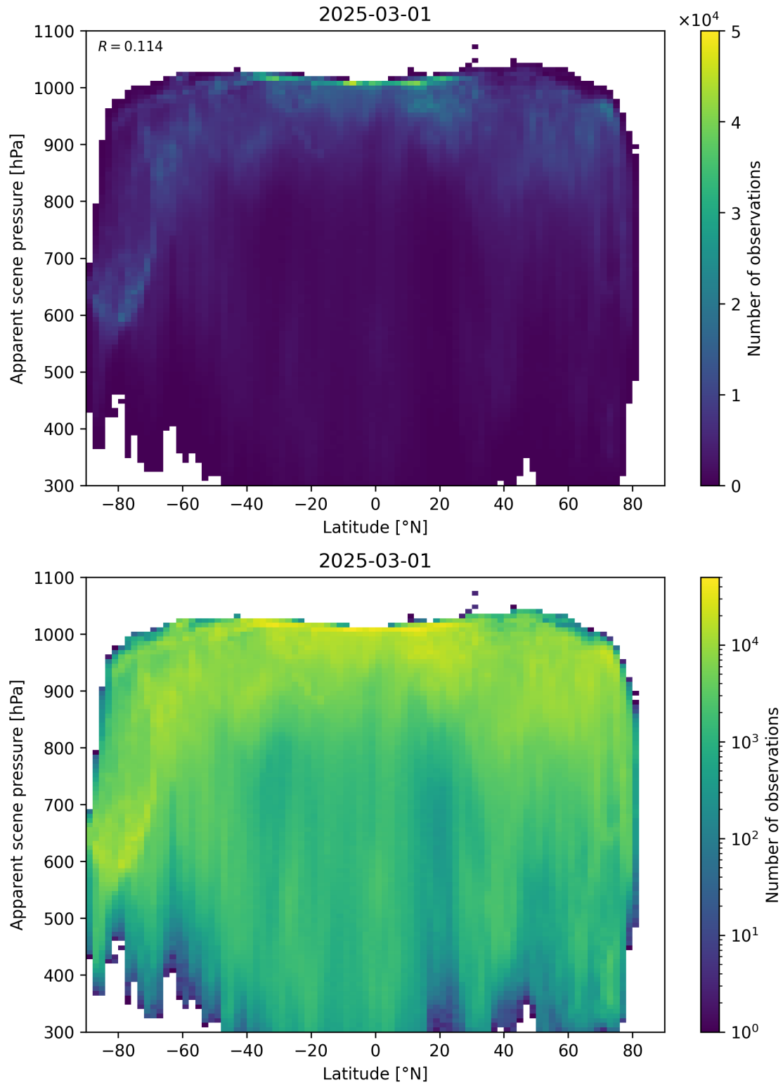
Figure 88: Scatter density plot of “Latitude” against “Apparent scene pressure” for 2025-03-01 to 2025-03-02.
