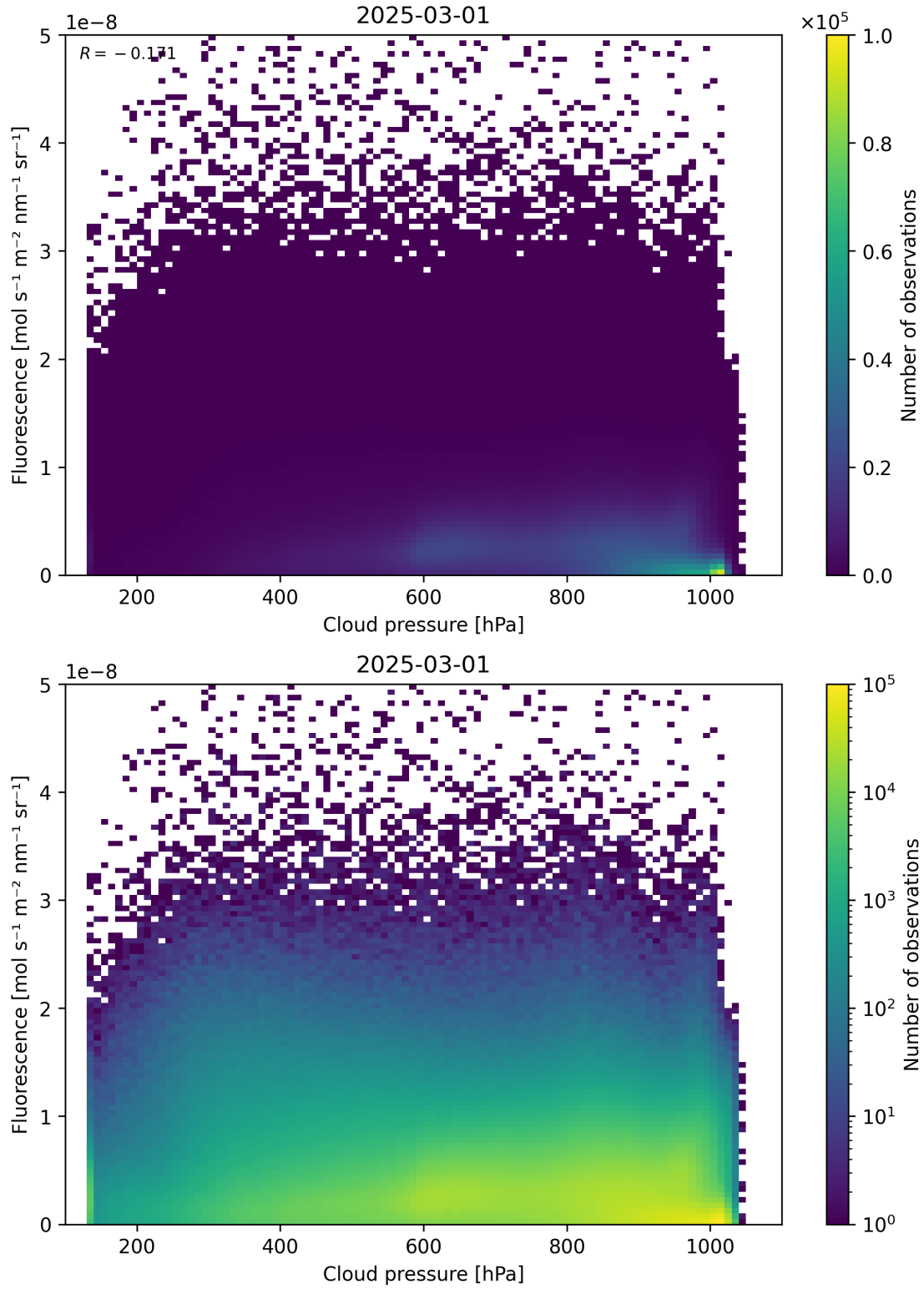
Figure 80: Scatter density plot of “Cloud pressure” against “Fluorescence” for 2025-03-01 to 2025-03-02.
