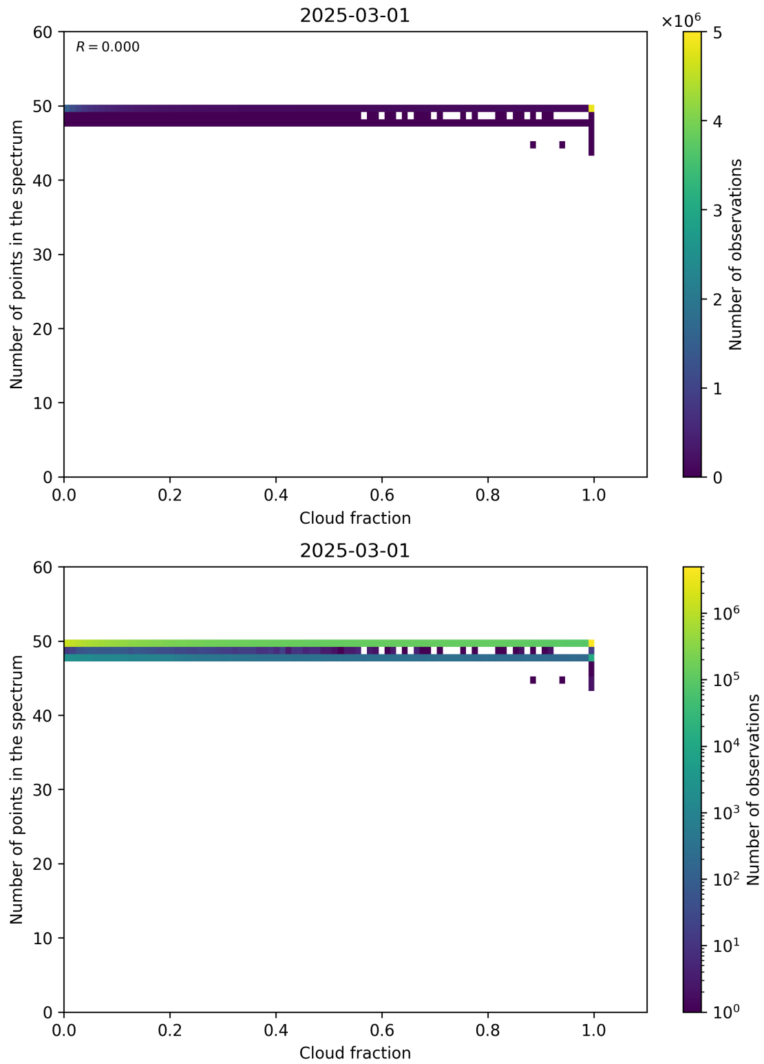
Figure 74: Scatter density plot of “Cloud fraction” against “Number of points in the spectrum” for 2025-03-01 to 2025-03-02.
