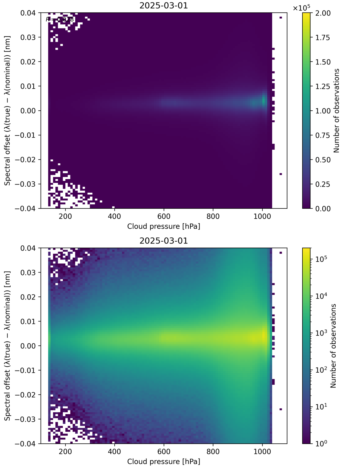
Figure 84: Scatter density plot of “Cloud pressure” against “Spectral offset ( \lambda_{\text{true}} - \lambda_{\text{nominal}} )” for 2025-03-01 to 2025-03-02.
