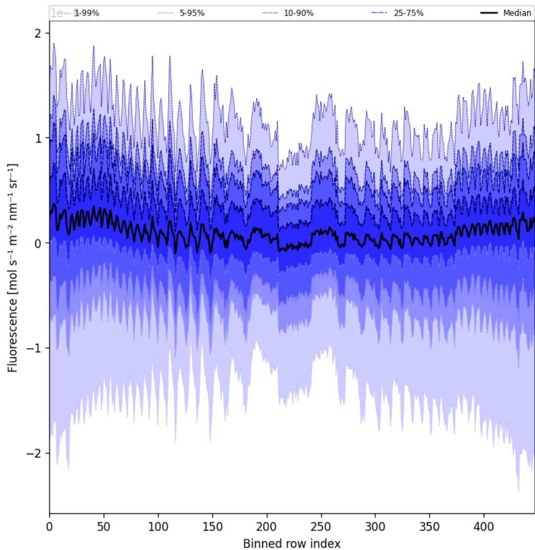
Figure 57: Along track statistics of “Fluorescence” for 2025-03-01 to 2025-03-02
