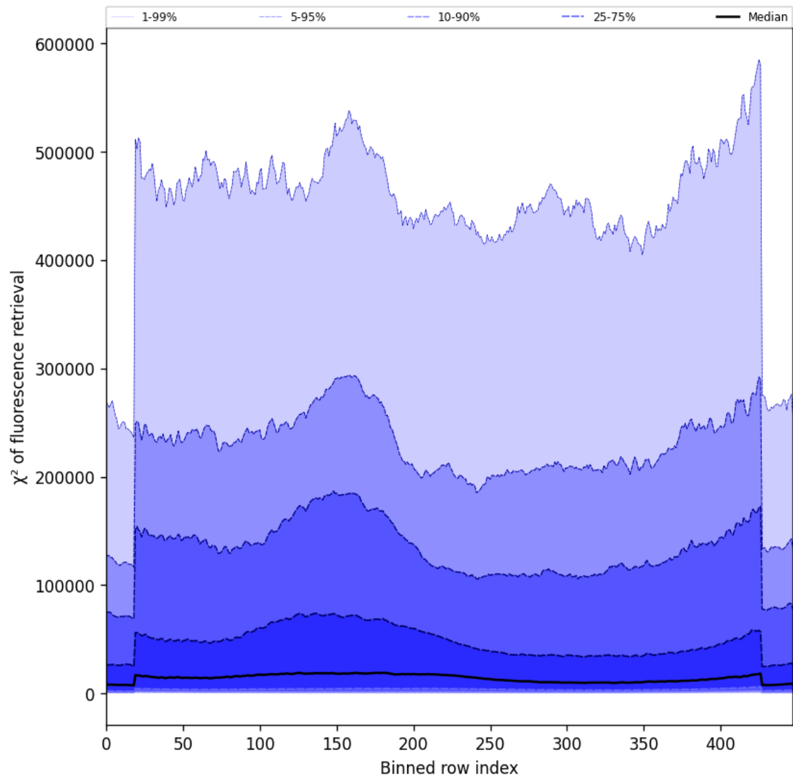
Figure 59: Along track statistics of “ \chi^2 of fluorescence retrieval” for 2025-03-01 to 2025-03-02
