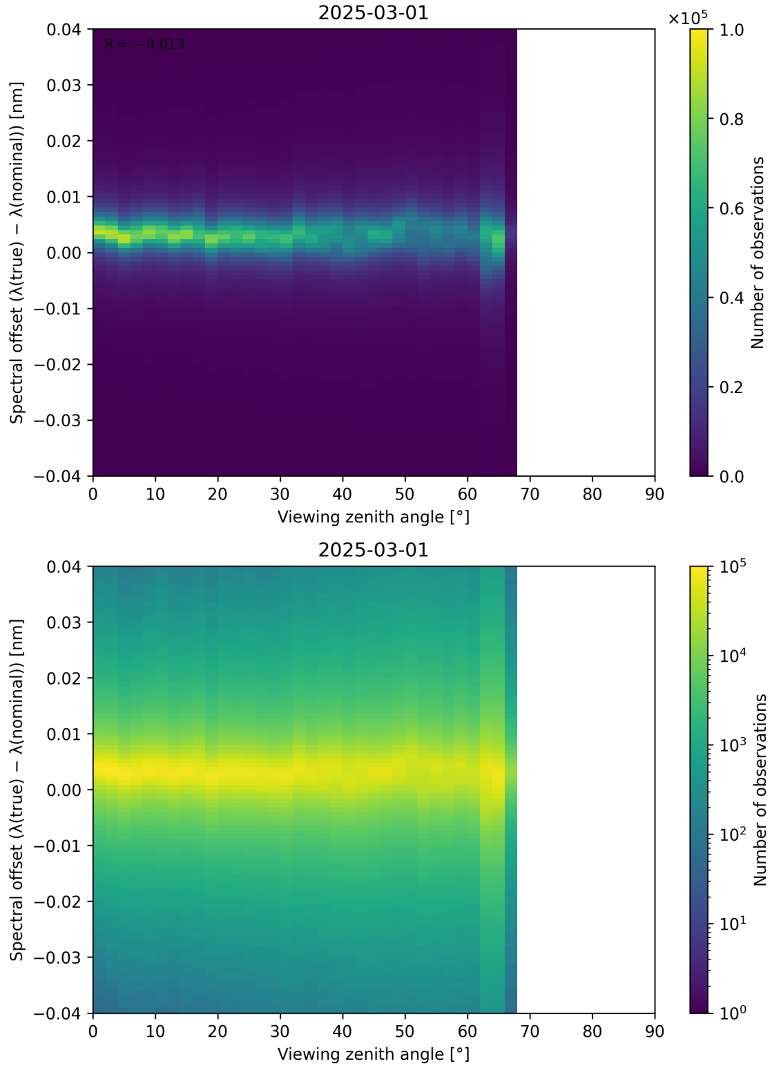
Figure 128: Scatter density plot of “Viewing zenith angle” against “Spectral offset ( \lambda_{\text{true}} - \lambda_{\text{nominal}} )” for 2025-03-01 to 2025-03-02.
