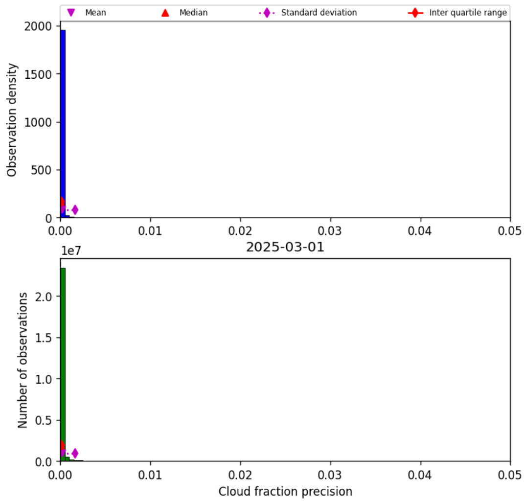
Figure 33: Histogram of “Cloud fraction precision” for 2025-03-01 to 2025-03-02
