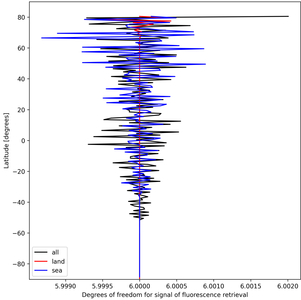
Figure 26: Zonal average of “Degrees of freedom for signal of fluorescence retrieval” for 2025-03-01 to 2025-03-02.
