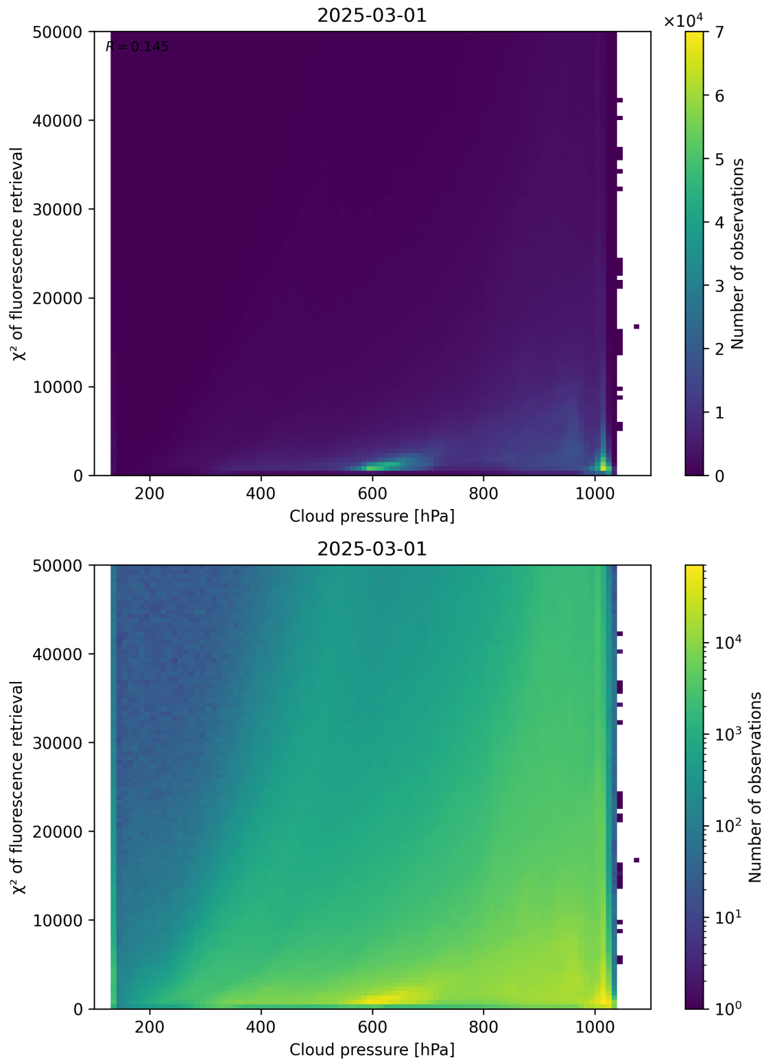
Figure 78: Scatter density plot of “Cloud pressure” against “ \chi^2 of fluorescence retrieval” for 2025-03-01 to 2025-03-02.
