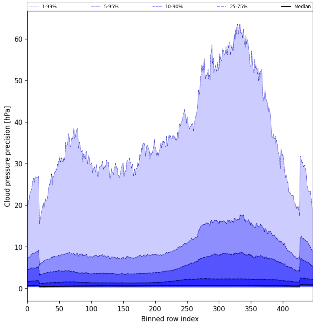
Figure 48: Along track statistics of “Cloud pressure precision” for 2025-03-01 to 2025-03-02
