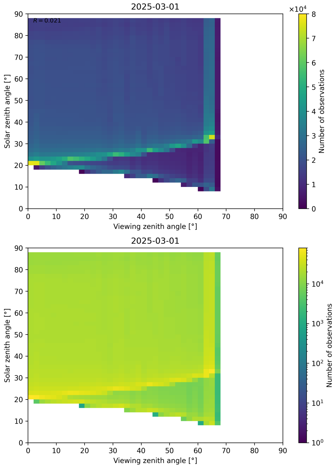
Figure 127: Scatter density plot of “Viewing zenith angle” against “Solar zenith angle” for 2025-03-01 to 2025-03-02.
