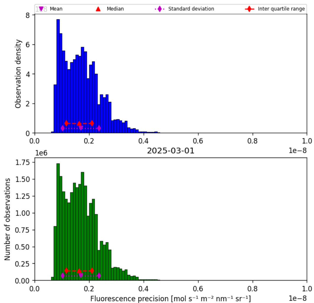
Figure 41: Histogram of “Fluorescence precision” for 2025-03-01 to 2025-03-02
