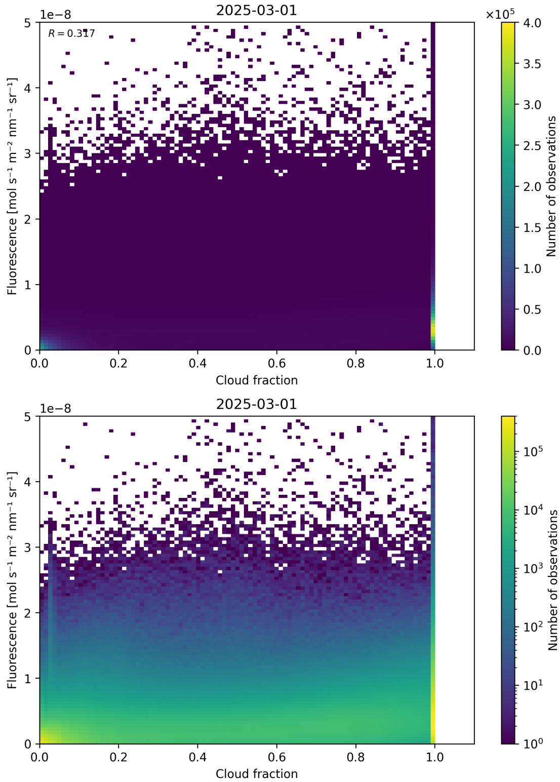
Figure 72: Scatter density plot of “Cloud fraction” against “Fluorescence” for 2025-03-01 to 2025-03-02.
