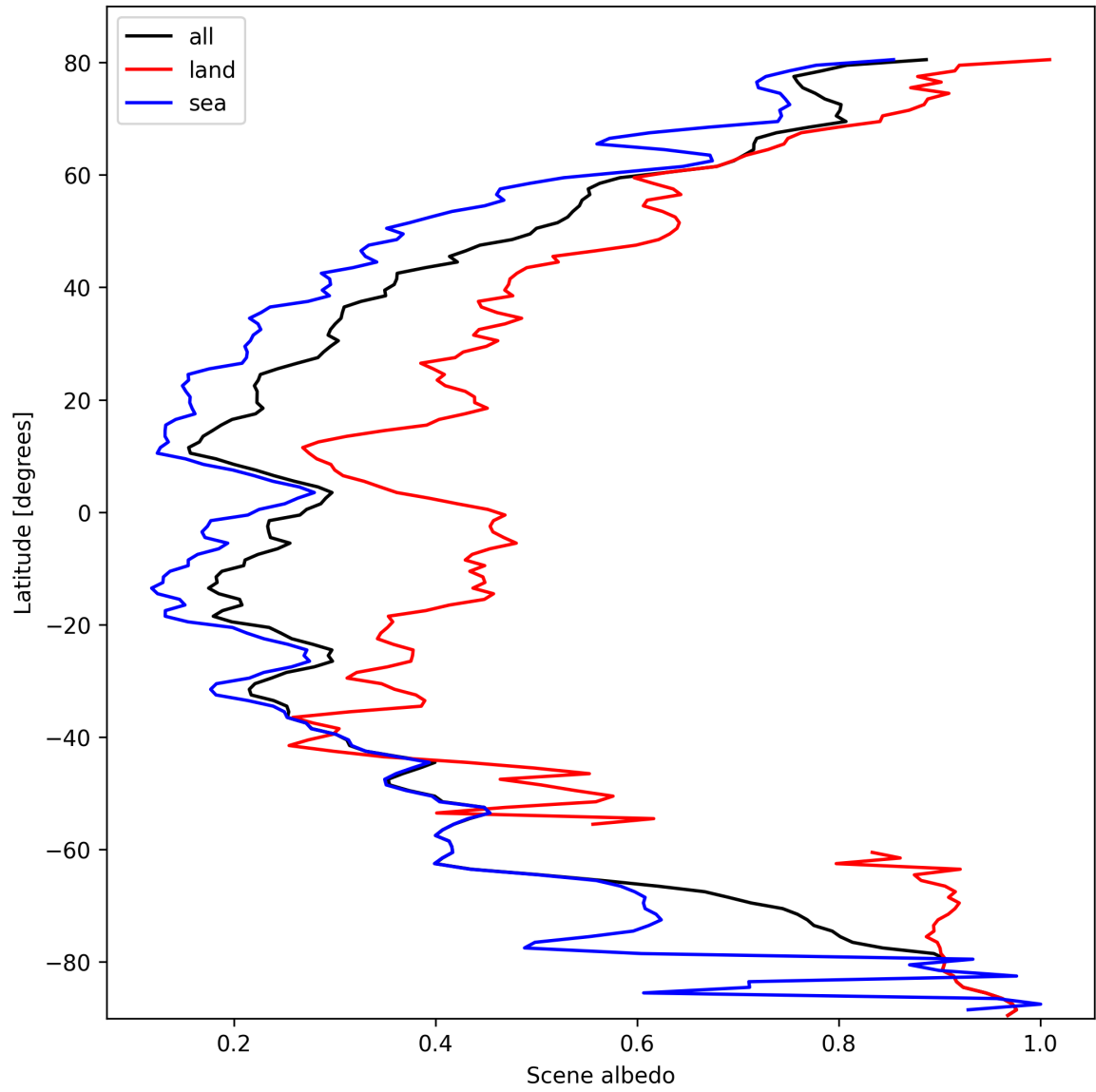
Figure 17: Zonal average of “Scene albedo” for 2025-03-01 to 2025-03-02.
