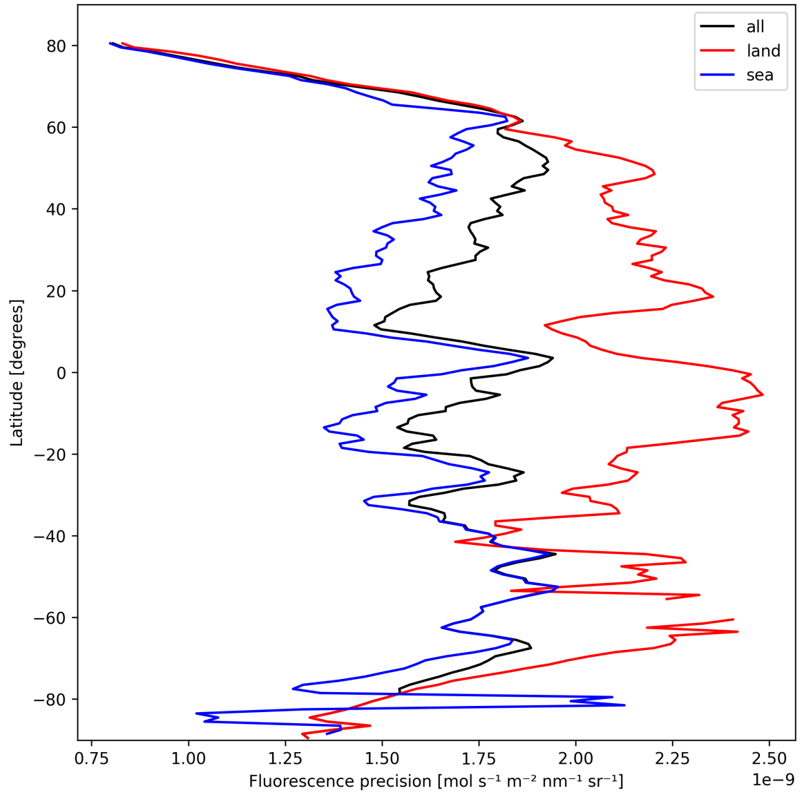
Figure 24: Zonal average of “Fluorescence precision” for 2025-03-01 to 2025-03-02.
