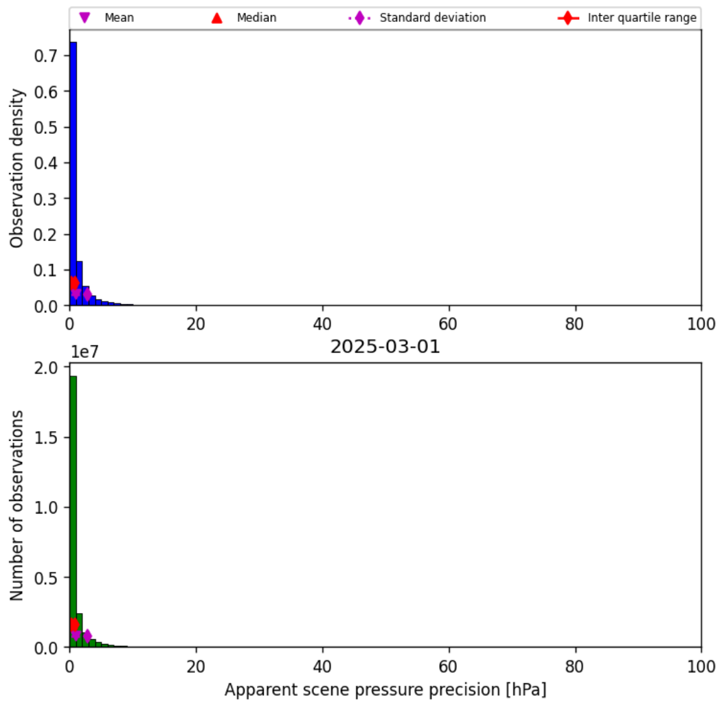
Figure 37: Histogram of “Apparent scene pressure precision” for 2025-03-01 to 2025-03-02
