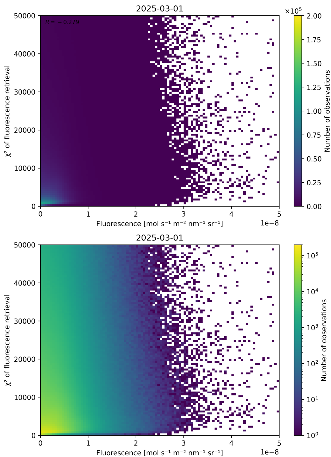
Figure 85: Scatter density plot of “Fluorescence” against “ \chi^2 of fluorescence retrieval” for 2025-03-01 to 2025-03-02.
