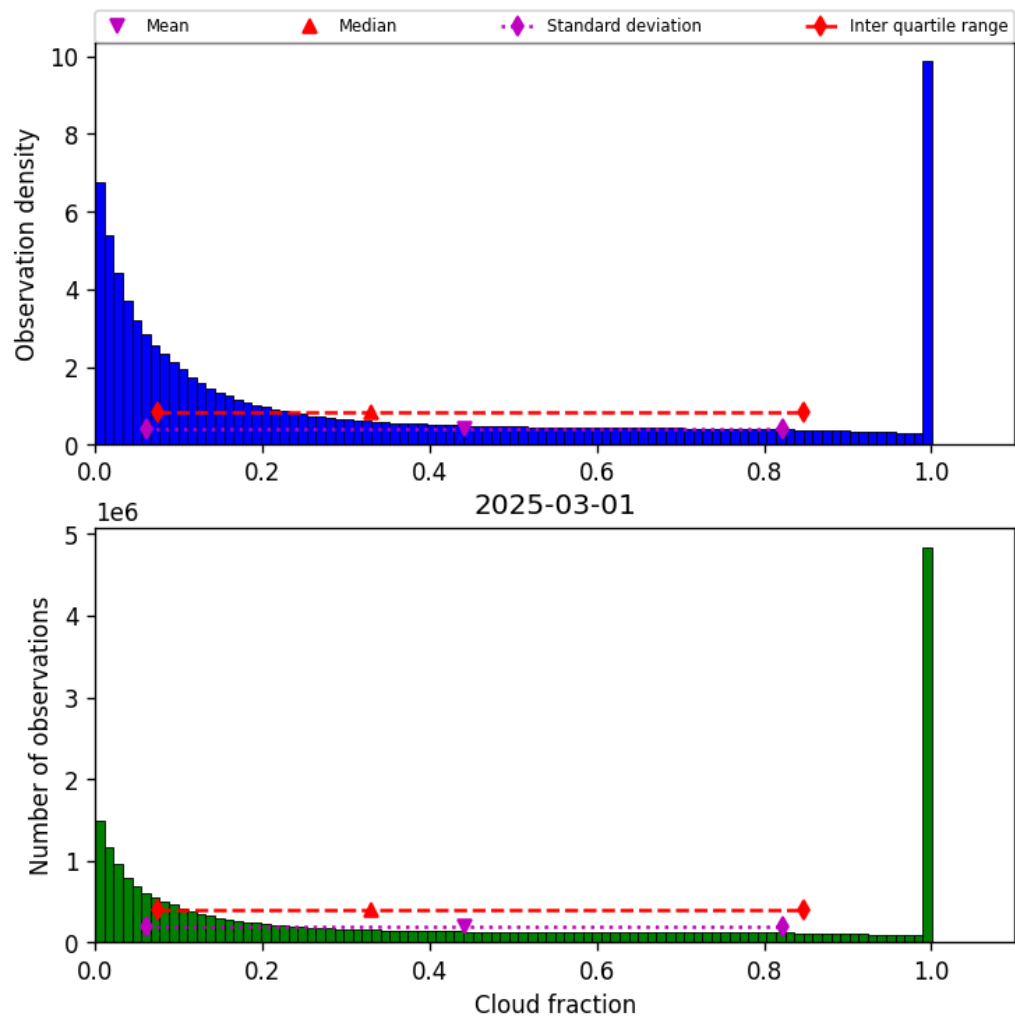
Figure 32: Histogram of “Cloud fraction” for 2025-03-01 to 2025-03-02
