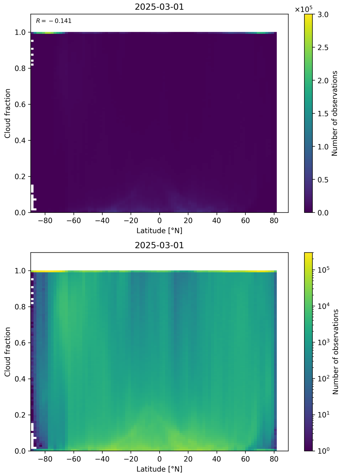
Figure 90: Scatter density plot of “Latitude” against “Cloud fraction” for 2025-03-01 to 2025-03-02.
