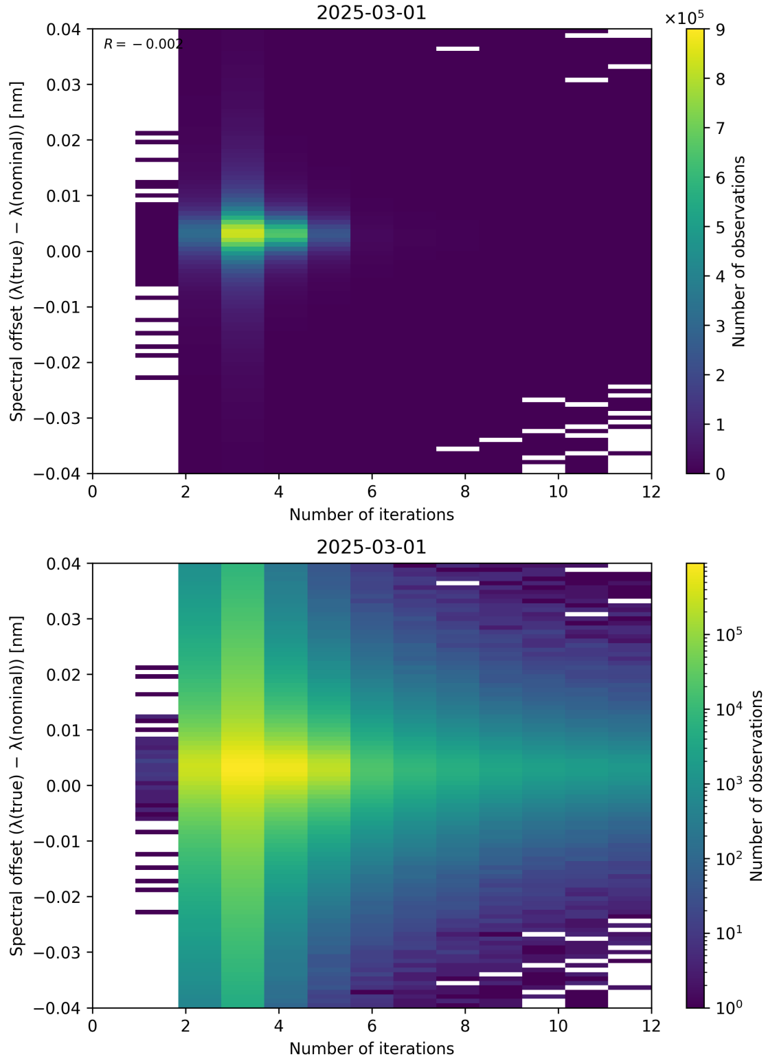
Figure 100: Scatter density plot of “Number of iterations” against “Spectral offset ( \lambda_{\text{true}} - \lambda_{\text{nominal}} )” for 2025-03-01 to 2025-03-02.
