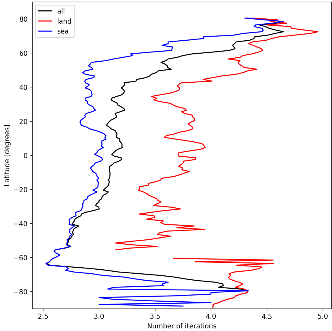
Figure 22: Zonal average of “Number of iterations” for 2025-03-01 to 2025-03-02.
