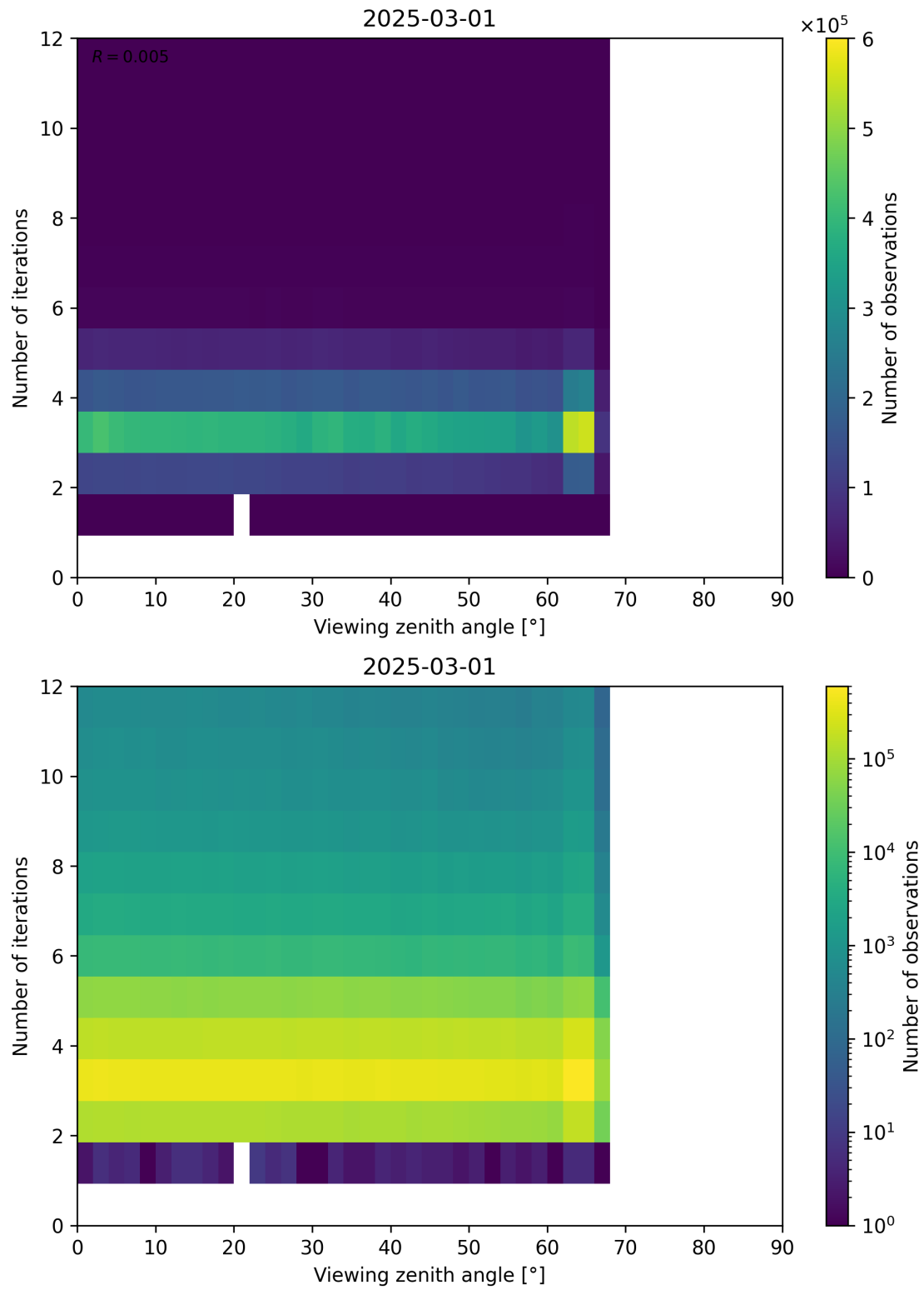
Figure 124: Scatter density plot of “Viewing zenith angle” against “Number of iterations” for 2025-03-01 to 2025-03-02.
