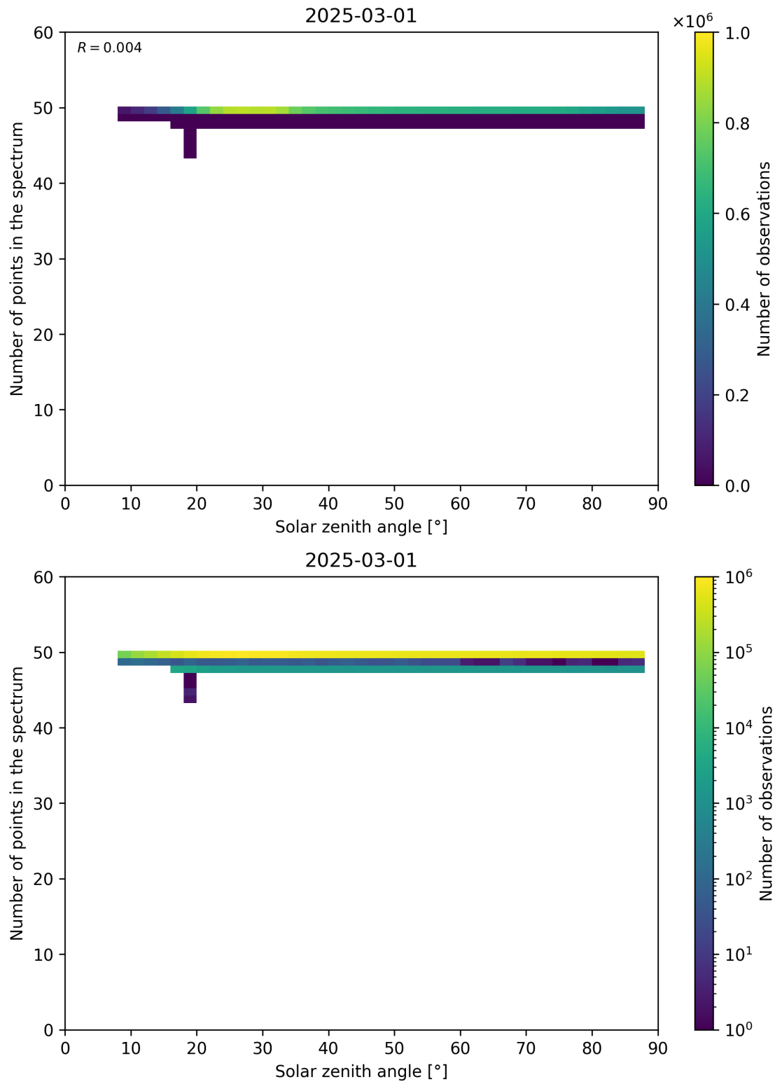
Figure 115: Scatter density plot of “Solar zenith angle” against “Number of points in the spectrum” for 2025-03-01 to 2025-03-02.
