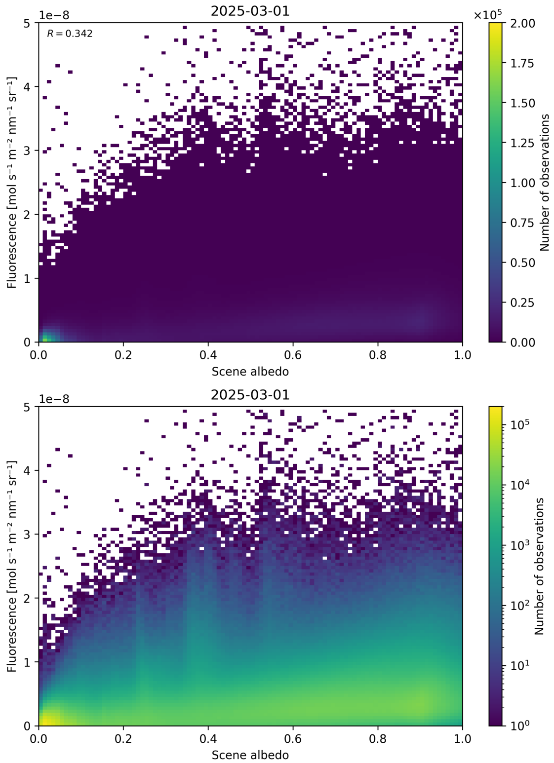
Figure 104: Scatter density plot of “Scene albedo” against “Fluorescence” for 2025-03-01 to 2025-03-02.
