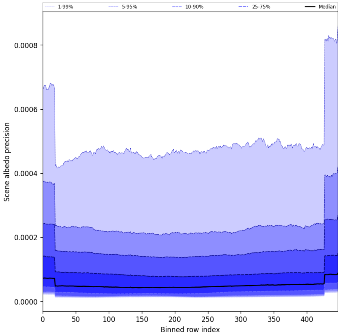
Figure 52: Along track statistics of “Scene albedo precision” for 2025-03-01 to 2025-03-02
