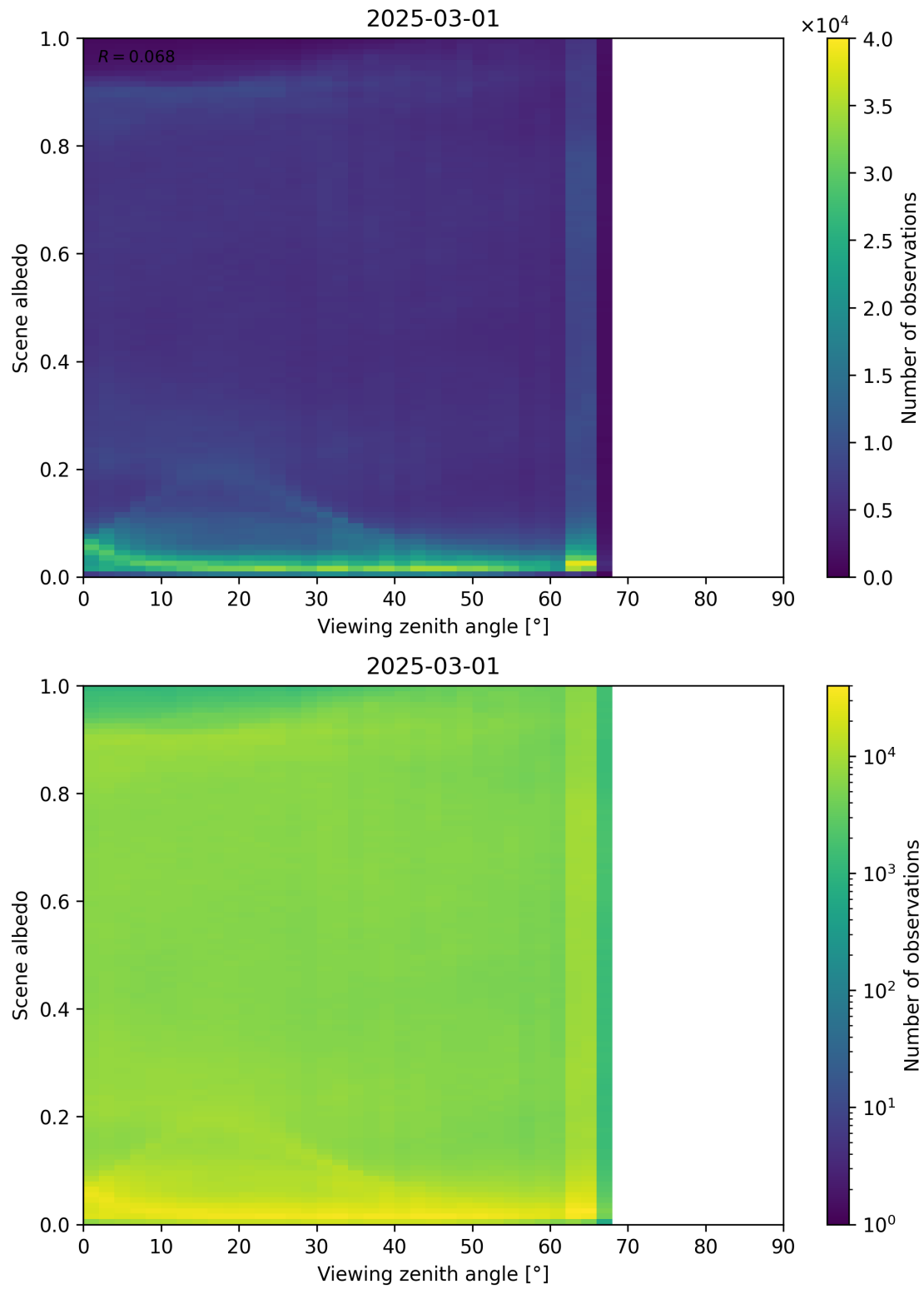
Figure 126: Scatter density plot of “Viewing zenith angle” against “Scene albedo” for 2025-03-01 to 2025-03-02.
