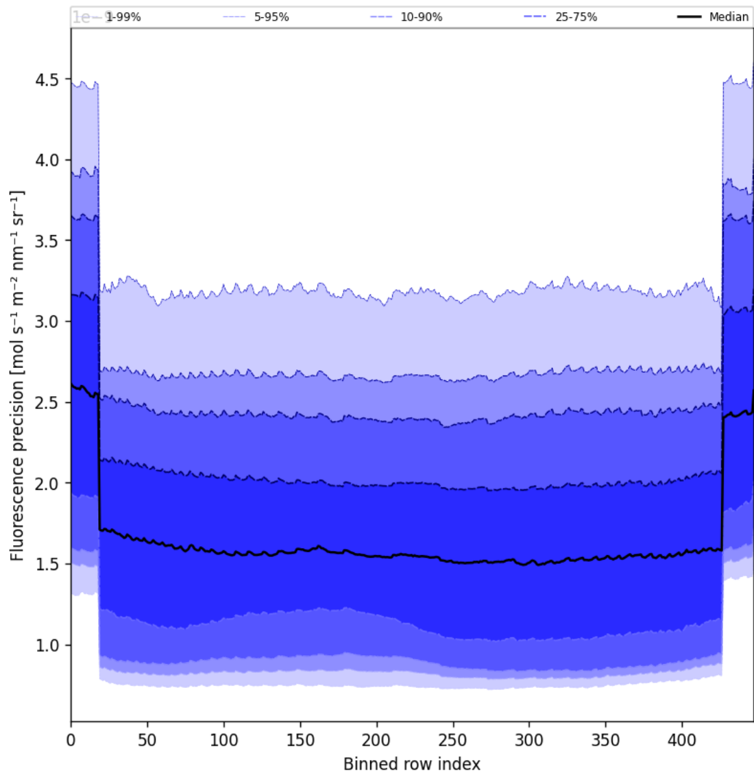
Figure 58: Along track statistics of “Fluorescence precision” for 2025-03-01 to 2025-03-02
