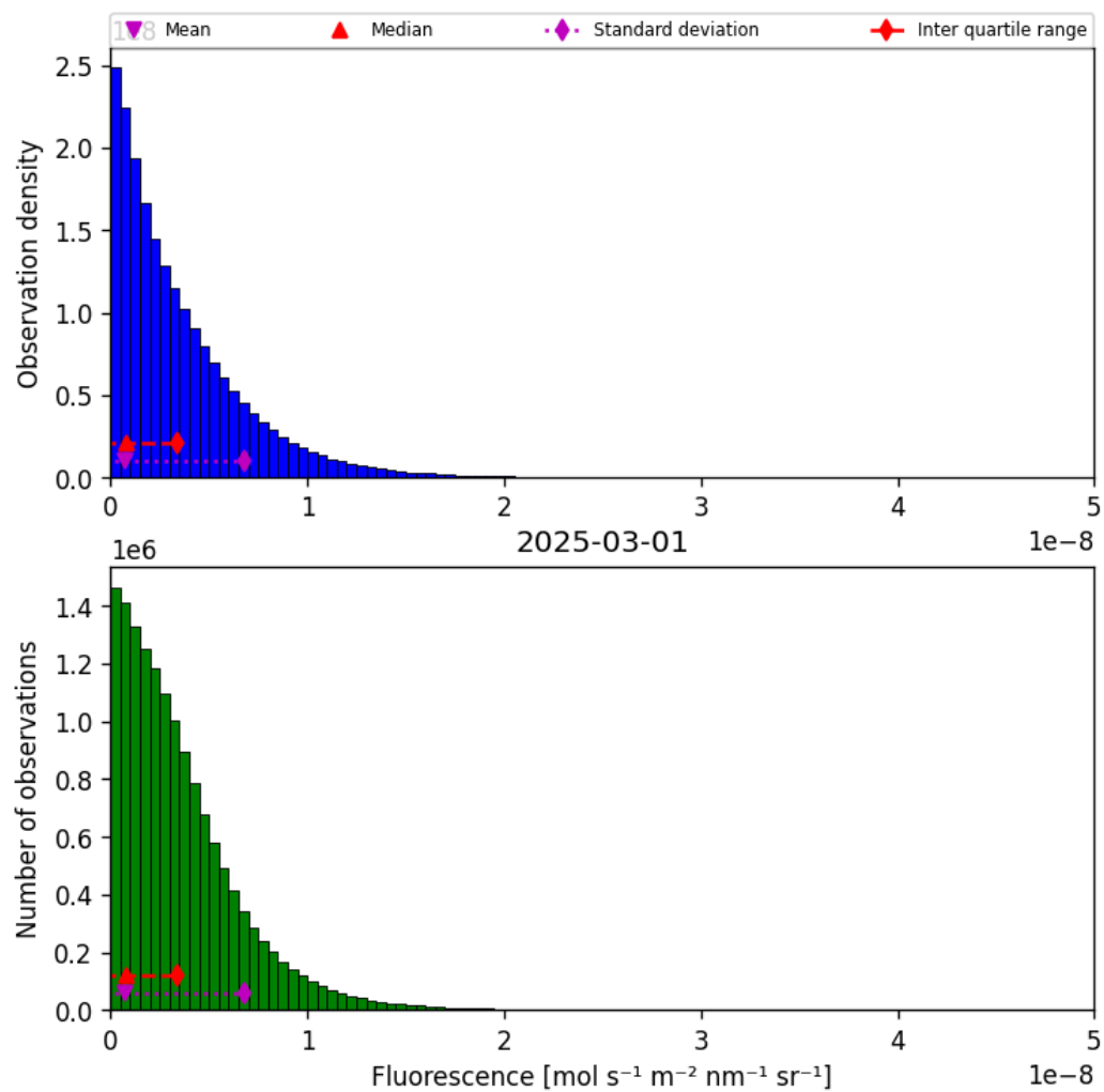
Figure 40: Histogram of “Fluorescence” for 2025-03-01 to 2025-03-02
