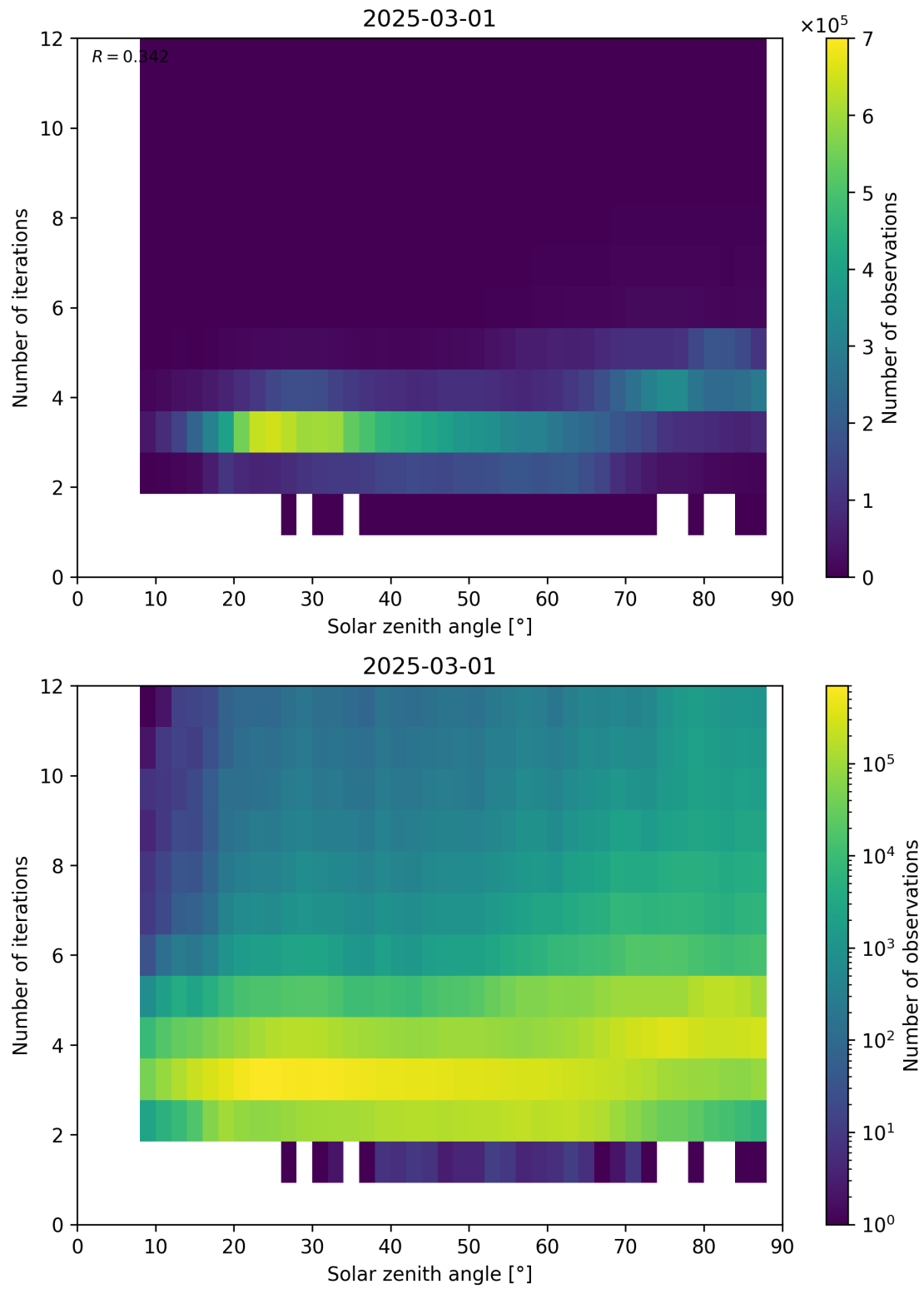
Figure 114: Scatter density plot of “Solar zenith angle” against “Number of iterations” for 2025-03-01 to 2025-03-02.
