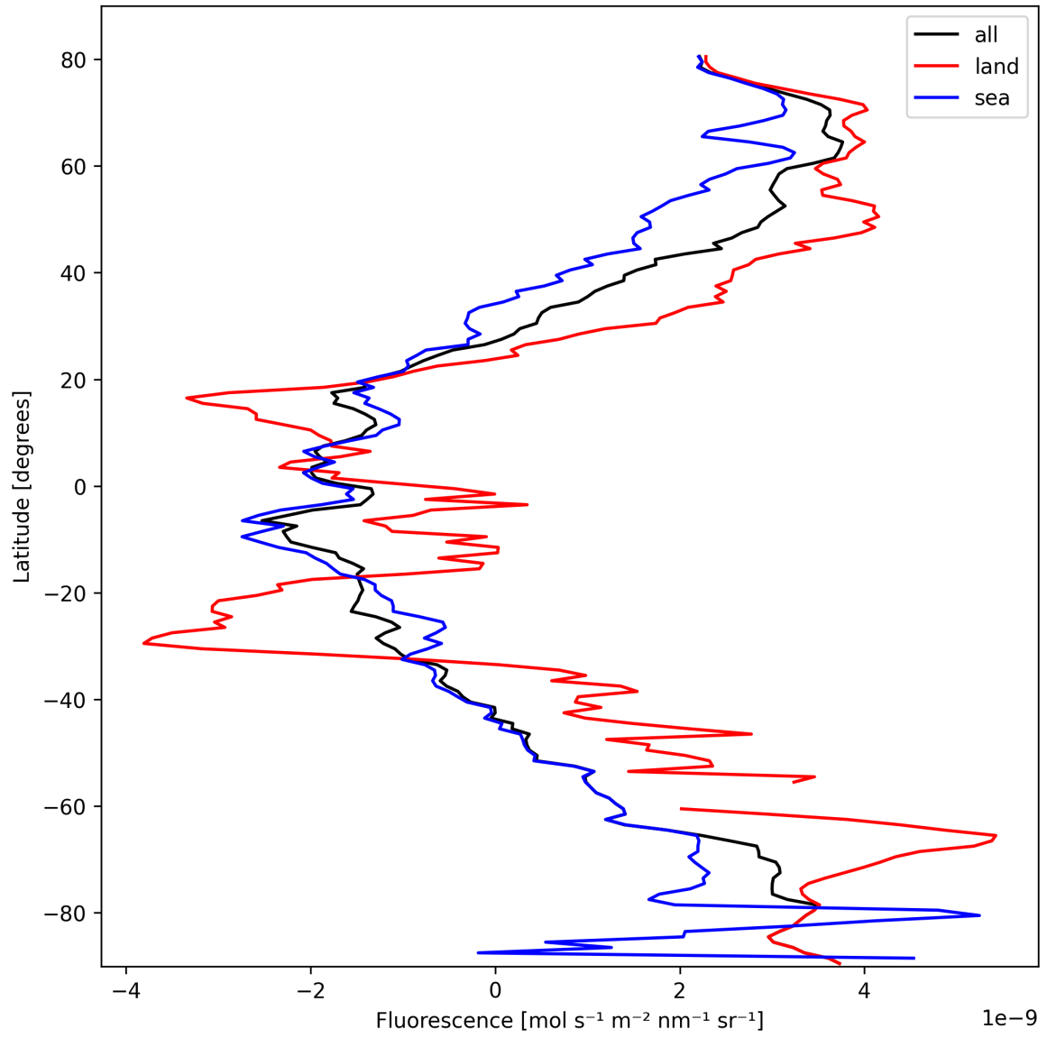
Figure 23: Zonal average of “Fluorescence” for 2025-03-01 to 2025-03-02.
