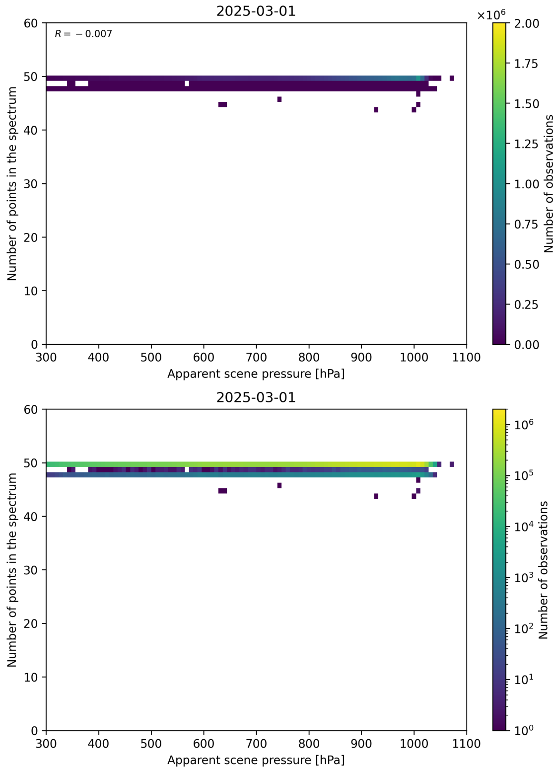
Figure 66: Scatter density plot of “Apparent scene pressure” against “Number of points in the spectrum” for 2025-03-01 to 2025-03-02.
