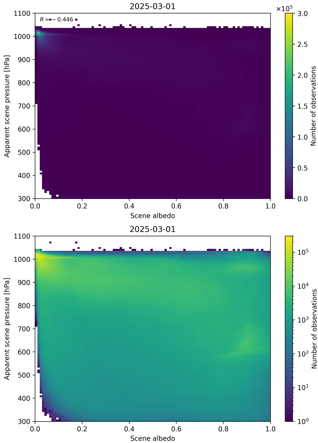
Figure 102: Scatter density plot of “Scene albedo” against “Apparent scene pressure” for 2025-03-01 to 2025-03-02.
