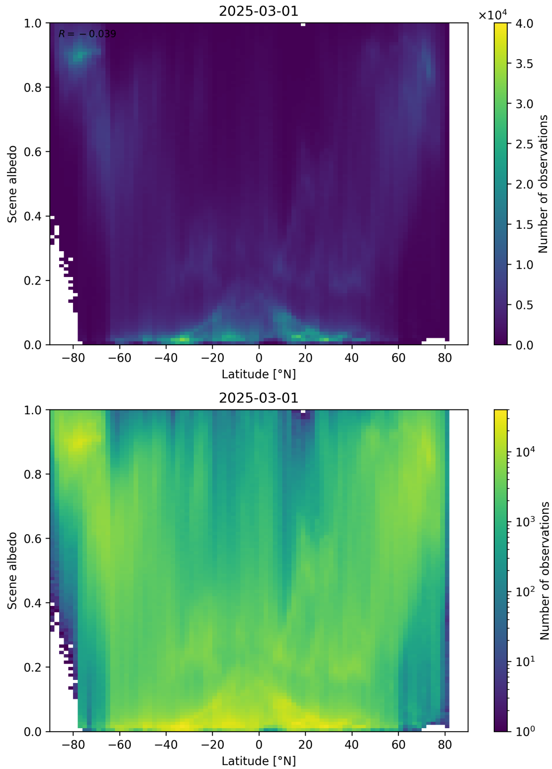
Figure 95: Scatter density plot of “Latitude” against “Scene albedo” for 2025-03-01 to 2025-03-02.
