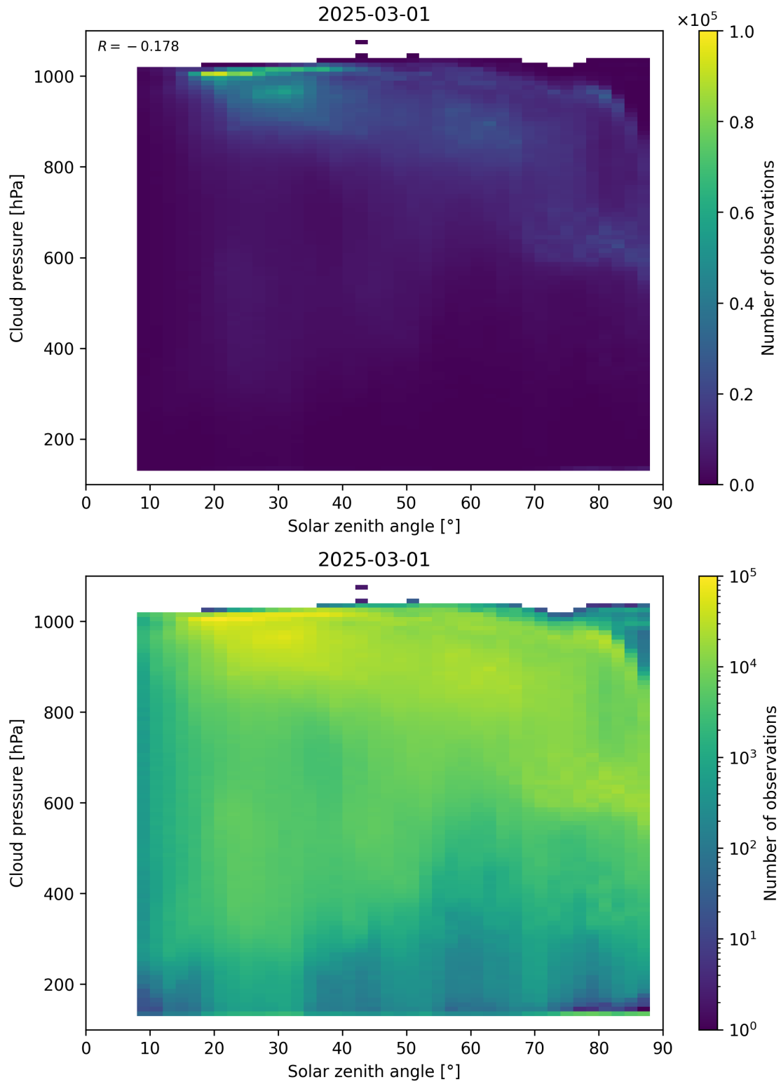
Figure 111: Scatter density plot of “Solar zenith angle” against “Cloud pressure” for 2025-03-01 to 2025-03-02.
