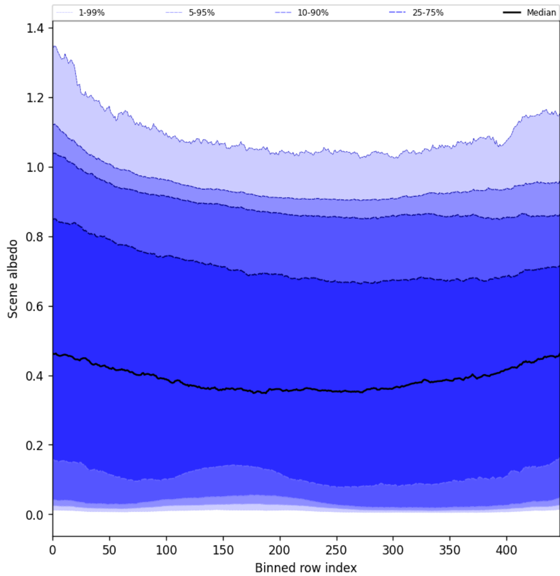
Figure 51: Along track statistics of “Scene albedo” for 2025-03-01 to 2025-03-02
