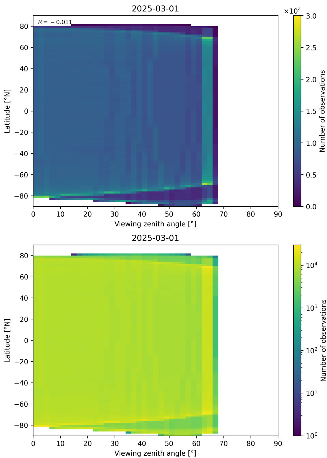
Figure 123: Scatter density plot of “Viewing zenith angle” against “Latitude” for 2025-03-01 to 2025-03-02.
