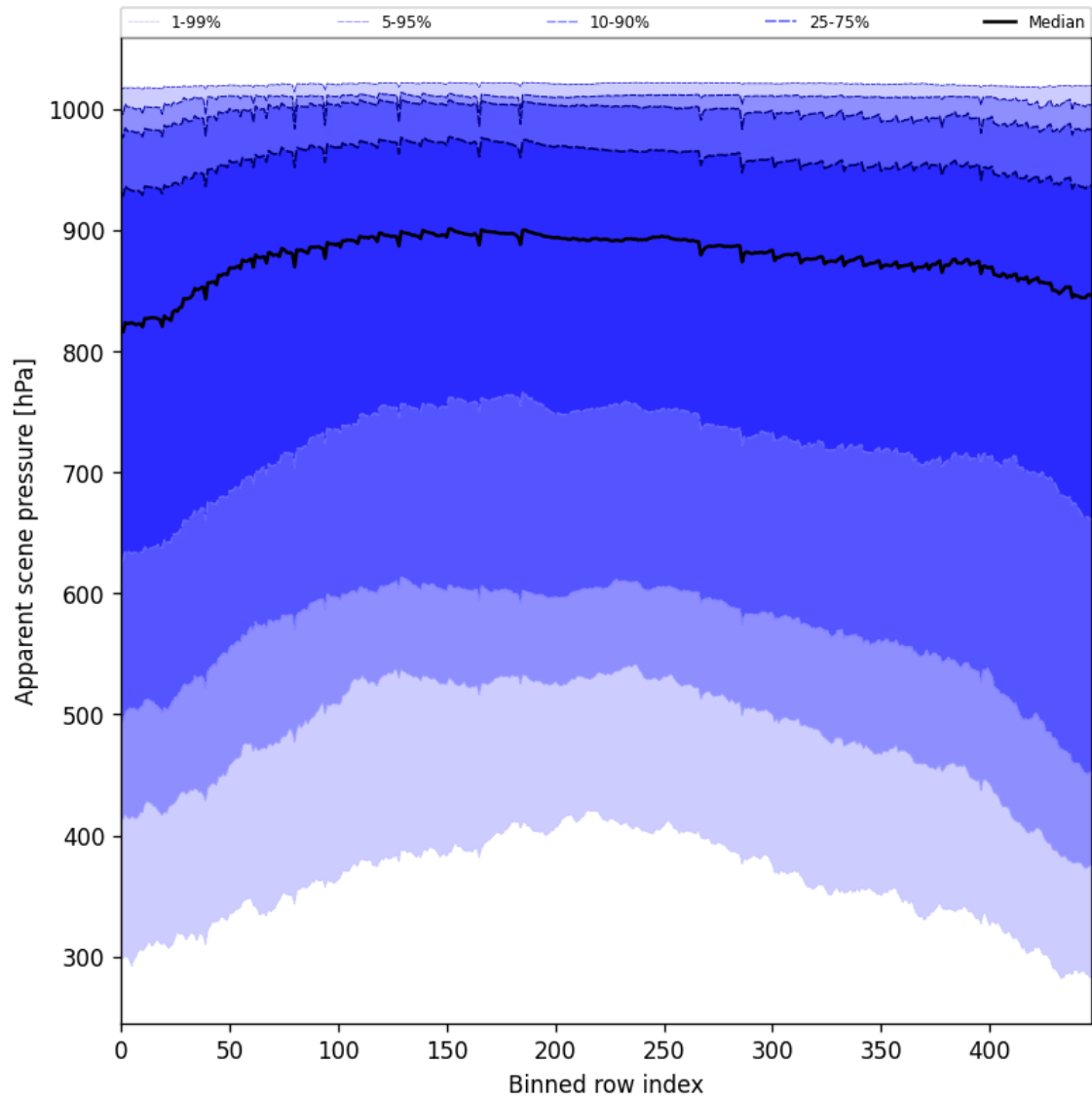
Figure 53: Along track statistics of “Apparent scene pressure” for 2025-03-01 to 2025-03-02
