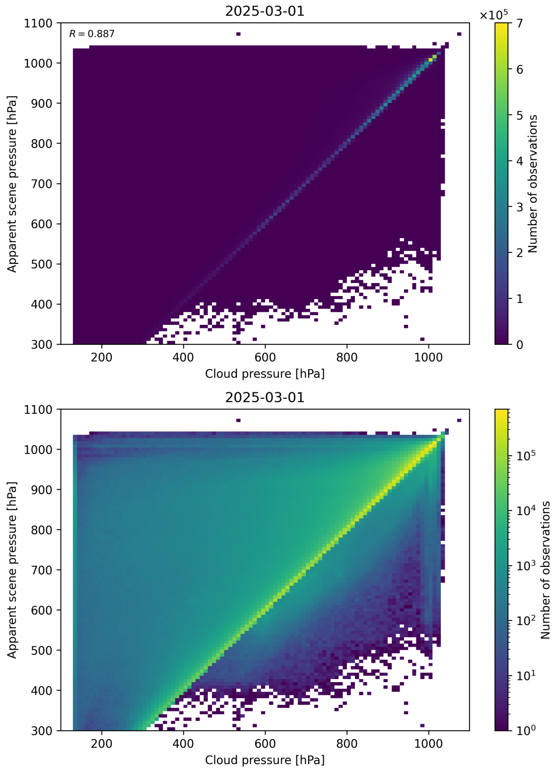
Figure 77: Scatter density plot of “Cloud pressure” against “Apparent scene pressure” for 2025-03-01 to 2025-03-02.
