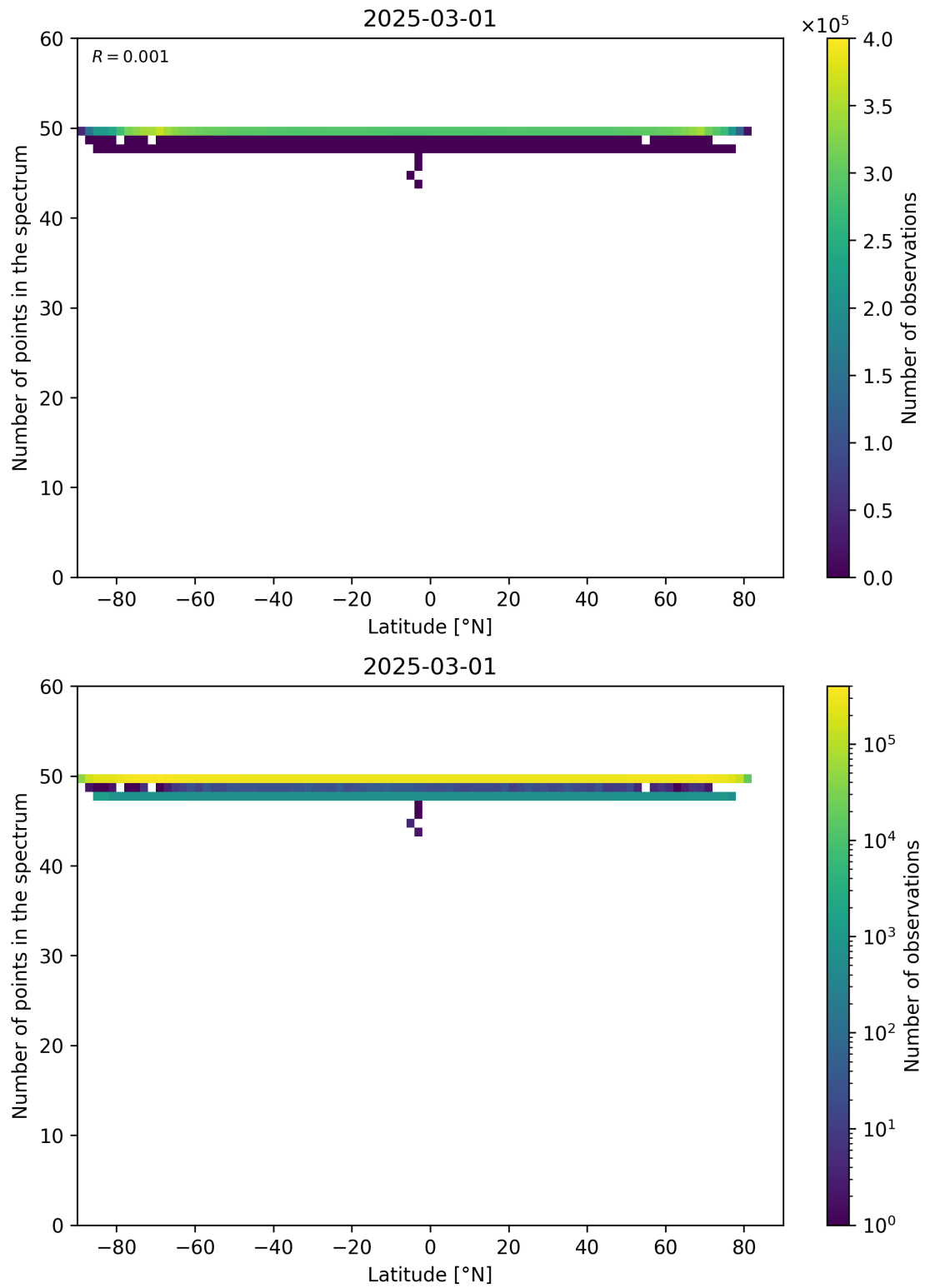
Figure 94: Scatter density plot of “Latitude” against “Number of points in the spectrum” for 2025-03-01 to 2025-03-02.
