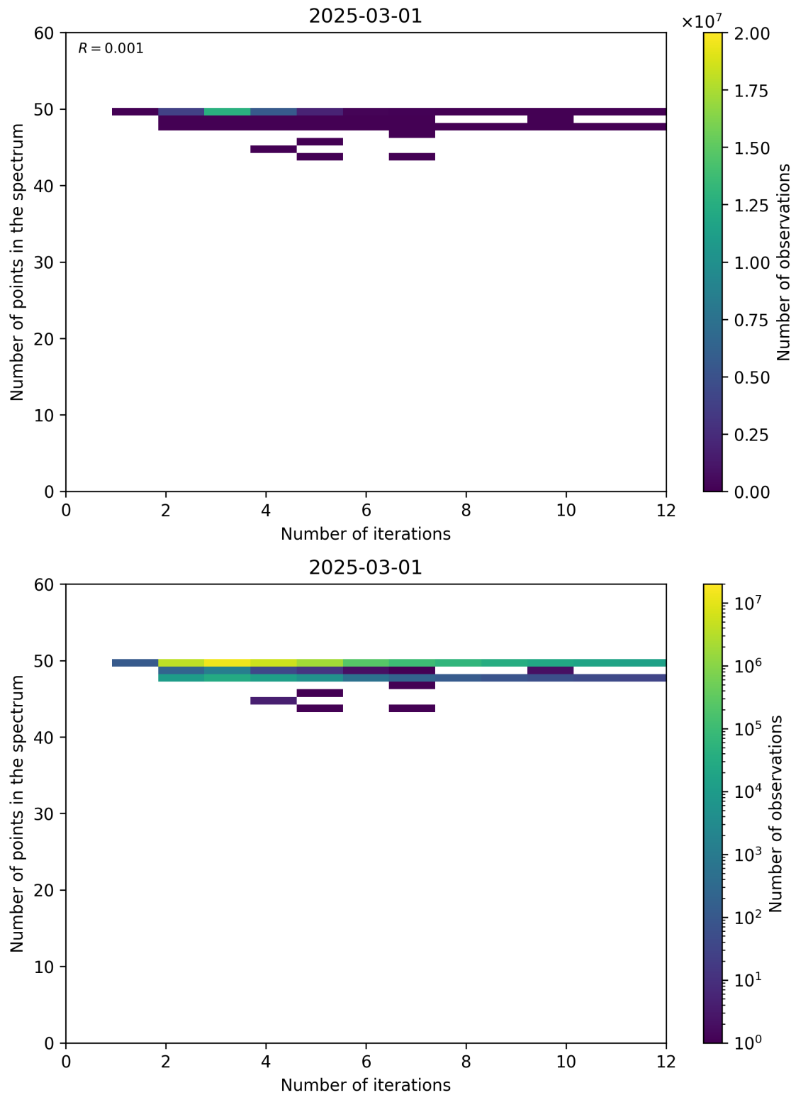
Figure 99: Scatter density plot of “Number of iterations” against “Number of points in the spectrum” for 2025-03-01 to 2025-03-02.
