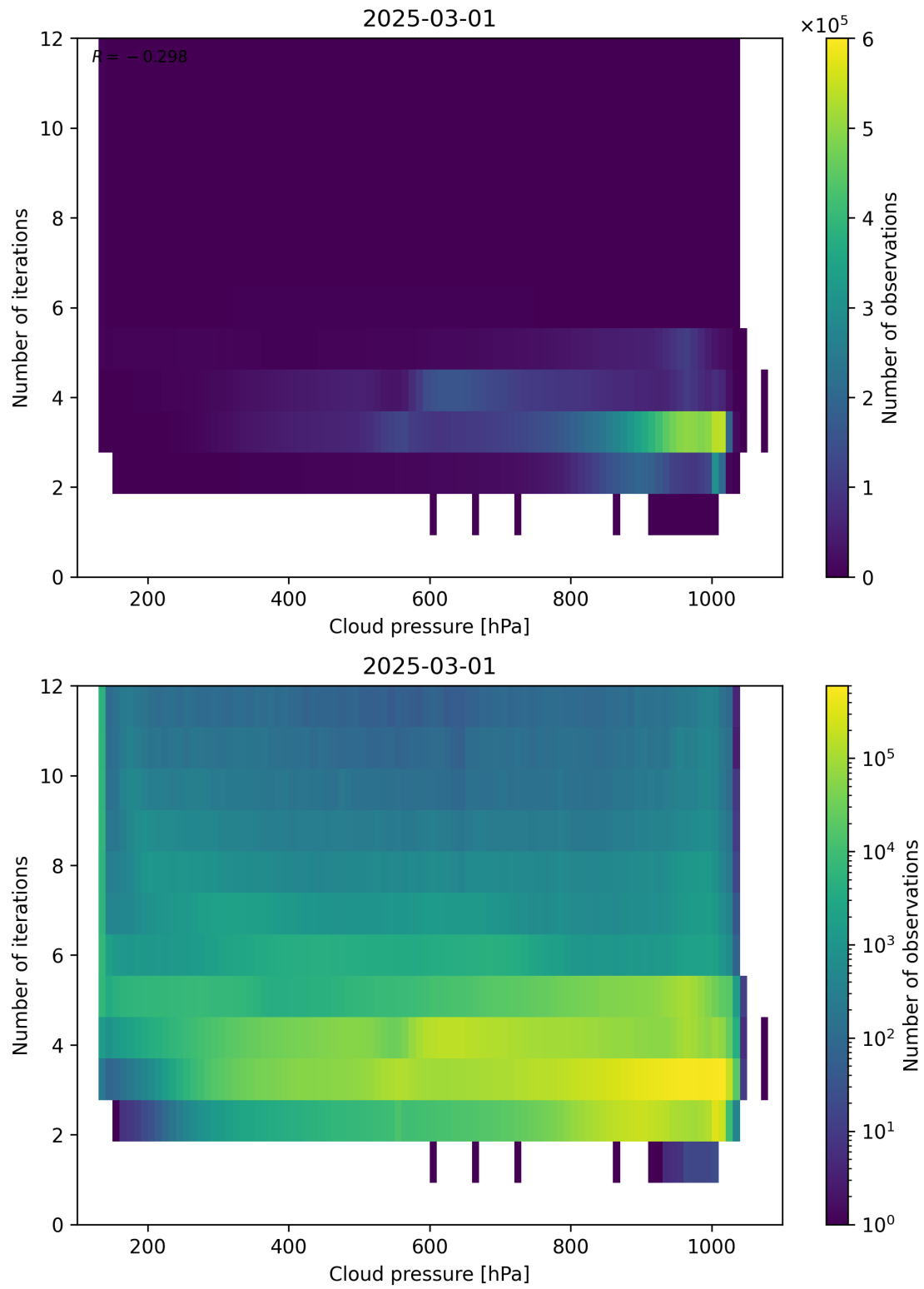
Figure 81: Scatter density plot of “Cloud pressure” against “Number of iterations” for 2025-03-01 to 2025-03-02.
