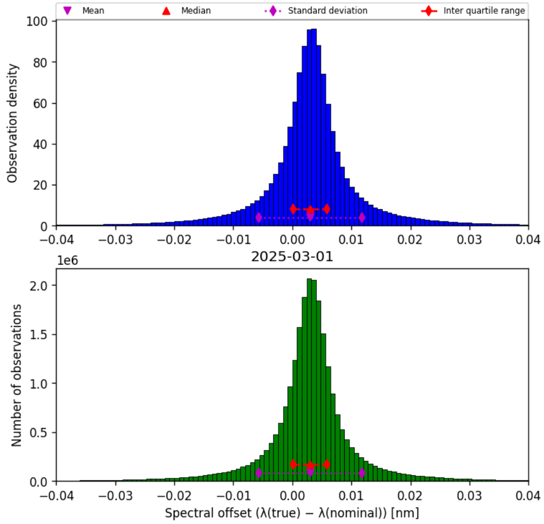
Figure 45: Histogram of “Spectral offset ( \lambda_{\text{true}} - \lambda_{\text{nominal}} )” for 2025-03-01 to 2025-03-02
