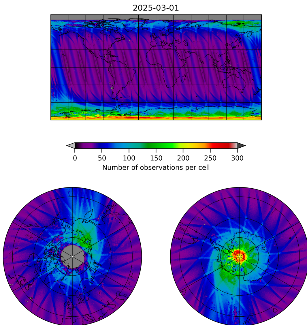
Figure 11: Map of the number of observations for 2025-03-01 to 2025-03-02
