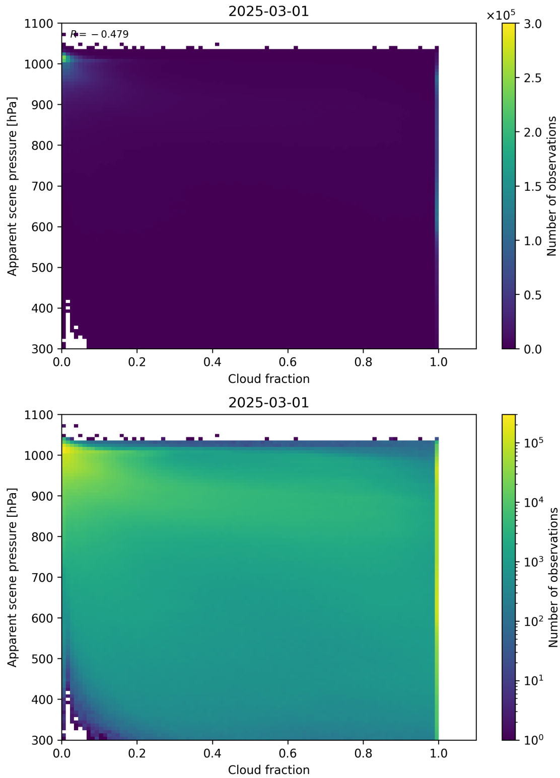
Figure 70: Scatter density plot of “Cloud fraction” against “Apparent scene pressure” for 2025-03-01 to 2025-03-02.
