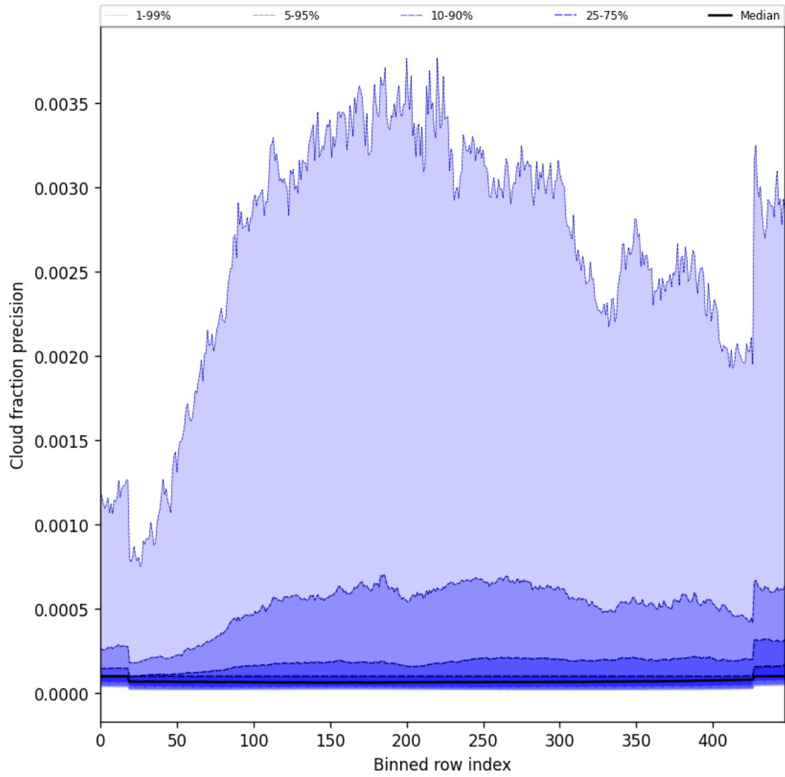
Figure 50: Along track statistics of “Cloud fraction precision” for 2025-03-01 to 2025-03-02
