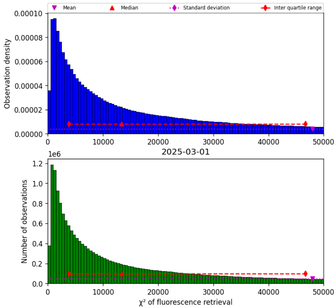
Figure 42: Histogram of “ \chi^2 of fluorescence retrieval” for 2025-03-01 to 2025-03-02
