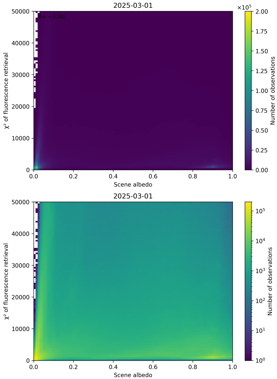
Figure 103: Scatter density plot of “Scene albedo” against “ \chi^2 of fluorescence retrieval” for 2025-03-01 to 2025-03-02.
