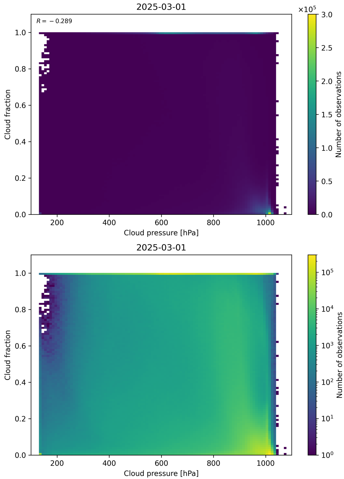
Figure 79: Scatter density plot of “Cloud pressure” against “Cloud fraction” for 2025-03-01 to 2025-03-02.
