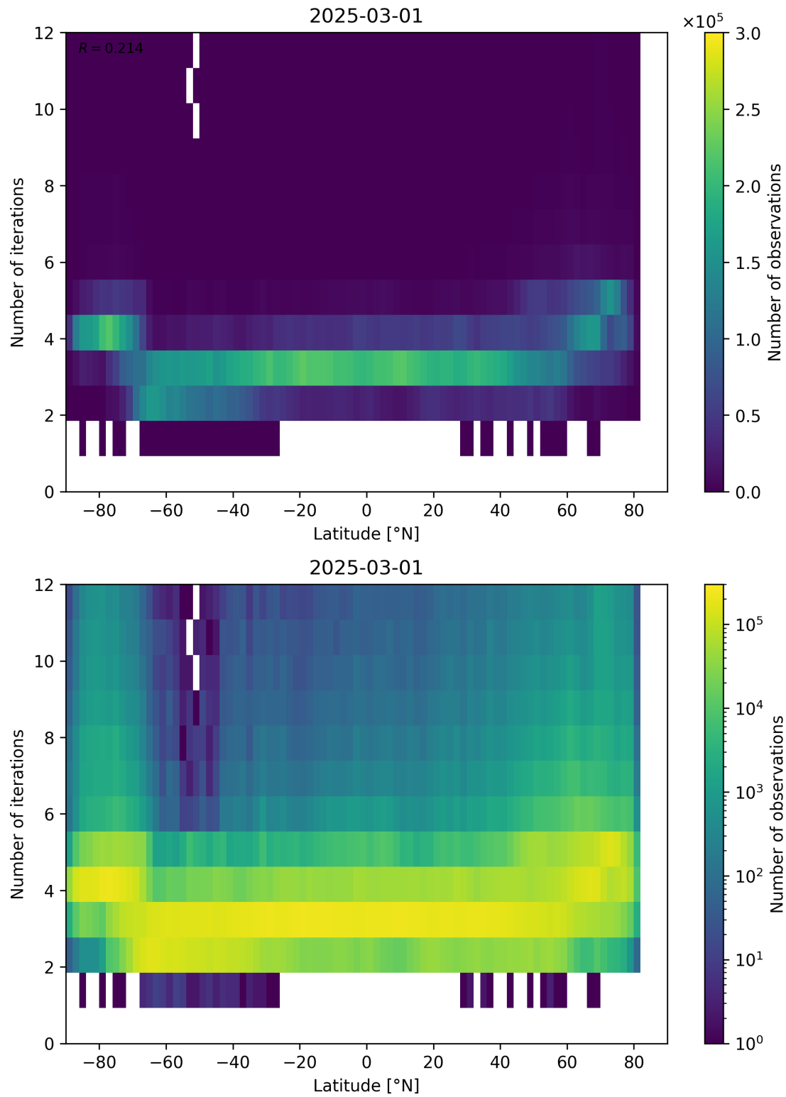
Figure 93: Scatter density plot of “Latitude” against “Number of iterations” for 2025-03-01 to 2025-03-02.
