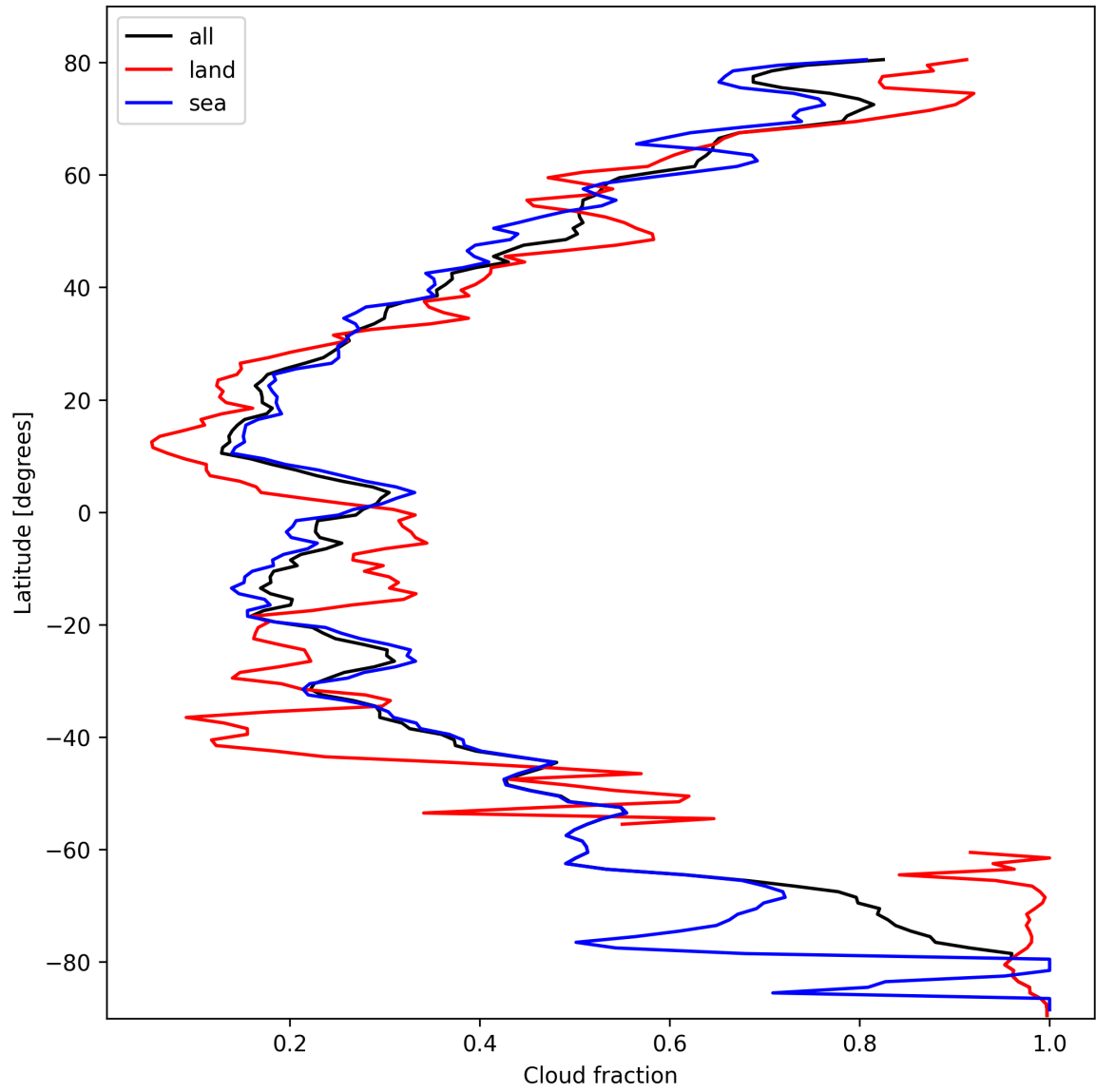
Figure 15: Zonal average of “Cloud fraction” for 2025-03-01 to 2025-03-02.
