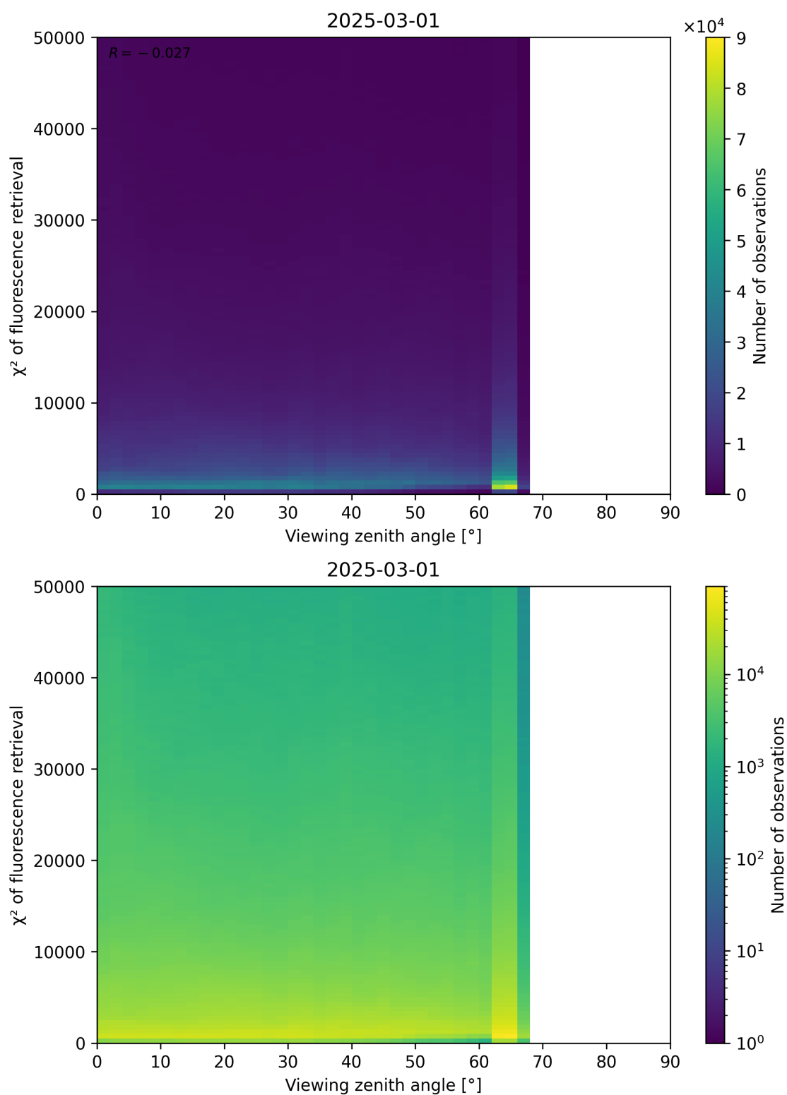
Figure 119: Scatter density plot of “Viewing zenith angle” against “ \chi^2 of fluorescence retrieval” for 2025-03-01 to 2025-03-02.
