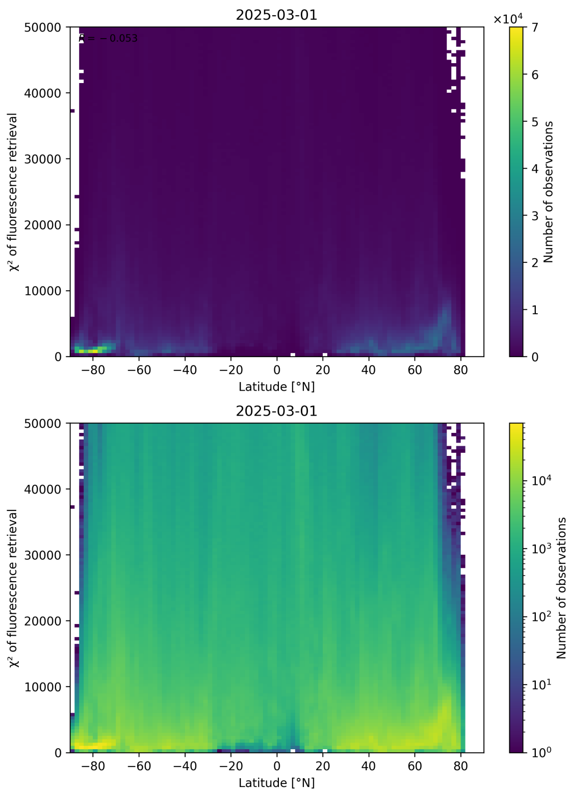
Figure 89: Scatter density plot of “Latitude” against “ \chi^2 of fluorescence retrieval” for 2025-03-01 to 2025-03-02.
