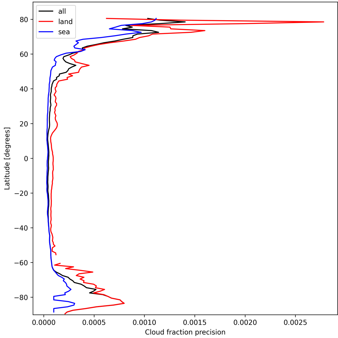
Figure 16: Zonal average of “Cloud fraction precision” for 2025-03-01 to 2025-03-02.
