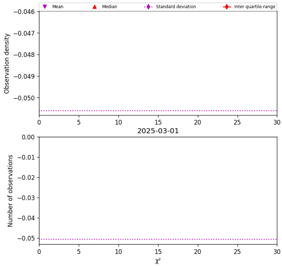
Figure 38: Histogram of “ \chi^2 ” for 2025-03-01 to 2025-03-02
