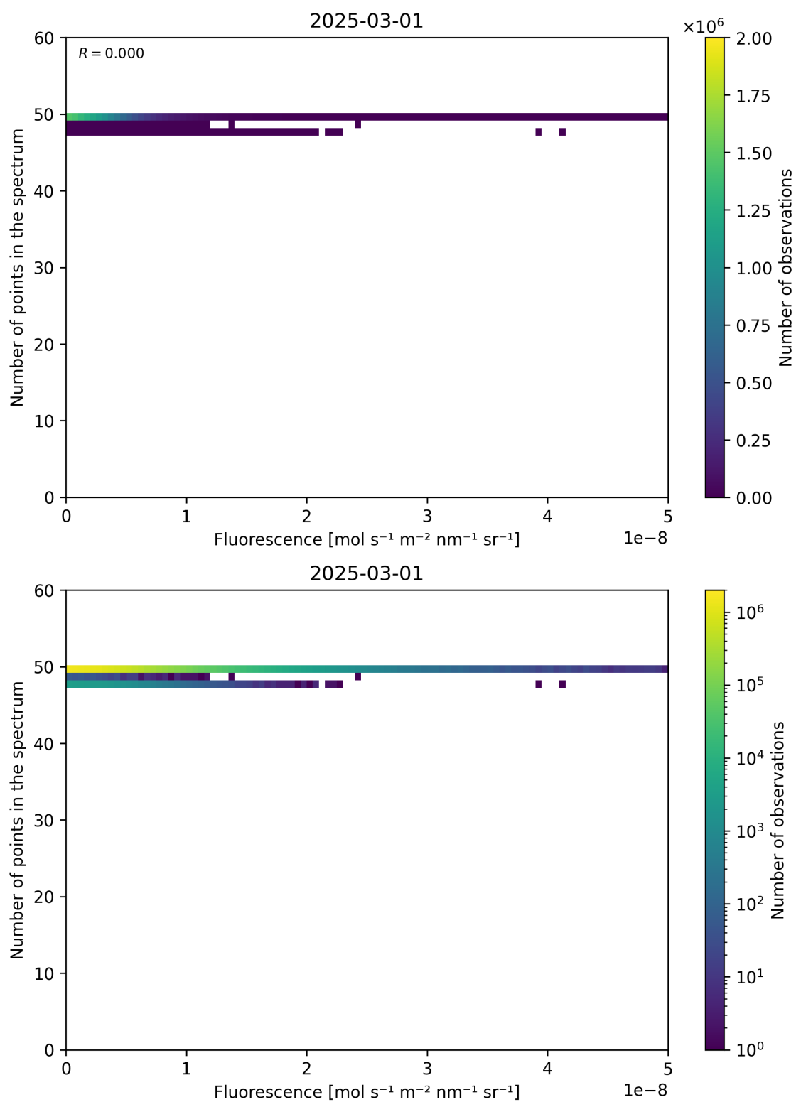
Figure 86: Scatter density plot of “Fluorescence” against “Number of points in the spectrum” for 2025-03-01 to 2025-03-02.
