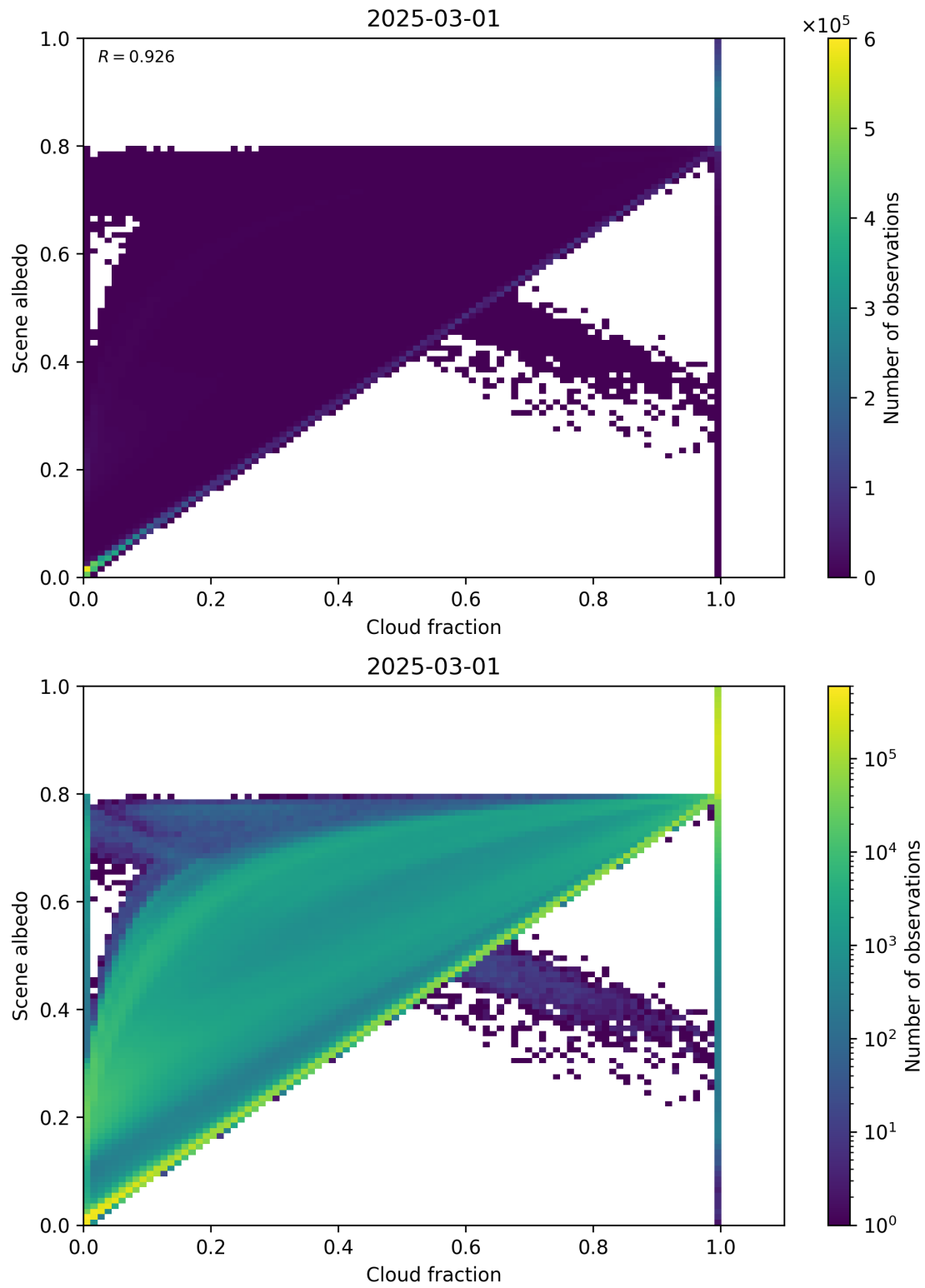
Figure 75: Scatter density plot of “Cloud fraction” against “Scene albedo” for 2025-03-01 to 2025-03-02.
