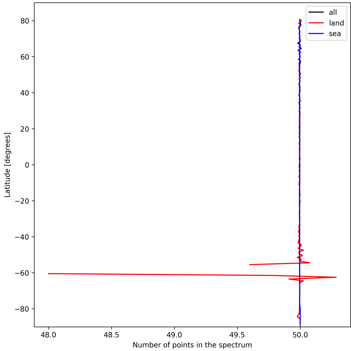
Figure 27: Zonal average of “Number of points in the spectrum” for 2025-03-01 to 2025-03-02.
