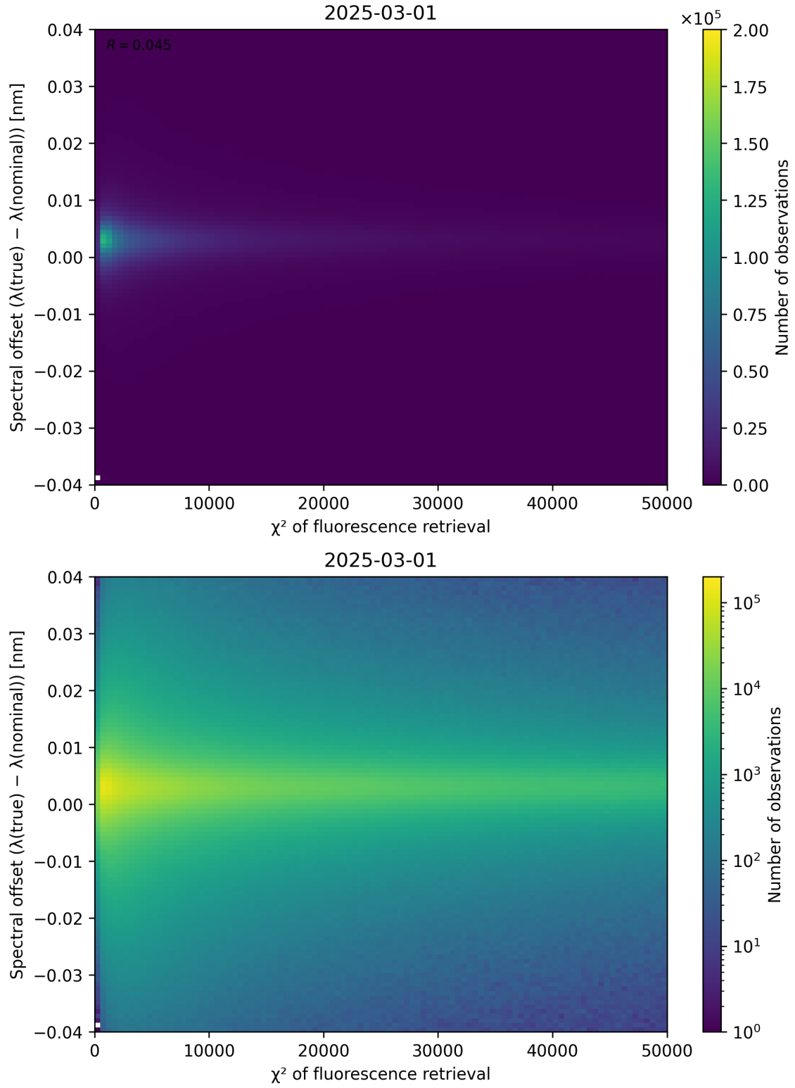
Figure 69: Scatter density plot of “ \chi^2 of fluorescence retrieval” against “Spectral offset ( \lambda_{\text{true}} - \lambda_{\text{nominal}} )” for 2025-03-01 to 2025-03-02.
