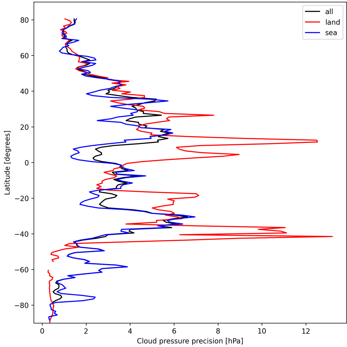
Figure 14: Zonal average of “Cloud pressure precision” for 2025-03-01 to 2025-03-02.
