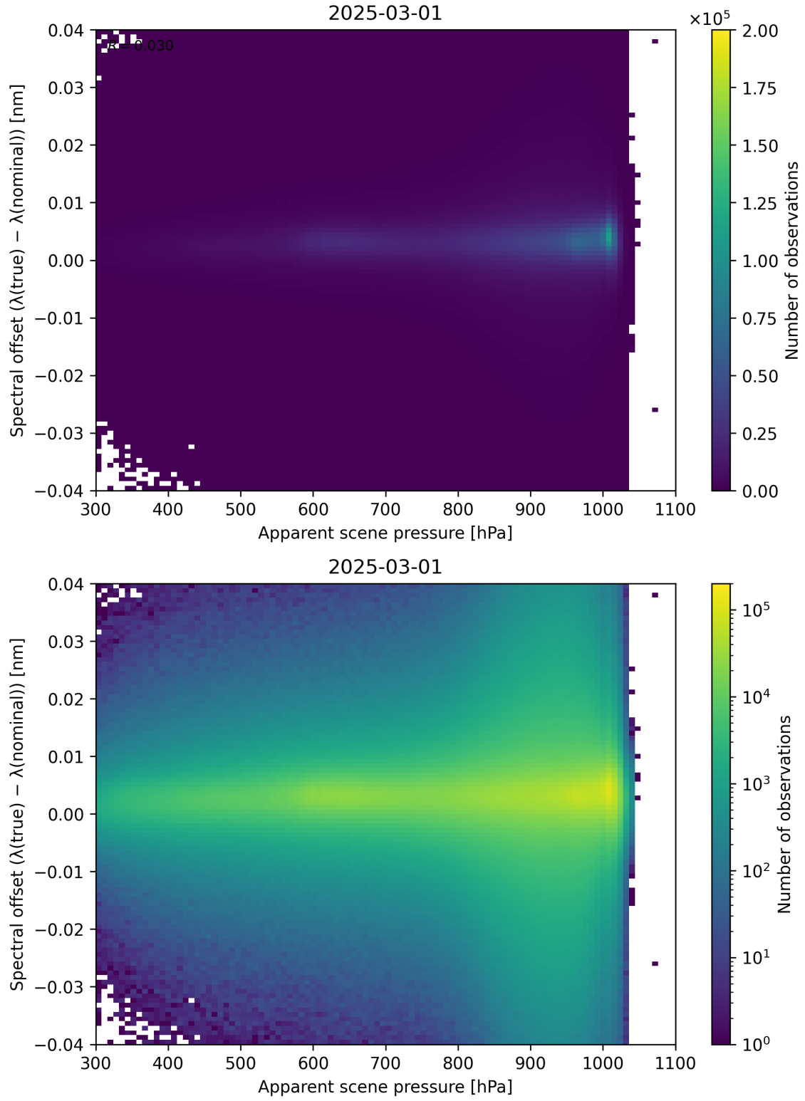
Figure 67: Scatter density plot of “Apparent scene pressure” against “Spectral offset ( \lambda_{\text{true}} - \lambda_{\text{nominal}} )” for 2025-03-01 to 2025-03-02.
