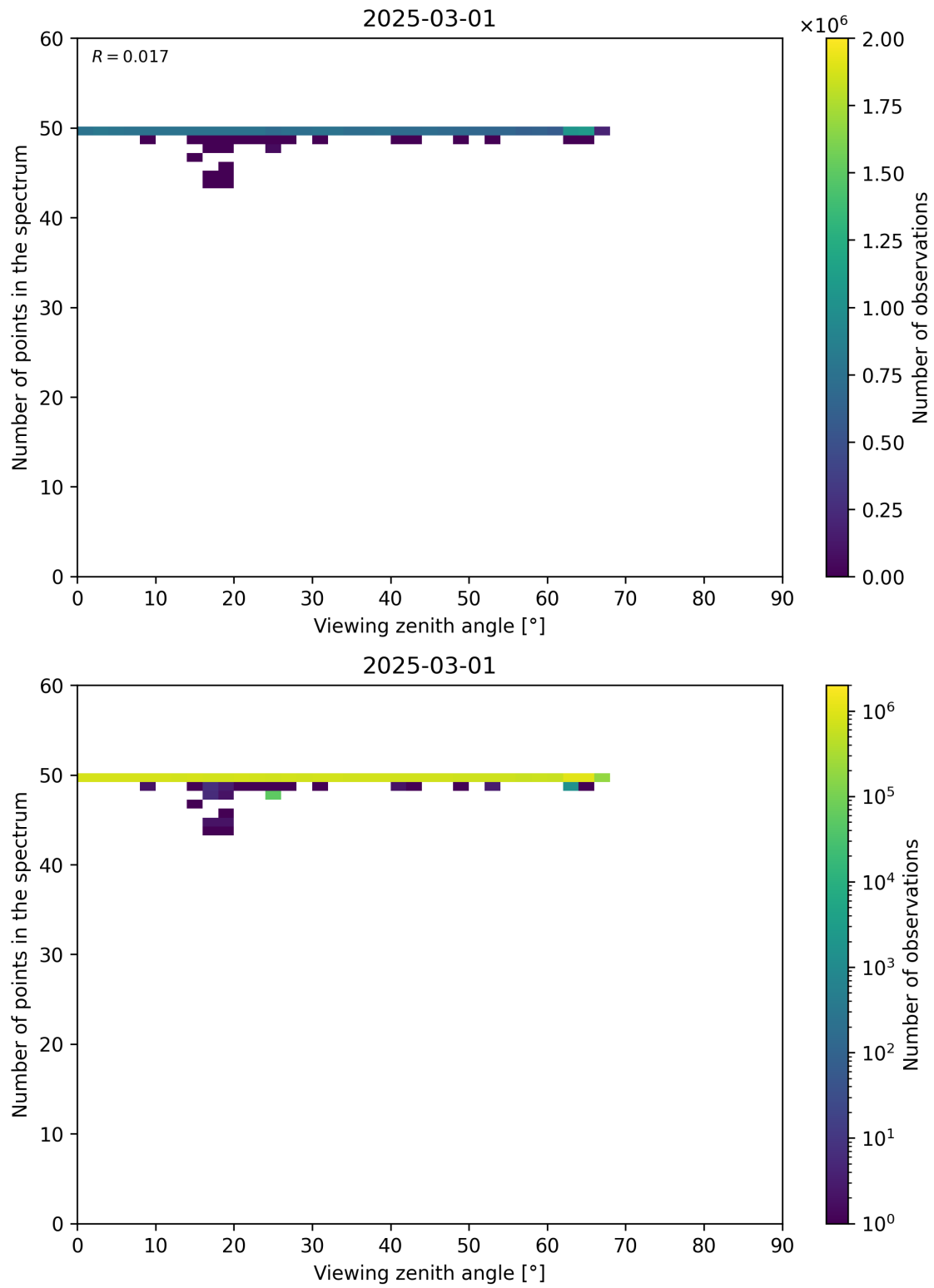
Figure 125: Scatter density plot of “Viewing zenith angle” against “Number of points in the spectrum” for 2025-03-01 to 2025-03-02.
