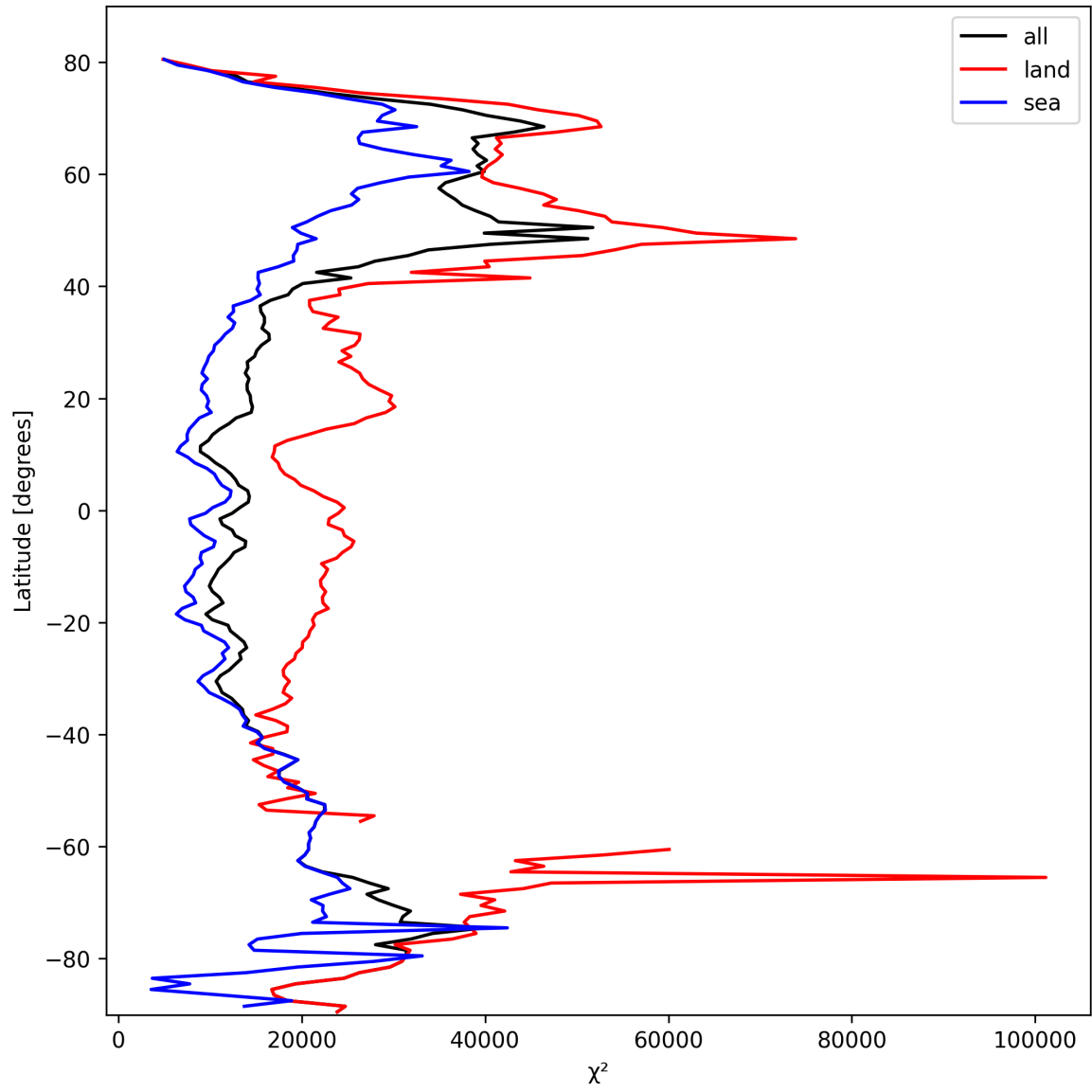
Figure 21: Zonal average of “ \chi^2 ” for 2025-03-01 to 2025-03-02.
