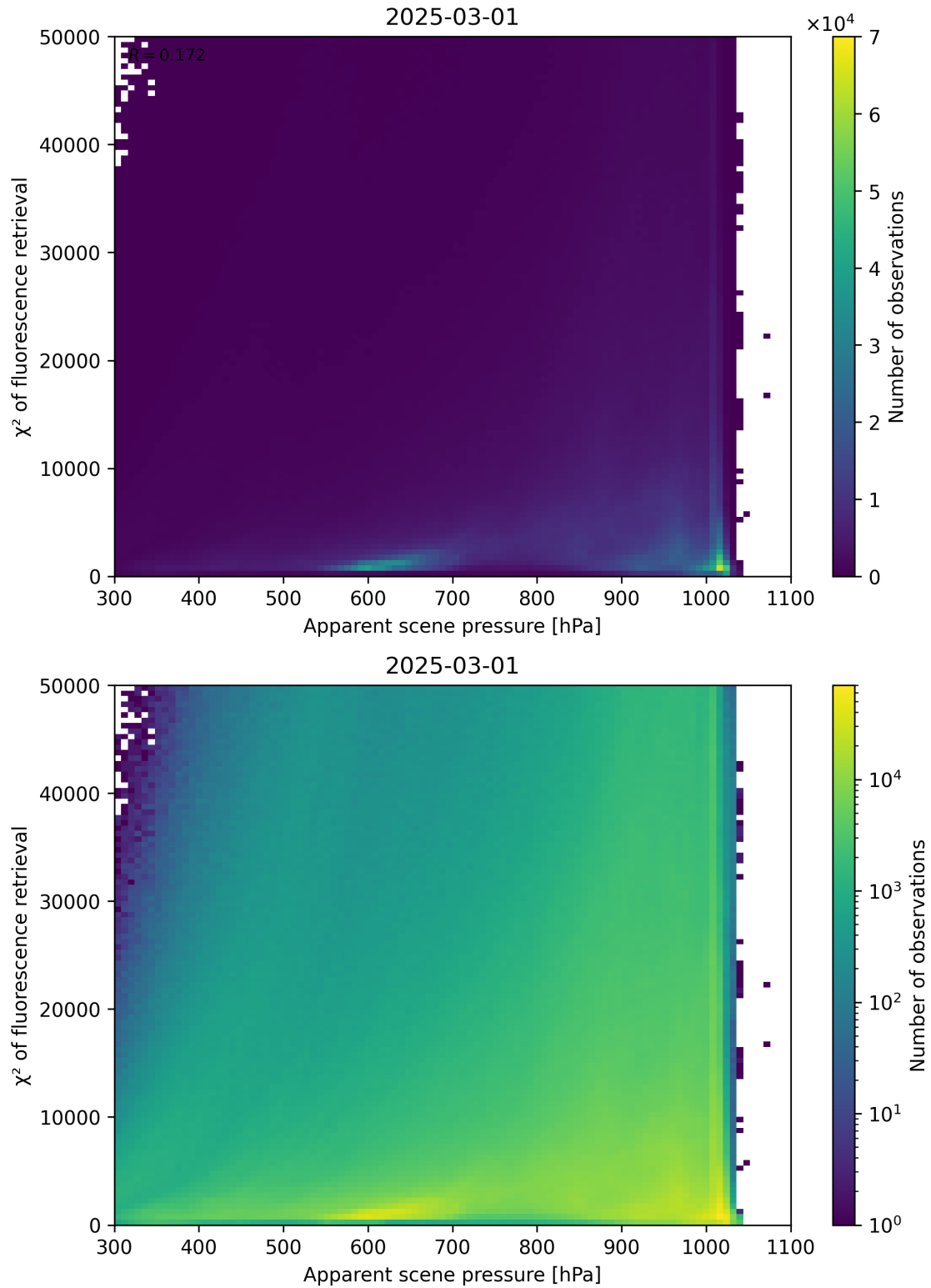
Figure 63: Scatter density plot of “Apparent scene pressure” against “ \chi^2 of fluorescence retrieval” for 2025-03-01 to 2025-03-02.
