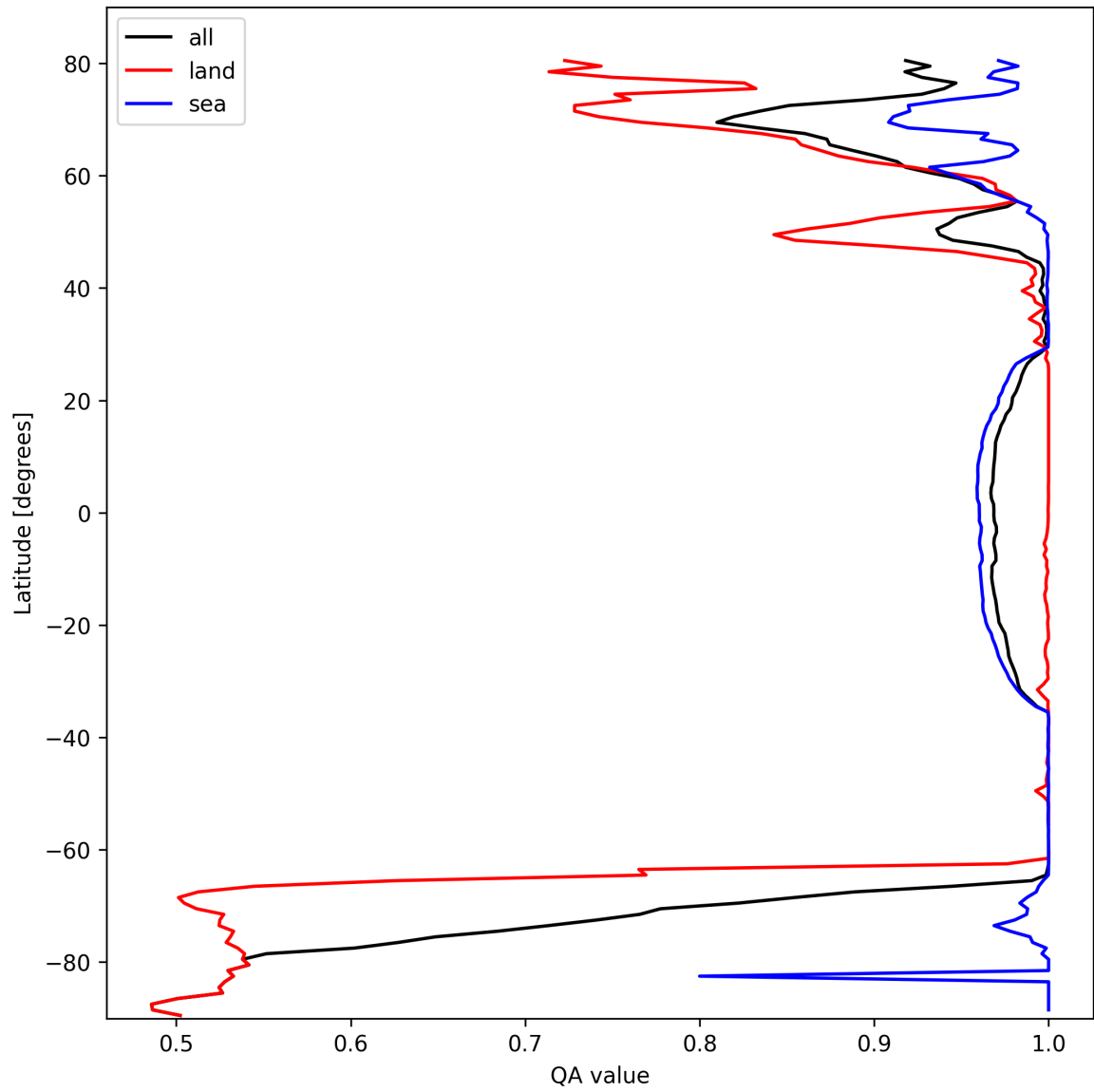
Figure 12: Zonal average of “QA value” for 2025-03-01 to 2025-03-02.
