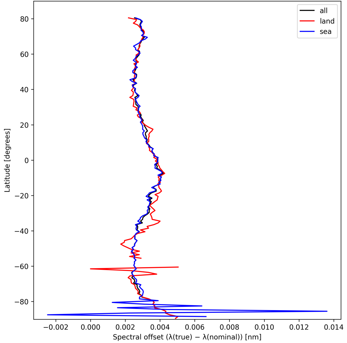
Figure 28: Zonal average of “Spectral offset ( \lambda_{\text{true}} - \lambda_{\text{nominal}} )” for 2025-03-01 to 2025-03-02.
