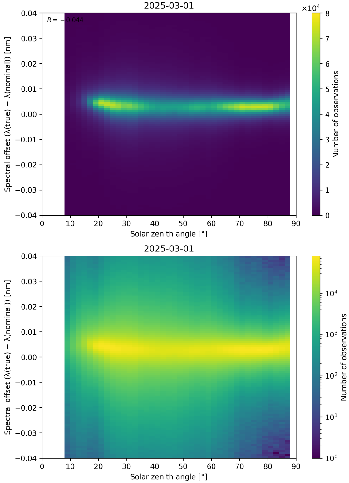
Figure 117: Scatter density plot of “Solar zenith angle” against “Spectral offset ( \lambda_{\text{true}} - \lambda_{\text{nominal}} )” for 2025-03-01 to 2025-03-02.
