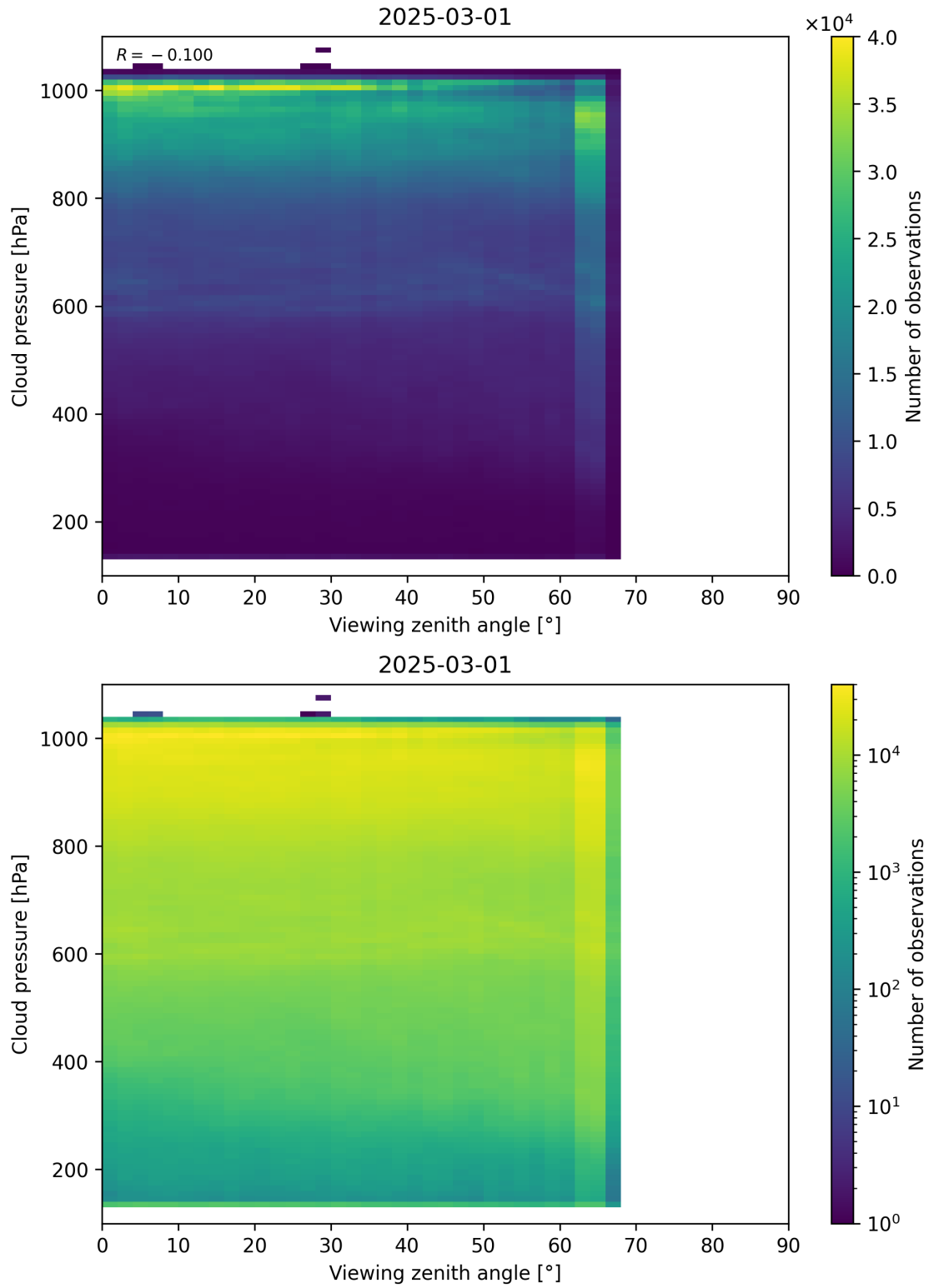
Figure 121: Scatter density plot of “Viewing zenith angle” against “Cloud pressure” for 2025-03-01 to 2025-03-02.
