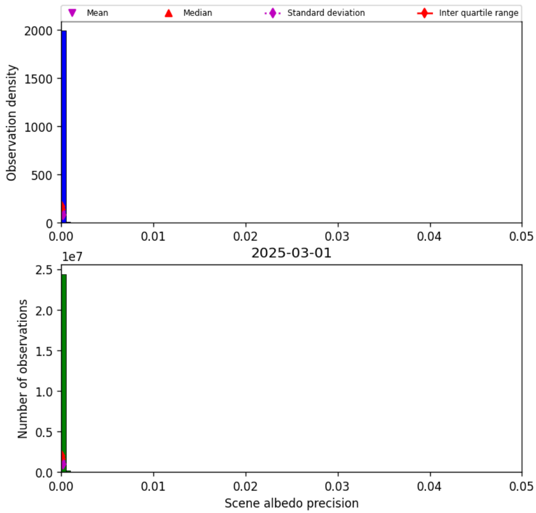
Figure 35: Histogram of “Scene albedo precision” for 2025-03-01 to 2025-03-02
