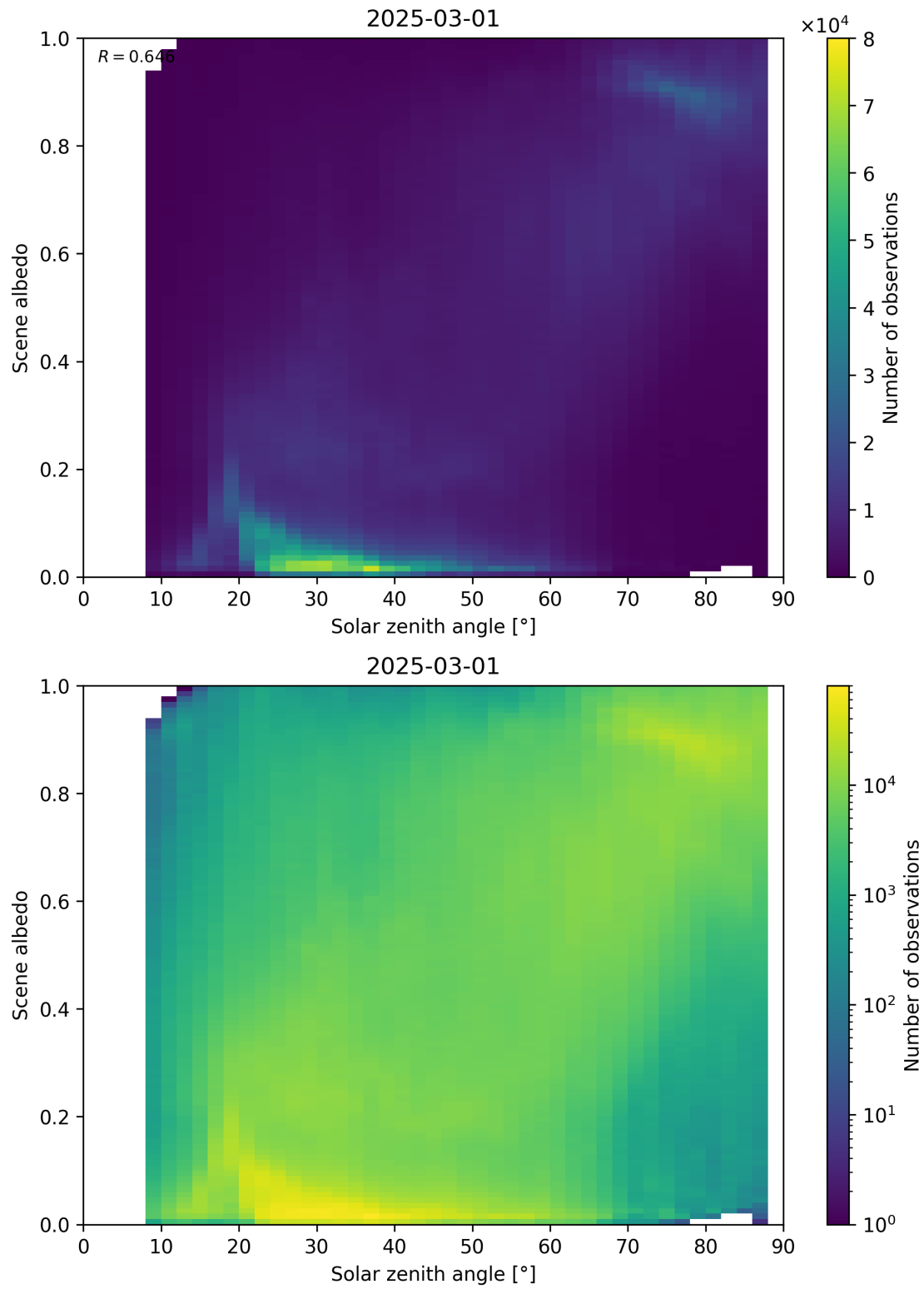
Figure 116: Scatter density plot of “Solar zenith angle” against “Scene albedo” for 2025-03-01 to 2025-03-02.
