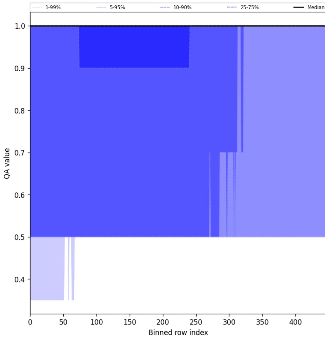
Figure 46: Along track statistics of “QA value” for 2025-03-01 to 2025-03-02
