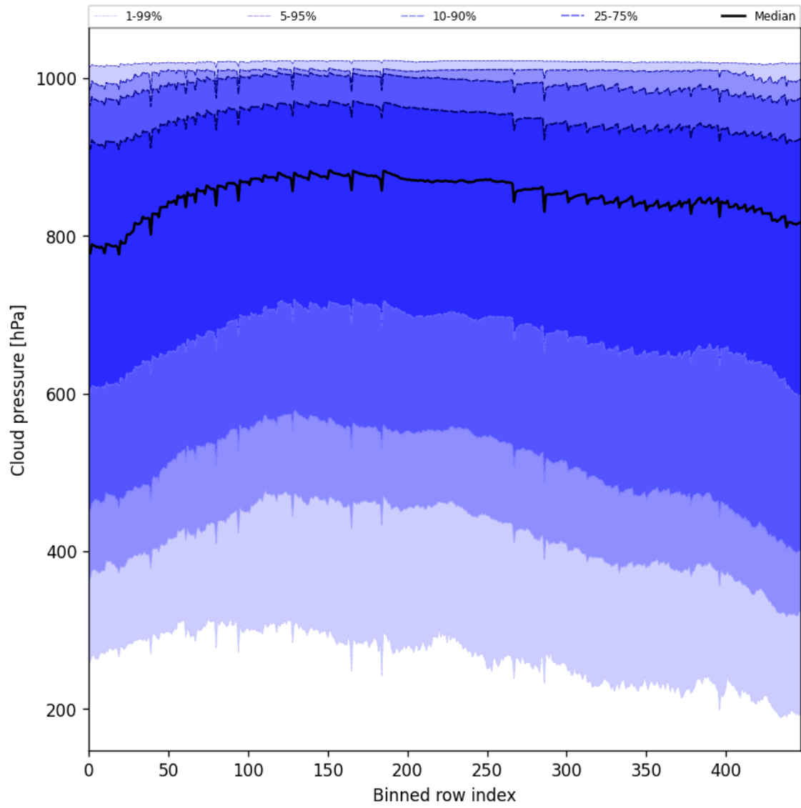
Figure 47: Along track statistics of “Cloud pressure” for 2025-03-01 to 2025-03-02
