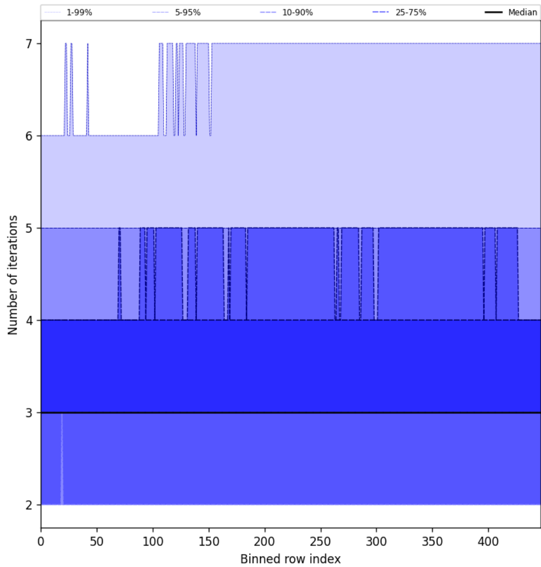
Figure 56: Along track statistics of “Number of iterations” for 2025-03-01 to 2025-03-02
