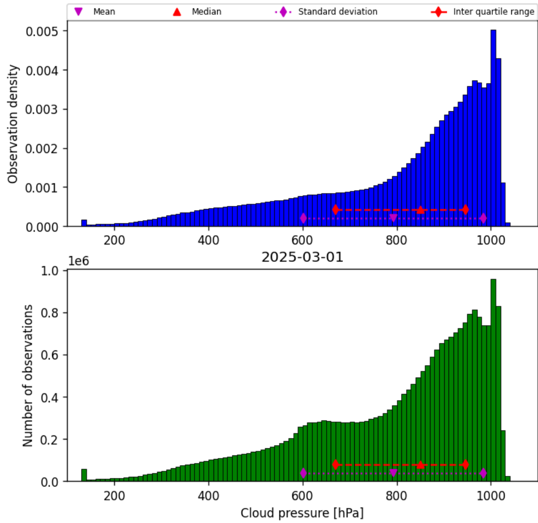
Figure 30: Histogram of “Cloud pressure” for 2025-03-01 to 2025-03-02
