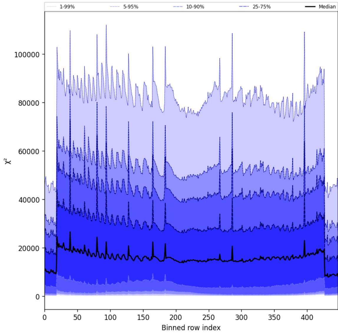
Figure 55: Along track statistics of “ \chi^2 ” for 2025-03-01 to 2025-03-02
