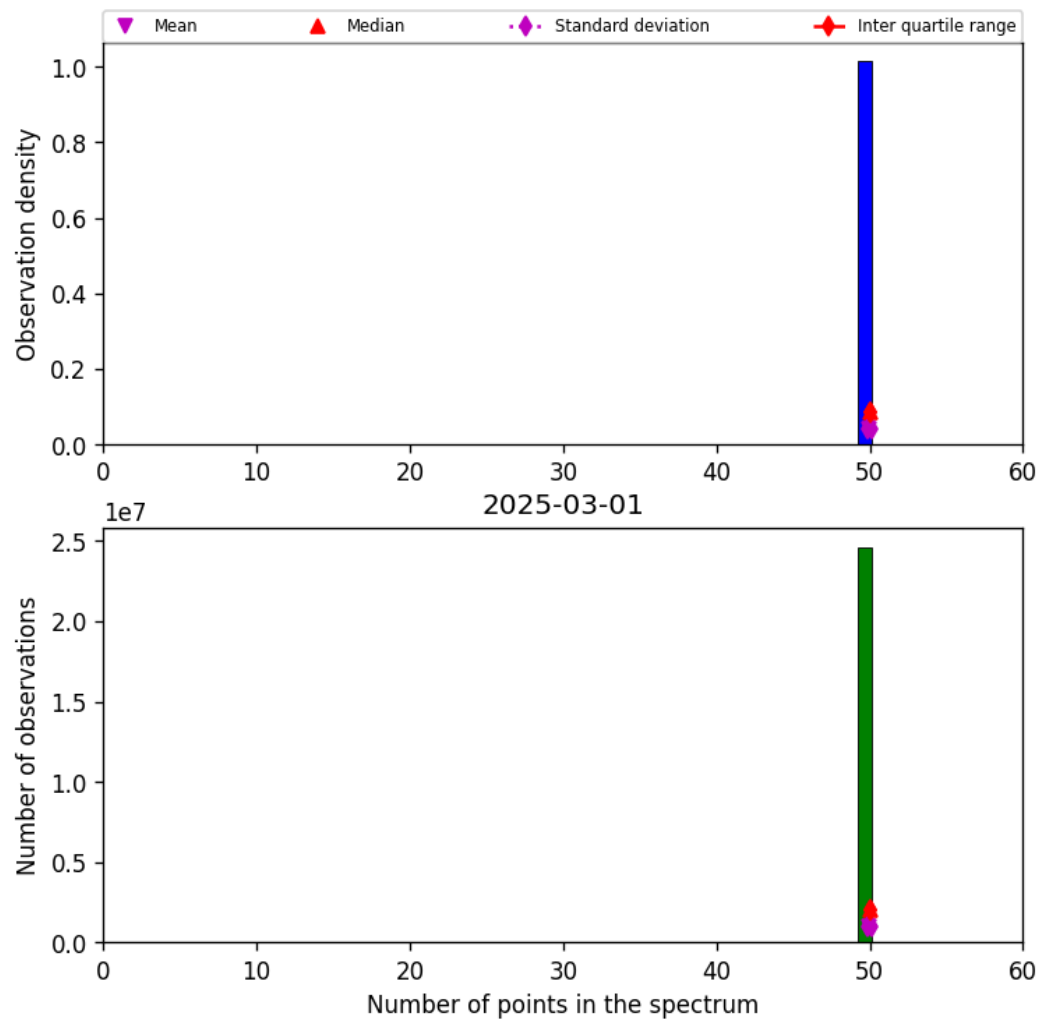
Figure 44: Histogram of “Number of points in the spectrum” for 2025-03-01 to 2025-03-02
