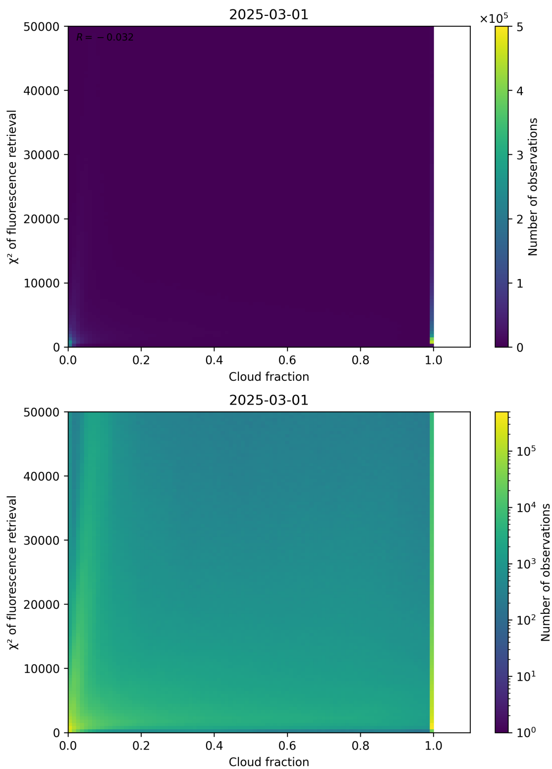
Figure 71: Scatter density plot of “Cloud fraction” against “ \chi^2 of fluorescence retrieval” for 2025-03-01 to 2025-03-02.
