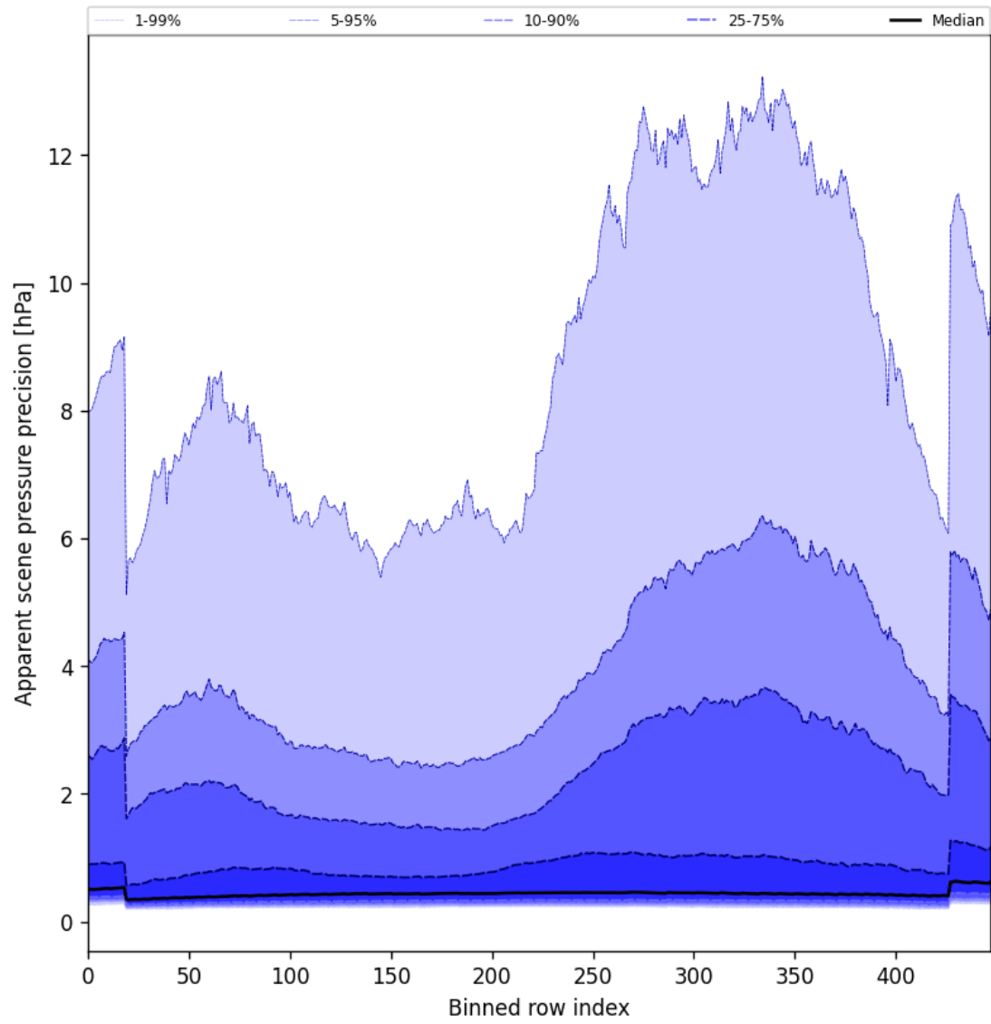
Figure 54: Along track statistics of “Apparent scene pressure precision” for 2025-03-01 to 2025-03-02
