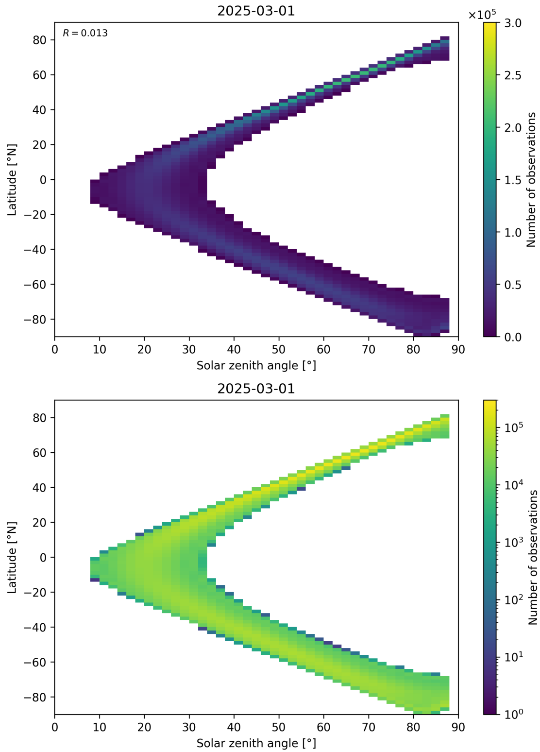
Figure 113: Scatter density plot of “Solar zenith angle” against “Latitude” for 2025-03-01 to 2025-03-02.
