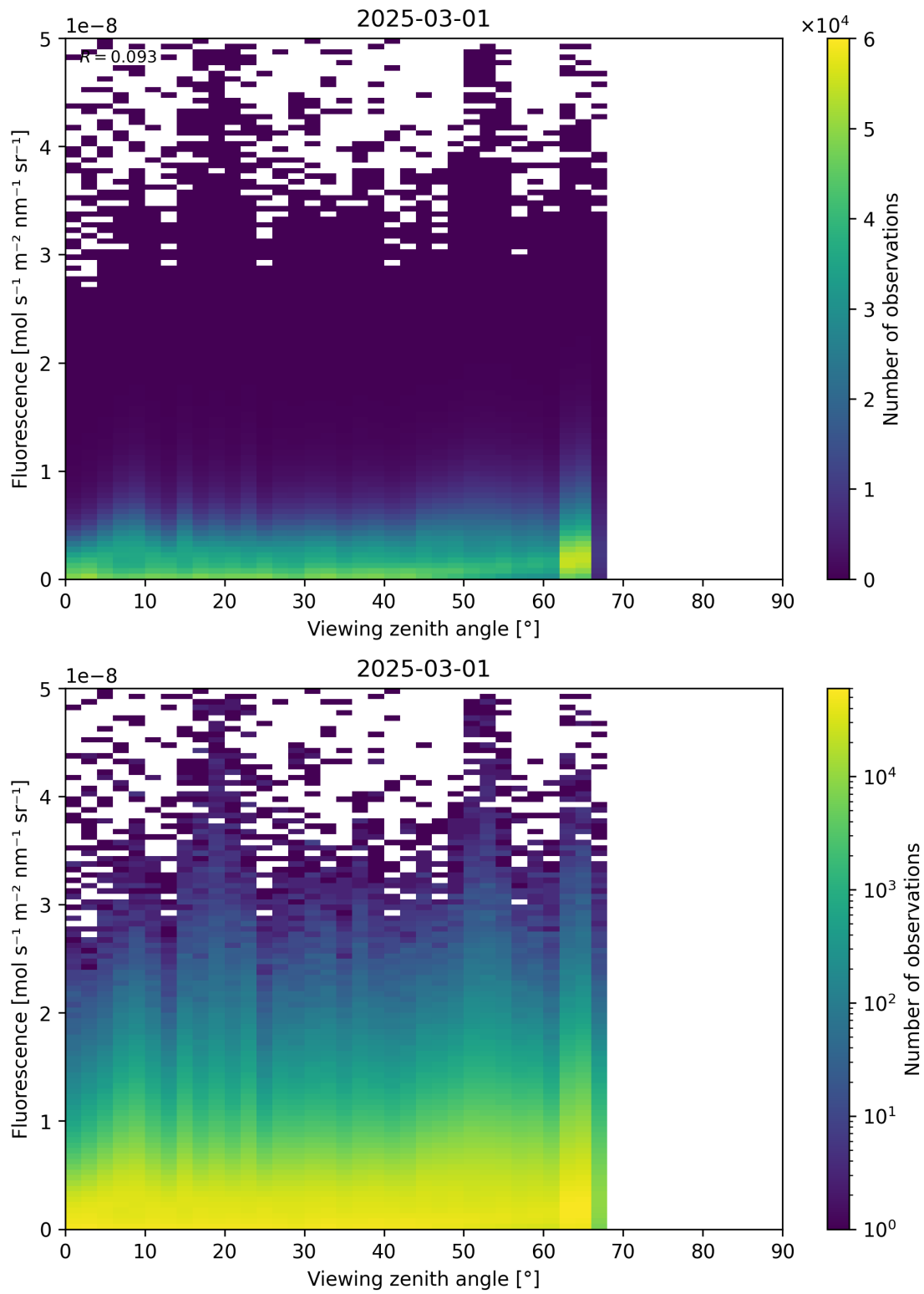
Figure 122: Scatter density plot of “Viewing zenith angle” against “Fluorescence” for 2025-03-01 to 2025-03-02.
