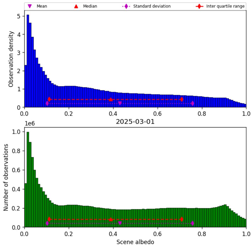
Figure 34: Histogram of “Scene albedo” for 2025-03-01 to 2025-03-02
