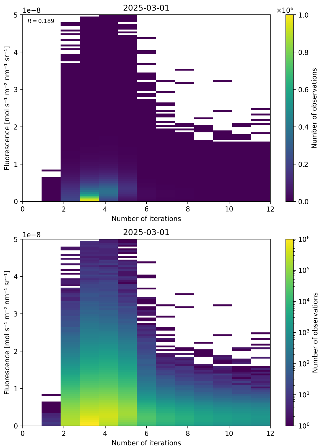
Figure 98: Scatter density plot of “Number of iterations” against “Fluorescence” for 2025-03-01 to 2025-03-02.
