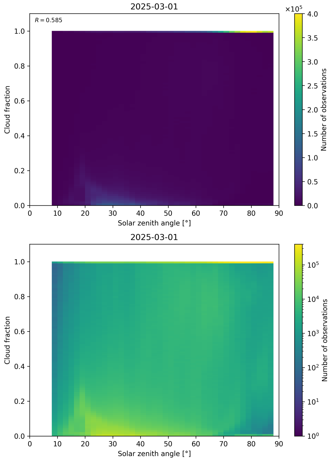
Figure 110: Scatter density plot of “Solar zenith angle” against “Cloud fraction” for 2025-03-01 to 2025-03-02.
