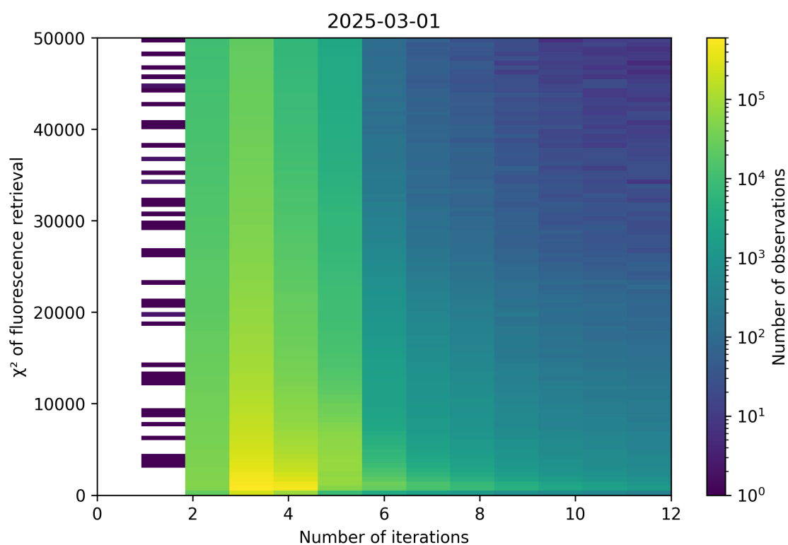
Figure 97: Scatter density plot of “Number of iterations” against “ \chi^2 of fluorescence retrieval” for 2025-03-01 to 2025-03-02.
