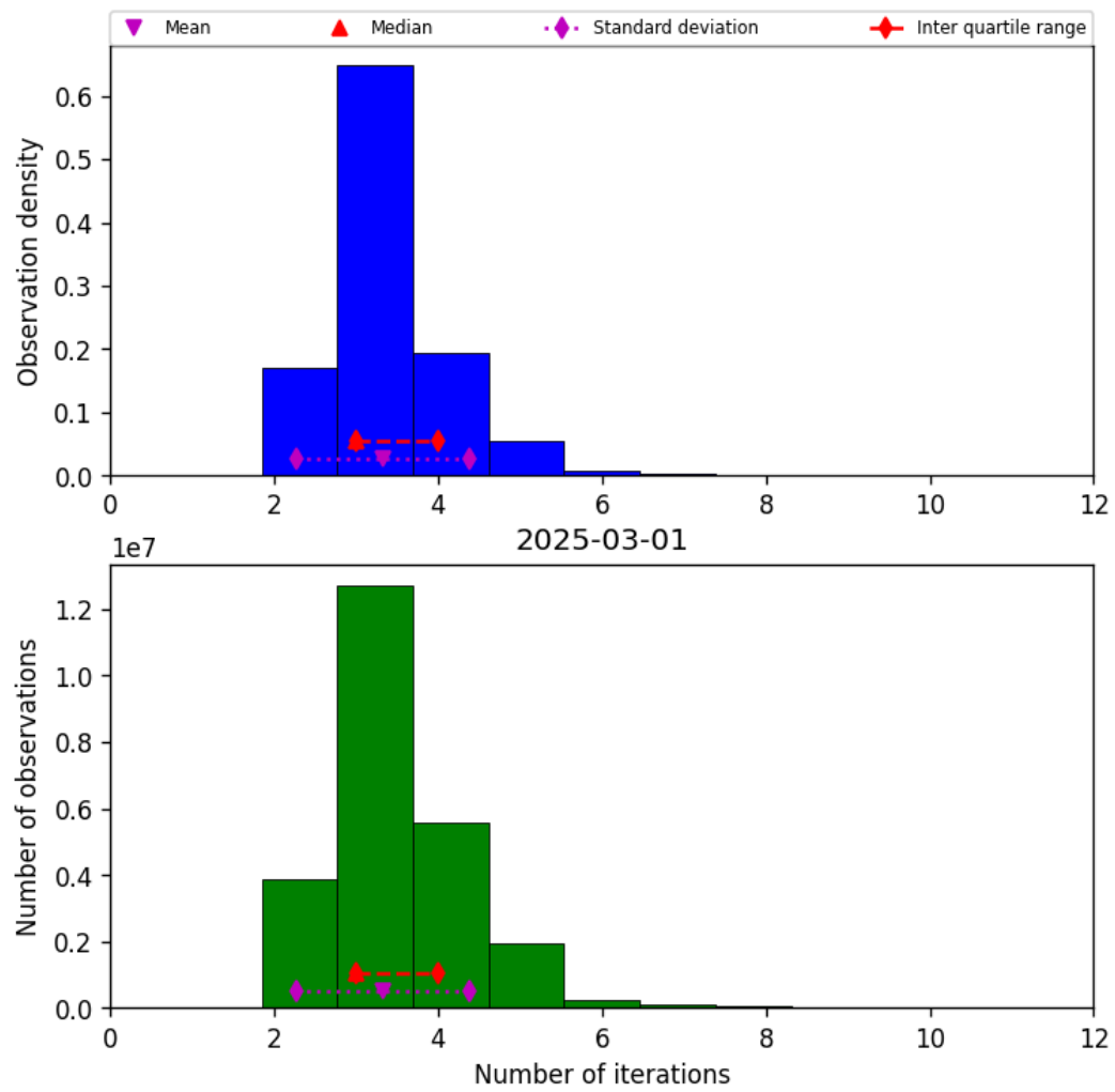
Figure 39: Histogram of “Number of iterations” for 2025-03-01 to 2025-03-02
