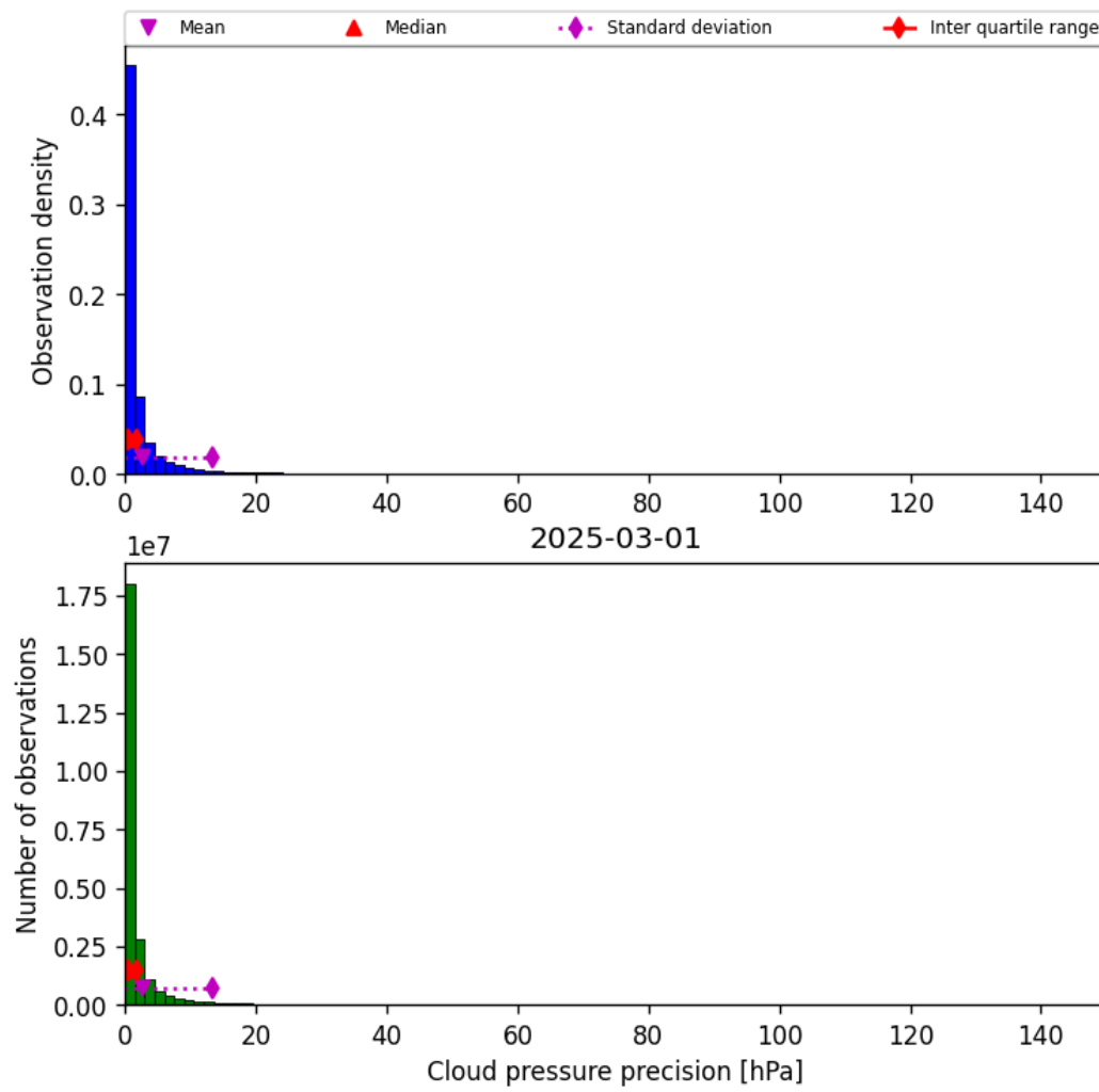
Figure 31: Histogram of “Cloud pressure precision” for 2025-03-01 to 2025-03-02
