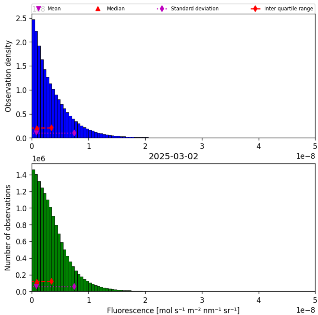
Figure 40: Histogram of “Fluorescence” for 2025-03-01 to 2025-03-03
