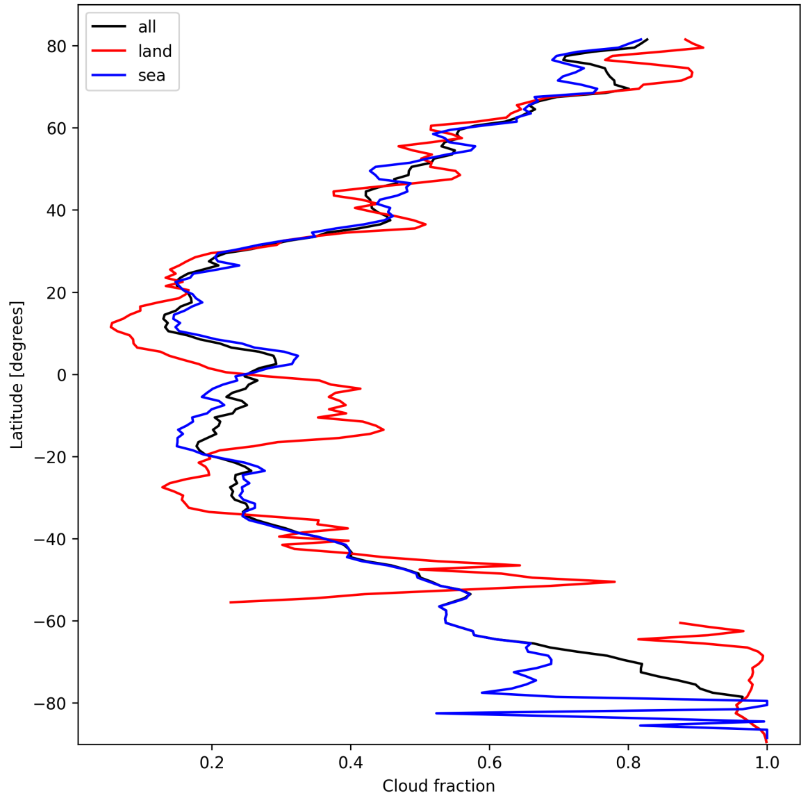
Figure 15: Zonal average of “Cloud fraction” for 2025-03-01 to 2025-03-03.
