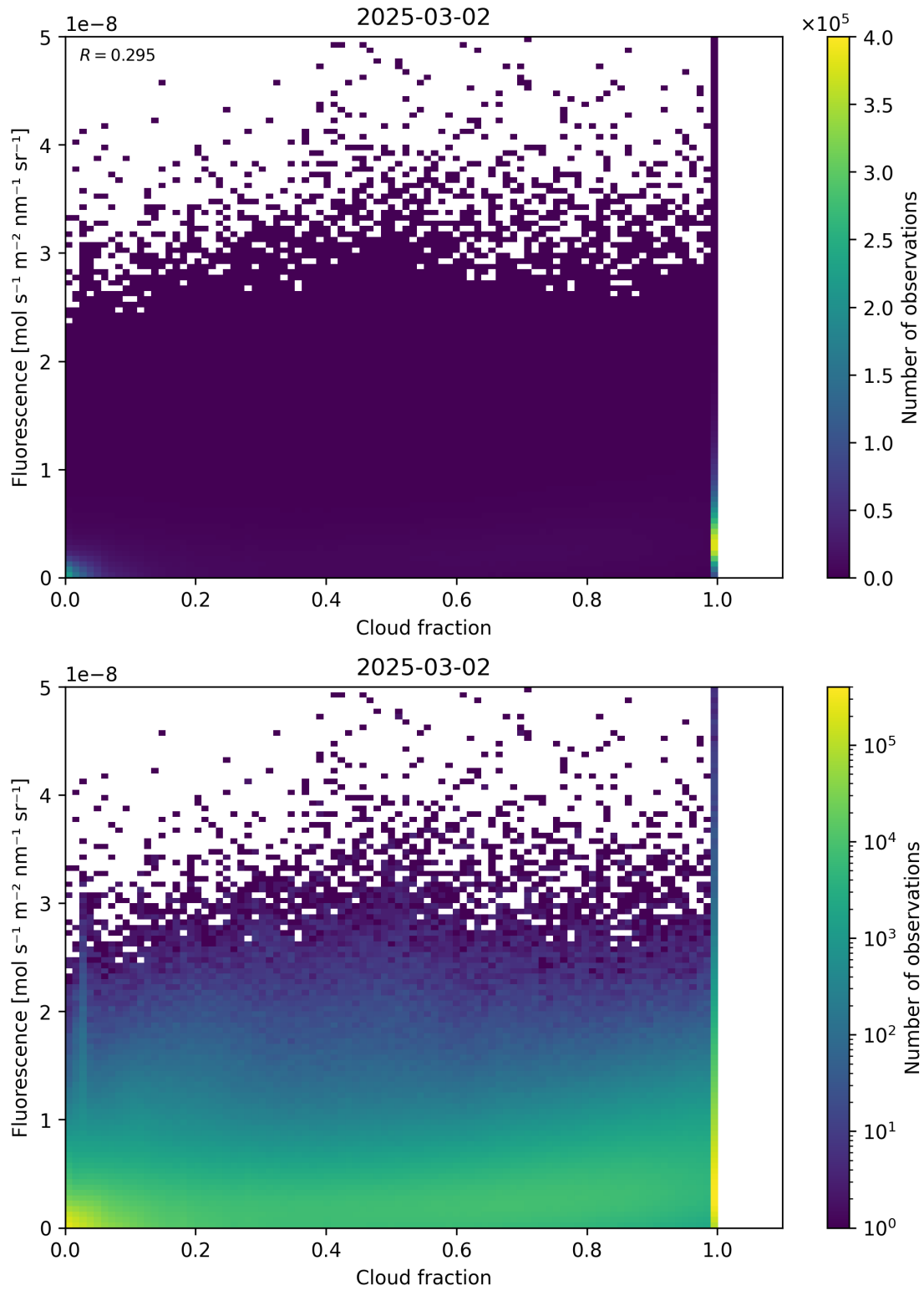
Figure 72: Scatter density plot of “Cloud fraction” against “Fluorescence” for 2025-03-01 to 2025-03-03.
