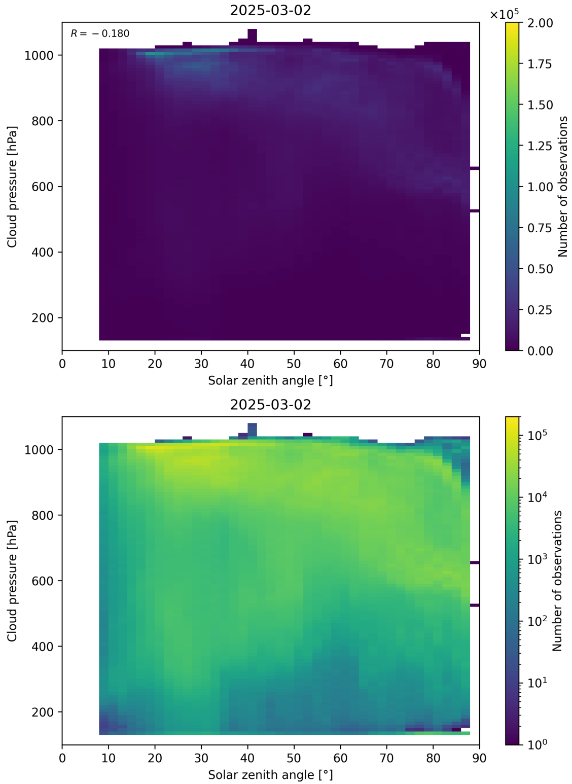
Figure 111: Scatter density plot of “Solar zenith angle” against “Cloud pressure” for 2025-03-01 to 2025-03-03.
