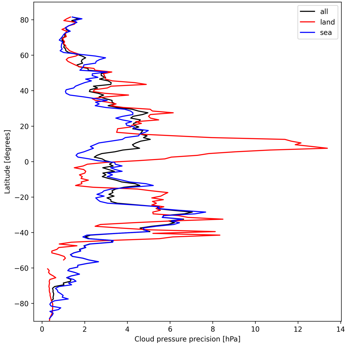
Figure 14: Zonal average of “Cloud pressure precision” for 2025-03-01 to 2025-03-03.
