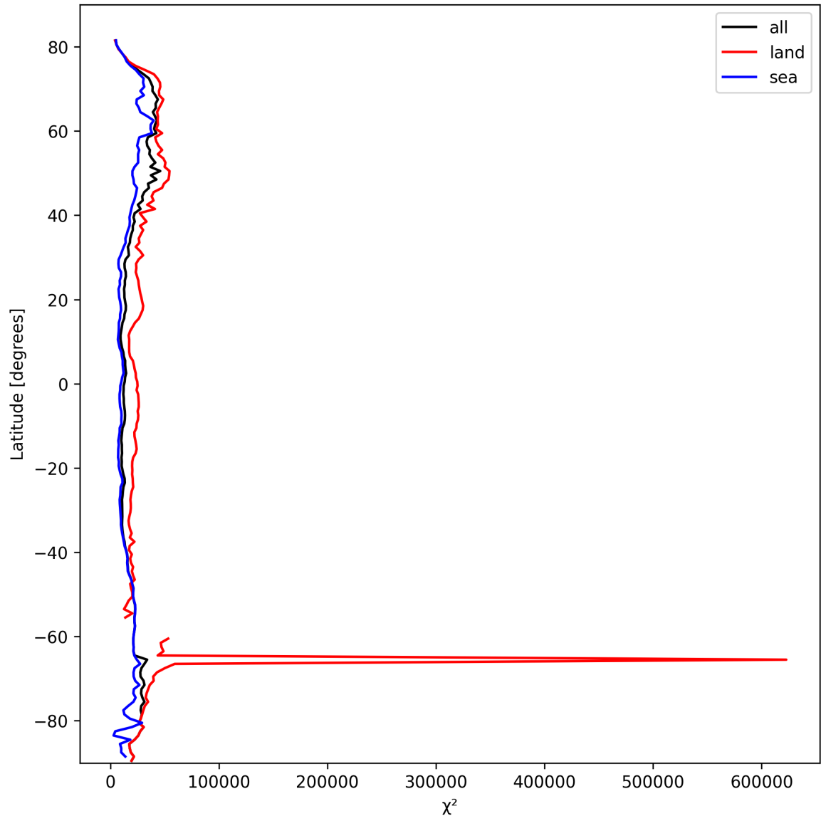
Figure 21: Zonal average of “ \chi^2 ” for 2025-03-01 to 2025-03-03.
