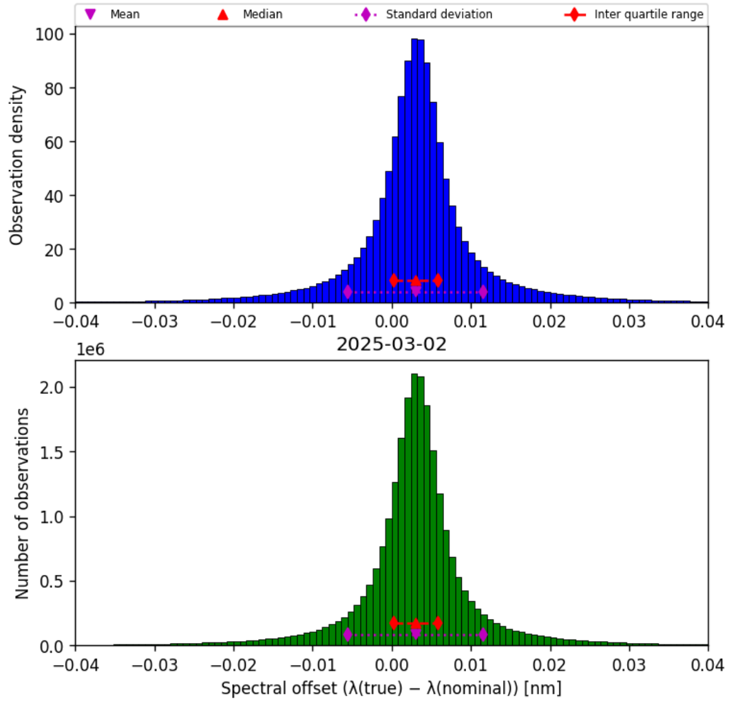
Figure 45: Histogram of “Spectral offset ( \lambda_{\text{true}} - \lambda_{\text{nominal}} )” for 2025-03-01 to 2025-03-03
