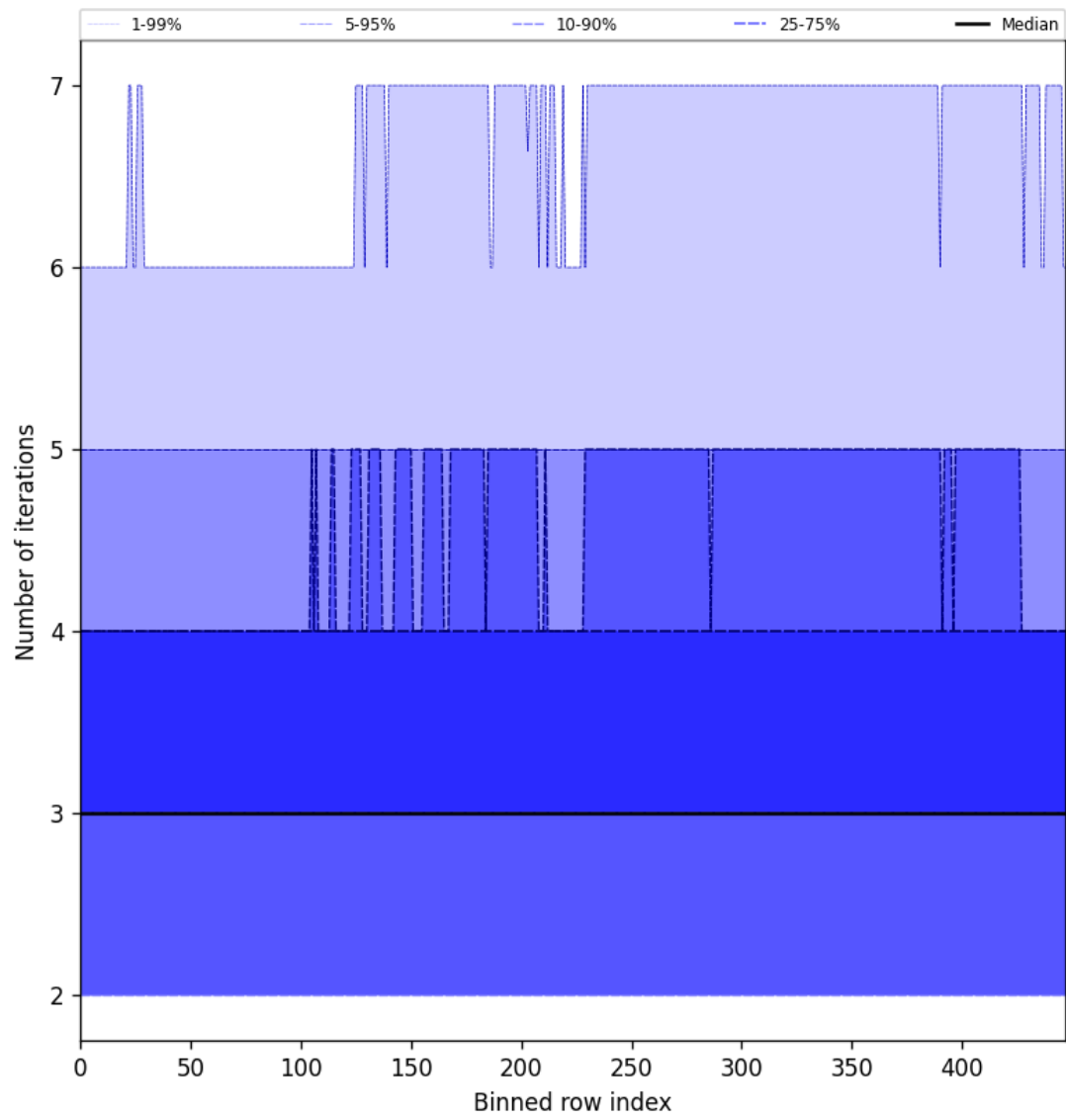
Figure 56: Along track statistics of “Number of iterations” for 2025-03-01 to 2025-03-03
