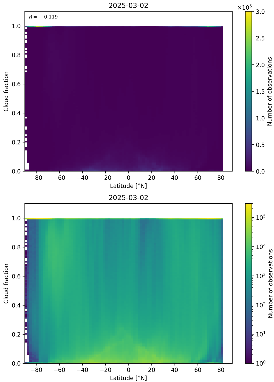
Figure 90: Scatter density plot of “Latitude” against “Cloud fraction” for 2025-03-01 to 2025-03-03.
