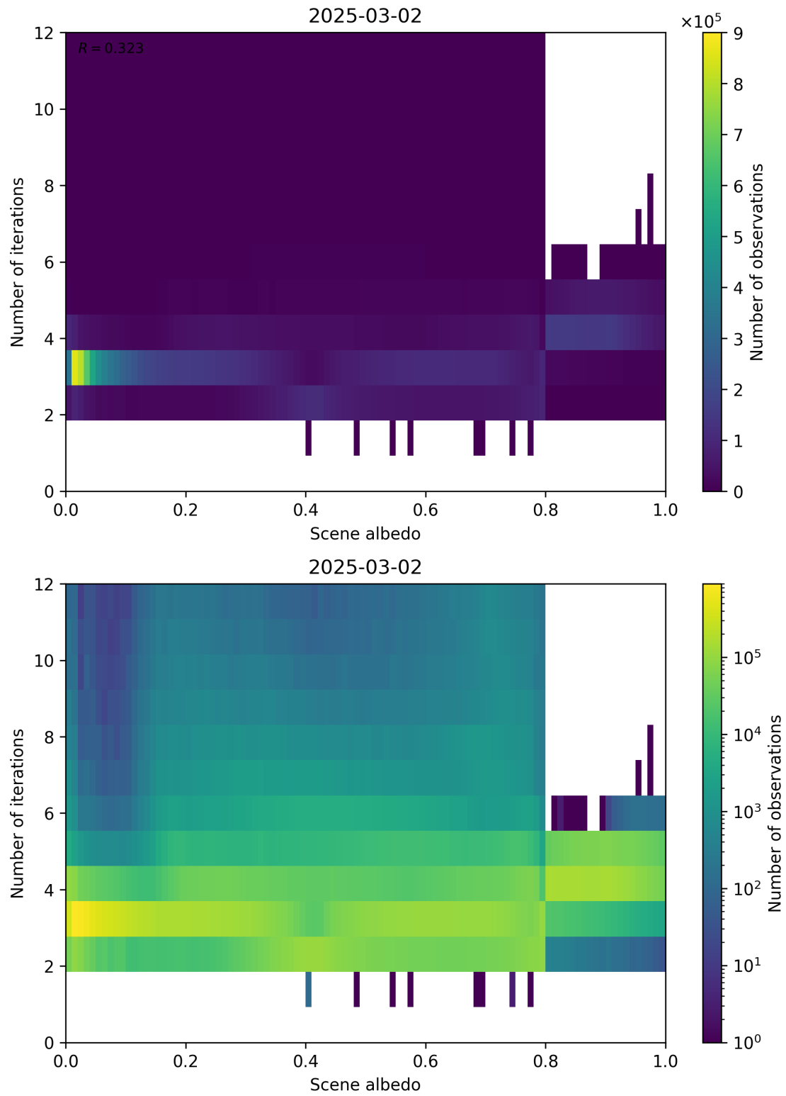
Figure 105: Scatter density plot of “Scene albedo” against “Number of iterations” for 2025-03-01 to 2025-03-03.
