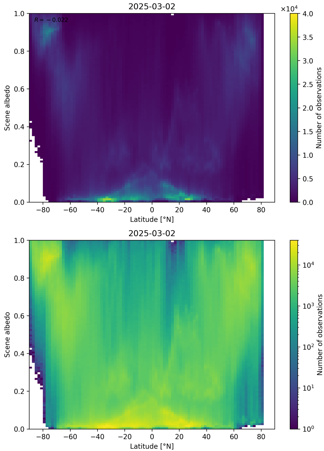
Figure 95: Scatter density plot of “Latitude” against “Scene albedo” for 2025-03-01 to 2025-03-03.
