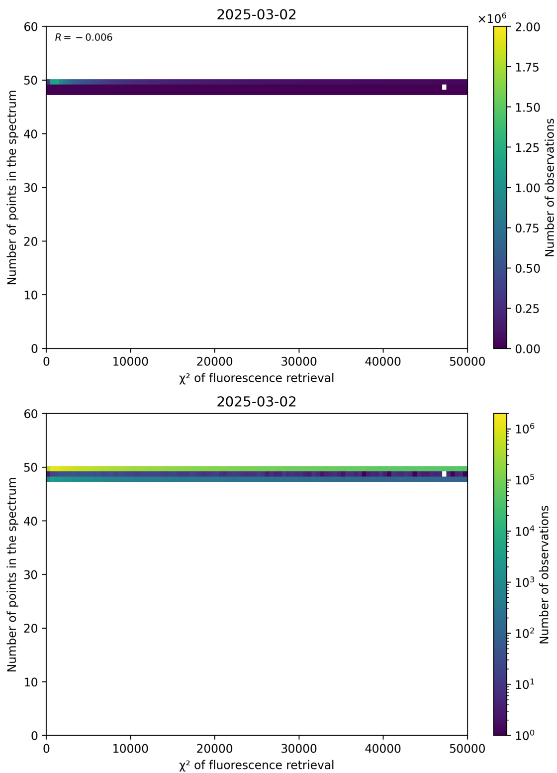
Figure 68: Scatter density plot of “ \chi^2 of fluorescence retrieval” against “Number of points in the spectrum” for 2025-03-01 to 2025-03-03.
