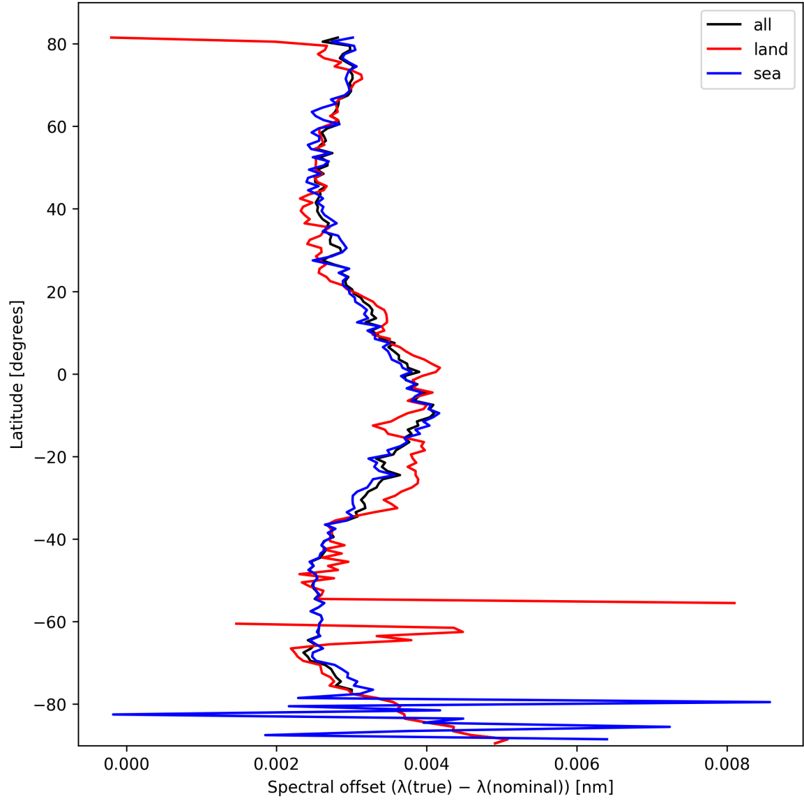
Figure 28: Zonal average of “Spectral offset ( \lambda_{\text{true}} - \lambda_{\text{nominal}} )” for 2025-03-01 to 2025-03-03.
