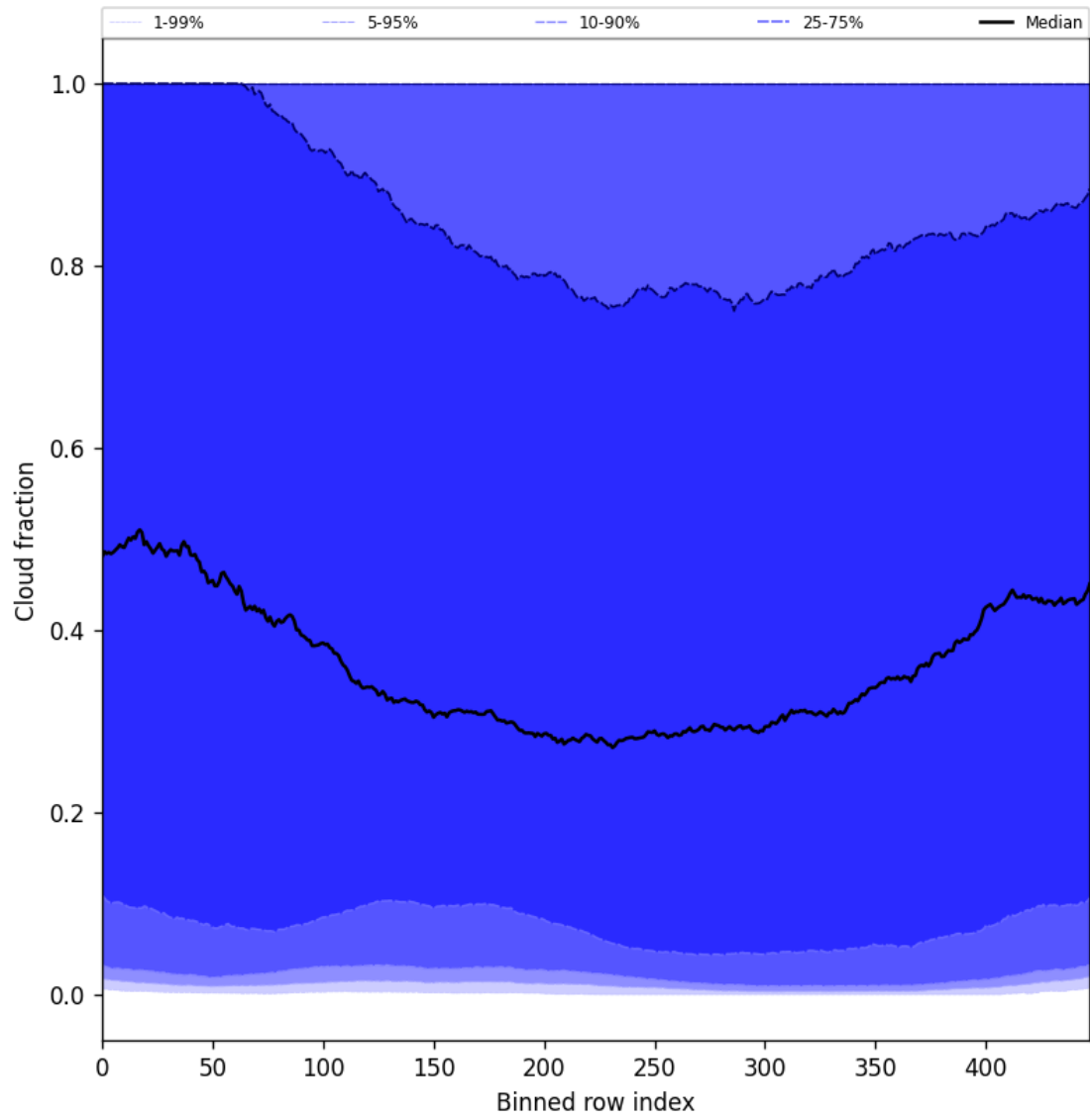
Figure 49: Along track statistics of “Cloud fraction” for 2025-03-01 to 2025-03-03
