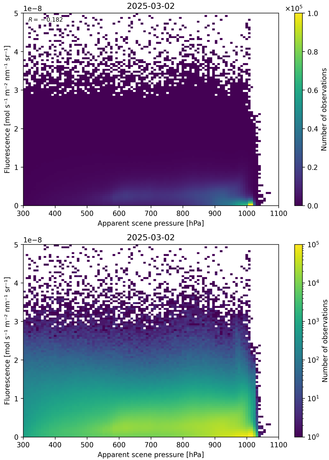
Figure 64: Scatter density plot of “Apparent scene pressure” against “Fluorescence” for 2025-03-01 to 2025-03-03.
