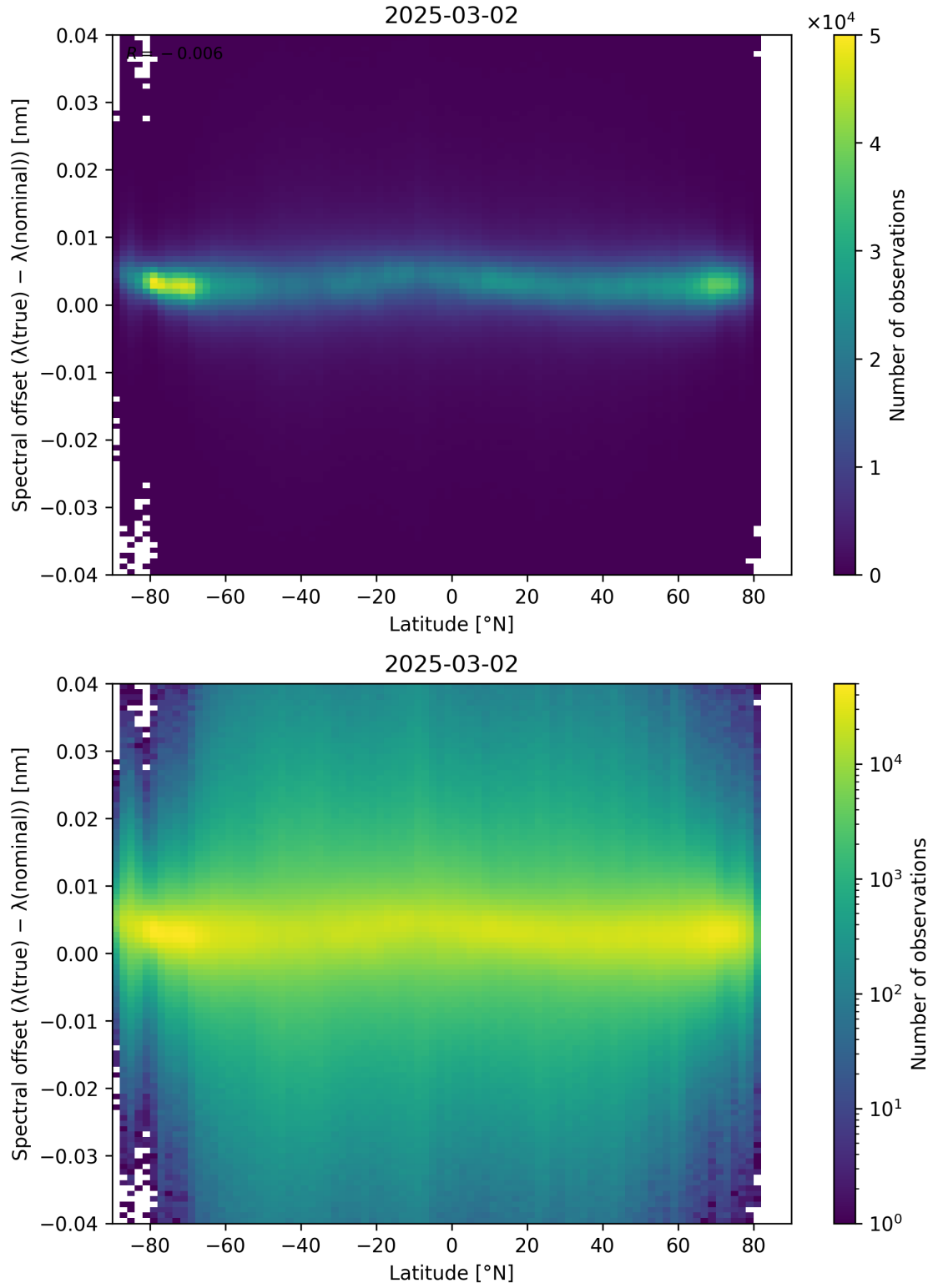
Figure 96: Scatter density plot of “Latitude” against “Spectral offset ( \lambda_{\text{true}} - \lambda_{\text{nominal}} )” for 2025-03-01 to 2025-03-03.
