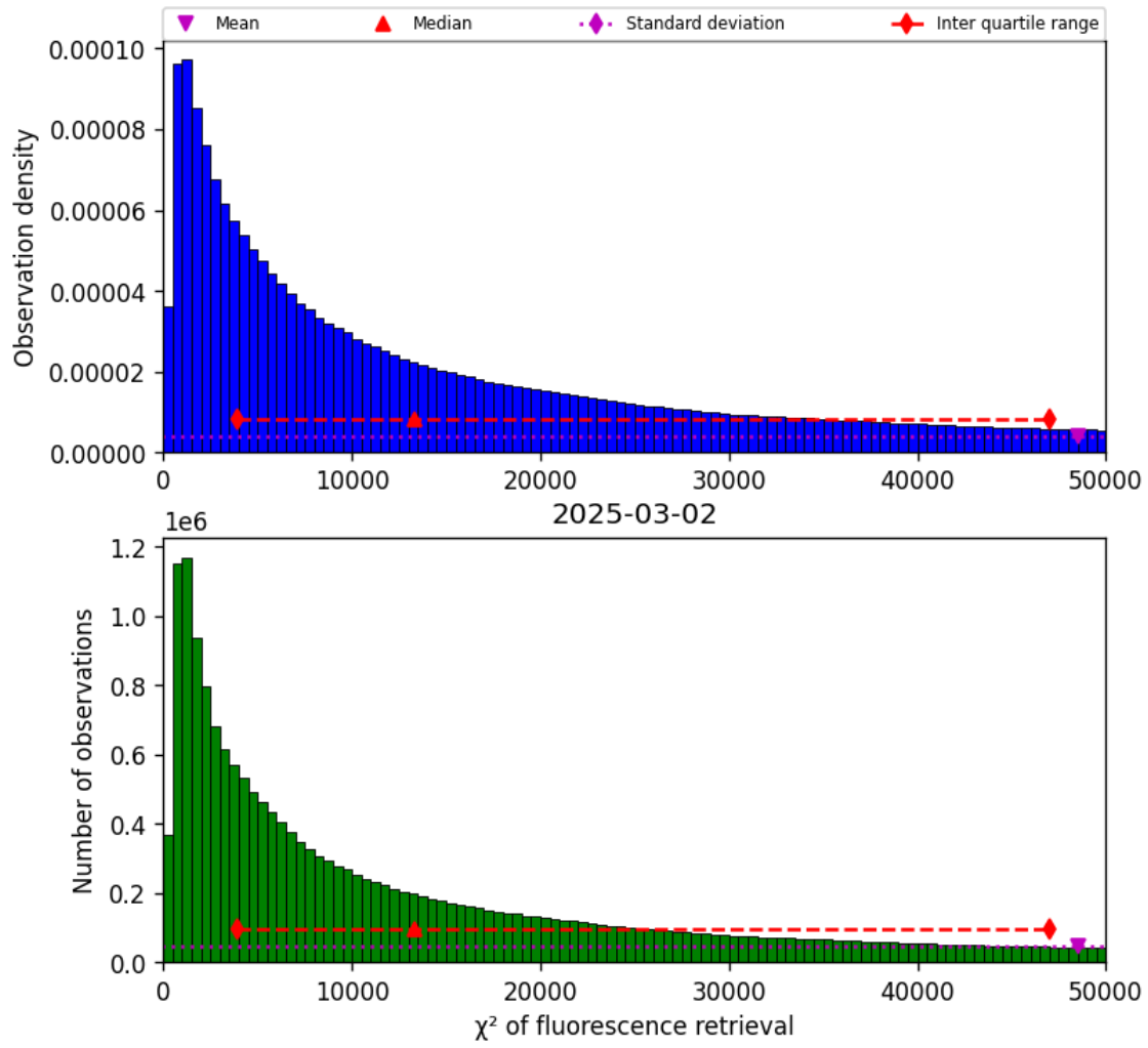
Figure 42: Histogram of “ \chi^2 of fluorescence retrieval” for 2025-03-01 to 2025-03-03
