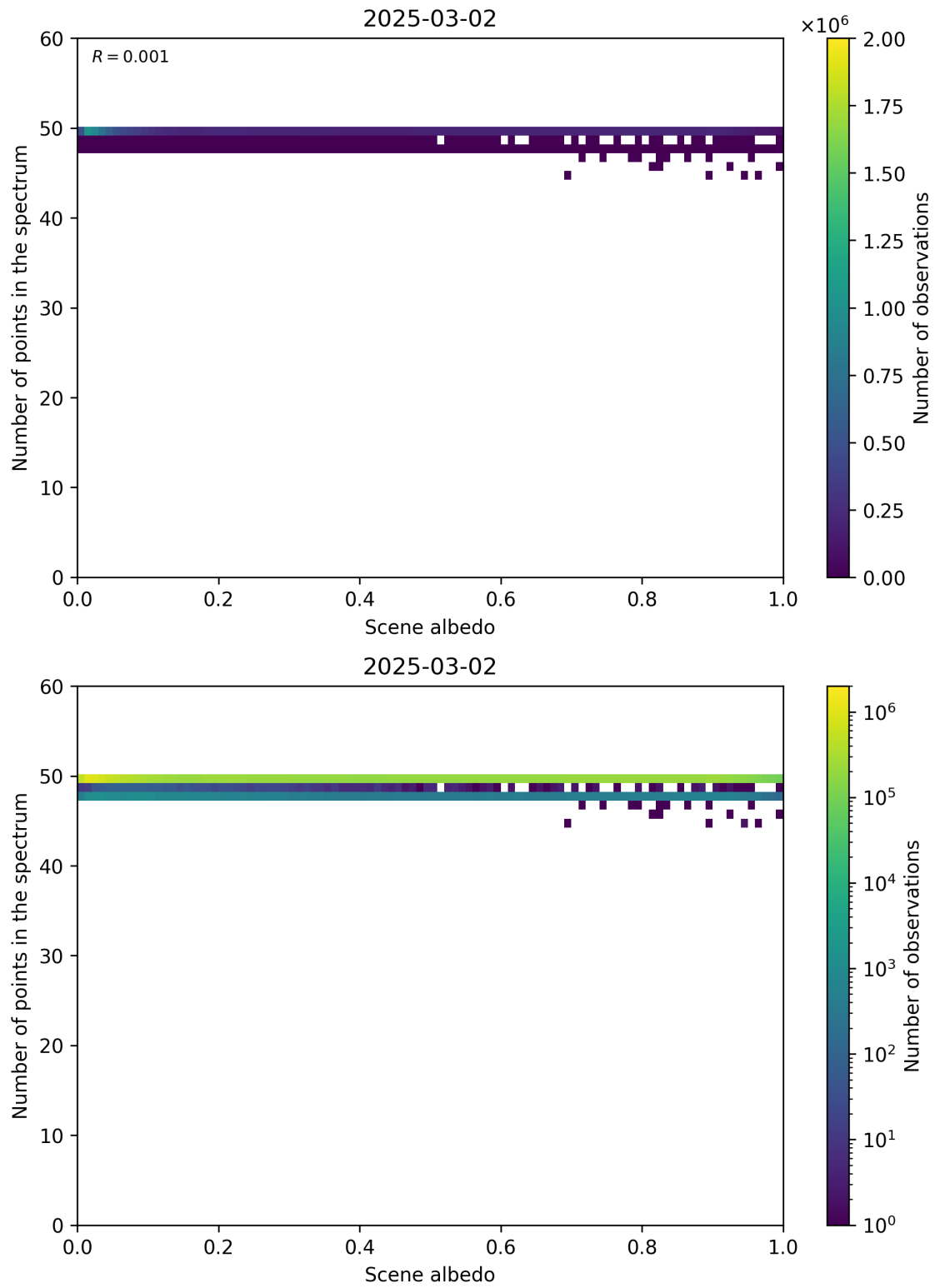
Figure 106: Scatter density plot of “Scene albedo” against “Number of points in the spectrum” for 2025-03-01 to 2025-03-03.
