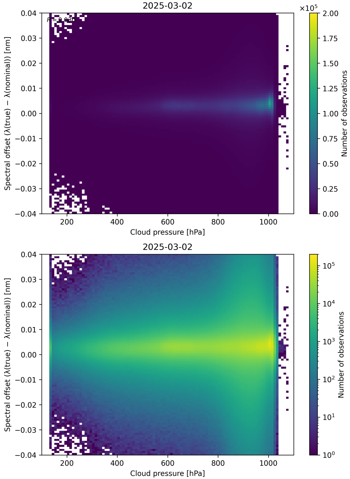
Figure 84: Scatter density plot of “Cloud pressure” against “Spectral offset ( \lambda_{\text{true}} - \lambda_{\text{nominal}} )” for 2025-03-01 to 2025-03-03.
