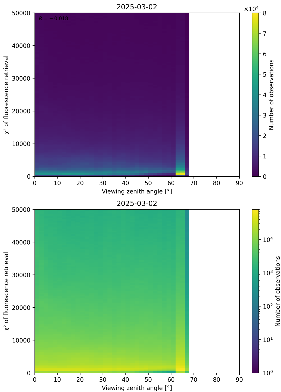
Figure 119: Scatter density plot of “Viewing zenith angle” against “ \chi^2 of fluorescence retrieval” for 2025-03-01 to 2025-03-03.
