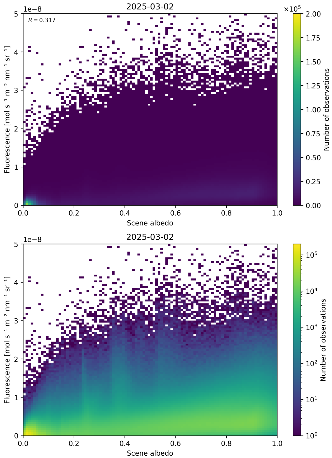
Figure 104: Scatter density plot of “Scene albedo” against “Fluorescence” for 2025-03-01 to 2025-03-03.
