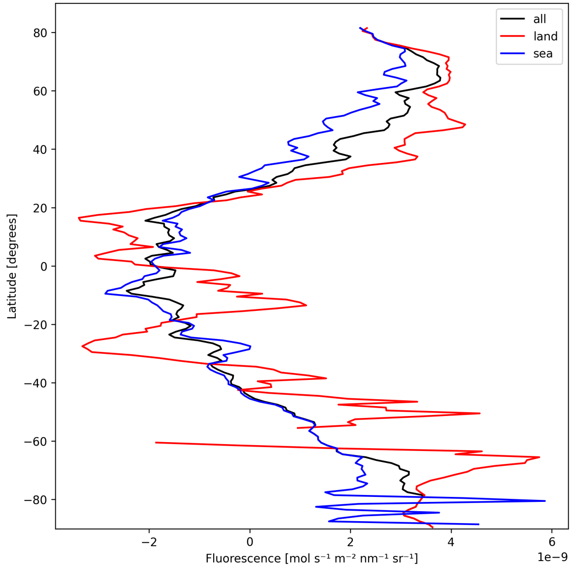
Figure 23: Zonal average of “Fluorescence” for 2025-03-01 to 2025-03-03.
