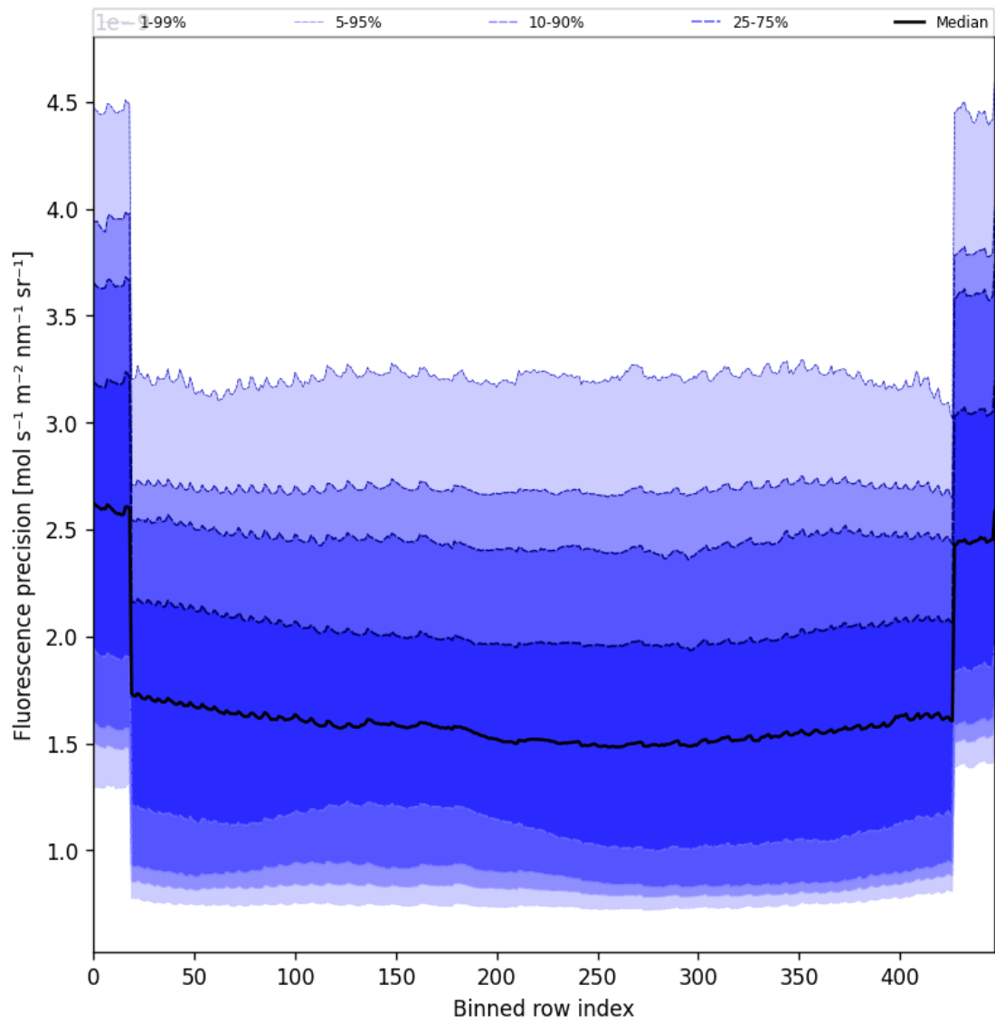
Figure 58: Along track statistics of “Fluorescence precision” for 2025-03-01 to 2025-03-03
