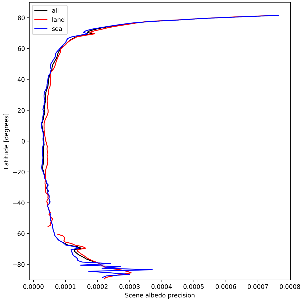
Figure 18: Zonal average of “Scene albedo precision” for 2025-03-01 to 2025-03-03.
