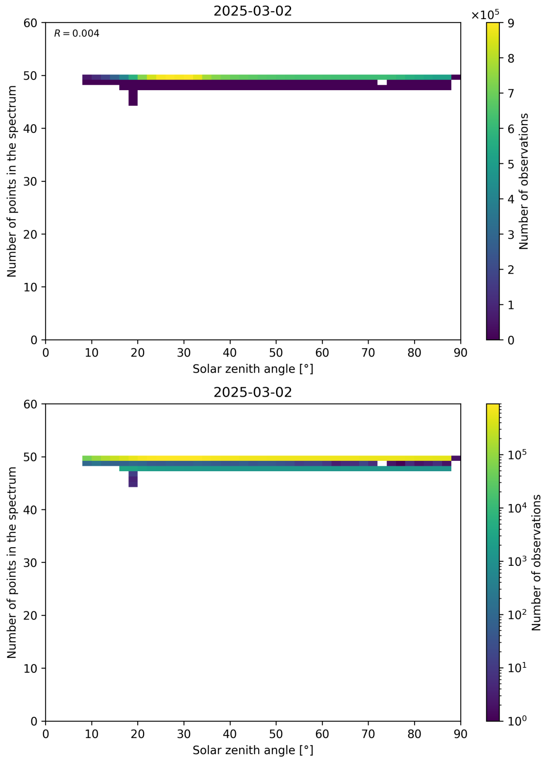
Figure 115: Scatter density plot of “Solar zenith angle” against “Number of points in the spectrum” for 2025-03-01 to 2025-03-03.
