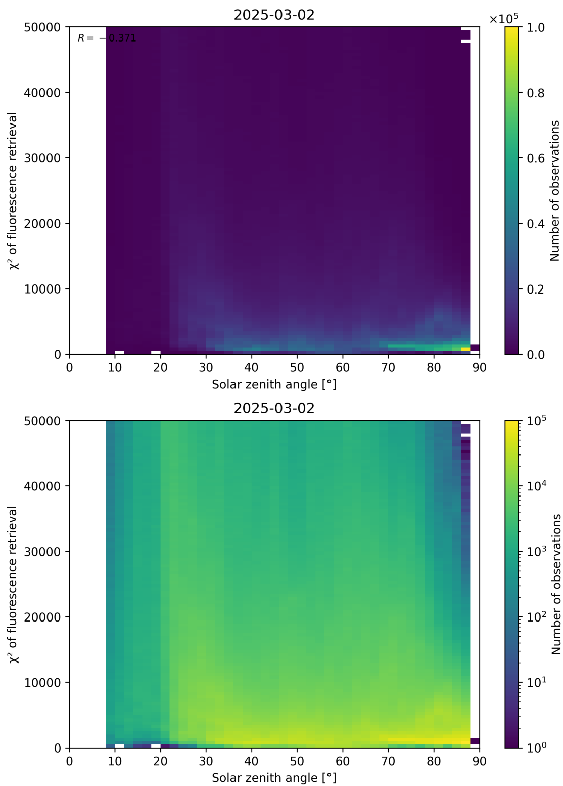
Figure 109: Scatter density plot of “Solar zenith angle” against “ \chi^2 of fluorescence retrieval” for 2025-03-01 to 2025-03-03.
