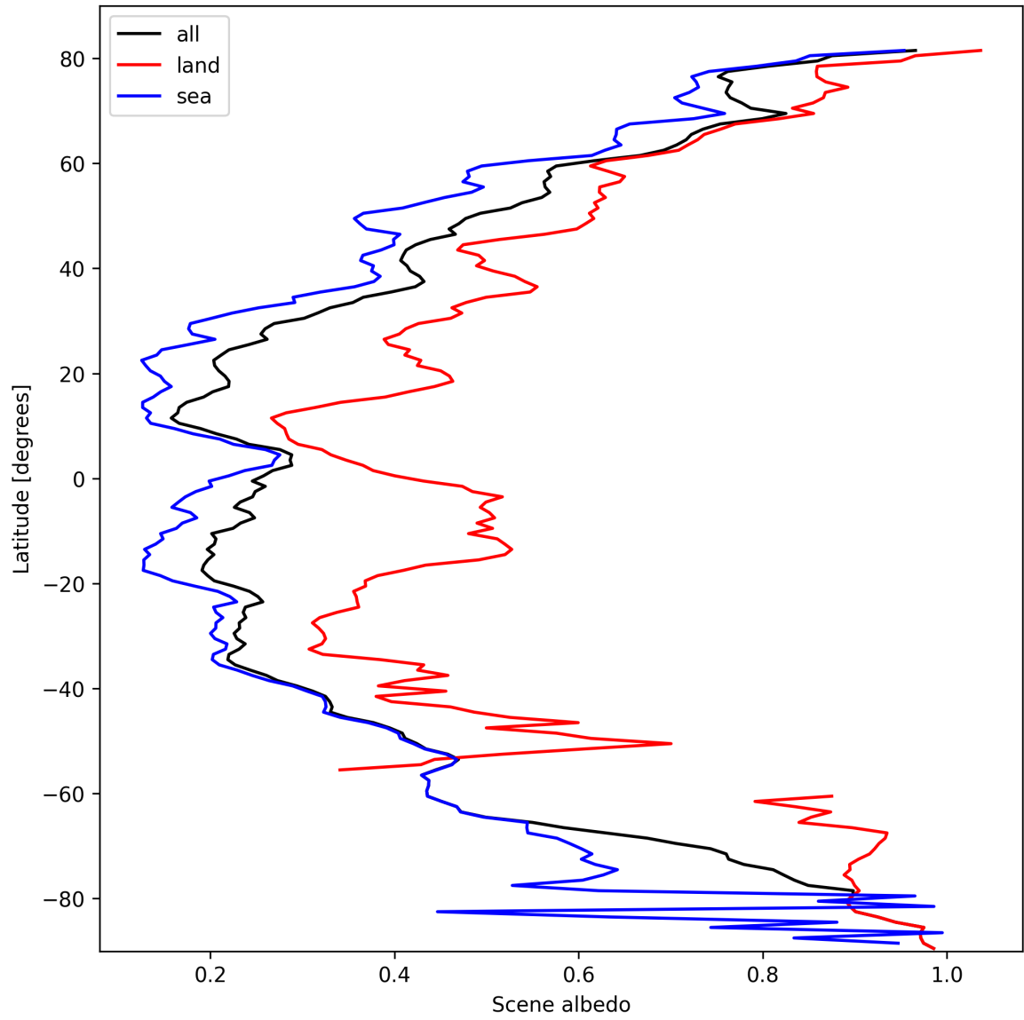
Figure 17: Zonal average of “Scene albedo” for 2025-03-01 to 2025-03-03.
