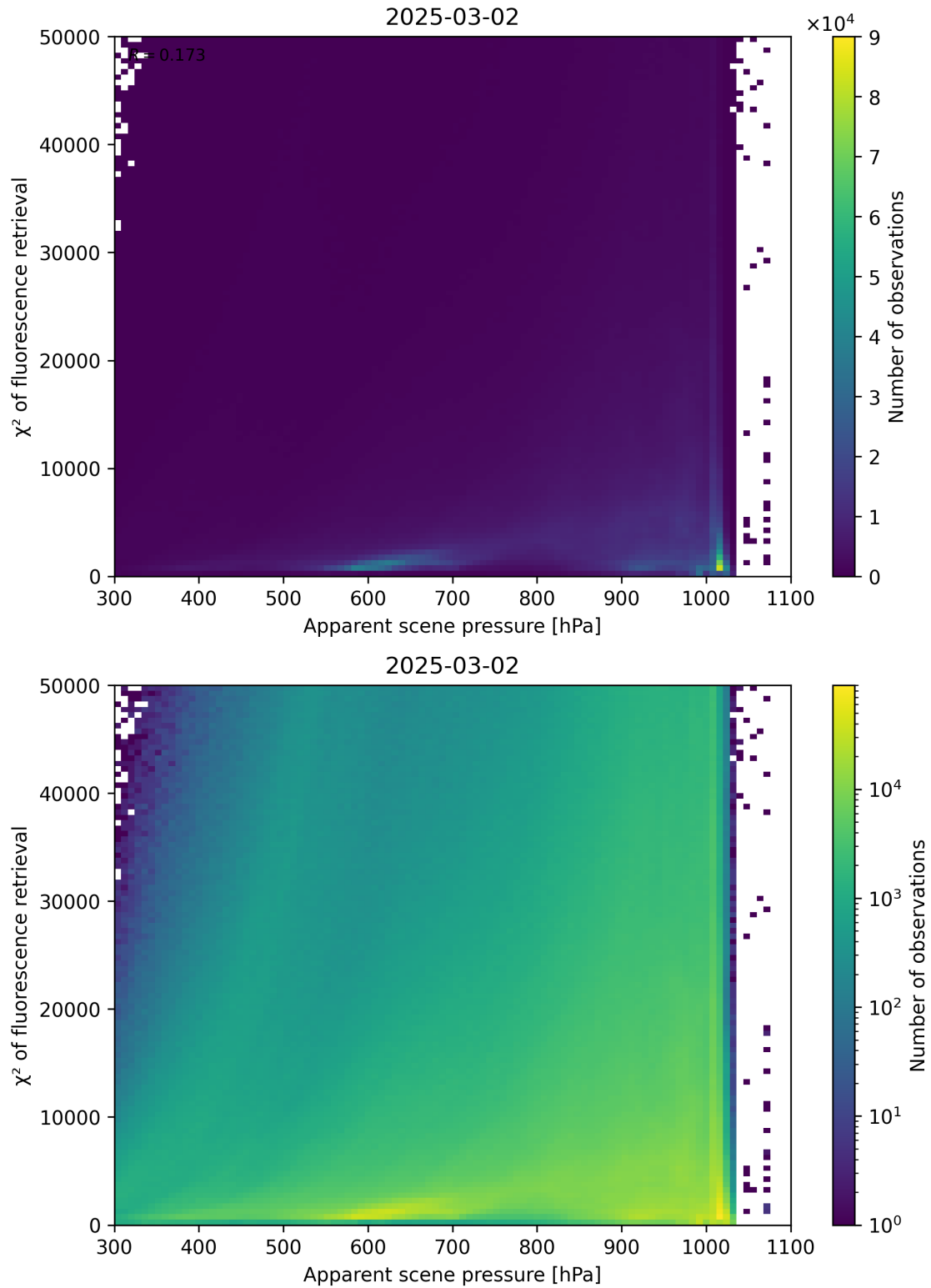
Figure 63: Scatter density plot of “Apparent scene pressure” against “ \chi^2 of fluorescence retrieval” for 2025-03-01 to 2025-03-03.
