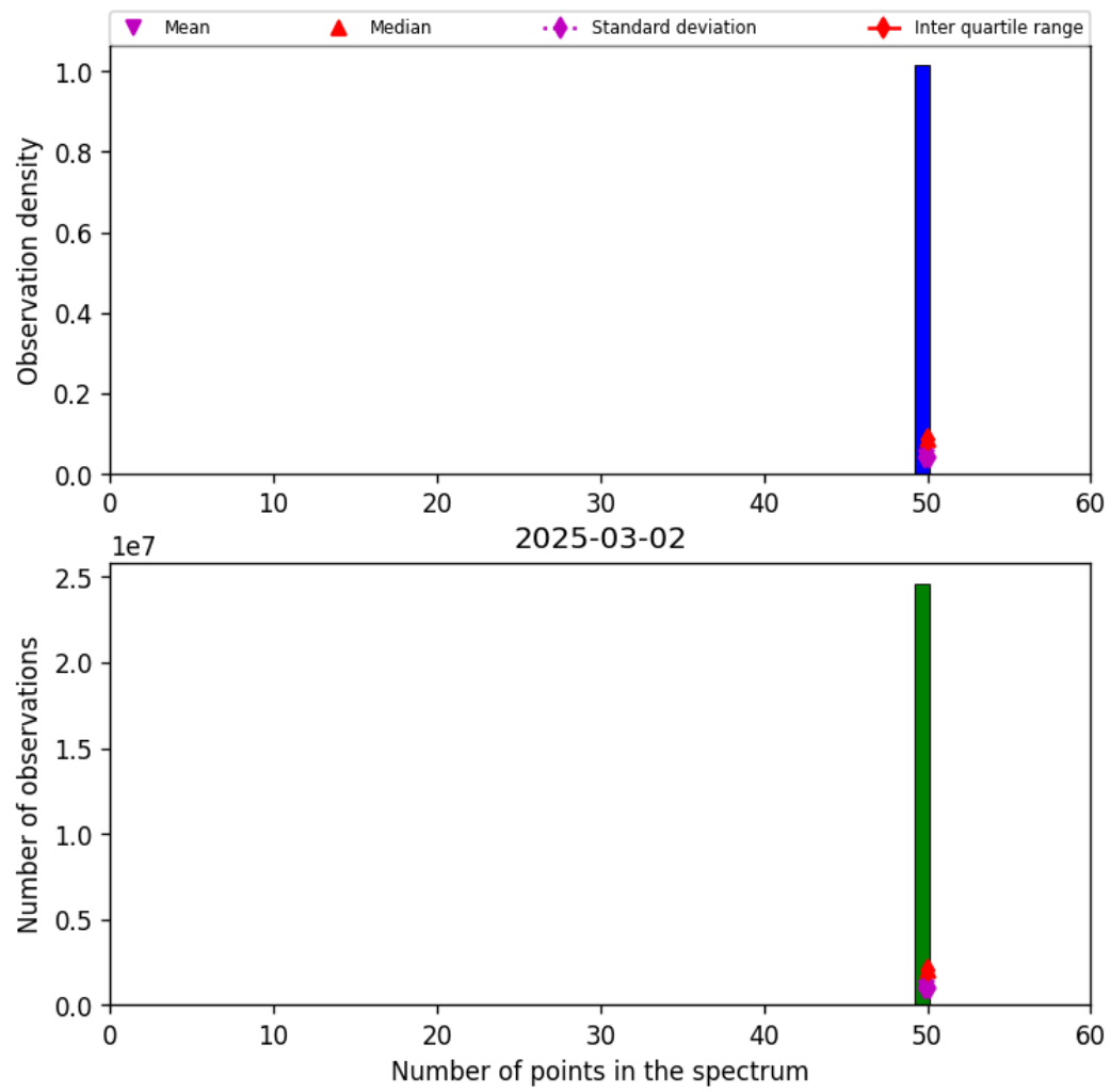
Figure 44: Histogram of “Number of points in the spectrum” for 2025-03-01 to 2025-03-03
