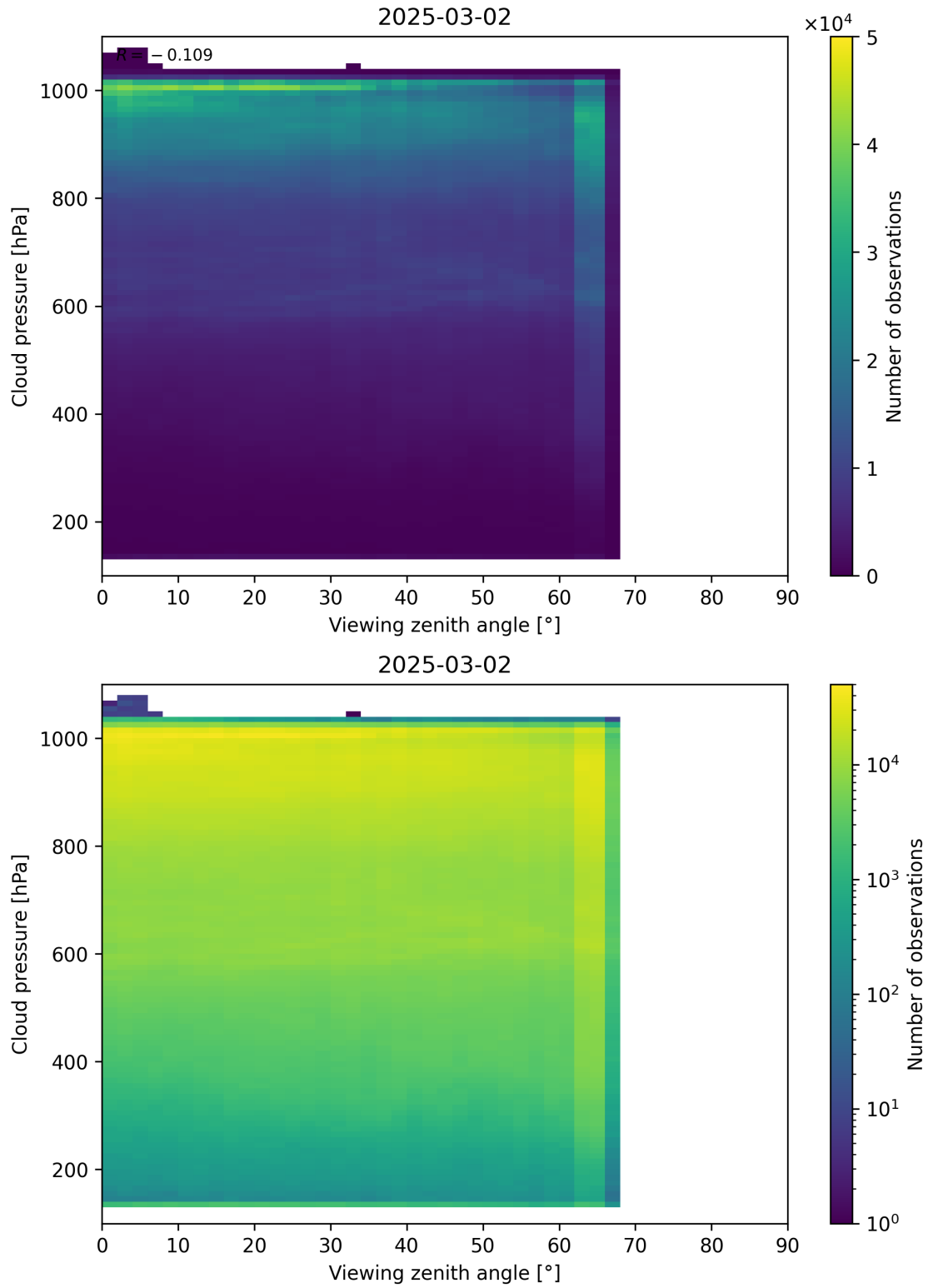
Figure 121: Scatter density plot of “Viewing zenith angle” against “Cloud pressure” for 2025-03-01 to 2025-03-03.
