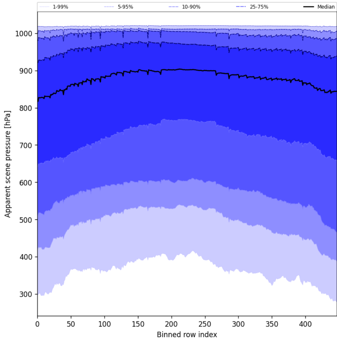
Figure 53: Along track statistics of “Apparent scene pressure” for 2025-03-01 to 2025-03-03
