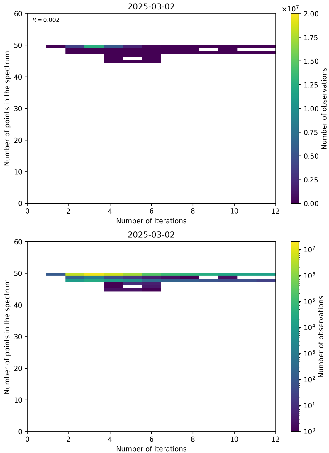
Figure 99: Scatter density plot of “Number of iterations” against “Number of points in the spectrum” for 2025-03-01 to 2025-03-03.
