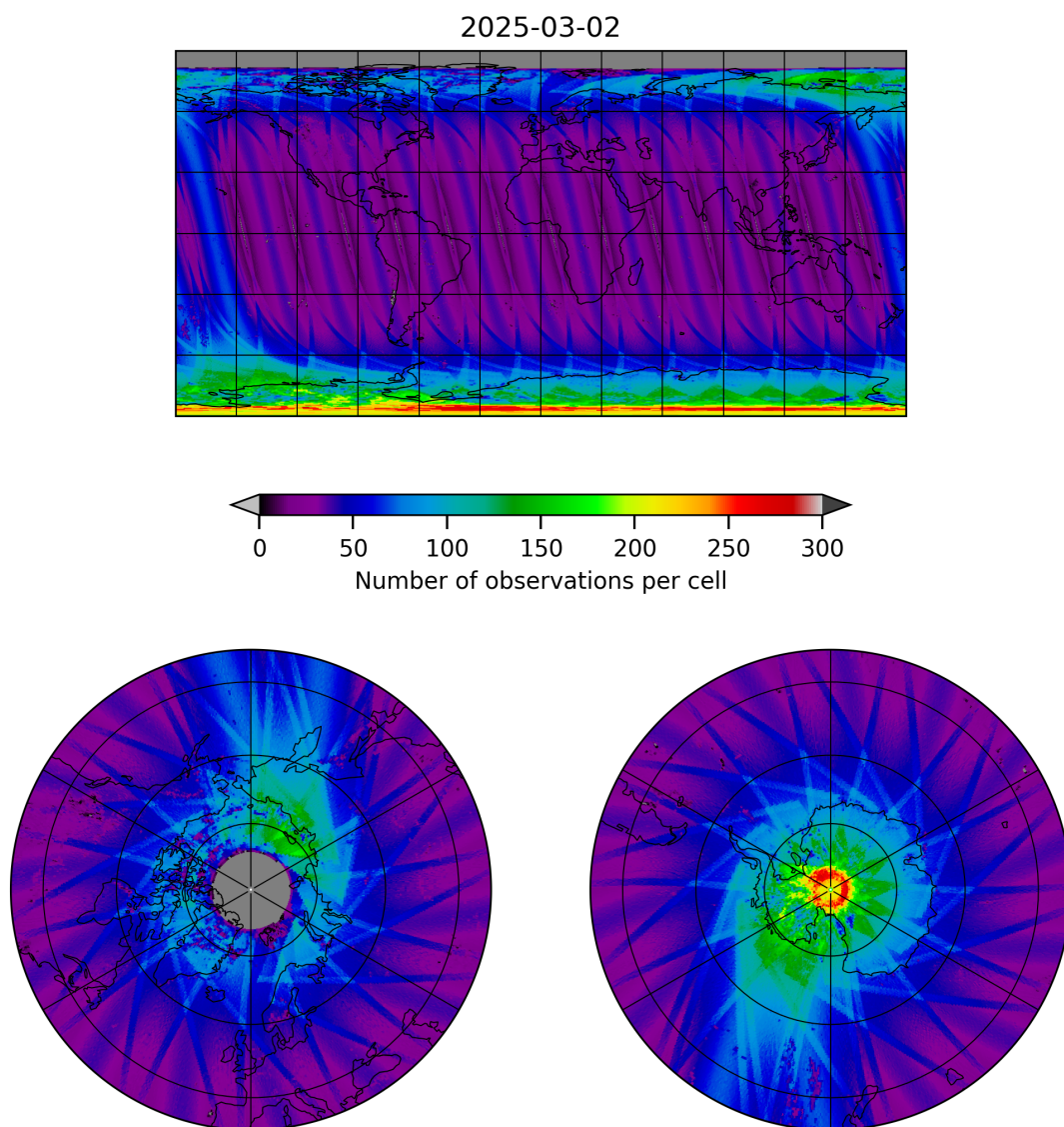
Figure 11: Map of the number of observations for 2025-03-01 to 2025-03-03
