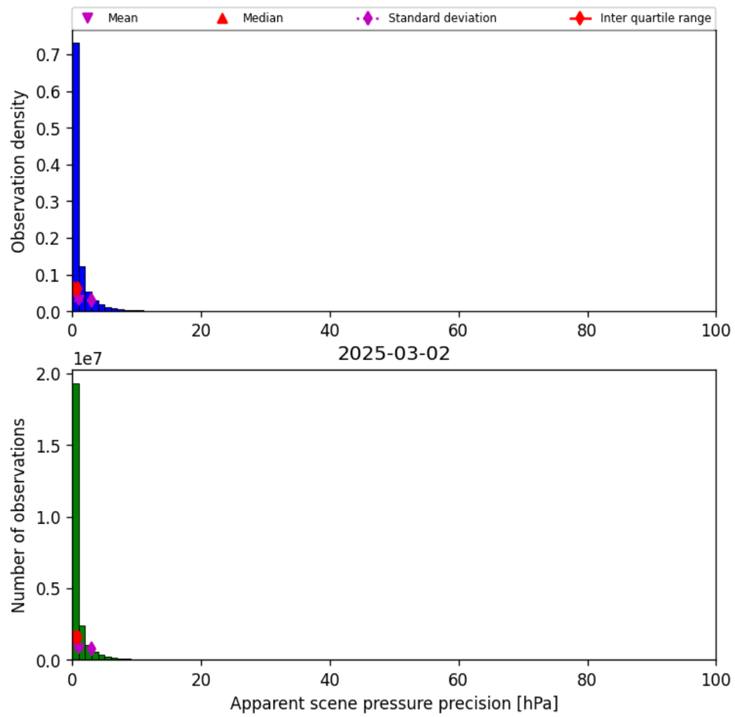
Figure 37: Histogram of “Apparent scene pressure precision” for 2025-03-01 to 2025-03-03
