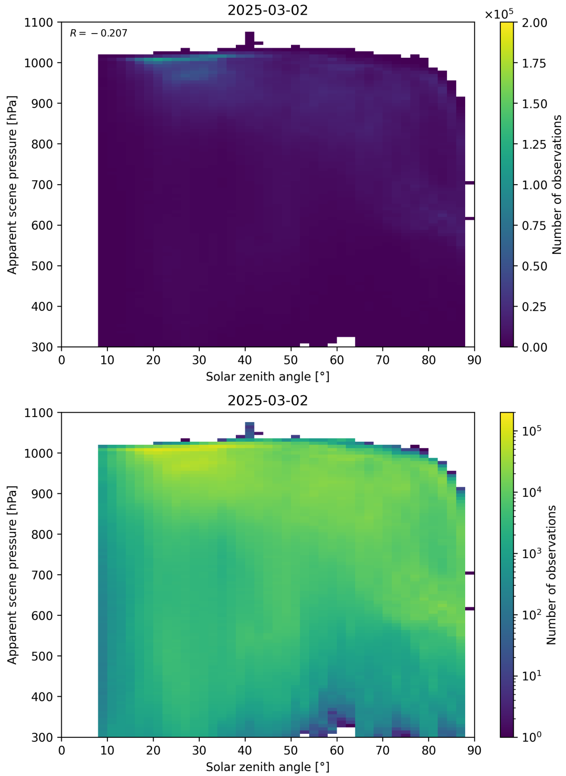
Figure 108: Scatter density plot of “Solar zenith angle” against “Apparent scene pressure” for 2025-03-01 to 2025-03-03.
