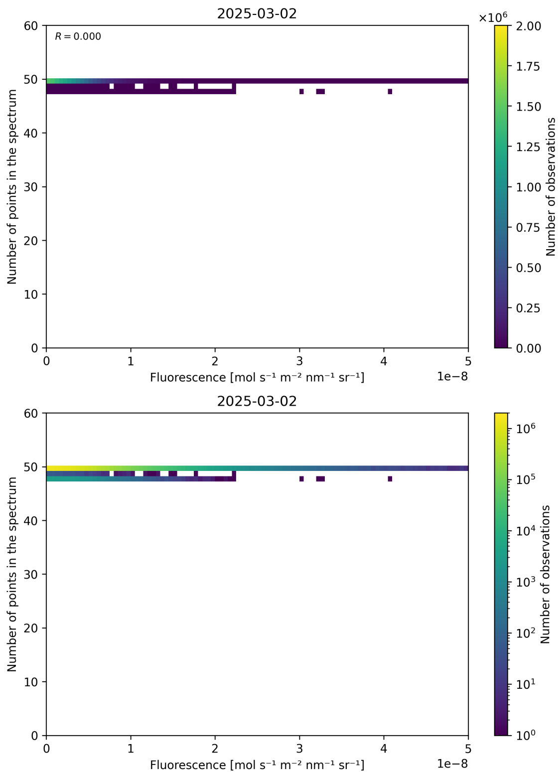
Figure 86: Scatter density plot of “Fluorescence” against “Number of points in the spectrum” for 2025-03-01 to 2025-03-03.
