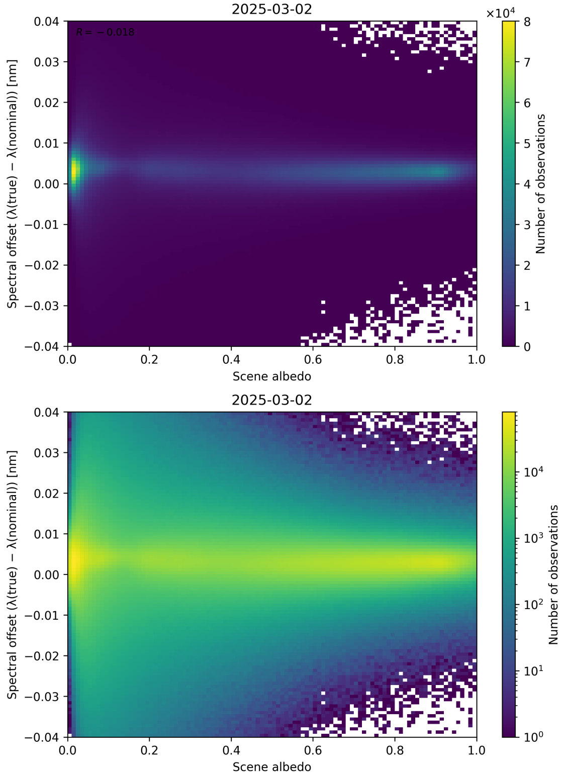
Figure 107: Scatter density plot of “Scene albedo” against “Spectral offset ( \lambda_{\text{true}} - \lambda_{\text{nominal}} )” for 2025-03-01 to 2025-03-03.
