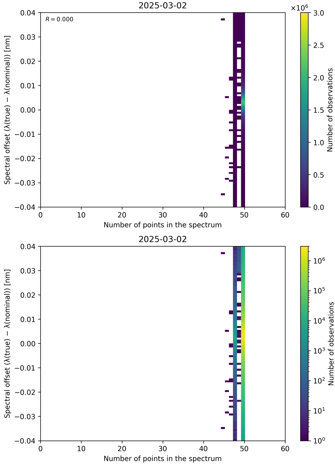
Figure 101: Scatter density plot of “Number of points in the spectrum” against “Spectral offset ( \lambda_{\text{true}} - \lambda_{\text{nominal}} )” for 2025-03-01 to 2025-03-03.
