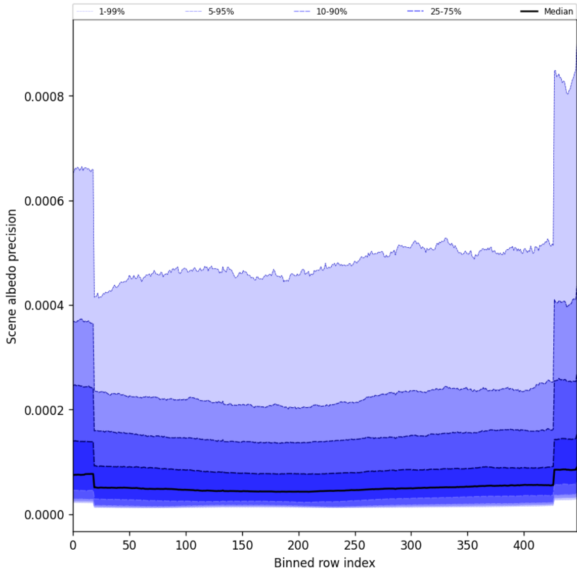
Figure 52: Along track statistics of “Scene albedo precision” for 2025-03-01 to 2025-03-03
