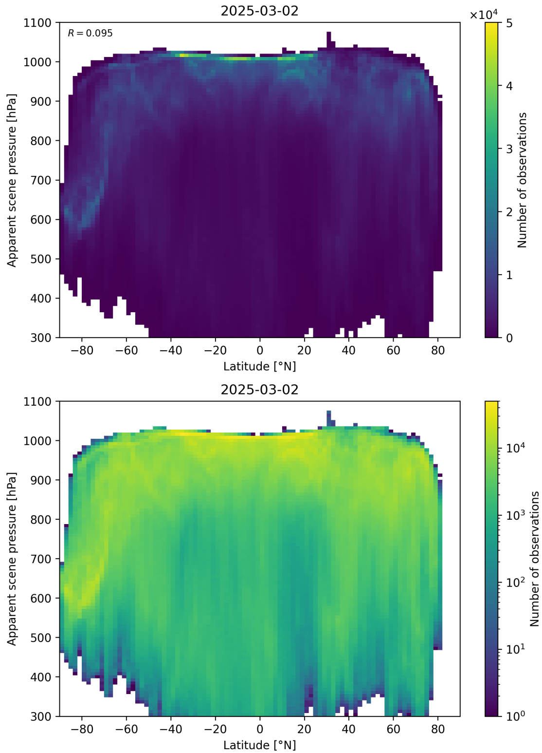
Figure 88: Scatter density plot of “Latitude” against “Apparent scene pressure” for 2025-03-01 to 2025-03-03.
