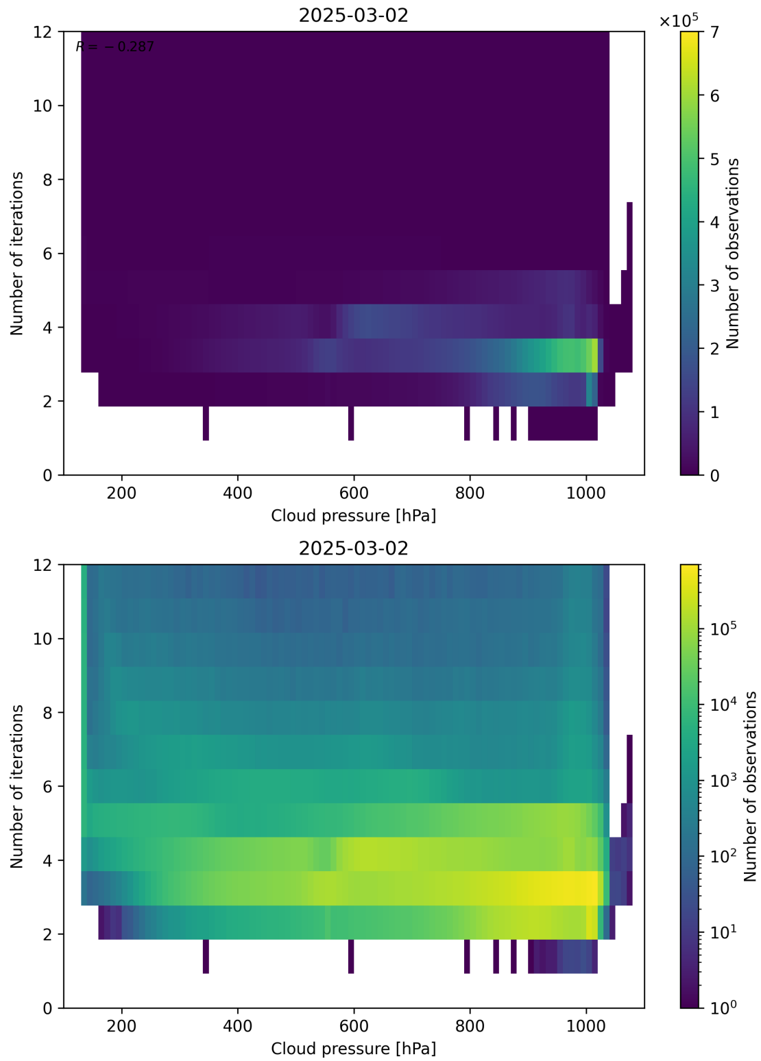
Figure 81: Scatter density plot of “Cloud pressure” against “Number of iterations” for 2025-03-01 to 2025-03-03.
