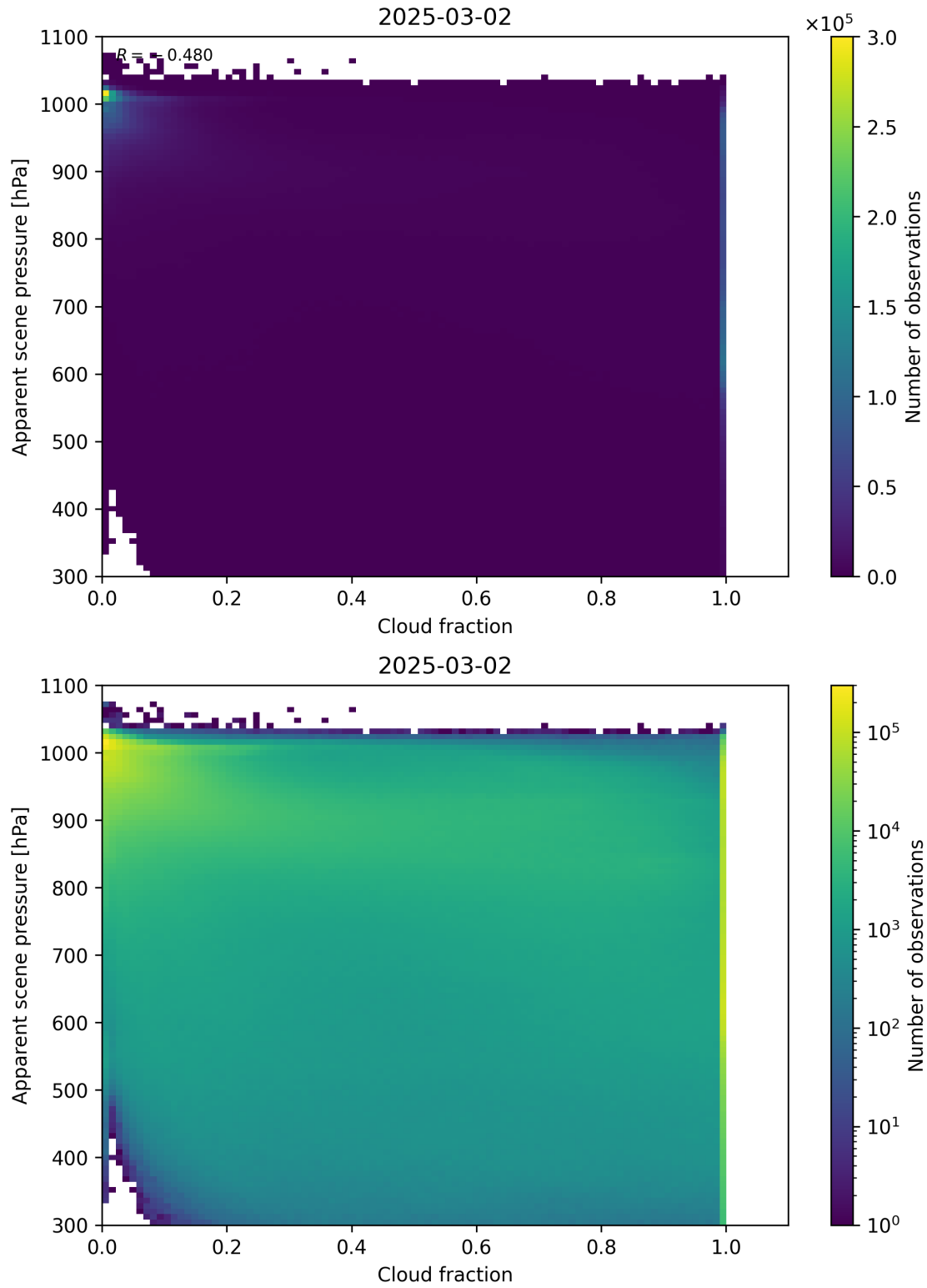
Figure 70: Scatter density plot of “Cloud fraction” against “Apparent scene pressure” for 2025-03-01 to 2025-03-03.
