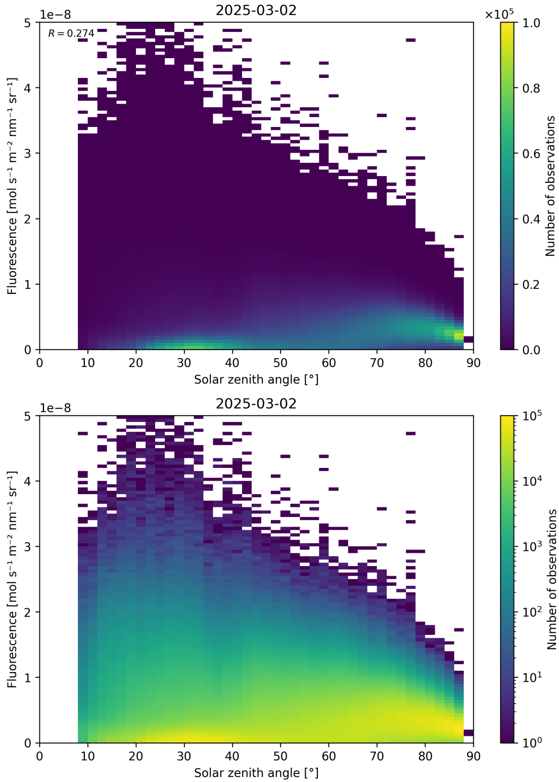
Figure 112: Scatter density plot of “Solar zenith angle” against “Fluorescence” for 2025-03-01 to 2025-03-03.
