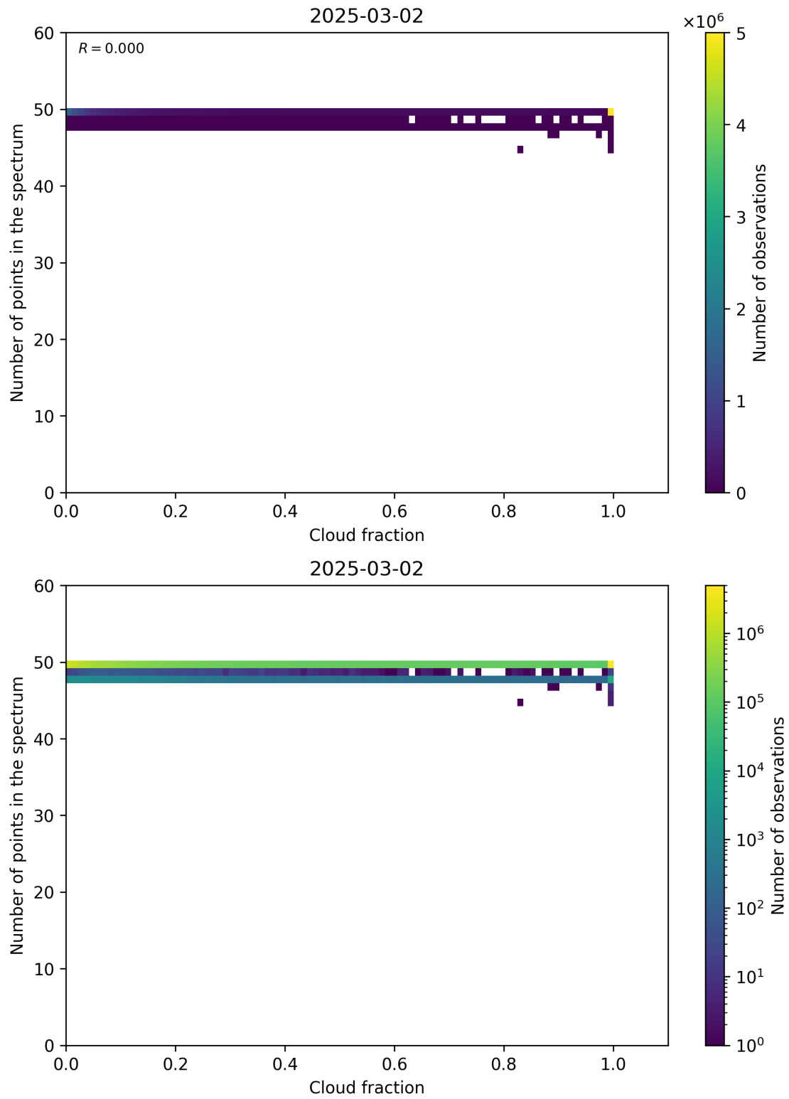
Figure 74: Scatter density plot of “Cloud fraction” against “Number of points in the spectrum” for 2025-03-01 to 2025-03-03.
