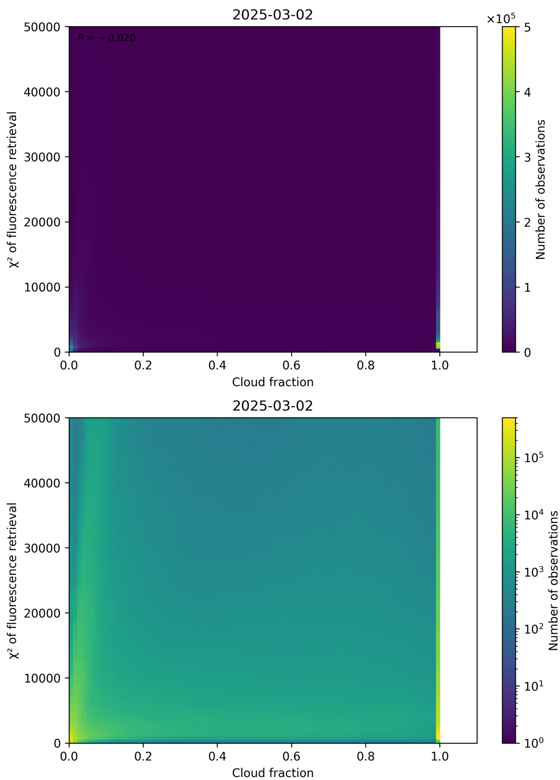
Figure 71: Scatter density plot of “Cloud fraction” against “ \chi^2 of fluorescence retrieval” for 2025-03-01 to 2025-03-03.
