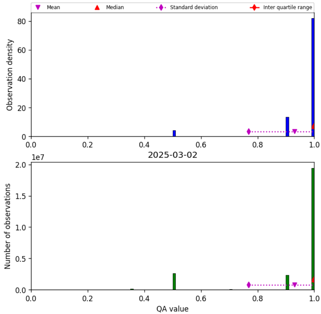
Figure 29: Histogram of “QA value” for 2025-03-01 to 2025-03-03
