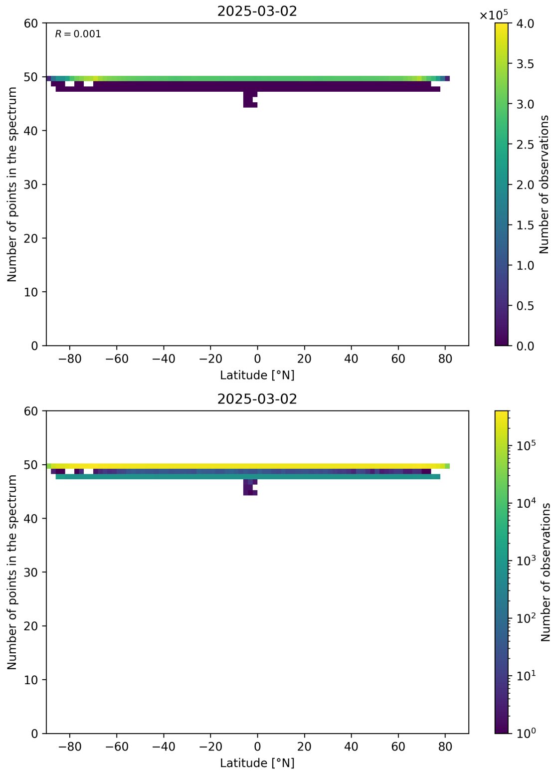
Figure 94: Scatter density plot of “Latitude” against “Number of points in the spectrum” for 2025-03-01 to 2025-03-03.
