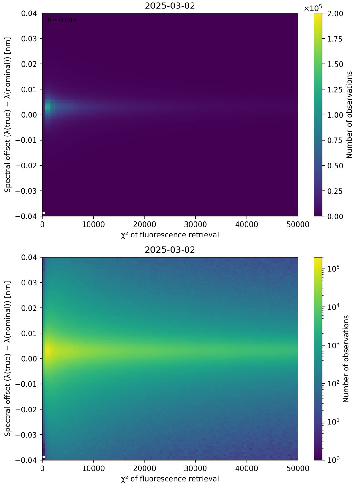
Figure 69: Scatter density plot of “ \chi^2 of fluorescence retrieval” against “Spectral offset ( \lambda_{\text{true}} - \lambda_{\text{nominal}} )” for 2025-03-01 to 2025-03-03.
