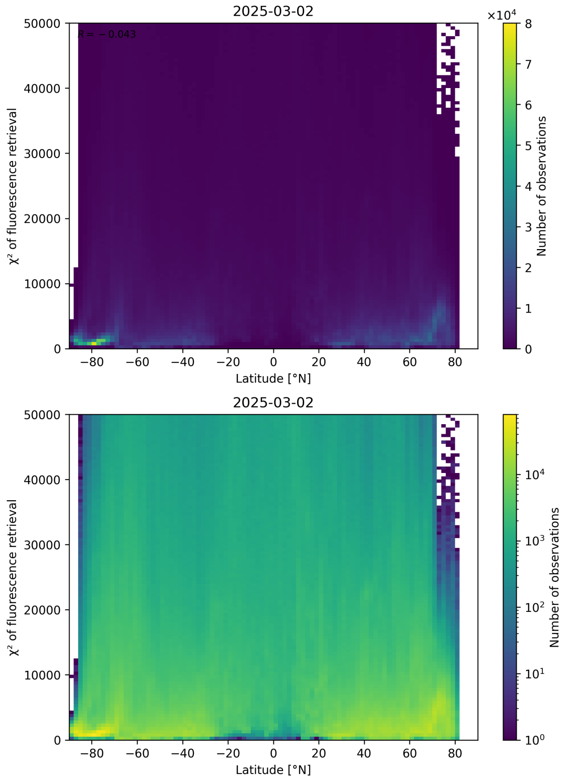
Figure 89: Scatter density plot of “Latitude” against “ \chi^2 of fluorescence retrieval” for 2025-03-01 to 2025-03-03.
