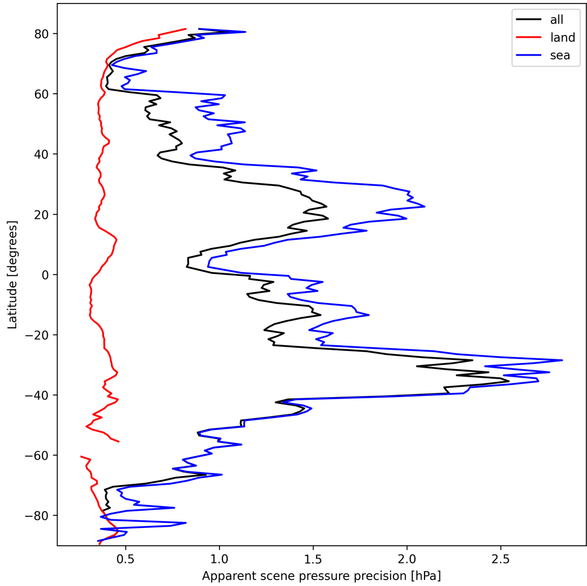
Figure 20: Zonal average of “Apparent scene pressure precision” for 2025-03-01 to 2025-03-03.
