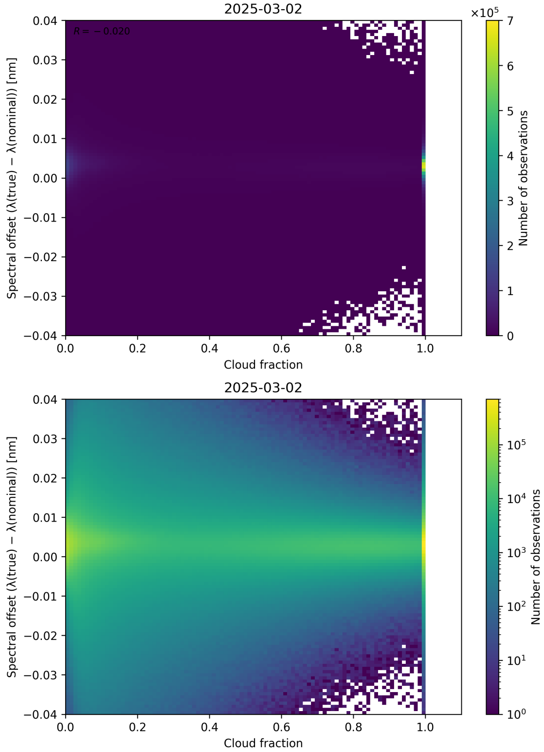
Figure 76: Scatter density plot of “Cloud fraction” against “Spectral offset ( \lambda_{\text{true}} - \lambda_{\text{nominal}} )” for 2025-03-01 to 2025-03-03.
