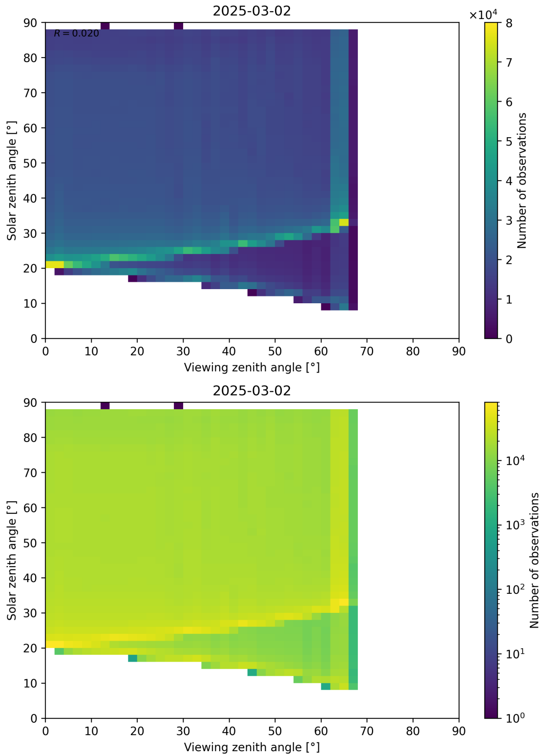
Figure 127: Scatter density plot of “Viewing zenith angle” against “Solar zenith angle” for 2025-03-01 to 2025-03-03.
