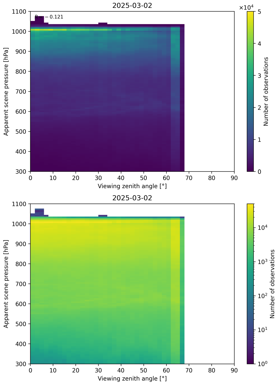
Figure 118: Scatter density plot of “Viewing zenith angle” against “Apparent scene pressure” for 2025-03-01 to 2025-03-03.
