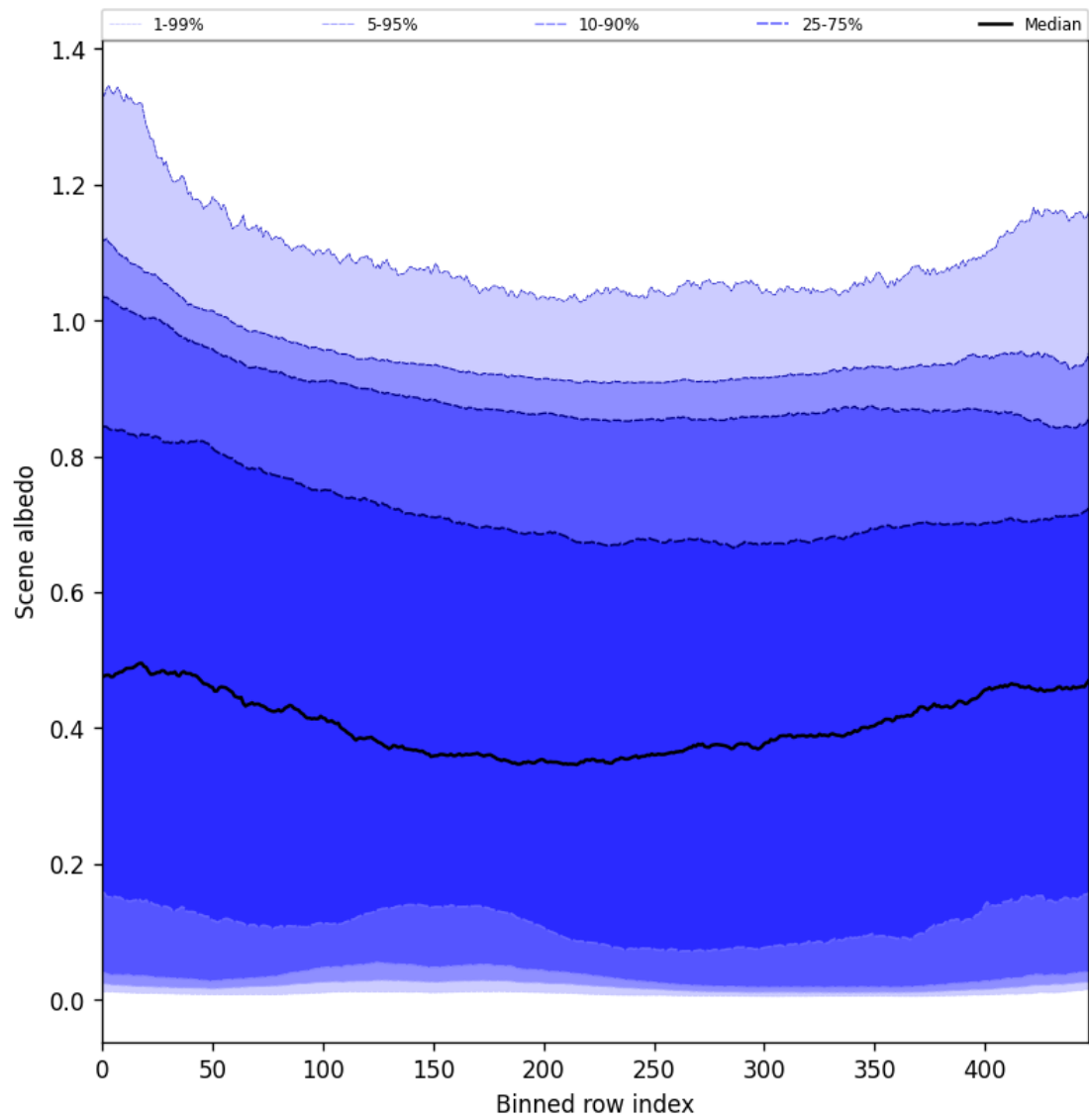
Figure 51: Along track statistics of “Scene albedo” for 2025-03-01 to 2025-03-03
