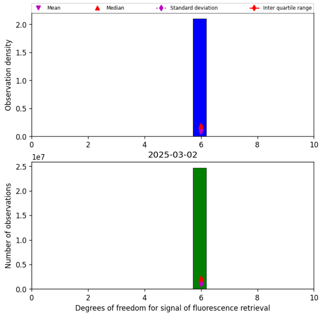
Figure 43: Histogram of "Degrees of freedom for signal of fluorescence retrieval" for 2025-03-01 to 2025-03-03
