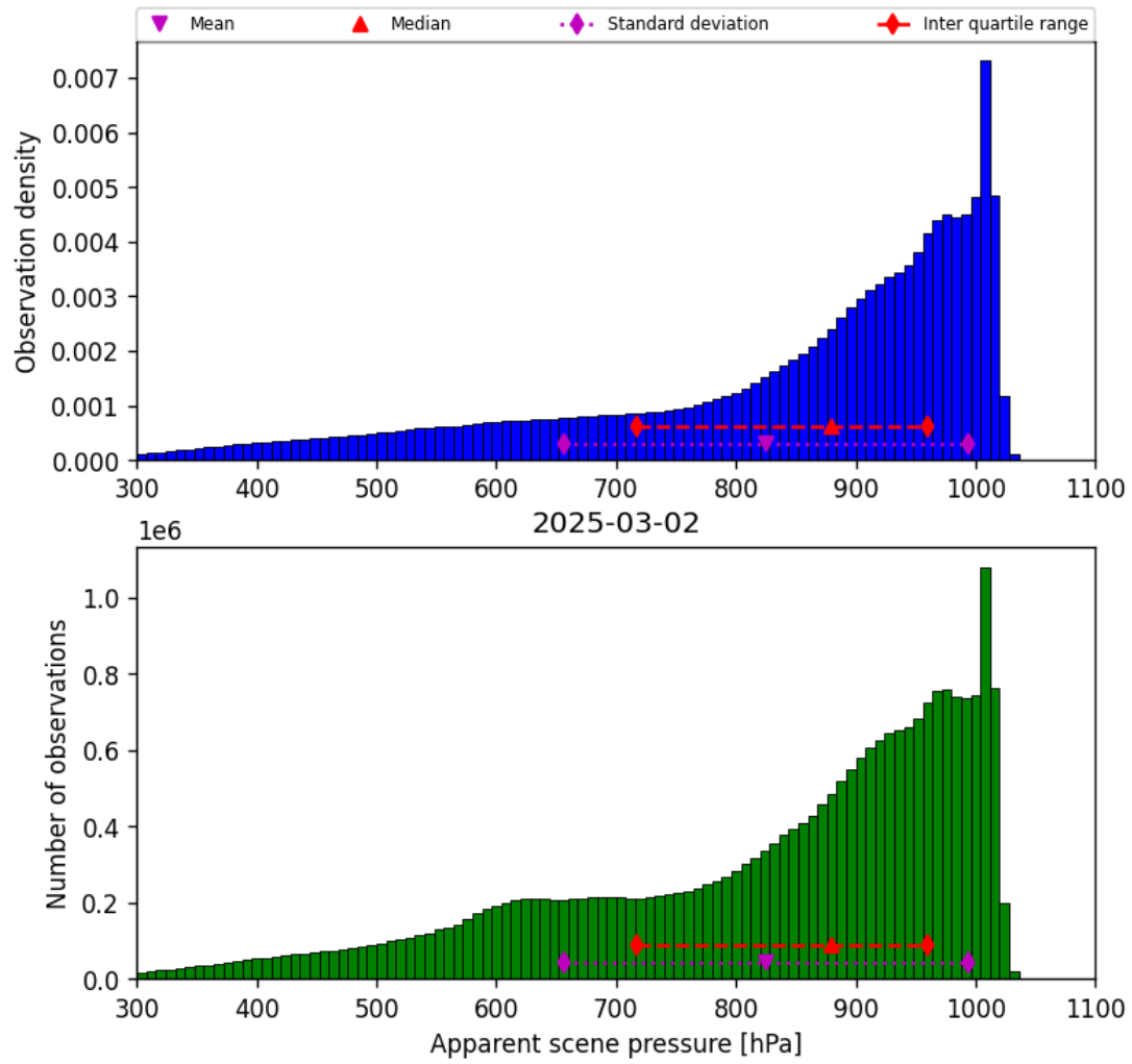
Figure 36: Histogram of “Apparent scene pressure” for 2025-03-01 to 2025-03-03
