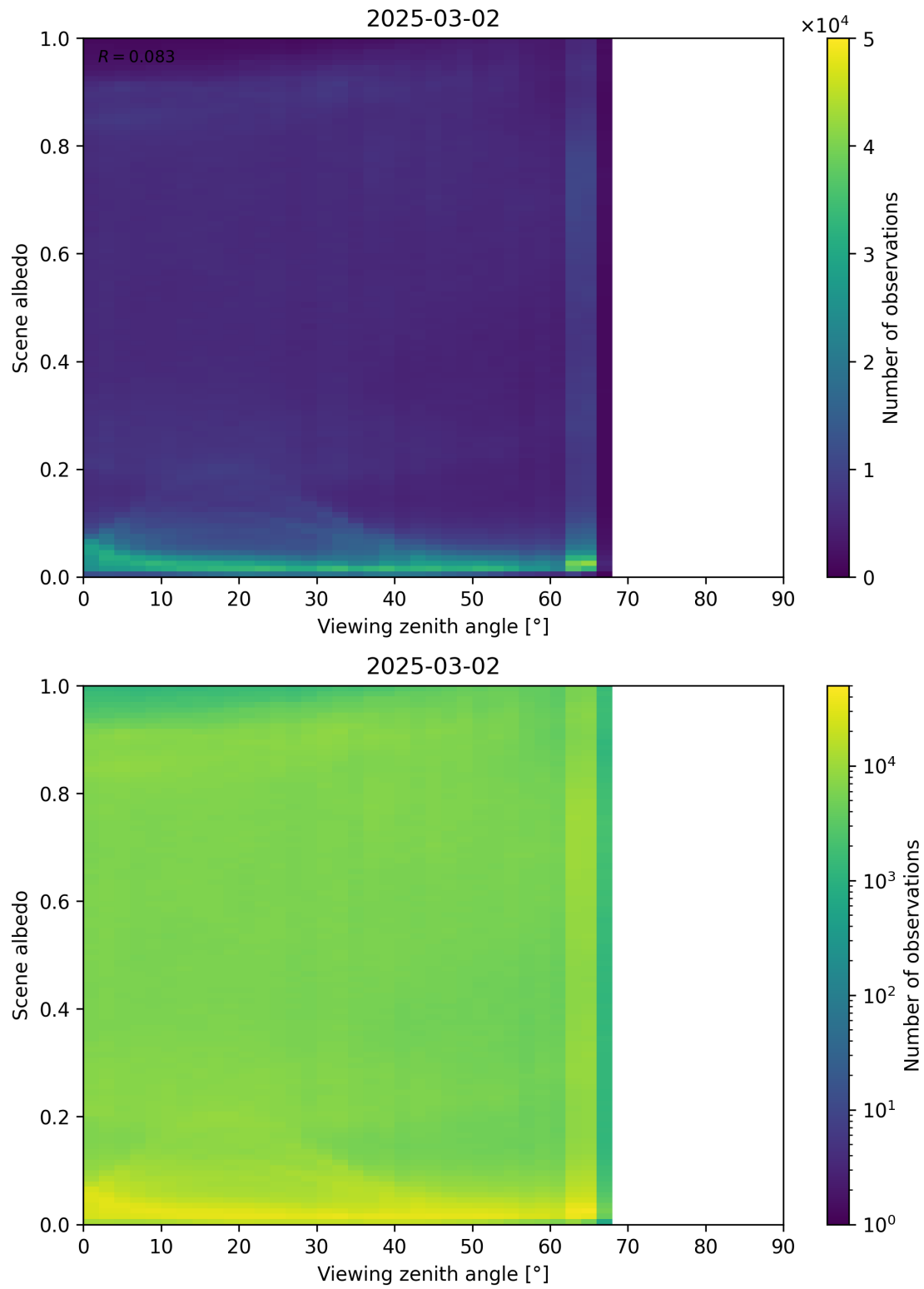
Figure 126: Scatter density plot of “Viewing zenith angle” against “Scene albedo” for 2025-03-01 to 2025-03-03.
