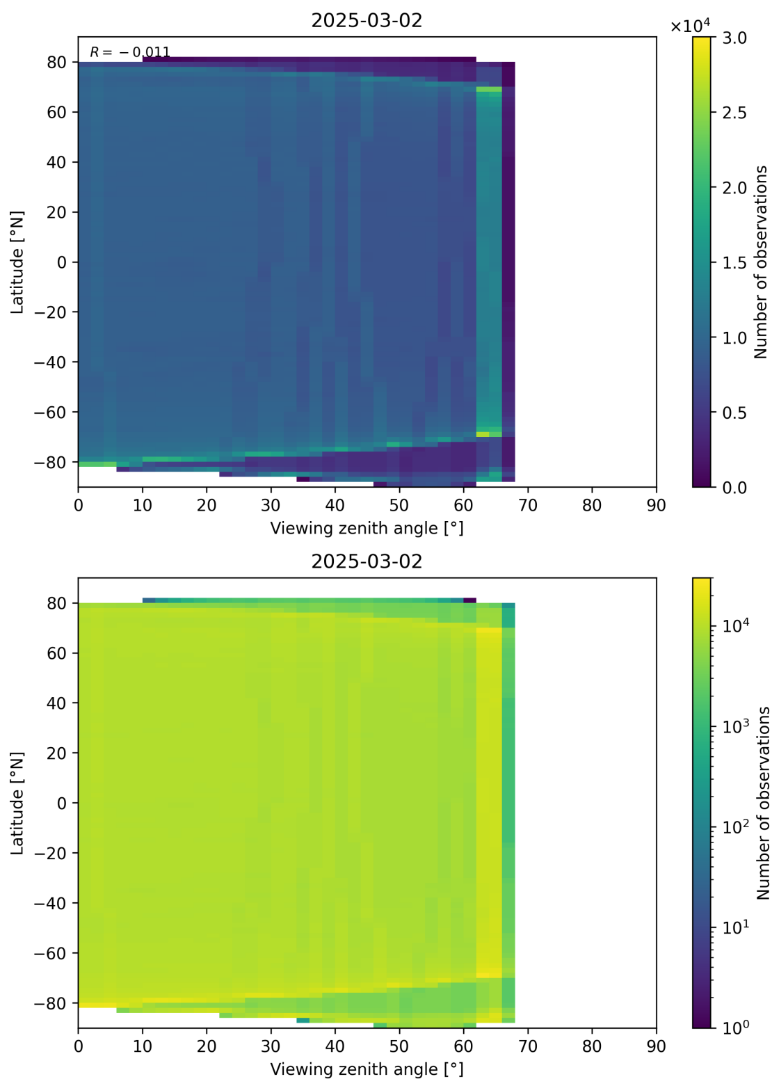
Figure 123: Scatter density plot of “Viewing zenith angle” against “Latitude” for 2025-03-01 to 2025-03-03.
