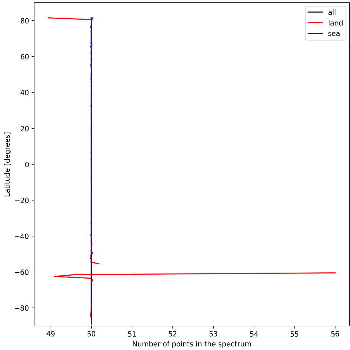
Figure 27: Zonal average of “Number of points in the spectrum” for 2025-03-01 to 2025-03-03.
