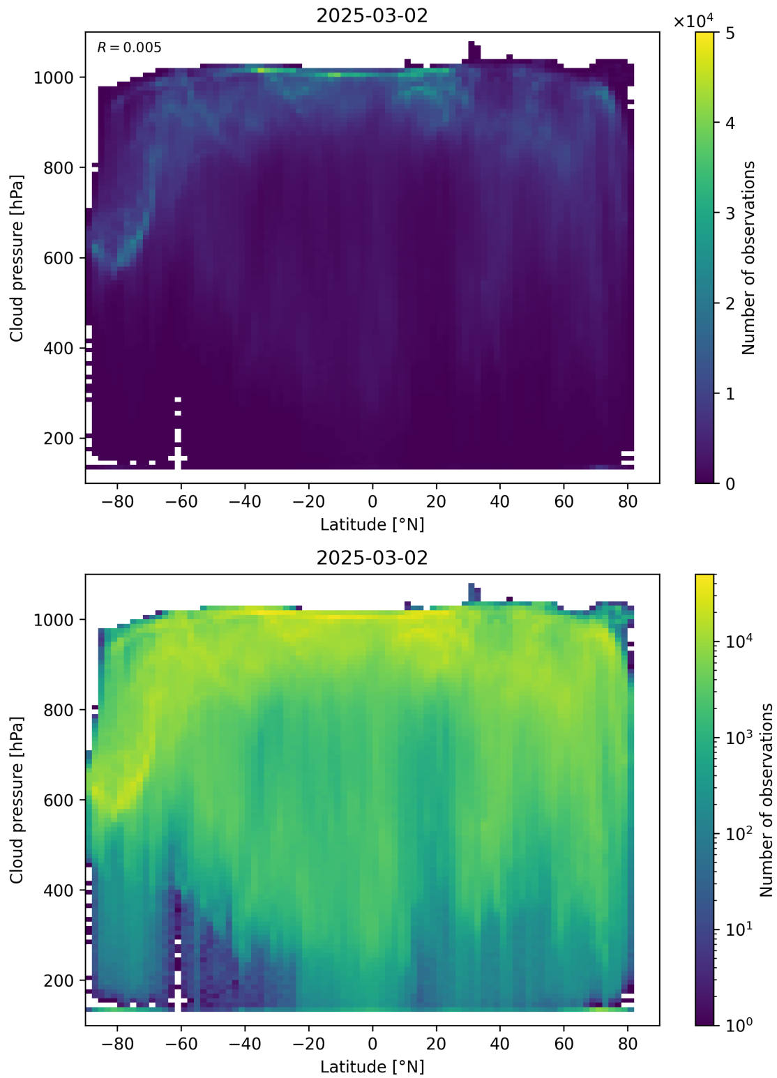
Figure 91: Scatter density plot of “Latitude” against “Cloud pressure” for 2025-03-01 to 2025-03-03.
