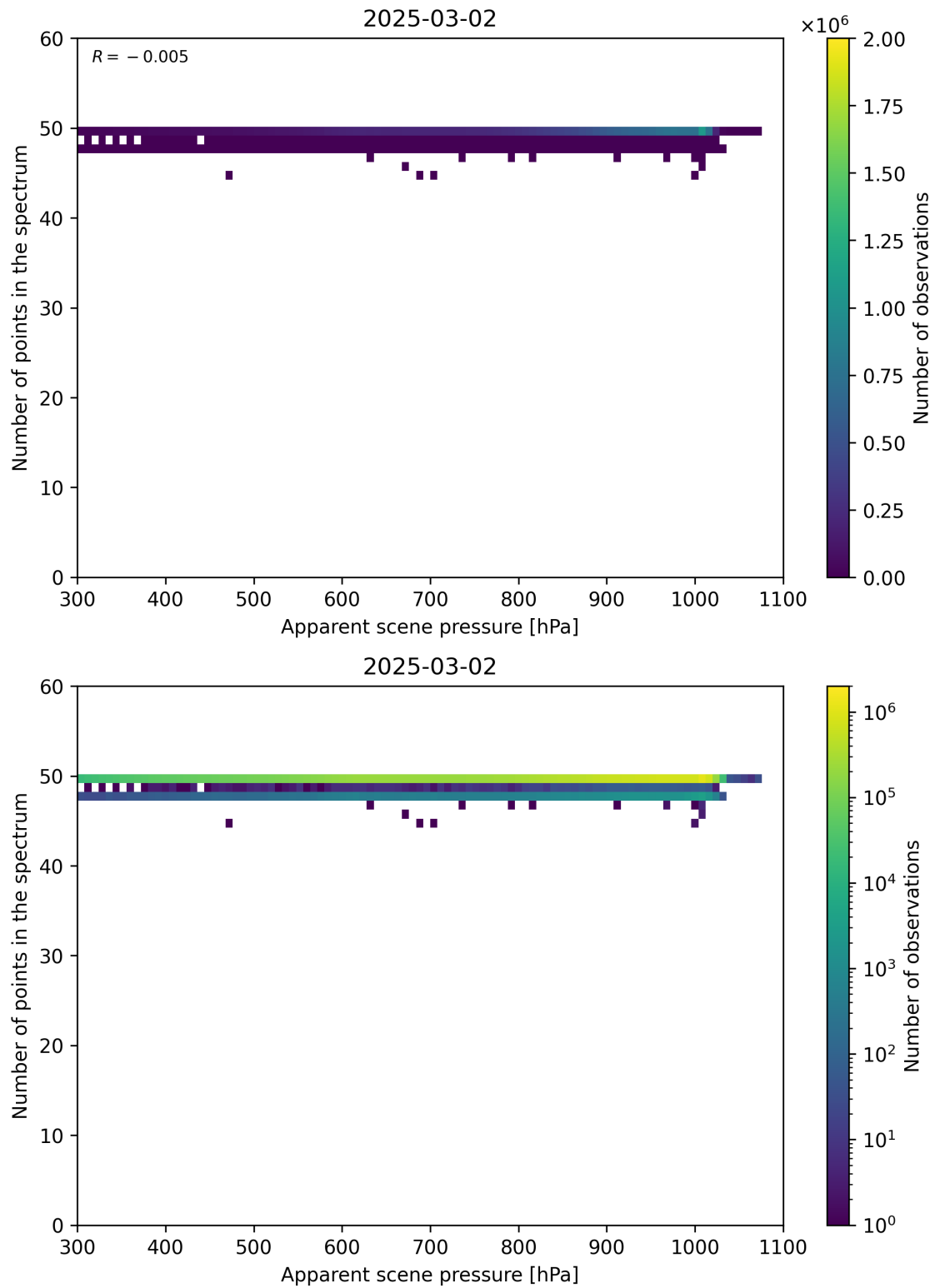
Figure 66: Scatter density plot of “Apparent scene pressure” against “Number of points in the spectrum” for 2025-03-01 to 2025-03-03.
