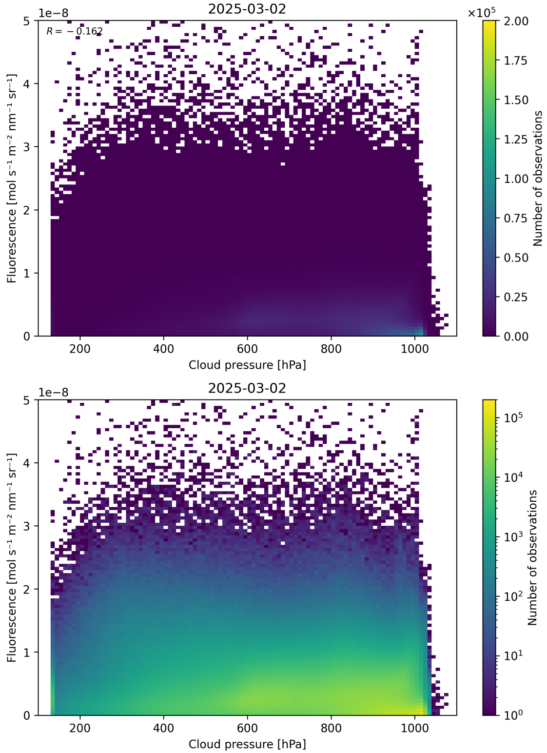
Figure 80: Scatter density plot of “Cloud pressure” against “Fluorescence” for 2025-03-01 to 2025-03-03.
