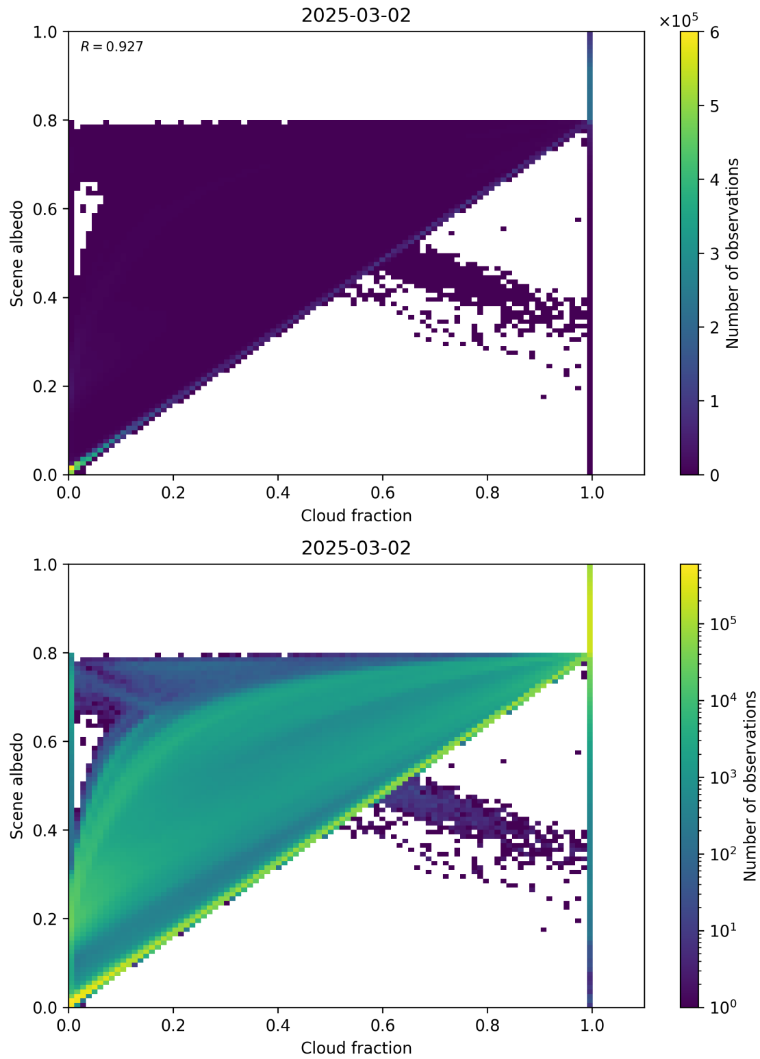
Figure 75: Scatter density plot of “Cloud fraction” against “Scene albedo” for 2025-03-01 to 2025-03-03.
