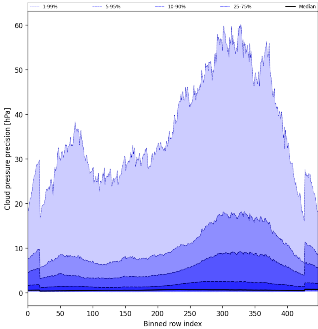
Figure 48: Along track statistics of “Cloud pressure precision” for 2025-03-01 to 2025-03-03
