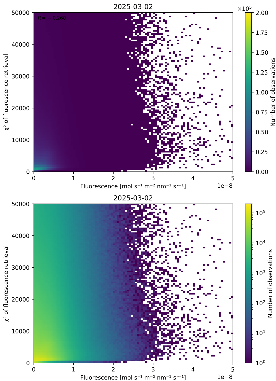
Figure 85: Scatter density plot of “Fluorescence” against “ \chi^2 of fluorescence retrieval” for 2025-03-01 to 2025-03-03.
