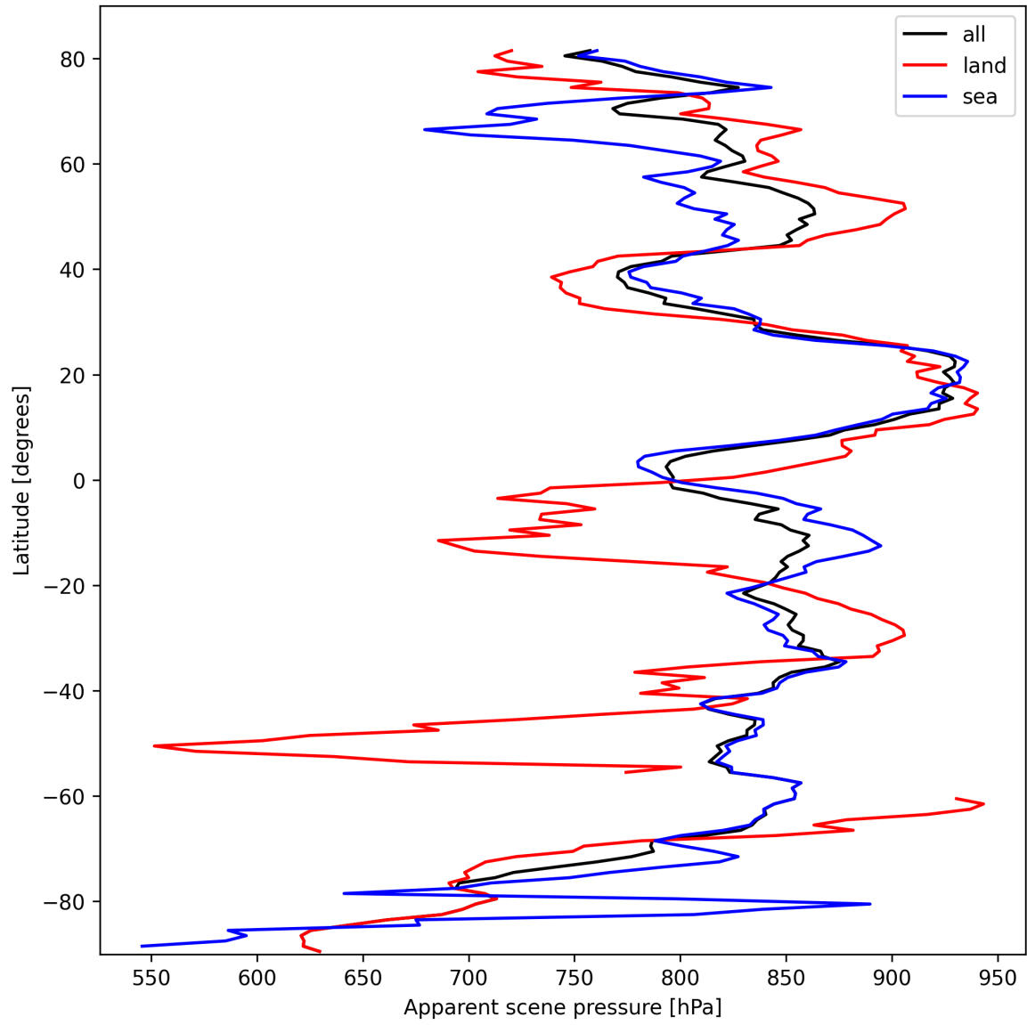
Figure 19: Zonal average of “Apparent scene pressure” for 2025-03-01 to 2025-03-03.
