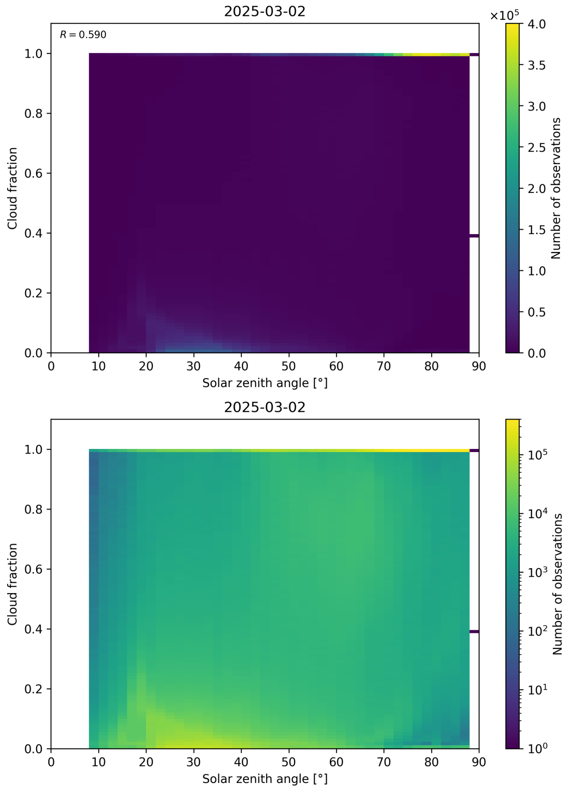
Figure 110: Scatter density plot of “Solar zenith angle” against “Cloud fraction” for 2025-03-01 to 2025-03-03.
