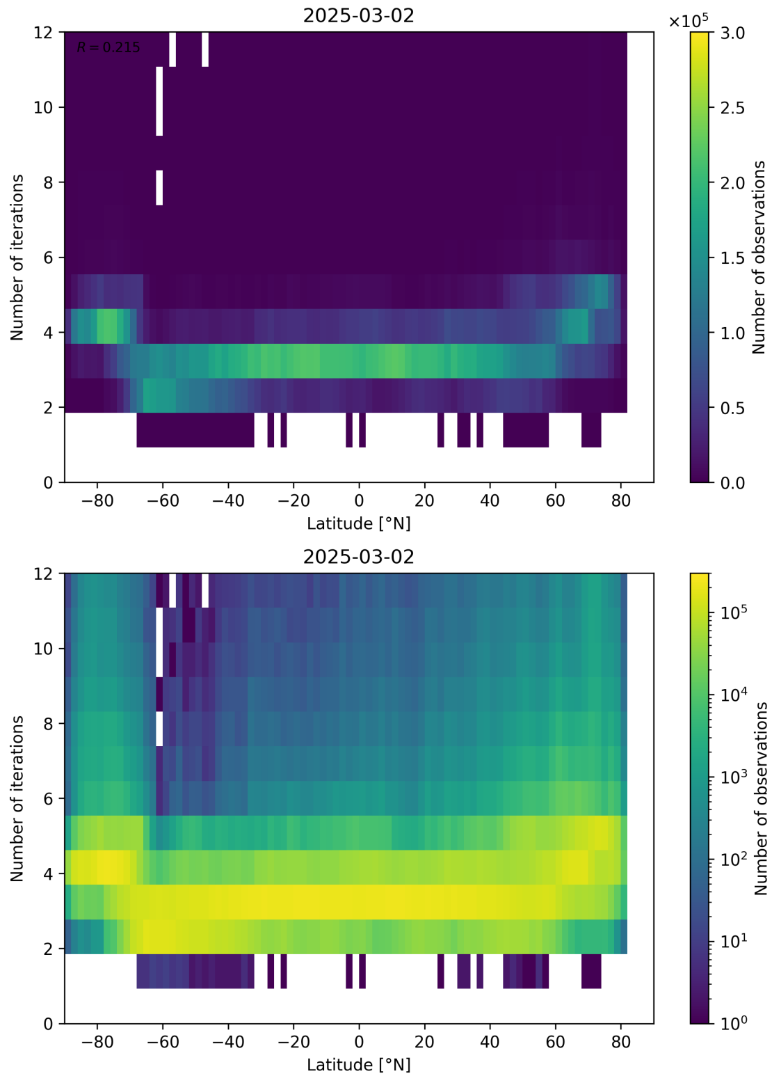
Figure 93: Scatter density plot of “Latitude” against “Number of iterations” for 2025-03-01 to 2025-03-03.
