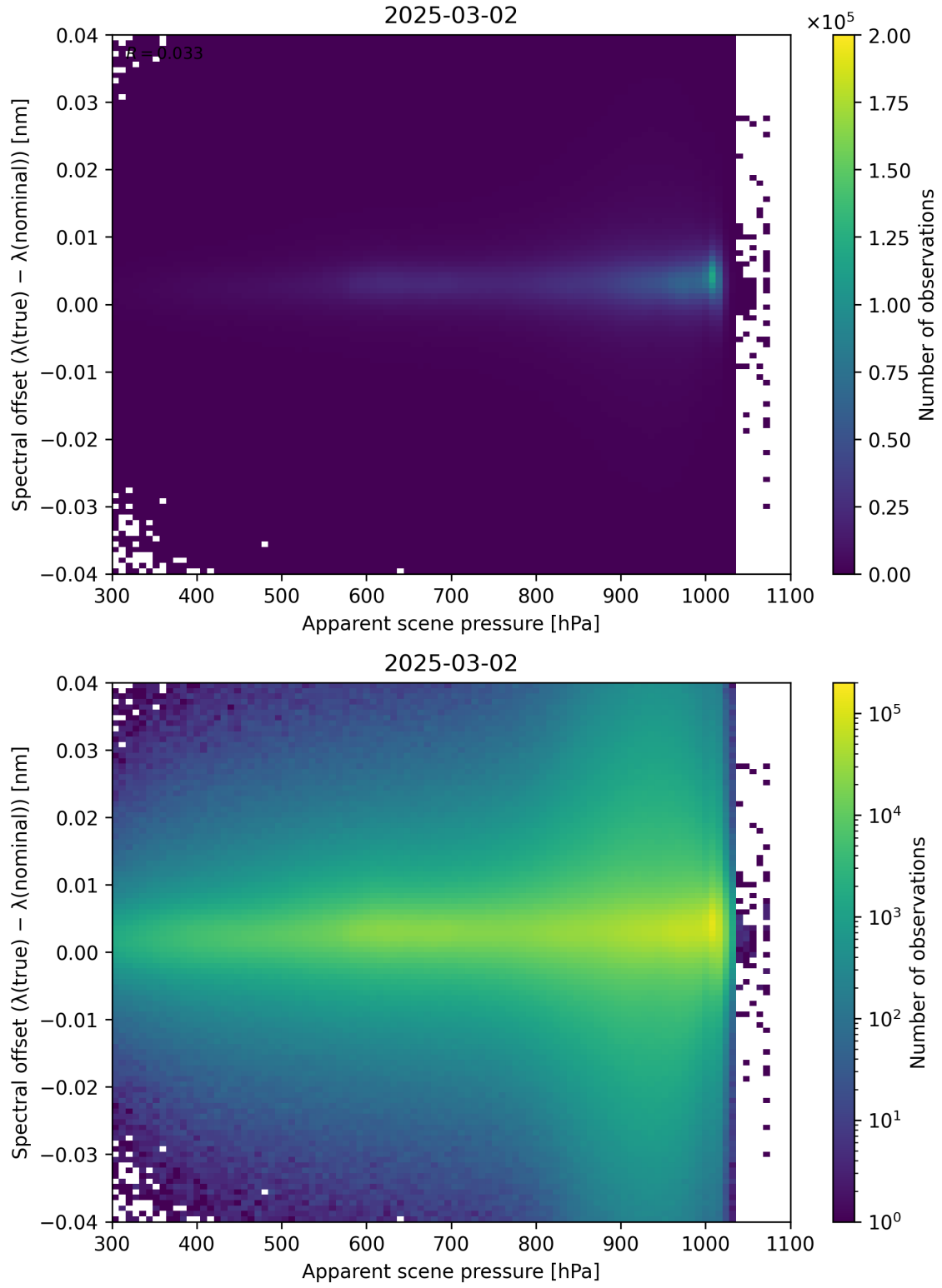
Figure 67: Scatter density plot of “Apparent scene pressure” against “Spectral offset ( \lambda_{\text{true}} - \lambda_{\text{nominal}} )” for 2025-03-01 to 2025-03-03.
