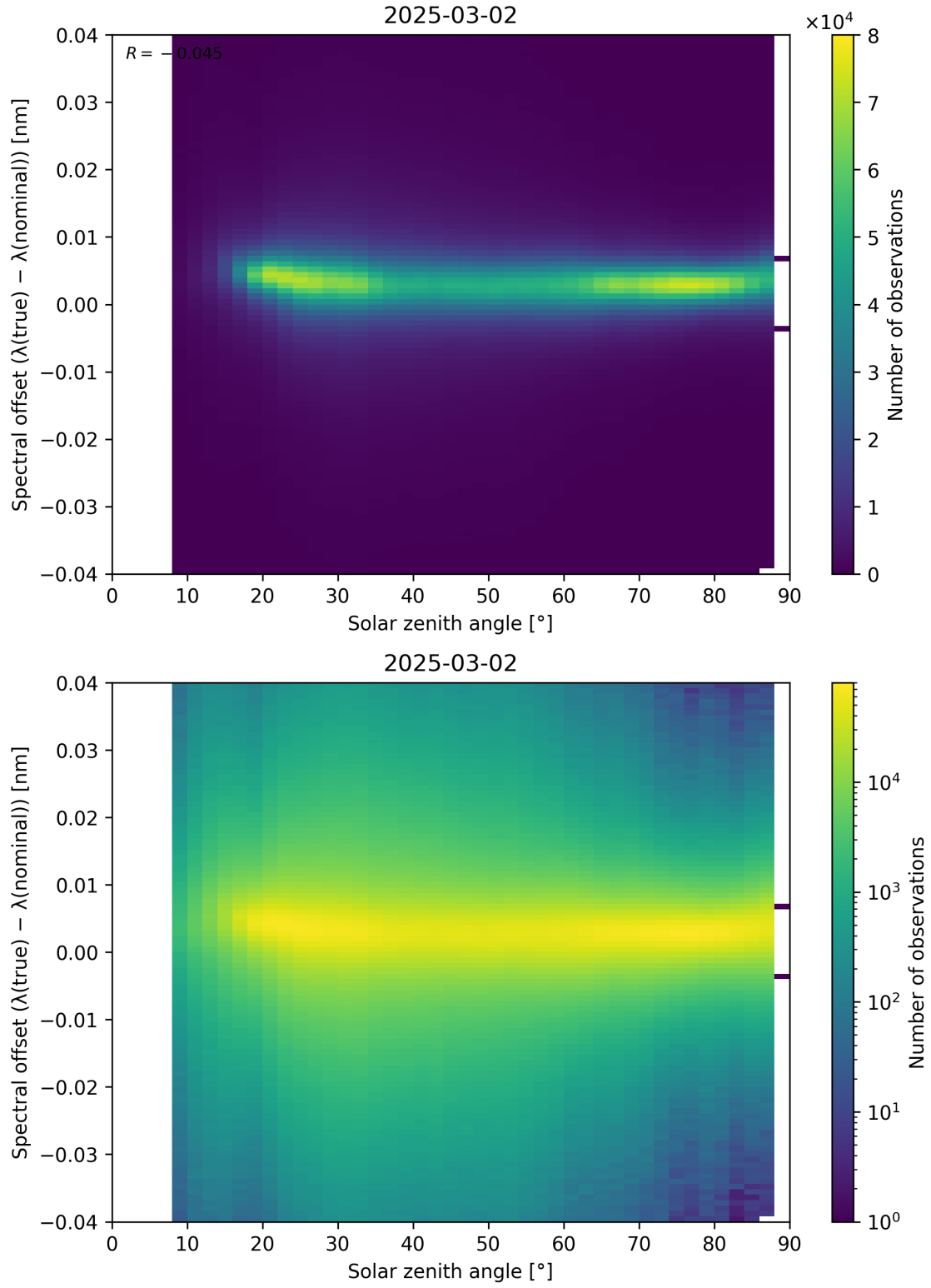
Figure 117: Scatter density plot of “Solar zenith angle” against “Spectral offset ( \lambda_{\text{true}} - \lambda_{\text{nominal}} )” for 2025-03-01 to 2025-03-03.
