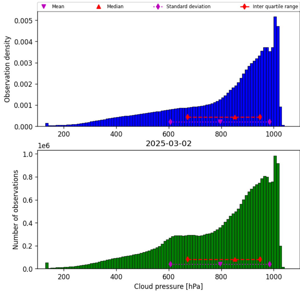
Figure 30: Histogram of “Cloud pressure” for 2025-03-01 to 2025-03-03
