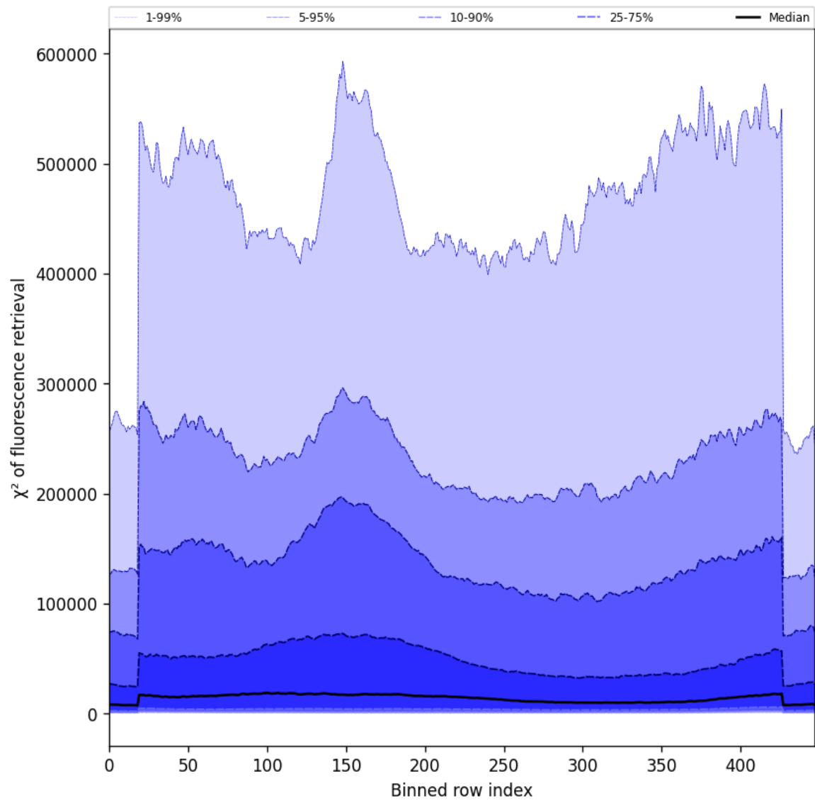
Figure 59: Along track statistics of “ \chi^2 of fluorescence retrieval” for 2025-03-01 to 2025-03-03
