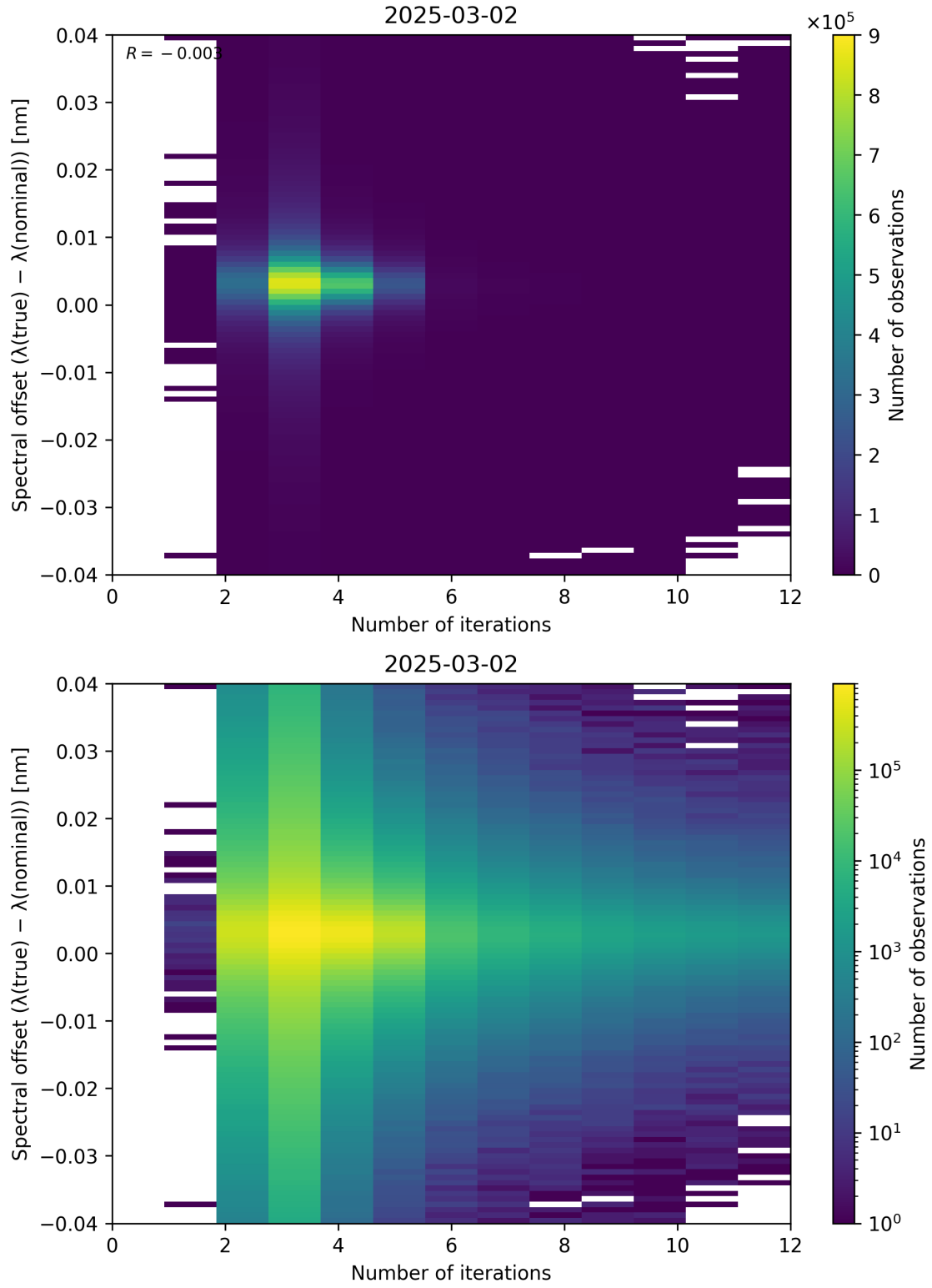
Figure 100: Scatter density plot of “Number of iterations” against “Spectral offset ( \lambda_{\text{true}} - \lambda_{\text{nominal}} )” for 2025-03-01 to 2025-03-03.
