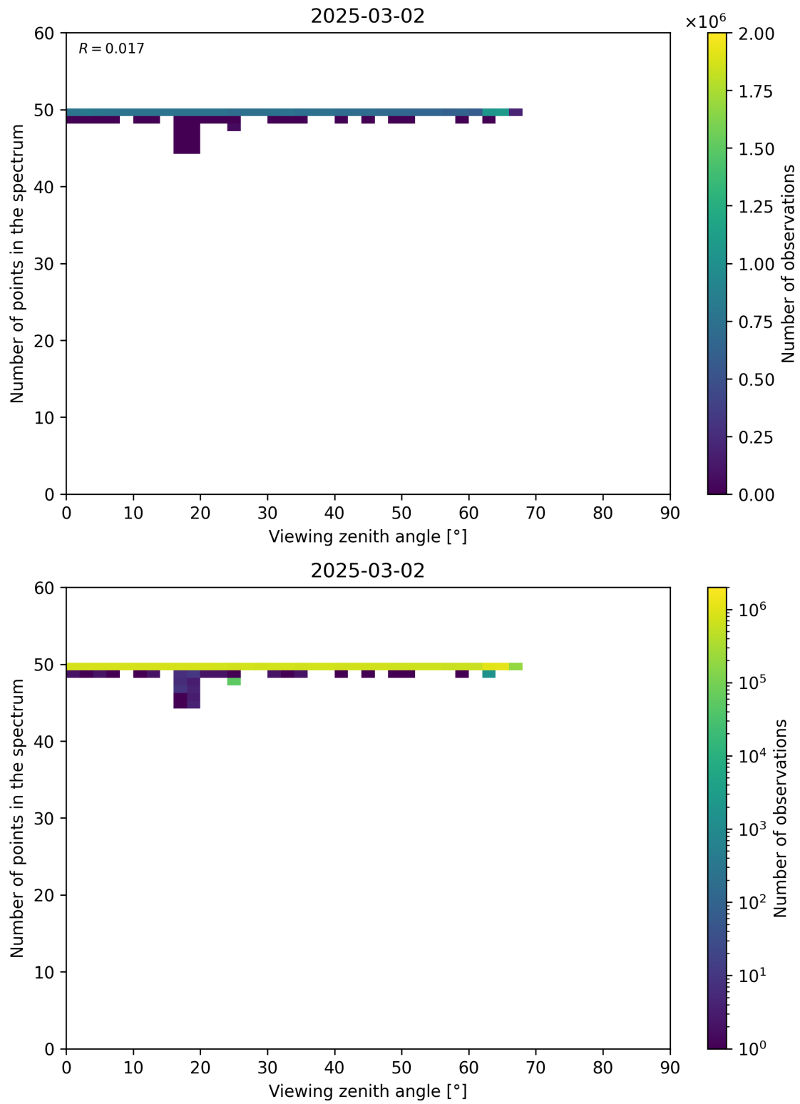
Figure 125: Scatter density plot of “Viewing zenith angle” against “Number of points in the spectrum” for 2025-03-01 to 2025-03-03.
