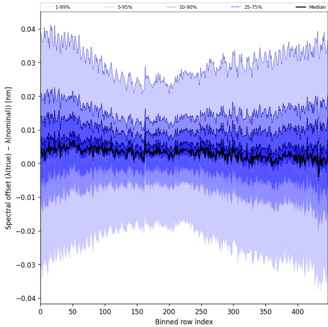
Figure 62: Along track statistics of “Spectral offset ( \lambda_{\text{true}} - \lambda_{\text{nominal}} )” for 2025-03-01 to 2025-03-03
