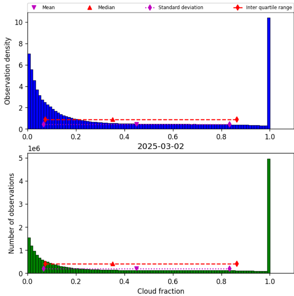
Figure 32: Histogram of “Cloud fraction” for 2025-03-01 to 2025-03-03
