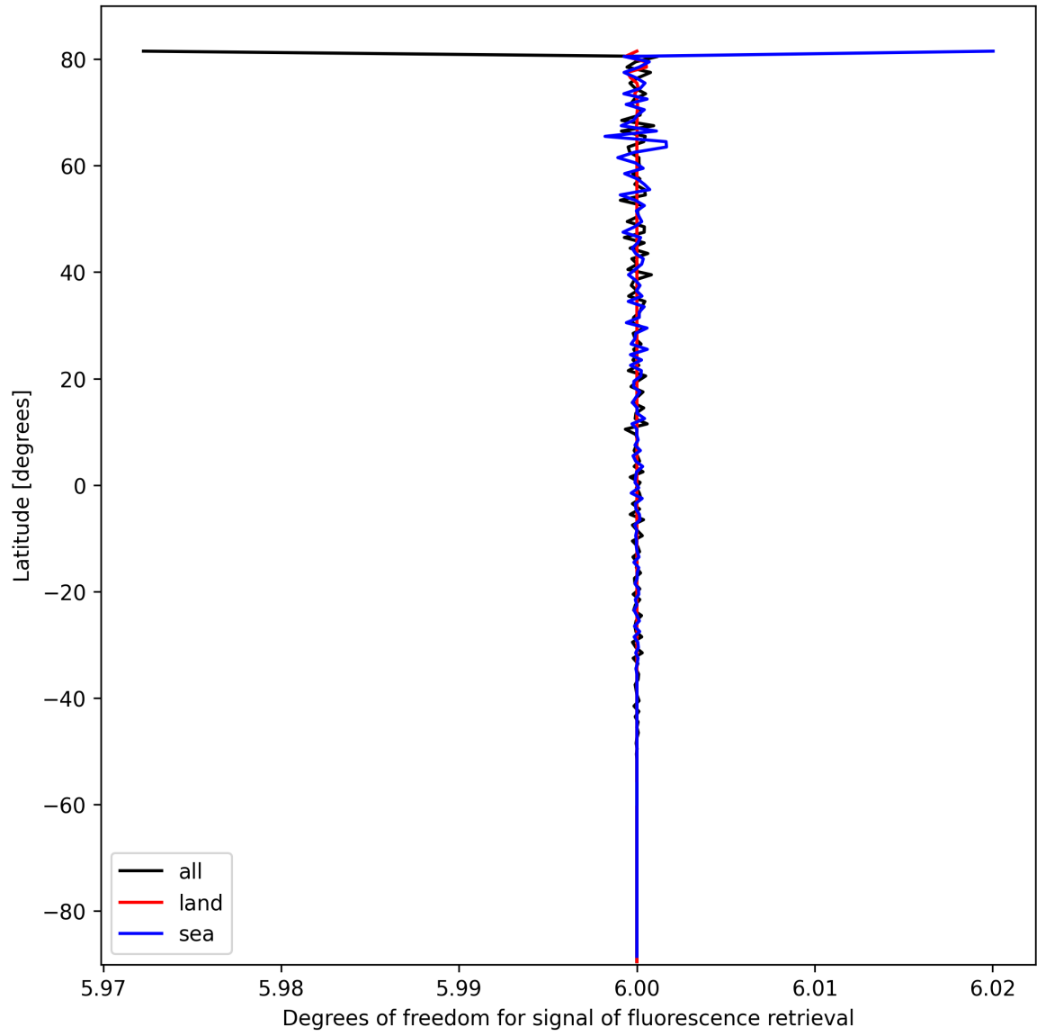
Figure 26: Zonal average of “Degrees of freedom for signal of fluorescence retrieval” for 2025-03-01 to 2025-03-03.
