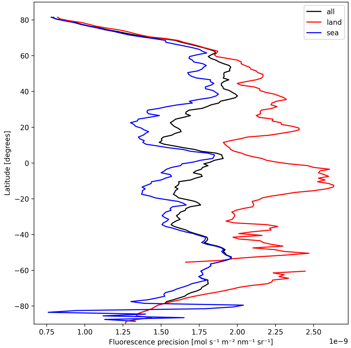
Figure 24: Zonal average of “Fluorescence precision” for 2025-03-01 to 2025-03-03.
