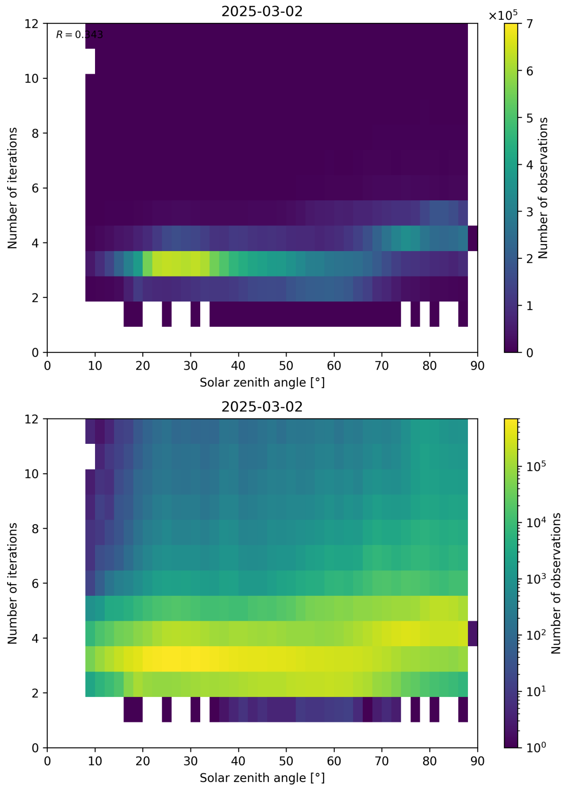
Figure 114: Scatter density plot of “Solar zenith angle” against “Number of iterations” for 2025-03-01 to 2025-03-03.
