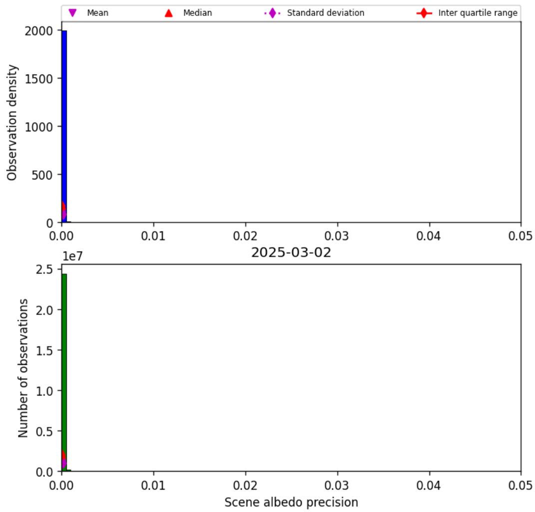
Figure 35: Histogram of “Scene albedo precision” for 2025-03-01 to 2025-03-03
