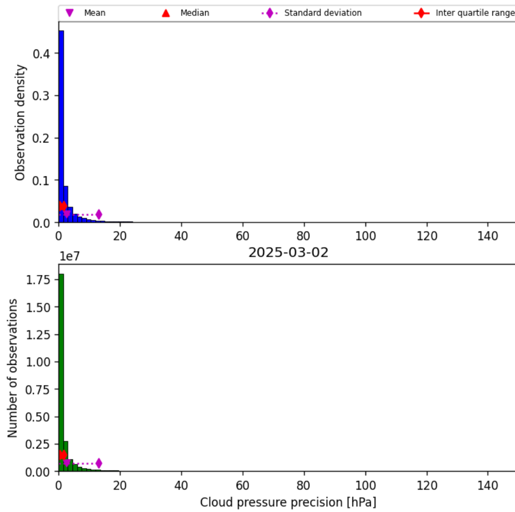
Figure 31: Histogram of “Cloud pressure precision” for 2025-03-01 to 2025-03-03
