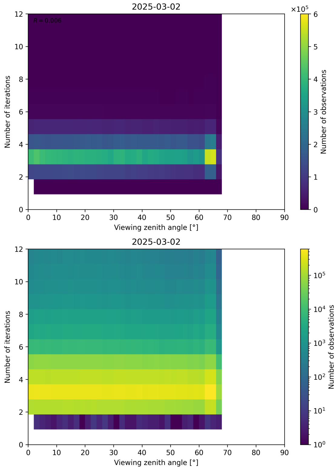
Figure 124: Scatter density plot of “Viewing zenith angle” against “Number of iterations” for 2025-03-01 to 2025-03-03.
