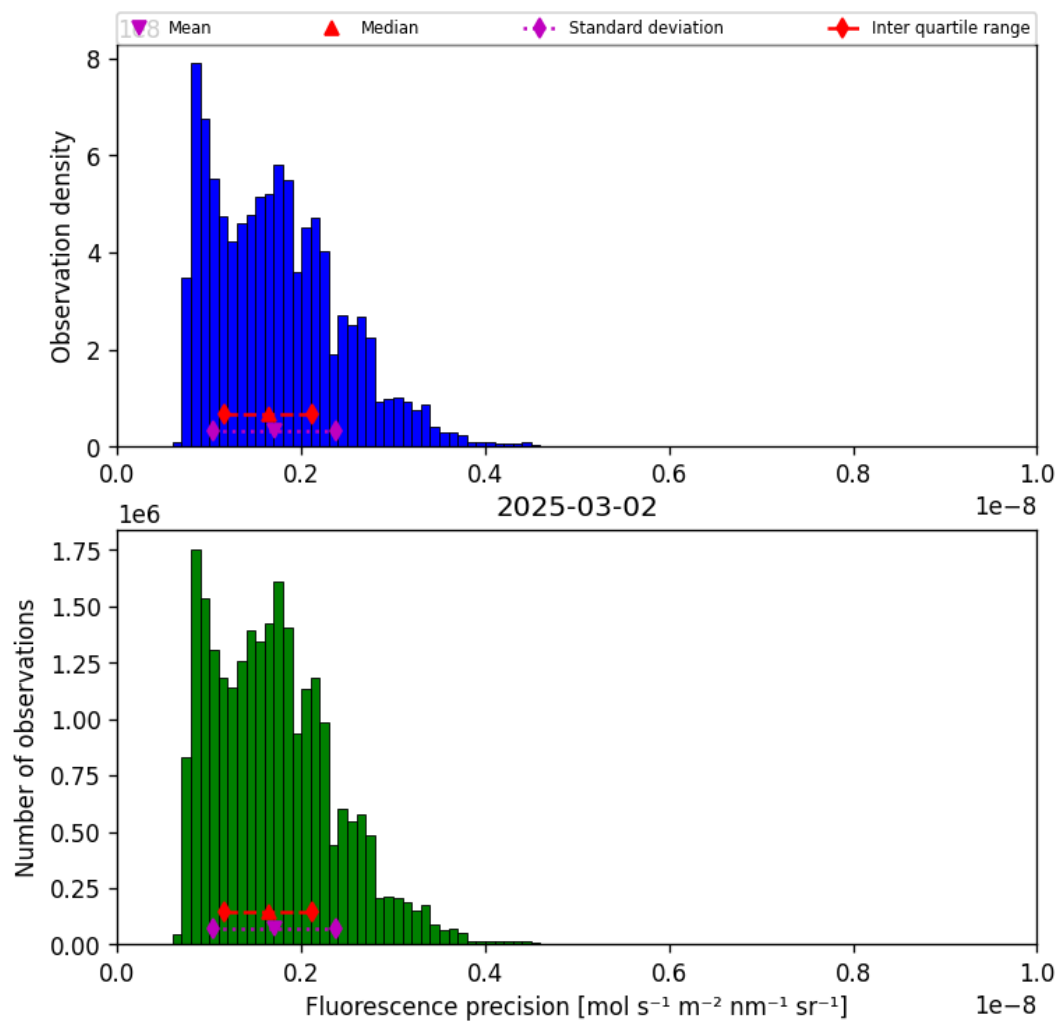
Figure 41: Histogram of “Fluorescence precision” for 2025-03-01 to 2025-03-03
