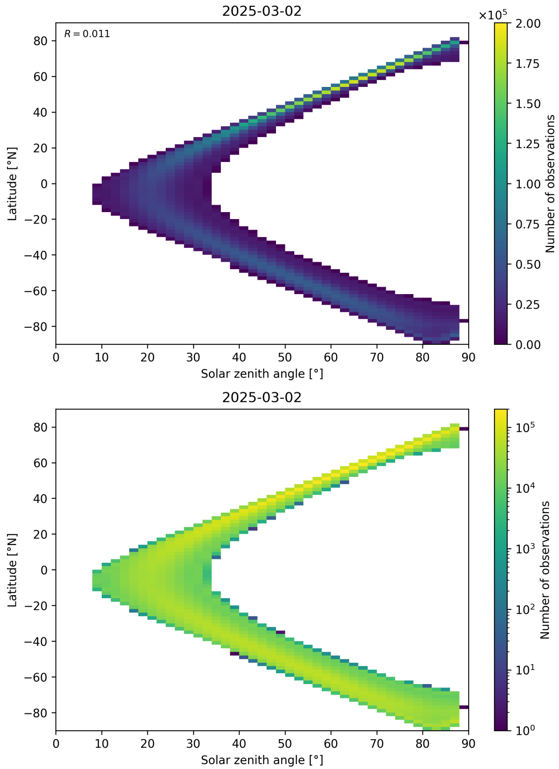
Figure 113: Scatter density plot of “Solar zenith angle” against “Latitude” for 2025-03-01 to 2025-03-03.
