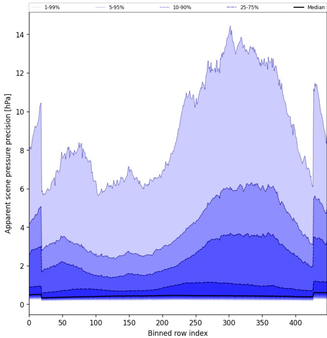
Figure 54: Along track statistics of “Apparent scene pressure precision” for 2025-03-01 to 2025-03-03
