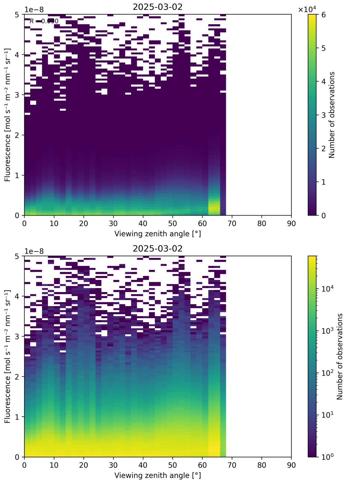
Figure 122: Scatter density plot of “Viewing zenith angle” against “Fluorescence” for 2025-03-01 to 2025-03-03.
