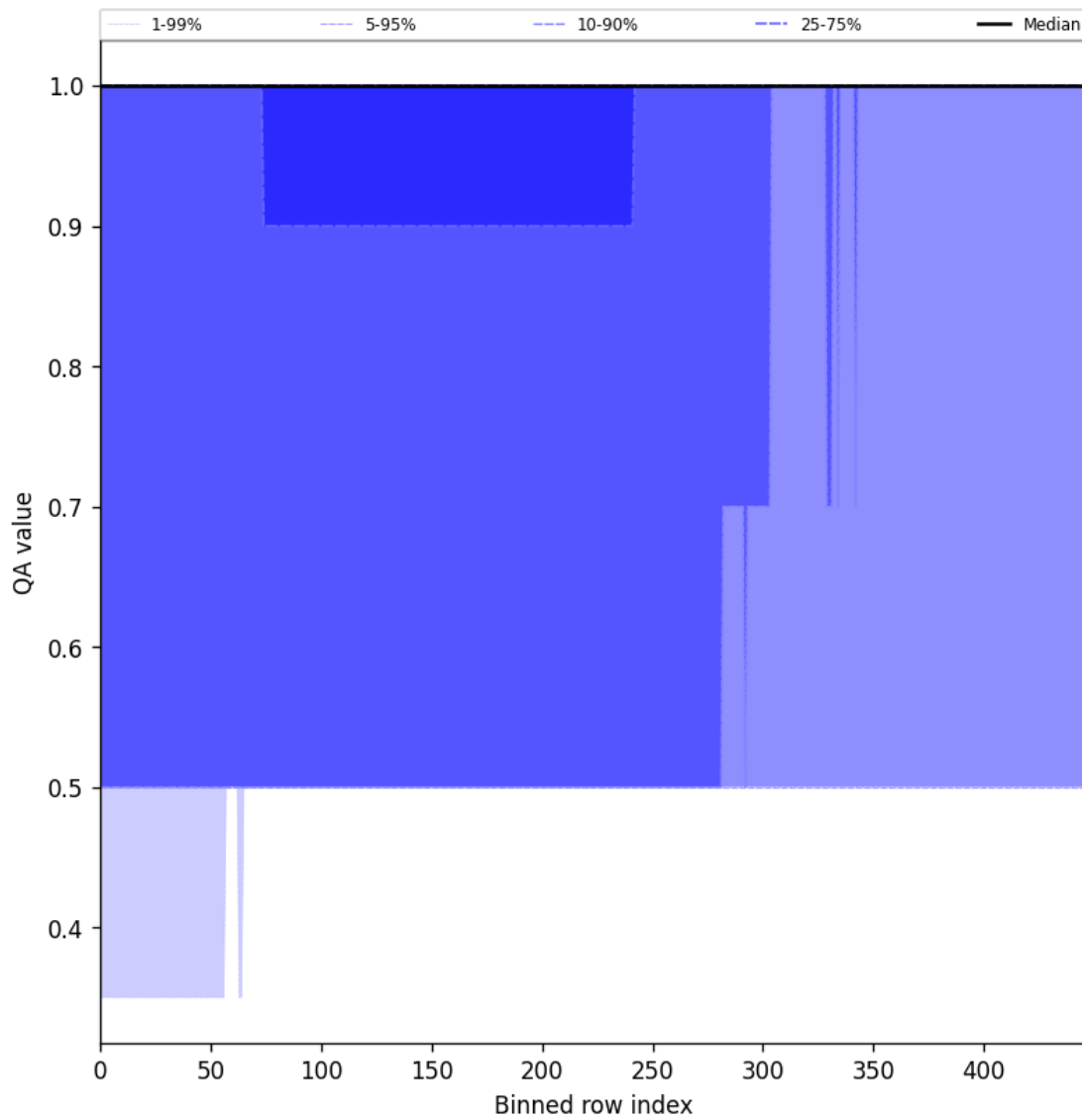
Figure 46: Along track statistics of “QA value” for 2025-03-01 to 2025-03-03
