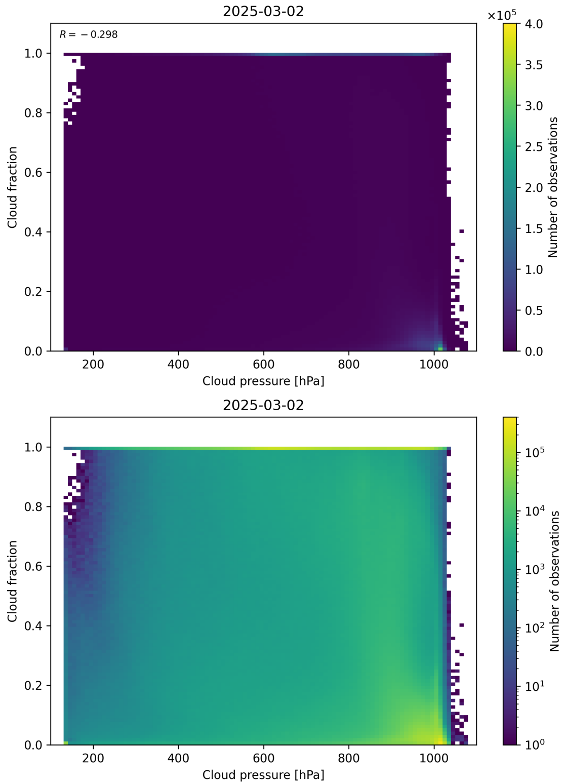
Figure 79: Scatter density plot of “Cloud pressure” against “Cloud fraction” for 2025-03-01 to 2025-03-03.
