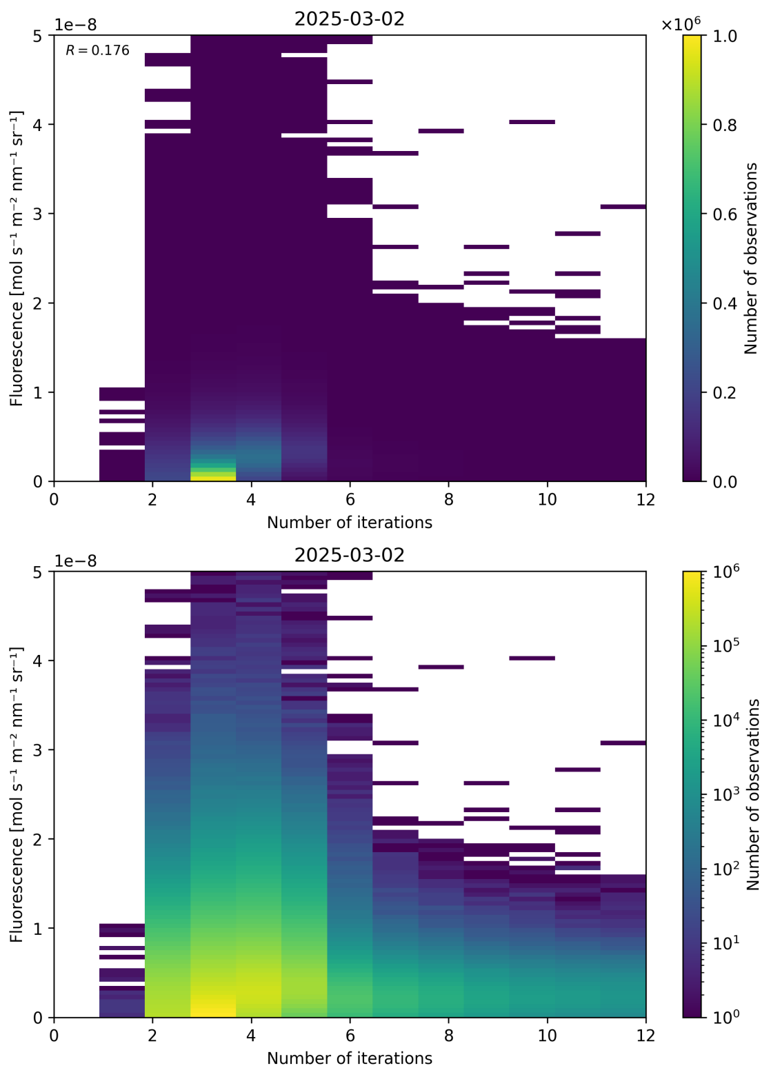
Figure 98: Scatter density plot of “Number of iterations” against “Fluorescence” for 2025-03-01 to 2025-03-03.
