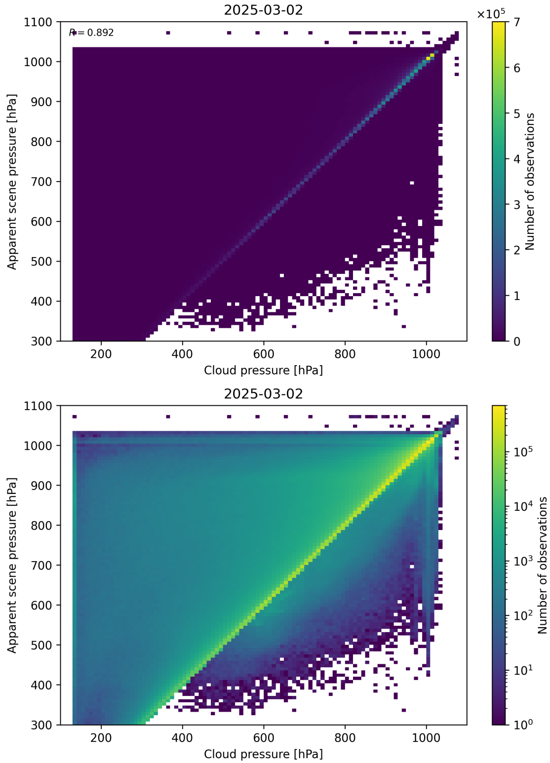
Figure 77: Scatter density plot of “Cloud pressure” against “Apparent scene pressure” for 2025-03-01 to 2025-03-03.
