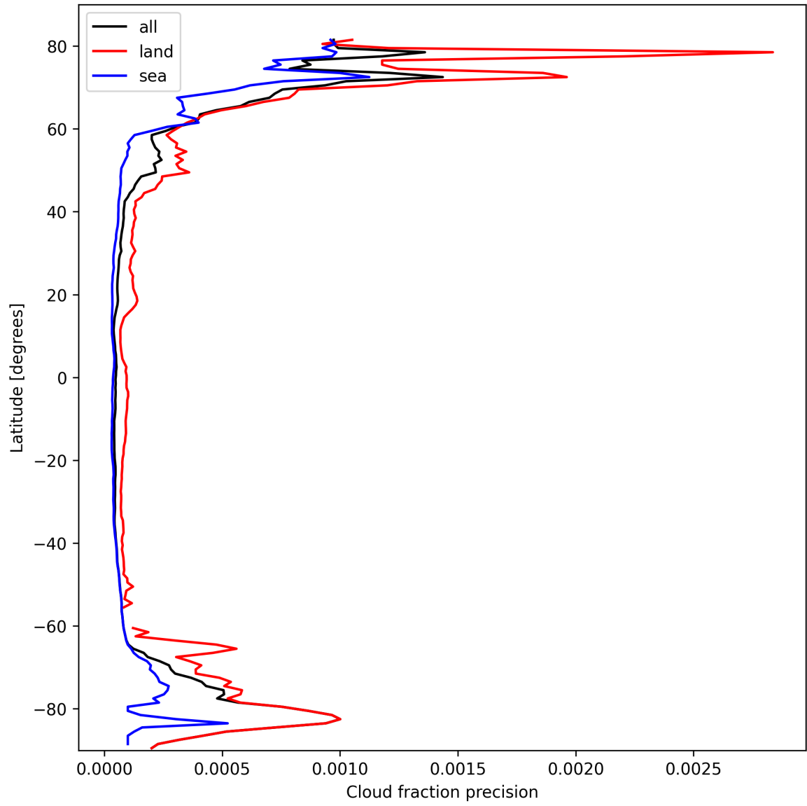
Figure 16: Zonal average of “Cloud fraction precision” for 2025-03-01 to 2025-03-03.
