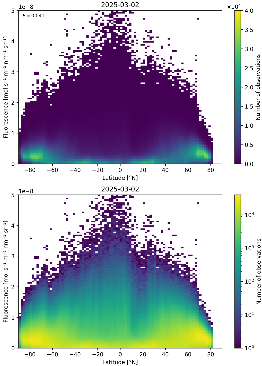
Figure 92: Scatter density plot of “Latitude” against “Fluorescence” for 2025-03-01 to 2025-03-03.
