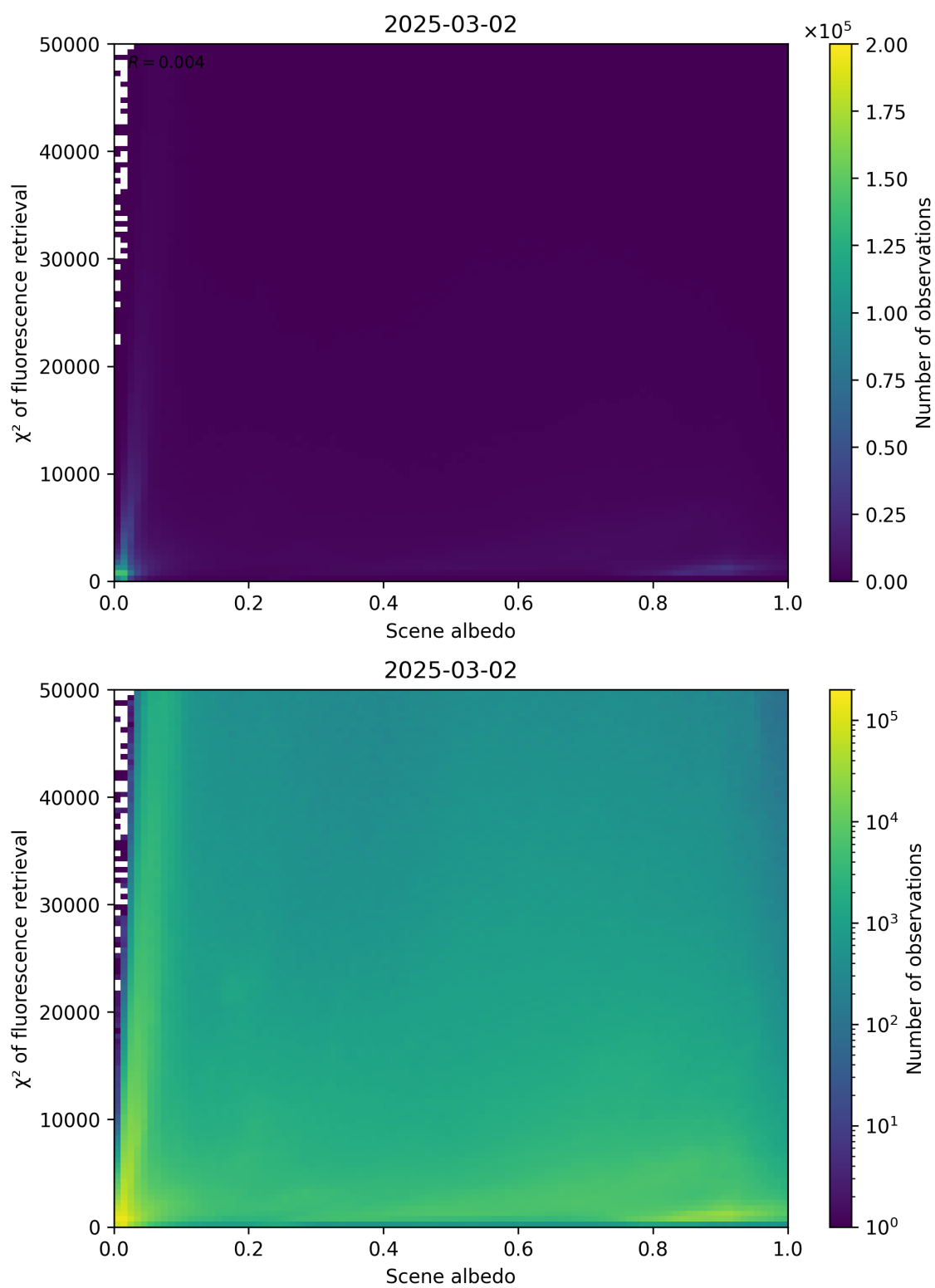
Figure 103: Scatter density plot of “Scene albedo” against “ \chi^2 of fluorescence retrieval” for 2025-03-01 to 2025-03-03.
