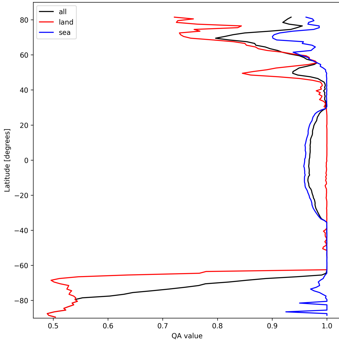
Figure 12: Zonal average of “QA value” for 2025-03-01 to 2025-03-03.
