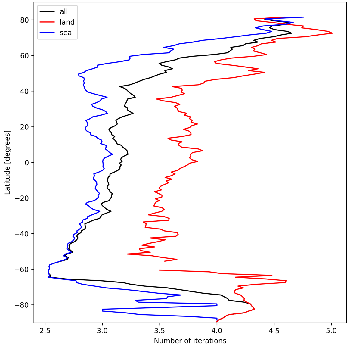
Figure 22: Zonal average of “Number of iterations” for 2025-03-01 to 2025-03-03.
