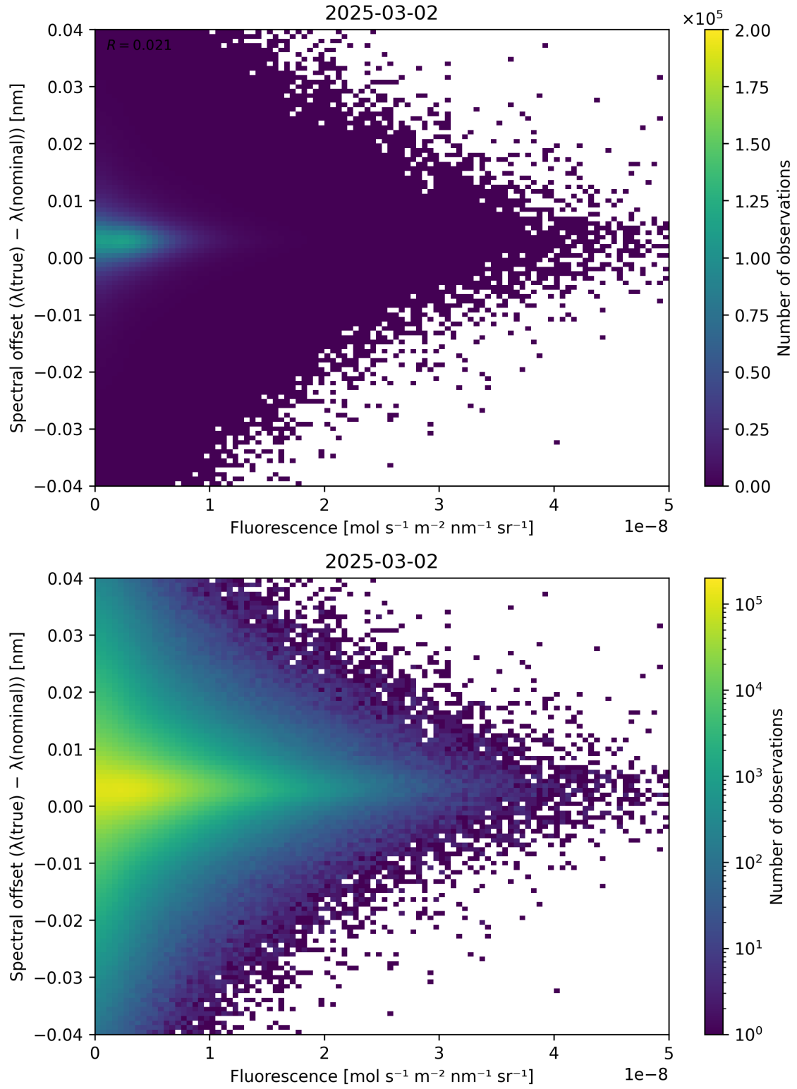
Figure 87: Scatter density plot of “Fluorescence” against “Spectral offset ( \lambda_{\text{true}} - \lambda_{\text{nominal}} )” for 2025-03-01 to 2025-03-03.
