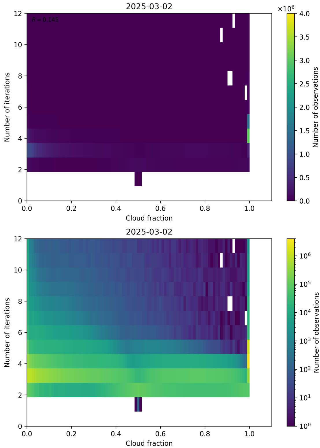
Figure 73: Scatter density plot of “Cloud fraction” against “Number of iterations” for 2025-03-01 to 2025-03-03.
