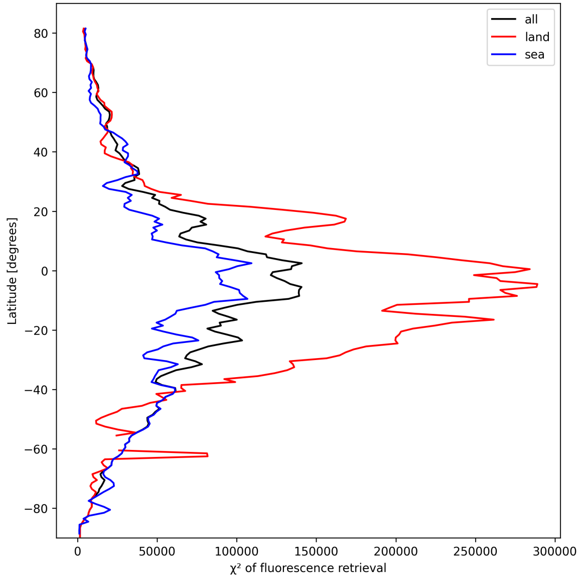
Figure 25: Zonal average of “ \chi^2 of fluorescence retrieval” for 2025-03-01 to 2025-03-03.
