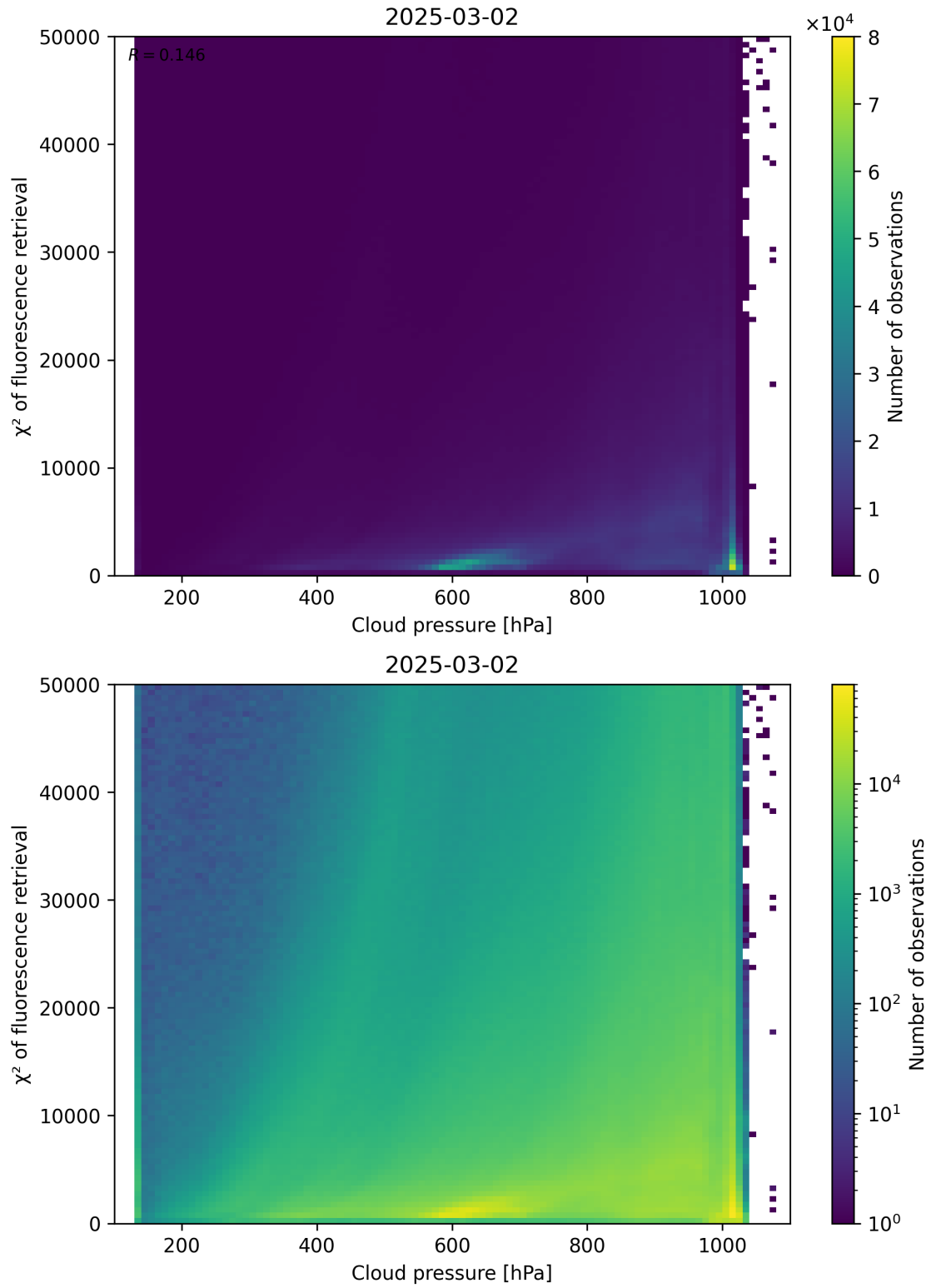
Figure 78: Scatter density plot of “Cloud pressure” against “ \chi^2 of fluorescence retrieval” for 2025-03-01 to 2025-03-03.
