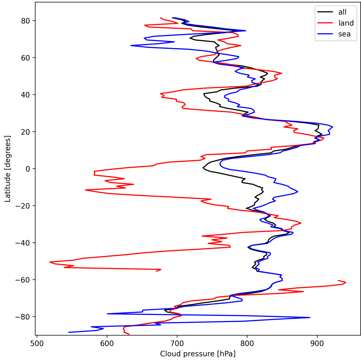
Figure 13: Zonal average of “Cloud pressure” for 2025-03-01 to 2025-03-03.
