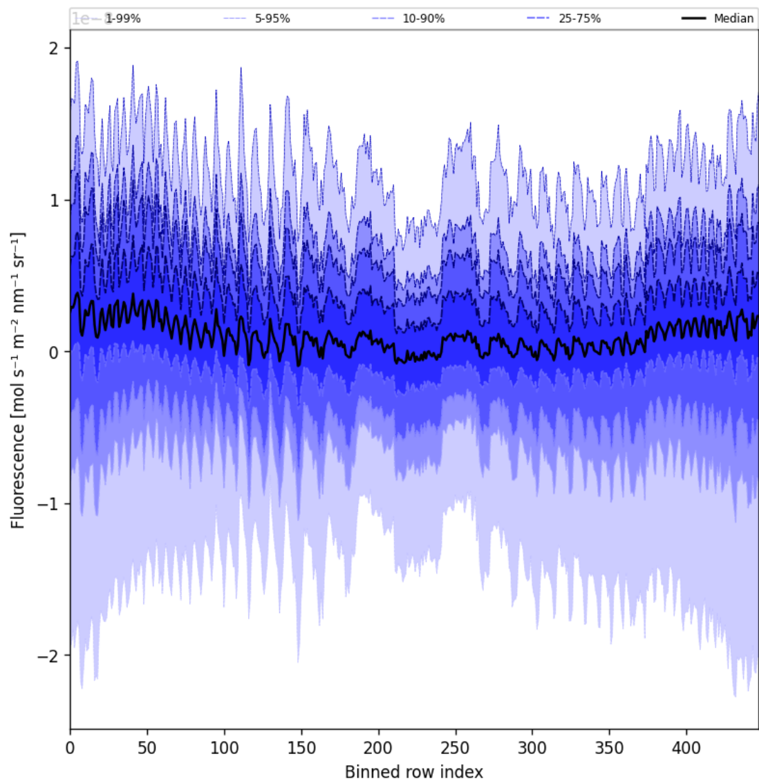
Figure 57: Along track statistics of “Fluorescence” for 2025-03-01 to 2025-03-03
