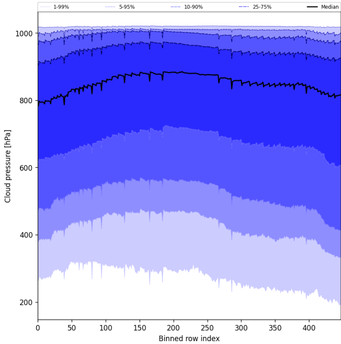
Figure 47: Along track statistics of “Cloud pressure” for 2025-03-01 to 2025-03-03
