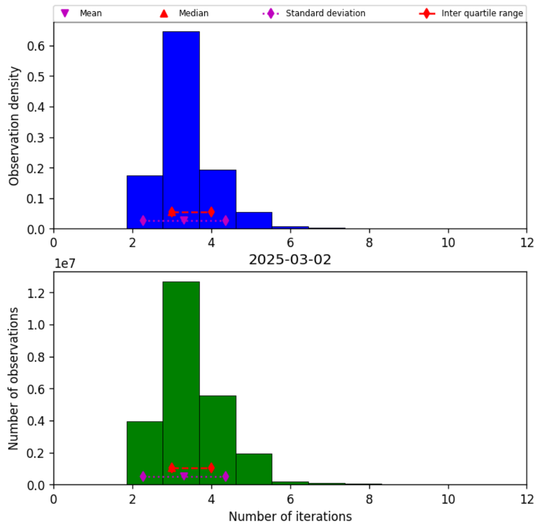
Figure 39: Histogram of “Number of iterations” for 2025-03-01 to 2025-03-03
