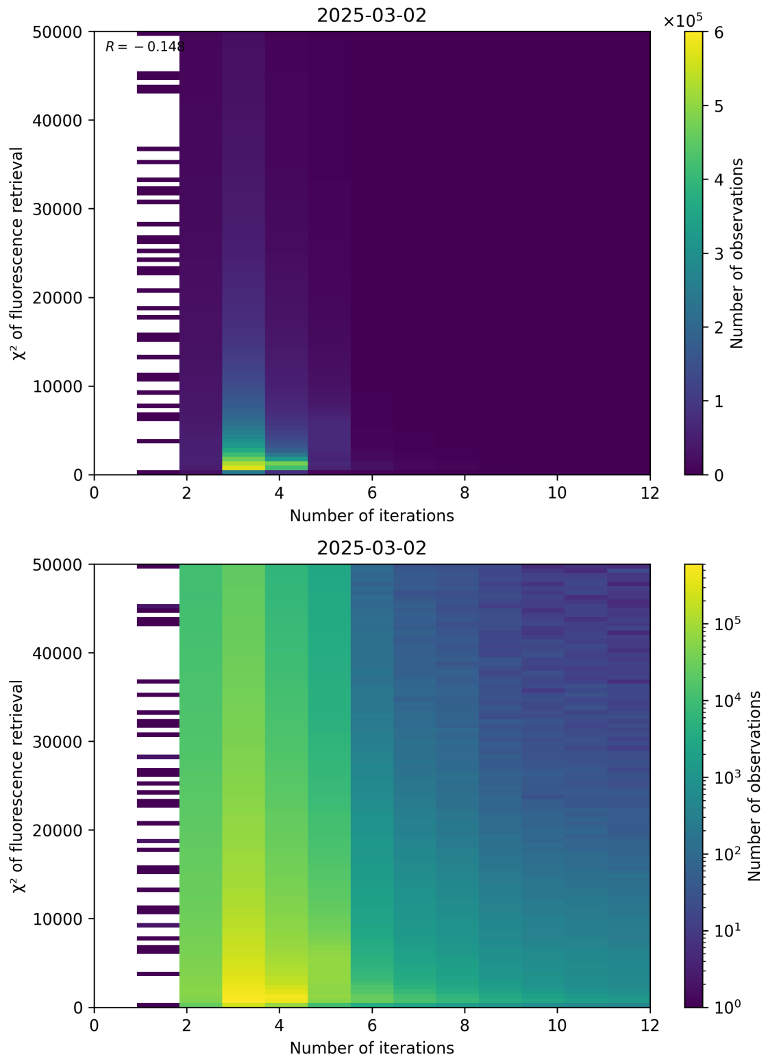
Figure 97: Scatter density plot of “Number of iterations” against “ \chi^2 of fluorescence retrieval” for 2025-03-01 to 2025-03-03.
