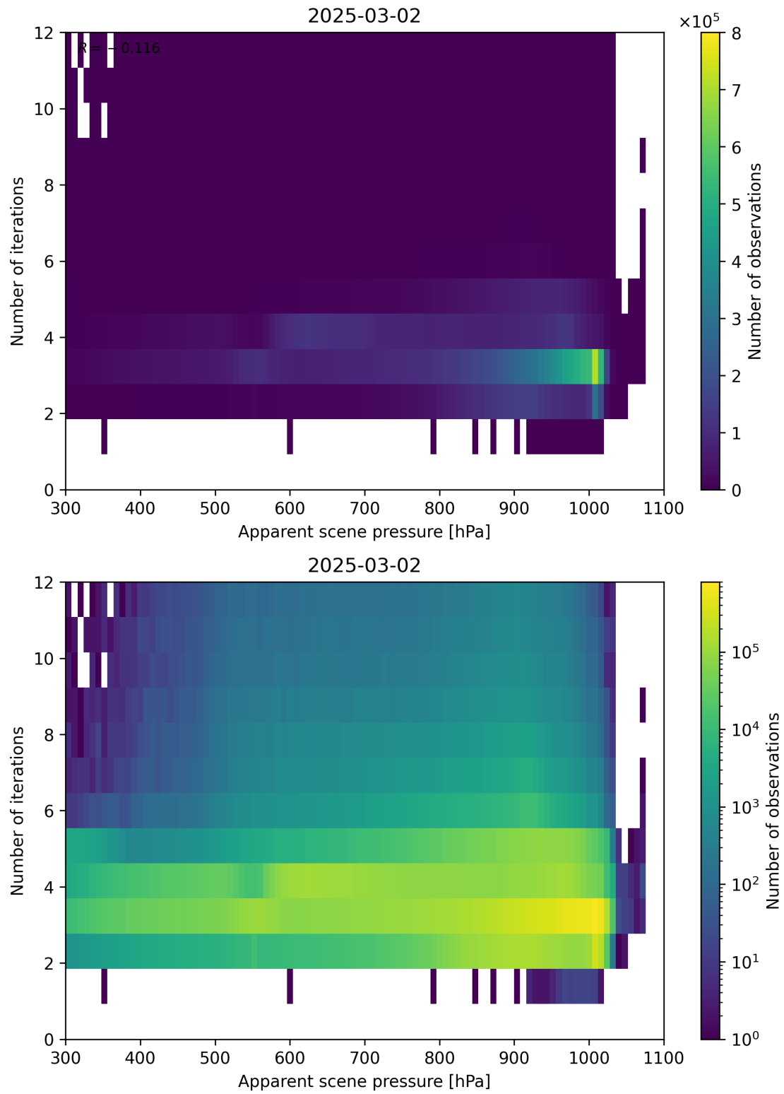
Figure 65: Scatter density plot of “Apparent scene pressure” against “Number of iterations” for 2025-03-01 to 2025-03-03.
