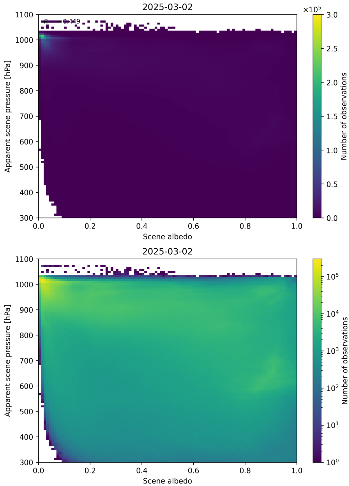
Figure 102: Scatter density plot of “Scene albedo” against “Apparent scene pressure” for 2025-03-01 to 2025-03-03.
