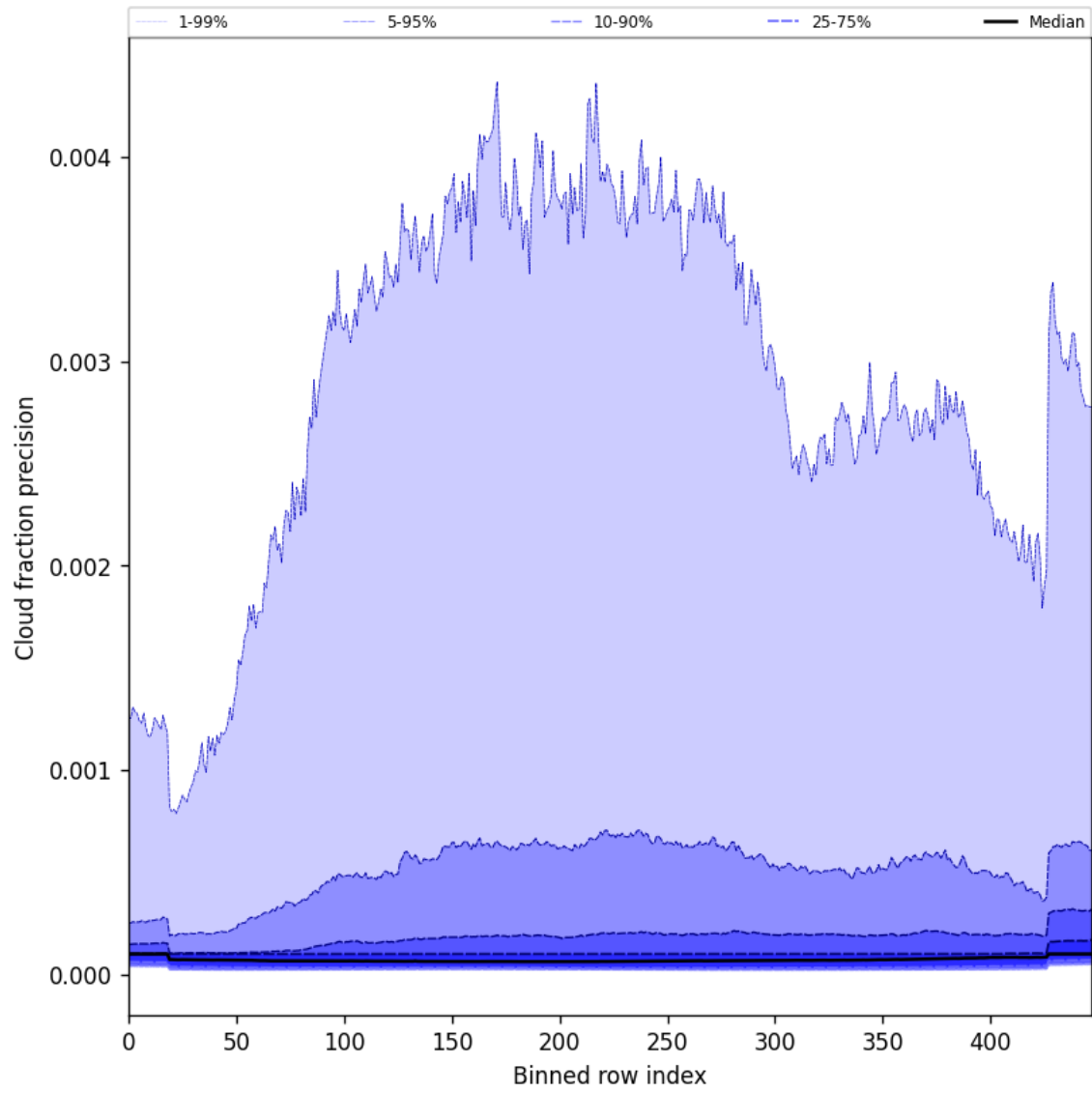
Figure 50: Along track statistics of “Cloud fraction precision” for 2025-03-01 to 2025-03-03
