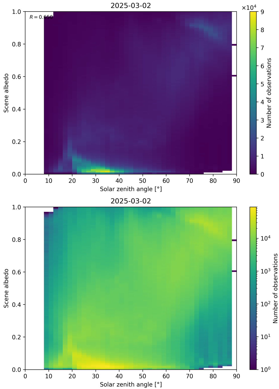
Figure 116: Scatter density plot of “Solar zenith angle” against “Scene albedo” for 2025-03-01 to 2025-03-03.
