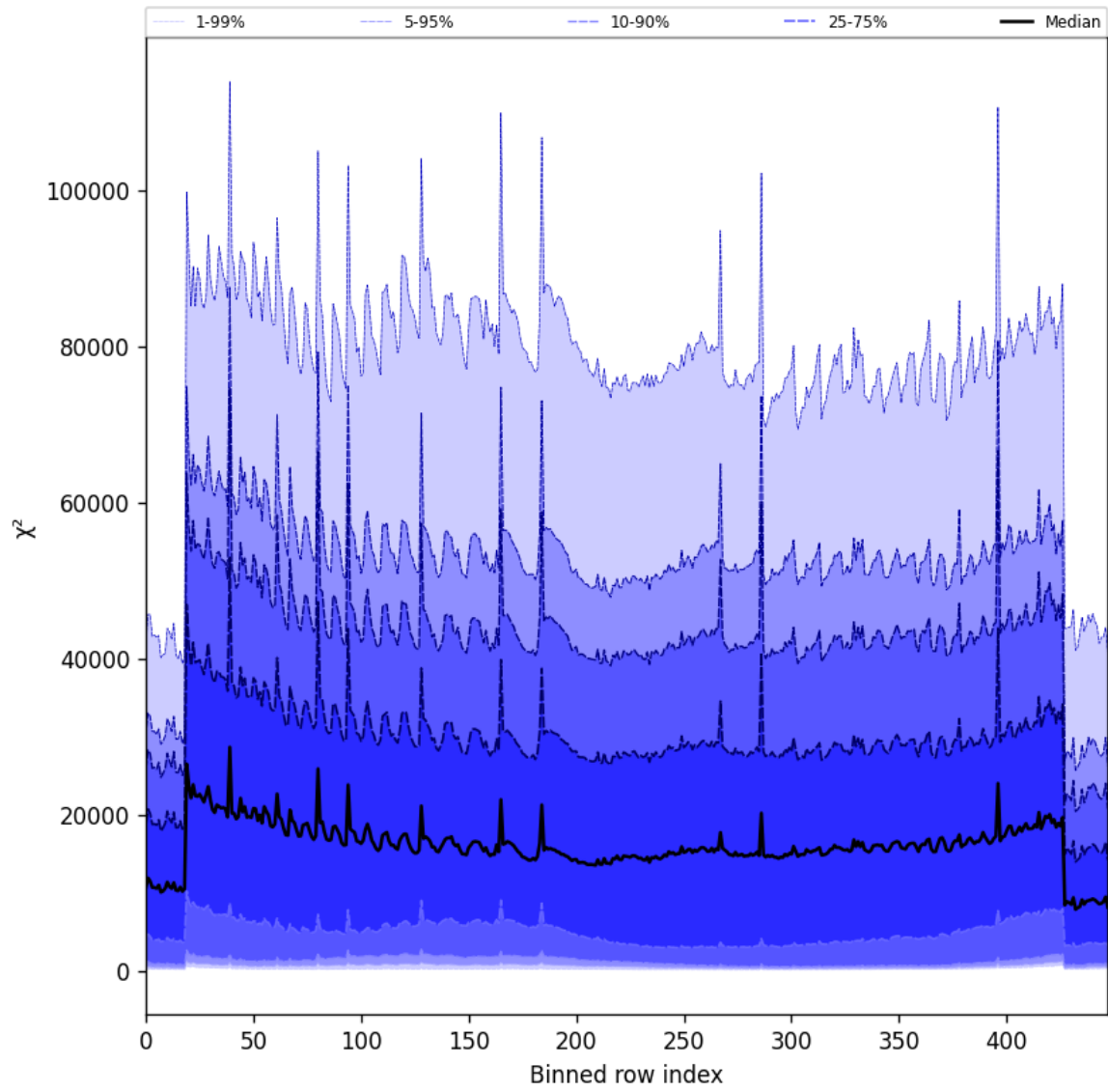
Figure 55: Along track statistics of “ \chi^2 ” for 2025-03-01 to 2025-03-03
