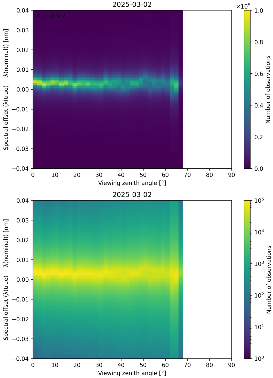
Figure 128: Scatter density plot of “Viewing zenith angle” against “Spectral offset ( \lambda_{\text{true}} - \lambda_{\text{nominal}} )” for 2025-03-01 to 2025-03-03.
