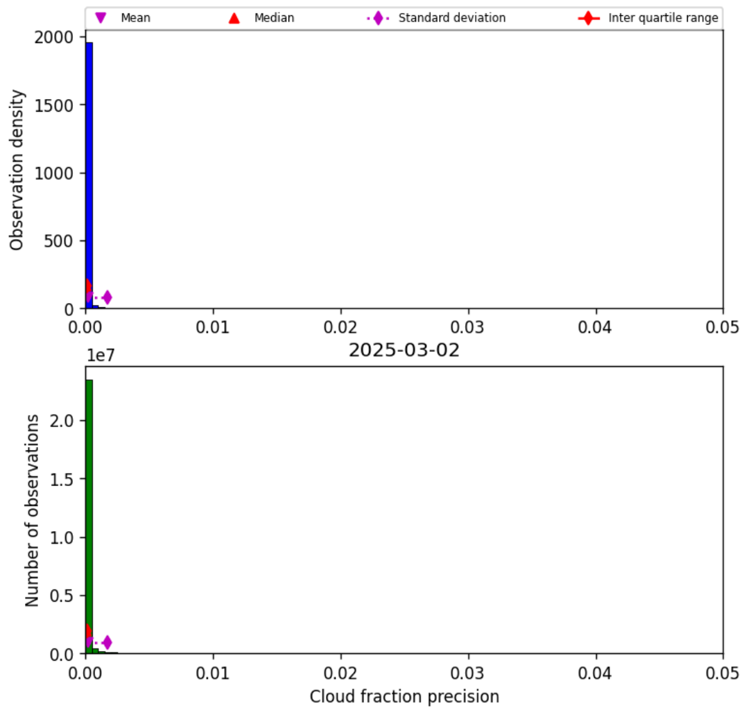
Figure 33: Histogram of “Cloud fraction precision” for 2025-03-01 to 2025-03-03
