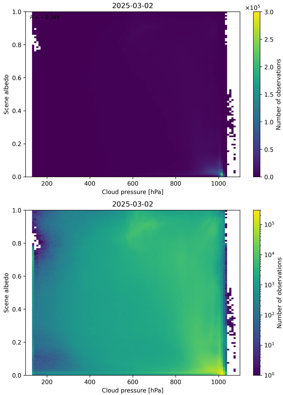
Figure 83: Scatter density plot of “Cloud pressure” against “Scene albedo” for 2025-03-01 to 2025-03-03.
