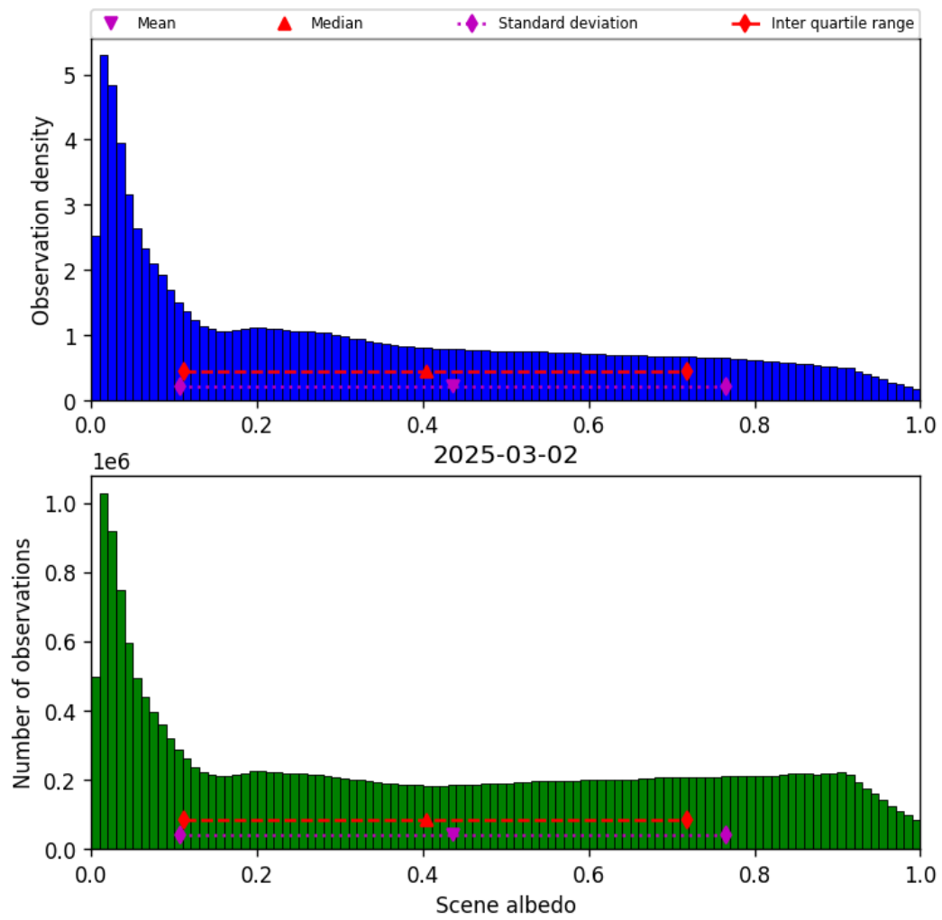
Figure 34: Histogram of “Scene albedo” for 2025-03-01 to 2025-03-03
