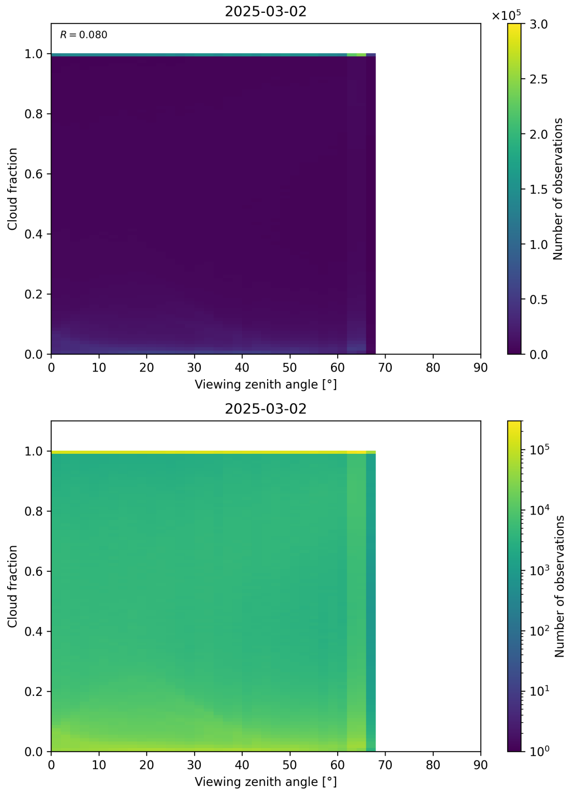
Figure 120: Scatter density plot of “Viewing zenith angle” against “Cloud fraction” for 2025-03-01 to 2025-03-03.
