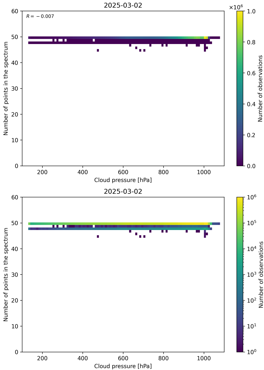
Figure 82: Scatter density plot of “Cloud pressure” against “Number of points in the spectrum” for 2025-03-01 to 2025-03-03.
