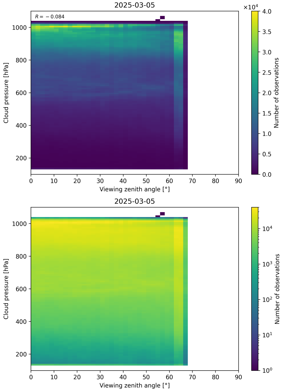
Figure 121: Scatter density plot of “Viewing zenith angle” against “Cloud pressure” for 2025-03-04 to 2025-03-06.
