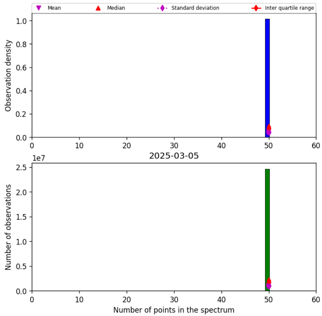
Figure 44: Histogram of “Number of points in the spectrum” for 2025-03-04 to 2025-03-06
