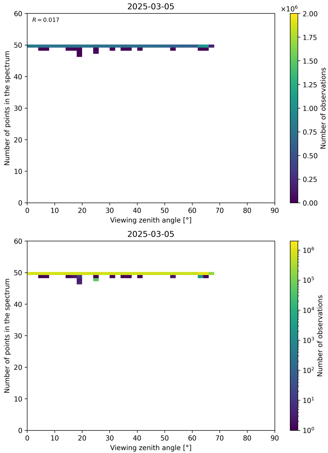
Figure 125: Scatter density plot of “Viewing zenith angle” against “Number of points in the spectrum” for 2025-03-04 to 2025-03-06.
