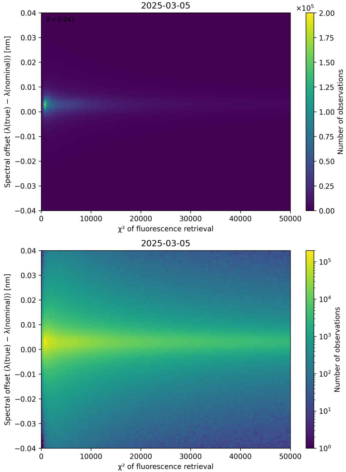
Figure 69: Scatter density plot of “ \chi^2 of fluorescence retrieval” against “Spectral offset ( \lambda_{\text{true}} - \lambda_{\text{nominal}} )” for 2025-03-04 to 2025-03-06.
