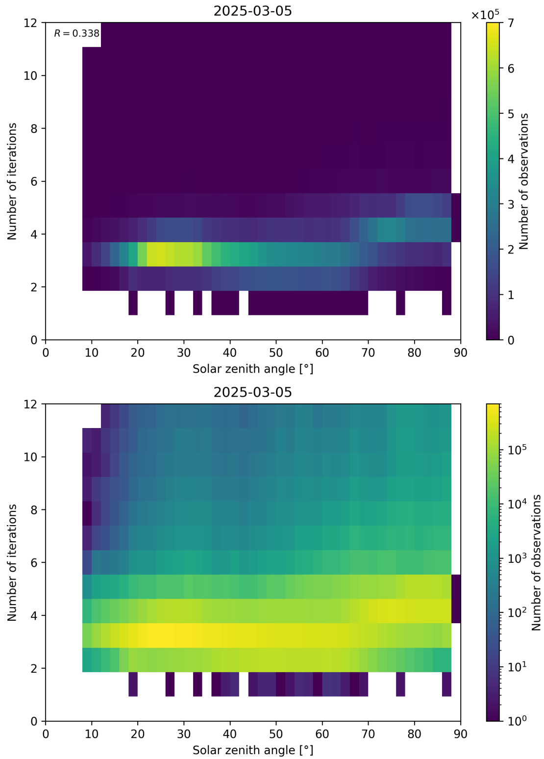
Figure 114: Scatter density plot of “Solar zenith angle” against “Number of iterations” for 2025-03-04 to 2025-03-06.
