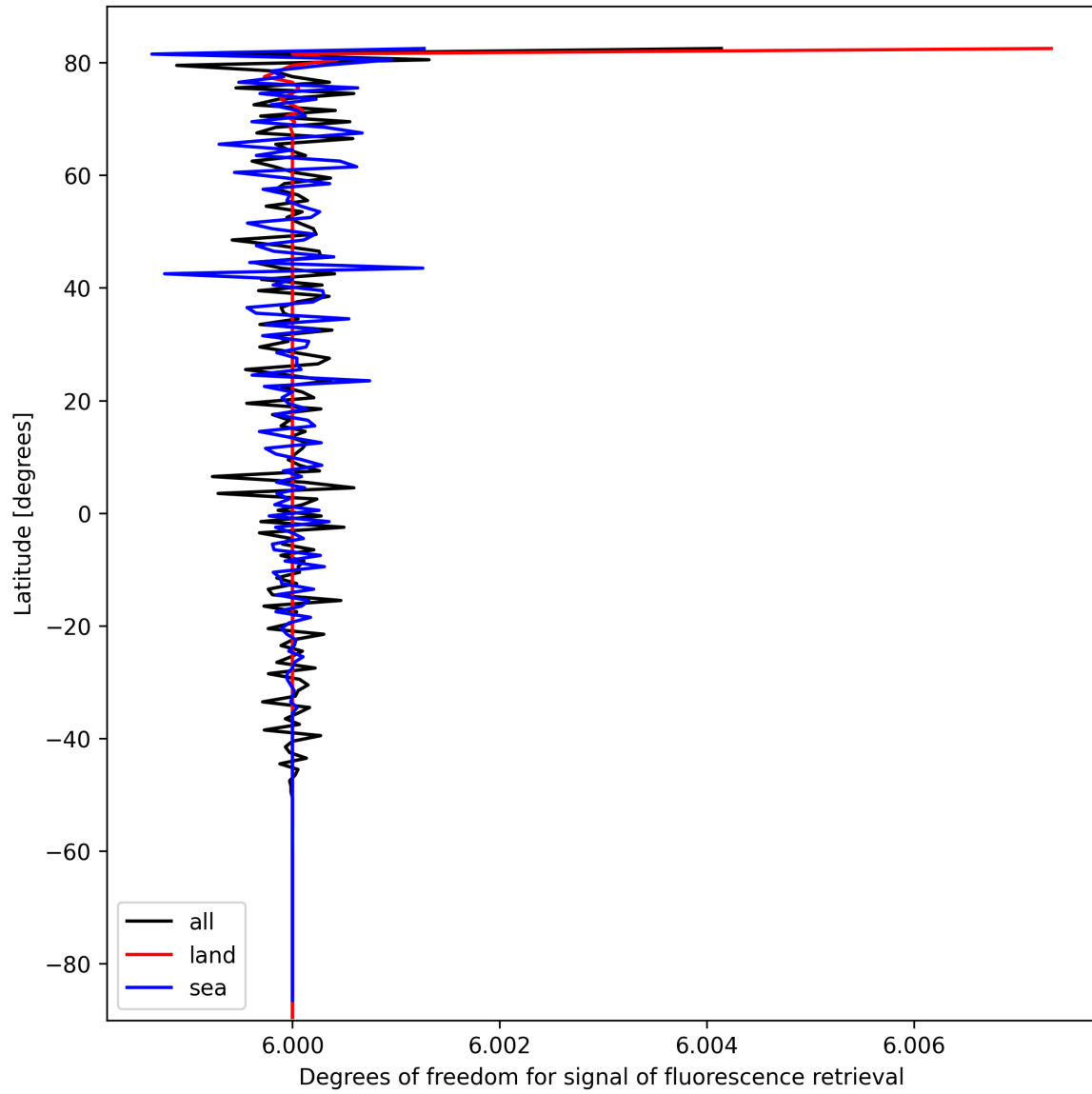
Figure 26: Zonal average of “Degrees of freedom for signal of fluorescence retrieval” for 2025-03-04 to 2025-03-06.
