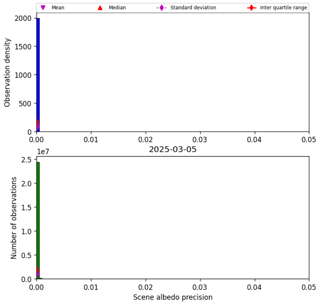
Figure 35: Histogram of “Scene albedo precision” for 2025-03-04 to 2025-03-06
