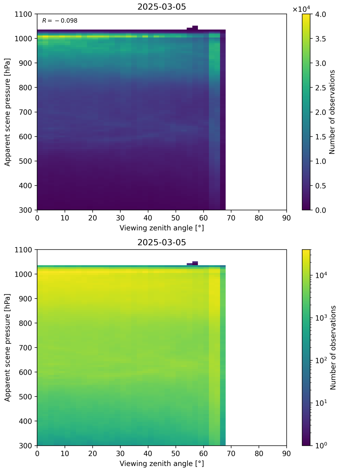
Figure 118: Scatter density plot of “Viewing zenith angle” against “Apparent scene pressure” for 2025-03-04 to 2025-03-06.
