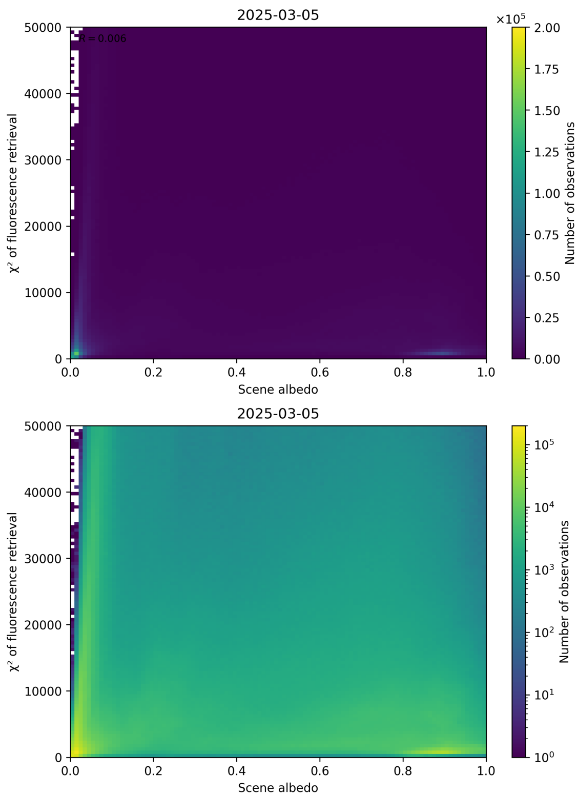
Figure 103: Scatter density plot of “Scene albedo” against “ \chi^2 of fluorescence retrieval” for 2025-03-04 to 2025-03-06.
