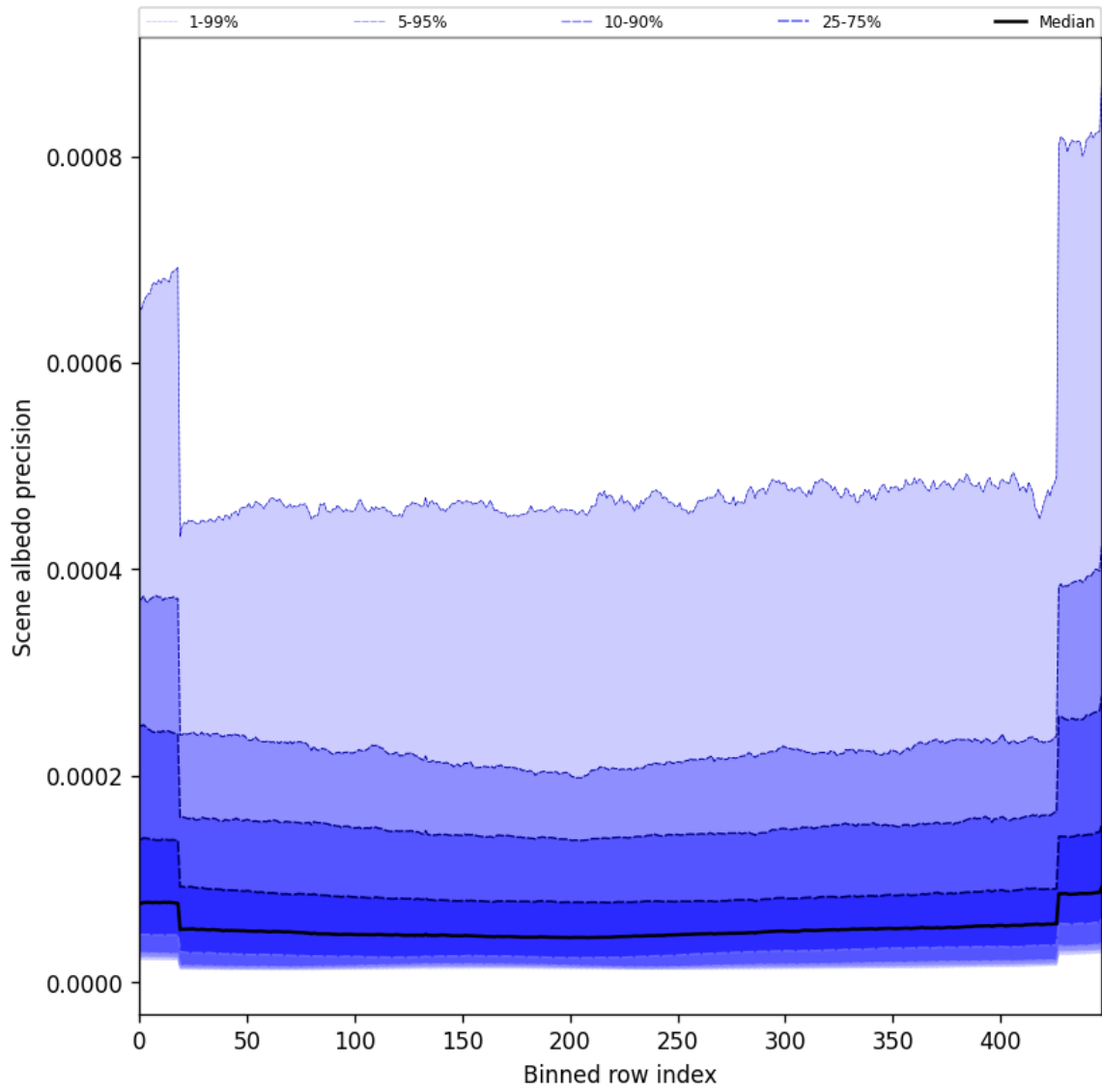
Figure 52: Along track statistics of “Scene albedo precision” for 2025-03-04 to 2025-03-06
