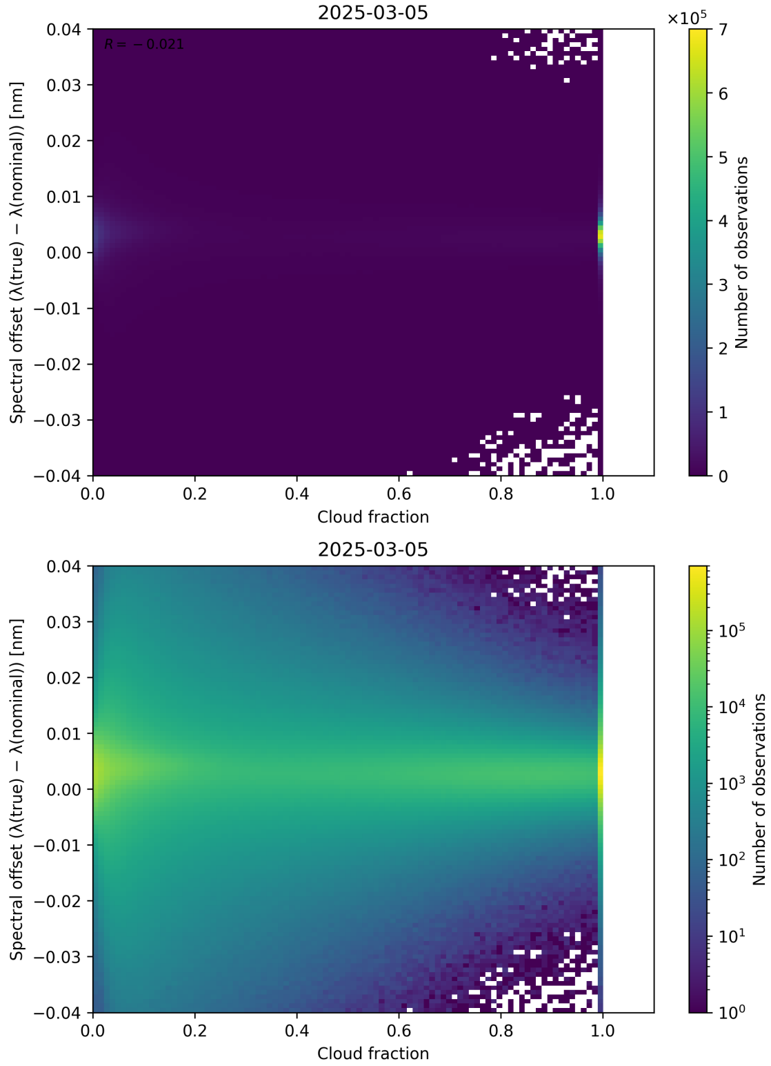
Figure 76: Scatter density plot of “Cloud fraction” against “Spectral offset ( \lambda_{\text{true}} - \lambda_{\text{nominal}} )” for 2025-03-04 to 2025-03-06.
