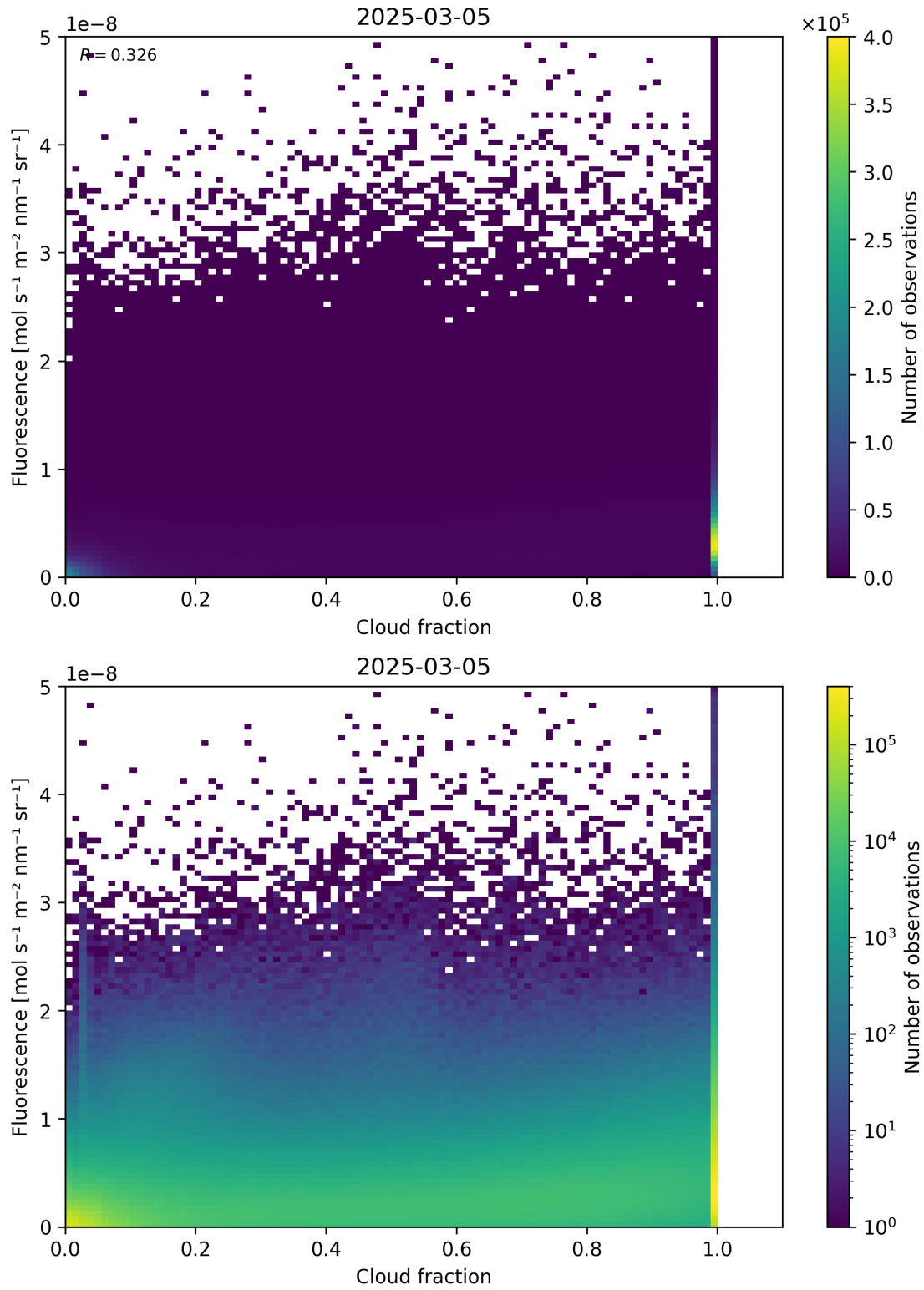
Figure 72: Scatter density plot of “Cloud fraction” against “Fluorescence” for 2025-03-04 to 2025-03-06.
