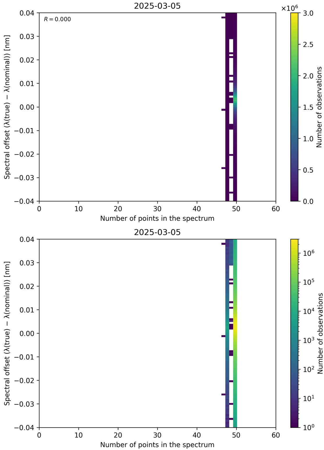
Figure 101: Scatter density plot of “Number of points in the spectrum” against “Spectral offset ( \lambda_{\text{true}} - \lambda_{\text{nominal}} )” for 2025-03-04 to 2025-03-06.
