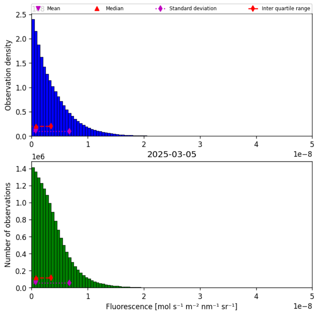
Figure 40: Histogram of “Fluorescence” for 2025-03-04 to 2025-03-06
