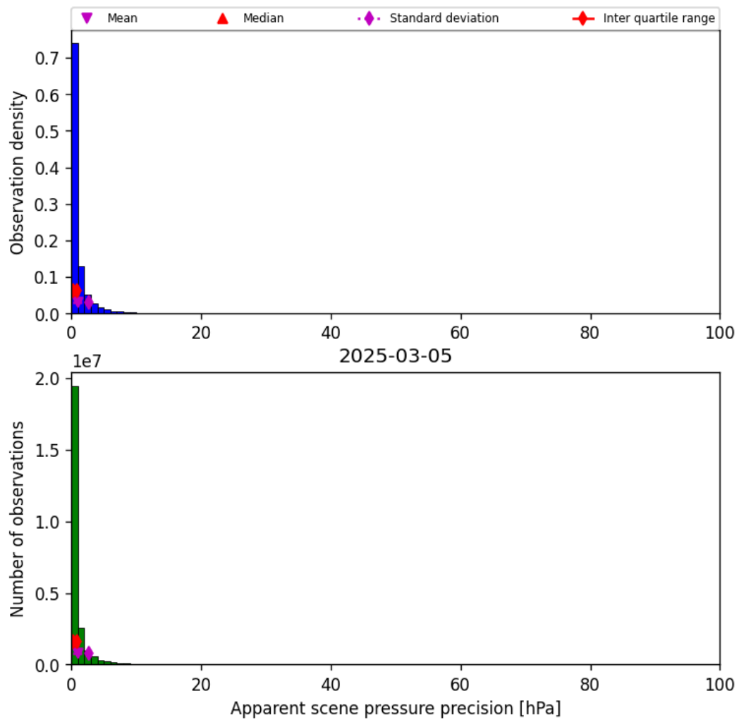
Figure 37: Histogram of “Apparent scene pressure precision” for 2025-03-04 to 2025-03-06
