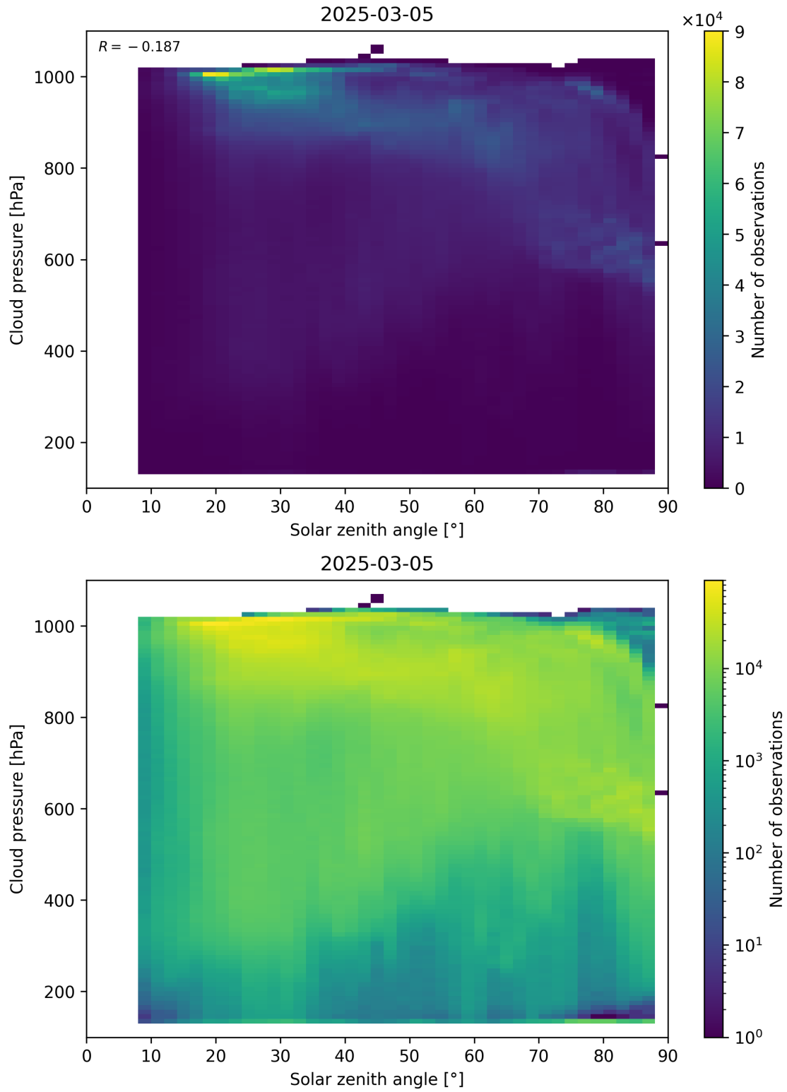
Figure 111: Scatter density plot of “Solar zenith angle” against “Cloud pressure” for 2025-03-04 to 2025-03-06.
