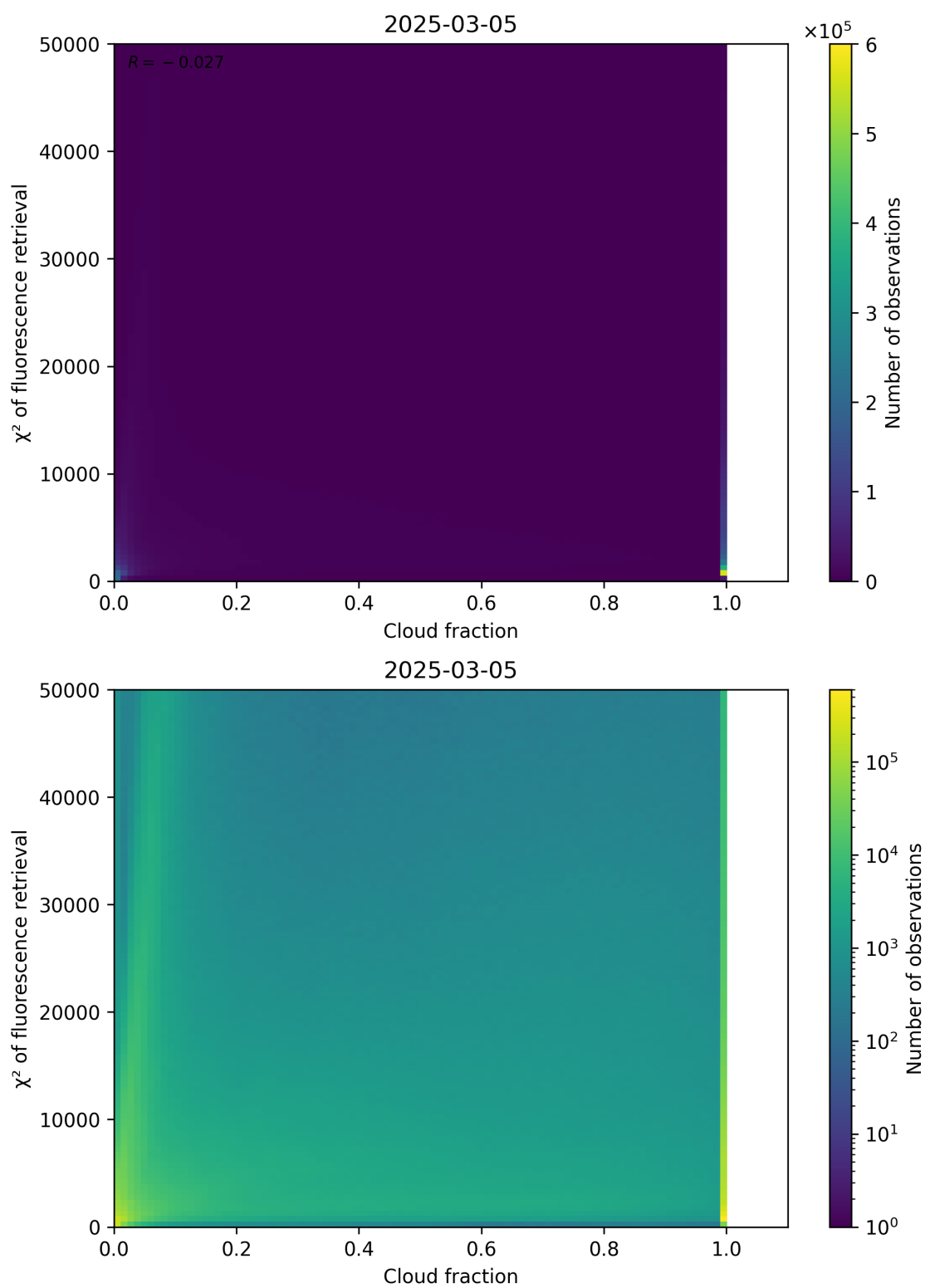
Figure 71: Scatter density plot of “Cloud fraction” against “ \chi^2 of fluorescence retrieval” for 2025-03-04 to 2025-03-06.
