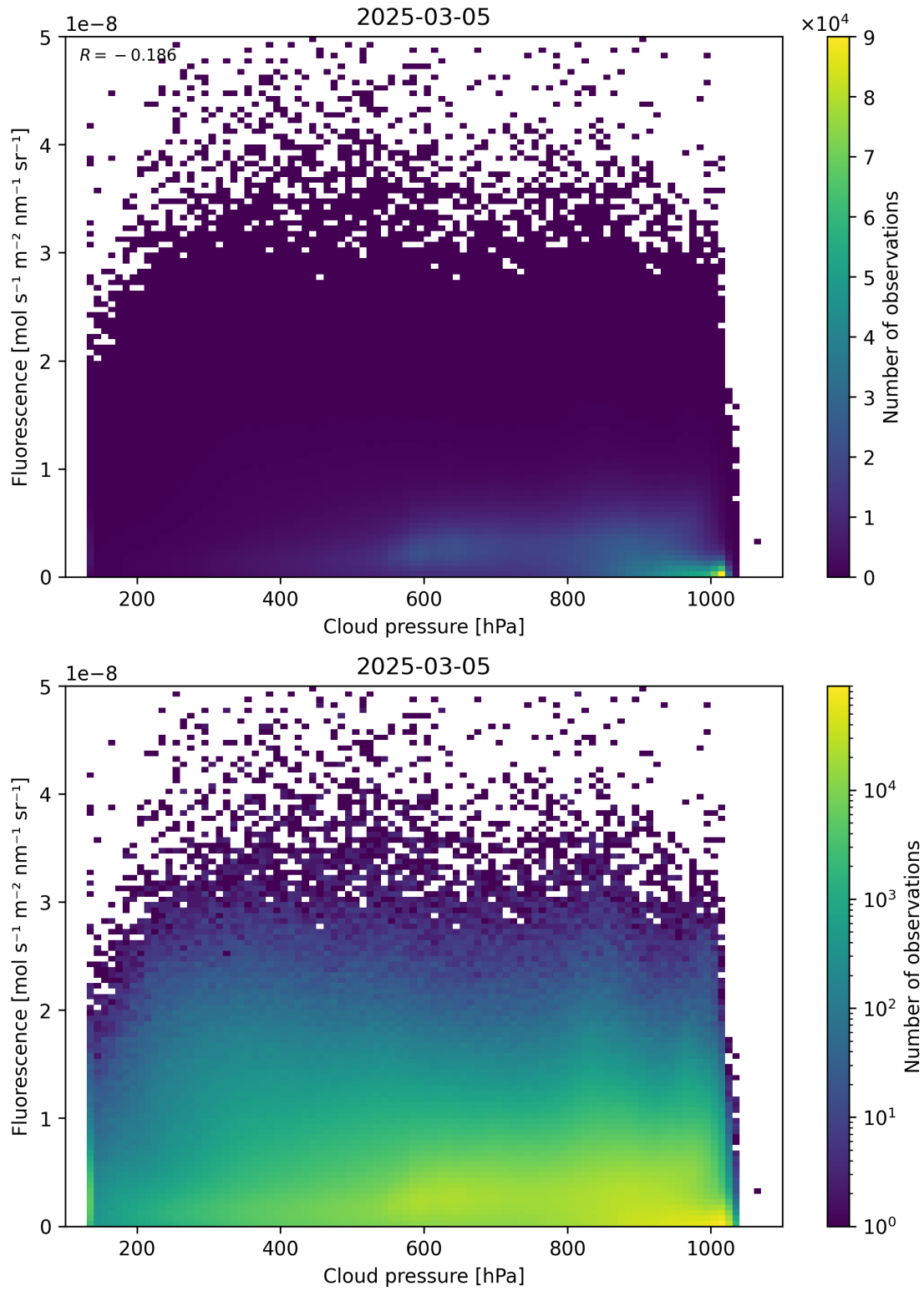
Figure 80: Scatter density plot of “Cloud pressure” against “Fluorescence” for 2025-03-04 to 2025-03-06.
