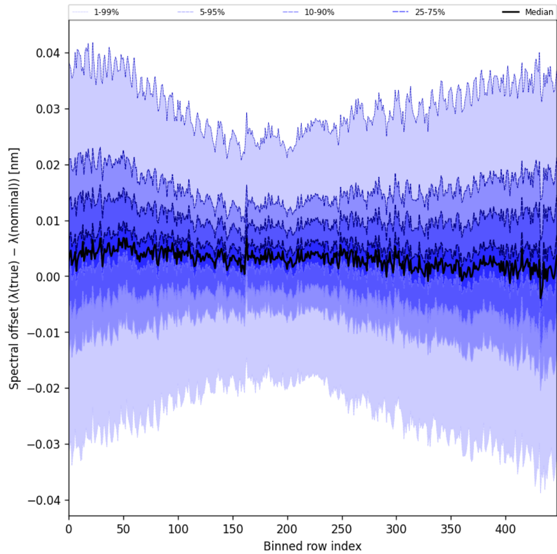
Figure 62: Along track statistics of “Spectral offset ( \lambda_{\text{true}} - \lambda_{\text{nominal}} )” for 2025-03-04 to 2025-03-06
