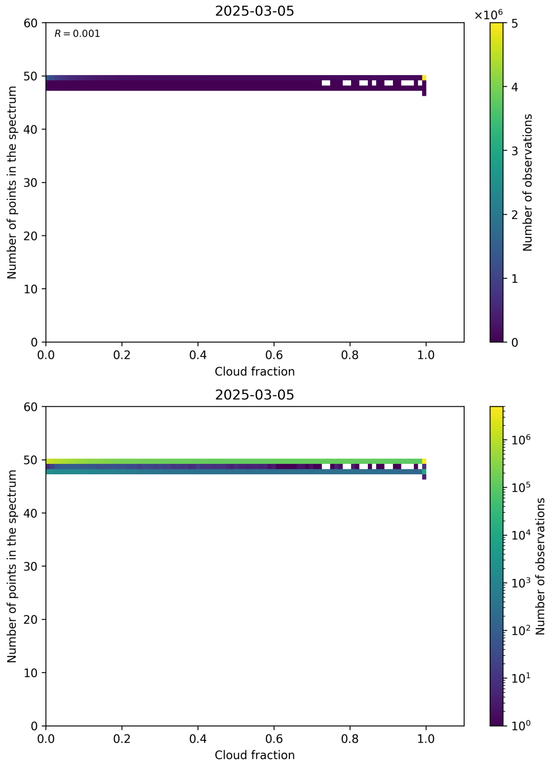
Figure 74: Scatter density plot of “Cloud fraction” against “Number of points in the spectrum” for 2025-03-04 to 2025-03-06.
