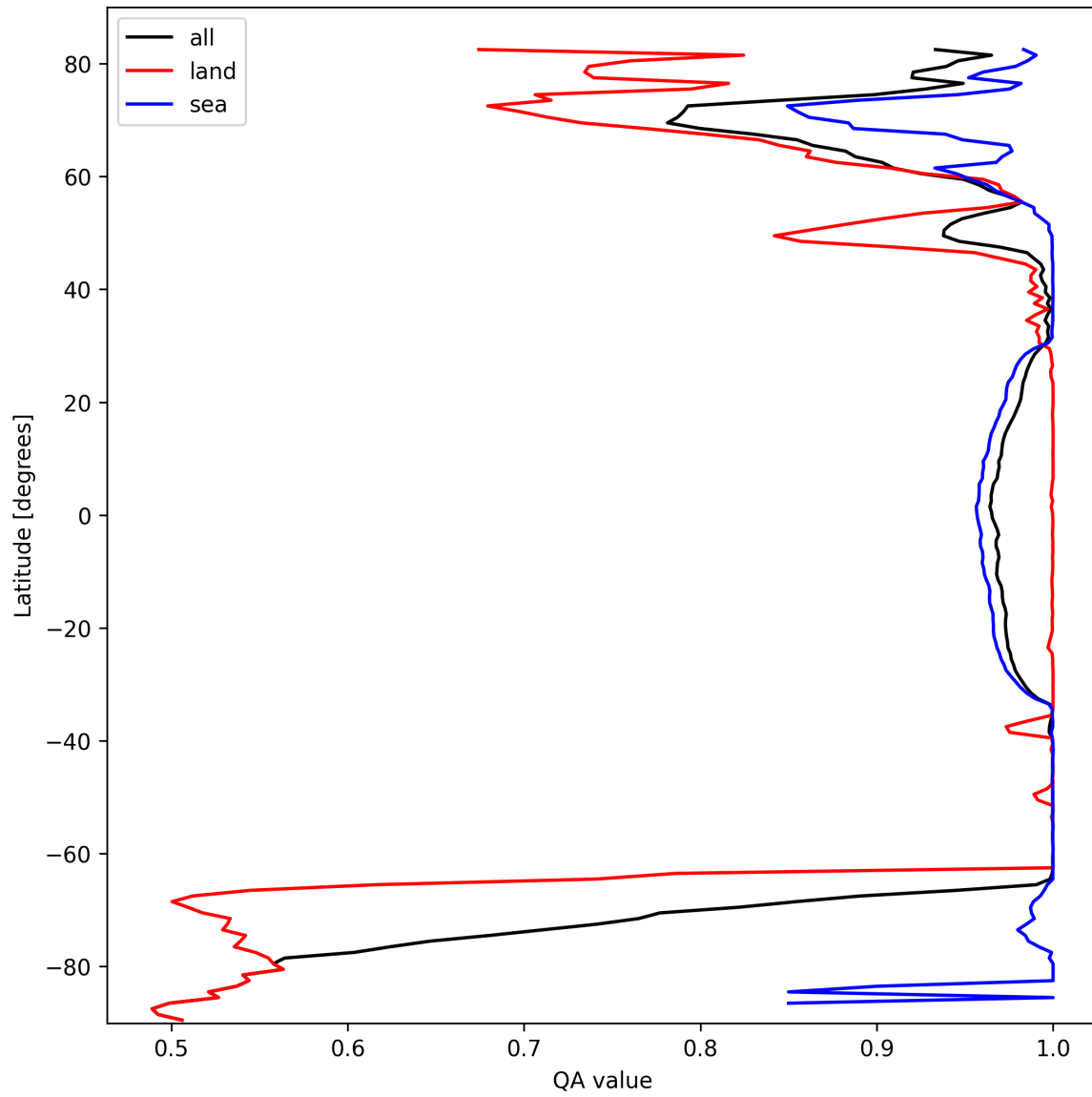
Figure 12: Zonal average of “QA value” for 2025-03-04 to 2025-03-06.
