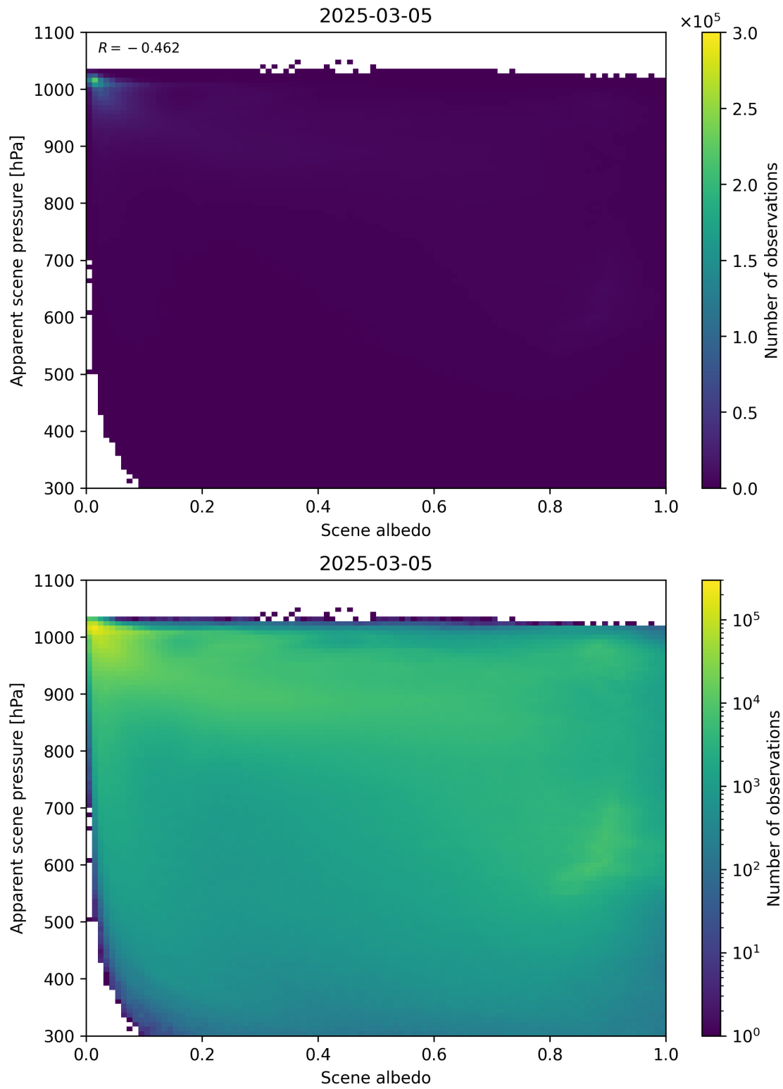
Figure 102: Scatter density plot of “Scene albedo” against “Apparent scene pressure” for 2025-03-04 to 2025-03-06.
