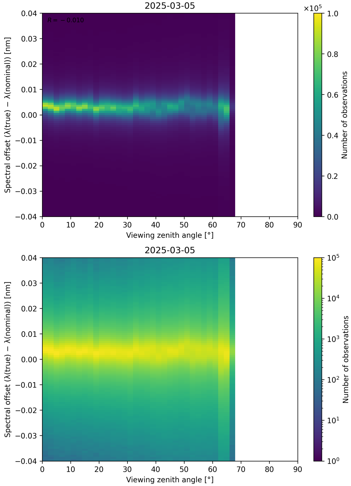
Figure 128: Scatter density plot of “Viewing zenith angle” against “Spectral offset ( \lambda_{\text{true}} - \lambda_{\text{nominal}} )” for 2025-03-04 to 2025-03-06.
