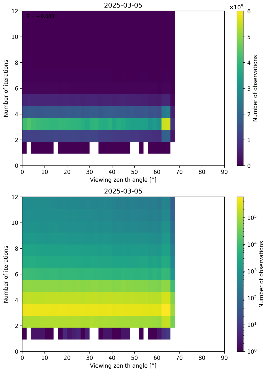
Figure 124: Scatter density plot of “Viewing zenith angle” against “Number of iterations” for 2025-03-04 to 2025-03-06.
