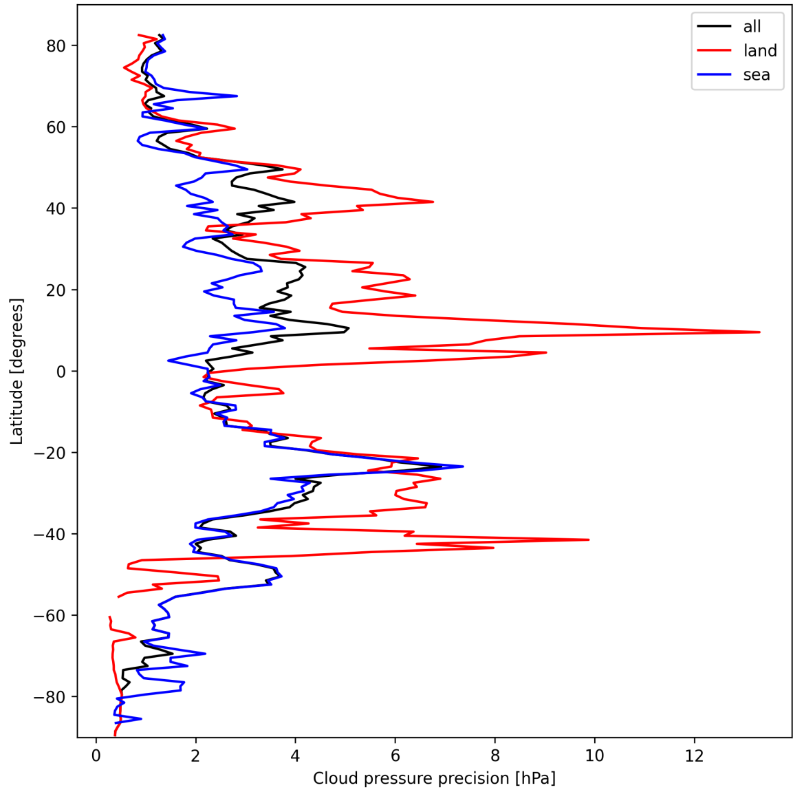
Figure 14: Zonal average of "Cloud pressure precision" for 2025-03-04 to 2025-03-06.
