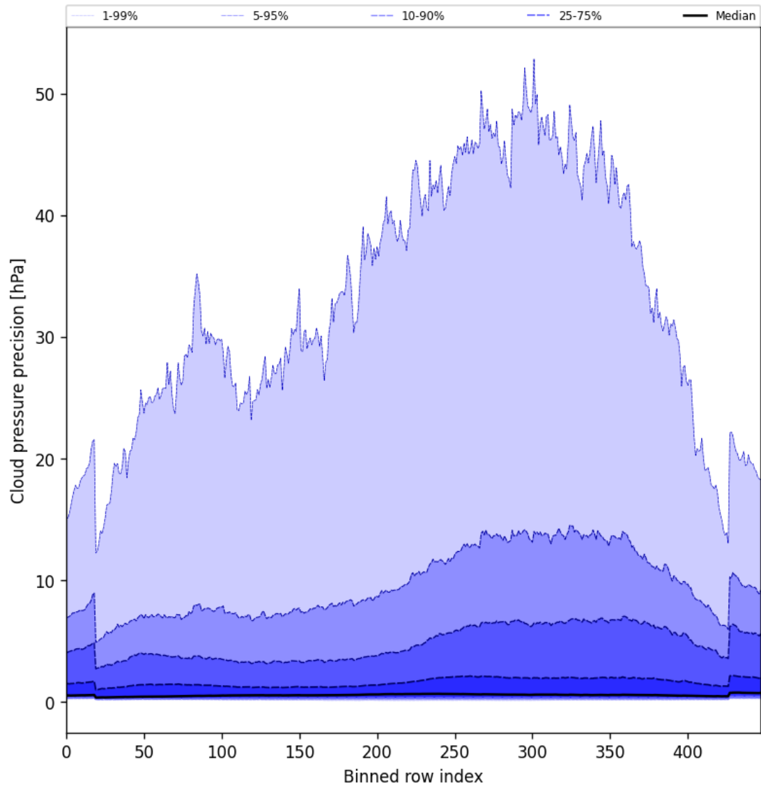
Figure 48: Along track statistics of “Cloud pressure precision” for 2025-03-04 to 2025-03-06
