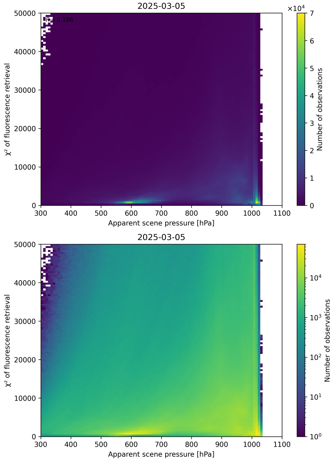
Figure 63: Scatter density plot of “Apparent scene pressure” against “ \chi^2 of fluorescence retrieval” for 2025-03-04 to 2025-03-06.
