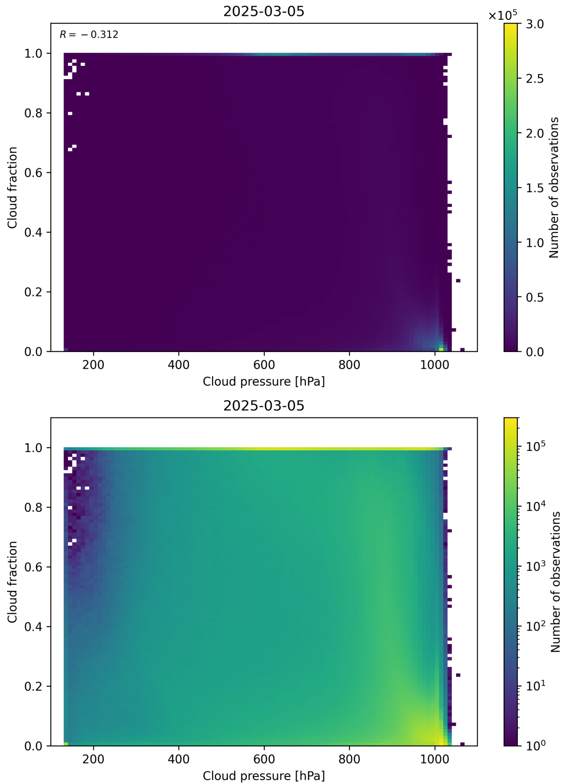
Figure 79: Scatter density plot of “Cloud pressure” against “Cloud fraction” for 2025-03-04 to 2025-03-06.
