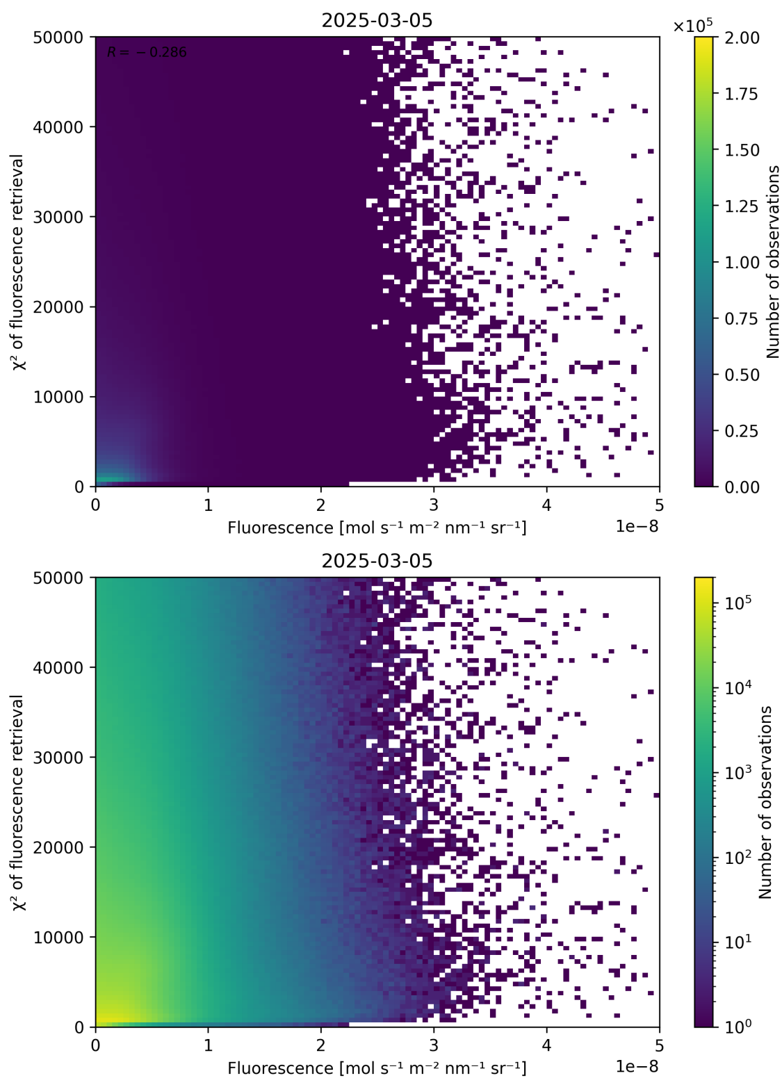
Figure 85: Scatter density plot of “Fluorescence” against “ \chi^2 of fluorescence retrieval” for 2025-03-04 to 2025-03-06.
