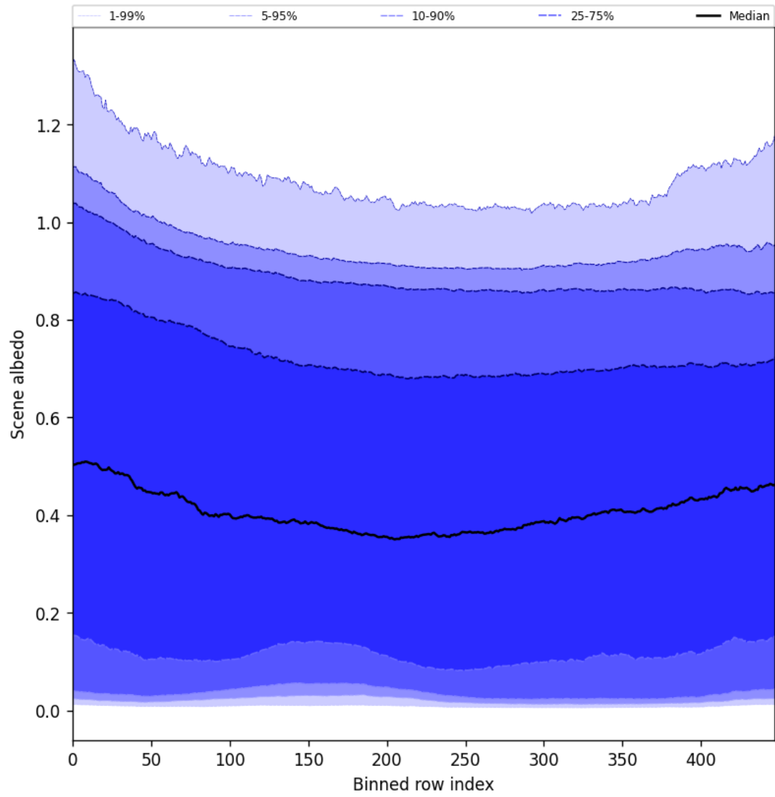
Figure 51: Along track statistics of “Scene albedo” for 2025-03-04 to 2025-03-06
