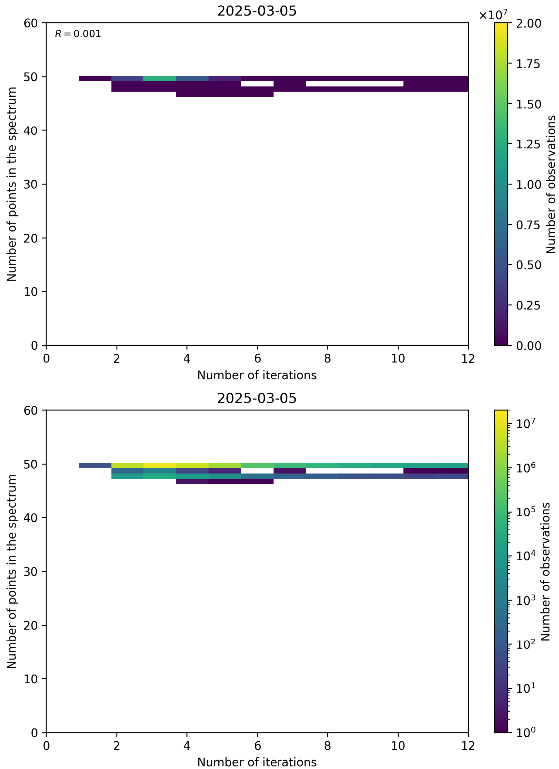
Figure 99: Scatter density plot of “Number of iterations” against “Number of points in the spectrum” for 2025-03-04 to 2025-03-06.
