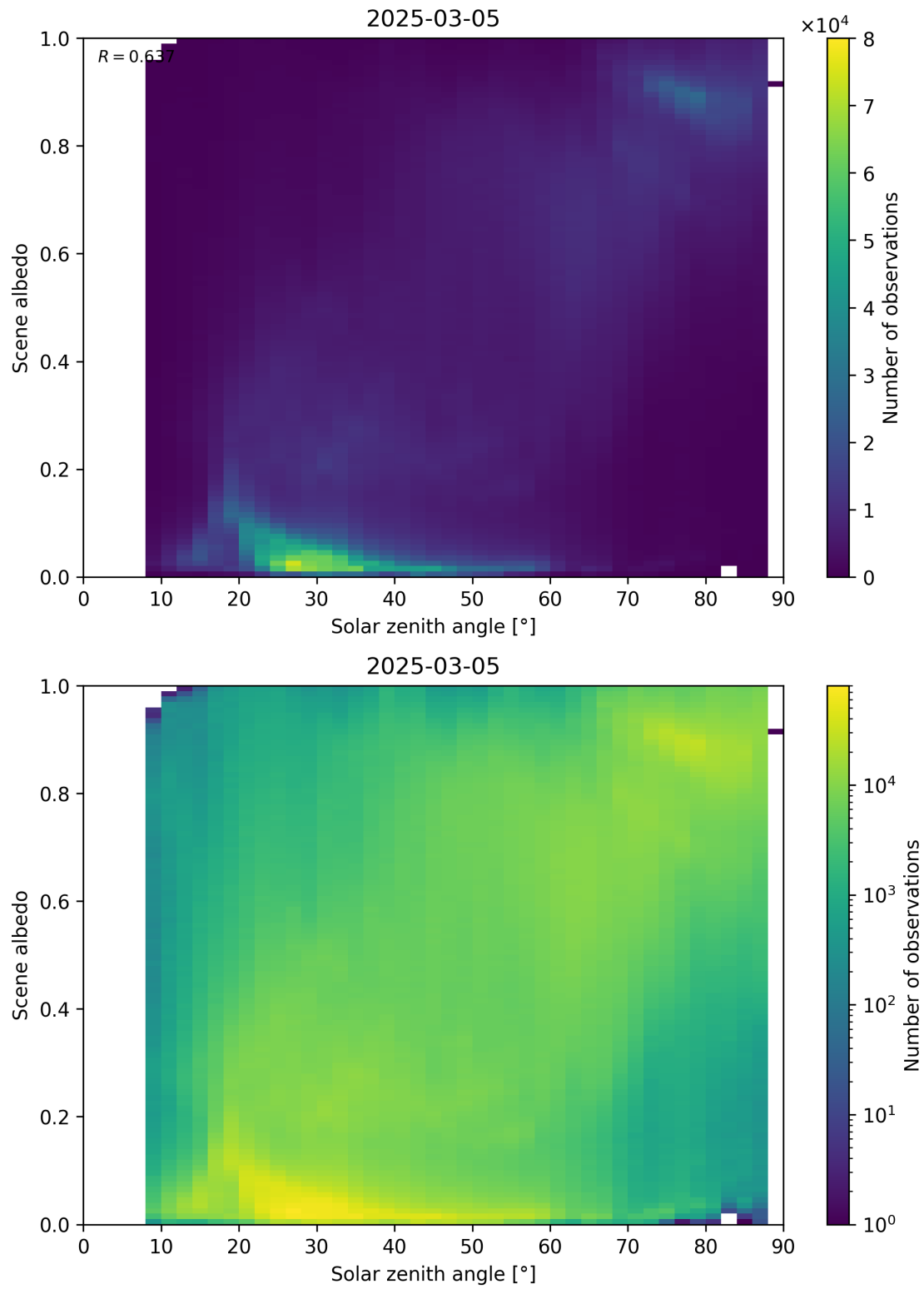
Figure 116: Scatter density plot of “Solar zenith angle” against “Scene albedo” for 2025-03-04 to 2025-03-06.
