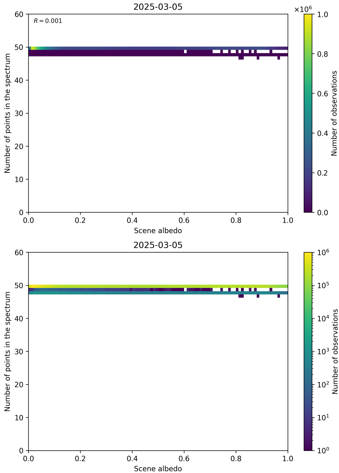
Figure 106: Scatter density plot of “Scene albedo” against “Number of points in the spectrum” for 2025-03-04 to 2025-03-06.
