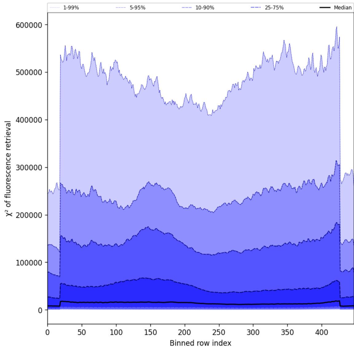
Figure 59: Along track statistics of “ \chi^2 of fluorescence retrieval” for 2025-03-04 to 2025-03-06
