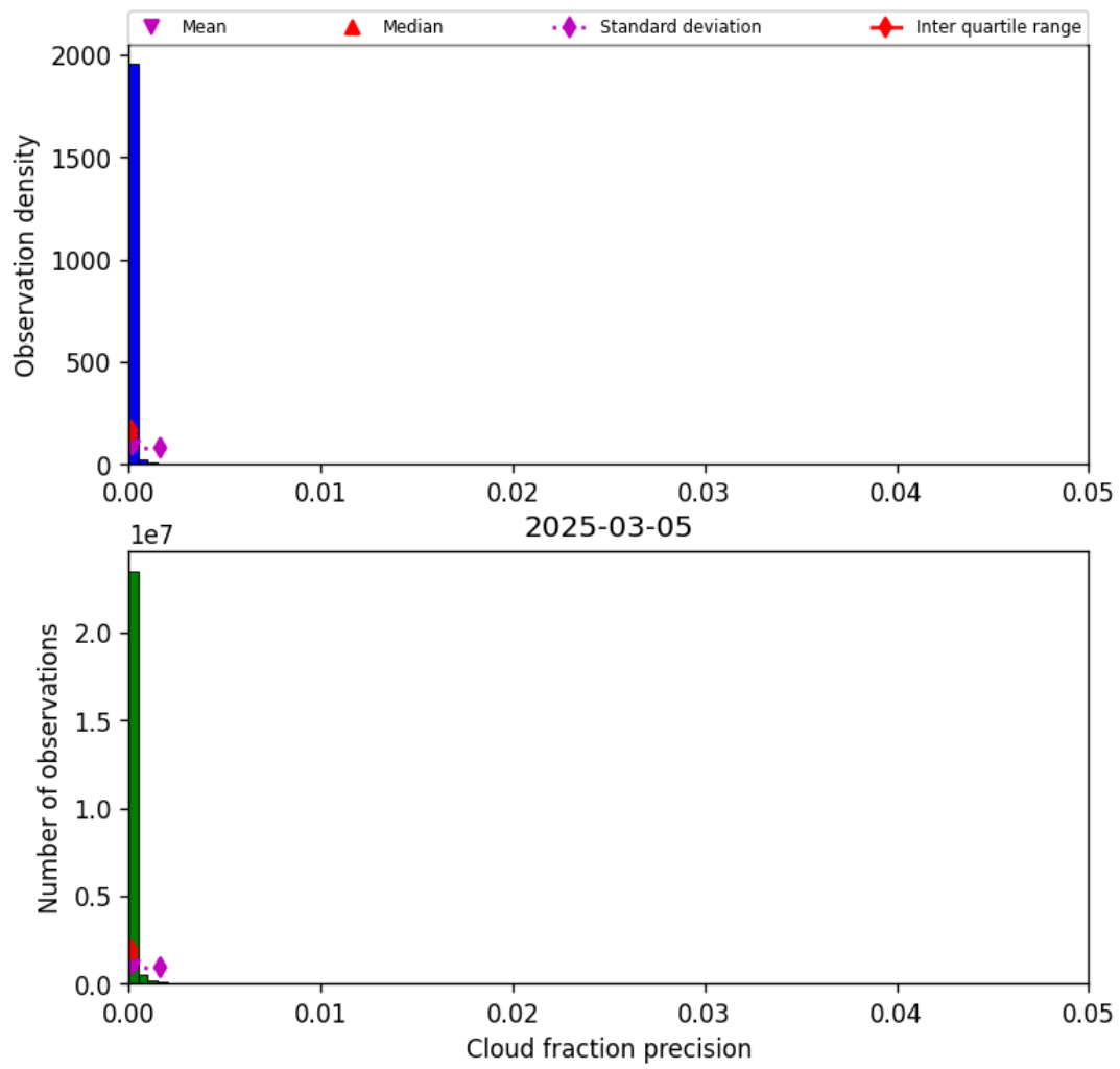
Figure 33: Histogram of “Cloud fraction precision” for 2025-03-04 to 2025-03-06
