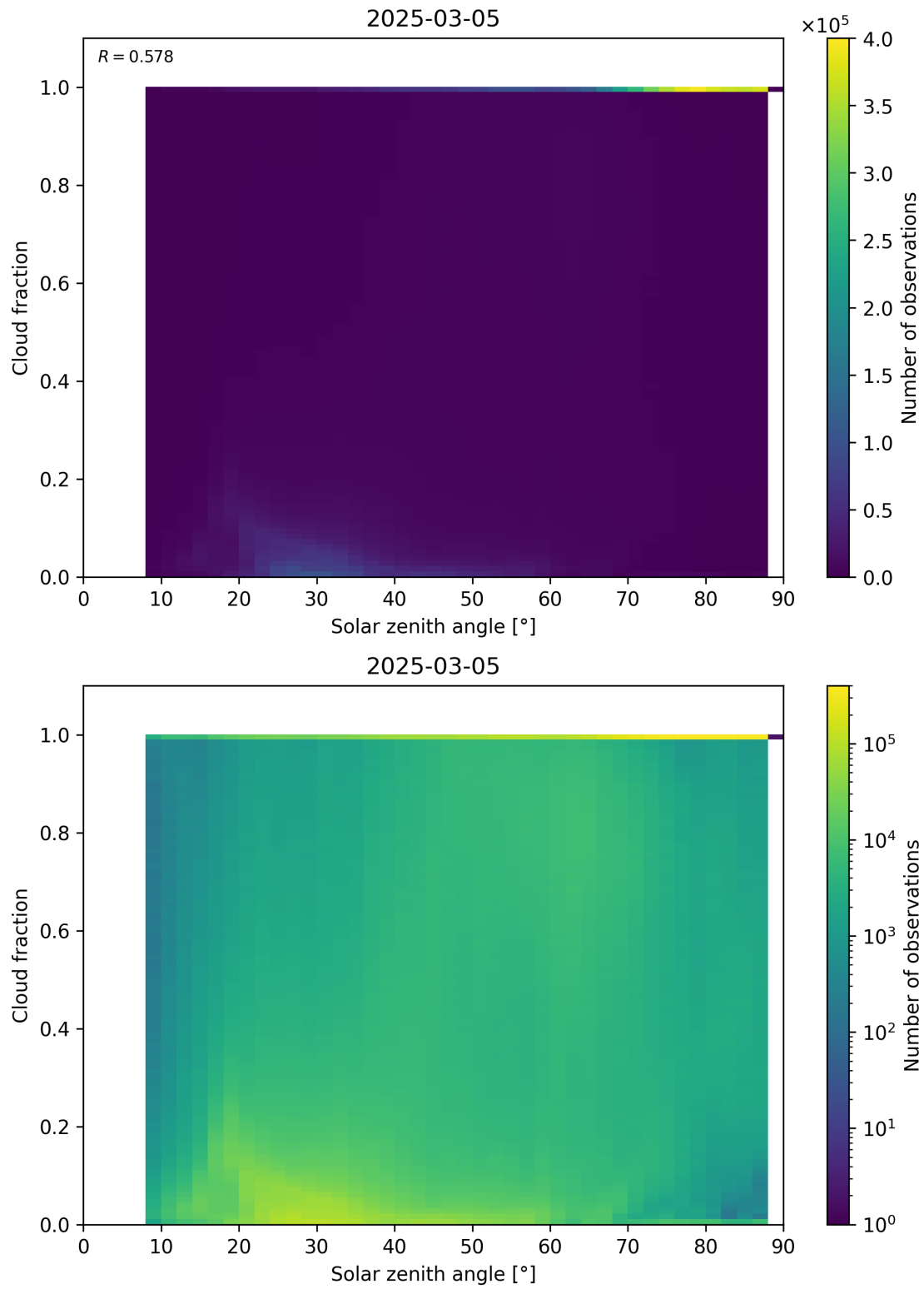
Figure 110: Scatter density plot of “Solar zenith angle” against “Cloud fraction” for 2025-03-04 to 2025-03-06.
