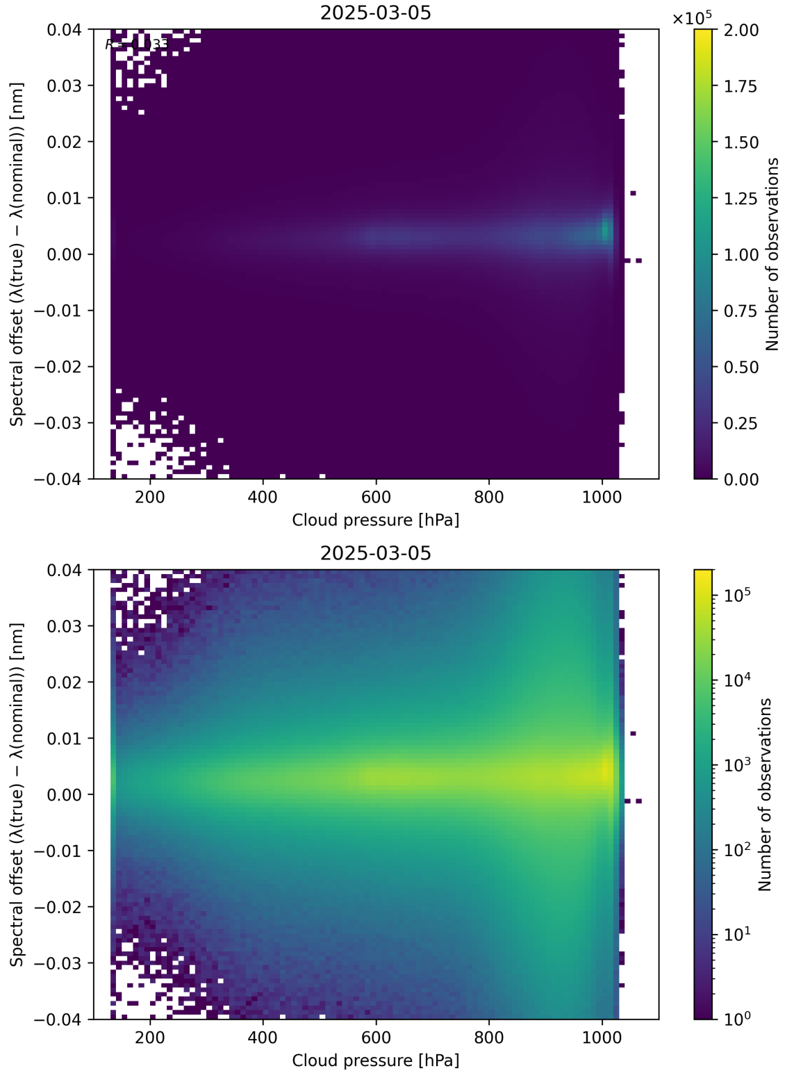
Figure 84: Scatter density plot of “Cloud pressure” against “Spectral offset ( \lambda_{\text{true}} - \lambda_{\text{nominal}} )” for 2025-03-04 to 2025-03-06.
