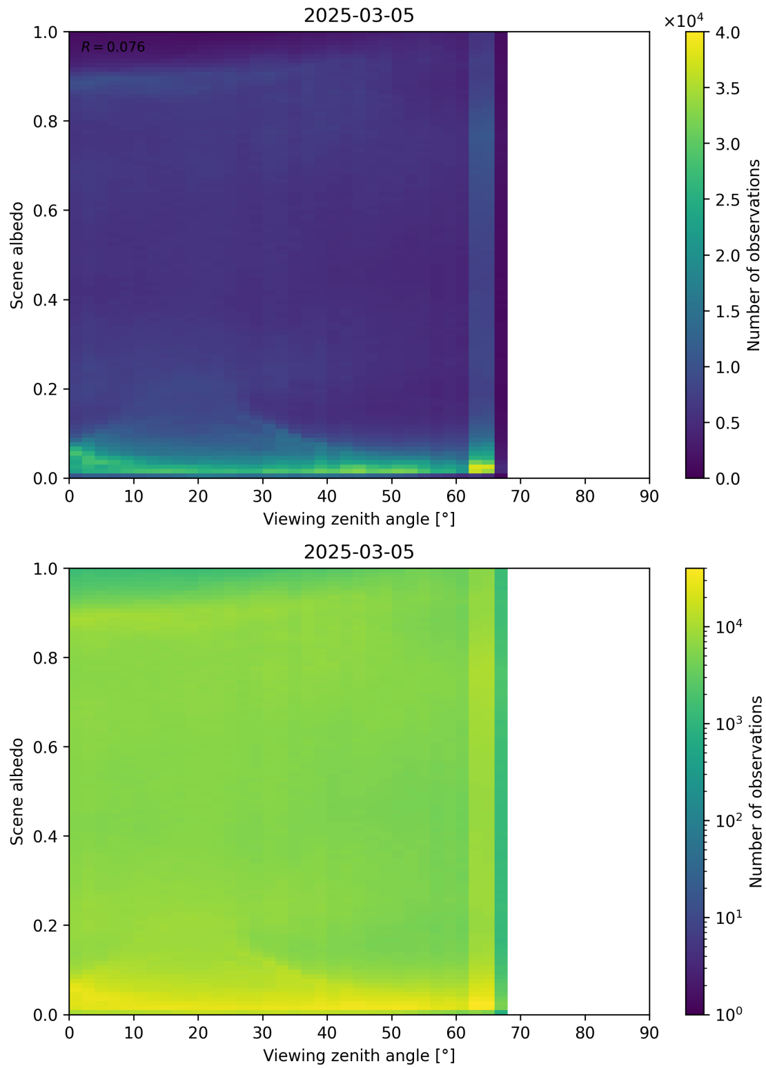
Figure 126: Scatter density plot of “Viewing zenith angle” against “Scene albedo” for 2025-03-04 to 2025-03-06.
