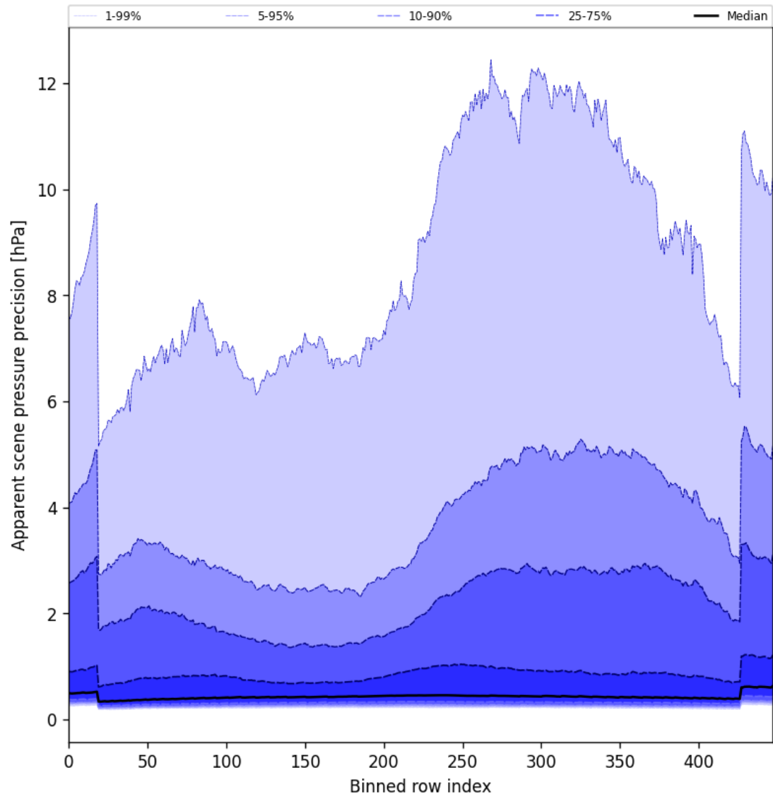
Figure 54: Along track statistics of “Apparent scene pressure precision” for 2025-03-04 to 2025-03-06
