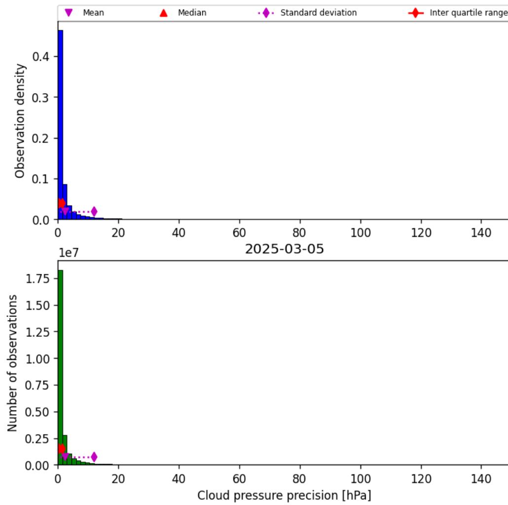
Figure 31: Histogram of “Cloud pressure precision” for 2025-03-04 to 2025-03-06
