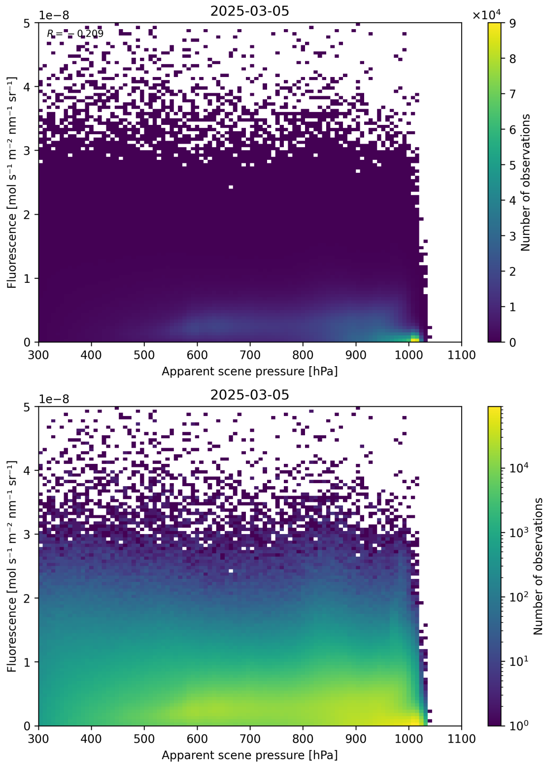
Figure 64: Scatter density plot of “Apparent scene pressure” against “Fluorescence” for 2025-03-04 to 2025-03-06.
