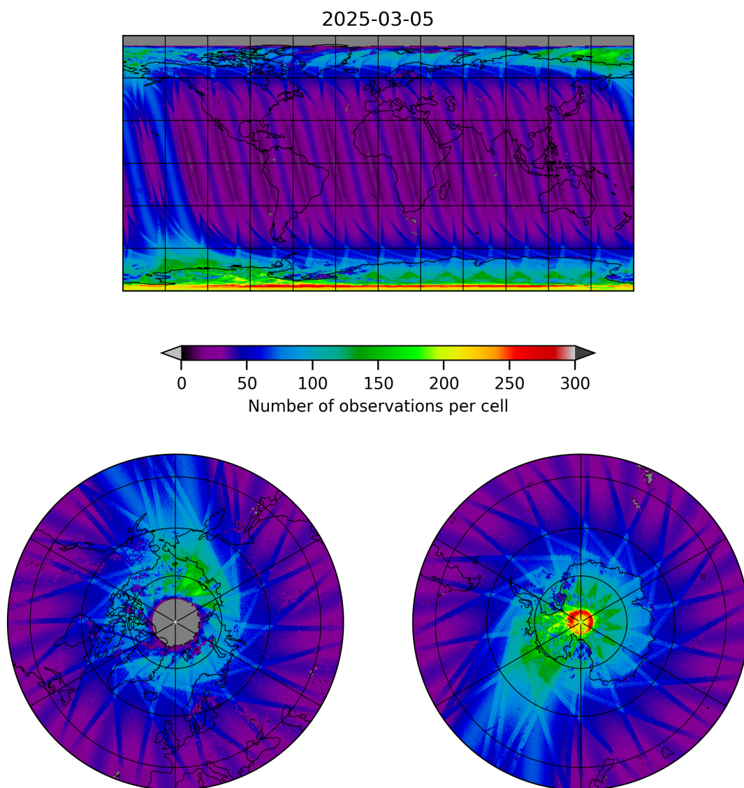
Figure 11: Map of the number of observations for 2025-03-04 to 2025-03-06
