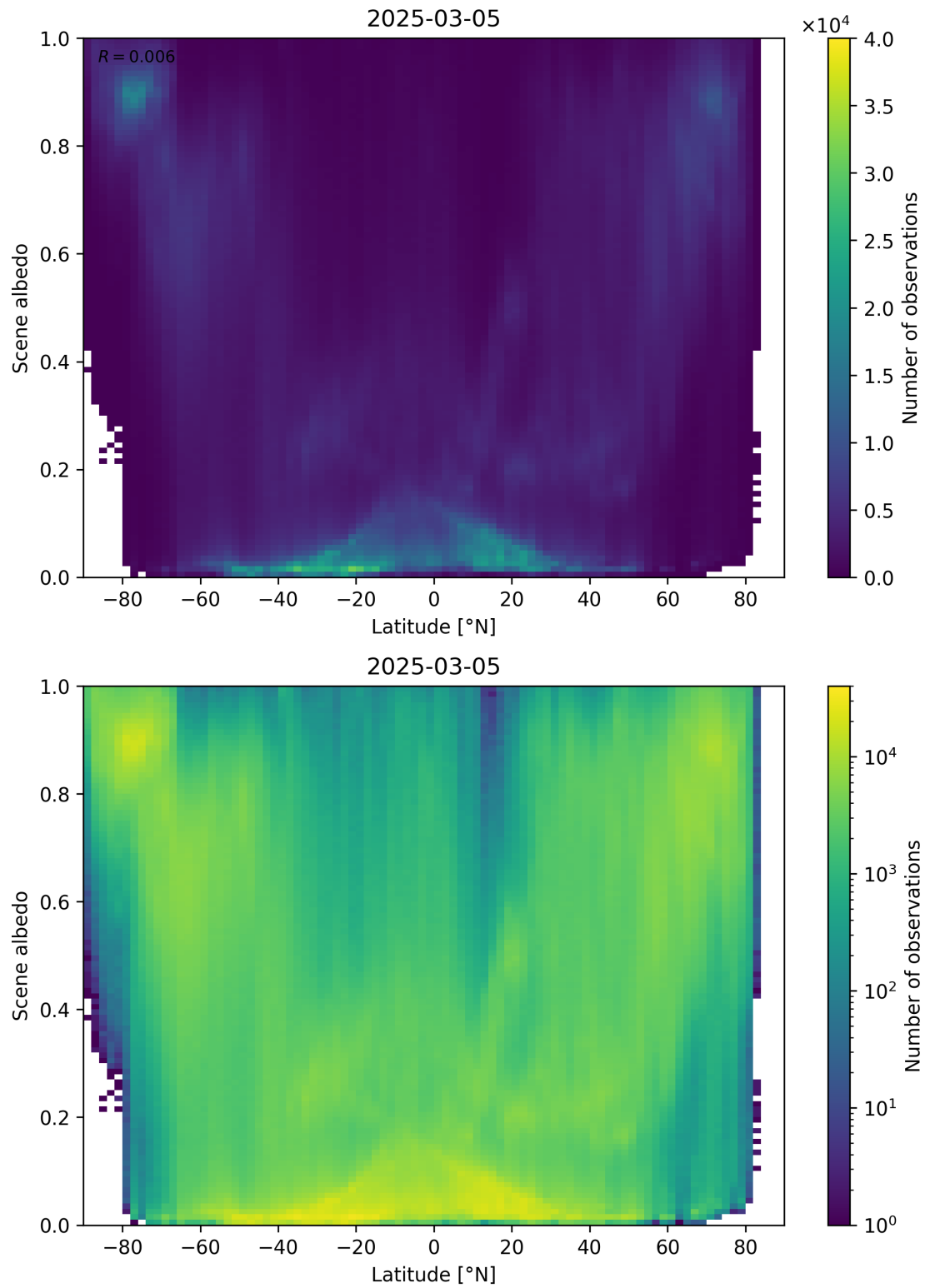
Figure 95: Scatter density plot of “Latitude” against “Scene albedo” for 2025-03-04 to 2025-03-06.
