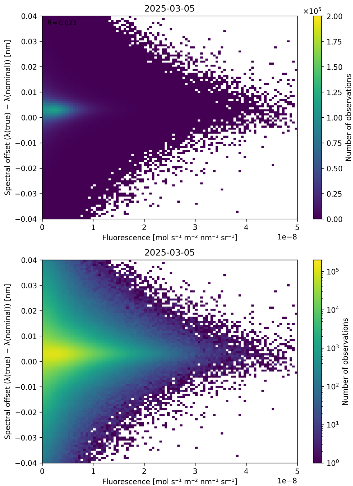
Figure 87: Scatter density plot of “Fluorescence” against “Spectral offset ( \lambda_{\text{true}} - \lambda_{\text{nominal}} )” for 2025-03-04 to 2025-03-06.
