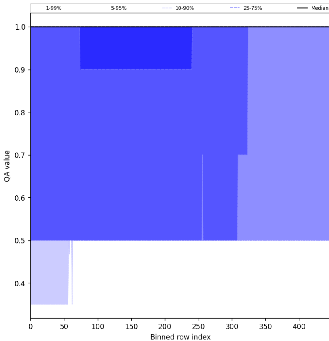
Figure 46: Along track statistics of “QA value” for 2025-03-04 to 2025-03-06
