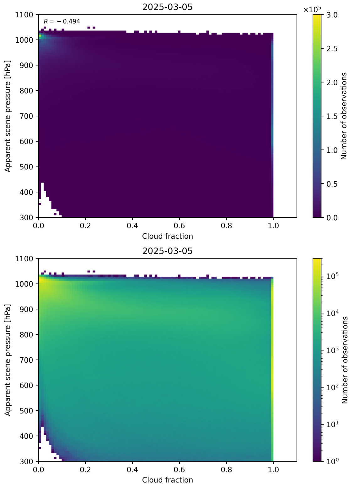
Figure 70: Scatter density plot of “Cloud fraction” against “Apparent scene pressure” for 2025-03-04 to 2025-03-06.
