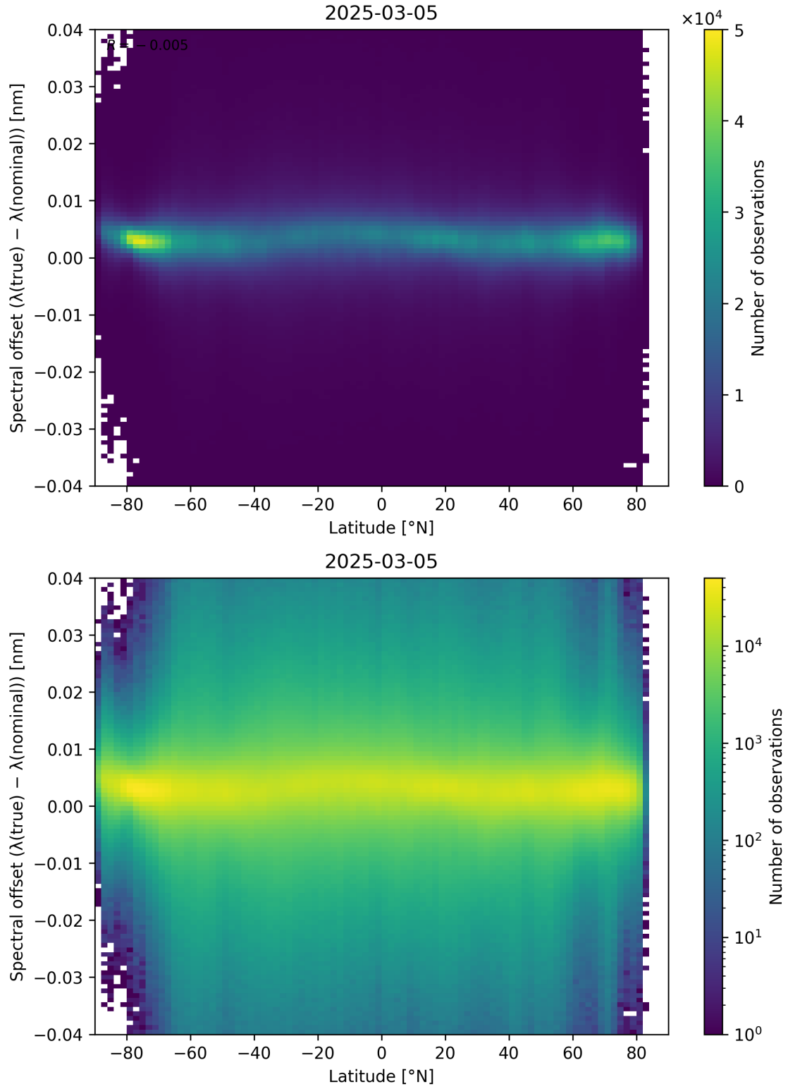
Figure 96: Scatter density plot of “Latitude” against “Spectral offset ( \lambda_{\text{true}} - \lambda_{\text{nominal}} )” for 2025-03-04 to 2025-03-06.
