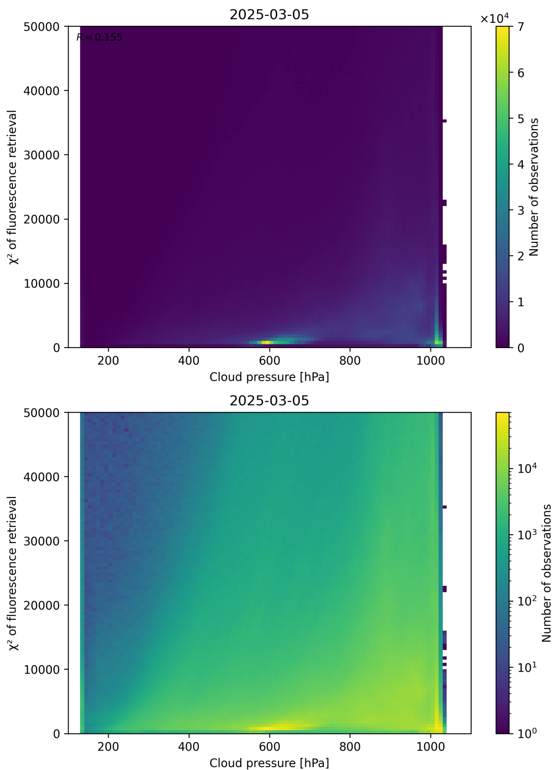
Figure 78: Scatter density plot of “Cloud pressure” against “ \chi^2 of fluorescence retrieval” for 2025-03-04 to 2025-03-06.
