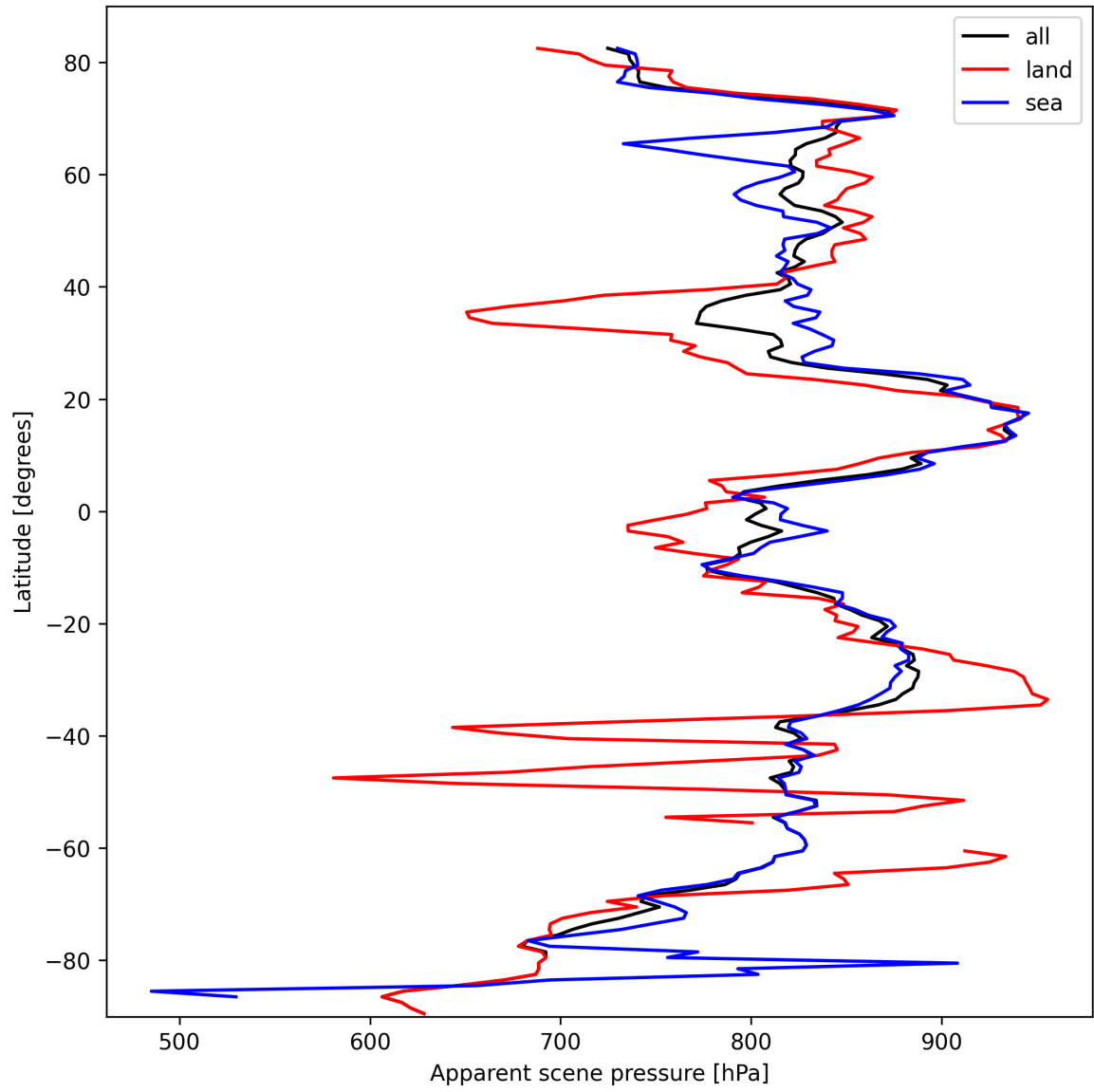
Figure 19: Zonal average of “Apparent scene pressure” for 2025-03-04 to 2025-03-06.
