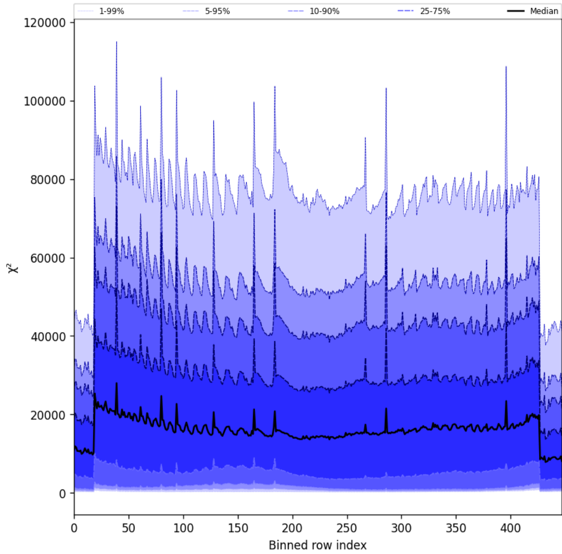
Figure 55: Along track statistics of “ \chi^2 ” for 2025-03-04 to 2025-03-06
