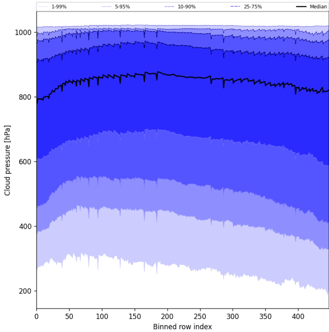
Figure 47: Along track statistics of “Cloud pressure” for 2025-03-04 to 2025-03-06
