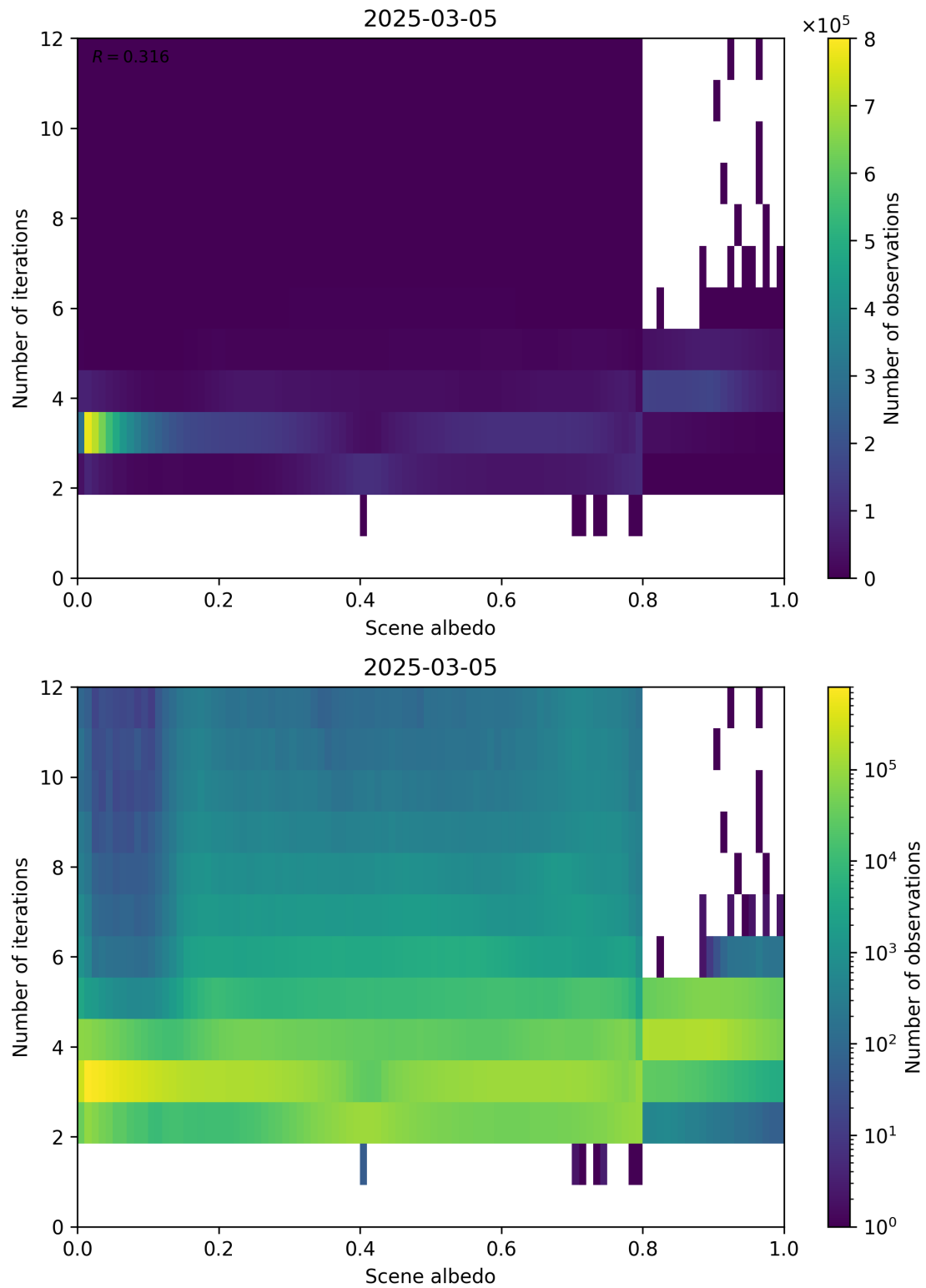
Figure 105: Scatter density plot of “Scene albedo” against “Number of iterations” for 2025-03-04 to 2025-03-06.
