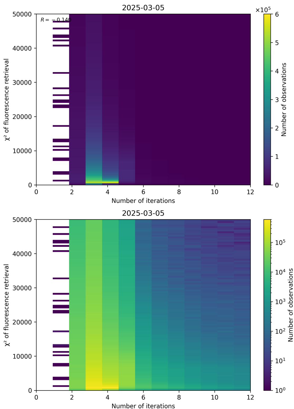
Figure 97: Scatter density plot of “Number of iterations” against “ \chi^2 of fluorescence retrieval” for 2025-03-04 to 2025-03-06.
