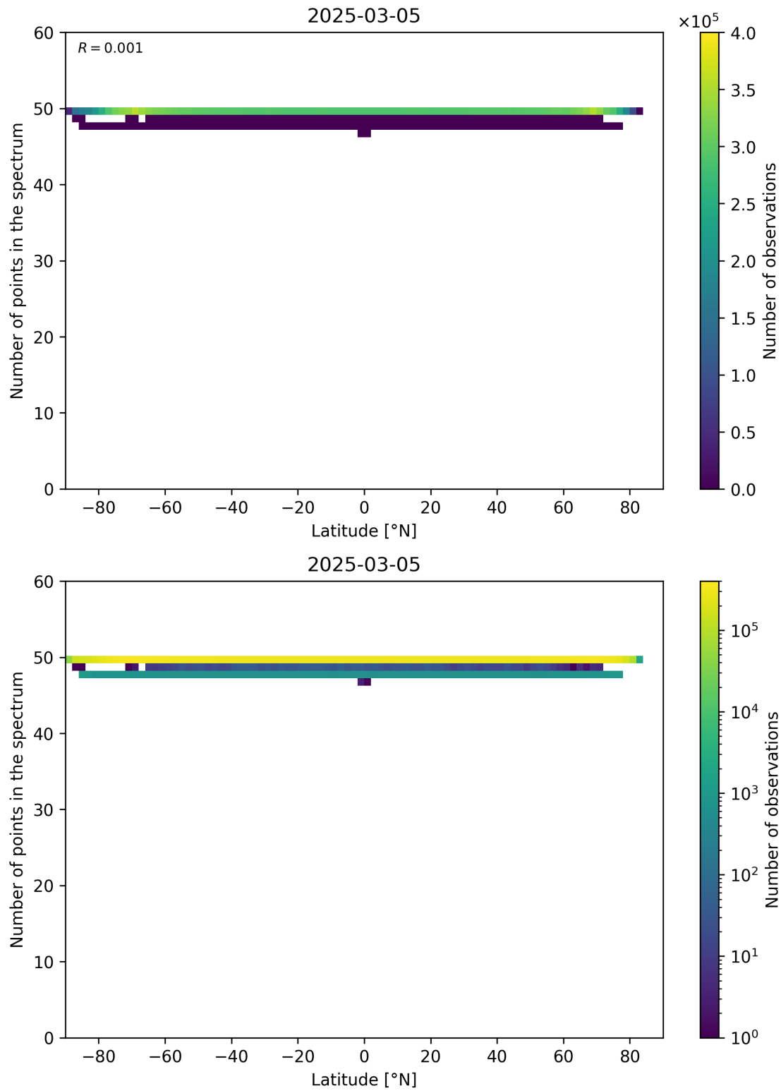
Figure 94: Scatter density plot of “Latitude” against “Number of points in the spectrum” for 2025-03-04 to 2025-03-06.
