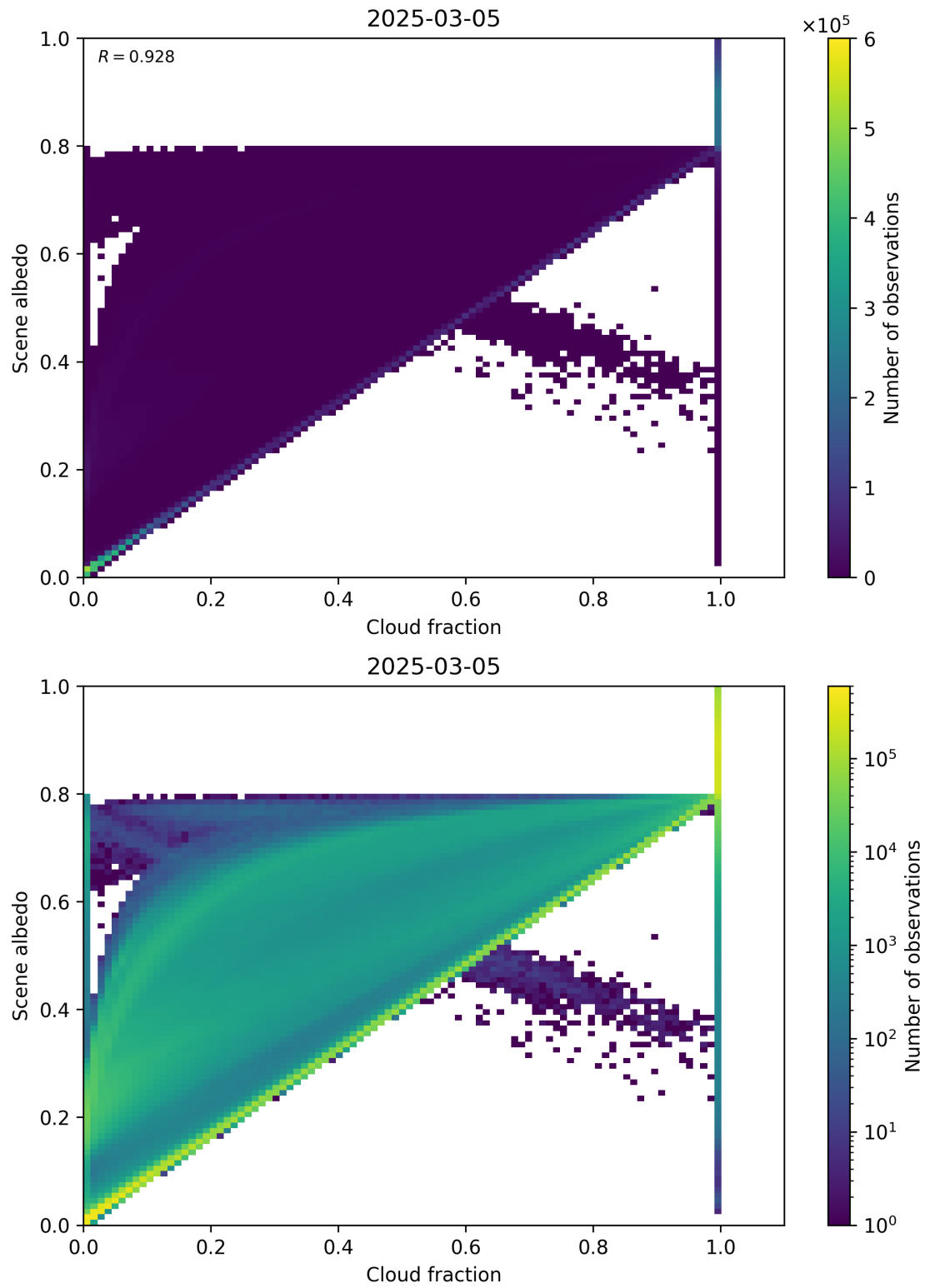
Figure 75: Scatter density plot of “Cloud fraction” against “Scene albedo” for 2025-03-04 to 2025-03-06.
