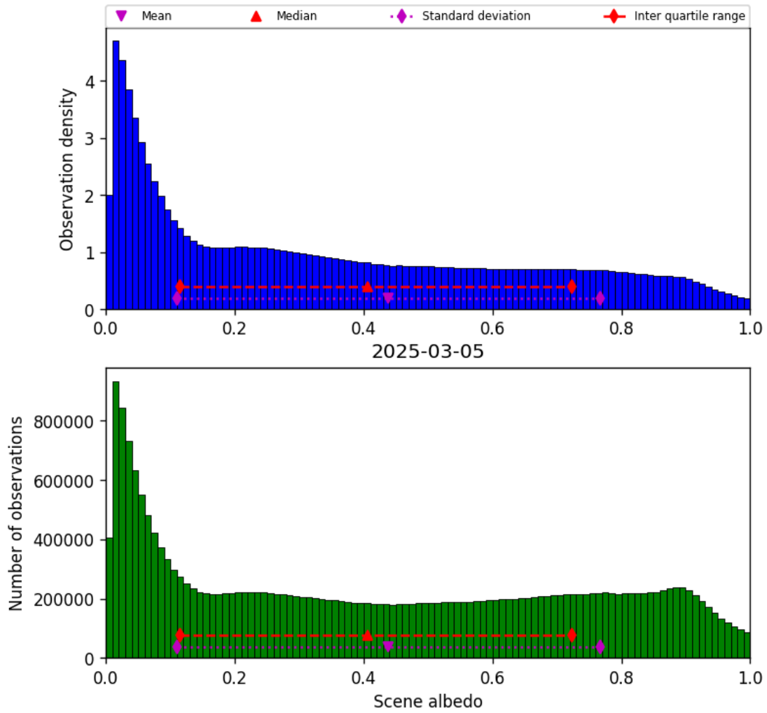
Figure 34: Histogram of “Scene albedo” for 2025-03-04 to 2025-03-06
