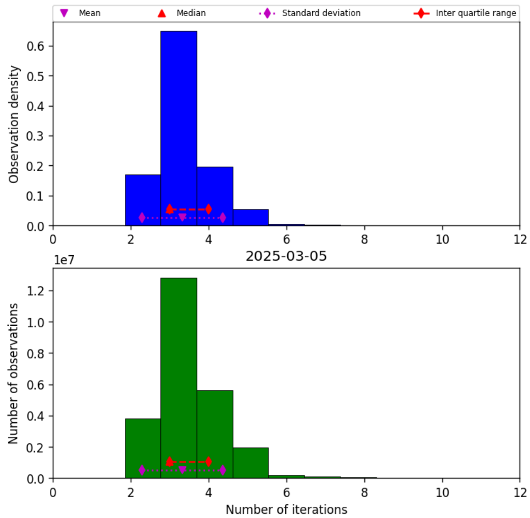
Figure 39: Histogram of “Number of iterations” for 2025-03-04 to 2025-03-06
