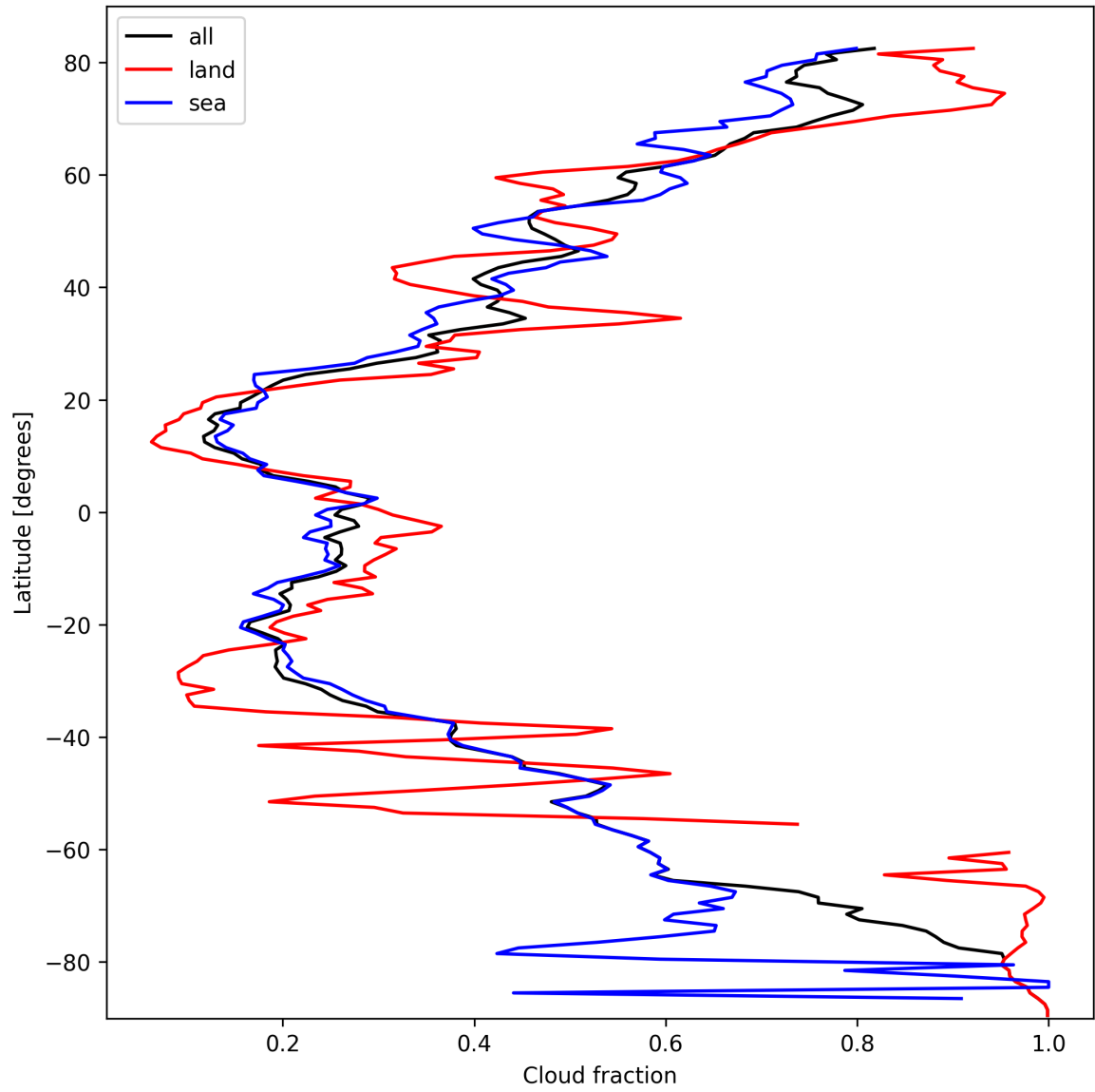
Figure 15: Zonal average of “Cloud fraction” for 2025-03-04 to 2025-03-06.
