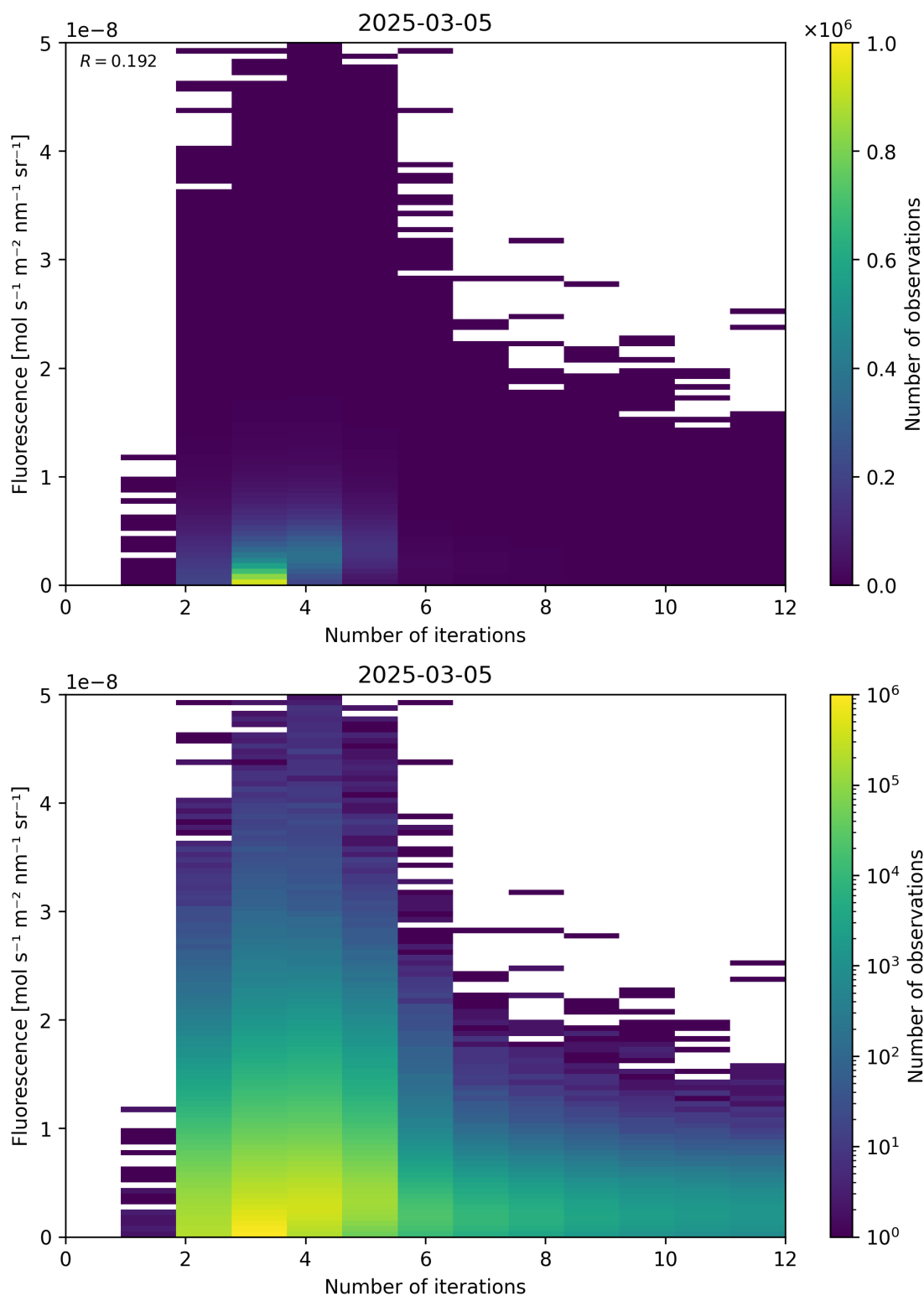
Figure 98: Scatter density plot of “Number of iterations” against “Fluorescence” for 2025-03-04 to 2025-03-06.
