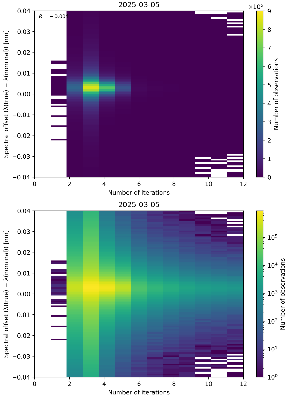
Figure 100: Scatter density plot of “Number of iterations” against “Spectral offset ( \lambda_{\text{true}} - \lambda_{\text{nominal}} )” for 2025-03-04 to 2025-03-06.
