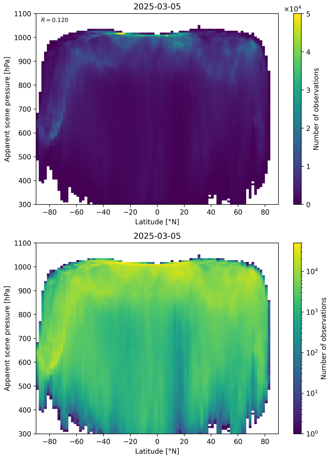
Figure 88: Scatter density plot of “Latitude” against “Apparent scene pressure” for 2025-03-04 to 2025-03-06.
