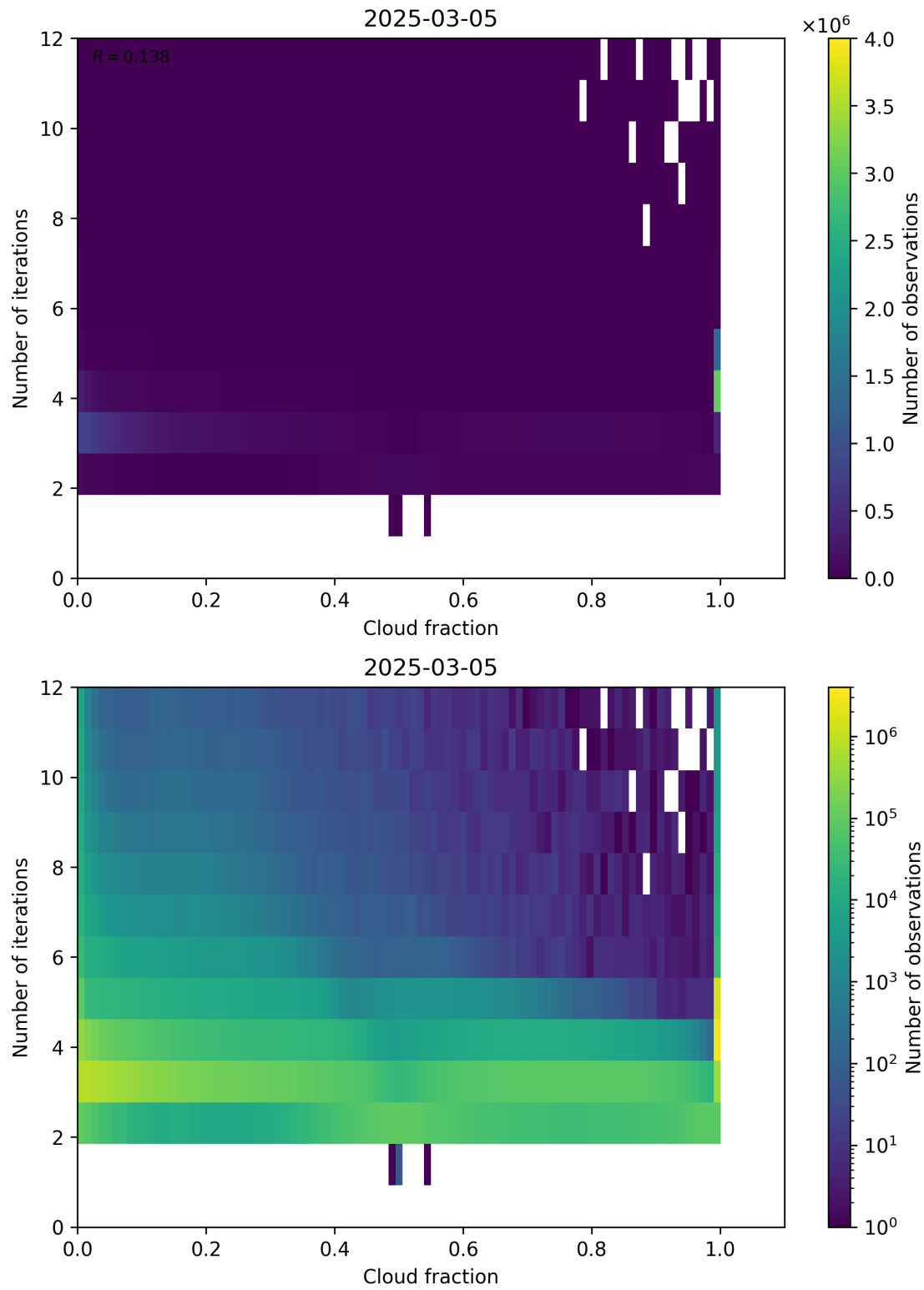
Figure 73: Scatter density plot of “Cloud fraction” against “Number of iterations” for 2025-03-04 to 2025-03-06.
