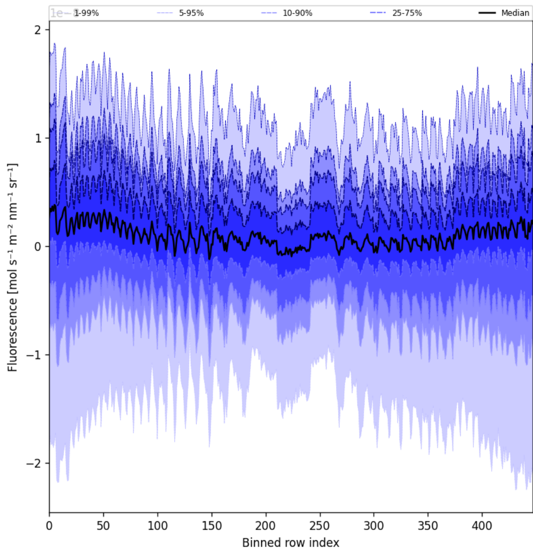
Figure 57: Along track statistics of “Fluorescence” for 2025-03-04 to 2025-03-06
