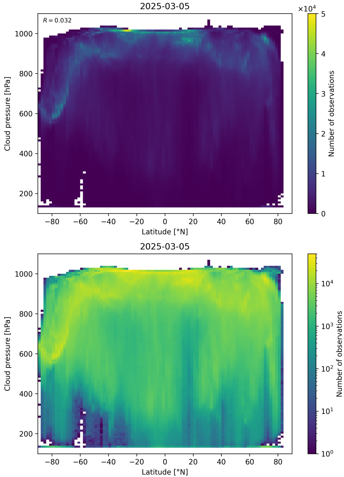
Figure 91: Scatter density plot of “Latitude” against “Cloud pressure” for 2025-03-04 to 2025-03-06.
