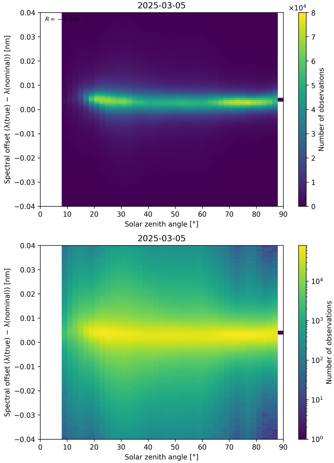
Figure 117: Scatter density plot of “Solar zenith angle” against “Spectral offset ( \lambda_{\text{true}} - \lambda_{\text{nominal}} )” for 2025-03-04 to 2025-03-06.
