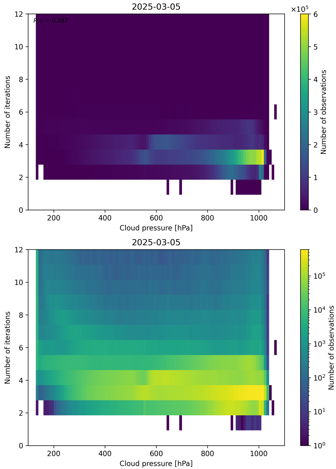
Figure 81: Scatter density plot of “Cloud pressure” against “Number of iterations” for 2025-03-04 to 2025-03-06.
