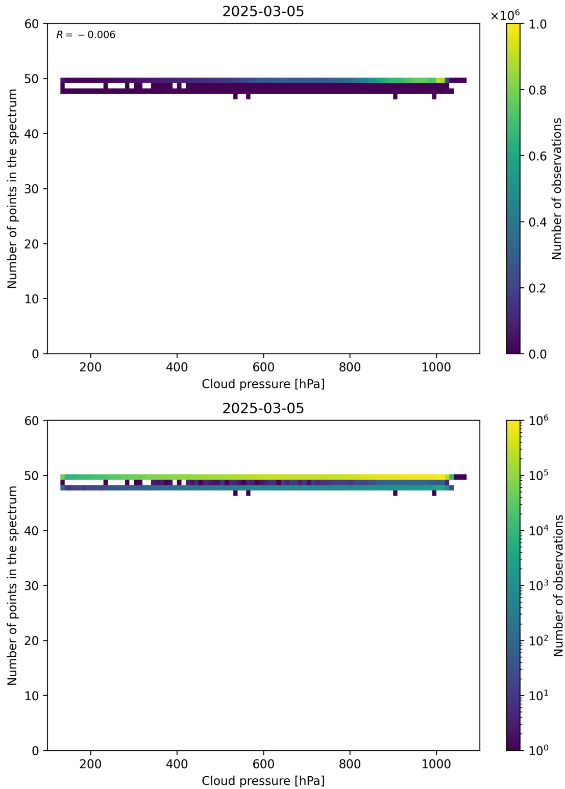
Figure 82: Scatter density plot of “Cloud pressure” against “Number of points in the spectrum” for 2025-03-04 to 2025-03-06.
