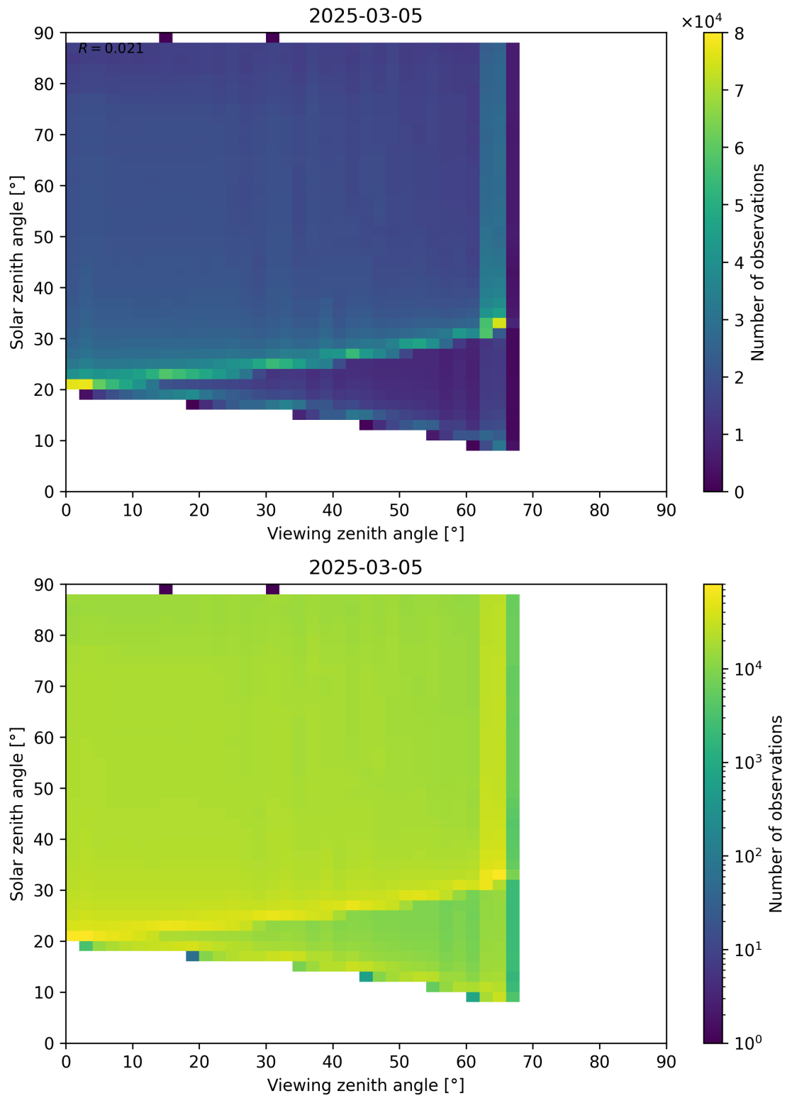
Figure 127: Scatter density plot of “Viewing zenith angle” against “Solar zenith angle” for 2025-03-04 to 2025-03-06.
