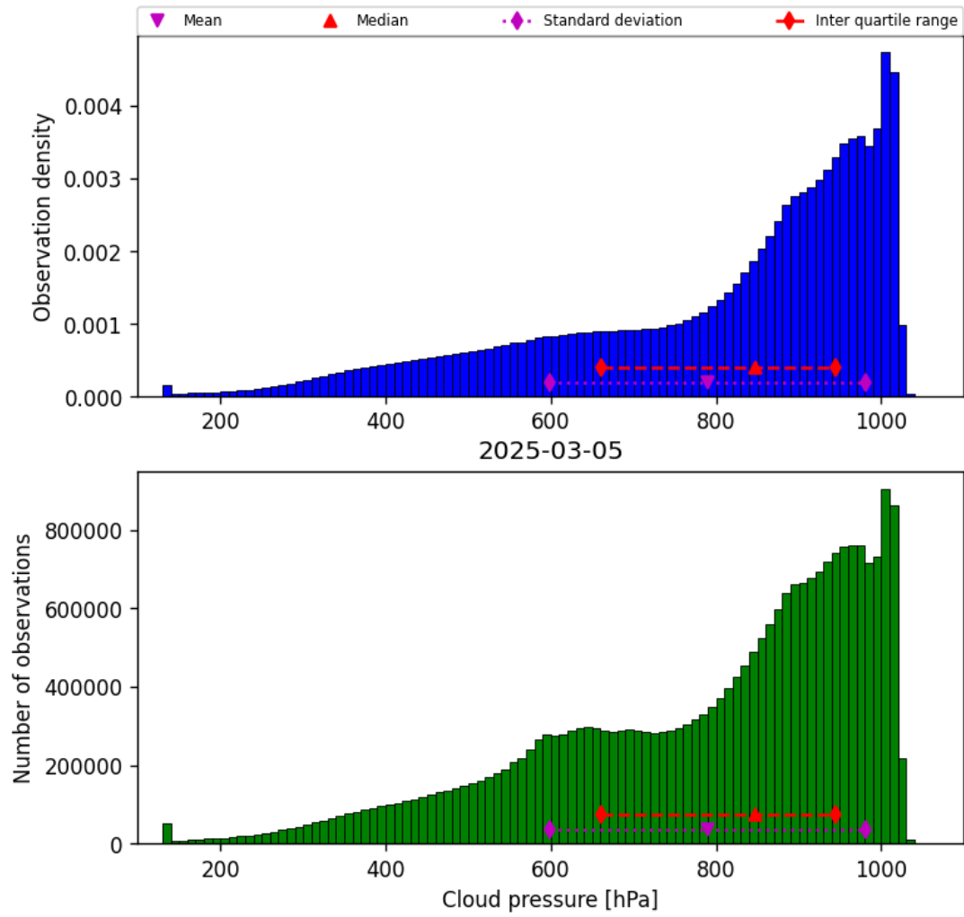
Figure 30: Histogram of “Cloud pressure” for 2025-03-04 to 2025-03-06
