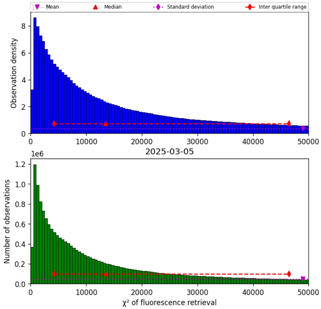
Figure 42: Histogram of “ \chi^2 of fluorescence retrieval” for 2025-03-04 to 2025-03-06
