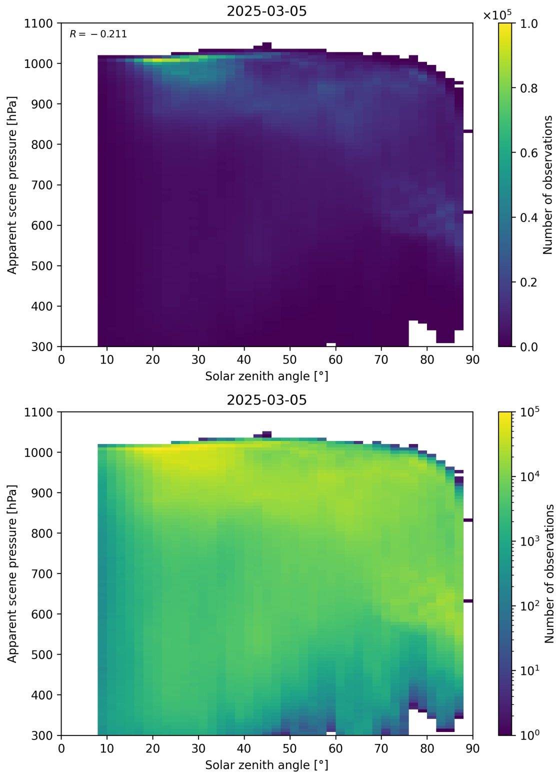
Figure 108: Scatter density plot of “Solar zenith angle” against “Apparent scene pressure” for 2025-03-04 to 2025-03-06.
