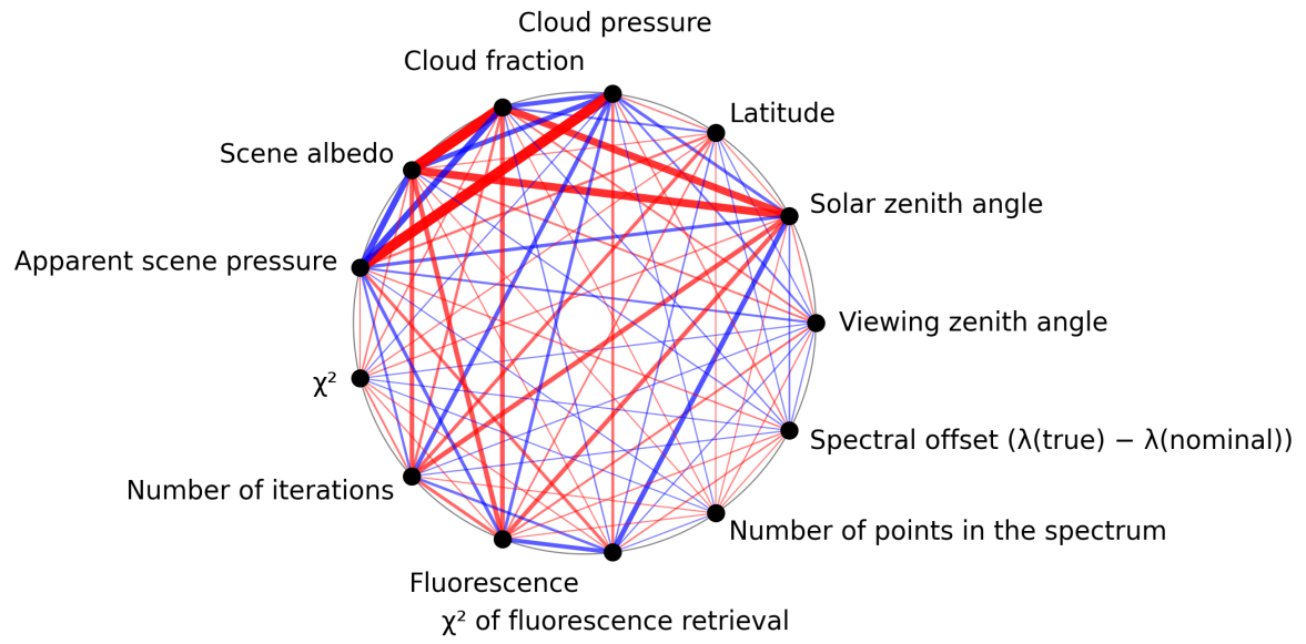
Figure 1: Map of correlation graph for 2025-03-04 to 2025-03-06.
