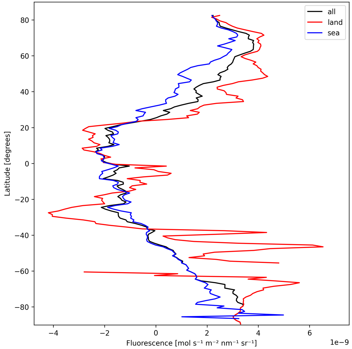
Figure 23: Zonal average of “Fluorescence” for 2025-03-04 to 2025-03-06.
