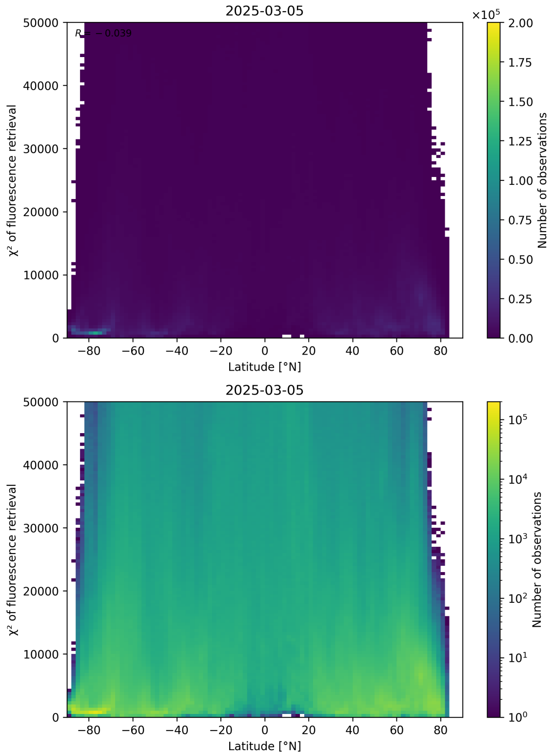
Figure 89: Scatter density plot of “Latitude” against “ \chi^2 of fluorescence retrieval” for 2025-03-04 to 2025-03-06.
