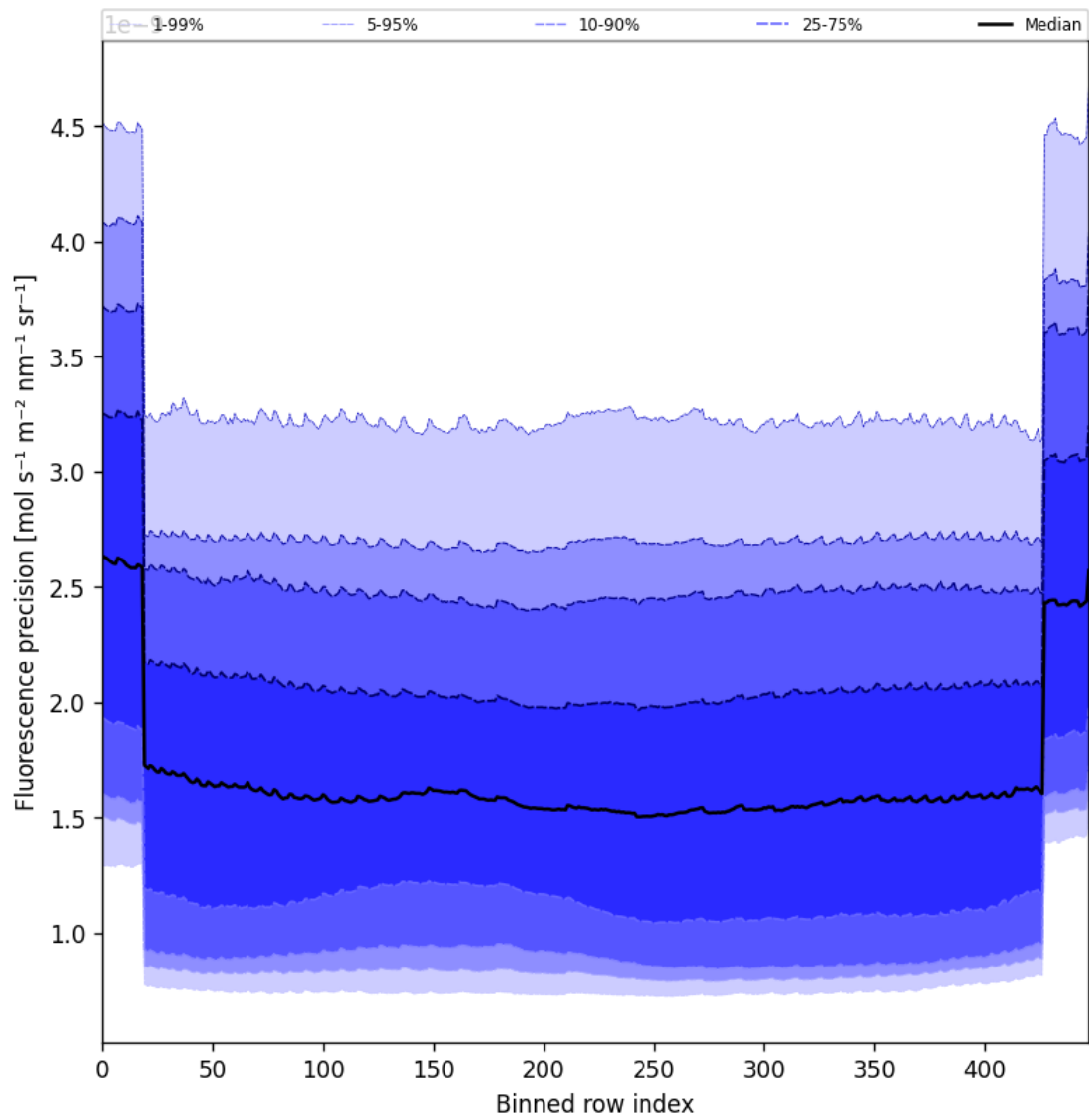
Figure 58: Along track statistics of “Fluorescence precision” for 2025-03-04 to 2025-03-06
