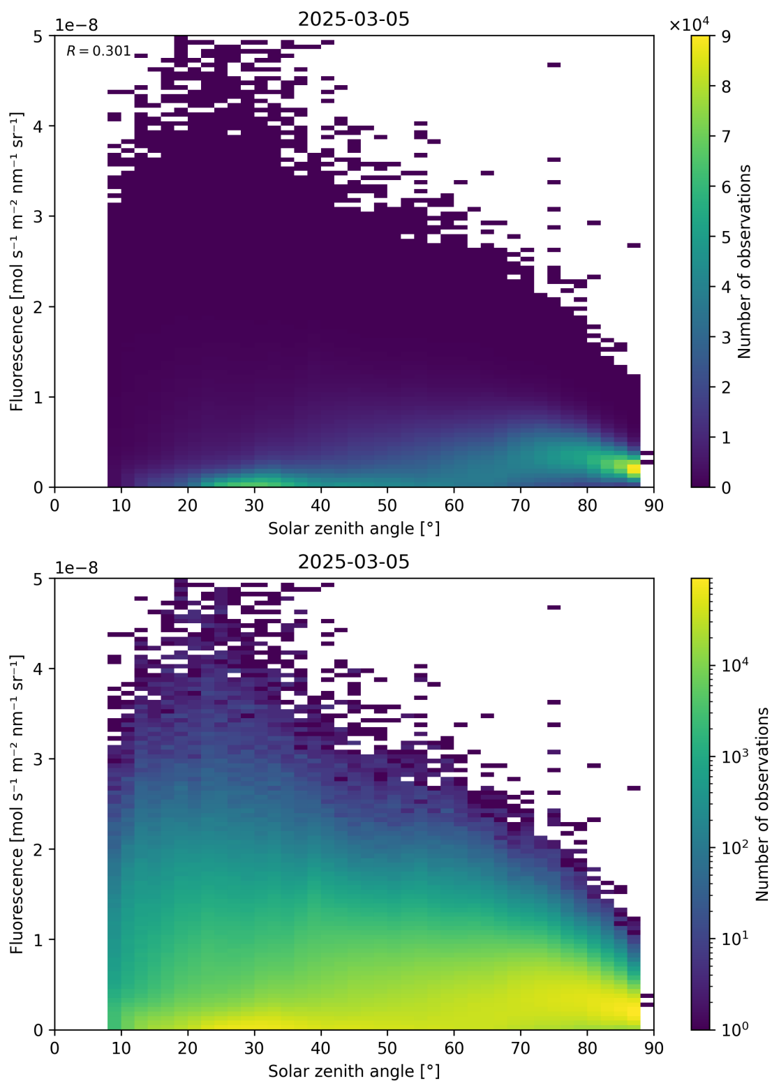
Figure 112: Scatter density plot of “Solar zenith angle” against “Fluorescence” for 2025-03-04 to 2025-03-06.
