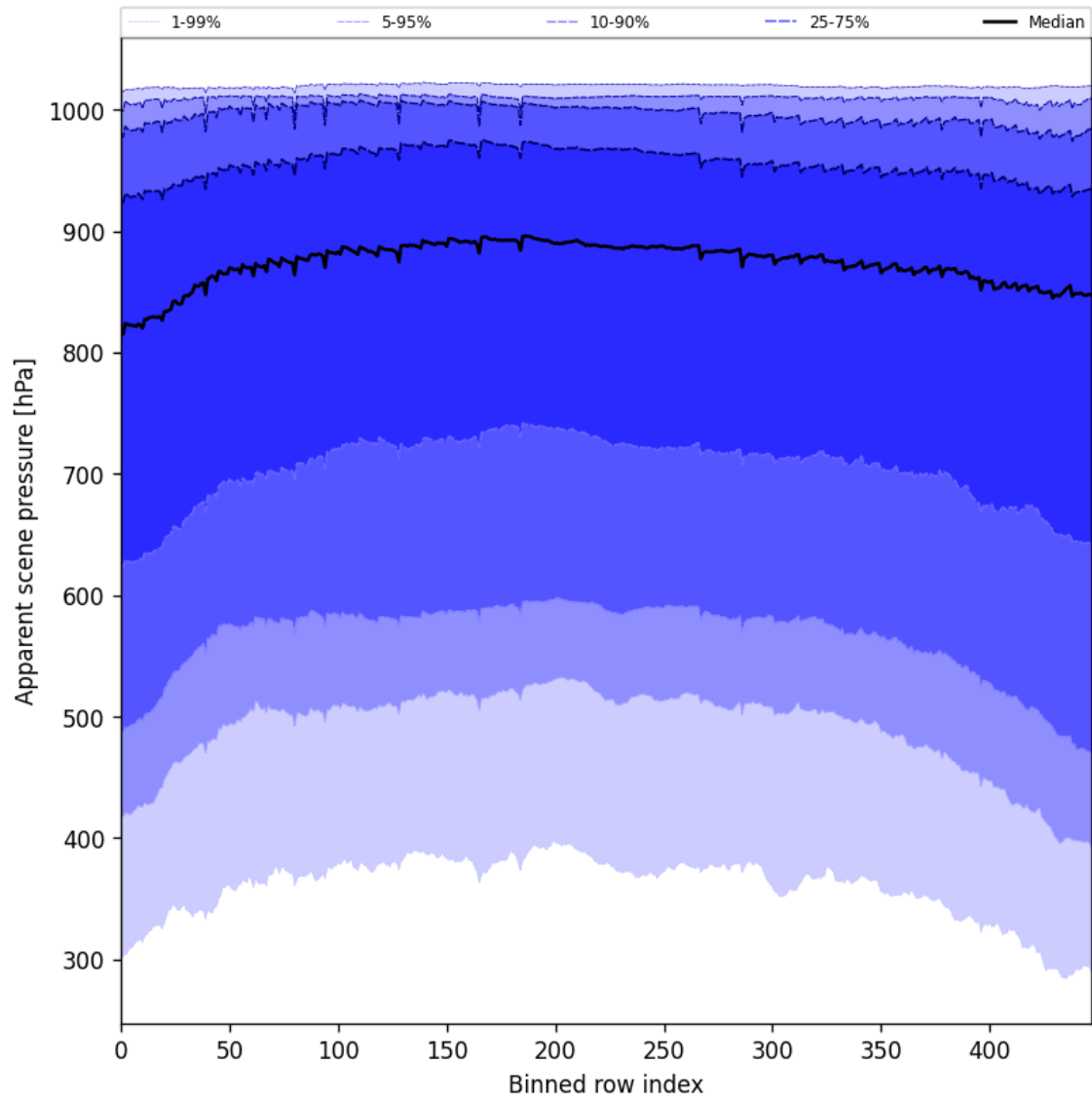
Figure 53: Along track statistics of “Apparent scene pressure” for 2025-03-04 to 2025-03-06
