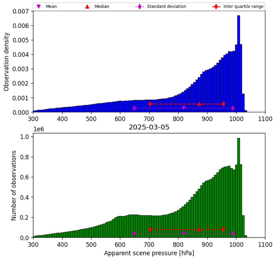
Figure 36: Histogram of “Apparent scene pressure” for 2025-03-04 to 2025-03-06
