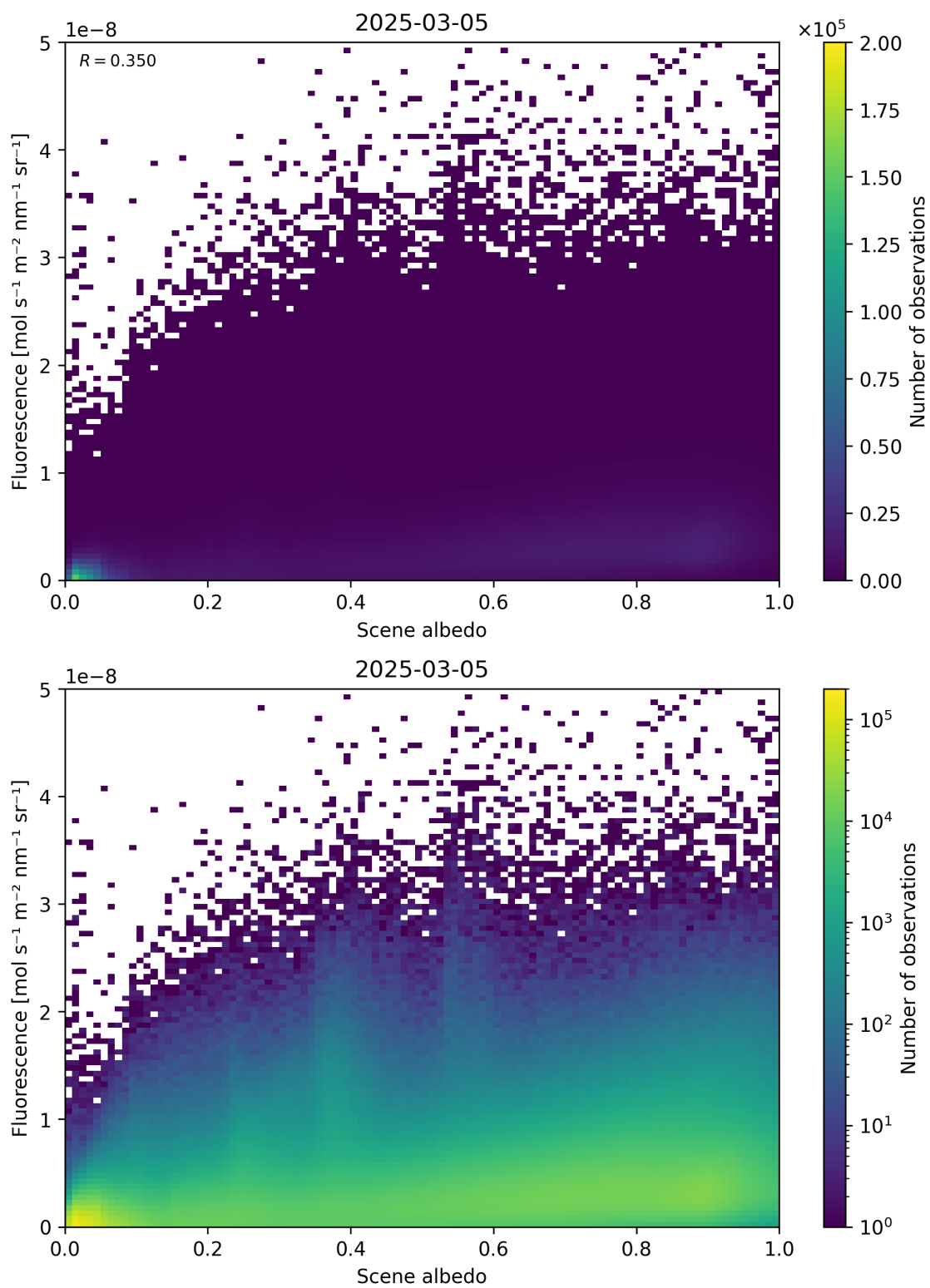
Figure 104: Scatter density plot of “Scene albedo” against “Fluorescence” for 2025-03-04 to 2025-03-06.
