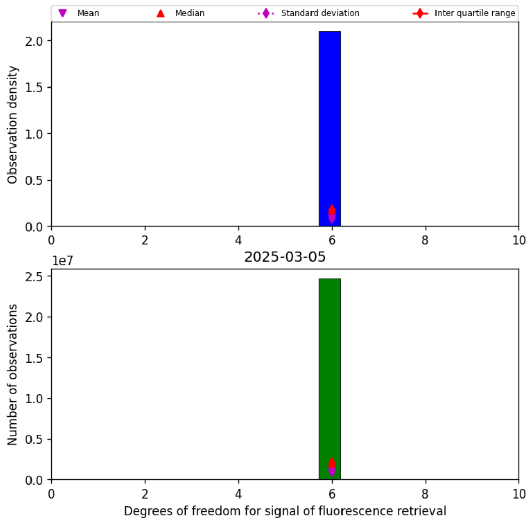
Figure 43: Histogram of “Degrees of freedom for signal of fluorescence retrieval” for 2025-03-04 to 2025-03-06
