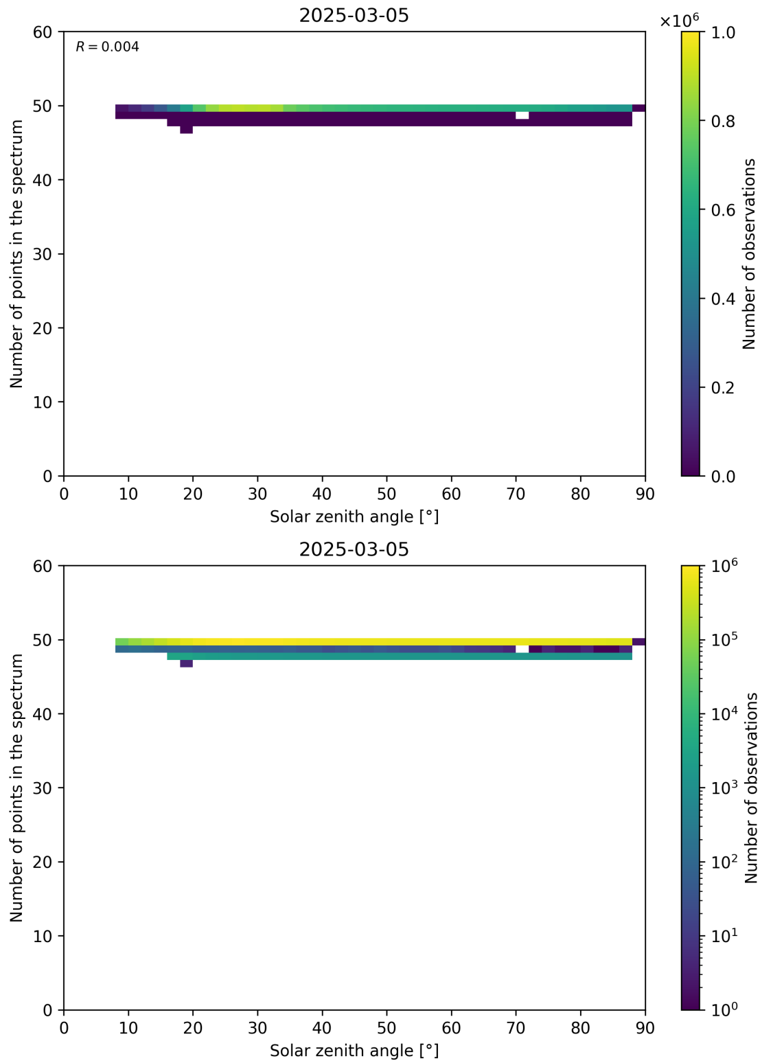
Figure 115: Scatter density plot of “Solar zenith angle” against “Number of points in the spectrum” for 2025-03-04 to 2025-03-06.
