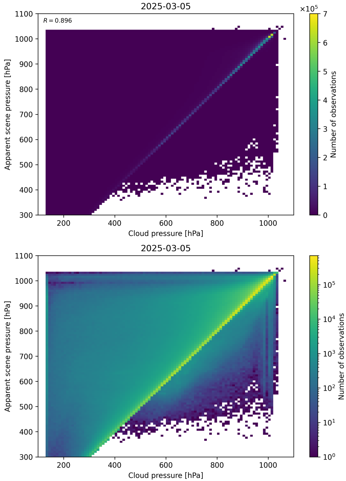
Figure 77: Scatter density plot of “Cloud pressure” against “Apparent scene pressure” for 2025-03-04 to 2025-03-06.
