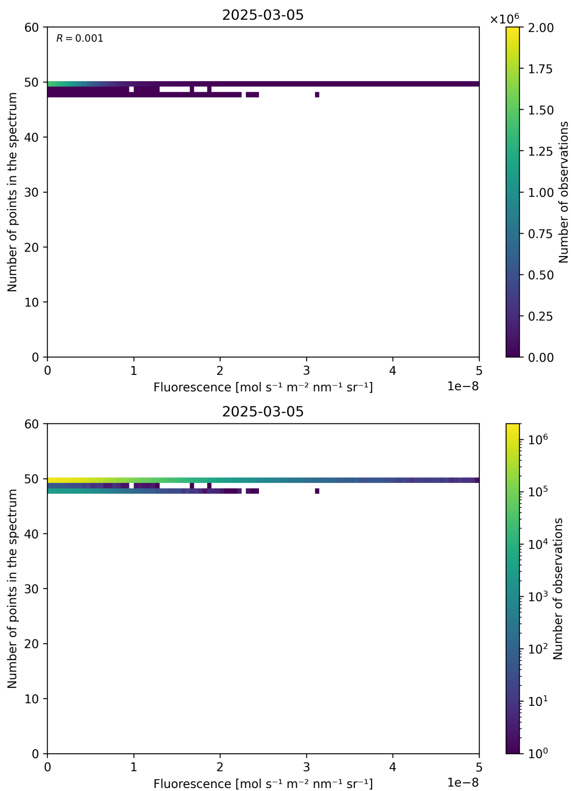
Figure 86: Scatter density plot of “Fluorescence” against “Number of points in the spectrum” for 2025-03-04 to 2025-03-06.
