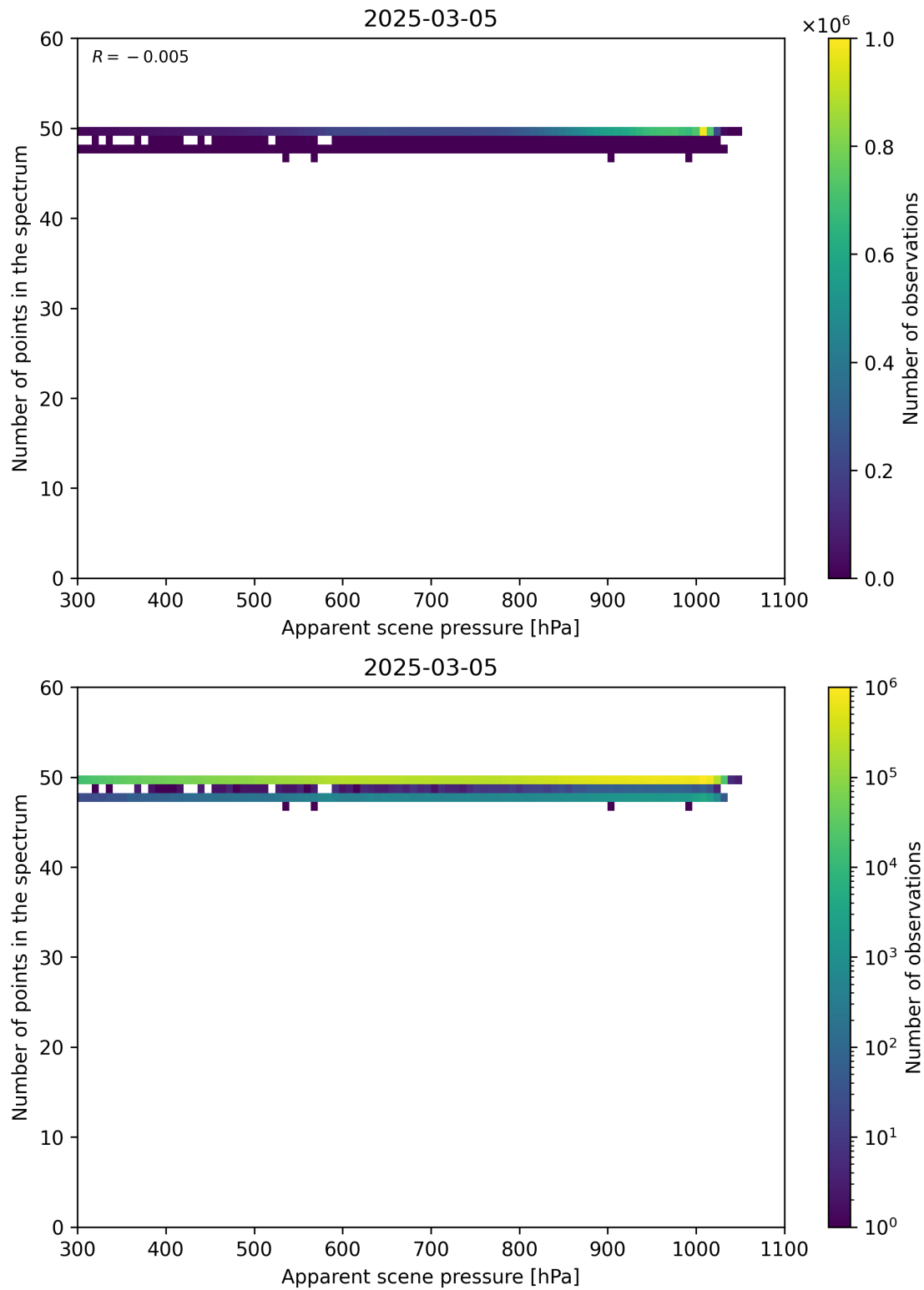
Figure 66: Scatter density plot of “Apparent scene pressure” against “Number of points in the spectrum” for 2025-03-04 to 2025-03-06.
