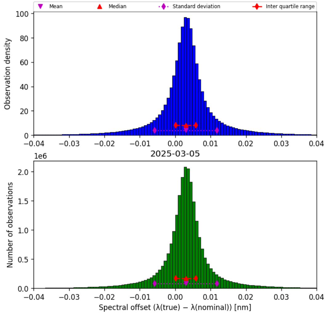
Figure 45: Histogram of “Spectral offset ( \lambda_{\text{true}} - \lambda_{\text{nominal}} )” for 2025-03-04 to 2025-03-06
