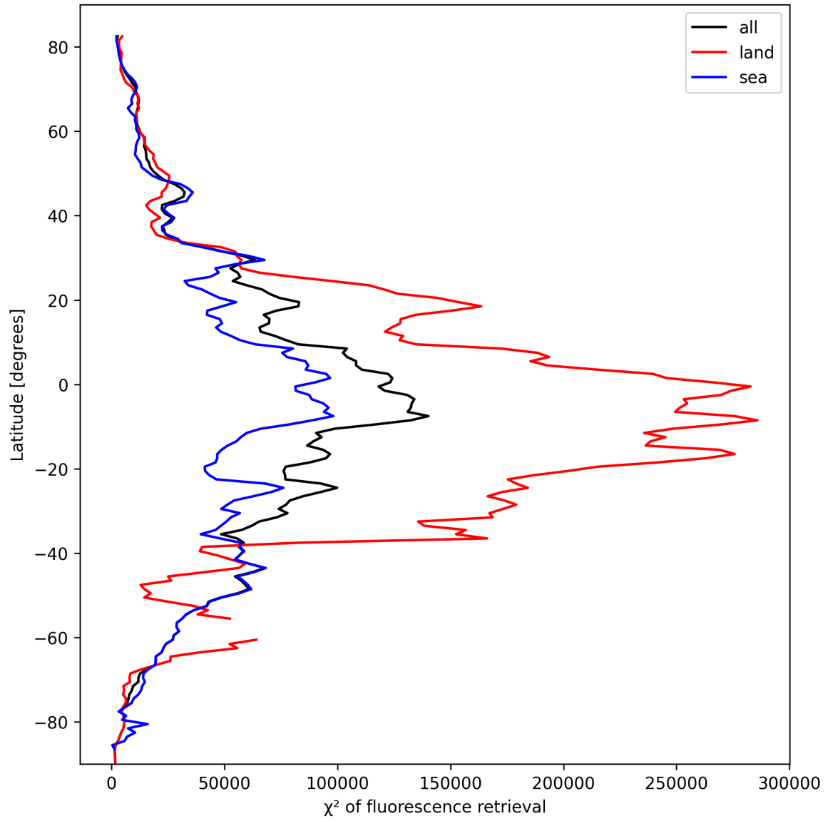
Figure 25: Zonal average of “ \chi^2 of fluorescence retrieval” for 2025-03-04 to 2025-03-06.
