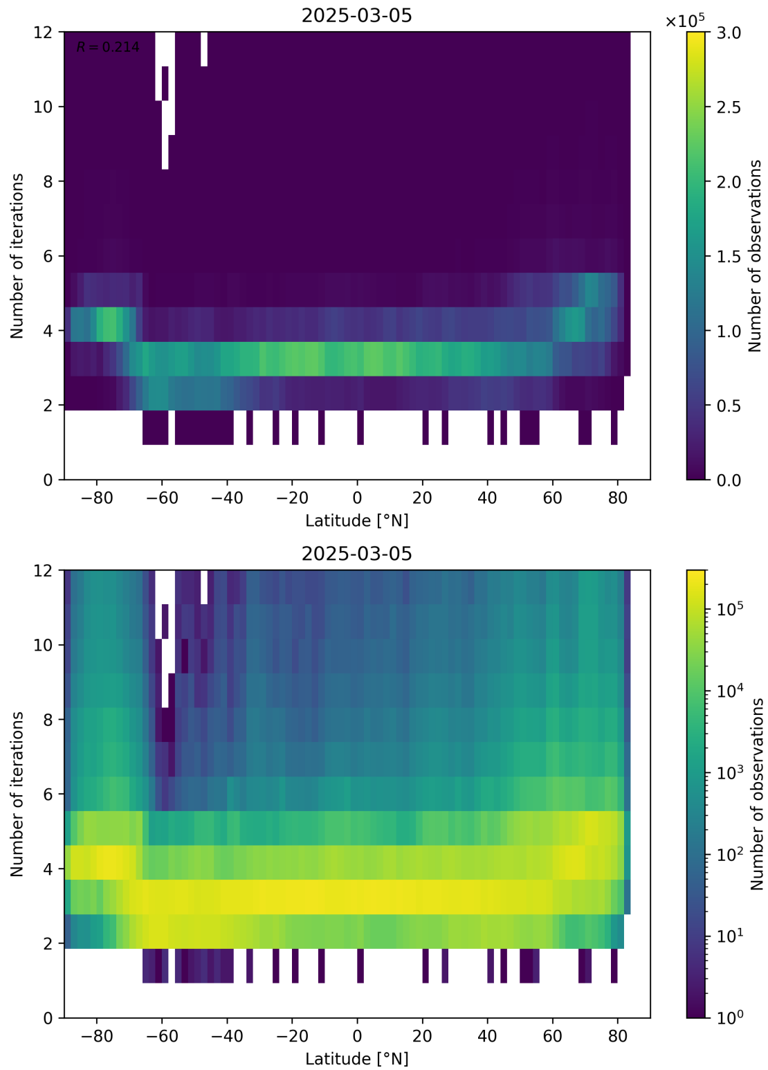
Figure 93: Scatter density plot of “Latitude” against “Number of iterations” for 2025-03-04 to 2025-03-06.
