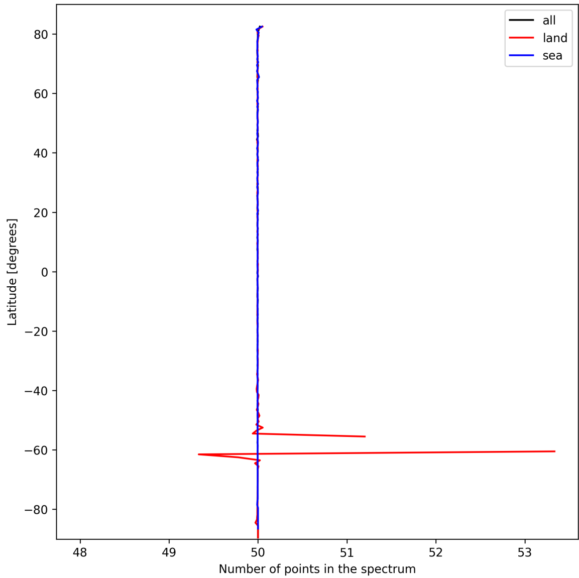
Figure 27: Zonal average of “Number of points in the spectrum” for 2025-03-04 to 2025-03-06.
