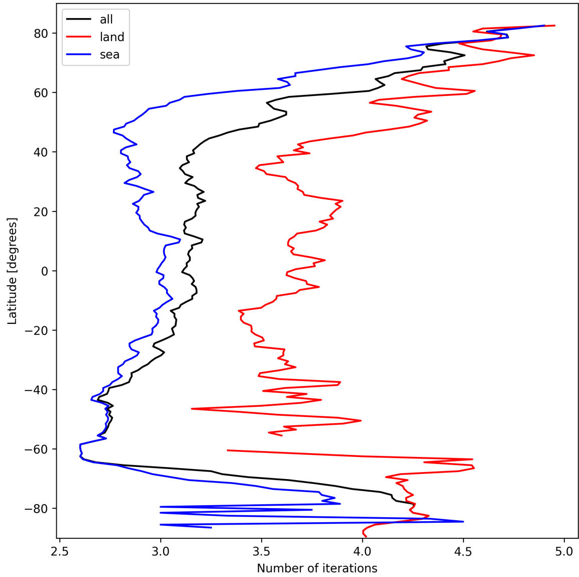
Figure 22: Zonal average of “Number of iterations” for 2025-03-04 to 2025-03-06.
