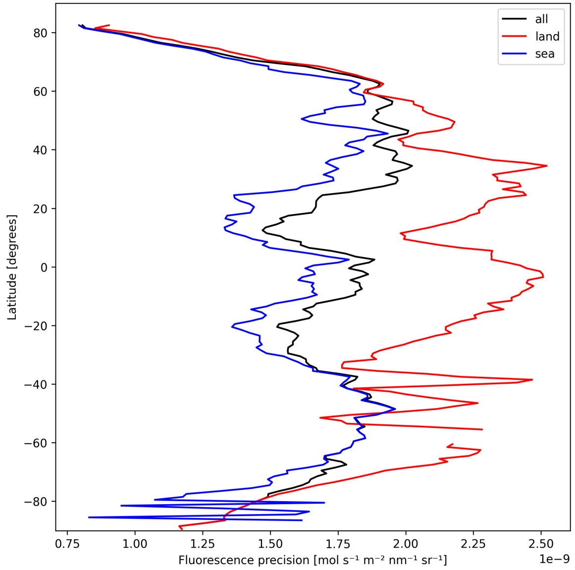
Figure 24: Zonal average of “Fluorescence precision” for 2025-03-04 to 2025-03-06.
