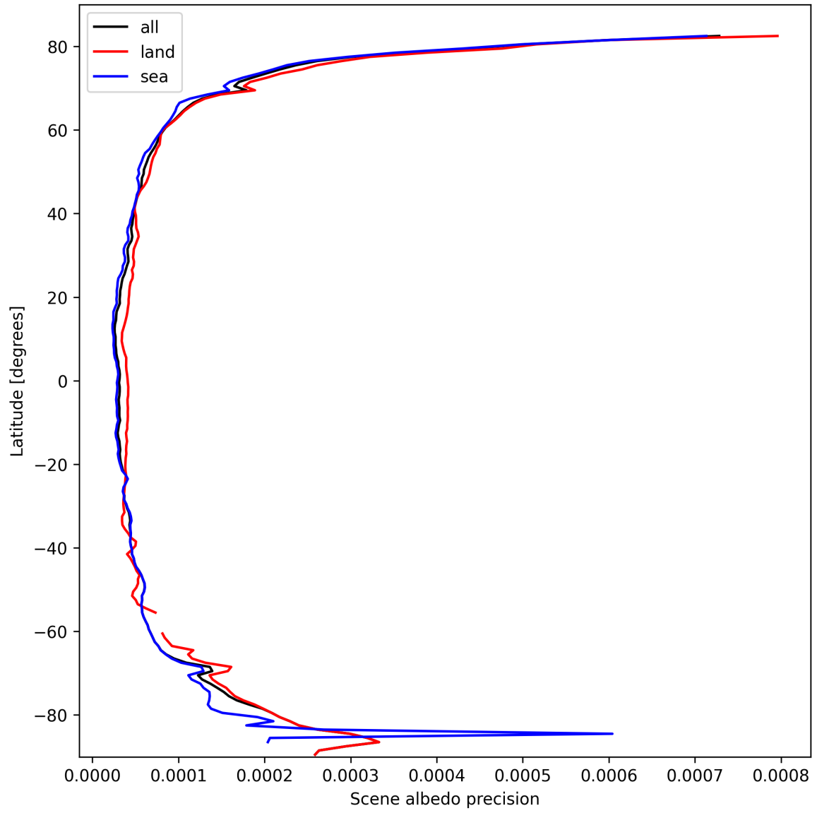
Figure 18: Zonal average of “Scene albedo precision” for 2025-03-04 to 2025-03-06.
