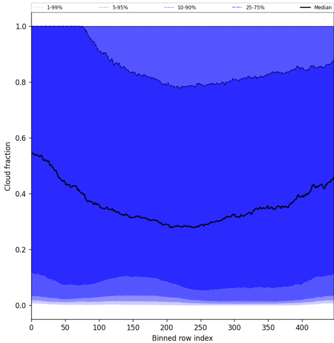
Figure 49: Along track statistics of “Cloud fraction” for 2025-03-04 to 2025-03-06
