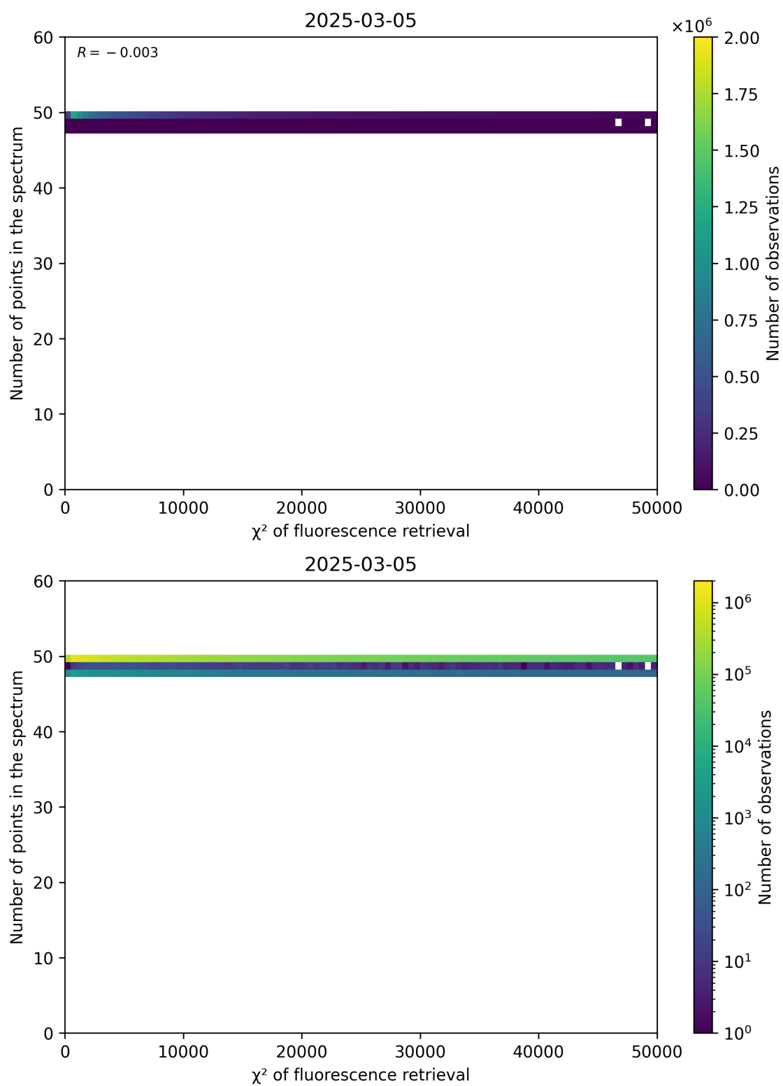
Figure 68: Scatter density plot of " \chi^2 of fluorescence retrieval" against "Number of points in the spectrum" for 2025-03-04 to 2025-03-06.
