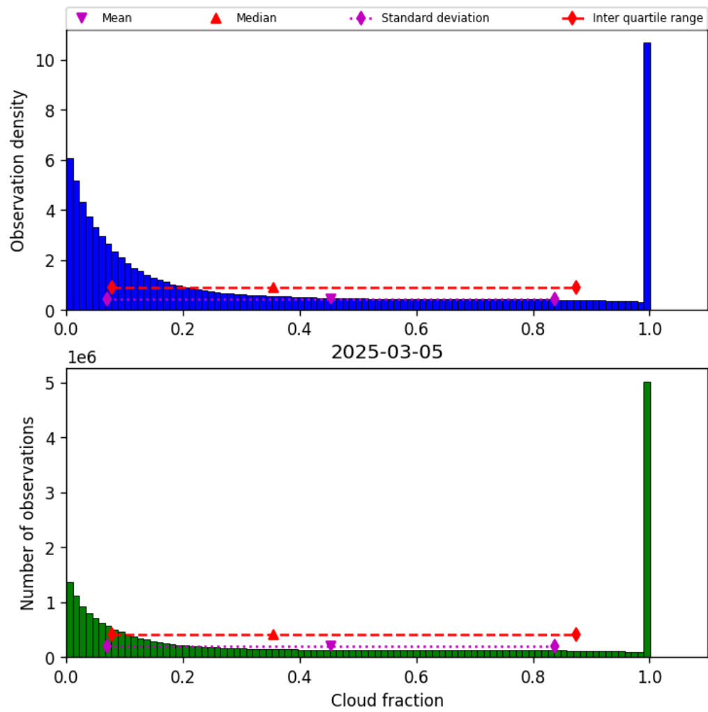
Figure 32: Histogram of “Cloud fraction” for 2025-03-04 to 2025-03-06
