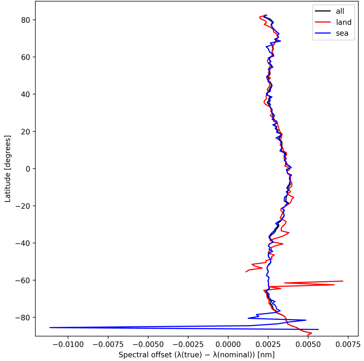
Figure 28: Zonal average of “Spectral offset ( \lambda_{\text{true}} - \lambda_{\text{nominal}} )” for 2025-03-04 to 2025-03-06.
