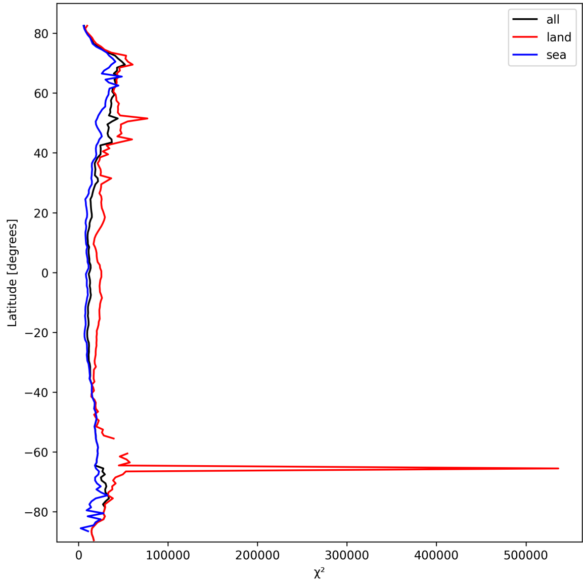
Figure 21: Zonal average of “ \chi^2 ” for 2025-03-04 to 2025-03-06.
