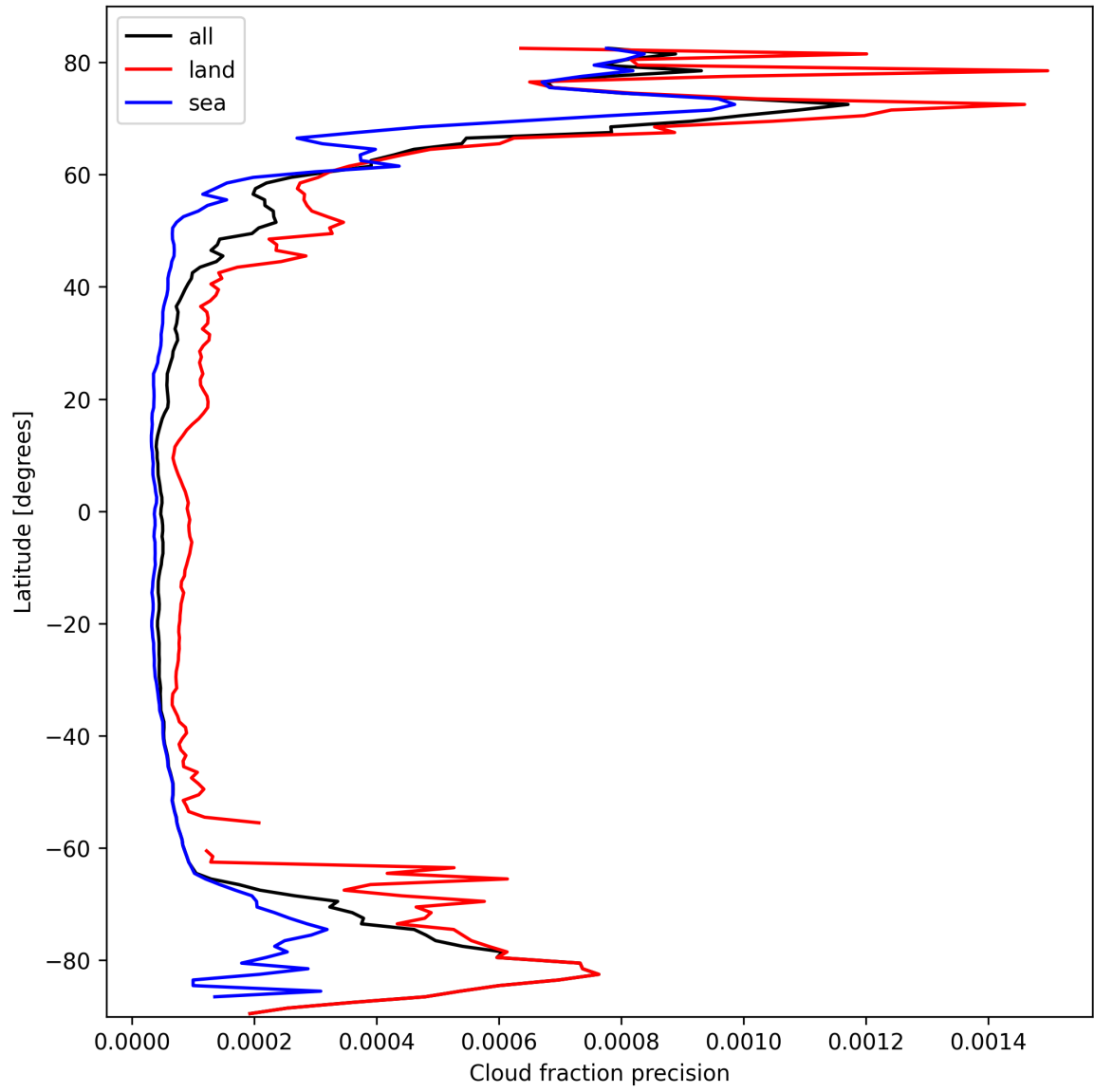
Figure 16: Zonal average of “Cloud fraction precision” for 2025-03-04 to 2025-03-06.
