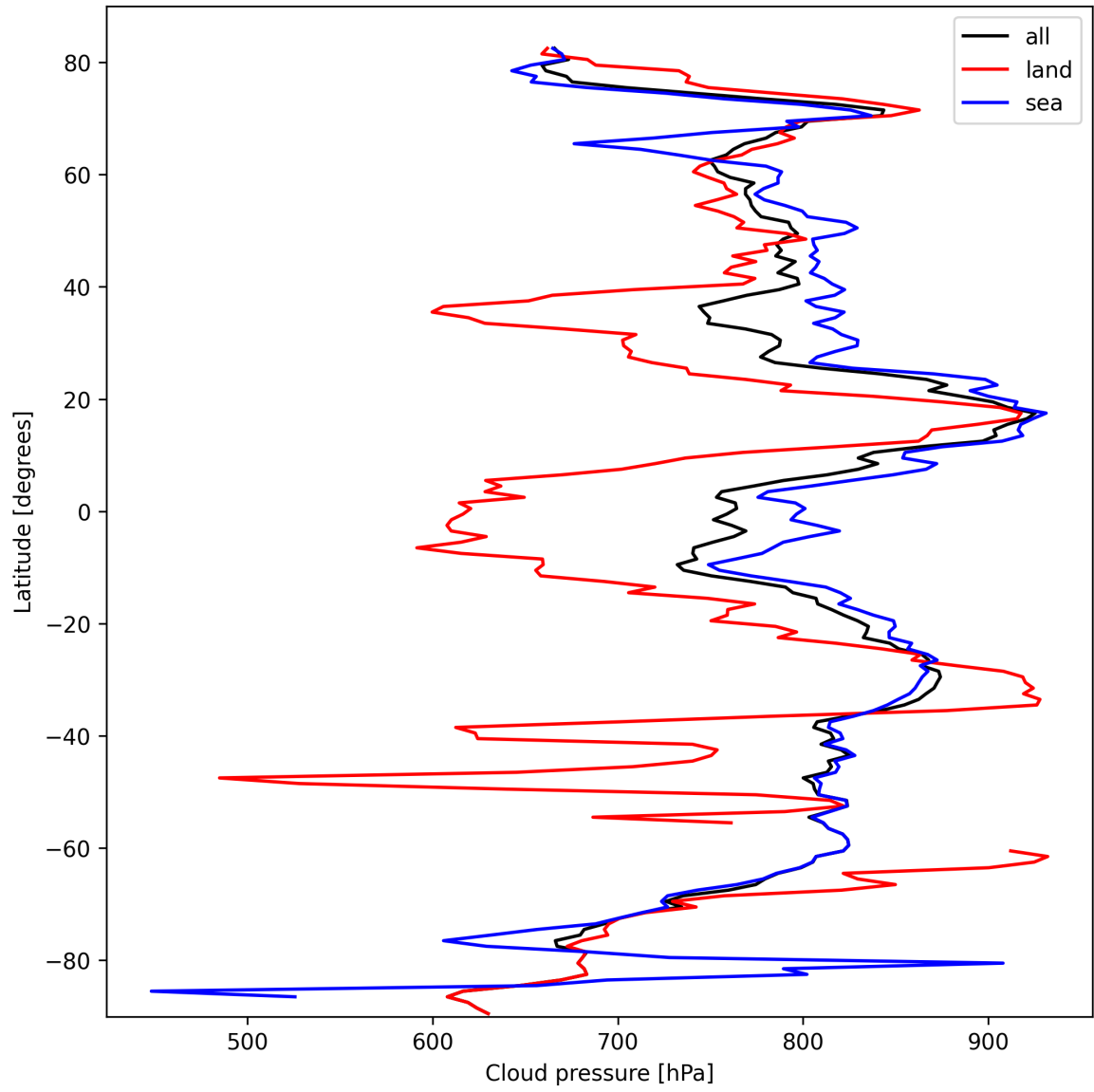
Figure 13: Zonal average of “Cloud pressure” for 2025-03-04 to 2025-03-06.
