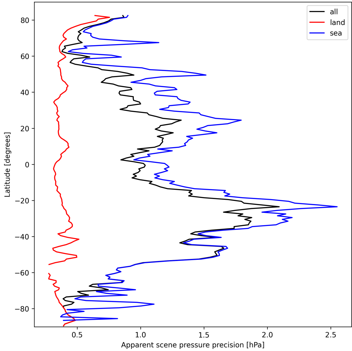
Figure 20: Zonal average of “Apparent scene pressure precision” for 2025-03-04 to 2025-03-06.
