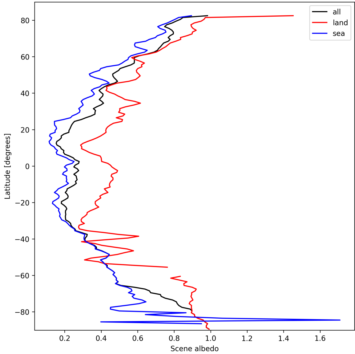
Figure 17: Zonal average of “Scene albedo” for 2025-03-04 to 2025-03-06.
