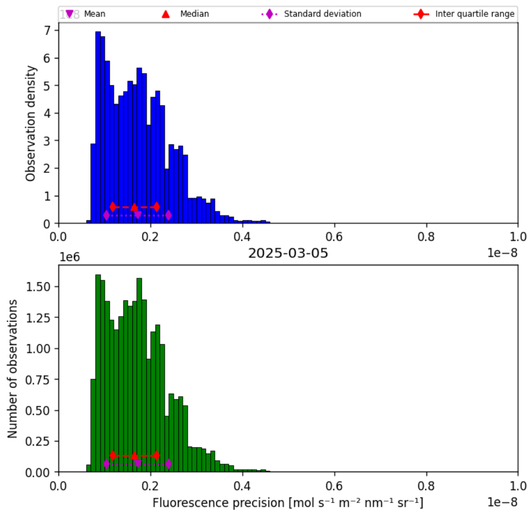
Figure 41: Histogram of “Fluorescence precision” for 2025-03-04 to 2025-03-06
