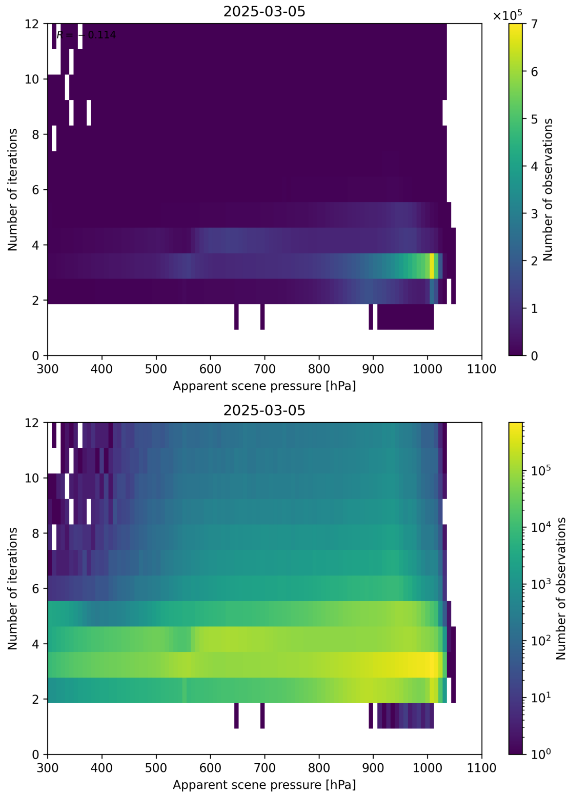
Figure 65: Scatter density plot of “Apparent scene pressure” against “Number of iterations” for 2025-03-04 to 2025-03-06.
