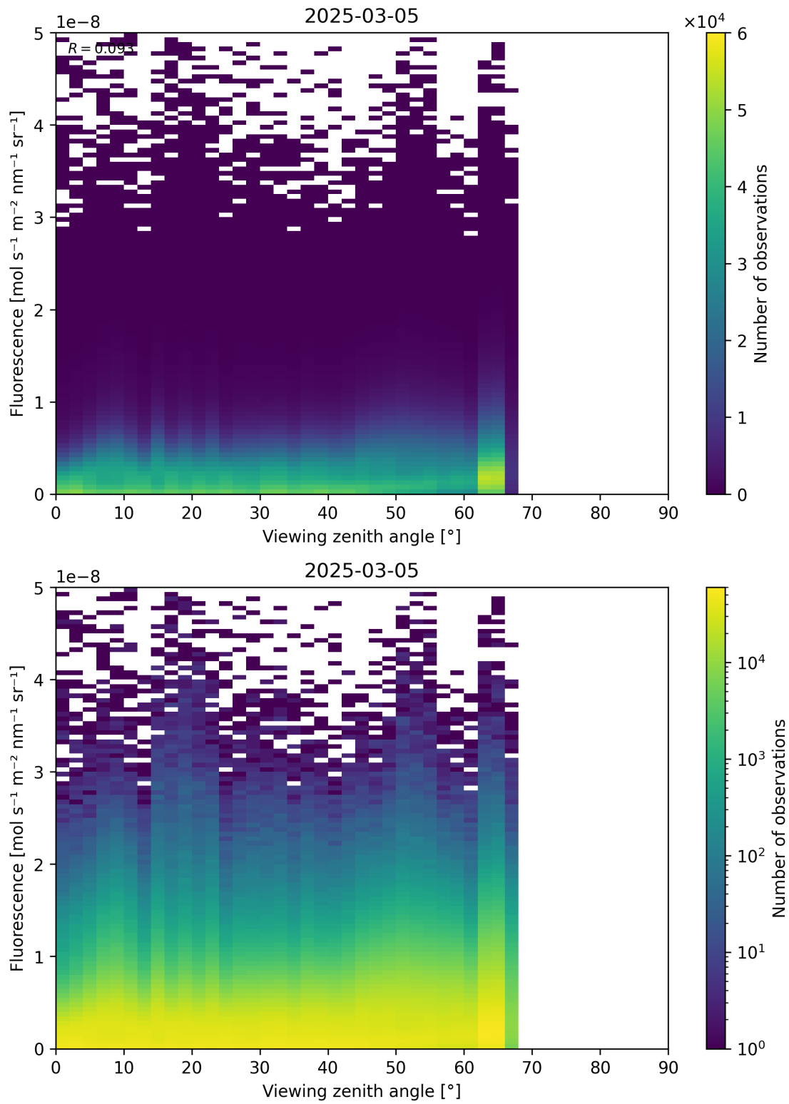
Figure 122: Scatter density plot of “Viewing zenith angle” against “Fluorescence” for 2025-03-04 to 2025-03-06.
