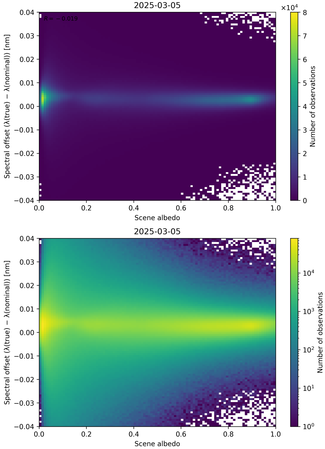
Figure 107: Scatter density plot of “Scene albedo” against “Spectral offset ( \lambda_{\text{true}} - \lambda_{\text{nominal}} )” for 2025-03-04 to 2025-03-06.
