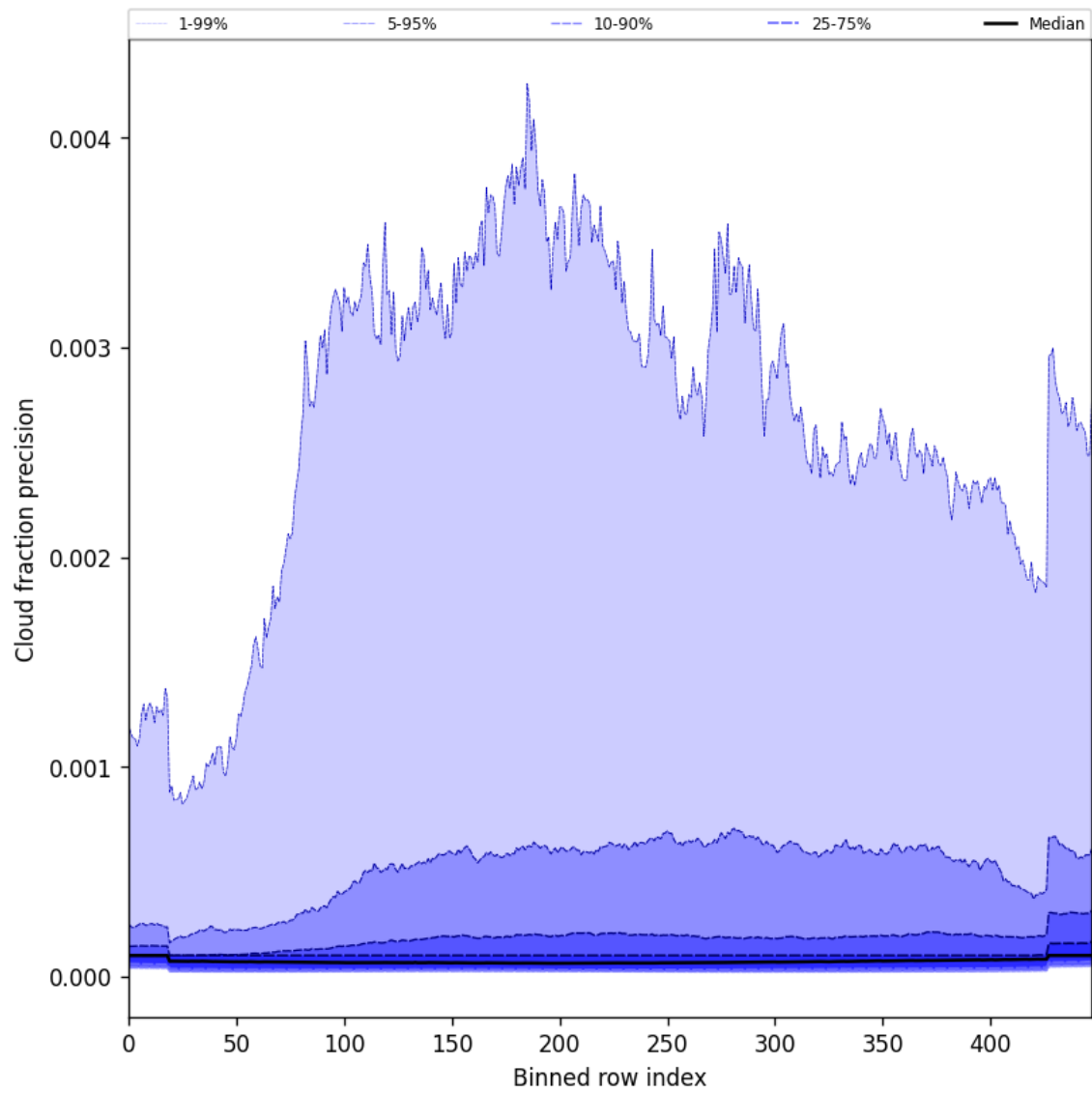
Figure 50: Along track statistics of “Cloud fraction precision” for 2025-03-04 to 2025-03-06
