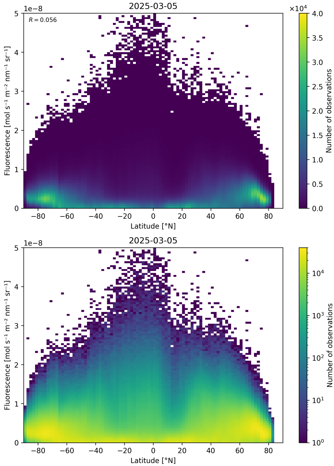
Figure 92: Scatter density plot of “Latitude” against “Fluorescence” for 2025-03-04 to 2025-03-06.
