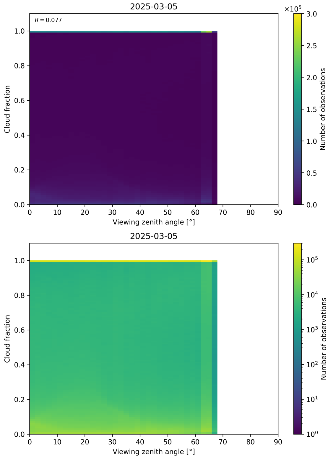
Figure 120: Scatter density plot of “Viewing zenith angle” against “Cloud fraction” for 2025-03-04 to 2025-03-06.
