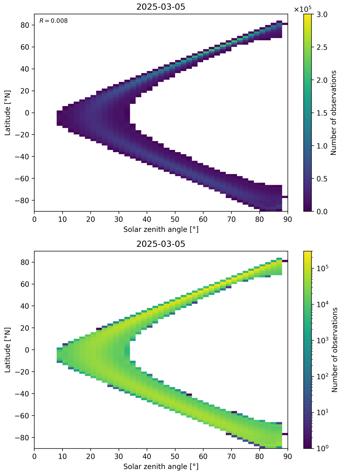
Figure 113: Scatter density plot of “Solar zenith angle” against “Latitude” for 2025-03-04 to 2025-03-06.
