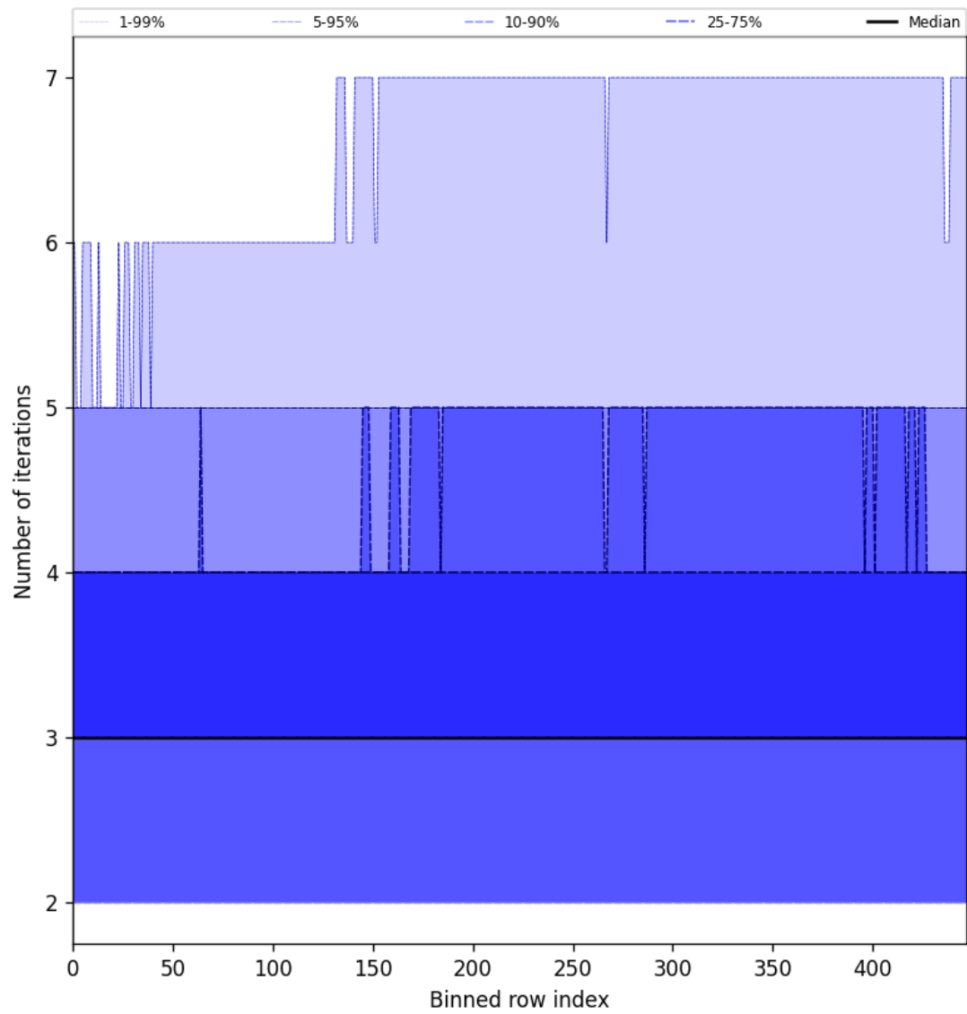
Figure 56: Along track statistics of “Number of iterations” for 2025-03-04 to 2025-03-06
