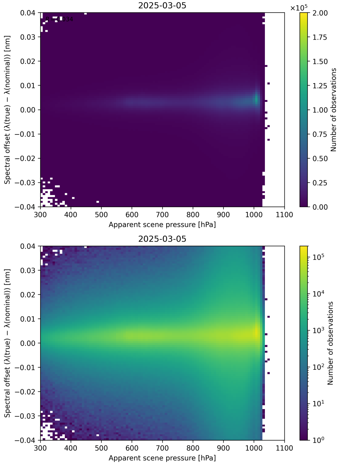
Figure 67: Scatter density plot of “Apparent scene pressure” against “Spectral offset ( \lambda_{\text{true}} - \lambda_{\text{nominal}} )” for 2025-03-04 to 2025-03-06.
