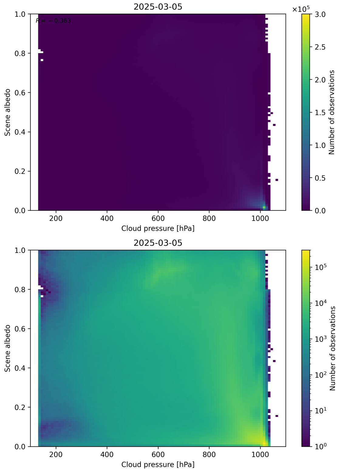
Figure 83: Scatter density plot of “Cloud pressure” against “Scene albedo” for 2025-03-04 to 2025-03-06.
