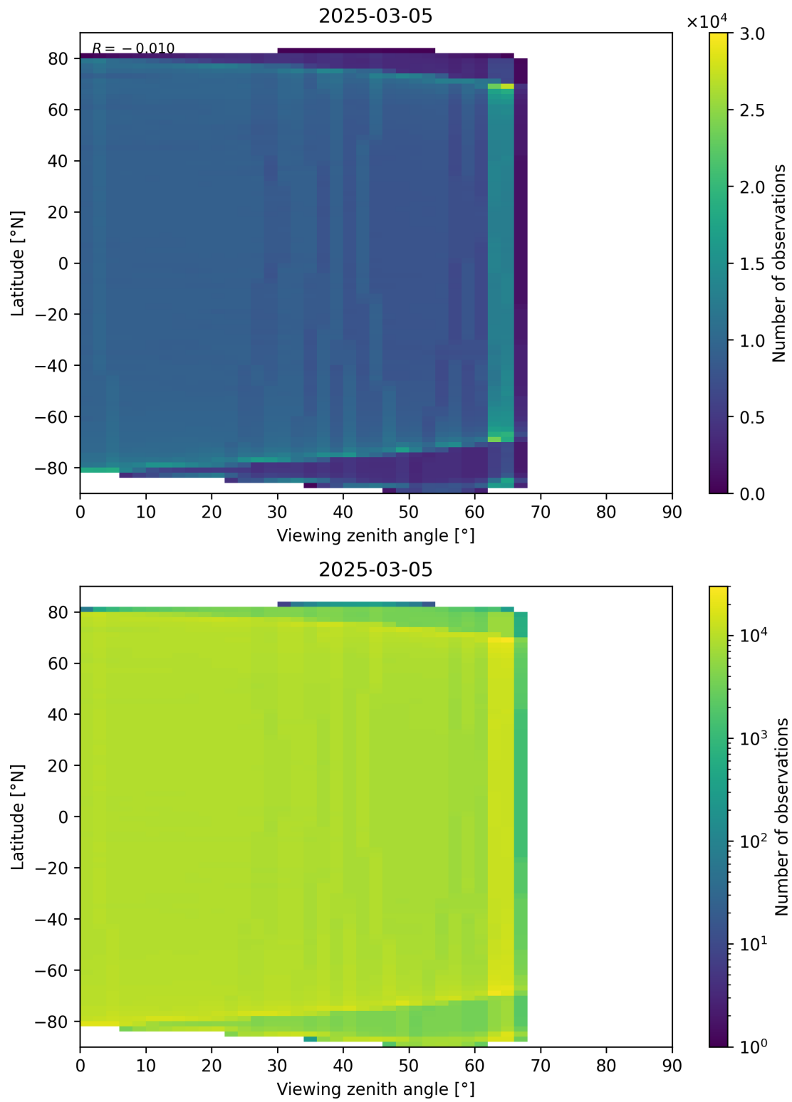
Figure 123: Scatter density plot of “Viewing zenith angle” against “Latitude” for 2025-03-04 to 2025-03-06.
