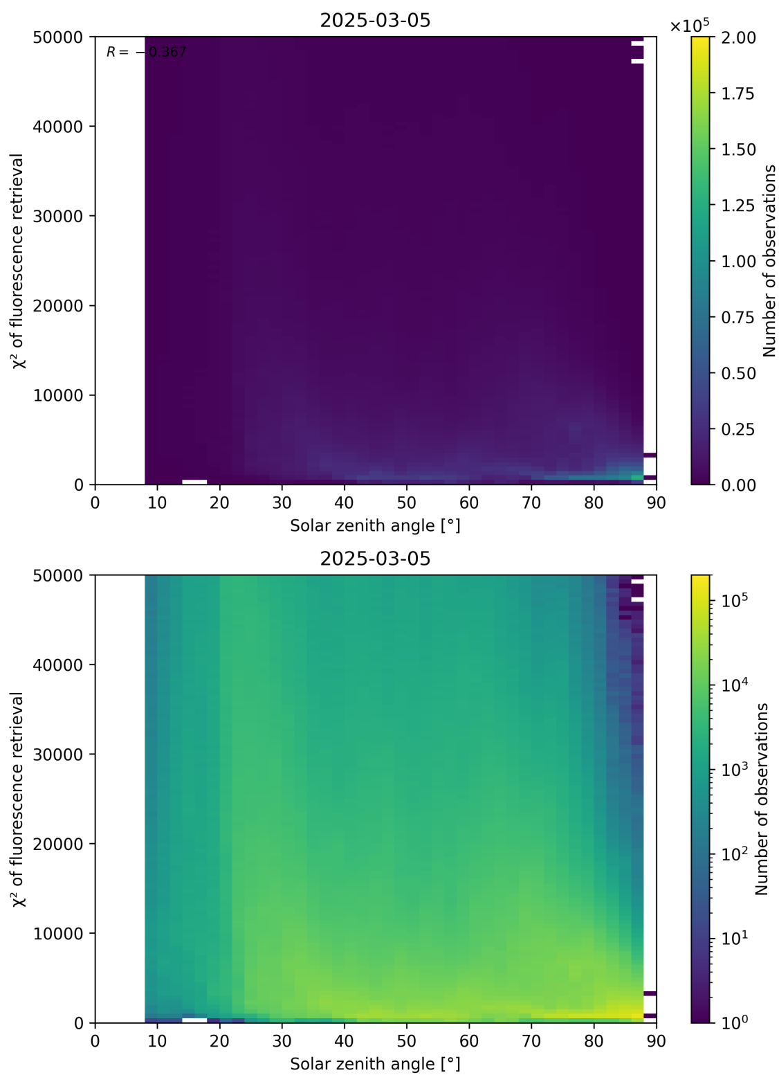
Figure 109: Scatter density plot of “Solar zenith angle” against “ \chi^2 of fluorescence retrieval” for 2025-03-04 to 2025-03-06.
