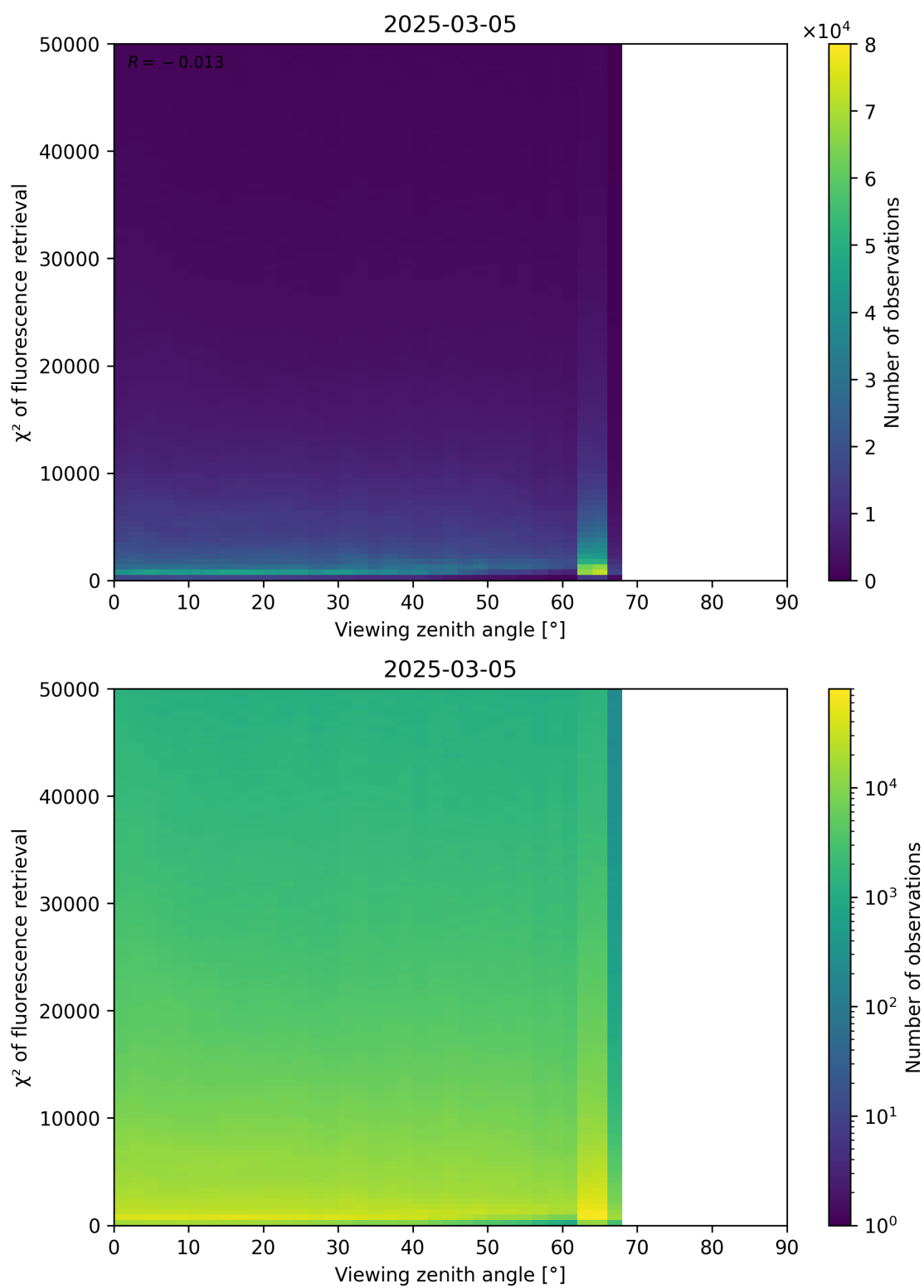
Figure 119: Scatter density plot of “Viewing zenith angle” against “ \chi^2 of fluorescence retrieval” for 2025-03-04 to 2025-03-06.
