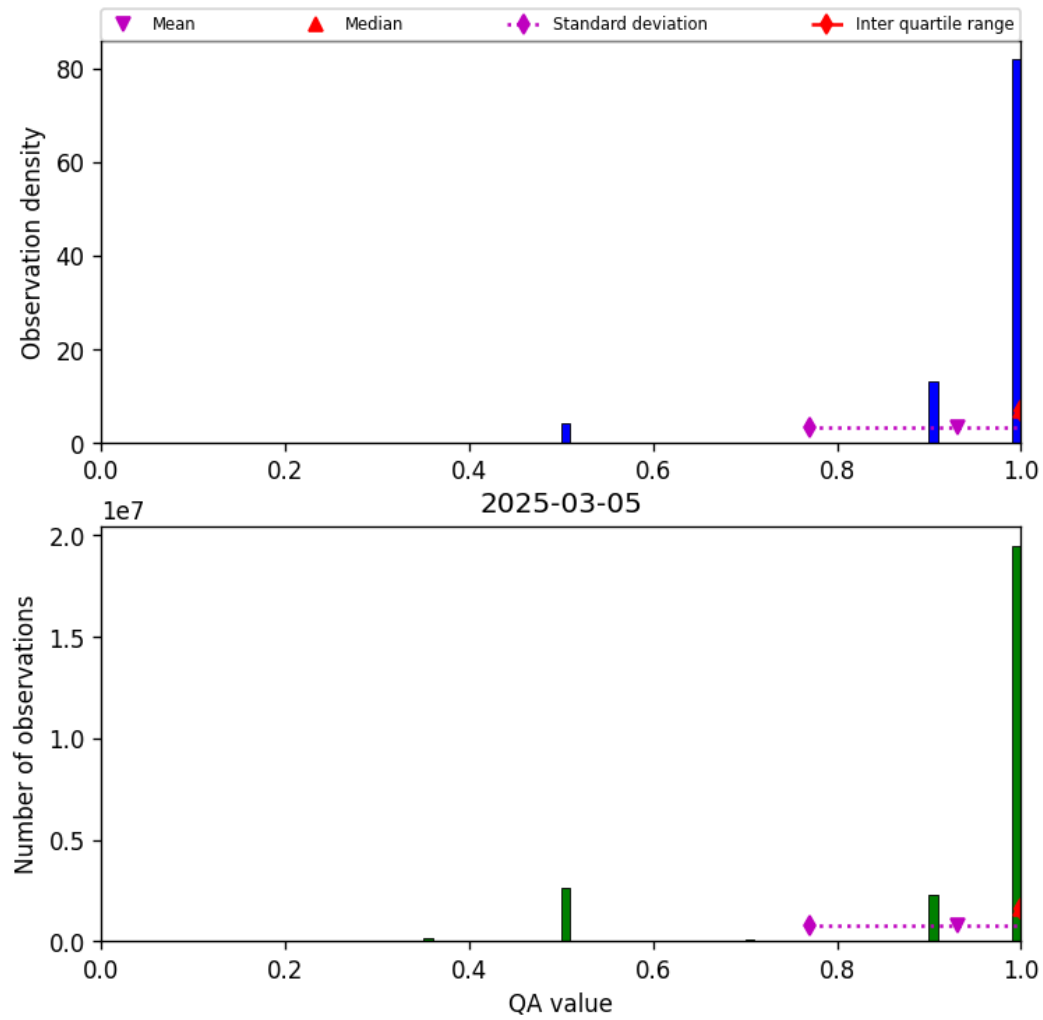
Figure 29: Histogram of “QA value” for 2025-03-04 to 2025-03-06
