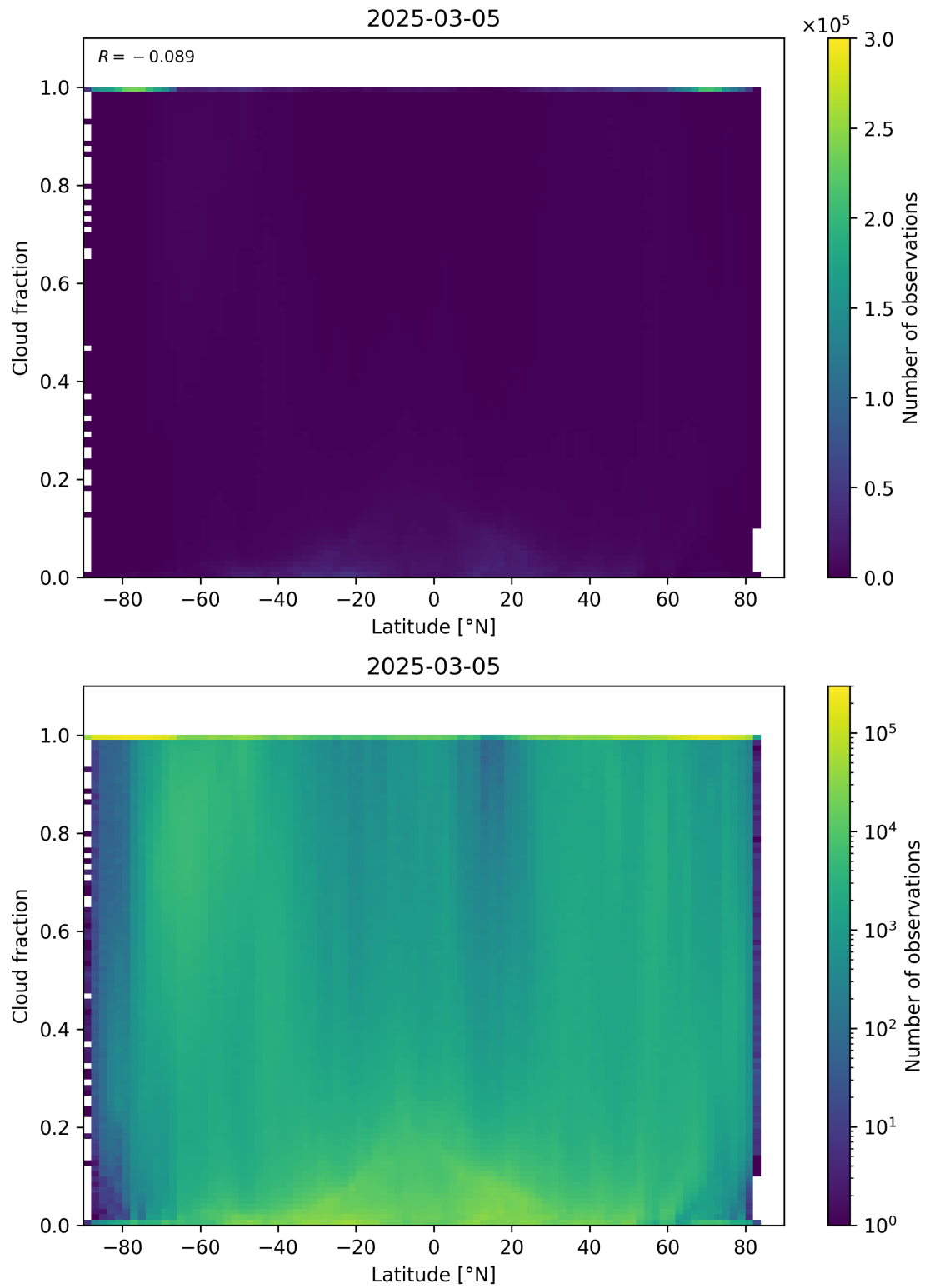
Figure 90: Scatter density plot of “Latitude” against “Cloud fraction” for 2025-03-04 to 2025-03-06.
