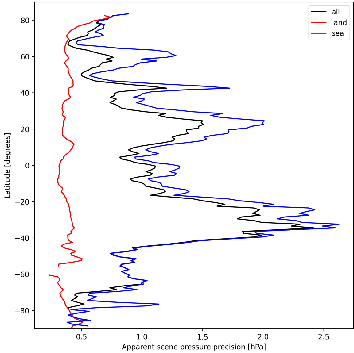
Figure 20: Zonal average of “Apparent scene pressure precision” for 2025-03-07 to 2025-03-08.
