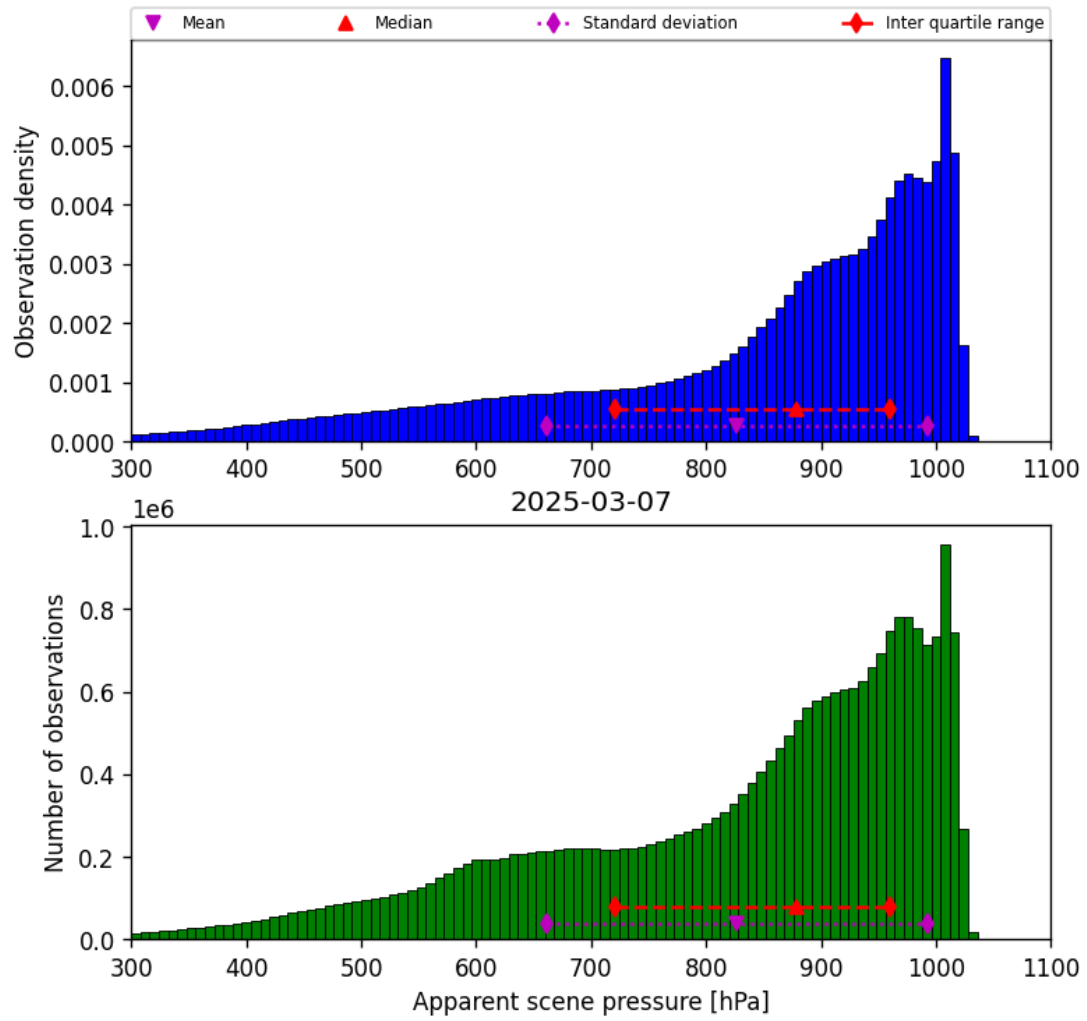
Figure 36: Histogram of “Apparent scene pressure” for 2025-03-07 to 2025-03-08
