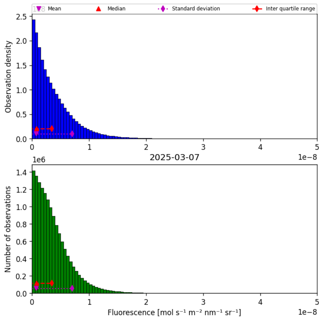
Figure 40: Histogram of “Fluorescence” for 2025-03-07 to 2025-03-08
