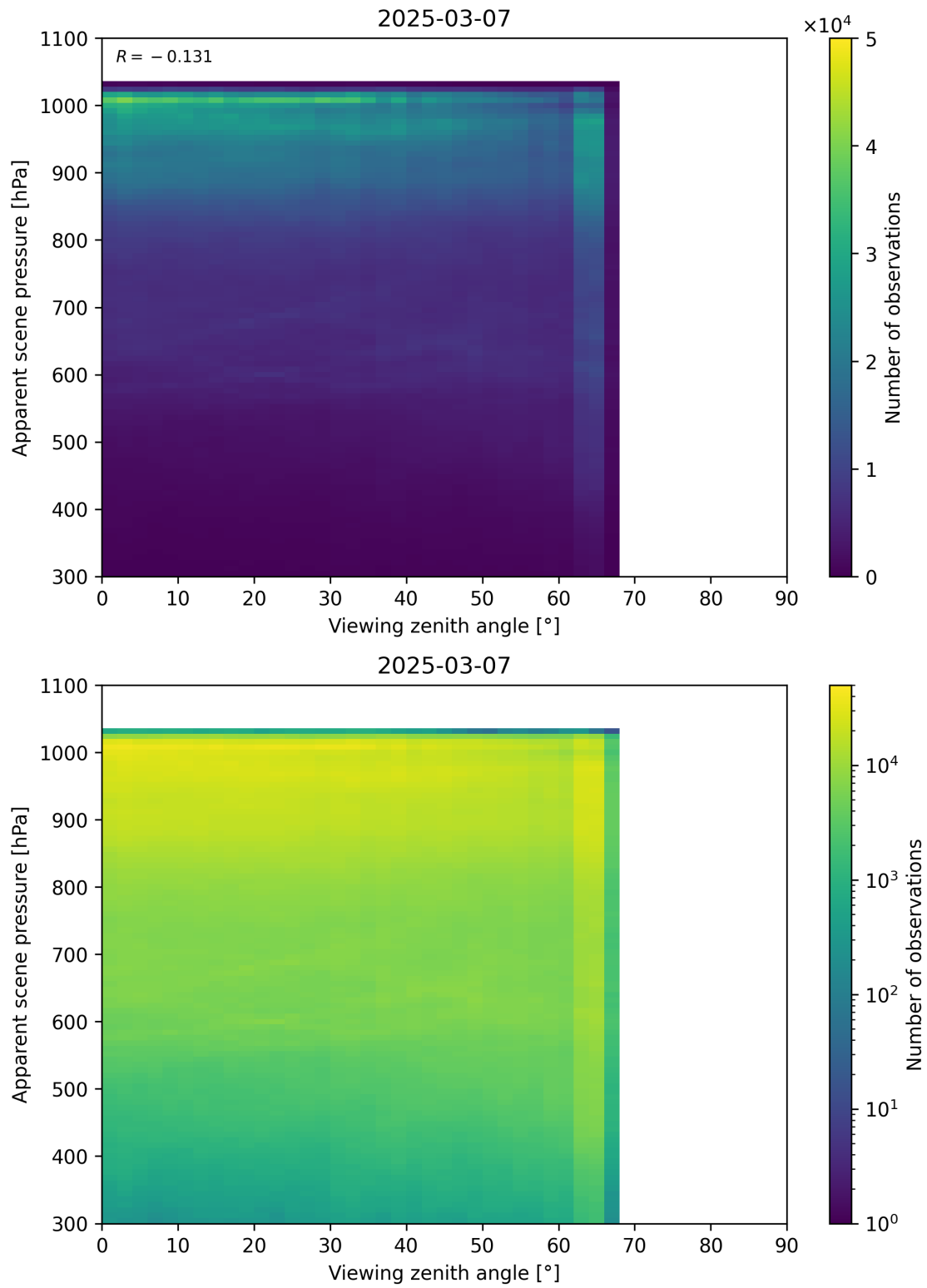
Figure 118: Scatter density plot of “Viewing zenith angle” against “Apparent scene pressure” for 2025-03-07 to 2025-03-08.
