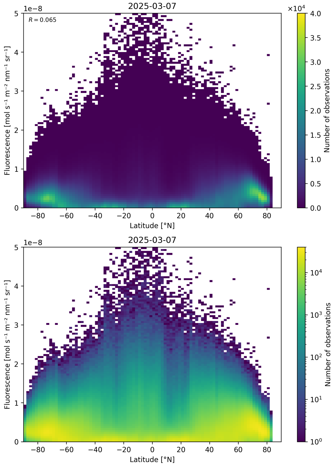
Figure 92: Scatter density plot of “Latitude” against “Fluorescence” for 2025-03-07 to 2025-03-08.
