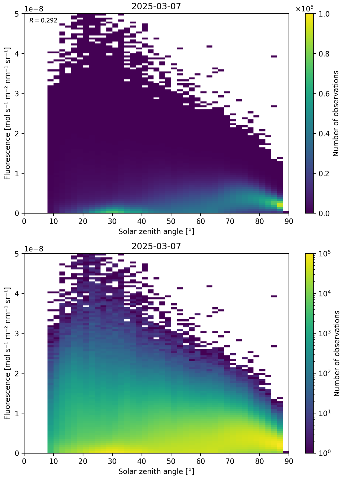
Figure 112: Scatter density plot of “Solar zenith angle” against “Fluorescence” for 2025-03-07 to 2025-03-08.
