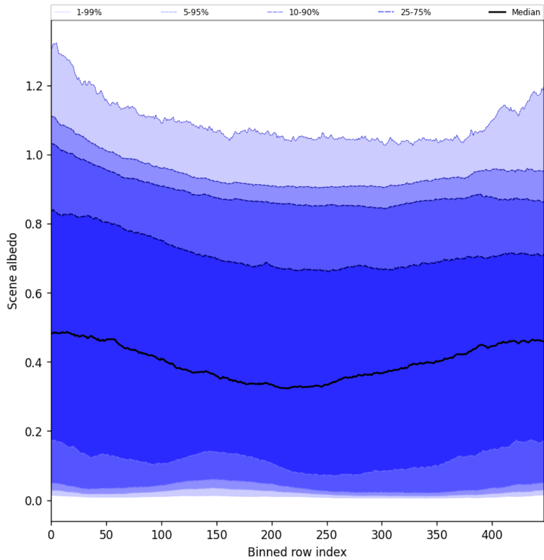
Figure 51: Along track statistics of “Scene albedo” for 2025-03-07 to 2025-03-08
