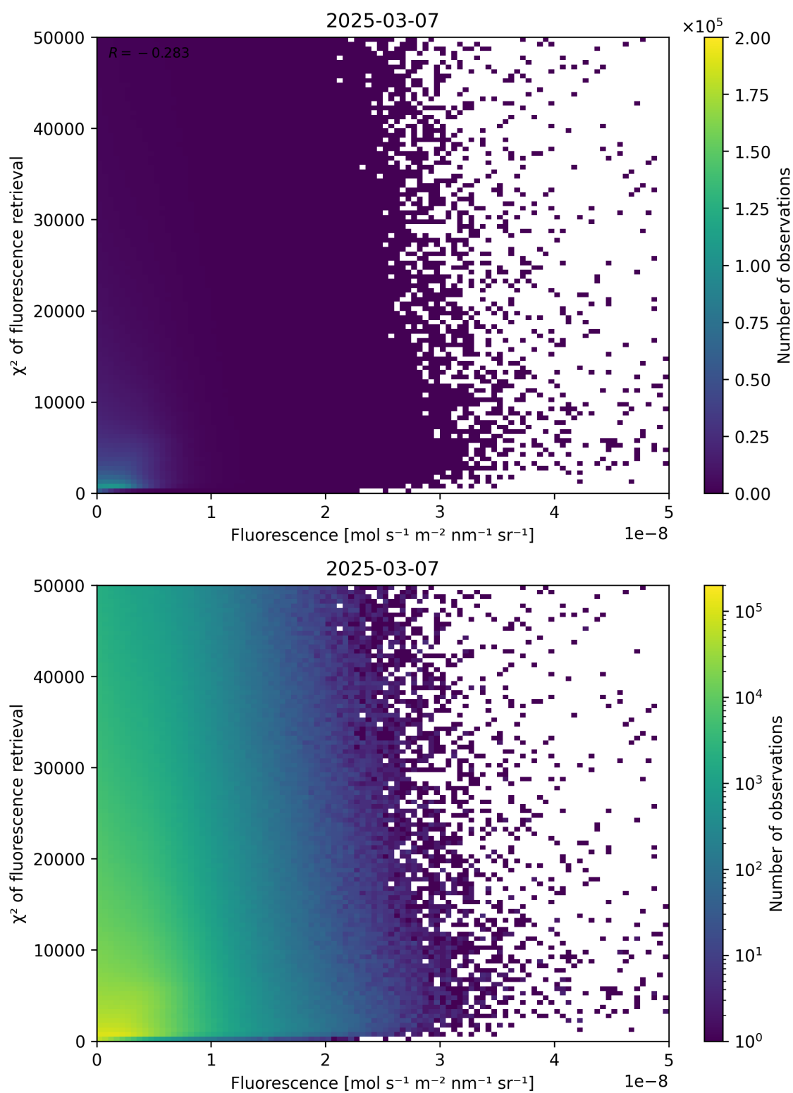
Figure 85: Scatter density plot of “Fluorescence” against “ \chi^2 of fluorescence retrieval” for 2025-03-07 to 2025-03-08.
