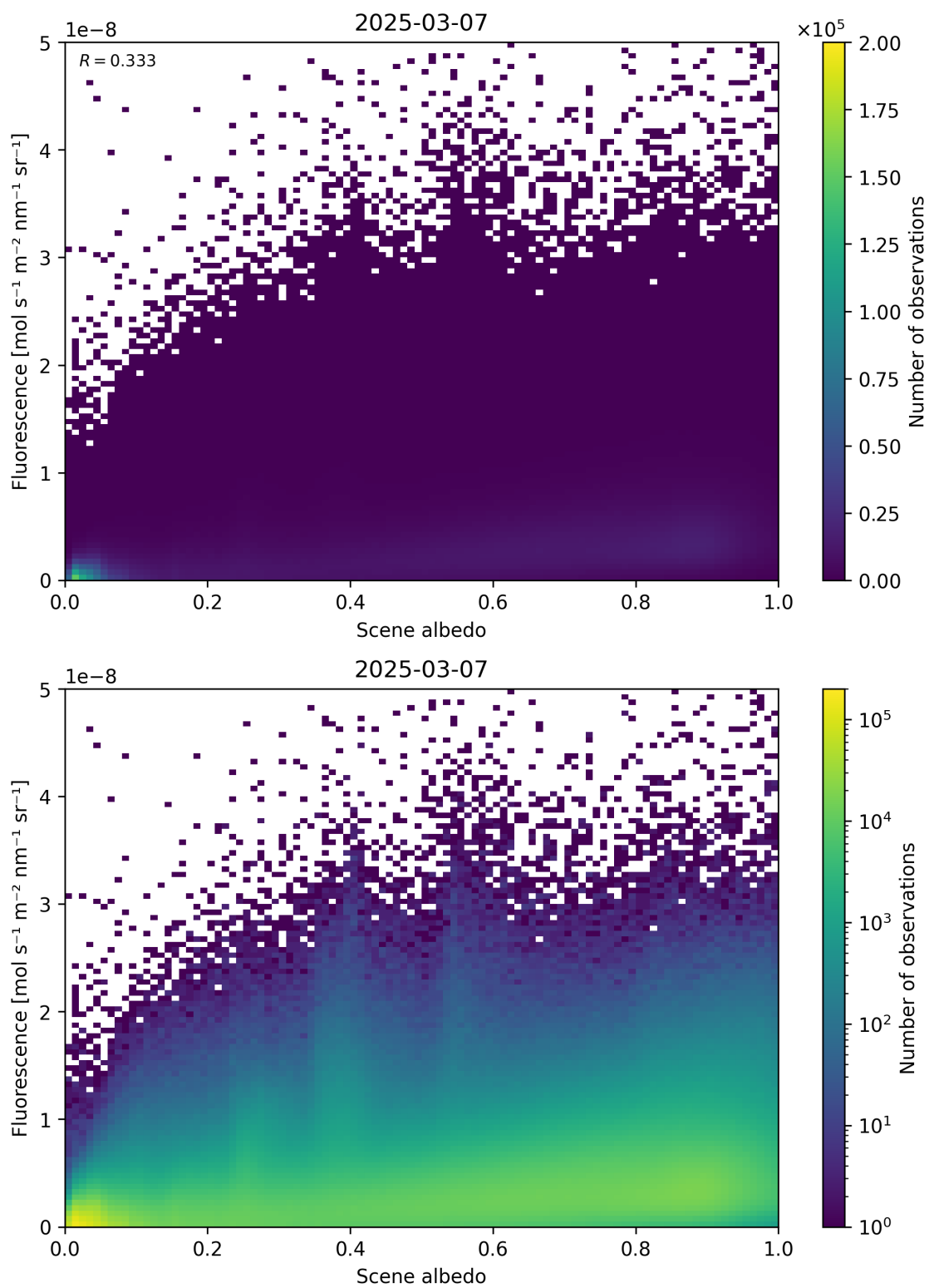
Figure 104: Scatter density plot of “Scene albedo” against “Fluorescence” for 2025-03-07 to 2025-03-08.
