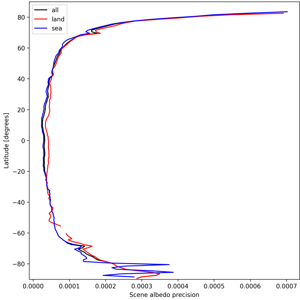
Figure 18: Zonal average of “Scene albedo precision” for 2025-03-07 to 2025-03-08.
