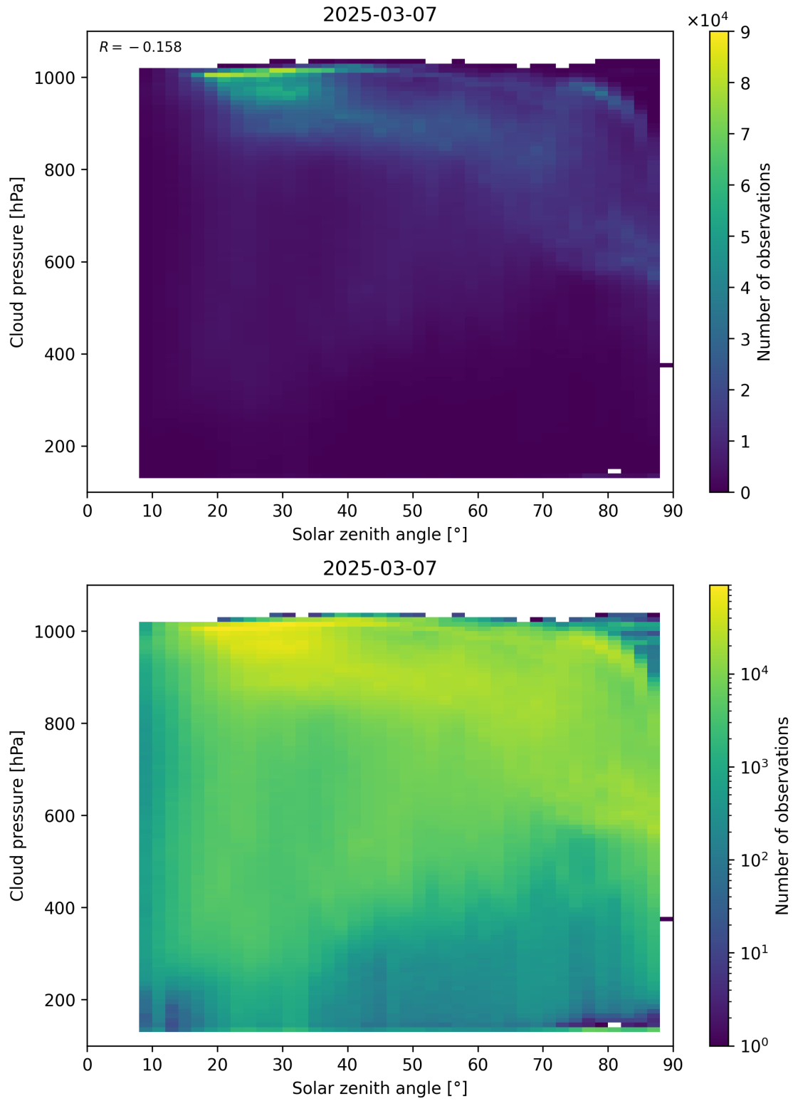
Figure 111: Scatter density plot of “Solar zenith angle” against “Cloud pressure” for 2025-03-07 to 2025-03-08.
