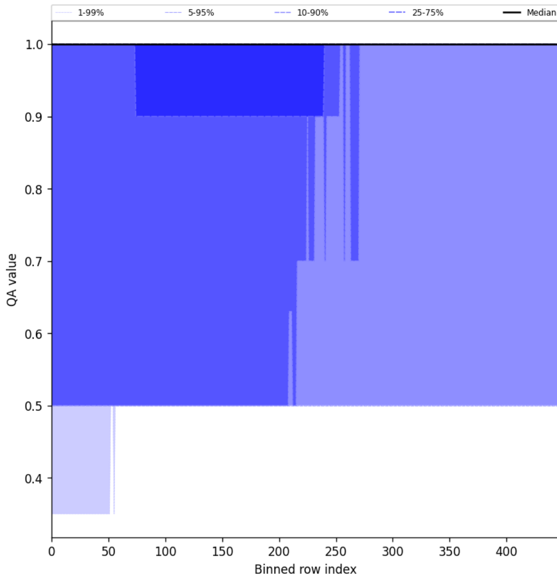
Figure 46: Along track statistics of “QA value” for 2025-03-07 to 2025-03-08
