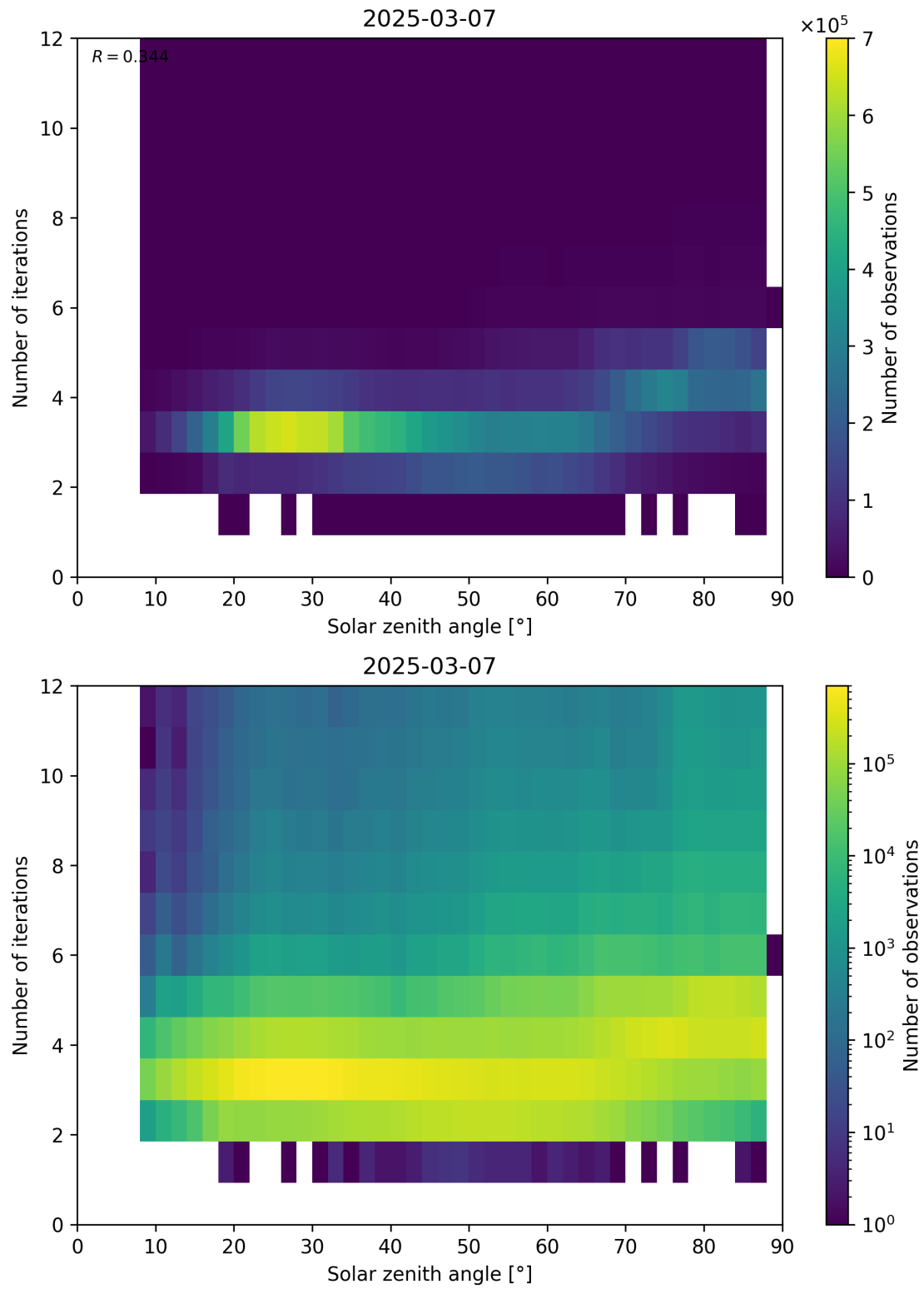
Figure 114: Scatter density plot of “Solar zenith angle” against “Number of iterations” for 2025-03-07 to 2025-03-08.
