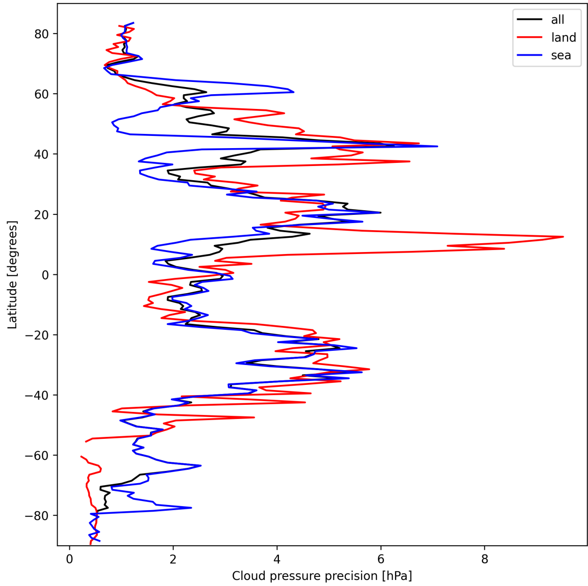
Figure 14: Zonal average of “Cloud pressure precision” for 2025-03-07 to 2025-03-08.
