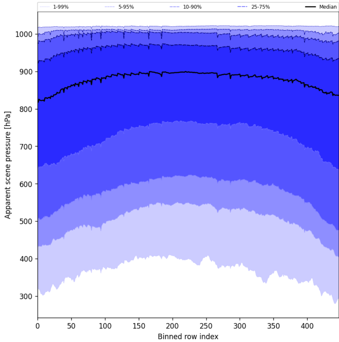
Figure 53: Along track statistics of “Apparent scene pressure” for 2025-03-07 to 2025-03-08
