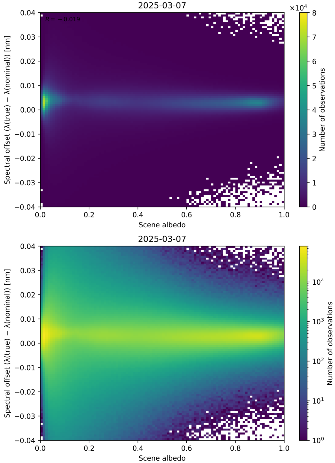
Figure 107: Scatter density plot of “Scene albedo” against “Spectral offset ( \lambda_{\text{true}} - \lambda_{\text{nominal}} )” for 2025-03-07 to 2025-03-08.
