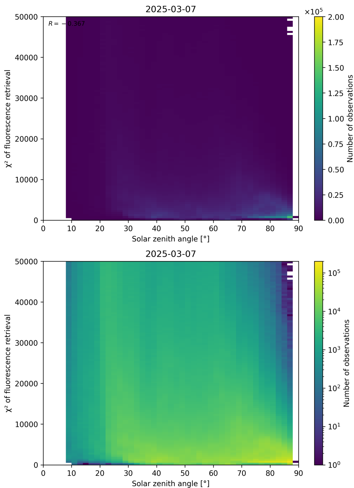
Figure 109: Scatter density plot of “Solar zenith angle” against “ \chi^2 of fluorescence retrieval” for 2025-03-07 to 2025-03-08.
