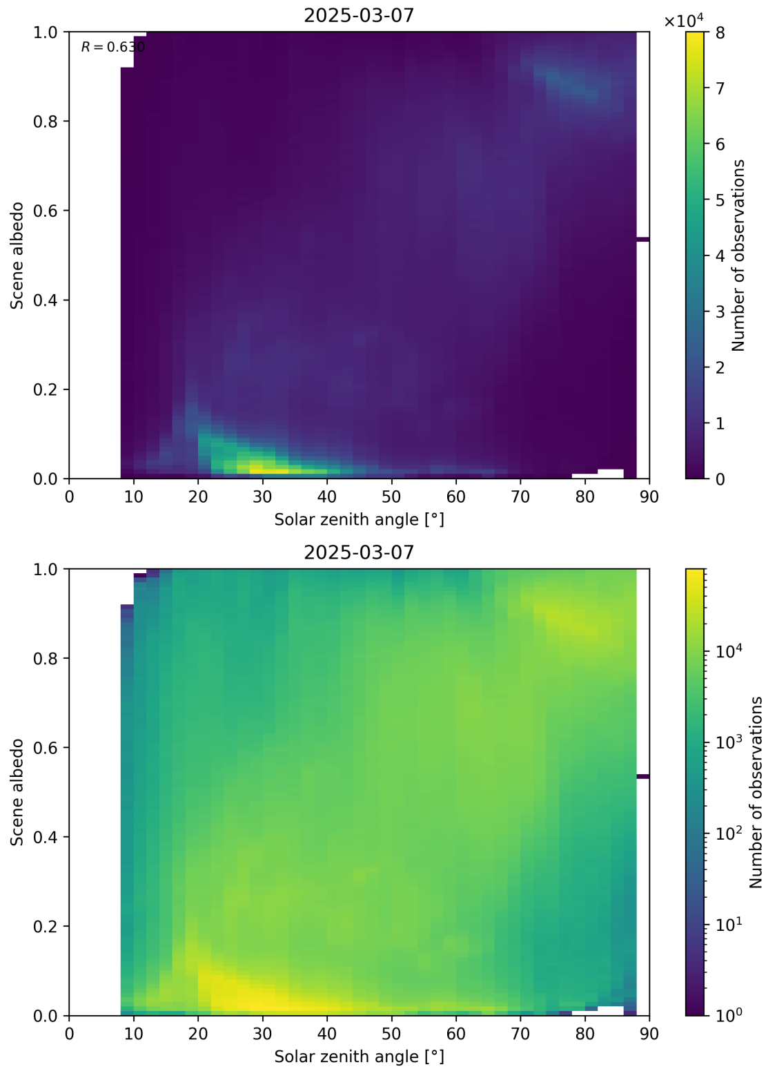
Figure 116: Scatter density plot of “Solar zenith angle” against “Scene albedo” for 2025-03-07 to 2025-03-08.
