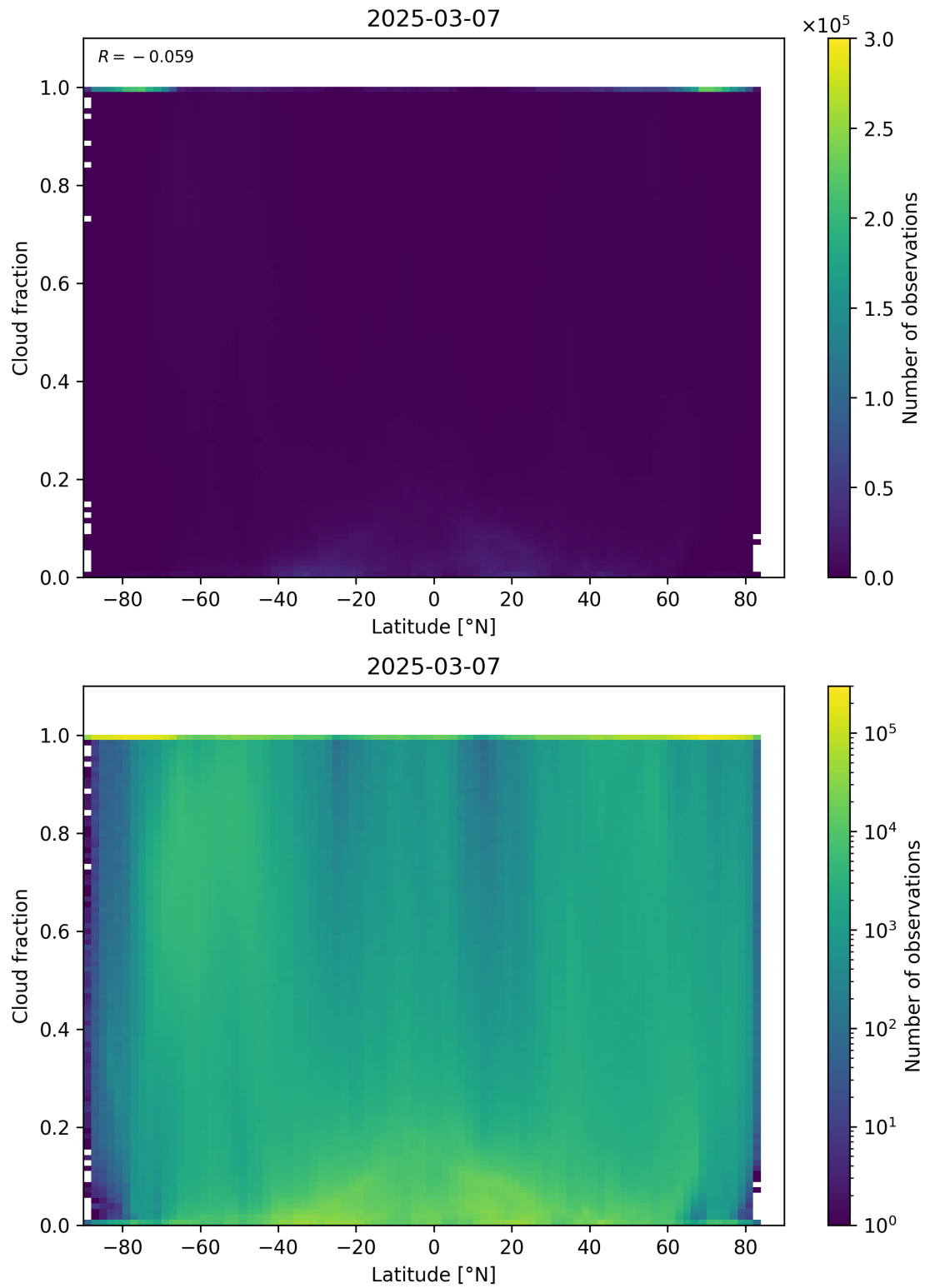
Figure 90: Scatter density plot of “Latitude” against “Cloud fraction” for 2025-03-07 to 2025-03-08.
