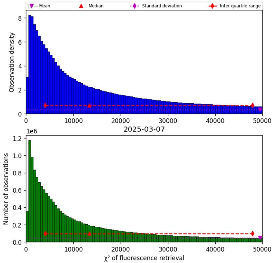
Figure 42: Histogram of “ \chi^2 of fluorescence retrieval” for 2025-03-07 to 2025-03-08
