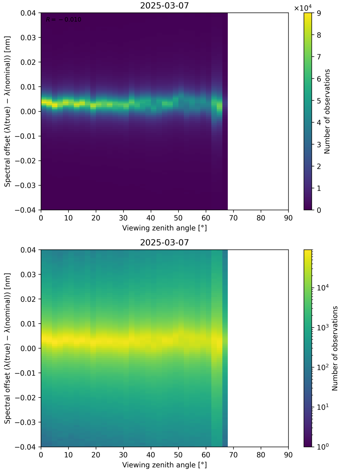
Figure 128: Scatter density plot of “Viewing zenith angle” against “Spectral offset ( \lambda_{\text{true}} - \lambda_{\text{nominal}} )” for 2025-03-07 to 2025-03-08.
