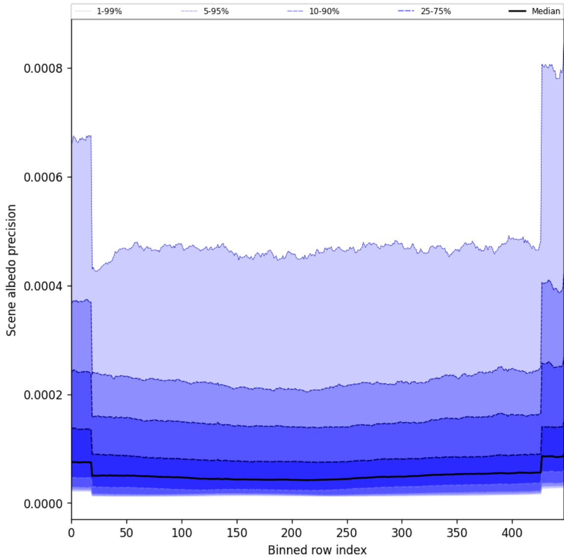
Figure 52: Along track statistics of “Scene albedo precision” for 2025-03-07 to 2025-03-08
