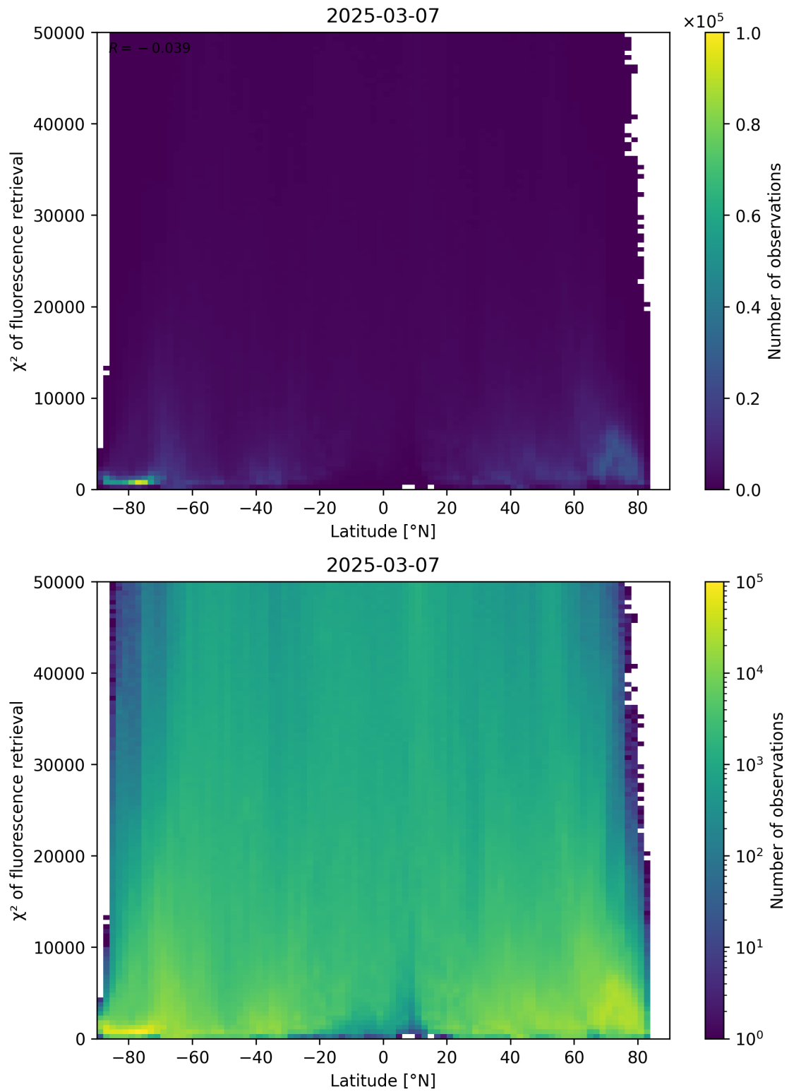
Figure 89: Scatter density plot of “Latitude” against “ \chi^2 of fluorescence retrieval” for 2025-03-07 to 2025-03-08.
