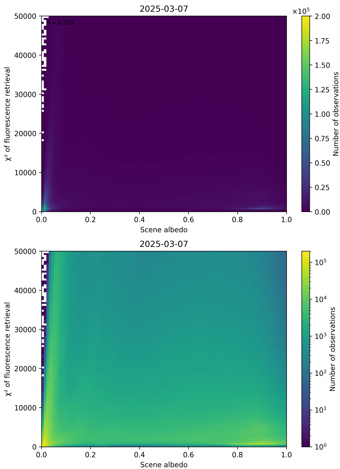
Figure 103: Scatter density plot of “Scene albedo” against “ \chi^2 of fluorescence retrieval” for 2025-03-07 to 2025-03-08.
