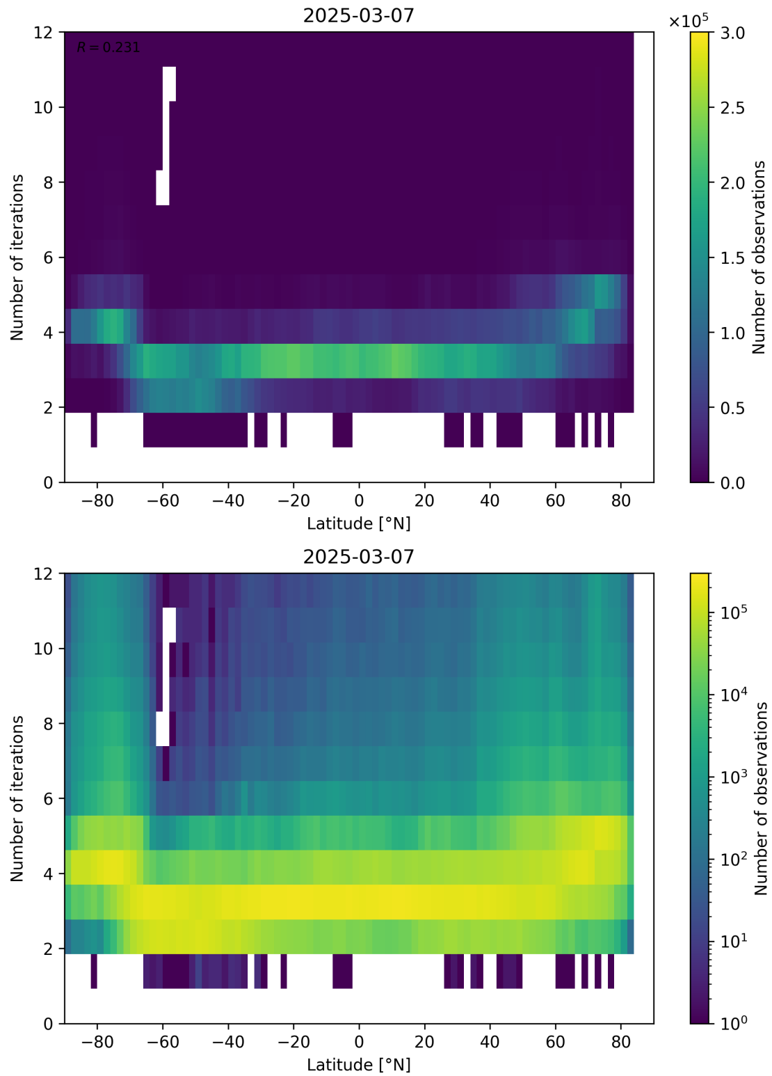
Figure 93: Scatter density plot of “Latitude” against “Number of iterations” for 2025-03-07 to 2025-03-08.
