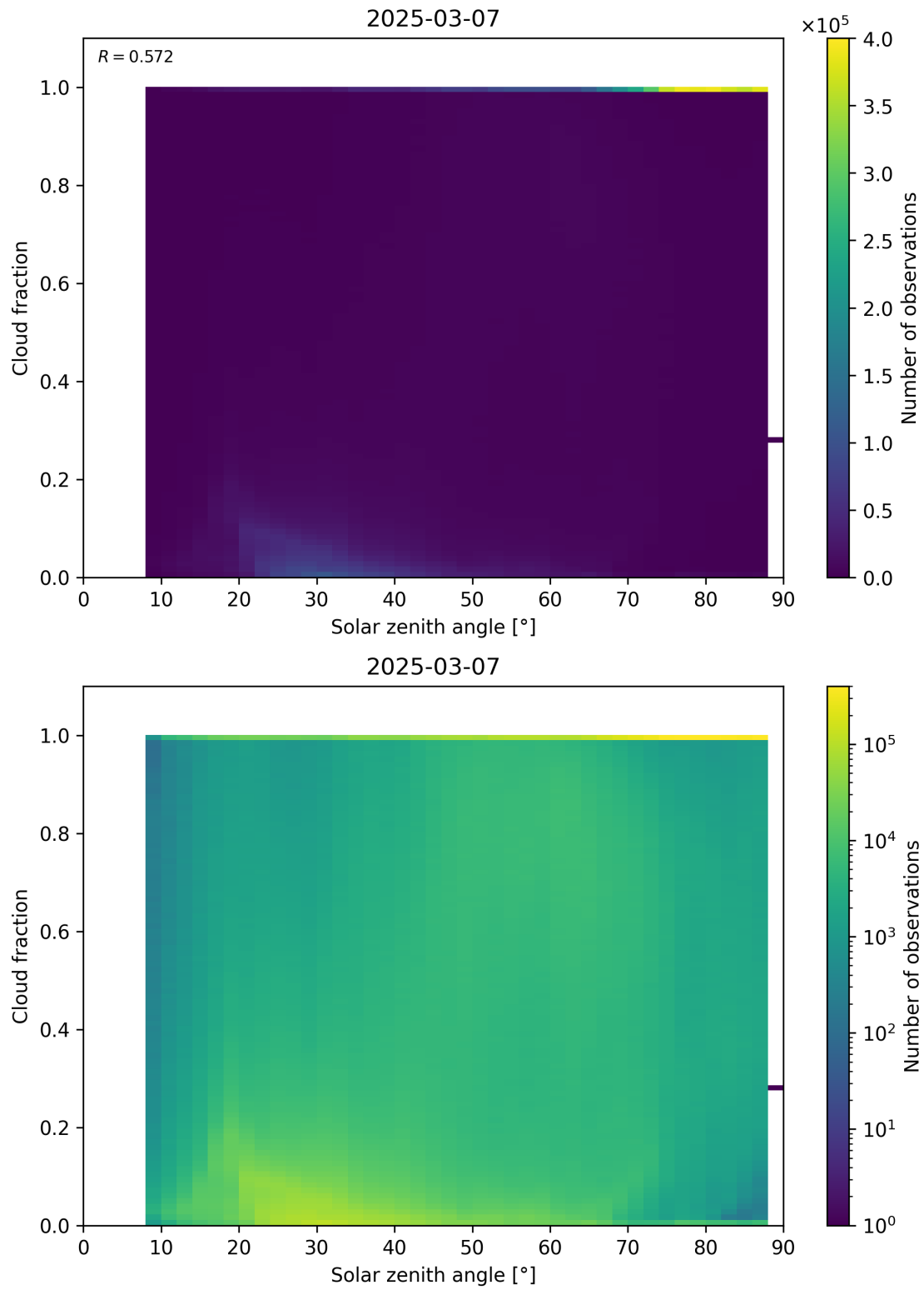
Figure 110: Scatter density plot of “Solar zenith angle” against “Cloud fraction” for 2025-03-07 to 2025-03-08.
