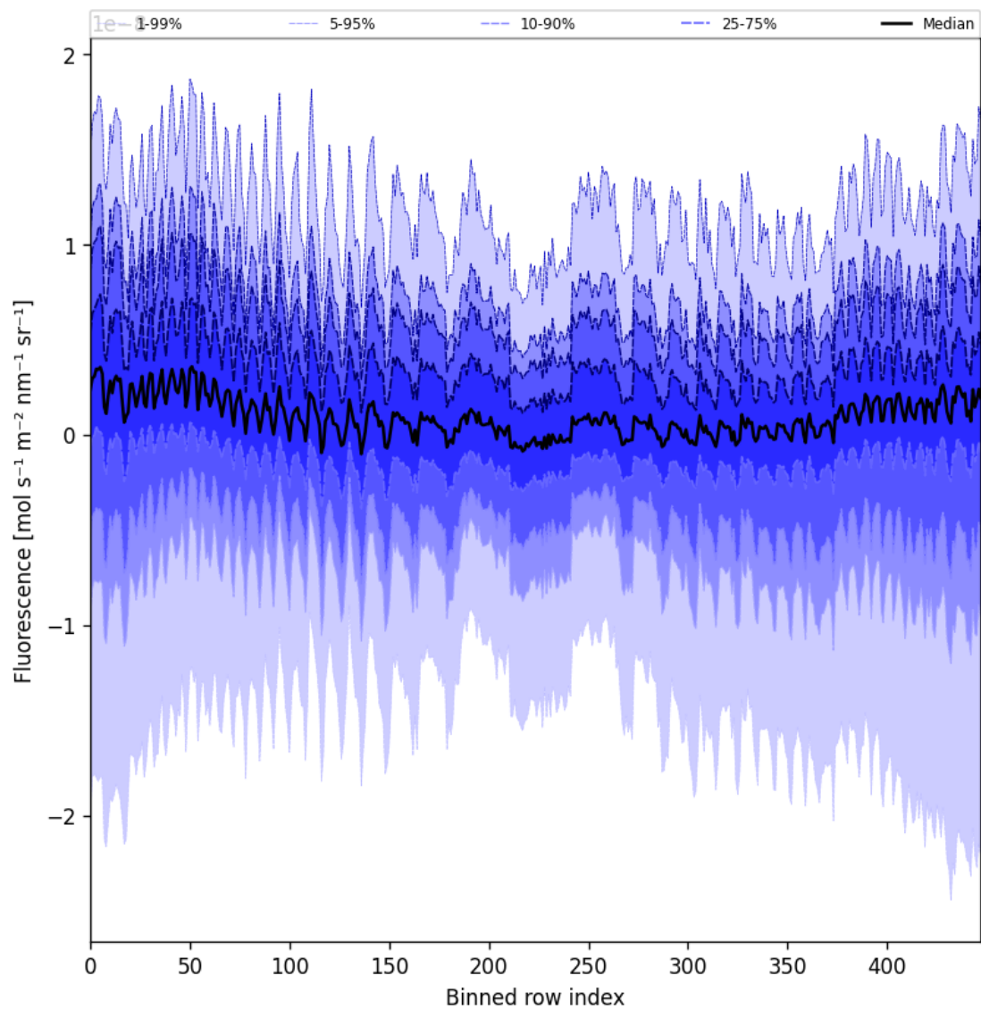
Figure 57: Along track statistics of “Fluorescence” for 2025-03-07 to 2025-03-08
