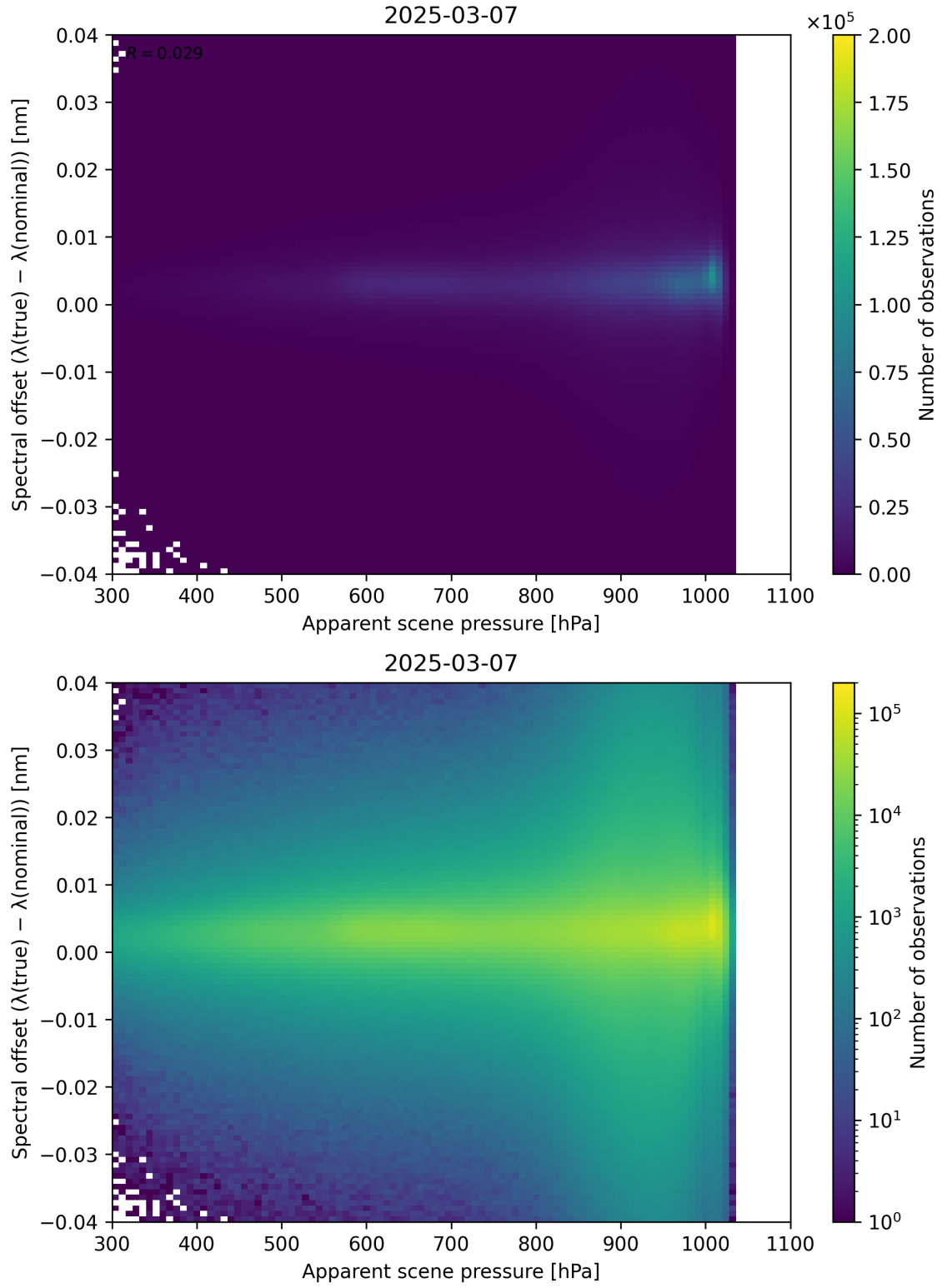
Figure 67: Scatter density plot of “Apparent scene pressure” against “Spectral offset ( \lambda_{\text{true}} - \lambda_{\text{nominal}} )” for 2025-03-07 to 2025-03-08.
