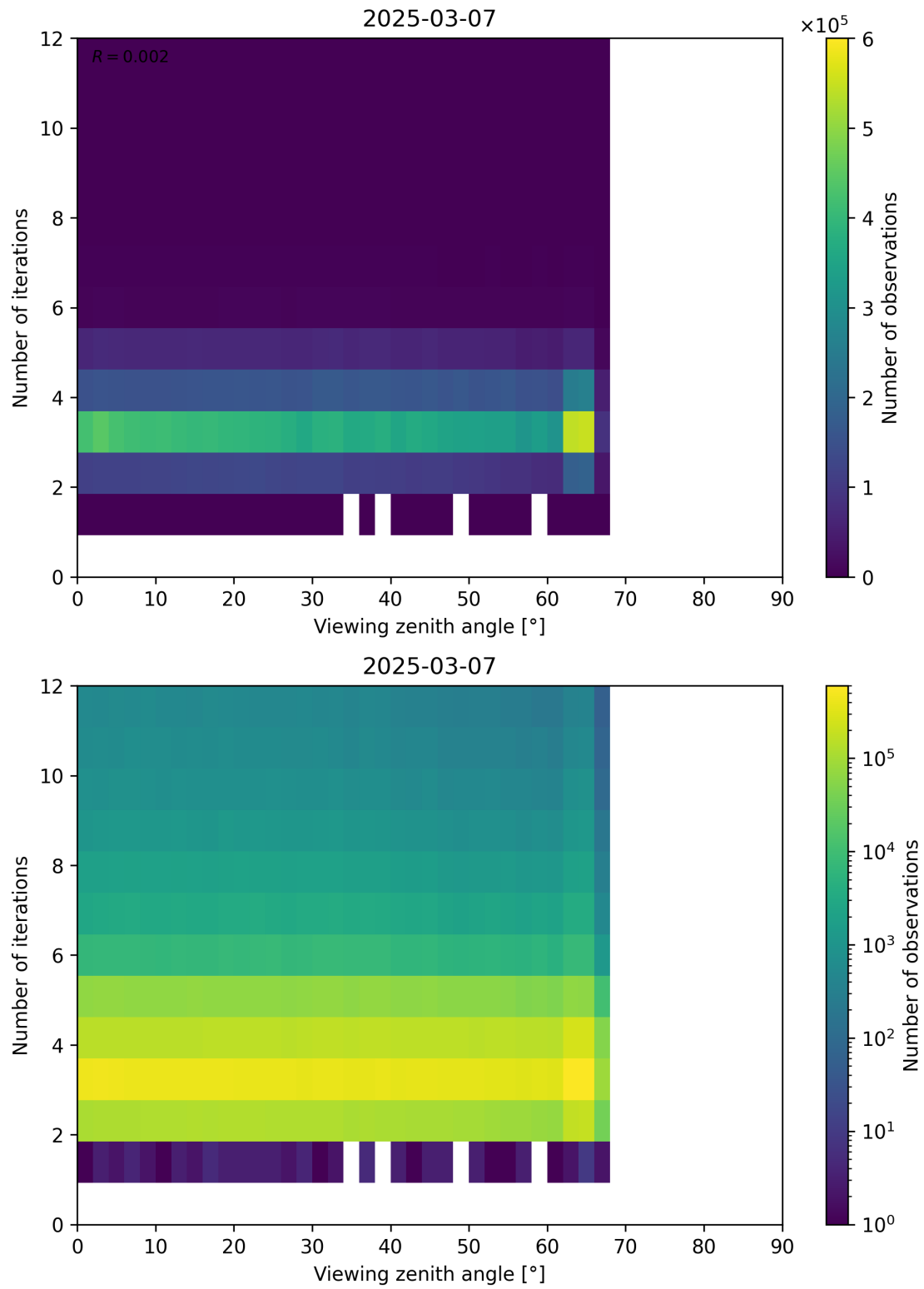
Figure 124: Scatter density plot of “Viewing zenith angle” against “Number of iterations” for 2025-03-07 to 2025-03-08.
