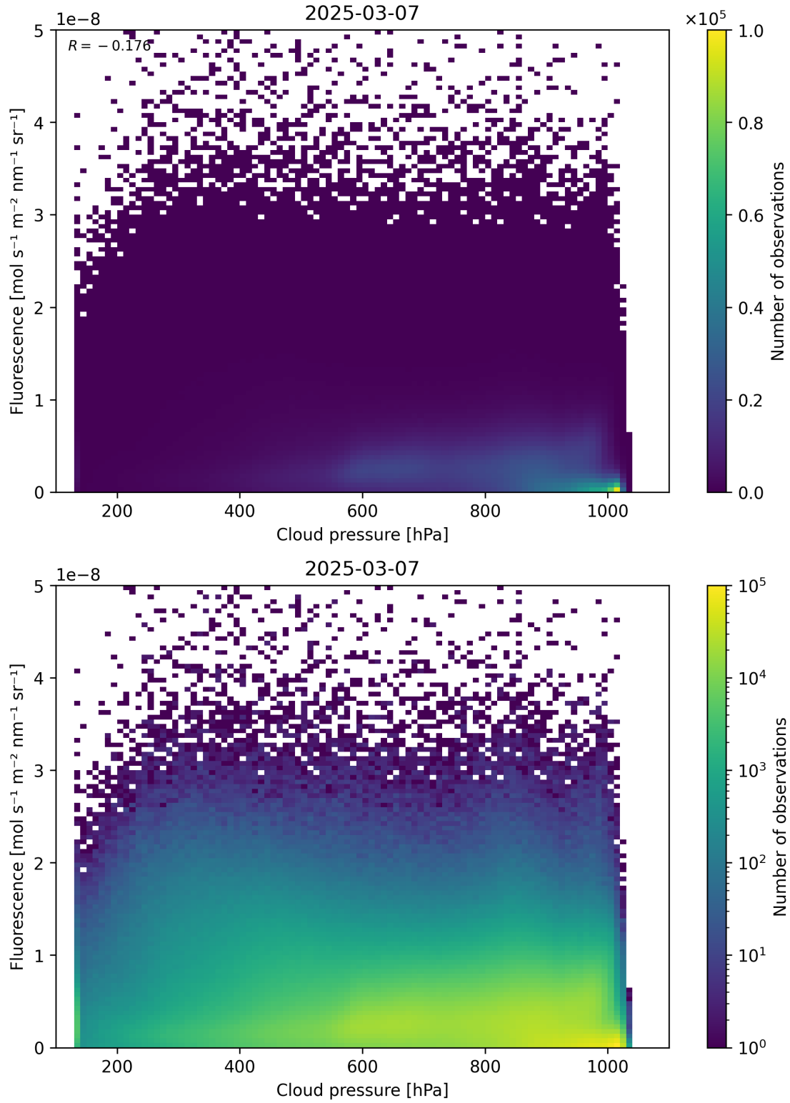
Figure 80: Scatter density plot of “Cloud pressure” against “Fluorescence” for 2025-03-07 to 2025-03-08.
