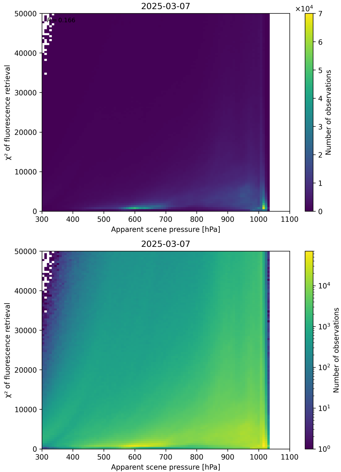
Figure 63: Scatter density plot of “Apparent scene pressure” against “ \chi^2 of fluorescence retrieval” for 2025-03-07 to 2025-03-08.
