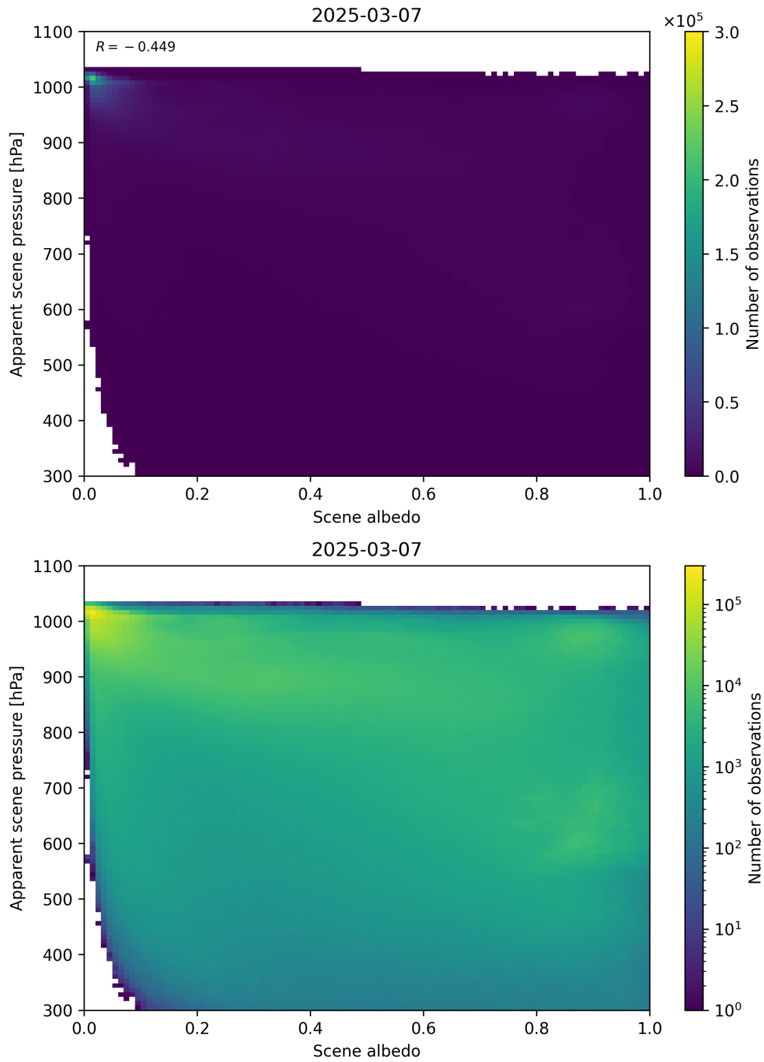
Figure 102: Scatter density plot of “Scene albedo” against “Apparent scene pressure” for 2025-03-07 to 2025-03-08.
