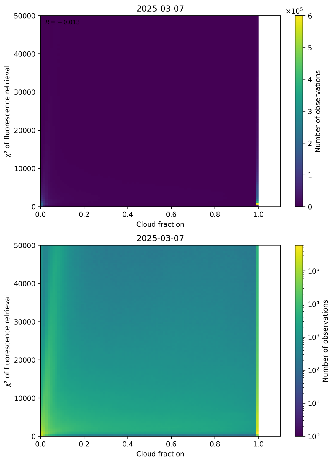
Figure 71: Scatter density plot of “Cloud fraction” against “ \chi^2 of fluorescence retrieval” for 2025-03-07 to 2025-03-08.
