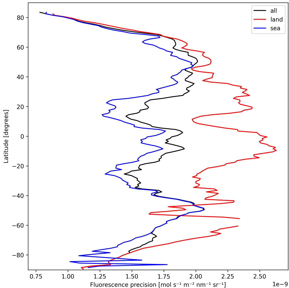
Figure 24: Zonal average of “Fluorescence precision” for 2025-03-07 to 2025-03-08.
