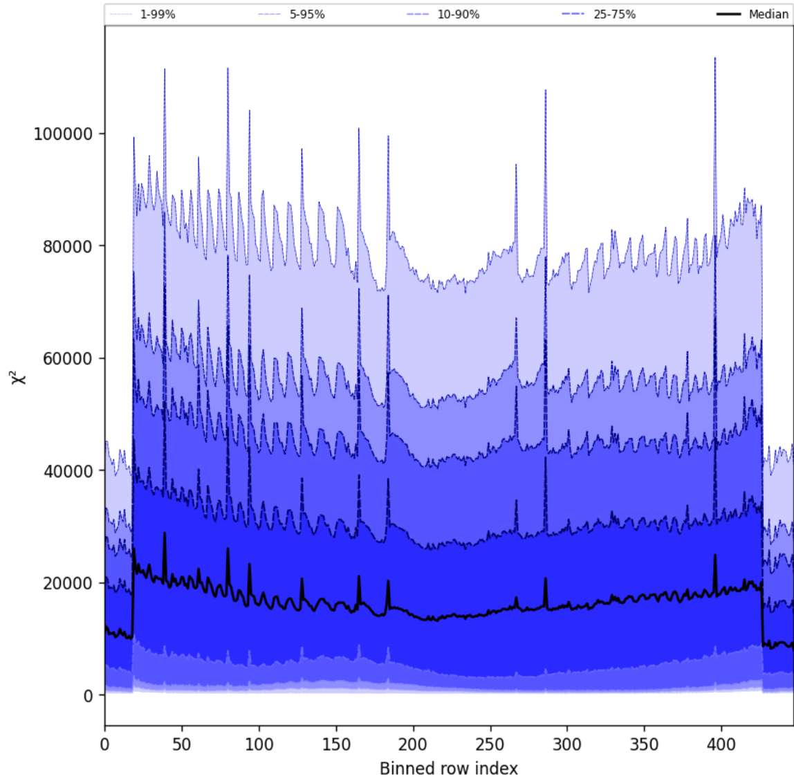
Figure 55: Along track statistics of “ \chi^2 ” for 2025-03-07 to 2025-03-08
