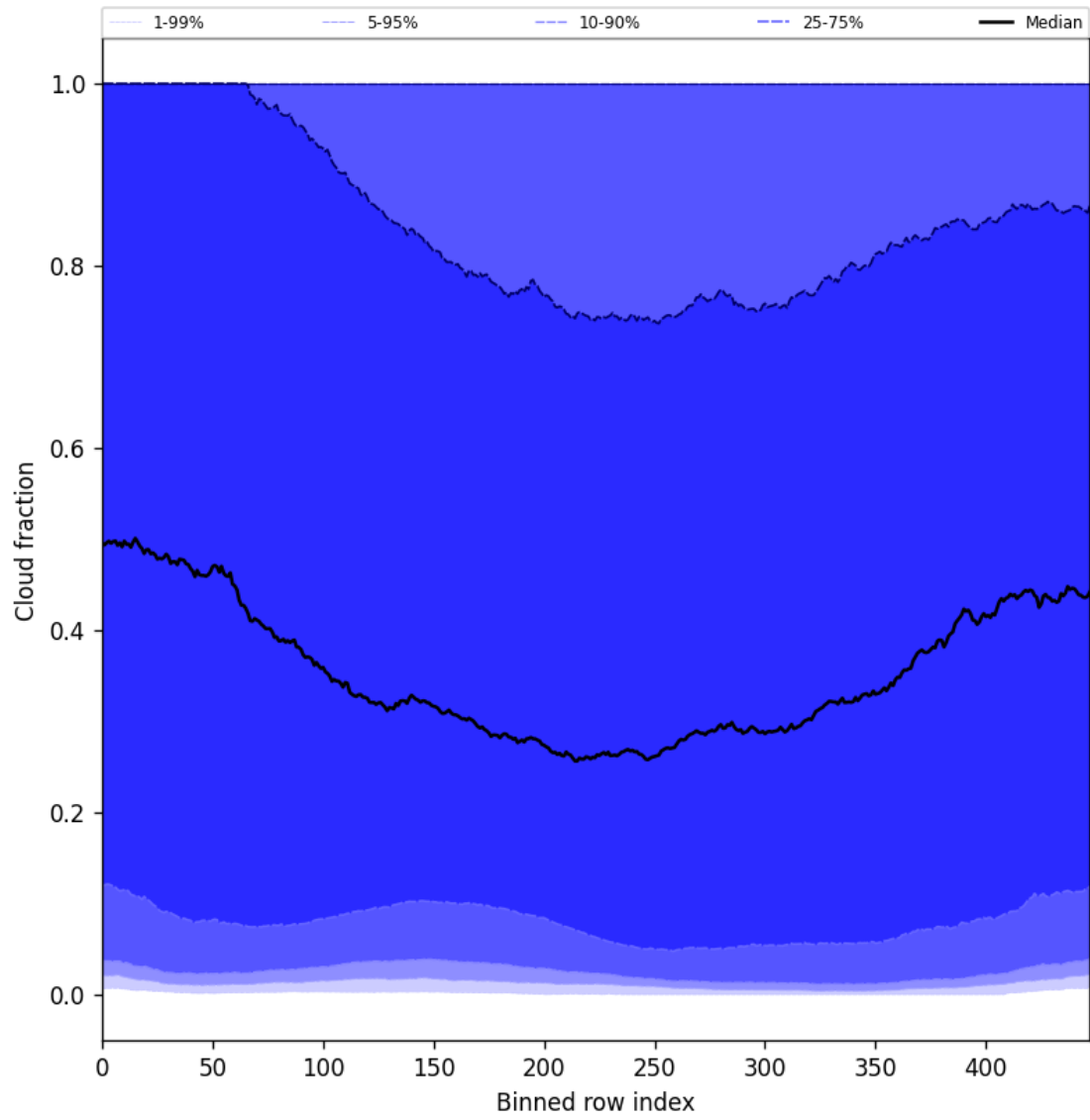
Figure 49: Along track statistics of “Cloud fraction” for 2025-03-07 to 2025-03-08
