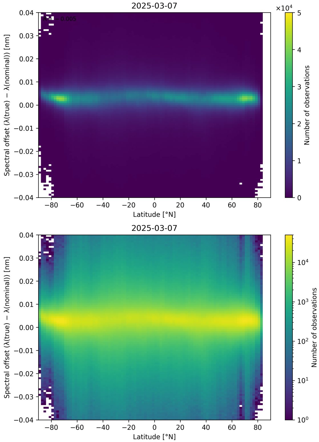
Figure 96: Scatter density plot of “Latitude” against “Spectral offset ( \lambda_{\text{true}} - \lambda_{\text{nominal}} )” for 2025-03-07 to 2025-03-08.
