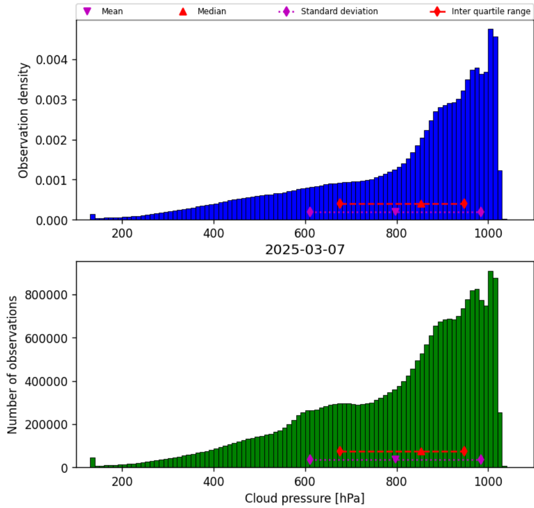
Figure 30: Histogram of “Cloud pressure” for 2025-03-07 to 2025-03-08
