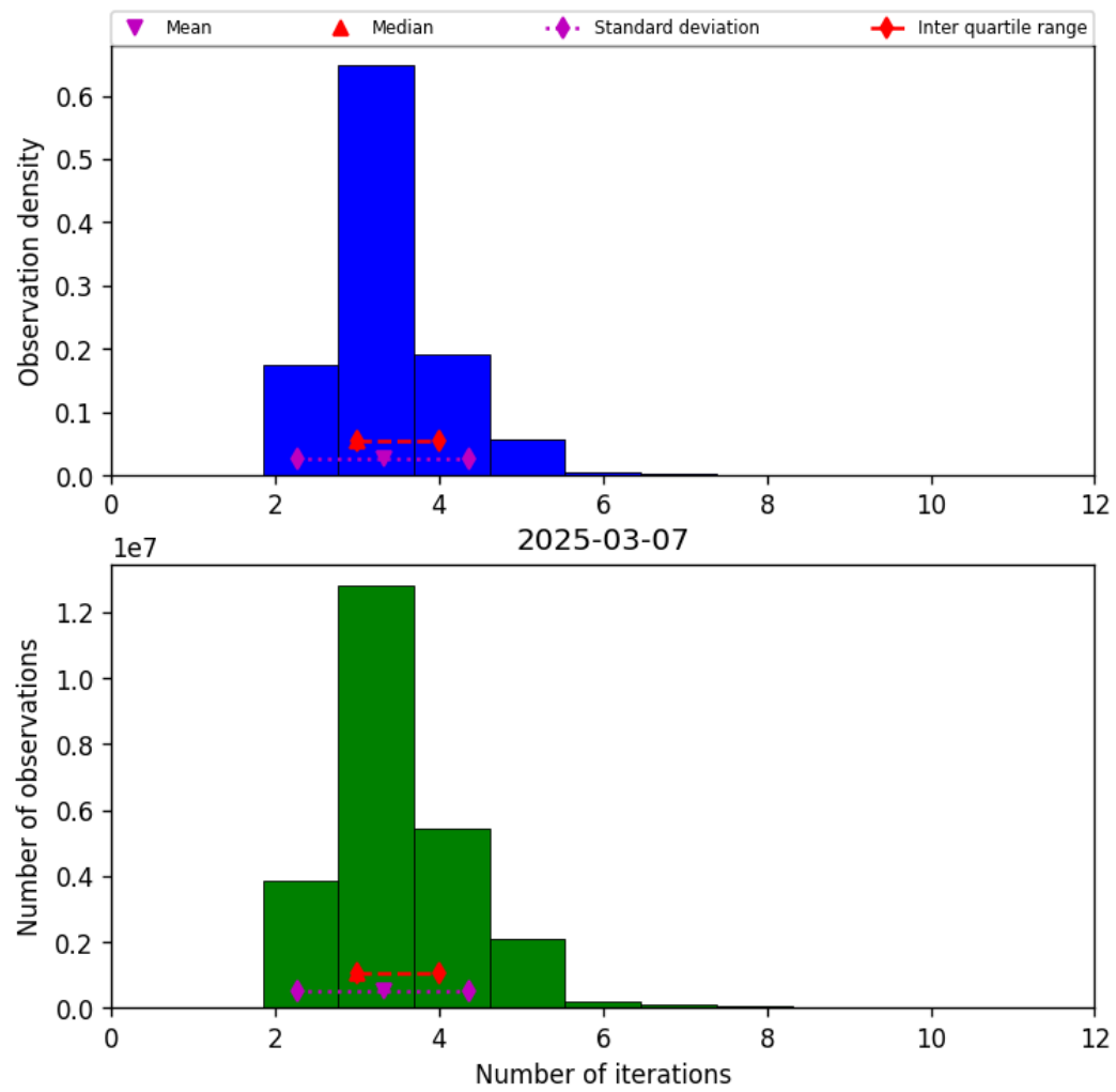
Figure 39: Histogram of “Number of iterations” for 2025-03-07 to 2025-03-08
