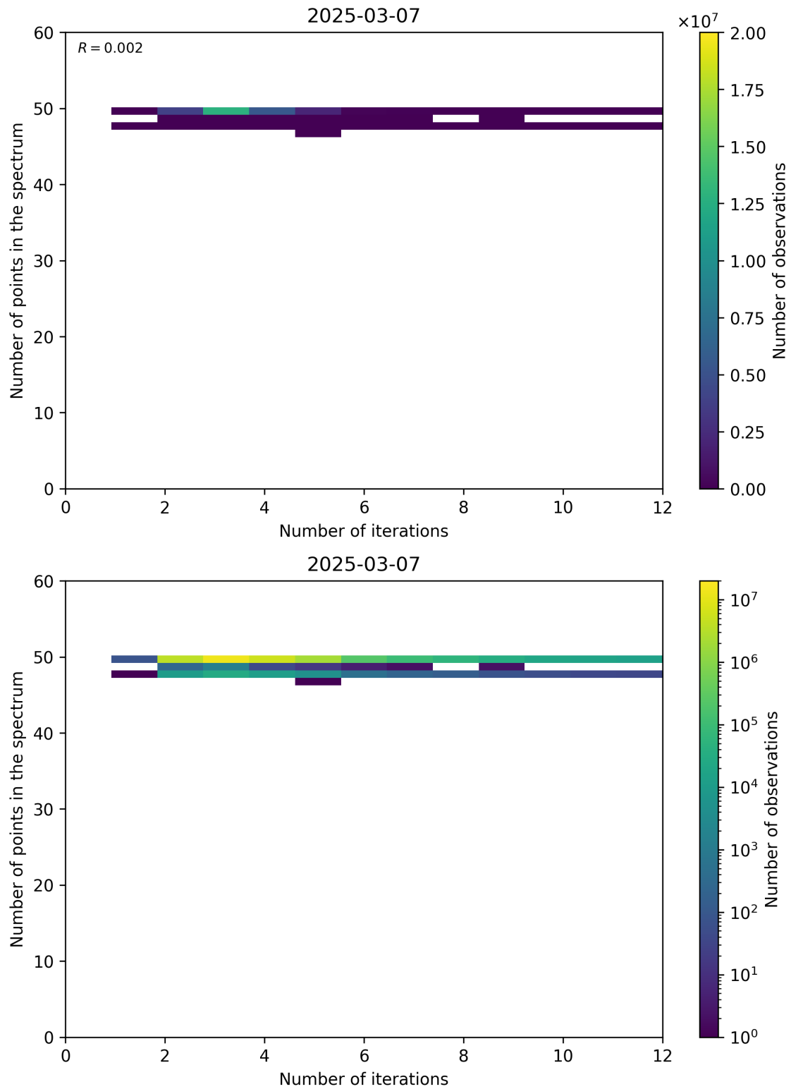
Figure 99: Scatter density plot of “Number of iterations” against “Number of points in the spectrum” for 2025-03-07 to 2025-03-08.
