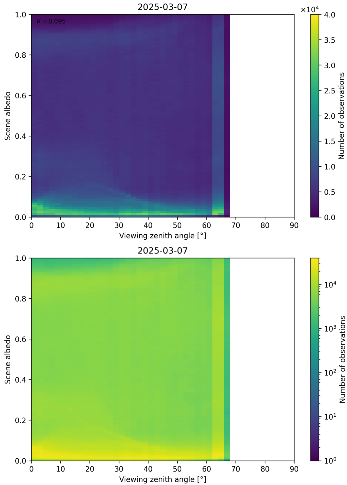
Figure 126: Scatter density plot of “Viewing zenith angle” against “Scene albedo” for 2025-03-07 to 2025-03-08.
