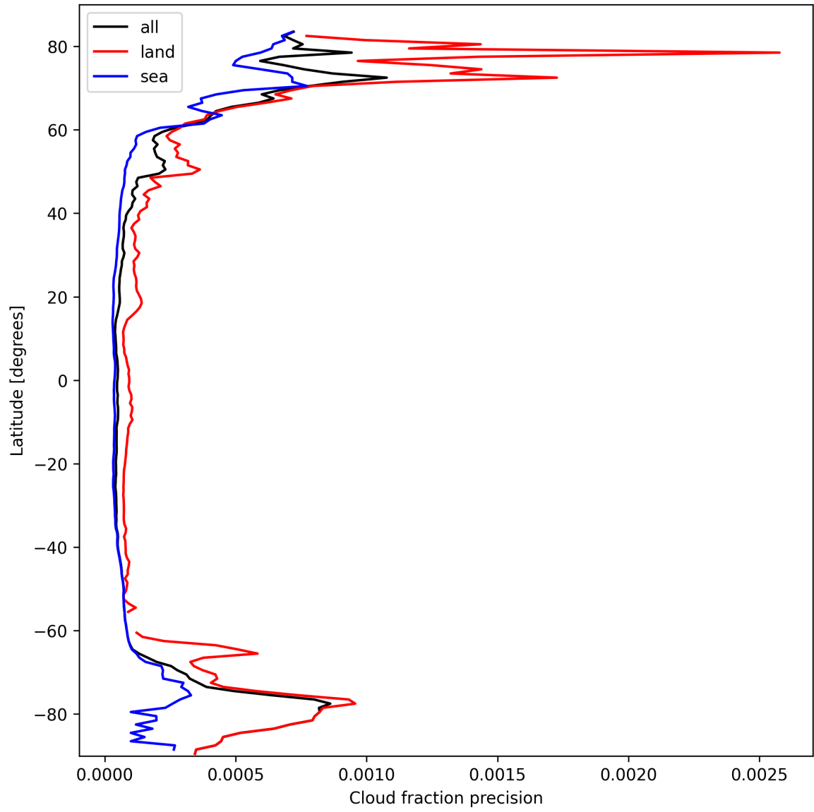
Figure 16: Zonal average of “Cloud fraction precision” for 2025-03-07 to 2025-03-08.
