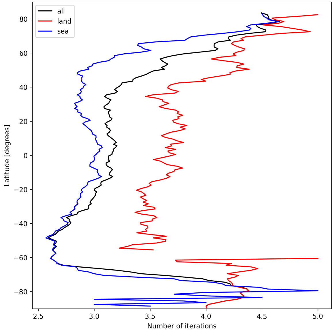
Figure 22: Zonal average of “Number of iterations” for 2025-03-07 to 2025-03-08.
