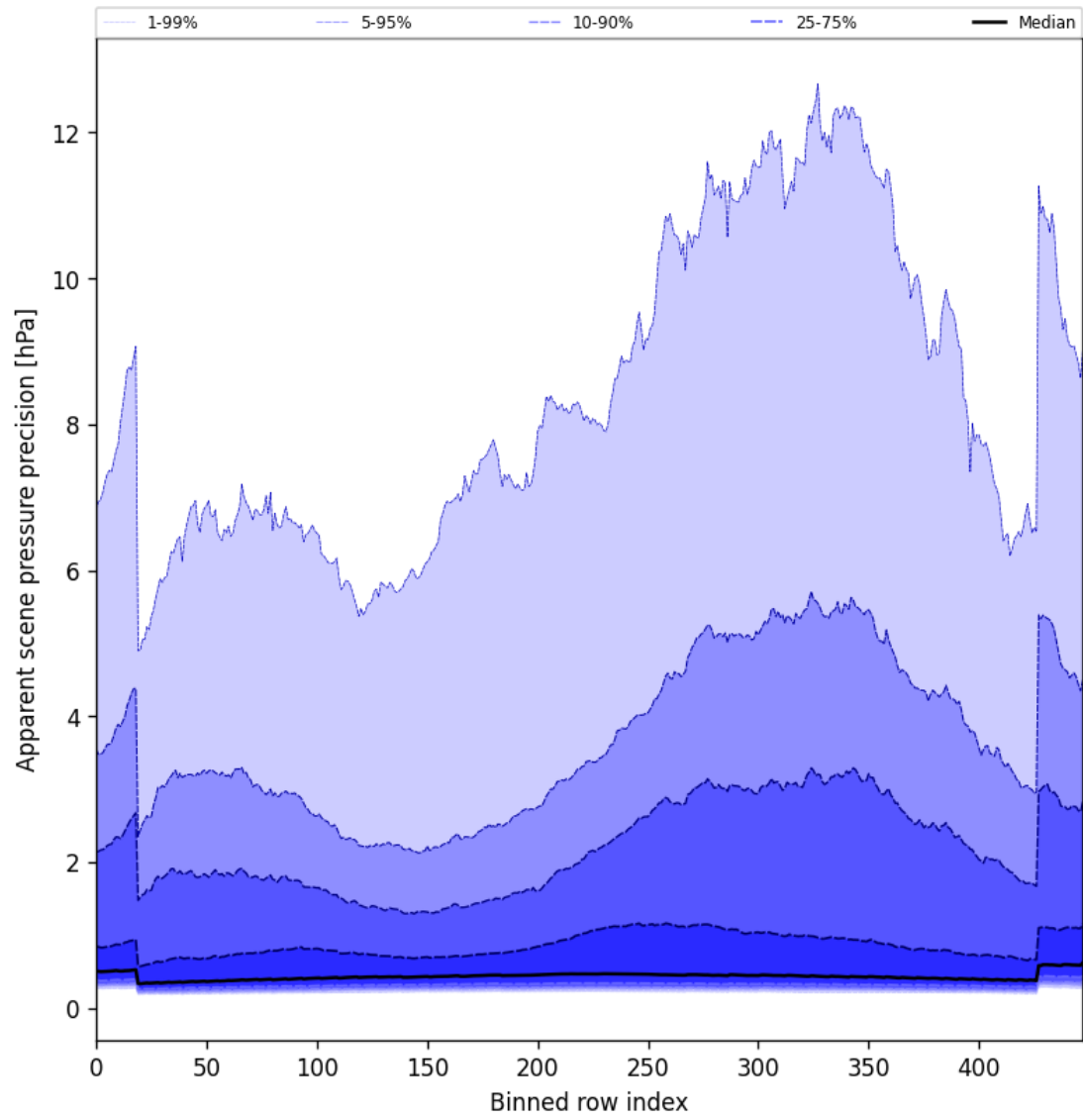
Figure 54: Along track statistics of “Apparent scene pressure precision” for 2025-03-07 to 2025-03-08
