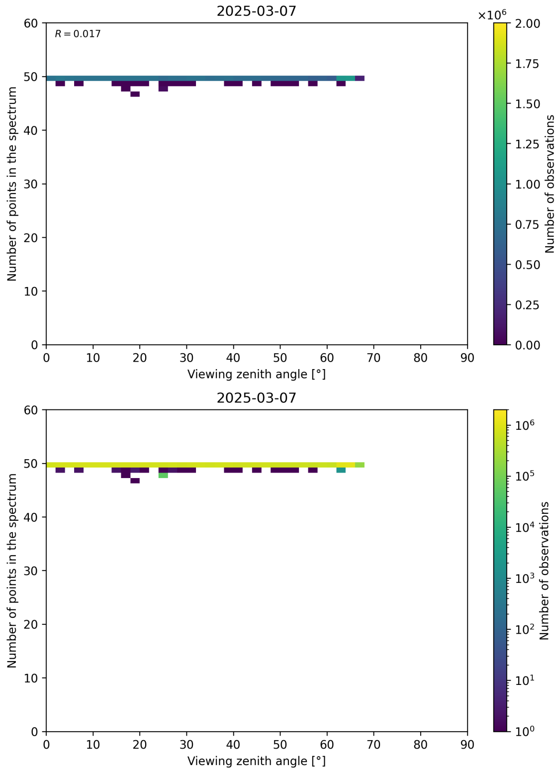
Figure 125: Scatter density plot of “Viewing zenith angle” against “Number of points in the spectrum” for 2025-03-07 to 2025-03-08.
