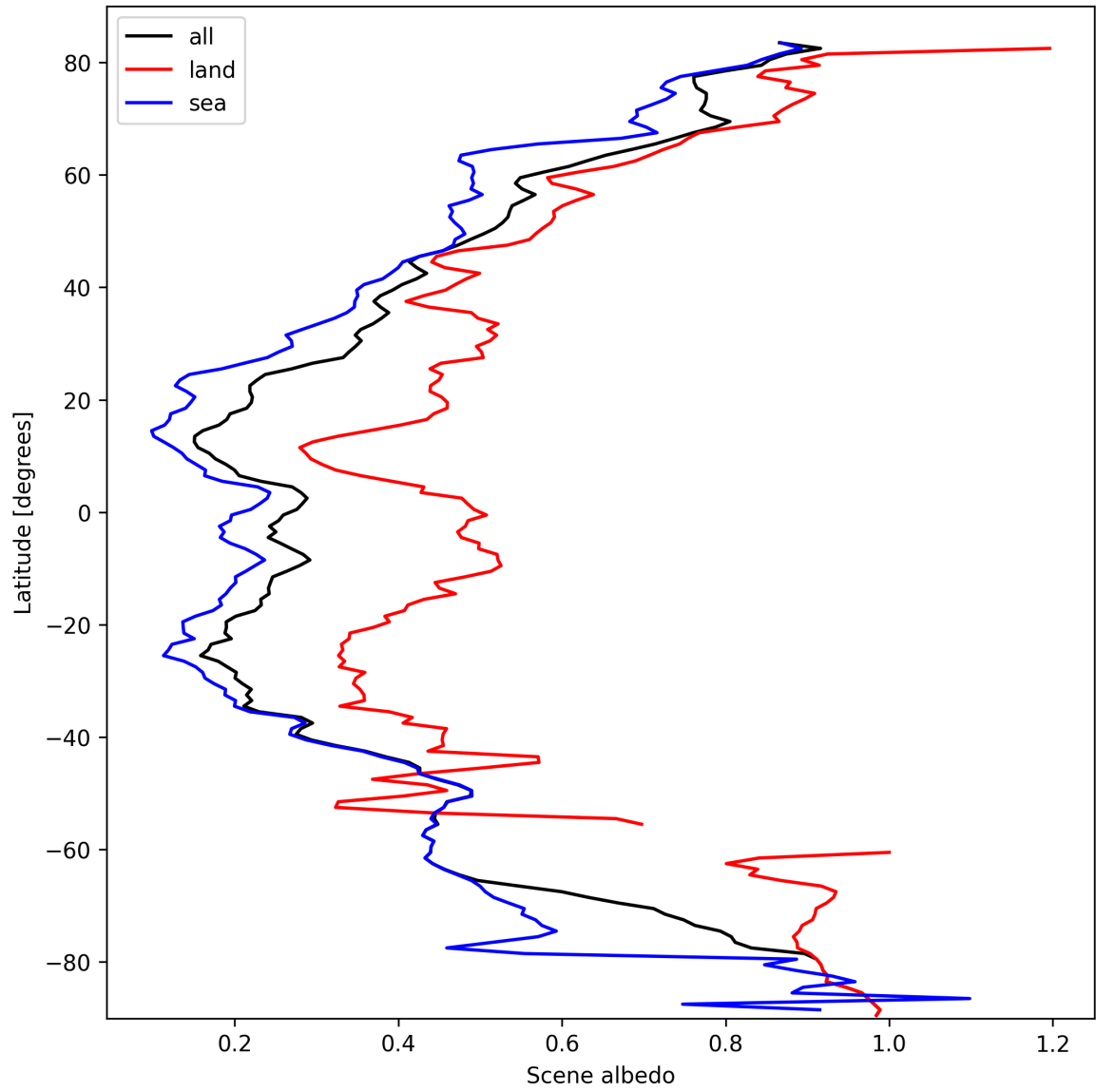
Figure 17: Zonal average of “Scene albedo” for 2025-03-07 to 2025-03-08.
