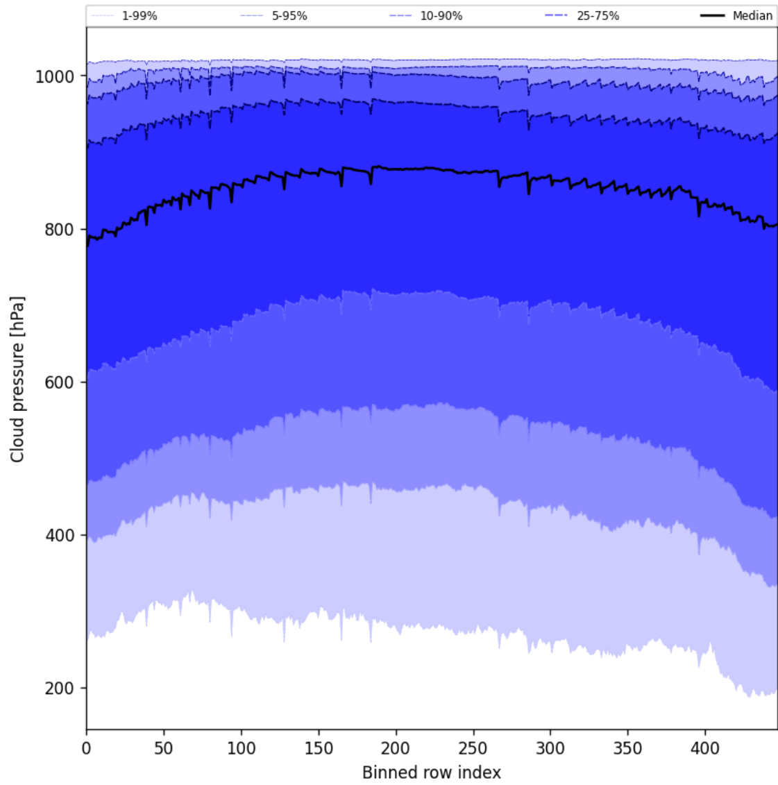
Figure 47: Along track statistics of “Cloud pressure” for 2025-03-07 to 2025-03-08
