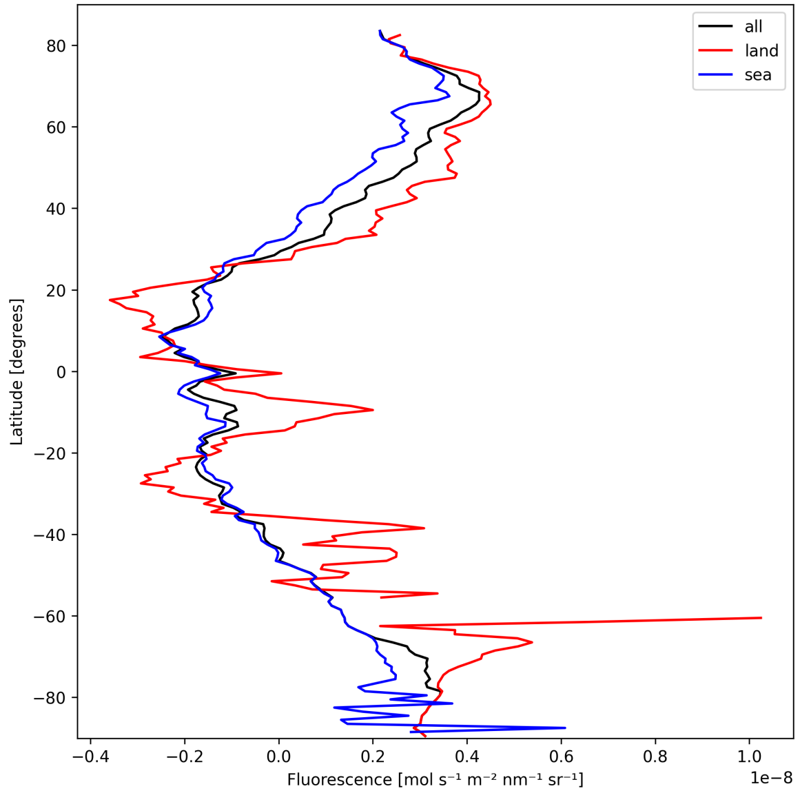
Figure 23: Zonal average of “Fluorescence” for 2025-03-07 to 2025-03-08.
