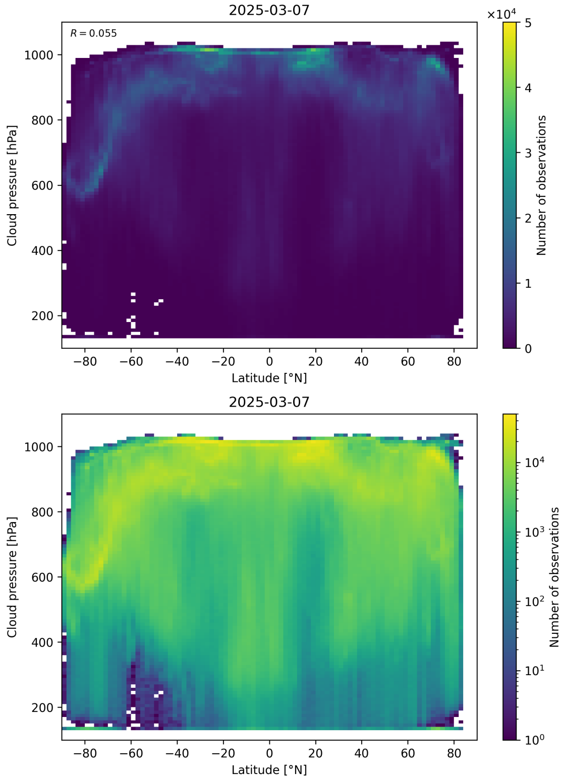
Figure 91: Scatter density plot of “Latitude” against “Cloud pressure” for 2025-03-07 to 2025-03-08.
