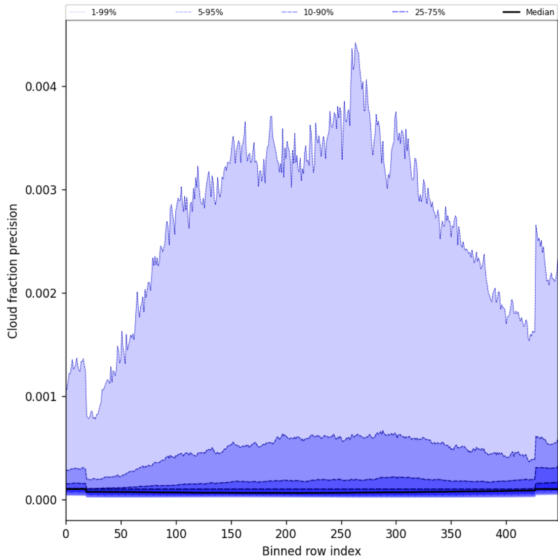
Figure 50: Along track statistics of “Cloud fraction precision” for 2025-03-07 to 2025-03-08
