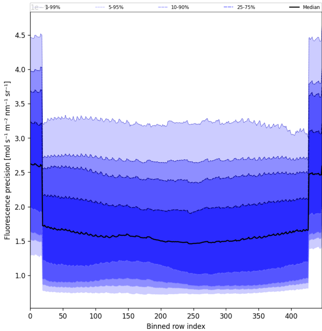
Figure 58: Along track statistics of “Fluorescence precision” for 2025-03-07 to 2025-03-08
