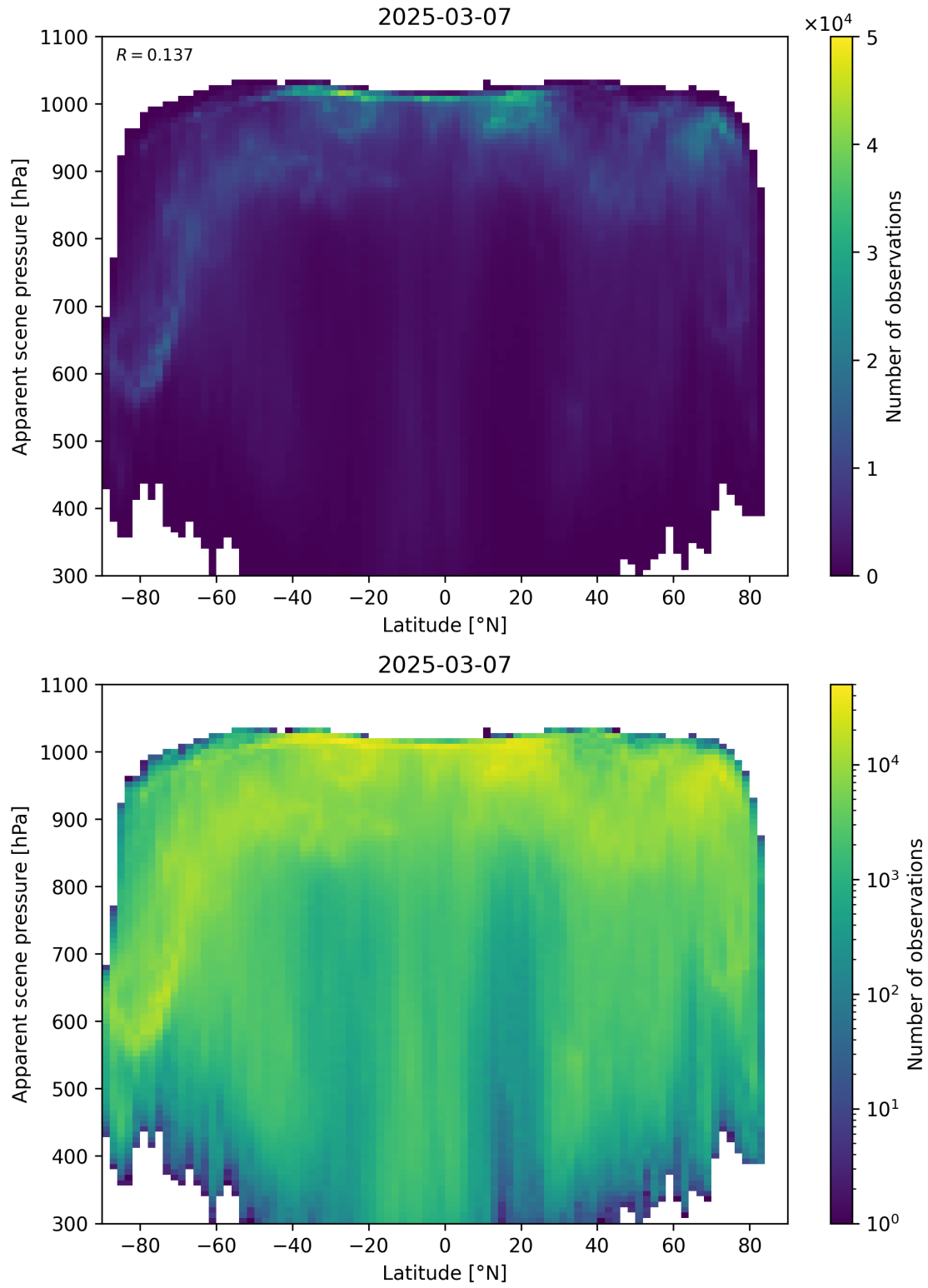
Figure 88: Scatter density plot of “Latitude” against “Apparent scene pressure” for 2025-03-07 to 2025-03-08.
