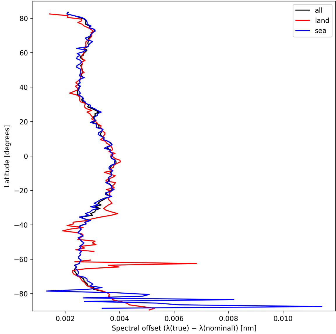
Figure 28: Zonal average of “Spectral offset ( \lambda_{\text{true}} - \lambda_{\text{nominal}} )” for 2025-03-07 to 2025-03-08.
