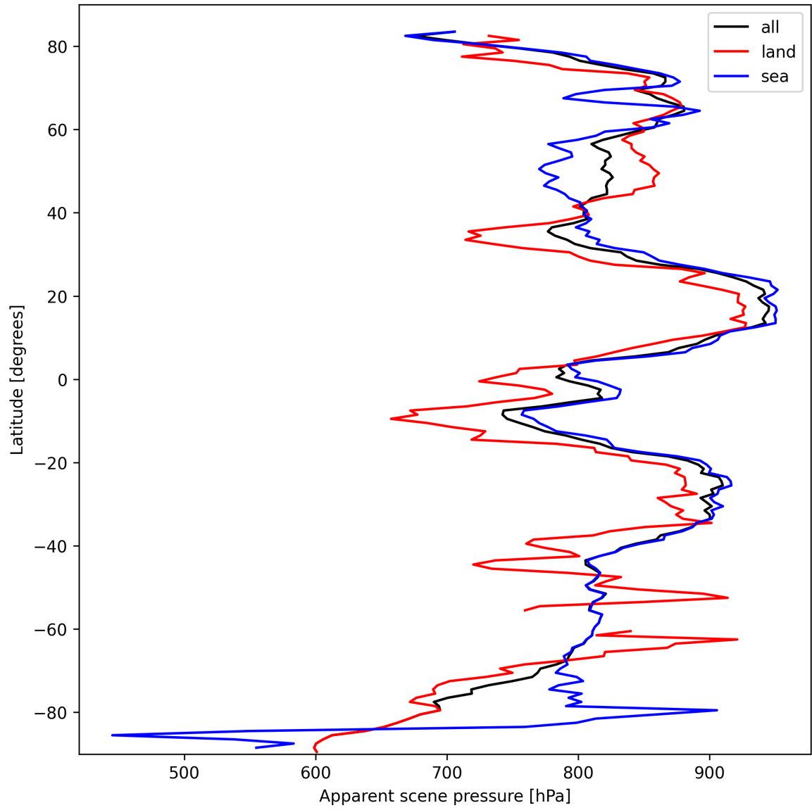
Figure 19: Zonal average of “Apparent scene pressure” for 2025-03-07 to 2025-03-08.
