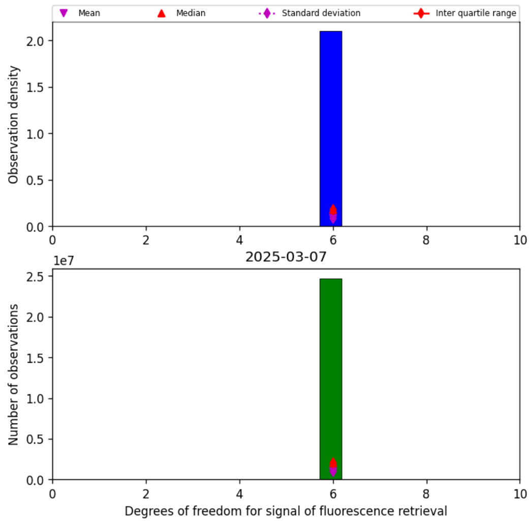
Figure 43: Histogram of “Degrees of freedom for signal of fluorescence retrieval” for 2025-03-07 to 2025-03-08
