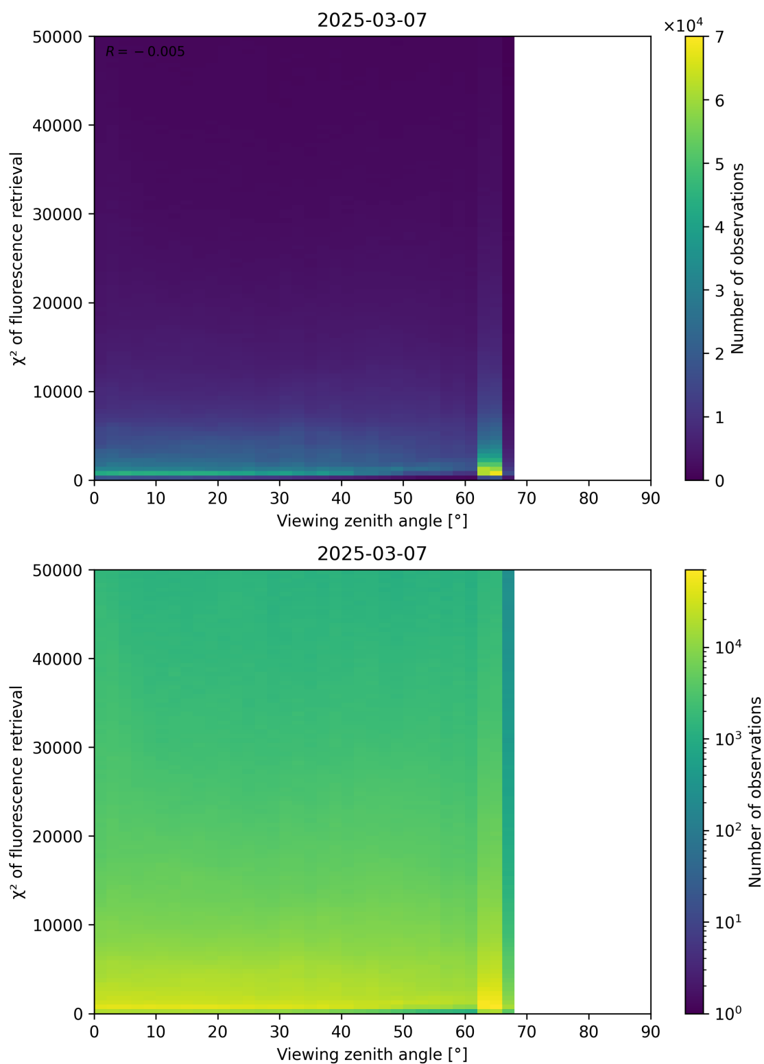
Figure 119: Scatter density plot of “Viewing zenith angle” against “ \chi^2 of fluorescence retrieval” for 2025-03-07 to 2025-03-08.
