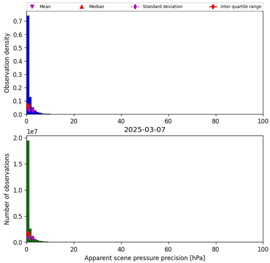
Figure 37: Histogram of “Apparent scene pressure precision” for 2025-03-07 to 2025-03-08
