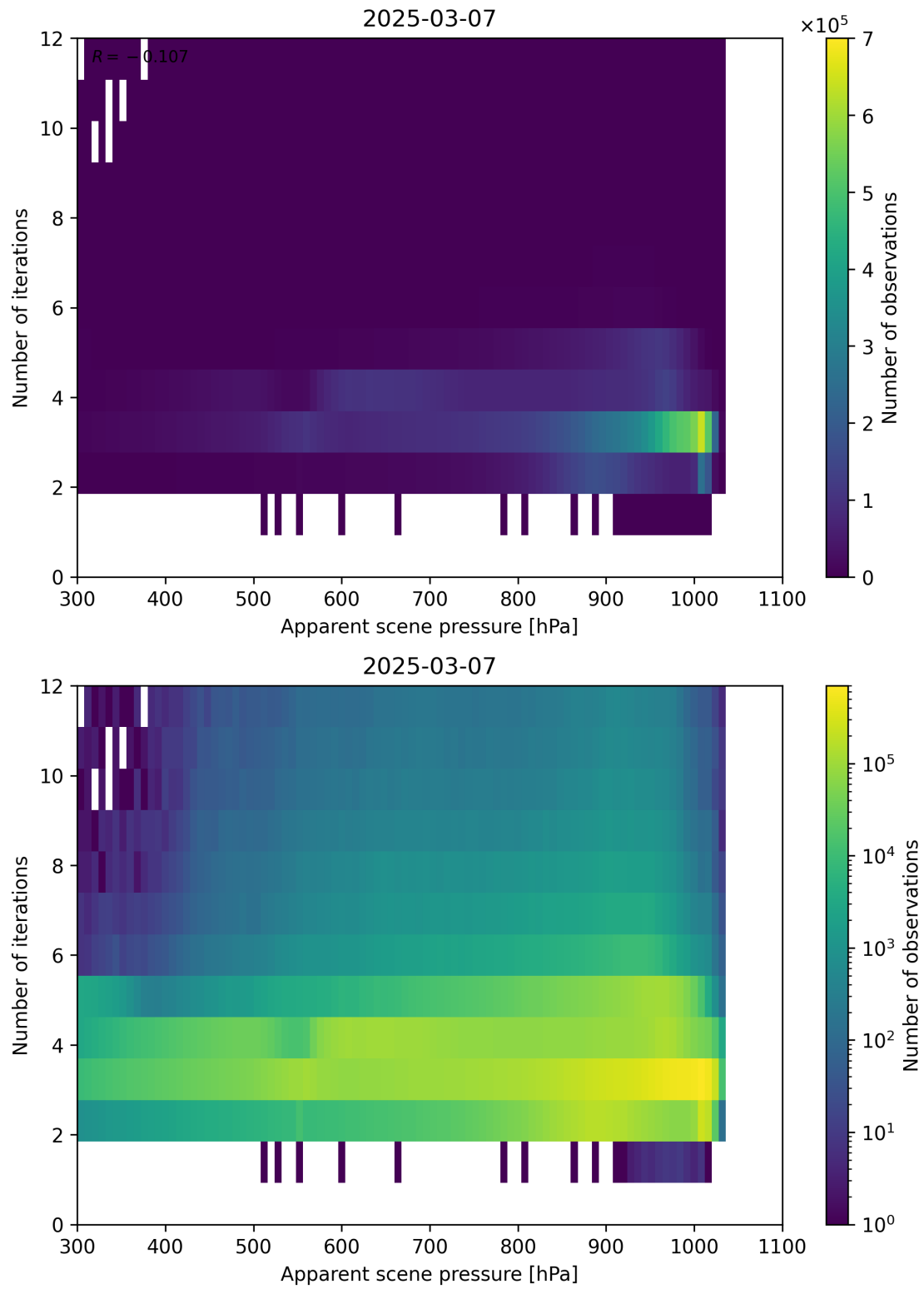
Figure 65: Scatter density plot of “Apparent scene pressure” against “Number of iterations” for 2025-03-07 to 2025-03-08.
