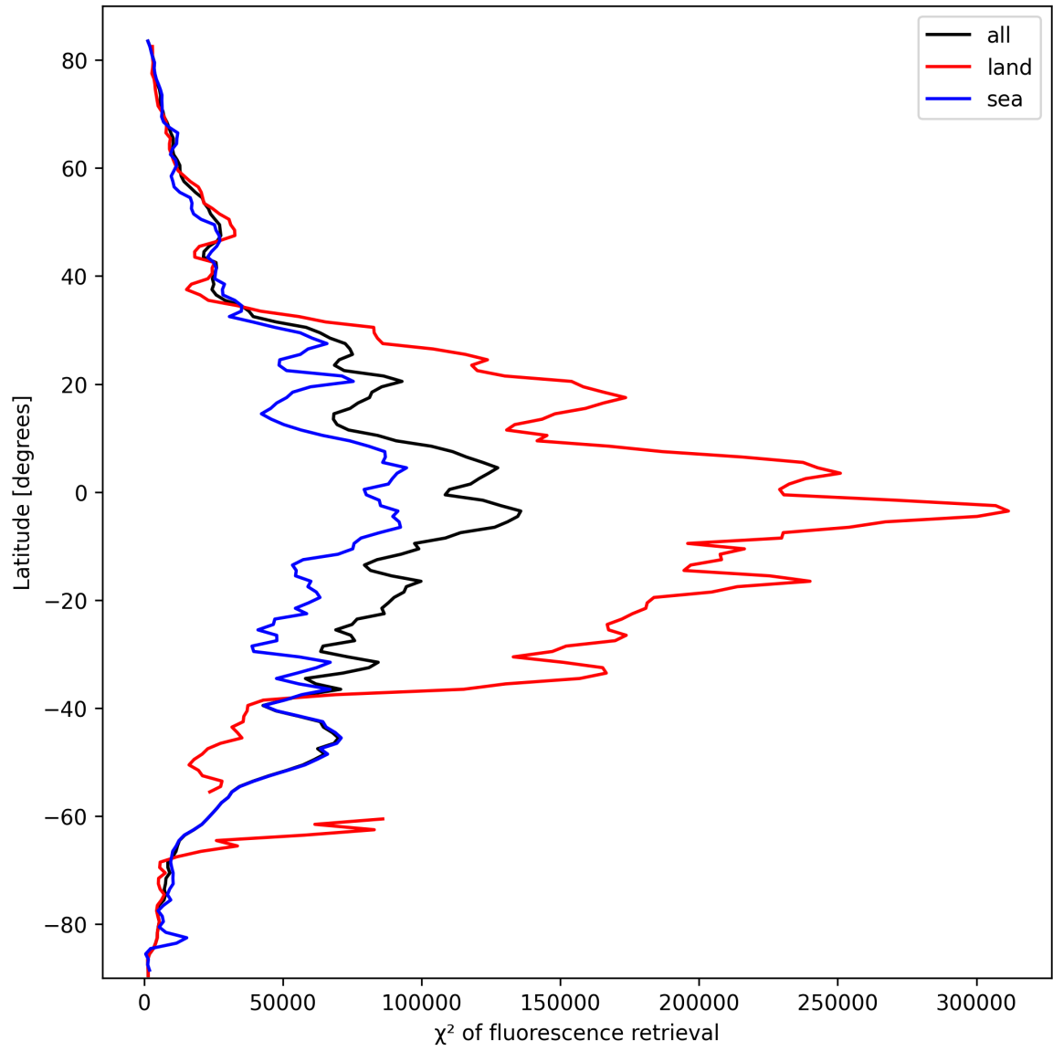
Figure 25: Zonal average of “ \chi^2 of fluorescence retrieval” for 2025-03-07 to 2025-03-08.
