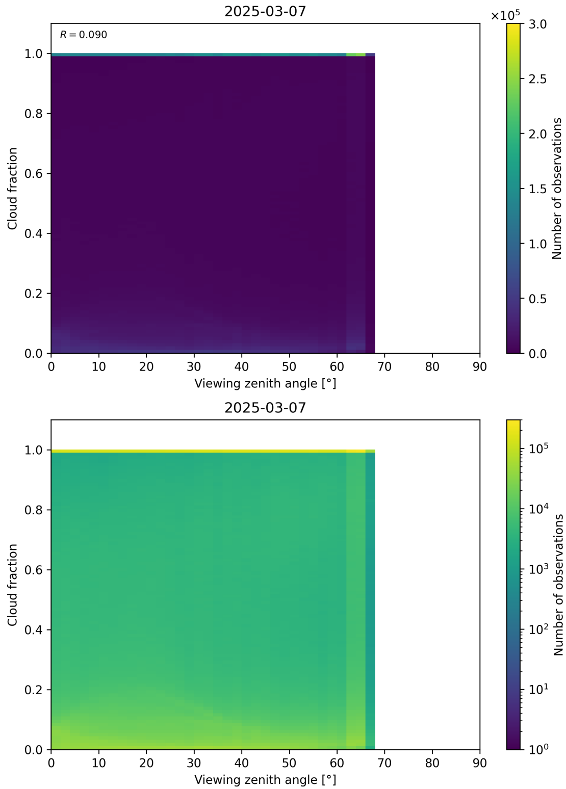
Figure 120: Scatter density plot of “Viewing zenith angle” against “Cloud fraction” for 2025-03-07 to 2025-03-08.
