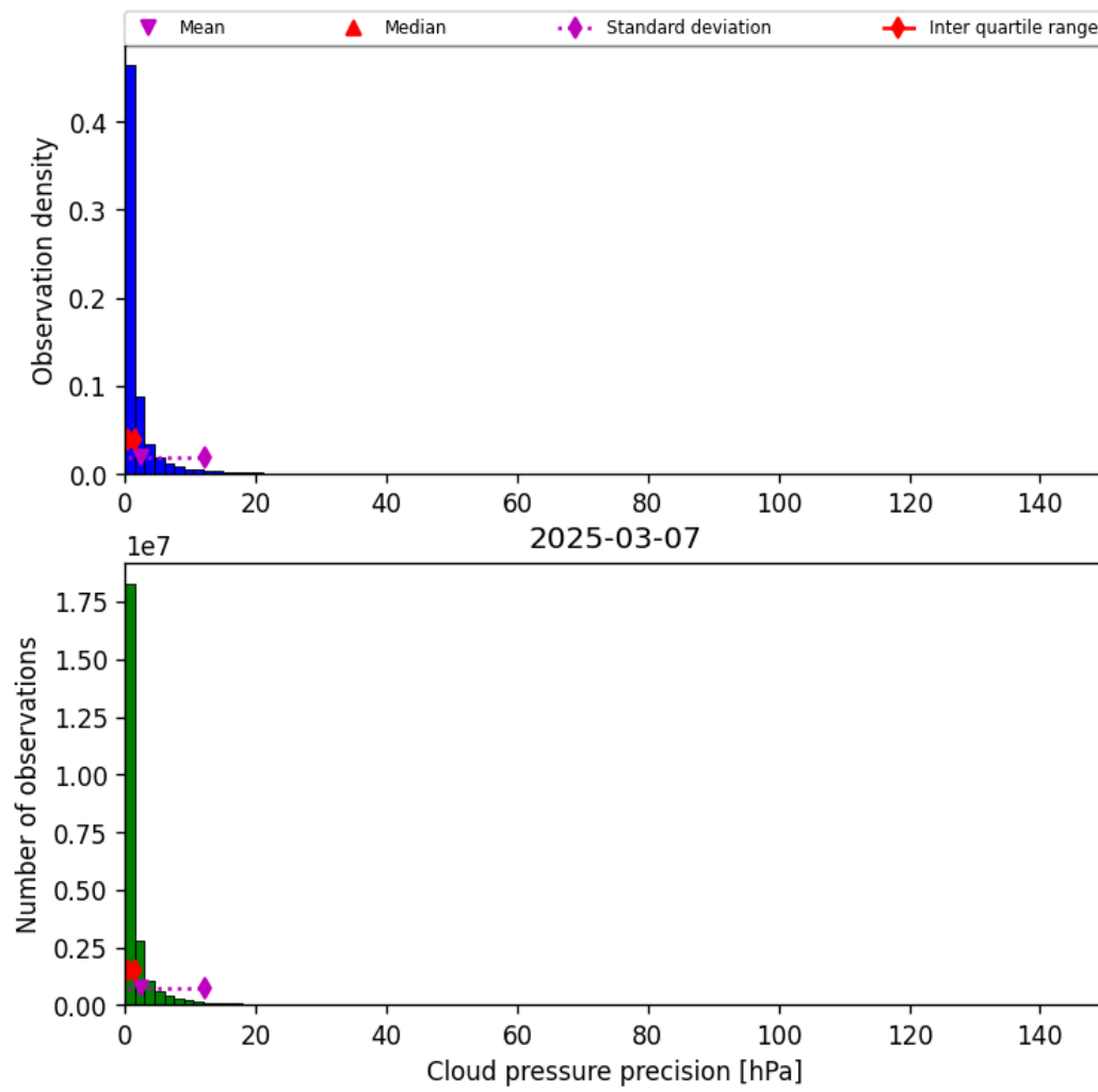
Figure 31: Histogram of “Cloud pressure precision” for 2025-03-07 to 2025-03-08
