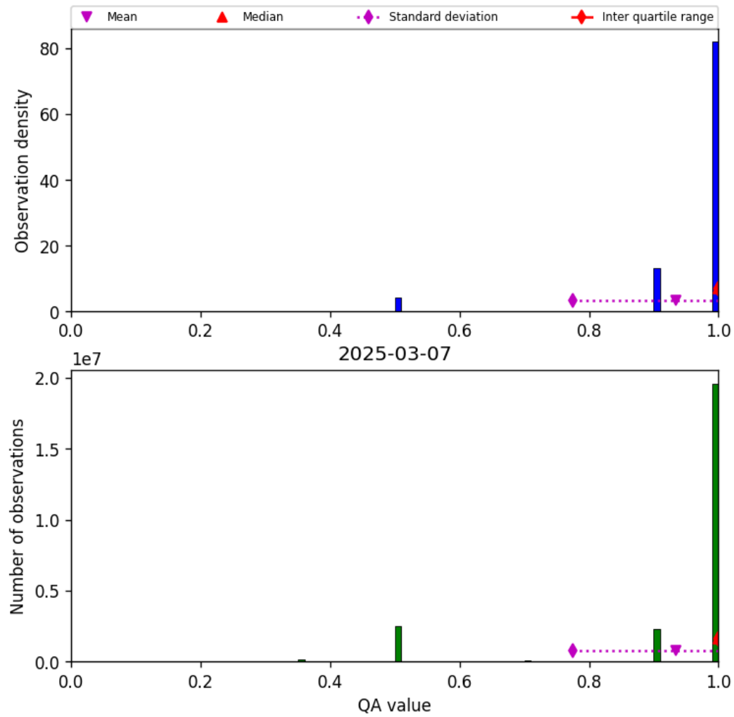
Figure 29: Histogram of “QA value” for 2025-03-07 to 2025-03-08
