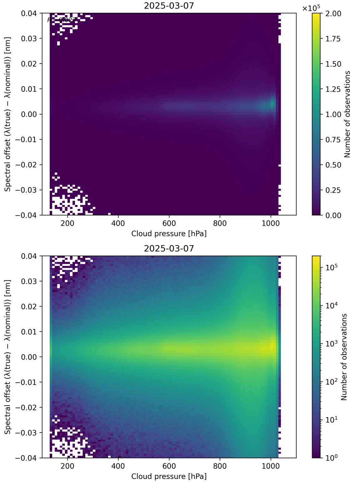
Figure 84: Scatter density plot of “Cloud pressure” against “Spectral offset ( \lambda_{\text{true}} - \lambda_{\text{nominal}} )” for 2025-03-07 to 2025-03-08.
