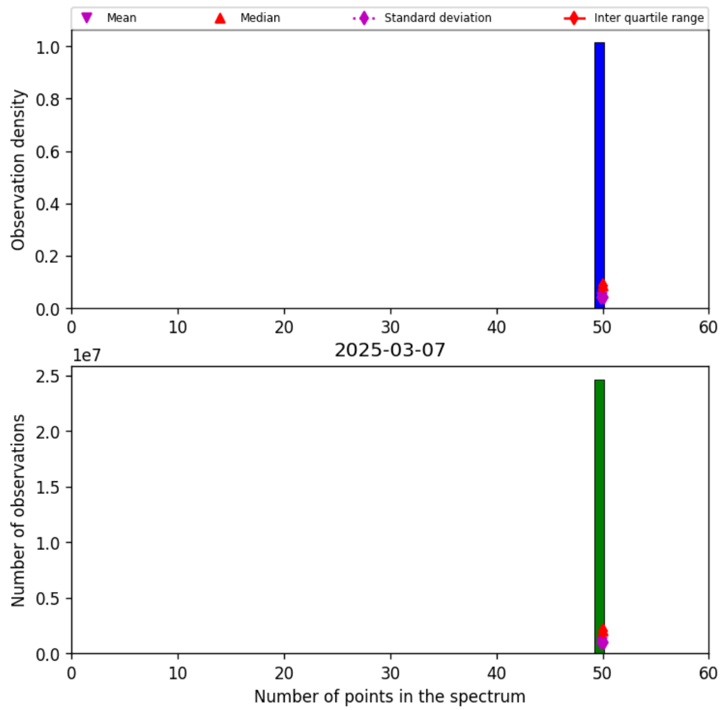
Figure 44: Histogram of “Number of points in the spectrum” for 2025-03-07 to 2025-03-08
