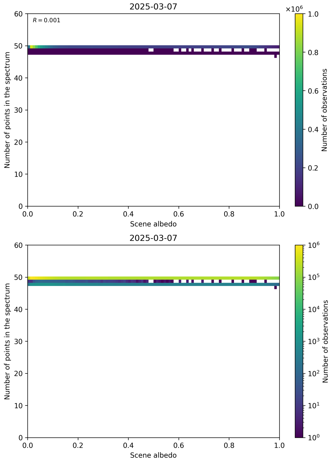
Figure 106: Scatter density plot of “Scene albedo” against “Number of points in the spectrum” for 2025-03-07 to 2025-03-08.
