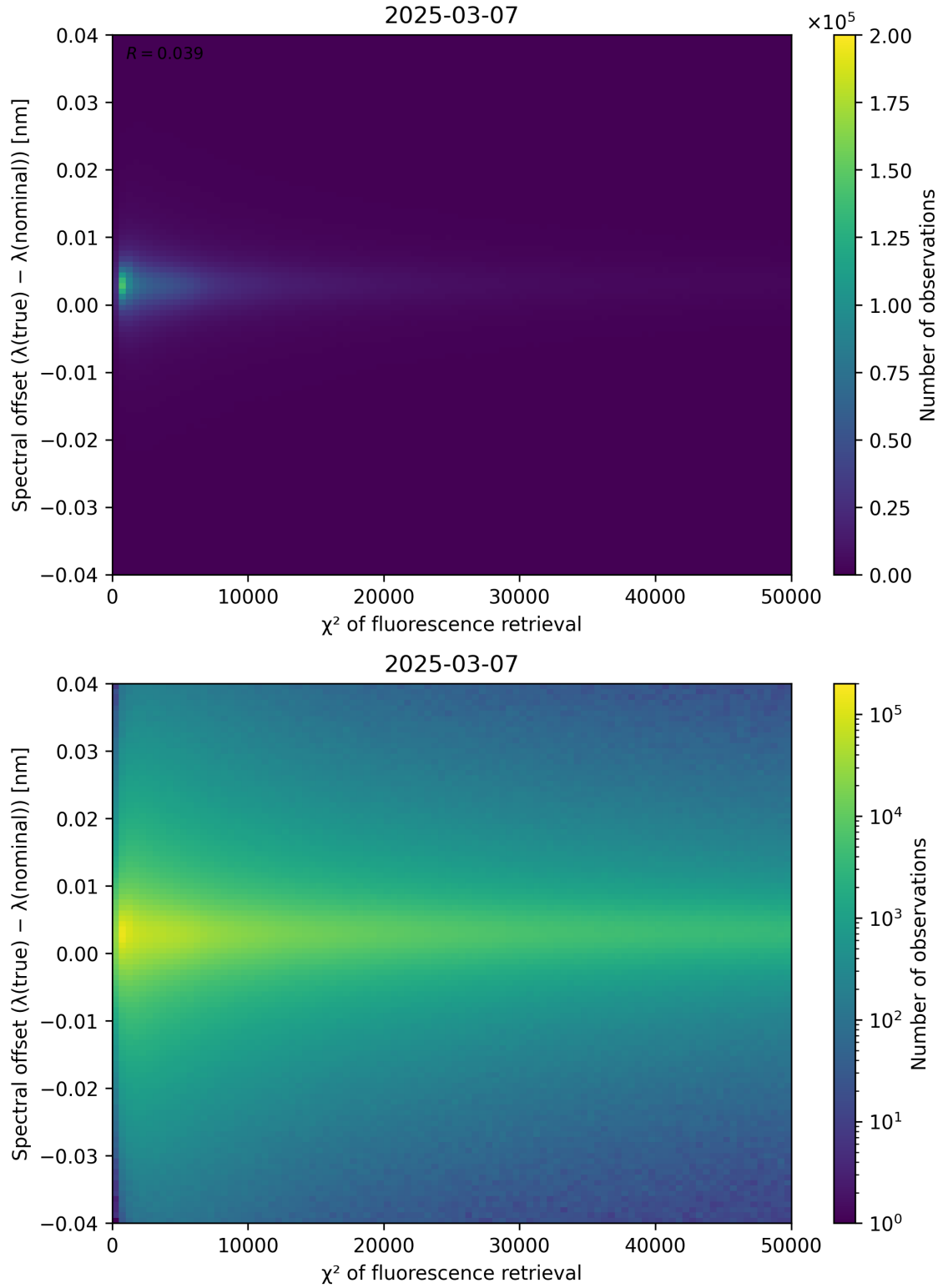
Figure 69: Scatter density plot of “ \chi^2 of fluorescence retrieval” against “Spectral offset ( \lambda_{\text{true}} - \lambda_{\text{nominal}} )” for 2025-03-07 to 2025-03-08.
