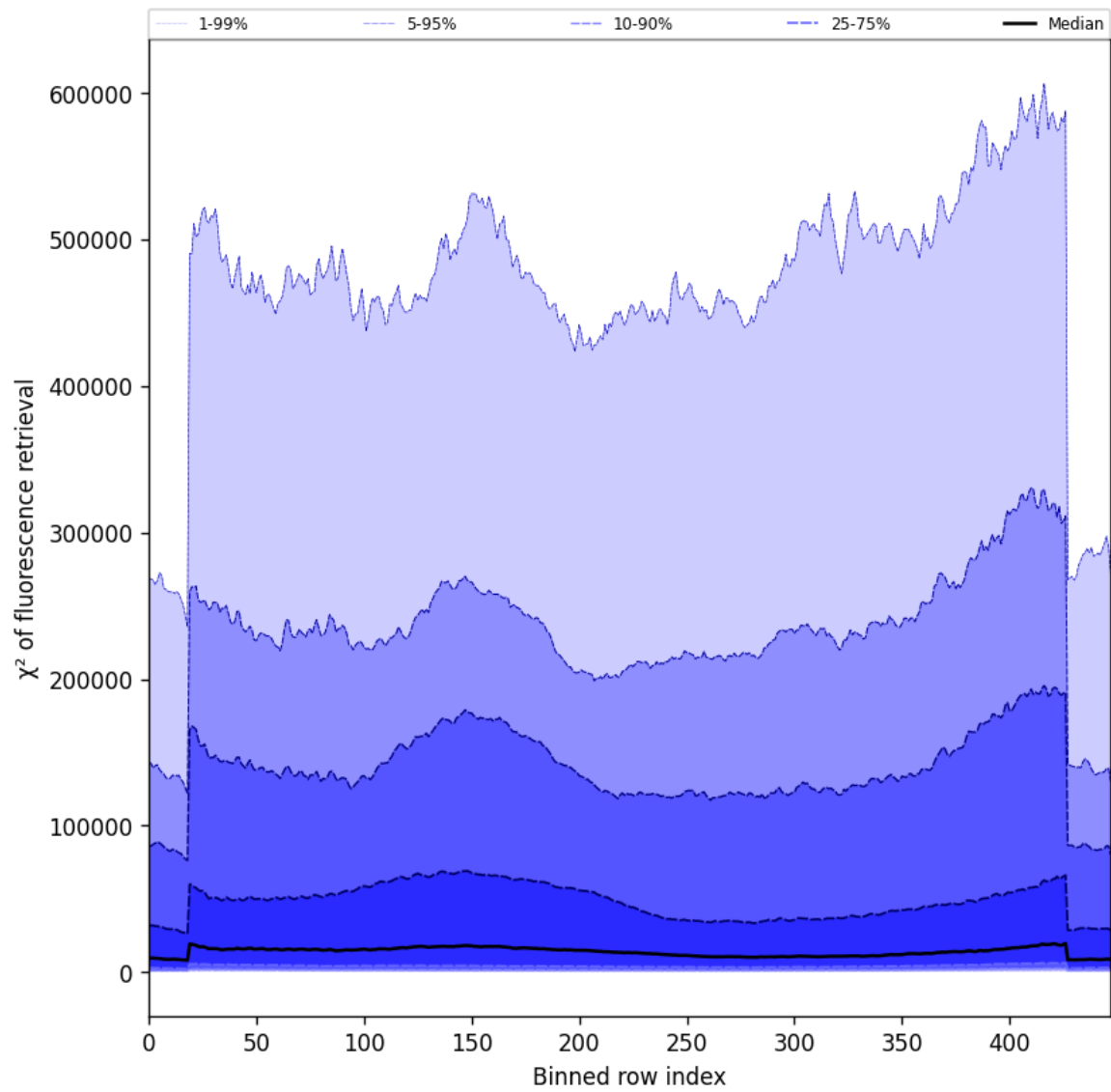
Figure 59: Along track statistics of “ \chi^2 of fluorescence retrieval” for 2025-03-07 to 2025-03-08
