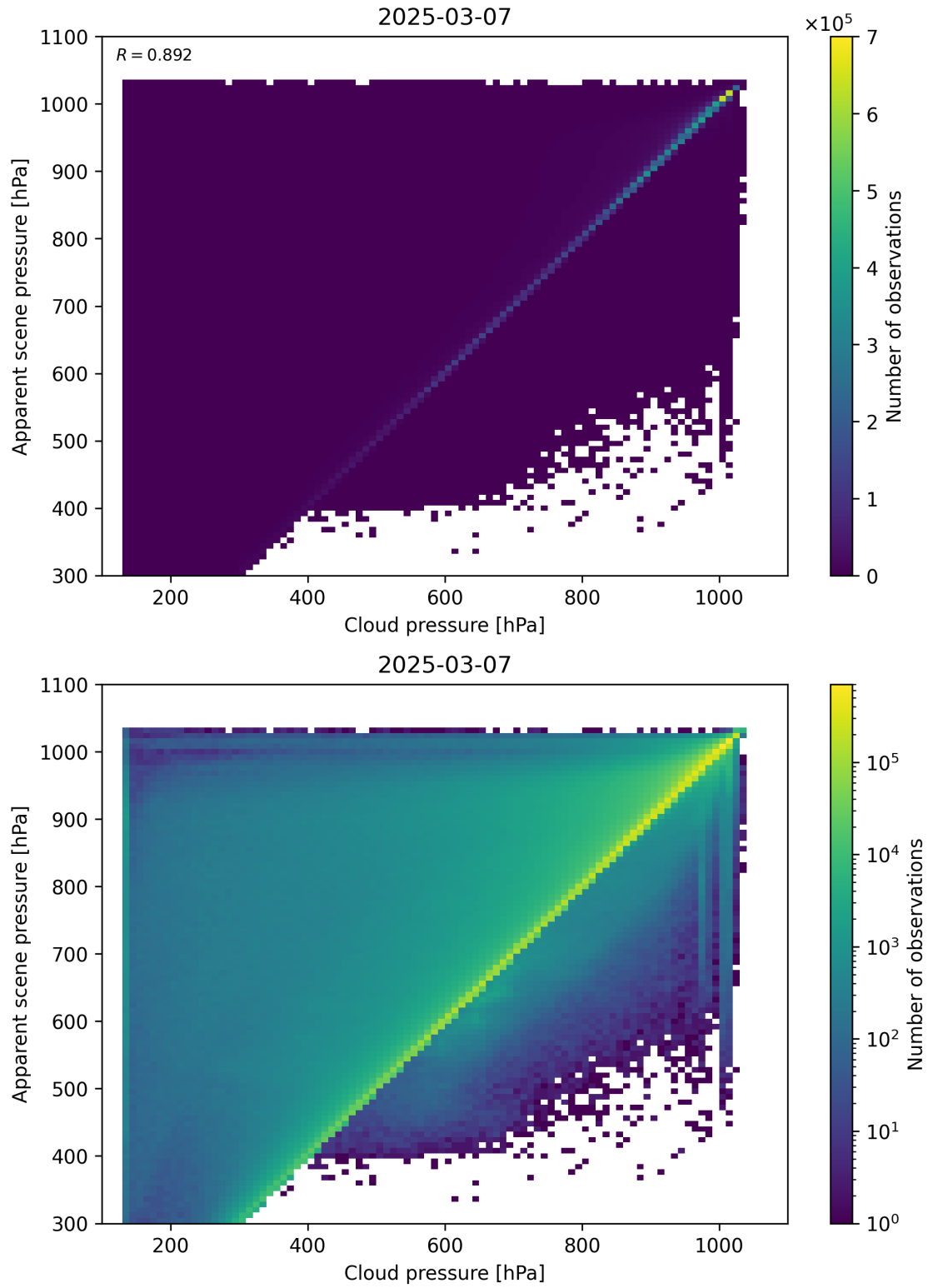
Figure 77: Scatter density plot of “Cloud pressure” against “Apparent scene pressure” for 2025-03-07 to 2025-03-08.
