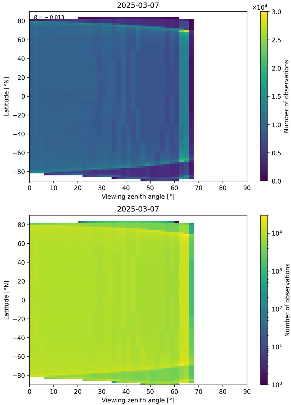
Figure 123: Scatter density plot of “Viewing zenith angle” against “Latitude” for 2025-03-07 to 2025-03-08.
