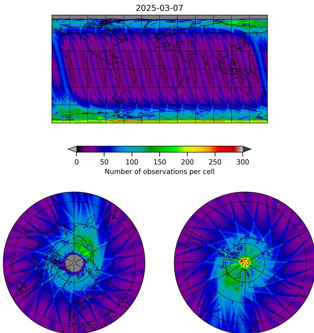
Figure 11: Map of the number of observations for 2025-03-07 to 2025-03-08
