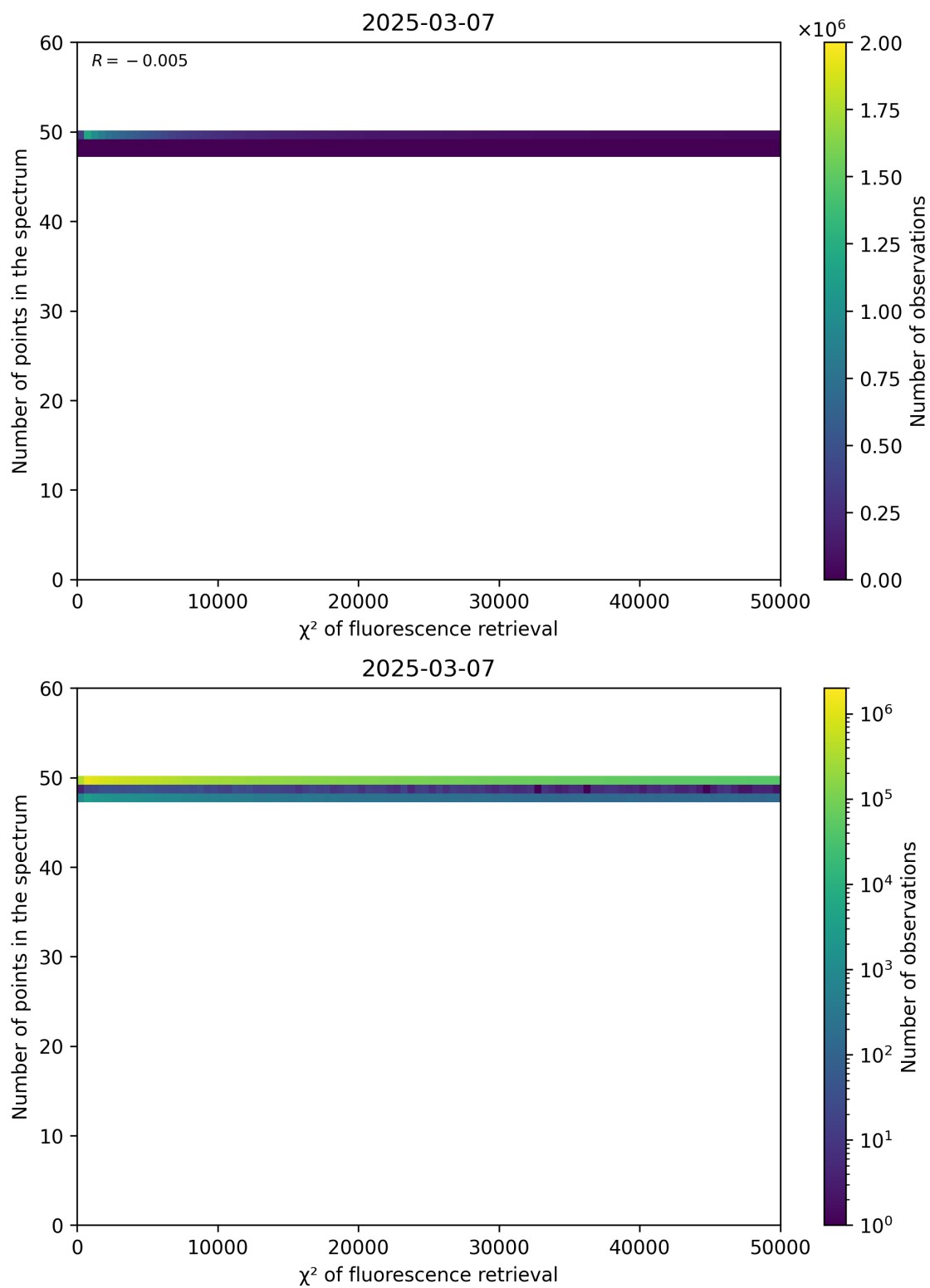
Figure 68: Scatter density plot of “ \chi^2 of fluorescence retrieval” against “Number of points in the spectrum” for 2025-03-07 to 2025-03-08.
