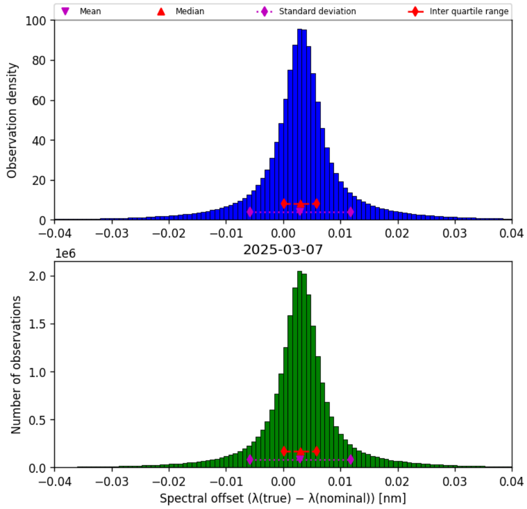
Figure 45: Histogram of “Spectral offset ( \lambda_{\text{true}} - \lambda_{\text{nominal}} )” for 2025-03-07 to 2025-03-08
