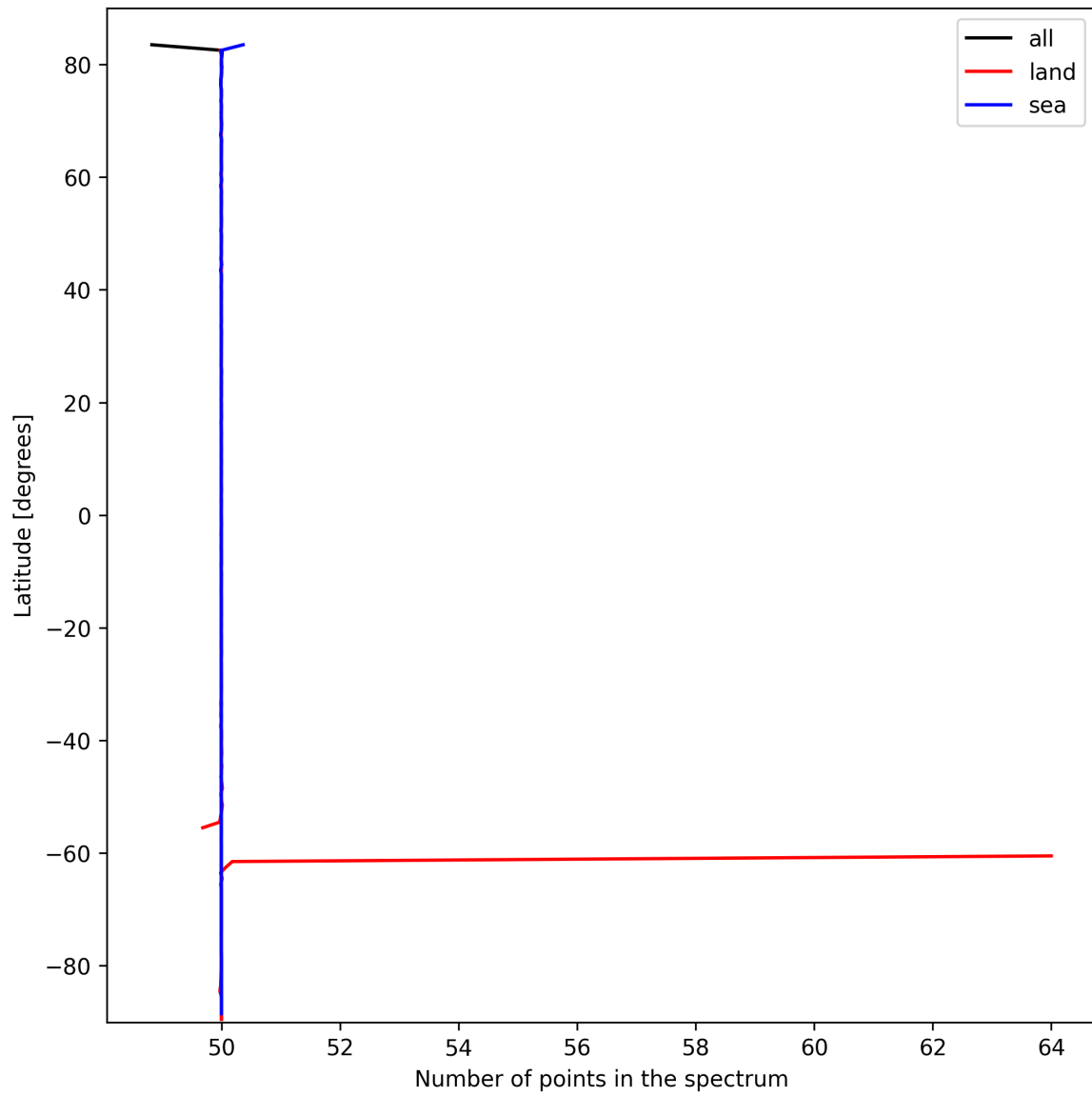
Figure 27: Zonal average of “Number of points in the spectrum” for 2025-03-07 to 2025-03-08.
