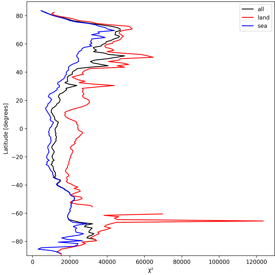
Figure 21: Zonal average of “ \chi^2 ” for 2025-03-07 to 2025-03-08.
