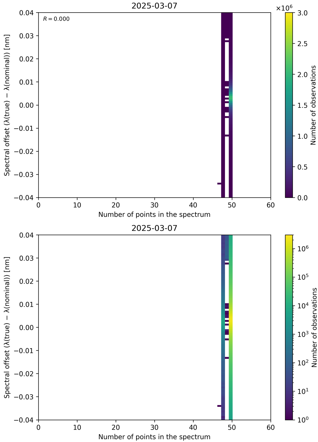
Figure 101: Scatter density plot of “Number of points in the spectrum” against “Spectral offset ( \lambda_{\text{true}} - \lambda_{\text{nominal}} )” for 2025-03-07 to 2025-03-08.
