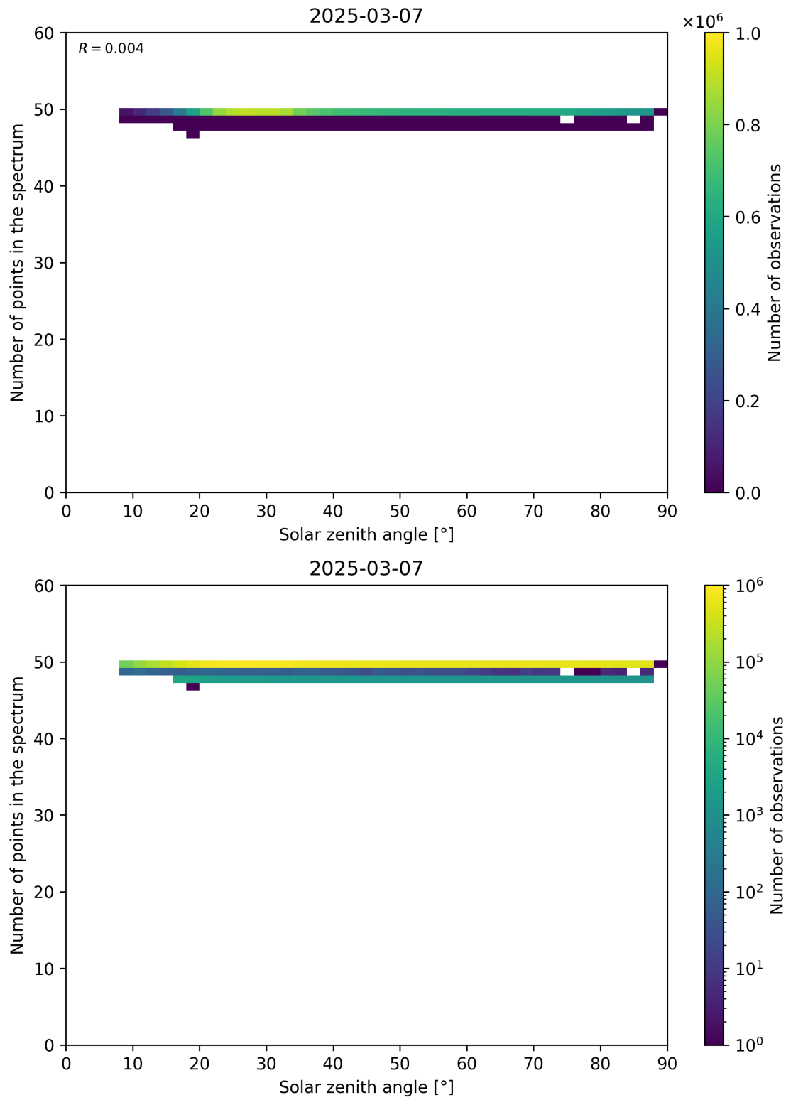
Figure 115: Scatter density plot of “Solar zenith angle” against “Number of points in the spectrum” for 2025-03-07 to 2025-03-08.
