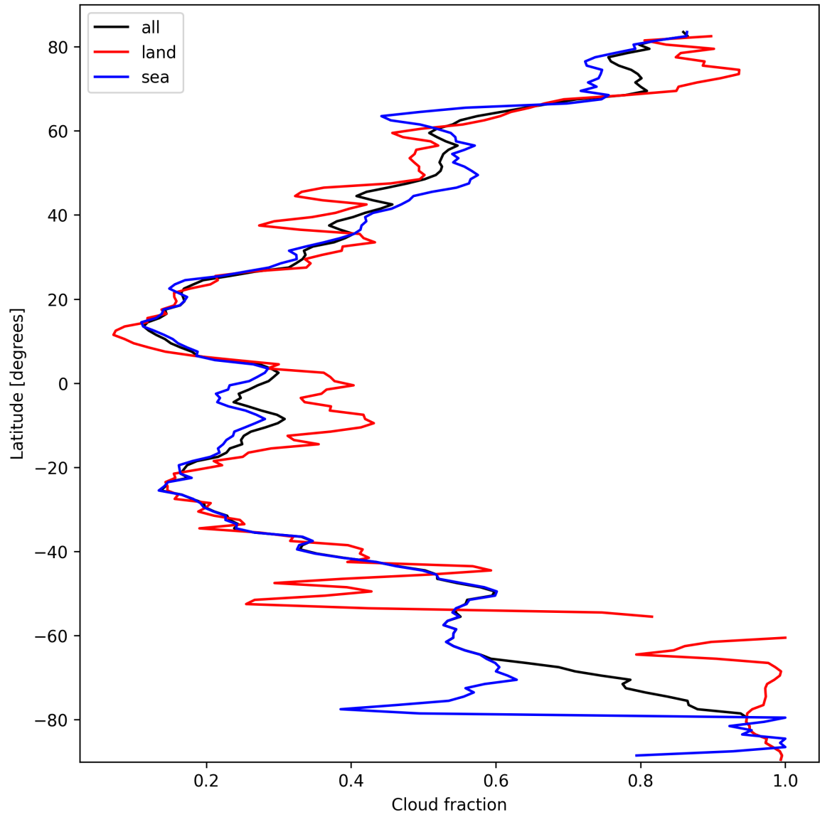
Figure 15: Zonal average of “Cloud fraction” for 2025-03-07 to 2025-03-08.
