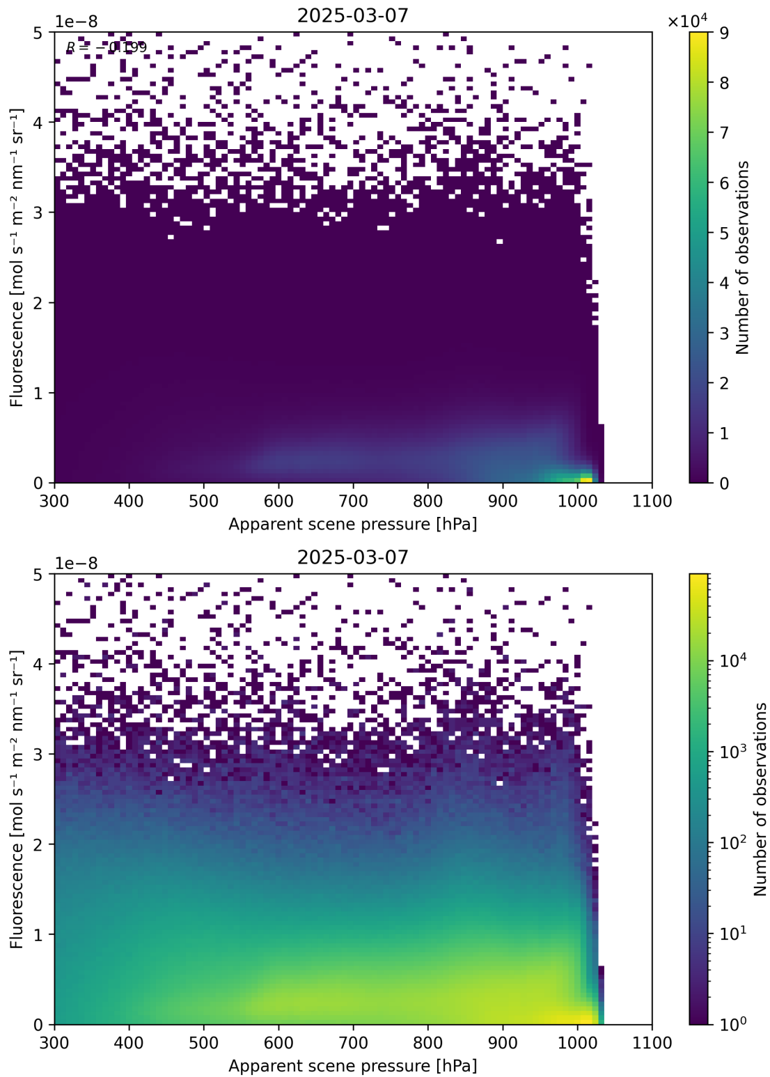
Figure 64: Scatter density plot of “Apparent scene pressure” against “Fluorescence” for 2025-03-07 to 2025-03-08.
