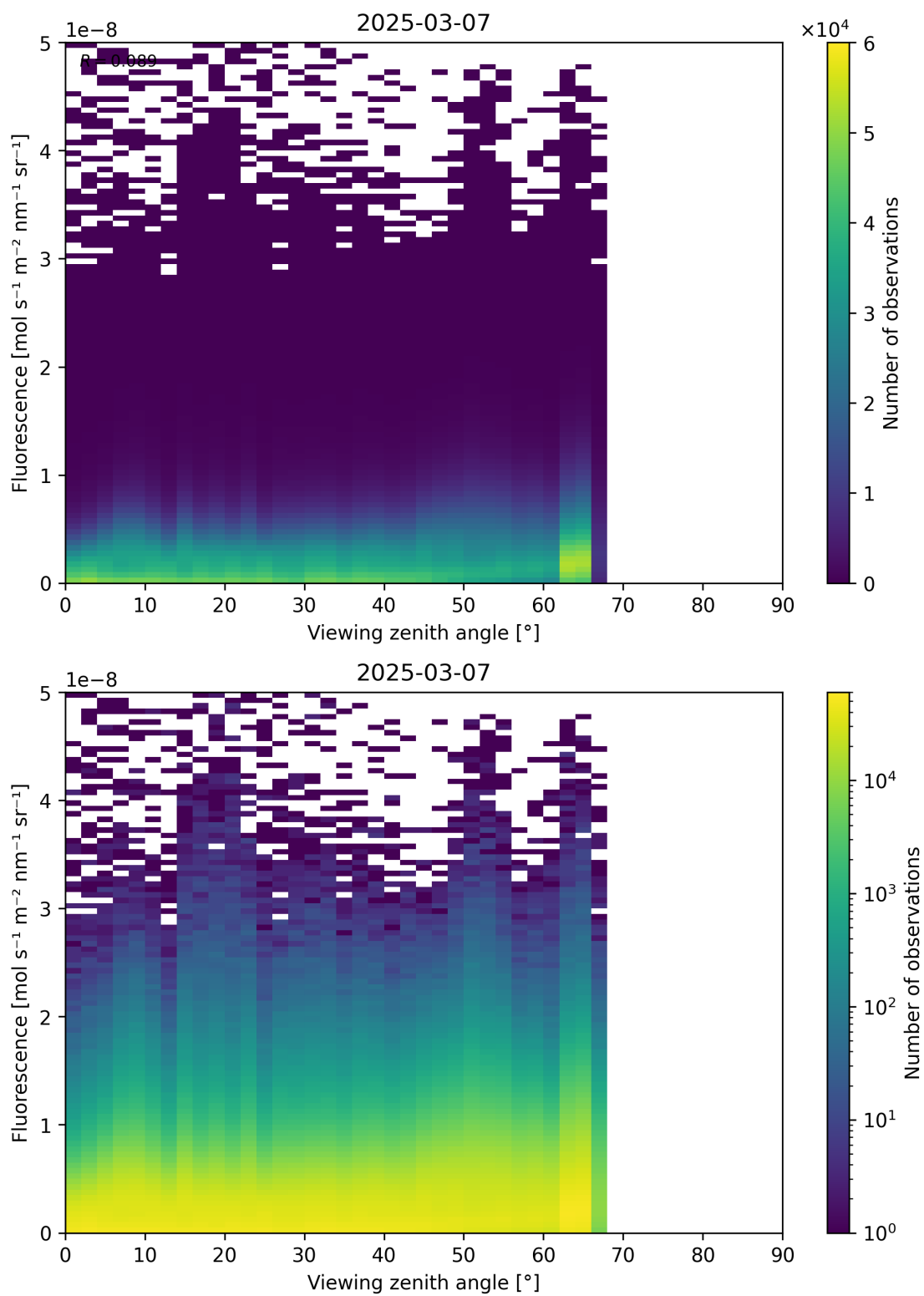
Figure 122: Scatter density plot of “Viewing zenith angle” against “Fluorescence” for 2025-03-07 to 2025-03-08.
