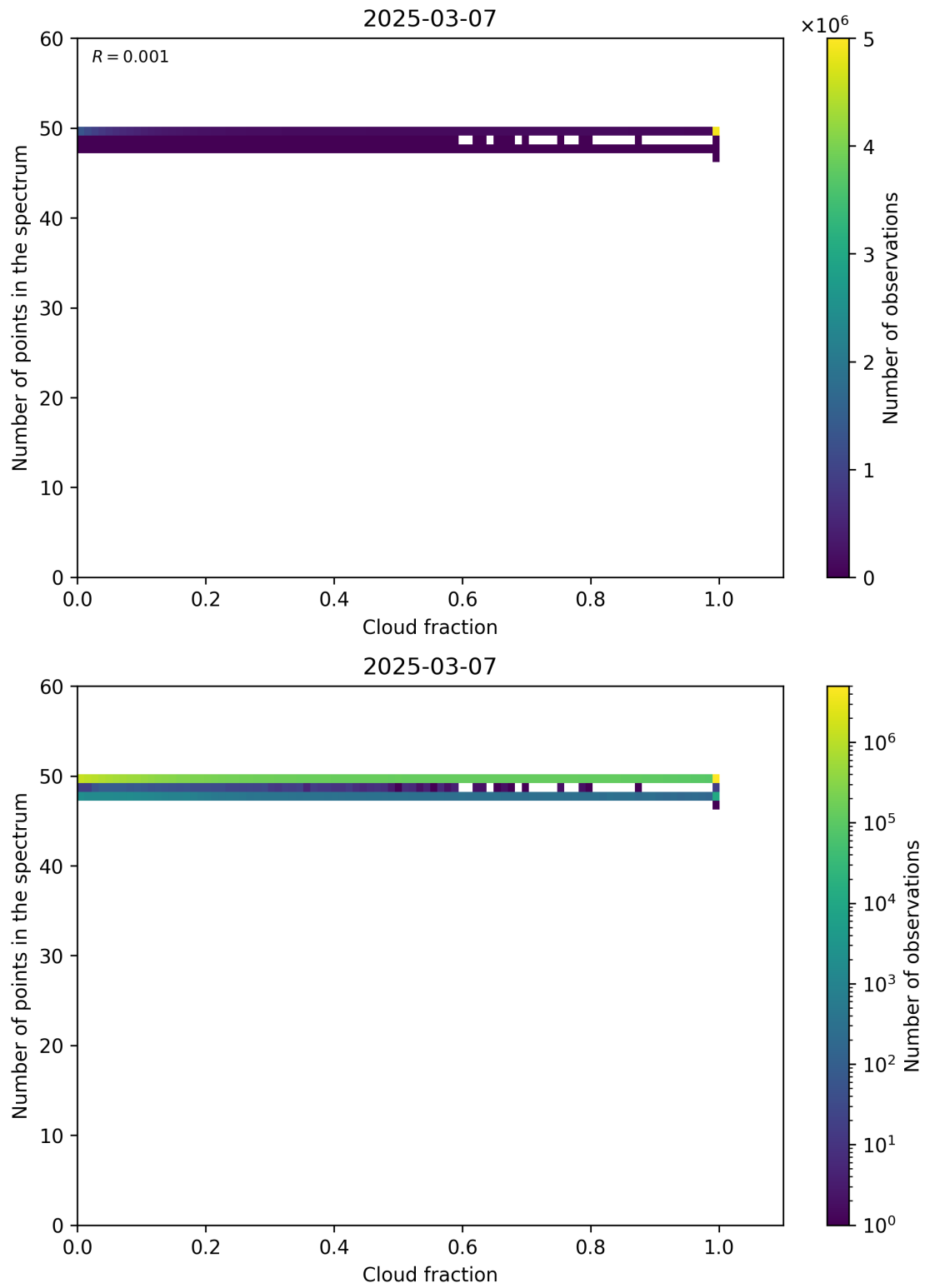
Figure 74: Scatter density plot of “Cloud fraction” against “Number of points in the spectrum” for 2025-03-07 to 2025-03-08.
