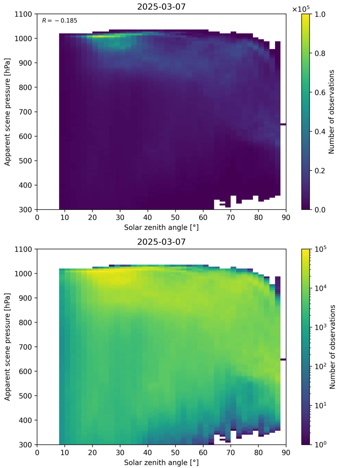
Figure 108: Scatter density plot of “Solar zenith angle” against “Apparent scene pressure” for 2025-03-07 to 2025-03-08.
