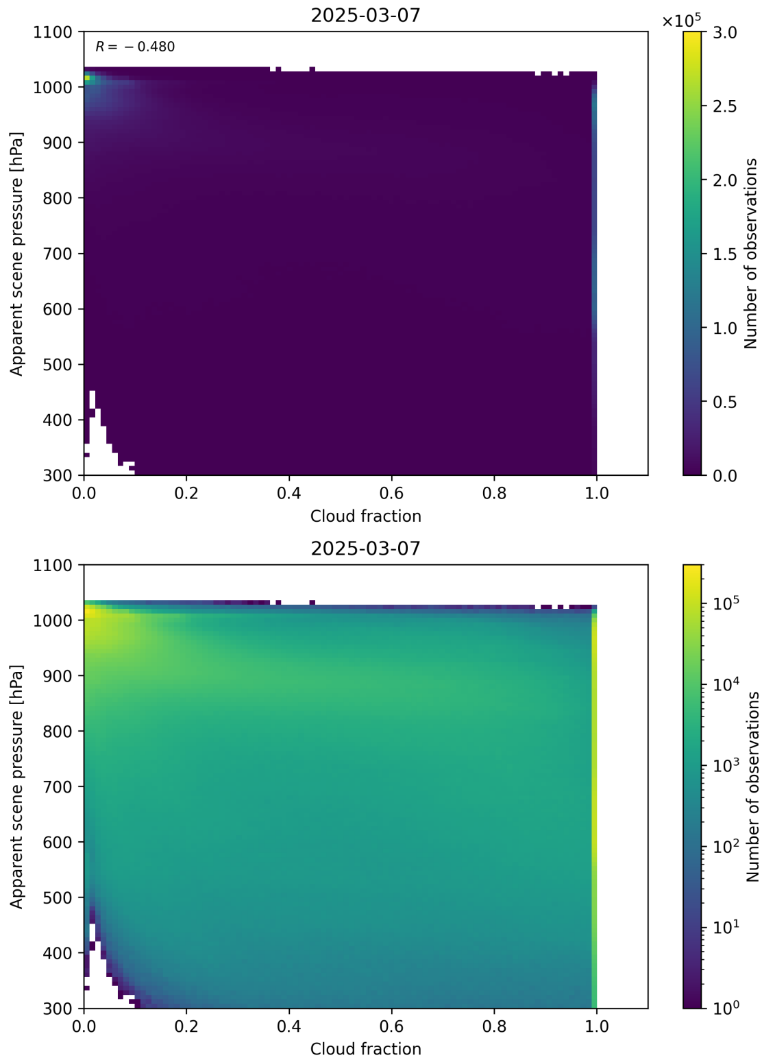
Figure 70: Scatter density plot of “Cloud fraction” against “Apparent scene pressure” for 2025-03-07 to 2025-03-08.
