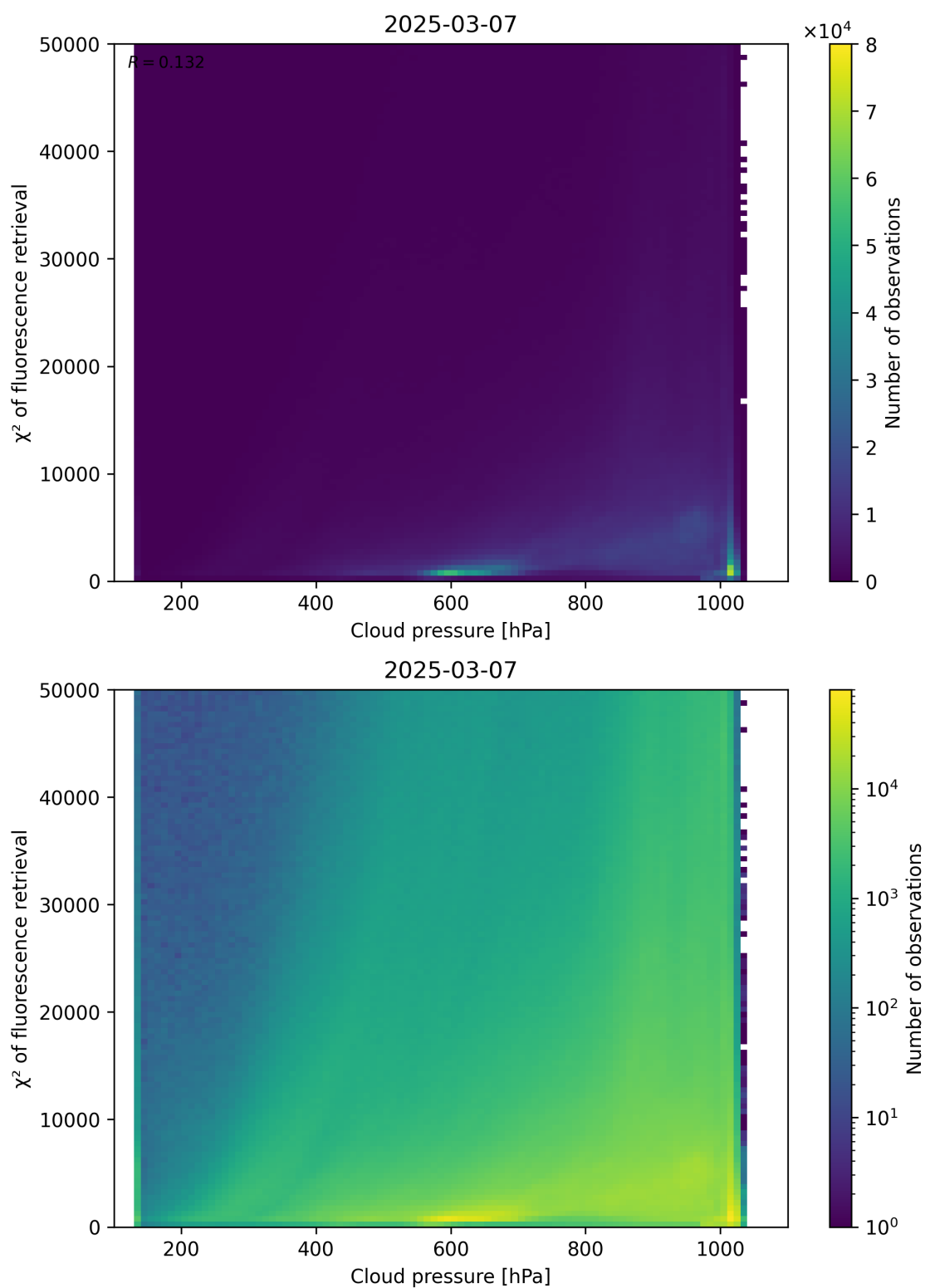
Figure 78: Scatter density plot of “Cloud pressure” against “ \chi^2 of fluorescence retrieval” for 2025-03-07 to 2025-03-08.
