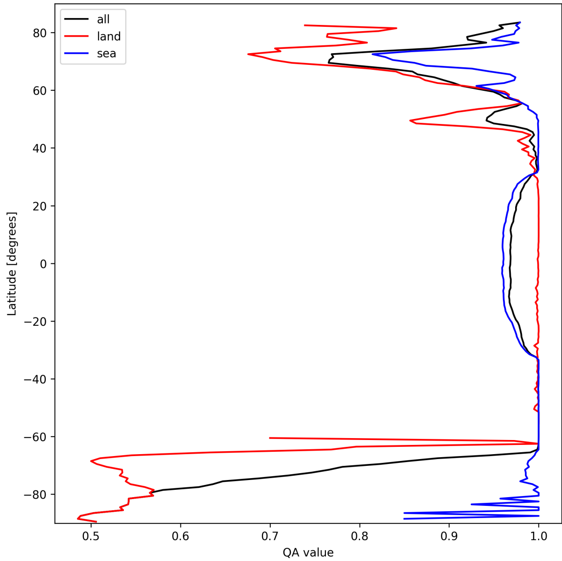
Figure 12: Zonal average of “QA value” for 2025-03-07 to 2025-03-08.
