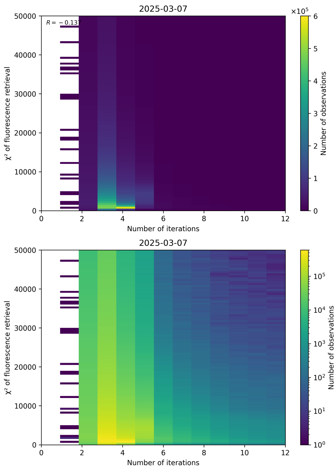
Figure 97: Scatter density plot of “Number of iterations” against “ \chi^2 of fluorescence retrieval” for 2025-03-07 to 2025-03-08.
