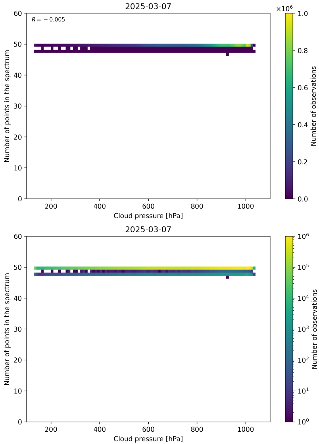
Figure 82: Scatter density plot of “Cloud pressure” against “Number of points in the spectrum” for 2025-03-07 to 2025-03-08.
