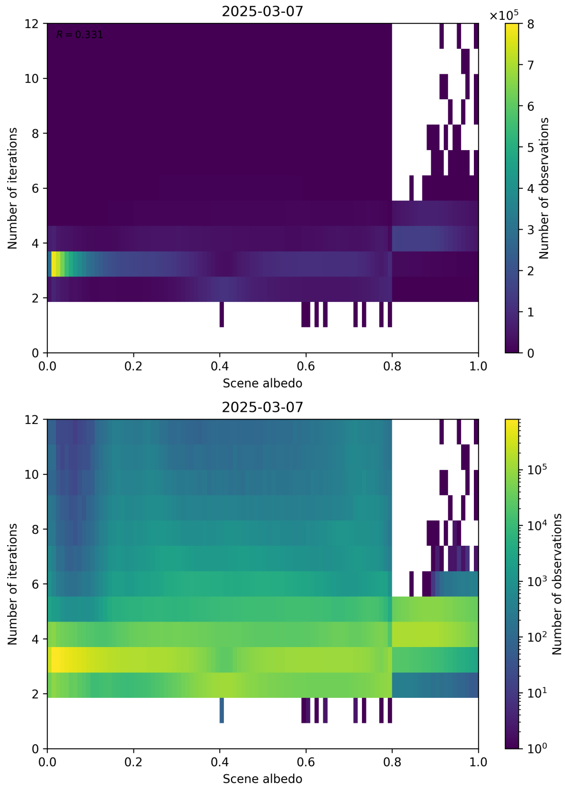
Figure 105: Scatter density plot of “Scene albedo” against “Number of iterations” for 2025-03-07 to 2025-03-08.
