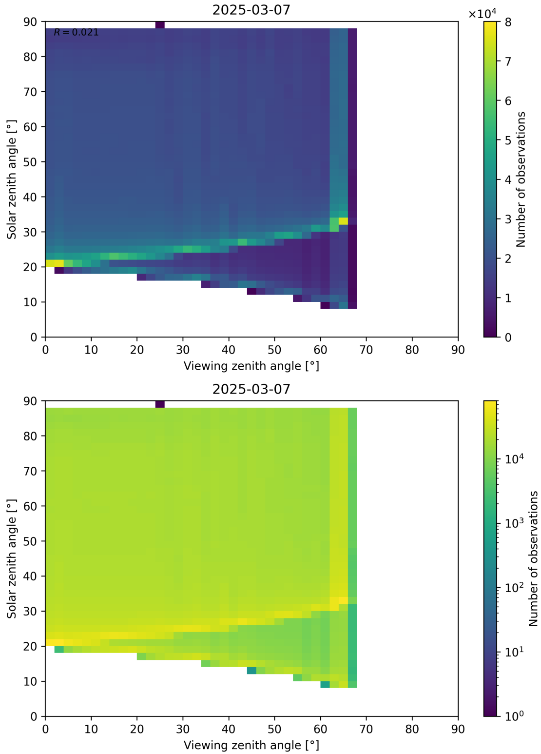
Figure 127: Scatter density plot of “Viewing zenith angle” against “Solar zenith angle” for 2025-03-07 to 2025-03-08.
