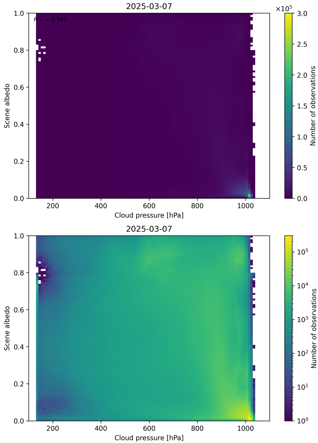
Figure 83: Scatter density plot of “Cloud pressure” against “Scene albedo” for 2025-03-07 to 2025-03-08.
