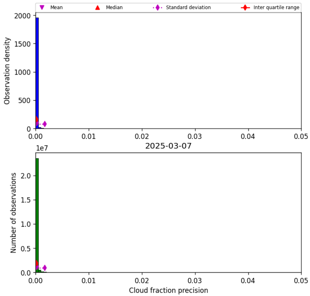
Figure 33: Histogram of “Cloud fraction precision” for 2025-03-07 to 2025-03-08
