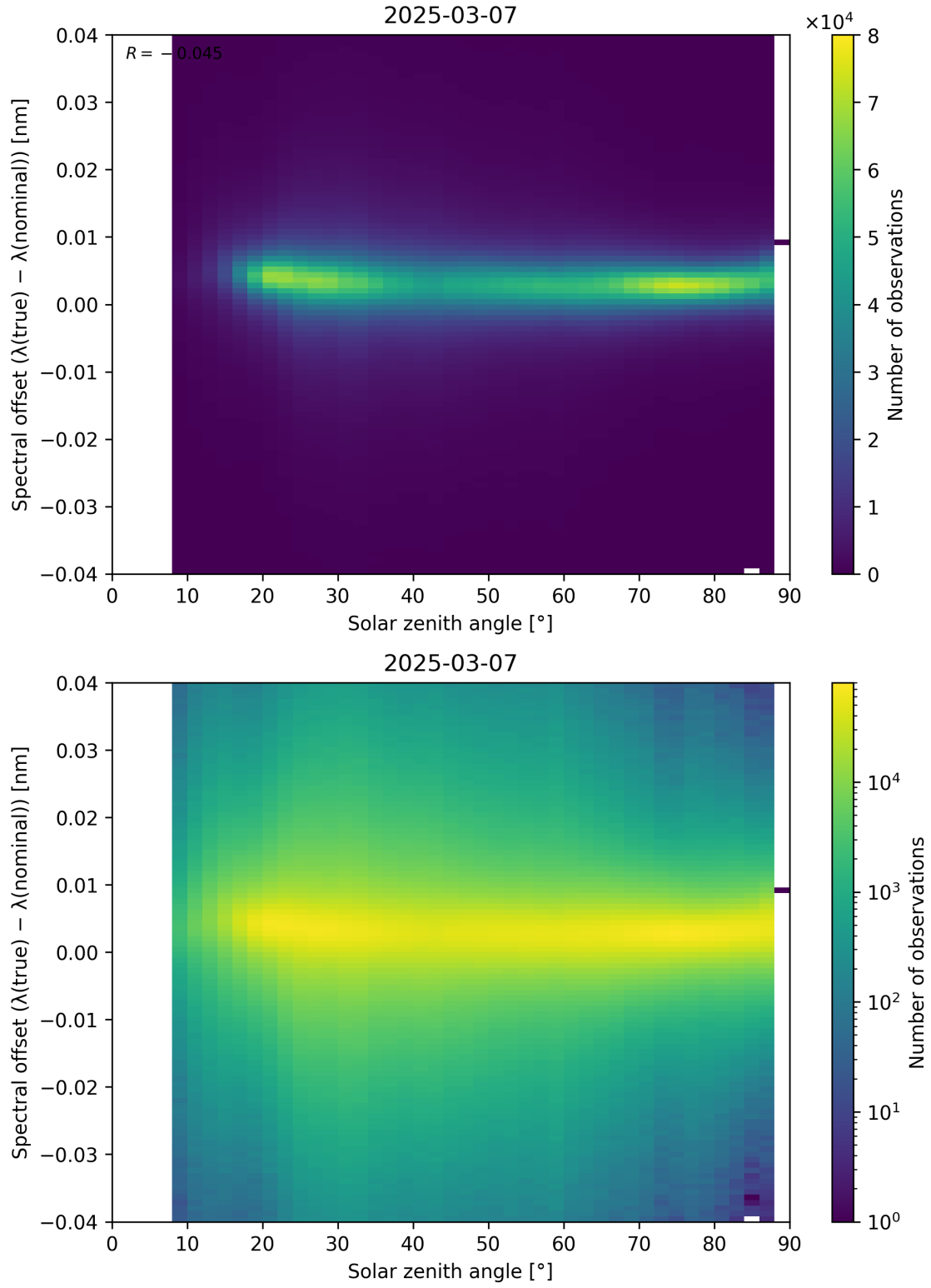
Figure 117: Scatter density plot of “Solar zenith angle” against “Spectral offset ( \lambda_{\text{true}} - \lambda_{\text{nominal}} )” for 2025-03-07 to 2025-03-08.
