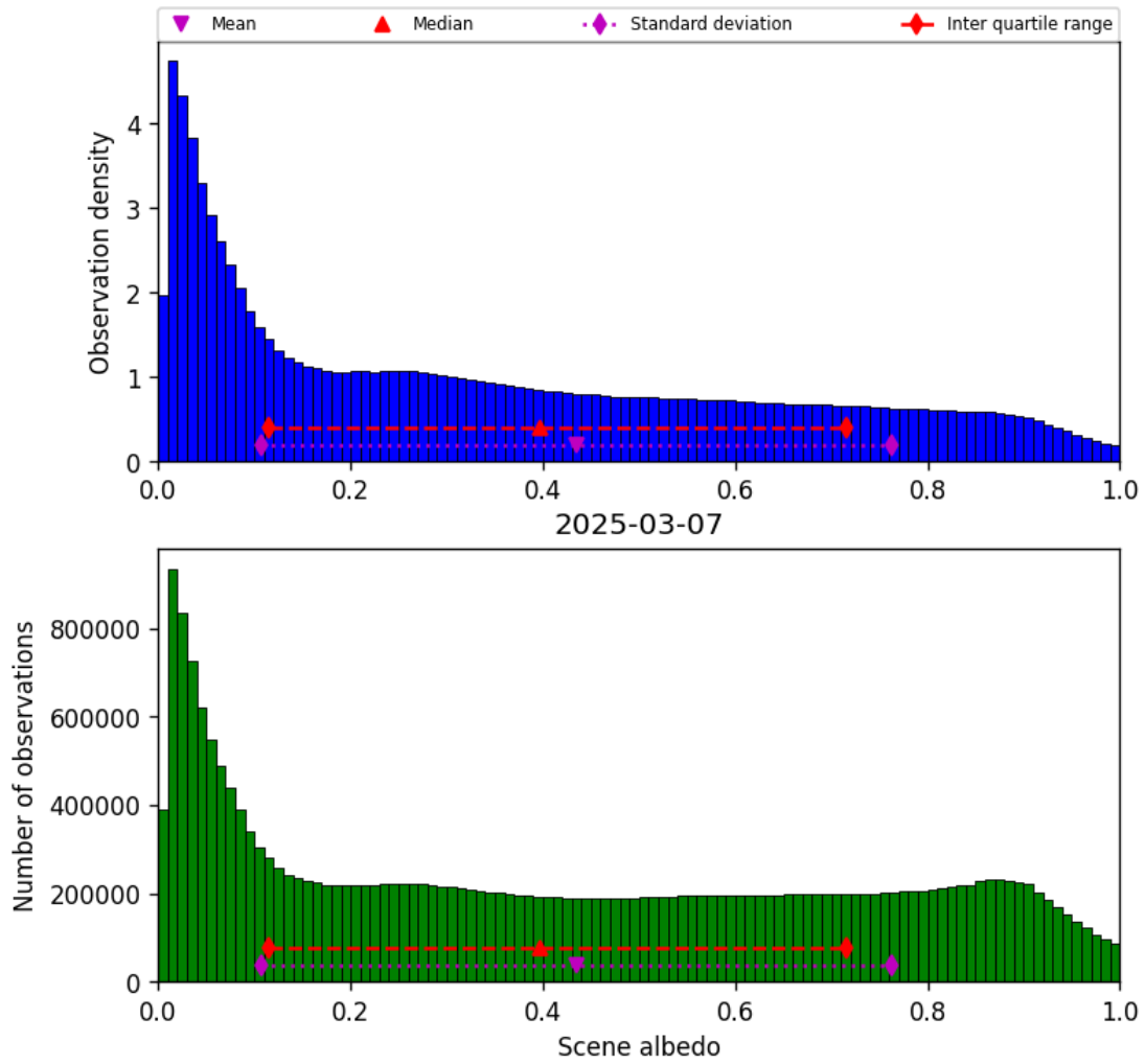
Figure 34: Histogram of “Scene albedo” for 2025-03-07 to 2025-03-08
