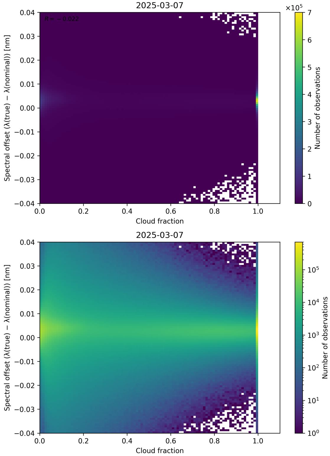
Figure 76: Scatter density plot of “Cloud fraction” against “Spectral offset ( \lambda_{\text{true}} - \lambda_{\text{nominal}} )” for 2025-03-07 to 2025-03-08.
