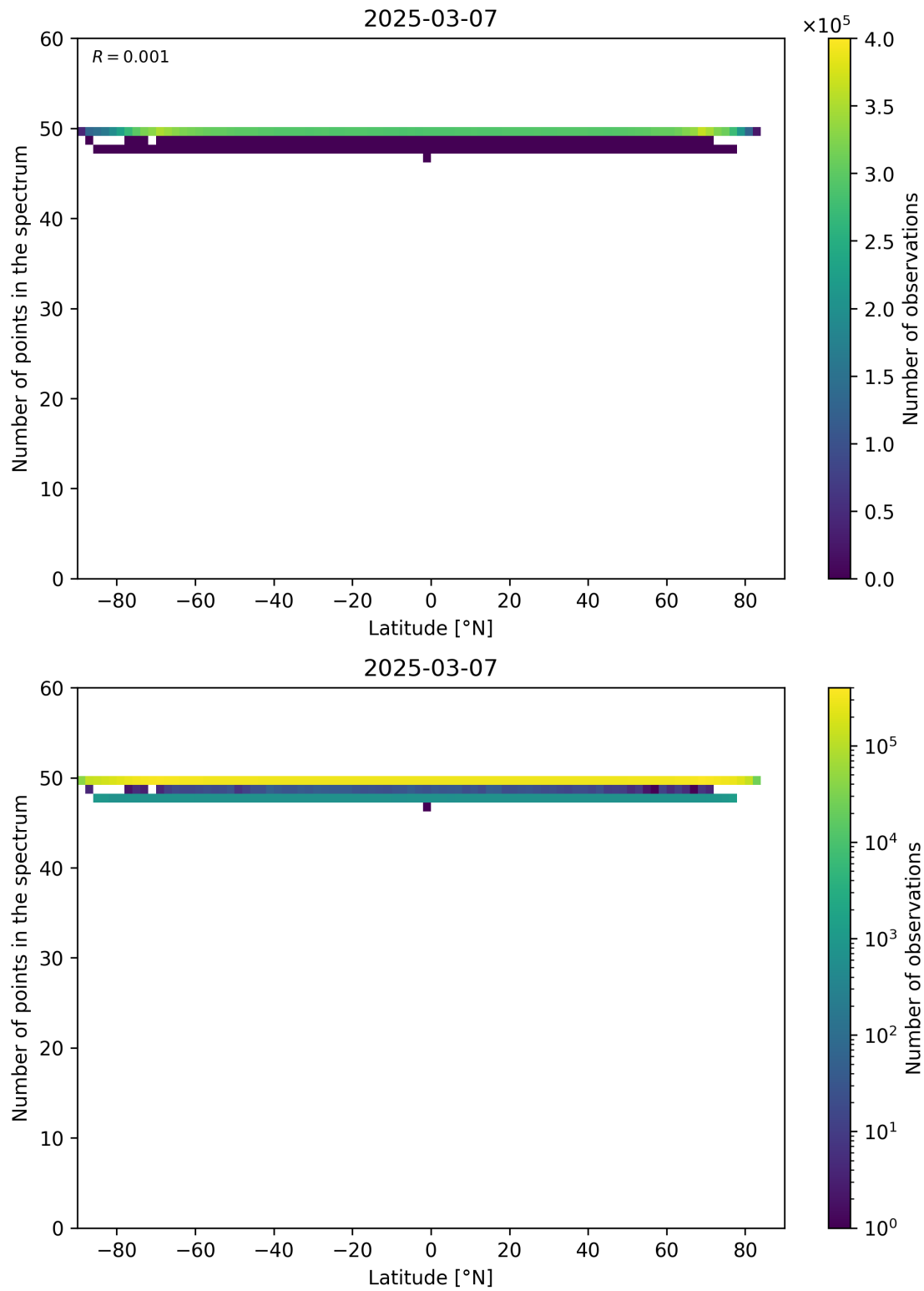
Figure 94: Scatter density plot of “Latitude” against “Number of points in the spectrum” for 2025-03-07 to 2025-03-08.
