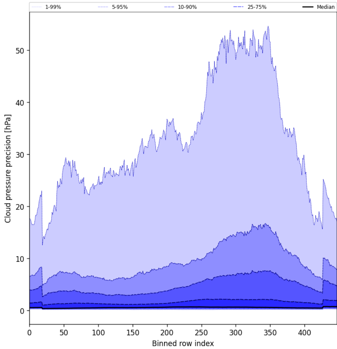
Figure 48: Along track statistics of “Cloud pressure precision” for 2025-03-07 to 2025-03-08
