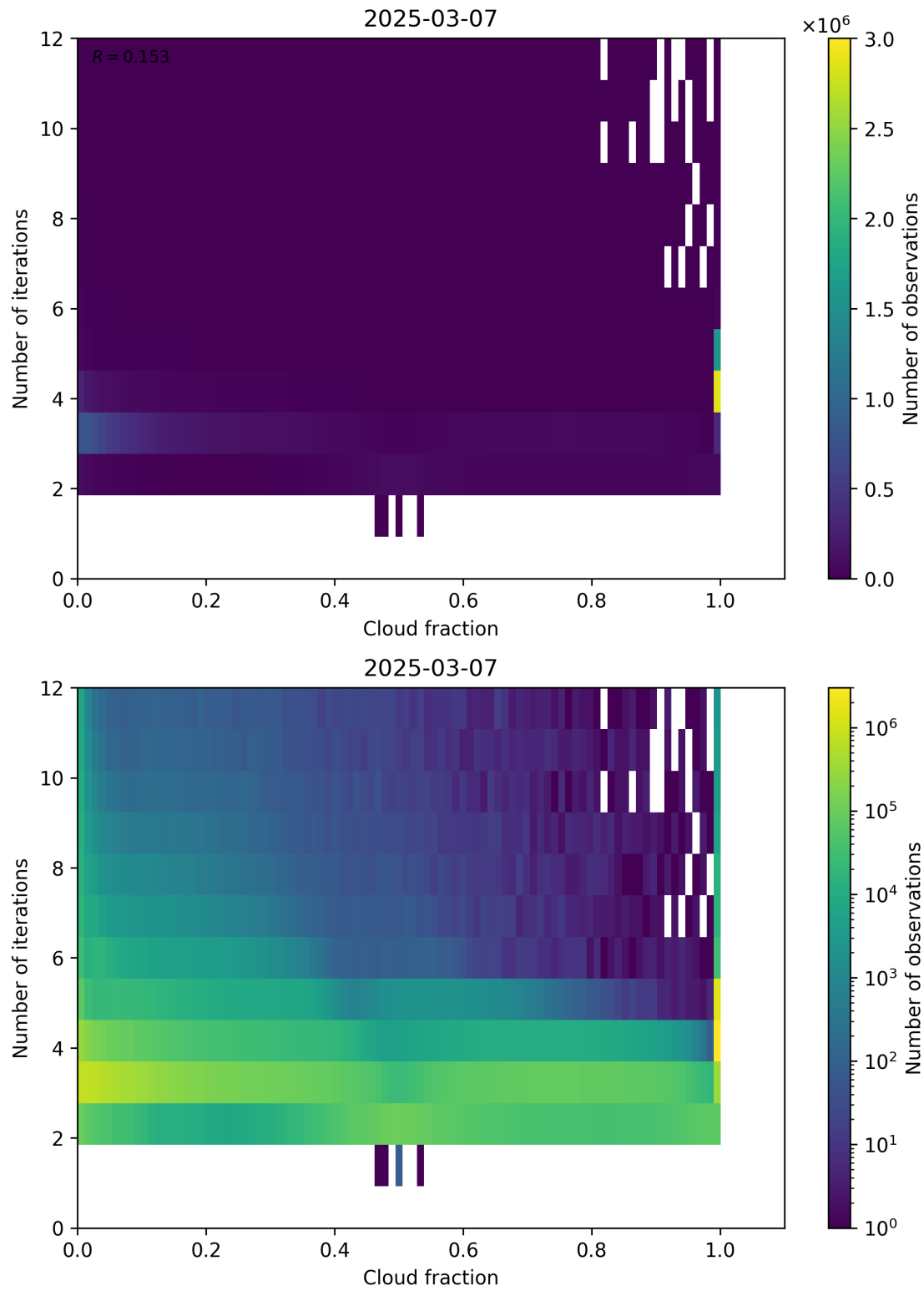
Figure 73: Scatter density plot of “Cloud fraction” against “Number of iterations” for 2025-03-07 to 2025-03-08.
