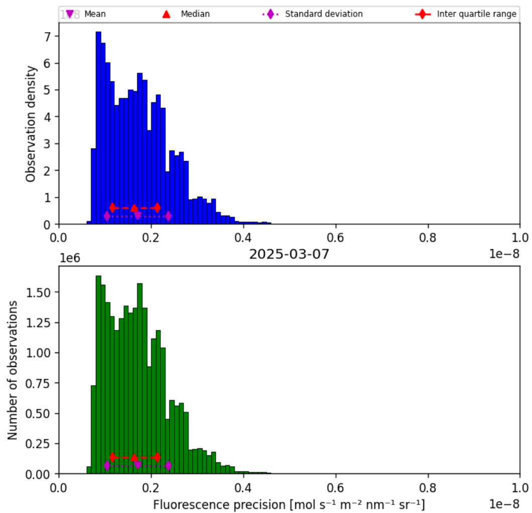
Figure 41: Histogram of “Fluorescence precision” for 2025-03-07 to 2025-03-08
