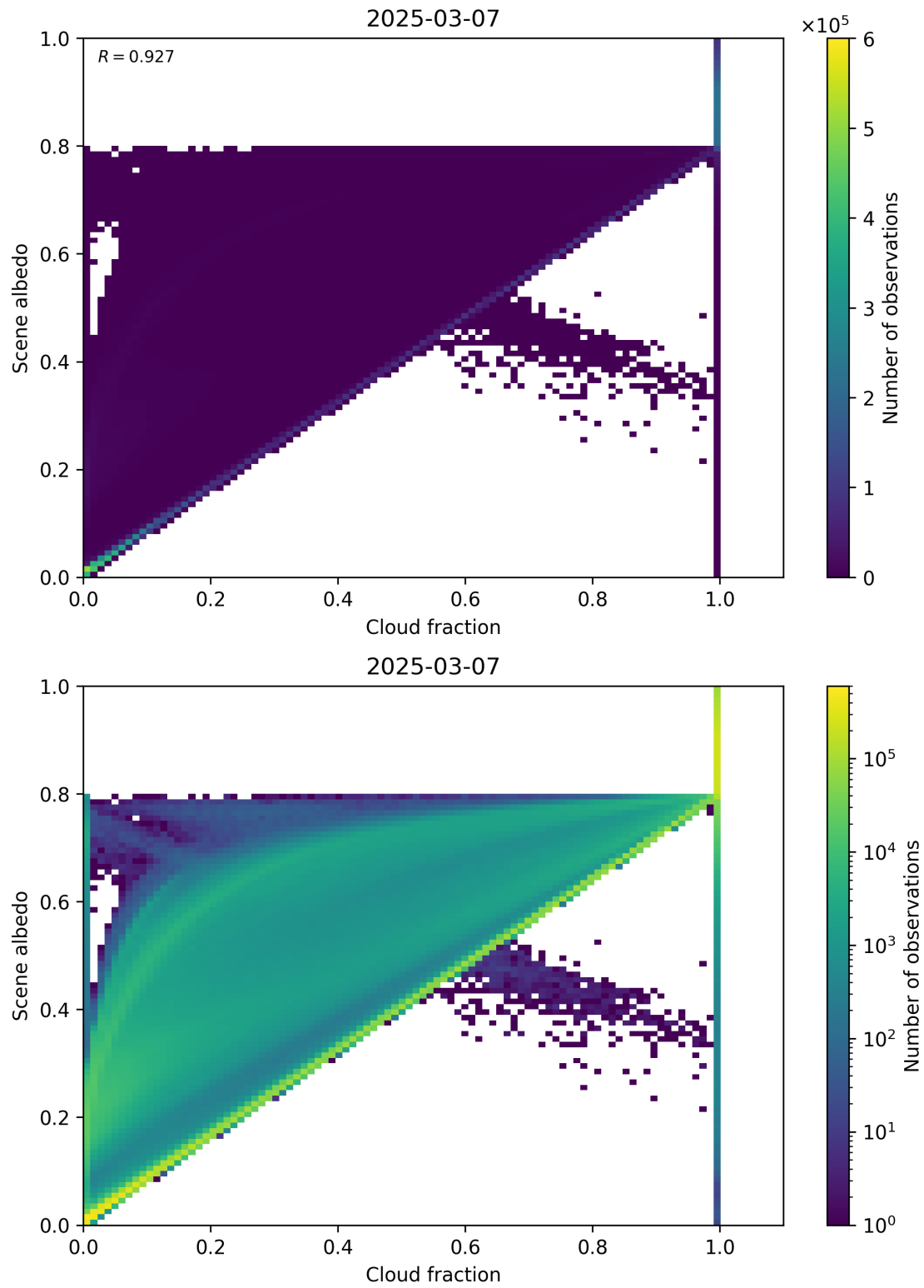
Figure 75: Scatter density plot of “Cloud fraction” against “Scene albedo” for 2025-03-07 to 2025-03-08.
