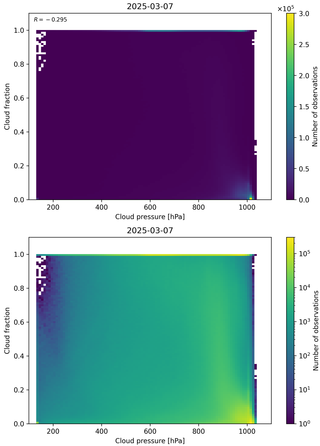
Figure 79: Scatter density plot of “Cloud pressure” against “Cloud fraction” for 2025-03-07 to 2025-03-08.
