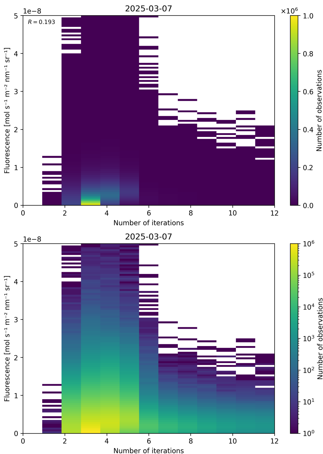
Figure 98: Scatter density plot of “Number of iterations” against “Fluorescence” for 2025-03-07 to 2025-03-08.
