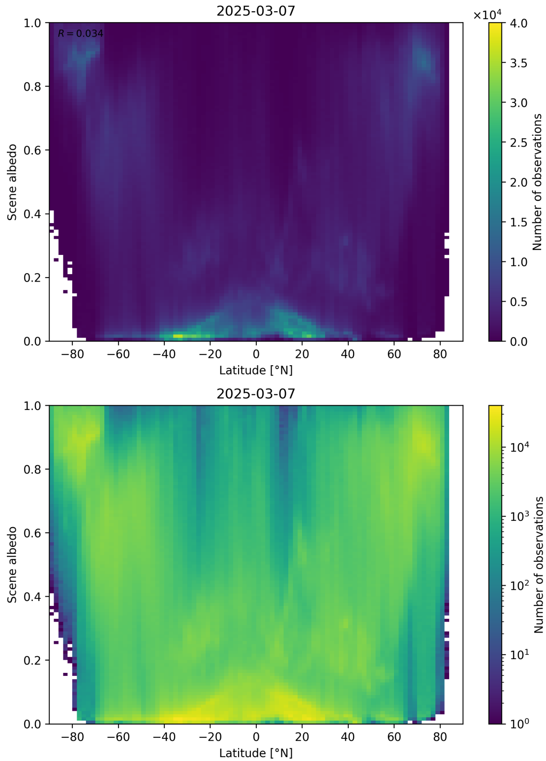
Figure 95: Scatter density plot of “Latitude” against “Scene albedo” for 2025-03-07 to 2025-03-08.
