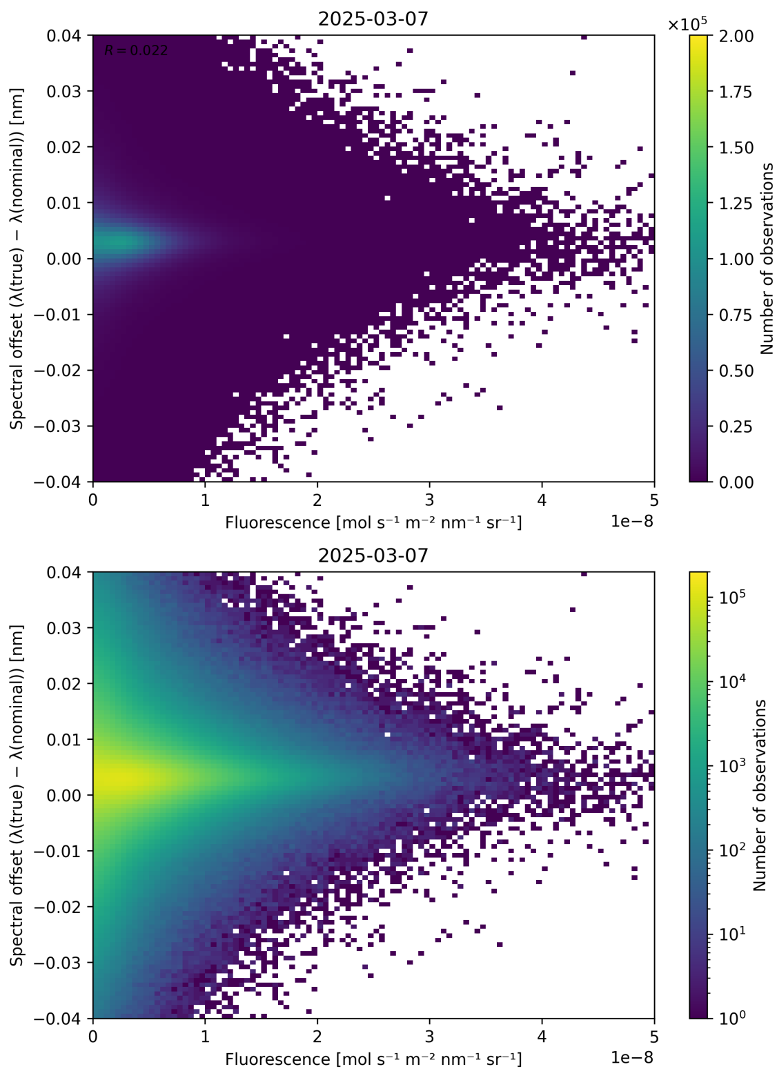
Figure 87: Scatter density plot of “Fluorescence” against “Spectral offset ( \lambda_{\text{true}} - \lambda_{\text{nominal}} )” for 2025-03-07 to 2025-03-08.
