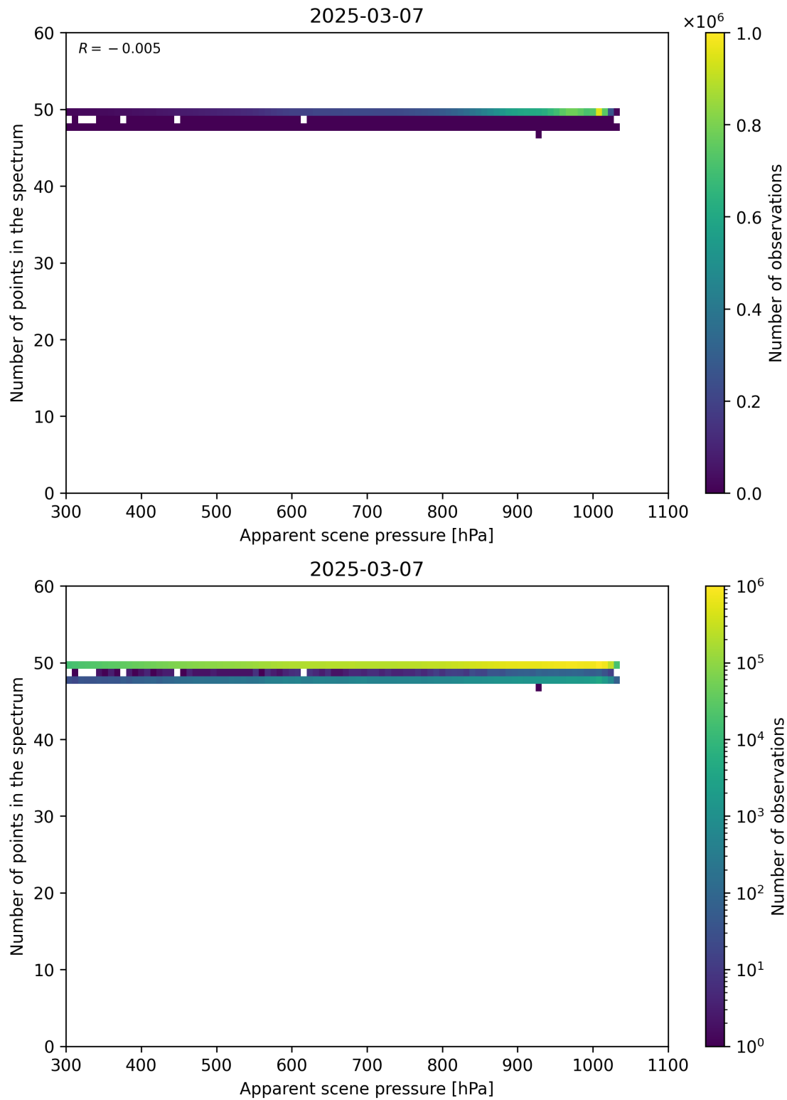
Figure 66: Scatter density plot of “Apparent scene pressure” against “Number of points in the spectrum” for 2025-03-07 to 2025-03-08.
