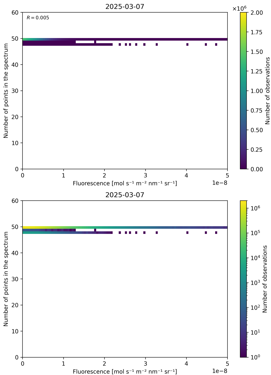
Figure 86: Scatter density plot of “Fluorescence” against “Number of points in the spectrum” for 2025-03-07 to 2025-03-08.
