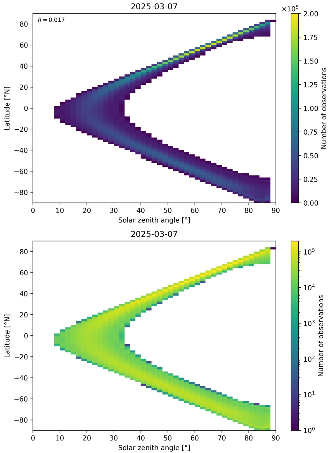
Figure 113: Scatter density plot of “Solar zenith angle” against “Latitude” for 2025-03-07 to 2025-03-08.
