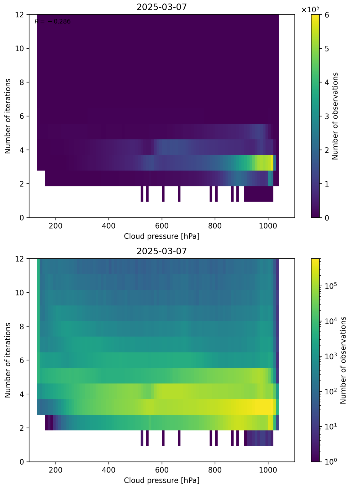
Figure 81: Scatter density plot of “Cloud pressure” against “Number of iterations” for 2025-03-07 to 2025-03-08.
