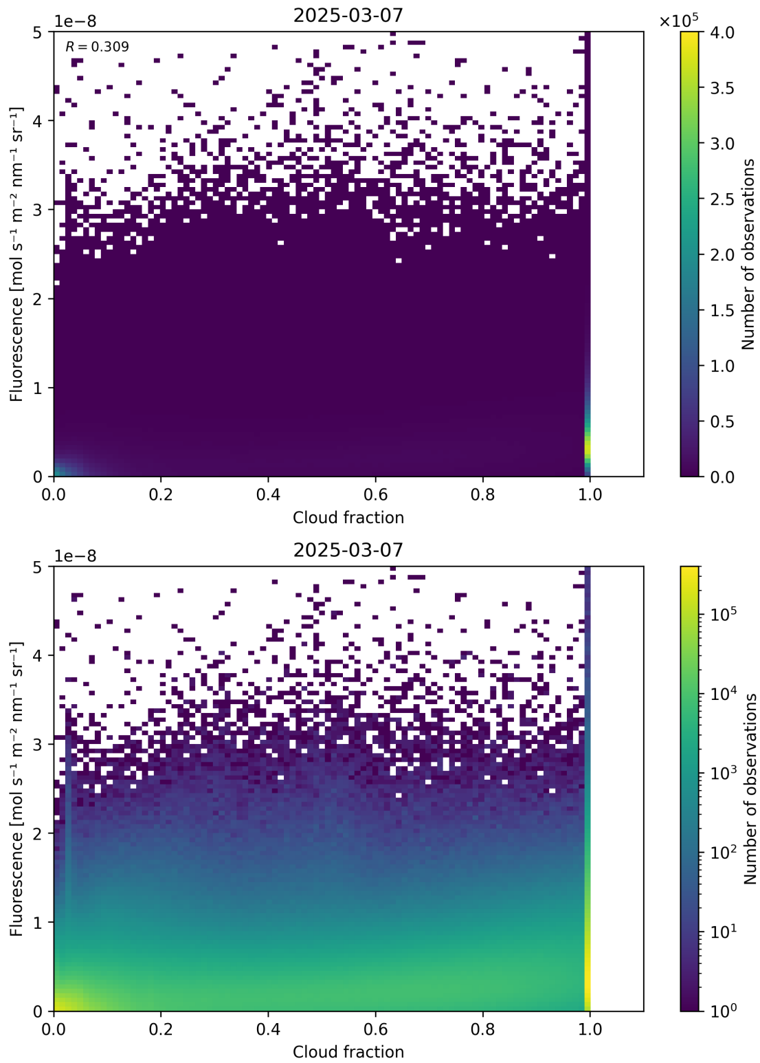
Figure 72: Scatter density plot of “Cloud fraction” against “Fluorescence” for 2025-03-07 to 2025-03-08.
