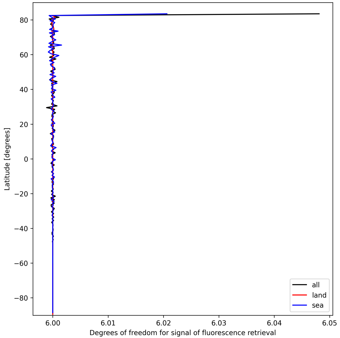
Figure 26: Zonal average of “Degrees of freedom for signal of fluorescence retrieval” for 2025-03-07 to 2025-03-08.
