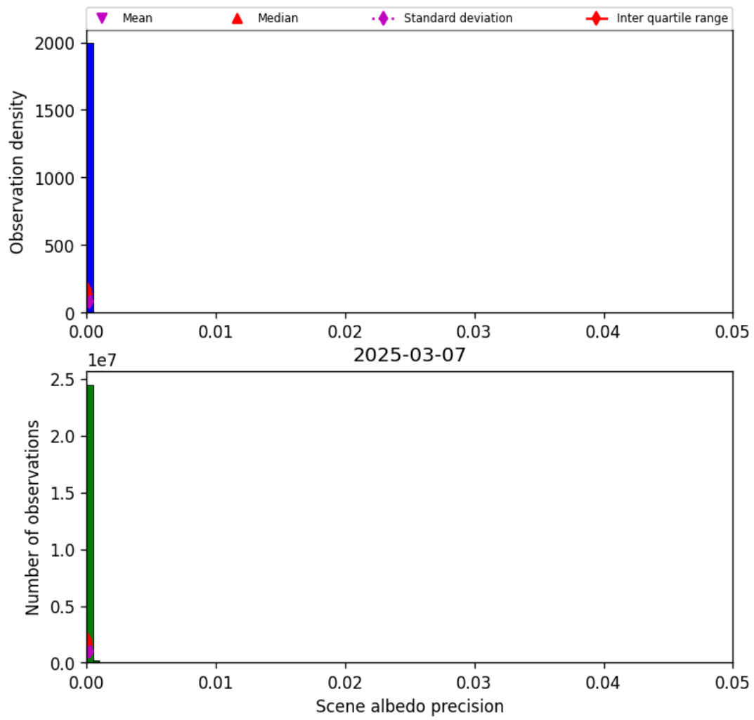
Figure 35: Histogram of “Scene albedo precision” for 2025-03-07 to 2025-03-08
