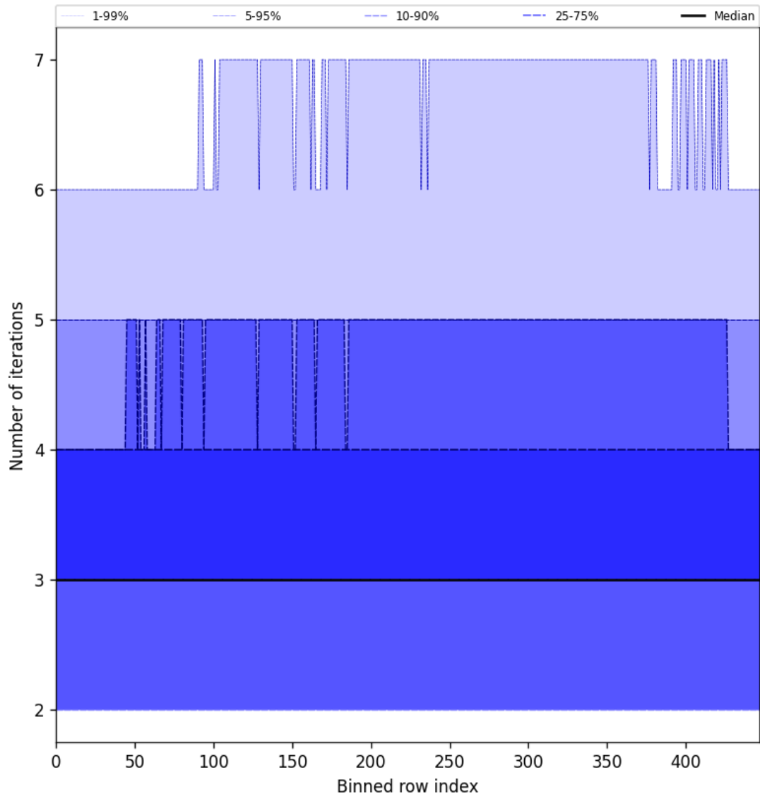
Figure 56: Along track statistics of “Number of iterations” for 2025-03-07 to 2025-03-08
