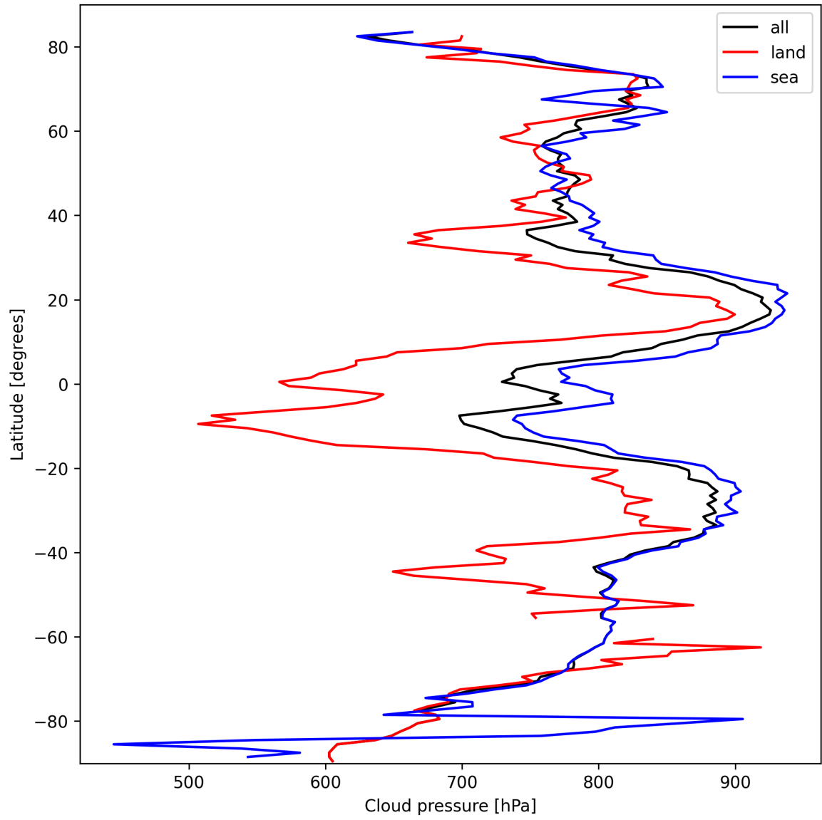
Figure 13: Zonal average of “Cloud pressure” for 2025-03-07 to 2025-03-08.
