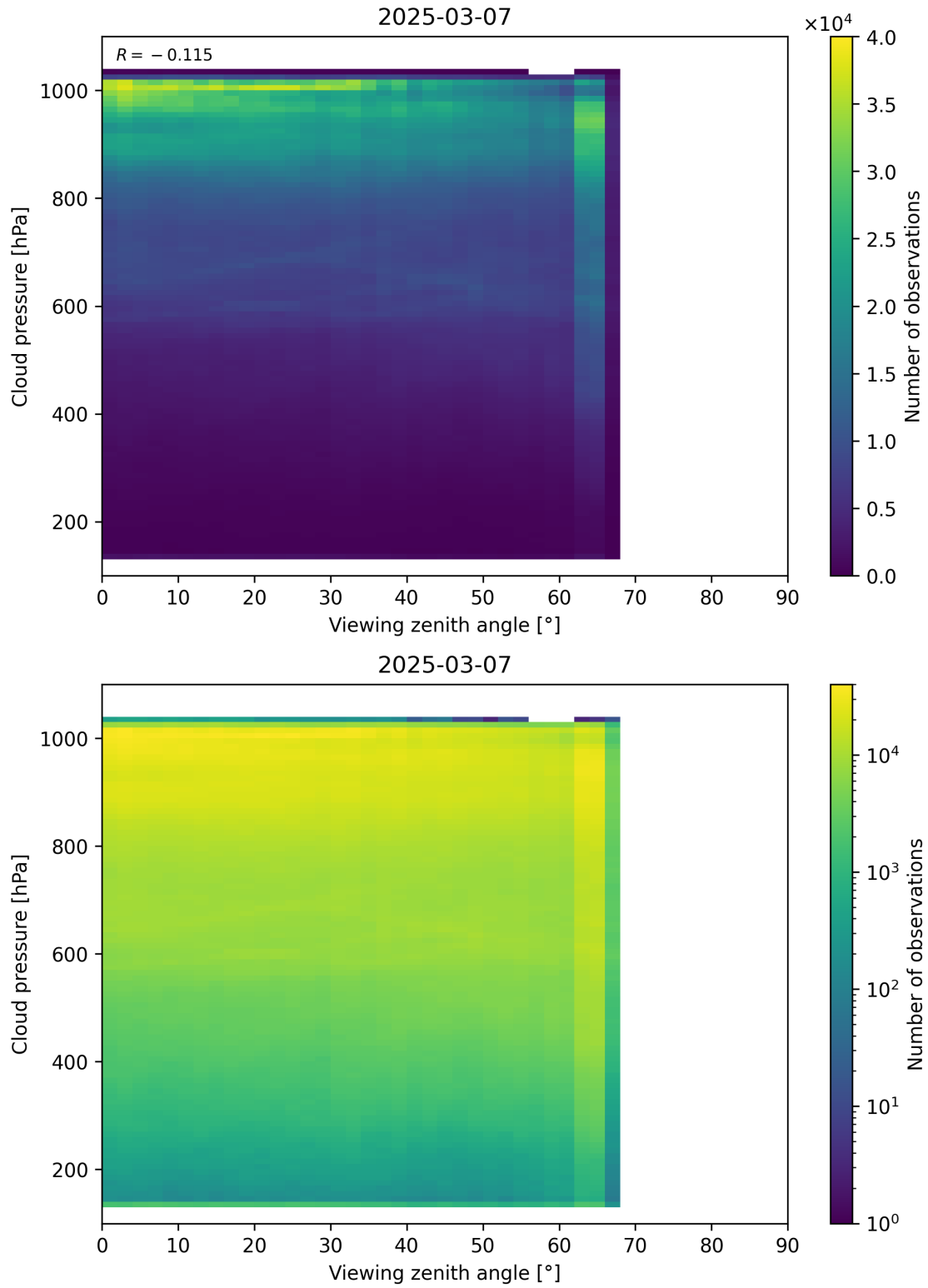
Figure 121: Scatter density plot of “Viewing zenith angle” against “Cloud pressure” for 2025-03-07 to 2025-03-08.
