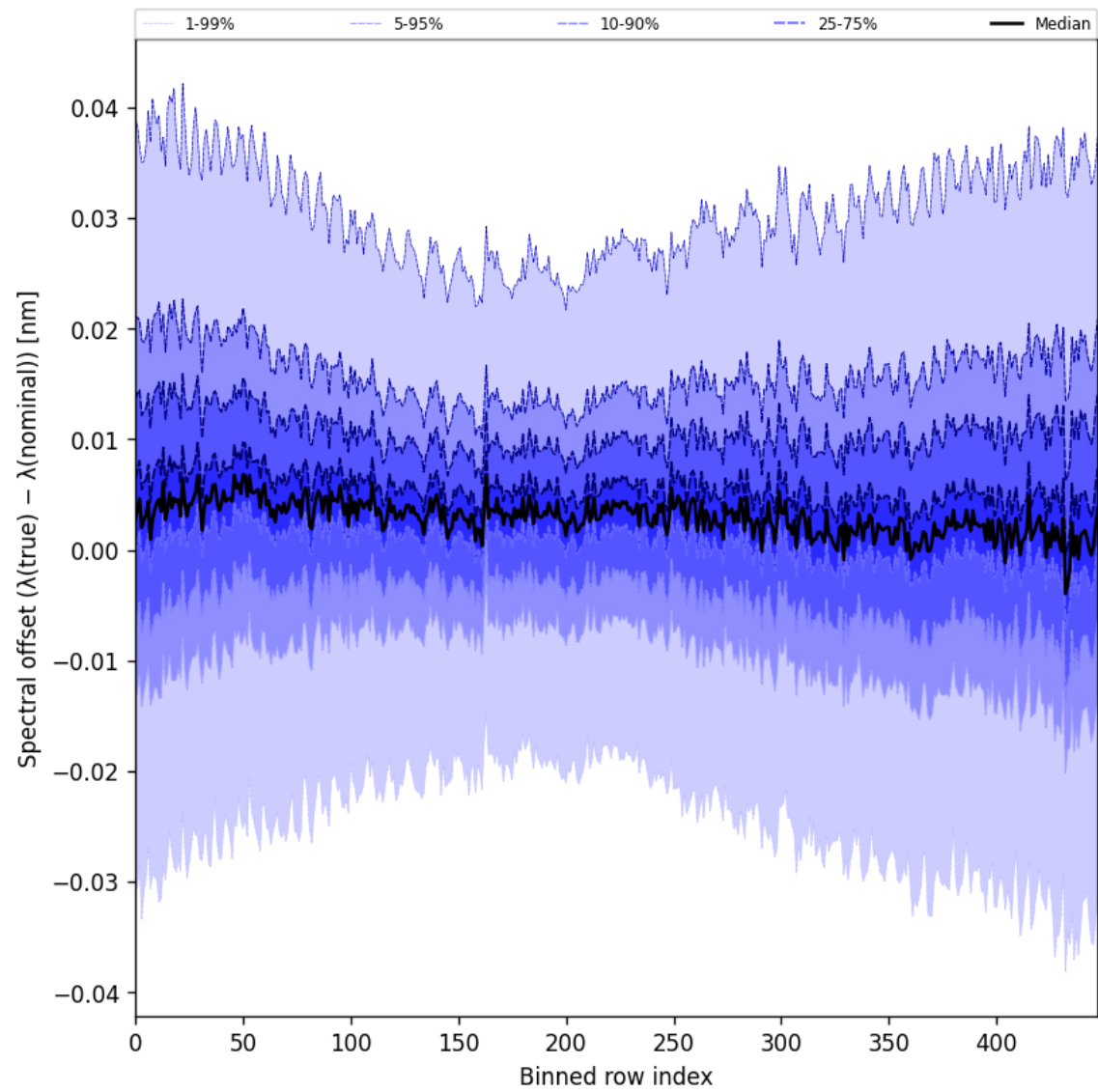
Figure 62: Along track statistics of “Spectral offset ( \lambda_{\text{true}} - \lambda_{\text{nominal}} )” for 2025-03-07 to 2025-03-08
