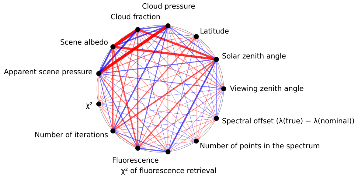
Figure 1: Map of correlation graph for 2025-03-07 to 2025-03-08.
