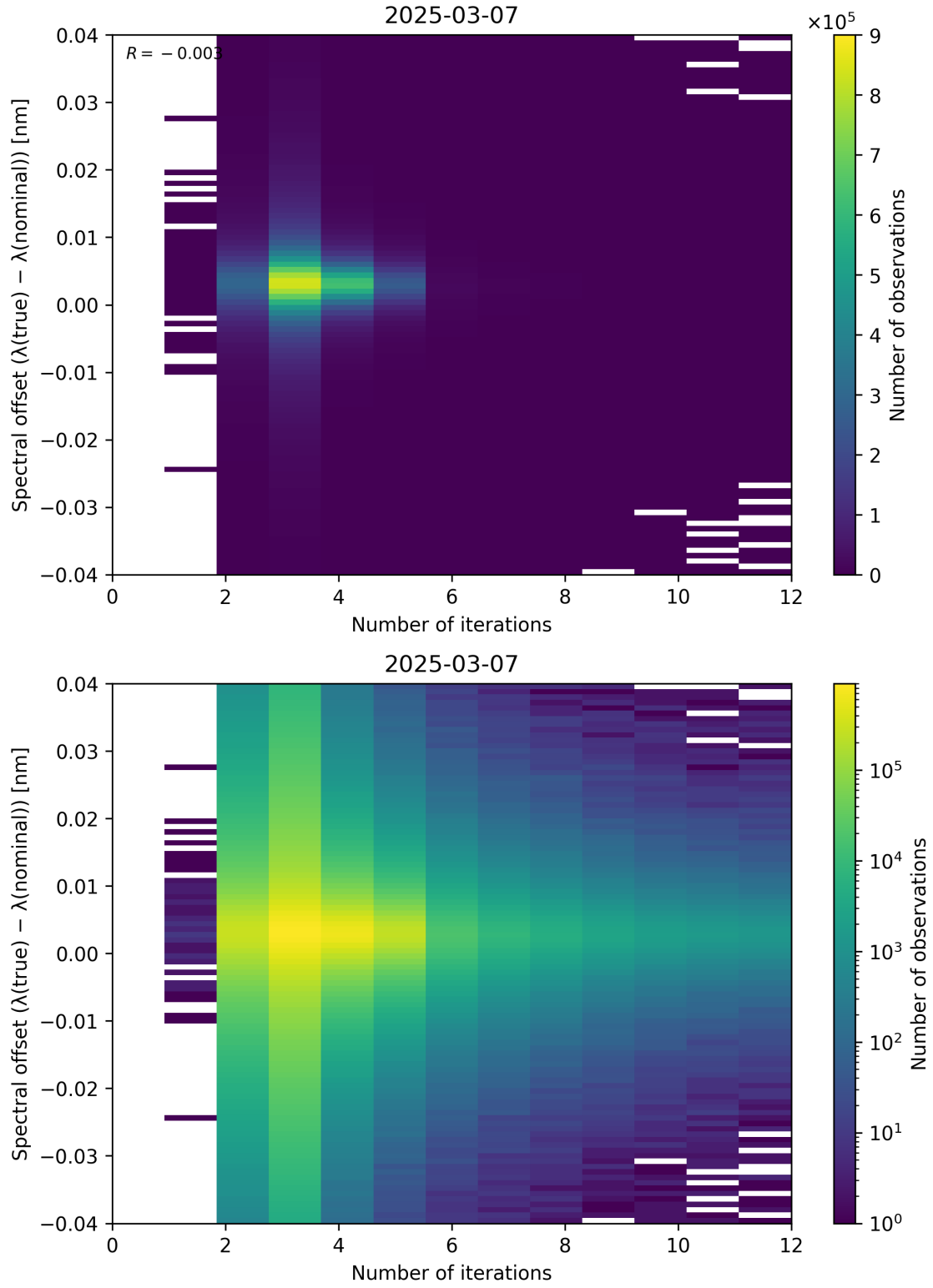
Figure 100: Scatter density plot of “Number of iterations” against “Spectral offset ( \lambda_{\text{true}} - \lambda_{\text{nominal}} )” for 2025-03-07 to 2025-03-08.
