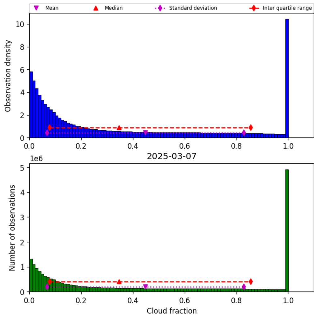
Figure 32: Histogram of “Cloud fraction” for 2025-03-07 to 2025-03-08
