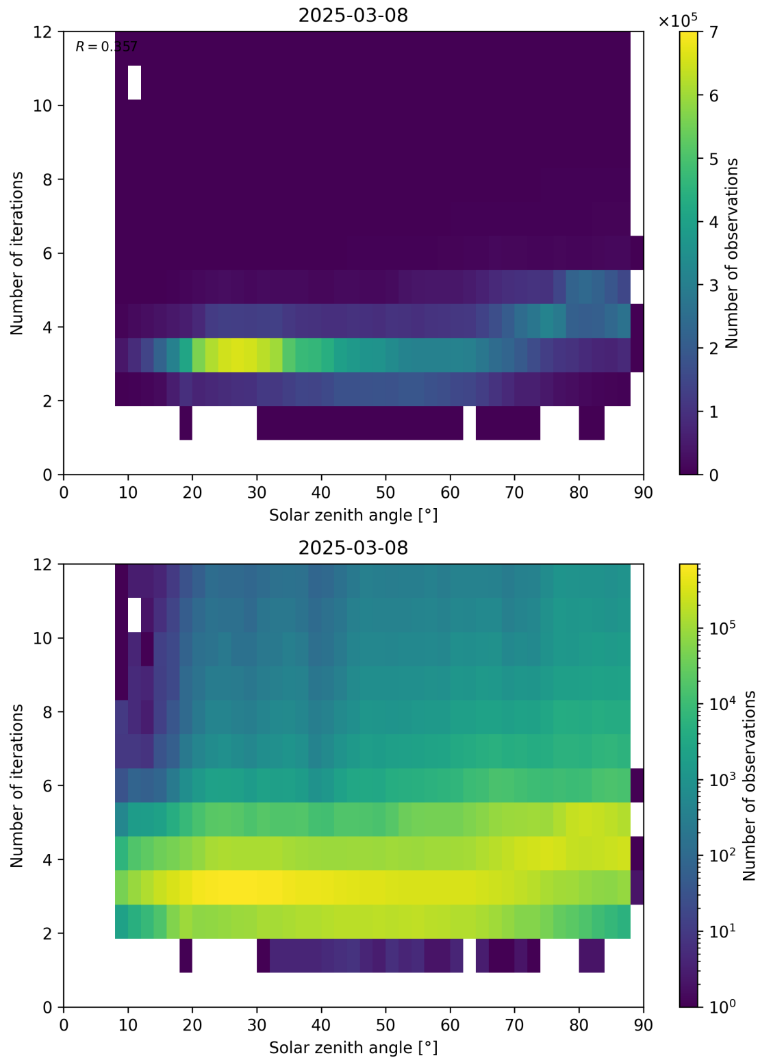
Figure 114: Scatter density plot of “Solar zenith angle” against “Number of iterations” for 2025-03-07 to 2025-03-09.
