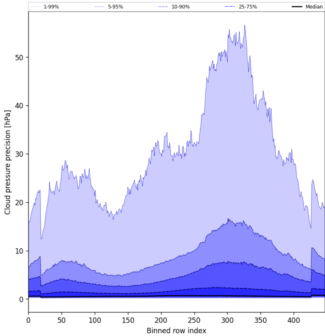
Figure 48: Along track statistics of “Cloud pressure precision” for 2025-03-07 to 2025-03-09
