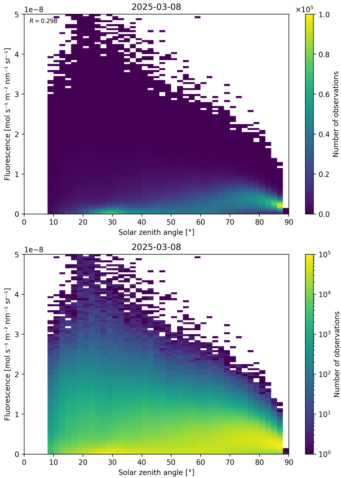
Figure 112: Scatter density plot of “Solar zenith angle” against “Fluorescence” for 2025-03-07 to 2025-03-09.
