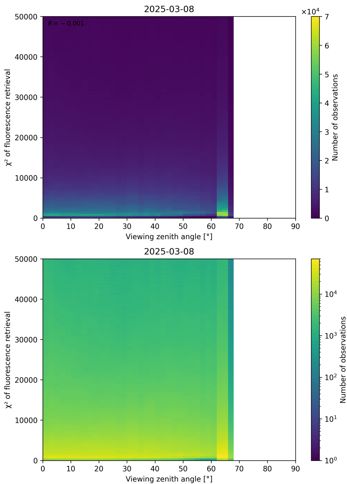
Figure 119: Scatter density plot of “Viewing zenith angle” against “ \chi^2 of fluorescence retrieval” for 2025-03-07 to 2025-03-09.
