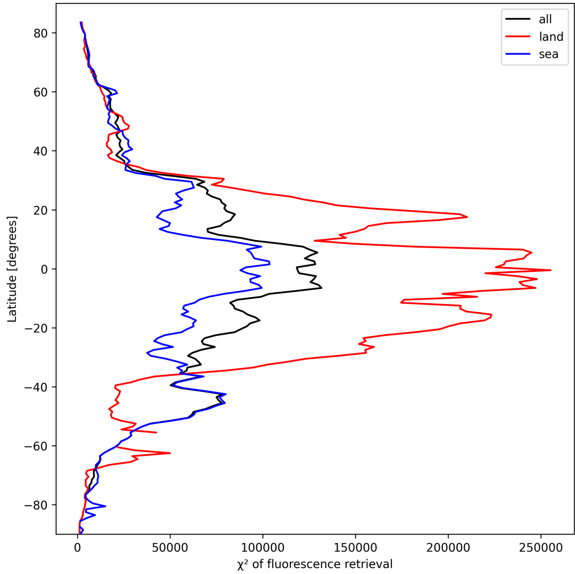
Figure 25: Zonal average of “ \chi^2 of fluorescence retrieval” for 2025-03-07 to 2025-03-09.
