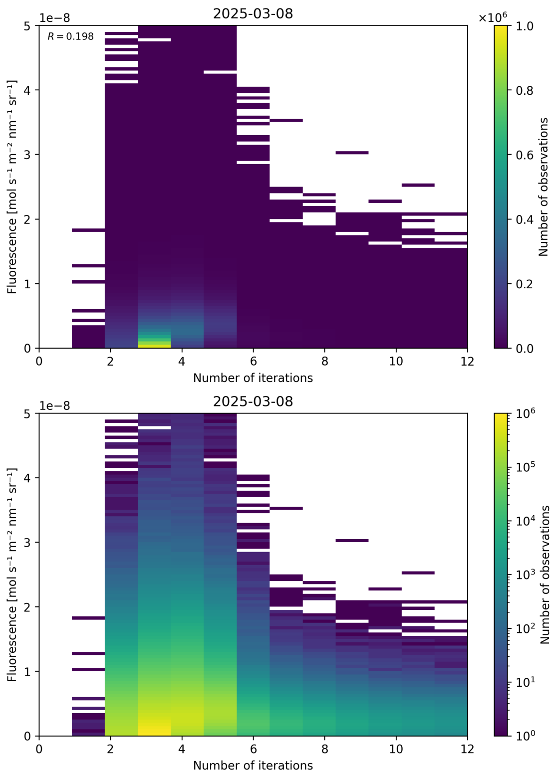
Figure 98: Scatter density plot of “Number of iterations” against “Fluorescence” for 2025-03-07 to 2025-03-09.
