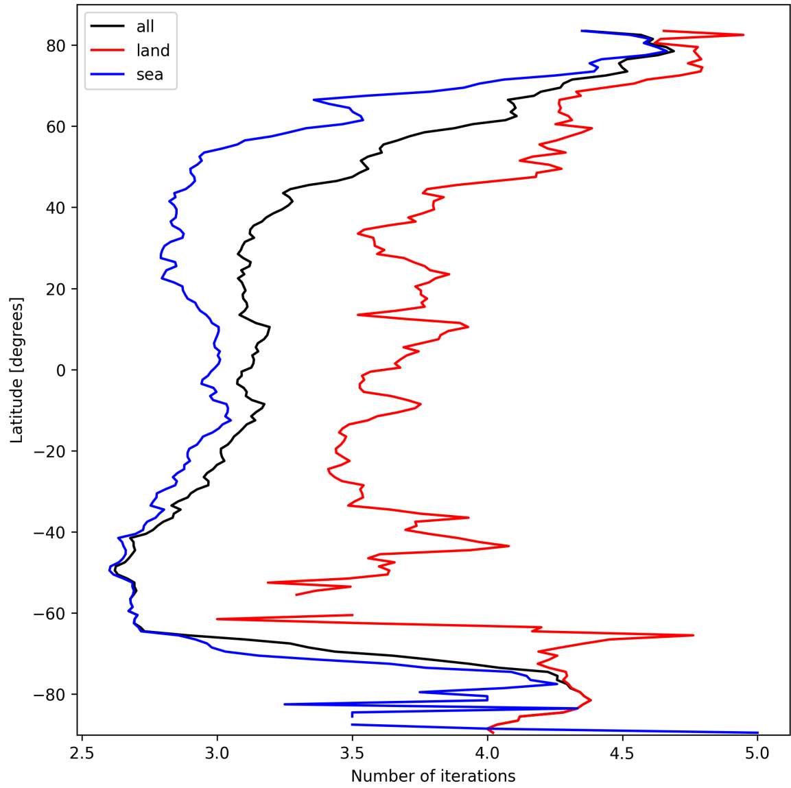
Figure 22: Zonal average of “Number of iterations” for 2025-03-07 to 2025-03-09.
