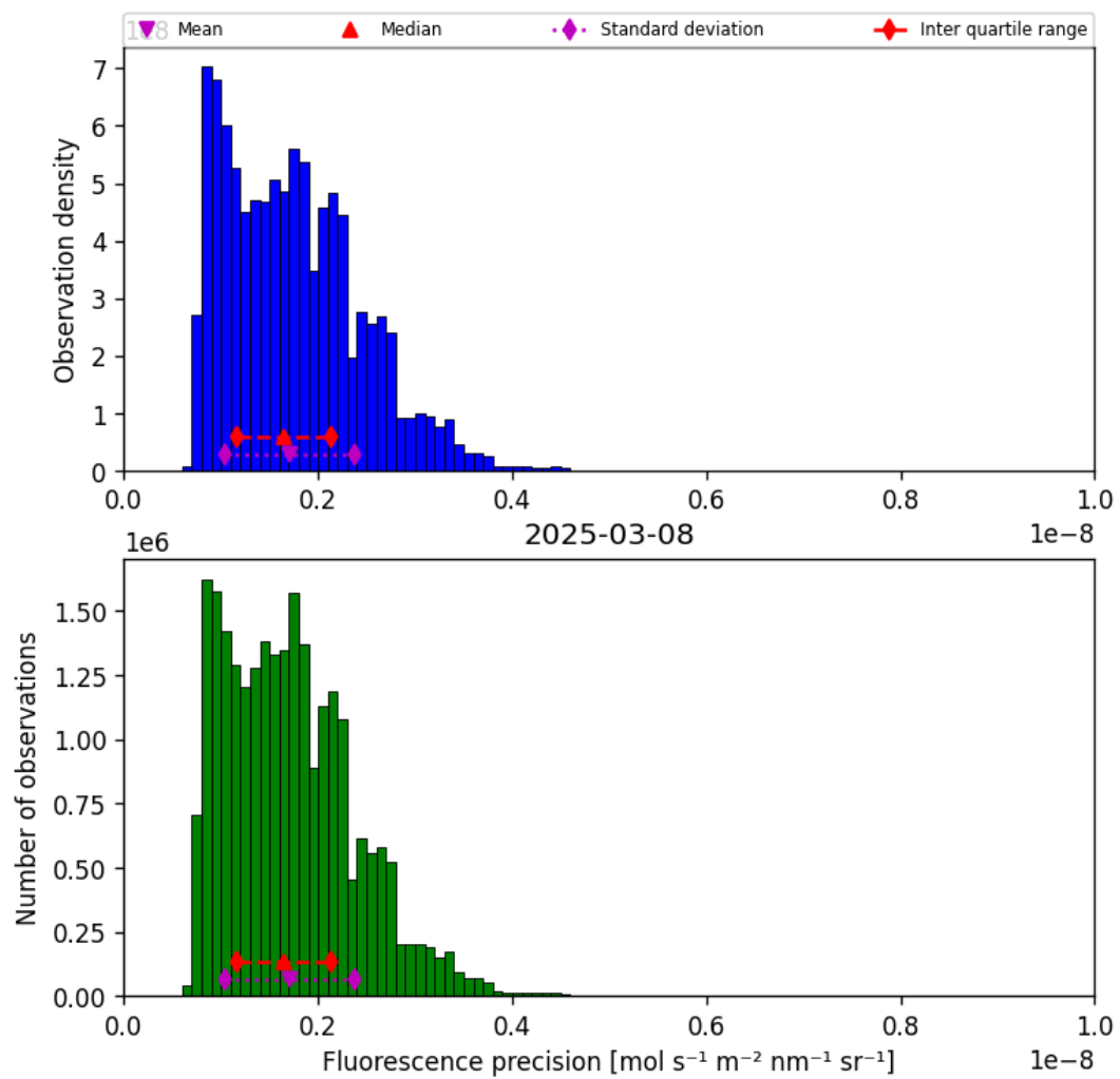
Figure 41: Histogram of “Fluorescence precision” for 2025-03-07 to 2025-03-09
