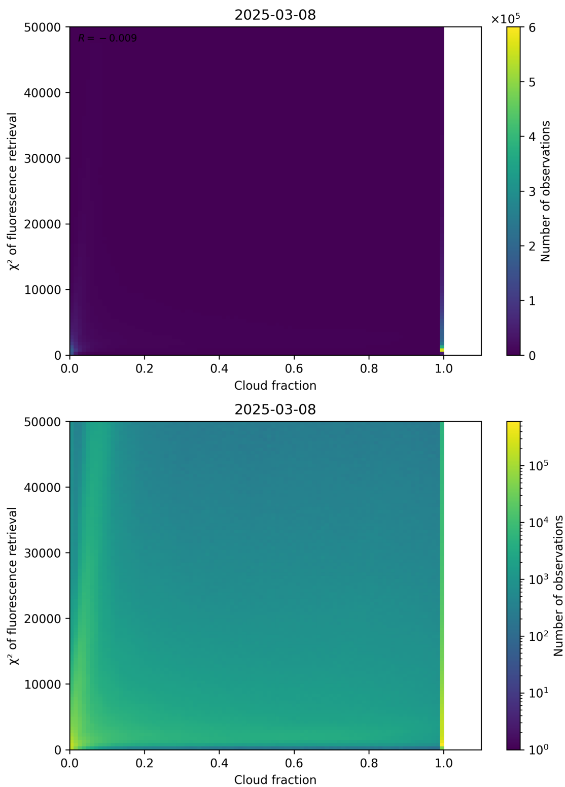
Figure 71: Scatter density plot of “Cloud fraction” against “ \chi^2 of fluorescence retrieval” for 2025-03-07 to 2025-03-09.
