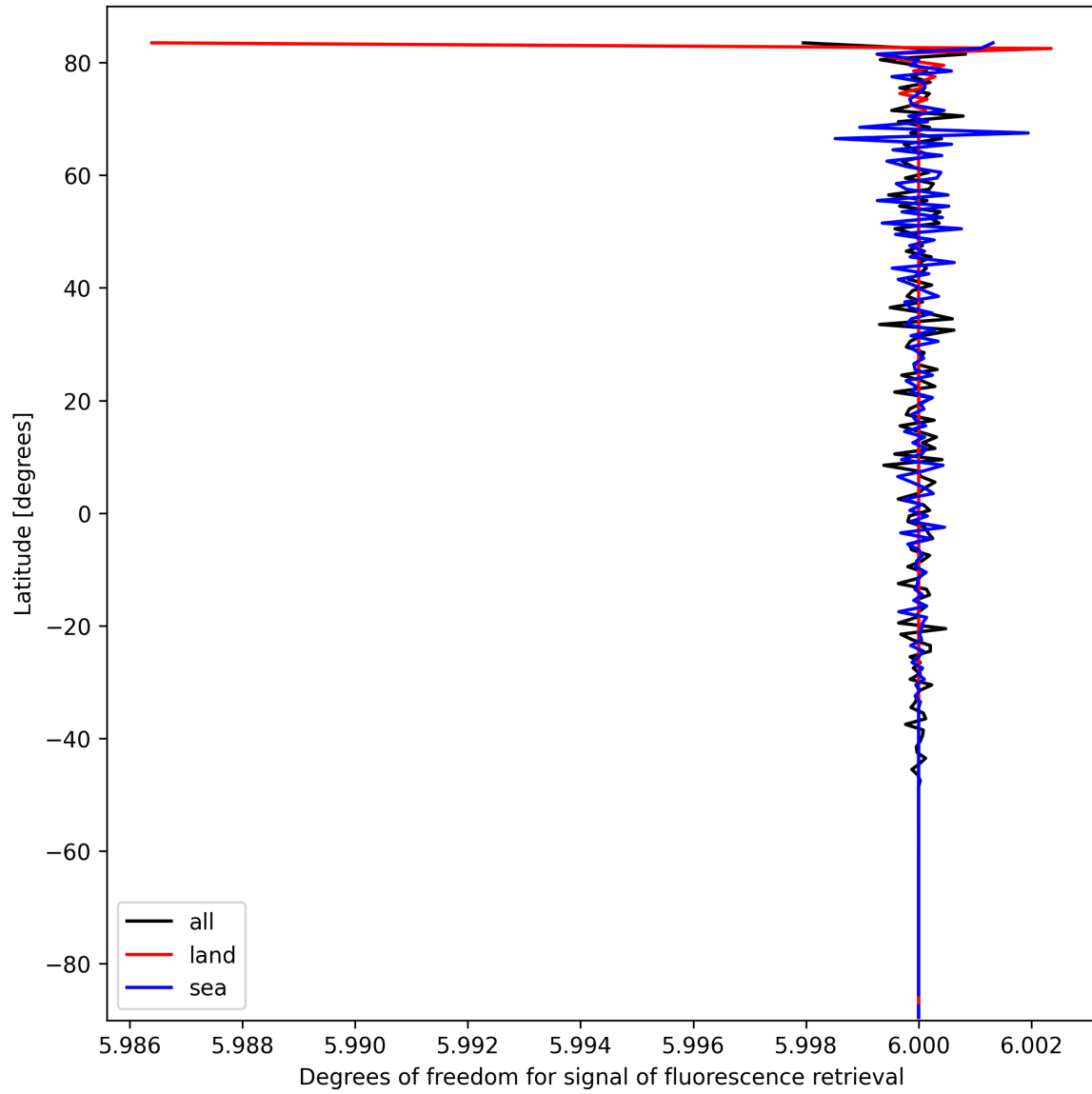
Figure 26: Zonal average of “Degrees of freedom for signal of fluorescence retrieval” for 2025-03-07 to 2025-03-09.
