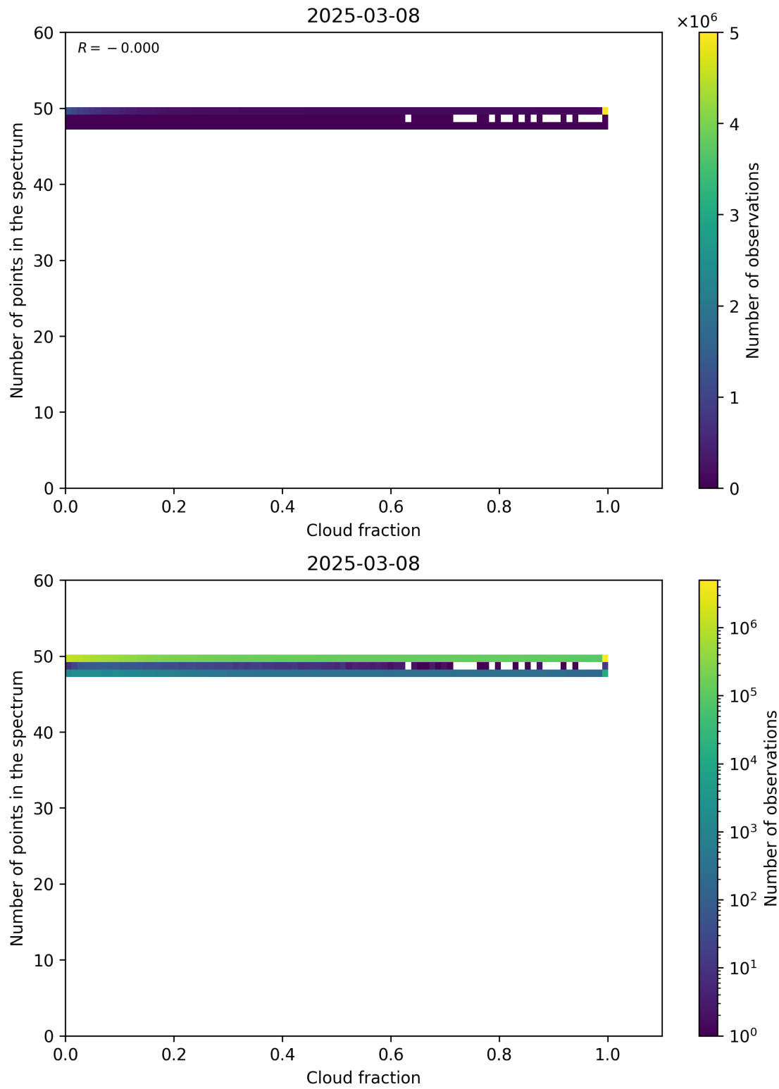
Figure 74: Scatter density plot of “Cloud fraction” against “Number of points in the spectrum” for 2025-03-07 to 2025-03-09.
