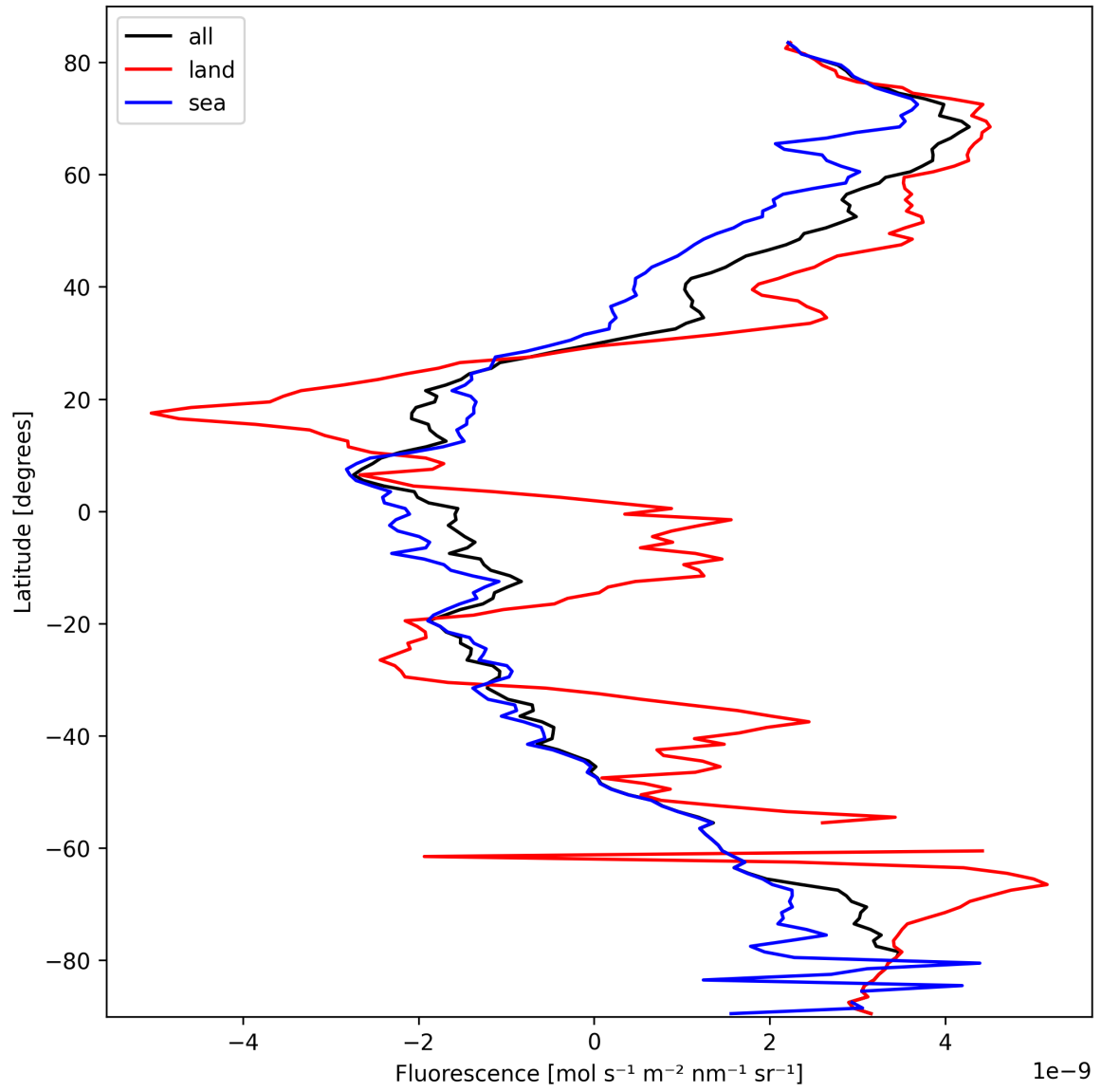
Figure 23: Zonal average of “Fluorescence” for 2025-03-07 to 2025-03-09.
