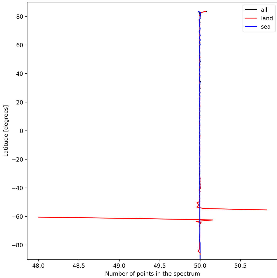
Figure 27: Zonal average of “Number of points in the spectrum” for 2025-03-07 to 2025-03-09.
