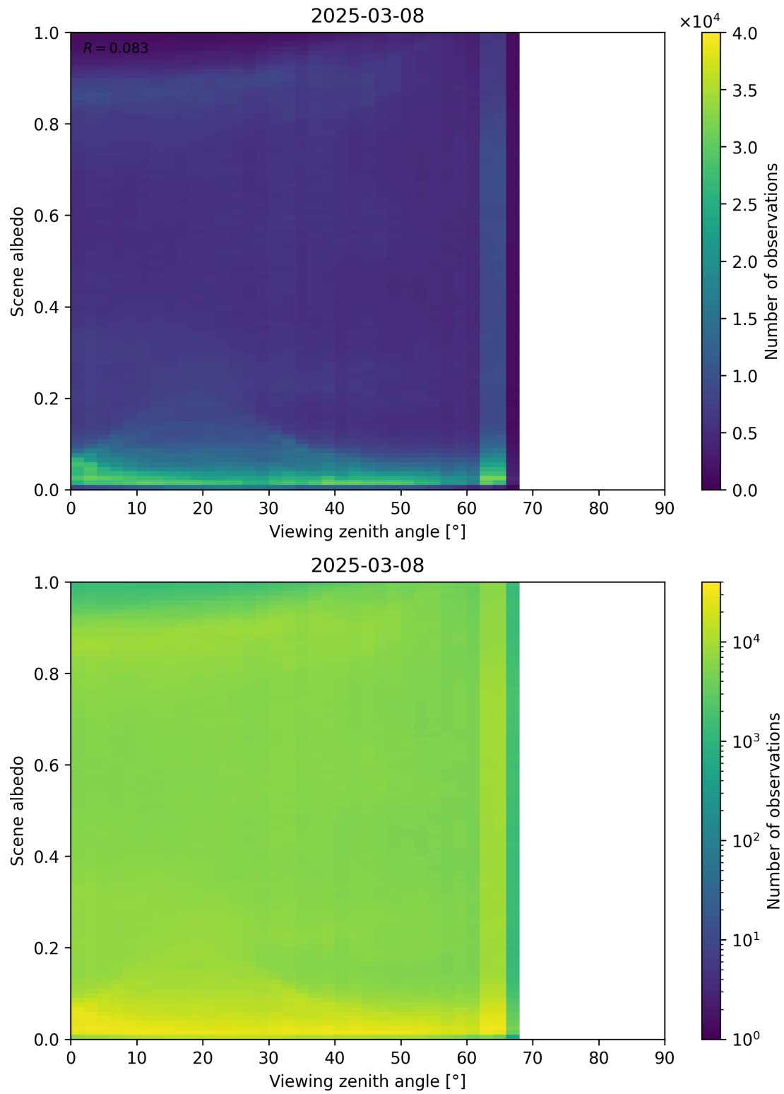
Figure 126: Scatter density plot of “Viewing zenith angle” against “Scene albedo” for 2025-03-07 to 2025-03-09.
