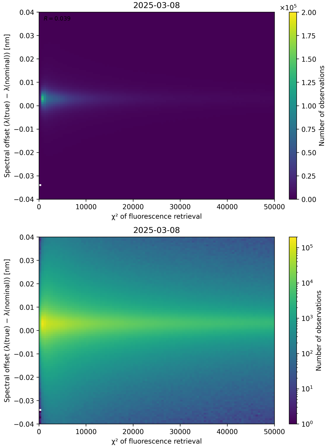
Figure 69: Scatter density plot of “ \chi^2 of fluorescence retrieval” against “Spectral offset ( \lambda_{\text{true}} - \lambda_{\text{nominal}} )” for 2025-03-07 to 2025-03-09.
