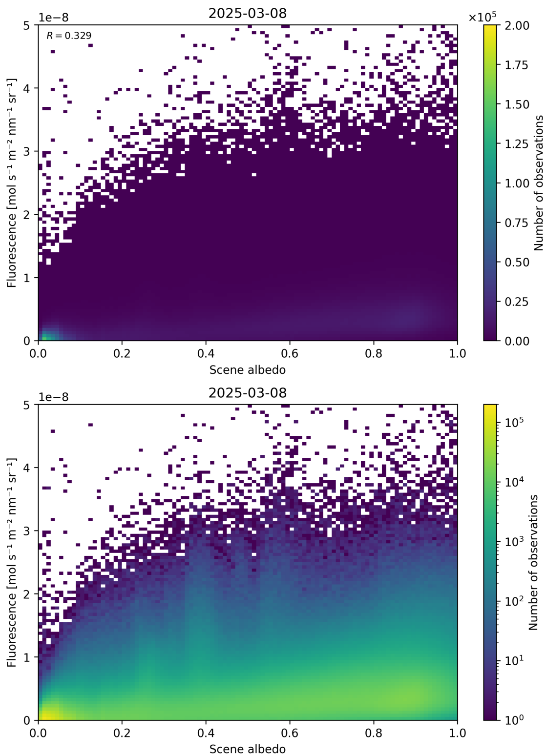
Figure 104: Scatter density plot of “Scene albedo” against “Fluorescence” for 2025-03-07 to 2025-03-09.
