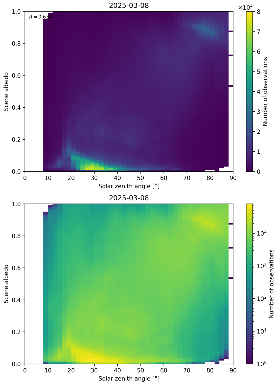
Figure 116: Scatter density plot of “Solar zenith angle” against “Scene albedo” for 2025-03-07 to 2025-03-09.
