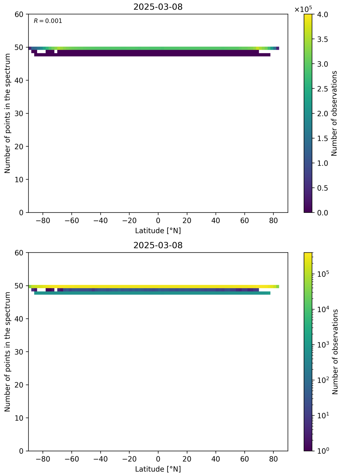
Figure 94: Scatter density plot of “Latitude” against “Number of points in the spectrum” for 2025-03-07 to 2025-03-09.
