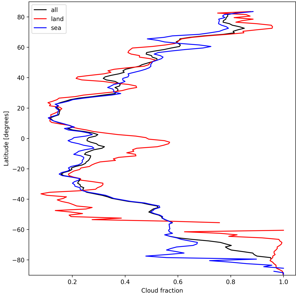
Figure 15: Zonal average of “Cloud fraction” for 2025-03-07 to 2025-03-09.
