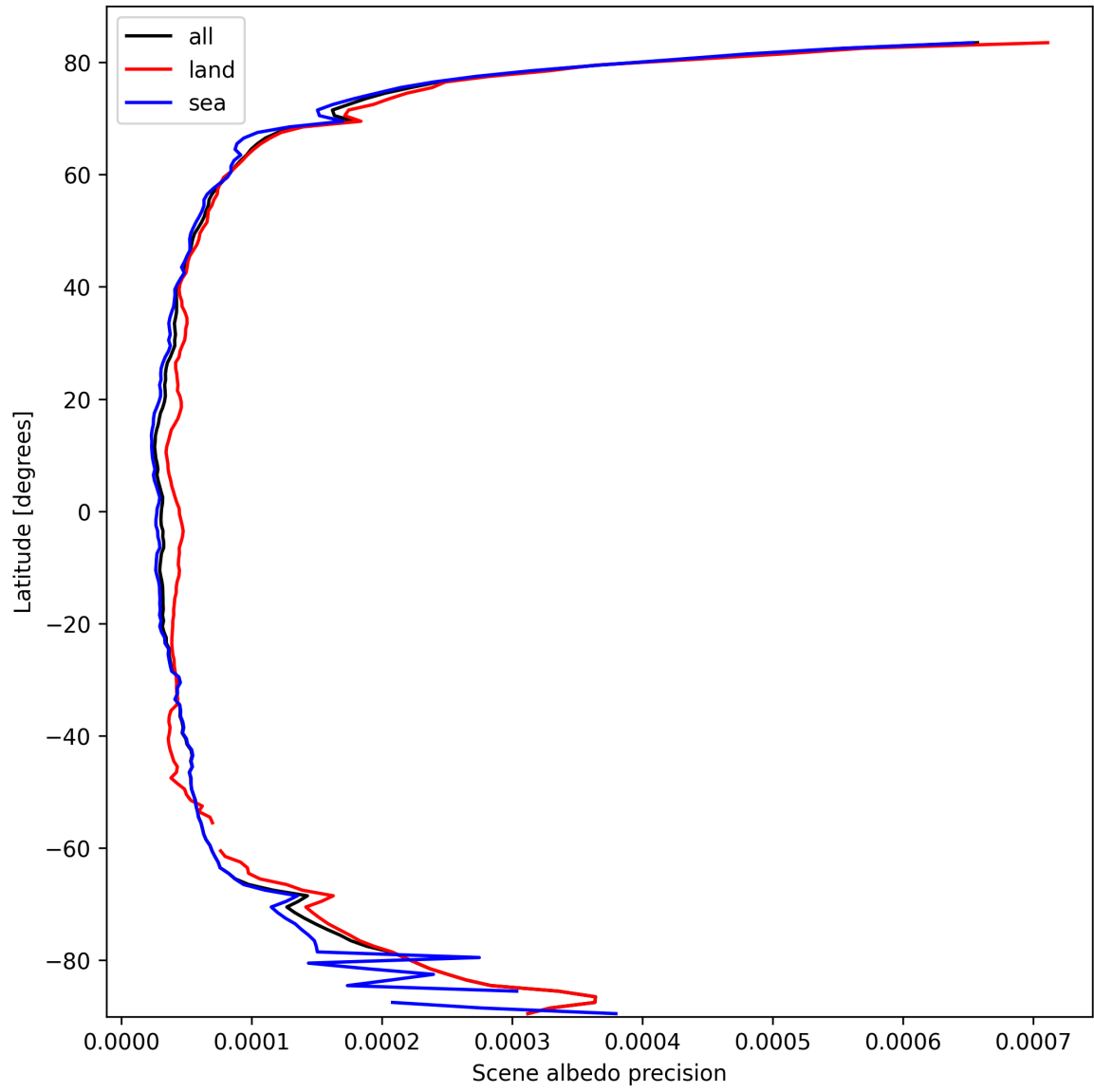
Figure 18: Zonal average of "Scene albedo precision" for 2025-03-07 to 2025-03-09.
