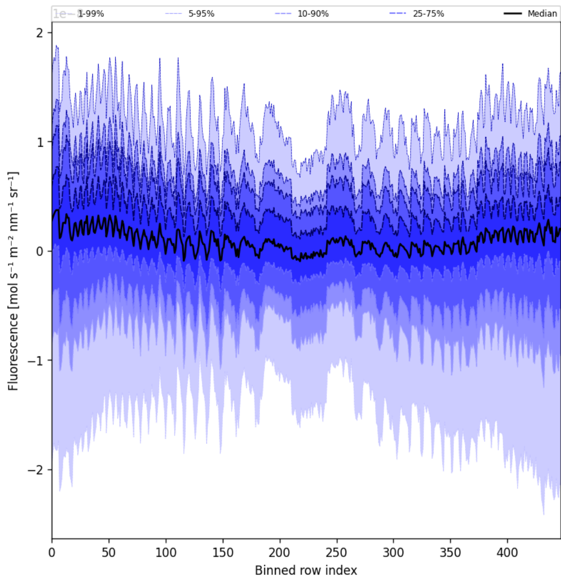
Figure 57: Along track statistics of “Fluorescence” for 2025-03-07 to 2025-03-09
