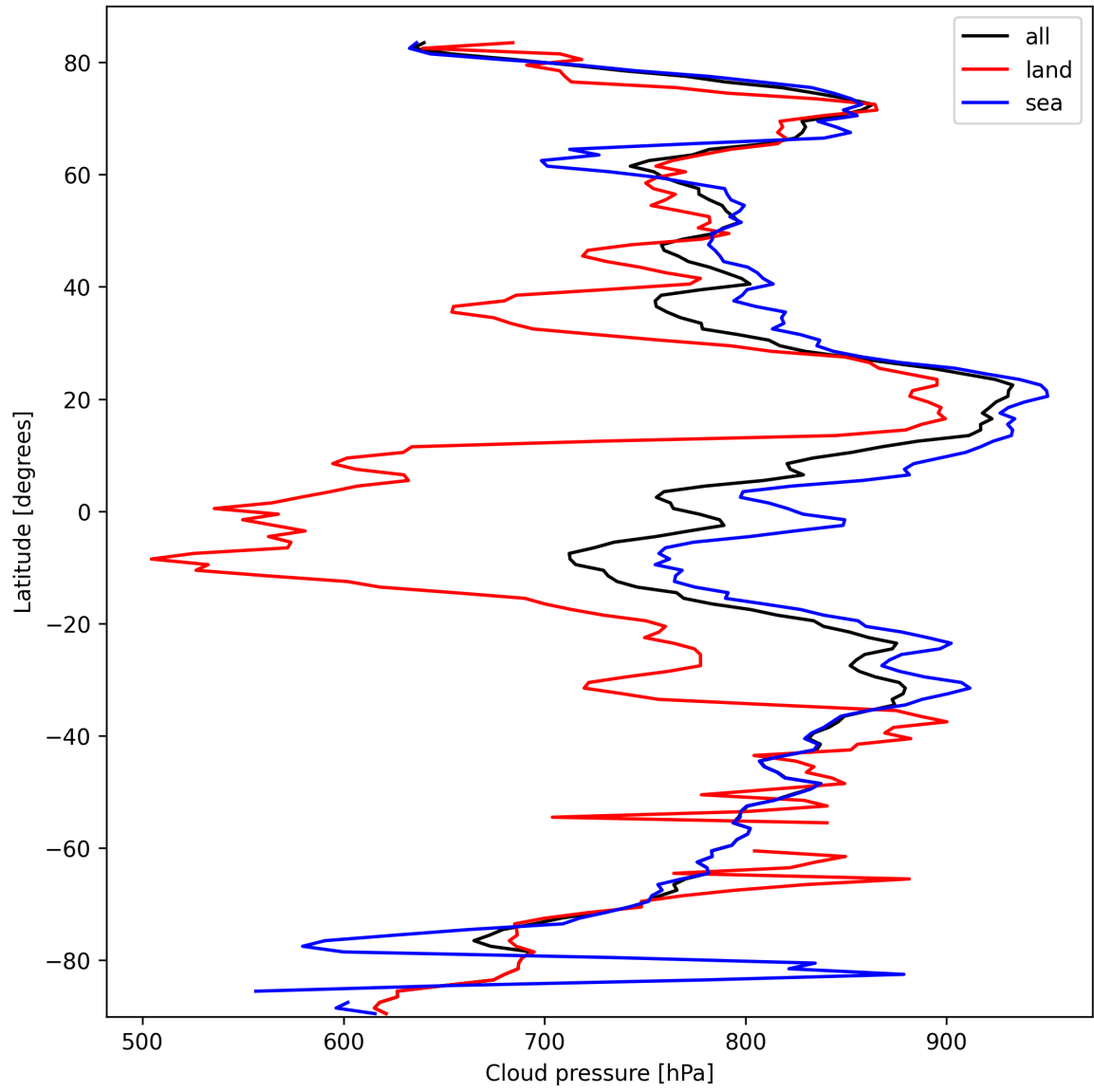
Figure 13: Zonal average of “Cloud pressure” for 2025-03-07 to 2025-03-09.
