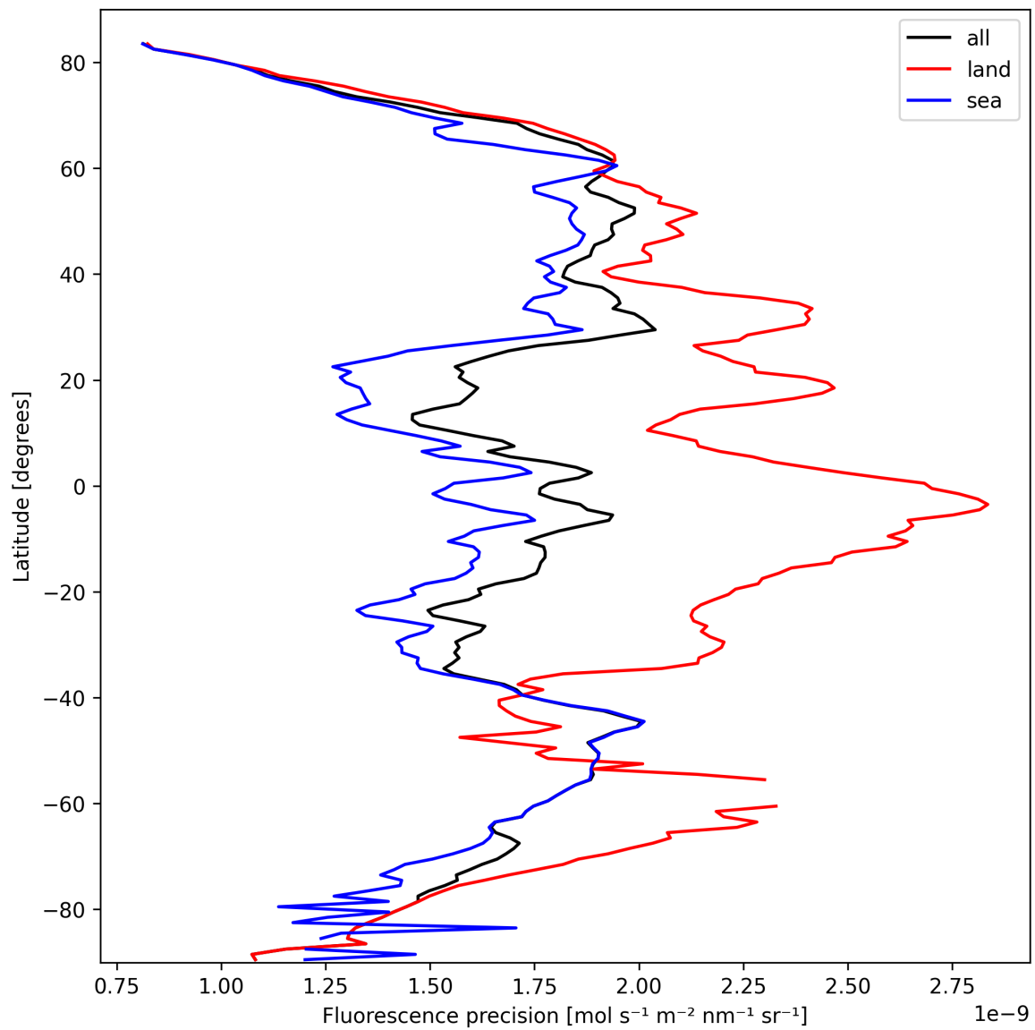
Figure 24: Zonal average of “Fluorescence precision” for 2025-03-07 to 2025-03-09.
