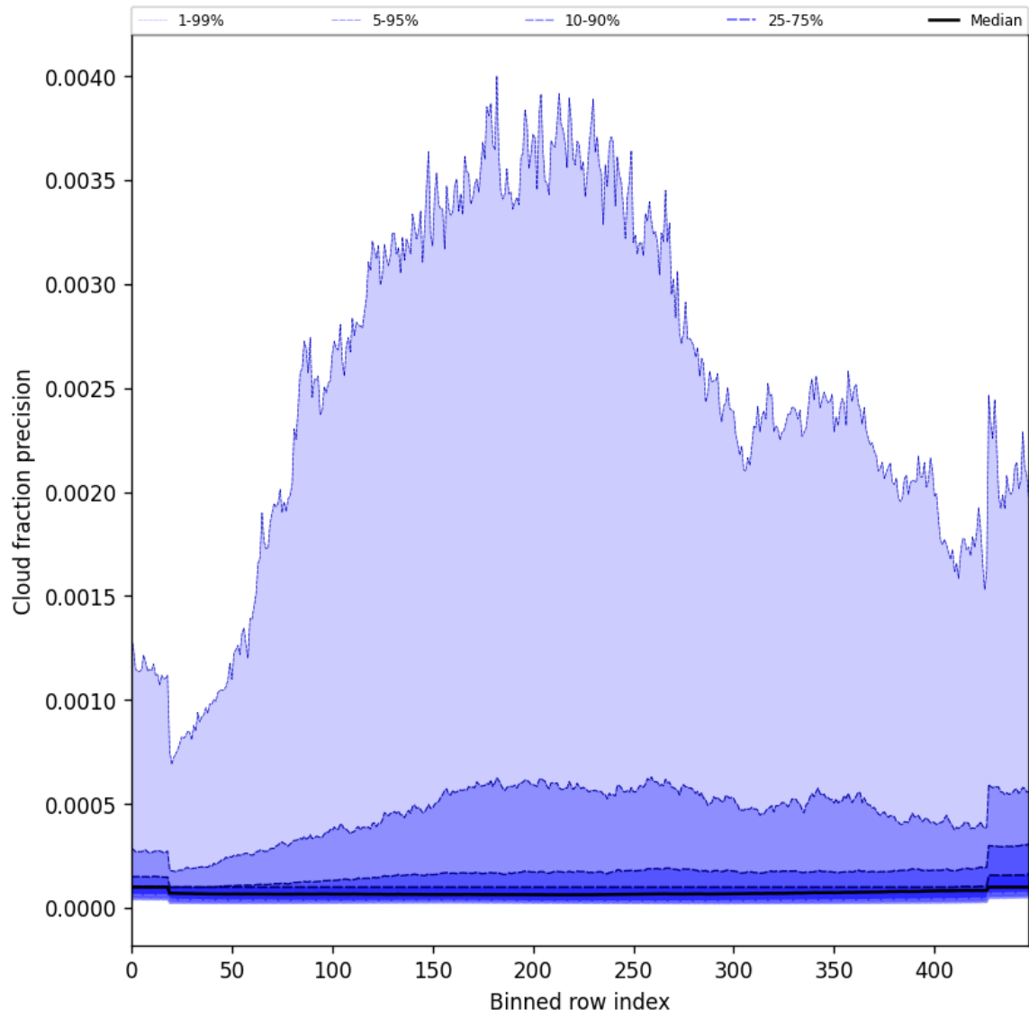
Figure 50: Along track statistics of “Cloud fraction precision” for 2025-03-07 to 2025-03-09
