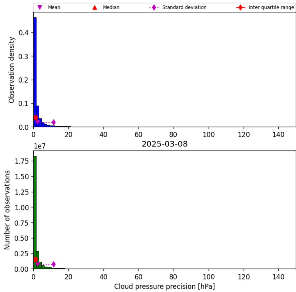
Figure 31: Histogram of “Cloud pressure precision” for 2025-03-07 to 2025-03-09
