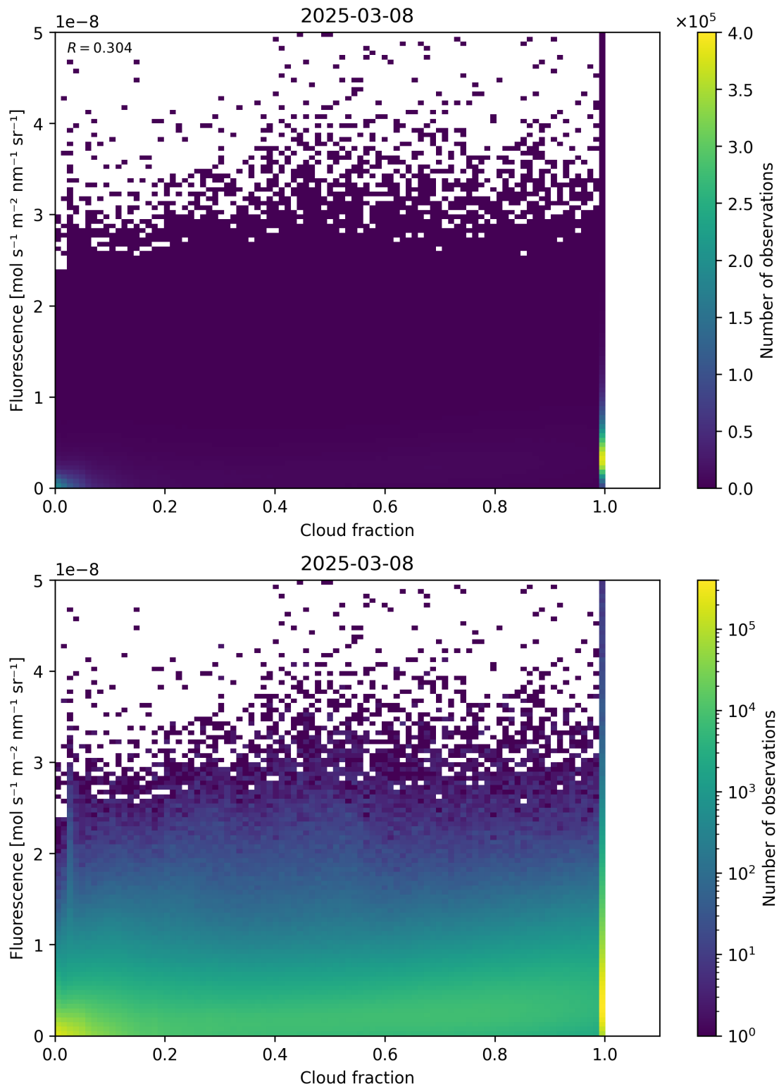
Figure 72: Scatter density plot of “Cloud fraction” against “Fluorescence” for 2025-03-07 to 2025-03-09.
