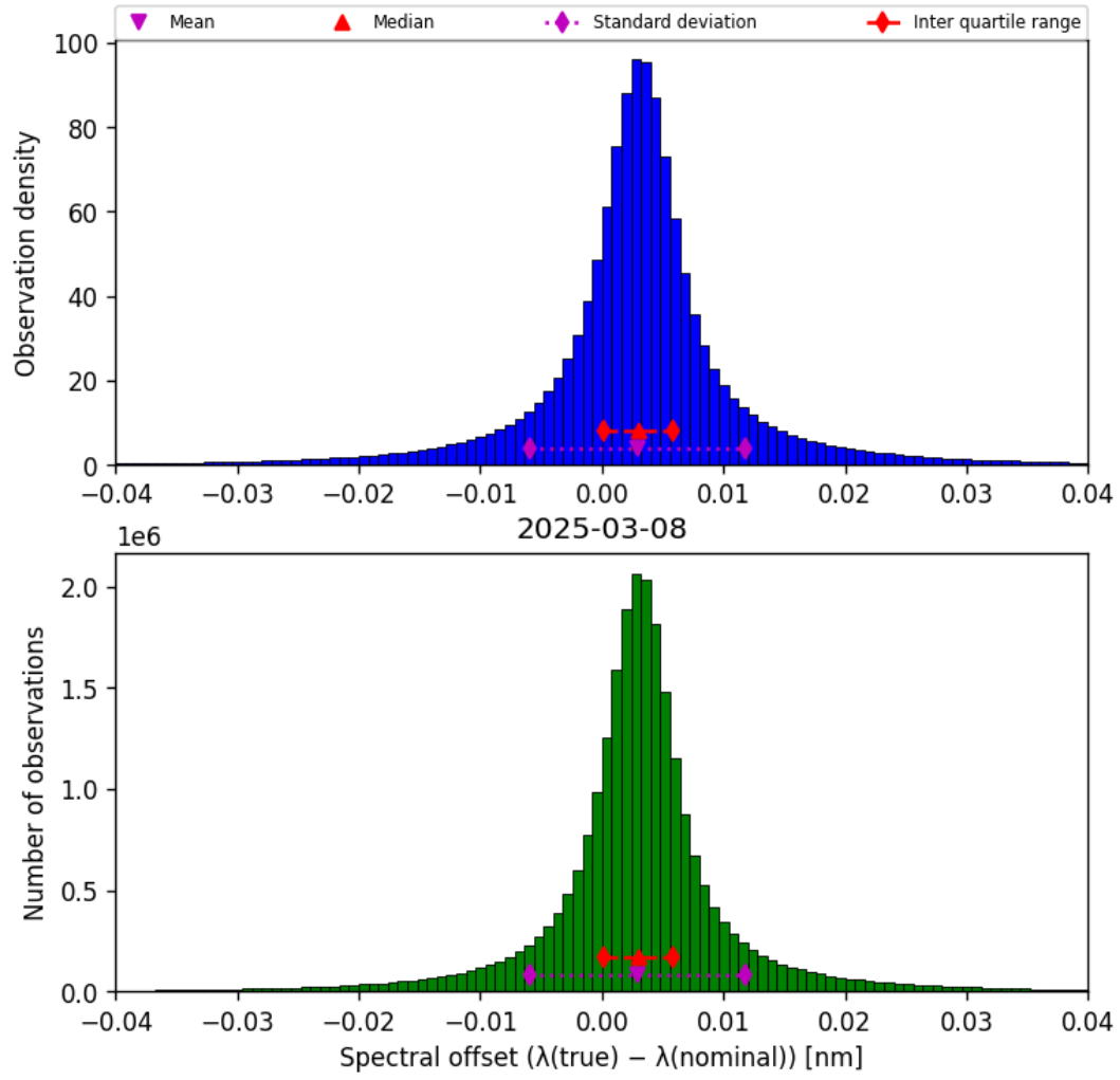
Figure 45: Histogram of “Spectral offset ( \lambda_{\text{true}} - \lambda_{\text{nominal}} )” for 2025-03-07 to 2025-03-09
