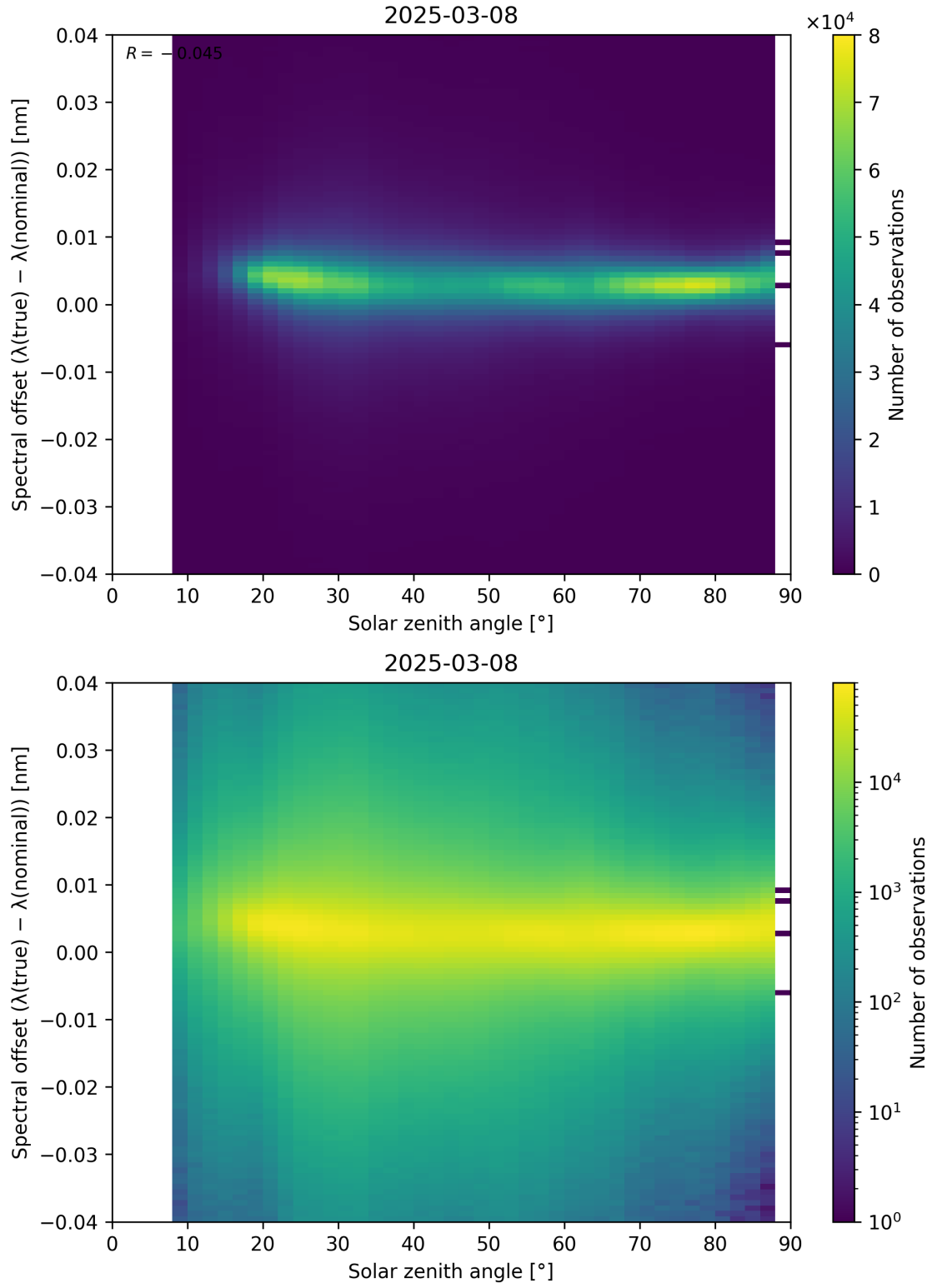
Figure 117: Scatter density plot of “Solar zenith angle” against “Spectral offset ( \lambda_{\text{true}} - \lambda_{\text{nominal}} )” for 2025-03-07 to 2025-03-09.
