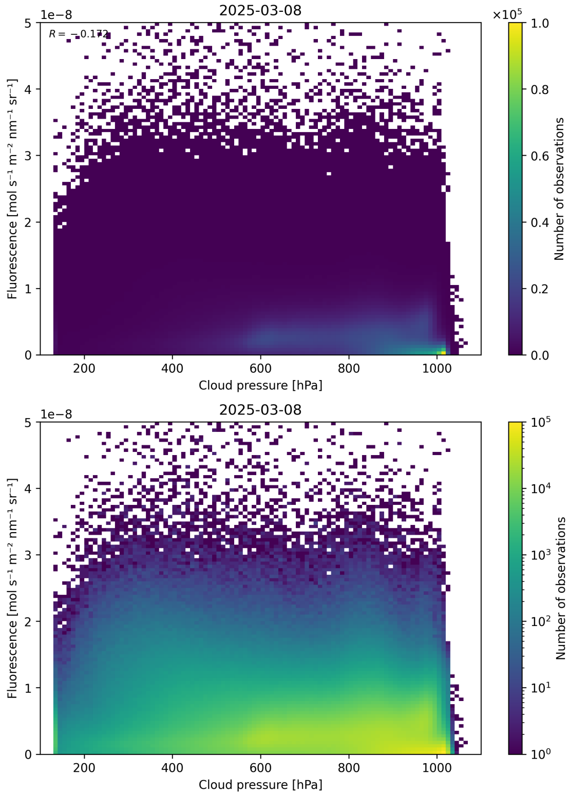
Figure 80: Scatter density plot of “Cloud pressure” against “Fluorescence” for 2025-03-07 to 2025-03-09.
