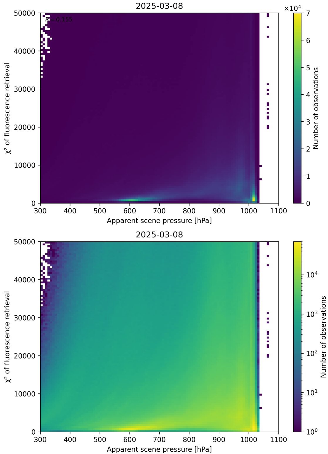
Figure 63: Scatter density plot of “Apparent scene pressure” against “ \chi^2 of fluorescence retrieval” for 2025-03-07 to 2025-03-09.
