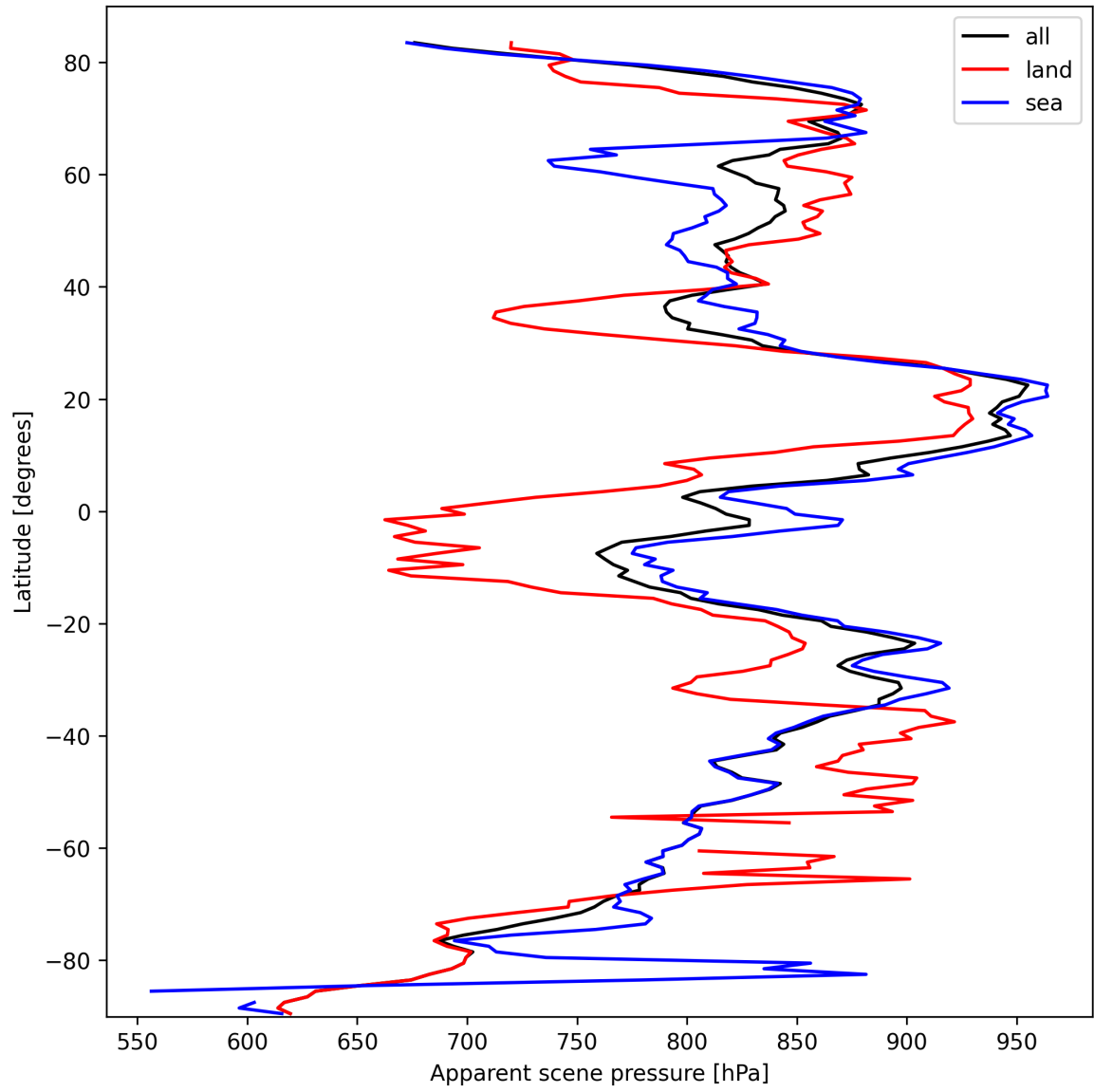
Figure 19: Zonal average of “Apparent scene pressure” for 2025-03-07 to 2025-03-09.
