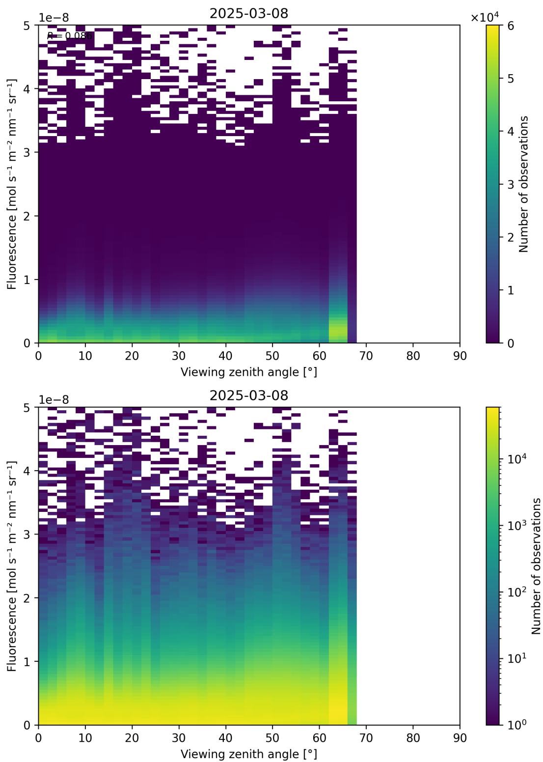
Figure 122: Scatter density plot of “Viewing zenith angle” against “Fluorescence” for 2025-03-07 to 2025-03-09.
