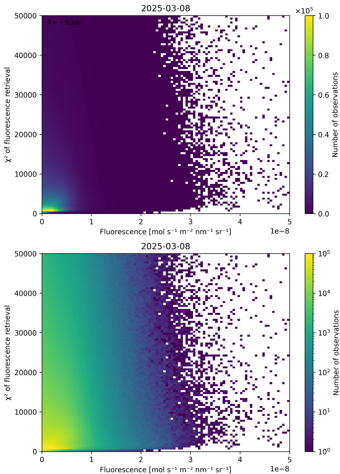
Figure 85: Scatter density plot of “Fluorescence” against “ \chi^2 of fluorescence retrieval” for 2025-03-07 to 2025-03-09.
