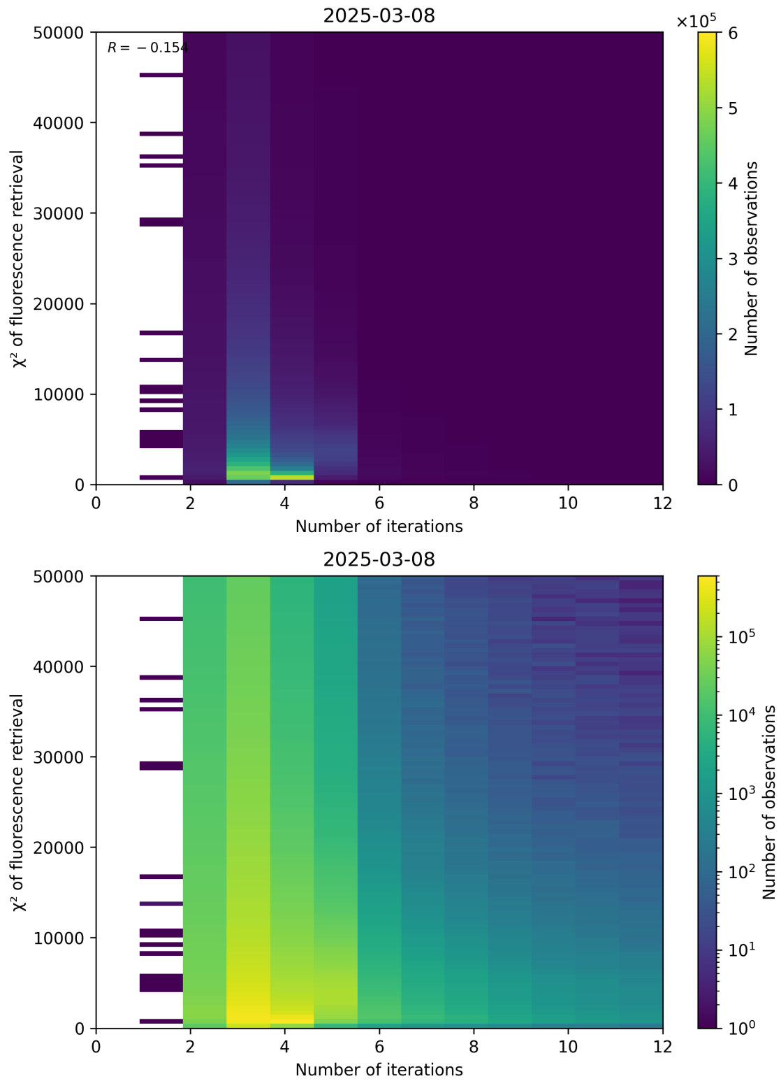
Figure 97: Scatter density plot of “Number of iterations” against “ \chi^2 of fluorescence retrieval” for 2025-03-07 to 2025-03-09.
