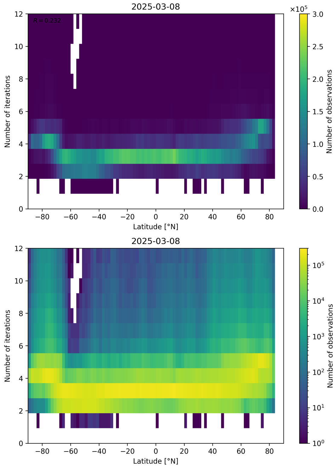
Figure 93: Scatter density plot of “Latitude” against “Number of iterations” for 2025-03-07 to 2025-03-09.
