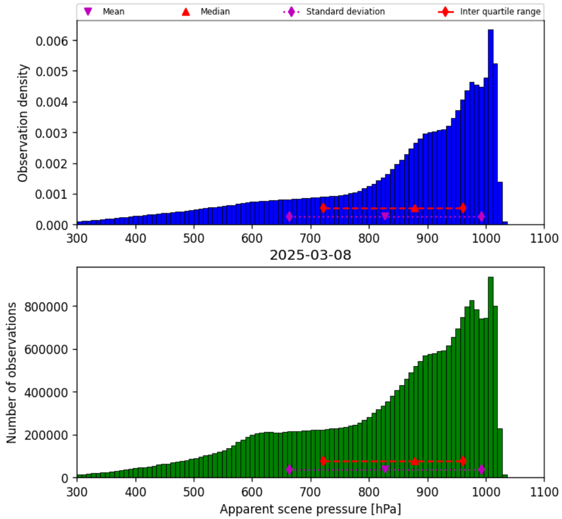
Figure 36: Histogram of “Apparent scene pressure” for 2025-03-07 to 2025-03-09
