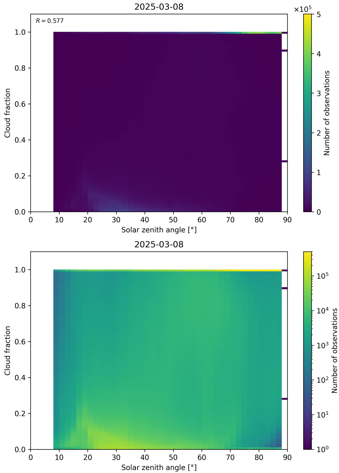
Figure 110: Scatter density plot of “Solar zenith angle” against “Cloud fraction” for 2025-03-07 to 2025-03-09.
