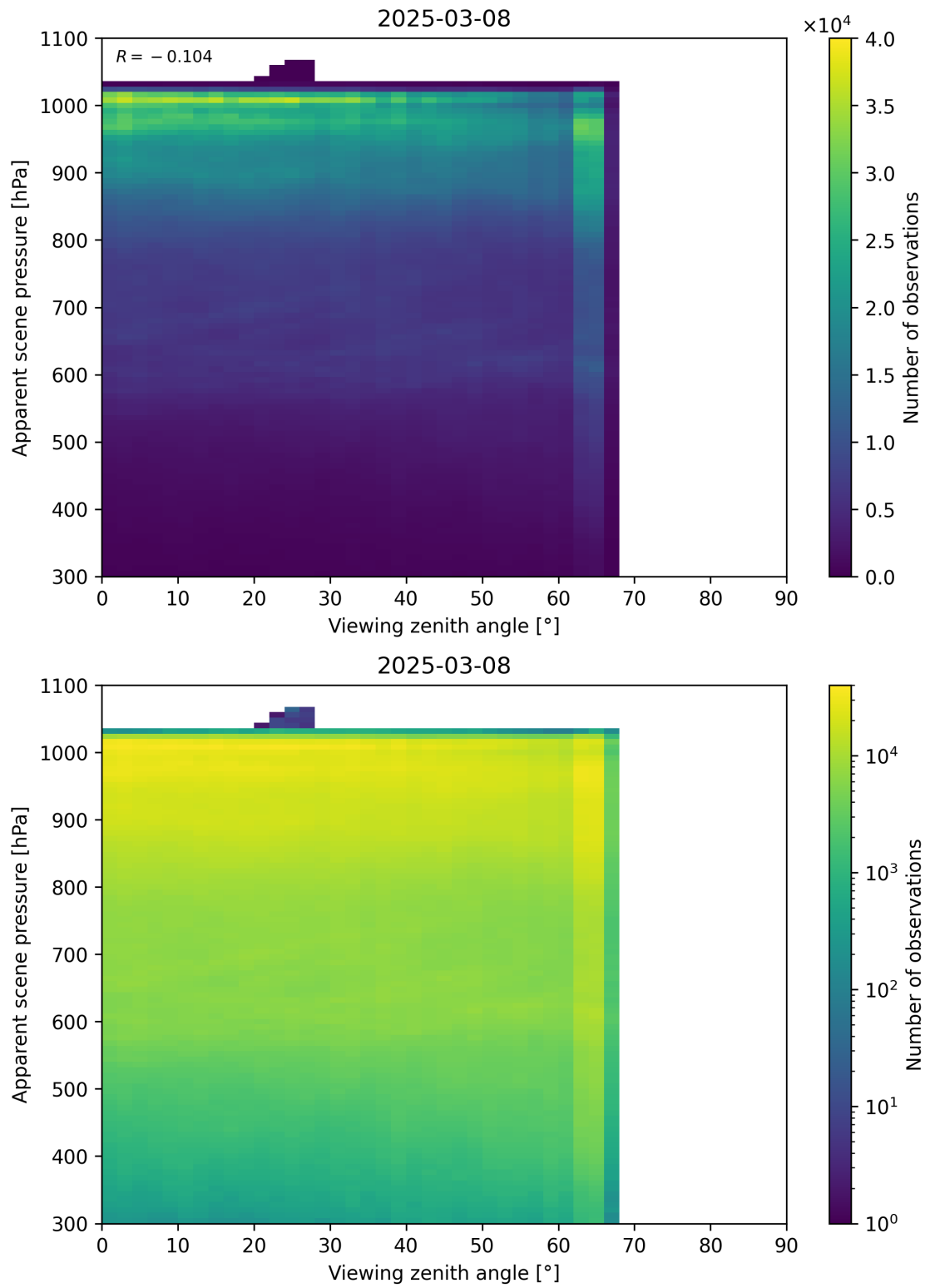
Figure 118: Scatter density plot of “Viewing zenith angle” against “Apparent scene pressure” for 2025-03-07 to 2025-03-09.
