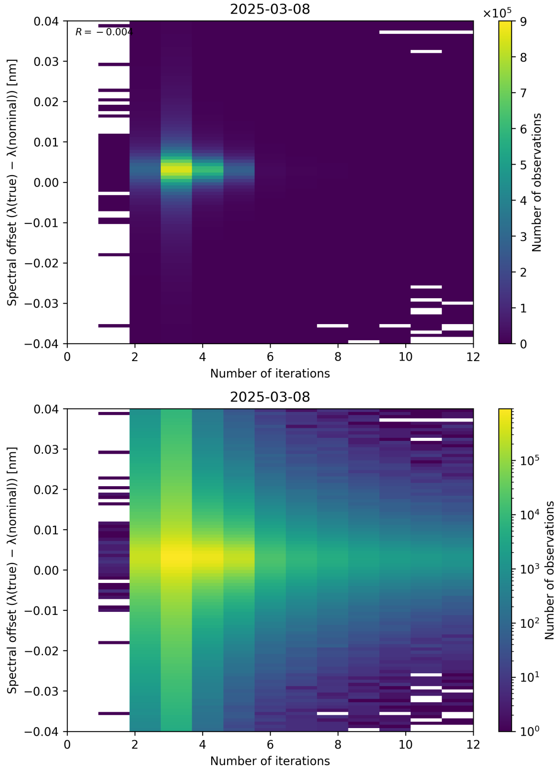
Figure 100: Scatter density plot of “Number of iterations” against “Spectral offset ( \lambda_{\text{true}} - \lambda_{\text{nominal}} )” for 2025-03-07 to 2025-03-09.
