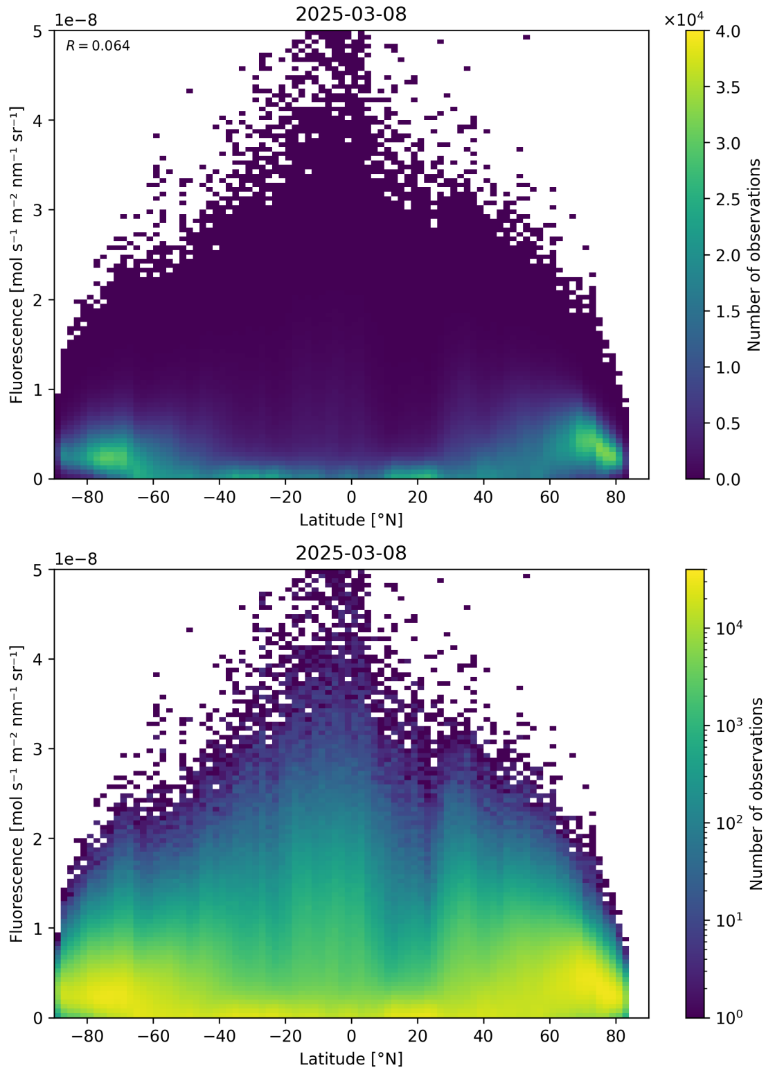
Figure 92: Scatter density plot of “Latitude” against “Fluorescence” for 2025-03-07 to 2025-03-09.
