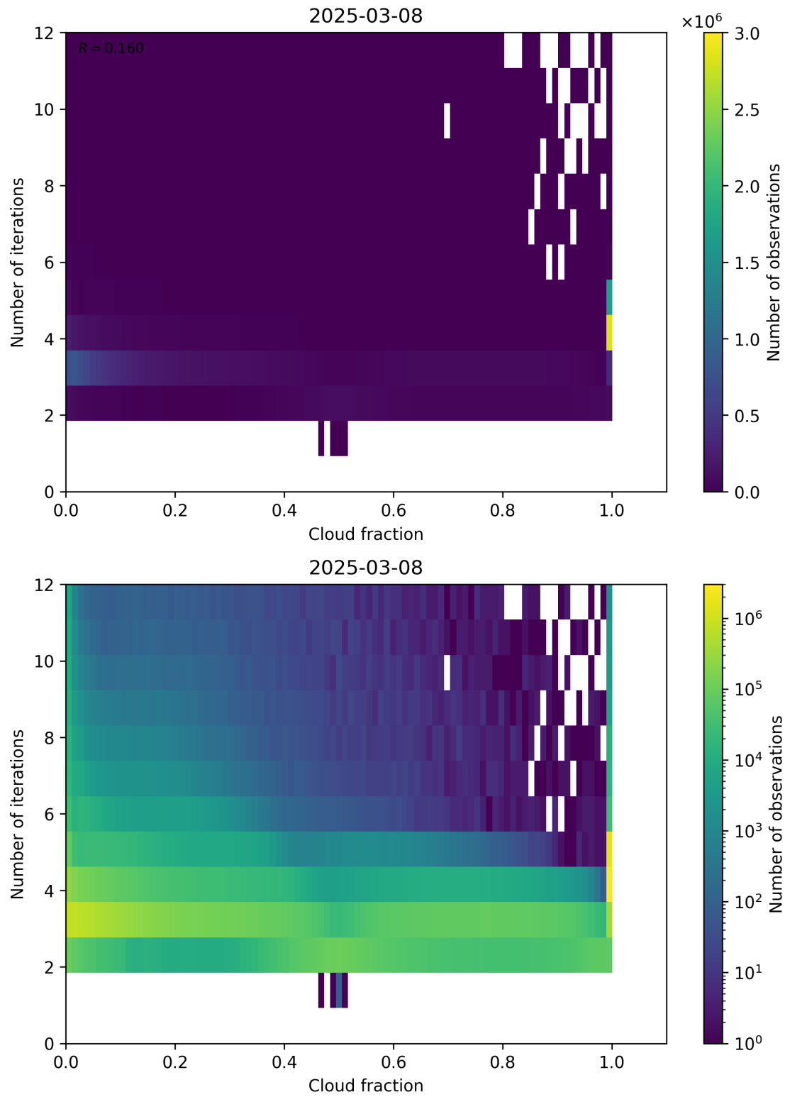
Figure 73: Scatter density plot of “Cloud fraction” against “Number of iterations” for 2025-03-07 to 2025-03-09.
