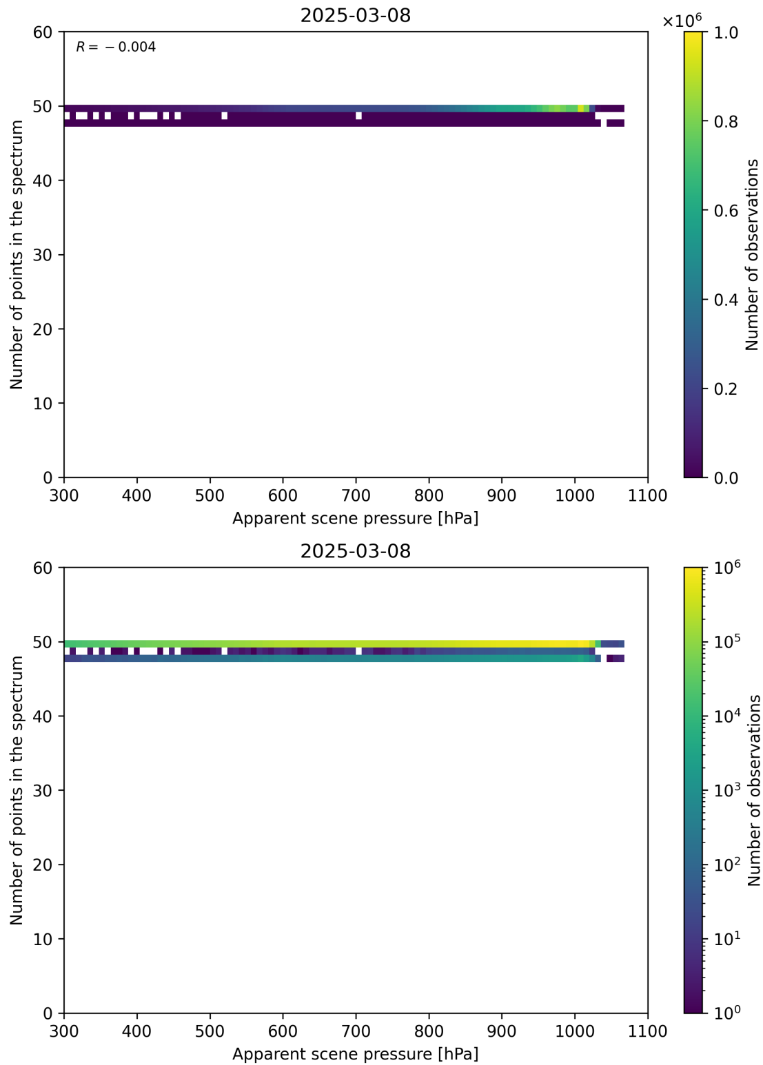
Figure 66: Scatter density plot of “Apparent scene pressure” against “Number of points in the spectrum” for 2025-03-07 to 2025-03-09.
