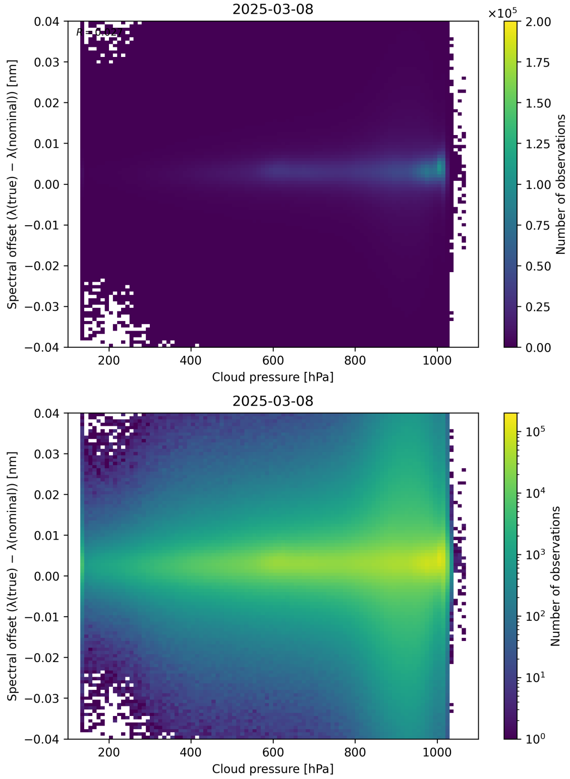
Figure 84: Scatter density plot of “Cloud pressure” against “Spectral offset ( \lambda_{\text{true}} - \lambda_{\text{nominal}} )” for 2025-03-07 to 2025-03-09.
