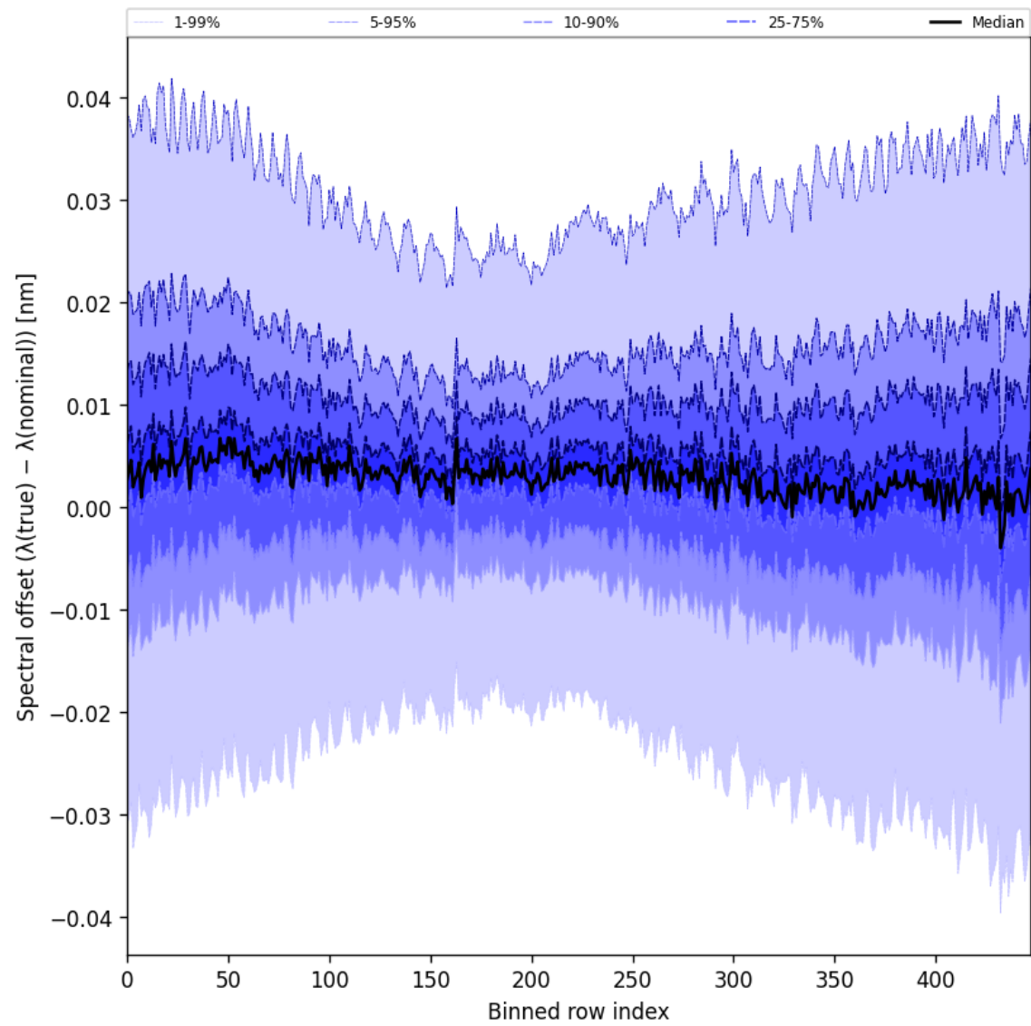
Figure 62: Along track statistics of “Spectral offset ( \lambda_{\text{true}} - \lambda_{\text{nominal}} )” for 2025-03-07 to 2025-03-09
