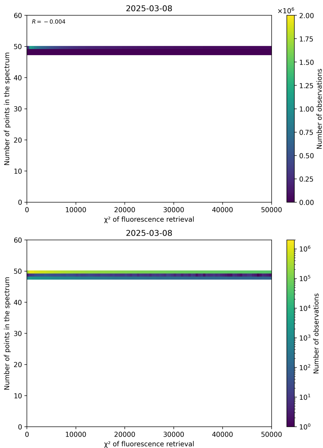
Figure 68: Scatter density plot of “ \chi^2 of fluorescence retrieval” against “Number of points in the spectrum” for 2025-03-07 to 2025-03-09.
