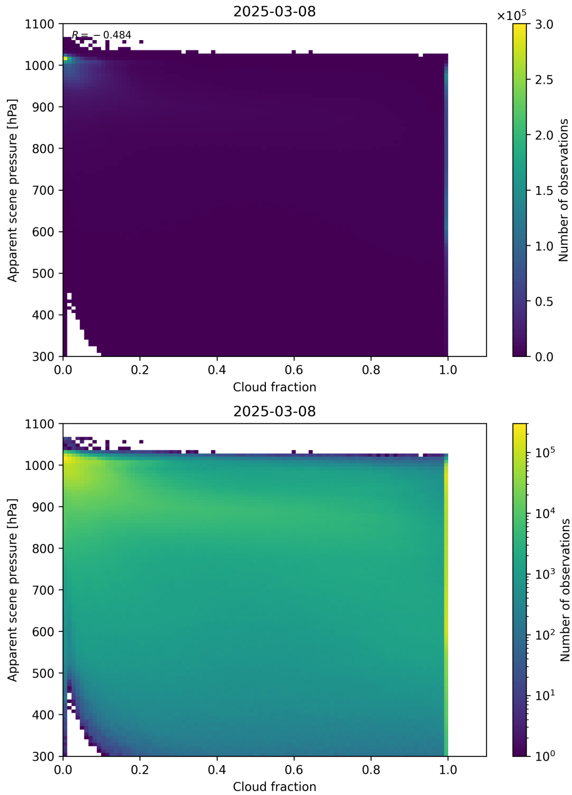
Figure 70: Scatter density plot of “Cloud fraction” against “Apparent scene pressure” for 2025-03-07 to 2025-03-09.
