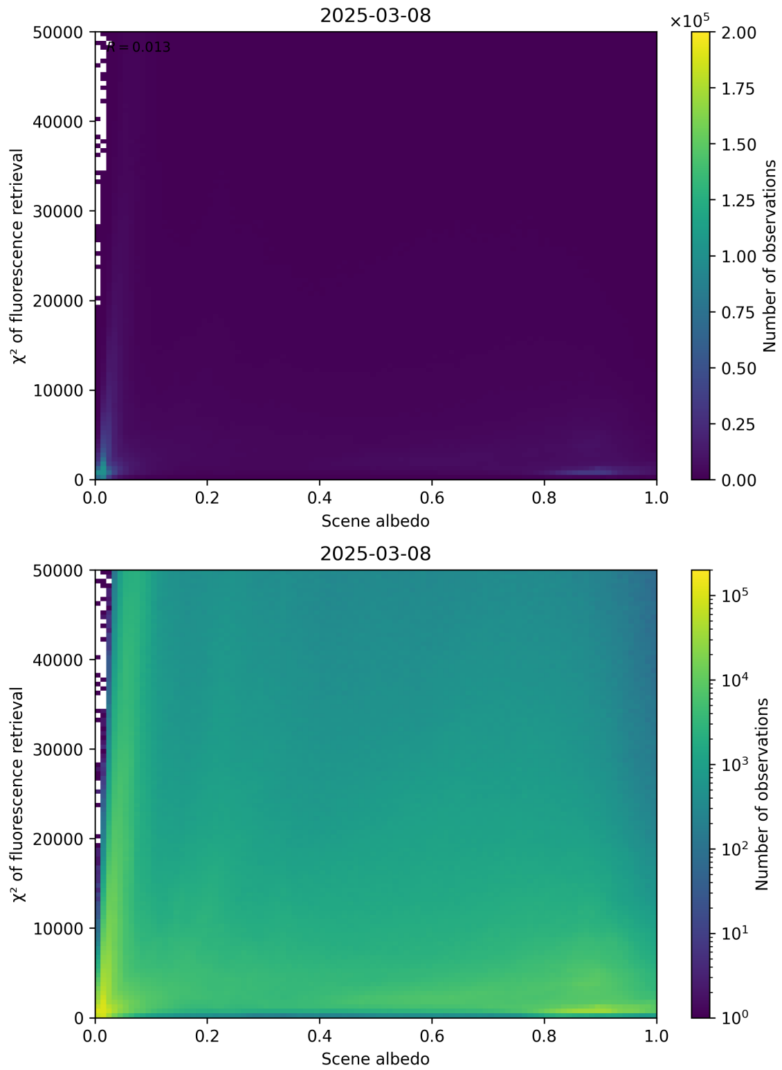
Figure 103: Scatter density plot of “Scene albedo” against “ \chi^2 of fluorescence retrieval” for 2025-03-07 to 2025-03-09.
