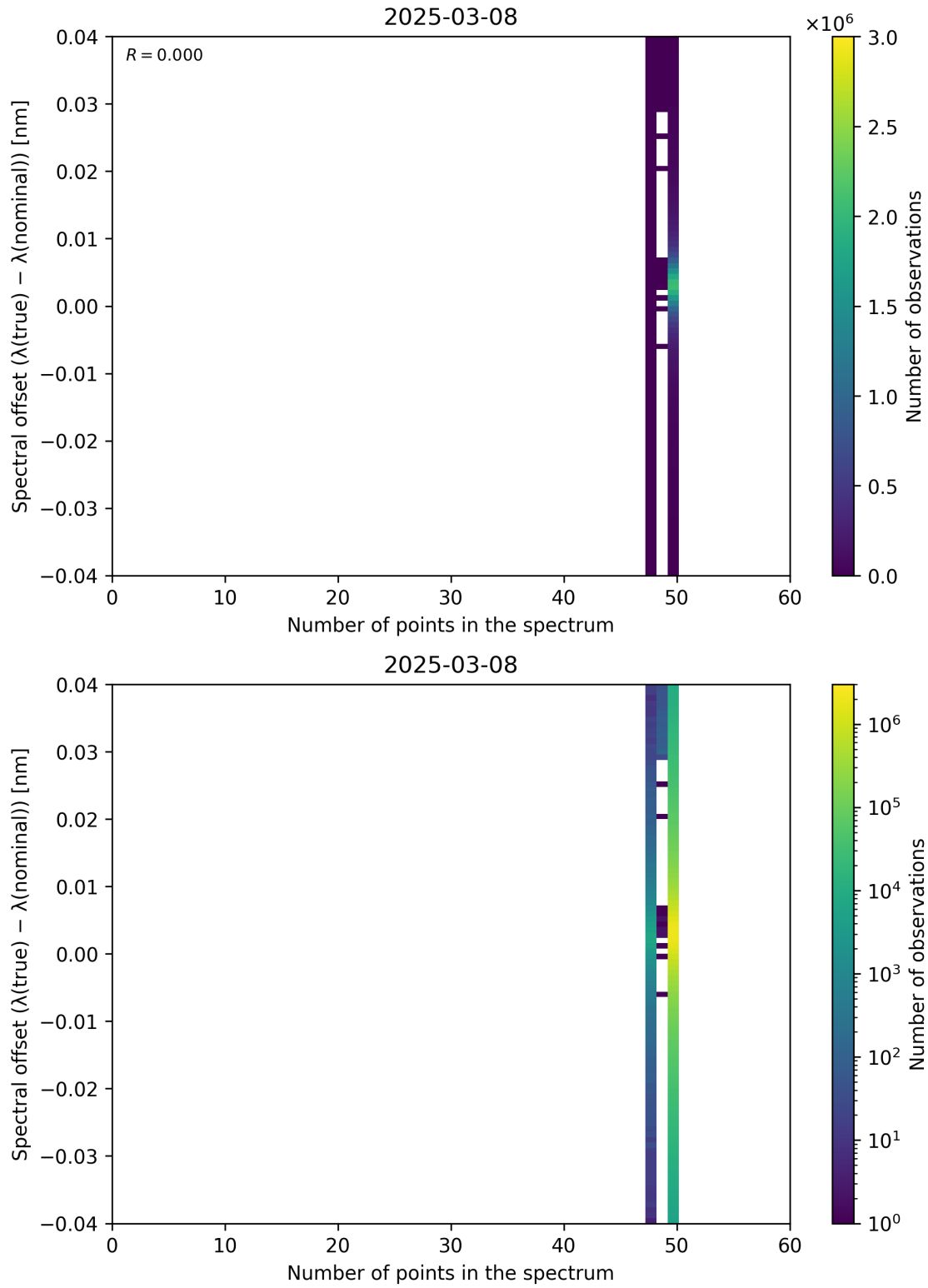
Figure 101: Scatter density plot of “Number of points in the spectrum” against “Spectral offset ( \lambda_{\text{true}} - \lambda_{\text{nominal}} )” for 2025-03-07 to 2025-03-09.
