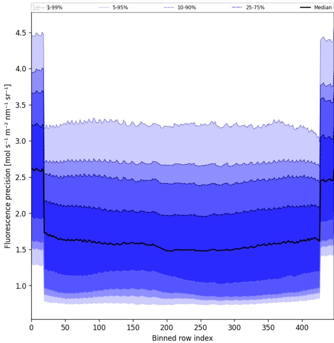
Figure 58: Along track statistics of “Fluorescence precision” for 2025-03-07 to 2025-03-09
