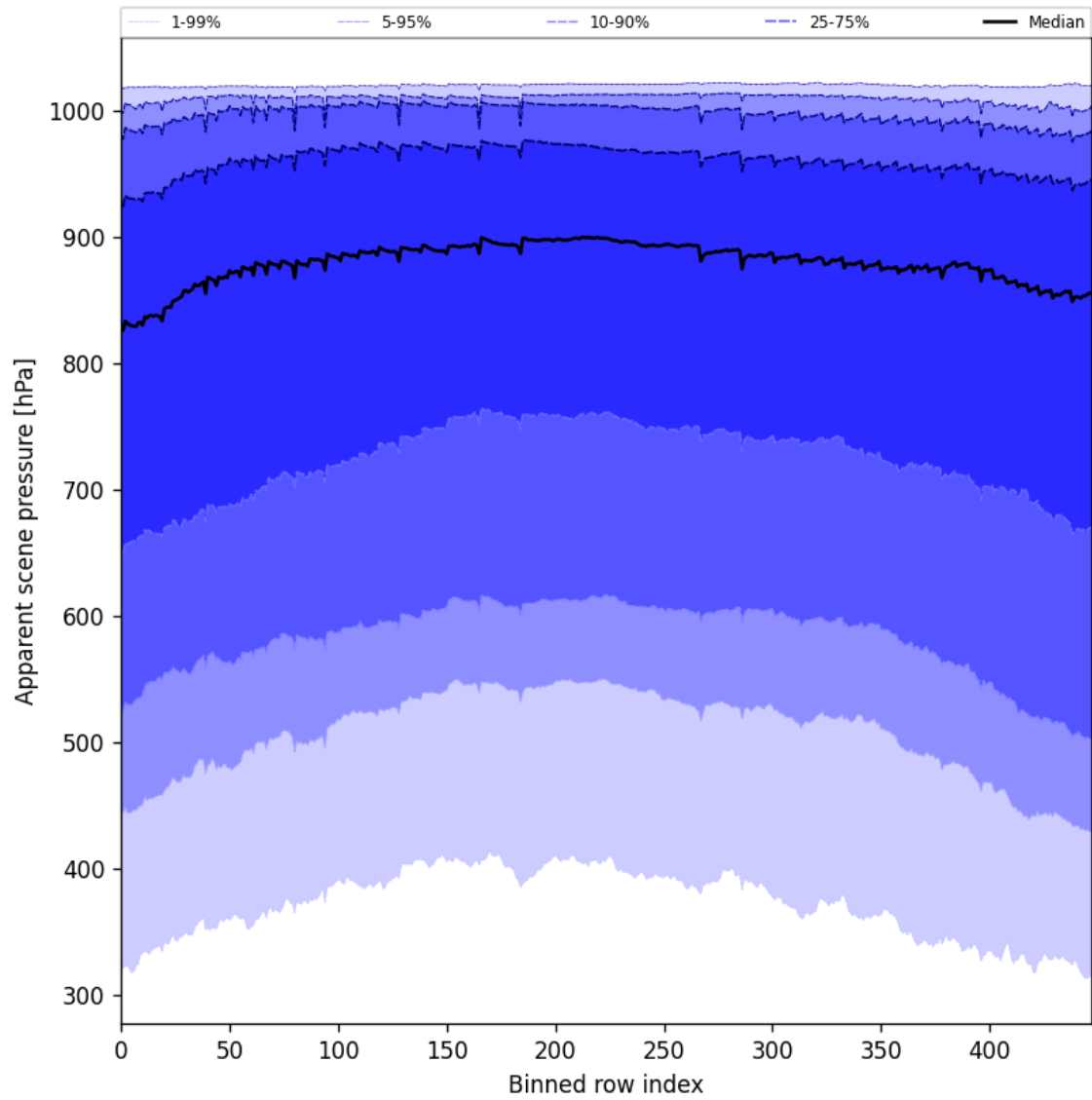
Figure 53: Along track statistics of “Apparent scene pressure” for 2025-03-07 to 2025-03-09
