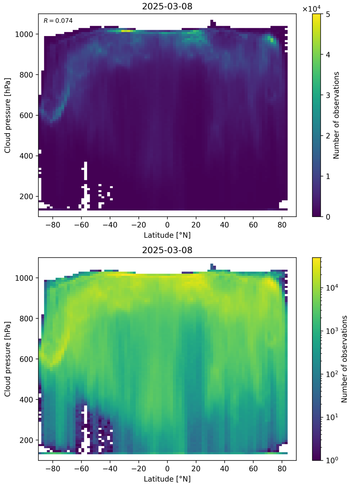
Figure 91: Scatter density plot of “Latitude” against “Cloud pressure” for 2025-03-07 to 2025-03-09.
