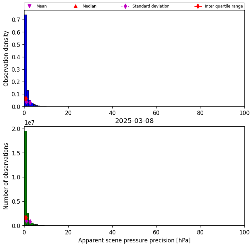
Figure 37: Histogram of “Apparent scene pressure precision” for 2025-03-07 to 2025-03-09
