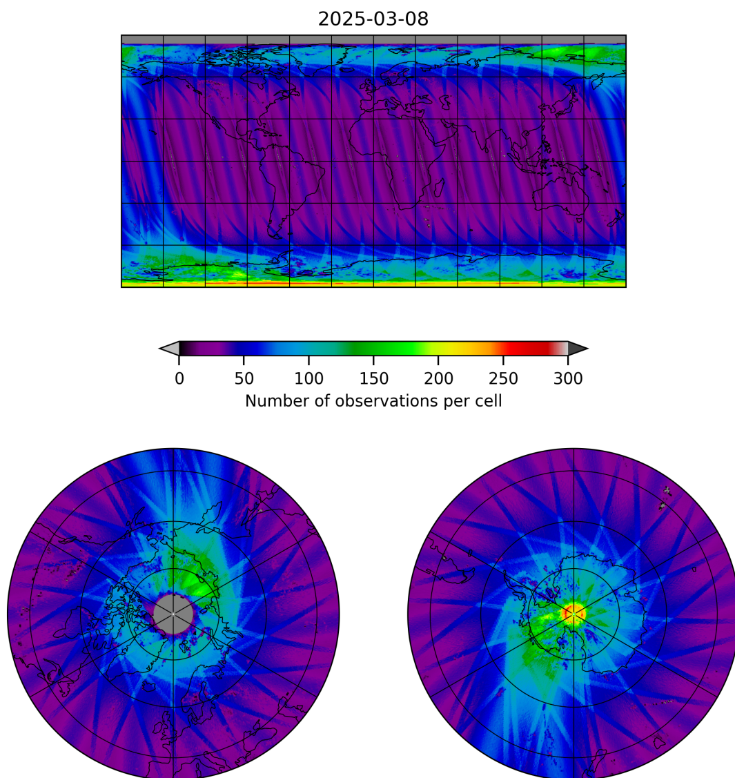
Figure 11: Map of the number of observations for 2025-03-07 to 2025-03-09
