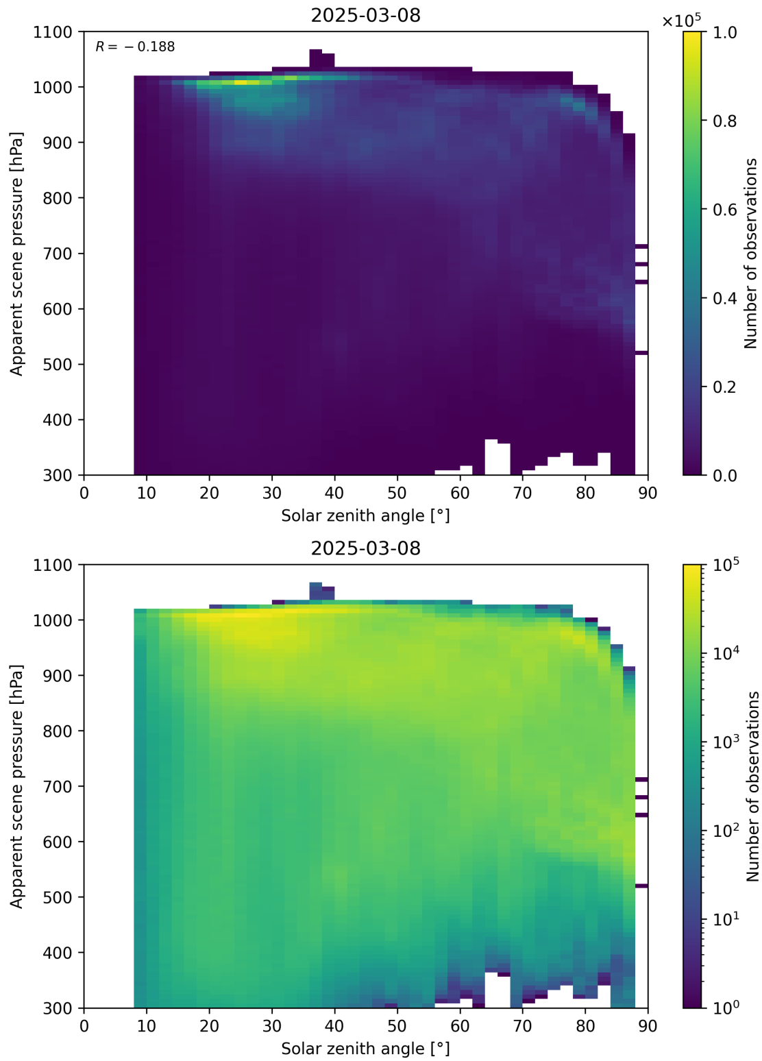
Figure 108: Scatter density plot of “Solar zenith angle” against “Apparent scene pressure” for 2025-03-07 to 2025-03-09.
