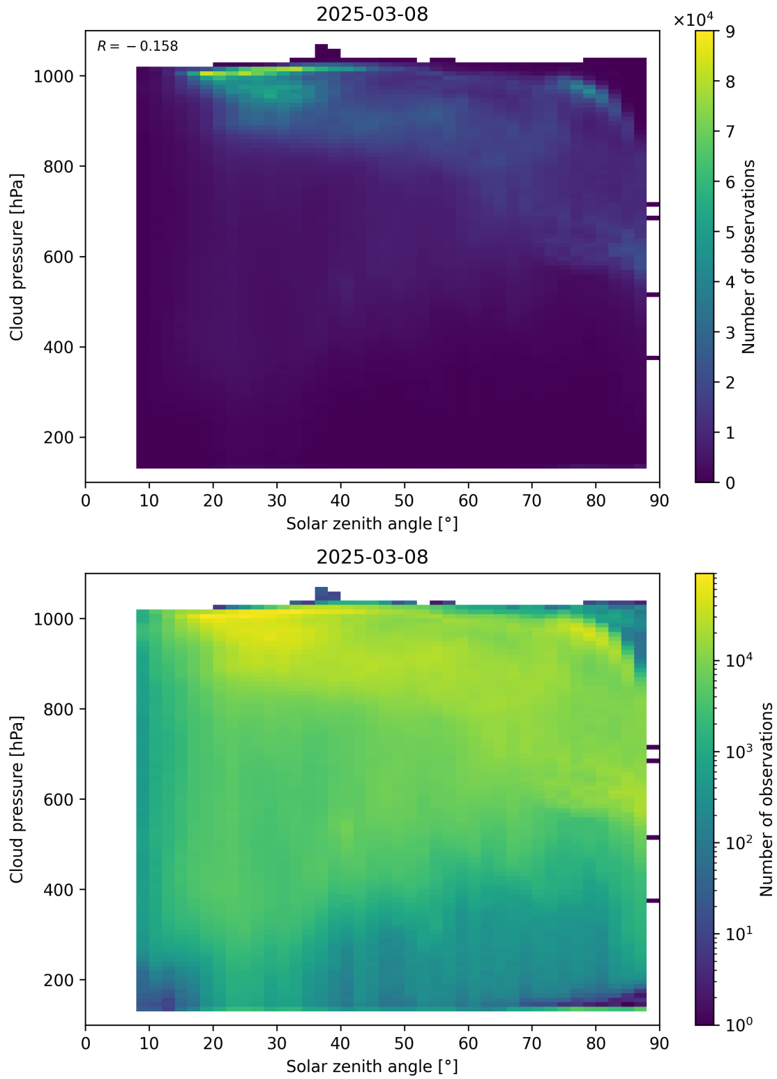
Figure 111: Scatter density plot of “Solar zenith angle” against “Cloud pressure” for 2025-03-07 to 2025-03-09.
