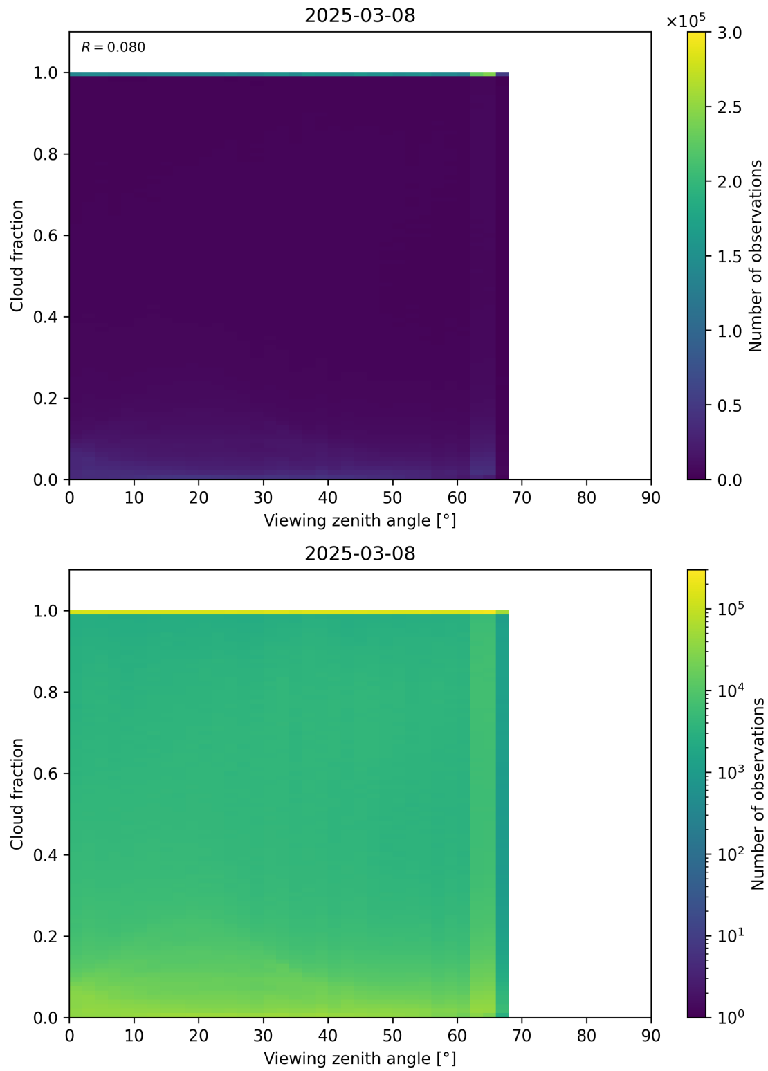
Figure 120: Scatter density plot of “Viewing zenith angle” against “Cloud fraction” for 2025-03-07 to 2025-03-09.
