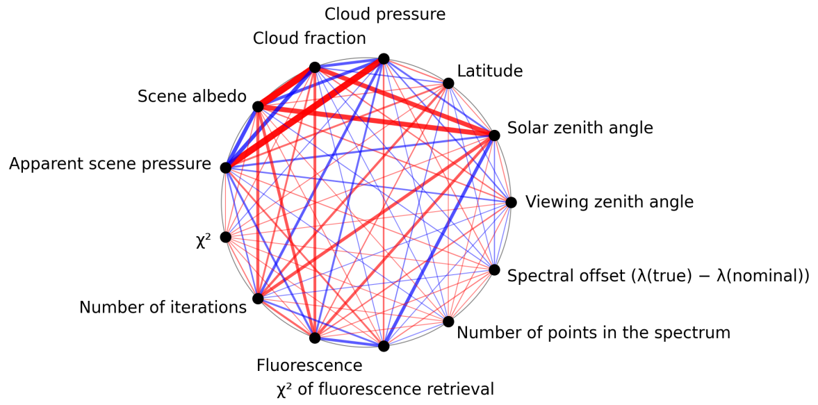
Figure 1: Map of correlation graph for 2025-03-07 to 2025-03-09.
