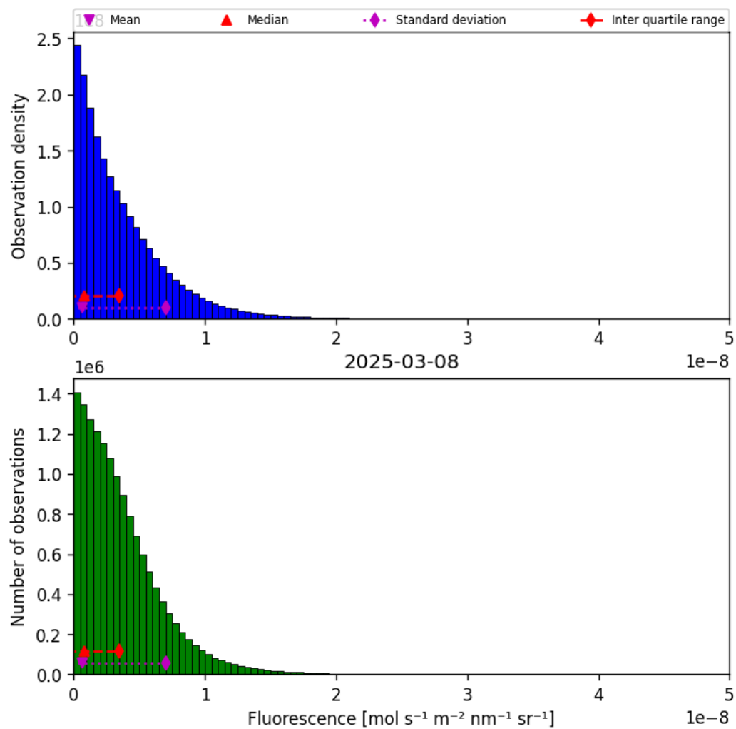
Figure 40: Histogram of “Fluorescence” for 2025-03-07 to 2025-03-09
