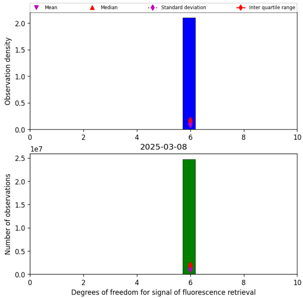
Figure 43: Histogram of “Degrees of freedom for signal of fluorescence retrieval” for 2025-03-07 to 2025-03-09
