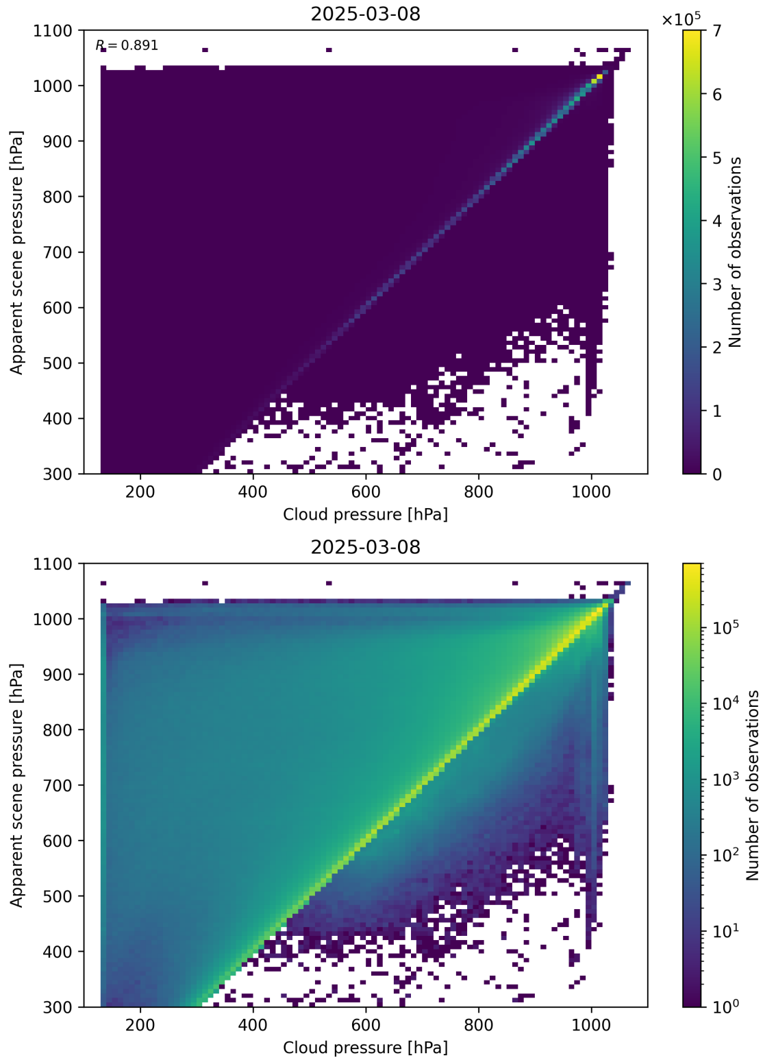
Figure 77: Scatter density plot of “Cloud pressure” against “Apparent scene pressure” for 2025-03-07 to 2025-03-09.
