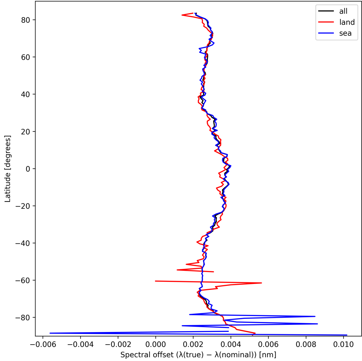
Figure 28: Zonal average of “Spectral offset ( \lambda_{\text{true}} - \lambda_{\text{nominal}} )” for 2025-03-07 to 2025-03-09.
