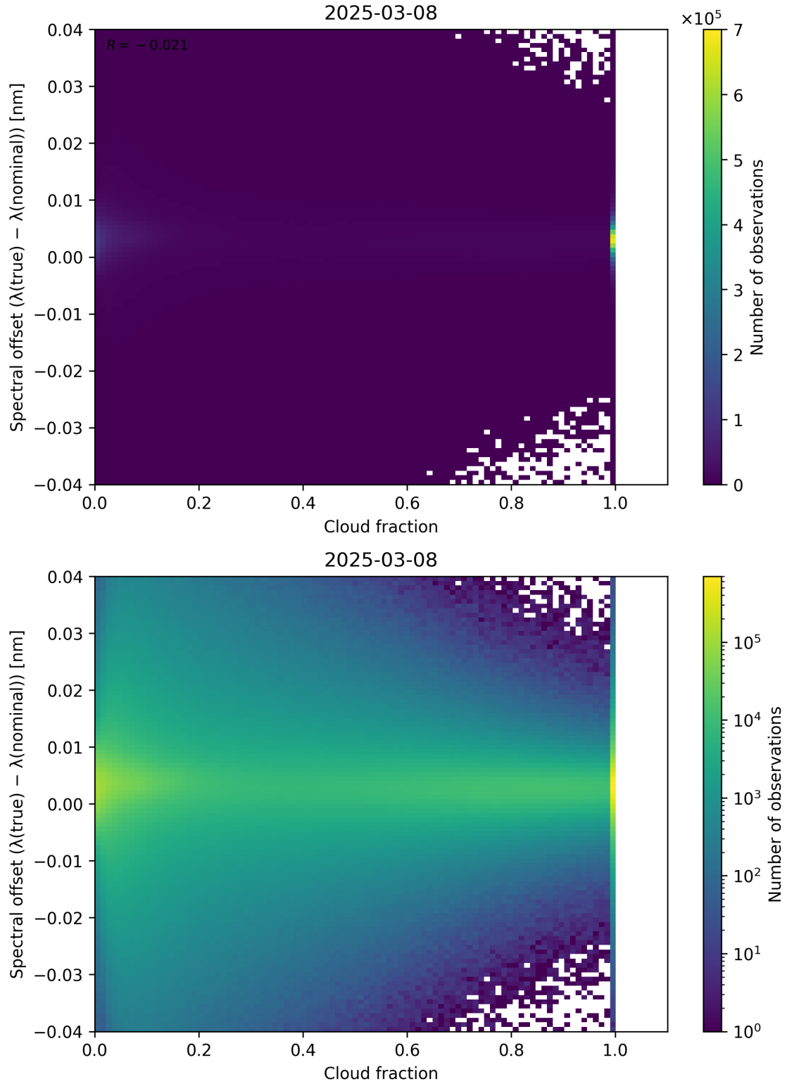
Figure 76: Scatter density plot of “Cloud fraction” against “Spectral offset ( \lambda_{\text{true}} - \lambda_{\text{nominal}} )” for 2025-03-07 to 2025-03-09.
