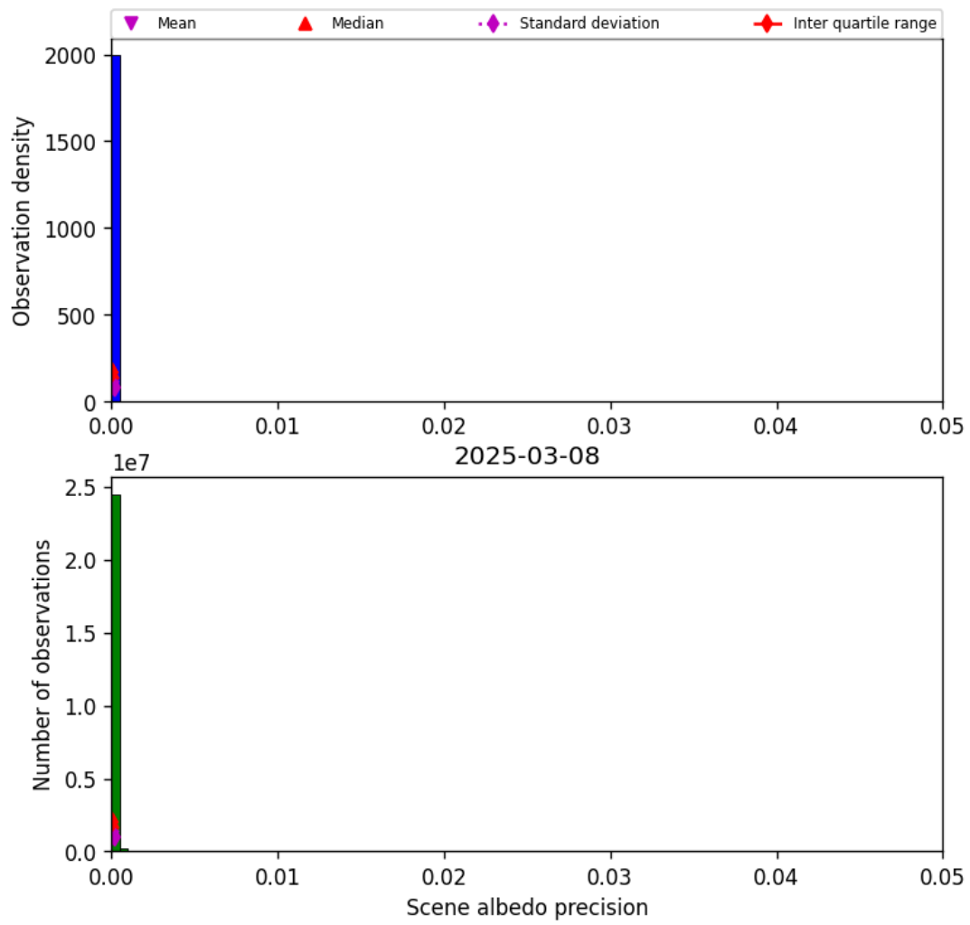
Figure 35: Histogram of “Scene albedo precision” for 2025-03-07 to 2025-03-09
