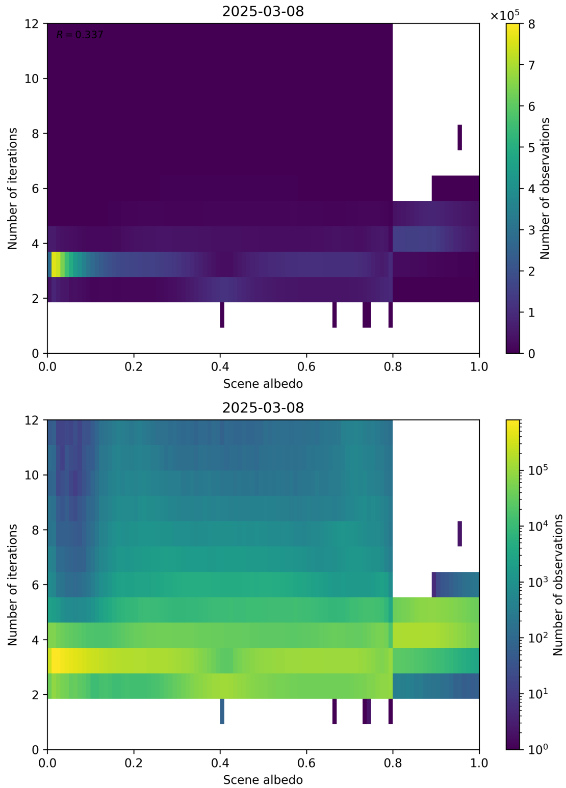
Figure 105: Scatter density plot of “Scene albedo” against “Number of iterations” for 2025-03-07 to 2025-03-09.
