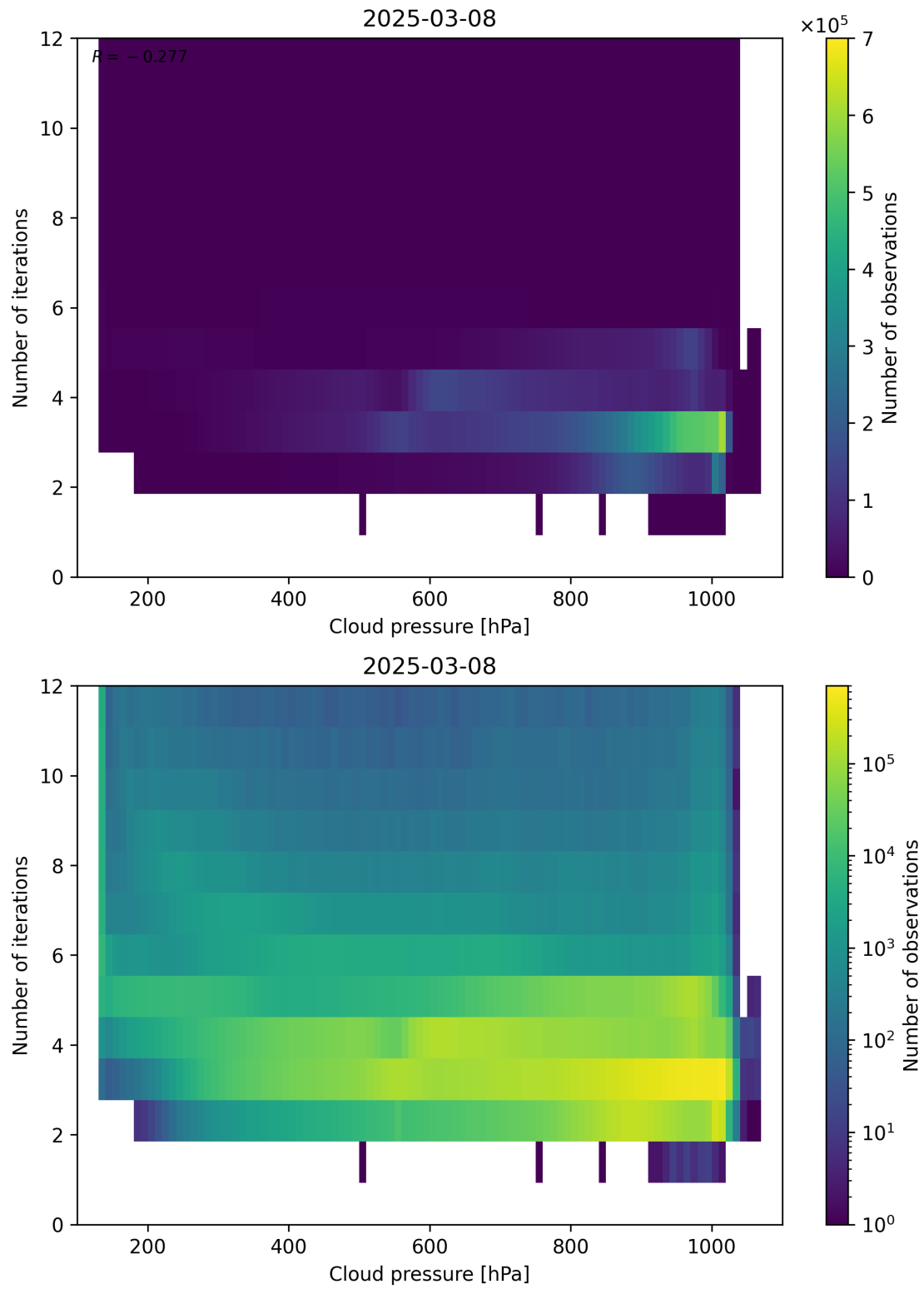
Figure 81: Scatter density plot of “Cloud pressure” against “Number of iterations” for 2025-03-07 to 2025-03-09.
