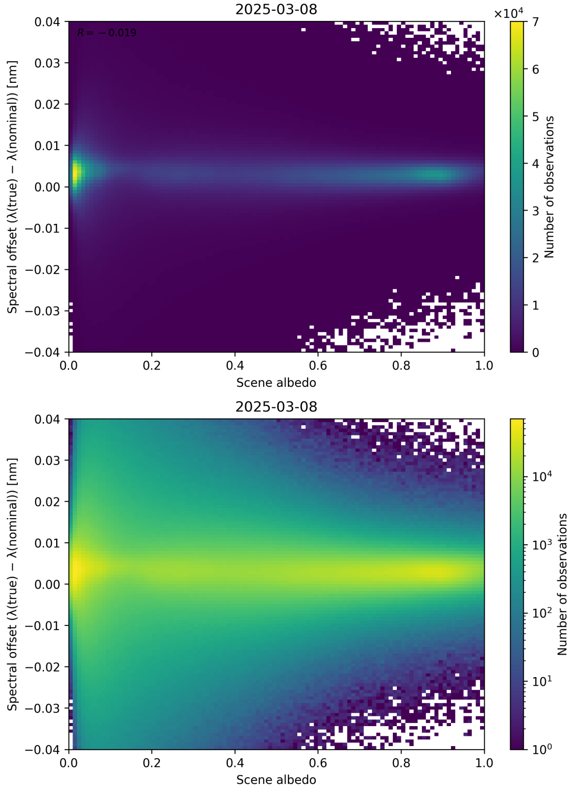
Figure 107: Scatter density plot of “Scene albedo” against “Spectral offset ( \lambda_{\text{true}} - \lambda_{\text{nominal}} )” for 2025-03-07 to 2025-03-09.
