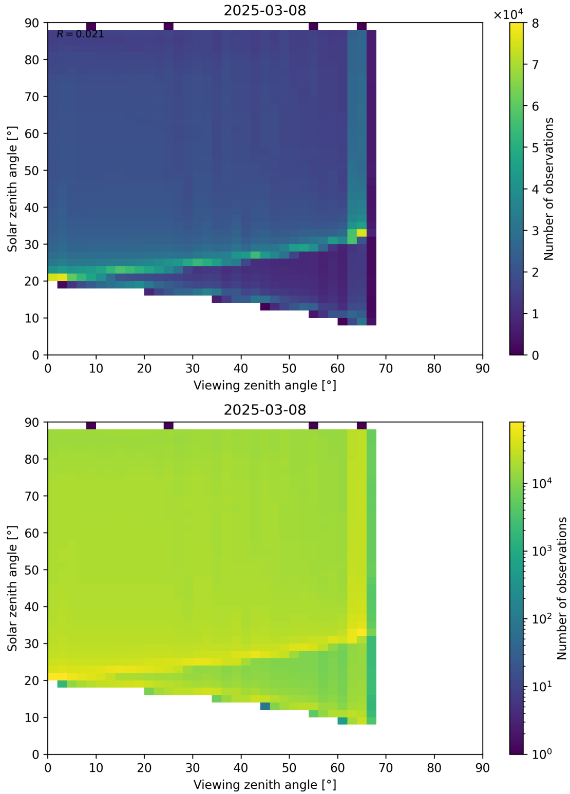
Figure 127: Scatter density plot of “Viewing zenith angle” against “Solar zenith angle” for 2025-03-07 to 2025-03-09.
