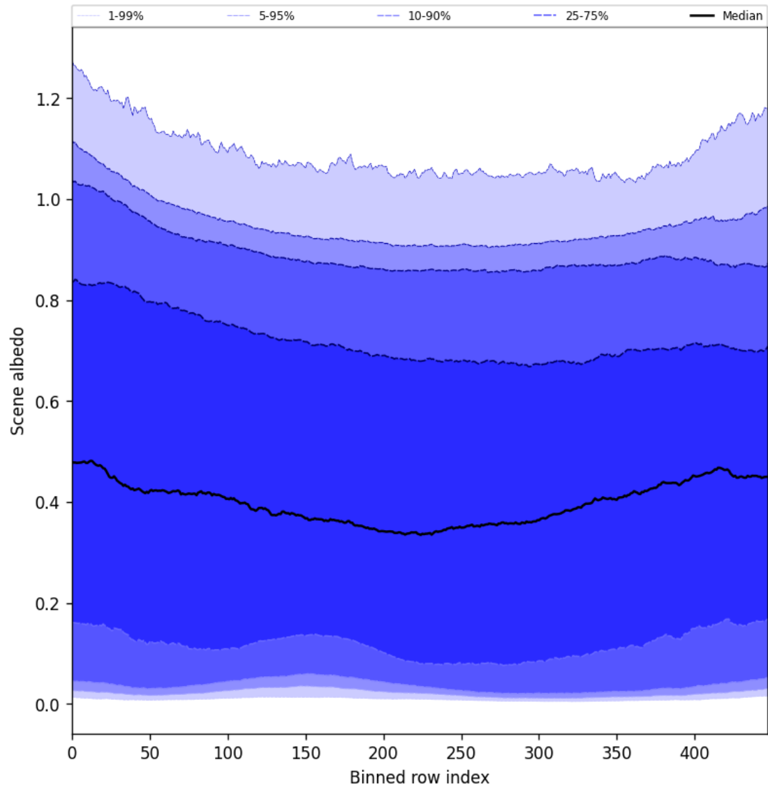
Figure 51: Along track statistics of “Scene albedo” for 2025-03-07 to 2025-03-09
