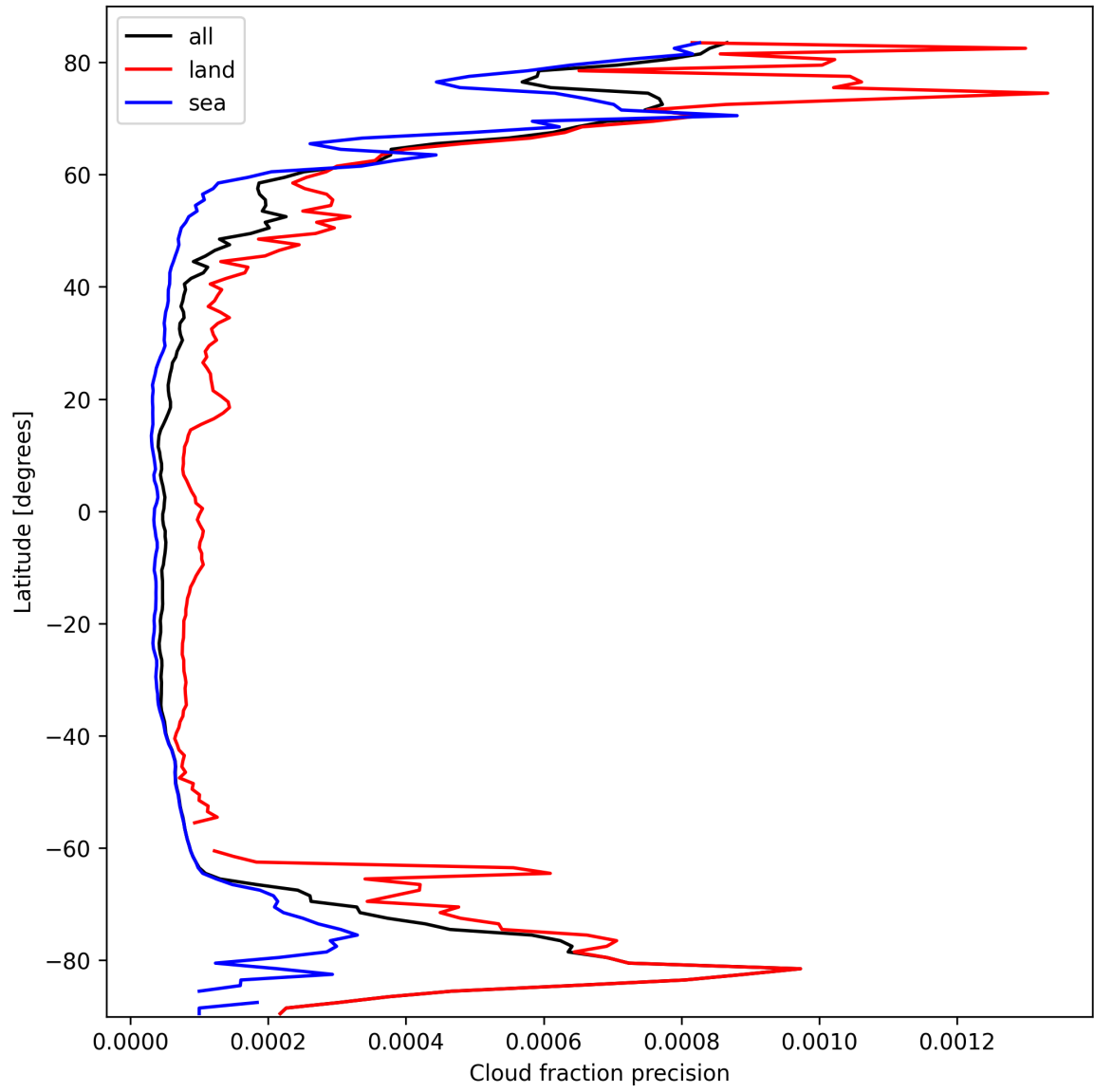
Figure 16: Zonal average of “Cloud fraction precision” for 2025-03-07 to 2025-03-09.
