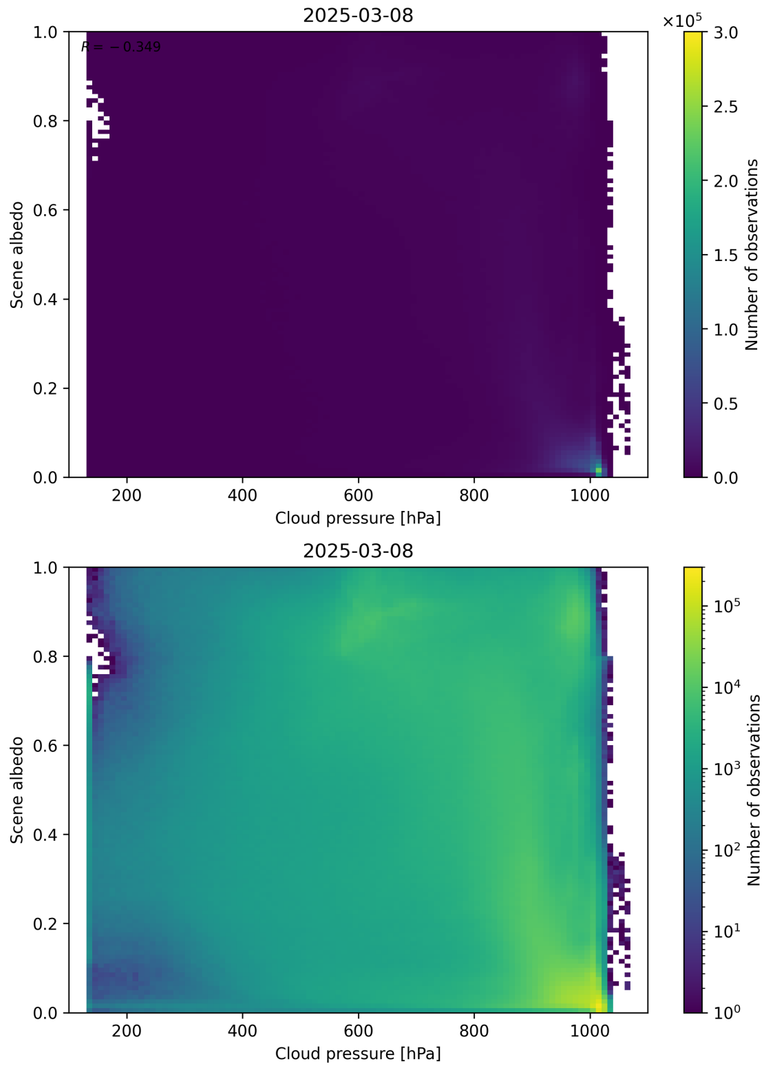
Figure 83: Scatter density plot of “Cloud pressure” against “Scene albedo” for 2025-03-07 to 2025-03-09.
