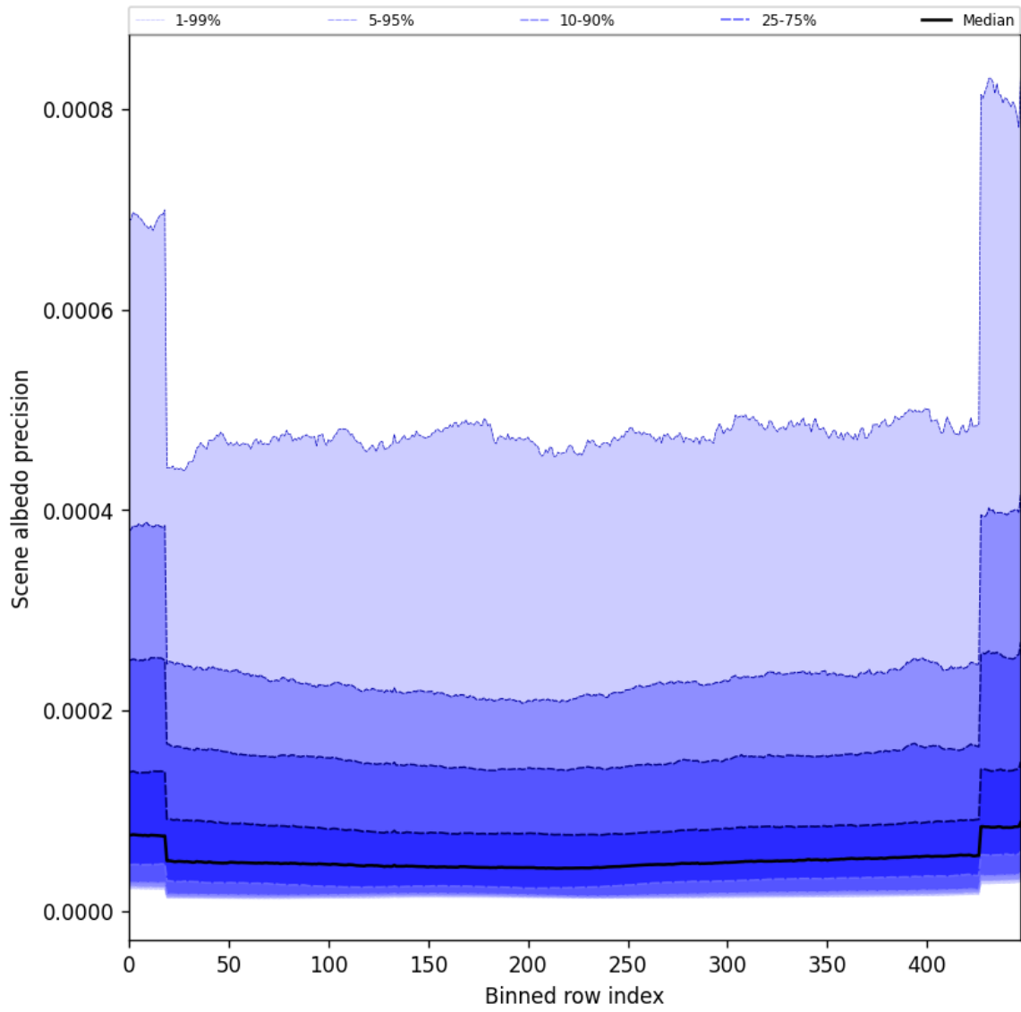
Figure 52: Along track statistics of “Scene albedo precision” for 2025-03-07 to 2025-03-09
