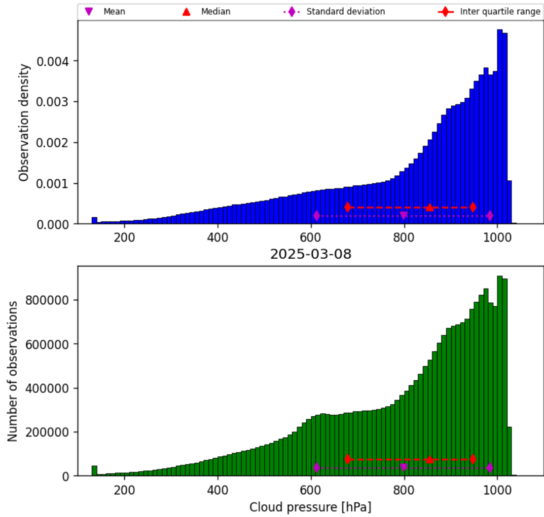
Figure 30: Histogram of “Cloud pressure” for 2025-03-07 to 2025-03-09
