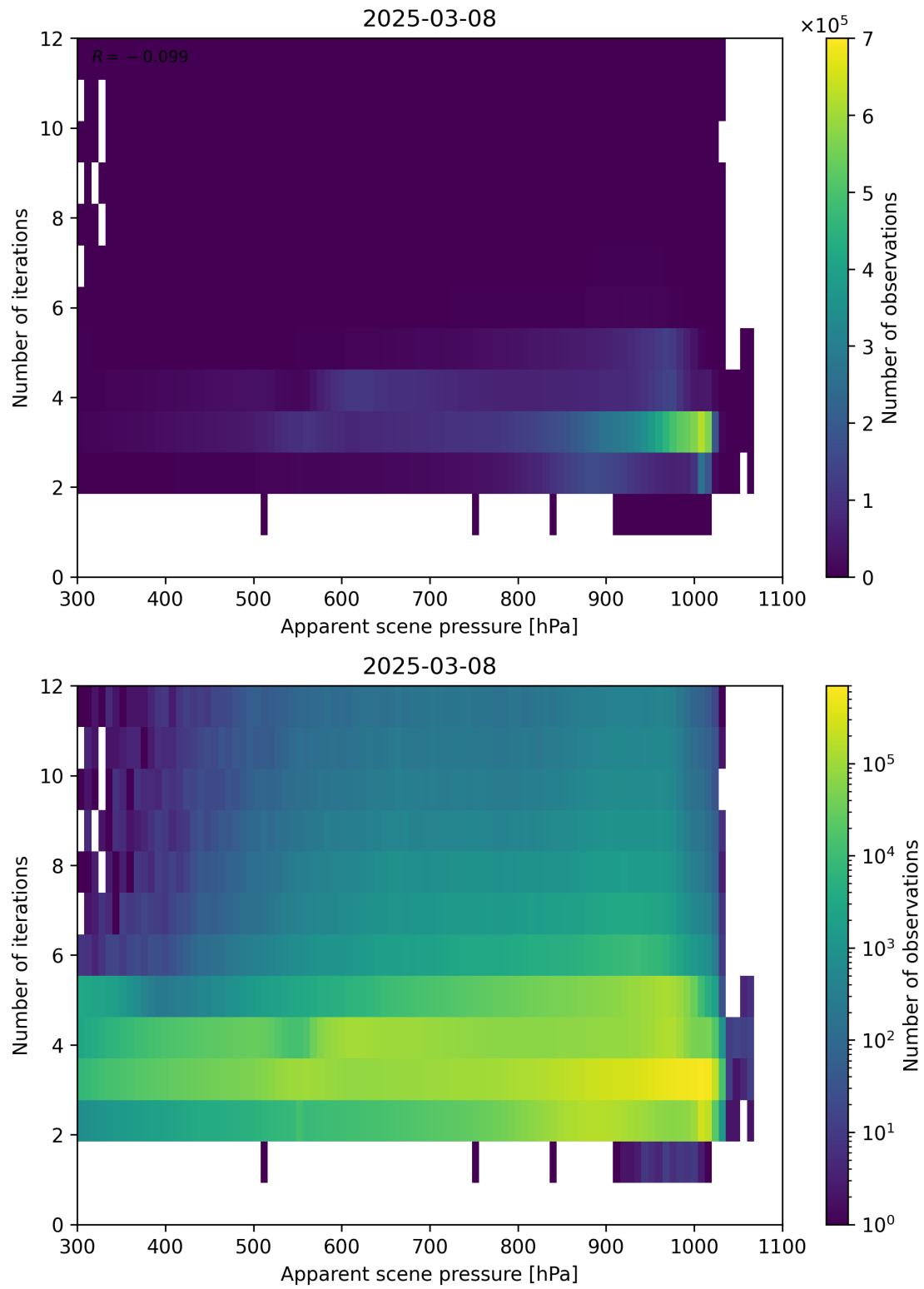
Figure 65: Scatter density plot of “Apparent scene pressure” against “Number of iterations” for 2025-03-07 to 2025-03-09.
