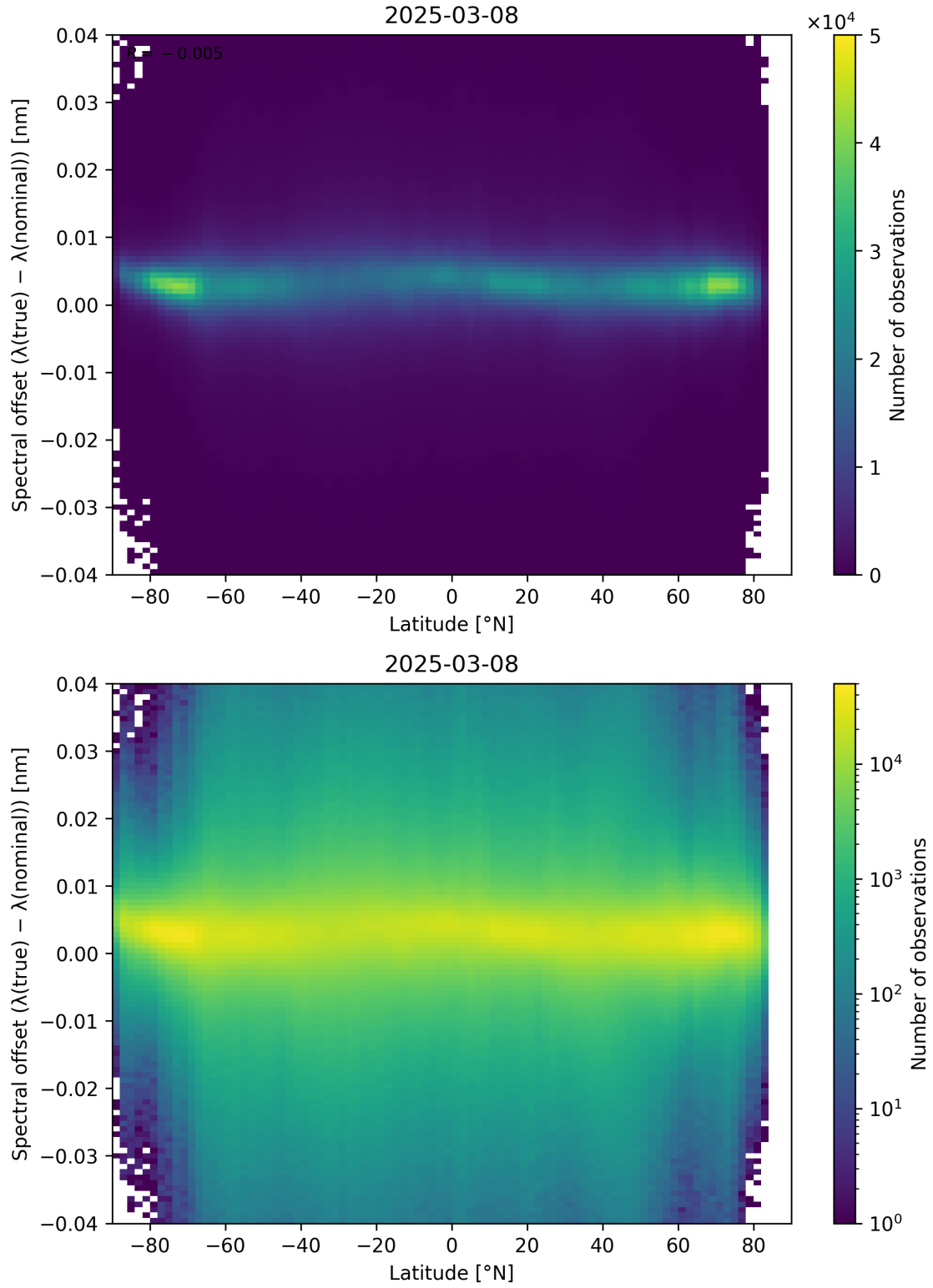
Figure 96: Scatter density plot of “Latitude” against “Spectral offset ( \lambda_{\text{true}} - \lambda_{\text{nominal}} )” for 2025-03-07 to 2025-03-09.
