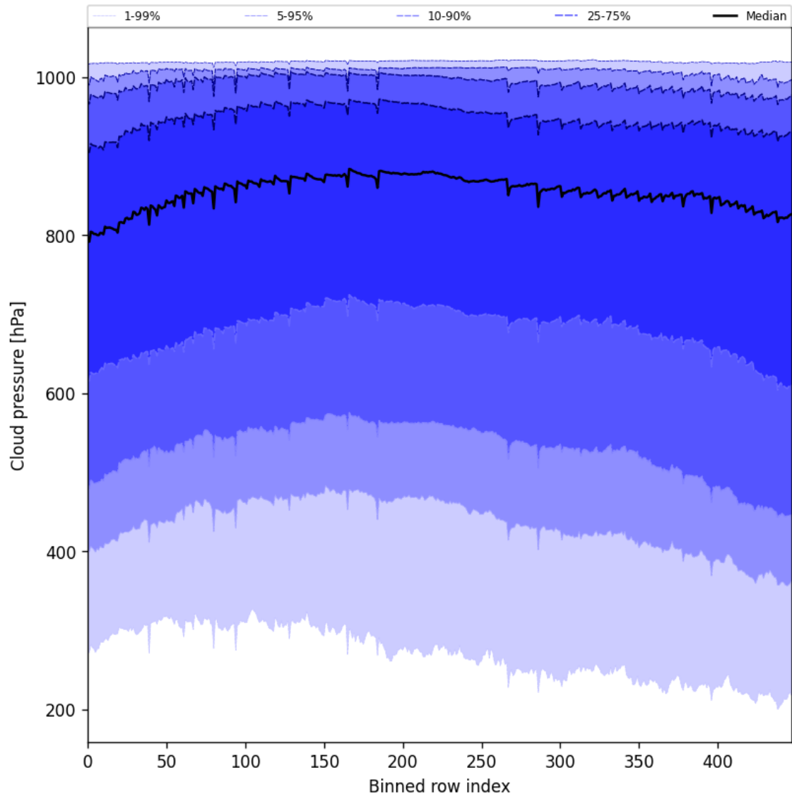
Figure 47: Along track statistics of “Cloud pressure” for 2025-03-07 to 2025-03-09
