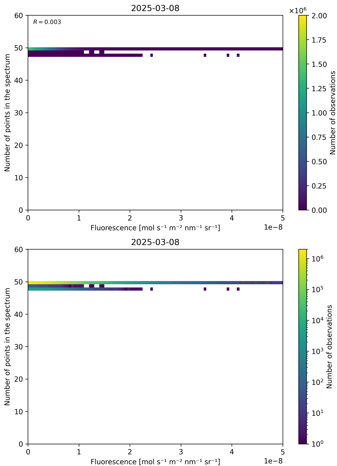
Figure 86: Scatter density plot of “Fluorescence” against “Number of points in the spectrum” for 2025-03-07 to 2025-03-09.
