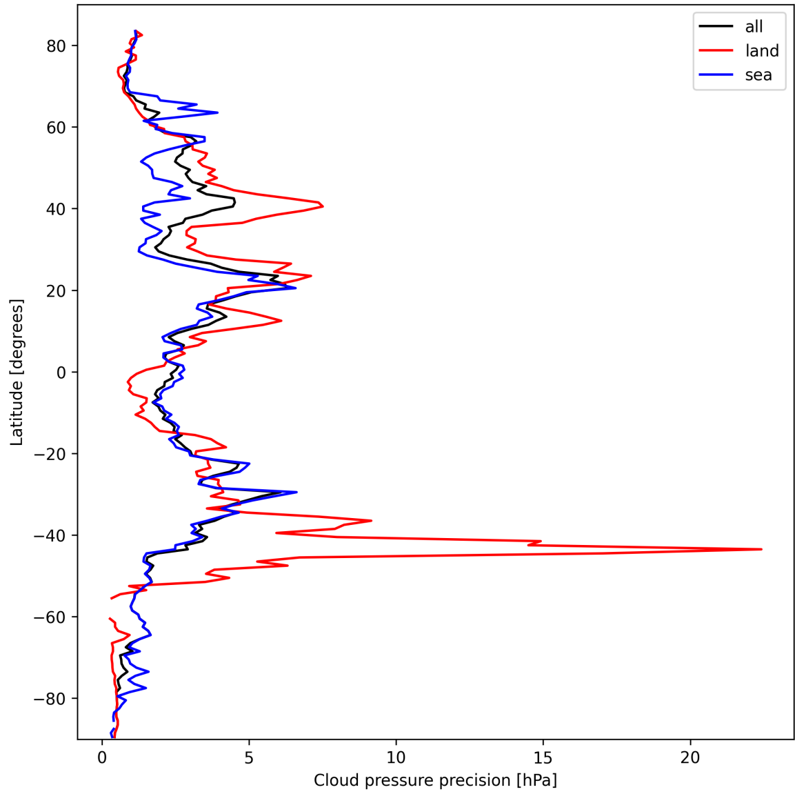
Figure 14: Zonal average of “Cloud pressure precision” for 2025-03-07 to 2025-03-09.
