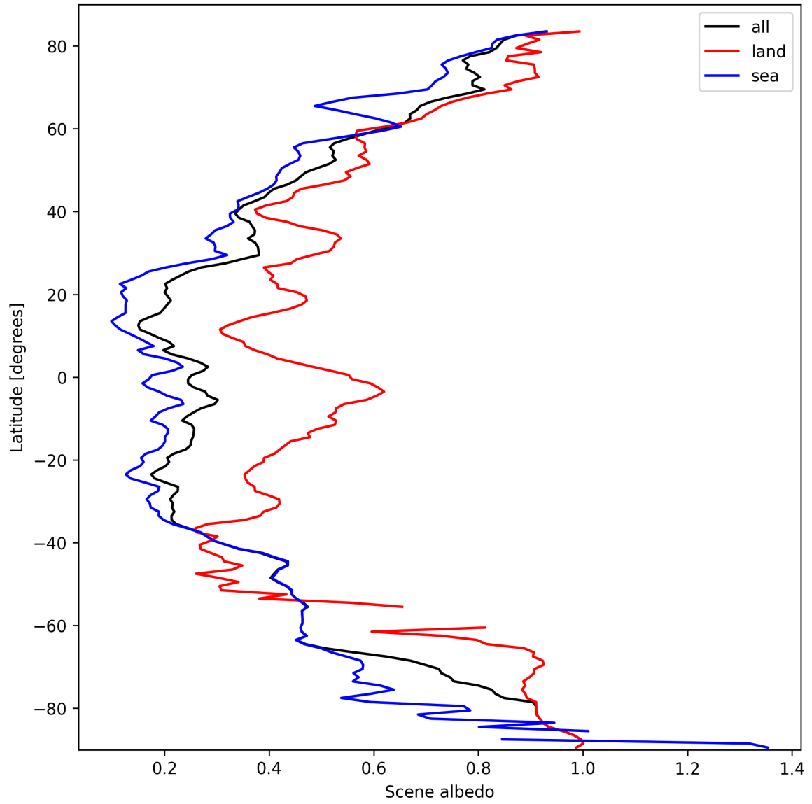
Figure 17: Zonal average of “Scene albedo” for 2025-03-07 to 2025-03-09.
