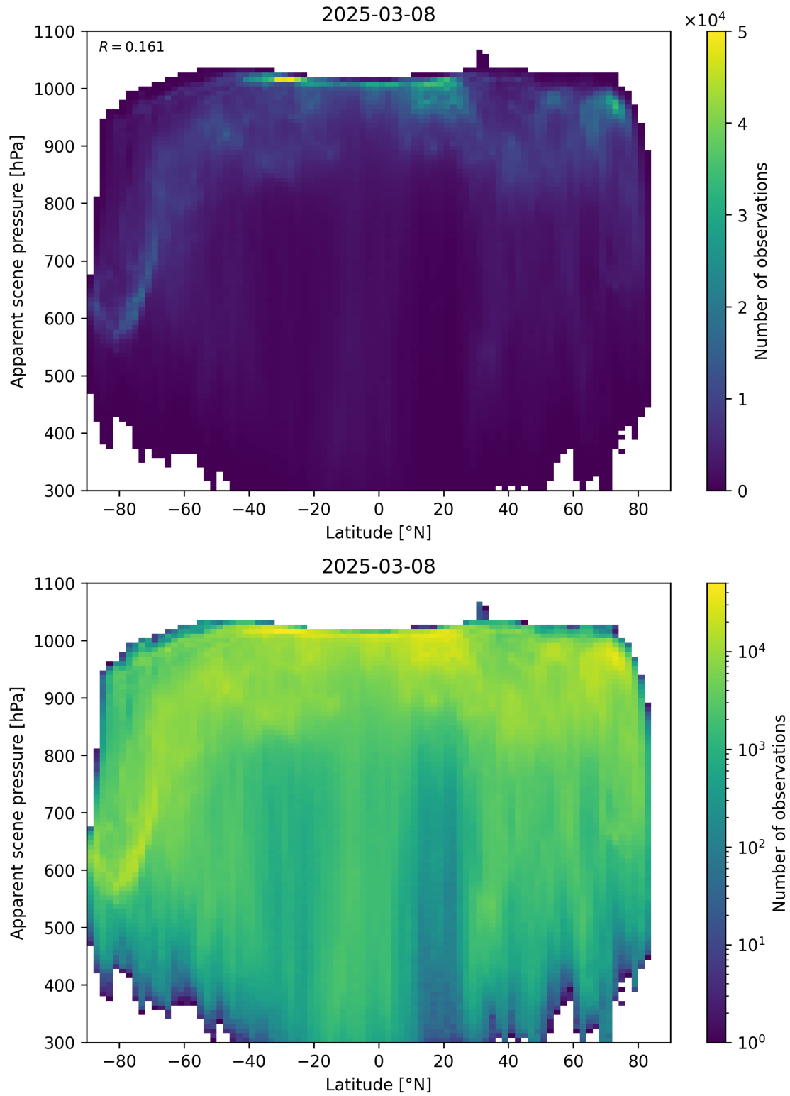
Figure 88: Scatter density plot of “Latitude” against “Apparent scene pressure” for 2025-03-07 to 2025-03-09.
