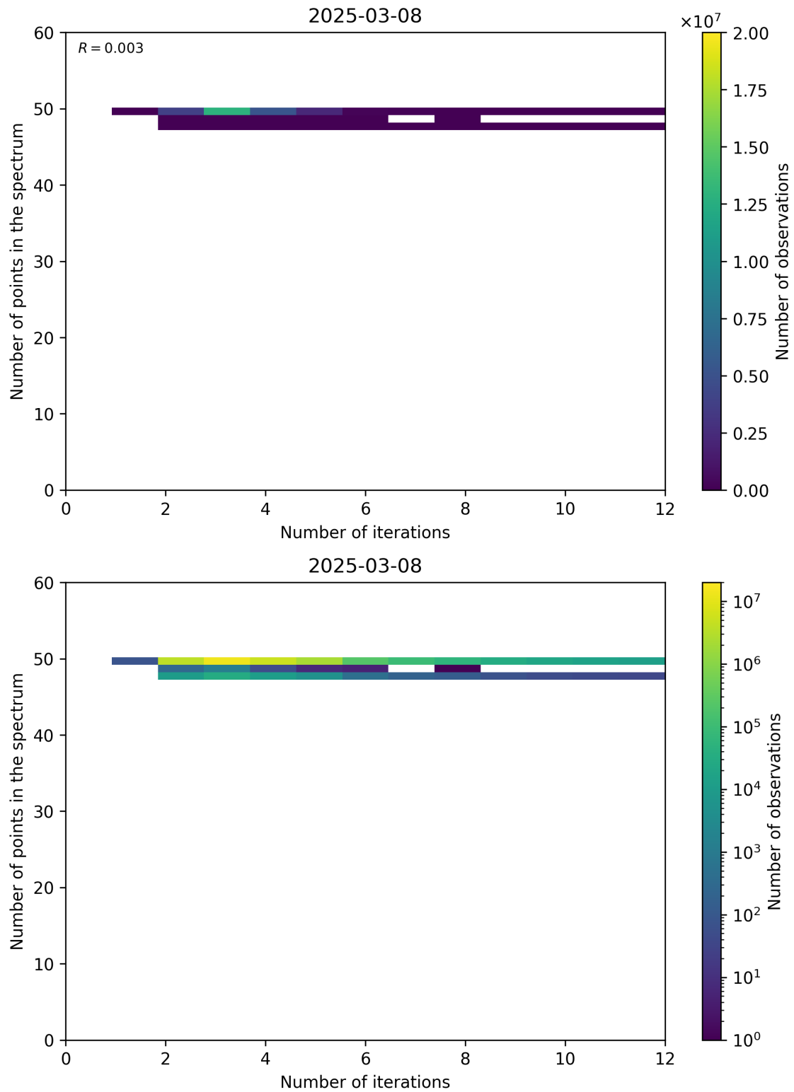
Figure 99: Scatter density plot of “Number of iterations” against “Number of points in the spectrum” for 2025-03-07 to 2025-03-09.
