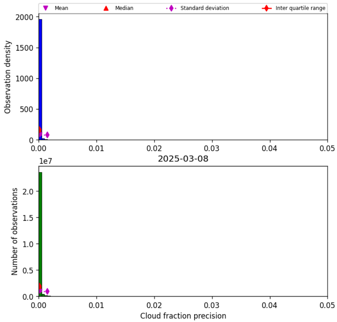
Figure 33: Histogram of “Cloud fraction precision” for 2025-03-07 to 2025-03-09
