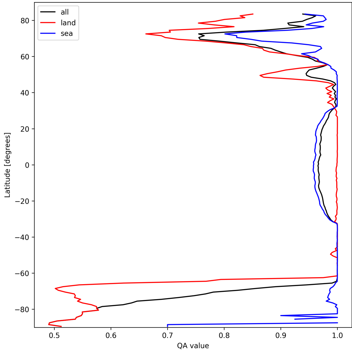
Figure 12: Zonal average of “QA value” for 2025-03-07 to 2025-03-09.
