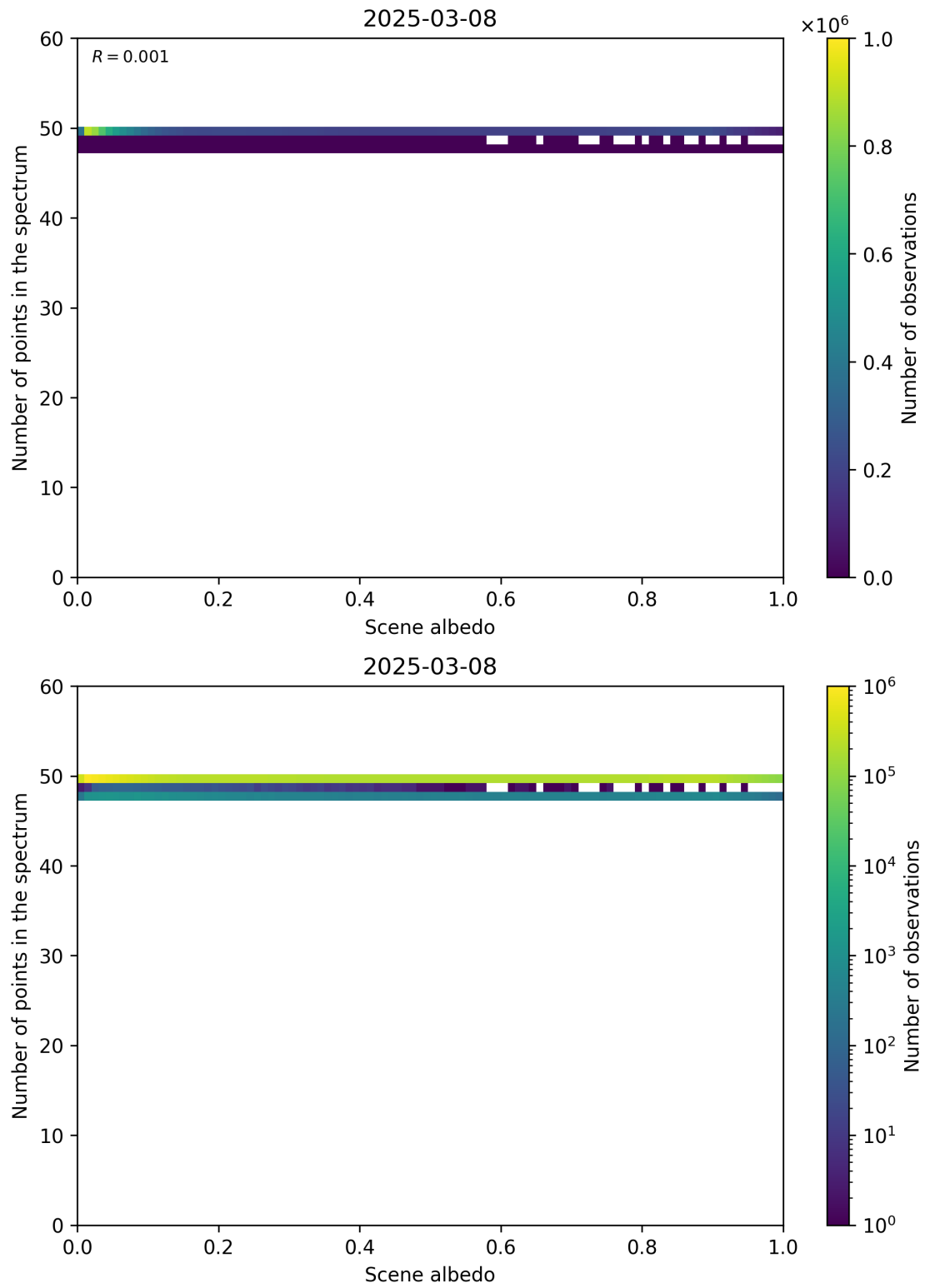
Figure 106: Scatter density plot of “Scene albedo” against “Number of points in the spectrum” for 2025-03-07 to 2025-03-09.
