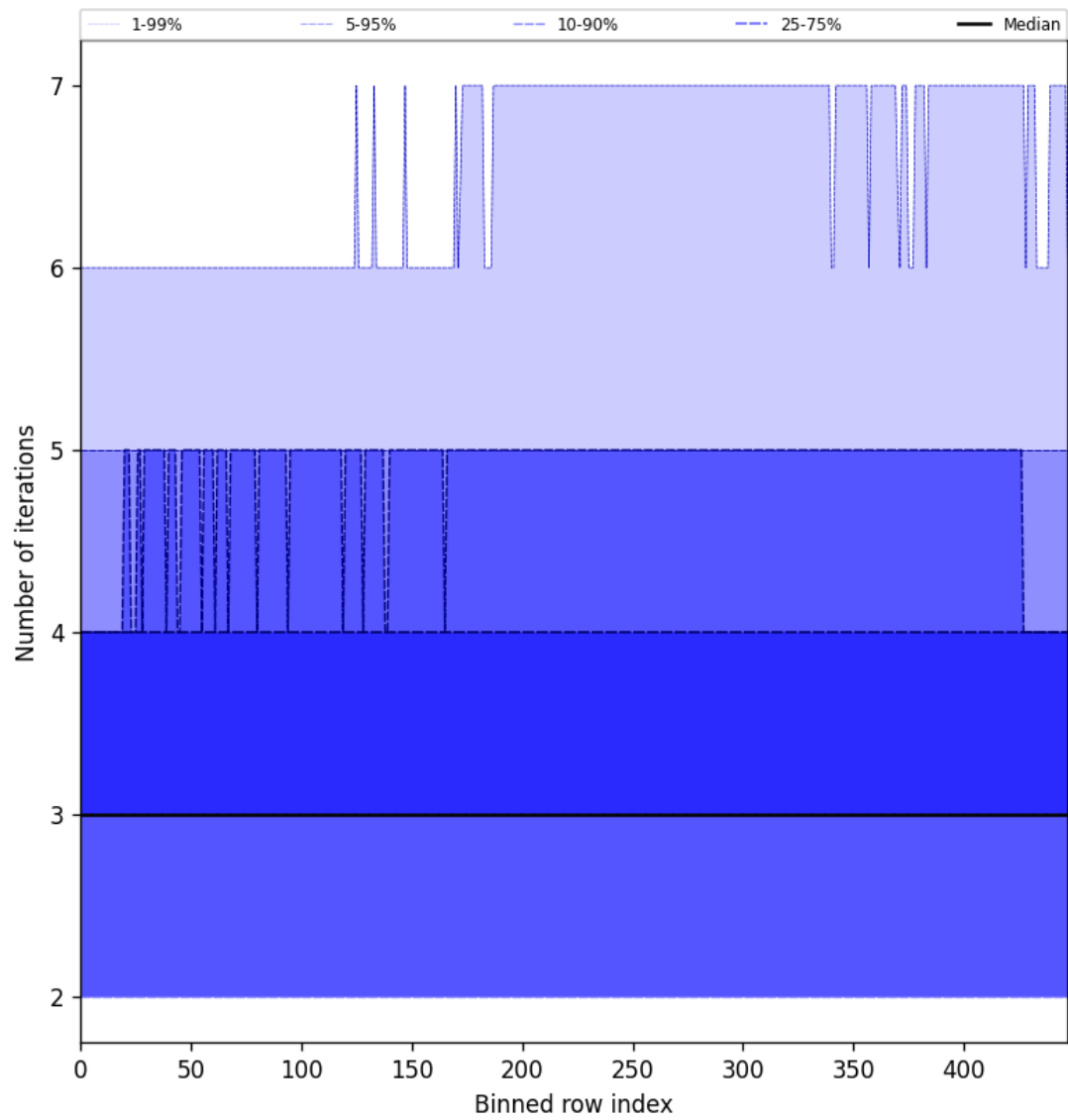
Figure 56: Along track statistics of “Number of iterations” for 2025-03-07 to 2025-03-09
