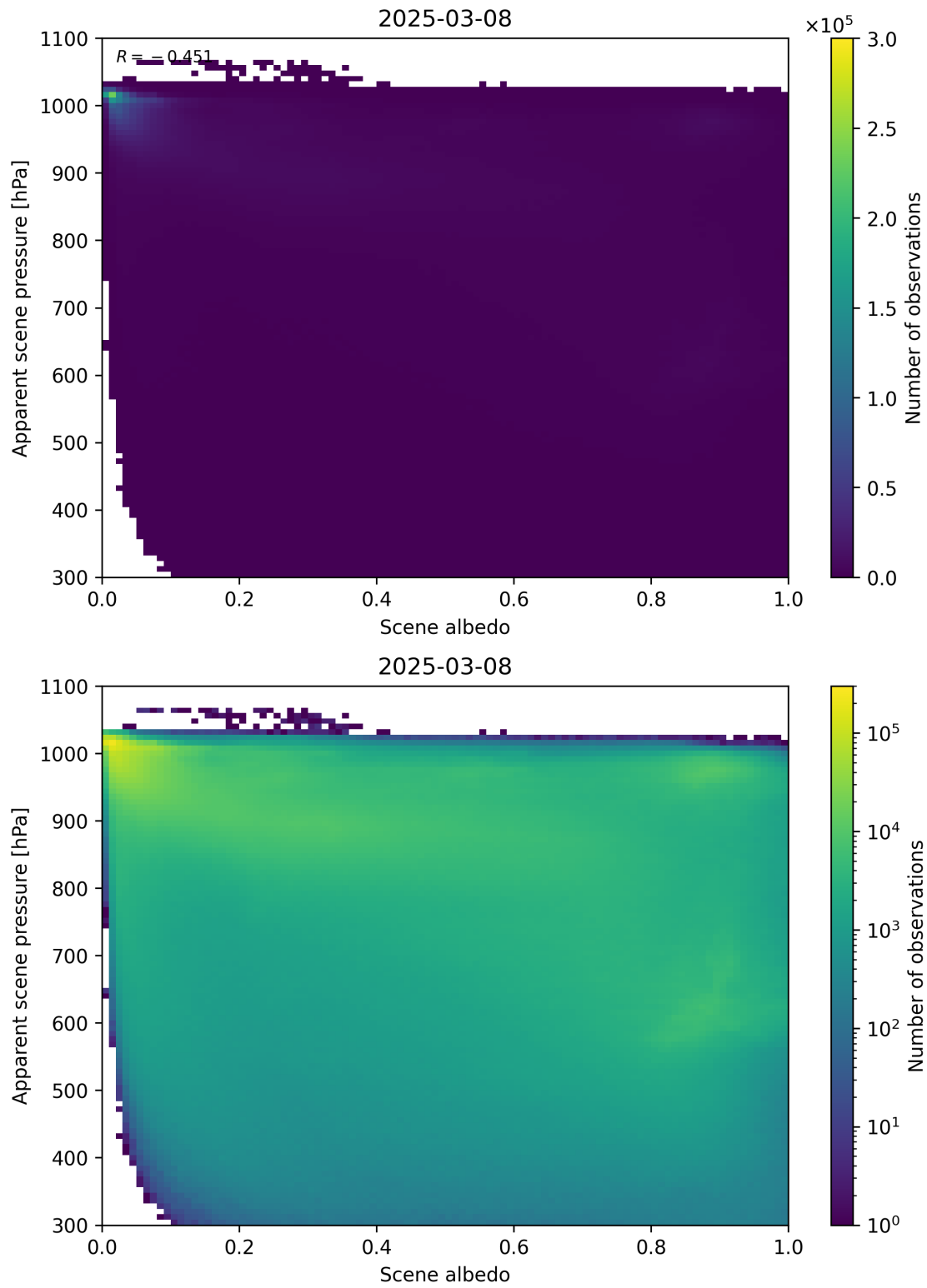
Figure 102: Scatter density plot of “Scene albedo” against “Apparent scene pressure” for 2025-03-07 to 2025-03-09.
