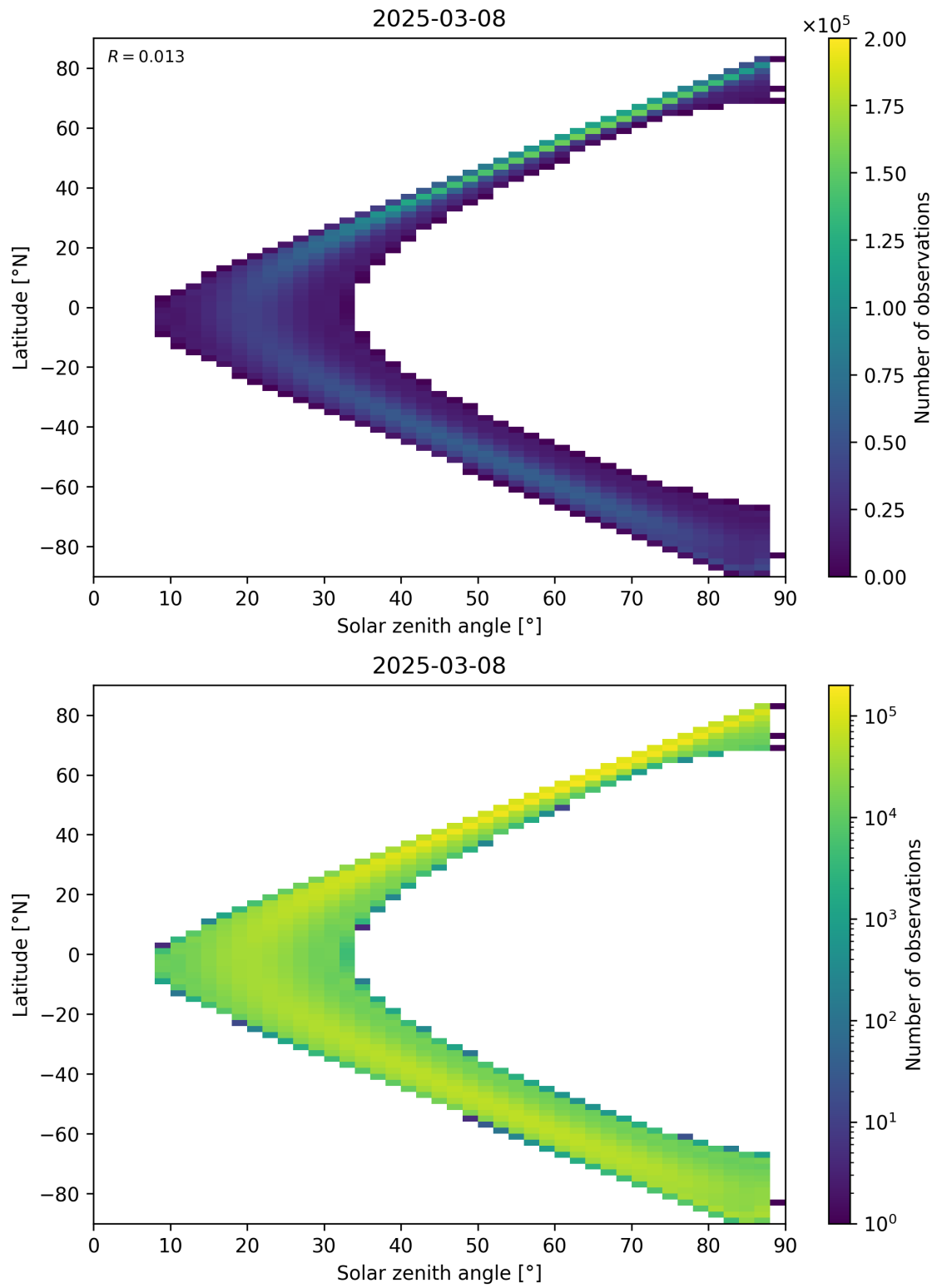
Figure 113: Scatter density plot of “Solar zenith angle” against “Latitude” for 2025-03-07 to 2025-03-09.
