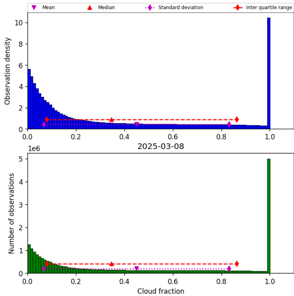
Figure 32: Histogram of “Cloud fraction” for 2025-03-07 to 2025-03-09
