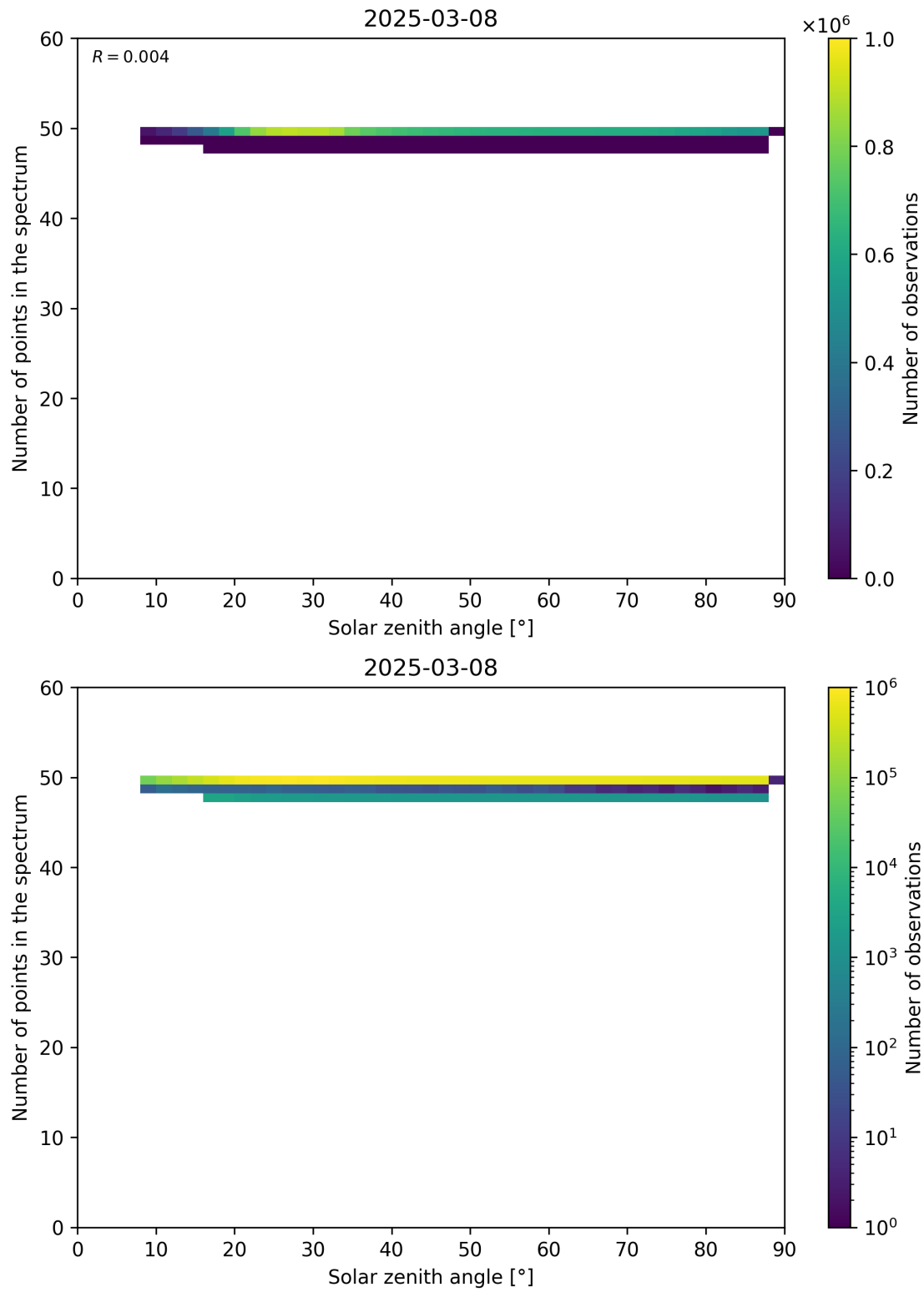
Figure 115: Scatter density plot of “Solar zenith angle” against “Number of points in the spectrum” for 2025-03-07 to 2025-03-09.
