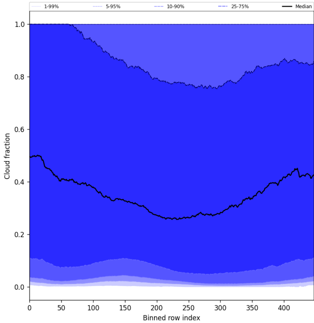
Figure 49: Along track statistics of “Cloud fraction” for 2025-03-07 to 2025-03-09
