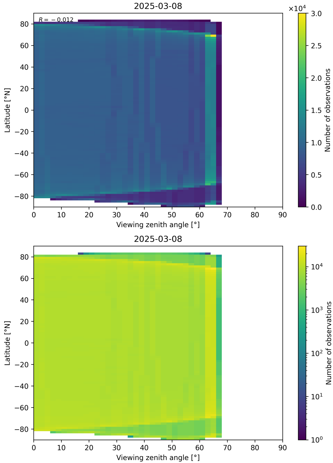
Figure 123: Scatter density plot of “Viewing zenith angle” against “Latitude” for 2025-03-07 to 2025-03-09.
