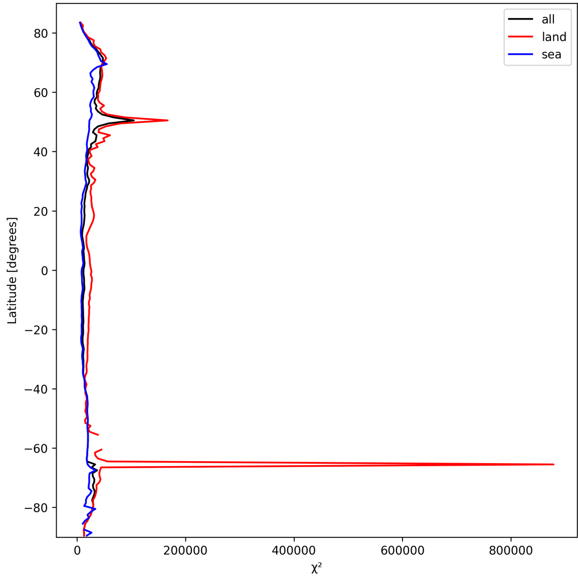
Figure 21: Zonal average of “ \chi^2 ” for 2025-03-07 to 2025-03-09.
