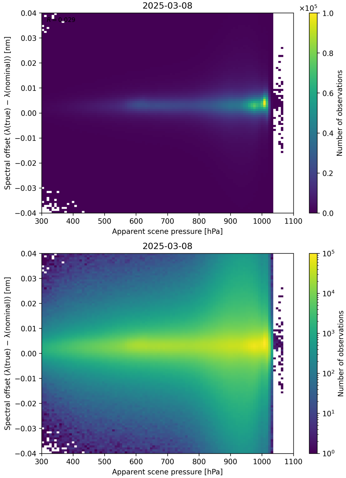
Figure 67: Scatter density plot of “Apparent scene pressure” against “Spectral offset ( \lambda_{\text{true}} - \lambda_{\text{nominal}} )” for 2025-03-07 to 2025-03-09.
