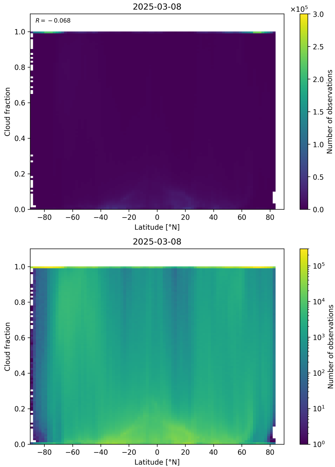
Figure 90: Scatter density plot of “Latitude” against “Cloud fraction” for 2025-03-07 to 2025-03-09.
