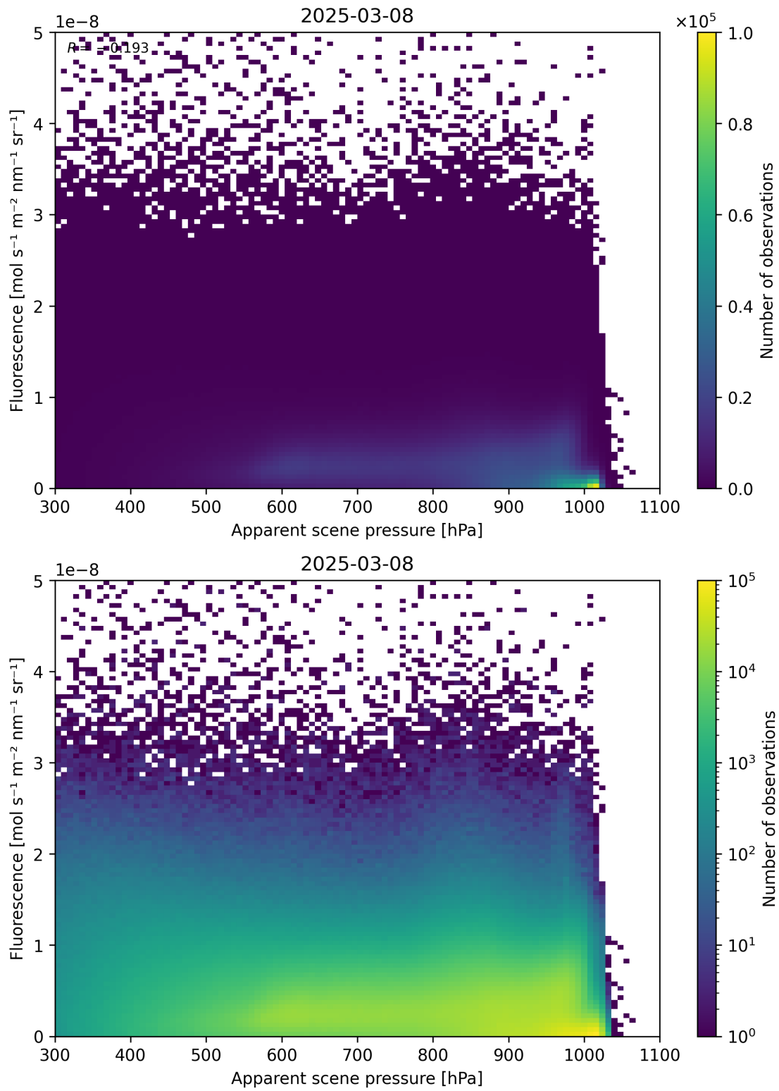
Figure 64: Scatter density plot of “Apparent scene pressure” against “Fluorescence” for 2025-03-07 to 2025-03-09.
