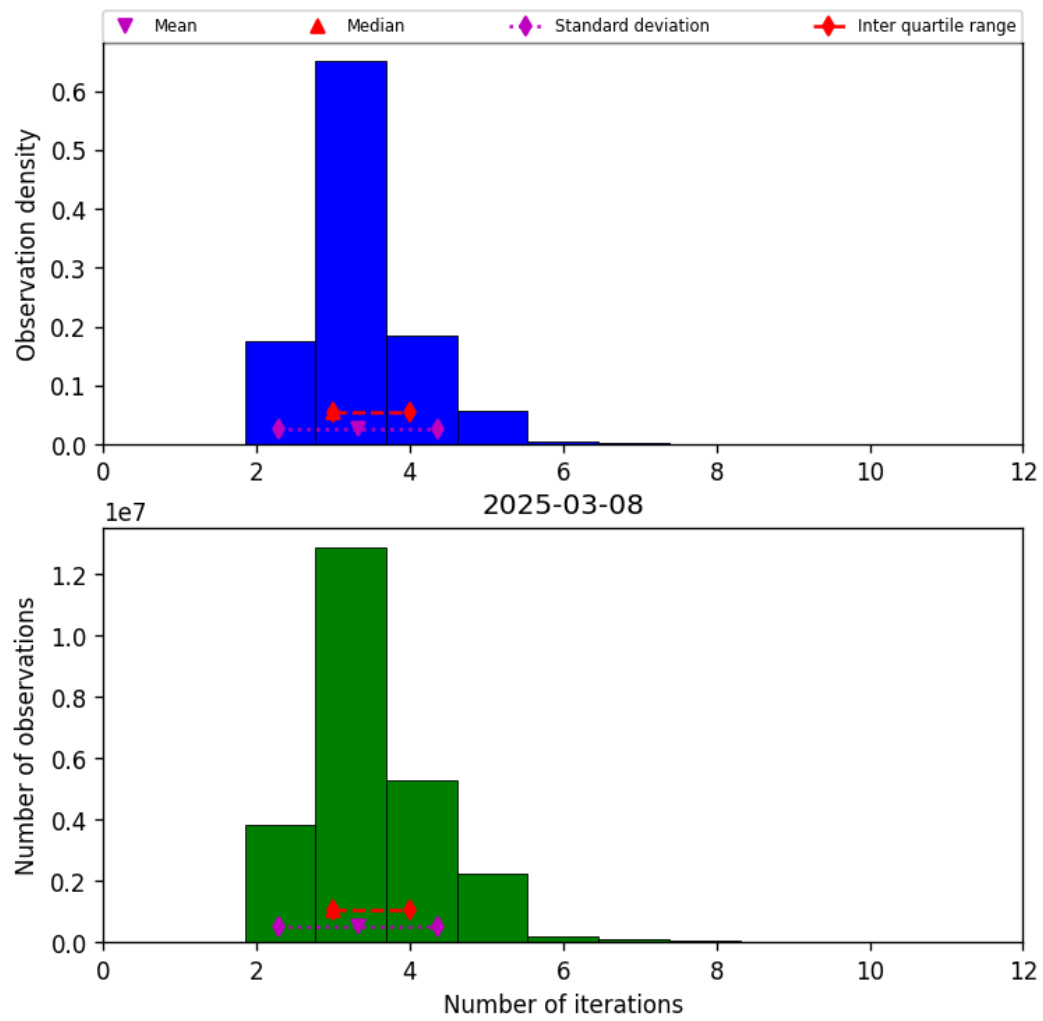
Figure 39: Histogram of “Number of iterations” for 2025-03-07 to 2025-03-09
