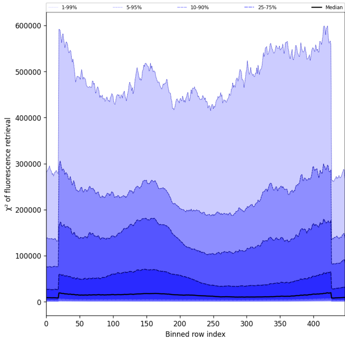
Figure 59: Along track statistics of “ \chi^2 of fluorescence retrieval” for 2025-03-07 to 2025-03-09
