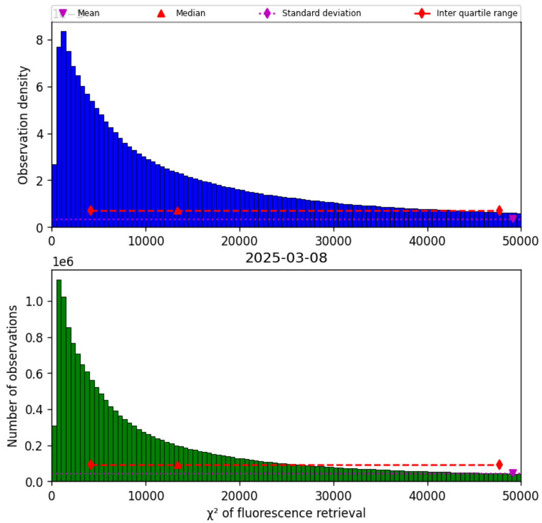
Figure 42: Histogram of “ \chi^2 of fluorescence retrieval” for 2025-03-07 to 2025-03-09
