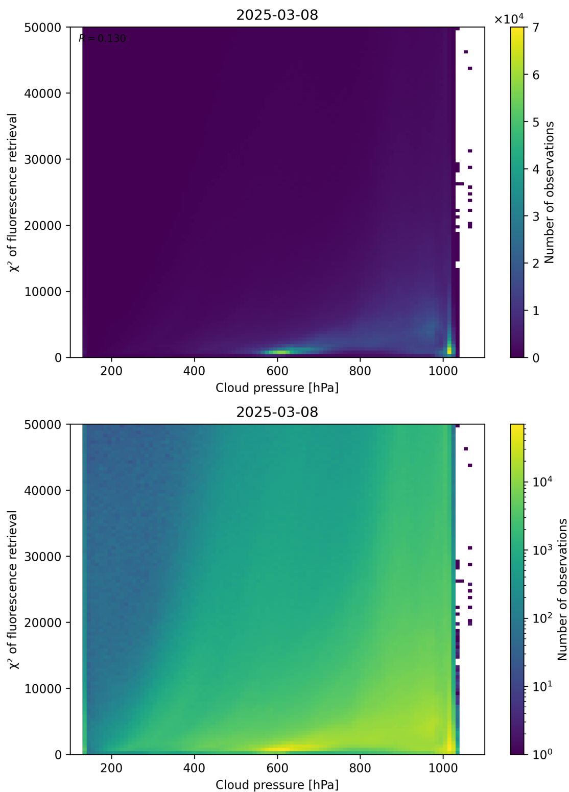
Figure 78: Scatter density plot of “Cloud pressure” against “ \chi^2 of fluorescence retrieval” for 2025-03-07 to 2025-03-09.
