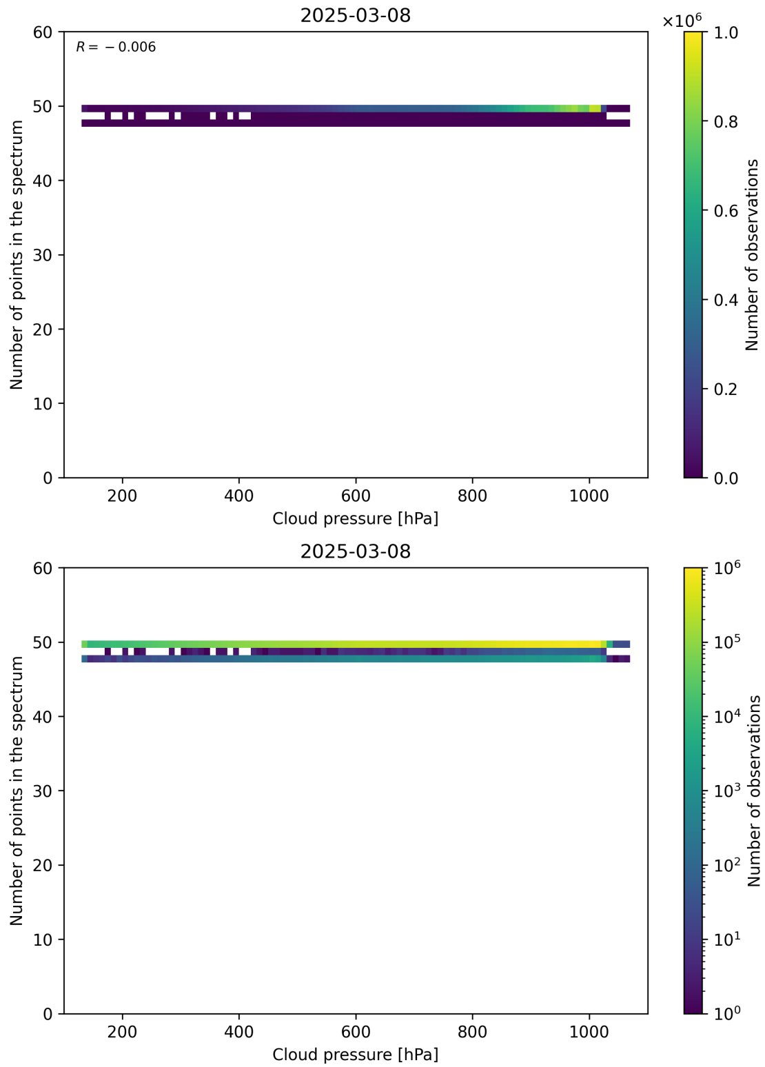
Figure 82: Scatter density plot of “Cloud pressure” against “Number of points in the spectrum” for 2025-03-07 to 2025-03-09.
