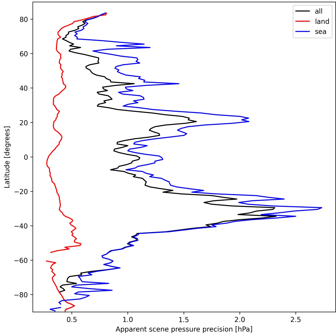
Figure 20: Zonal average of “Apparent scene pressure precision” for 2025-03-07 to 2025-03-09.
