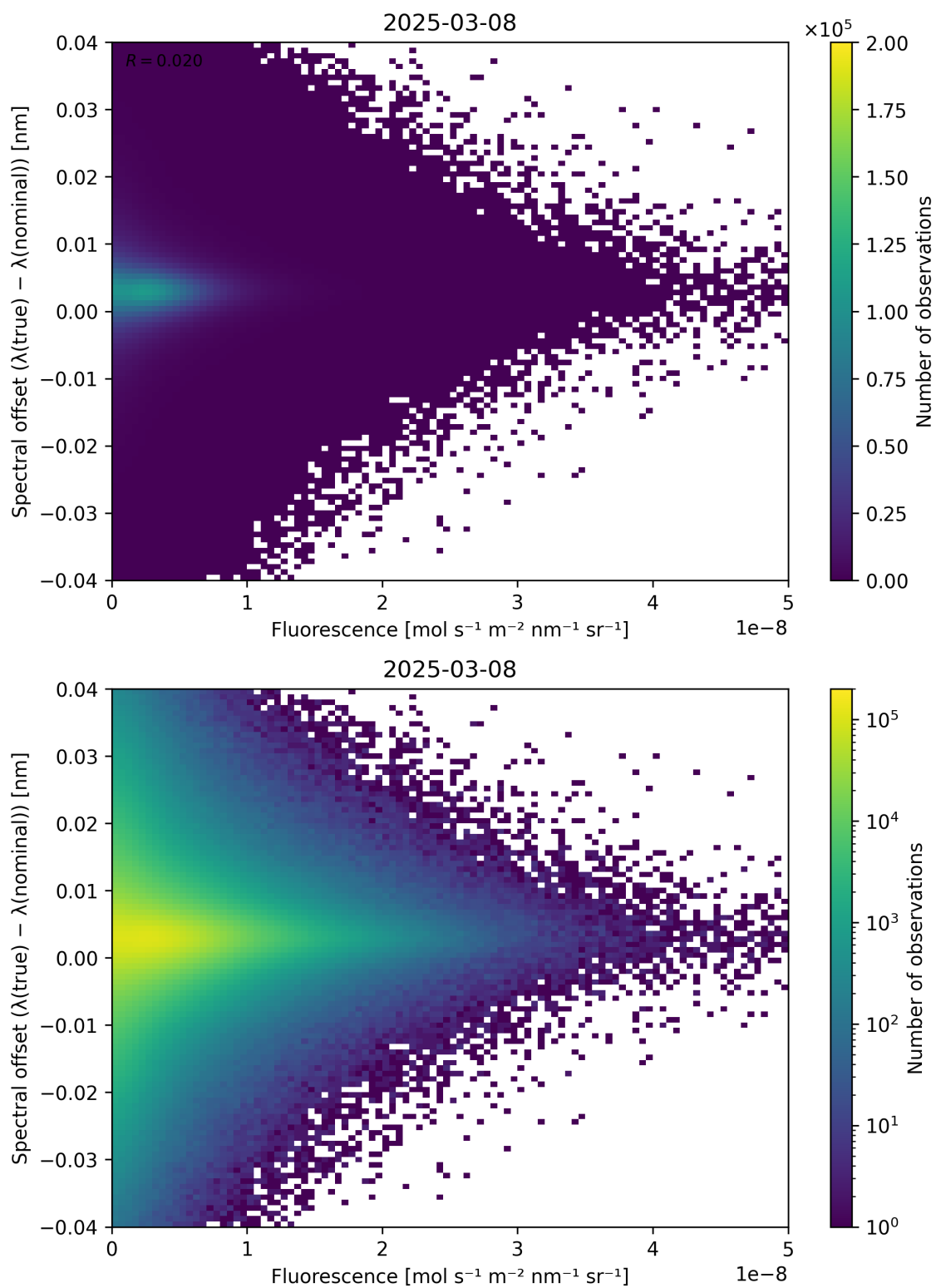
Figure 87: Scatter density plot of “Fluorescence” against “Spectral offset ( \lambda_{\text{true}} - \lambda_{\text{nominal}} )” for 2025-03-07 to 2025-03-09.
