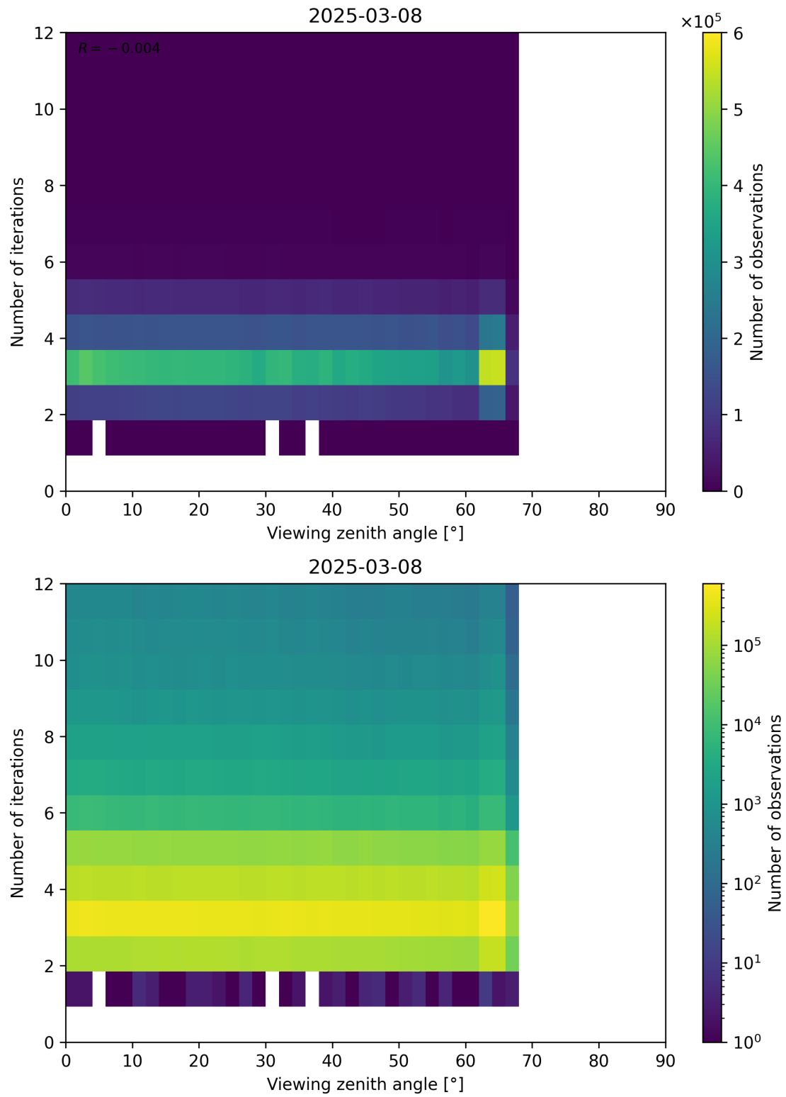
Figure 124: Scatter density plot of “Viewing zenith angle” against “Number of iterations” for 2025-03-07 to 2025-03-09.
