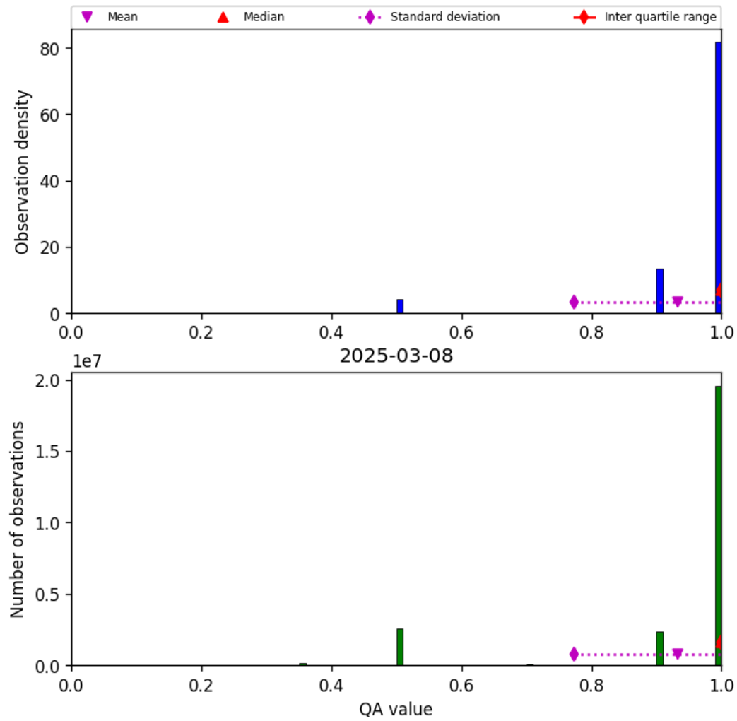
Figure 29: Histogram of “QA value” for 2025-03-07 to 2025-03-09
