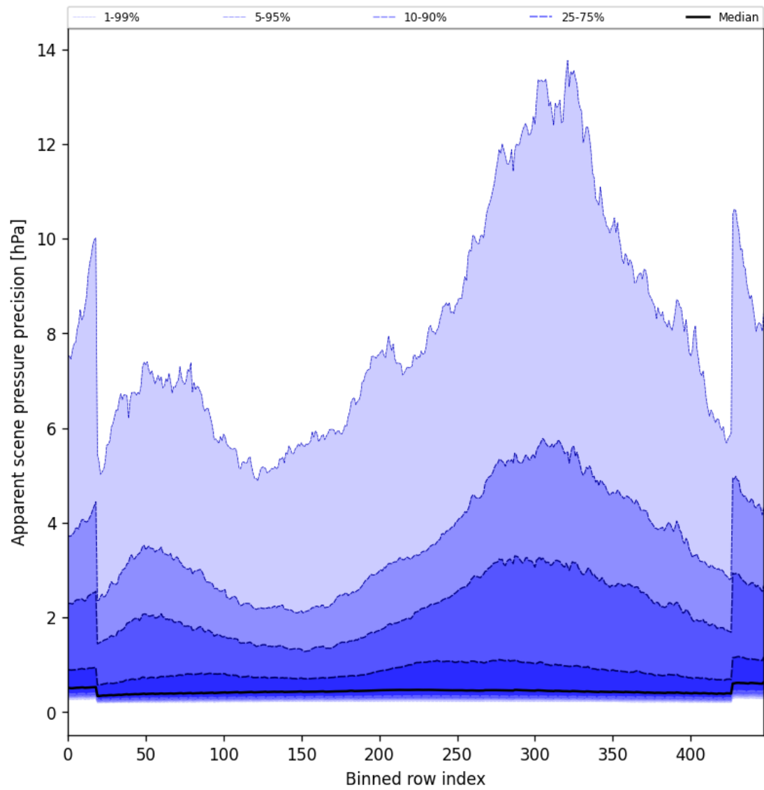
Figure 54: Along track statistics of “Apparent scene pressure precision” for 2025-03-07 to 2025-03-09
