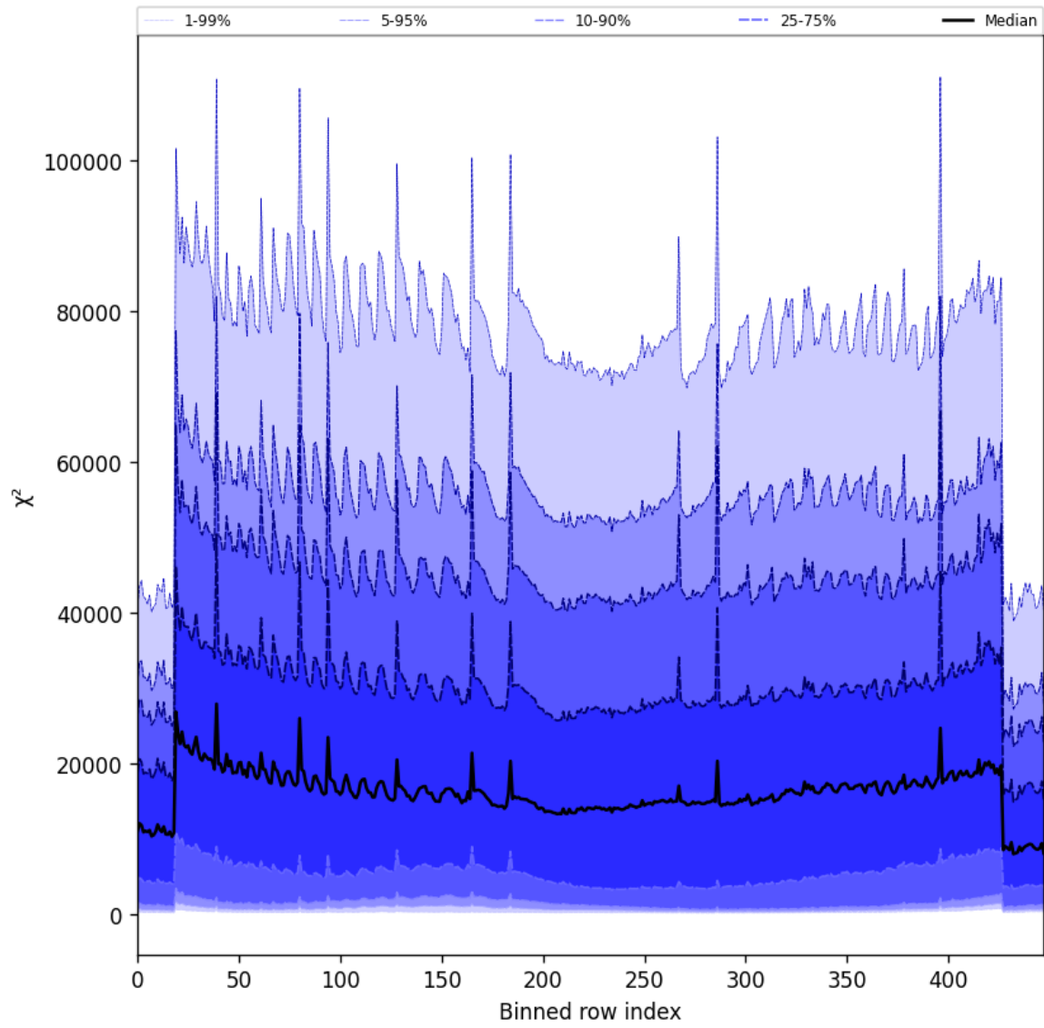
Figure 55: Along track statistics of “ \chi^2 ” for 2025-03-07 to 2025-03-09
