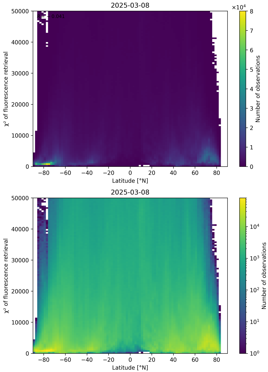
Figure 89: Scatter density plot of “Latitude” against “ \chi^2 of fluorescence retrieval” for 2025-03-07 to 2025-03-09.
