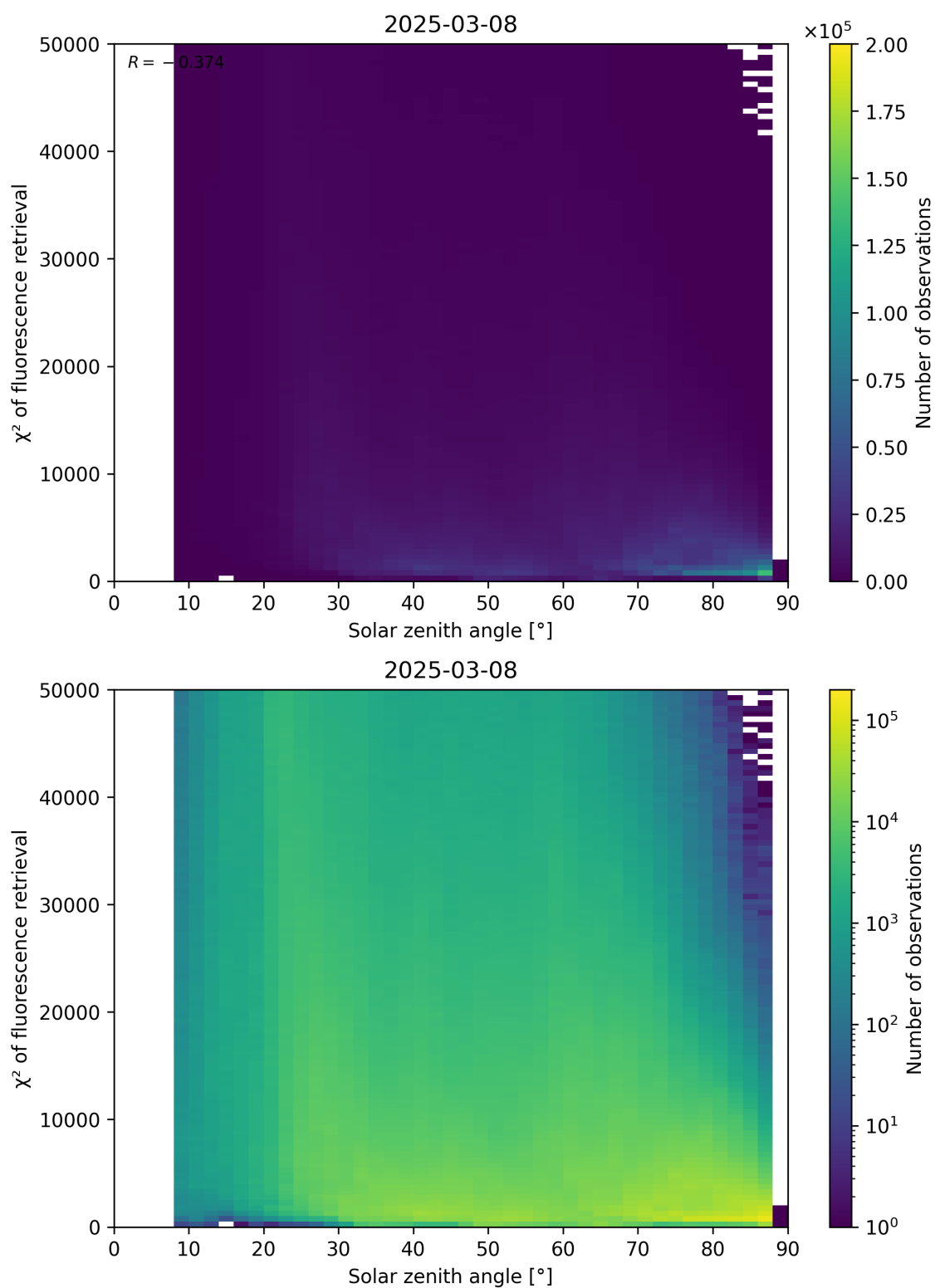
Figure 109: Scatter density plot of “Solar zenith angle” against “ \chi^2 of fluorescence retrieval” for 2025-03-07 to 2025-03-09.
