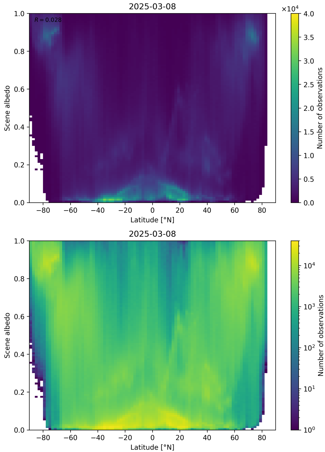
Figure 95: Scatter density plot of “Latitude” against “Scene albedo” for 2025-03-07 to 2025-03-09.
