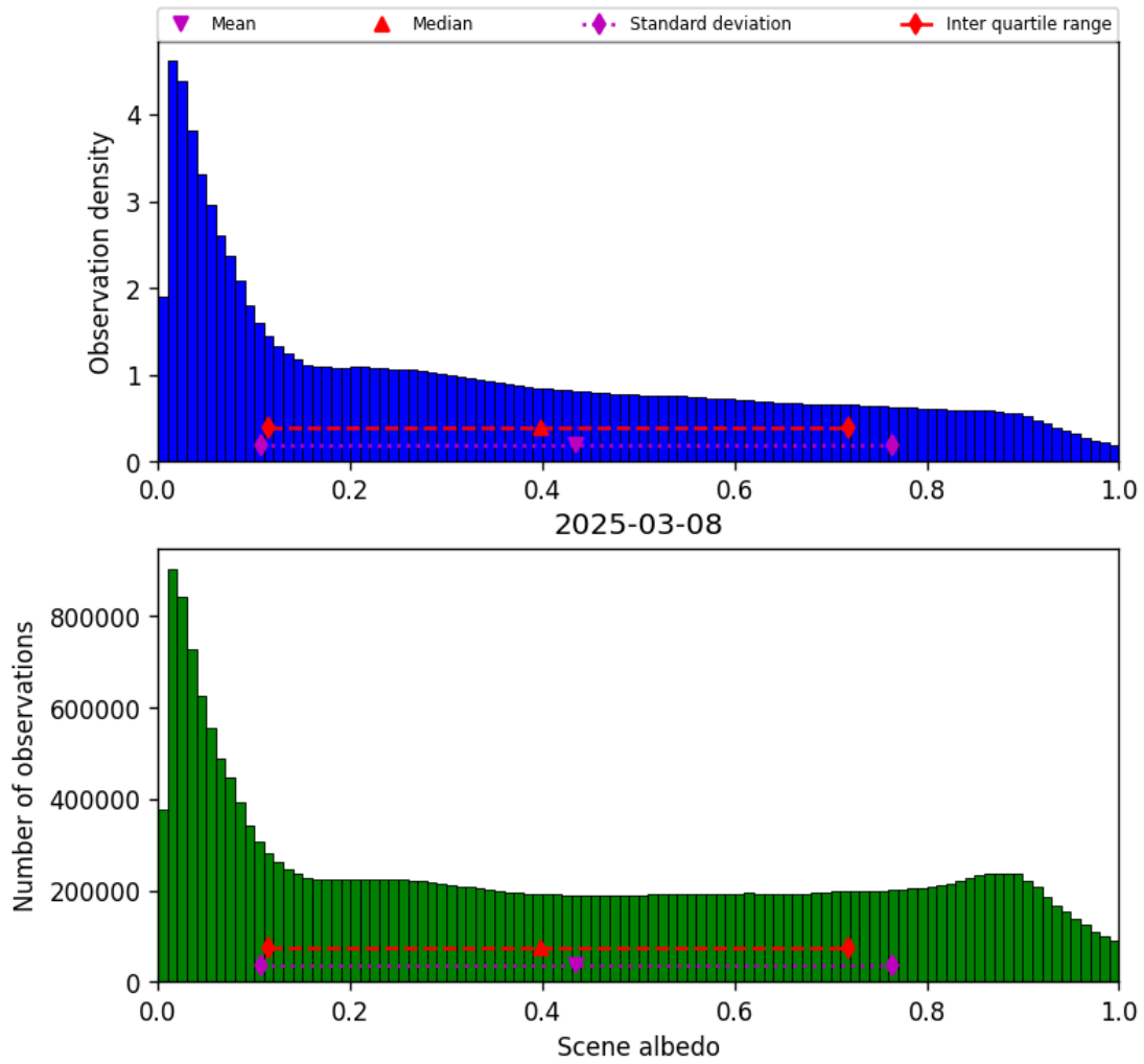
Figure 34: Histogram of “Scene albedo” for 2025-03-07 to 2025-03-09
