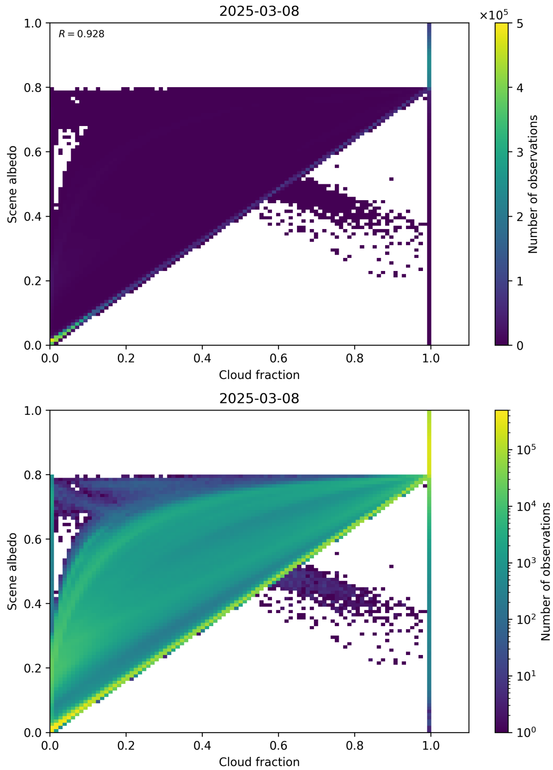
Figure 75: Scatter density plot of “Cloud fraction” against “Scene albedo” for 2025-03-07 to 2025-03-09.
