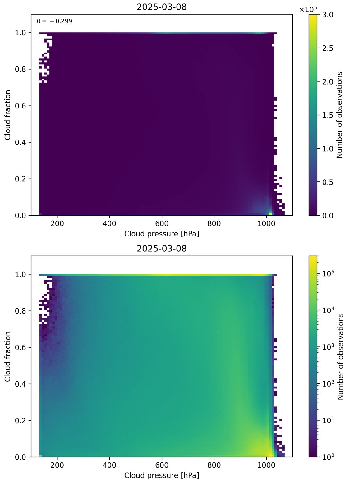
Figure 79: Scatter density plot of “Cloud pressure” against “Cloud fraction” for 2025-03-07 to 2025-03-09.
