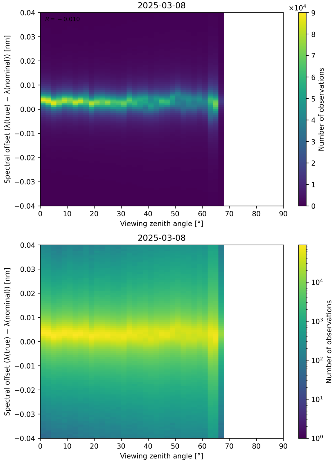
Figure 128: Scatter density plot of “Viewing zenith angle” against “Spectral offset ( \lambda_{\text{true}} - \lambda_{\text{nominal}} )” for 2025-03-07 to 2025-03-09.
