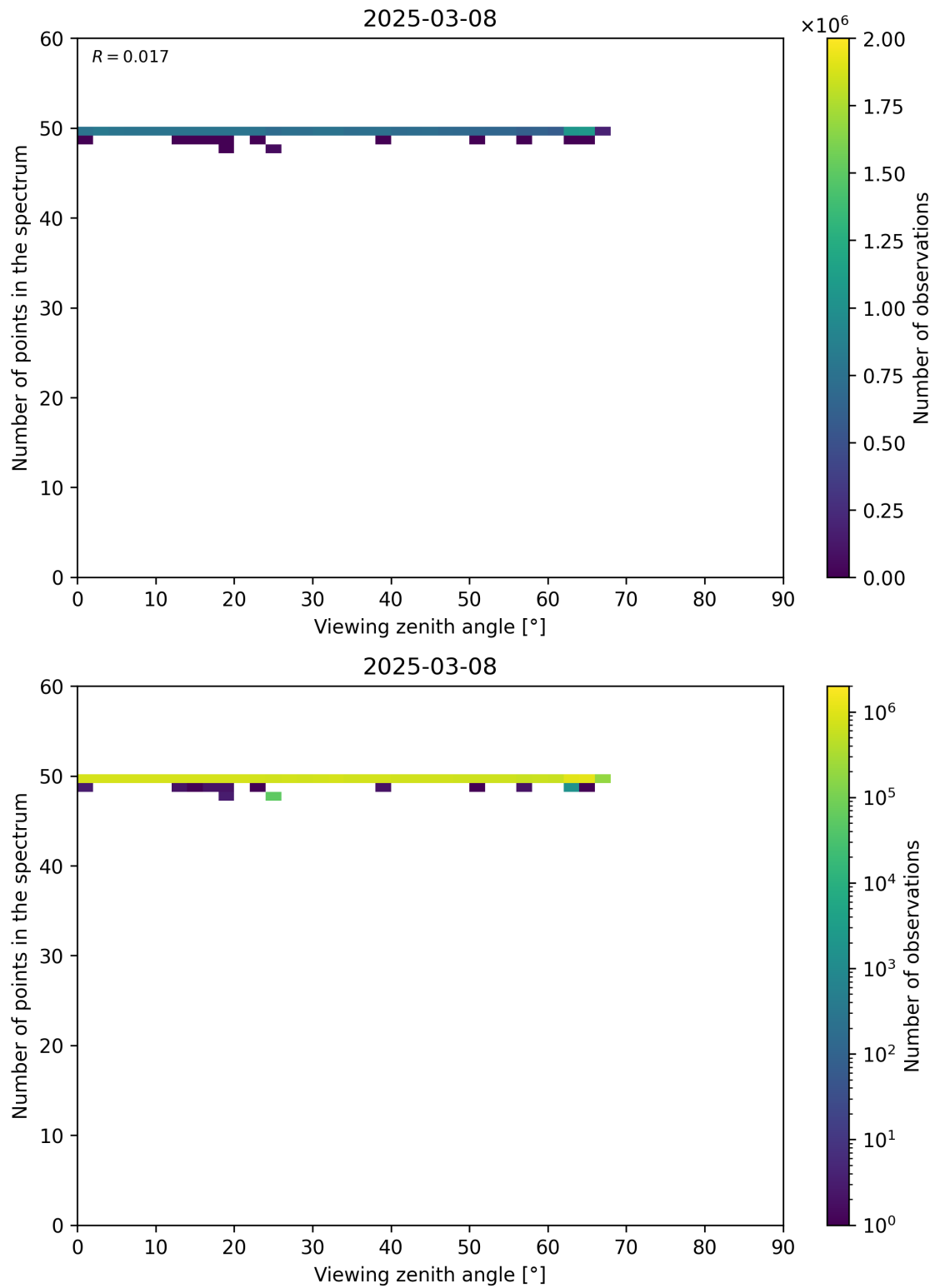
Figure 125: Scatter density plot of “Viewing zenith angle” against “Number of points in the spectrum” for 2025-03-07 to 2025-03-09.
