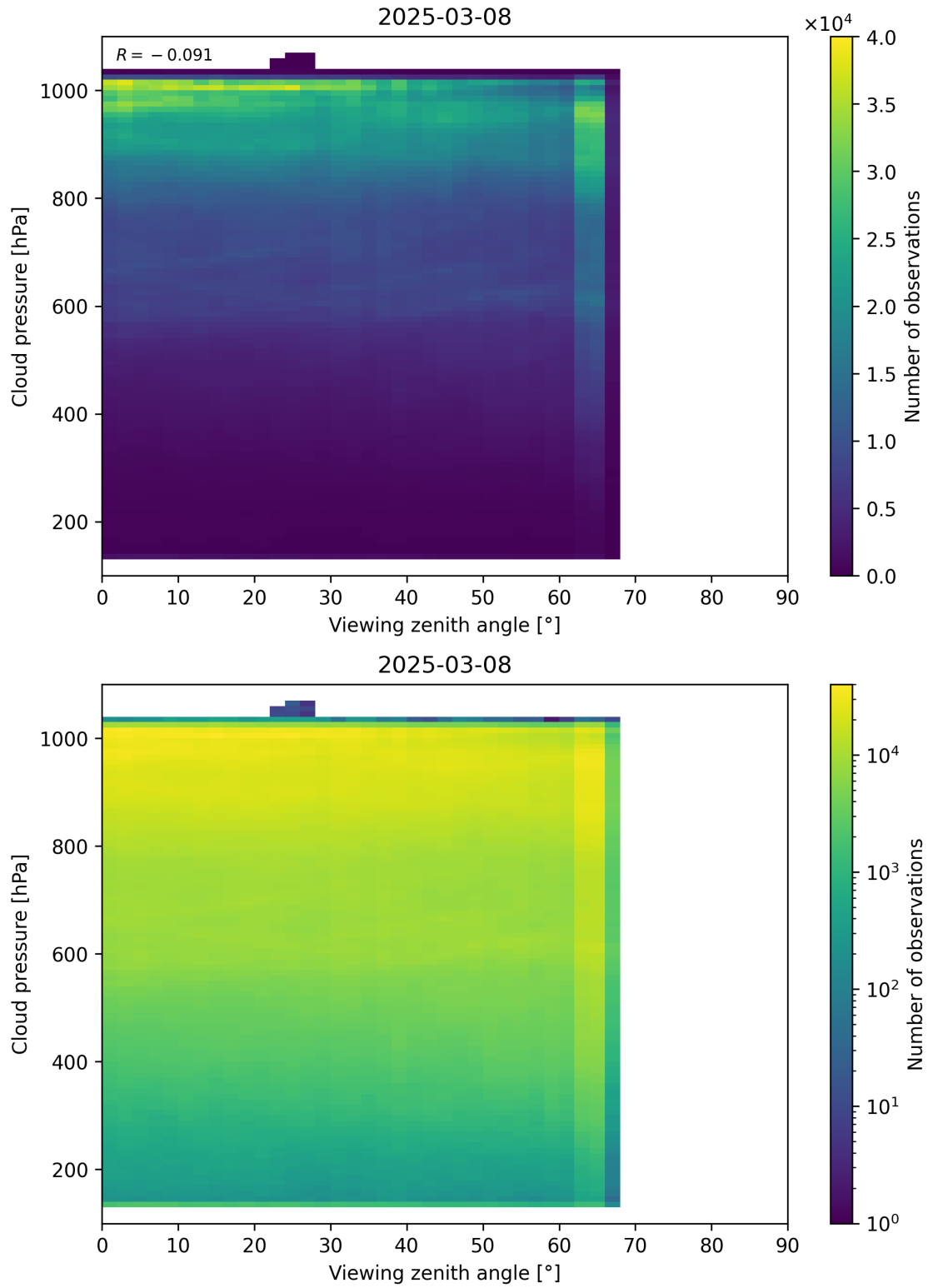
Figure 121: Scatter density plot of “Viewing zenith angle” against “Cloud pressure” for 2025-03-07 to 2025-03-09.
