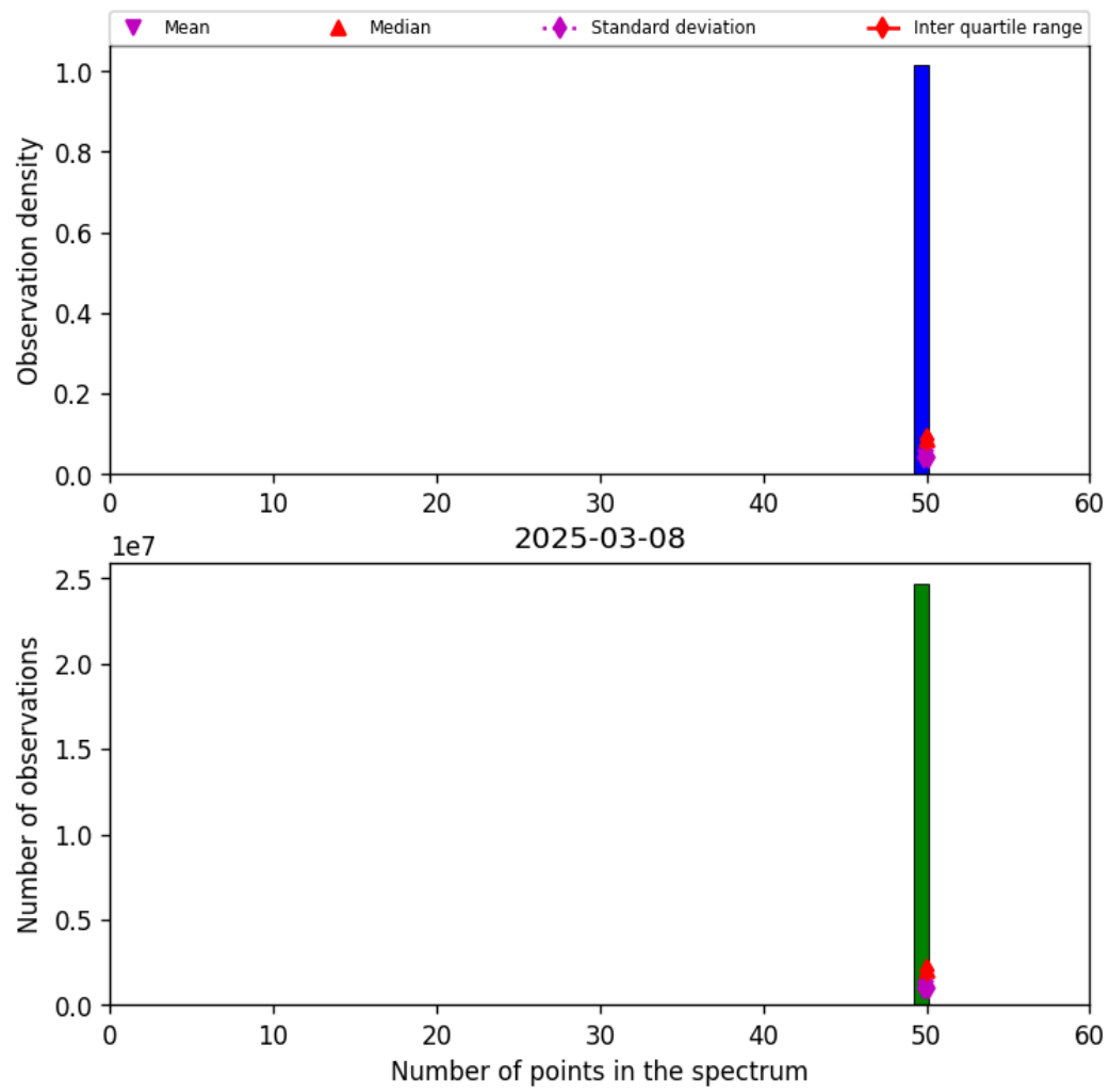
Figure 44: Histogram of “Number of points in the spectrum” for 2025-03-07 to 2025-03-09
