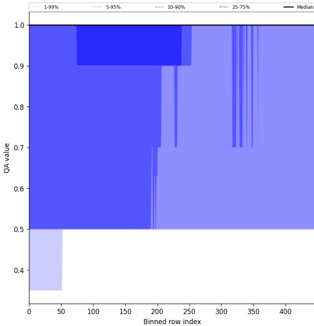
Figure 46: Along track statistics of “QA value” for 2025-03-07 to 2025-03-09
