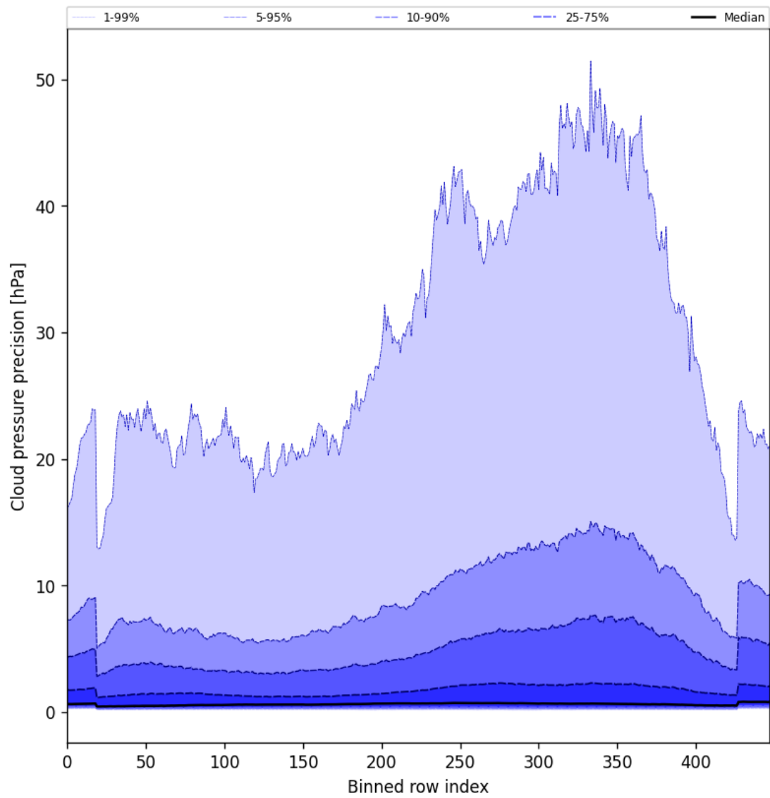
Figure 48: Along track statistics of “Cloud pressure precision” for 2025-03-08 to 2025-03-10
