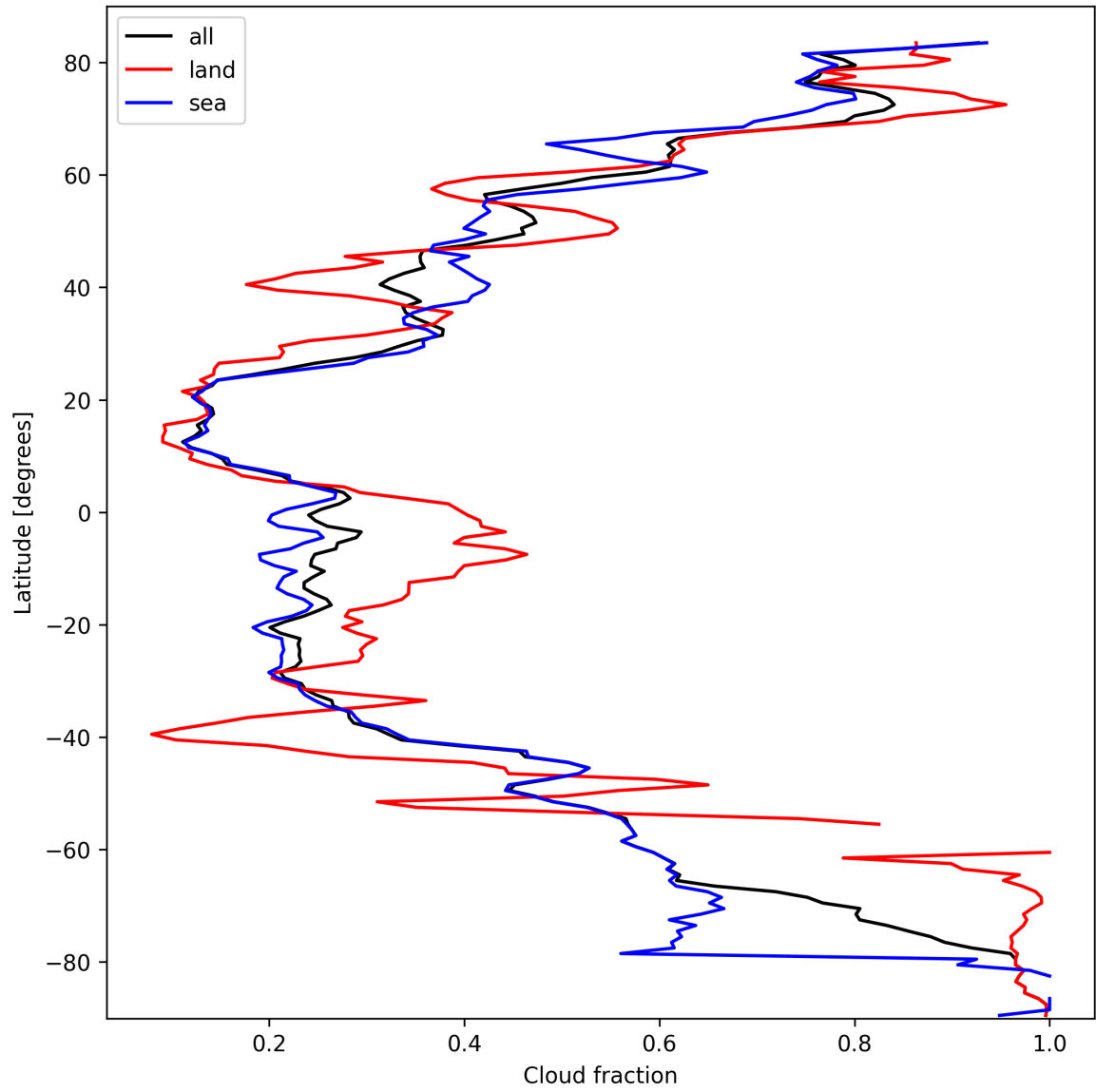
Figure 15: Zonal average of “Cloud fraction” for 2025-03-08 to 2025-03-10.
