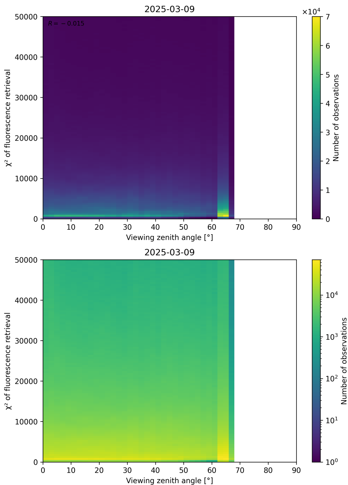
Figure 119: Scatter density plot of “Viewing zenith angle” against “ \chi^2 of fluorescence retrieval” for 2025-03-08 to 2025-03-10.
