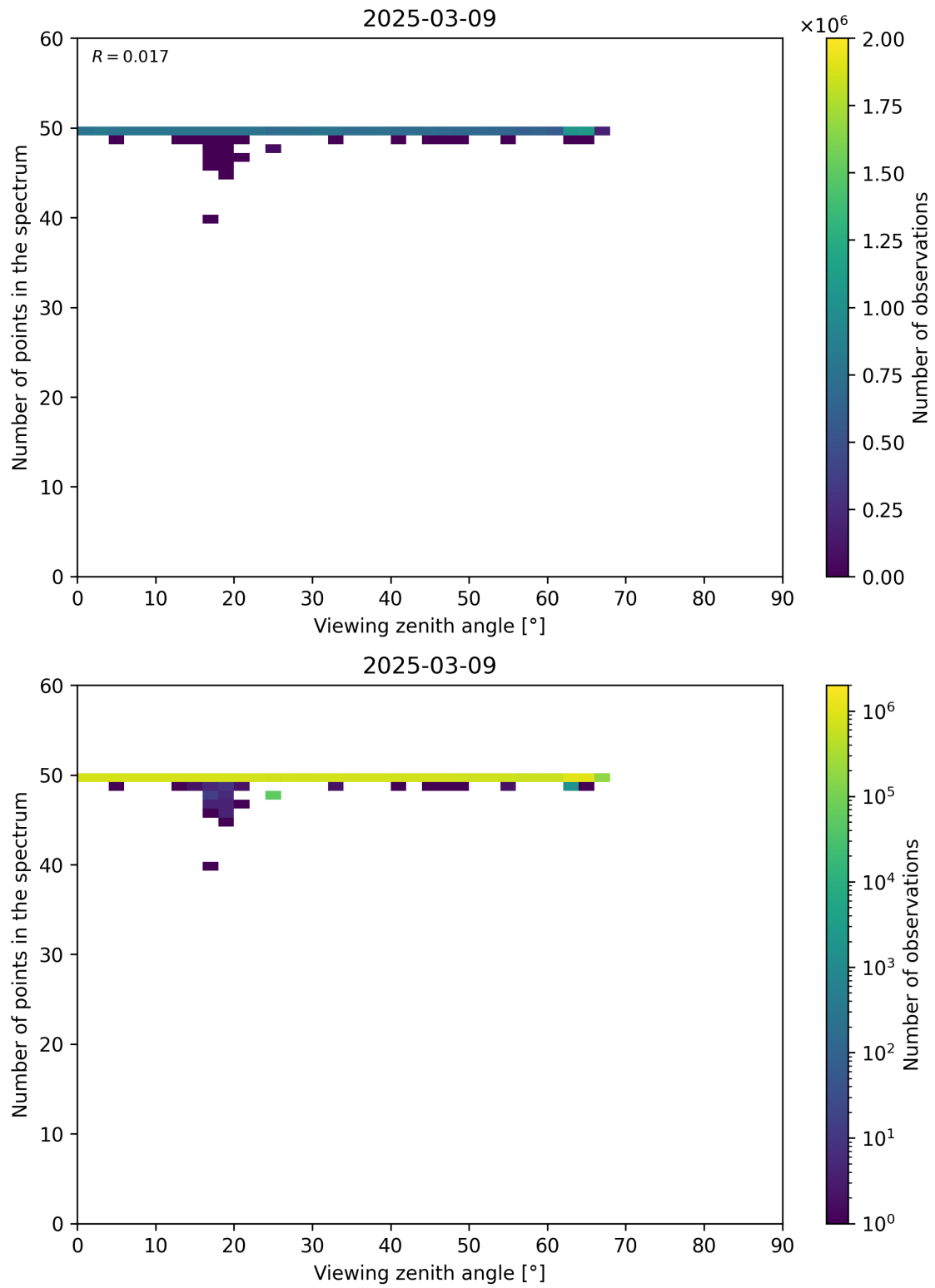
Figure 125: Scatter density plot of “Viewing zenith angle” against “Number of points in the spectrum” for 2025-03-08 to 2025-03-10.
