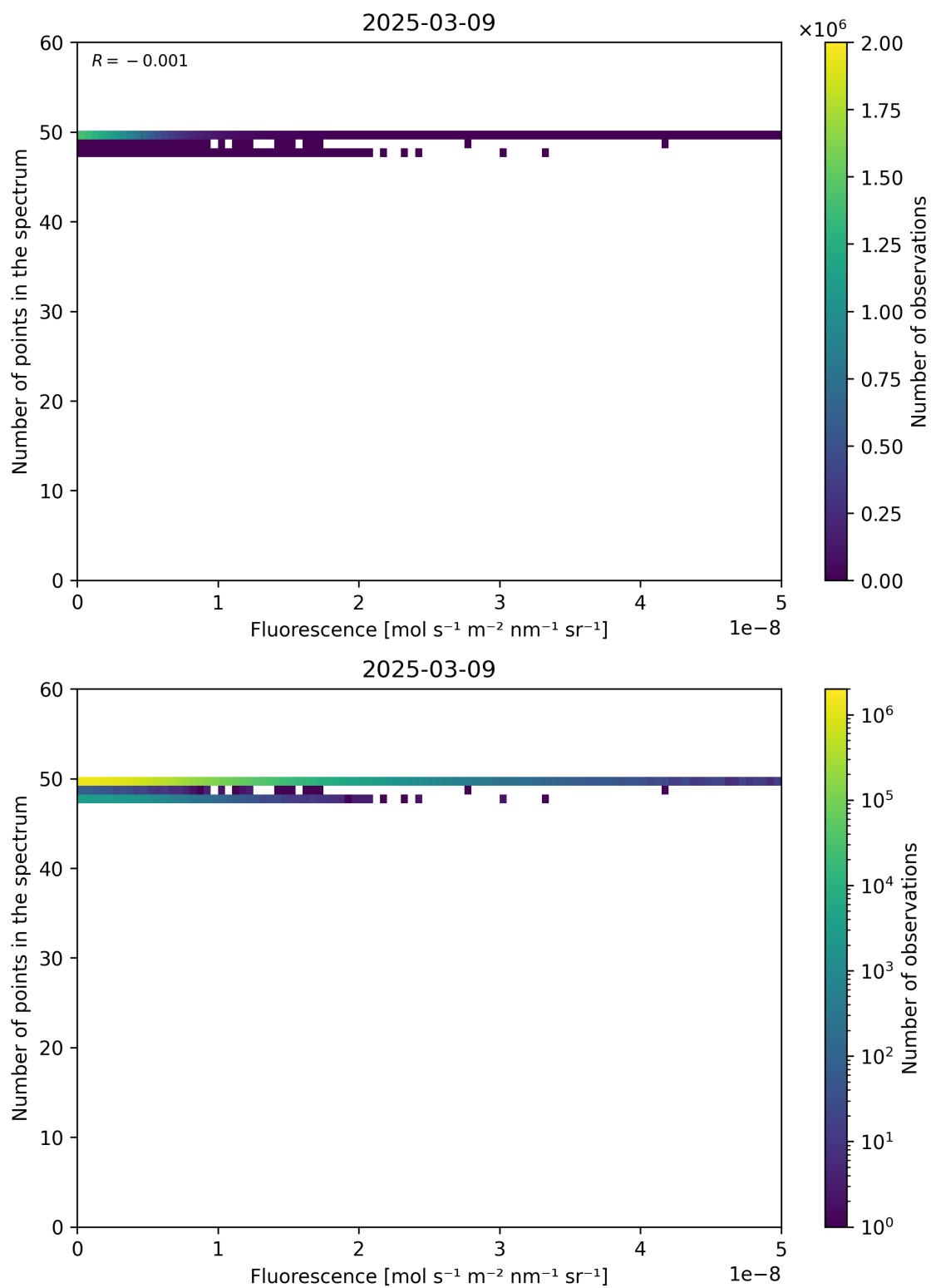
Figure 86: Scatter density plot of “Fluorescence” against “Number of points in the spectrum” for 2025-03-08 to 2025-03-10.
