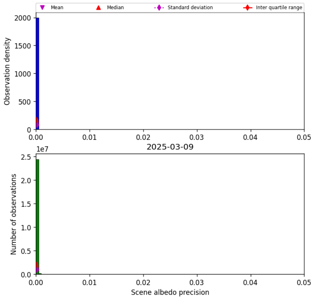
Figure 35: Histogram of “Scene albedo precision” for 2025-03-08 to 2025-03-10
