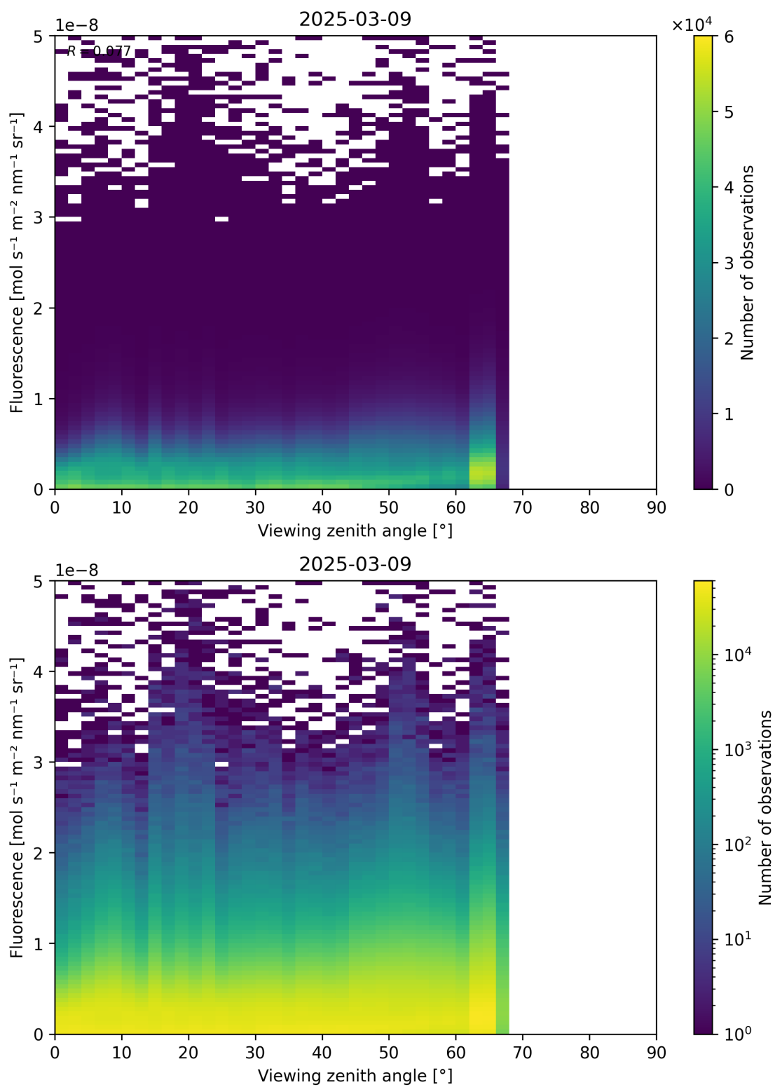
Figure 122: Scatter density plot of “Viewing zenith angle” against “Fluorescence” for 2025-03-08 to 2025-03-10.
