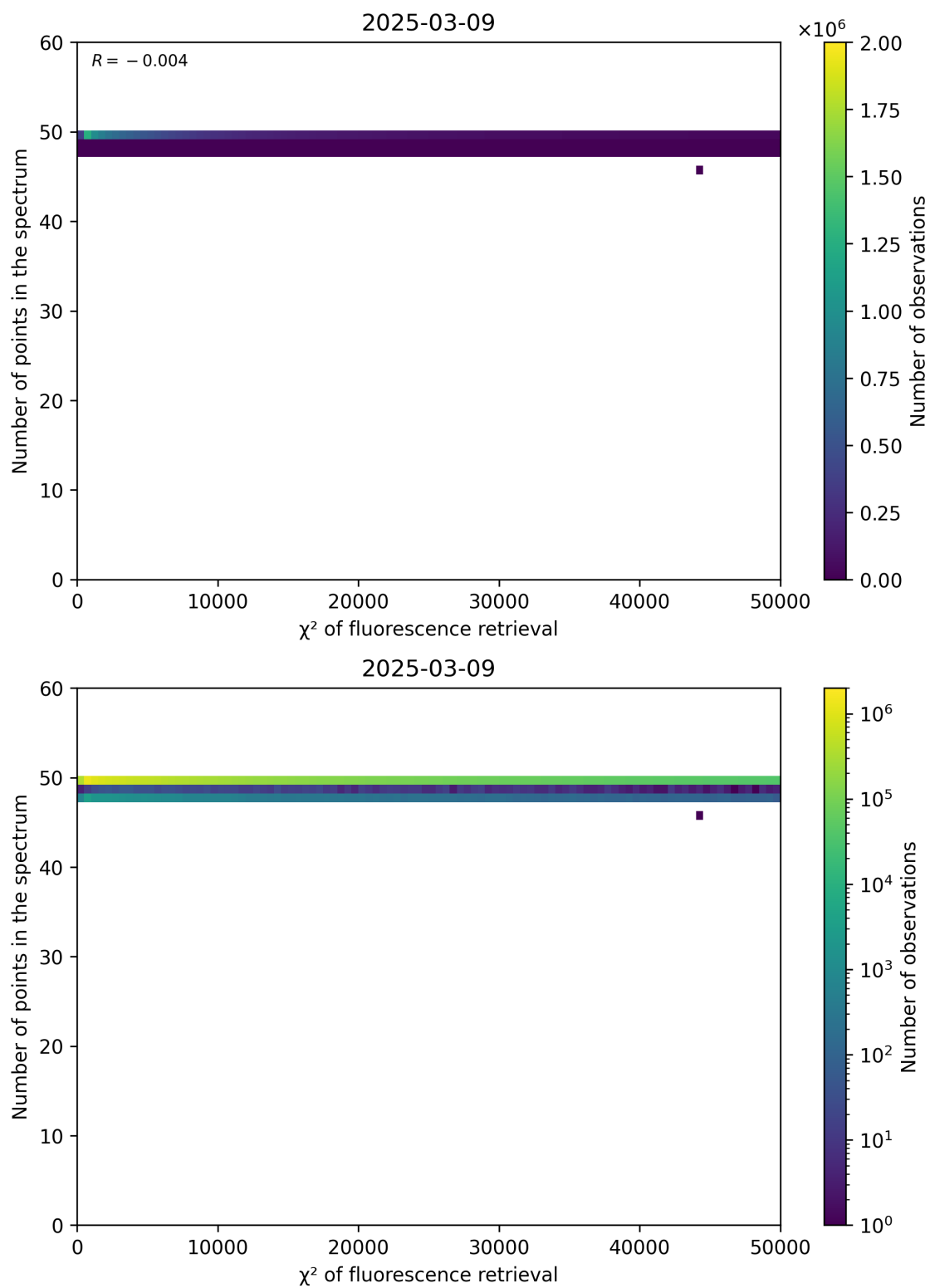
Figure 68: Scatter density plot of “ \chi^2 of fluorescence retrieval” against “Number of points in the spectrum” for 2025-03-08 to 2025-03-10.
