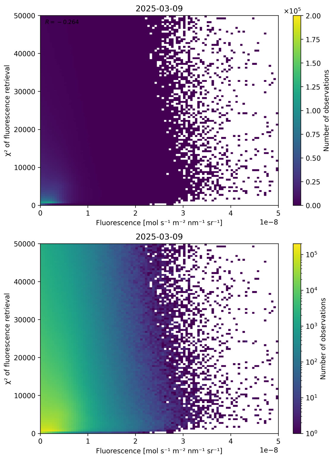
Figure 85: Scatter density plot of “Fluorescence” against “ \chi^2 of fluorescence retrieval” for 2025-03-08 to 2025-03-10.
