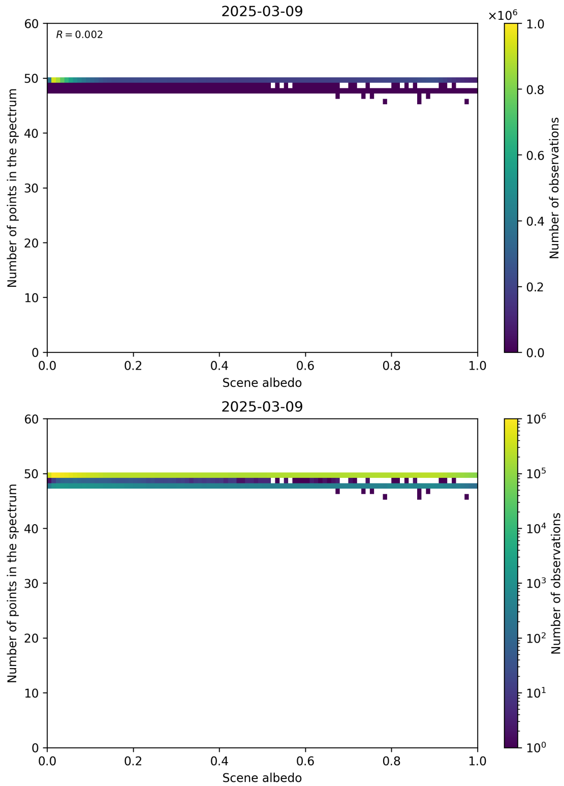
Figure 106: Scatter density plot of “Scene albedo” against “Number of points in the spectrum” for 2025-03-08 to 2025-03-10.
