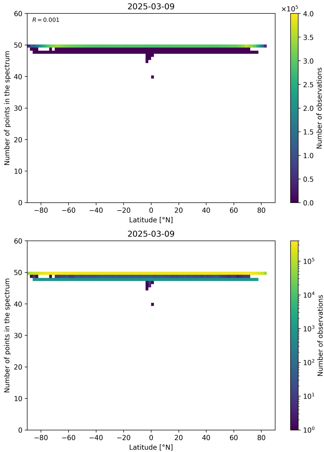
Figure 94: Scatter density plot of “Latitude” against “Number of points in the spectrum” for 2025-03-08 to 2025-03-10.
