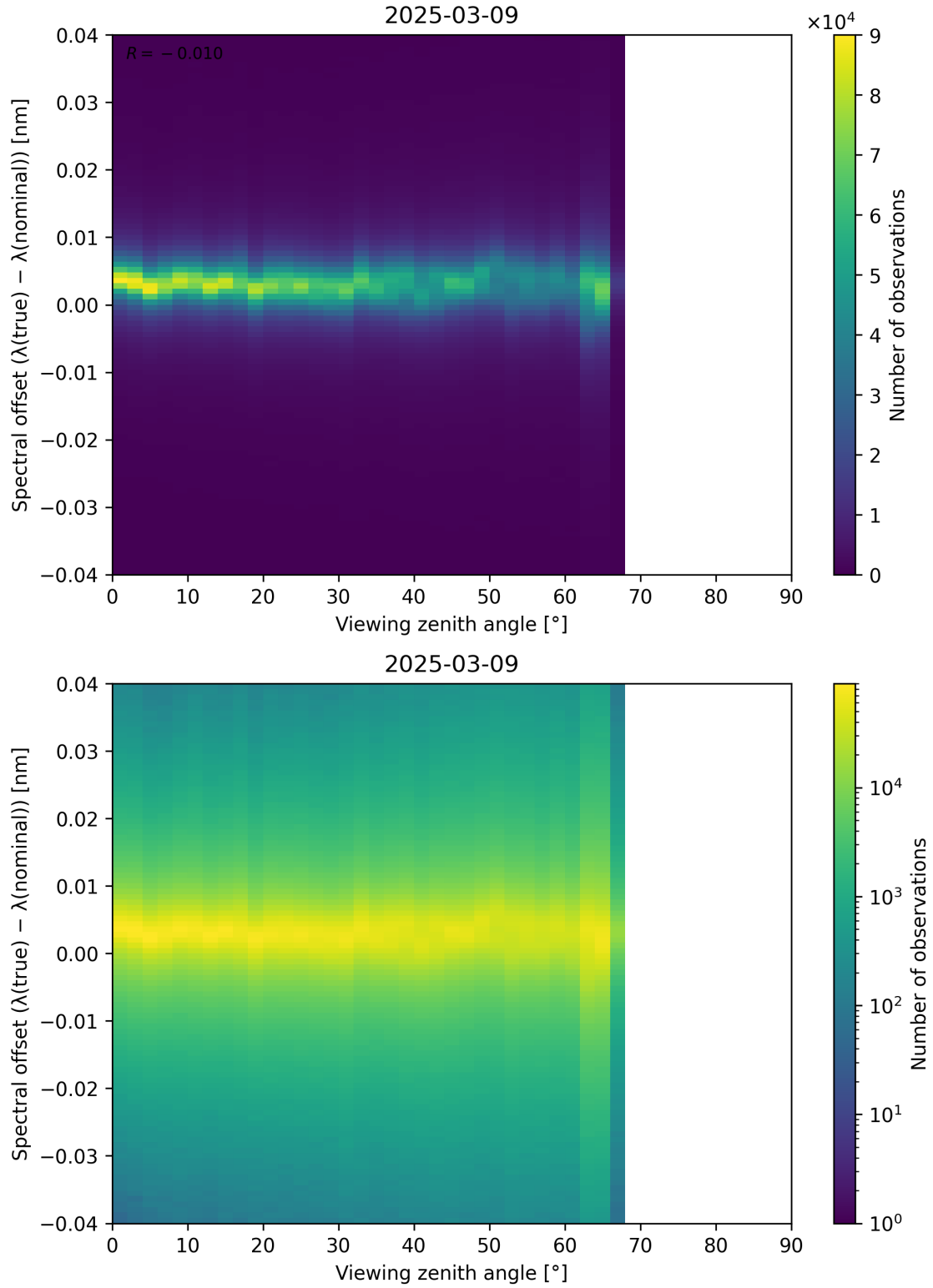
Figure 128: Scatter density plot of “Viewing zenith angle” against “Spectral offset ( \lambda_{\text{true}} - \lambda_{\text{nominal}} )” for 2025-03-08 to 2025-03-10.
