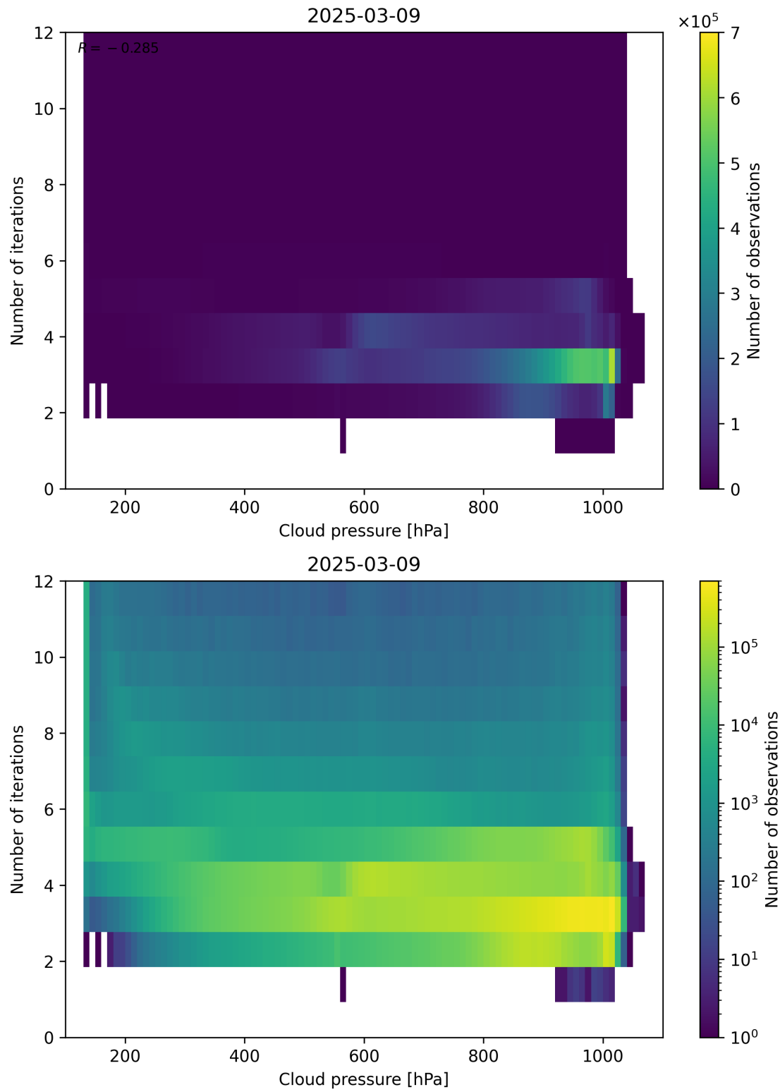
Figure 81: Scatter density plot of “Cloud pressure” against “Number of iterations” for 2025-03-08 to 2025-03-10.
