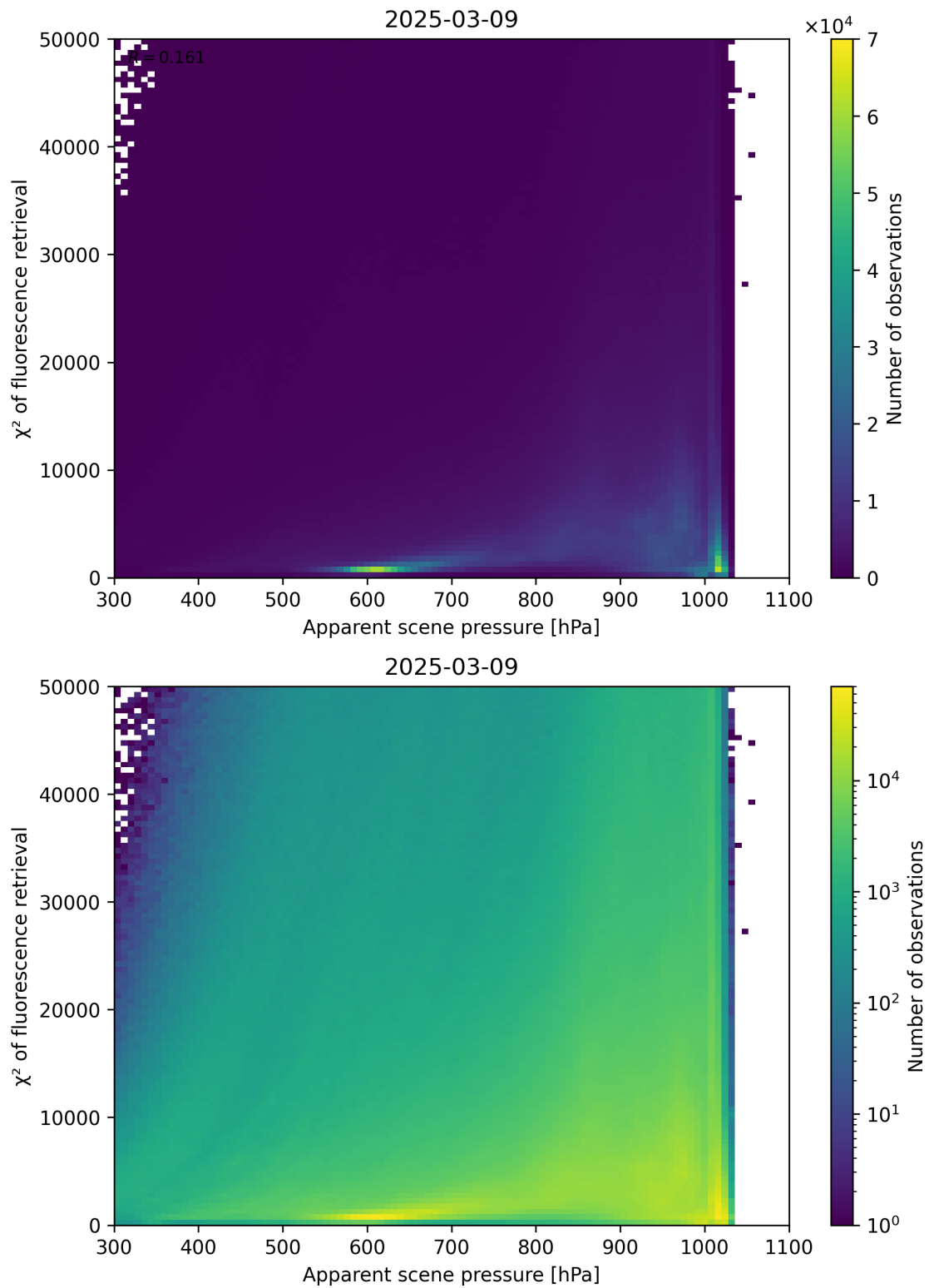
Figure 63: Scatter density plot of “Apparent scene pressure” against “ \chi^2 of fluorescence retrieval” for 2025-03-08 to 2025-03-10.
