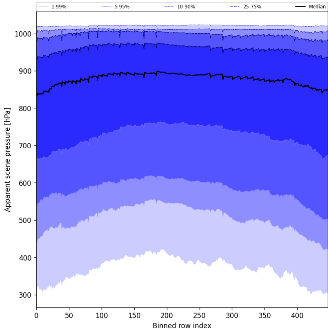
Figure 53: Along track statistics of “Apparent scene pressure” for 2025-03-08 to 2025-03-10
