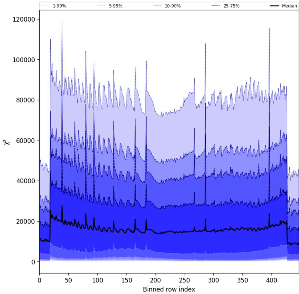
Figure 55: Along track statistics of “ \chi^2 ” for 2025-03-08 to 2025-03-10
