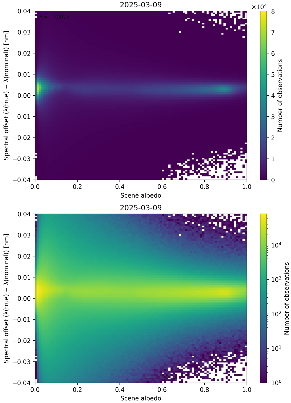
Figure 107: Scatter density plot of “Scene albedo” against “Spectral offset ( \lambda_{\text{true}} - \lambda_{\text{nominal}} )” for 2025-03-08 to 2025-03-10.
