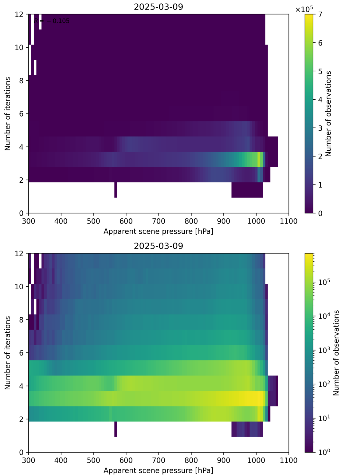
Figure 65: Scatter density plot of “Apparent scene pressure” against “Number of iterations” for 2025-03-08 to 2025-03-10.
