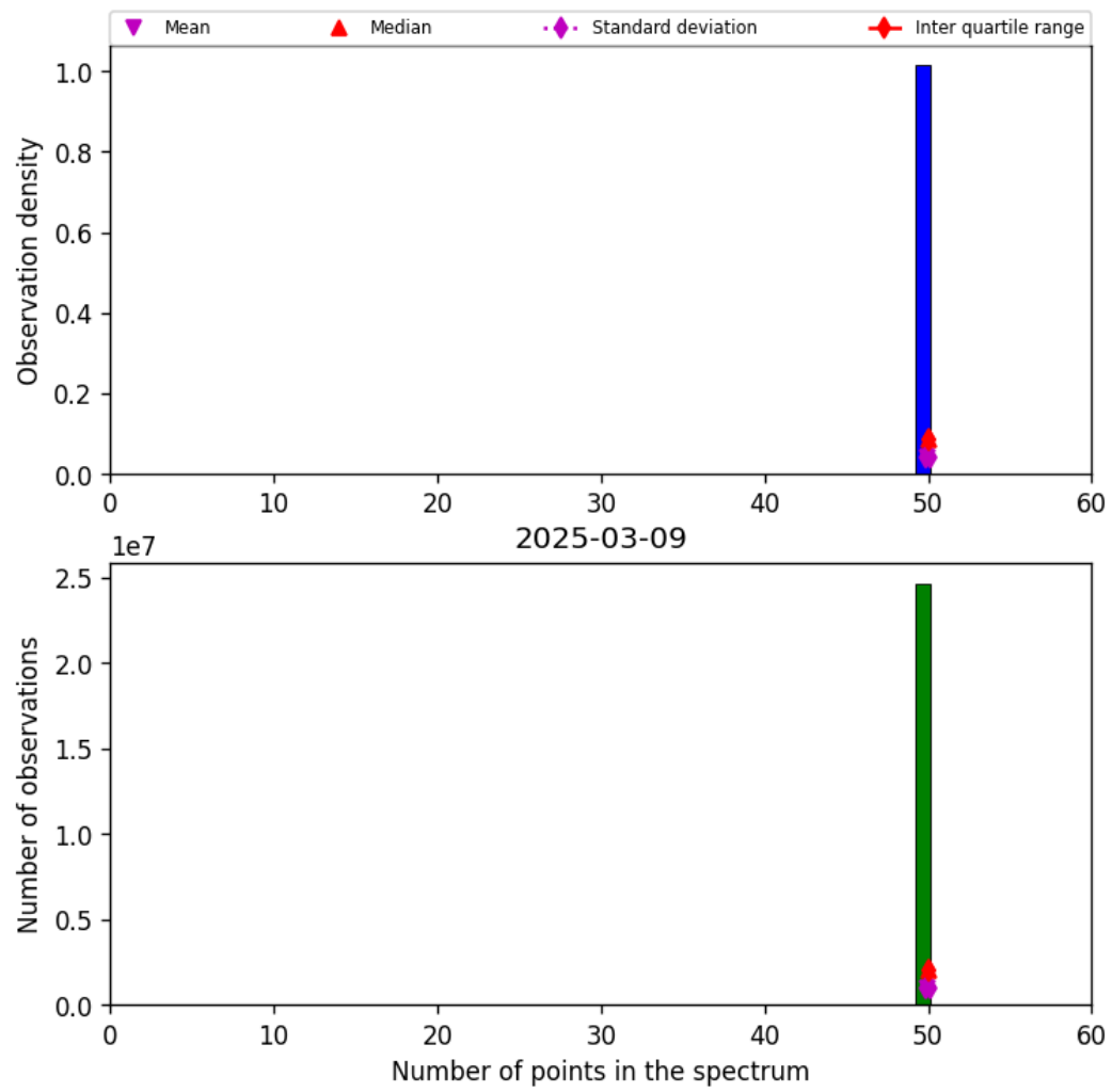
Figure 44: Histogram of "Number of points in the spectrum" for 2025-03-08 to 2025-03-10
