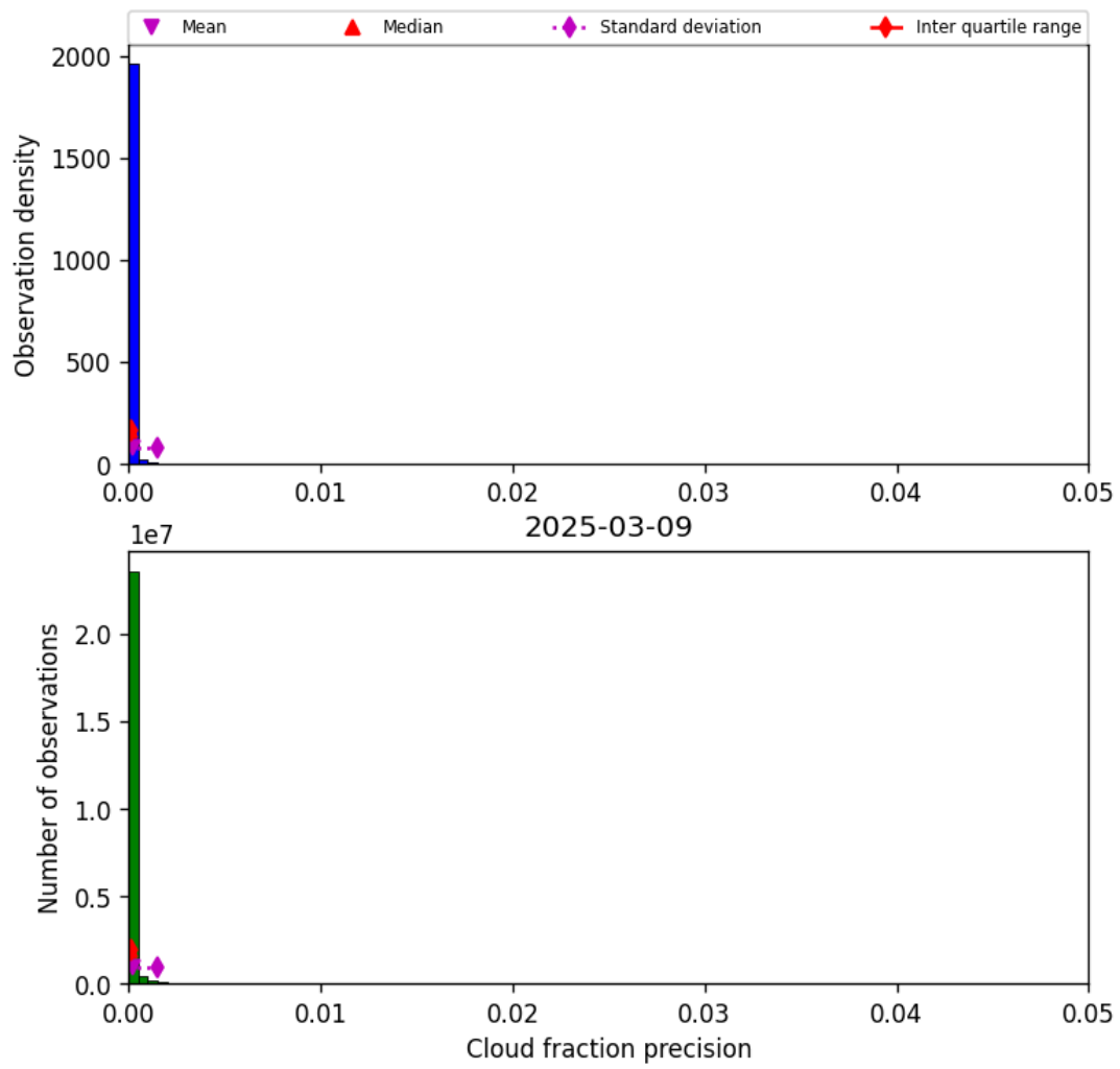
Figure 33: Histogram of “Cloud fraction precision” for 2025-03-08 to 2025-03-10
