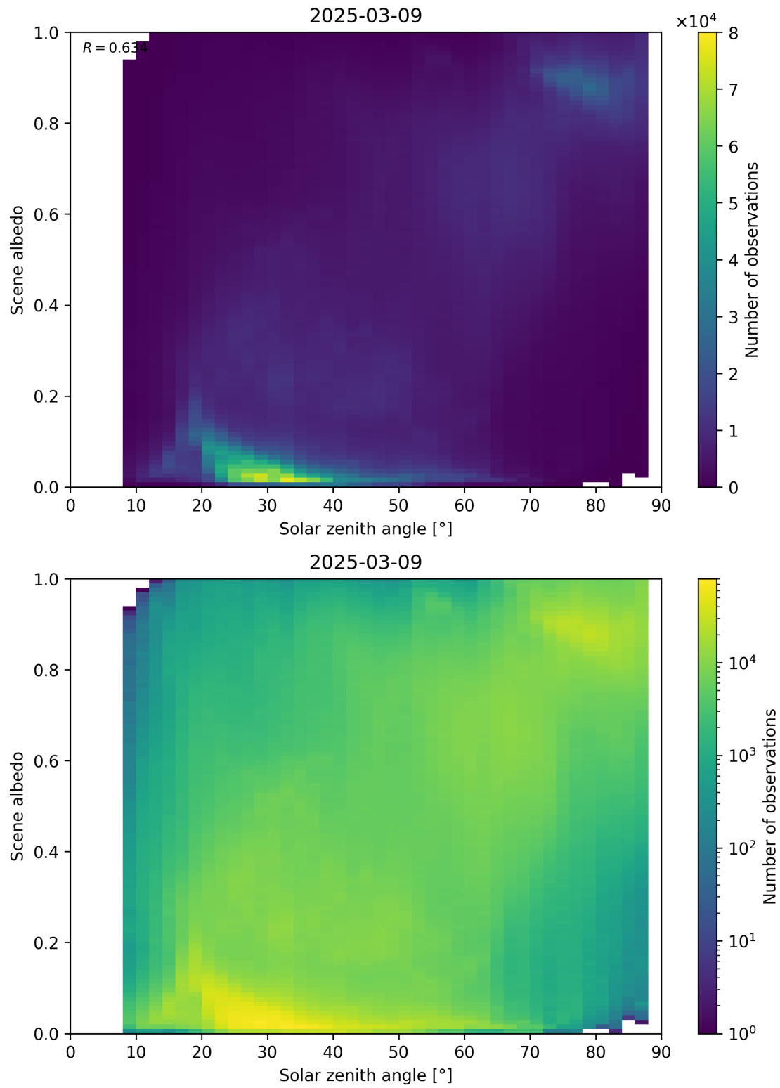
Figure 116: Scatter density plot of “Solar zenith angle” against “Scene albedo” for 2025-03-08 to 2025-03-10.
