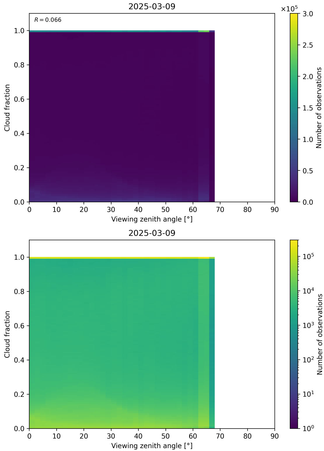
Figure 120: Scatter density plot of “Viewing zenith angle” against “Cloud fraction” for 2025-03-08 to 2025-03-10.
