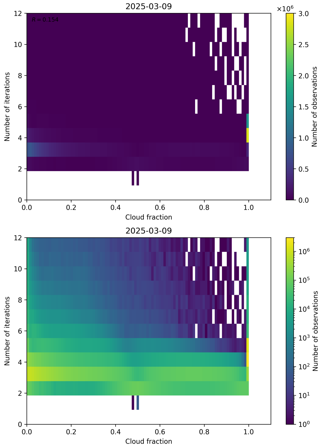
Figure 73: Scatter density plot of “Cloud fraction” against “Number of iterations” for 2025-03-08 to 2025-03-10.
