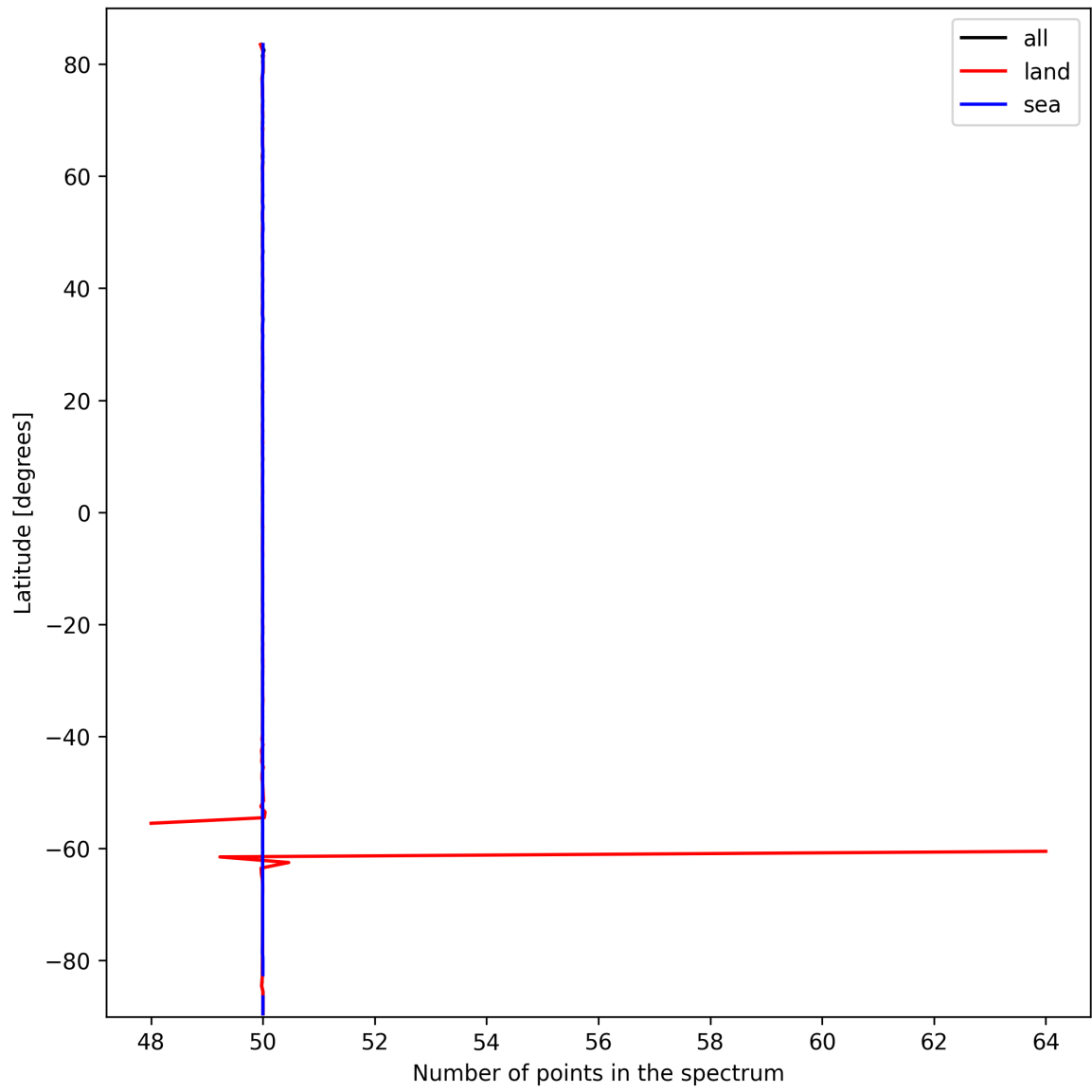
Figure 27: Zonal average of “Number of points in the spectrum” for 2025-03-08 to 2025-03-10.
