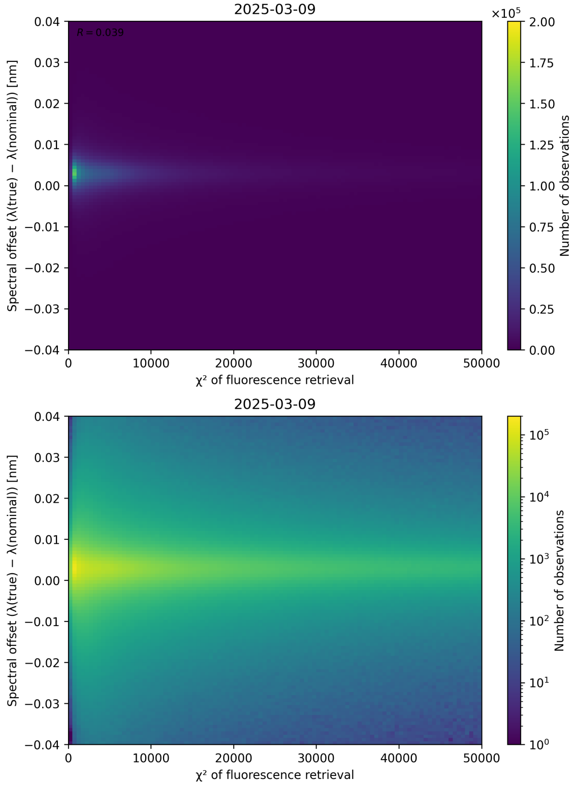
Figure 69: Scatter density plot of “ \chi^2 of fluorescence retrieval” against “Spectral offset ( \lambda_{\text{true}} - \lambda_{\text{nominal}} )” for 2025-03-08 to 2025-03-10.
