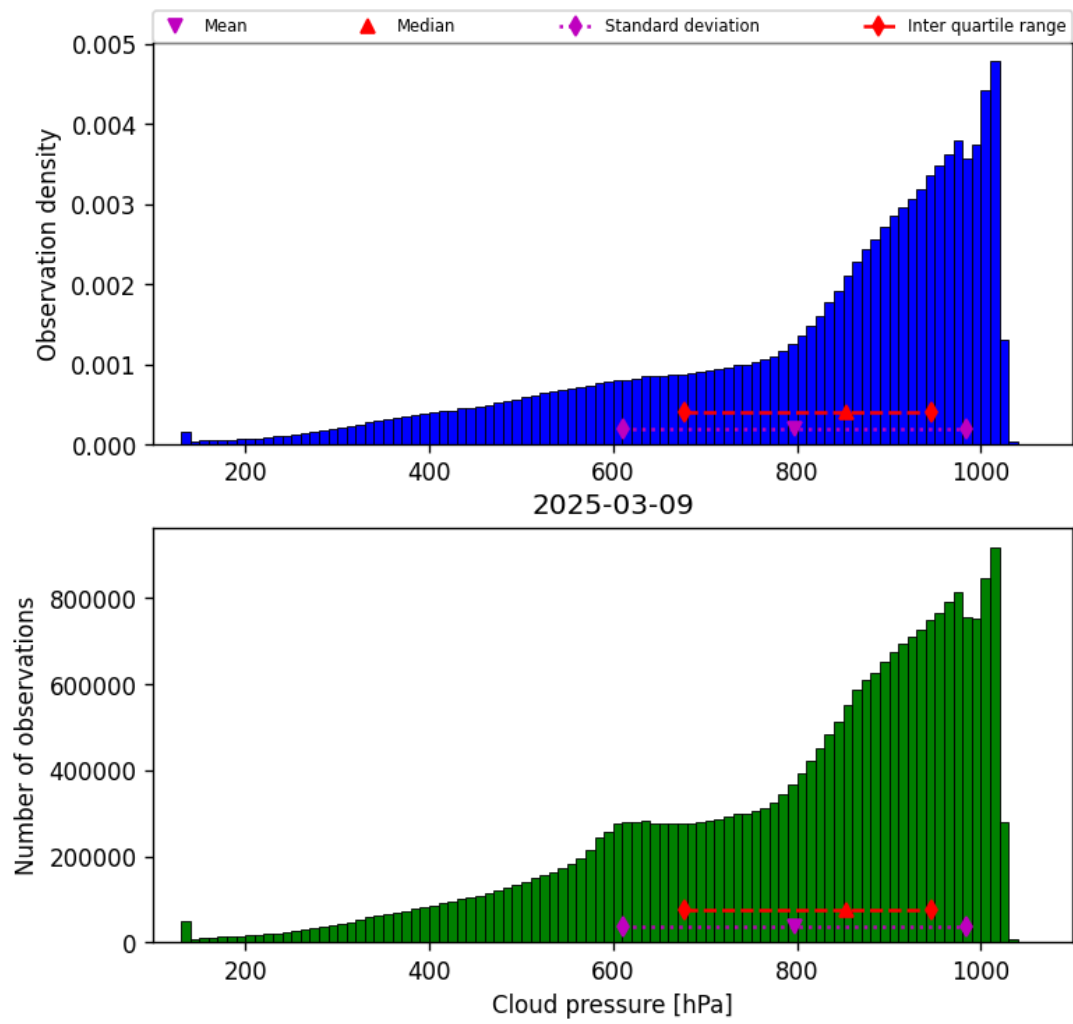
Figure 30: Histogram of “Cloud pressure” for 2025-03-08 to 2025-03-10
