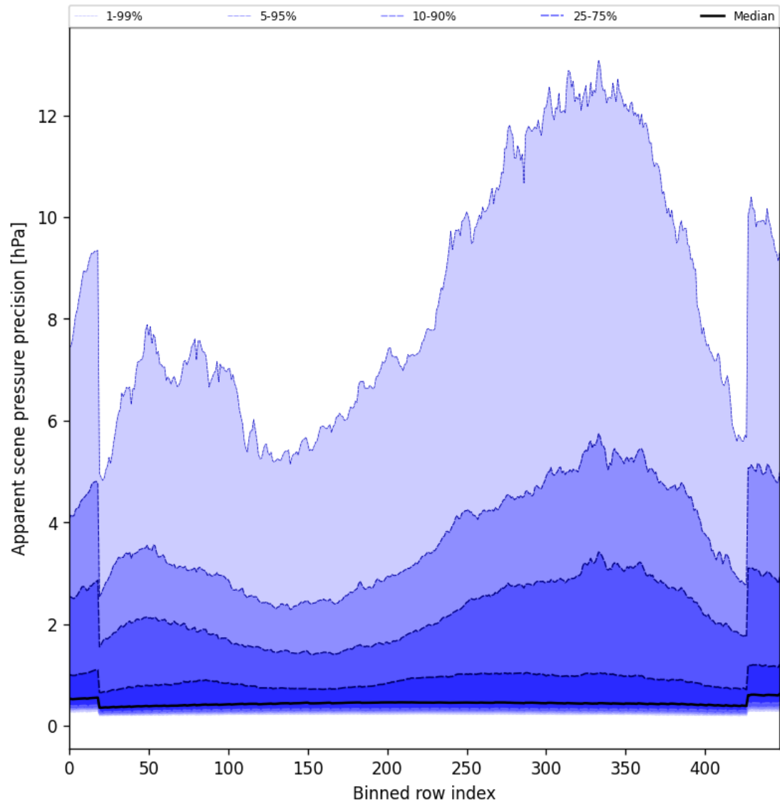
Figure 54: Along track statistics of “Apparent scene pressure precision” for 2025-03-08 to 2025-03-10
