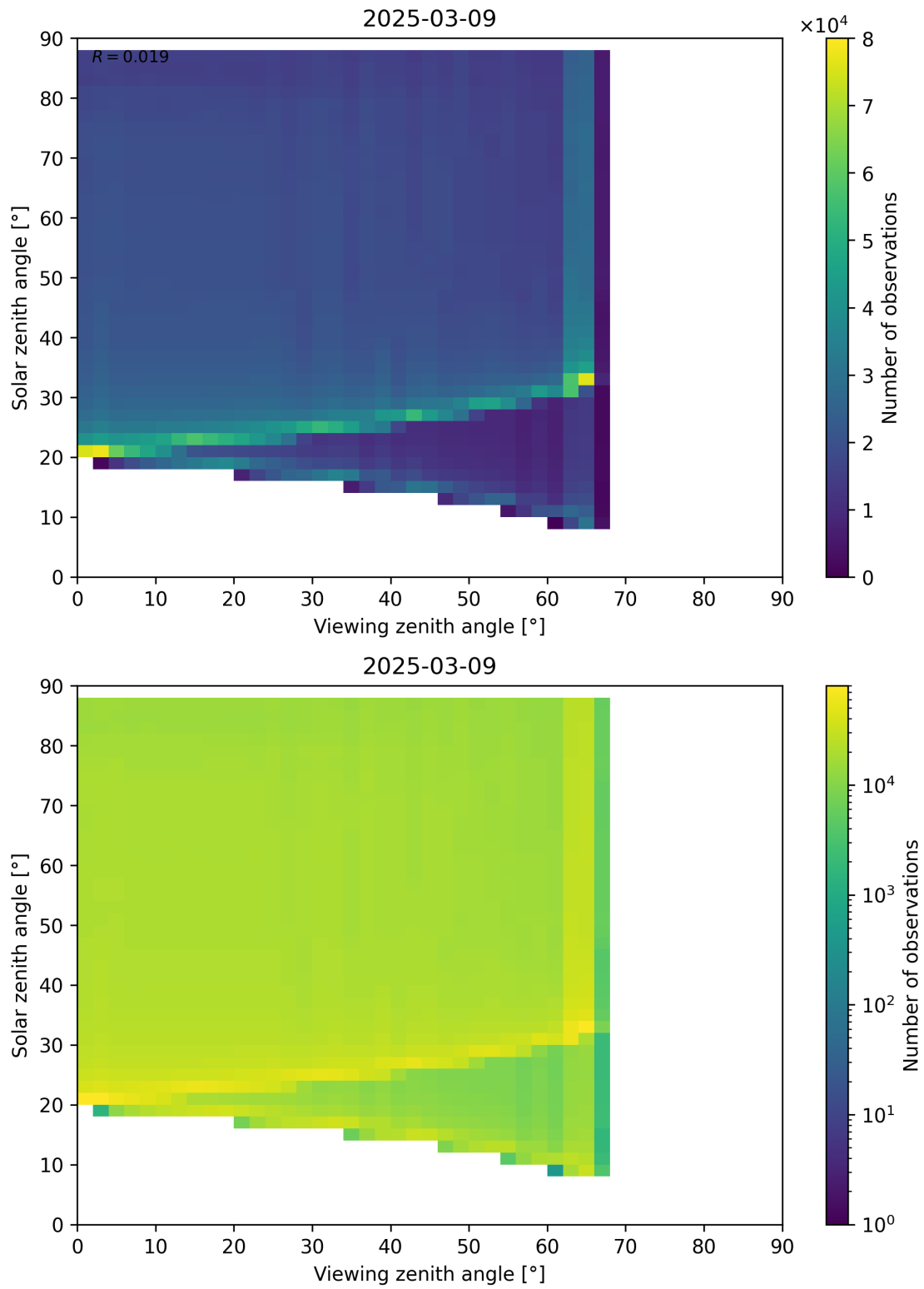
Figure 127: Scatter density plot of “Viewing zenith angle” against “Solar zenith angle” for 2025-03-08 to 2025-03-10.
