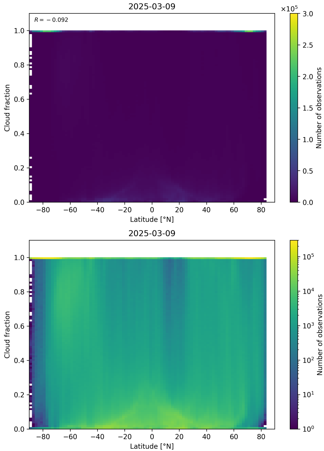
Figure 90: Scatter density plot of “Latitude” against “Cloud fraction” for 2025-03-08 to 2025-03-10.
