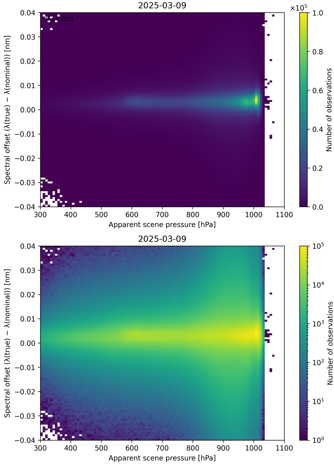
Figure 67: Scatter density plot of “Apparent scene pressure” against “Spectral offset ( \lambda_{\text{true}} - \lambda_{\text{nominal}} )” for 2025-03-08 to 2025-03-10.
