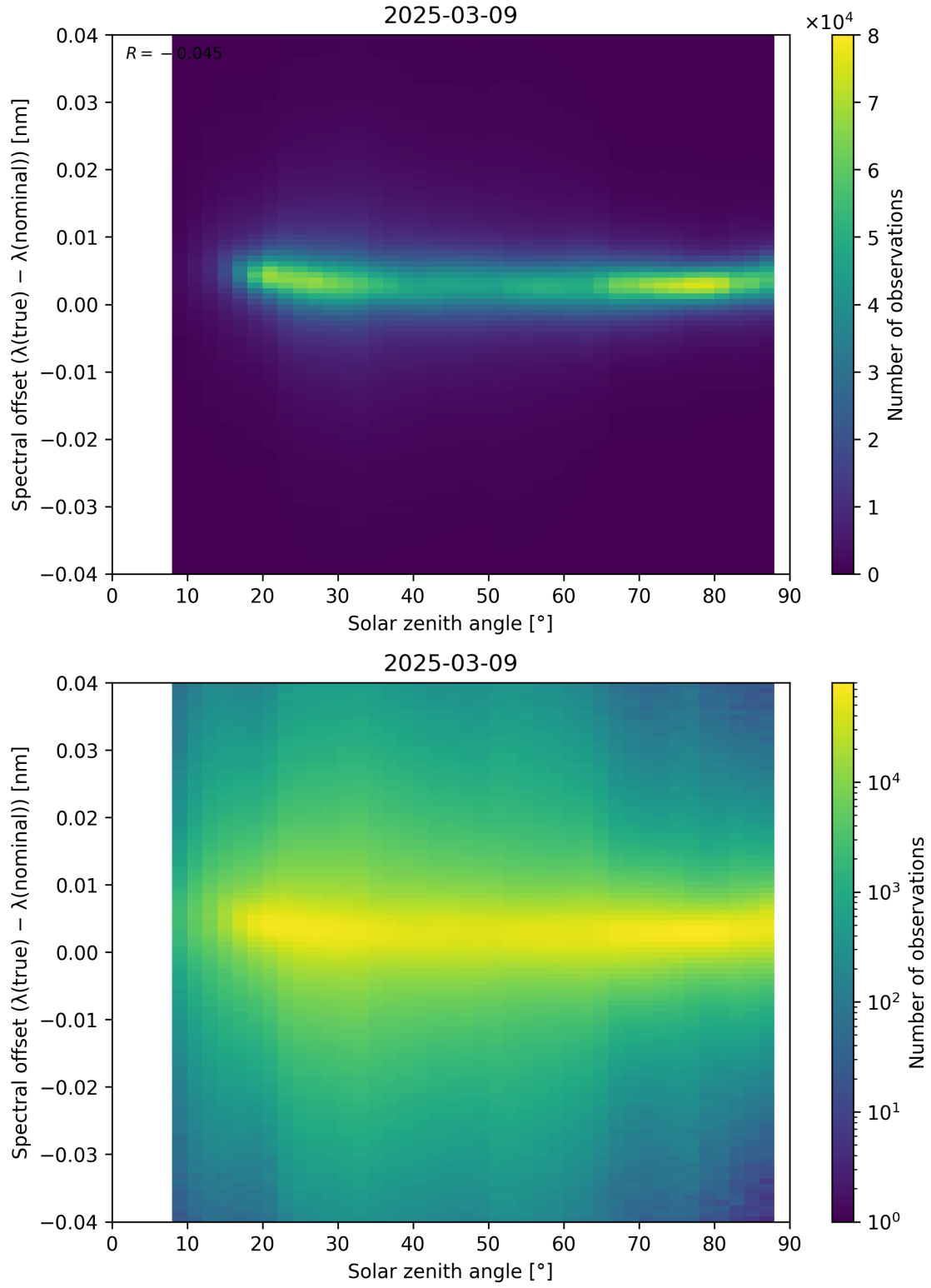
Figure 117: Scatter density plot of “Solar zenith angle” against “Spectral offset ( \lambda_{\text{true}} - \lambda_{\text{nominal}} )” for 2025-03-08 to 2025-03-10.
