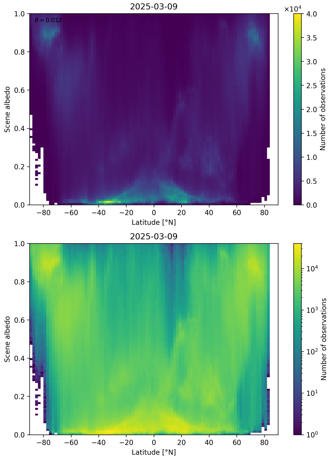
Figure 95: Scatter density plot of “Latitude” against “Scene albedo” for 2025-03-08 to 2025-03-10.
