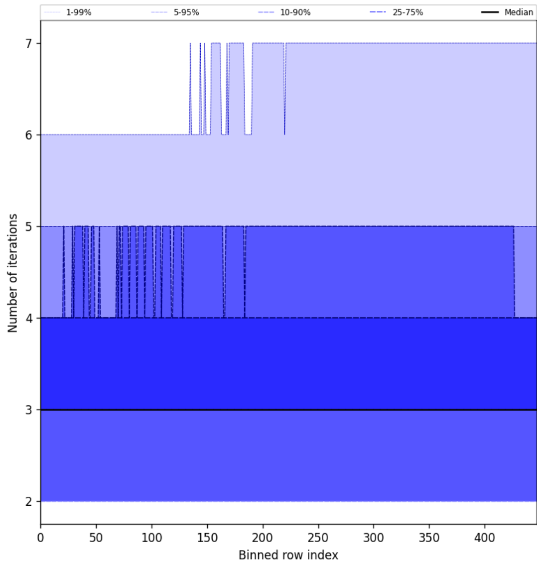
Figure 56: Along track statistics of “Number of iterations” for 2025-03-08 to 2025-03-10
