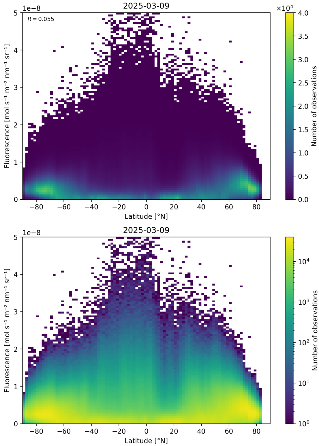
Figure 92: Scatter density plot of “Latitude” against “Fluorescence” for 2025-03-08 to 2025-03-10.
