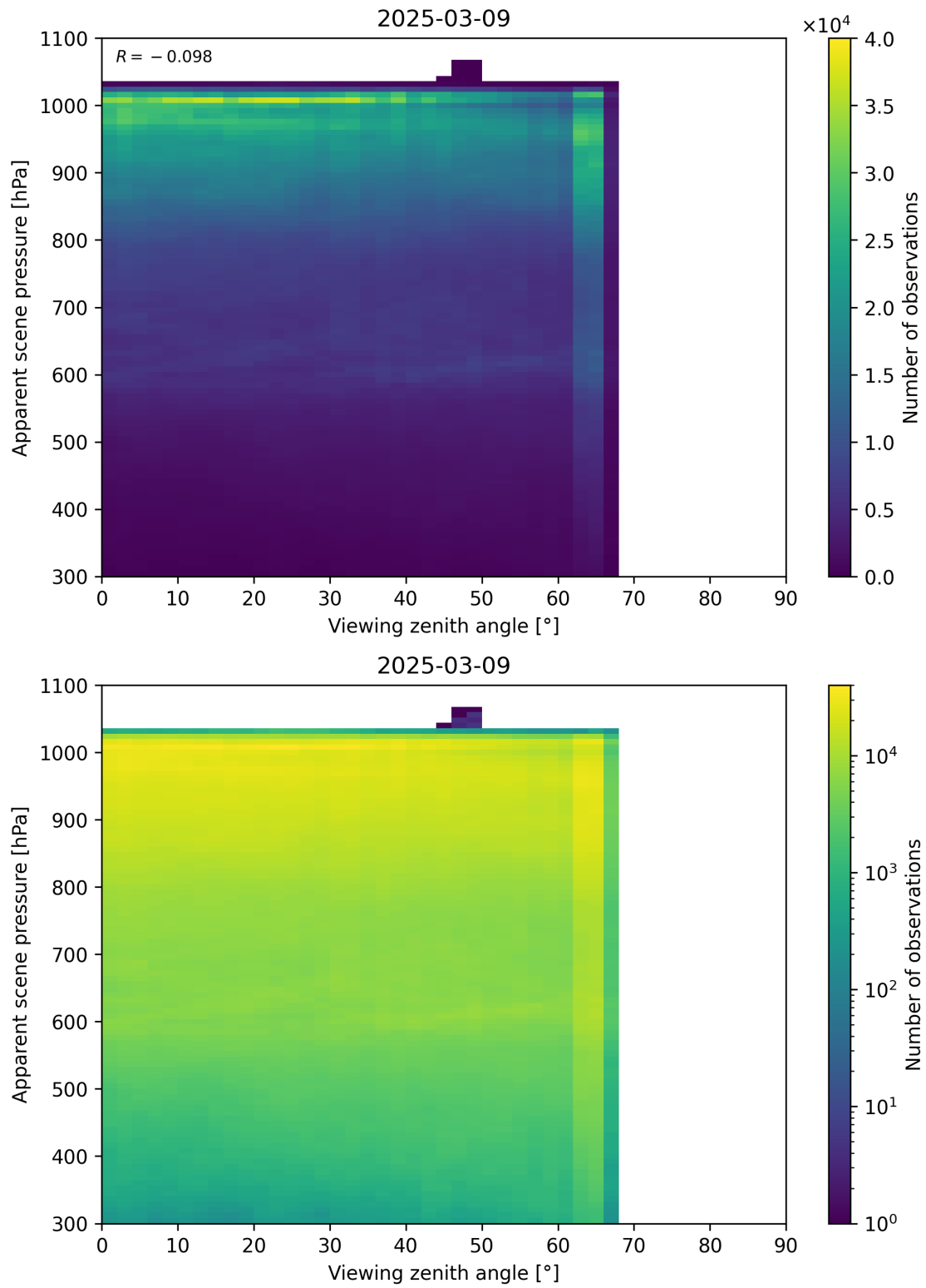
Figure 118: Scatter density plot of “Viewing zenith angle” against “Apparent scene pressure” for 2025-03-08 to 2025-03-10.
