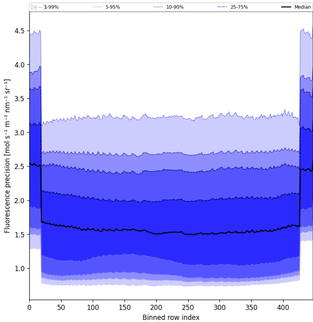
Figure 58: Along track statistics of “Fluorescence precision” for 2025-03-08 to 2025-03-10
