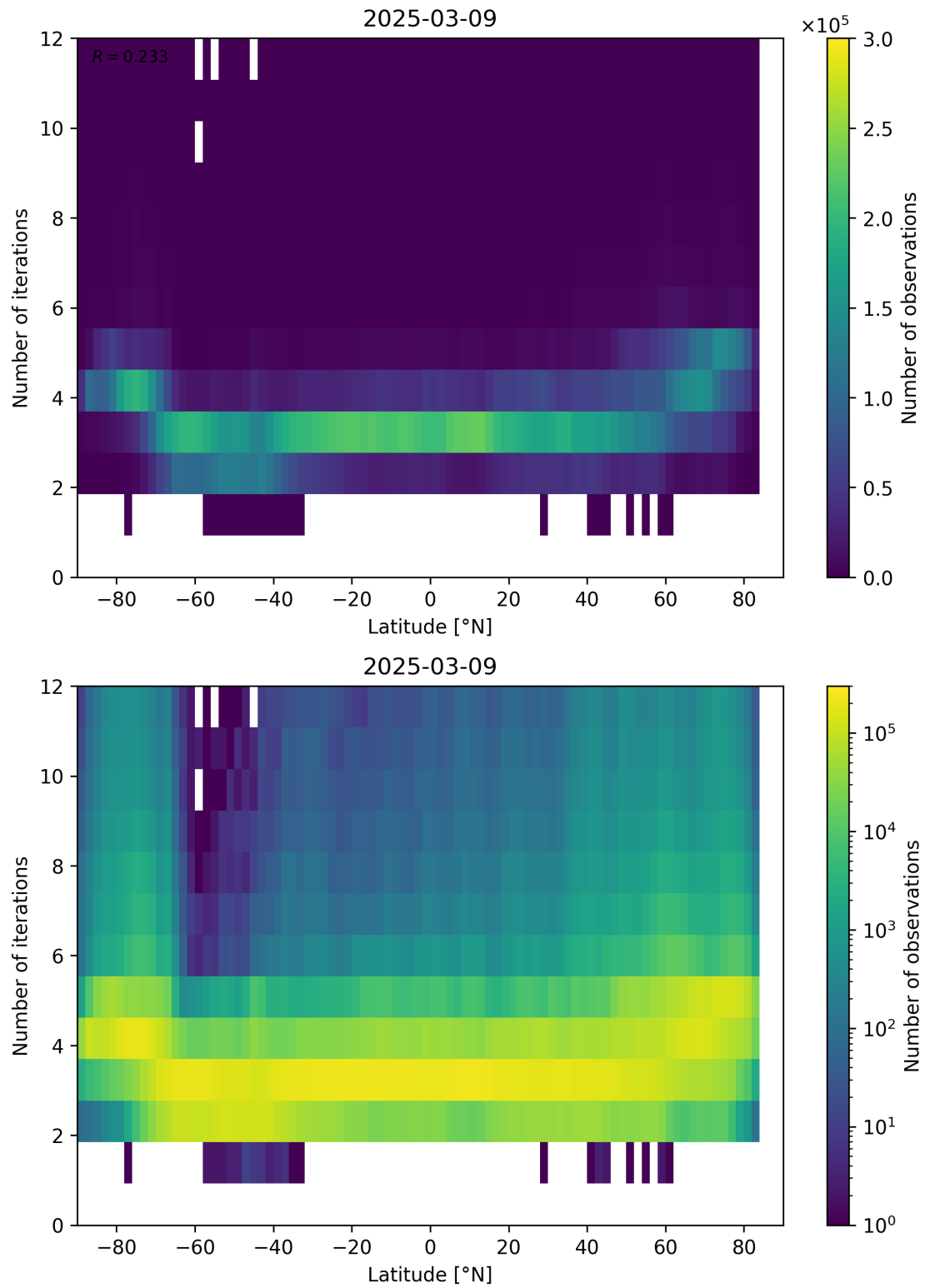
Figure 93: Scatter density plot of “Latitude” against “Number of iterations” for 2025-03-08 to 2025-03-10.
