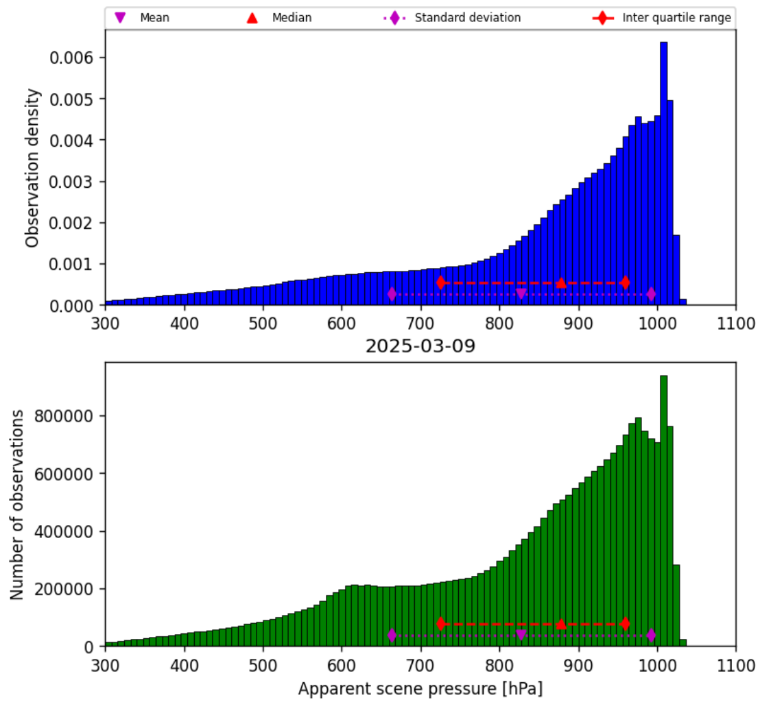
Figure 36: Histogram of “Apparent scene pressure” for 2025-03-08 to 2025-03-10
