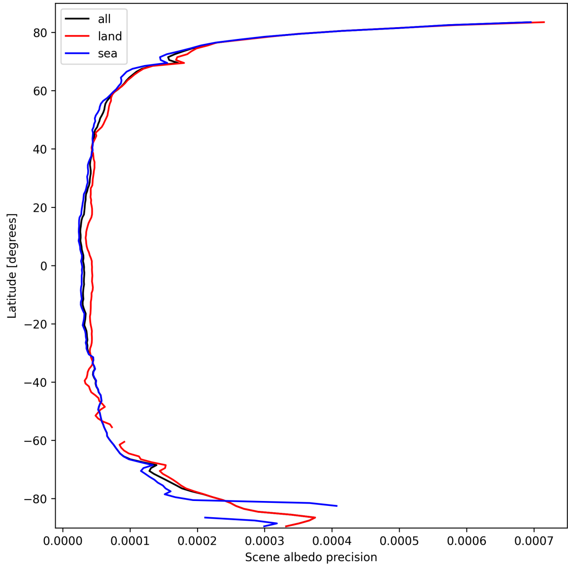
Figure 18: Zonal average of “Scene albedo precision” for 2025-03-08 to 2025-03-10.
