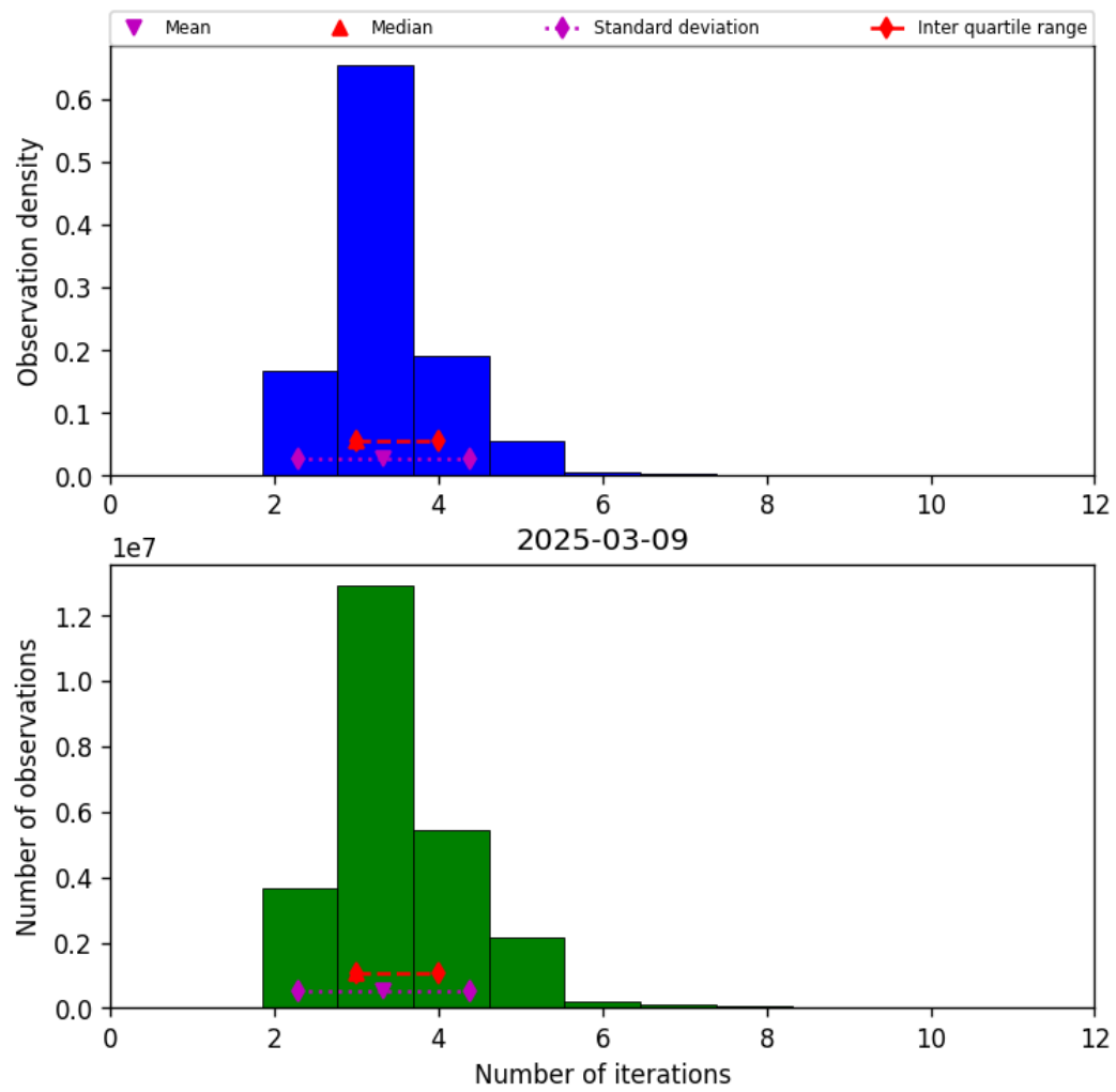
Figure 39: Histogram of “Number of iterations” for 2025-03-08 to 2025-03-10
