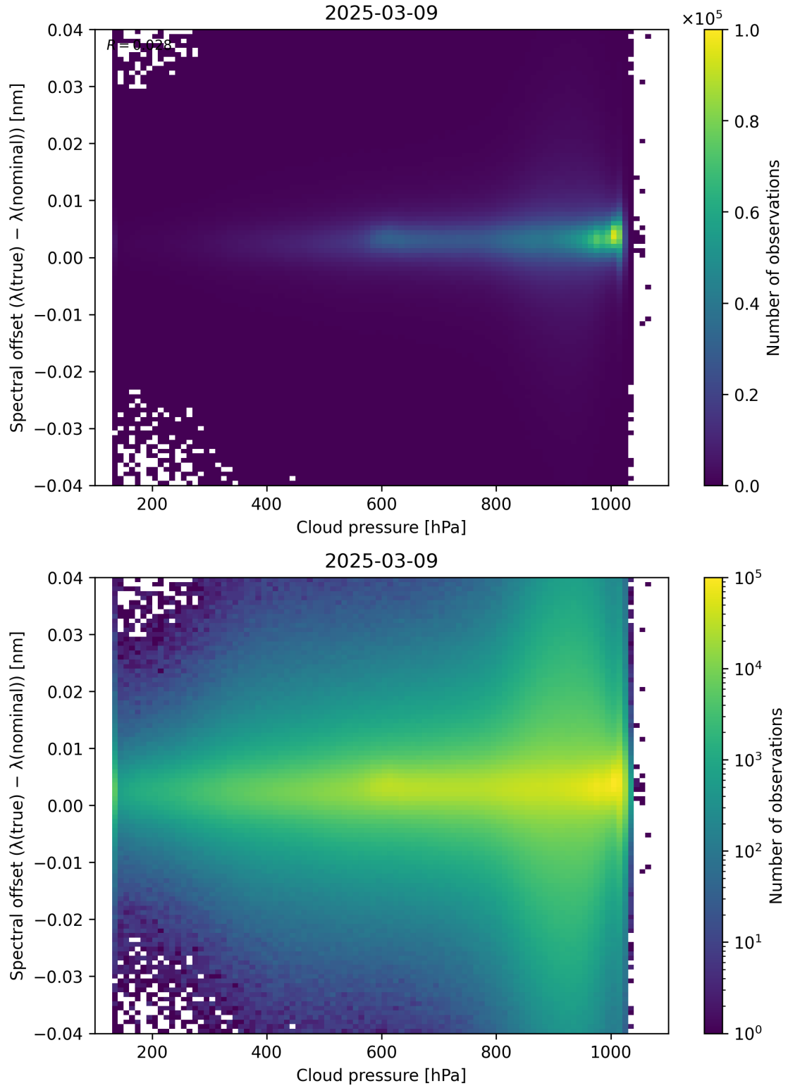
Figure 84: Scatter density plot of “Cloud pressure” against “Spectral offset ( \lambda_{\text{true}} - \lambda_{\text{nominal}} )” for 2025-03-08 to 2025-03-10.
