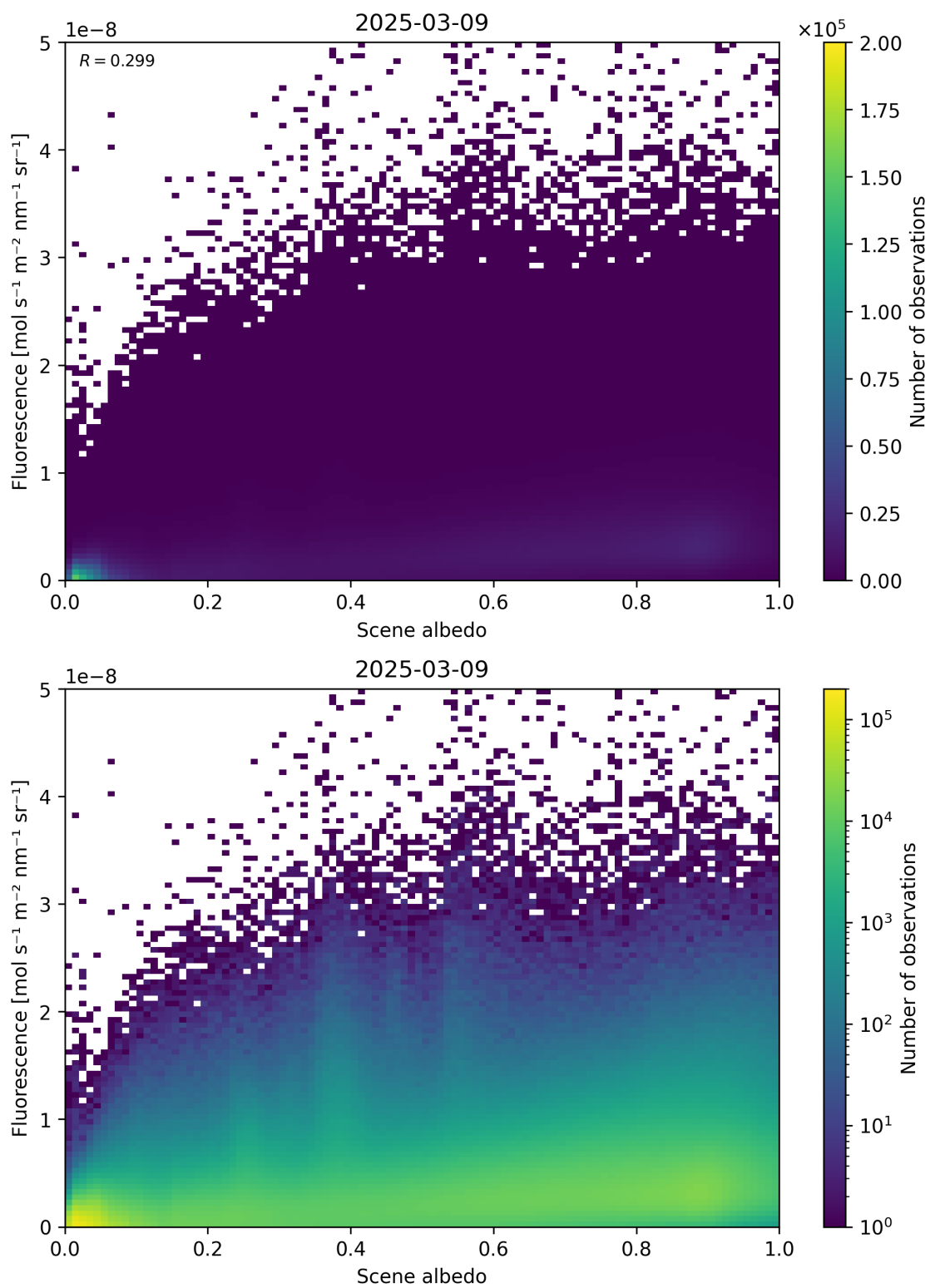
Figure 104: Scatter density plot of “Scene albedo” against “Fluorescence” for 2025-03-08 to 2025-03-10.
