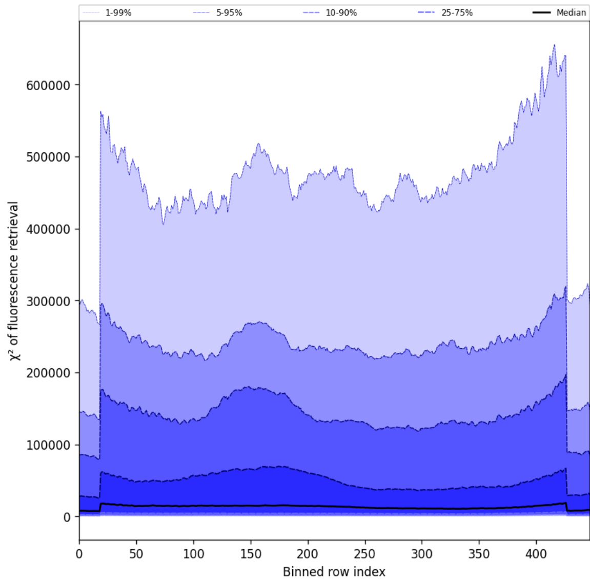
Figure 59: Along track statistics of “ \chi^2 of fluorescence retrieval” for 2025-03-08 to 2025-03-10
