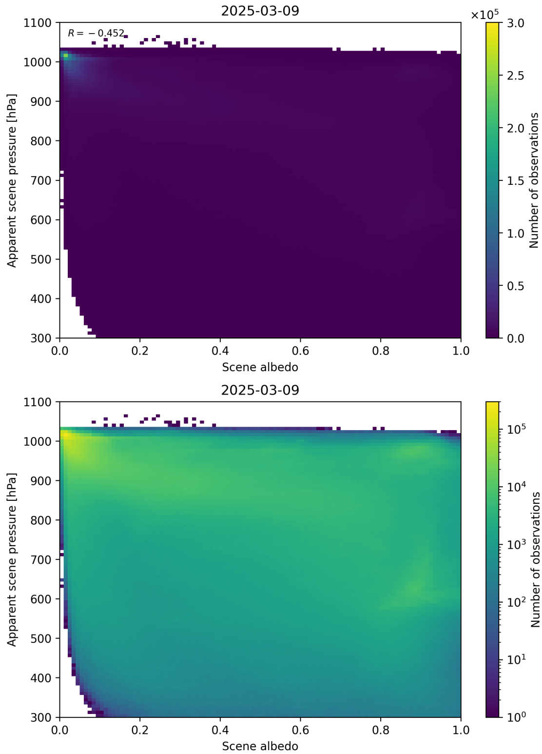
Figure 102: Scatter density plot of “Scene albedo” against “Apparent scene pressure” for 2025-03-08 to 2025-03-10.
