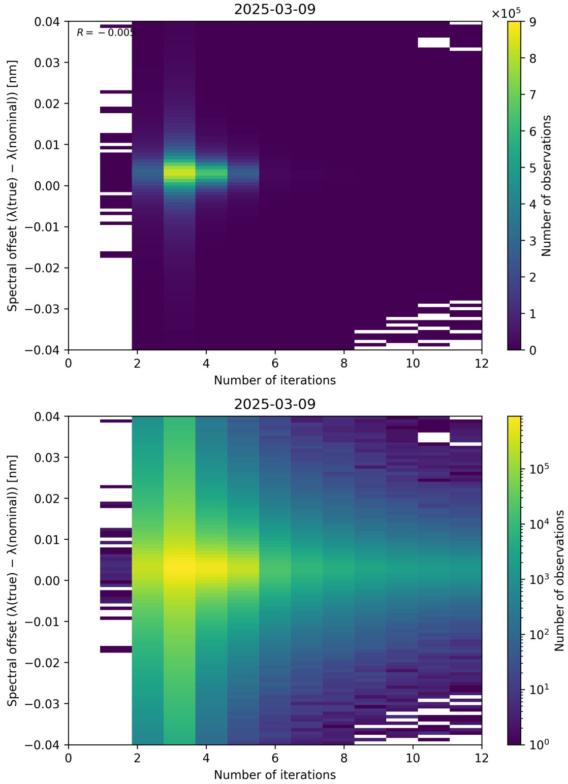
Figure 100: Scatter density plot of “Number of iterations” against “Spectral offset ( \lambda_{\text{true}} - \lambda_{\text{nominal}} )” for 2025-03-08 to 2025-03-10.
