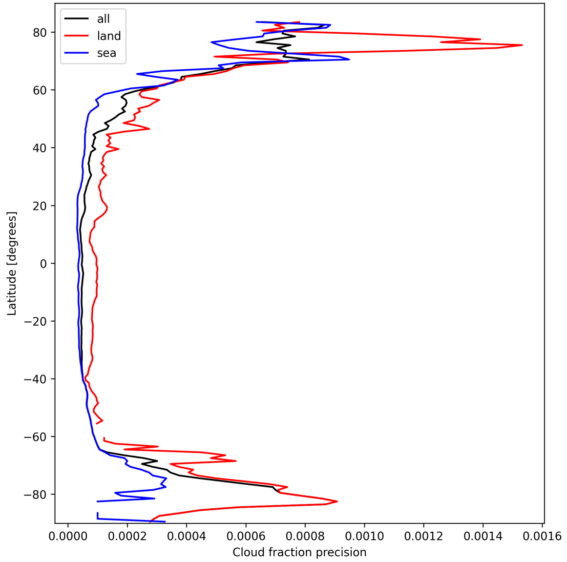
Figure 16: Zonal average of “Cloud fraction precision” for 2025-03-08 to 2025-03-10.
