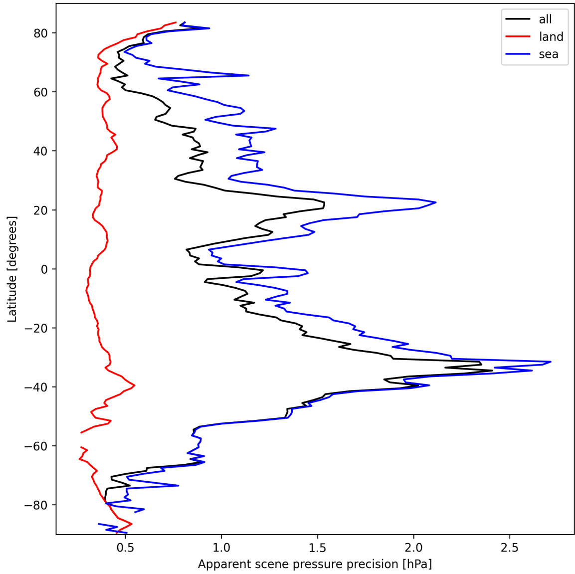
Figure 20: Zonal average of “Apparent scene pressure precision” for 2025-03-08 to 2025-03-10.
