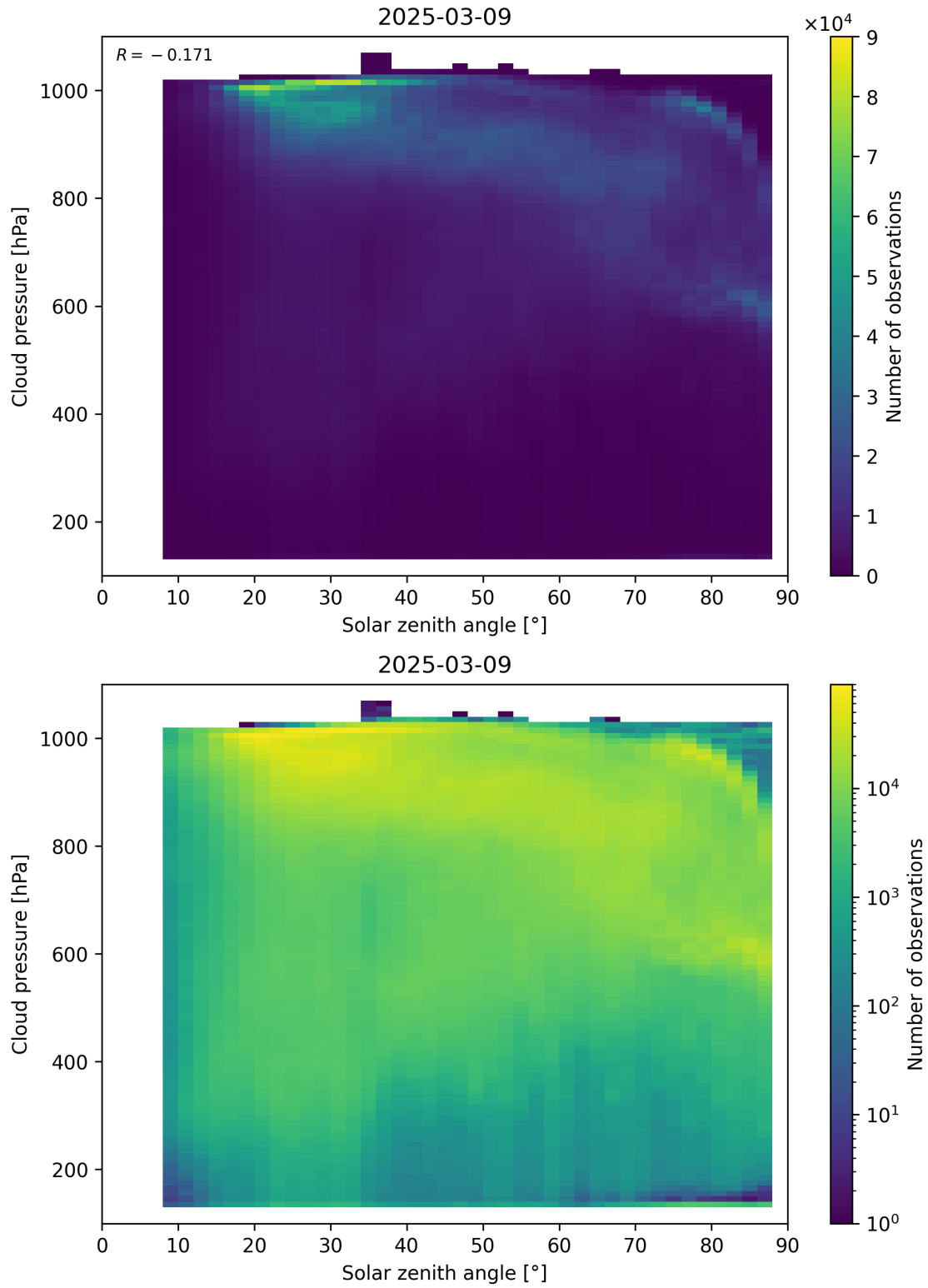
Figure 111: Scatter density plot of “Solar zenith angle” against “Cloud pressure” for 2025-03-08 to 2025-03-10.
