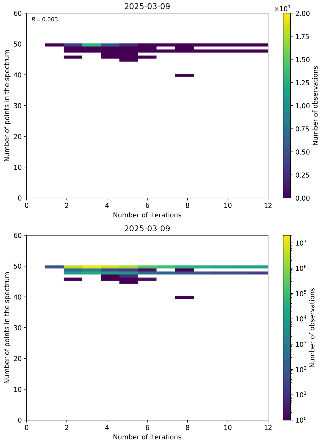
Figure 99: Scatter density plot of “Number of iterations” against “Number of points in the spectrum” for 2025-03-08 to 2025-03-10.
