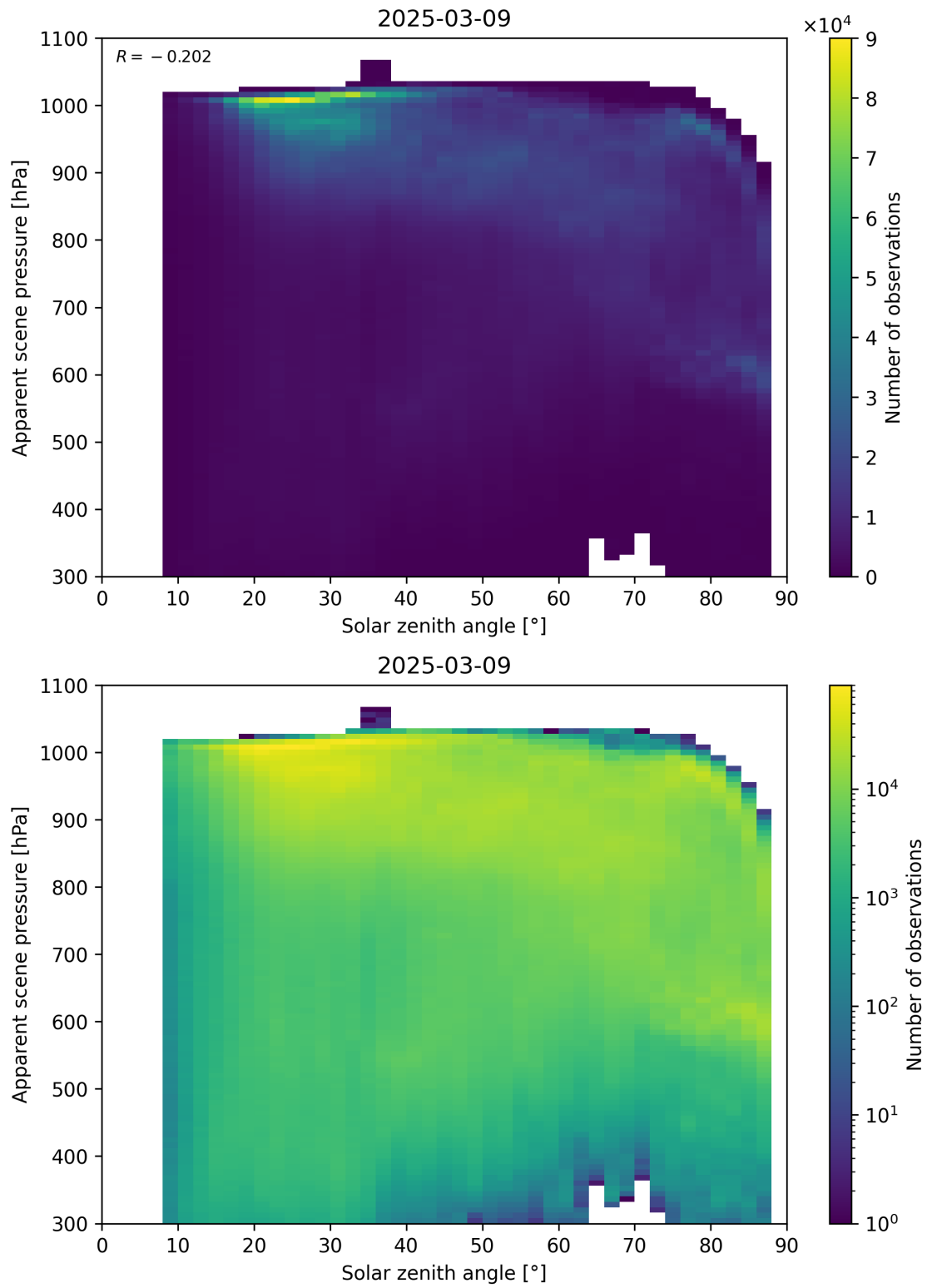
Figure 108: Scatter density plot of “Solar zenith angle” against “Apparent scene pressure” for 2025-03-08 to 2025-03-10.
