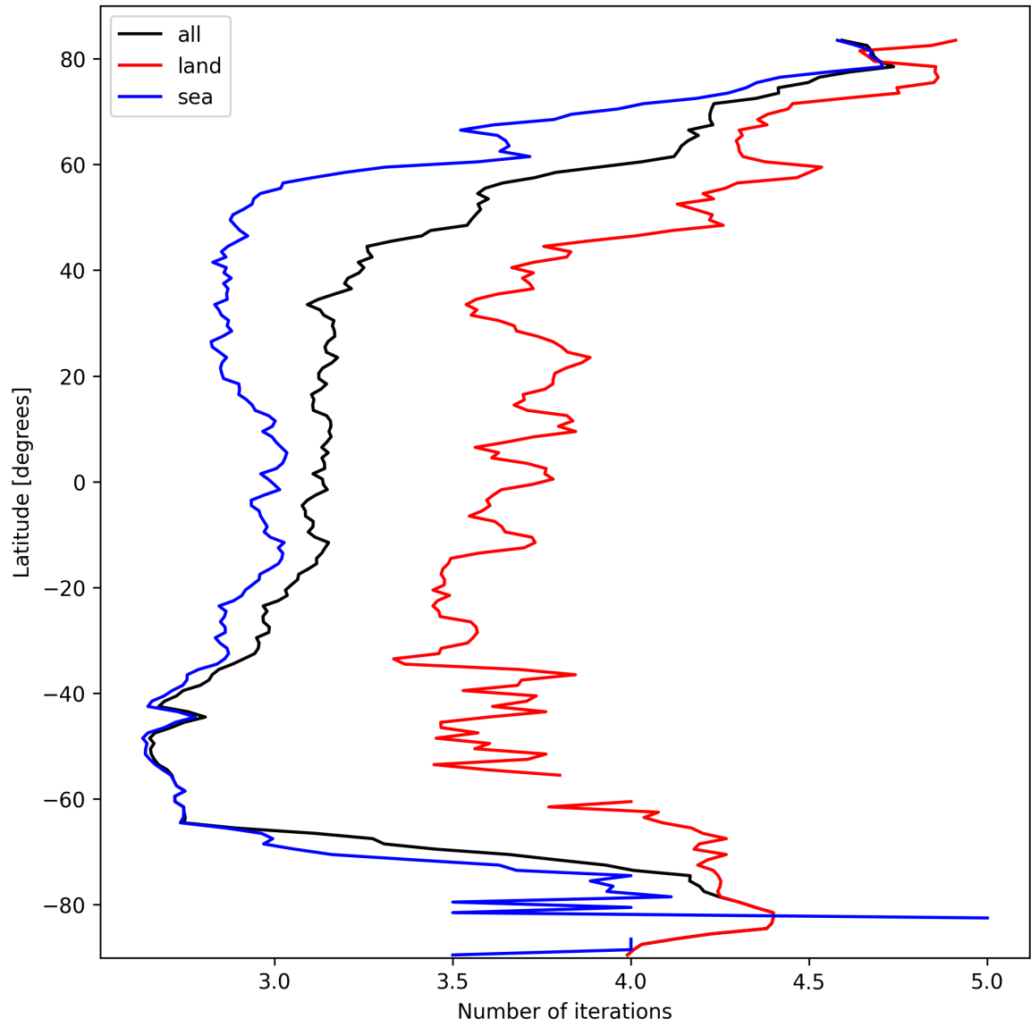
Figure 22: Zonal average of “Number of iterations” for 2025-03-08 to 2025-03-10.
