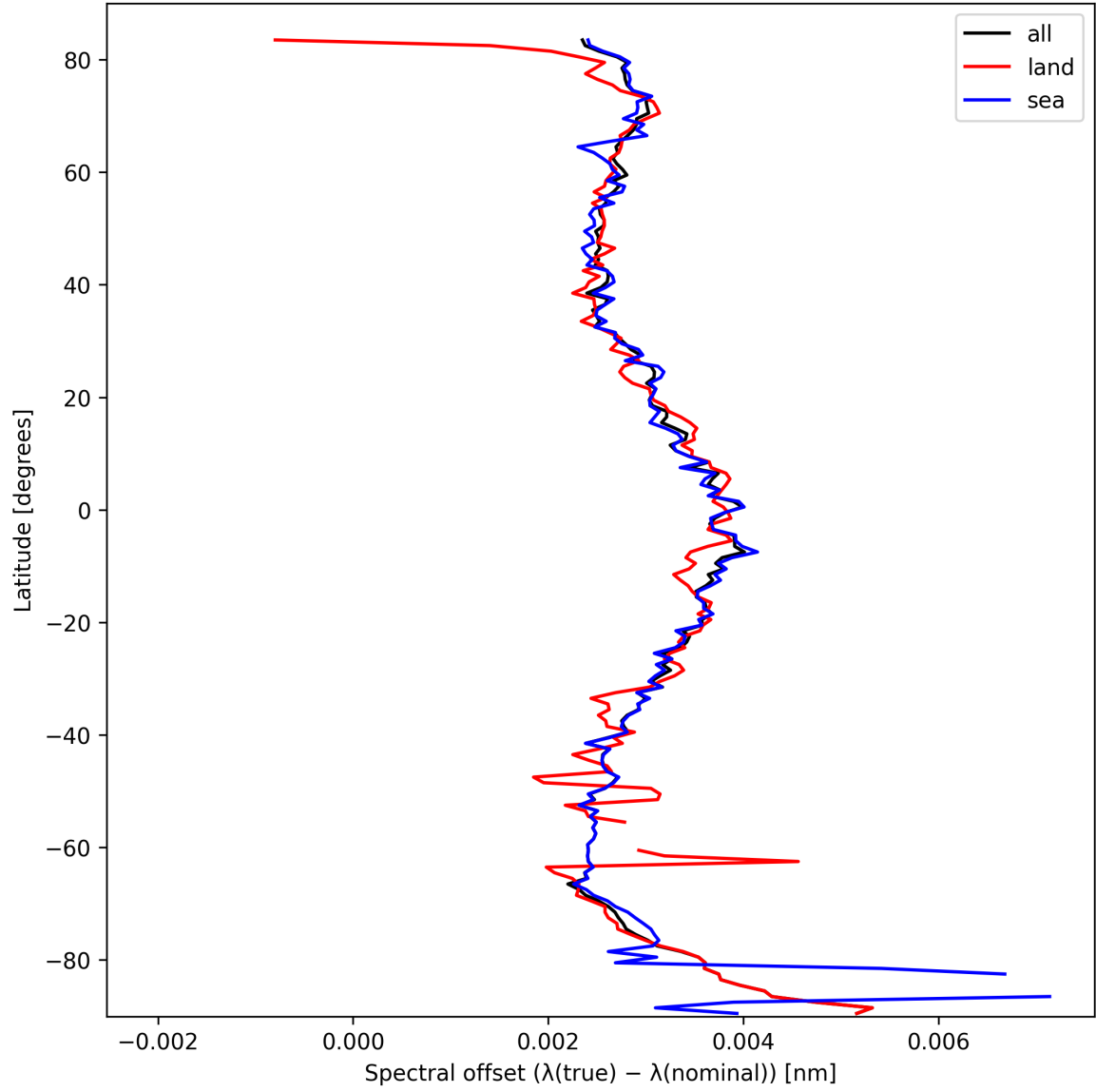
Figure 28: Zonal average of “Spectral offset ( \lambda_{\text{true}} - \lambda_{\text{nominal}} )” for 2025-03-08 to 2025-03-10.
