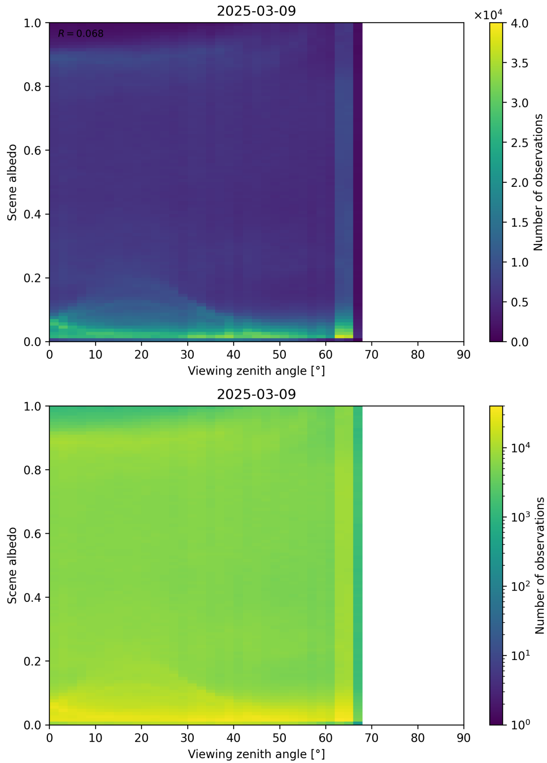
Figure 126: Scatter density plot of “Viewing zenith angle” against “Scene albedo” for 2025-03-08 to 2025-03-10.
