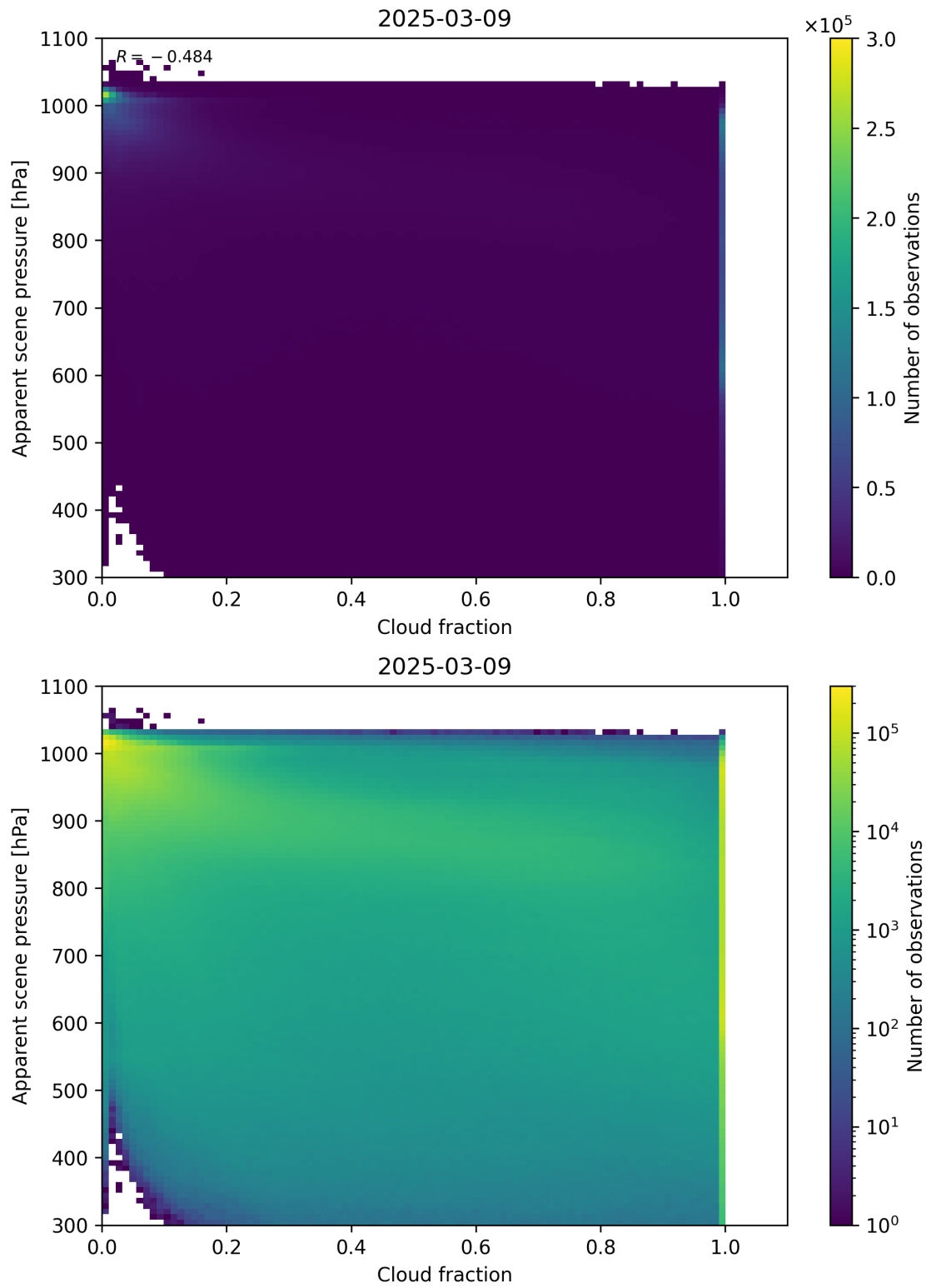
Figure 70: Scatter density plot of “Cloud fraction” against “Apparent scene pressure” for 2025-03-08 to 2025-03-10.
