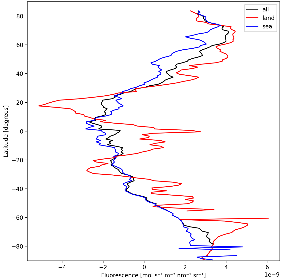
Figure 23: Zonal average of “Fluorescence” for 2025-03-08 to 2025-03-10.
