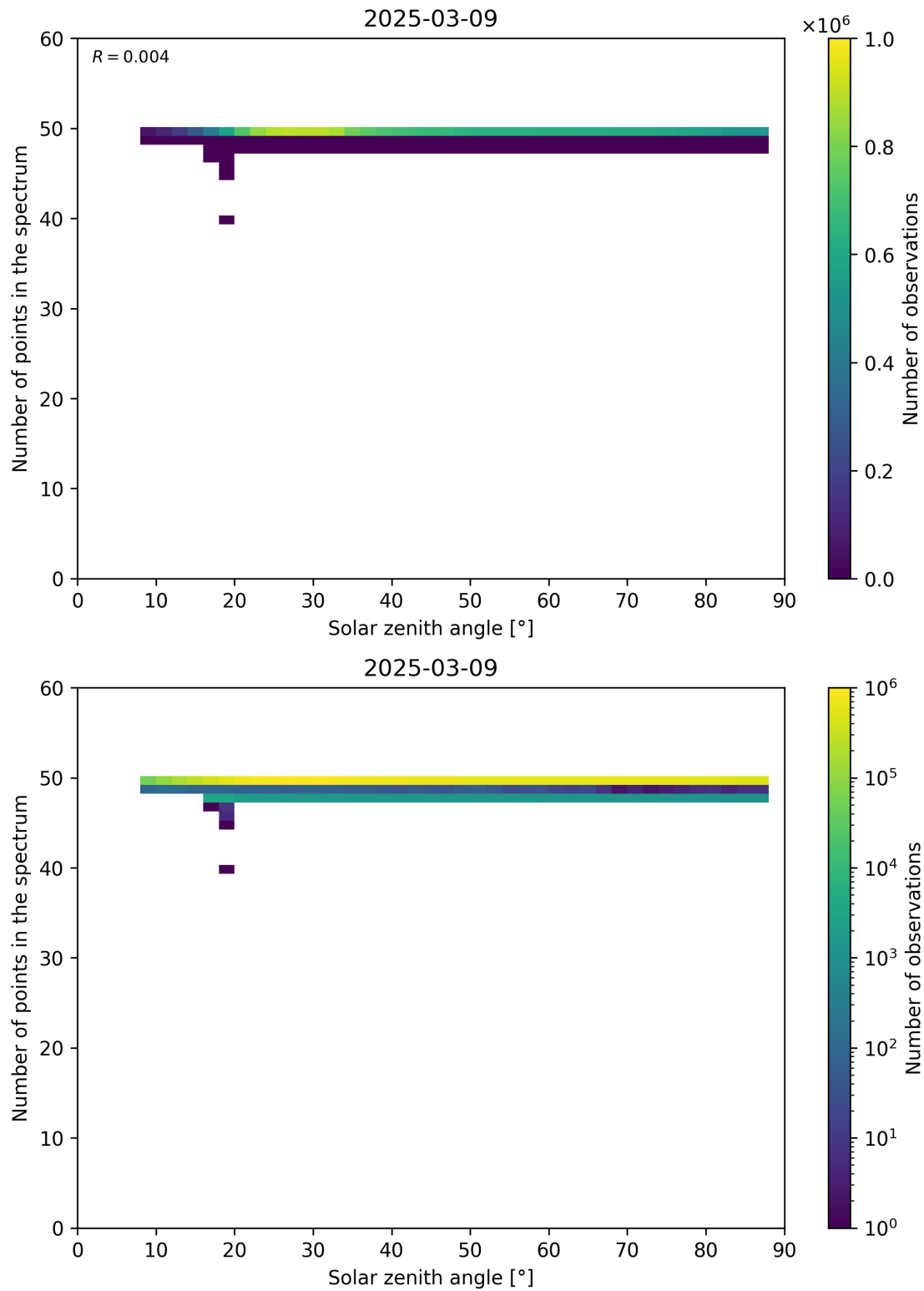
Figure 115: Scatter density plot of “Solar zenith angle” against “Number of points in the spectrum” for 2025-03-08 to 2025-03-10.
