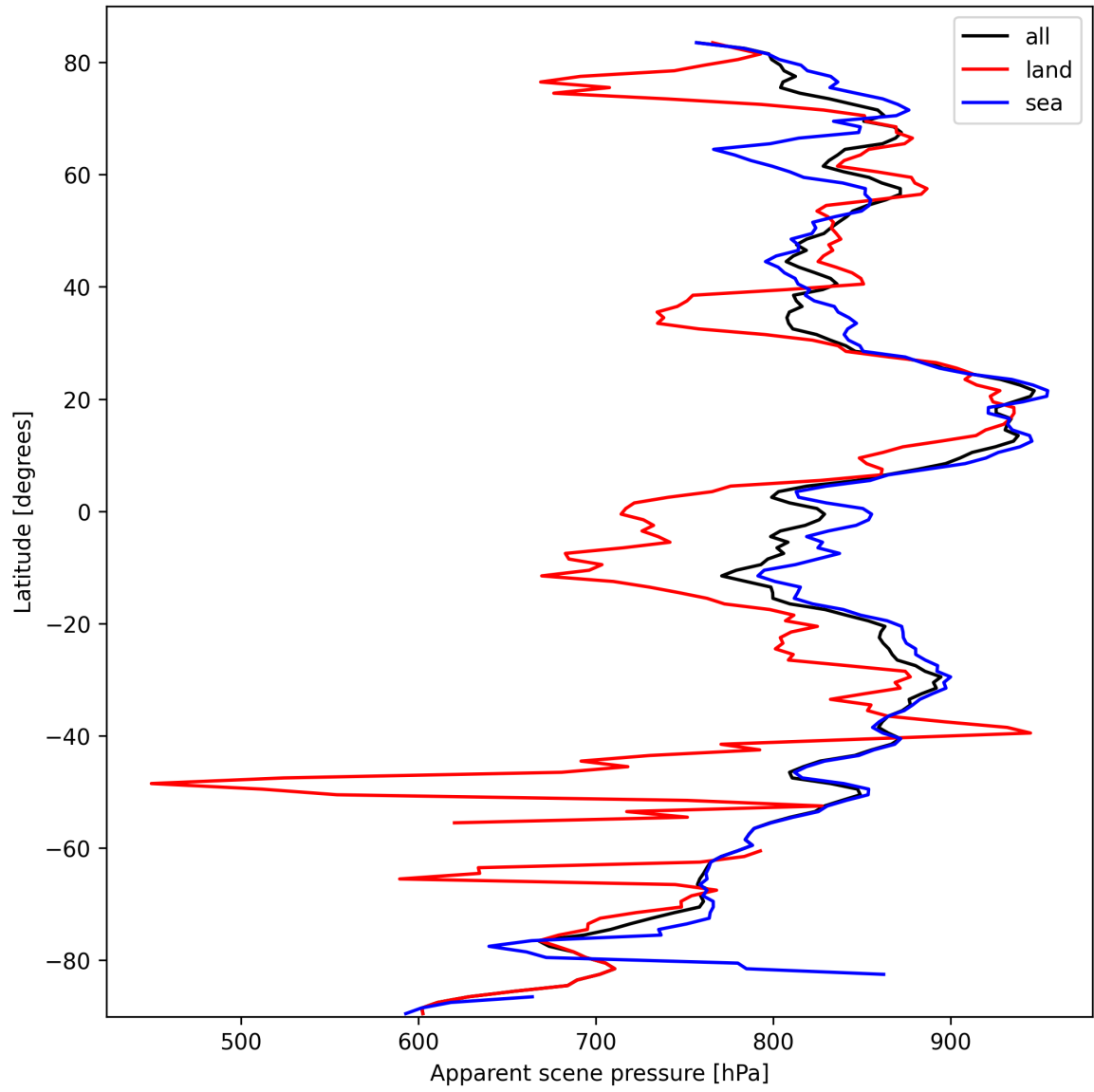
Figure 19: Zonal average of “Apparent scene pressure” for 2025-03-08 to 2025-03-10.
