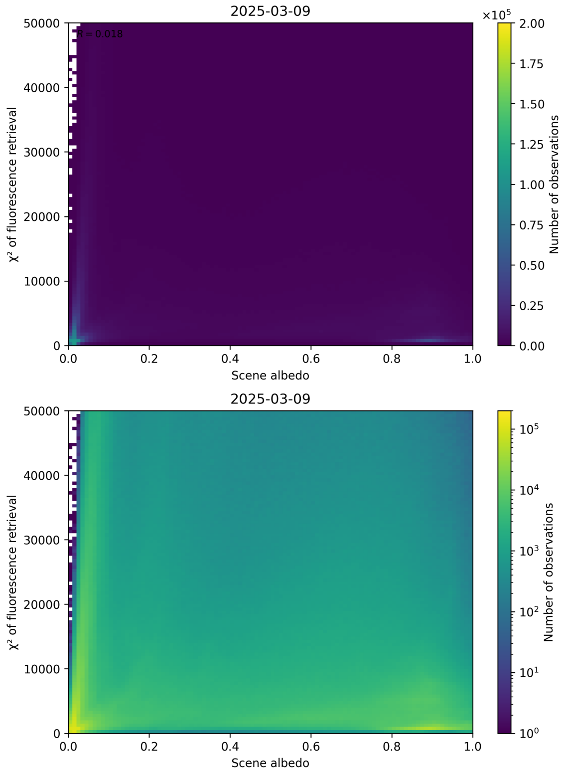
Figure 103: Scatter density plot of “Scene albedo” against “ \chi^2 of fluorescence retrieval” for 2025-03-08 to 2025-03-10.
