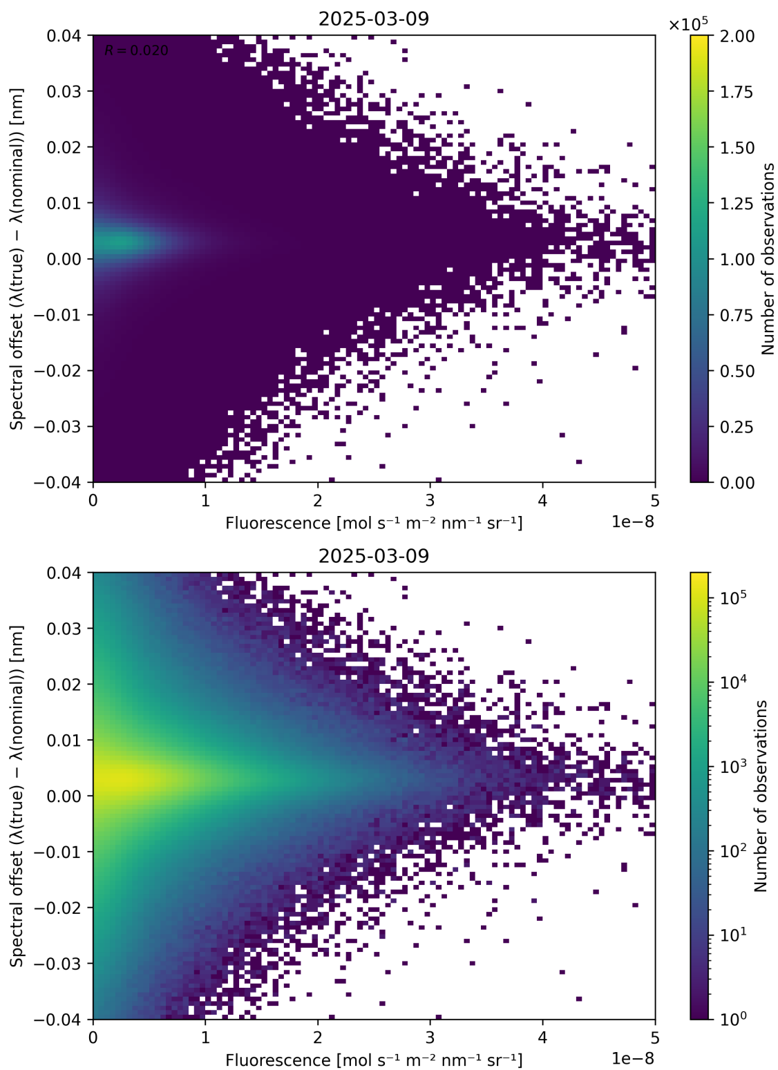
Figure 87: Scatter density plot of “Fluorescence” against “Spectral offset ( \lambda_{\text{true}} - \lambda_{\text{nominal}} )” for 2025-03-08 to 2025-03-10.
