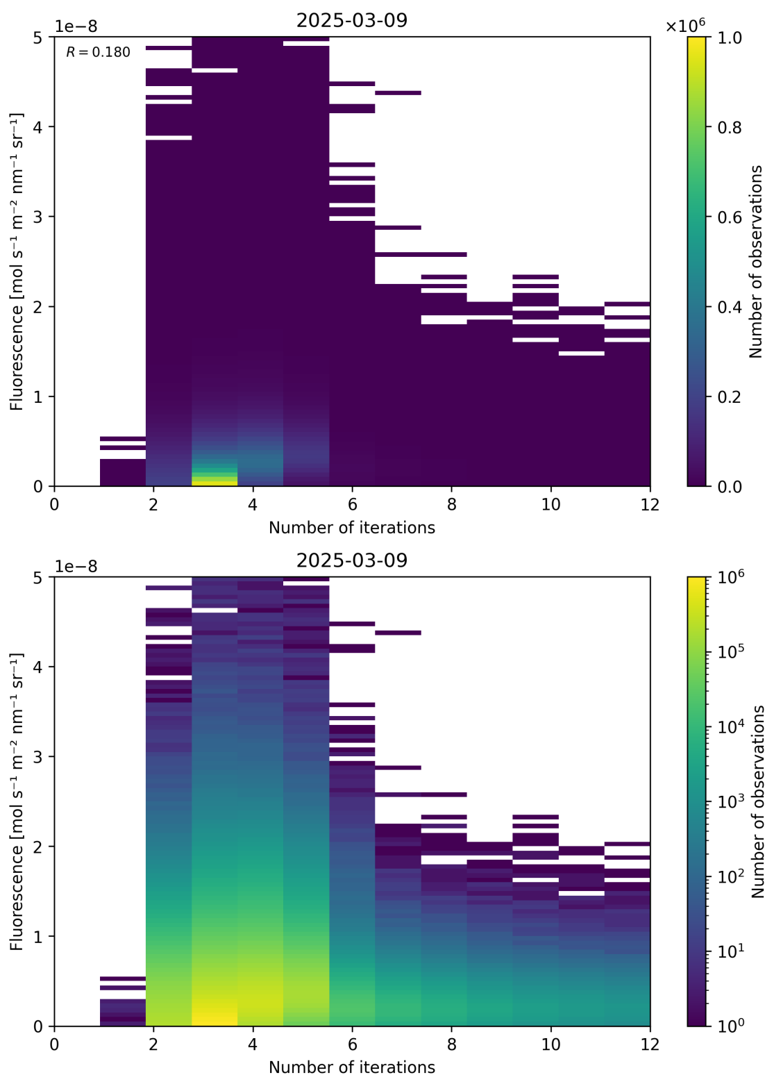
Figure 98: Scatter density plot of “Number of iterations” against “Fluorescence” for 2025-03-08 to 2025-03-10.
