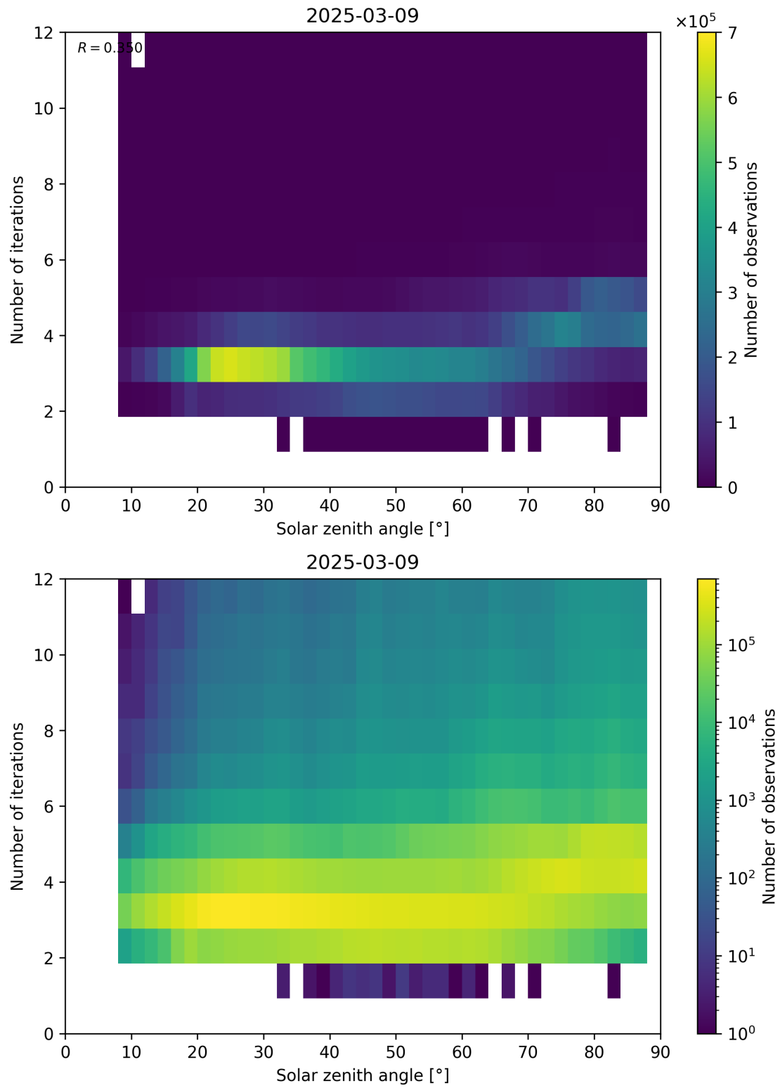
Figure 114: Scatter density plot of “Solar zenith angle” against “Number of iterations” for 2025-03-08 to 2025-03-10.
