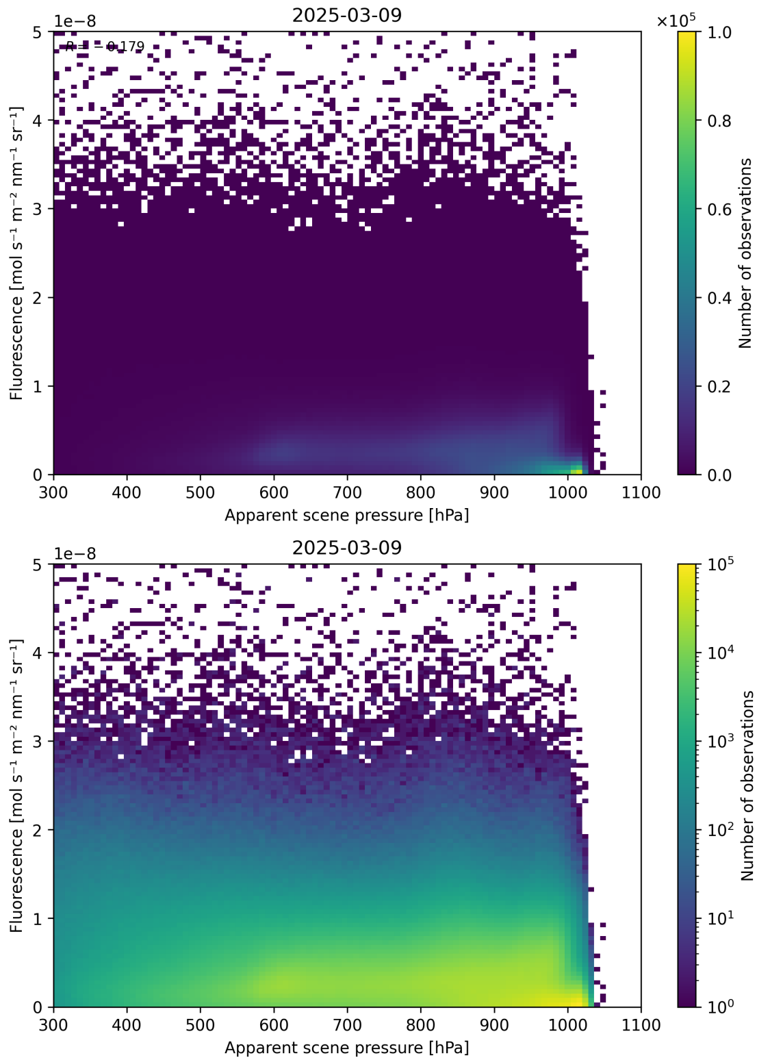
Figure 64: Scatter density plot of “Apparent scene pressure” against “Fluorescence” for 2025-03-08 to 2025-03-10.
