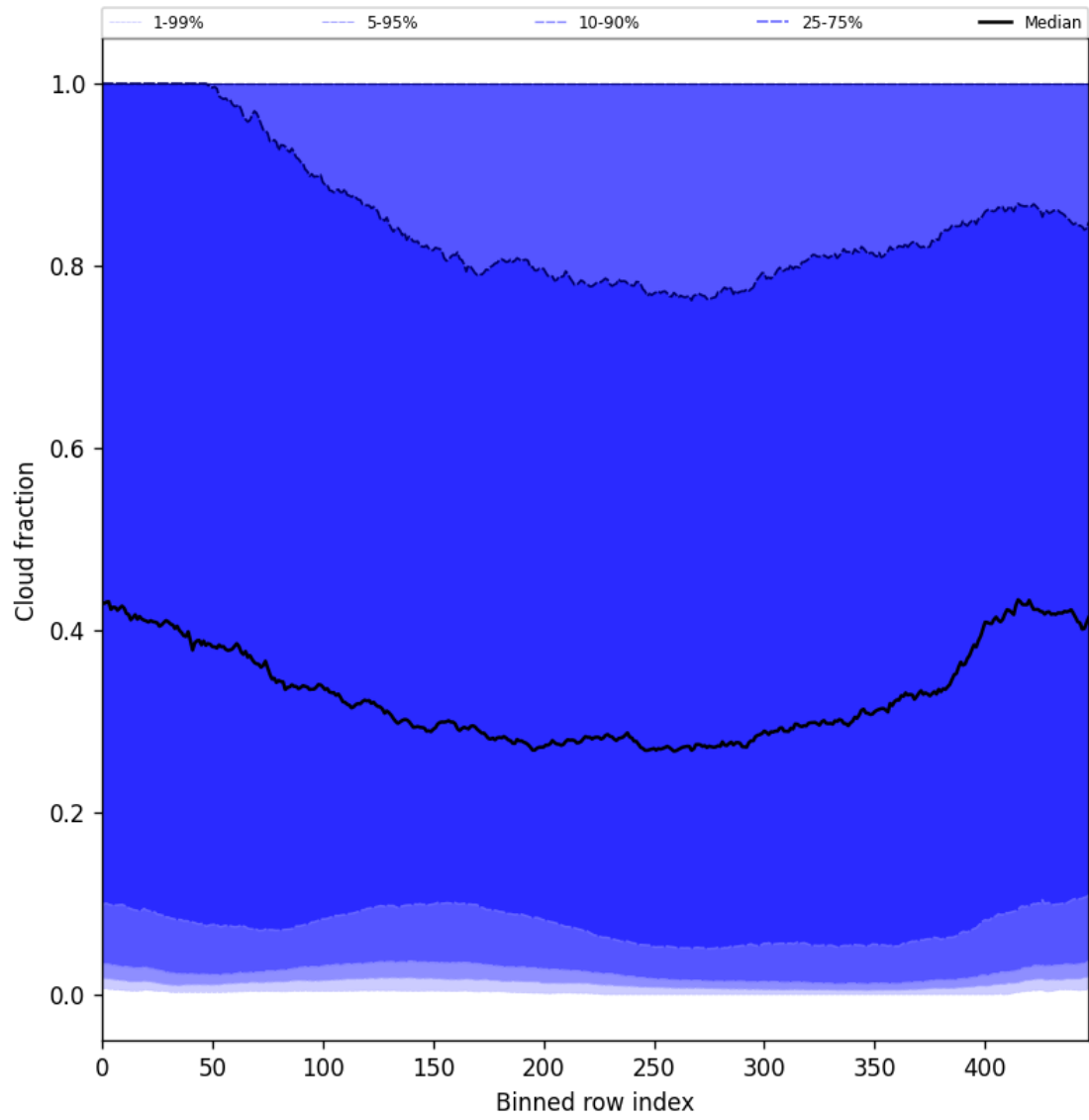
Figure 49: Along track statistics of “Cloud fraction” for 2025-03-08 to 2025-03-10
