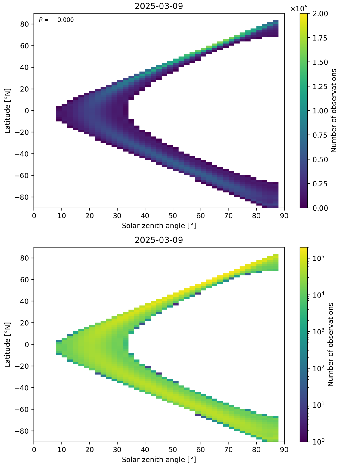
Figure 113: Scatter density plot of “Solar zenith angle” against “Latitude” for 2025-03-08 to 2025-03-10.
