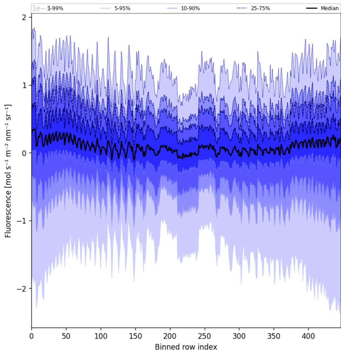
Figure 57: Along track statistics of “Fluorescence” for 2025-03-08 to 2025-03-10
