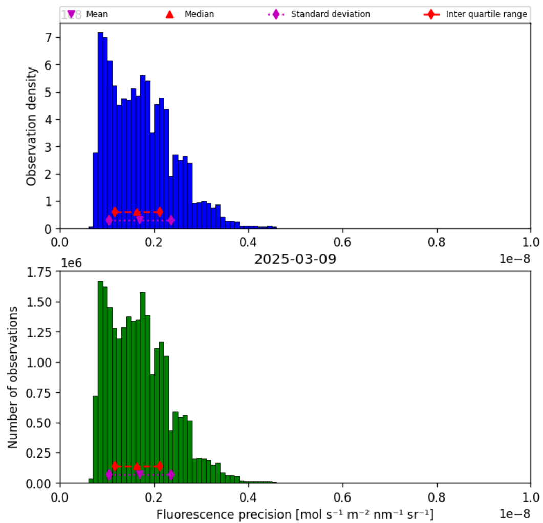
Figure 41: Histogram of “Fluorescence precision” for 2025-03-08 to 2025-03-10
