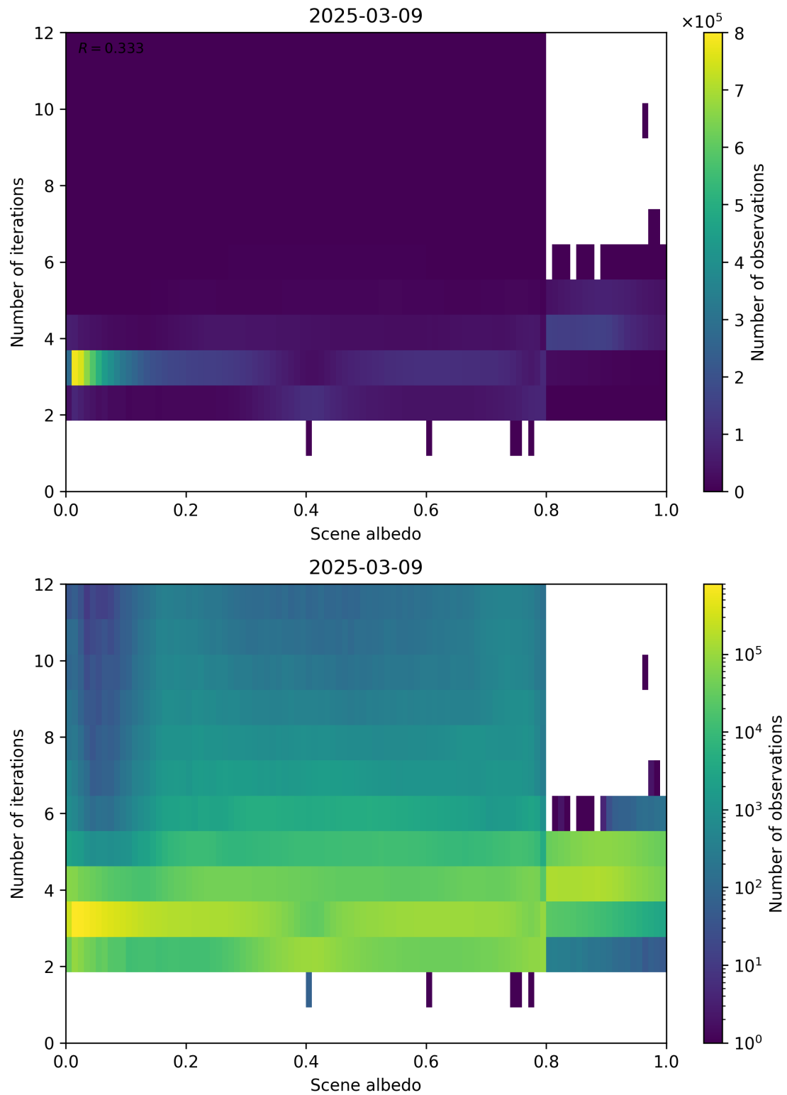
Figure 105: Scatter density plot of “Scene albedo” against “Number of iterations” for 2025-03-08 to 2025-03-10.
