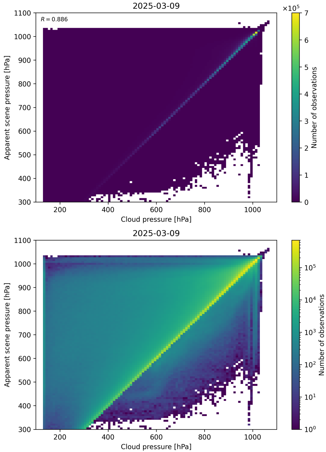
Figure 77: Scatter density plot of “Cloud pressure” against “Apparent scene pressure” for 2025-03-08 to 2025-03-10.
