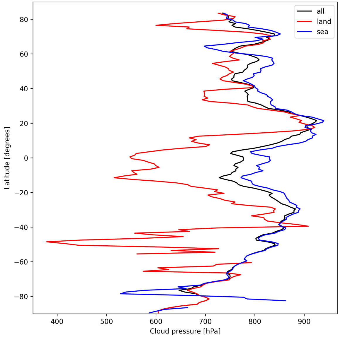
Figure 13: Zonal average of “Cloud pressure” for 2025-03-08 to 2025-03-10.
