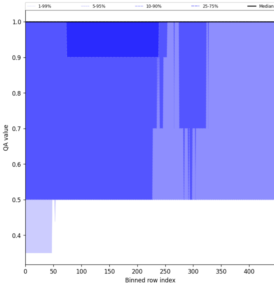
Figure 46: Along track statistics of “QA value” for 2025-03-08 to 2025-03-10
