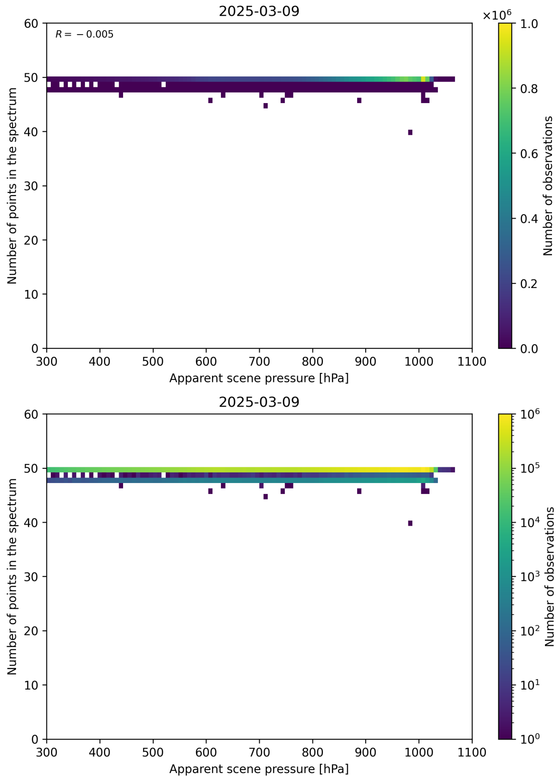
Figure 66: Scatter density plot of “Apparent scene pressure” against “Number of points in the spectrum” for 2025-03-08 to 2025-03-10.
