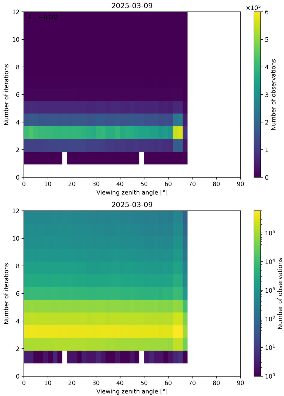
Figure 124: Scatter density plot of “Viewing zenith angle” against “Number of iterations” for 2025-03-08 to 2025-03-10.
