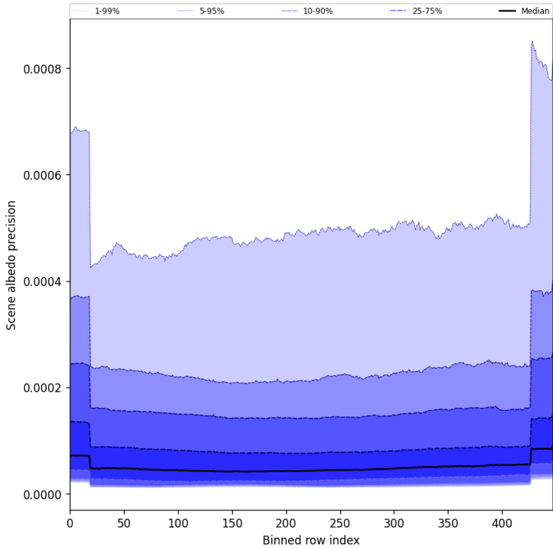
Figure 52: Along track statistics of “Scene albedo precision” for 2025-03-08 to 2025-03-10
