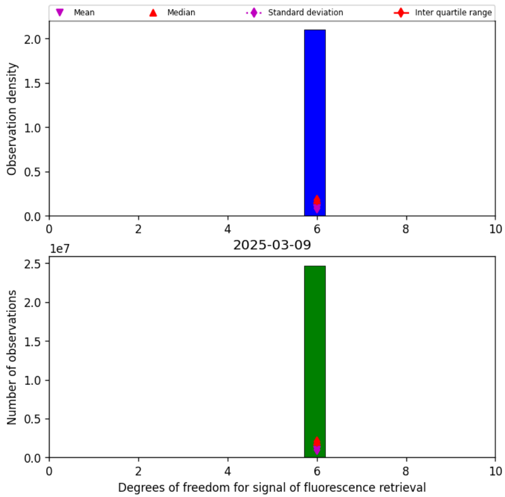
Figure 43: Histogram of "Degrees of freedom for signal of fluorescence retrieval" for 2025-03-08 to 2025-03-10
