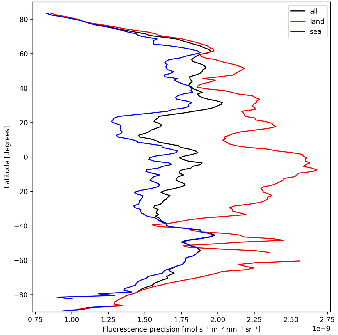
Figure 24: Zonal average of “Fluorescence precision” for 2025-03-08 to 2025-03-10.
