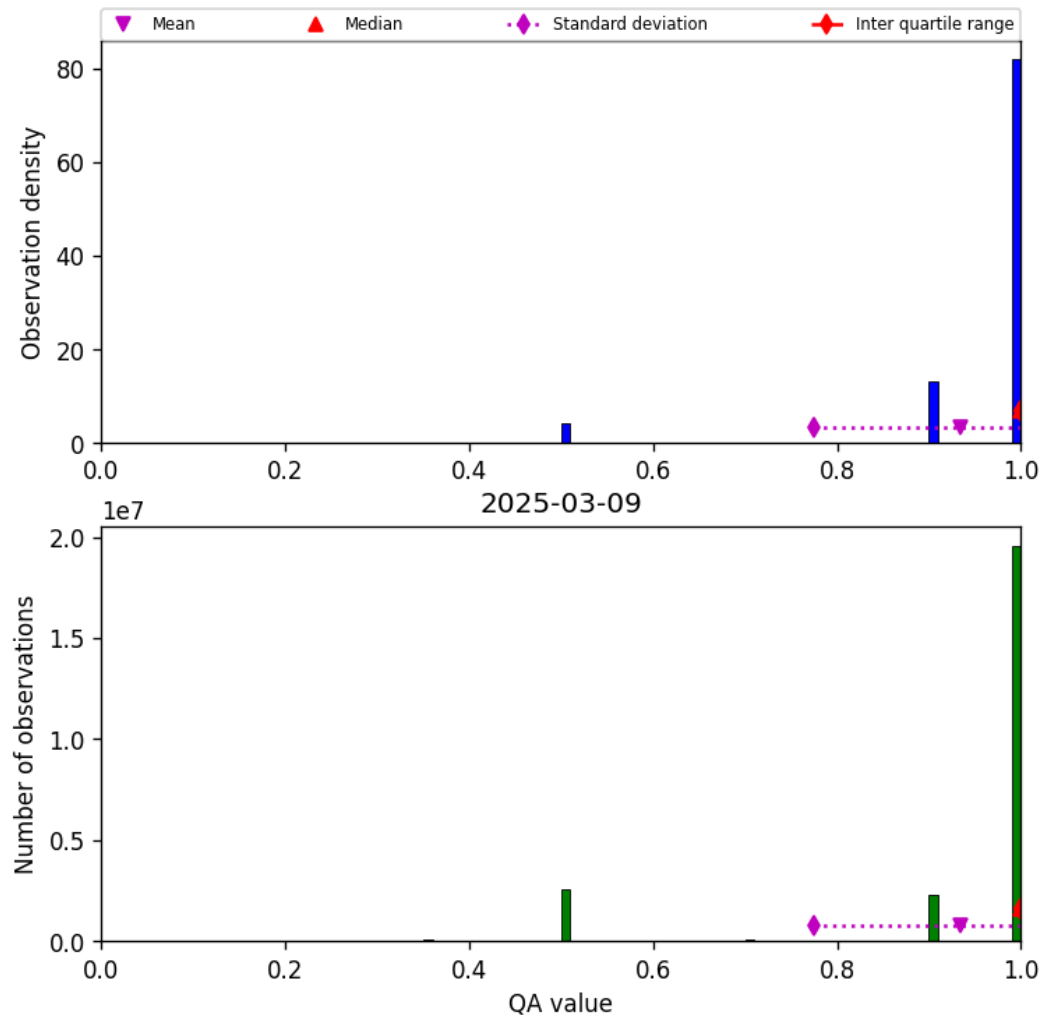
Figure 29: Histogram of “QA value” for 2025-03-08 to 2025-03-10
