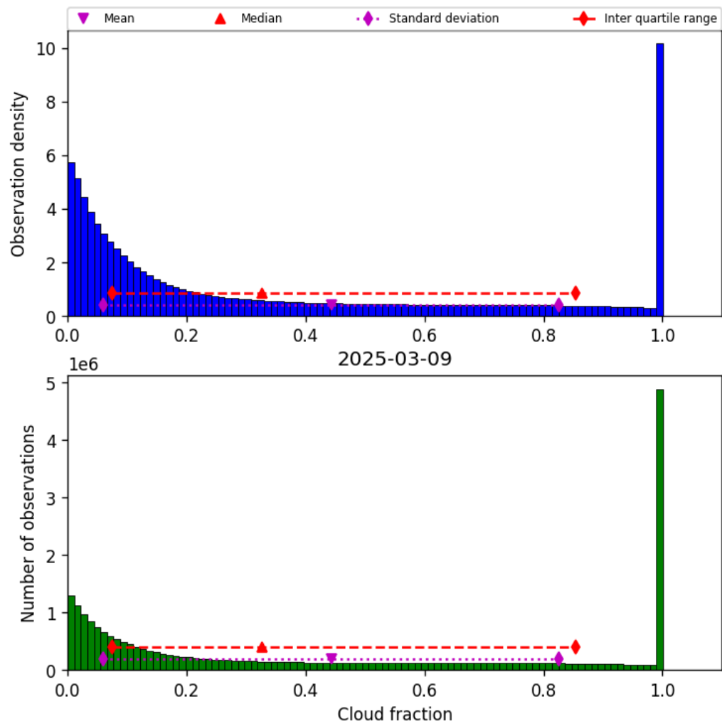
Figure 32: Histogram of “Cloud fraction” for 2025-03-08 to 2025-03-10
