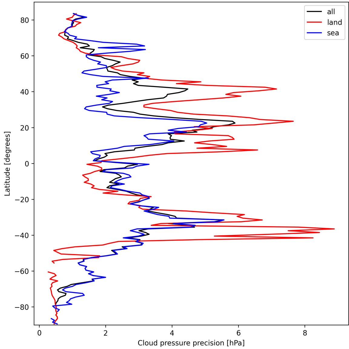
Figure 14: Zonal average of “Cloud pressure precision” for 2025-03-08 to 2025-03-10.
