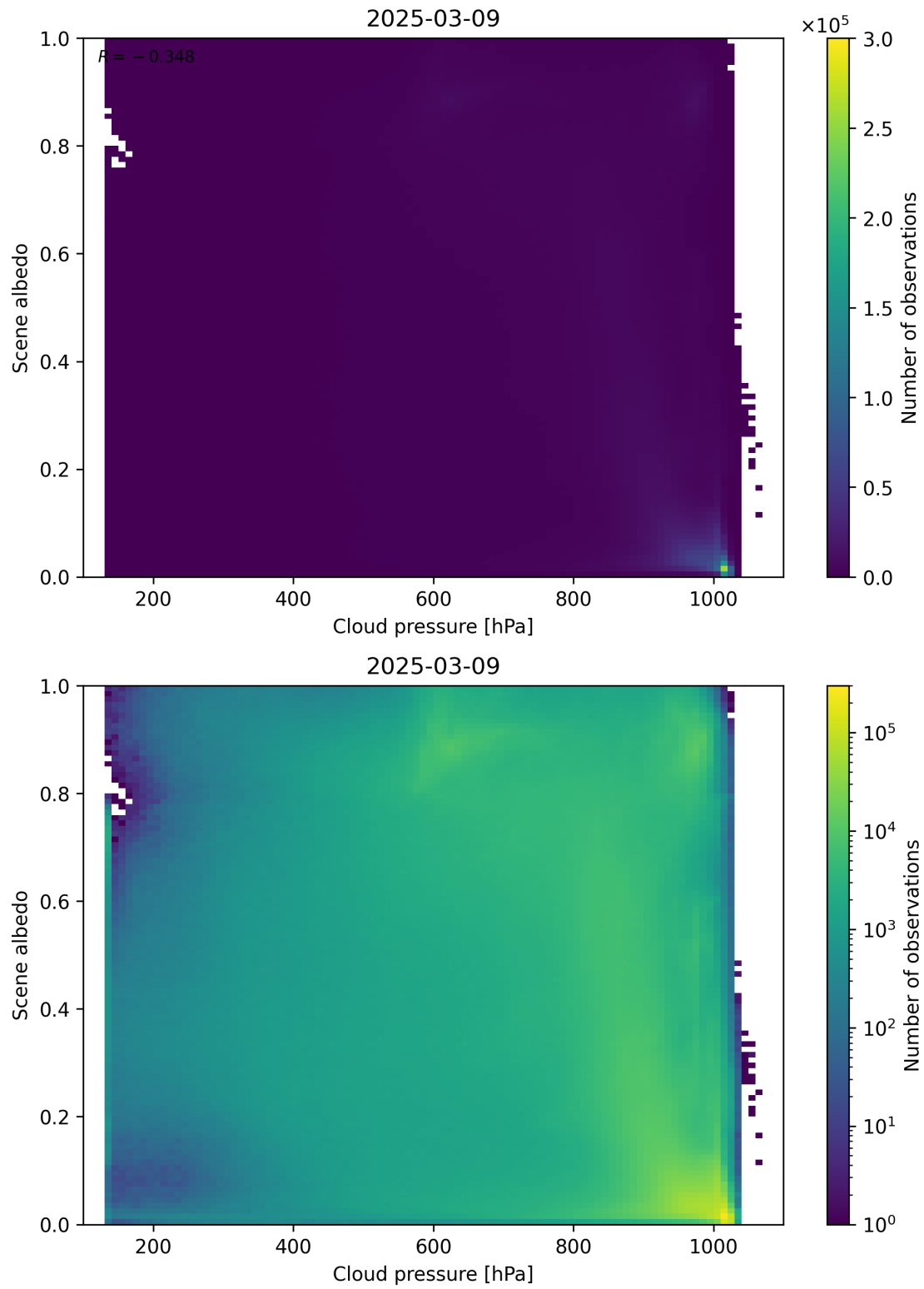
Figure 83: Scatter density plot of “Cloud pressure” against “Scene albedo” for 2025-03-08 to 2025-03-10.
