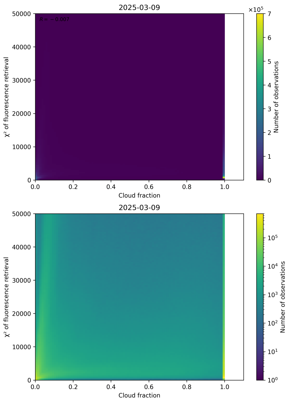
Figure 71: Scatter density plot of “Cloud fraction” against “ \chi^2 of fluorescence retrieval” for 2025-03-08 to 2025-03-10.
