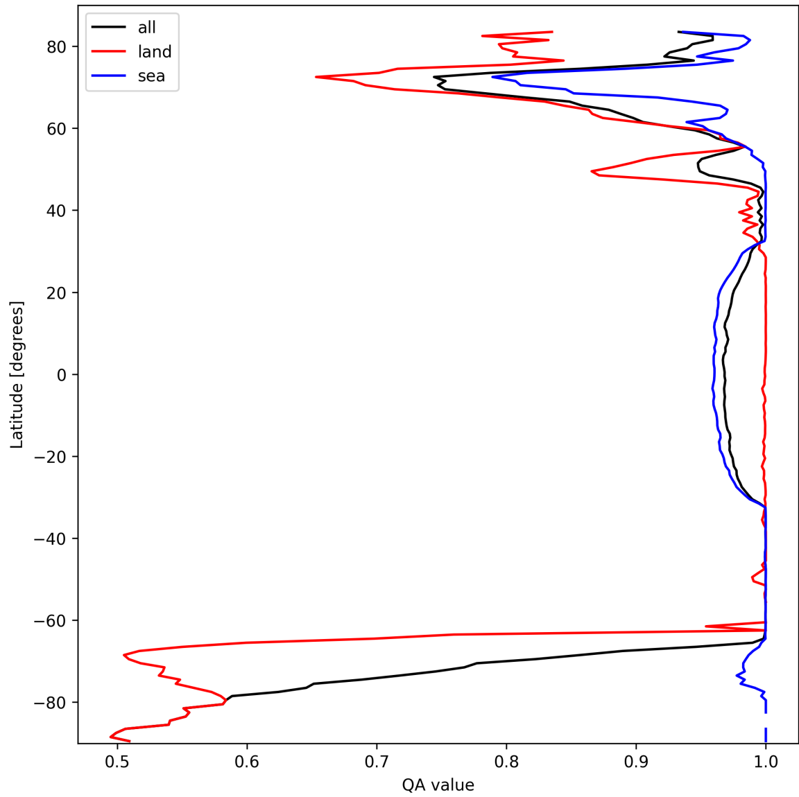
Figure 12: Zonal average of "QA value" for 2025-03-08 to 2025-03-10.
