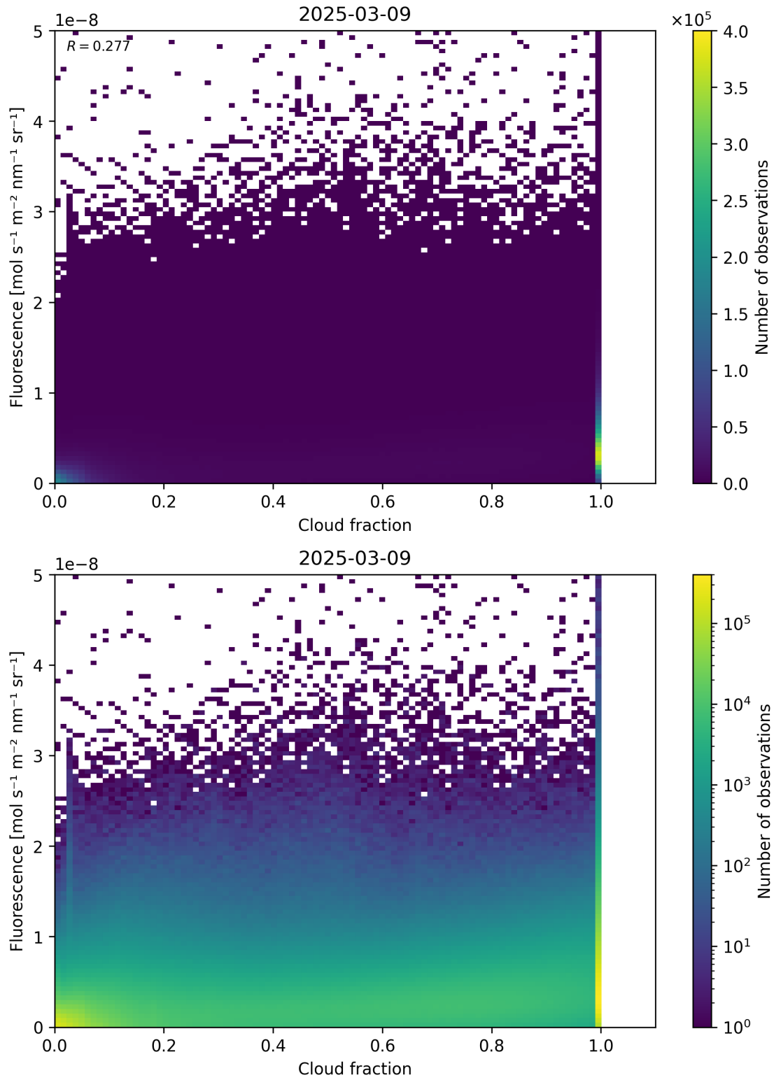
Figure 72: Scatter density plot of “Cloud fraction” against “Fluorescence” for 2025-03-08 to 2025-03-10.
