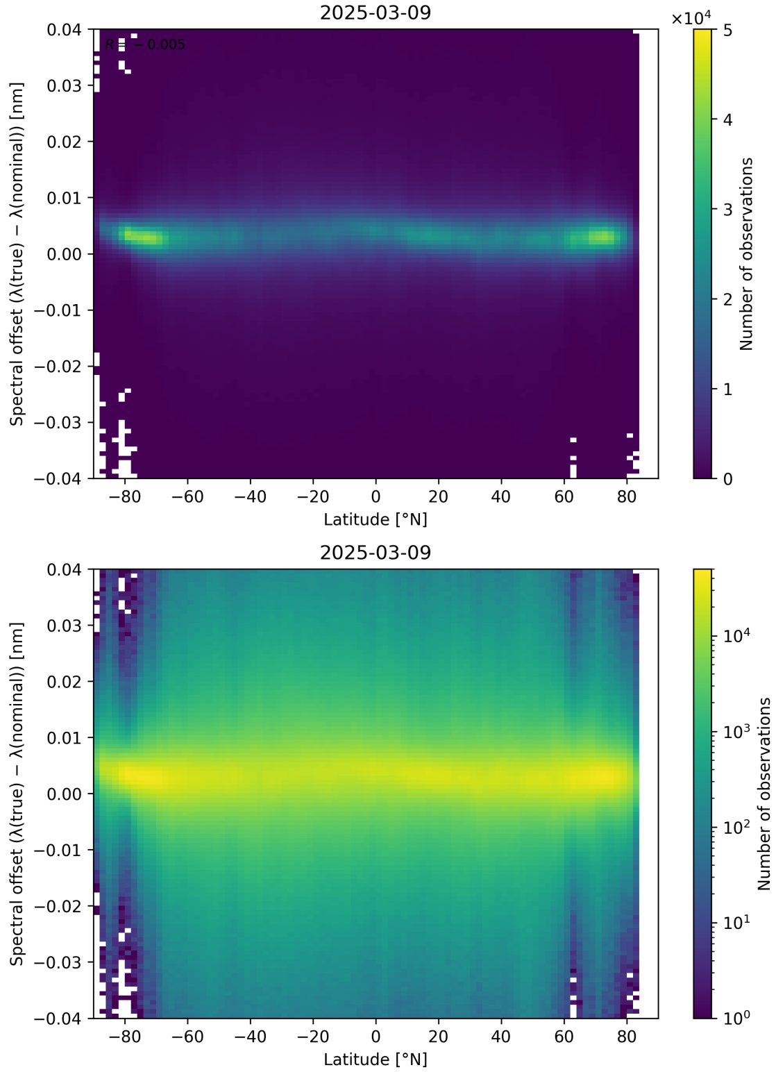
Figure 96: Scatter density plot of “Latitude” against “Spectral offset ( \lambda_{\text{true}} - \lambda_{\text{nominal}} )” for 2025-03-08 to 2025-03-10.
