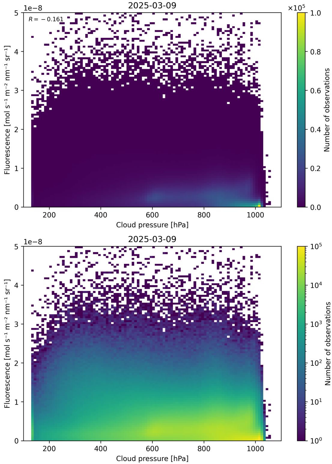
Figure 80: Scatter density plot of “Cloud pressure” against “Fluorescence” for 2025-03-08 to 2025-03-10.
