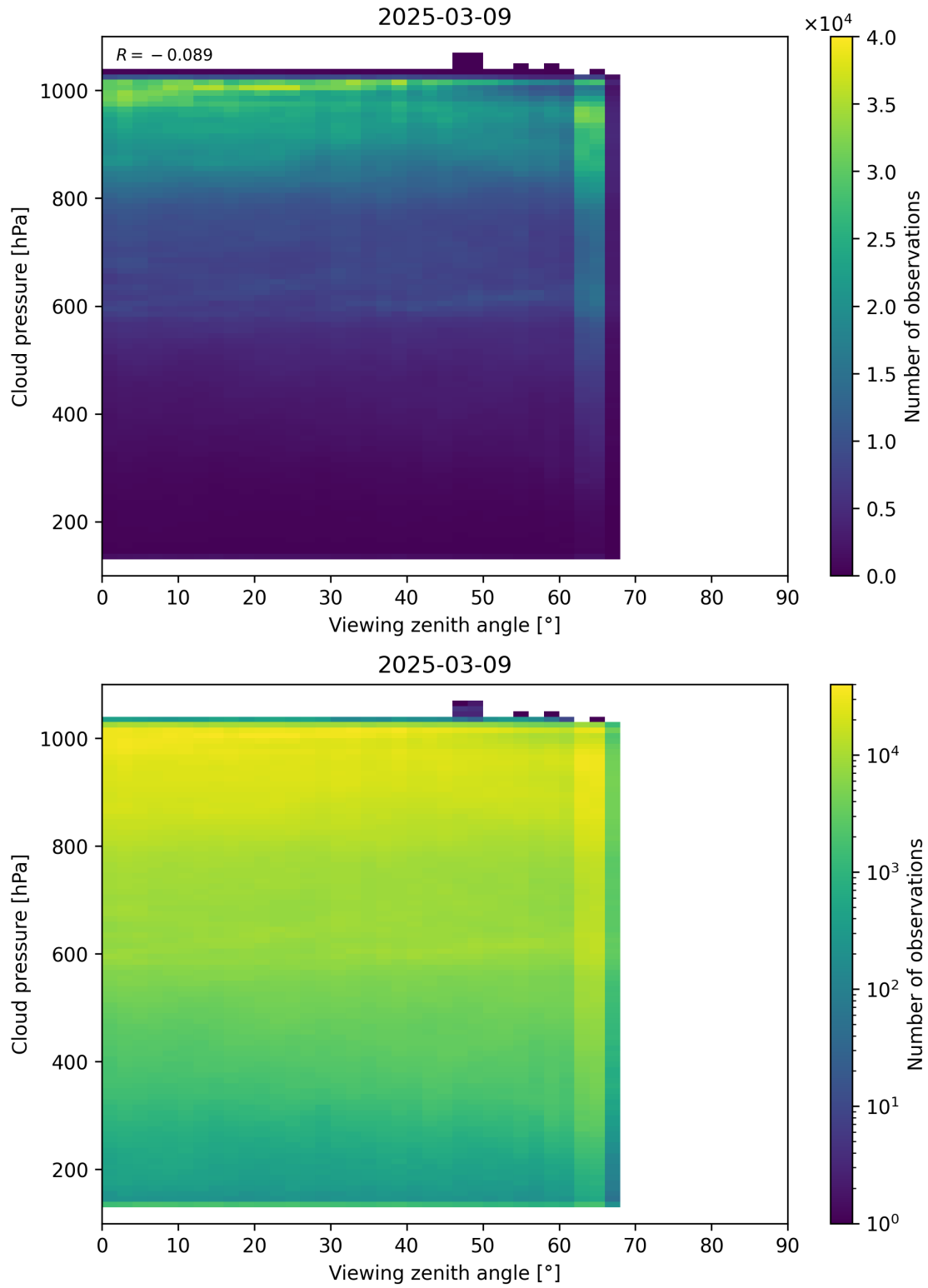
Figure 121: Scatter density plot of “Viewing zenith angle” against “Cloud pressure” for 2025-03-08 to 2025-03-10.
