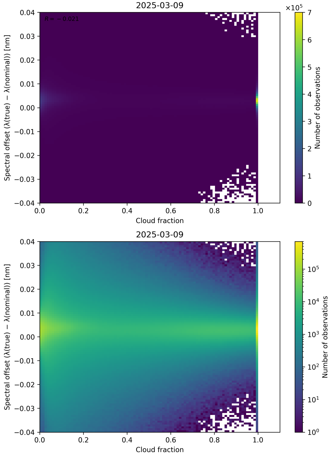
Figure 76: Scatter density plot of “Cloud fraction” against “Spectral offset ( \lambda_{\text{true}} - \lambda_{\text{nominal}} )” for 2025-03-08 to 2025-03-10.
