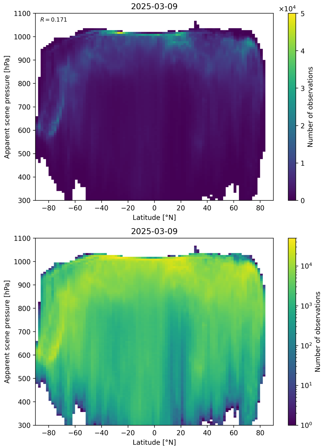
Figure 88: Scatter density plot of “Latitude” against “Apparent scene pressure” for 2025-03-08 to 2025-03-10.
