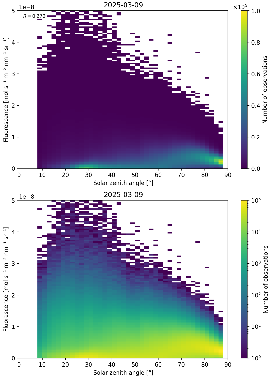
Figure 112: Scatter density plot of “Solar zenith angle” against “Fluorescence” for 2025-03-08 to 2025-03-10.
