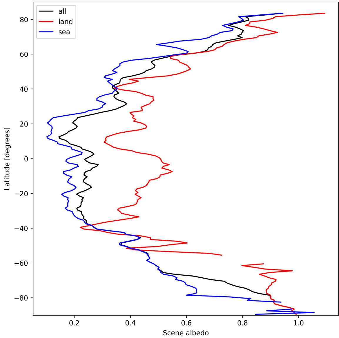
Figure 17: Zonal average of “Scene albedo” for 2025-03-08 to 2025-03-10.
