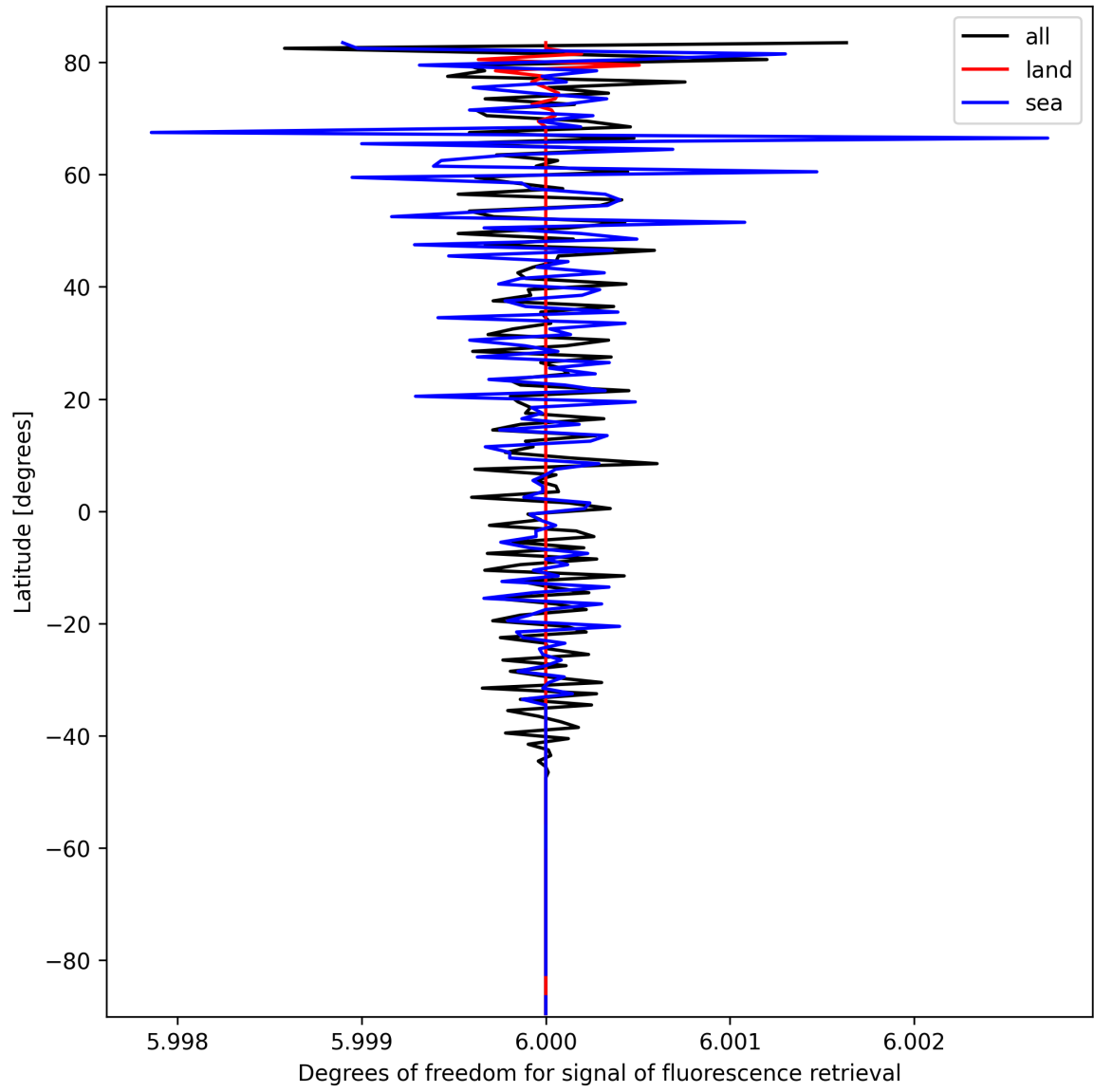
Figure 26: Zonal average of “Degrees of freedom for signal of fluorescence retrieval” for 2025-03-08 to 2025-03-10.
