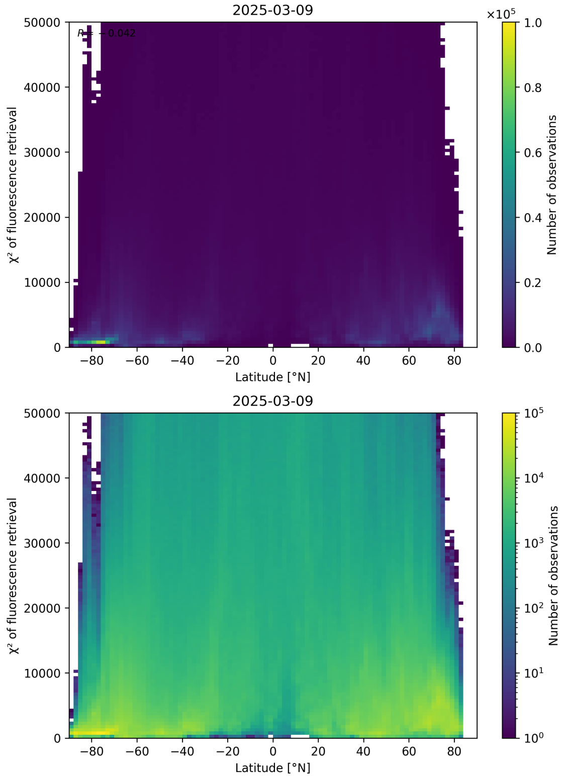
Figure 89: Scatter density plot of “Latitude” against “ \chi^2 of fluorescence retrieval” for 2025-03-08 to 2025-03-10.
