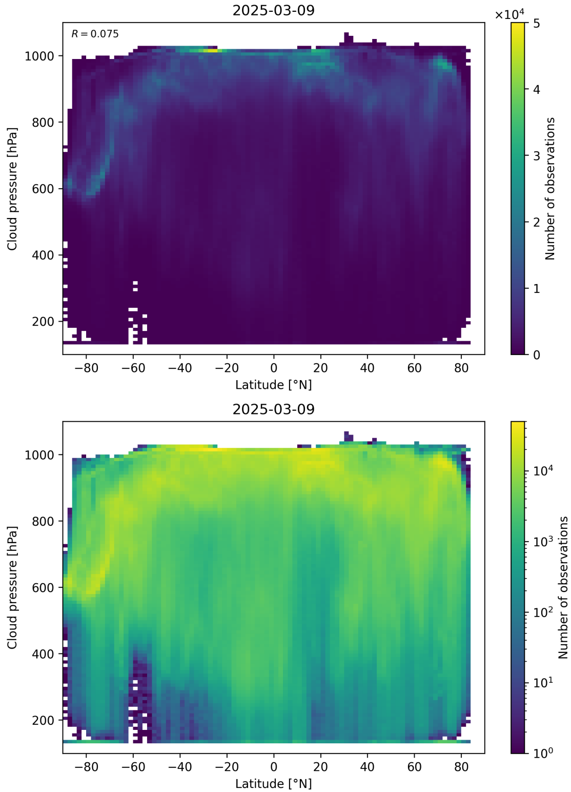
Figure 91: Scatter density plot of “Latitude” against “Cloud pressure” for 2025-03-08 to 2025-03-10.
