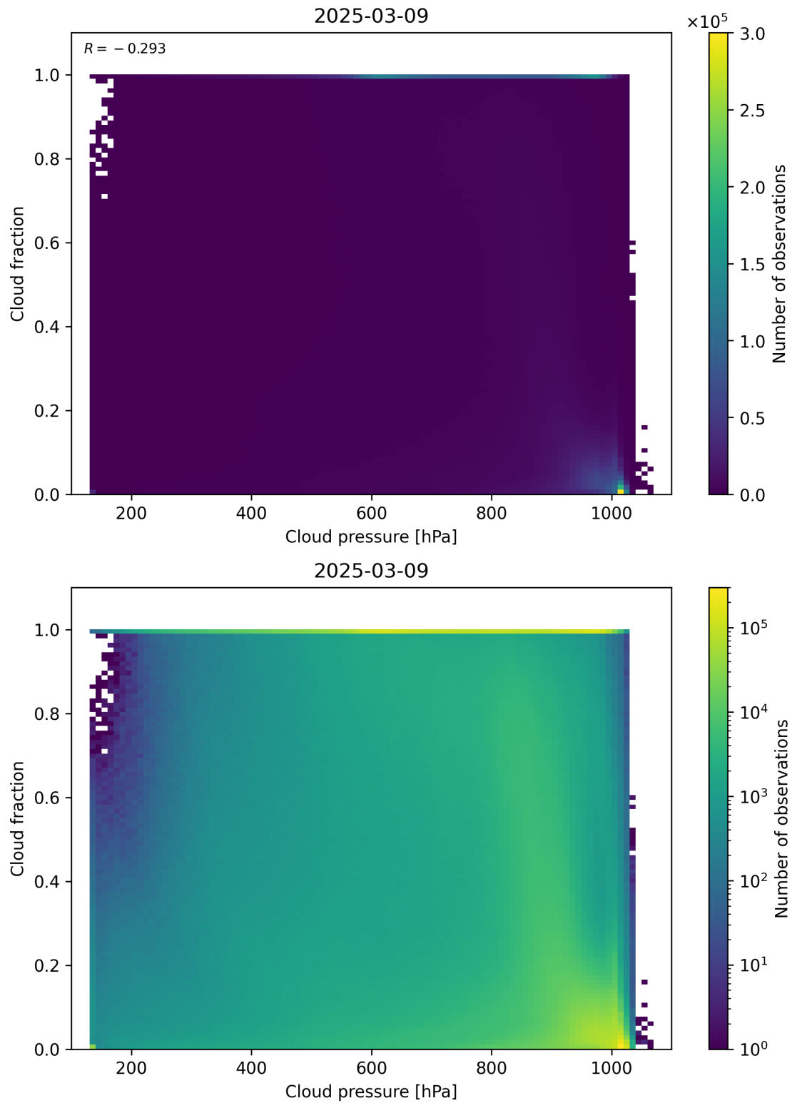
Figure 79: Scatter density plot of “Cloud pressure” against “Cloud fraction” for 2025-03-08 to 2025-03-10.
