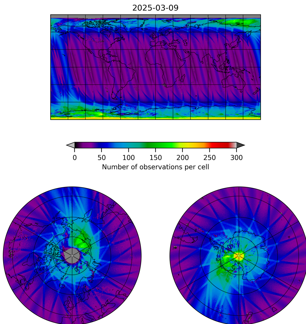
Figure 11: Map of the number of observations for 2025-03-08 to 2025-03-10
