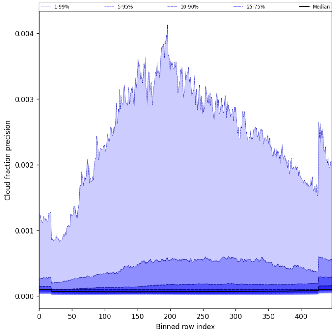
Figure 50: Along track statistics of “Cloud fraction precision” for 2025-03-08 to 2025-03-10
