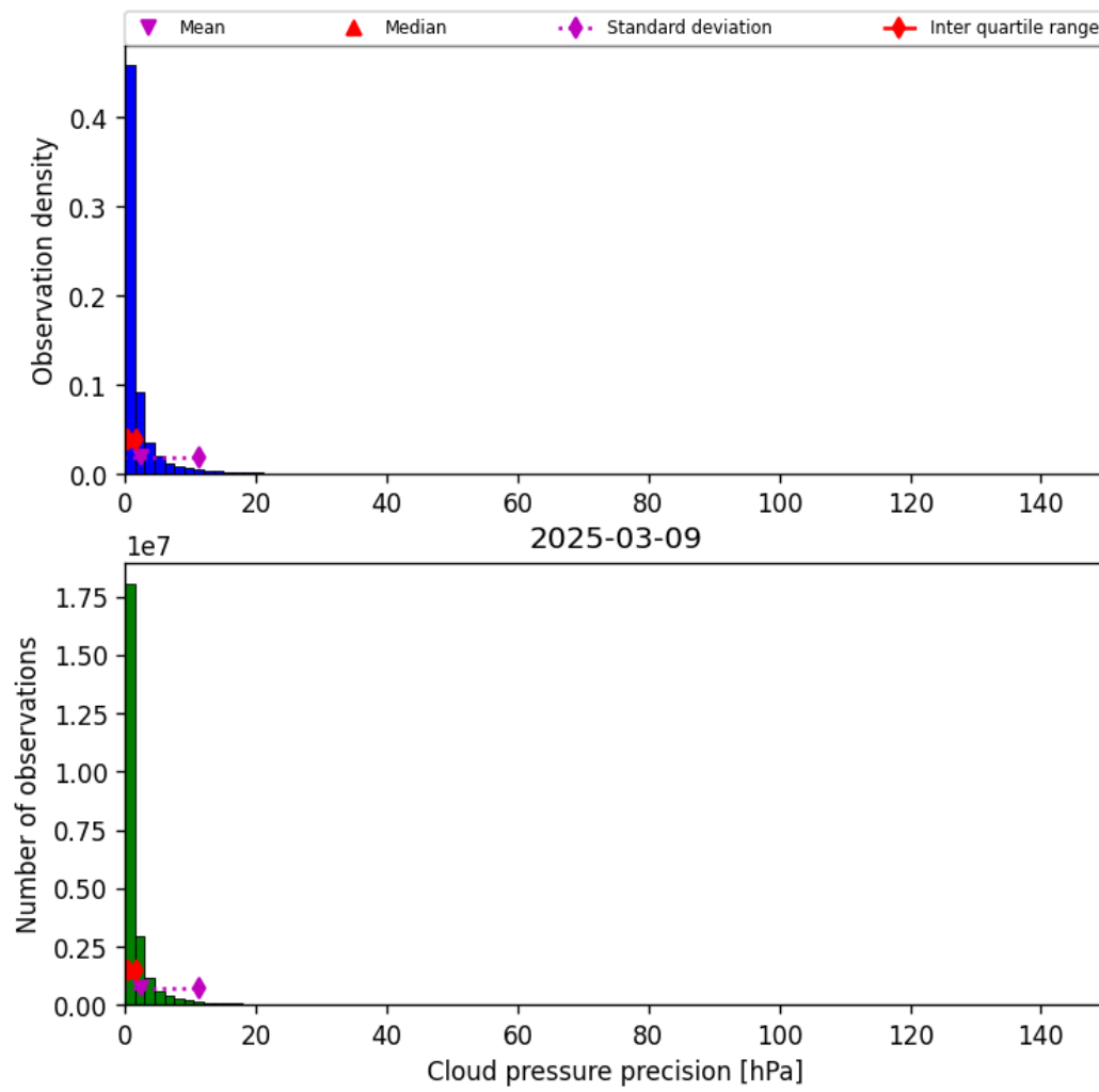
Figure 31: Histogram of “Cloud pressure precision” for 2025-03-08 to 2025-03-10
