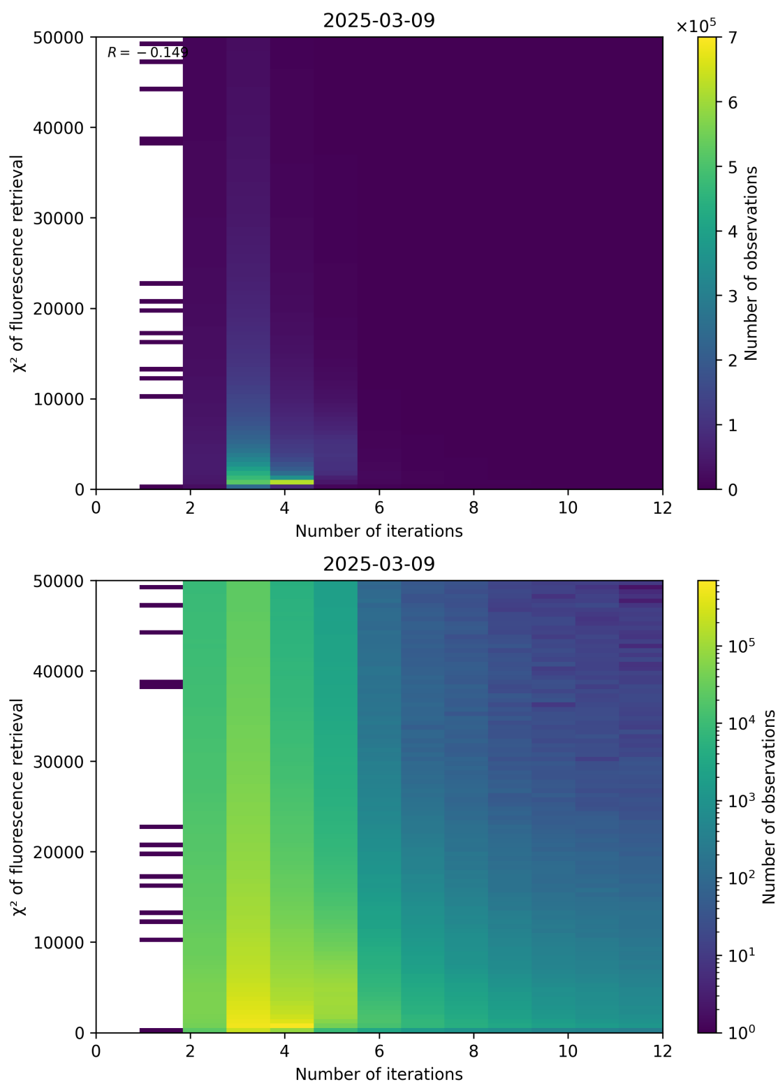
Figure 97: Scatter density plot of “Number of iterations” against “ \chi^2 of fluorescence retrieval” for 2025-03-08 to 2025-03-10.
