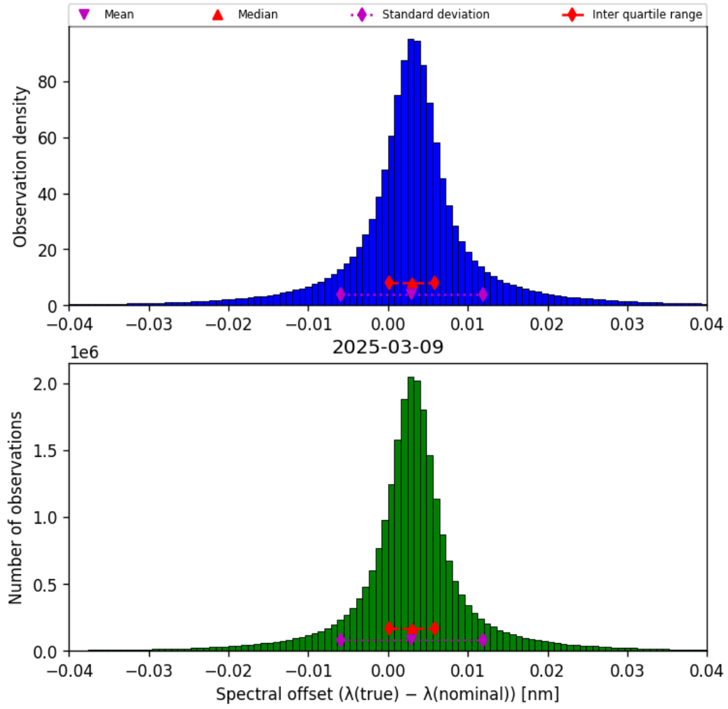
Figure 45: Histogram of “Spectral offset ( \lambda_{\text{true}} - \lambda_{\text{nominal}} )” for 2025-03-08 to 2025-03-10
