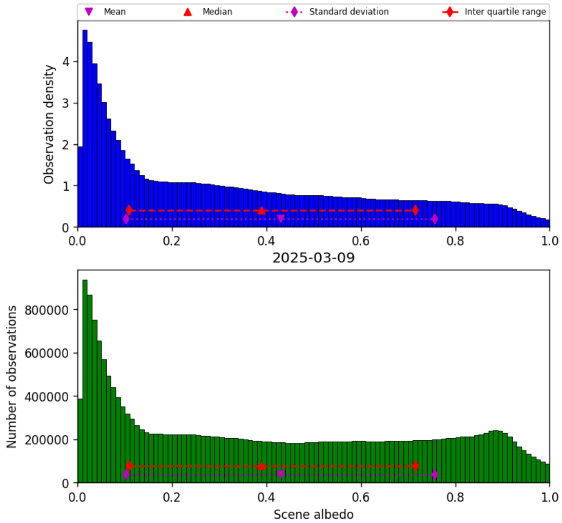
Figure 34: Histogram of “Scene albedo” for 2025-03-08 to 2025-03-10
