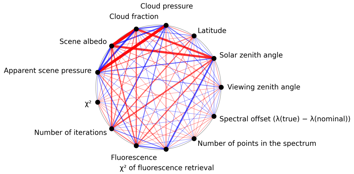
Figure 1: Map of correlation graph for 2025-03-08 to 2025-03-10.
