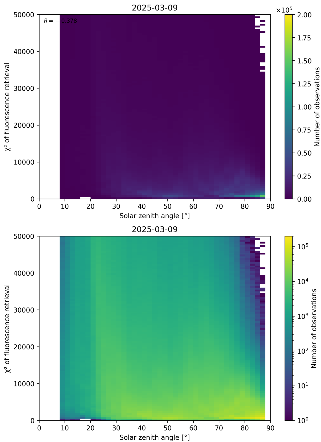
Figure 109: Scatter density plot of “Solar zenith angle” against “ \chi^2 of fluorescence retrieval” for 2025-03-08 to 2025-03-10.
