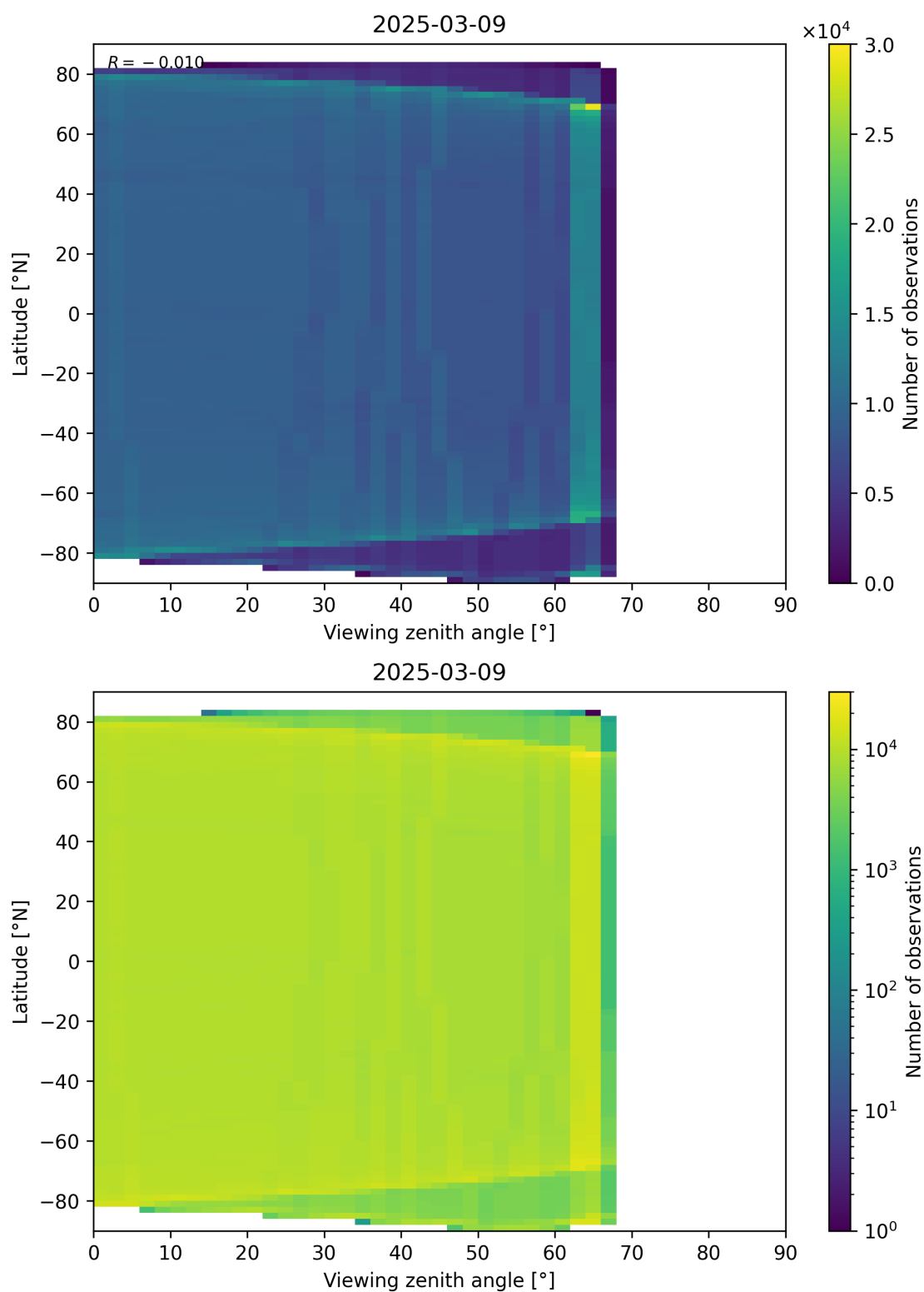
Figure 123: Scatter density plot of “Viewing zenith angle” against “Latitude” for 2025-03-08 to 2025-03-10.
