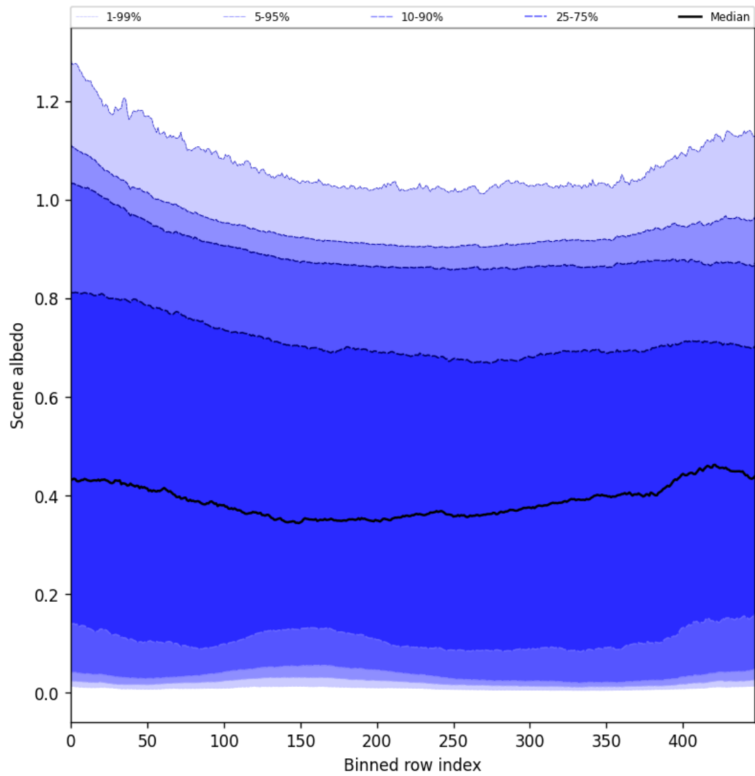
Figure 51: Along track statistics of “Scene albedo” for 2025-03-08 to 2025-03-10
