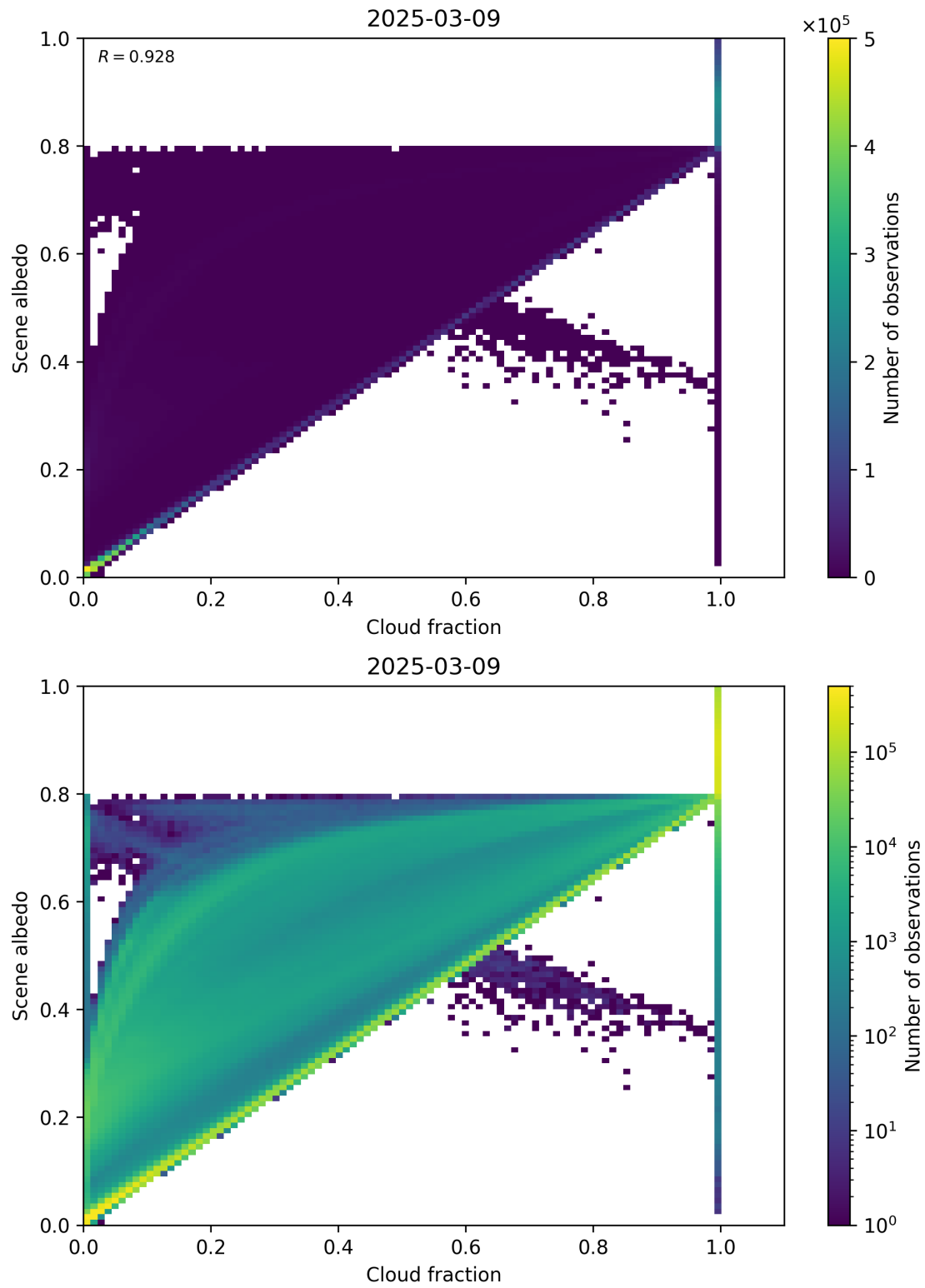
Figure 75: Scatter density plot of “Cloud fraction” against “Scene albedo” for 2025-03-08 to 2025-03-10.
