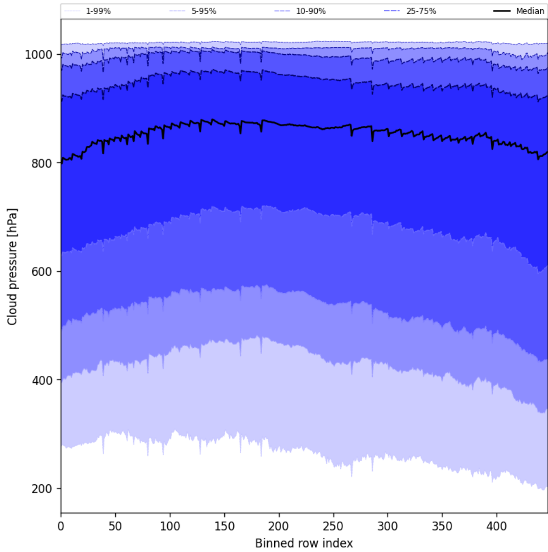
Figure 47: Along track statistics of “Cloud pressure” for 2025-03-08 to 2025-03-10
