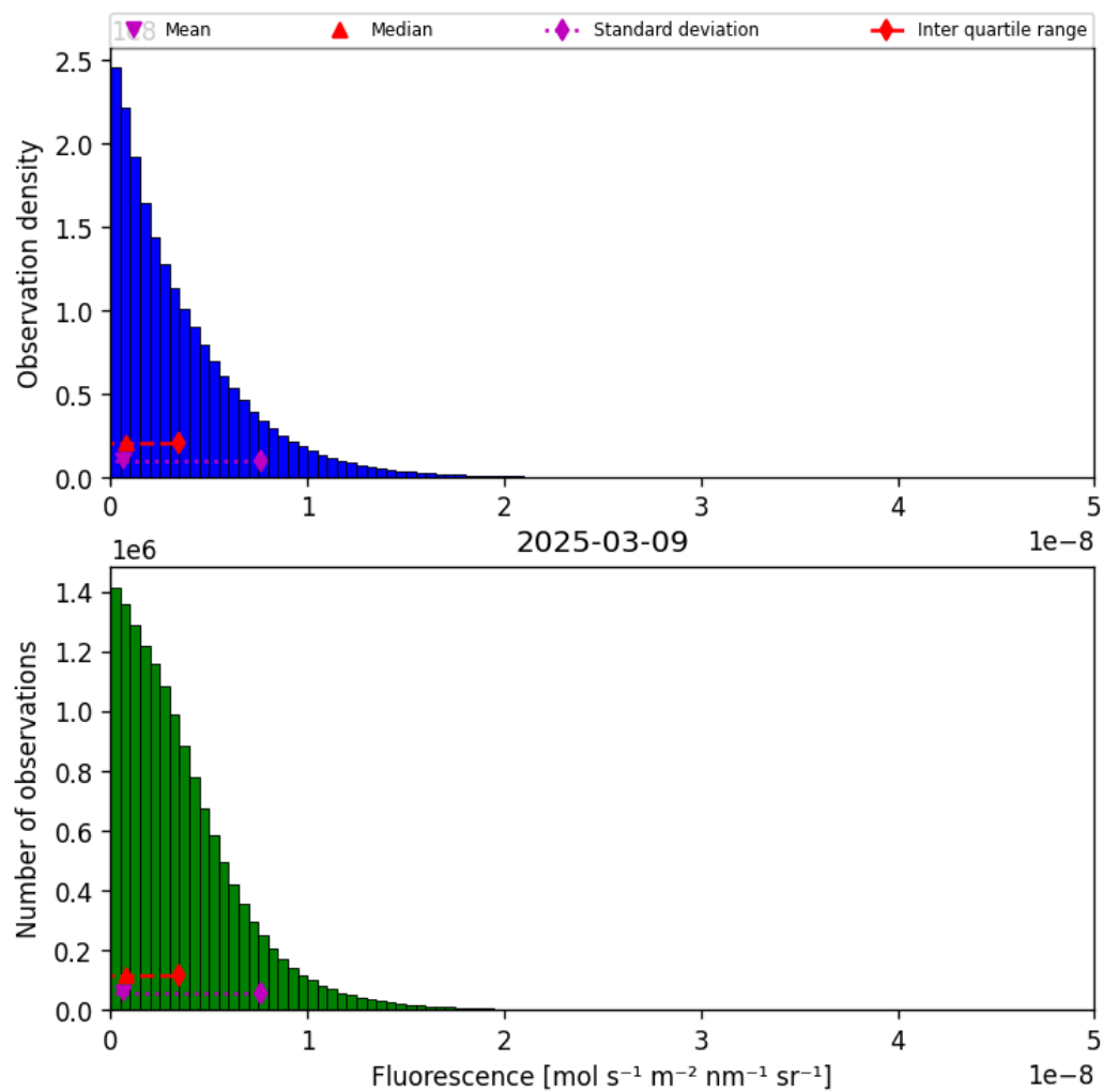
Figure 40: Histogram of “Fluorescence” for 2025-03-08 to 2025-03-10
