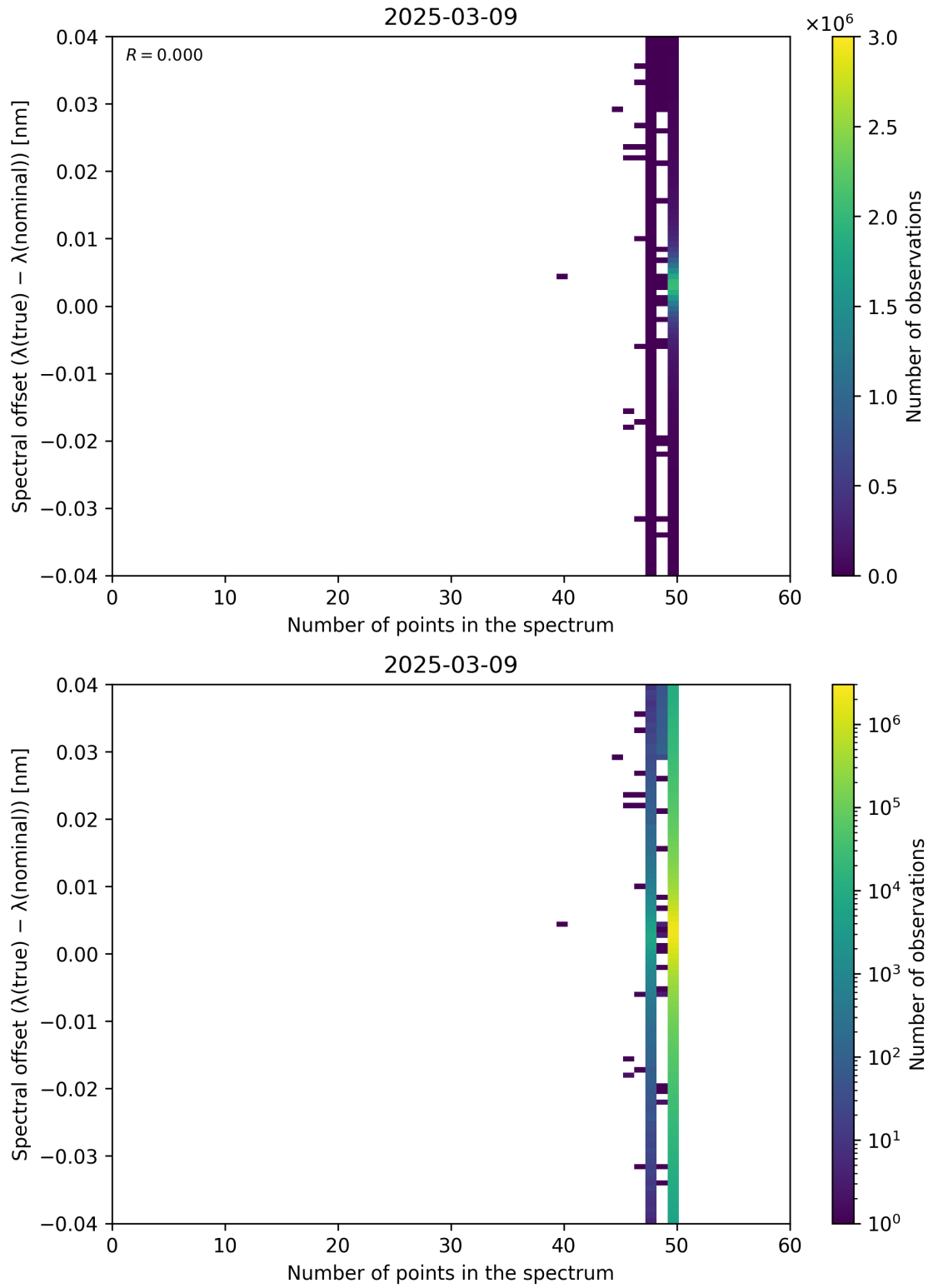
Figure 101: Scatter density plot of “Number of points in the spectrum” against “Spectral offset ( \lambda_{\text{true}} - \lambda_{\text{nominal}} )” for 2025-03-08 to 2025-03-10.
