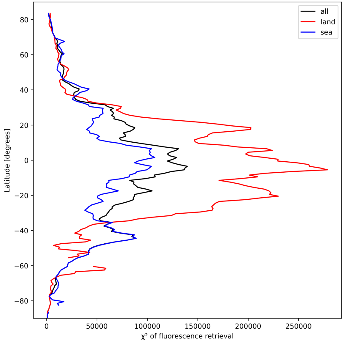
Figure 25: Zonal average of “ \chi^2 of fluorescence retrieval” for 2025-03-08 to 2025-03-10.
