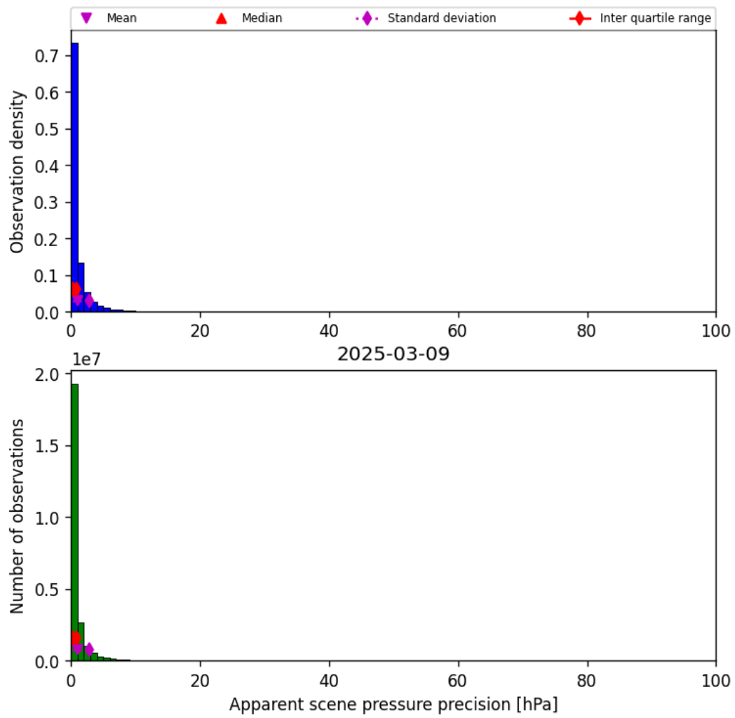
Figure 37: Histogram of “Apparent scene pressure precision” for 2025-03-08 to 2025-03-10
