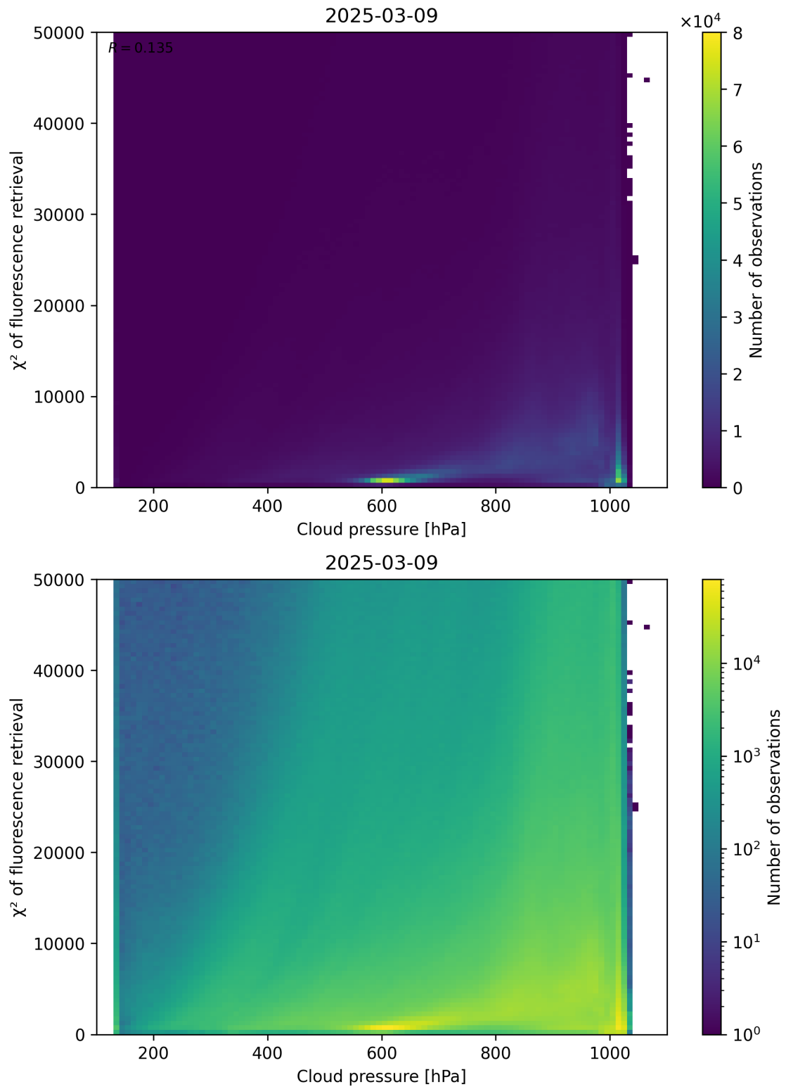
Figure 78: Scatter density plot of “Cloud pressure” against “ \chi^2 of fluorescence retrieval” for 2025-03-08 to 2025-03-10.
