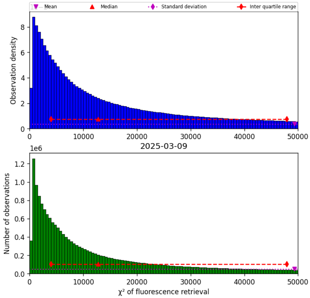
Figure 42: Histogram of “ \chi^2 of fluorescence retrieval” for 2025-03-08 to 2025-03-10
