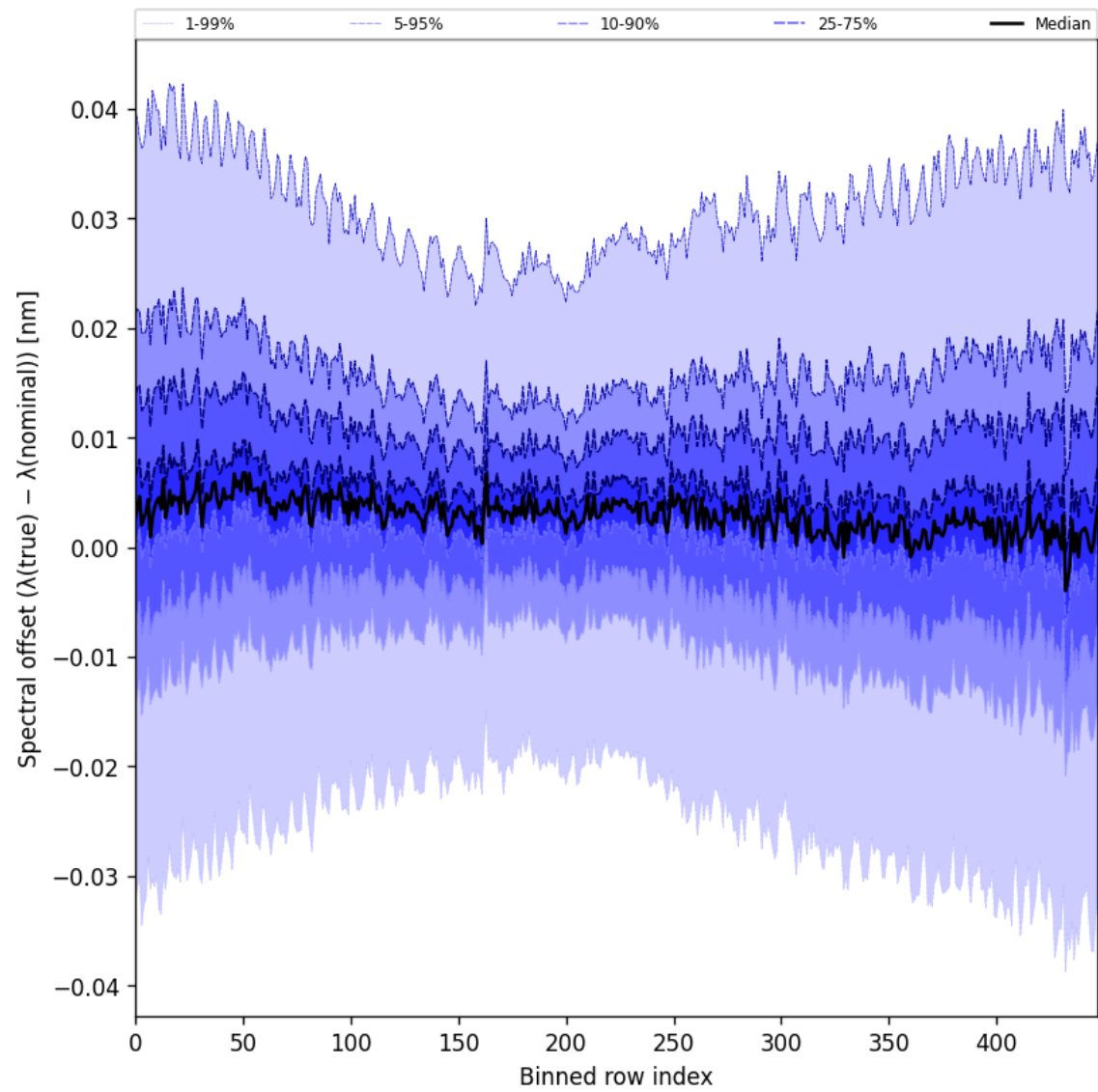
Figure 62: Along track statistics of “Spectral offset ( \lambda_{\text{true}} - \lambda_{\text{nominal}} )” for 2025-03-08 to 2025-03-10
