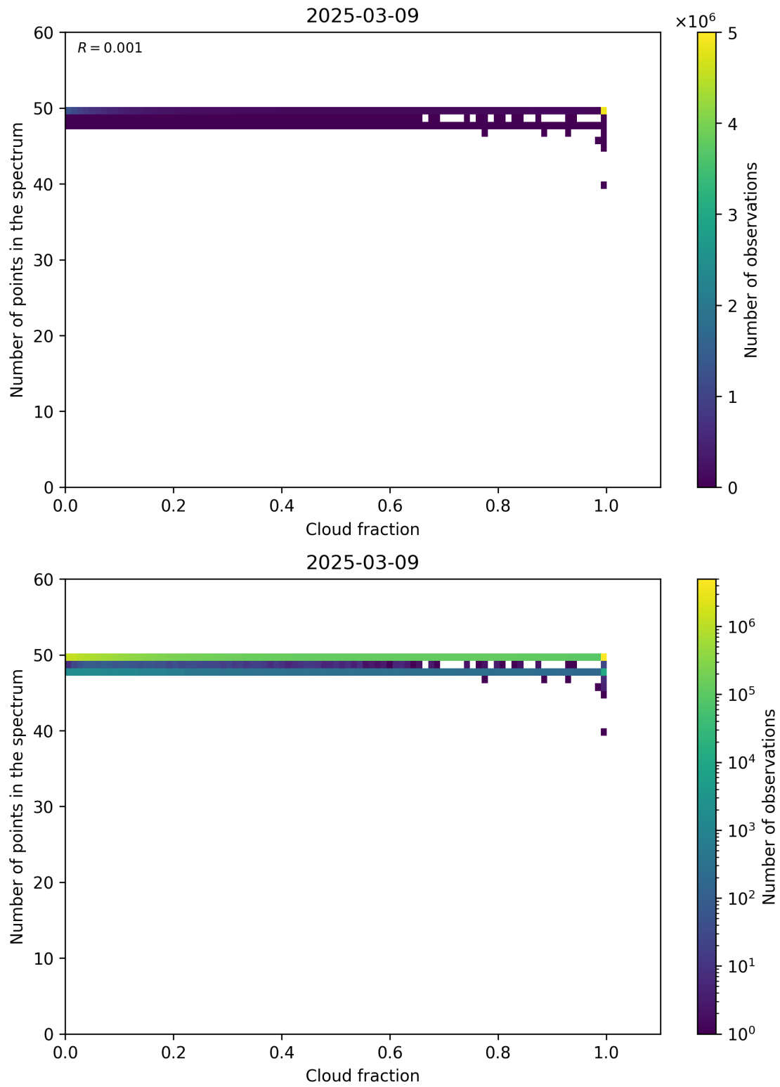
Figure 74: Scatter density plot of “Cloud fraction” against “Number of points in the spectrum” for 2025-03-08 to 2025-03-10.
