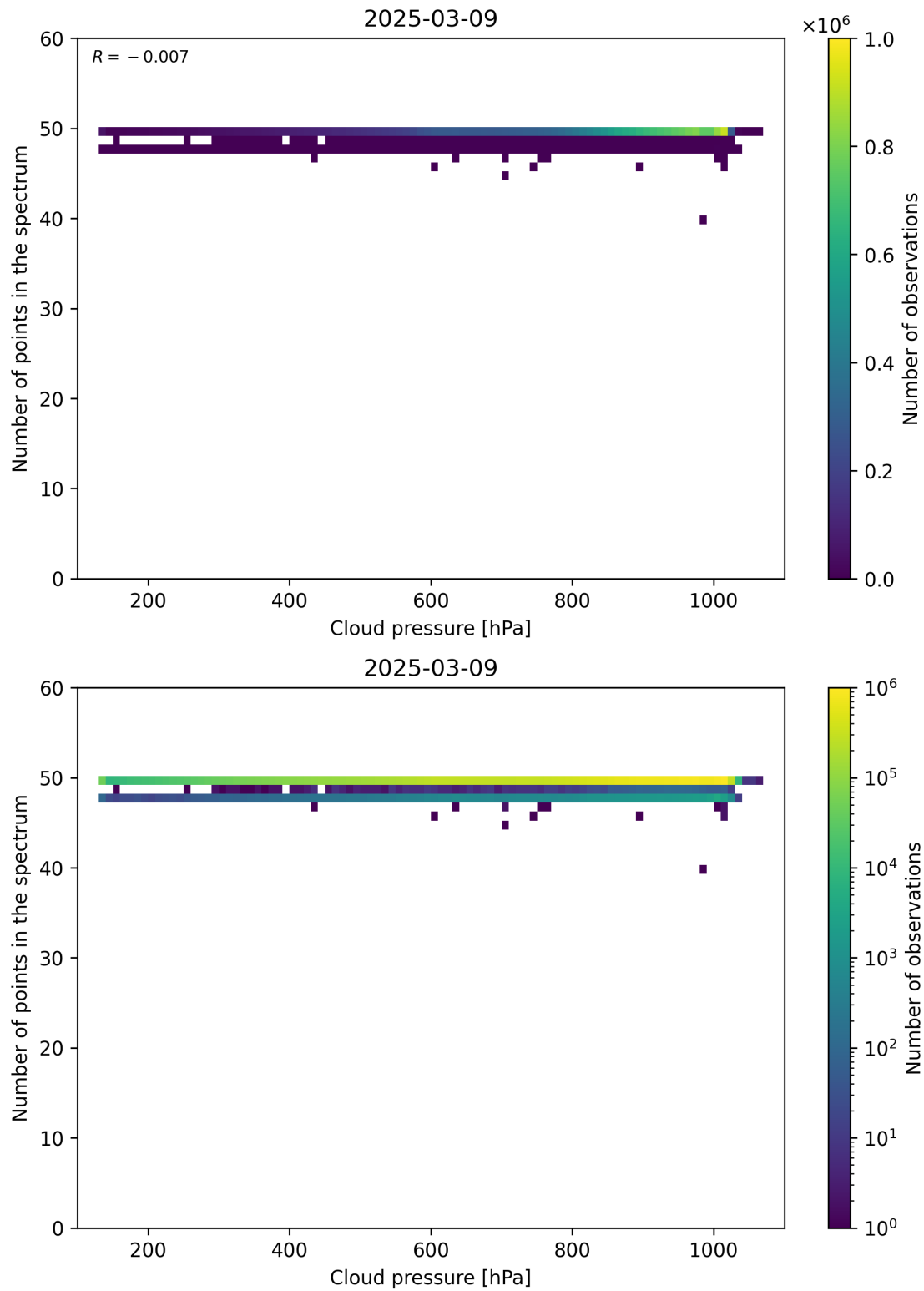
Figure 82: Scatter density plot of “Cloud pressure” against “Number of points in the spectrum” for 2025-03-08 to 2025-03-10.
