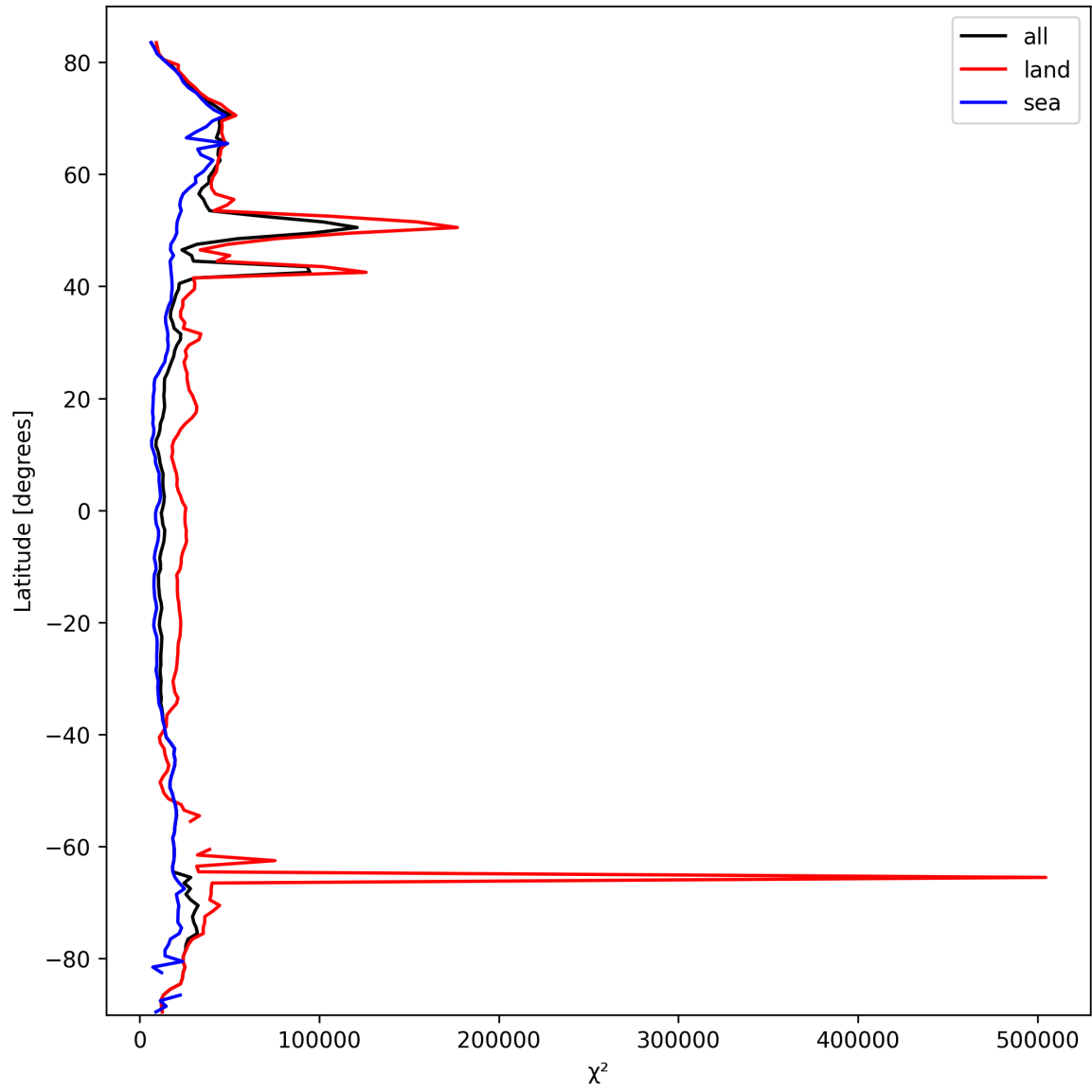
Figure 21: Zonal average of “ \chi^2 ” for 2025-03-08 to 2025-03-10.
