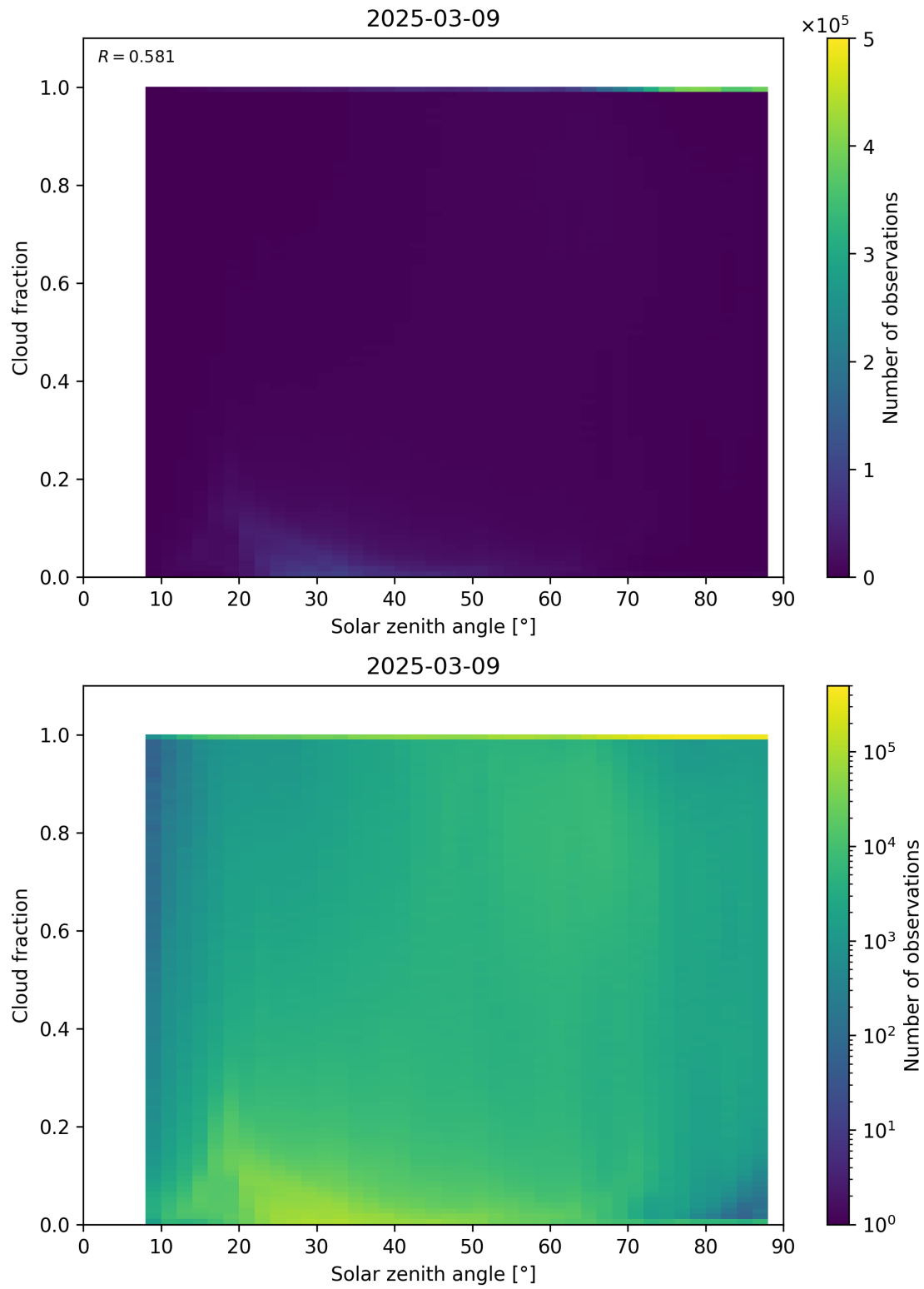
Figure 110: Scatter density plot of “Solar zenith angle” against “Cloud fraction” for 2025-03-08 to 2025-03-10.
