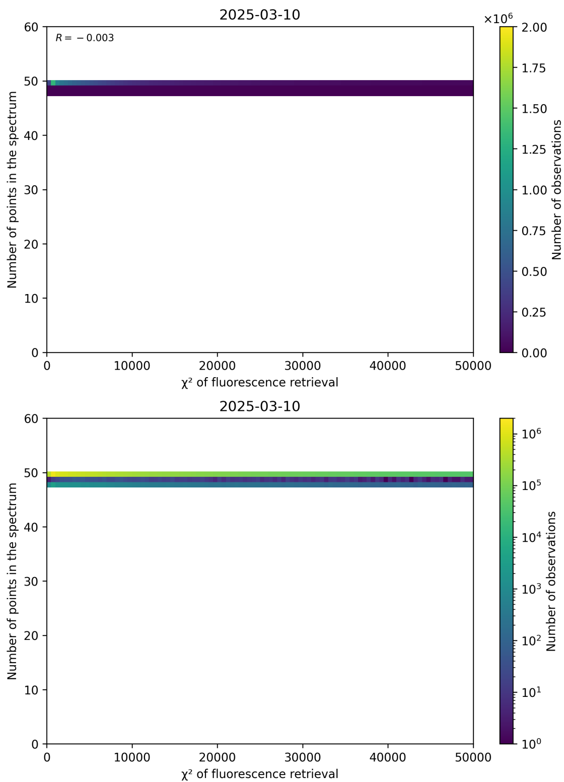
Figure 68: Scatter density plot of " \chi^2 of fluorescence retrieval" against "Number of points in the spectrum" for 2025-03-09 to 2025-03-11.
