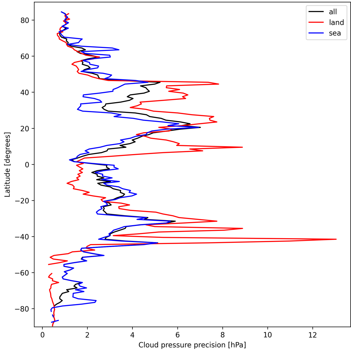
Figure 14: Zonal average of "Cloud pressure precision" for 2025-03-09 to 2025-03-11.
