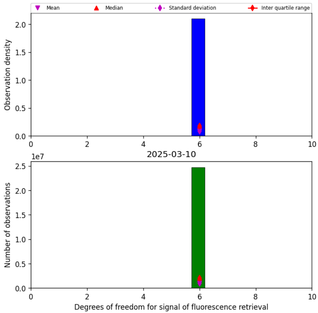
Figure 43: Histogram of “Degrees of freedom for signal of fluorescence retrieval” for 2025-03-09 to 2025-03-11
