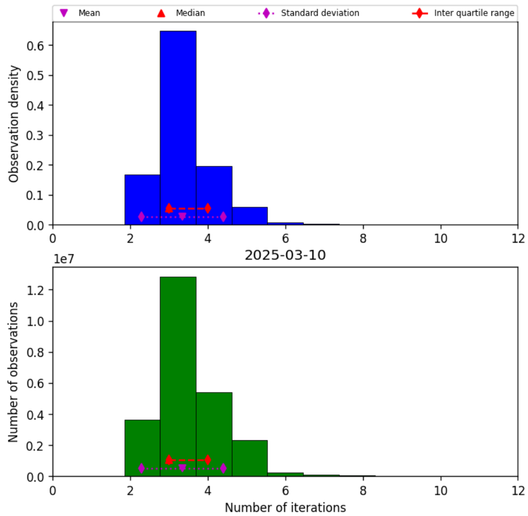
Figure 39: Histogram of “Number of iterations” for 2025-03-09 to 2025-03-11
