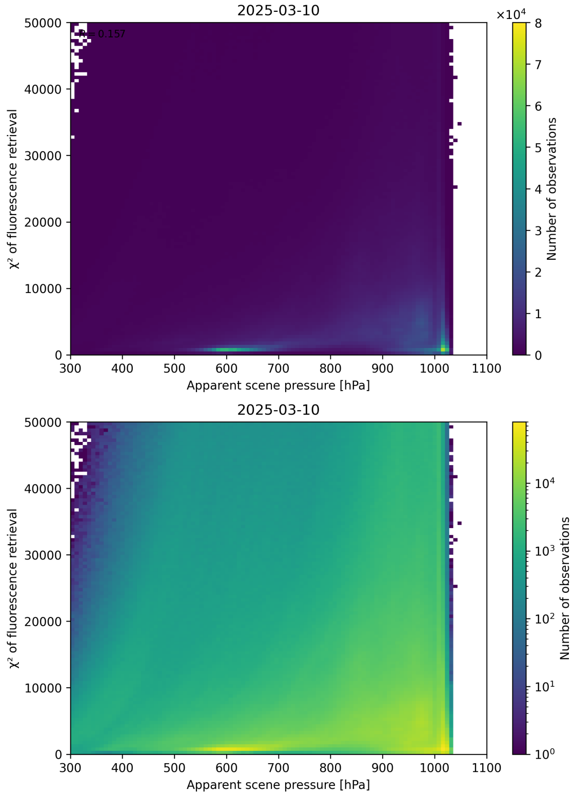
Figure 63: Scatter density plot of “Apparent scene pressure” against “ \chi^2 of fluorescence retrieval” for 2025-03-09 to 2025-03-11.
