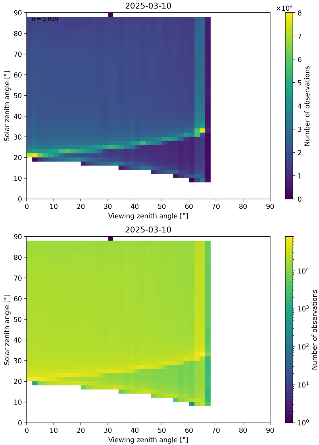
Figure 127: Scatter density plot of “Viewing zenith angle” against “Solar zenith angle” for 2025-03-09 to 2025-03-11.
