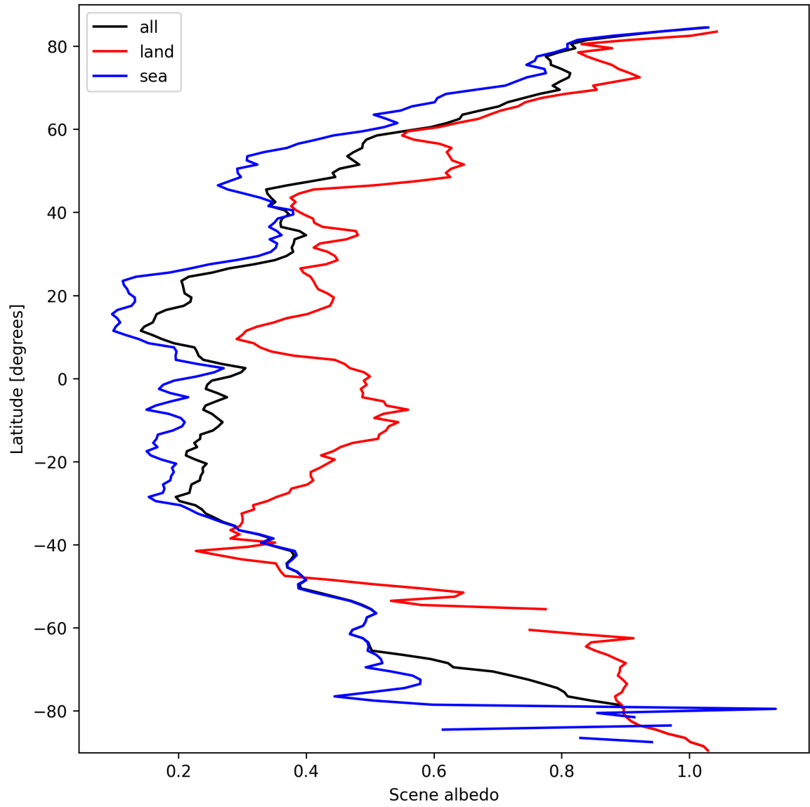
Figure 17: Zonal average of “Scene albedo” for 2025-03-09 to 2025-03-11.
