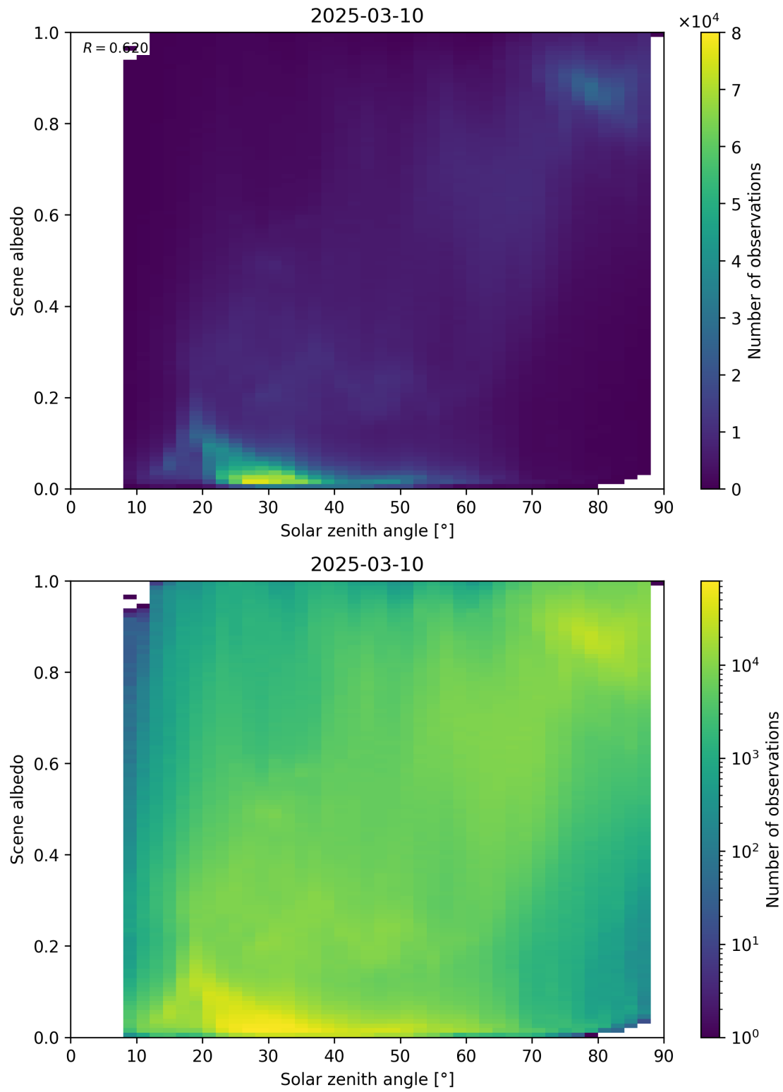
Figure 116: Scatter density plot of “Solar zenith angle” against “Scene albedo” for 2025-03-09 to 2025-03-11.
