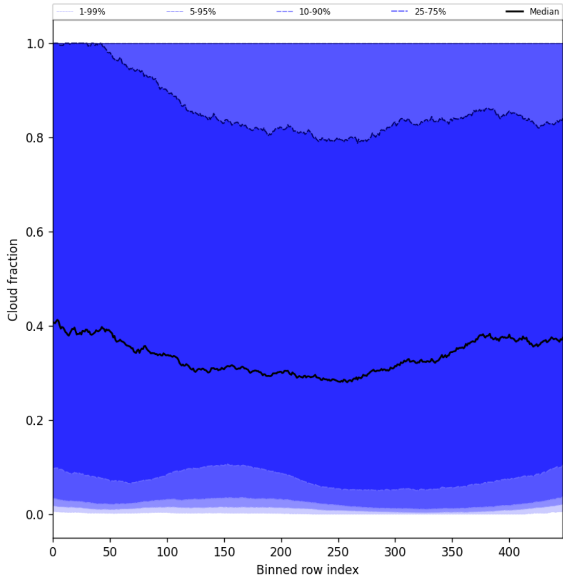
Figure 49: Along track statistics of “Cloud fraction” for 2025-03-09 to 2025-03-11
