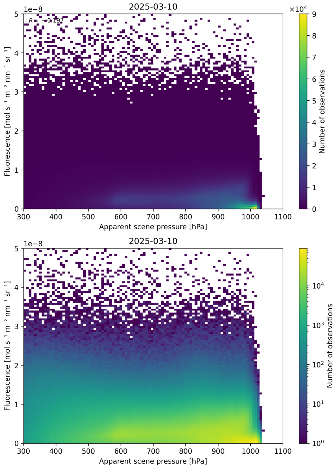
Figure 64: Scatter density plot of “Apparent scene pressure” against “Fluorescence” for 2025-03-09 to 2025-03-11.
