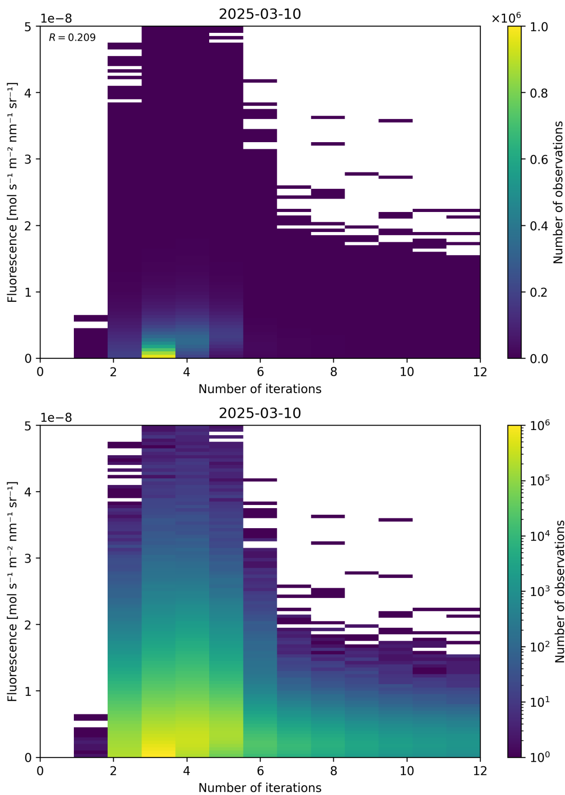
Figure 98: Scatter density plot of “Number of iterations” against “Fluorescence” for 2025-03-09 to 2025-03-11.
