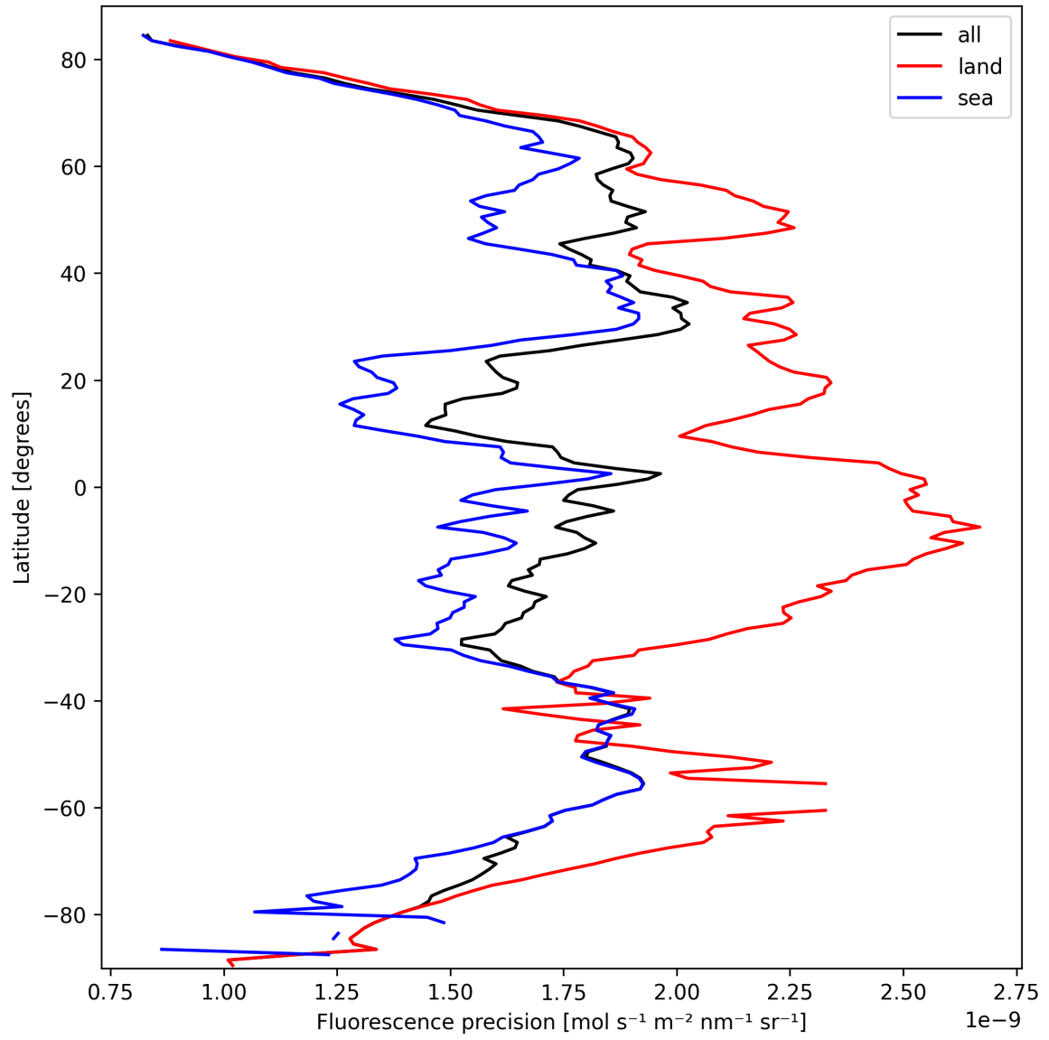
Figure 24: Zonal average of “Fluorescence precision” for 2025-03-09 to 2025-03-11.
