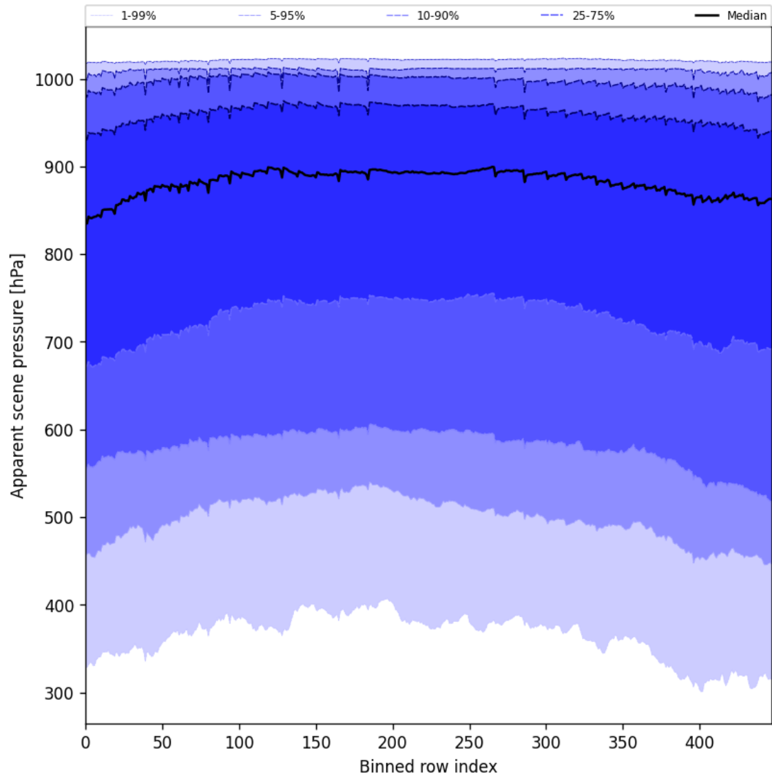
Figure 53: Along track statistics of “Apparent scene pressure” for 2025-03-09 to 2025-03-11
