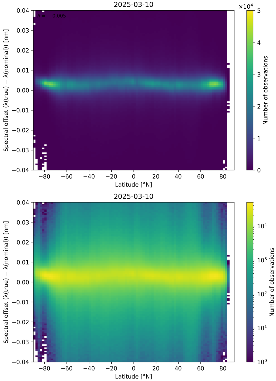
Figure 96: Scatter density plot of “Latitude” against “Spectral offset ( \lambda_{\text{true}} - \lambda_{\text{nominal}} )” for 2025-03-09 to 2025-03-11.
