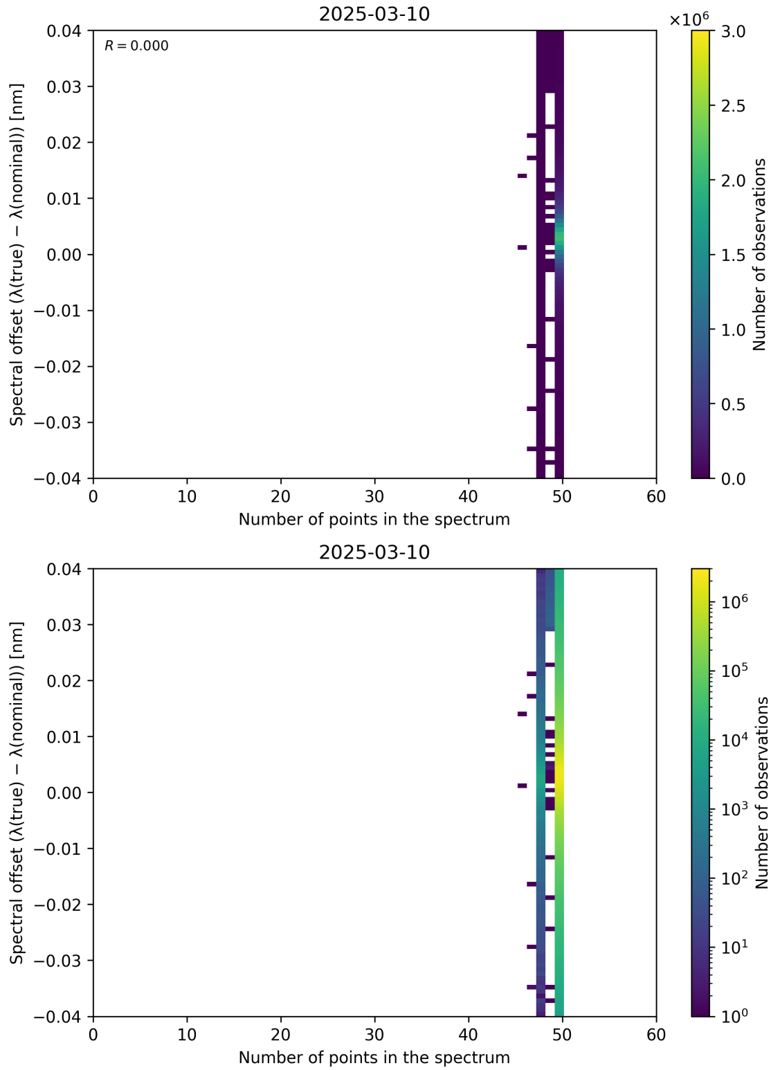
Figure 101: Scatter density plot of “Number of points in the spectrum” against “Spectral offset ( \lambda_{\text{true}} - \lambda_{\text{nominal}} )” for 2025-03-09 to 2025-03-11.
