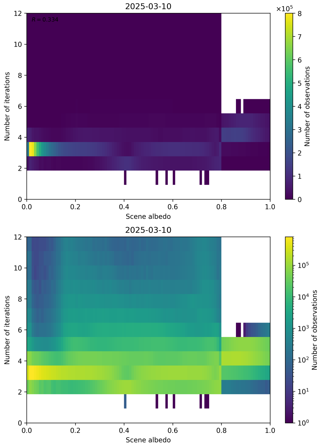
Figure 105: Scatter density plot of “Scene albedo” against “Number of iterations” for 2025-03-09 to 2025-03-11.
