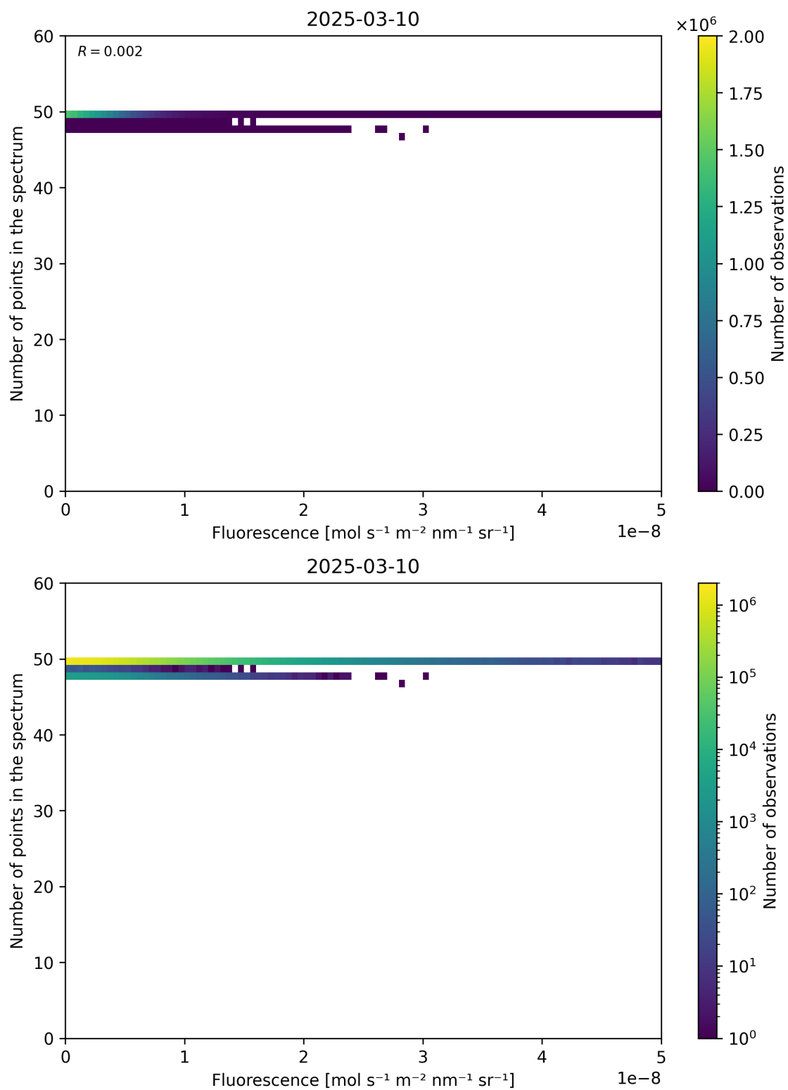
Figure 86: Scatter density plot of “Fluorescence” against “Number of points in the spectrum” for 2025-03-09 to 2025-03-11.
