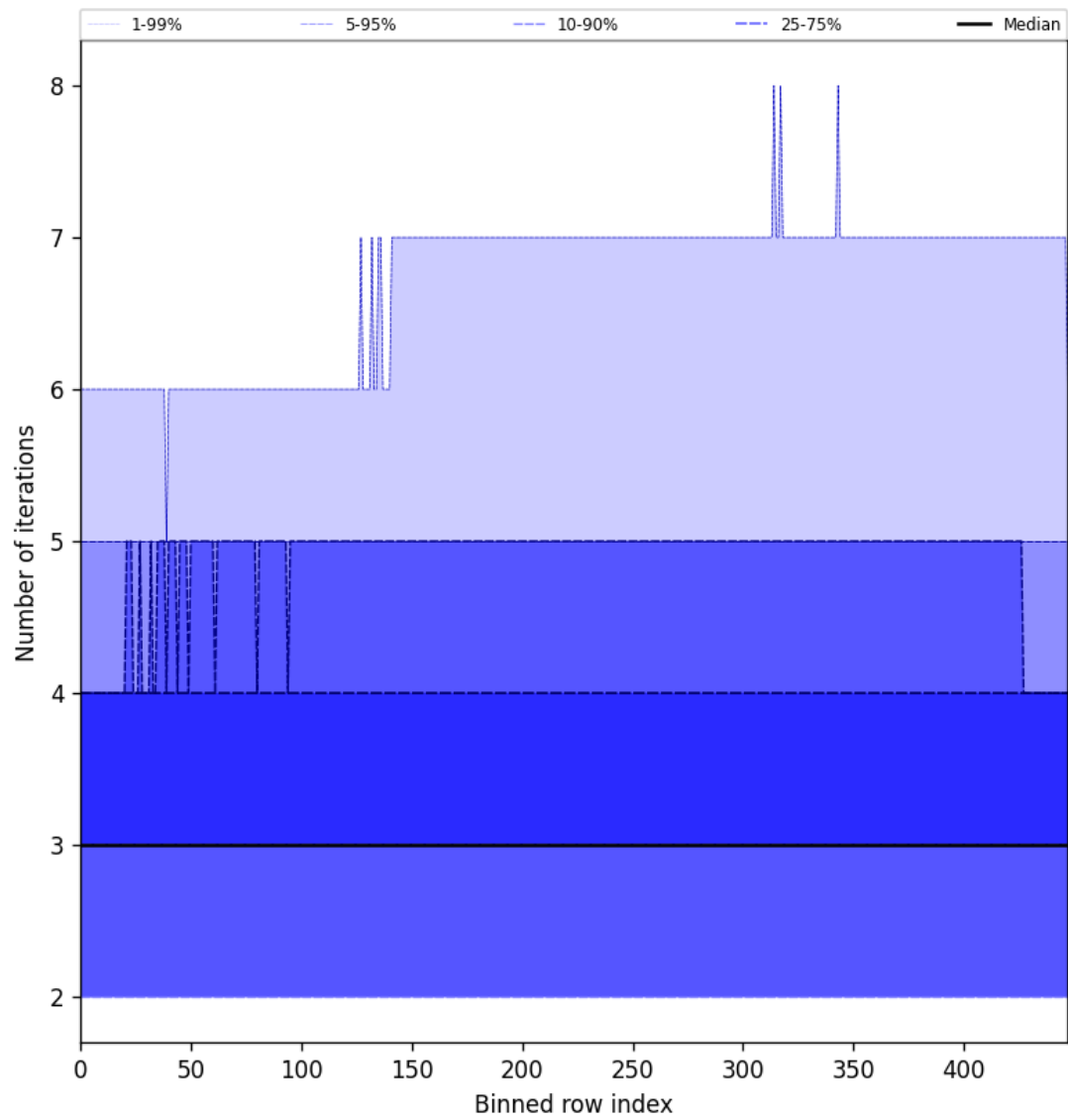
Figure 56: Along track statistics of “Number of iterations” for 2025-03-09 to 2025-03-11
