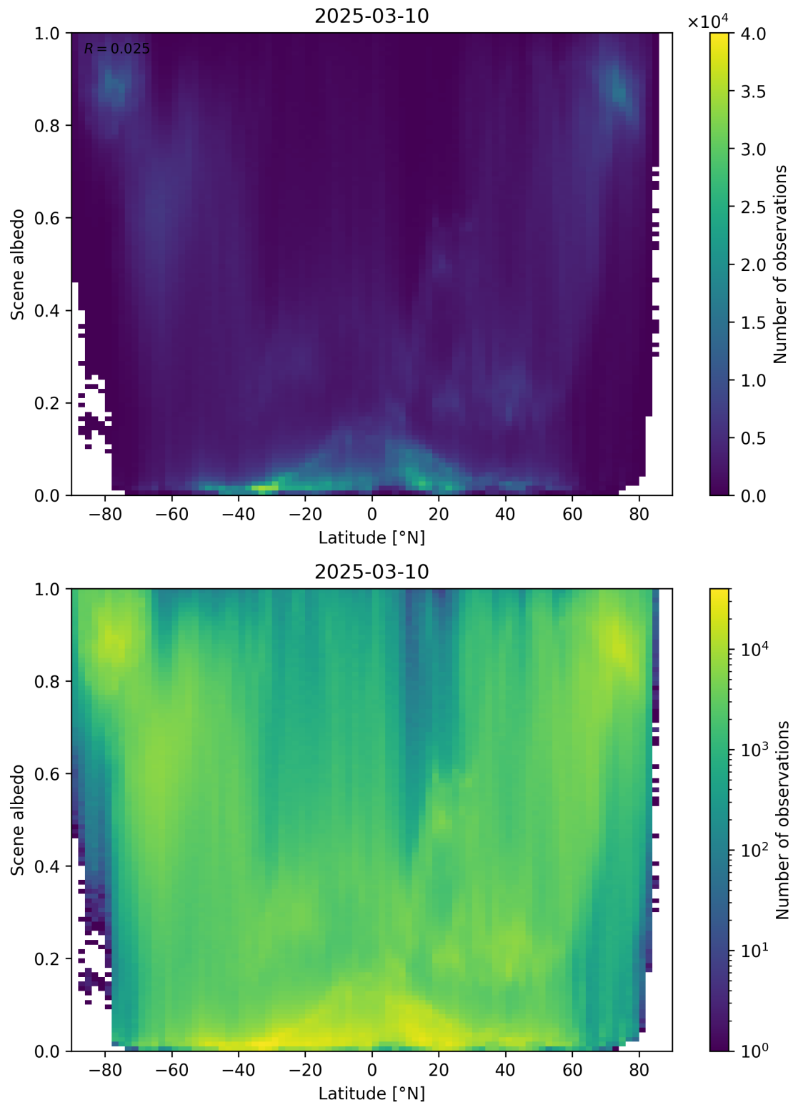
Figure 95: Scatter density plot of “Latitude” against “Scene albedo” for 2025-03-09 to 2025-03-11.
