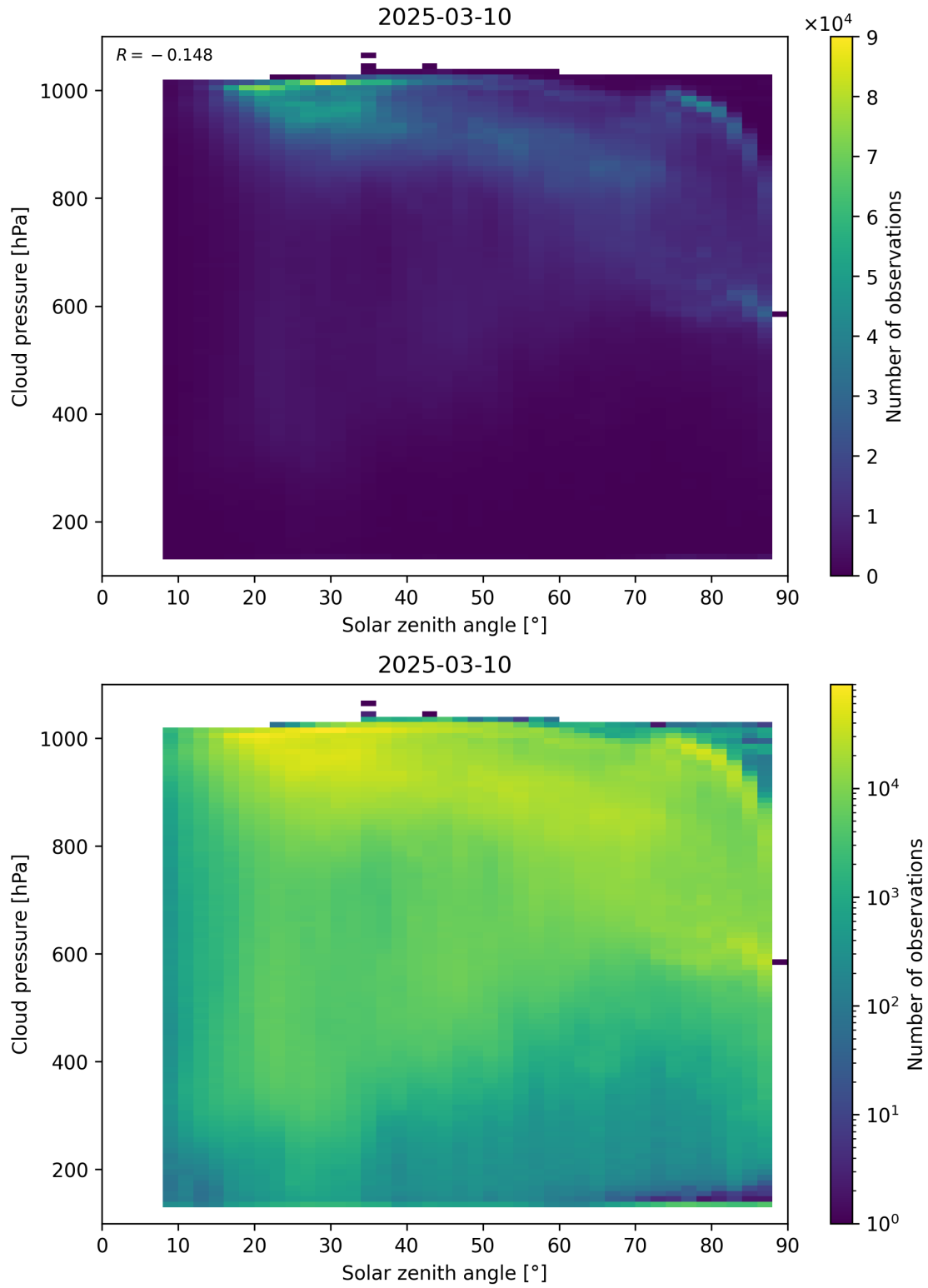
Figure 111: Scatter density plot of “Solar zenith angle” against “Cloud pressure” for 2025-03-09 to 2025-03-11.
