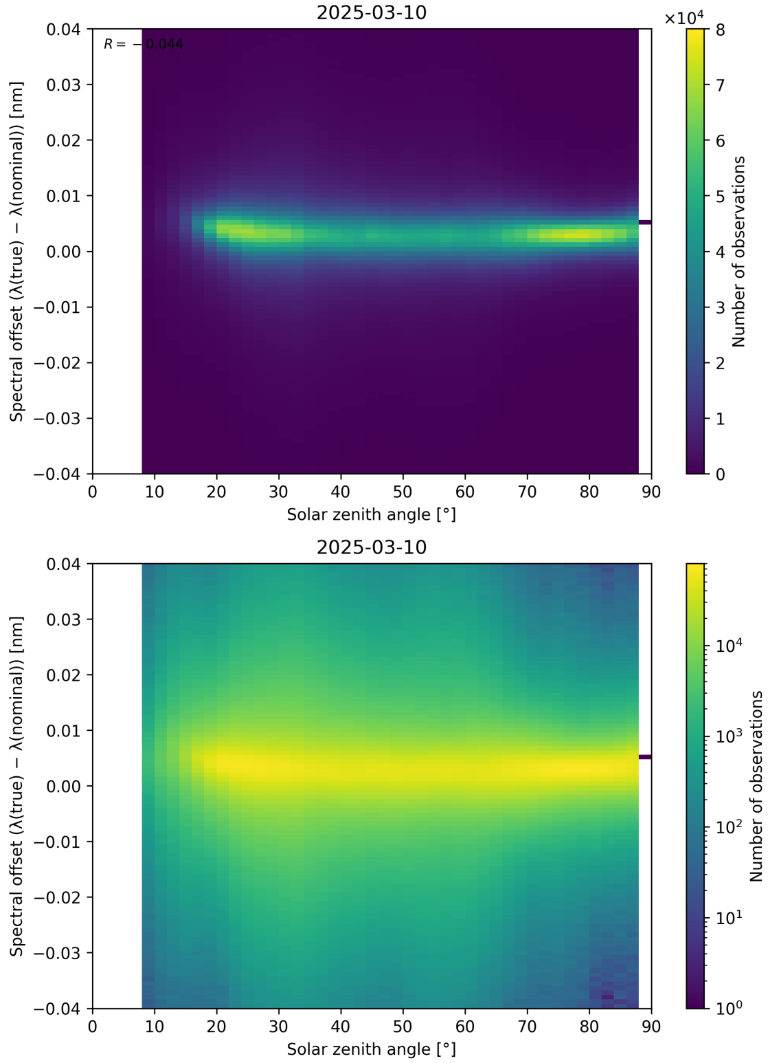
Figure 117: Scatter density plot of “Solar zenith angle” against “Spectral offset ( \lambda_{\text{true}} - \lambda_{\text{nominal}} )” for 2025-03-09 to 2025-03-11.
