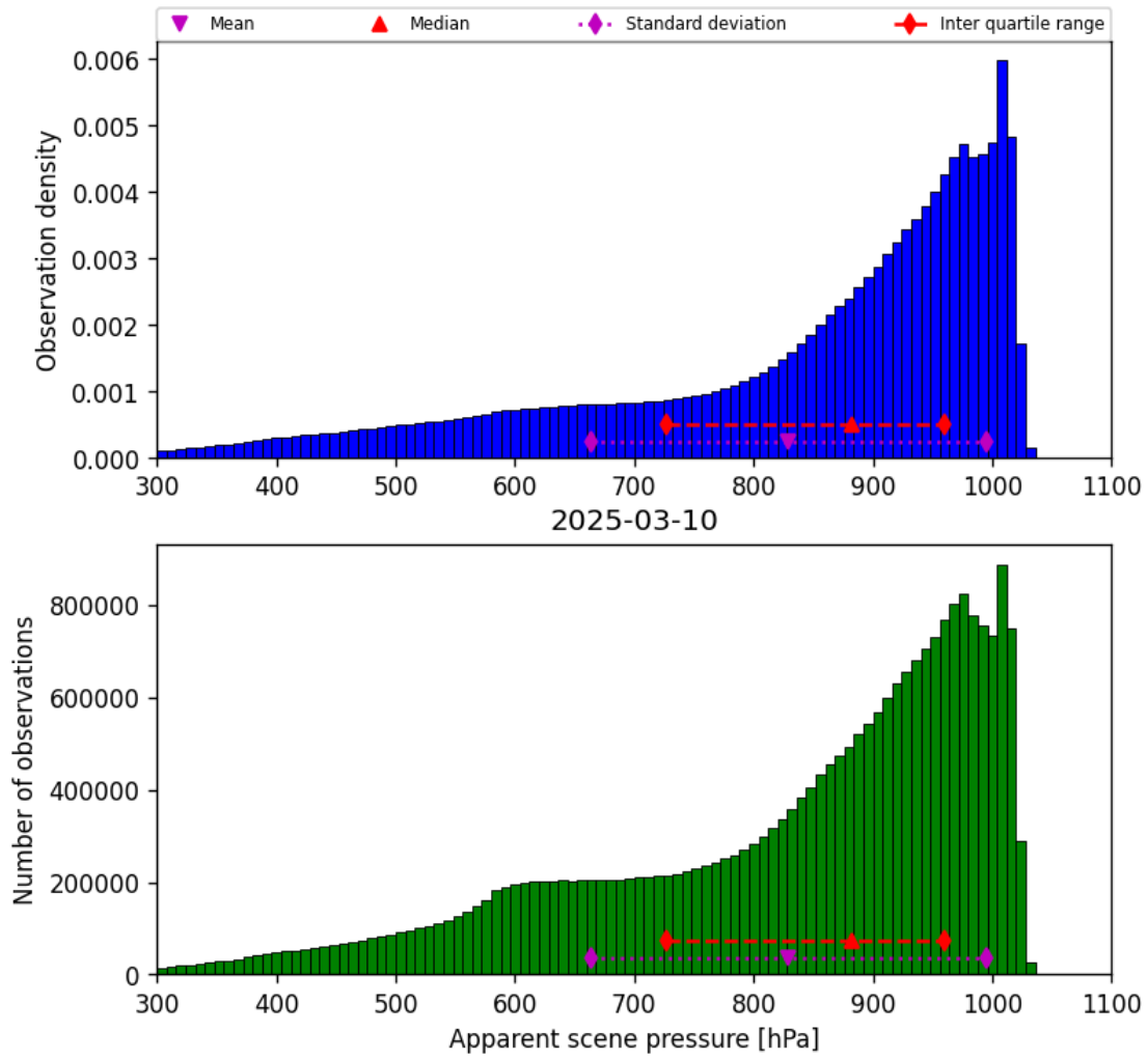
Figure 36: Histogram of “Apparent scene pressure” for 2025-03-09 to 2025-03-11
