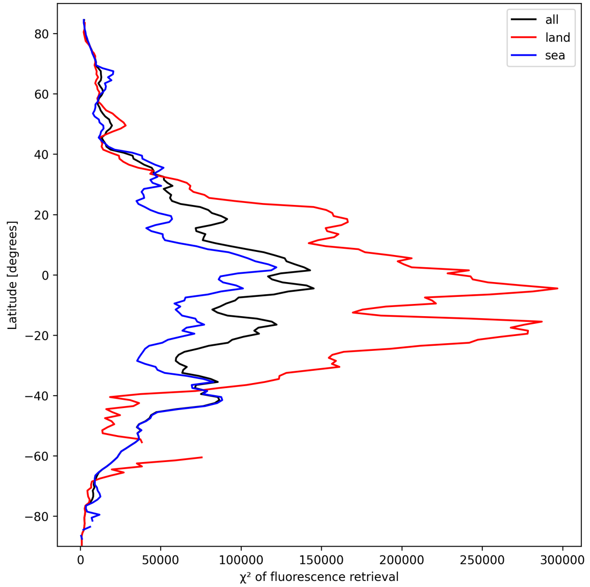
Figure 25: Zonal average of “ \chi^2 of fluorescence retrieval” for 2025-03-09 to 2025-03-11.
