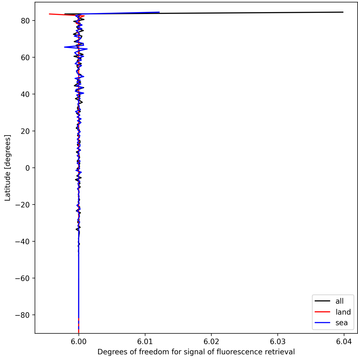
Figure 26: Zonal average of “Degrees of freedom for signal of fluorescence retrieval” for 2025-03-09 to 2025-03-11.
