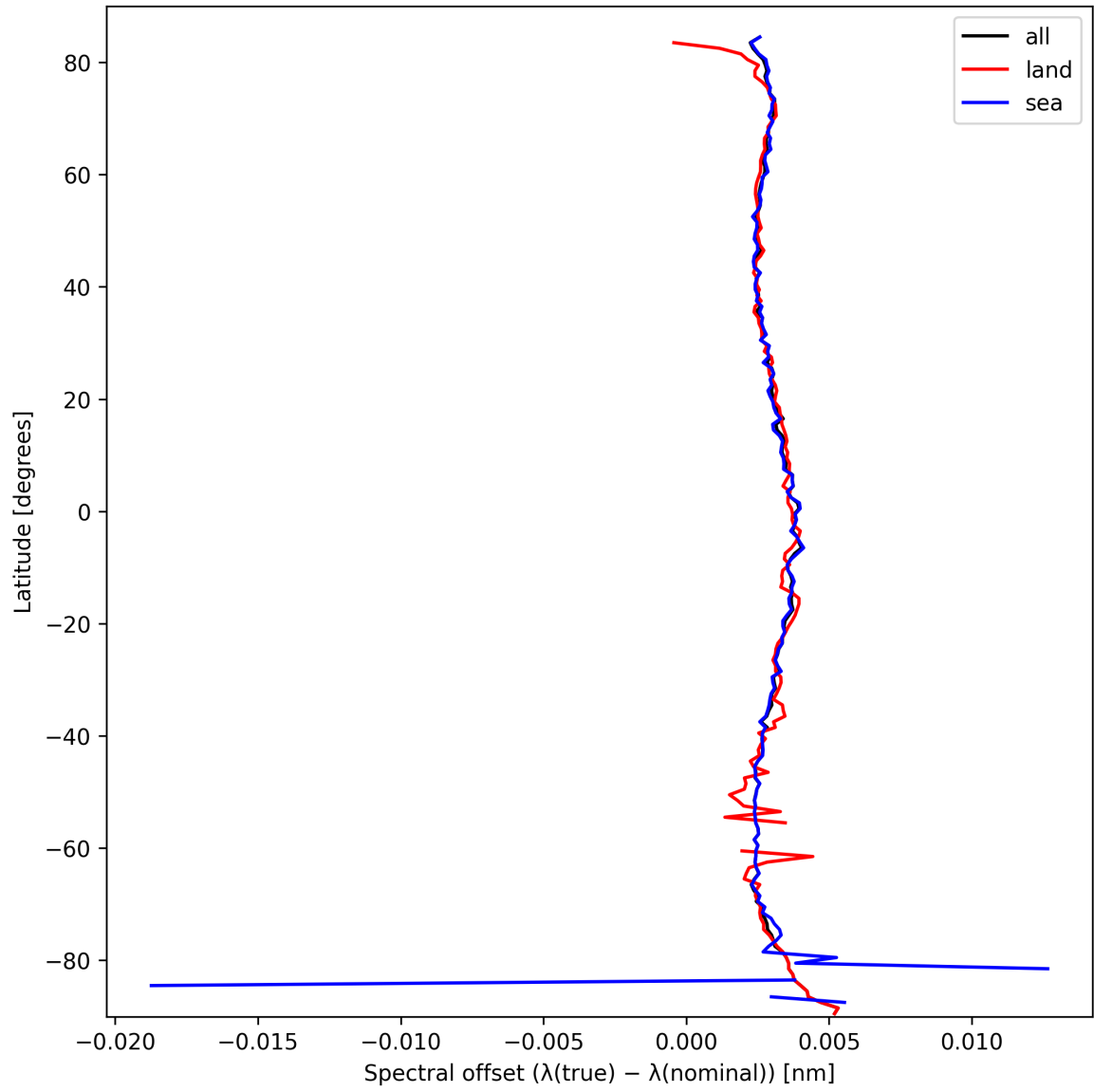
Figure 28: Zonal average of “Spectral offset ( \lambda_{\text{true}} - \lambda_{\text{nominal}} )” for 2025-03-09 to 2025-03-11.
