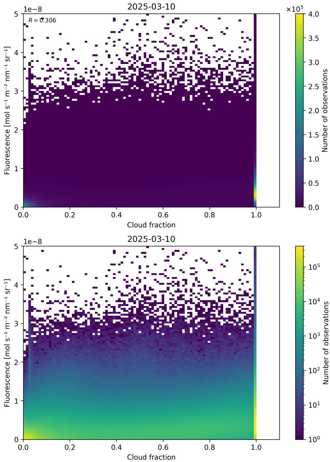
Figure 72: Scatter density plot of “Cloud fraction” against “Fluorescence” for 2025-03-09 to 2025-03-11.
