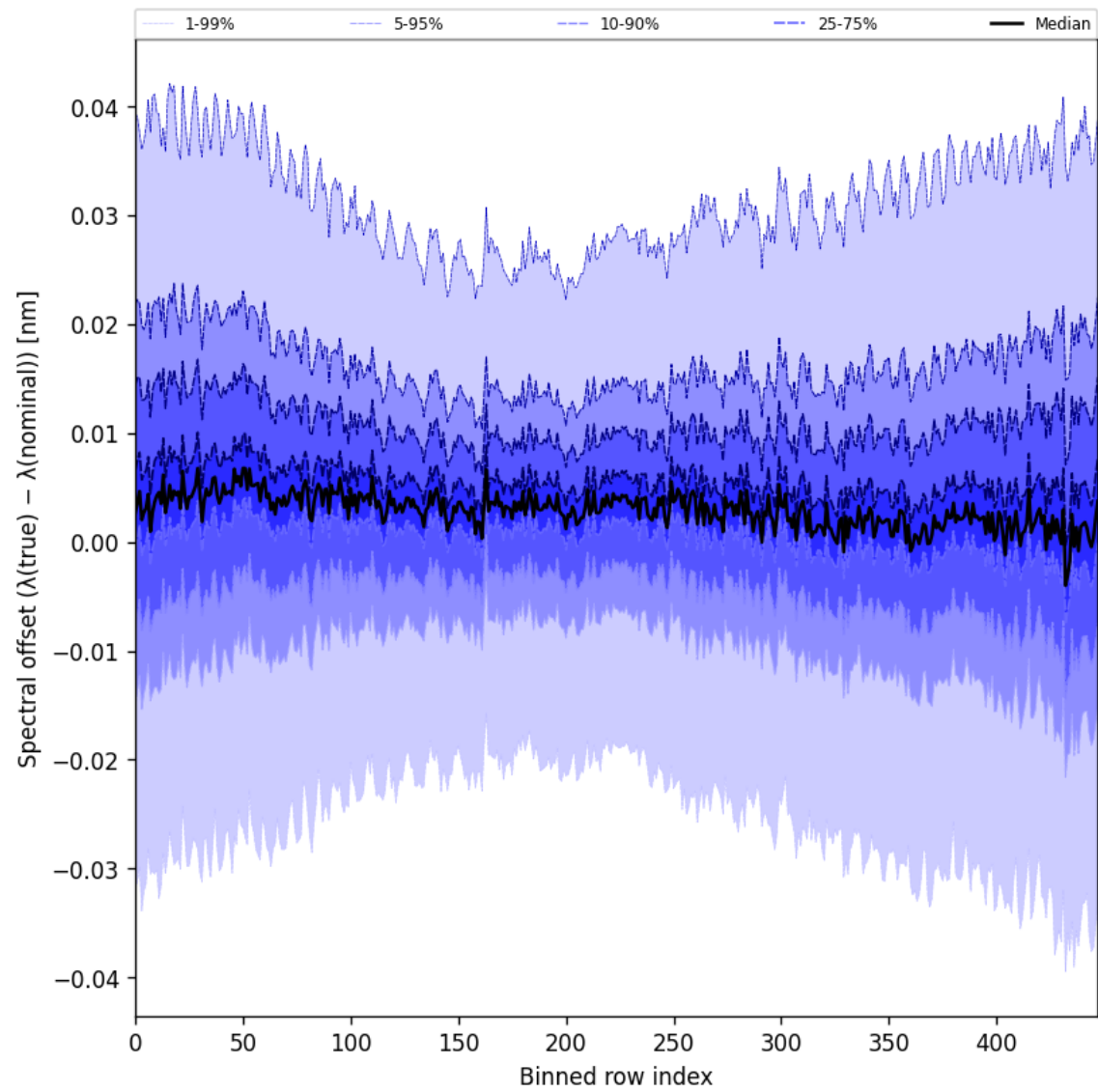
Figure 62: Along track statistics of “Spectral offset ( \lambda_{\text{true}} - \lambda_{\text{nominal}} )” for 2025-03-09 to 2025-03-11
