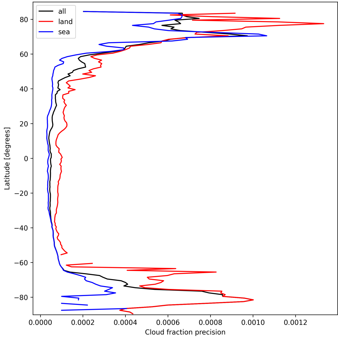
Figure 16: Zonal average of “Cloud fraction precision” for 2025-03-09 to 2025-03-11.
