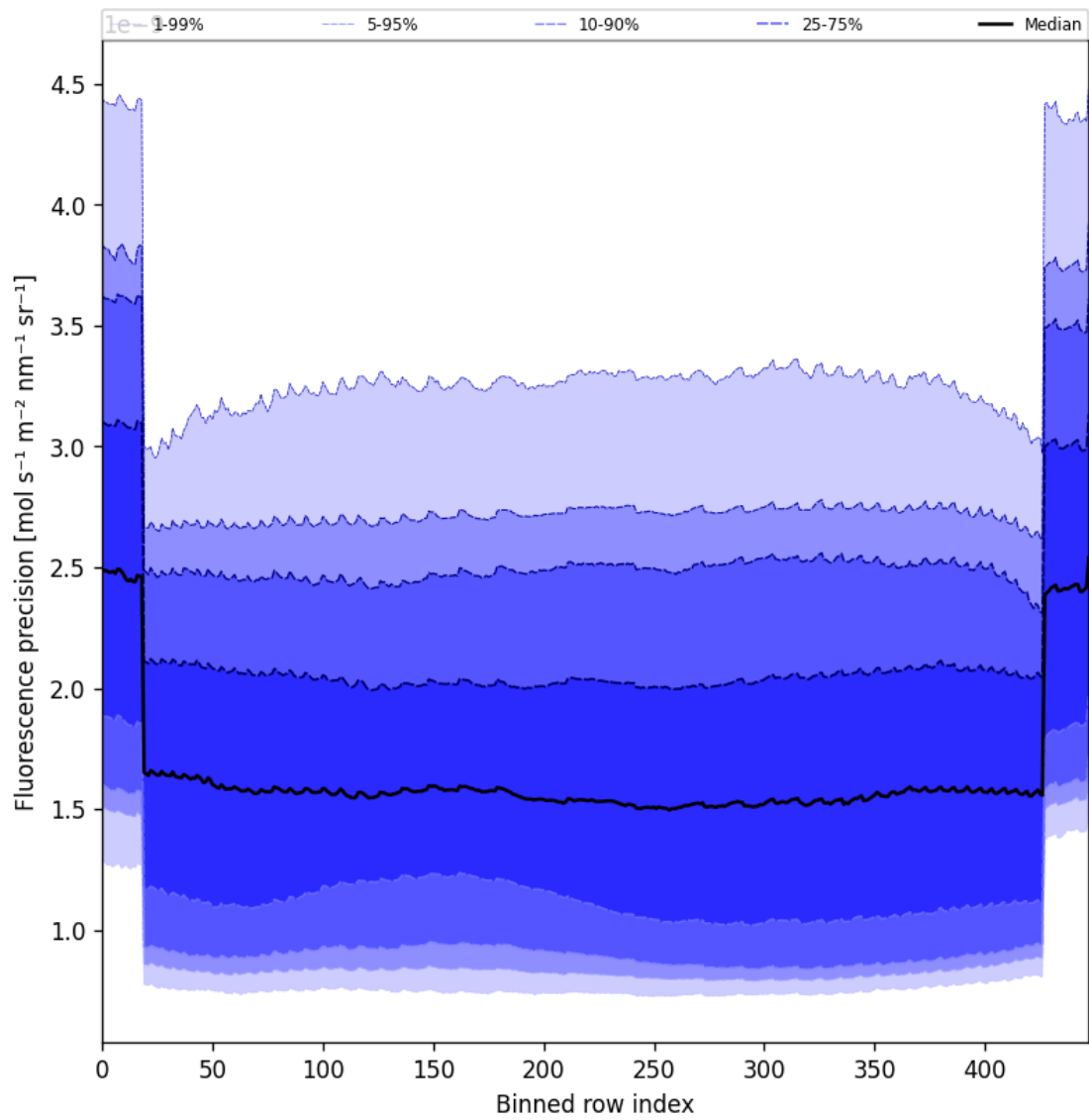
Figure 58: Along track statistics of “Fluorescence precision” for 2025-03-09 to 2025-03-11
