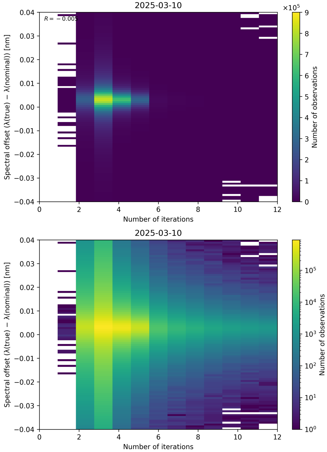
Figure 100: Scatter density plot of “Number of iterations” against “Spectral offset ( \lambda_{\text{true}} - \lambda_{\text{nominal}} )” for 2025-03-09 to 2025-03-11.
