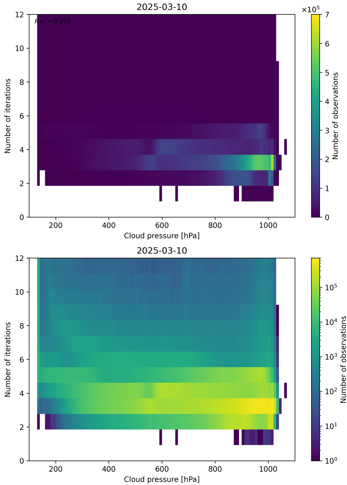
Figure 81: Scatter density plot of “Cloud pressure” against “Number of iterations” for 2025-03-09 to 2025-03-11.
