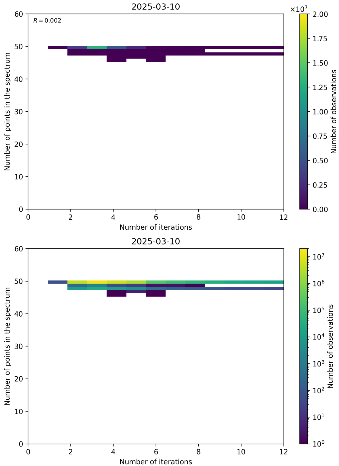
Figure 99: Scatter density plot of “Number of iterations” against “Number of points in the spectrum” for 2025-03-09 to 2025-03-11.
