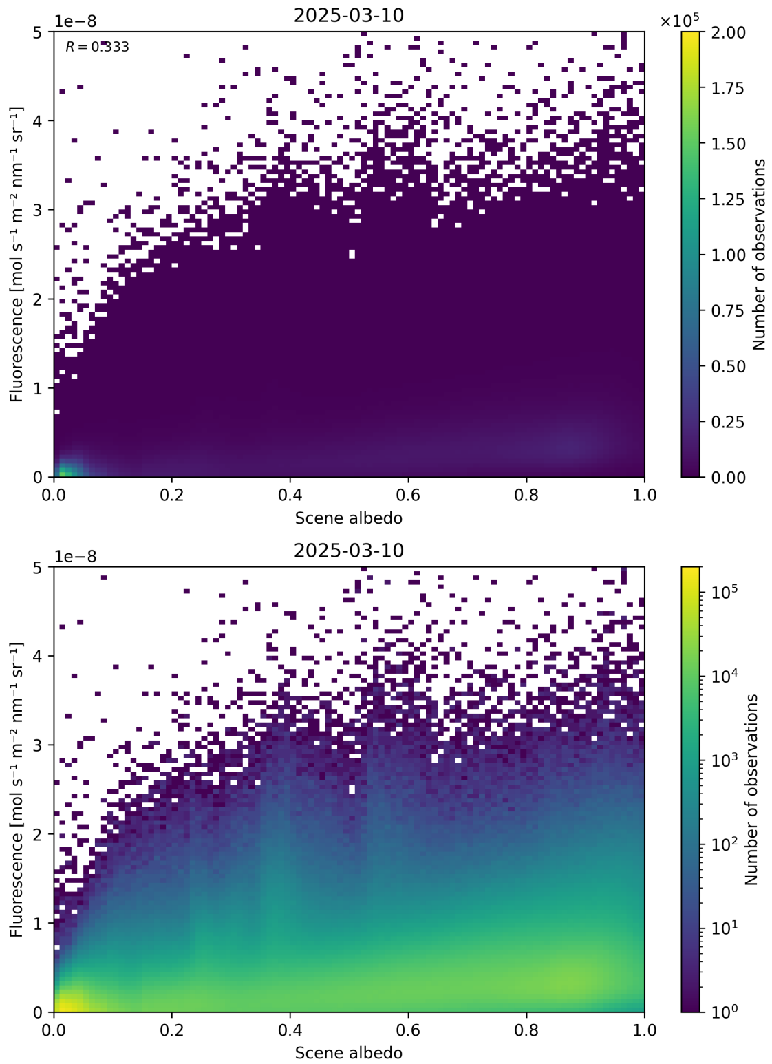
Figure 104: Scatter density plot of “Scene albedo” against “Fluorescence” for 2025-03-09 to 2025-03-11.
