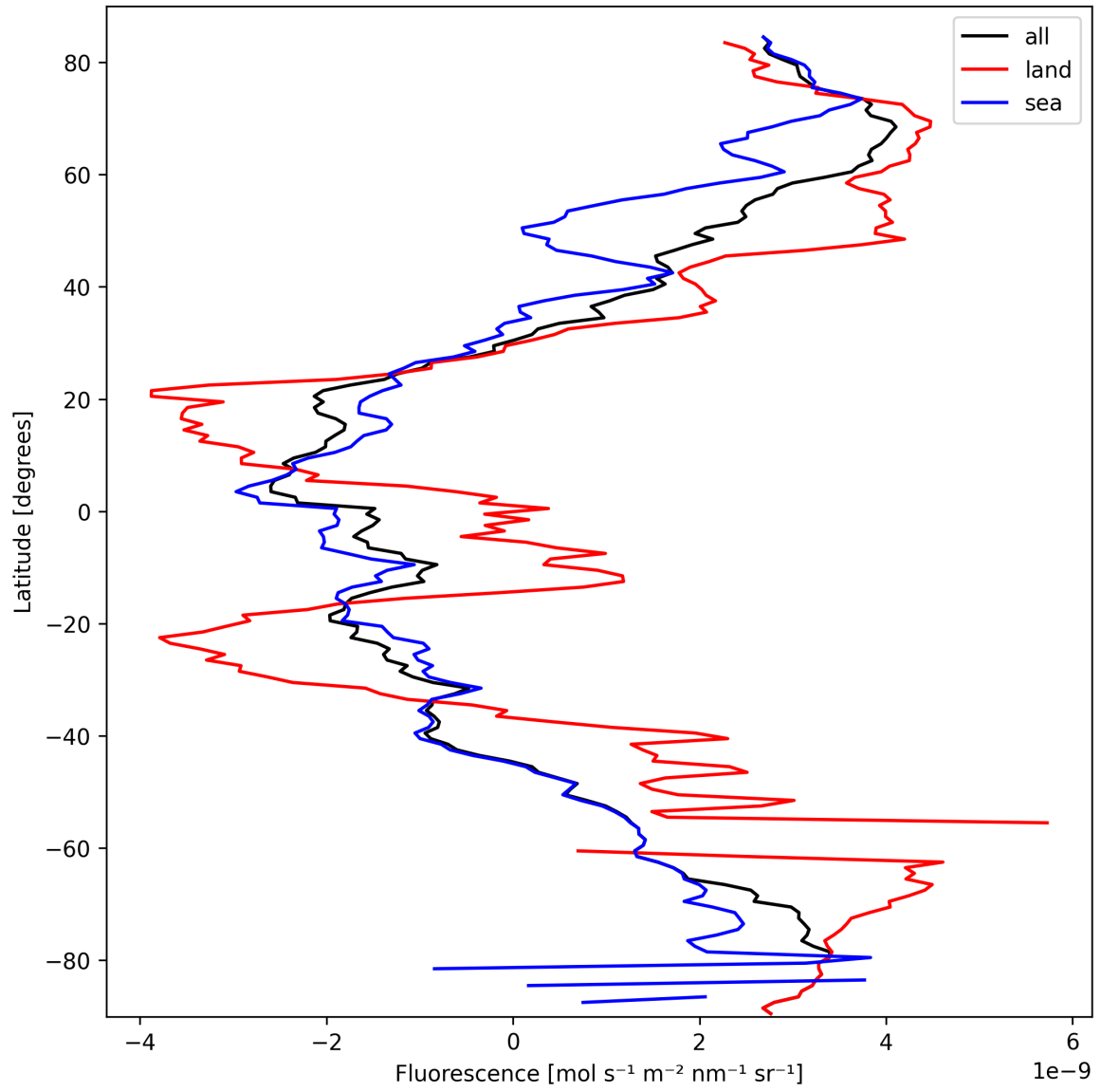
Figure 23: Zonal average of “Fluorescence” for 2025-03-09 to 2025-03-11.
