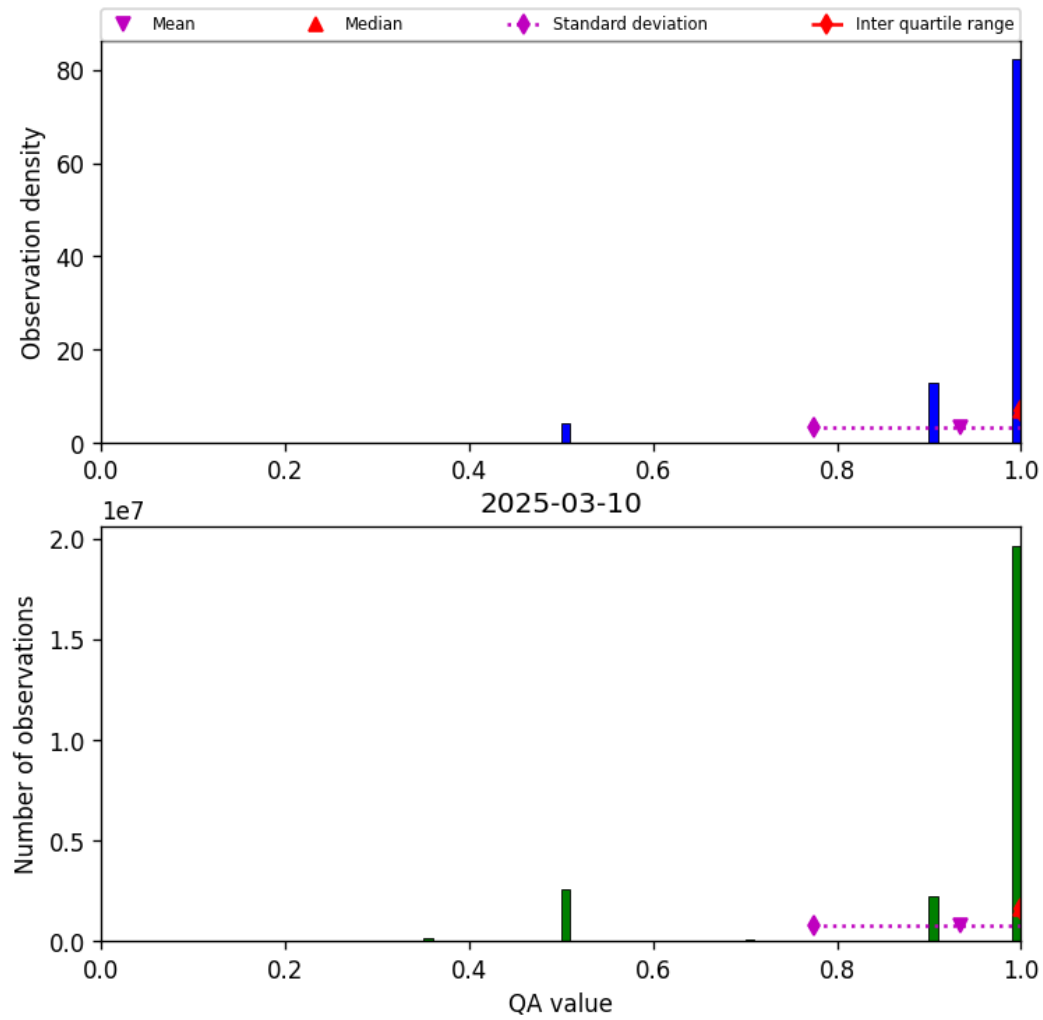
Figure 29: Histogram of “QA value” for 2025-03-09 to 2025-03-11
