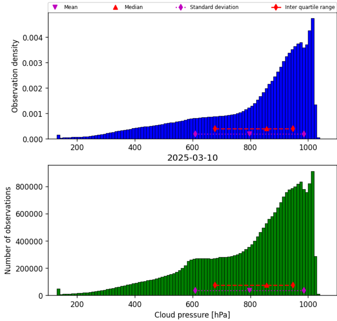
Figure 30: Histogram of “Cloud pressure” for 2025-03-09 to 2025-03-11
