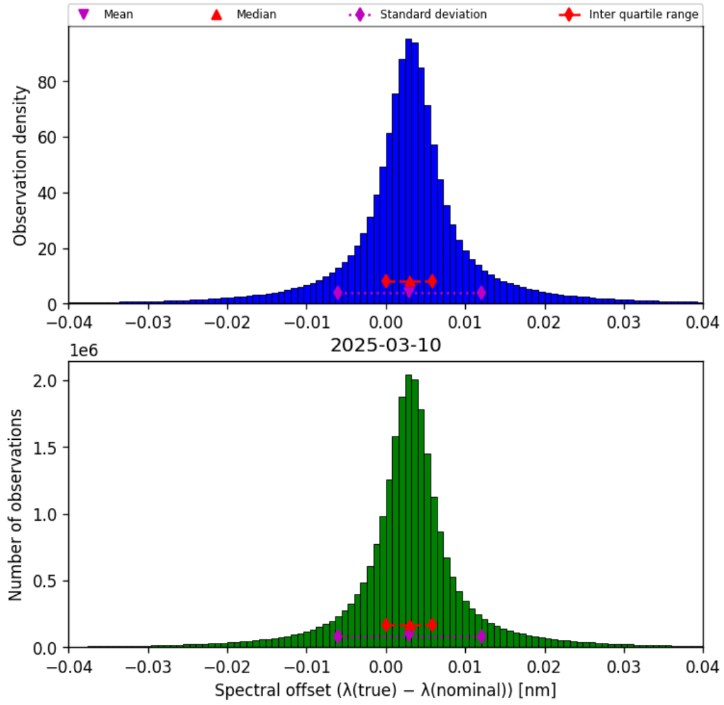
Figure 45: Histogram of “Spectral offset ( \lambda_{\text{true}} - \lambda_{\text{nominal}} )” for 2025-03-09 to 2025-03-11
