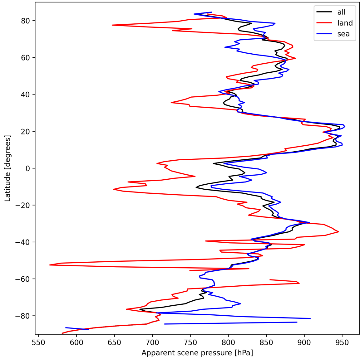
Figure 19: Zonal average of “Apparent scene pressure” for 2025-03-09 to 2025-03-11.
