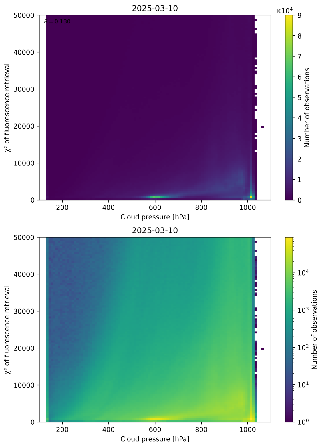
Figure 78: Scatter density plot of “Cloud pressure” against “ \chi^2 of fluorescence retrieval” for 2025-03-09 to 2025-03-11.
