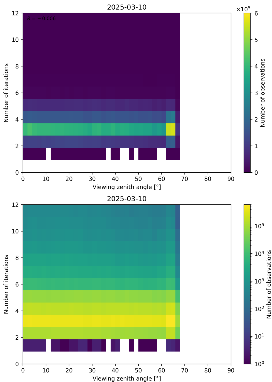
Figure 124: Scatter density plot of “Viewing zenith angle” against “Number of iterations” for 2025-03-09 to 2025-03-11.
