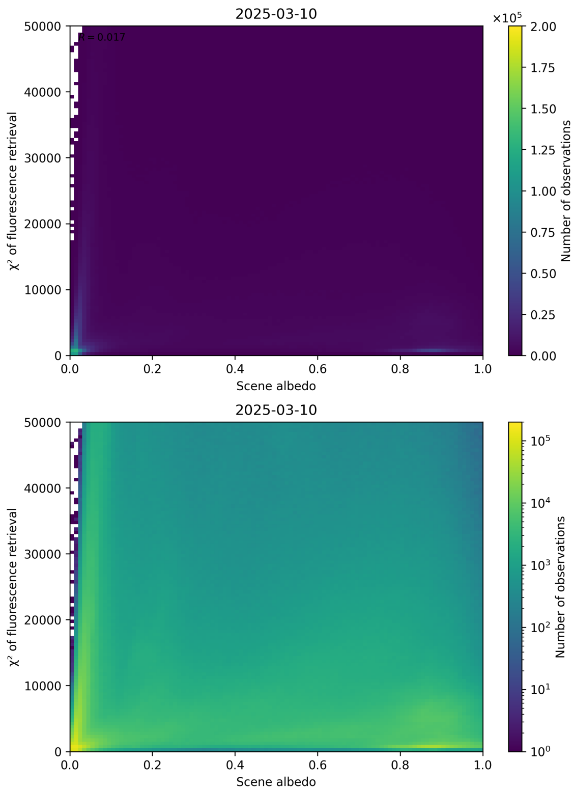
Figure 103: Scatter density plot of “Scene albedo” against “ \chi^2 of fluorescence retrieval” for 2025-03-09 to 2025-03-11.
