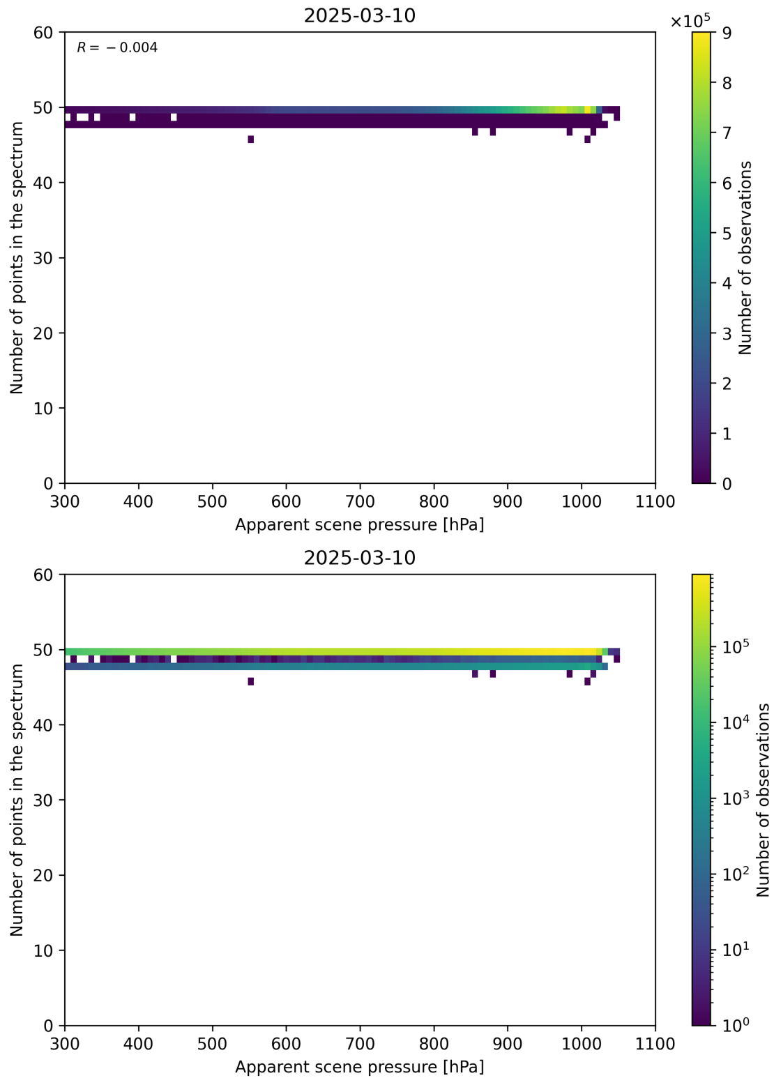
Figure 66: Scatter density plot of “Apparent scene pressure” against “Number of points in the spectrum” for 2025-03-09 to 2025-03-11.
