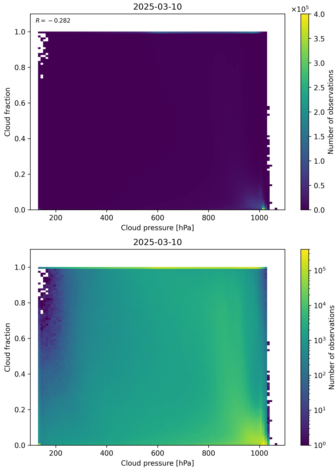
Figure 79: Scatter density plot of “Cloud pressure” against “Cloud fraction” for 2025-03-09 to 2025-03-11.
