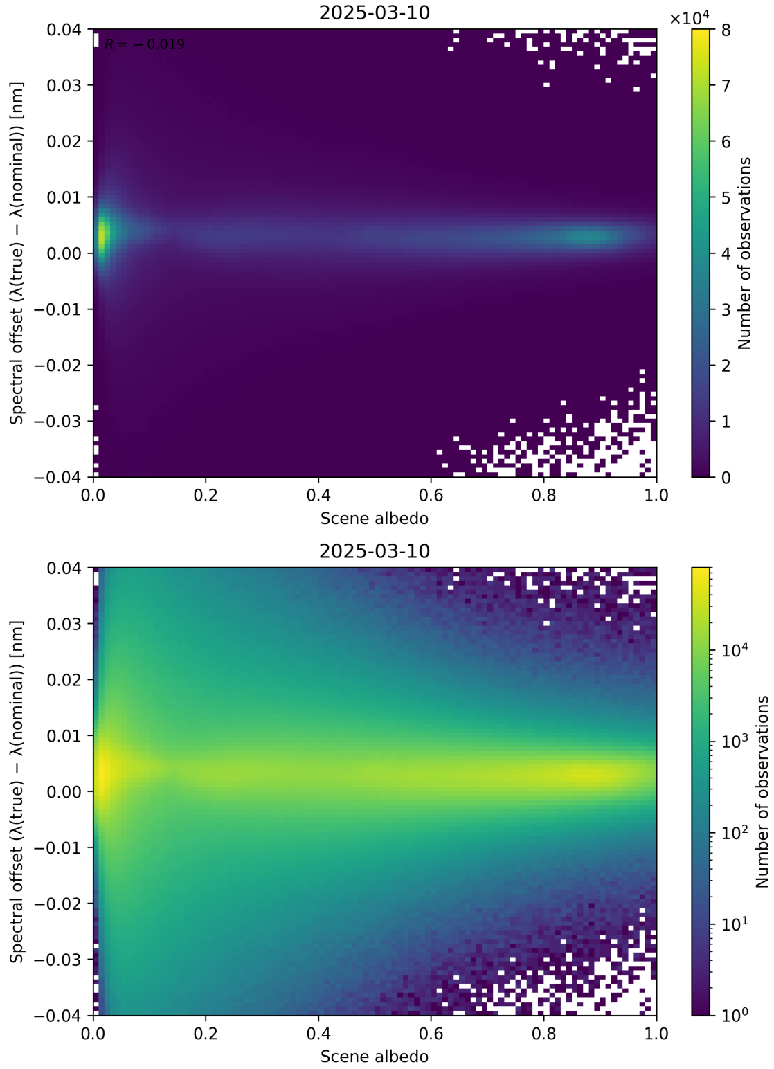
Figure 107: Scatter density plot of “Scene albedo” against “Spectral offset ( \lambda_{\text{true}} - \lambda_{\text{nominal}} )” for 2025-03-09 to 2025-03-11.
