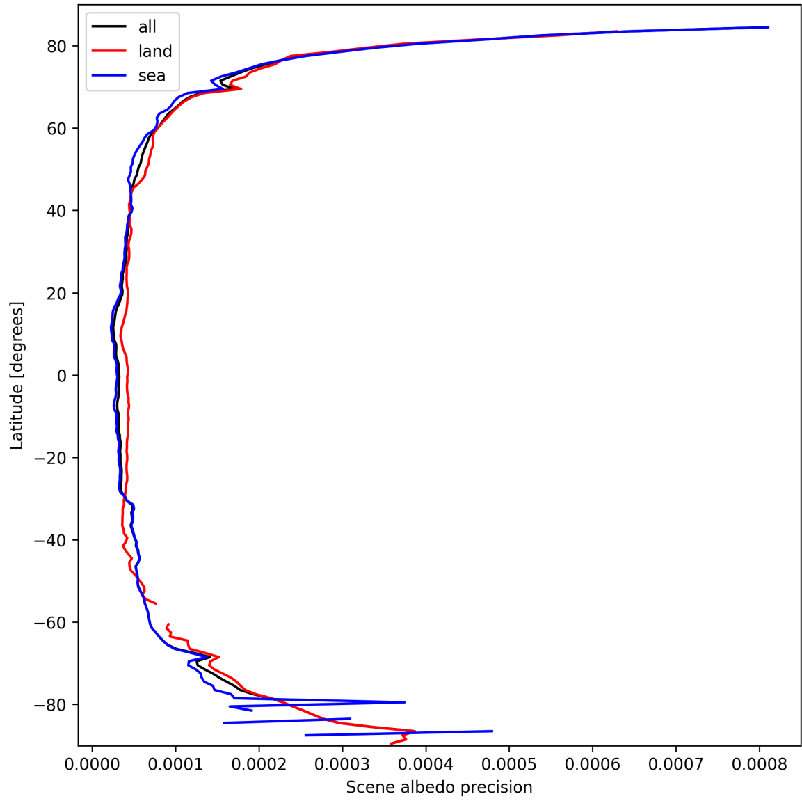
Figure 18: Zonal average of “Scene albedo precision” for 2025-03-09 to 2025-03-11.
