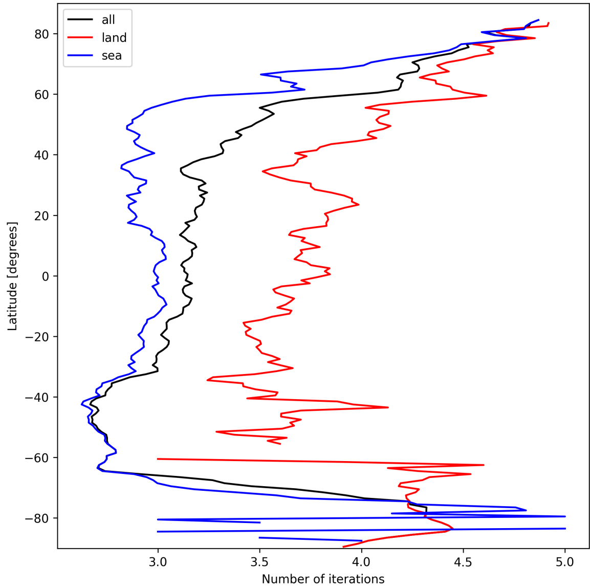
Figure 22: Zonal average of “Number of iterations” for 2025-03-09 to 2025-03-11.
