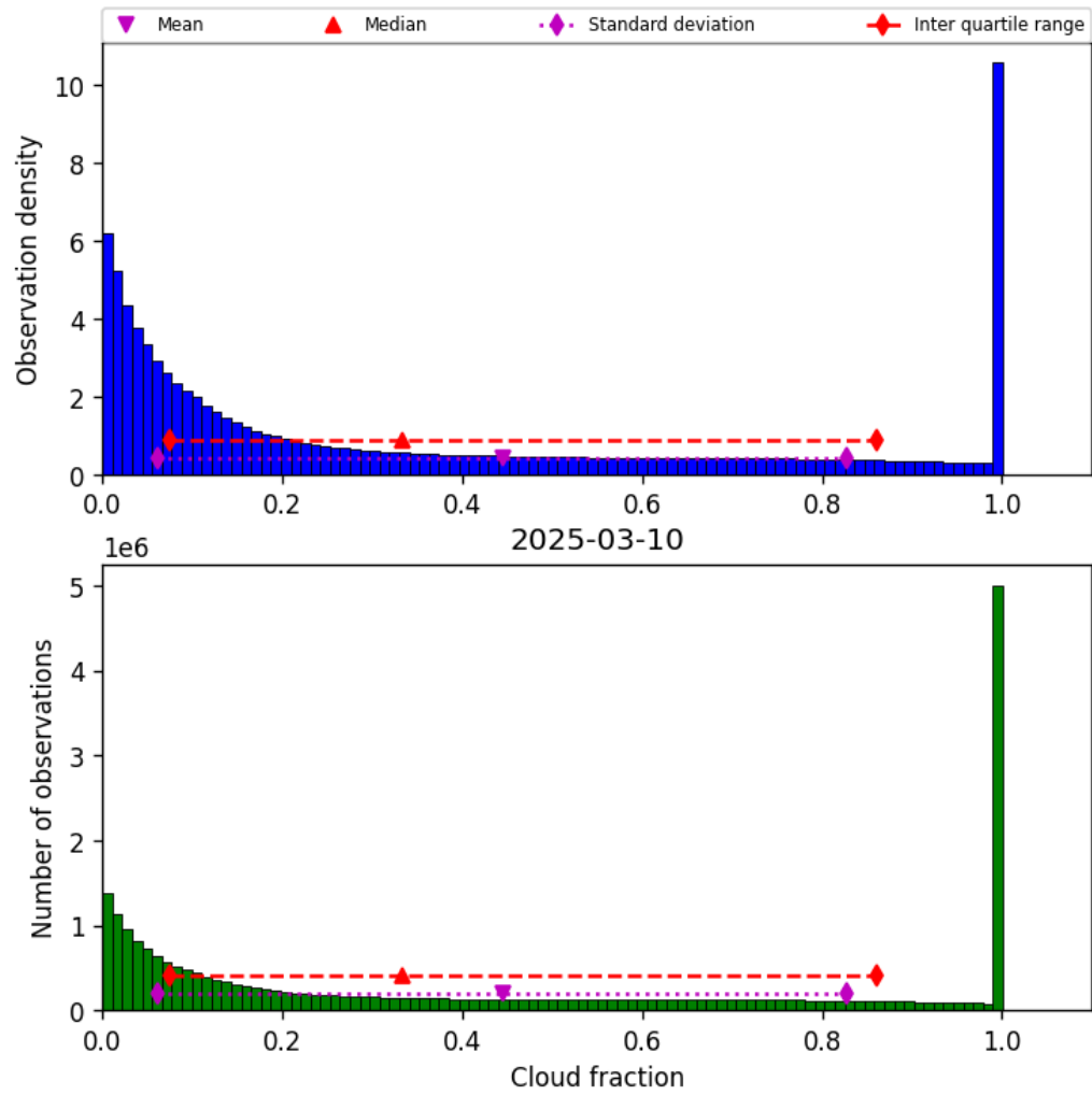
Figure 32: Histogram of “Cloud fraction” for 2025-03-09 to 2025-03-11
