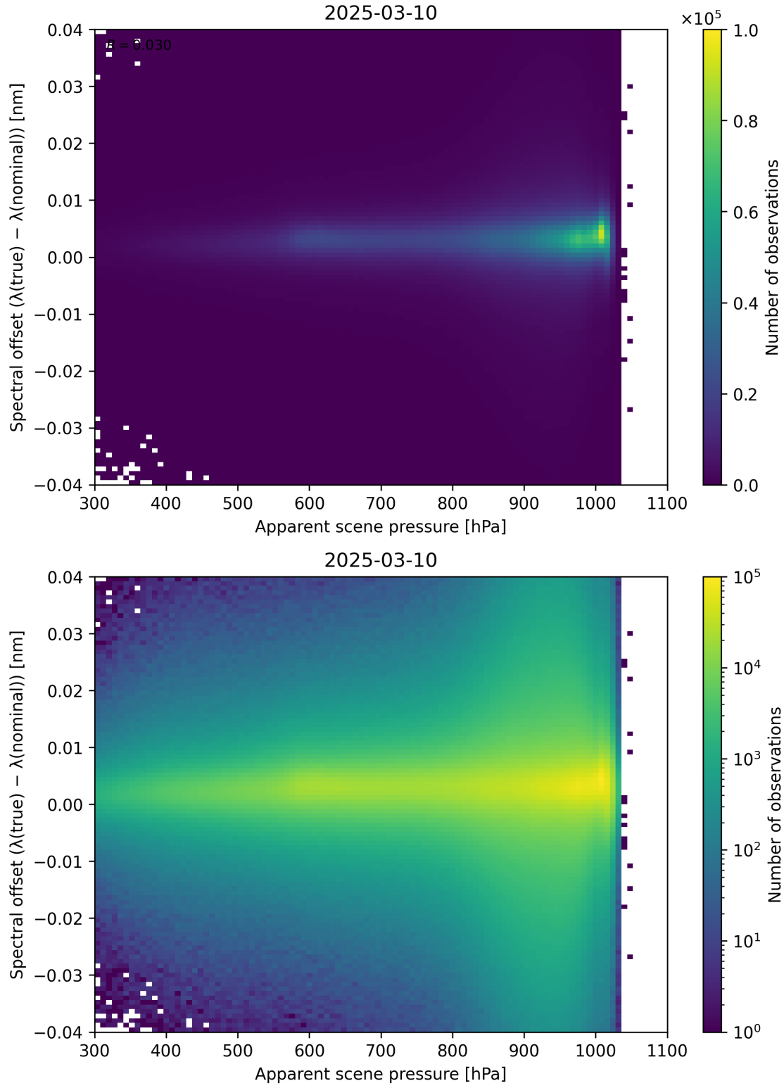
Figure 67: Scatter density plot of “Apparent scene pressure” against “Spectral offset ( \lambda_{\text{true}} - \lambda_{\text{nominal}} )” for 2025-03-09 to 2025-03-11.
