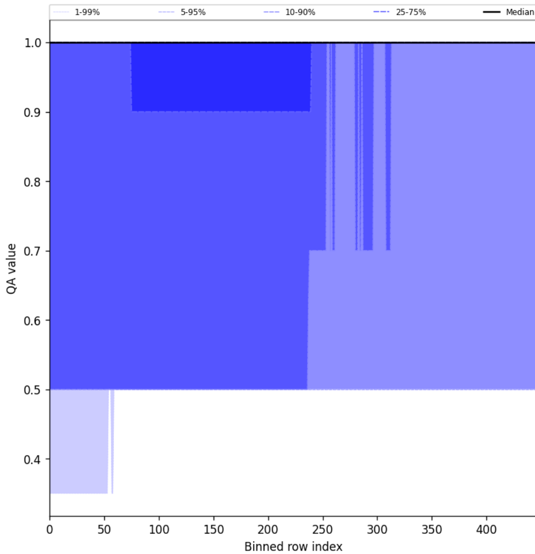
Figure 46: Along track statistics of “QA value” for 2025-03-09 to 2025-03-11
