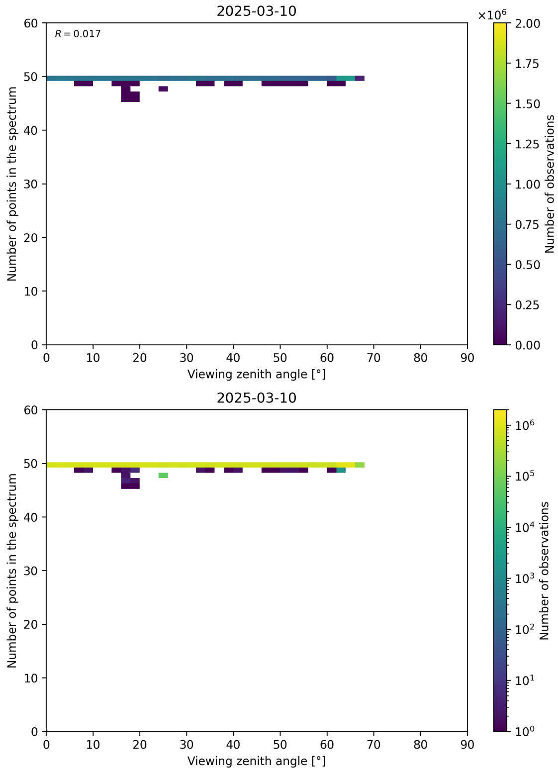
Figure 125: Scatter density plot of “Viewing zenith angle” against “Number of points in the spectrum” for 2025-03-09 to 2025-03-11.
