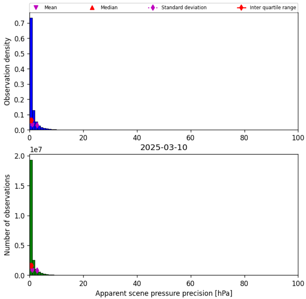
Figure 37: Histogram of “Apparent scene pressure precision” for 2025-03-09 to 2025-03-11
