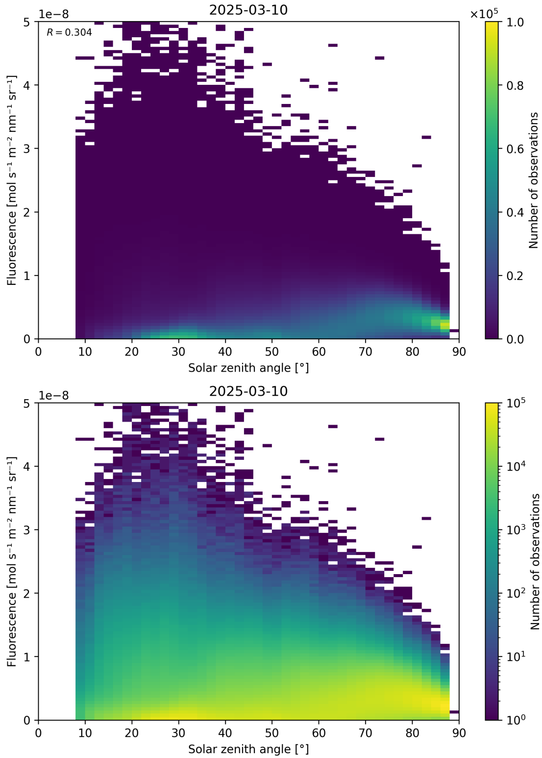
Figure 112: Scatter density plot of “Solar zenith angle” against “Fluorescence” for 2025-03-09 to 2025-03-11.
