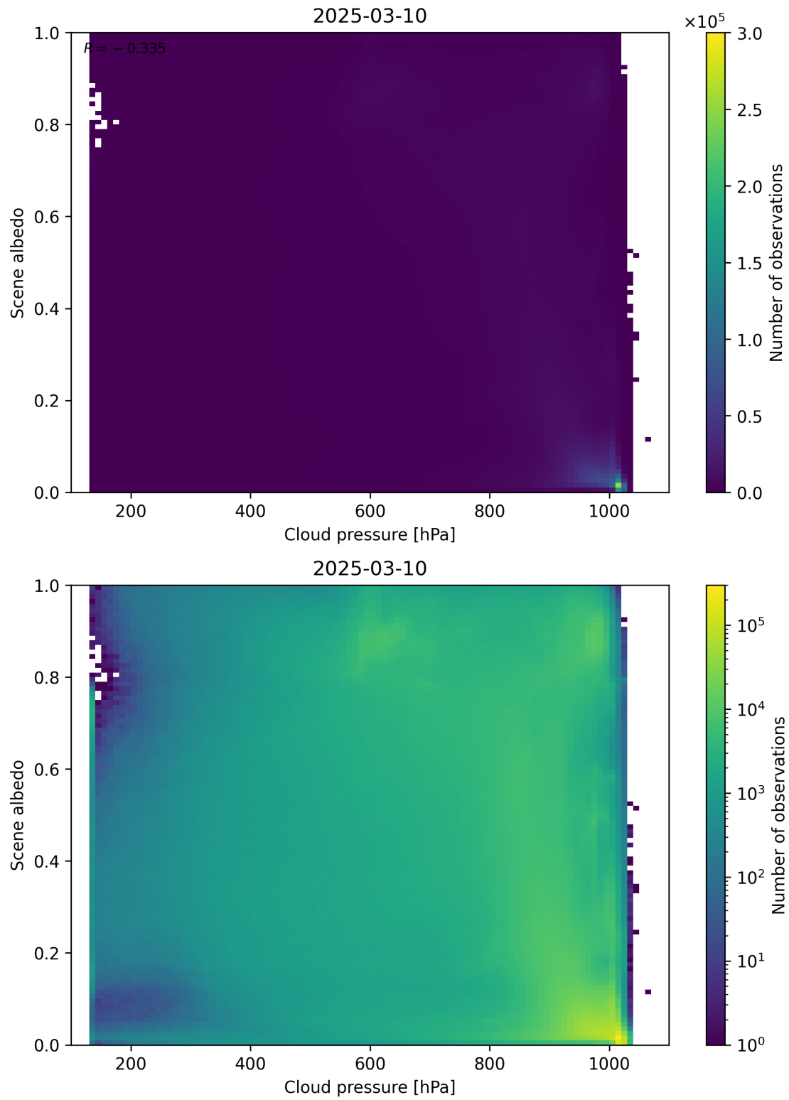
Figure 83: Scatter density plot of “Cloud pressure” against “Scene albedo” for 2025-03-09 to 2025-03-11.
