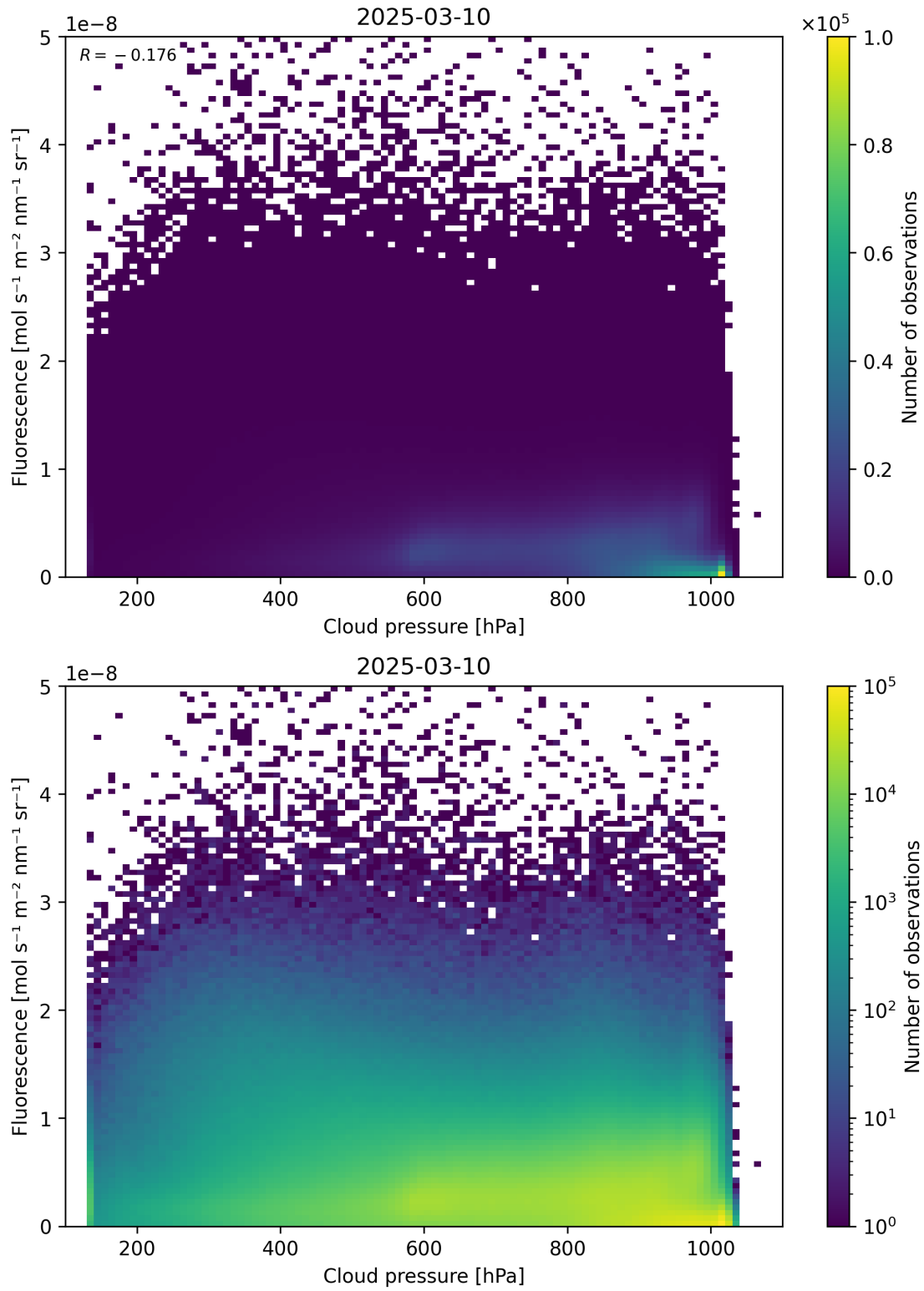
Figure 80: Scatter density plot of “Cloud pressure” against “Fluorescence” for 2025-03-09 to 2025-03-11.
