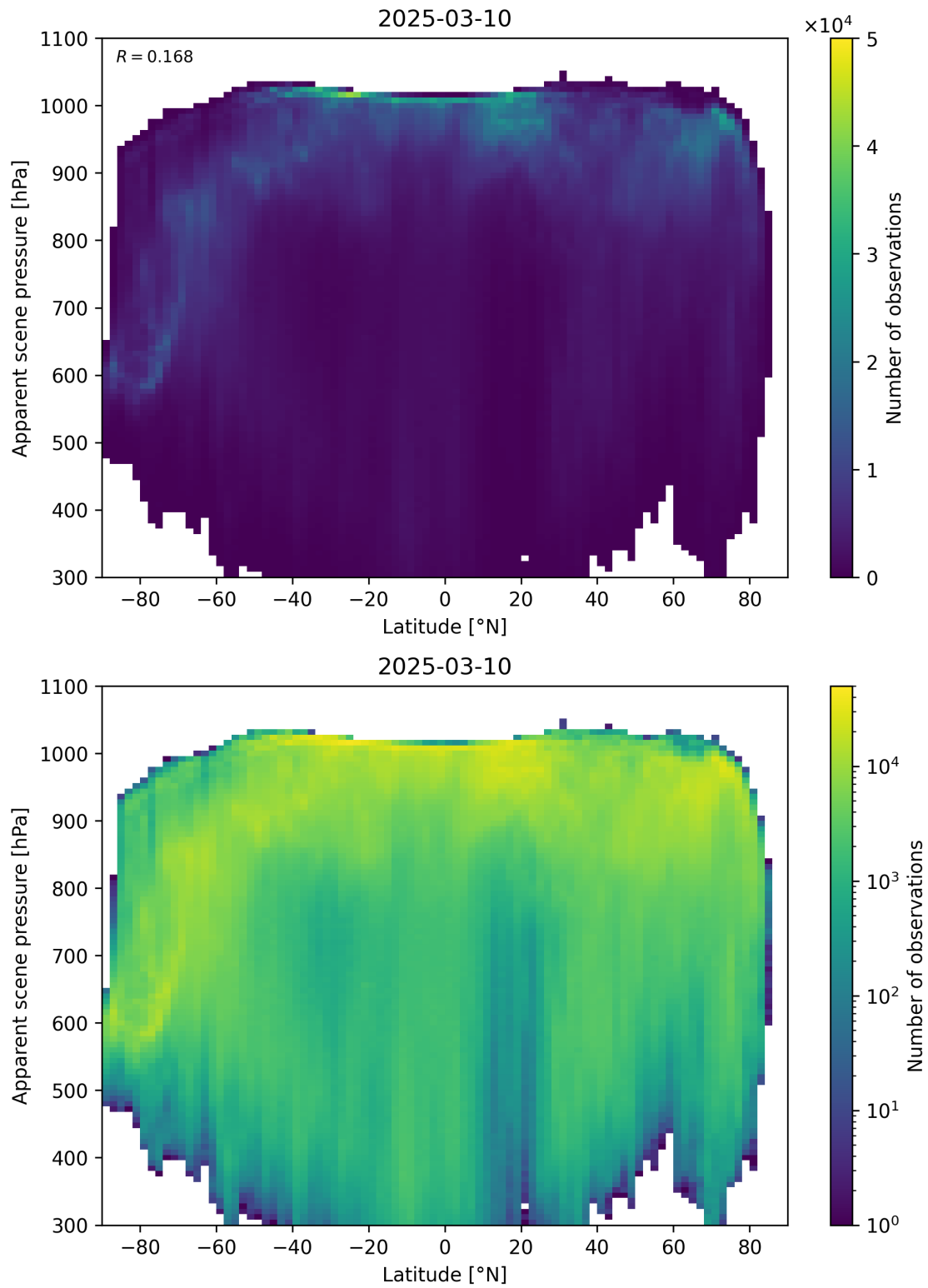
Figure 88: Scatter density plot of “Latitude” against “Apparent scene pressure” for 2025-03-09 to 2025-03-11.
