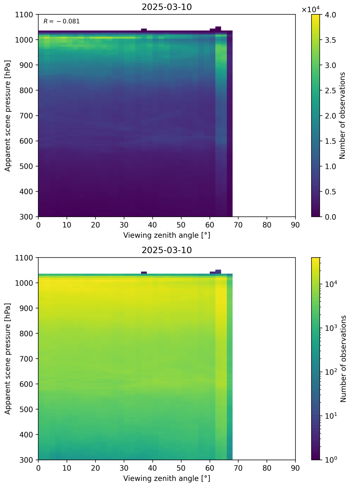
Figure 118: Scatter density plot of “Viewing zenith angle” against “Apparent scene pressure” for 2025-03-09 to 2025-03-11.
