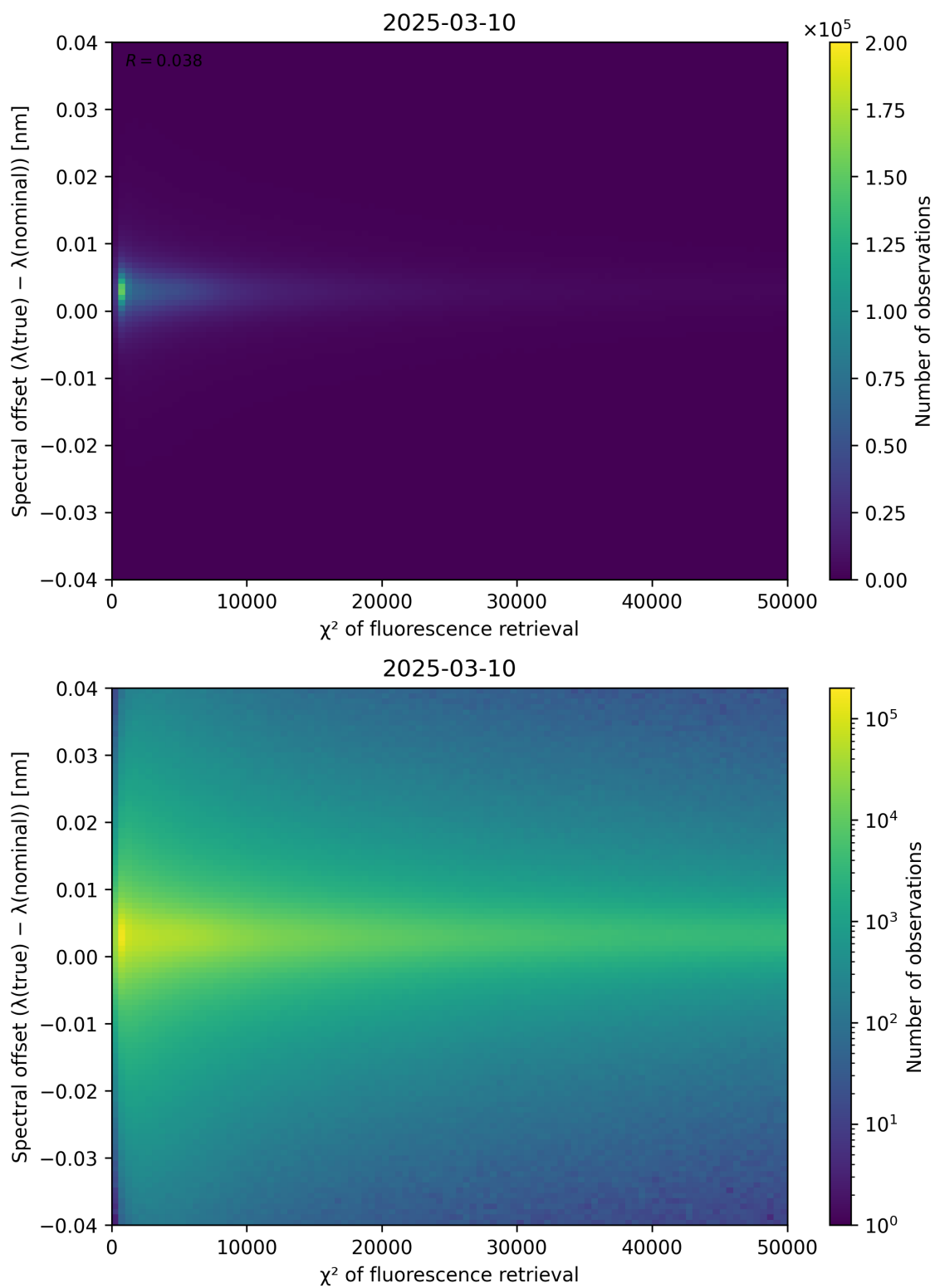
Figure 69: Scatter density plot of “ \chi^2 of fluorescence retrieval” against “Spectral offset ( \lambda_{\text{true}} - \lambda_{\text{nominal}} )” for 2025-03-09 to 2025-03-11.
