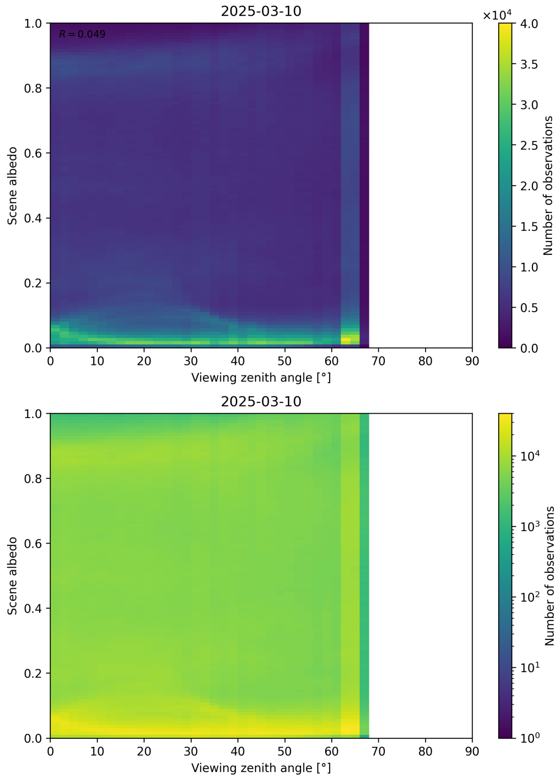
Figure 126: Scatter density plot of “Viewing zenith angle” against “Scene albedo” for 2025-03-09 to 2025-03-11.
