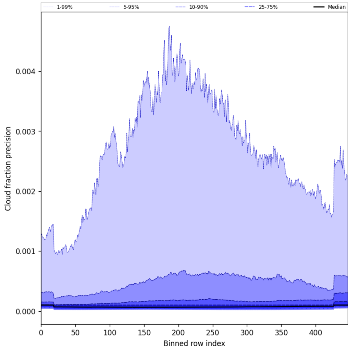
Figure 50: Along track statistics of “Cloud fraction precision” for 2025-03-09 to 2025-03-11
