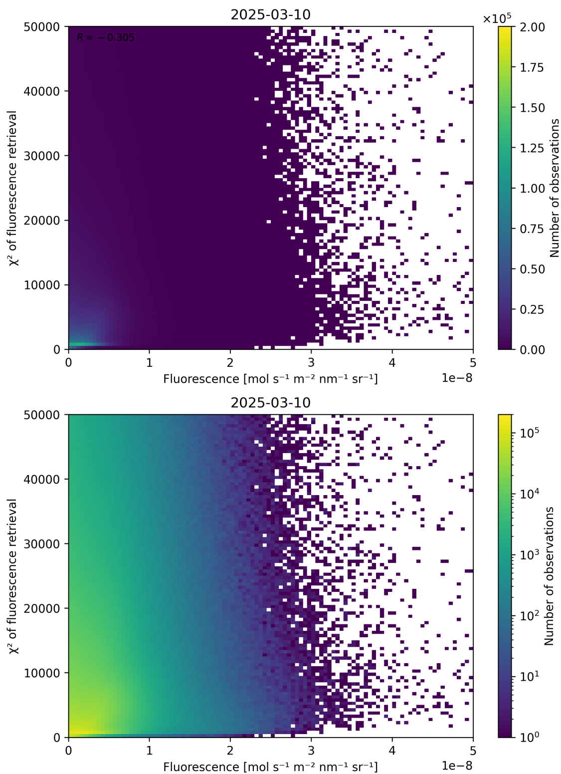
Figure 85: Scatter density plot of “Fluorescence” against “ \chi^2 of fluorescence retrieval” for 2025-03-09 to 2025-03-11.
