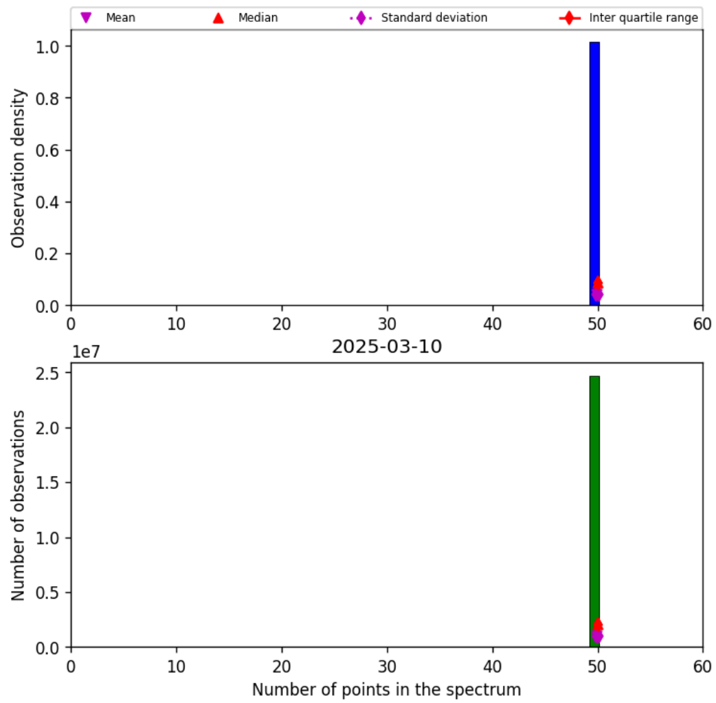
Figure 44: Histogram of "Number of points in the spectrum" for 2025-03-09 to 2025-03-11
