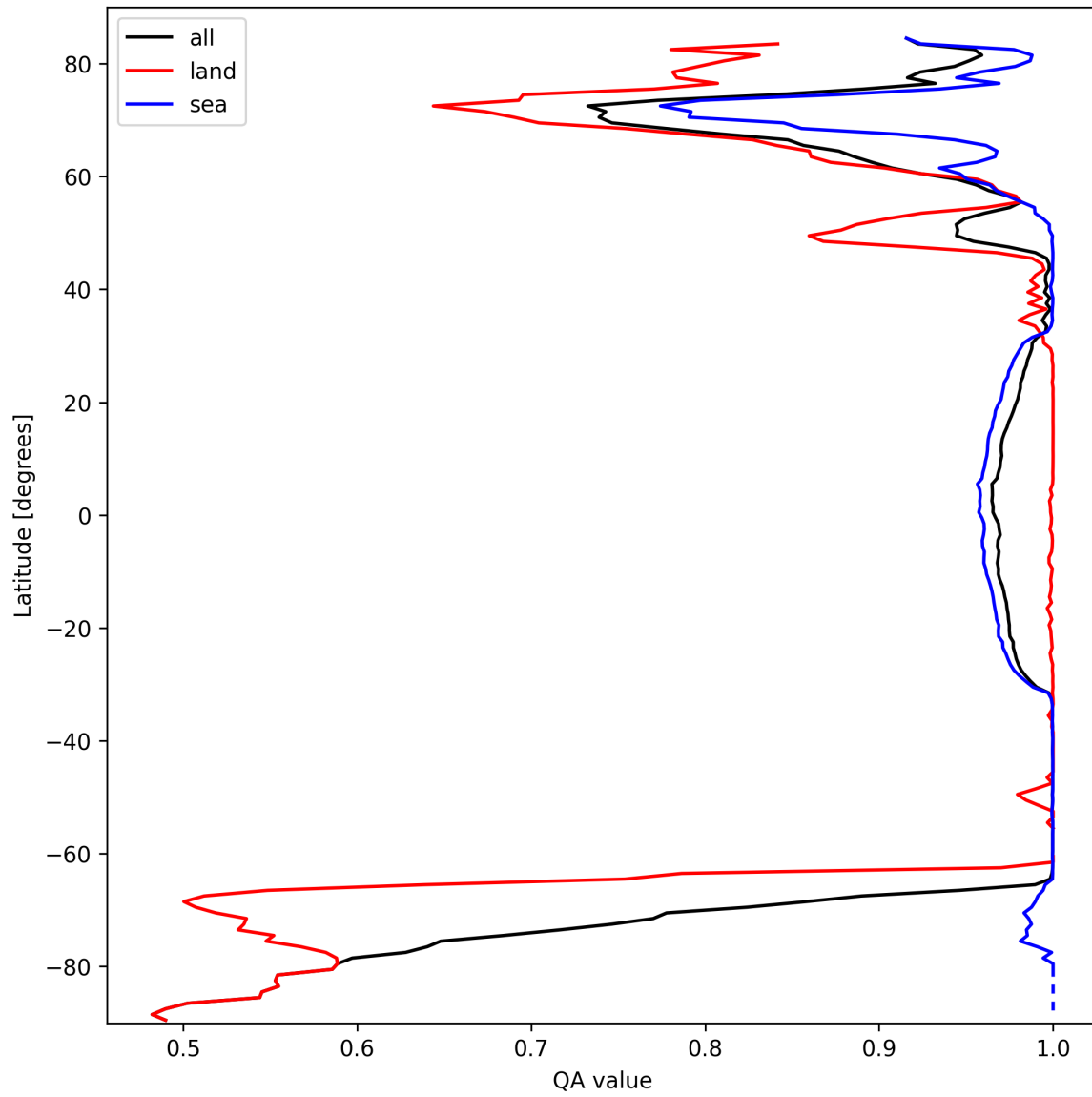
Figure 12: Zonal average of “QA value” for 2025-03-09 to 2025-03-11.
