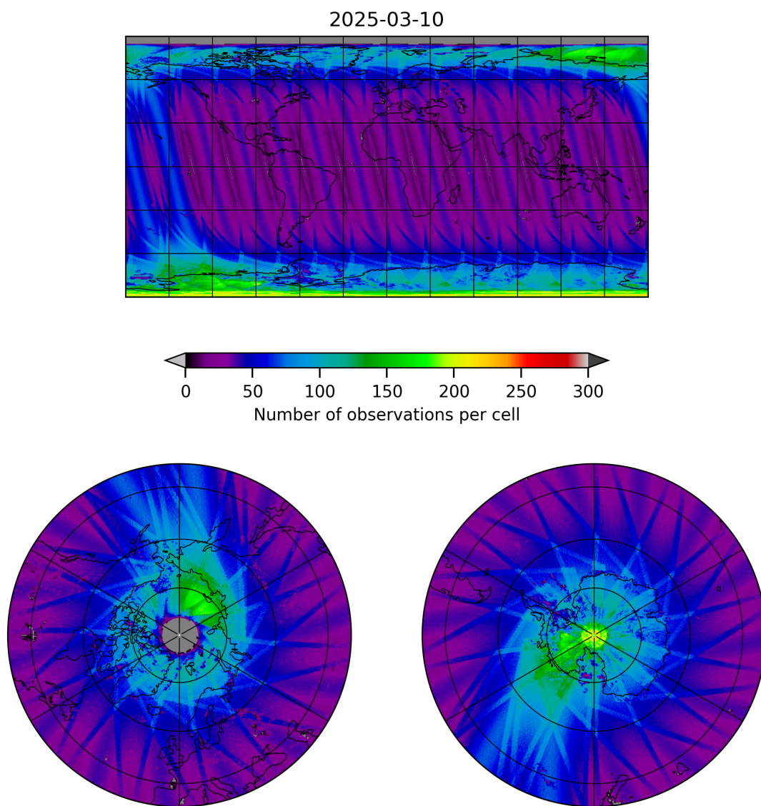
Figure 11: Map of the number of observations for 2025-03-09 to 2025-03-11
