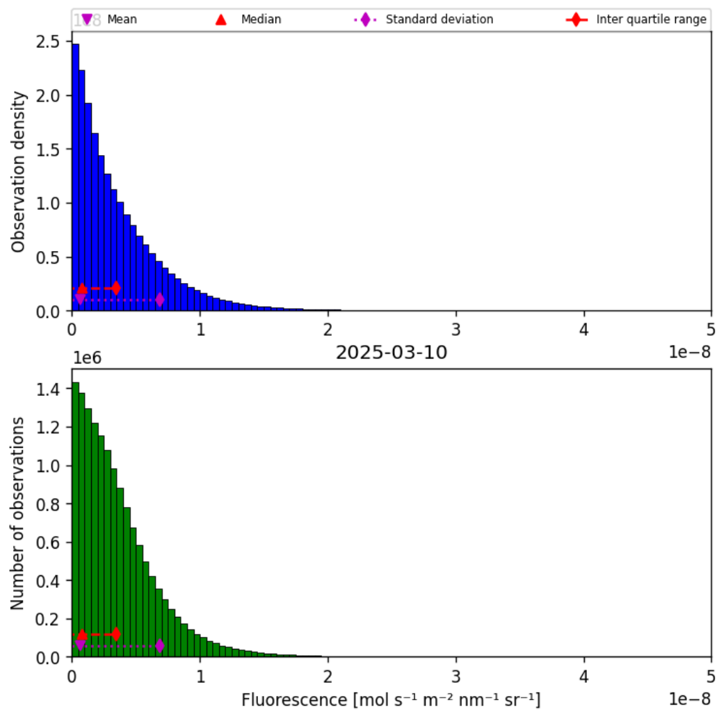
Figure 40: Histogram of “Fluorescence” for 2025-03-09 to 2025-03-11
