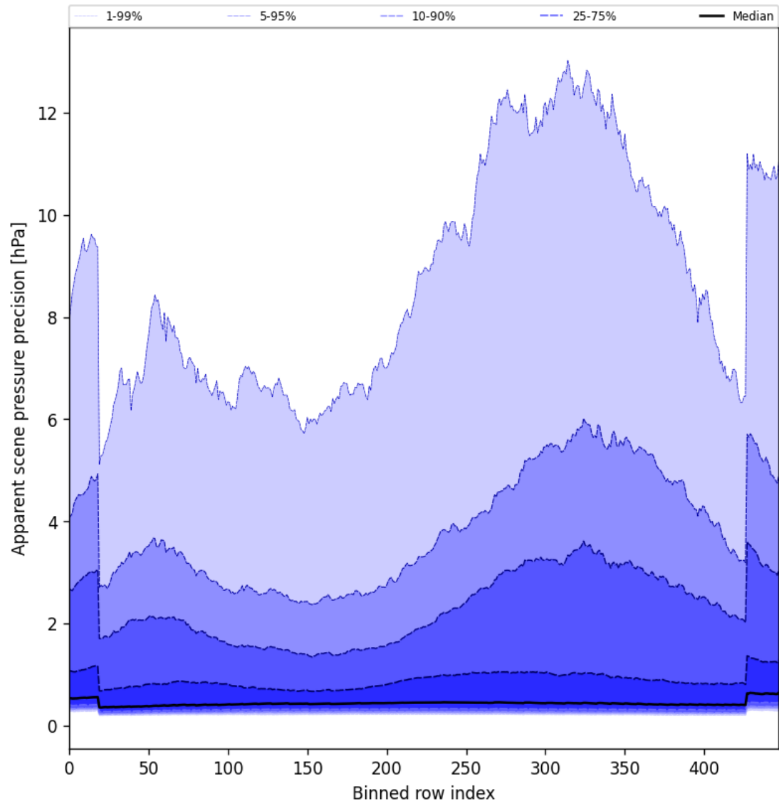
Figure 54: Along track statistics of “Apparent scene pressure precision” for 2025-03-09 to 2025-03-11
