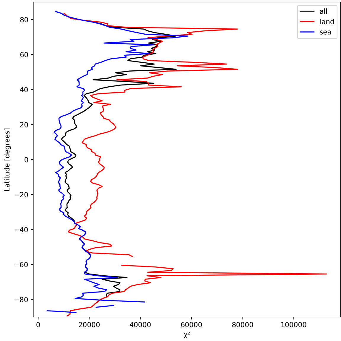
Figure 21: Zonal average of “ \chi^2 ” for 2025-03-09 to 2025-03-11.
