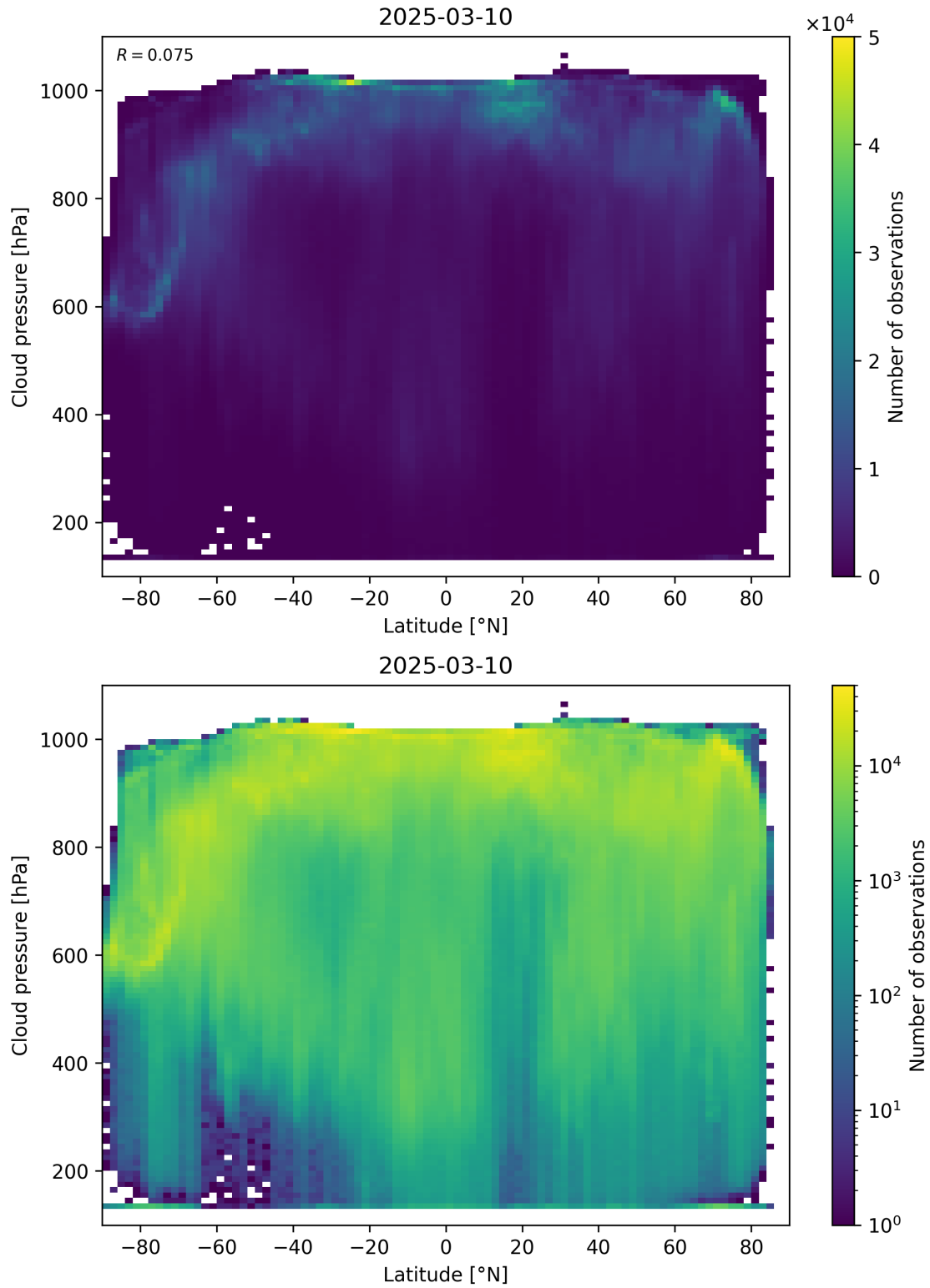
Figure 91: Scatter density plot of “Latitude” against “Cloud pressure” for 2025-03-09 to 2025-03-11.
