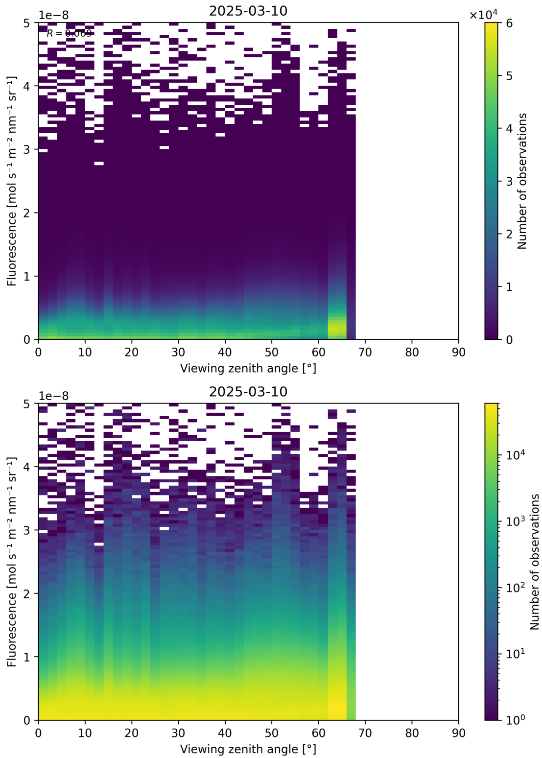
Figure 122: Scatter density plot of “Viewing zenith angle” against “Fluorescence” for 2025-03-09 to 2025-03-11.
