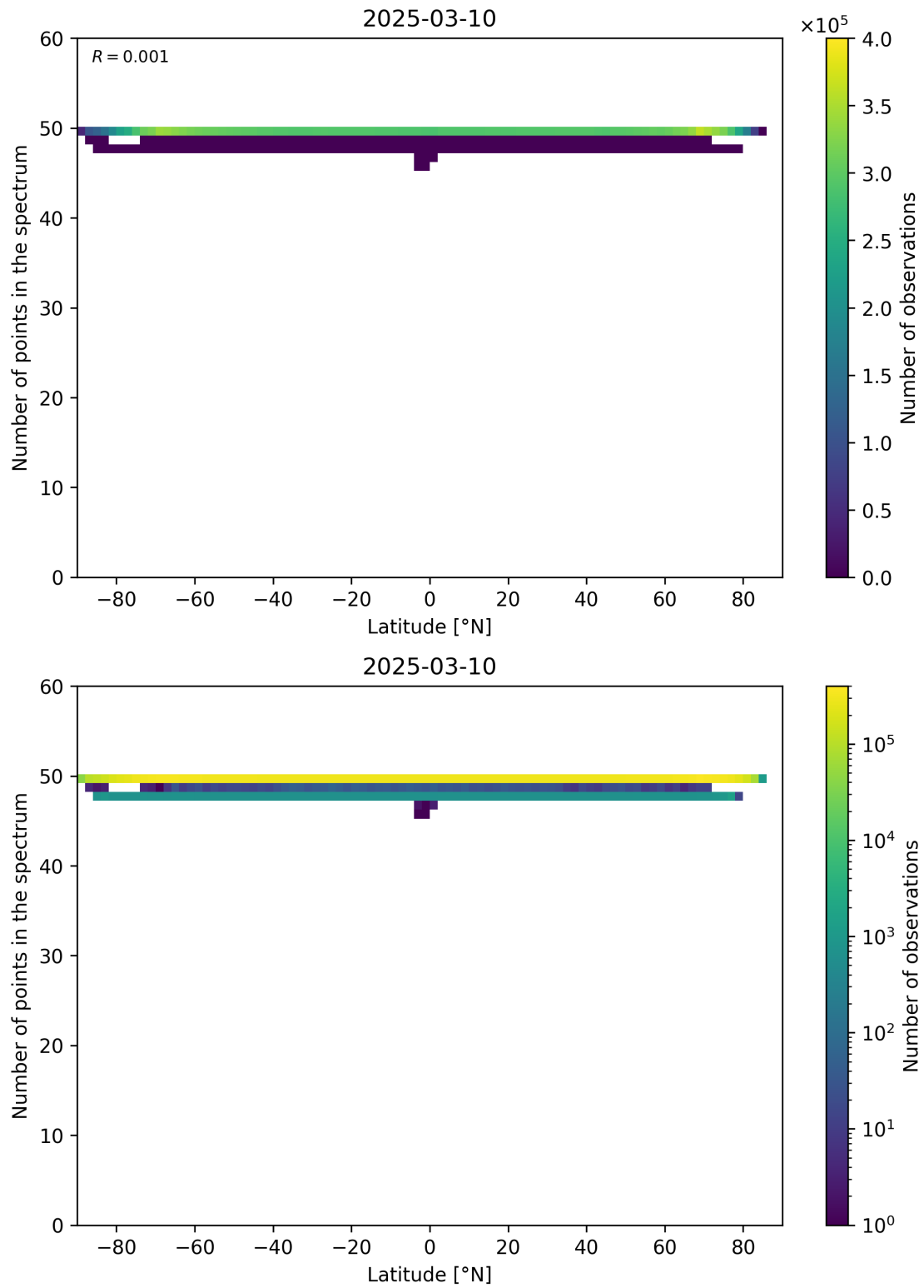
Figure 94: Scatter density plot of “Latitude” against “Number of points in the spectrum” for 2025-03-09 to 2025-03-11.
