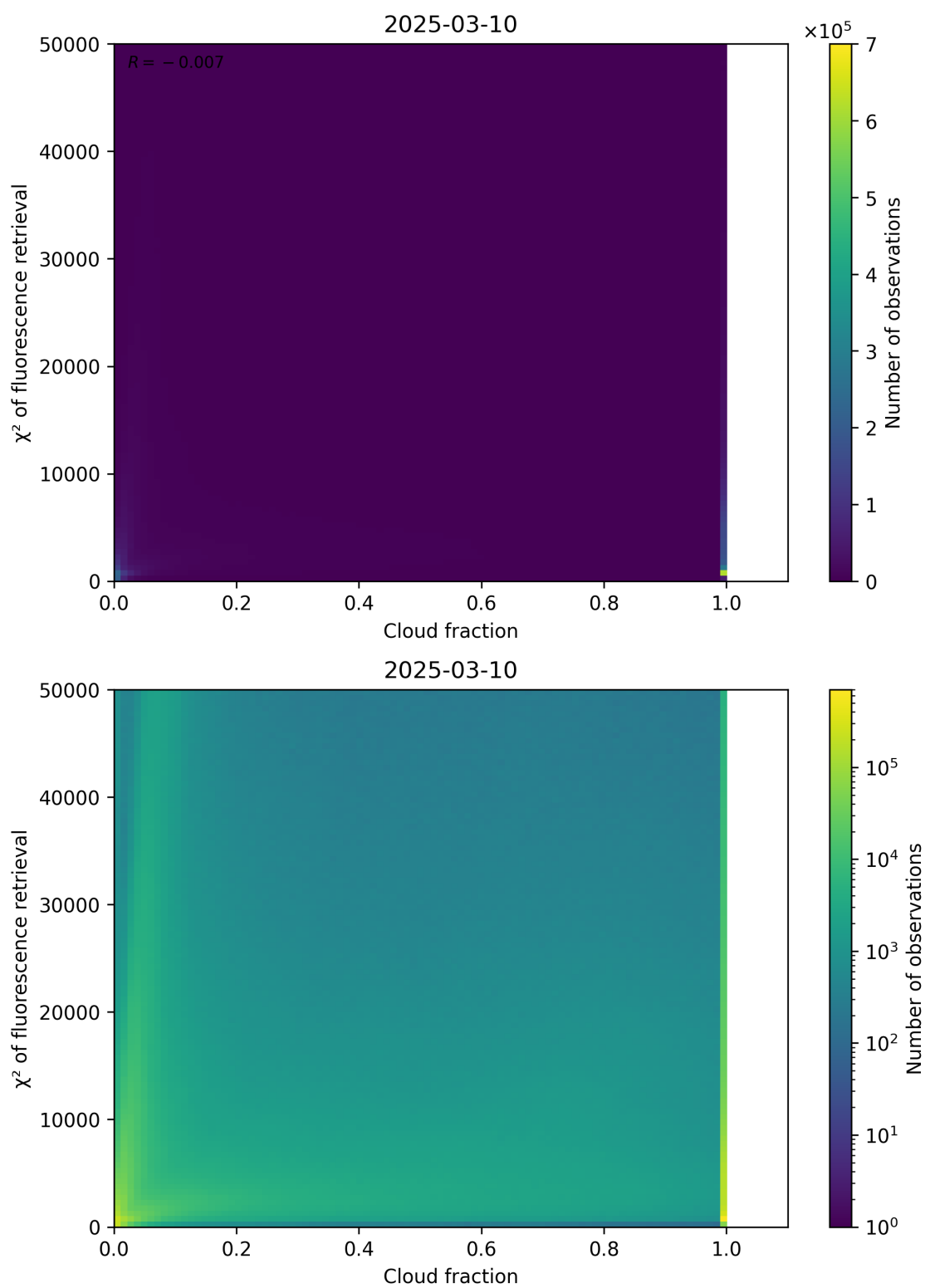
Figure 71: Scatter density plot of “Cloud fraction” against “ \chi^2 of fluorescence retrieval” for 2025-03-09 to 2025-03-11.
