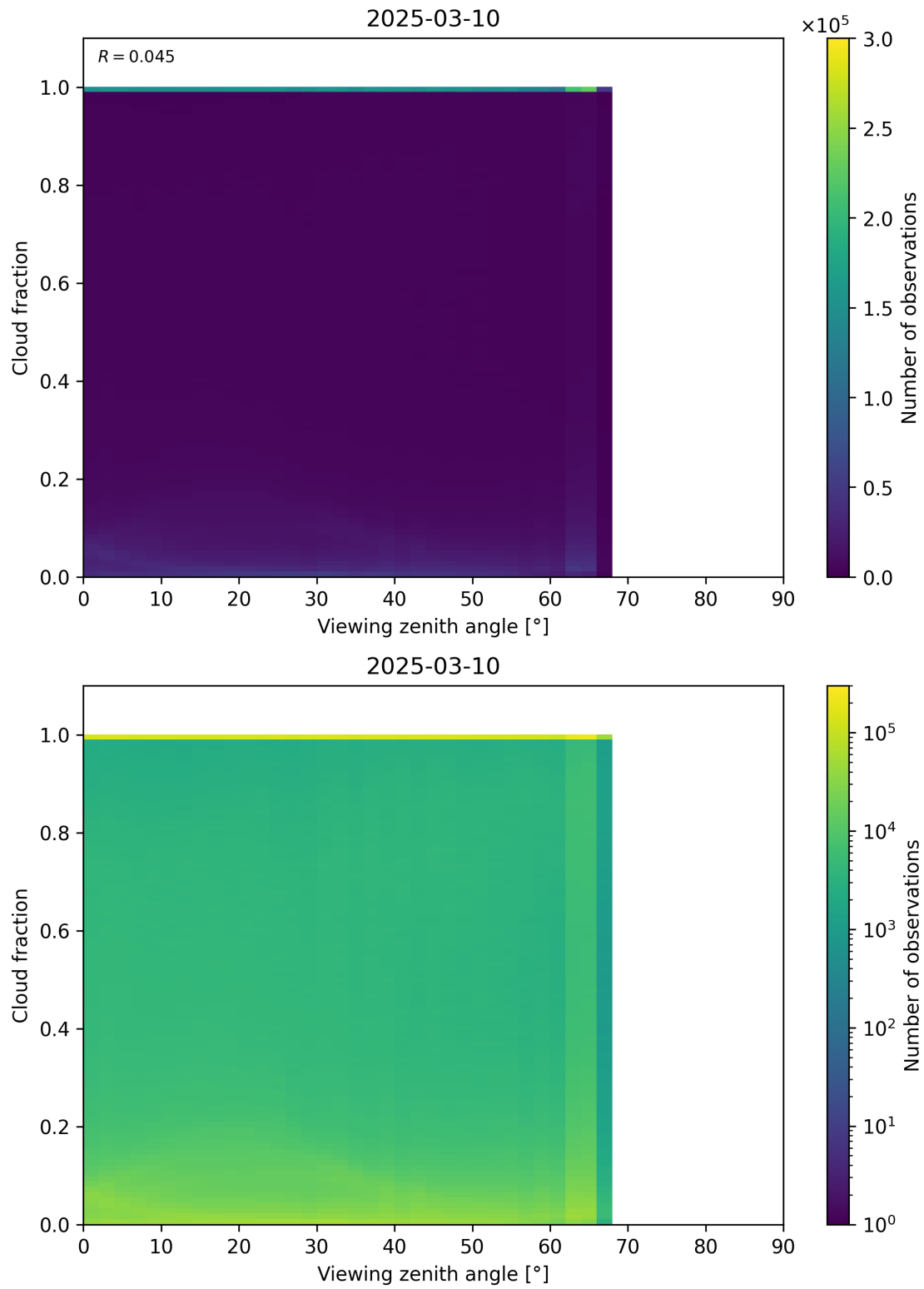
Figure 120: Scatter density plot of “Viewing zenith angle” against “Cloud fraction” for 2025-03-09 to 2025-03-11.
