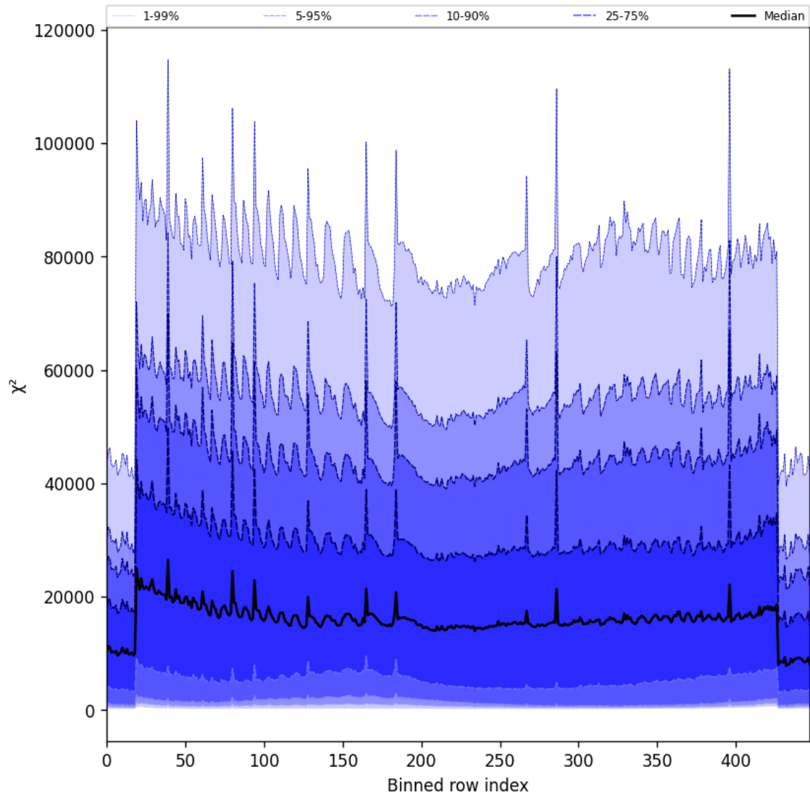
Figure 55: Along track statistics of “ \chi^2 ” for 2025-03-09 to 2025-03-11
