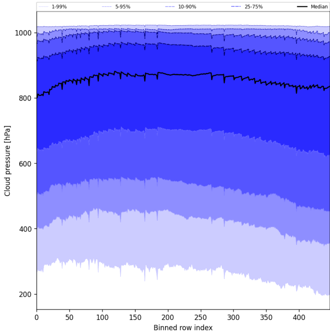
Figure 47: Along track statistics of “Cloud pressure” for 2025-03-09 to 2025-03-11
