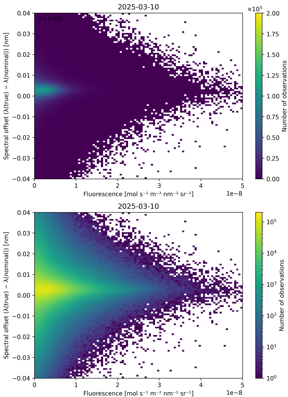
Figure 87: Scatter density plot of “Fluorescence” against “Spectral offset ( \lambda_{\text{true}} - \lambda_{\text{nominal}} )” for 2025-03-09 to 2025-03-11.
