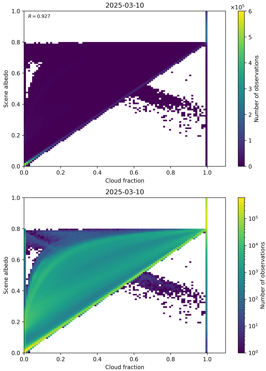
Figure 75: Scatter density plot of “Cloud fraction” against “Scene albedo” for 2025-03-09 to 2025-03-11.
