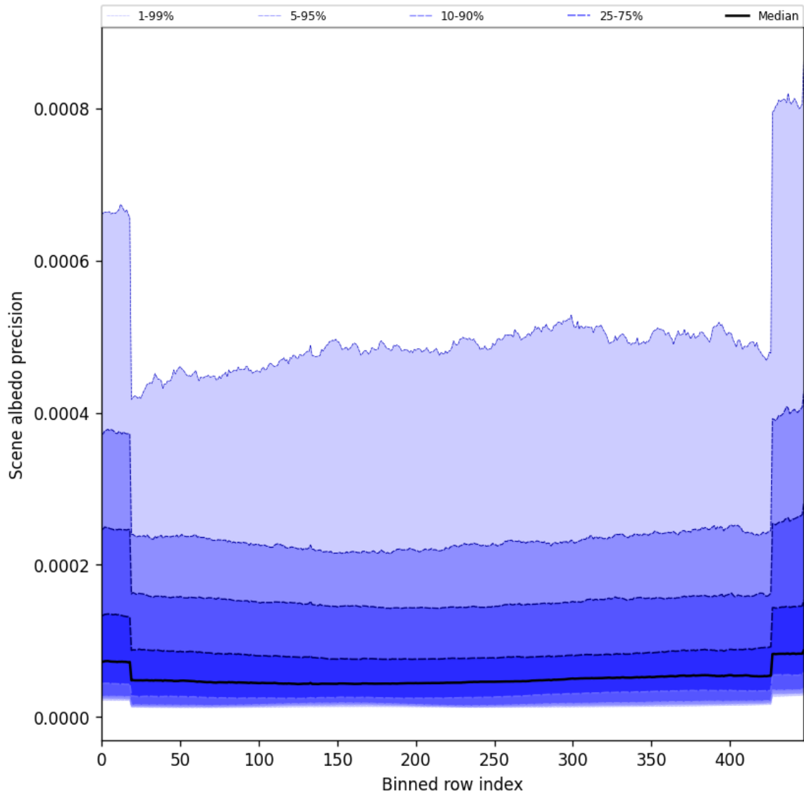
Figure 52: Along track statistics of “Scene albedo precision” for 2025-03-09 to 2025-03-11
