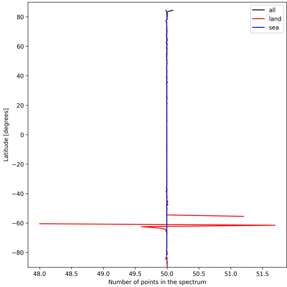
Figure 27: Zonal average of “Number of points in the spectrum” for 2025-03-09 to 2025-03-11.
