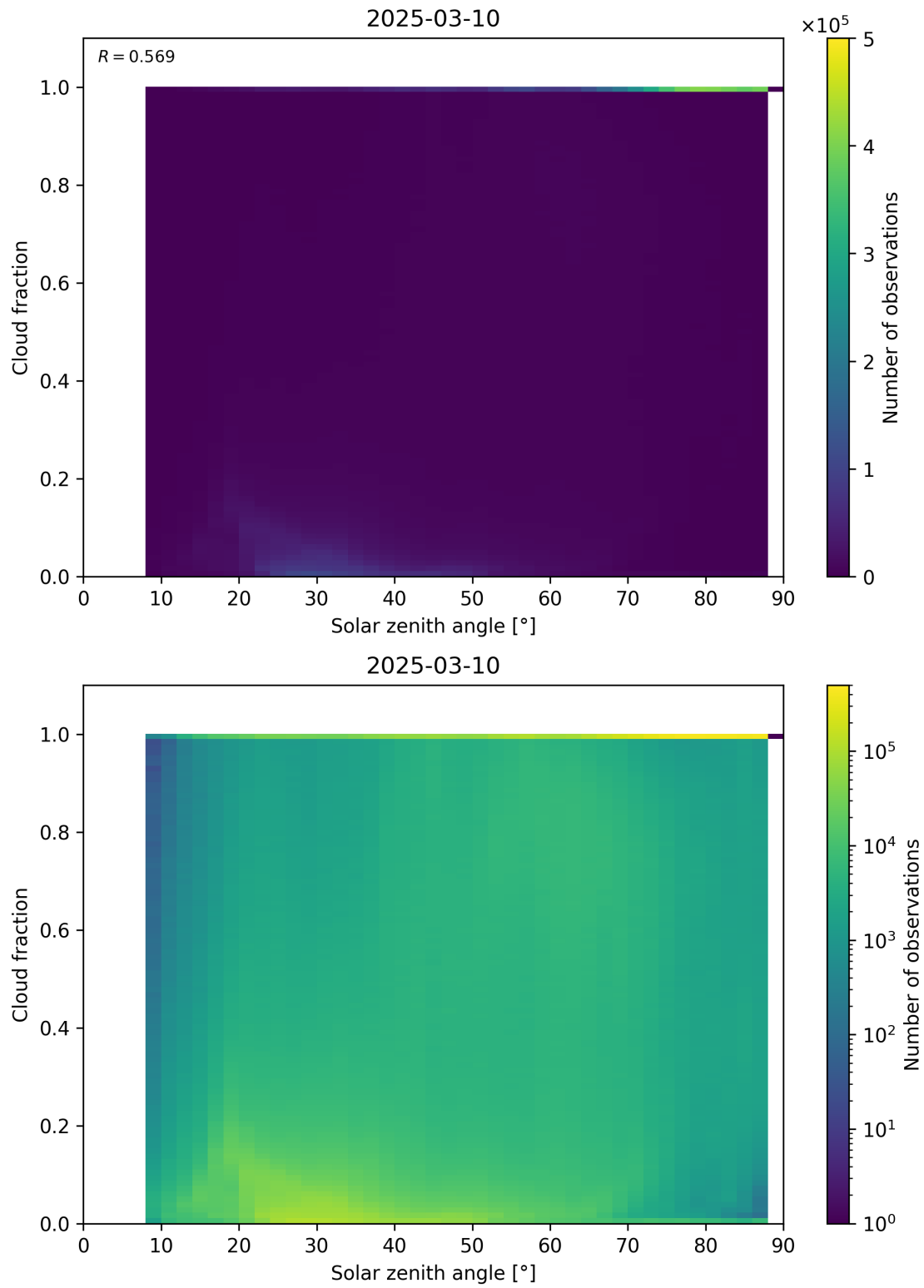
Figure 110: Scatter density plot of “Solar zenith angle” against “Cloud fraction” for 2025-03-09 to 2025-03-11.
