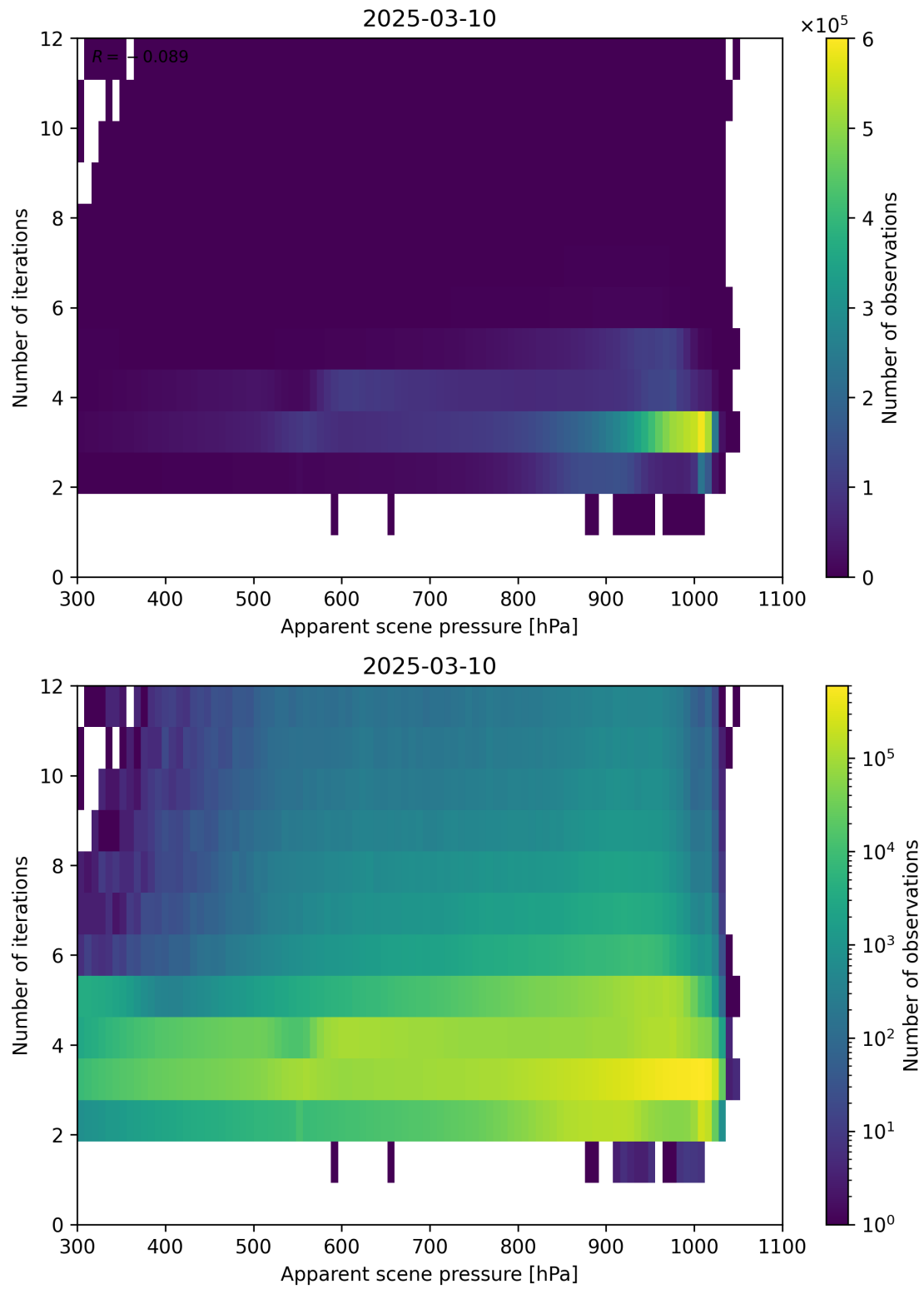
Figure 65: Scatter density plot of “Apparent scene pressure” against “Number of iterations” for 2025-03-09 to 2025-03-11.
