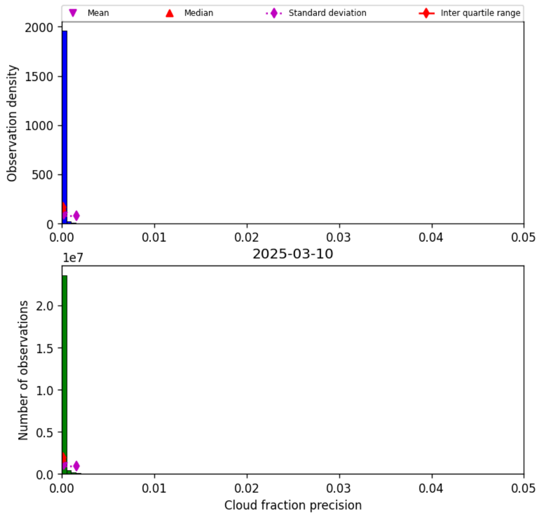
Figure 33: Histogram of “Cloud fraction precision” for 2025-03-09 to 2025-03-11
