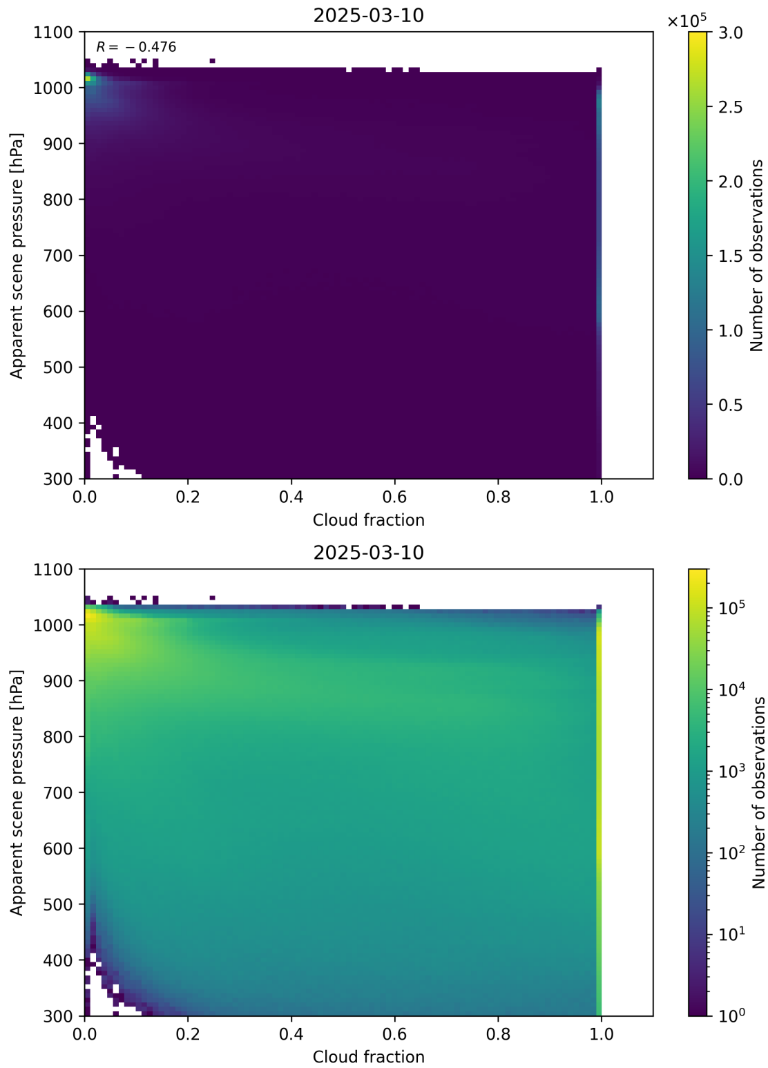
Figure 70: Scatter density plot of “Cloud fraction” against “Apparent scene pressure” for 2025-03-09 to 2025-03-11.
