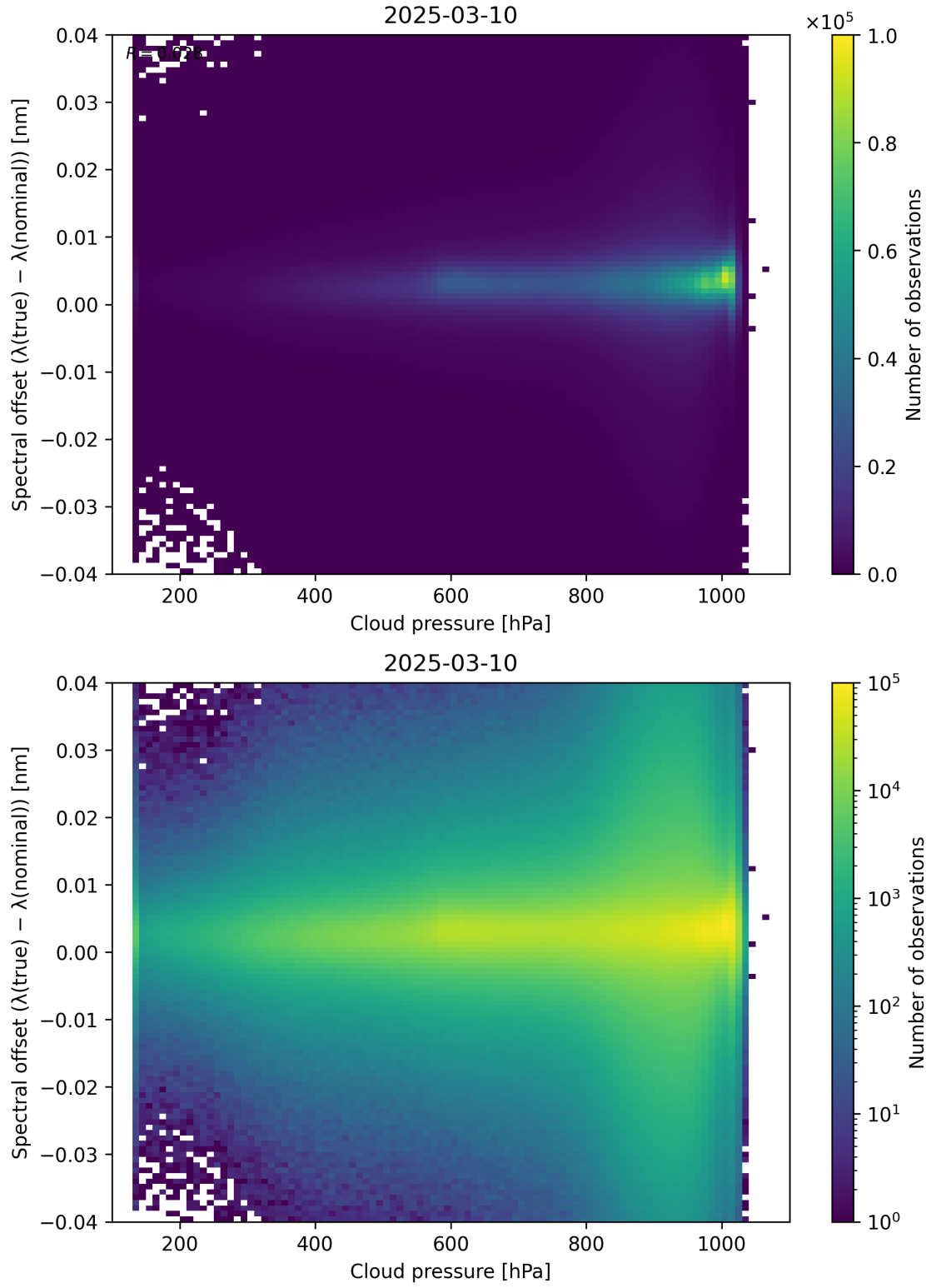
Figure 84: Scatter density plot of “Cloud pressure” against “Spectral offset ( \lambda_{\text{true}} - \lambda_{\text{nominal}} )” for 2025-03-09 to 2025-03-11.
