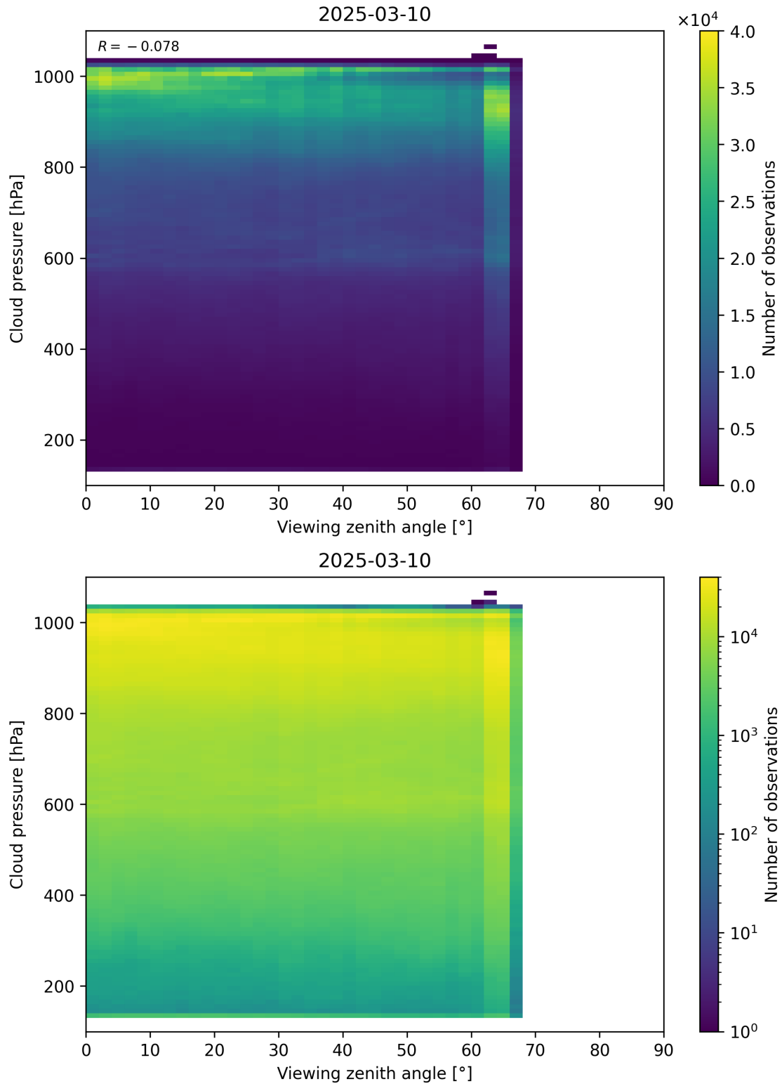
Figure 121: Scatter density plot of “Viewing zenith angle” against “Cloud pressure” for 2025-03-09 to 2025-03-11.
