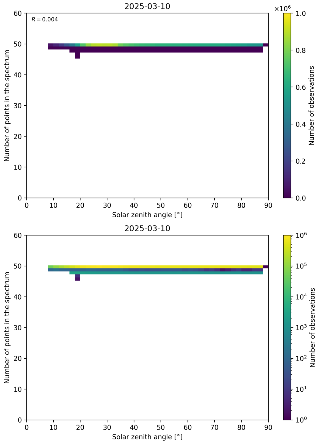
Figure 115: Scatter density plot of “Solar zenith angle” against “Number of points in the spectrum” for 2025-03-09 to 2025-03-11.
