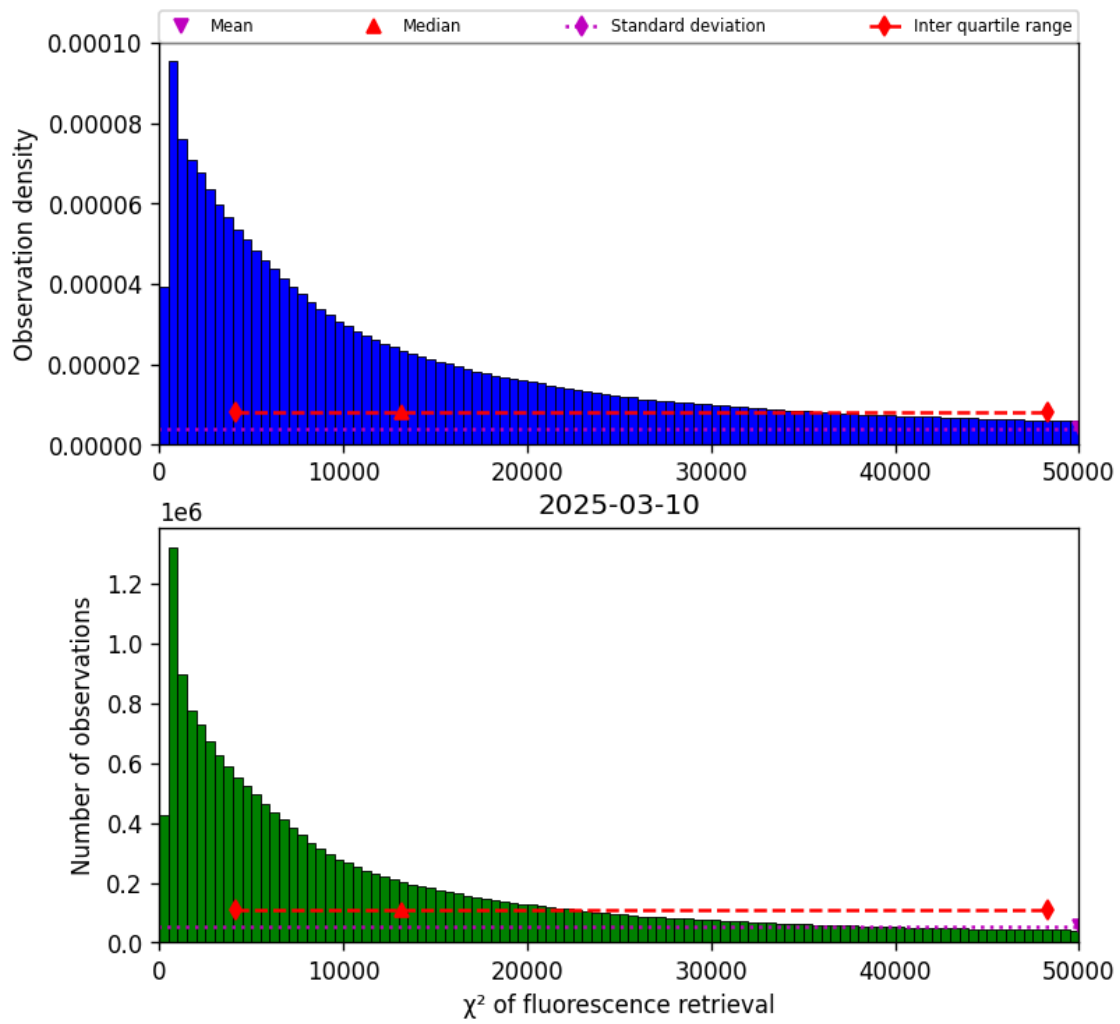
Figure 42: Histogram of “ \chi^2 of fluorescence retrieval” for 2025-03-09 to 2025-03-11
