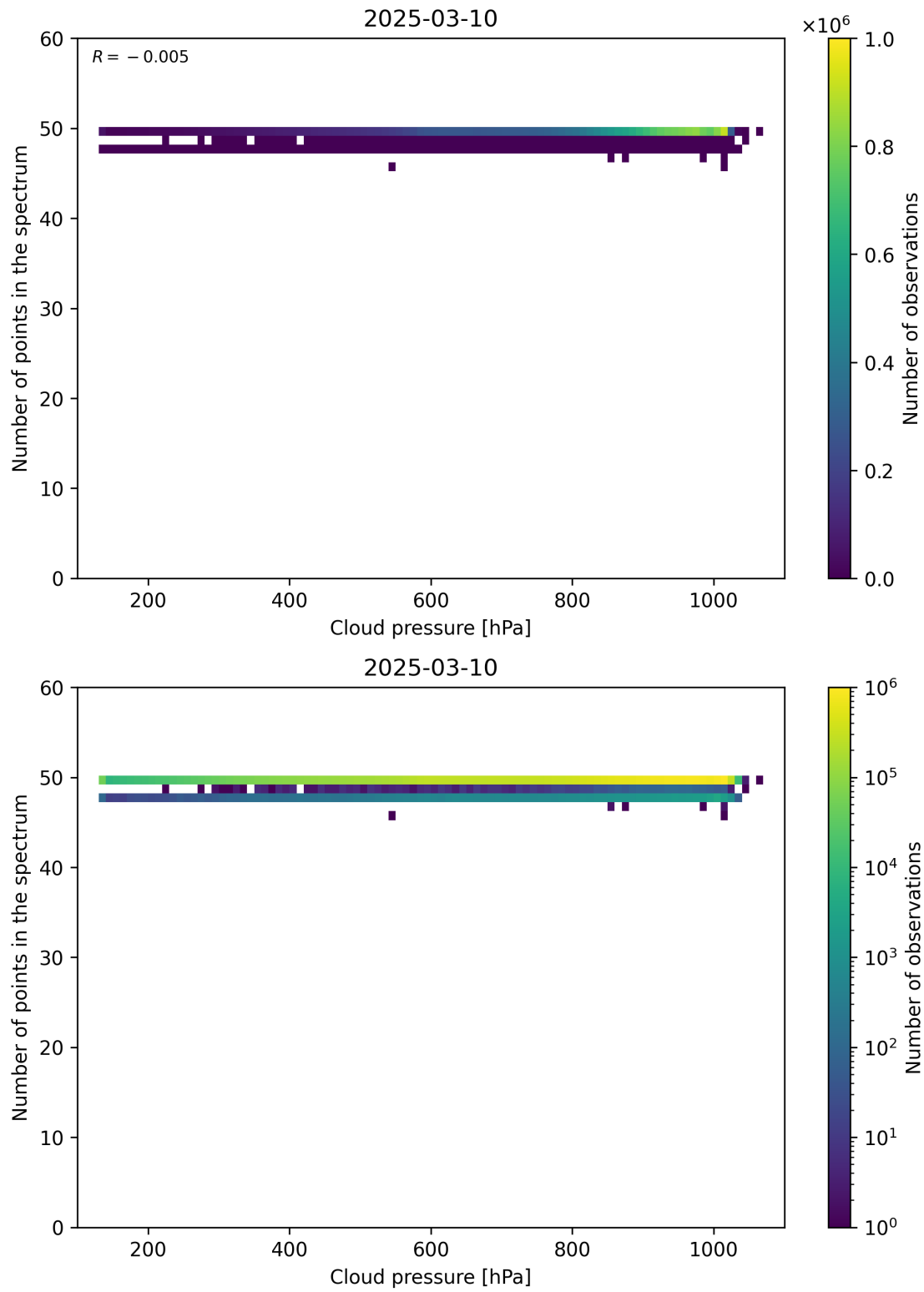
Figure 82: Scatter density plot of “Cloud pressure” against “Number of points in the spectrum” for 2025-03-09 to 2025-03-11.
