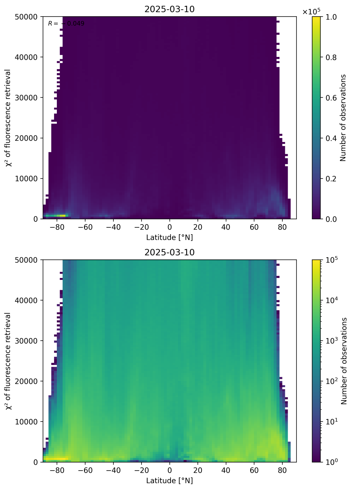
Figure 89: Scatter density plot of “Latitude” against “ \chi^2 of fluorescence retrieval” for 2025-03-09 to 2025-03-11.
