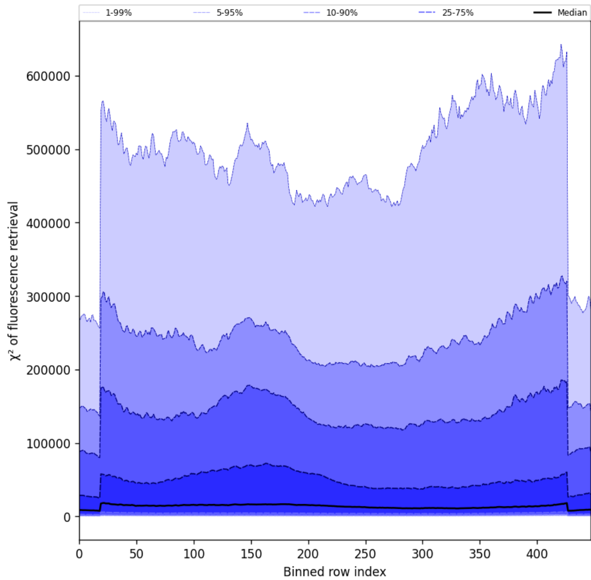
Figure 59: Along track statistics of “ \chi^2 of fluorescence retrieval” for 2025-03-09 to 2025-03-11
