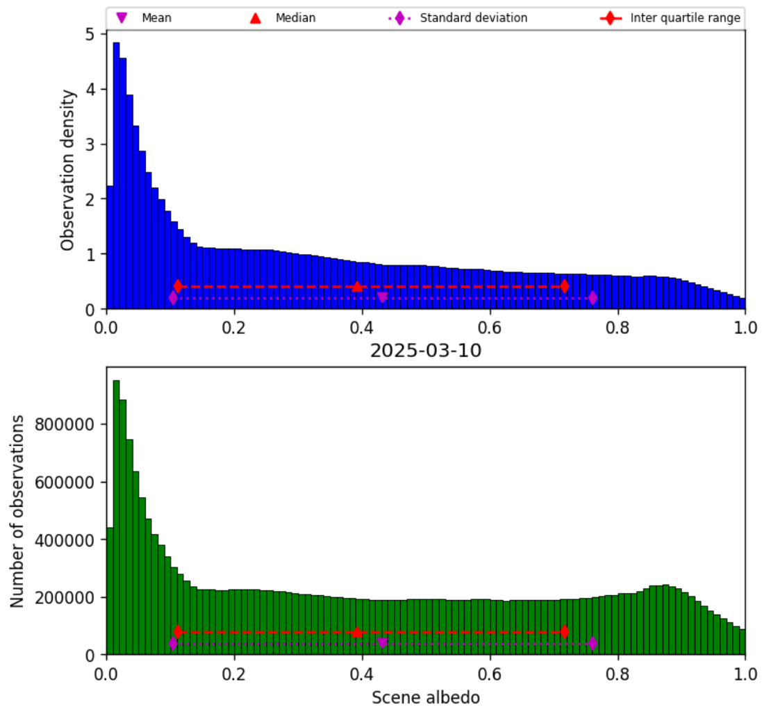
Figure 34: Histogram of “Scene albedo” for 2025-03-09 to 2025-03-11
