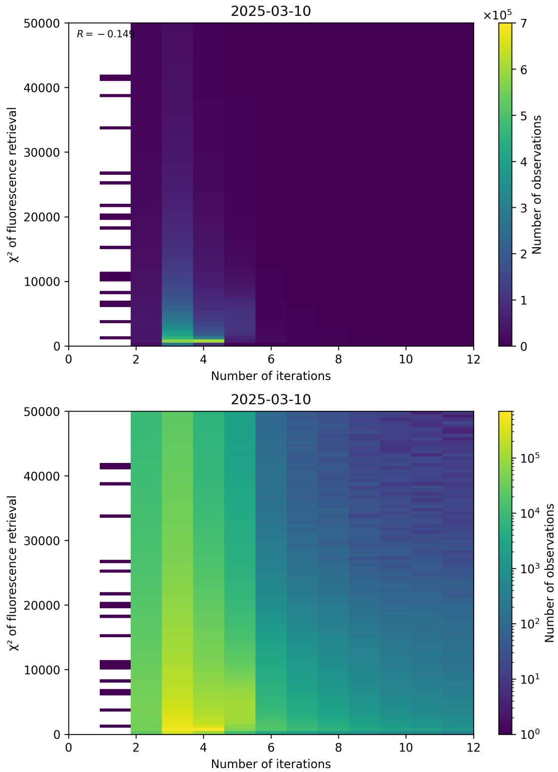
Figure 97: Scatter density plot of “Number of iterations” against “ \chi^2 of fluorescence retrieval” for 2025-03-09 to 2025-03-11.
