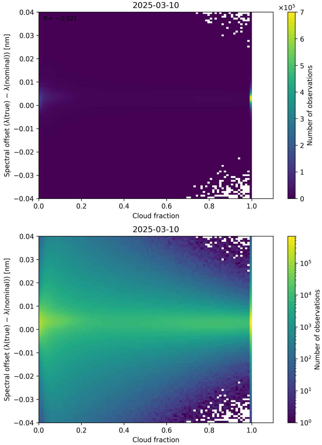
Figure 76: Scatter density plot of “Cloud fraction” against “Spectral offset ( \lambda_{\text{true}} - \lambda_{\text{nominal}} )” for 2025-03-09 to 2025-03-11.
