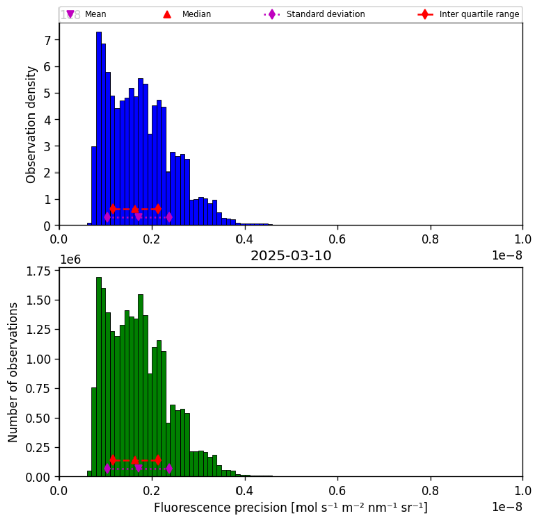
Figure 41: Histogram of “Fluorescence precision” for 2025-03-09 to 2025-03-11
