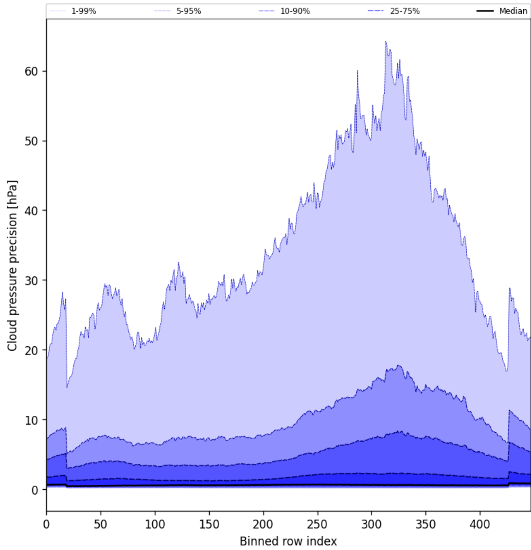
Figure 48: Along track statistics of “Cloud pressure precision” for 2025-03-09 to 2025-03-11
