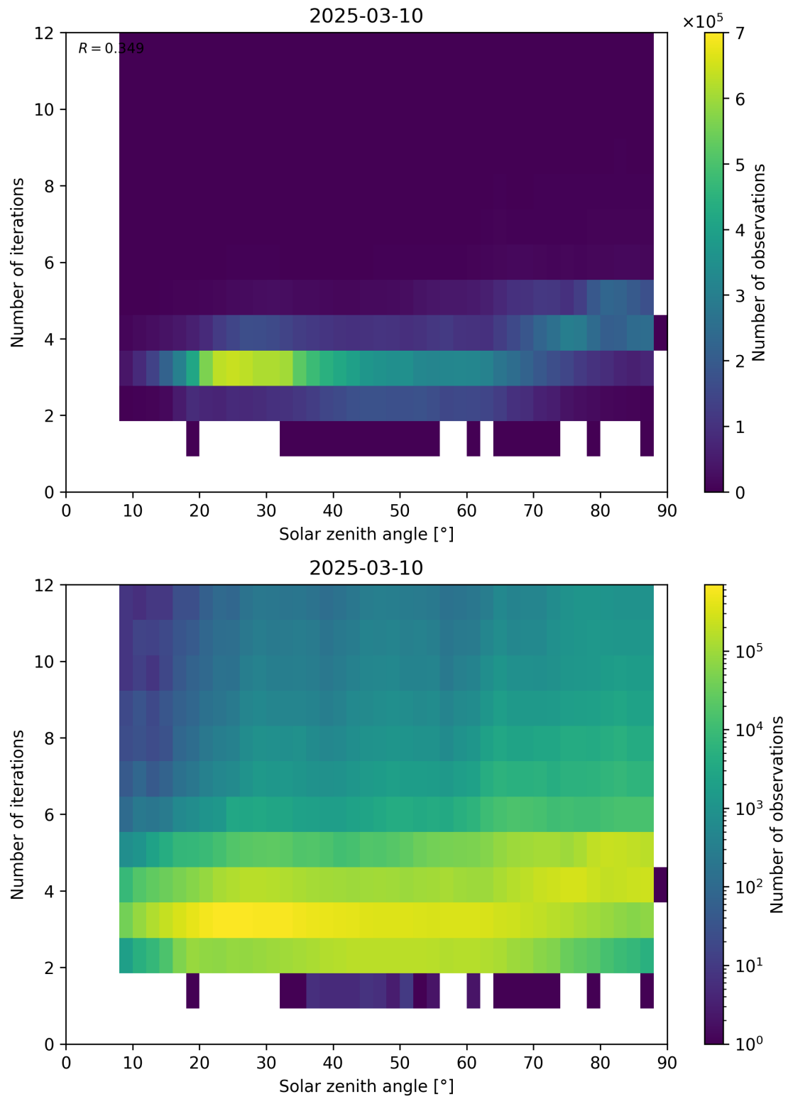
Figure 114: Scatter density plot of “Solar zenith angle” against “Number of iterations” for 2025-03-09 to 2025-03-11.
