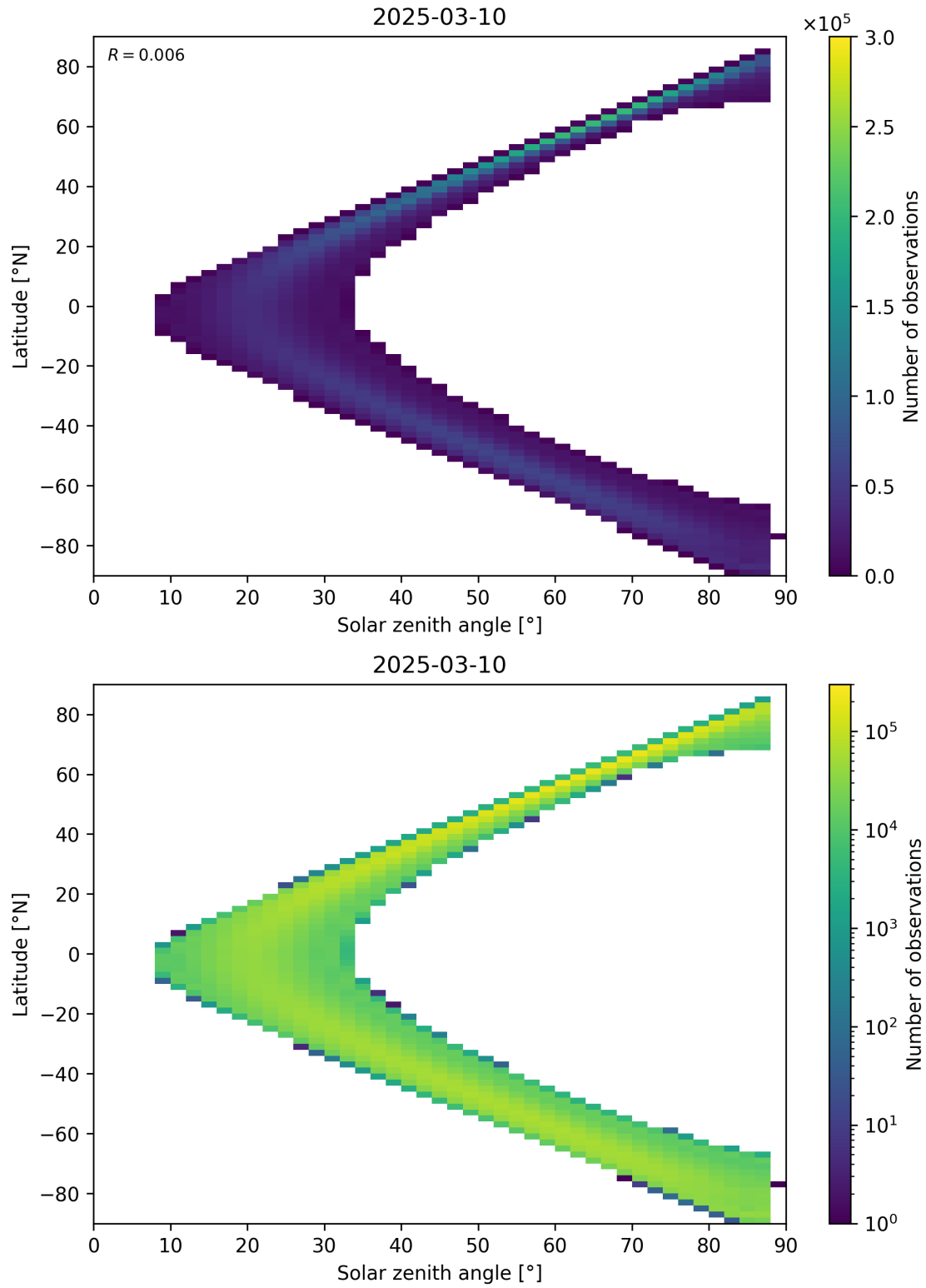
Figure 113: Scatter density plot of “Solar zenith angle” against “Latitude” for 2025-03-09 to 2025-03-11.
