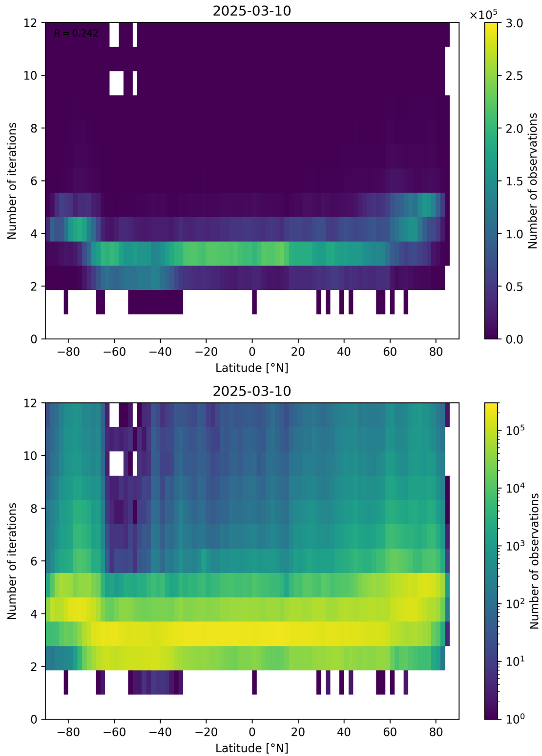
Figure 93: Scatter density plot of “Latitude” against “Number of iterations” for 2025-03-09 to 2025-03-11.
