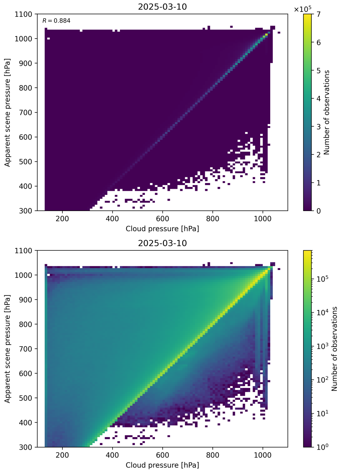
Figure 77: Scatter density plot of “Cloud pressure” against “Apparent scene pressure” for 2025-03-09 to 2025-03-11.
