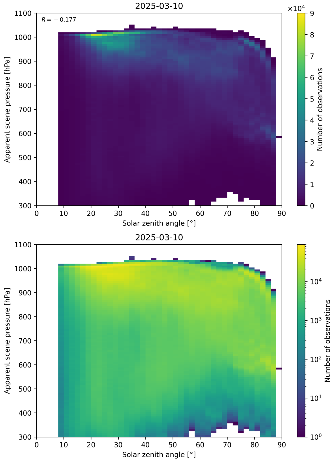
Figure 108: Scatter density plot of “Solar zenith angle” against “Apparent scene pressure” for 2025-03-09 to 2025-03-11.
