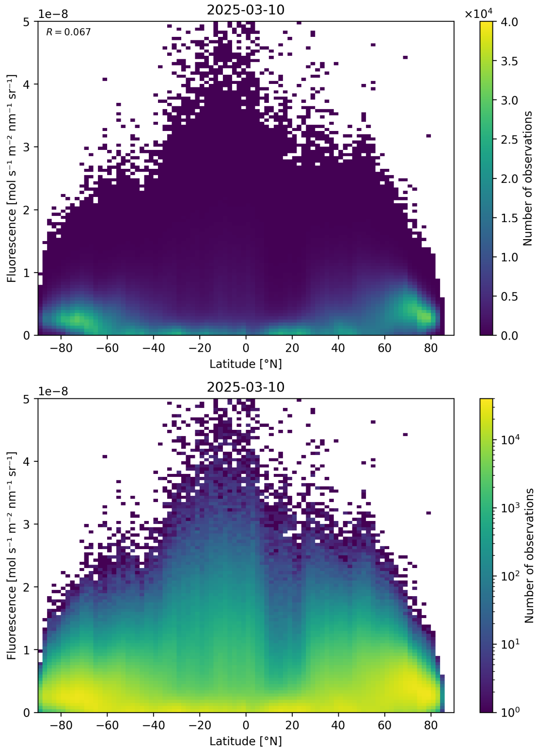
Figure 92: Scatter density plot of “Latitude” against “Fluorescence” for 2025-03-09 to 2025-03-11.
