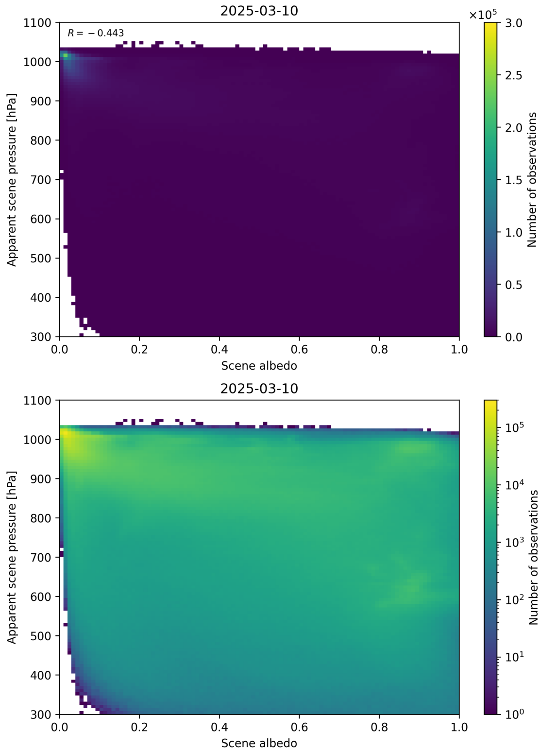
Figure 102: Scatter density plot of “Scene albedo” against “Apparent scene pressure” for 2025-03-09 to 2025-03-11.
