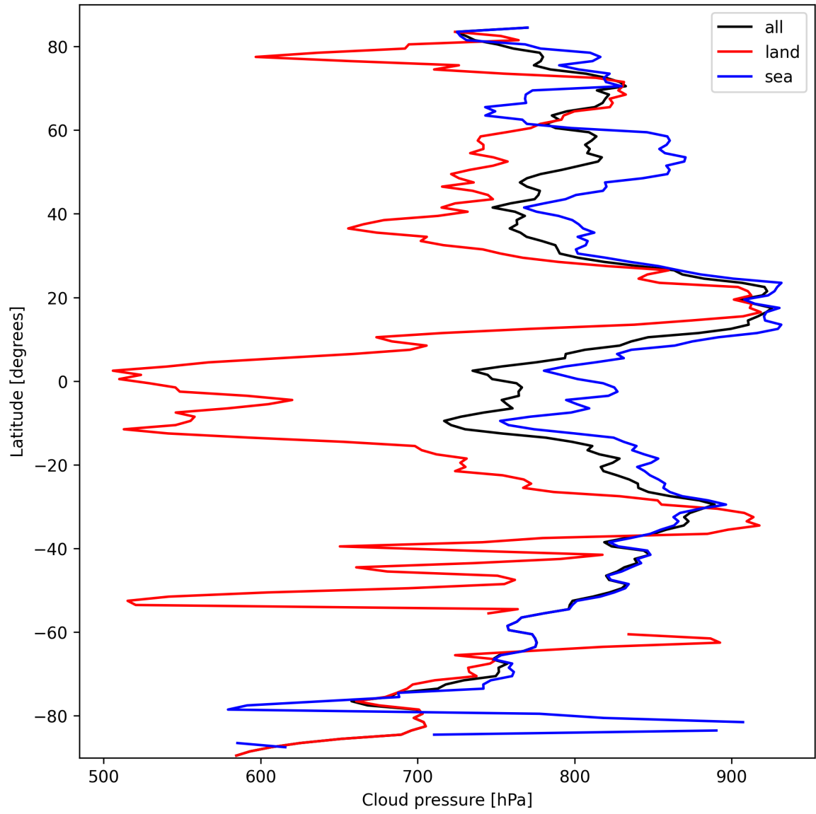
Figure 13: Zonal average of “Cloud pressure” for 2025-03-09 to 2025-03-11.
