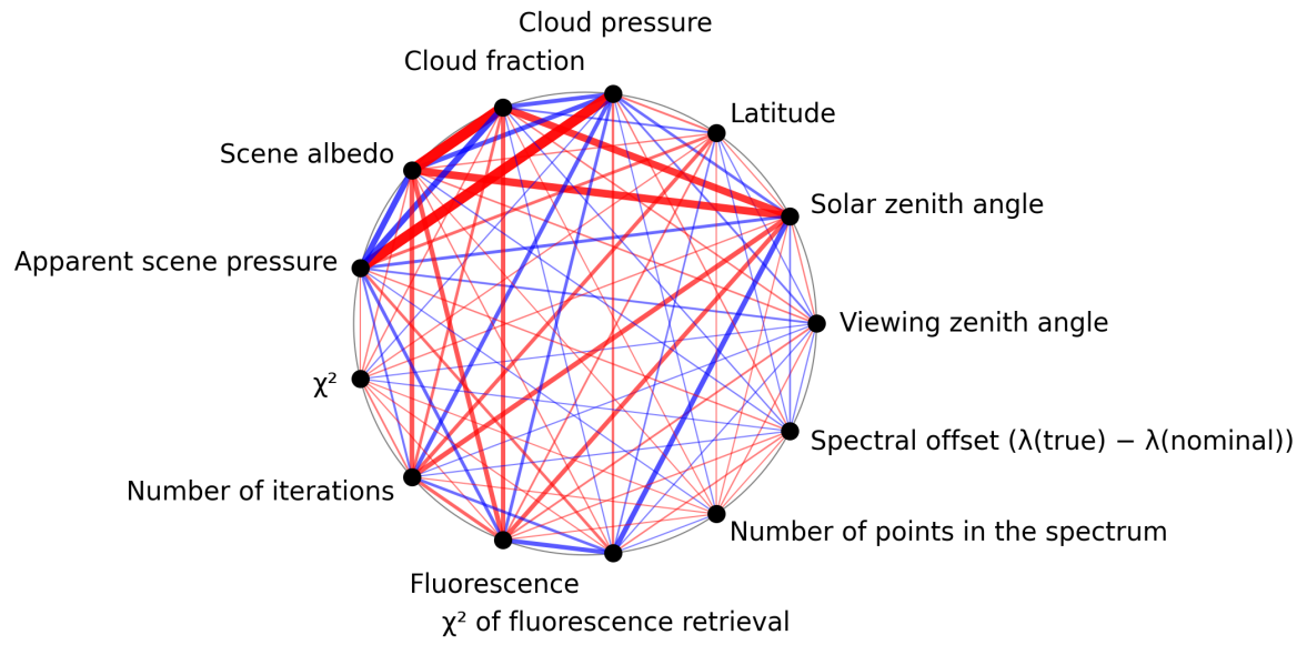
Figure 1: Map of correlation graph for 2025-03-09 to 2025-03-11.
