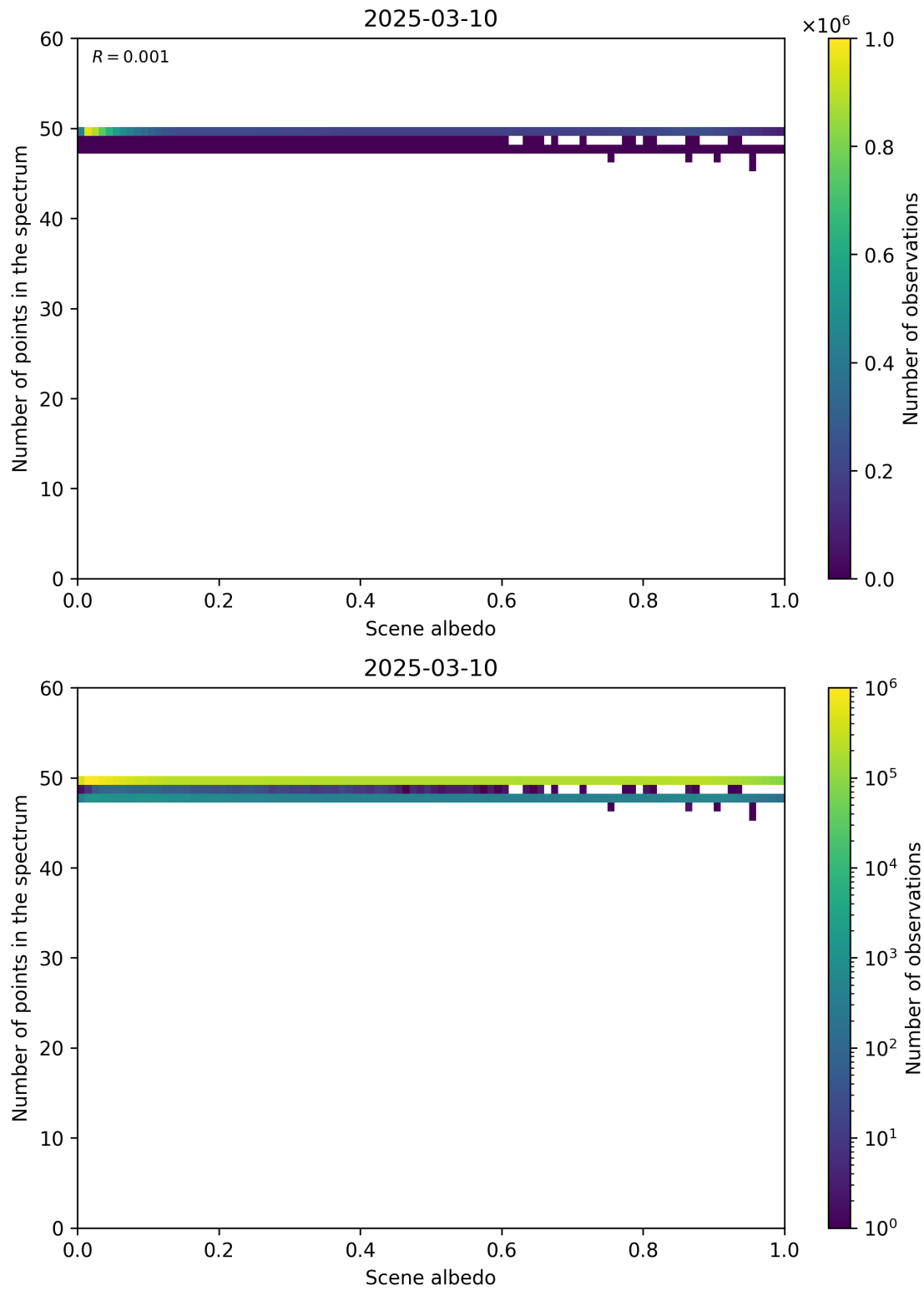
Figure 106: Scatter density plot of “Scene albedo” against “Number of points in the spectrum” for 2025-03-09 to 2025-03-11.
