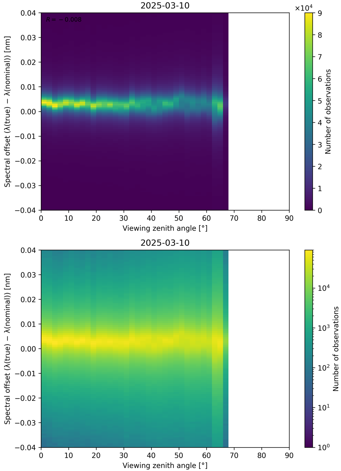
Figure 128: Scatter density plot of “Viewing zenith angle” against “Spectral offset ( \lambda_{\text{true}} - \lambda_{\text{nominal}} )” for 2025-03-09 to 2025-03-11.
