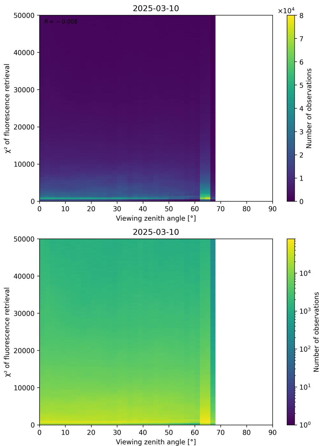
Figure 119: Scatter density plot of “Viewing zenith angle” against “ \chi^2 of fluorescence retrieval” for 2025-03-09 to 2025-03-11.
