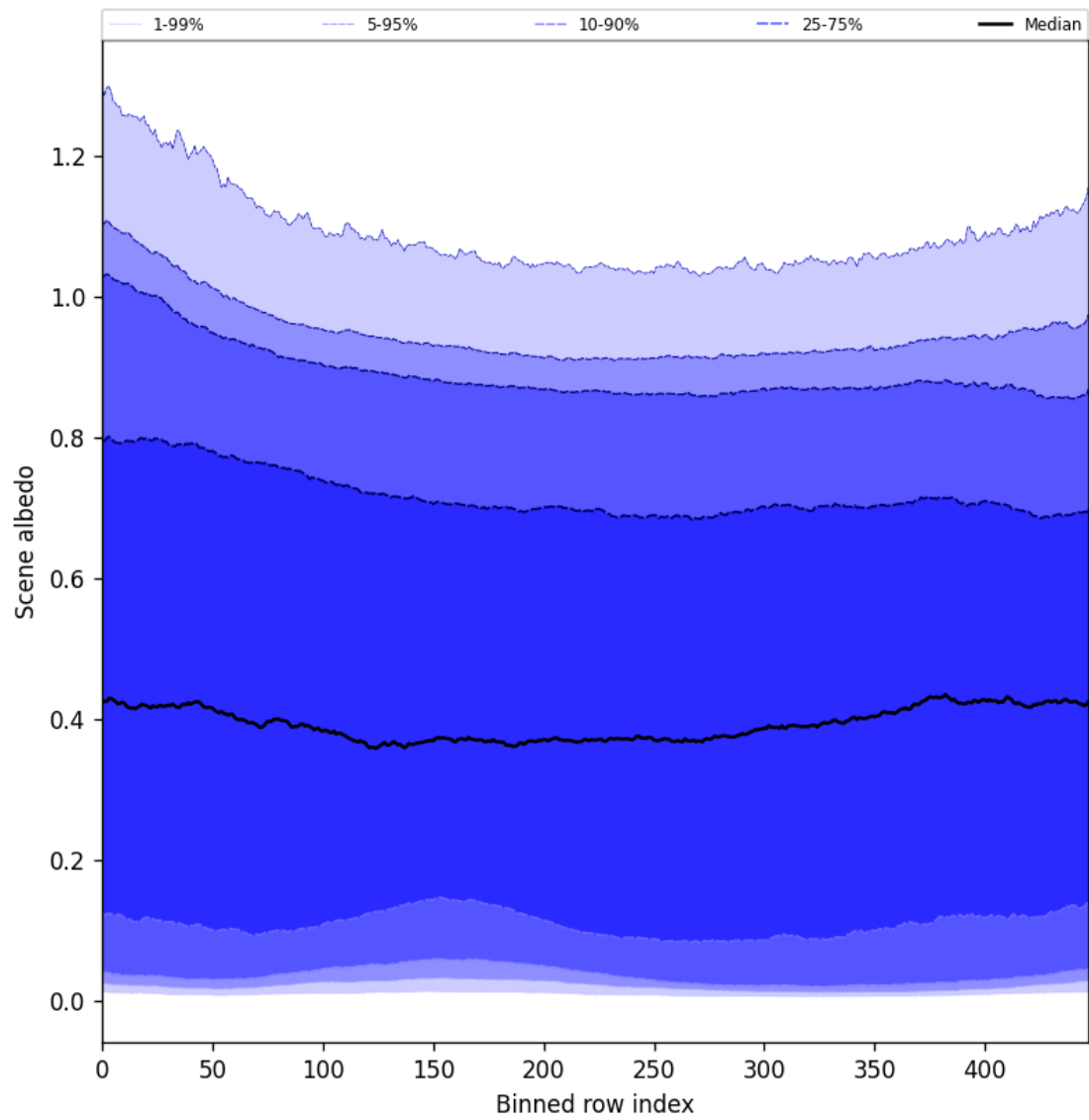
Figure 51: Along track statistics of “Scene albedo” for 2025-03-09 to 2025-03-11
