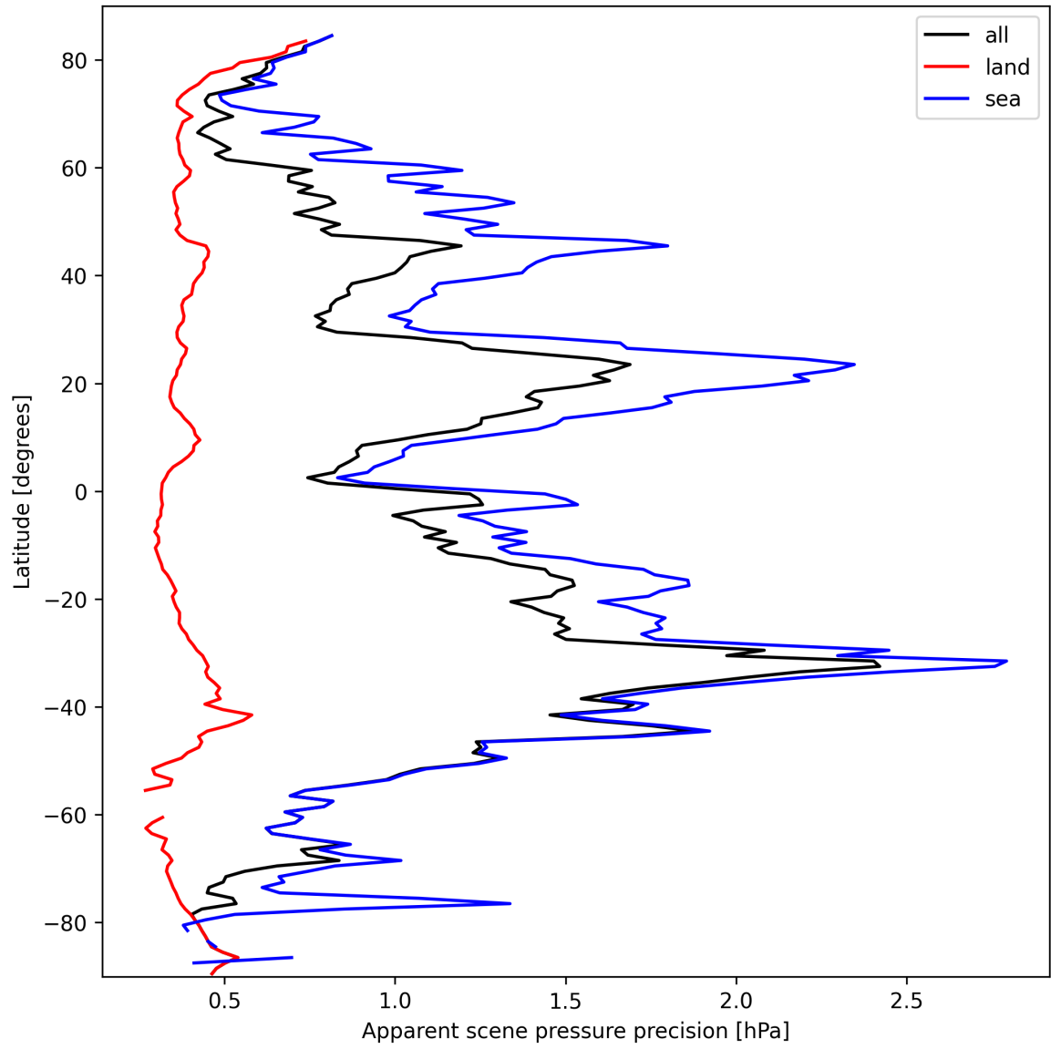
Figure 20: Zonal average of “Apparent scene pressure precision” for 2025-03-09 to 2025-03-11.
