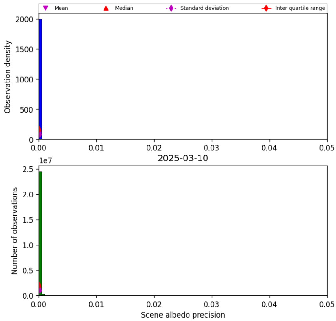
Figure 35: Histogram of “Scene albedo precision” for 2025-03-09 to 2025-03-11
