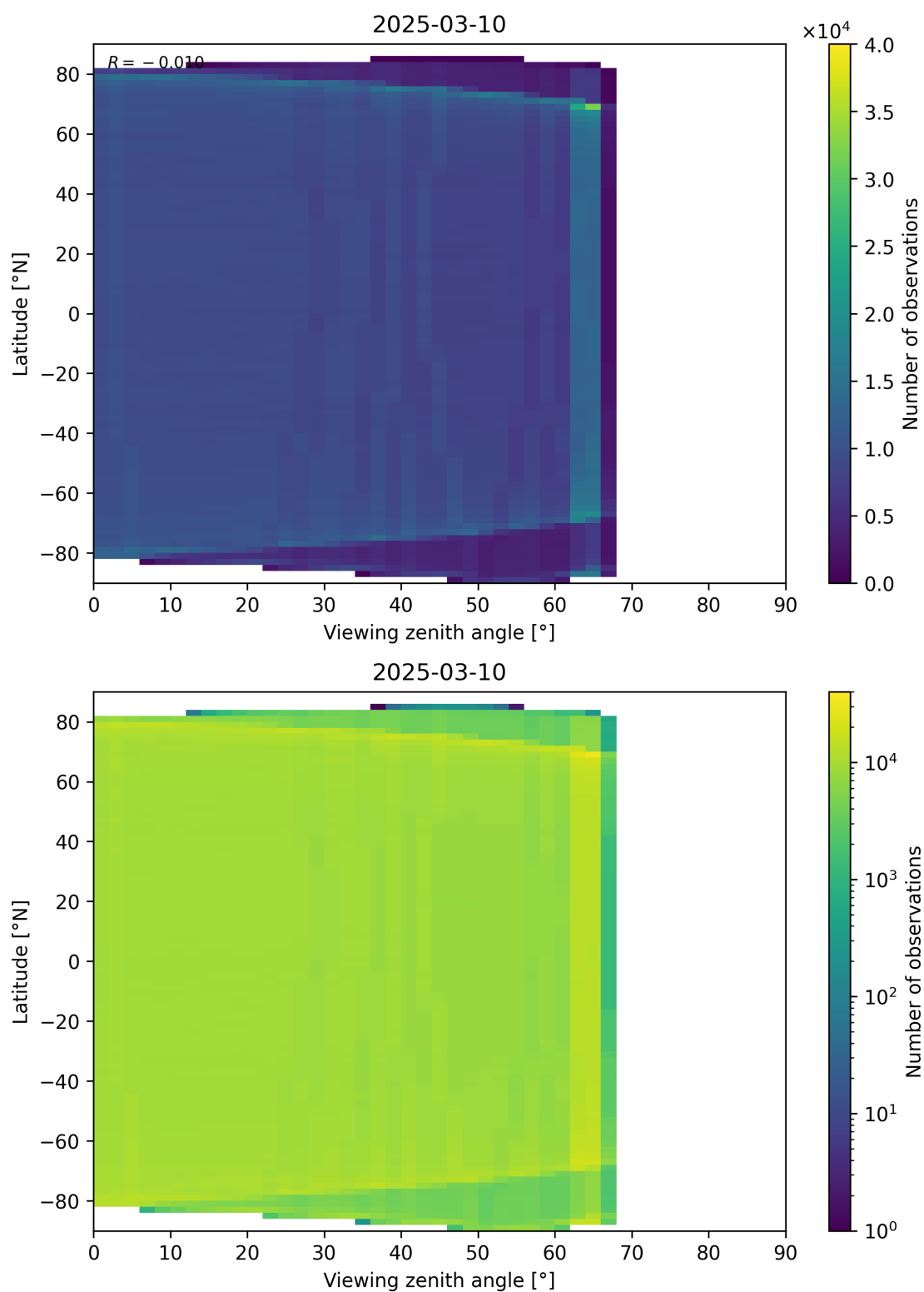
Figure 123: Scatter density plot of “Viewing zenith angle” against “Latitude” for 2025-03-09 to 2025-03-11.
