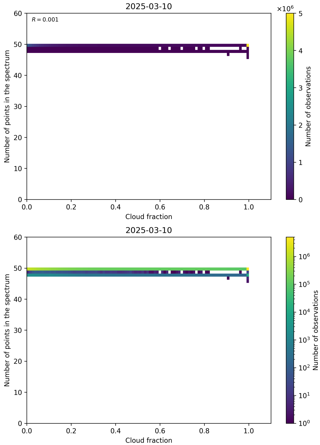
Figure 74: Scatter density plot of “Cloud fraction” against “Number of points in the spectrum” for 2025-03-09 to 2025-03-11.
