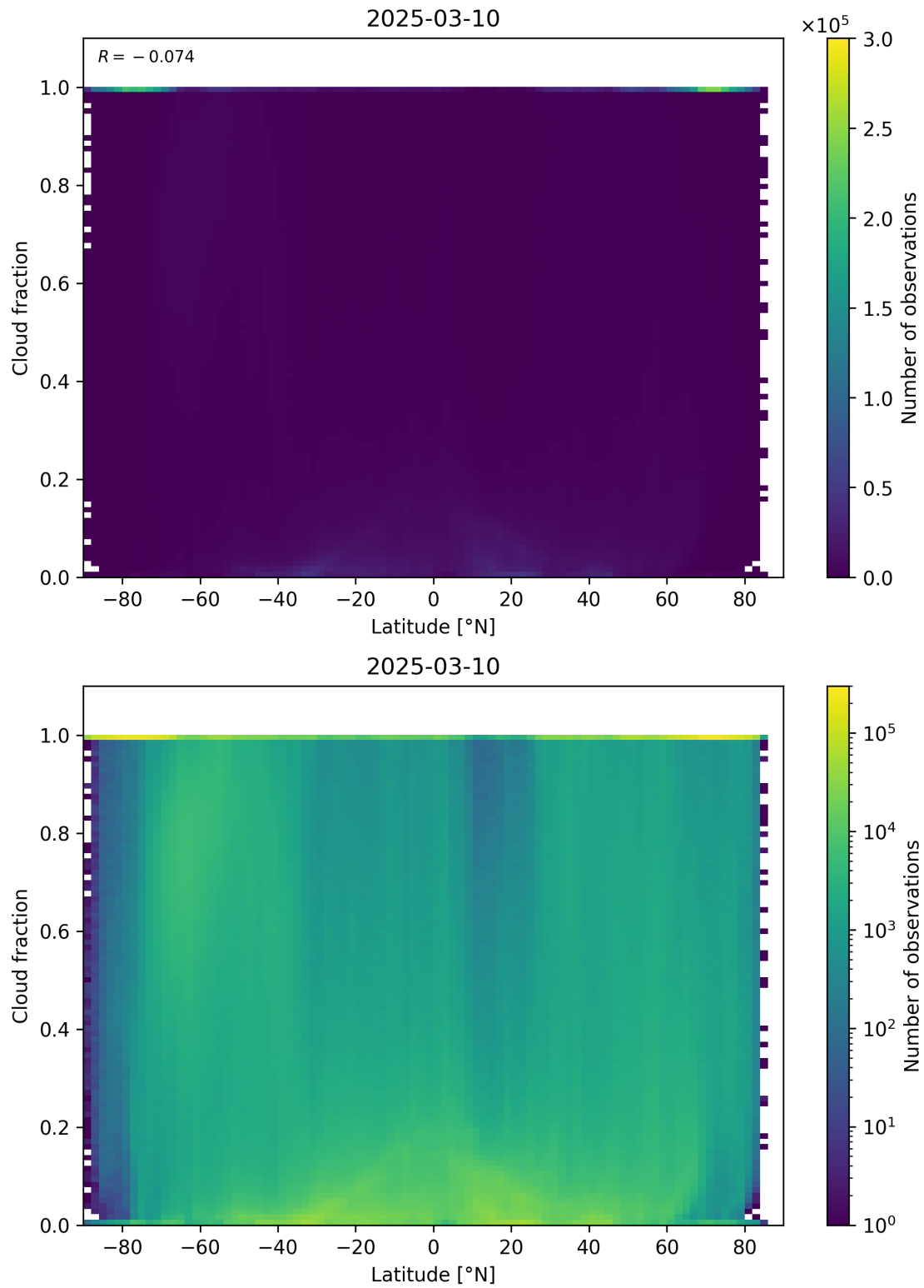
Figure 90: Scatter density plot of “Latitude” against “Cloud fraction” for 2025-03-09 to 2025-03-11.
