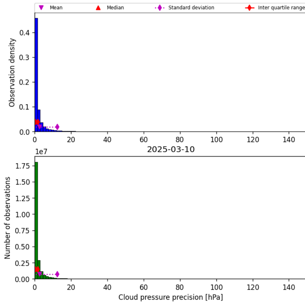
Figure 31: Histogram of “Cloud pressure precision” for 2025-03-09 to 2025-03-11
