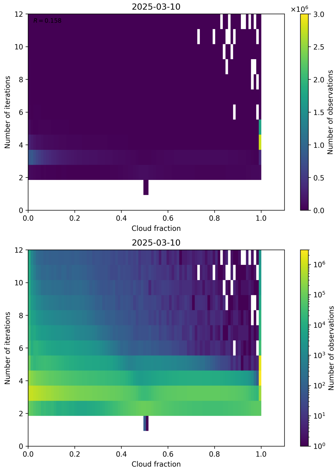
Figure 73: Scatter density plot of “Cloud fraction” against “Number of iterations” for 2025-03-09 to 2025-03-11.
