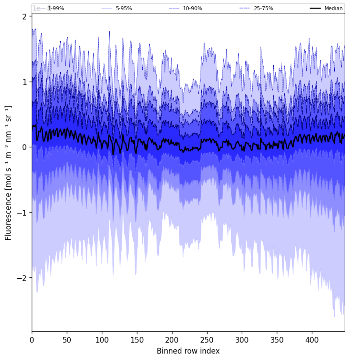
Figure 57: Along track statistics of “Fluorescence” for 2025-03-09 to 2025-03-11
