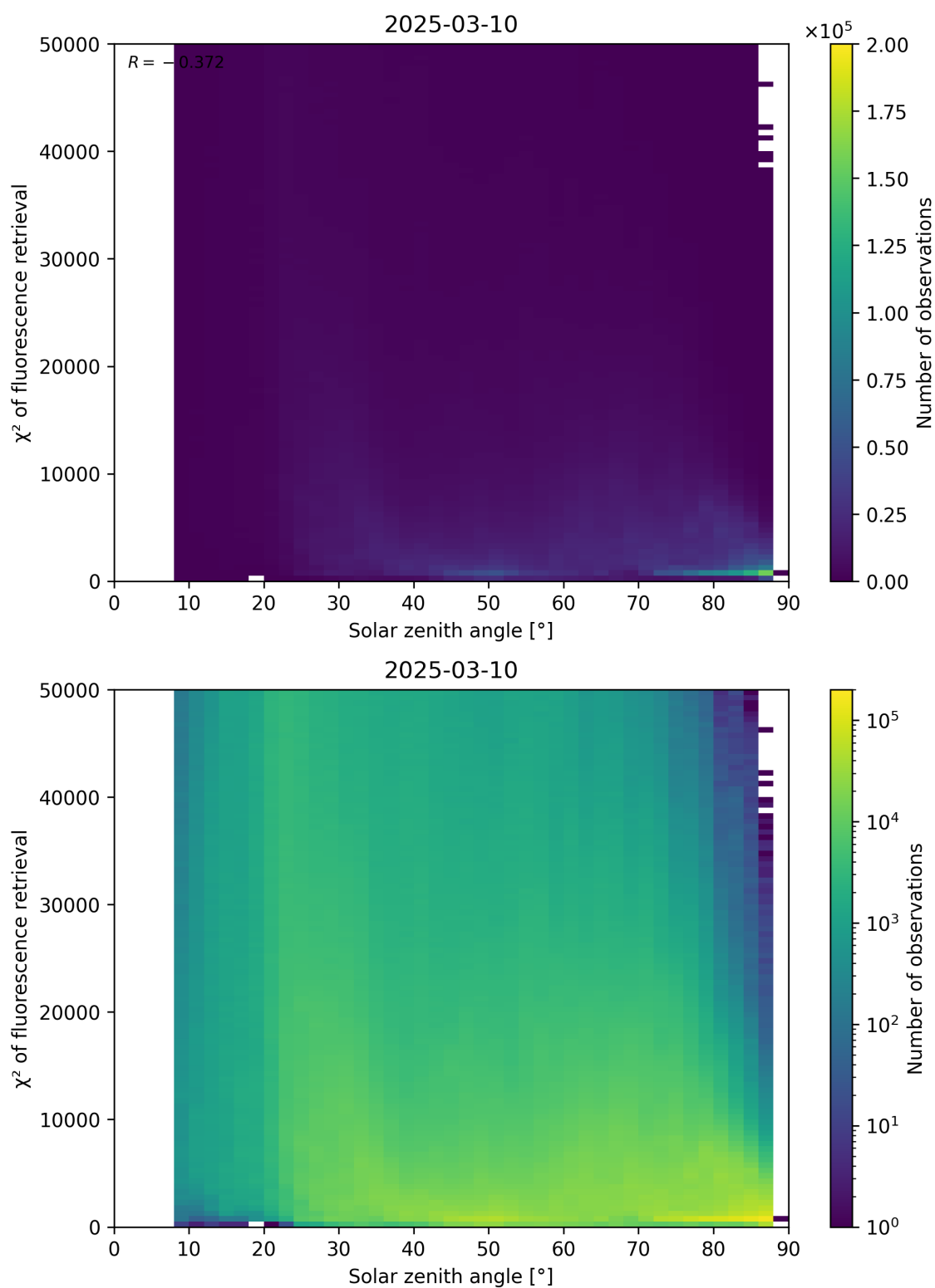
Figure 109: Scatter density plot of “Solar zenith angle” against “ \chi^2 of fluorescence retrieval” for 2025-03-09 to 2025-03-11.
