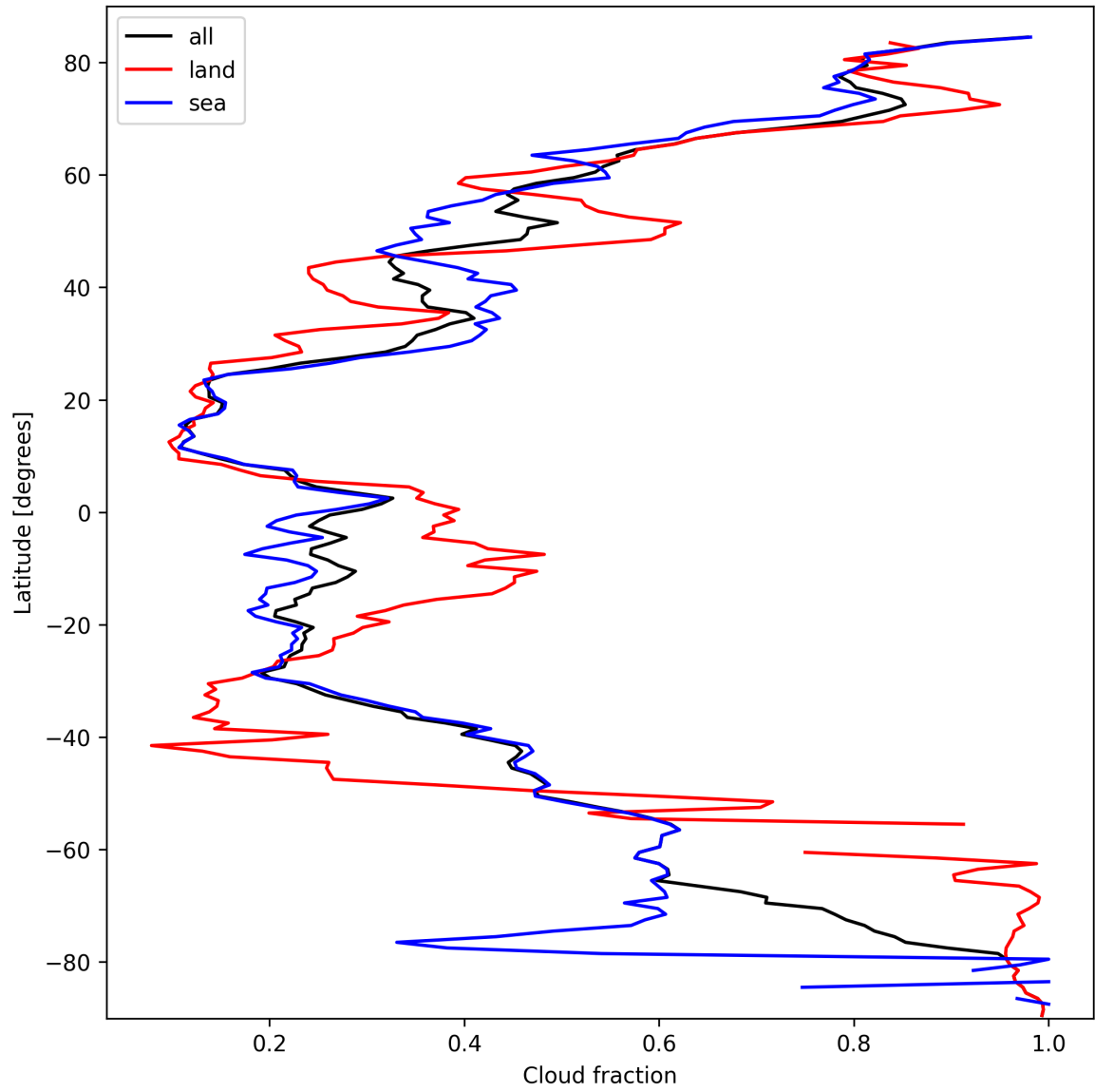
Figure 15: Zonal average of “Cloud fraction” for 2025-03-09 to 2025-03-11.
