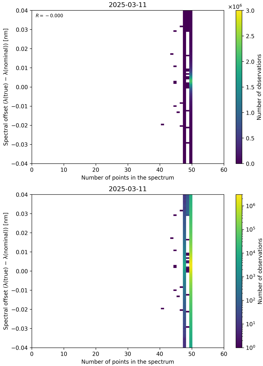
Figure 101: Scatter density plot of “Number of points in the spectrum” against “Spectral offset ( \lambda_{\text{true}} - \lambda_{\text{nominal}} )” for 2025-03-10 to 2025-03-12.
