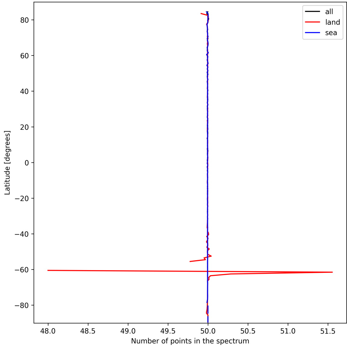
Figure 27: Zonal average of “Number of points in the spectrum” for 2025-03-10 to 2025-03-12.
