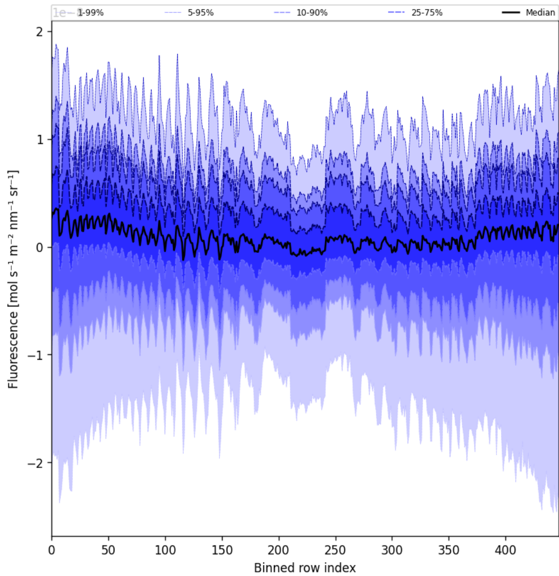
Figure 57: Along track statistics of “Fluorescence” for 2025-03-10 to 2025-03-12
