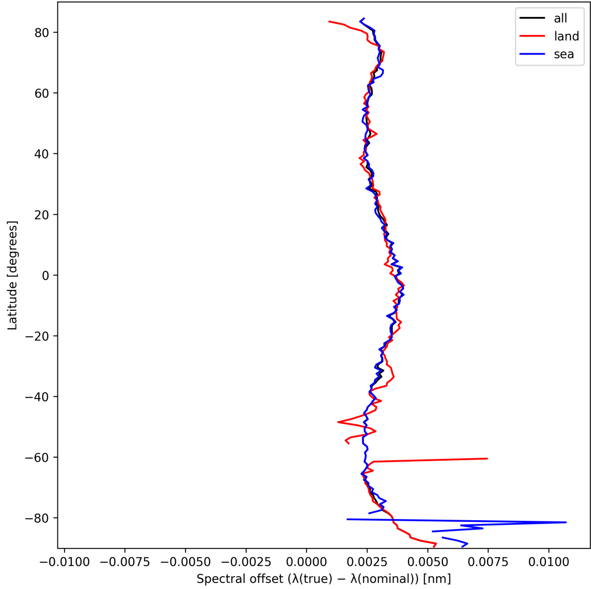
Figure 28: Zonal average of “Spectral offset ( \lambda_{\text{true}} - \lambda_{\text{nominal}} )” for 2025-03-10 to 2025-03-12.
