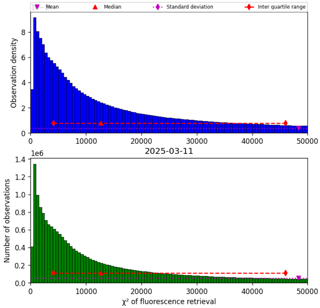
Figure 42: Histogram of “ \chi^2 of fluorescence retrieval” for 2025-03-10 to 2025-03-12
