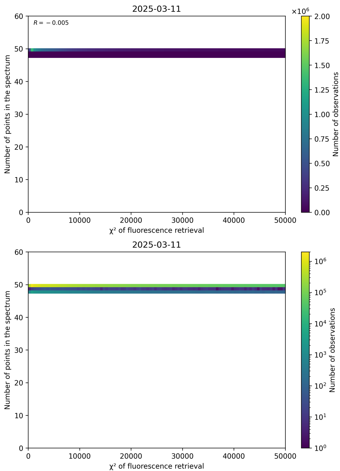
Figure 68: Scatter density plot of “ \chi^2 of fluorescence retrieval” against “Number of points in the spectrum” for 2025-03-10 to 2025-03-12.
