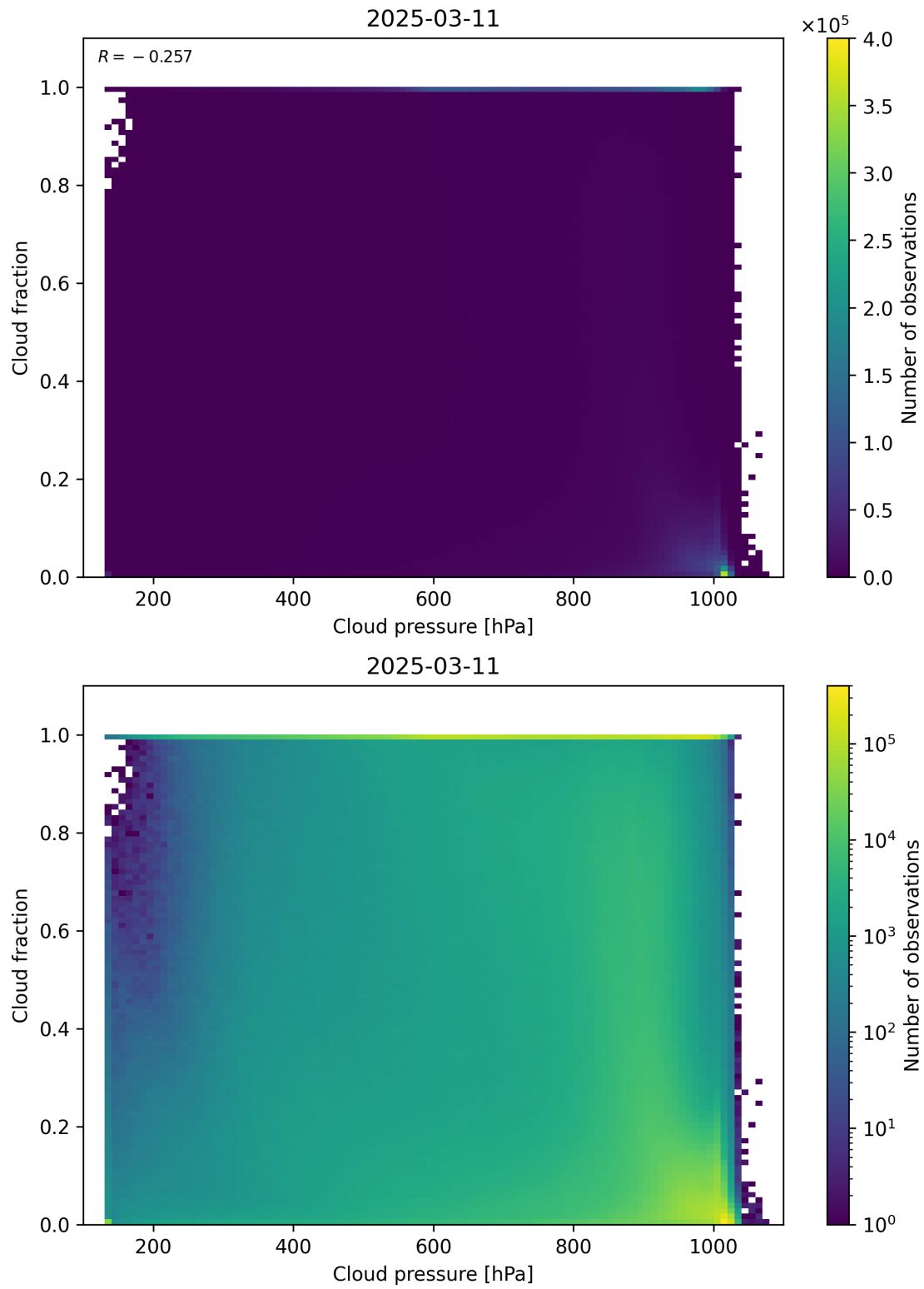
Figure 79: Scatter density plot of “Cloud pressure” against “Cloud fraction” for 2025-03-10 to 2025-03-12.
