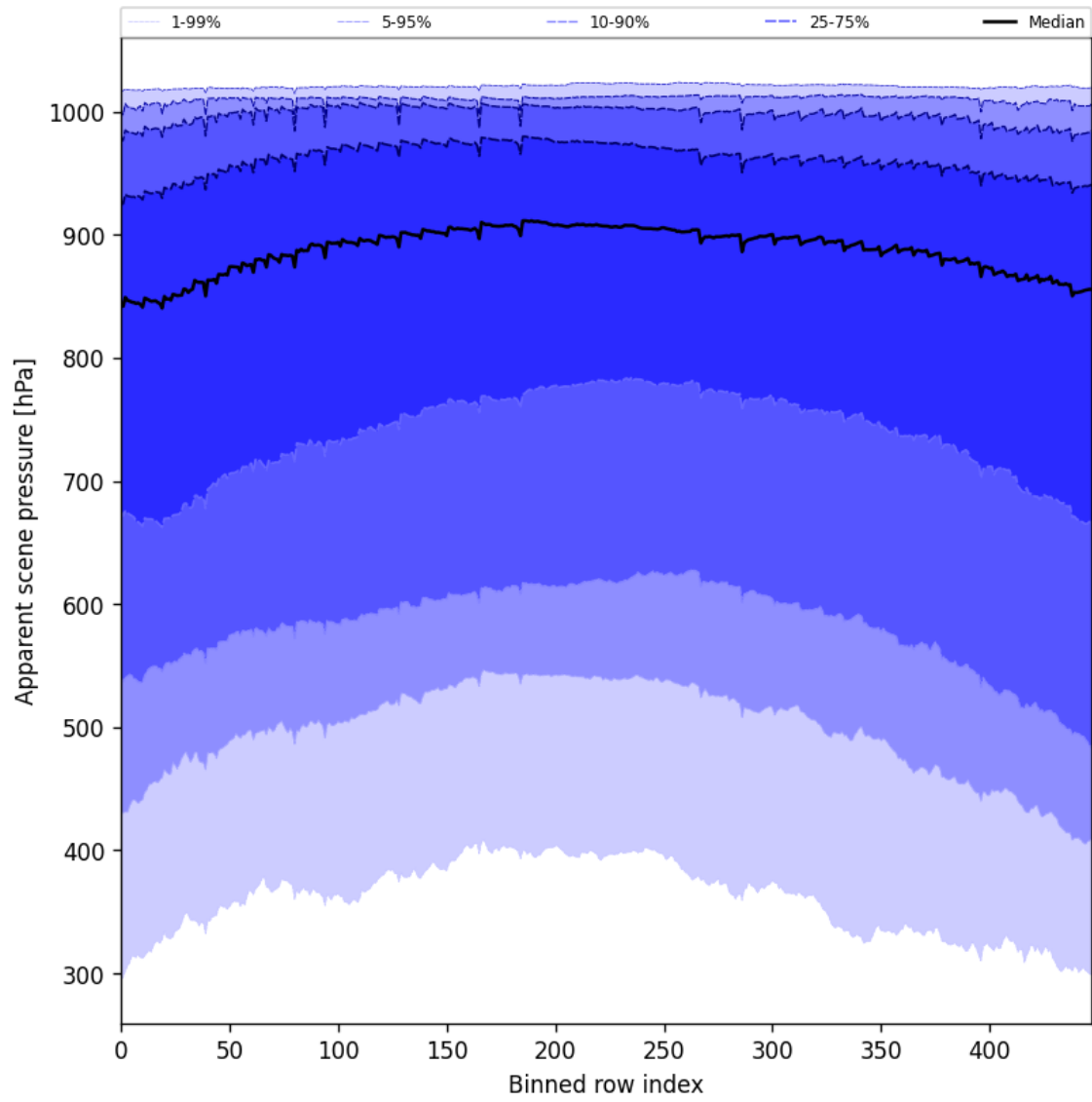
Figure 53: Along track statistics of “Apparent scene pressure” for 2025-03-10 to 2025-03-12
