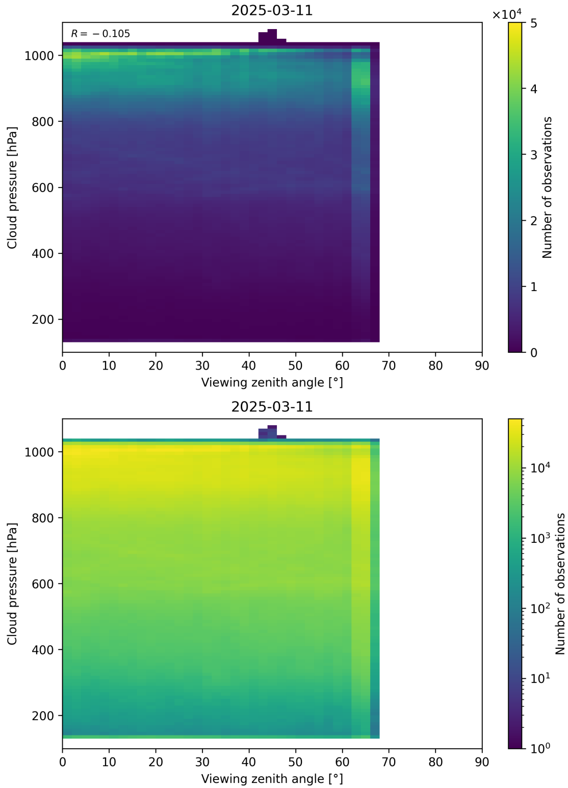
Figure 121: Scatter density plot of “Viewing zenith angle” against “Cloud pressure” for 2025-03-10 to 2025-03-12.
