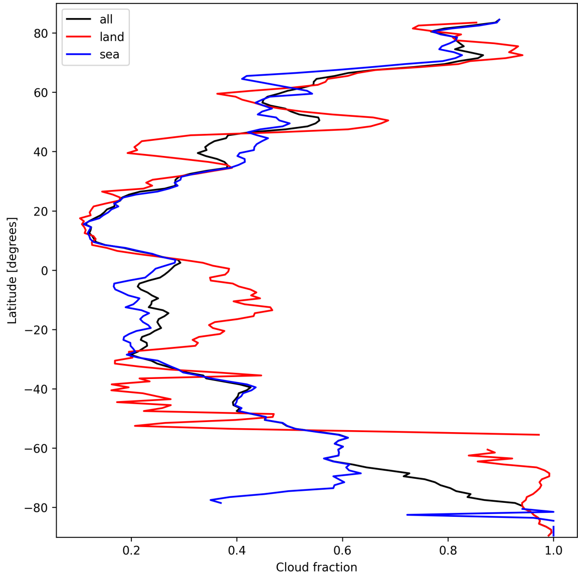
Figure 15: Zonal average of “Cloud fraction” for 2025-03-10 to 2025-03-12.
