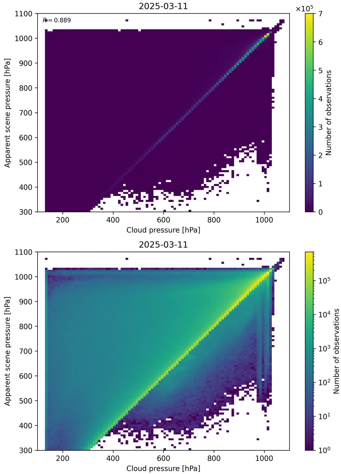
Figure 77: Scatter density plot of “Cloud pressure” against “Apparent scene pressure” for 2025-03-10 to 2025-03-12.
