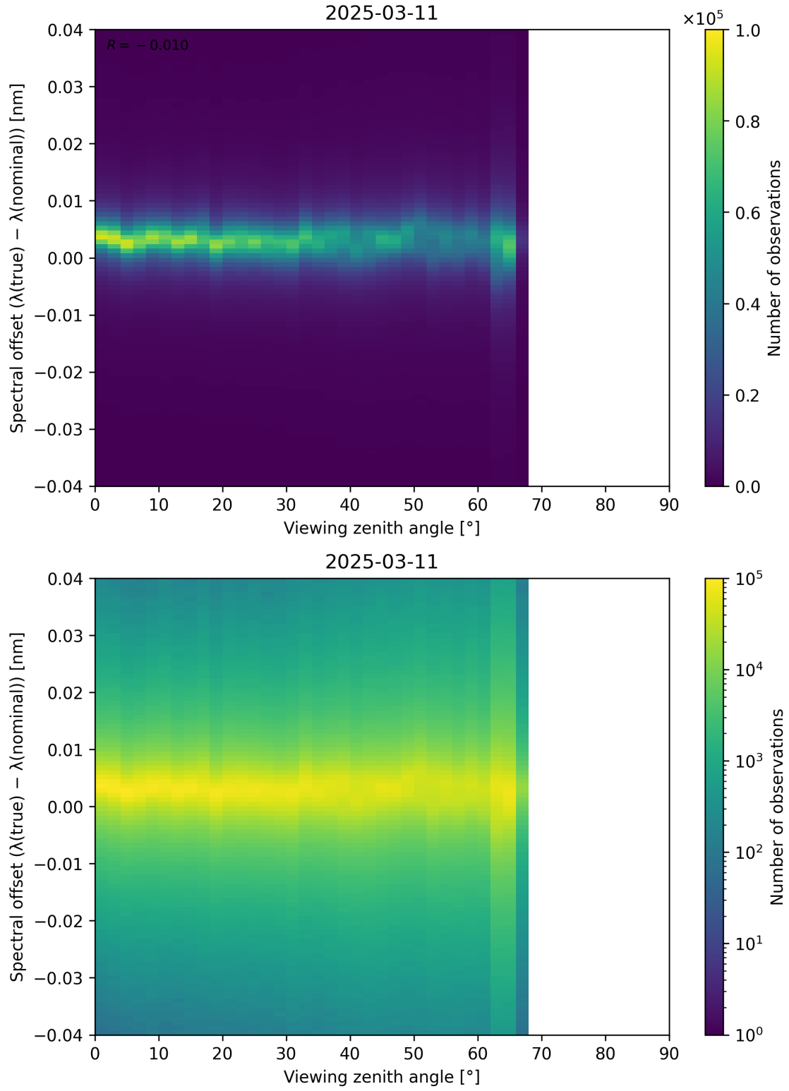
Figure 128: Scatter density plot of “Viewing zenith angle” against “Spectral offset ( \lambda_{\text{true}} - \lambda_{\text{nominal}} )” for 2025-03-10 to 2025-03-12.
