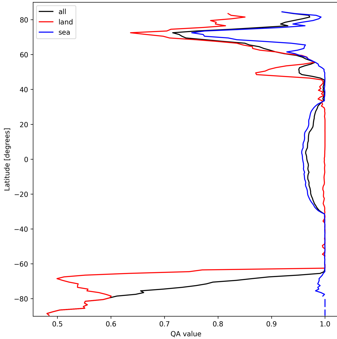
Figure 12: Zonal average of “QA value” for 2025-03-10 to 2025-03-12.
