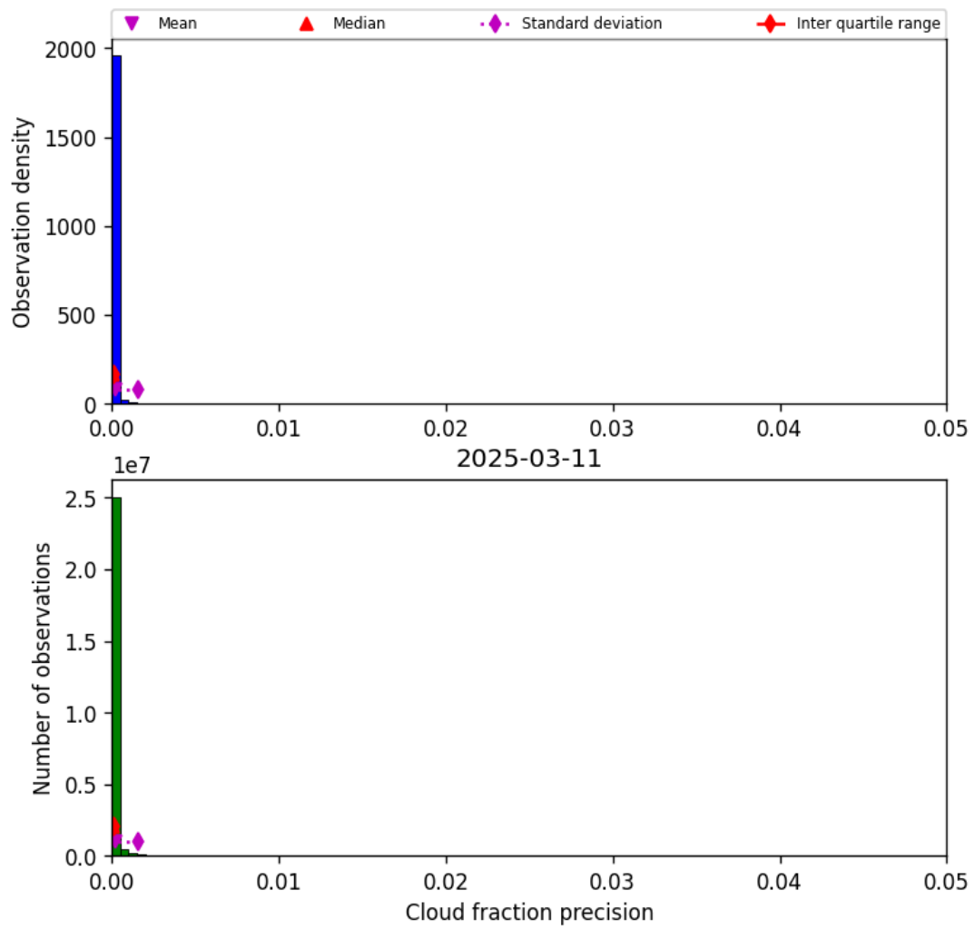
Figure 33: Histogram of “Cloud fraction precision” for 2025-03-10 to 2025-03-12
