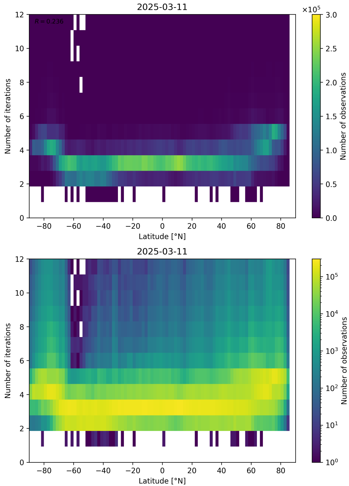
Figure 93: Scatter density plot of “Latitude” against “Number of iterations” for 2025-03-10 to 2025-03-12.
