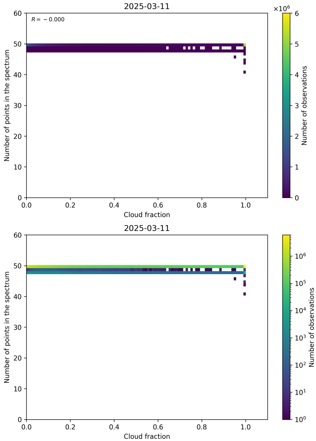
Figure 74: Scatter density plot of “Cloud fraction” against “Number of points in the spectrum” for 2025-03-10 to 2025-03-12.
