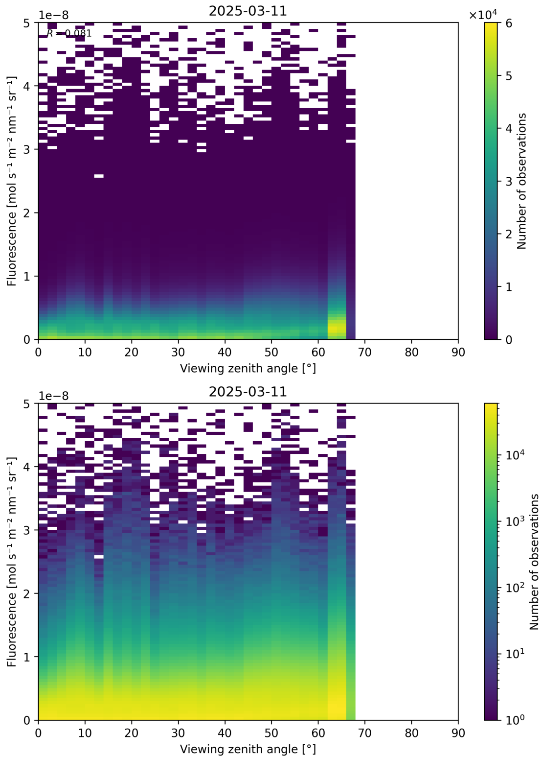
Figure 122: Scatter density plot of “Viewing zenith angle” against “Fluorescence” for 2025-03-10 to 2025-03-12.
