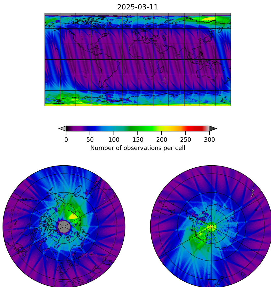
Figure 11: Map of the number of observations for 2025-03-10 to 2025-03-12
