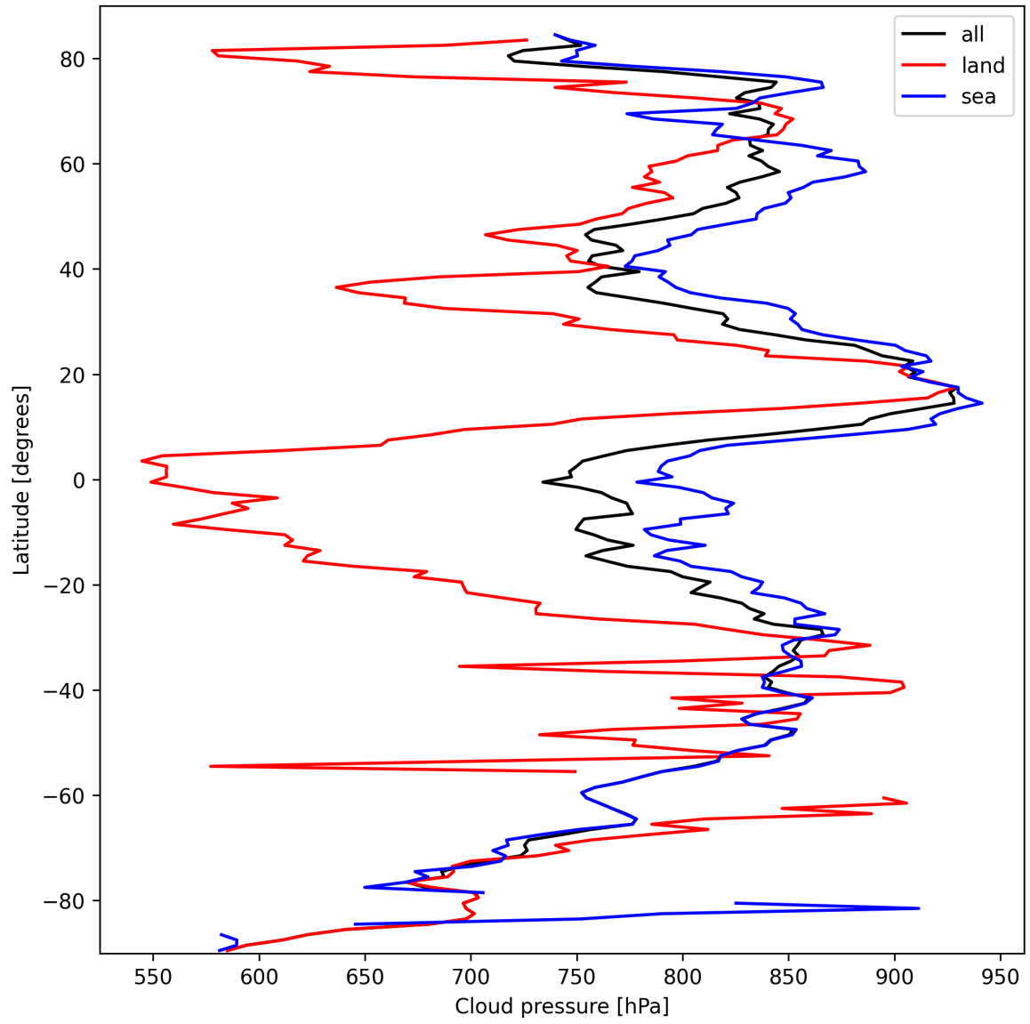
Figure 13: Zonal average of “Cloud pressure” for 2025-03-10 to 2025-03-12.
