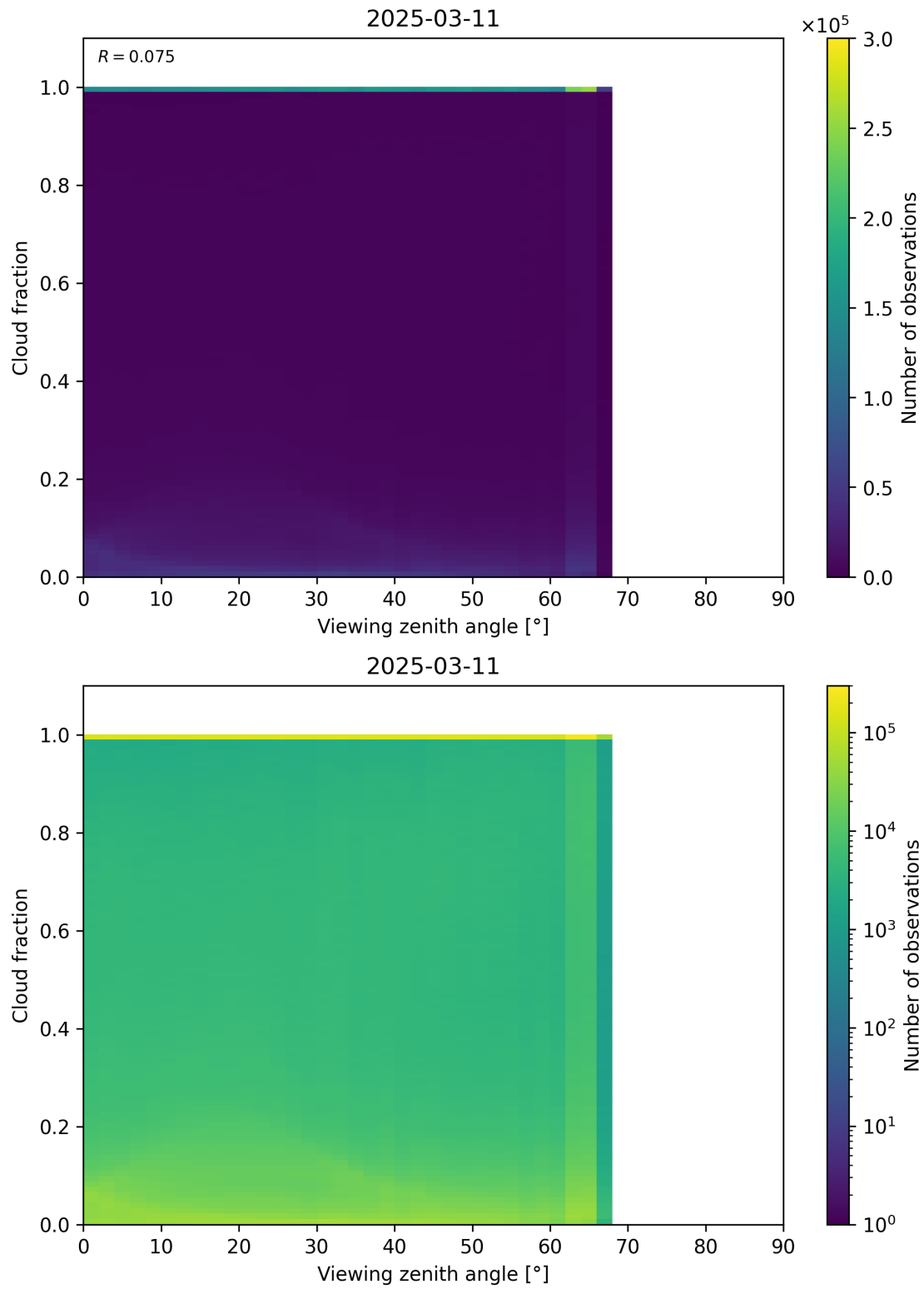
Figure 120: Scatter density plot of “Viewing zenith angle” against “Cloud fraction” for 2025-03-10 to 2025-03-12.
