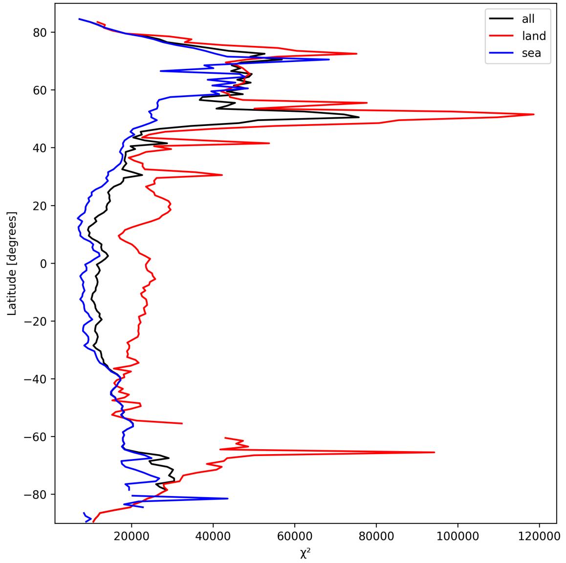
Figure 21: Zonal average of “ \chi^2 ” for 2025-03-10 to 2025-03-12.
