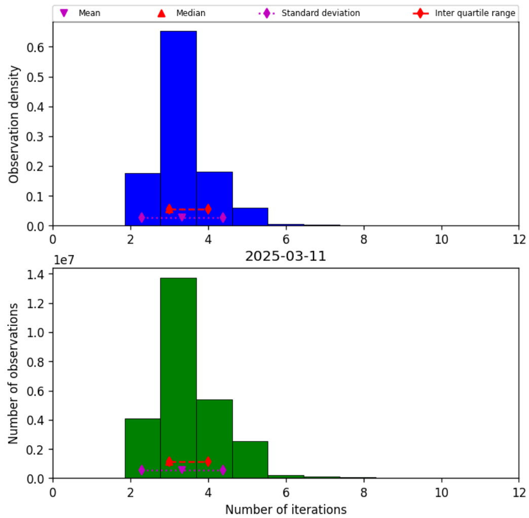
Figure 39: Histogram of “Number of iterations” for 2025-03-10 to 2025-03-12
