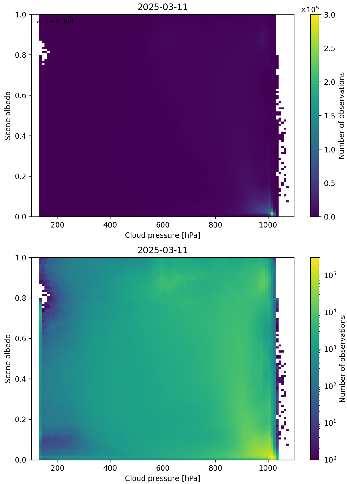
Figure 83: Scatter density plot of “Cloud pressure” against “Scene albedo” for 2025-03-10 to 2025-03-12.
