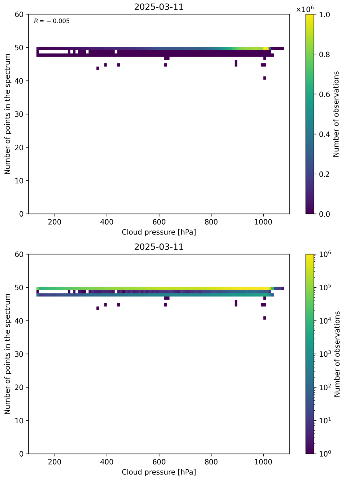
Figure 82: Scatter density plot of “Cloud pressure” against “Number of points in the spectrum” for 2025-03-10 to 2025-03-12.
