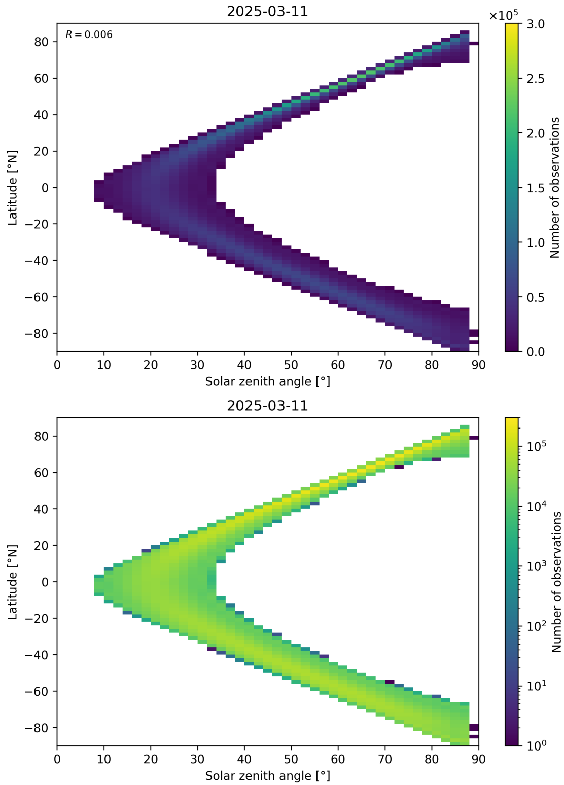
Figure 113: Scatter density plot of “Solar zenith angle” against “Latitude” for 2025-03-10 to 2025-03-12.
