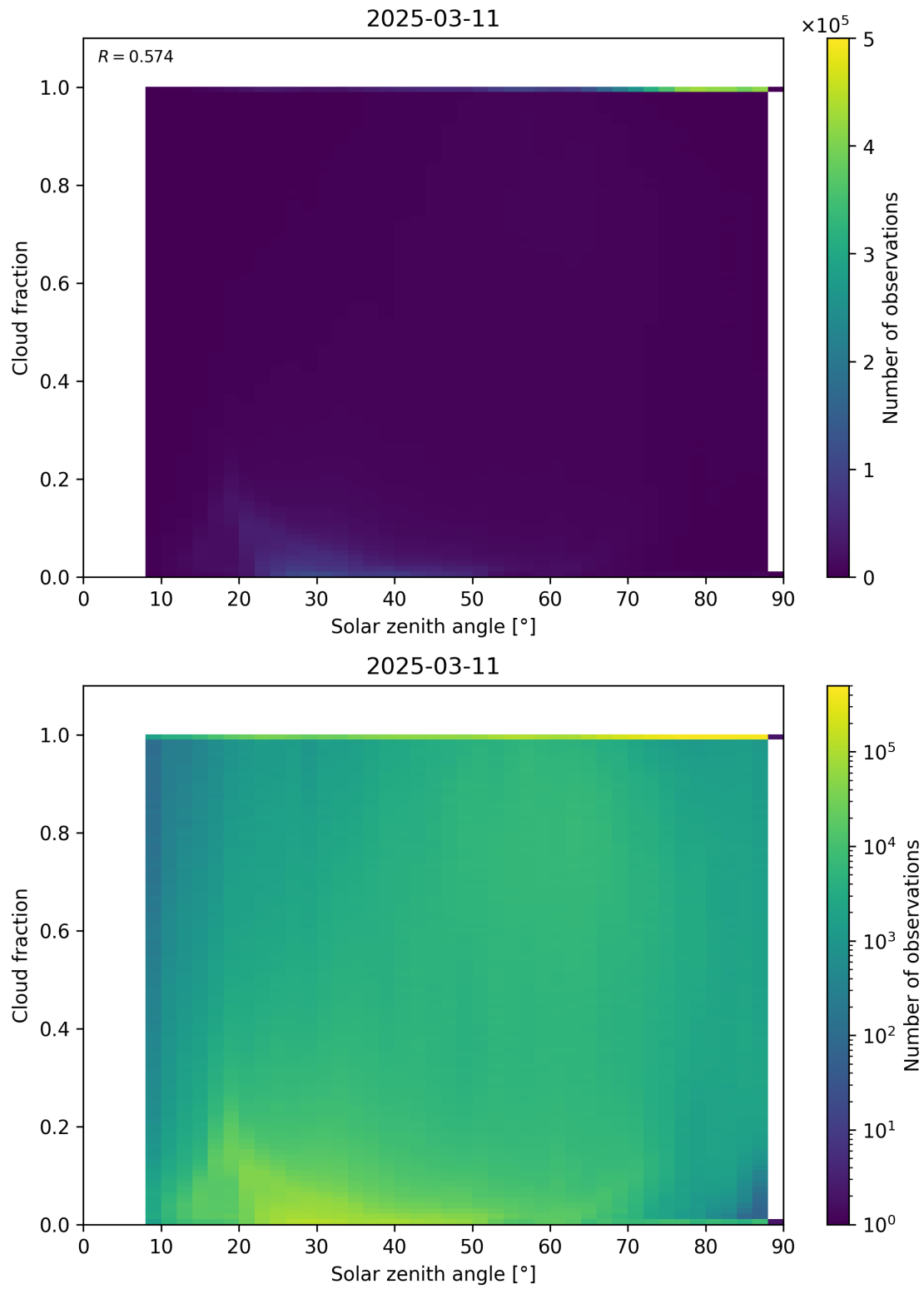
Figure 110: Scatter density plot of “Solar zenith angle” against “Cloud fraction” for 2025-03-10 to 2025-03-12.
