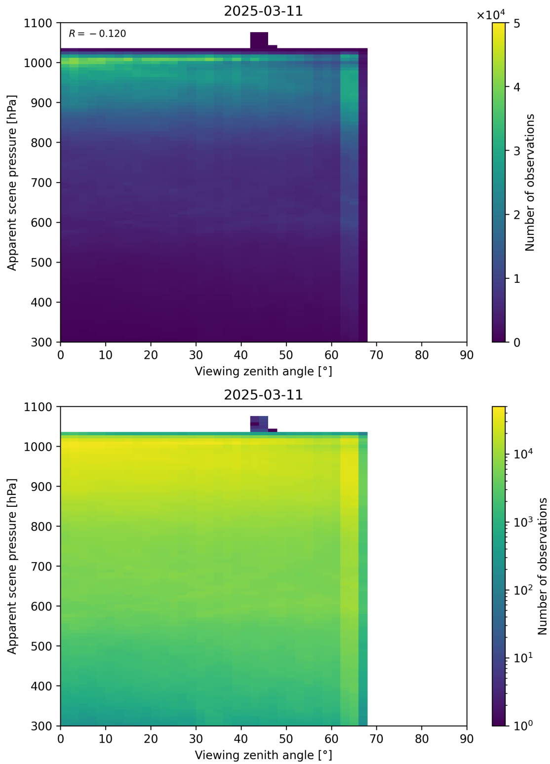
Figure 118: Scatter density plot of “Viewing zenith angle” against “Apparent scene pressure” for 2025-03-10 to 2025-03-12.
