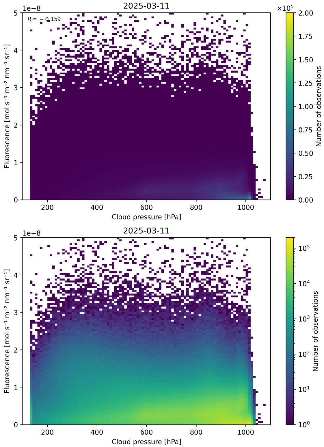
Figure 80: Scatter density plot of “Cloud pressure” against “Fluorescence” for 2025-03-10 to 2025-03-12.
