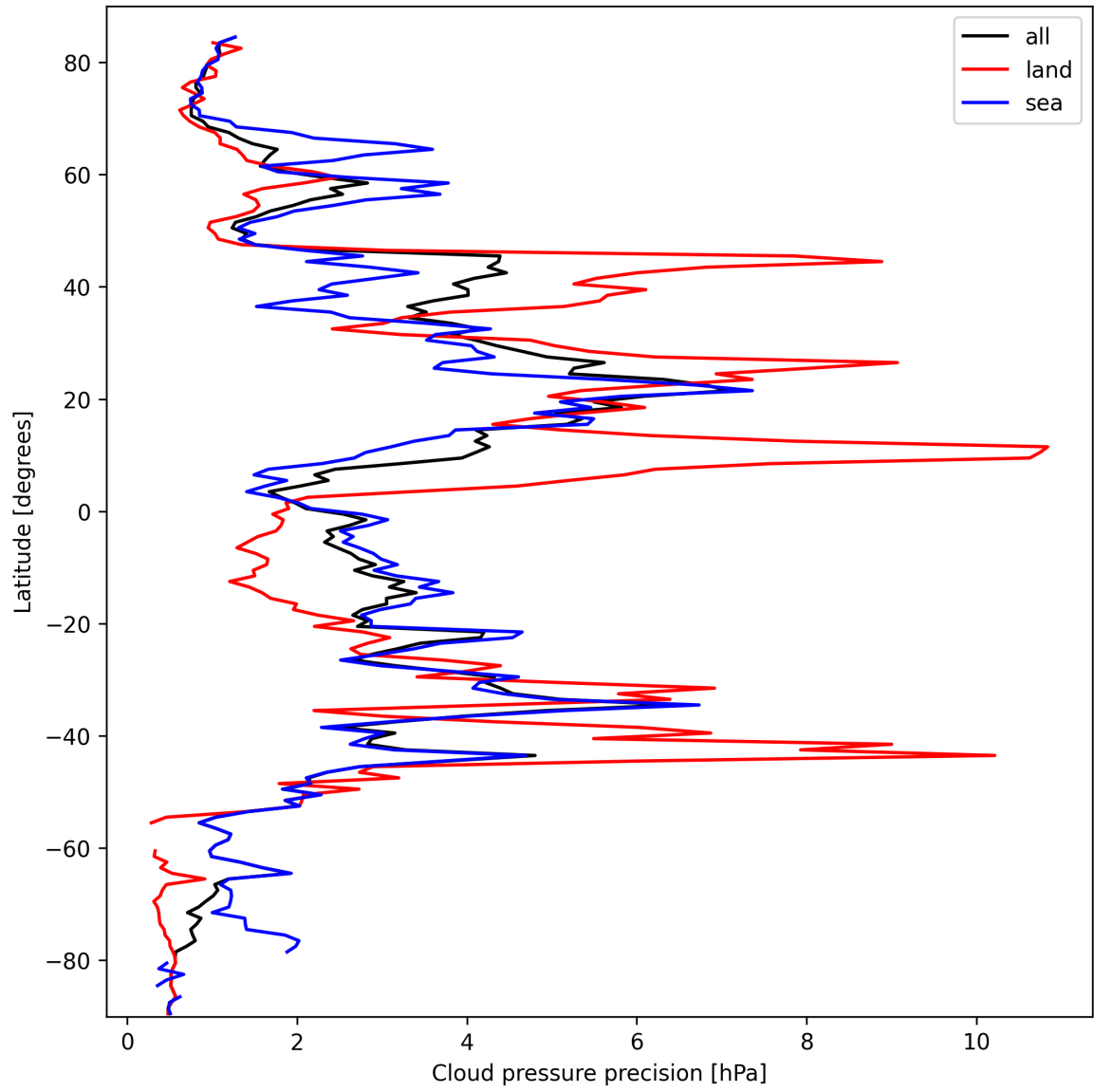
Figure 14: Zonal average of “Cloud pressure precision” for 2025-03-10 to 2025-03-12.
