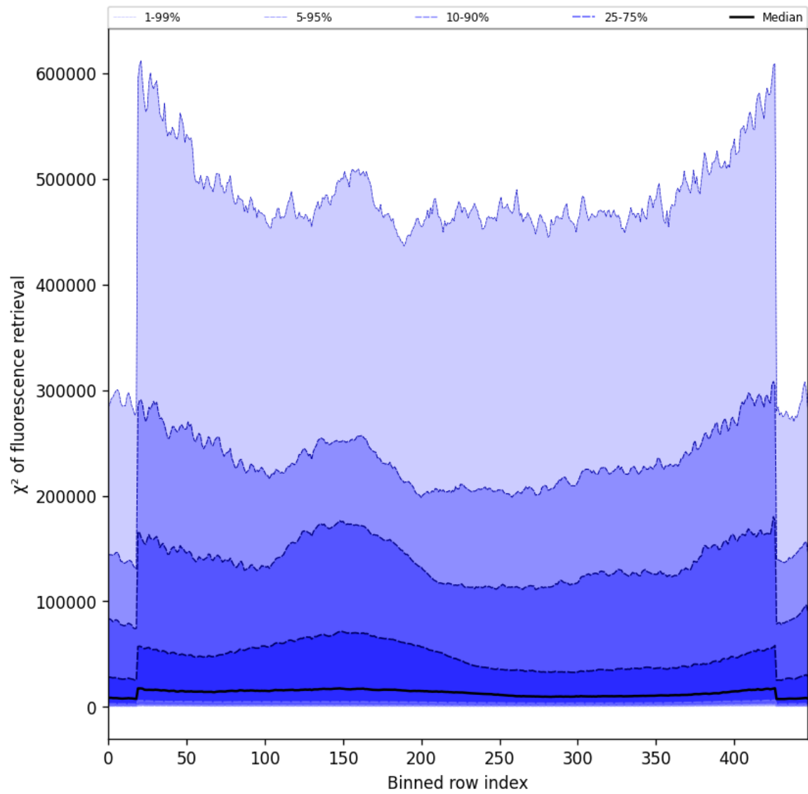
Figure 59: Along track statistics of “ \chi^2 of fluorescence retrieval” for 2025-03-10 to 2025-03-12
