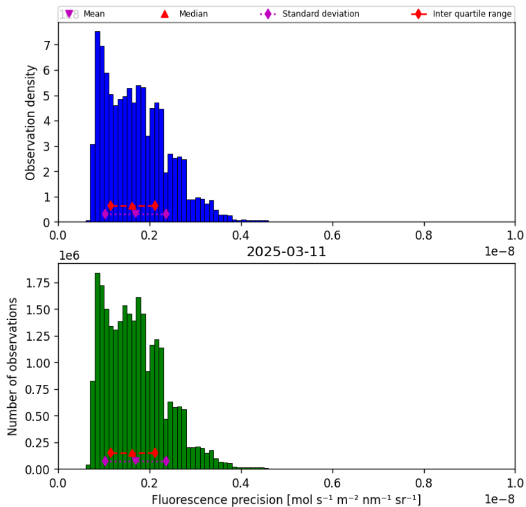
Figure 41: Histogram of “Fluorescence precision” for 2025-03-10 to 2025-03-12
