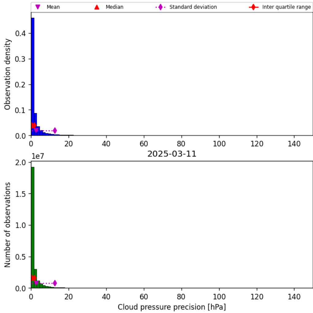
Figure 31: Histogram of “Cloud pressure precision” for 2025-03-10 to 2025-03-12
