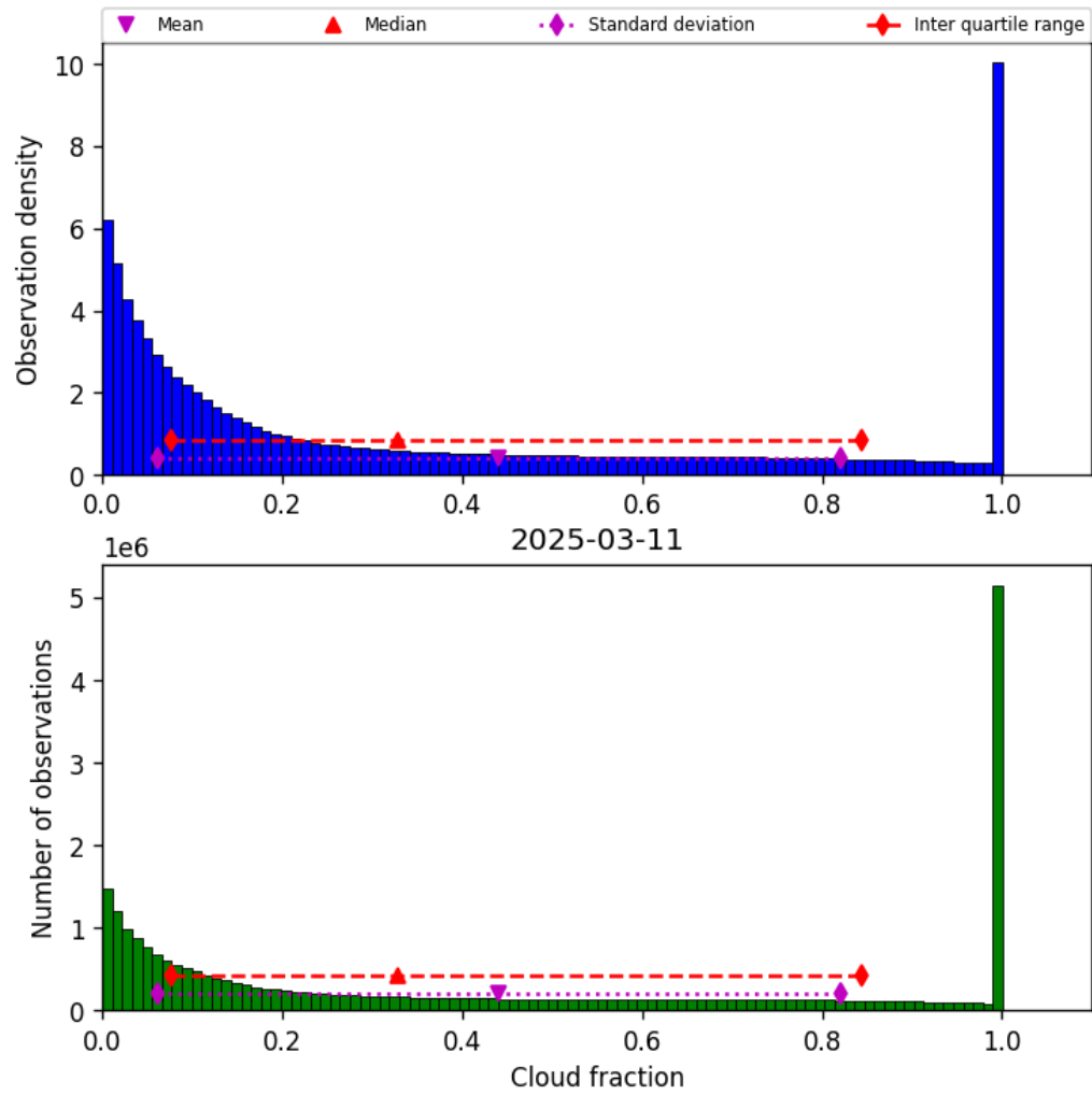
Figure 32: Histogram of “Cloud fraction” for 2025-03-10 to 2025-03-12
