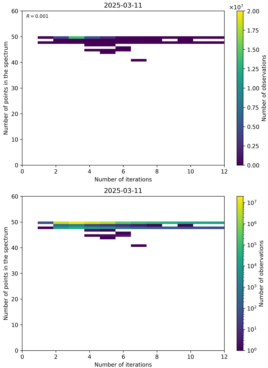
Figure 99: Scatter density plot of “Number of iterations” against “Number of points in the spectrum” for 2025-03-10 to 2025-03-12.
