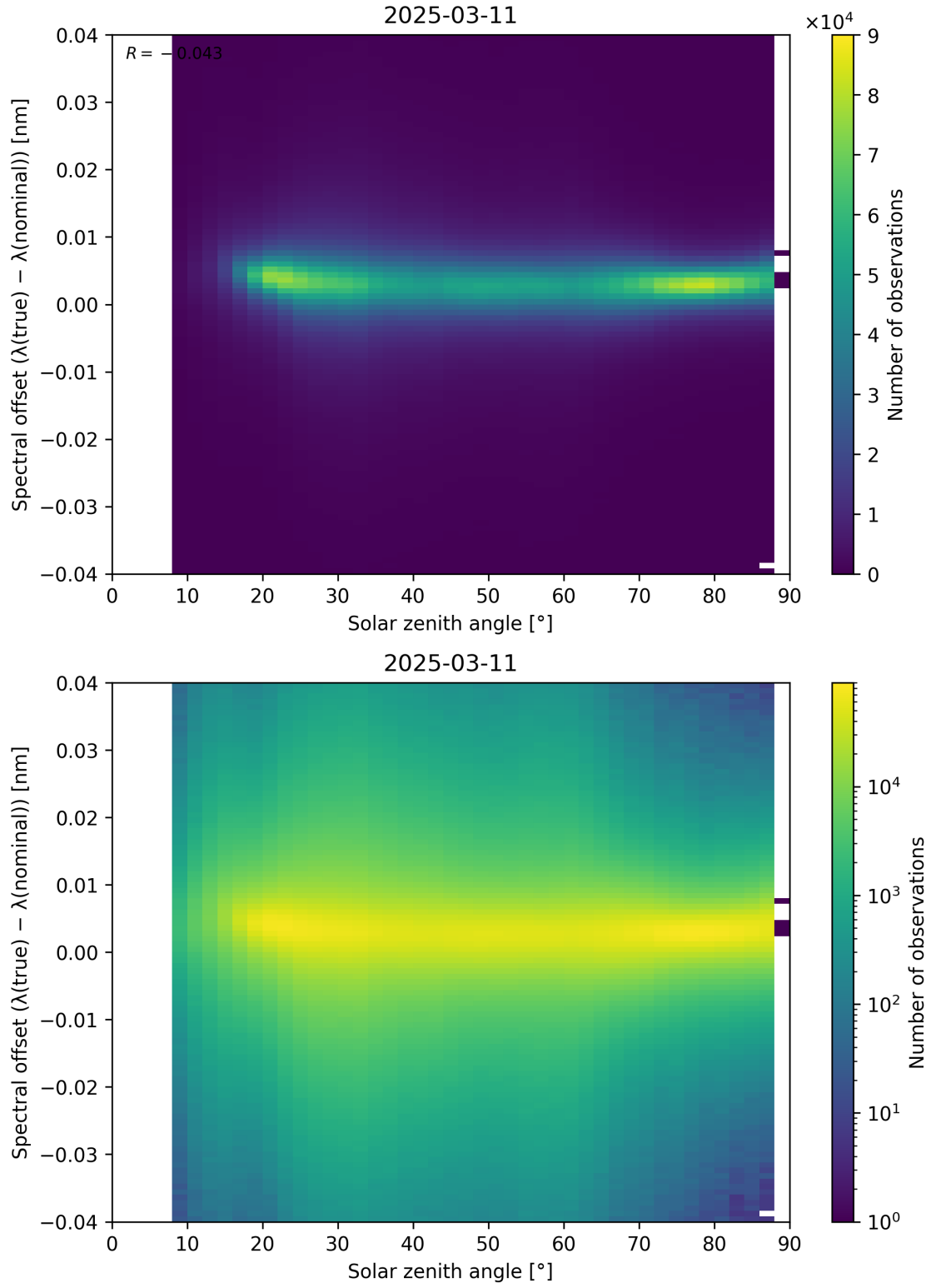
Figure 117: Scatter density plot of “Solar zenith angle” against “Spectral offset ( \lambda_{\text{true}} - \lambda_{\text{nominal}} )” for 2025-03-10 to 2025-03-12.
