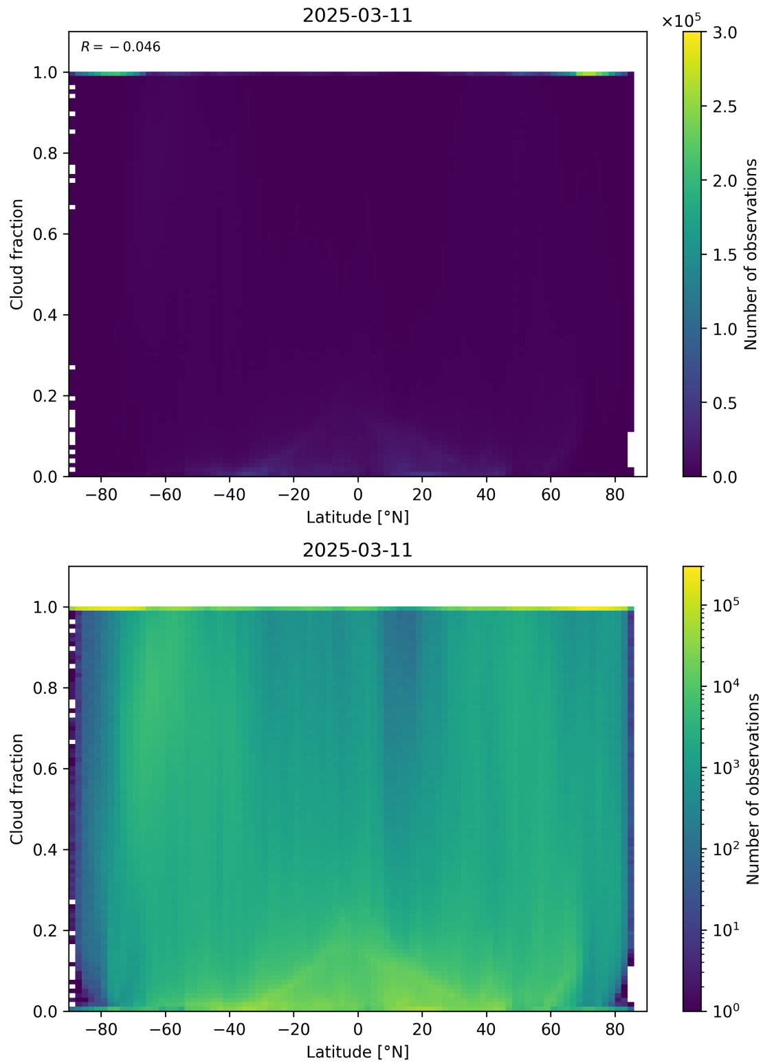
Figure 90: Scatter density plot of “Latitude” against “Cloud fraction” for 2025-03-10 to 2025-03-12.
