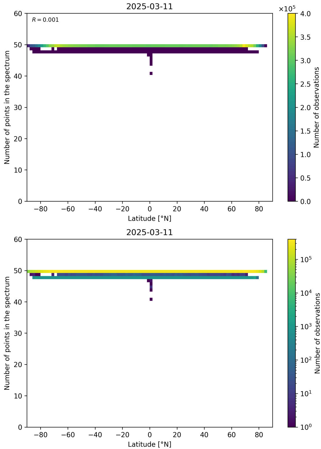
Figure 94: Scatter density plot of “Latitude” against “Number of points in the spectrum” for 2025-03-10 to 2025-03-12.
