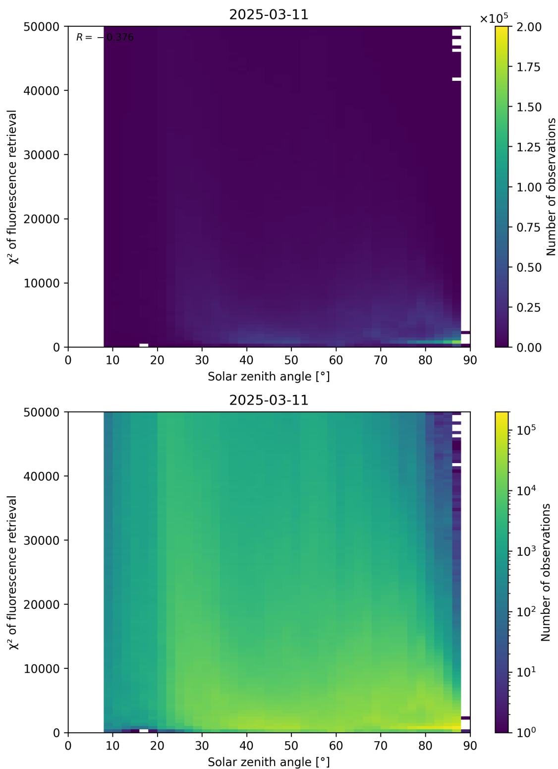
Figure 109: Scatter density plot of “Solar zenith angle” against “ \chi^2 of fluorescence retrieval” for 2025-03-10 to 2025-03-12.
