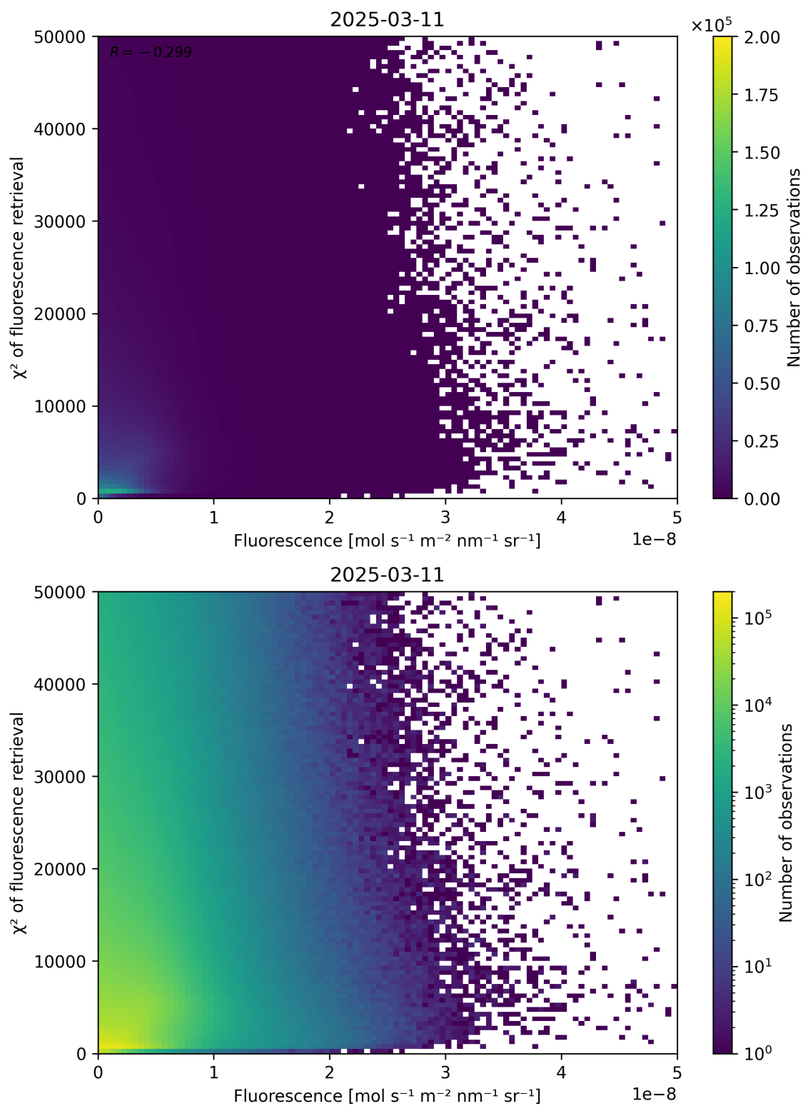
Figure 85: Scatter density plot of “Fluorescence” against “ \chi^2 of fluorescence retrieval” for 2025-03-10 to 2025-03-12.
