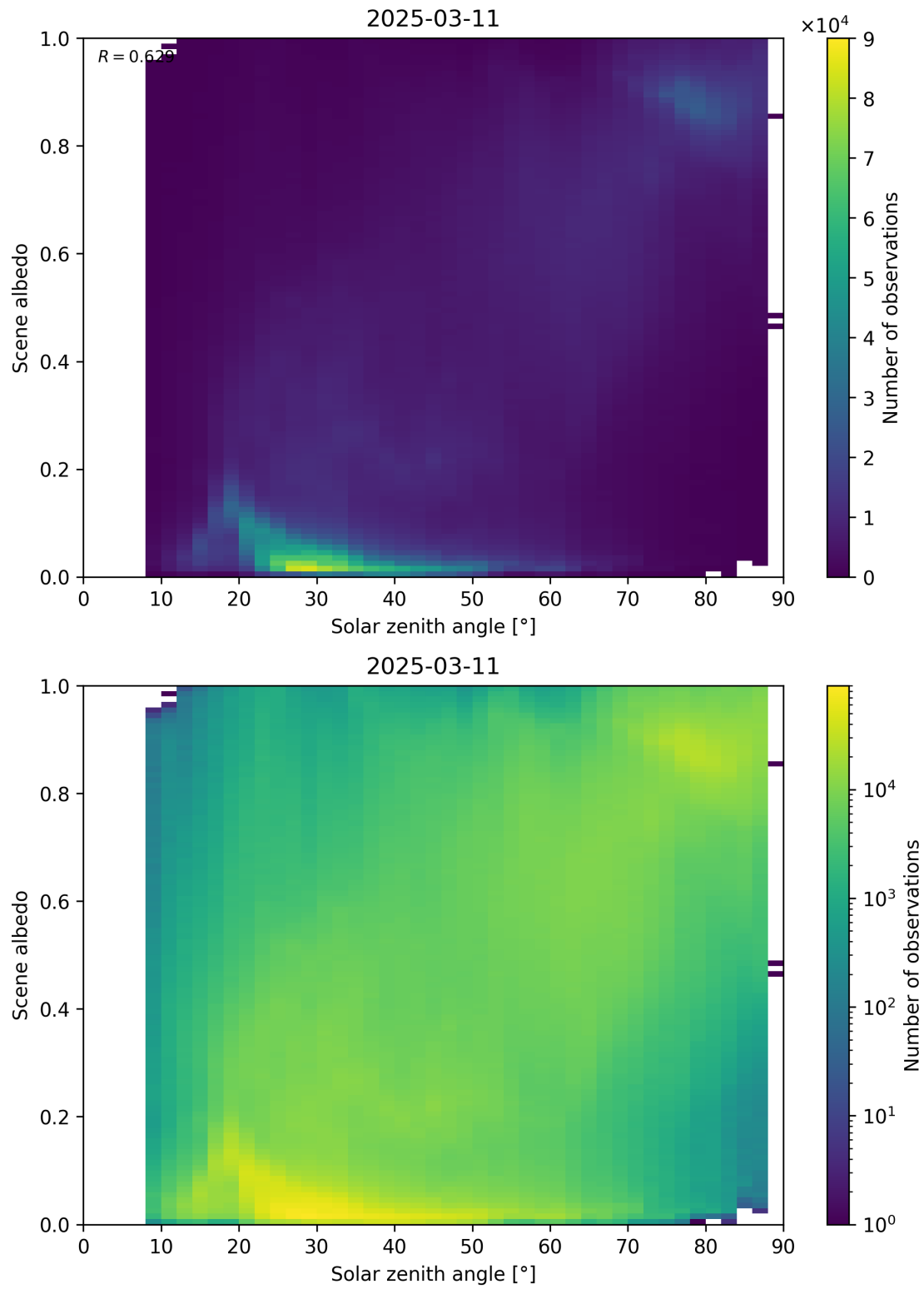
Figure 116: Scatter density plot of “Solar zenith angle” against “Scene albedo” for 2025-03-10 to 2025-03-12.
