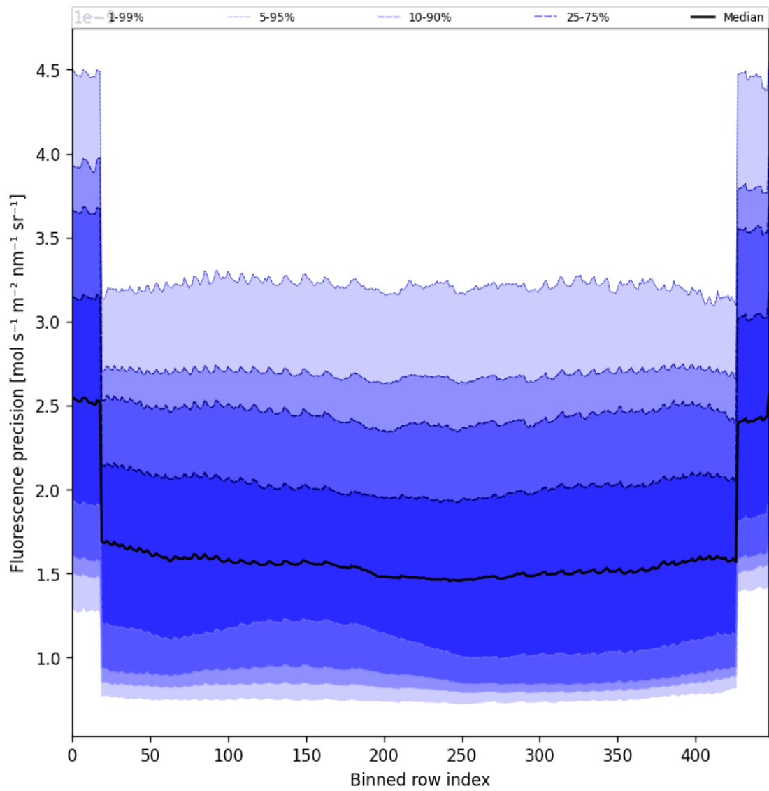
Figure 58: Along track statistics of “Fluorescence precision” for 2025-03-10 to 2025-03-12
