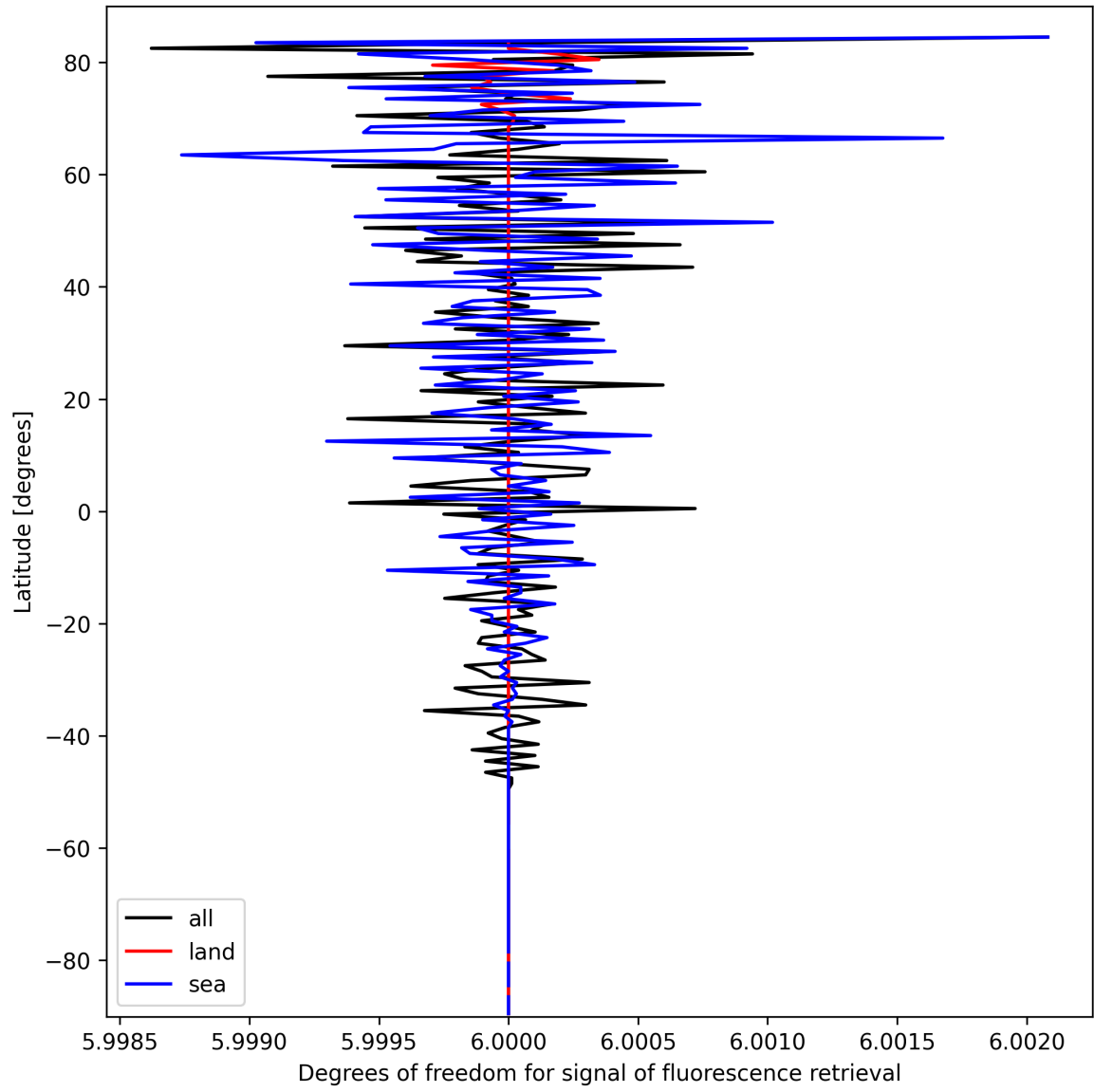
Figure 26: Zonal average of “Degrees of freedom for signal of fluorescence retrieval” for 2025-03-10 to 2025-03-12.
