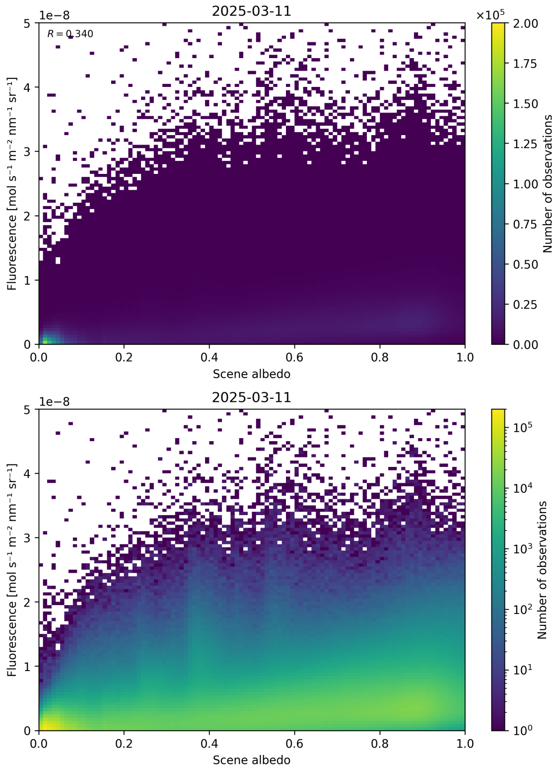
Figure 104: Scatter density plot of “Scene albedo” against “Fluorescence” for 2025-03-10 to 2025-03-12.
