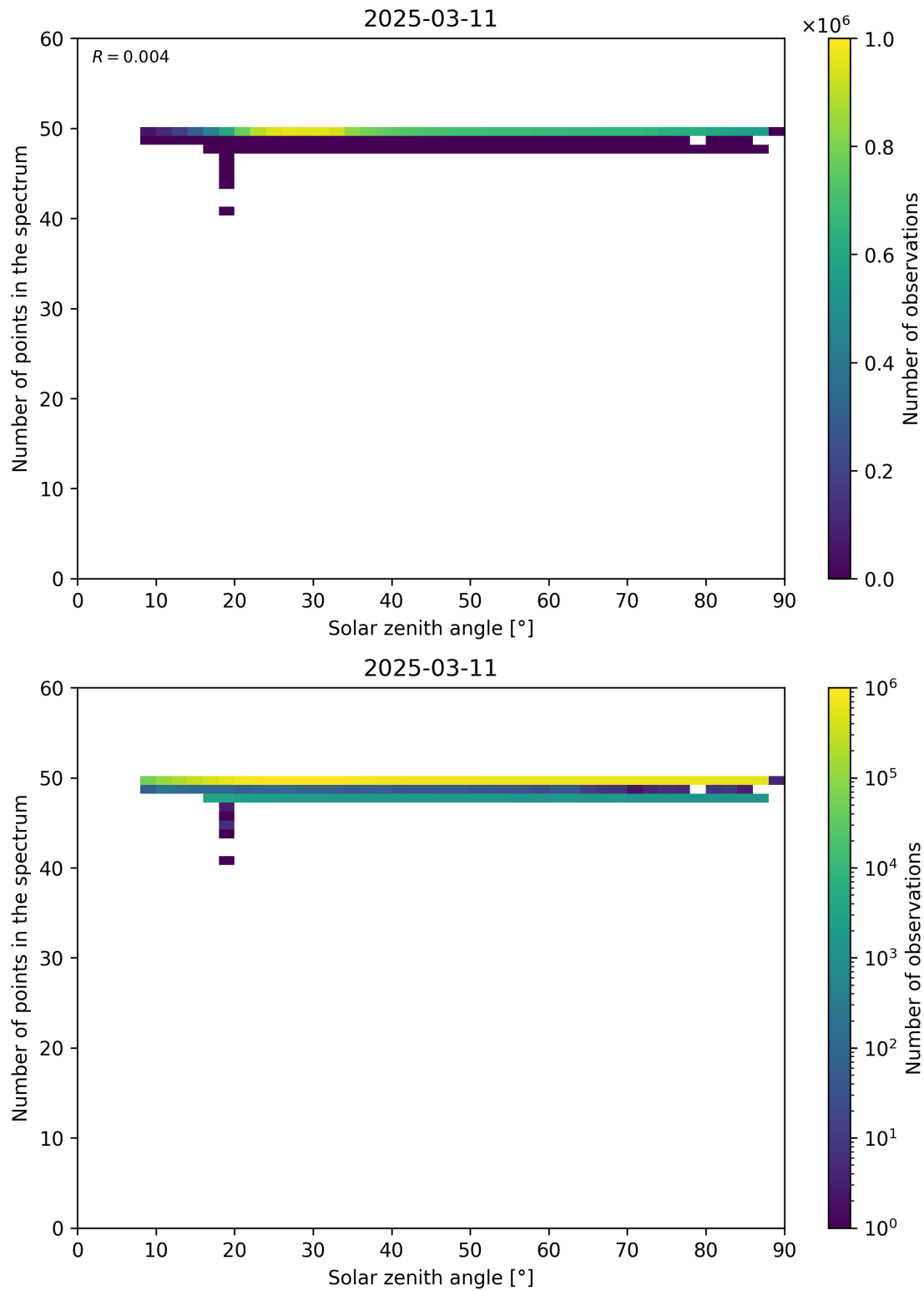
Figure 115: Scatter density plot of “Solar zenith angle” against “Number of points in the spectrum” for 2025-03-10 to 2025-03-12.
