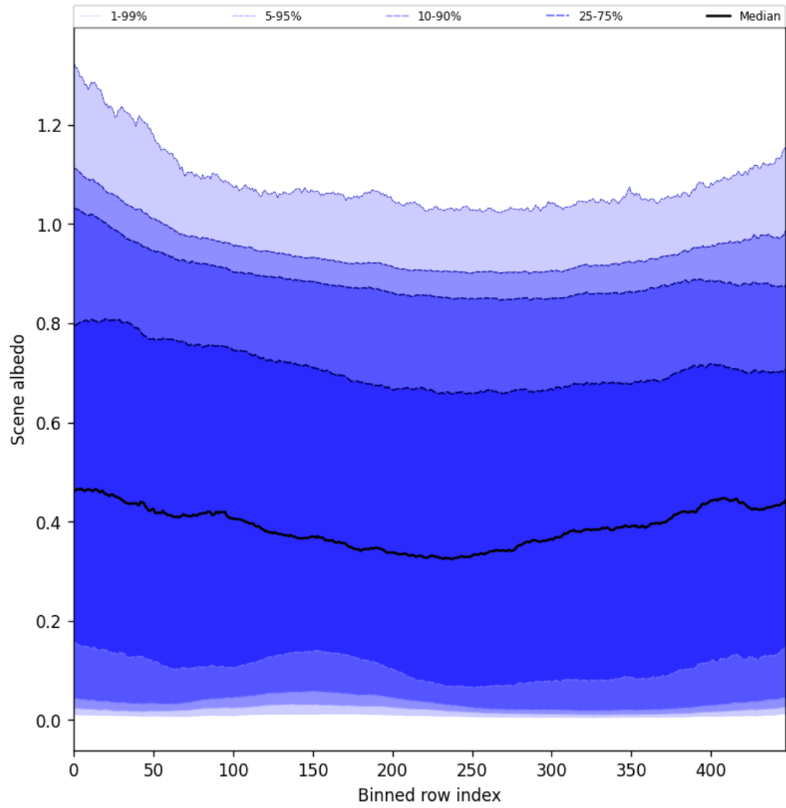
Figure 51: Along track statistics of “Scene albedo” for 2025-03-10 to 2025-03-12
