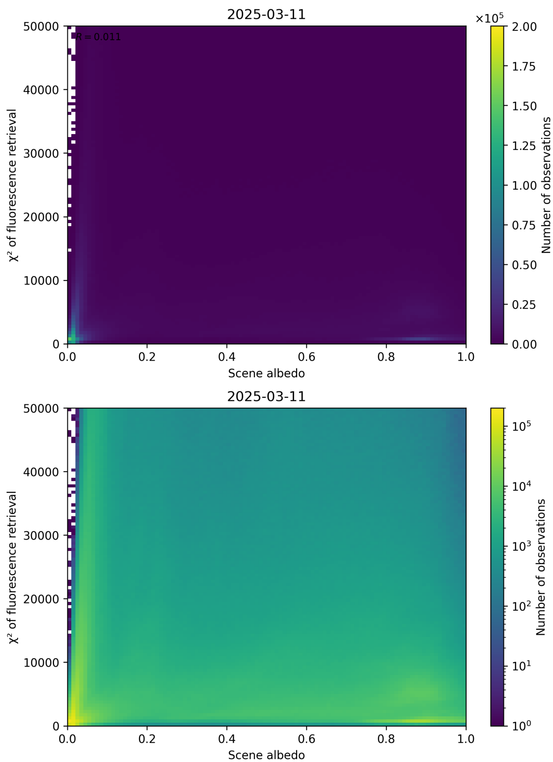
Figure 103: Scatter density plot of “Scene albedo” against “ \chi^2 of fluorescence retrieval” for 2025-03-10 to 2025-03-12.
