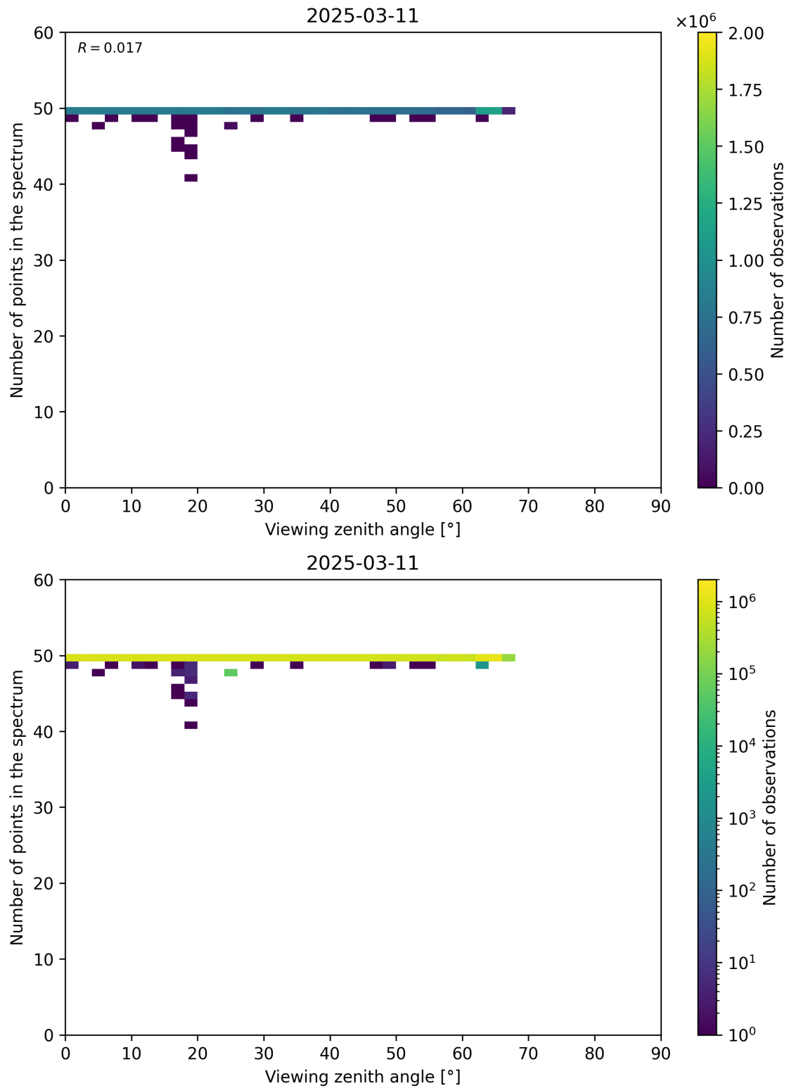
Figure 125: Scatter density plot of “Viewing zenith angle” against “Number of points in the spectrum” for 2025-03-10 to 2025-03-12.
