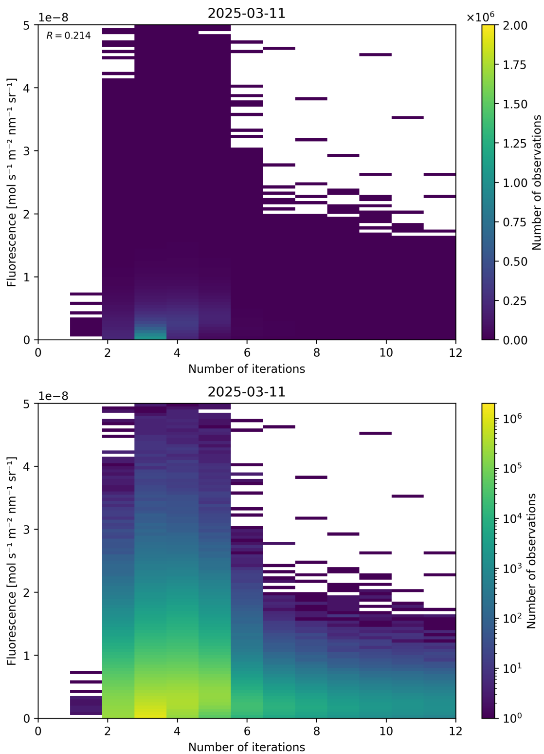
Figure 98: Scatter density plot of “Number of iterations” against “Fluorescence” for 2025-03-10 to 2025-03-12.
