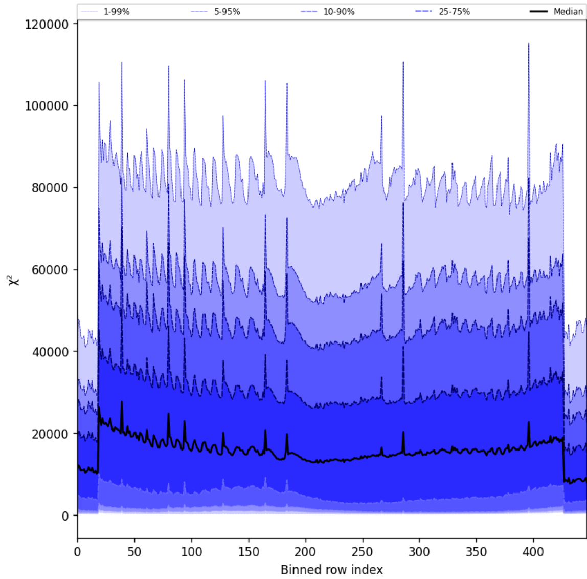
Figure 55: Along track statistics of “ \chi^2 ” for 2025-03-10 to 2025-03-12
