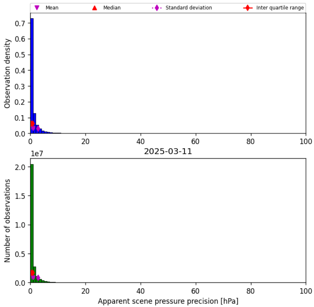
Figure 37: Histogram of “Apparent scene pressure precision” for 2025-03-10 to 2025-03-12
