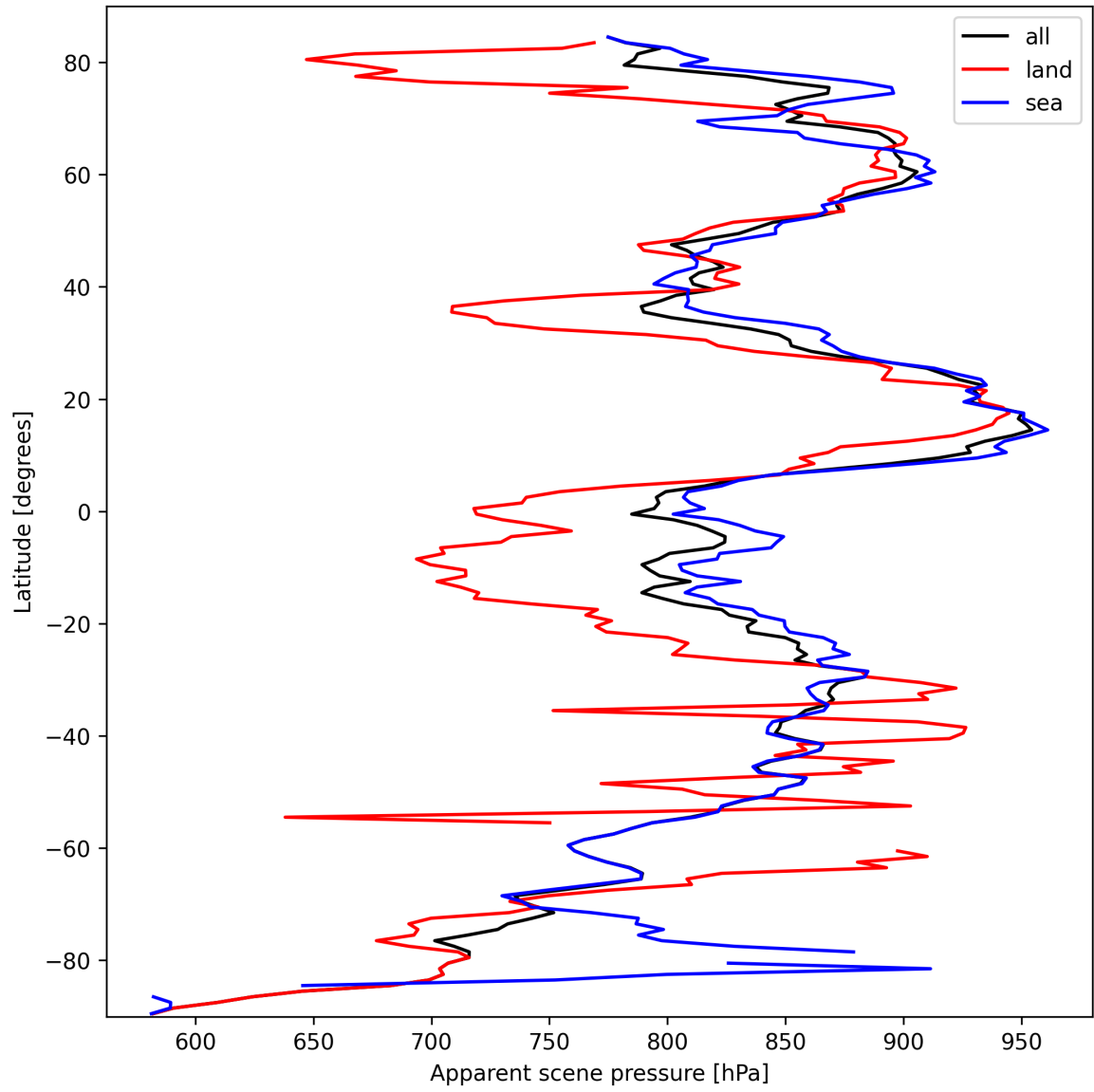
Figure 19: Zonal average of “Apparent scene pressure” for 2025-03-10 to 2025-03-12.
