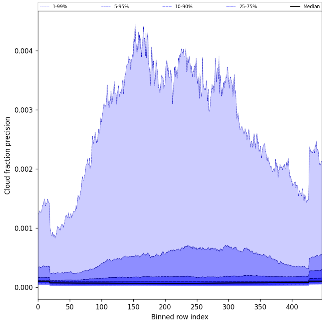
Figure 50: Along track statistics of “Cloud fraction precision” for 2025-03-10 to 2025-03-12
