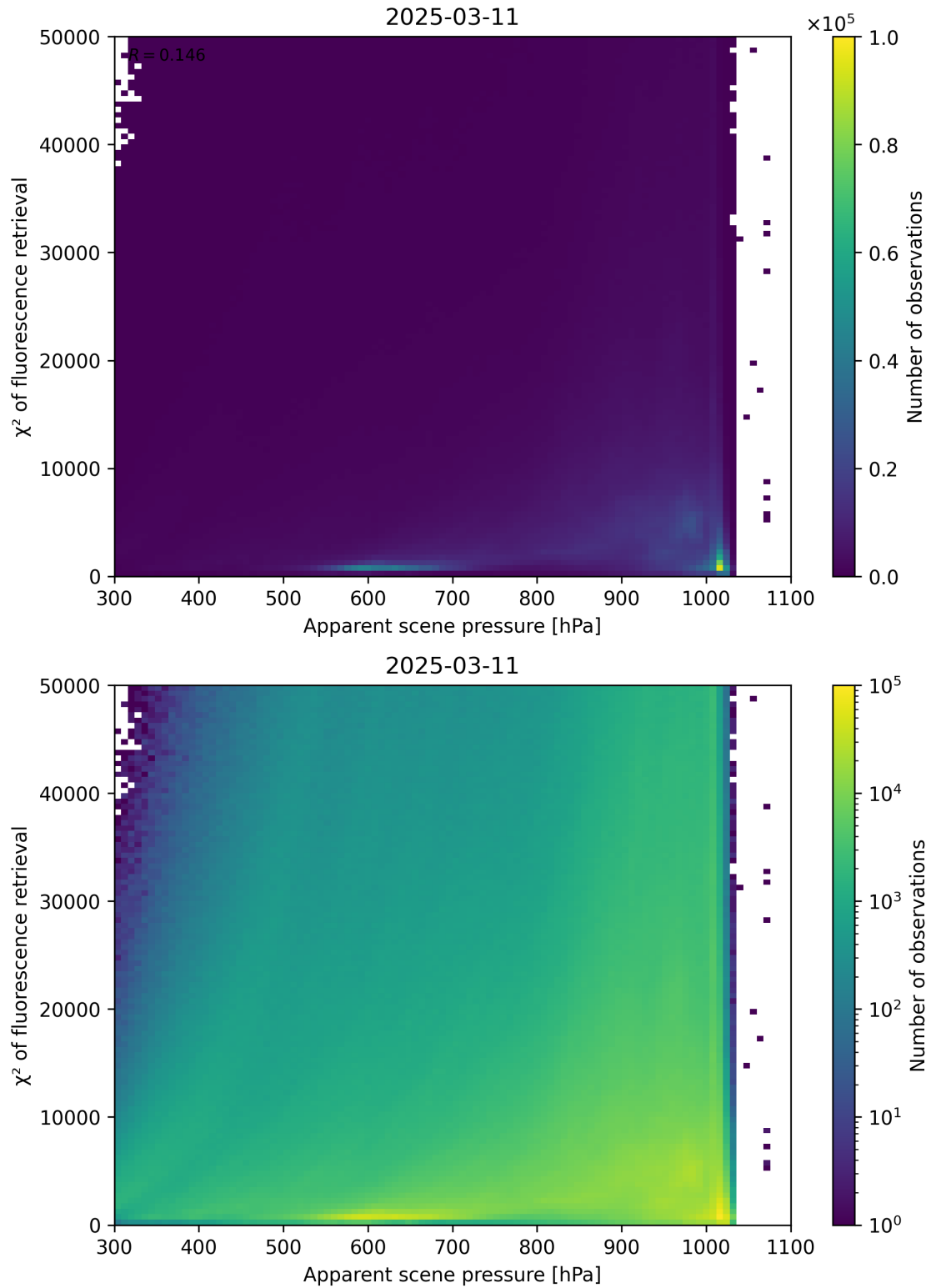
Figure 63: Scatter density plot of “Apparent scene pressure” against “ \chi^2 of fluorescence retrieval” for 2025-03-10 to 2025-03-12.
