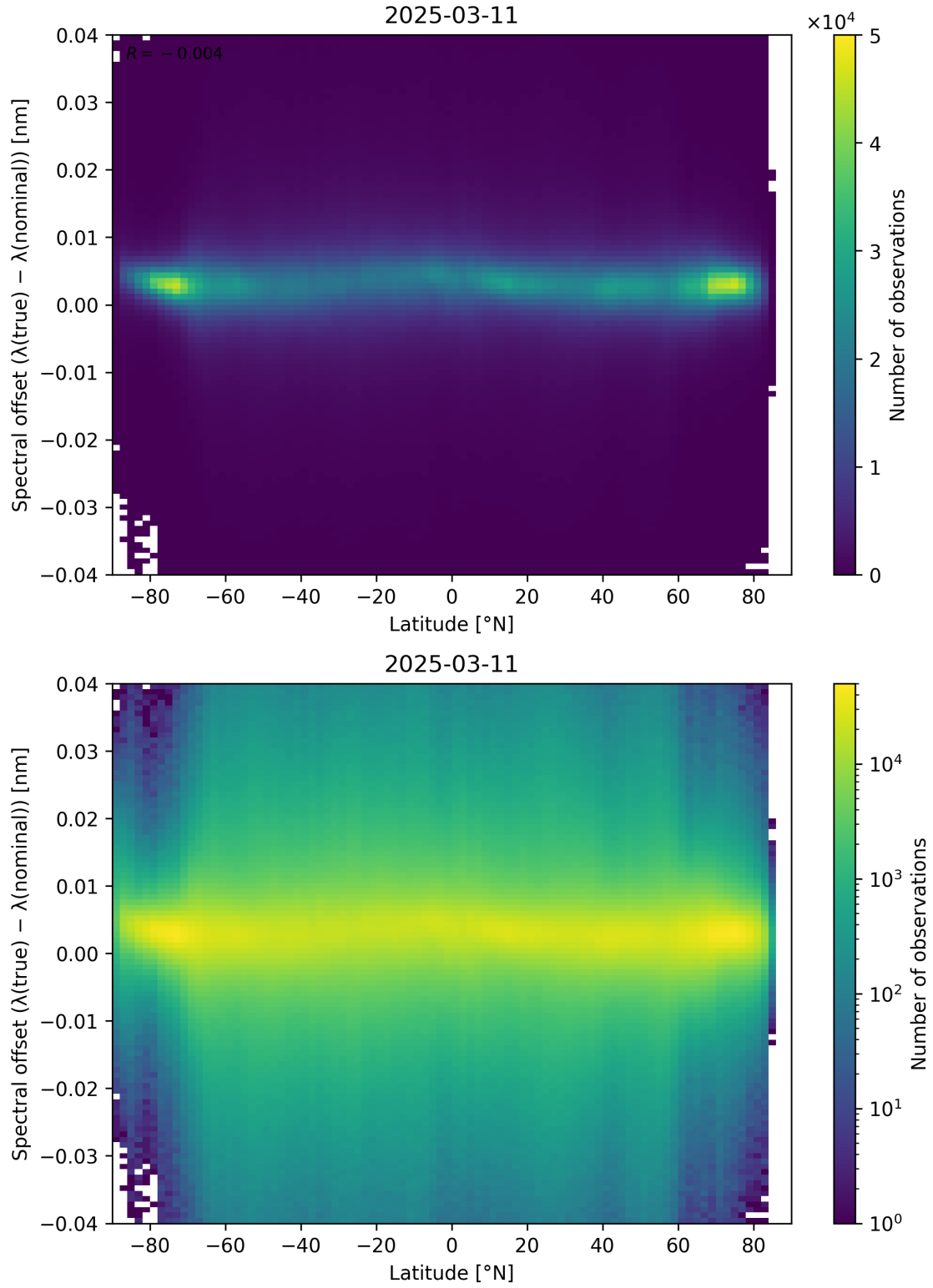
Figure 96: Scatter density plot of “Latitude” against “Spectral offset ( \lambda_{\text{true}} - \lambda_{\text{nominal}} )” for 2025-03-10 to 2025-03-12.
