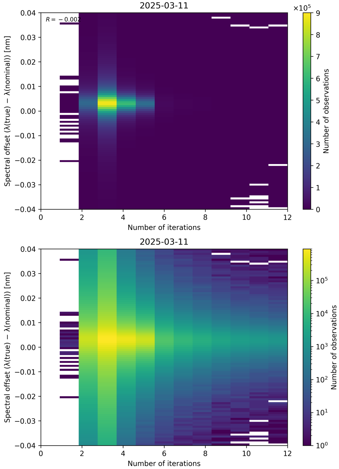
Figure 100: Scatter density plot of “Number of iterations” against “Spectral offset ( \lambda_{\text{true}} - \lambda_{\text{nominal}} )” for 2025-03-10 to 2025-03-12.
