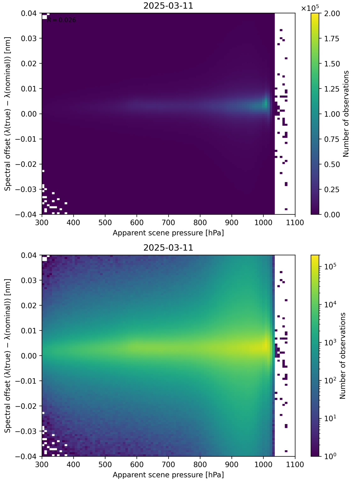
Figure 67: Scatter density plot of “Apparent scene pressure” against “Spectral offset ( \lambda_{\text{true}} - \lambda_{\text{nominal}} )” for 2025-03-10 to 2025-03-12.
