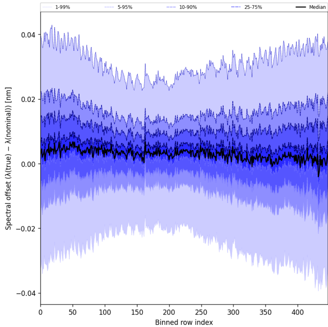
Figure 62: Along track statistics of “Spectral offset ( \lambda_{\text{true}} - \lambda_{\text{nominal}} )” for 2025-03-10 to 2025-03-12
