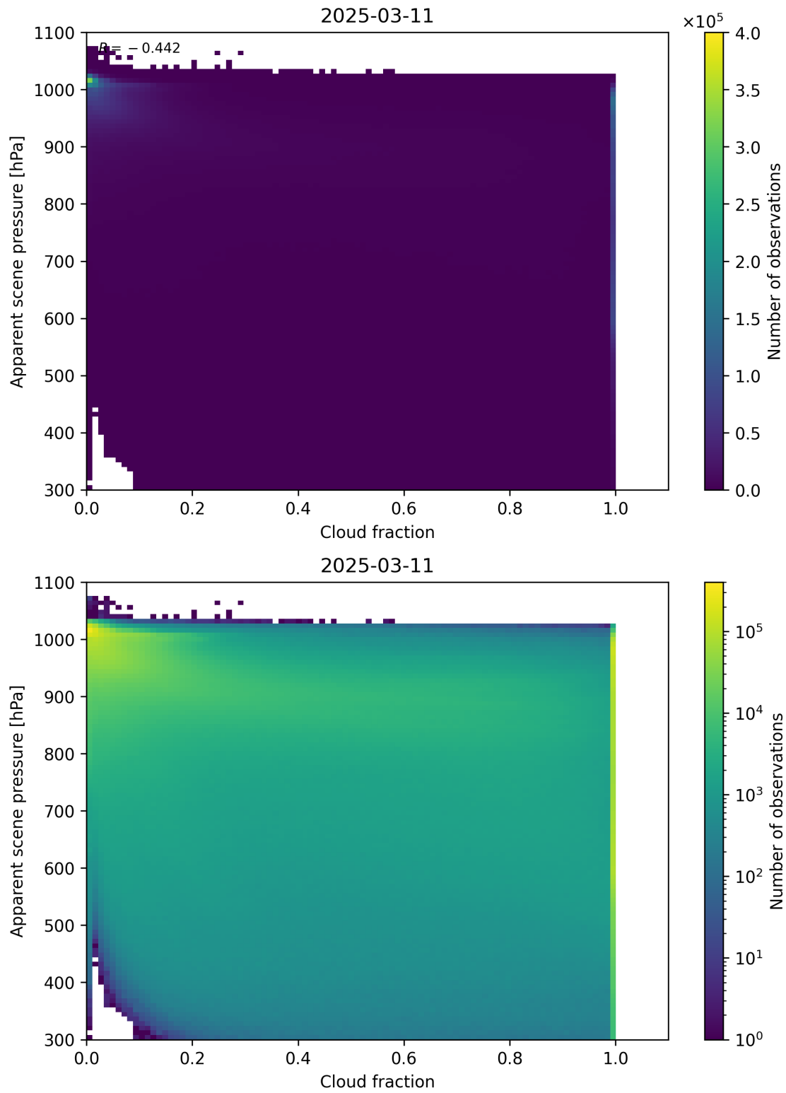
Figure 70: Scatter density plot of “Cloud fraction” against “Apparent scene pressure” for 2025-03-10 to 2025-03-12.
