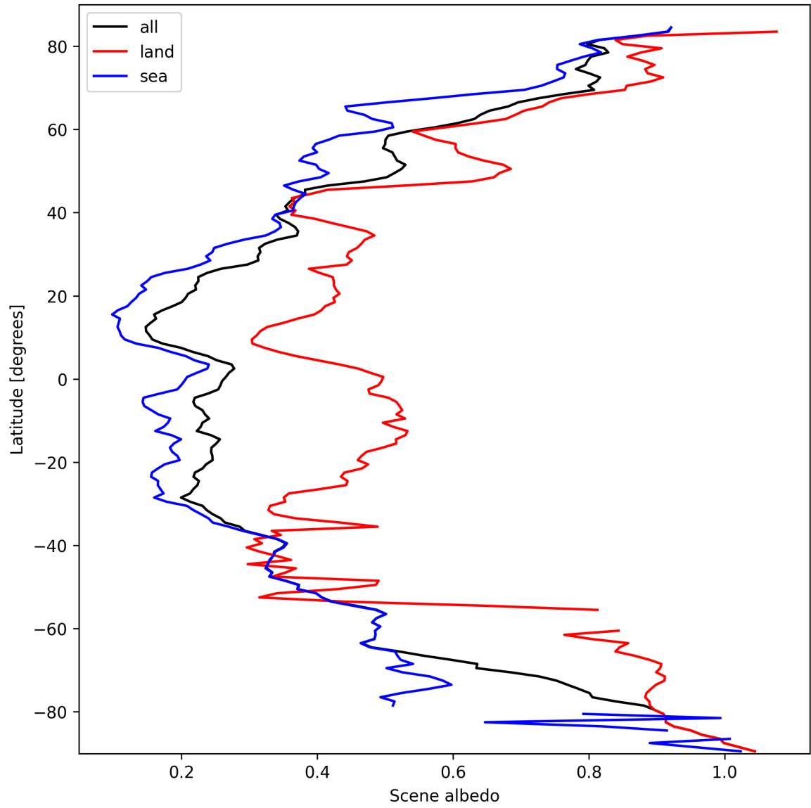
Figure 17: Zonal average of "Scene albedo" for 2025-03-10 to 2025-03-12.
