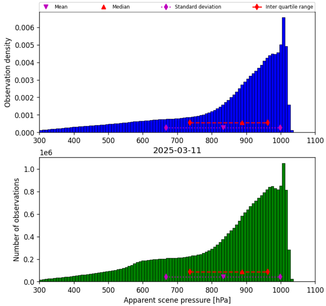
Figure 36: Histogram of “Apparent scene pressure” for 2025-03-10 to 2025-03-12
