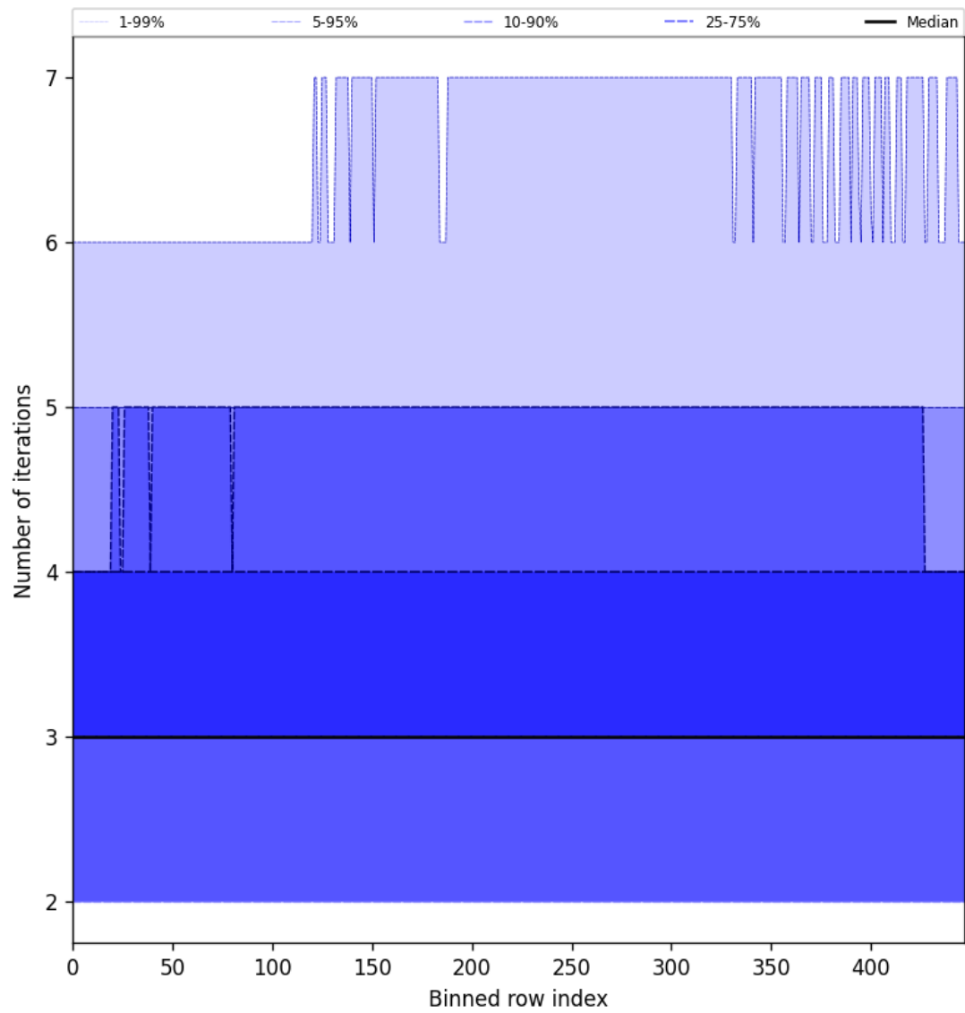
Figure 56: Along track statistics of “Number of iterations” for 2025-03-10 to 2025-03-12
