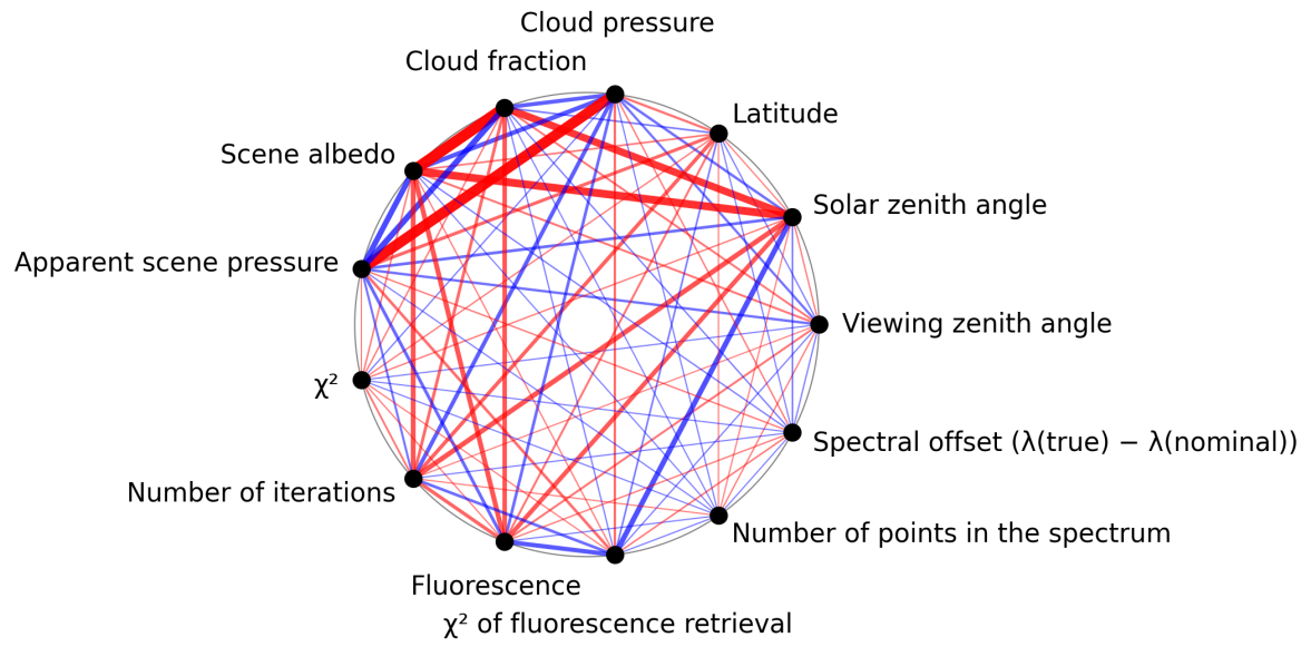
Figure 1: Map of correlation graph for 2025-03-10 to 2025-03-12.
