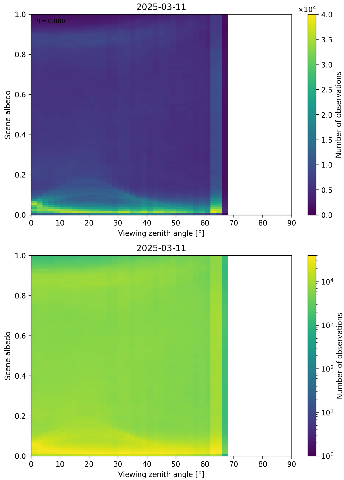
Figure 126: Scatter density plot of “Viewing zenith angle” against “Scene albedo” for 2025-03-10 to 2025-03-12.
