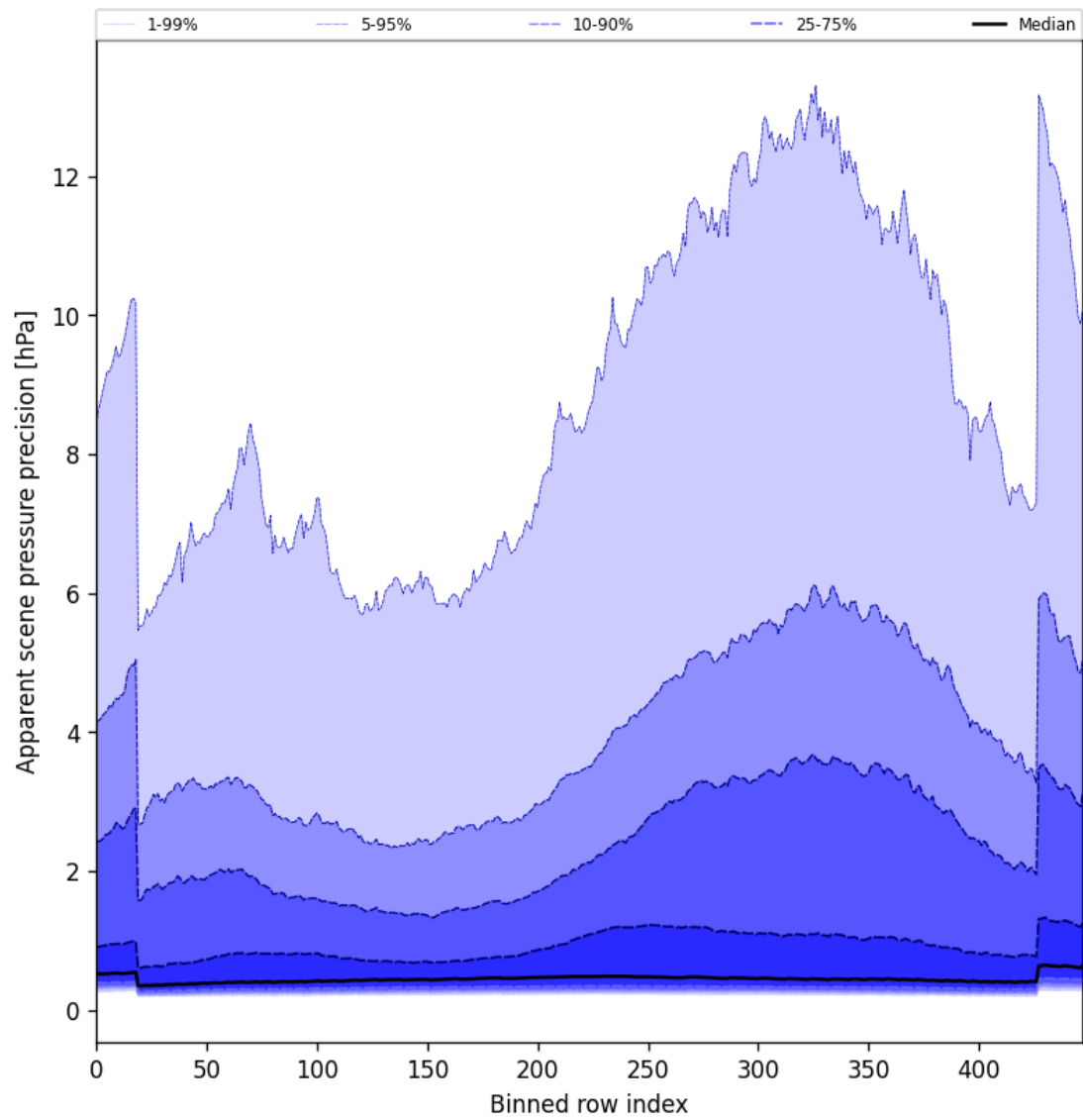
Figure 54: Along track statistics of “Apparent scene pressure precision” for 2025-03-10 to 2025-03-12
