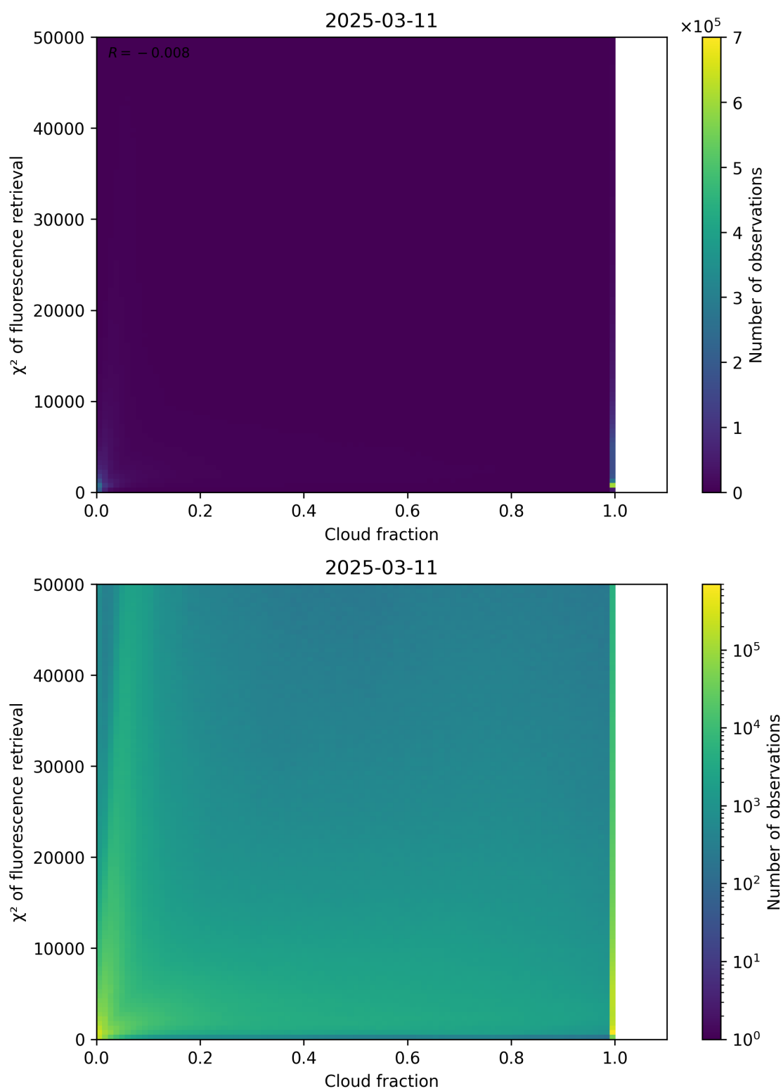
Figure 71: Scatter density plot of “Cloud fraction” against “ \chi^2 of fluorescence retrieval” for 2025-03-10 to 2025-03-12.
