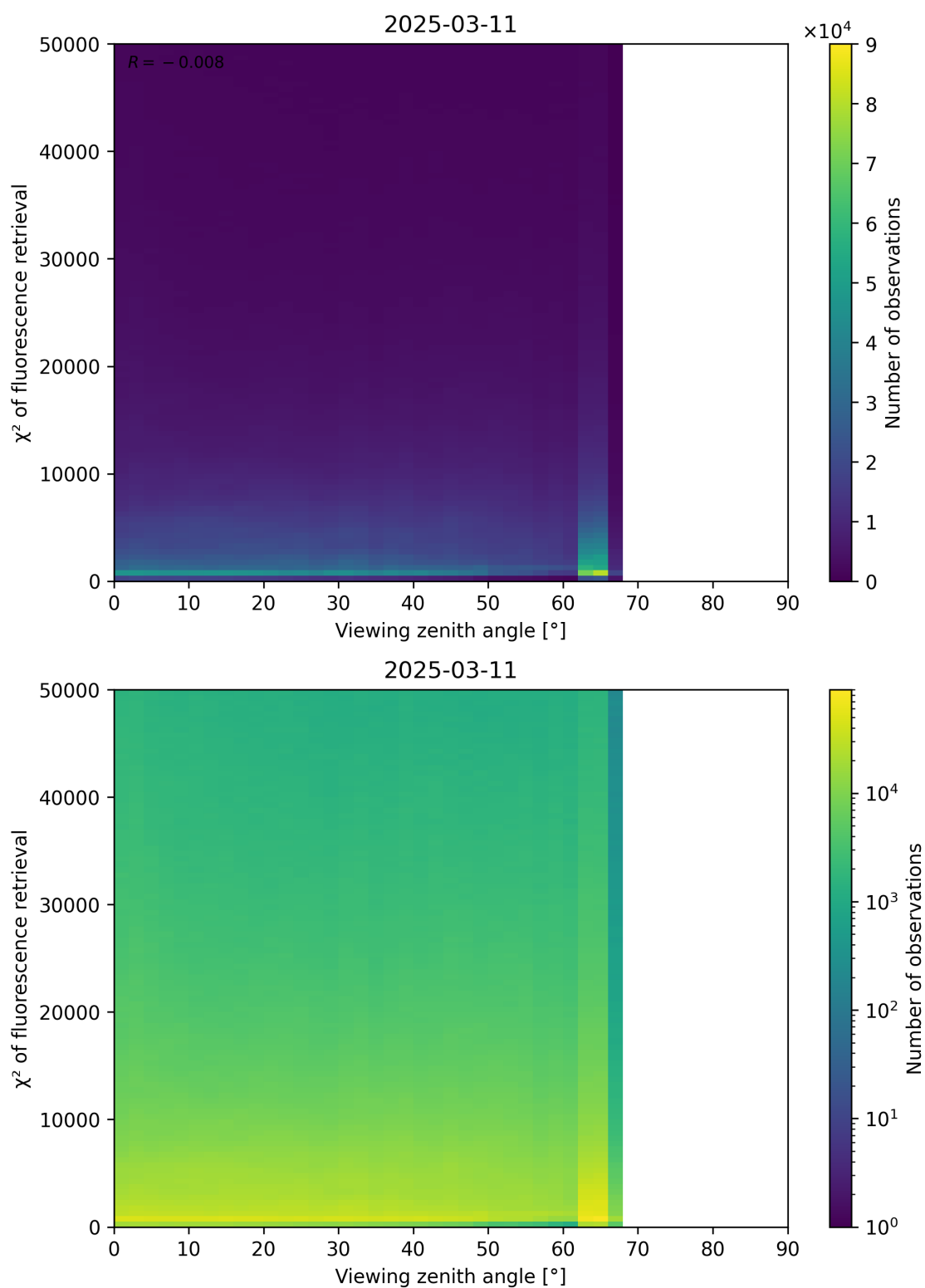
Figure 119: Scatter density plot of “Viewing zenith angle” against “ \chi^2 of fluorescence retrieval” for 2025-03-10 to 2025-03-12.
