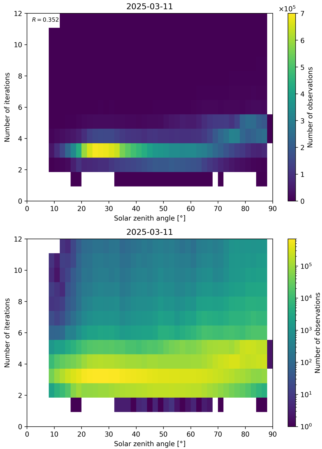
Figure 114: Scatter density plot of “Solar zenith angle” against “Number of iterations” for 2025-03-10 to 2025-03-12.
