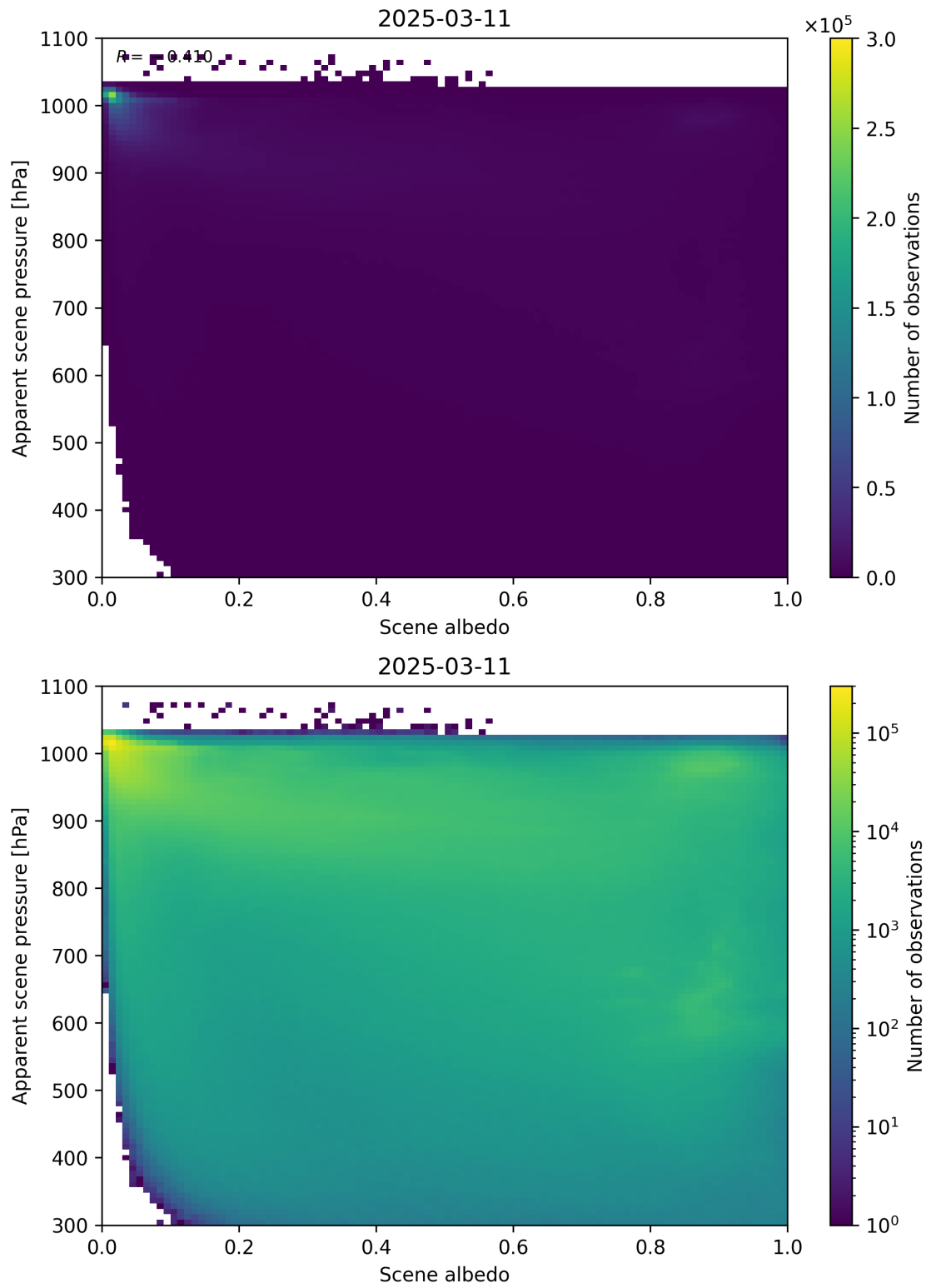
Figure 102: Scatter density plot of “Scene albedo” against “Apparent scene pressure” for 2025-03-10 to 2025-03-12.
