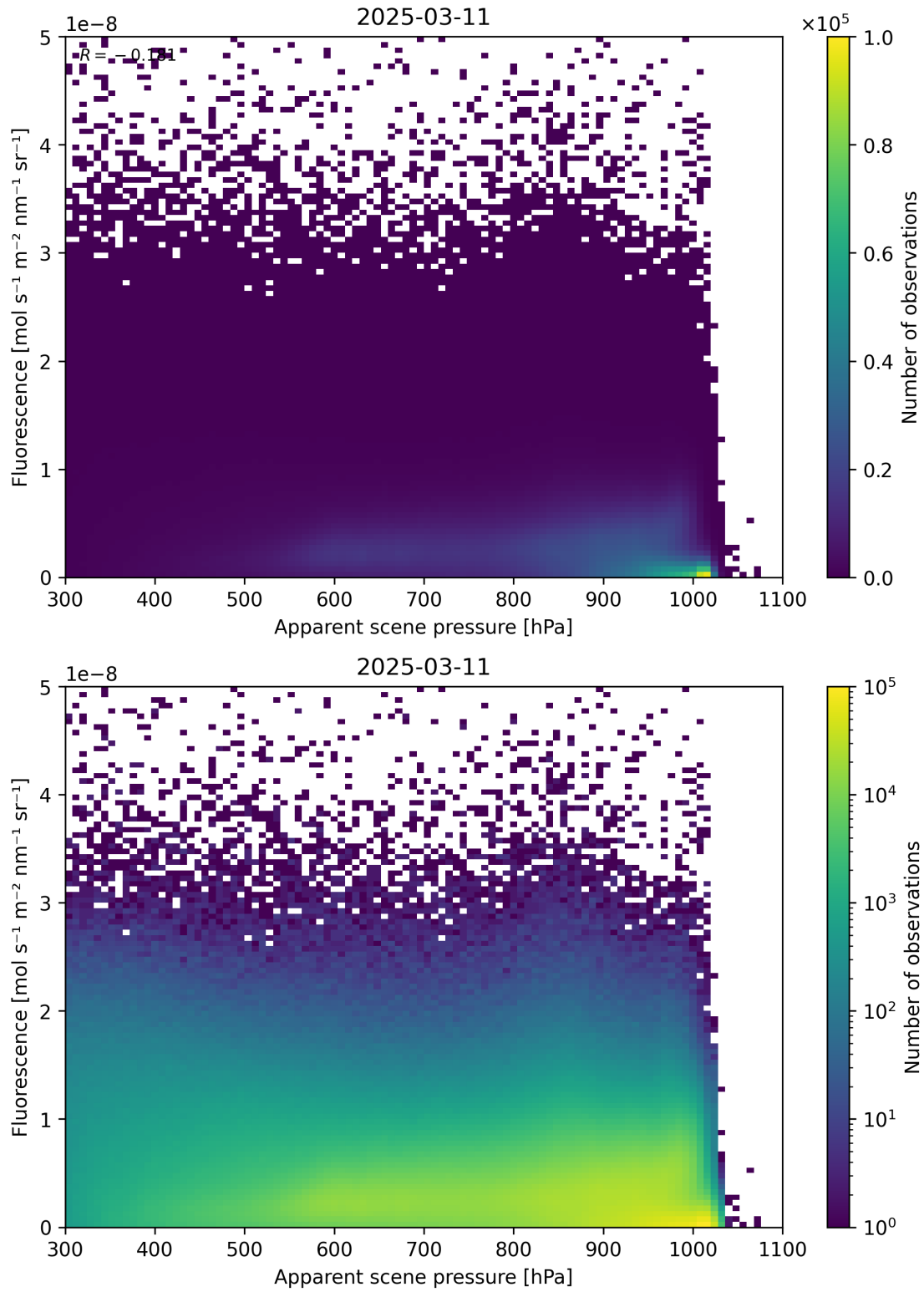
Figure 64: Scatter density plot of “Apparent scene pressure” against “Fluorescence” for 2025-03-10 to 2025-03-12.
