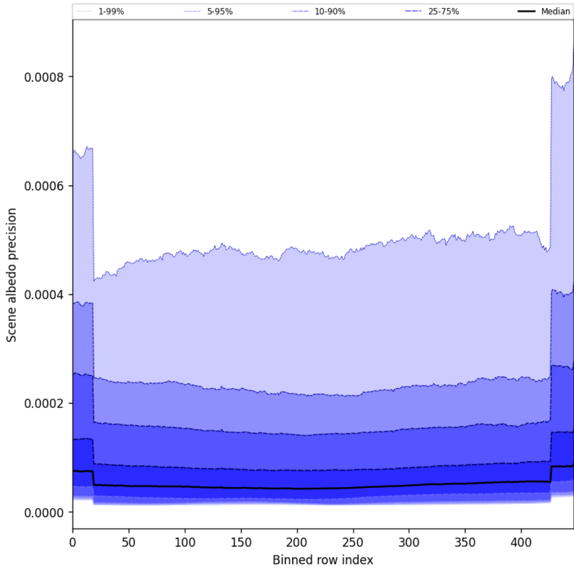
Figure 52: Along track statistics of “Scene albedo precision” for 2025-03-10 to 2025-03-12
