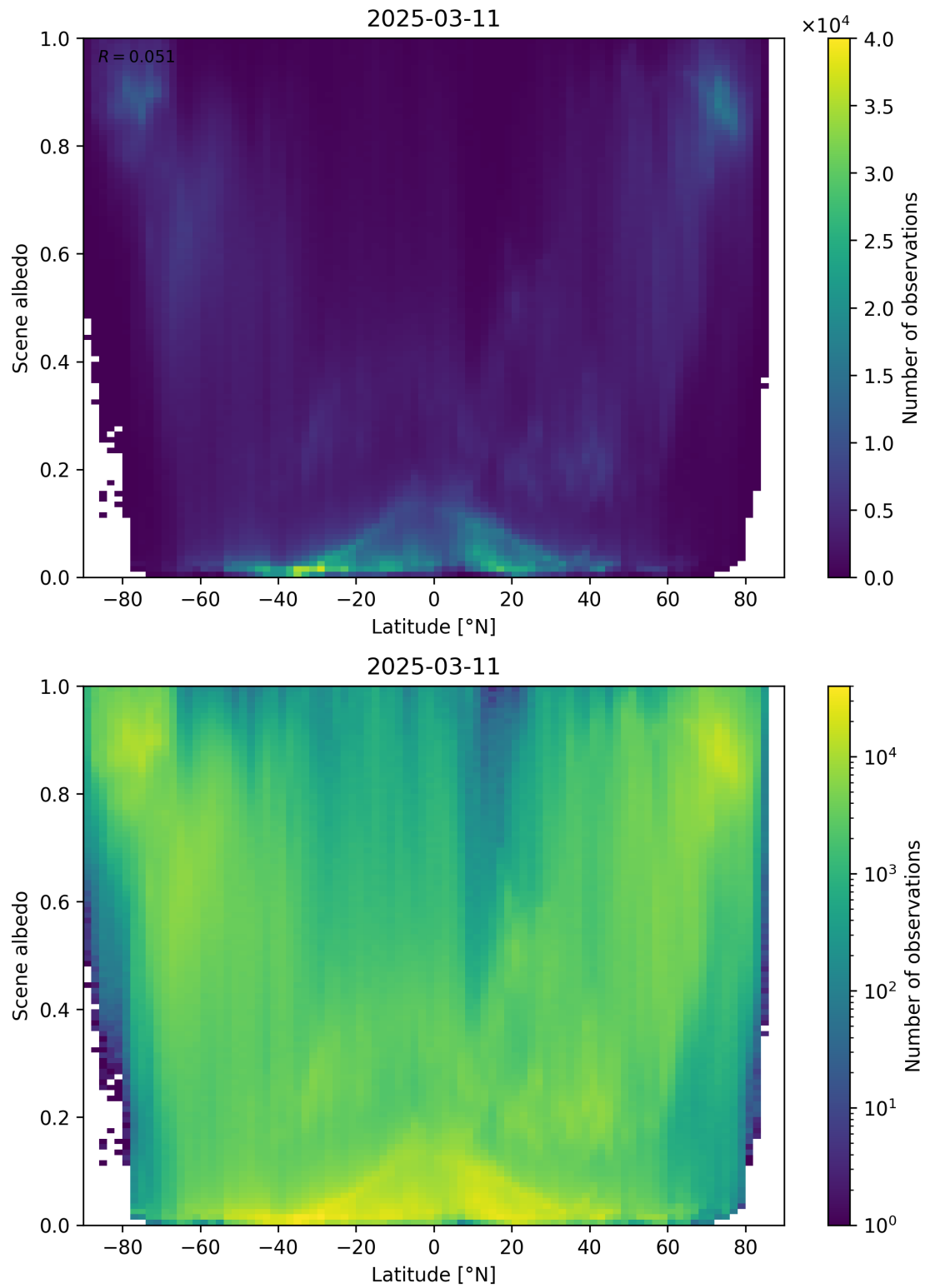
Figure 95: Scatter density plot of “Latitude” against “Scene albedo” for 2025-03-10 to 2025-03-12.
