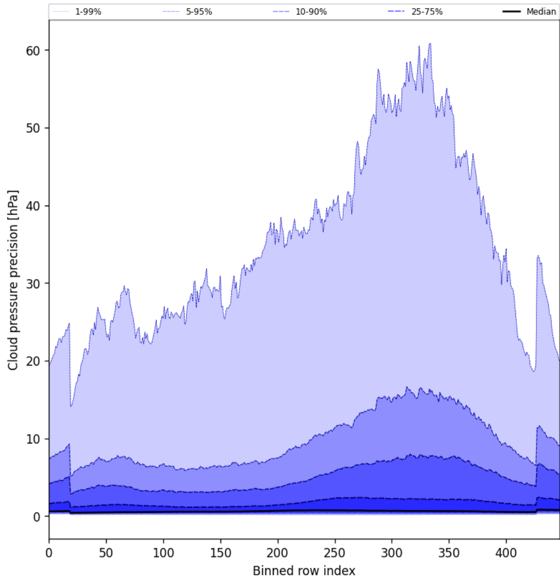
Figure 48: Along track statistics of “Cloud pressure precision” for 2025-03-10 to 2025-03-12
