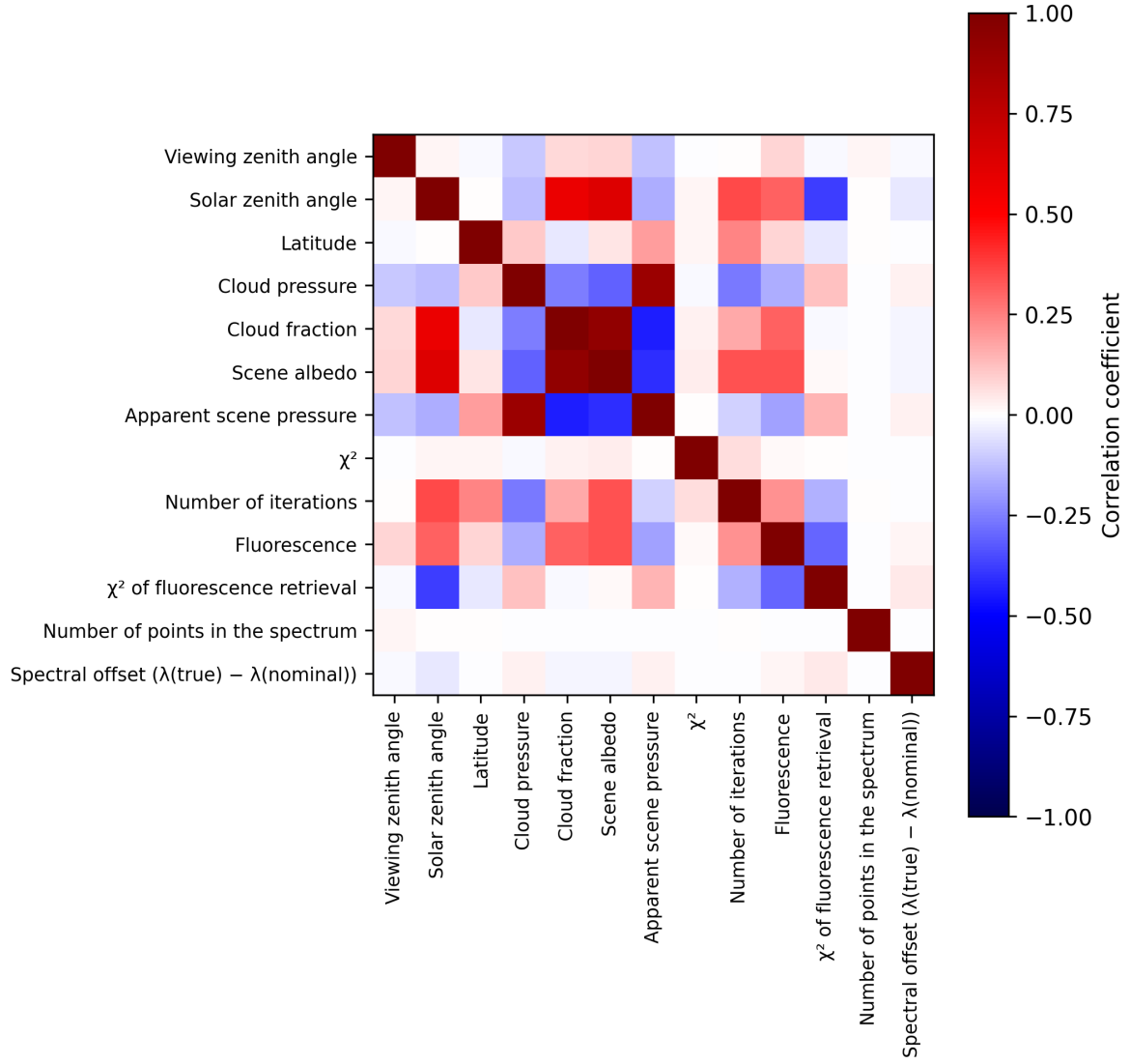
Figure 2: Map of correlation matrix for 2025-03-10 to 2025-03-12.
