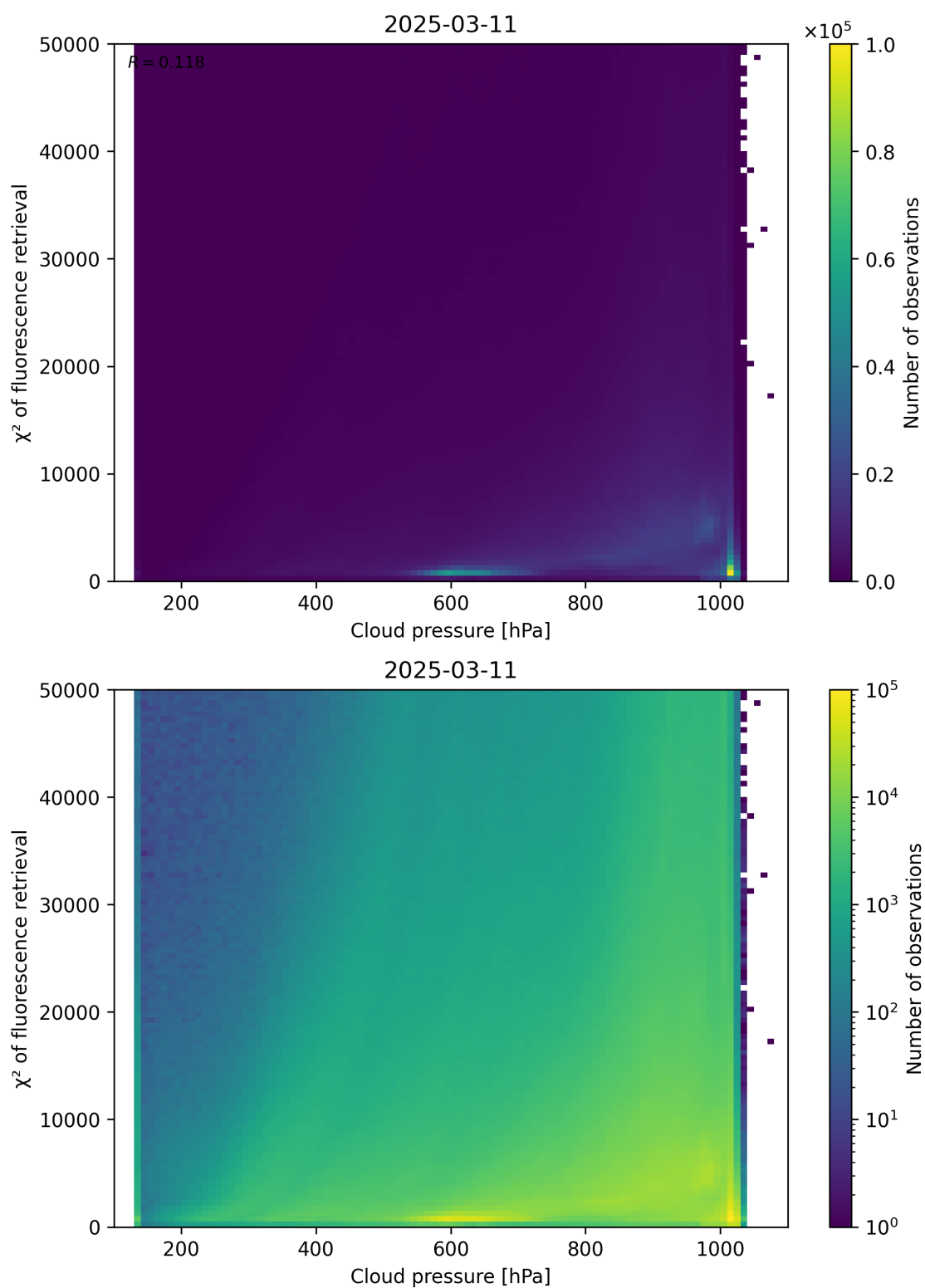
Figure 78: Scatter density plot of “Cloud pressure” against “ \chi^2 of fluorescence retrieval” for 2025-03-10 to 2025-03-12.
