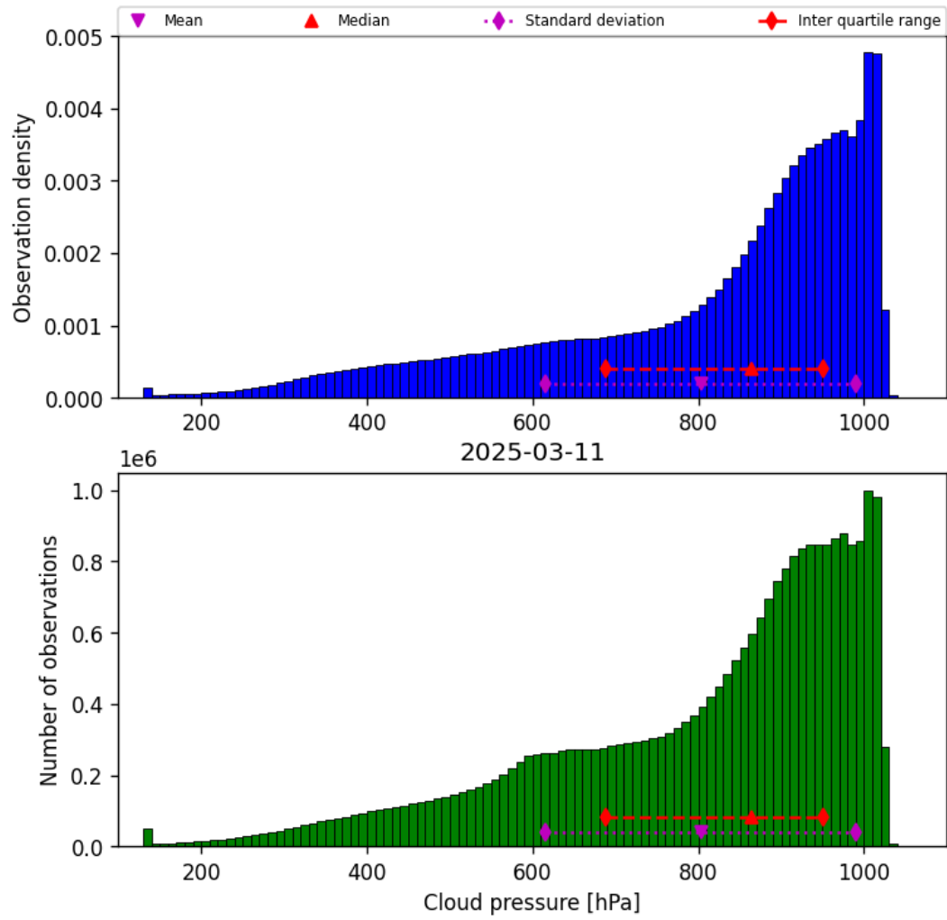
Figure 30: Histogram of “Cloud pressure” for 2025-03-10 to 2025-03-12
