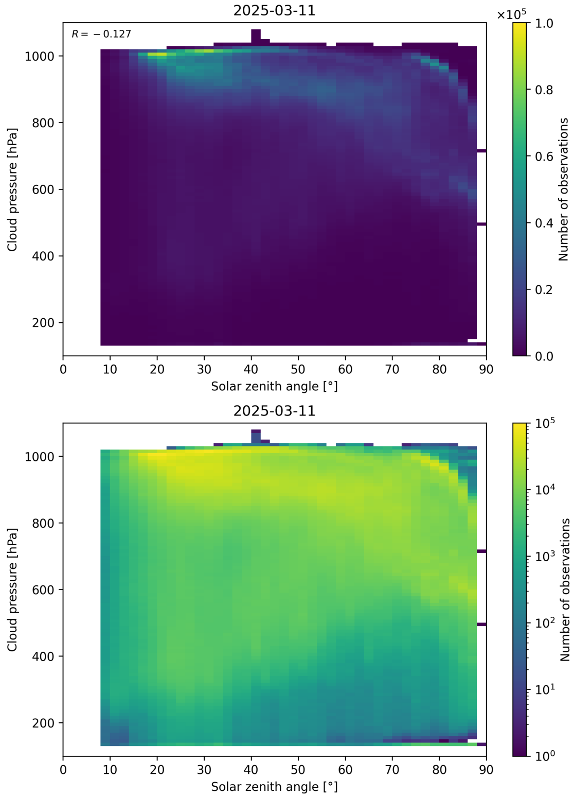
Figure 111: Scatter density plot of “Solar zenith angle” against “Cloud pressure” for 2025-03-10 to 2025-03-12.
