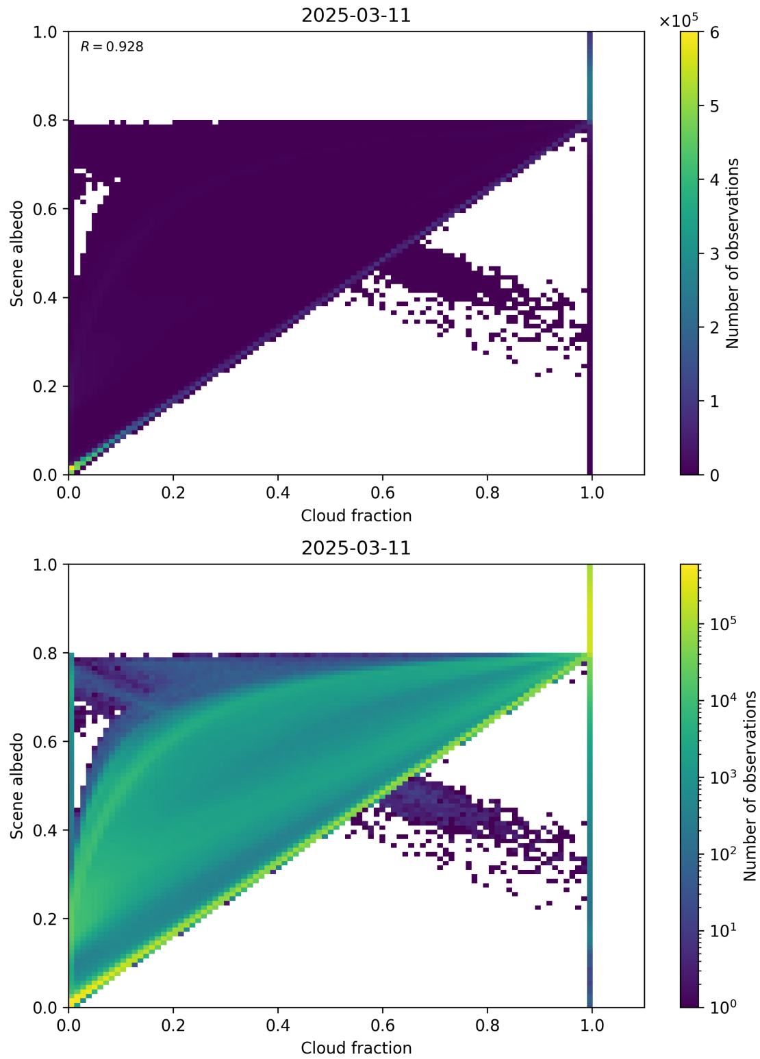
Figure 75: Scatter density plot of “Cloud fraction” against “Scene albedo” for 2025-03-10 to 2025-03-12.
