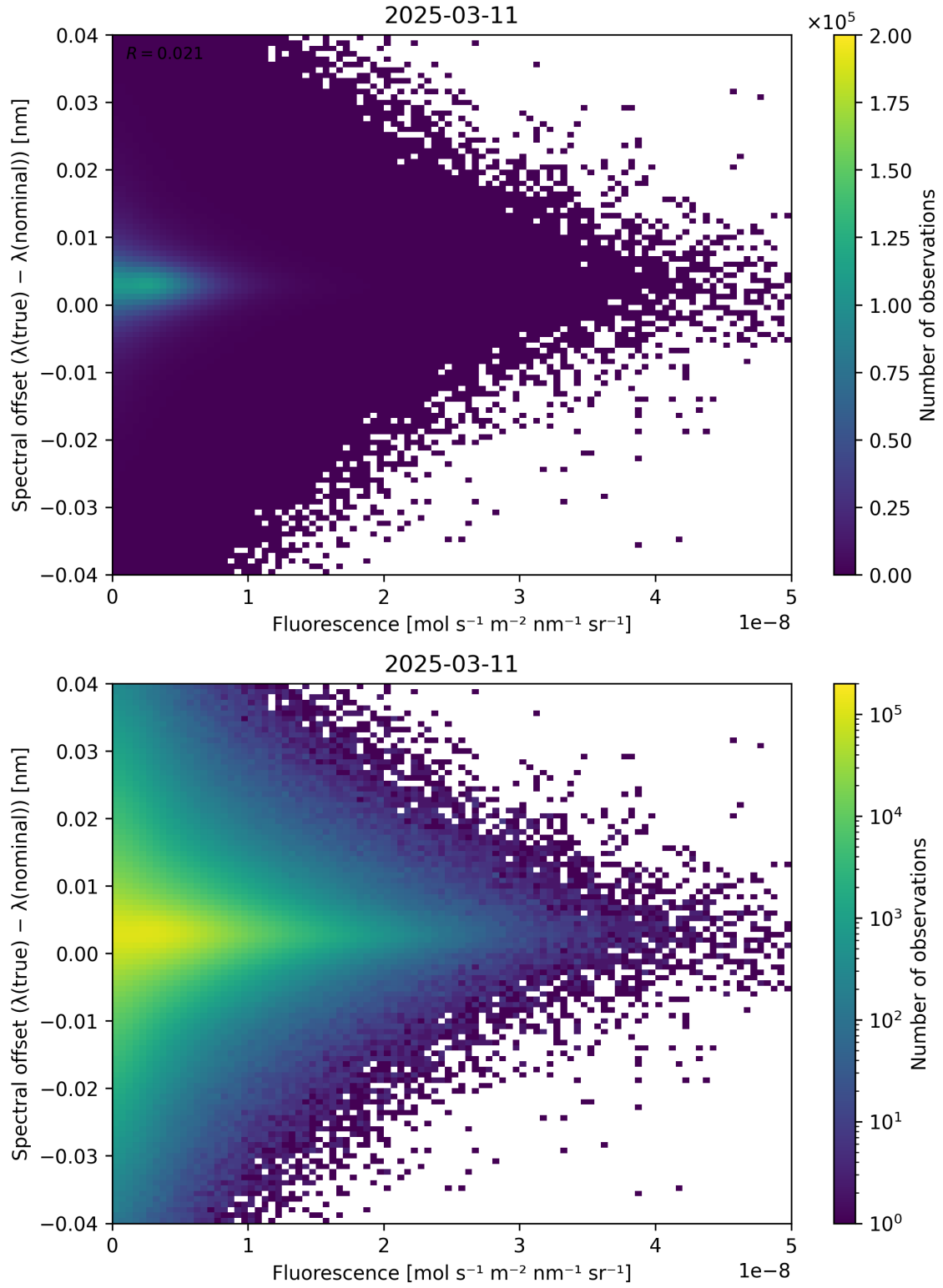
Figure 87: Scatter density plot of “Fluorescence” against “Spectral offset ( \lambda_{\text{true}} - \lambda_{\text{nominal}} )” for 2025-03-10 to 2025-03-12.
