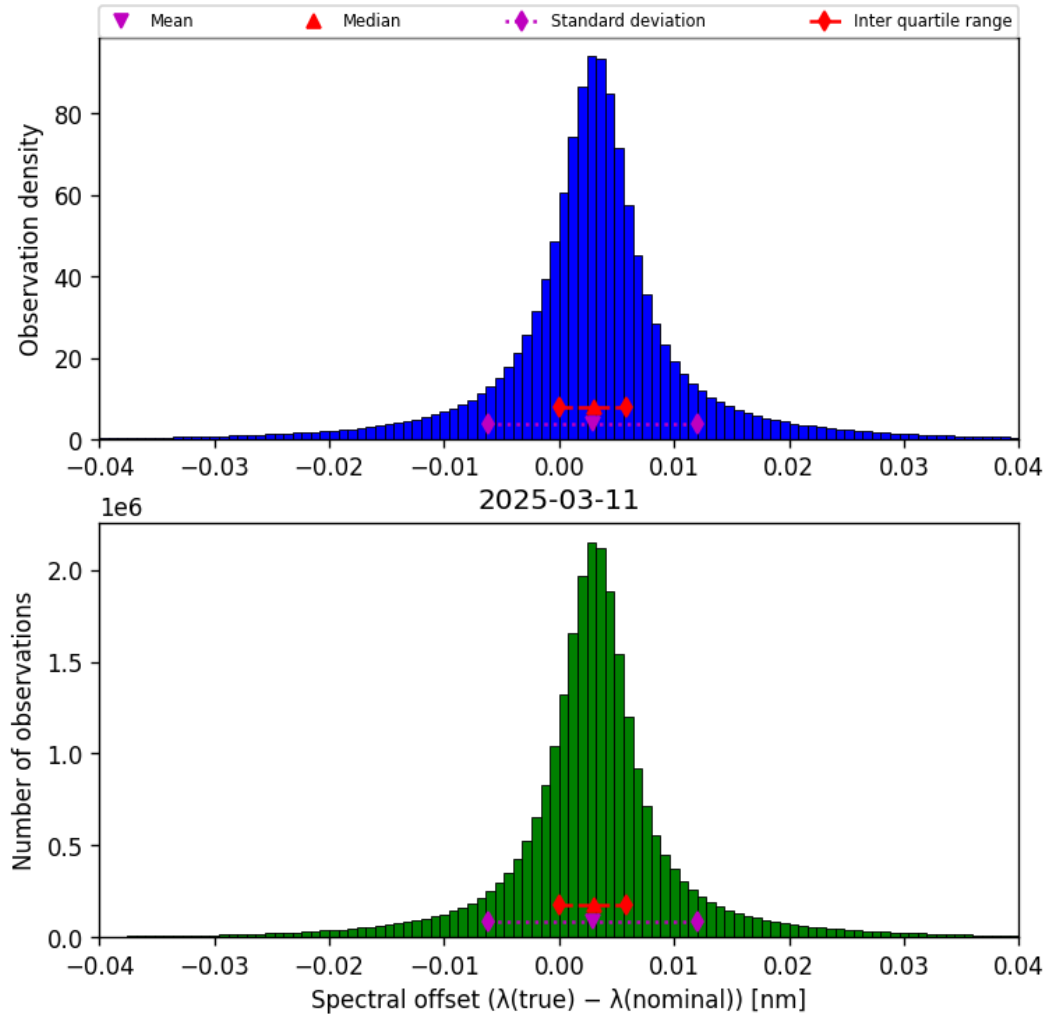
Figure 45: Histogram of “Spectral offset ( \lambda_{\text{true}} - \lambda_{\text{nominal}} )” for 2025-03-10 to 2025-03-12
