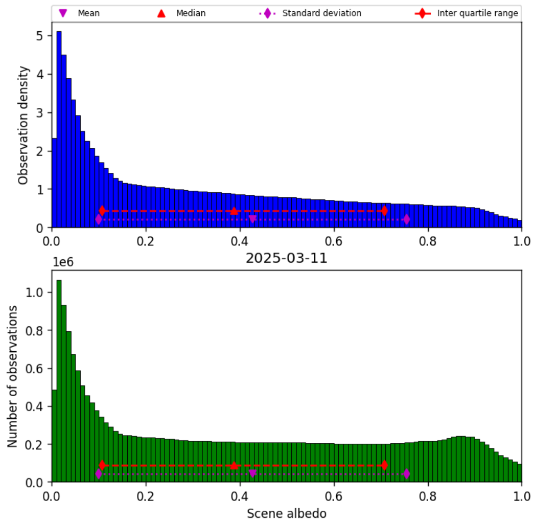
Figure 34: Histogram of “Scene albedo” for 2025-03-10 to 2025-03-12
