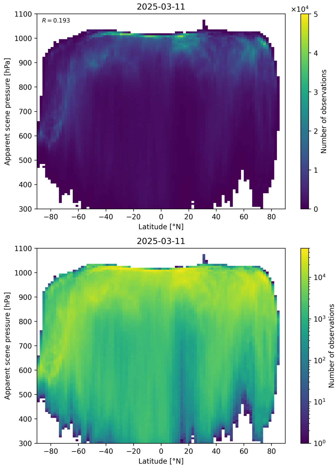
Figure 88: Scatter density plot of “Latitude” against “Apparent scene pressure” for 2025-03-10 to 2025-03-12.
