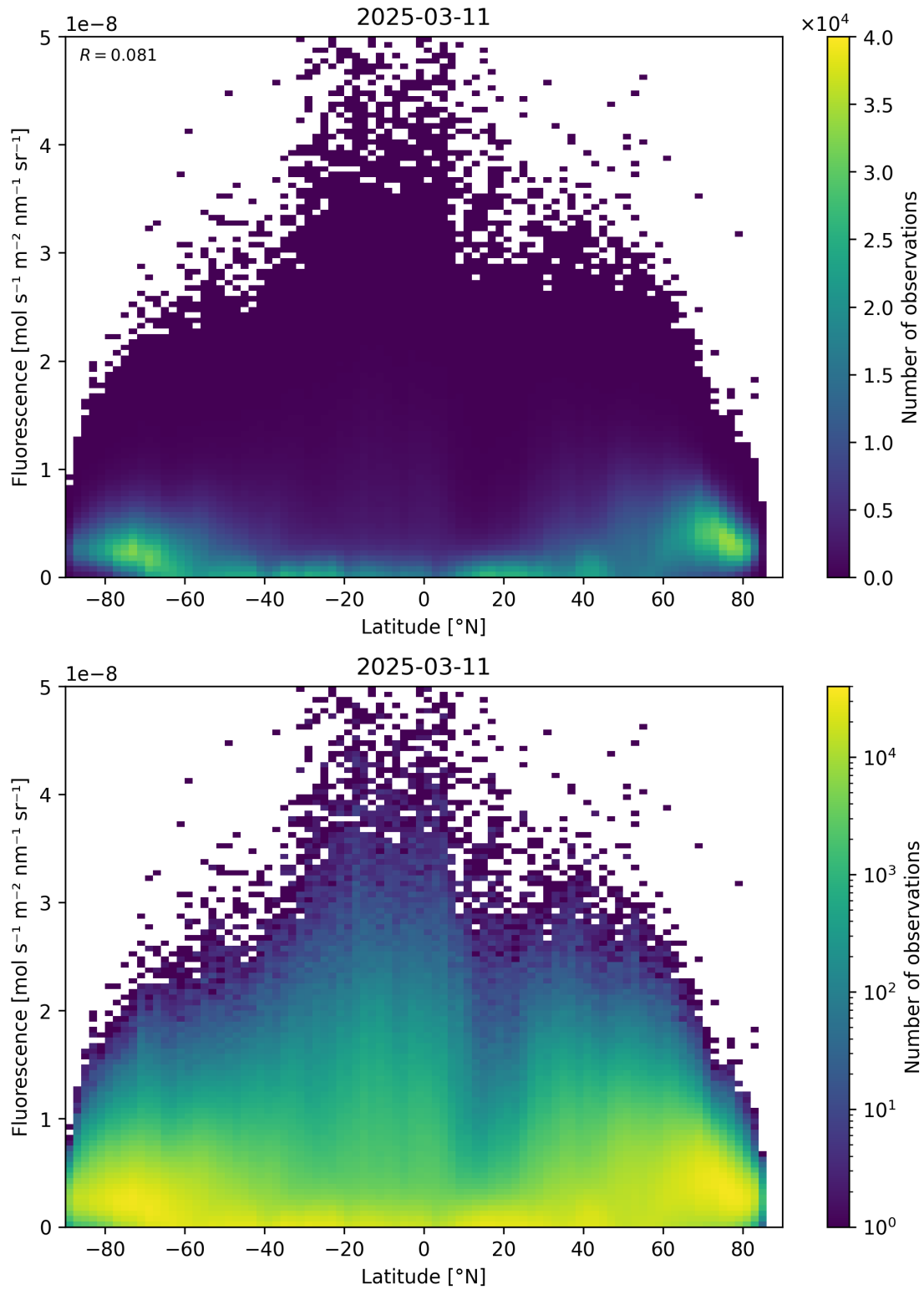
Figure 92: Scatter density plot of “Latitude” against “Fluorescence” for 2025-03-10 to 2025-03-12.
