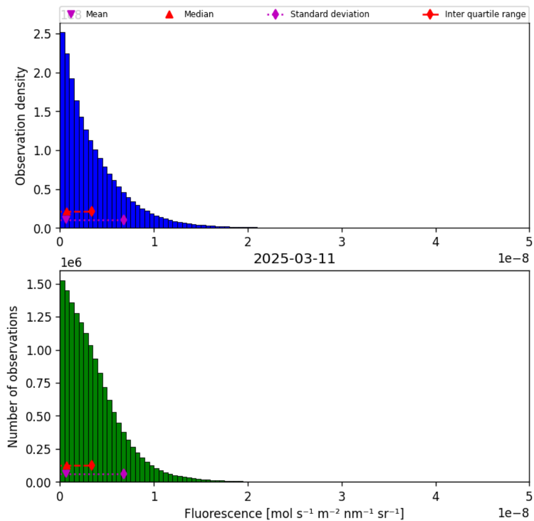
Figure 40: Histogram of “Fluorescence” for 2025-03-10 to 2025-03-12
