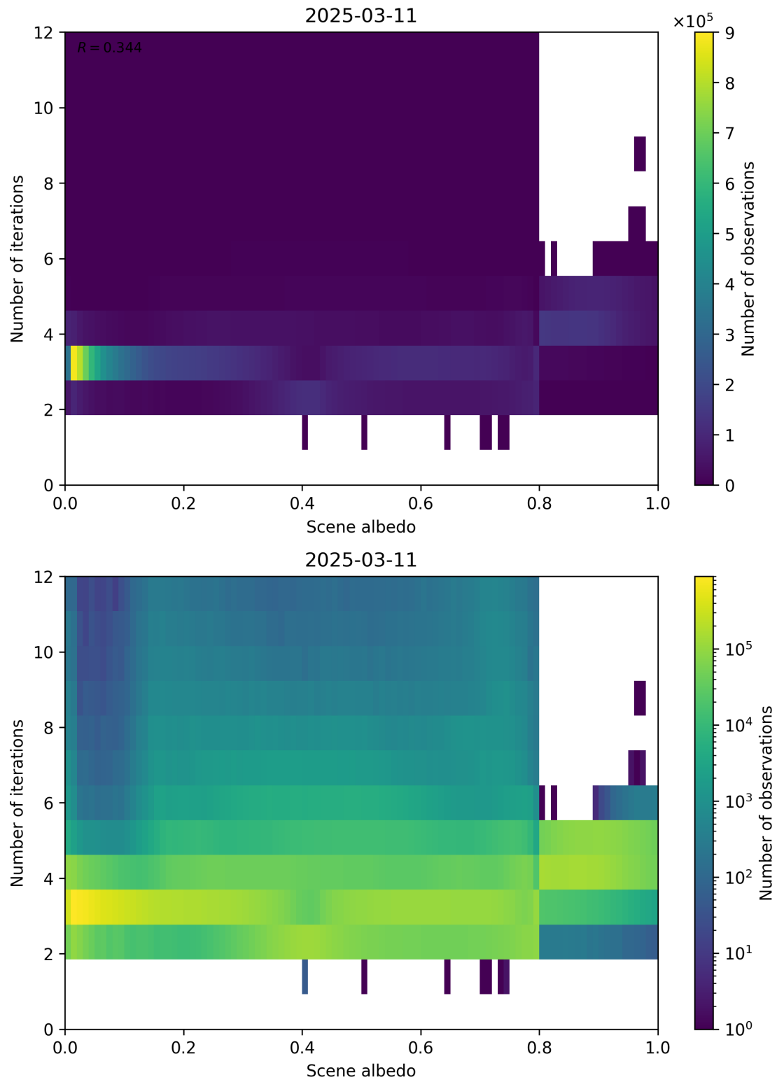
Figure 105: Scatter density plot of “Scene albedo” against “Number of iterations” for 2025-03-10 to 2025-03-12.
