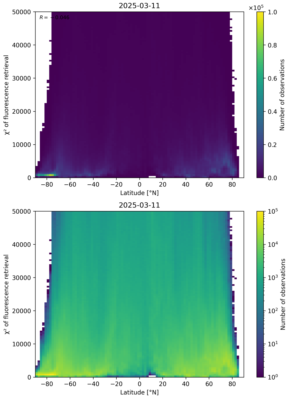
Figure 89: Scatter density plot of “Latitude” against “ \chi^2 of fluorescence retrieval” for 2025-03-10 to 2025-03-12.
