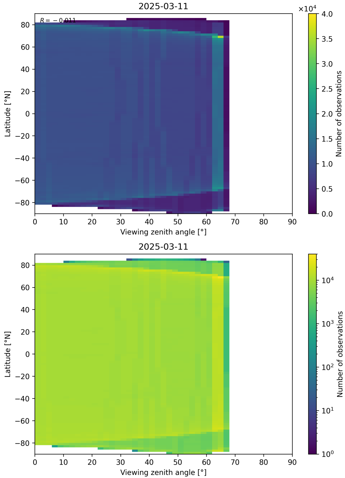
Figure 123: Scatter density plot of “Viewing zenith angle” against “Latitude” for 2025-03-10 to 2025-03-12.
