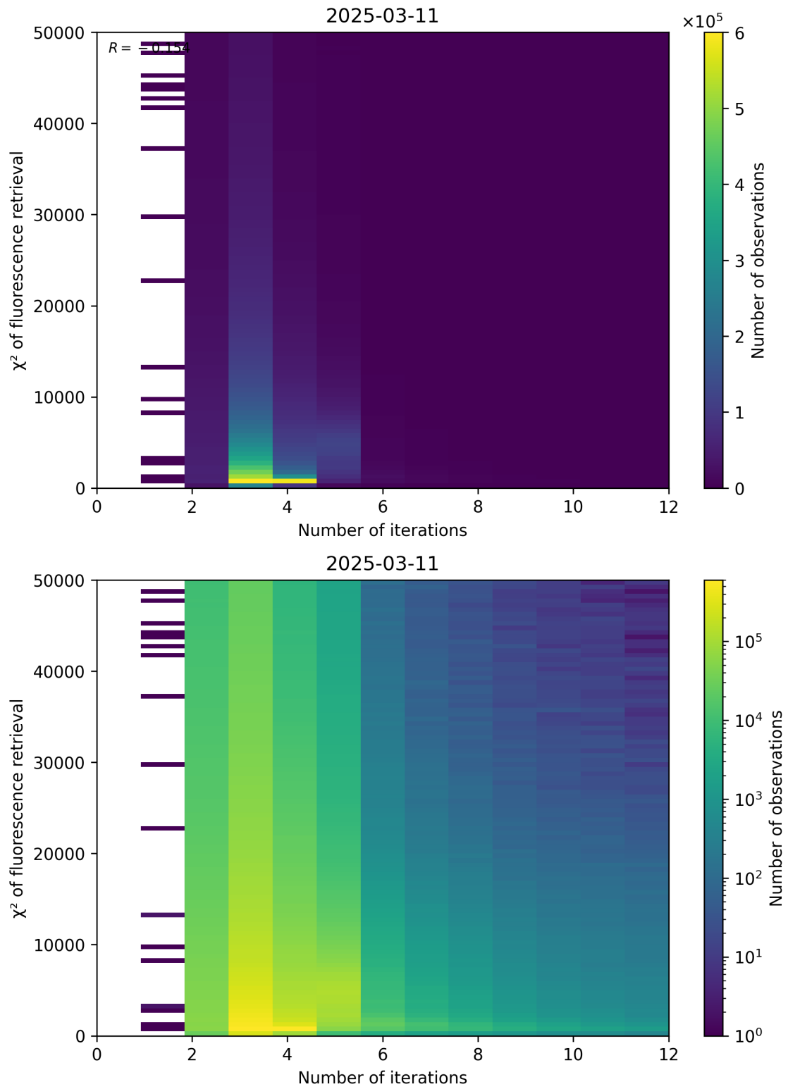
Figure 97: Scatter density plot of “Number of iterations” against “ \chi^2 of fluorescence retrieval” for 2025-03-10 to 2025-03-12.
