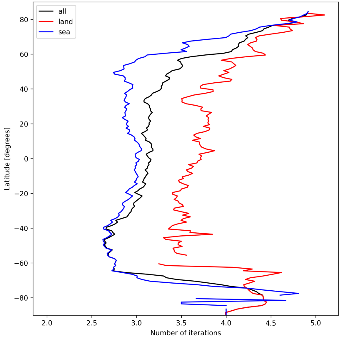
Figure 22: Zonal average of “Number of iterations” for 2025-03-10 to 2025-03-12.
