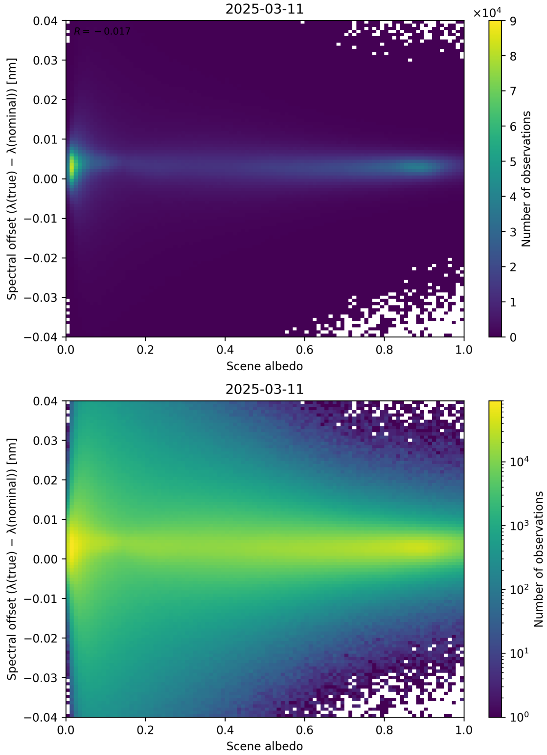
Figure 107: Scatter density plot of “Scene albedo” against “Spectral offset ( \lambda_{\text{true}} - \lambda_{\text{nominal}} )” for 2025-03-10 to 2025-03-12.
