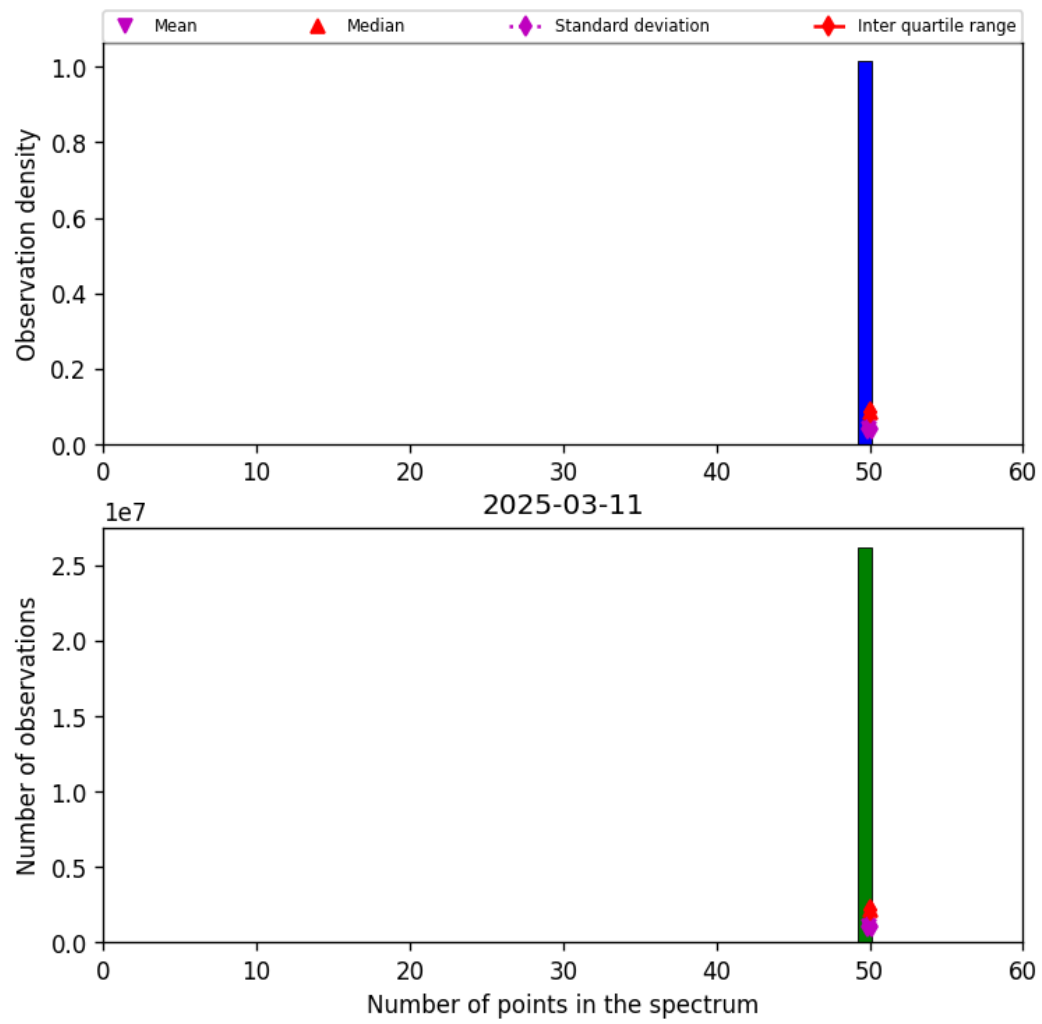
Figure 44: Histogram of “Number of points in the spectrum” for 2025-03-10 to 2025-03-12
