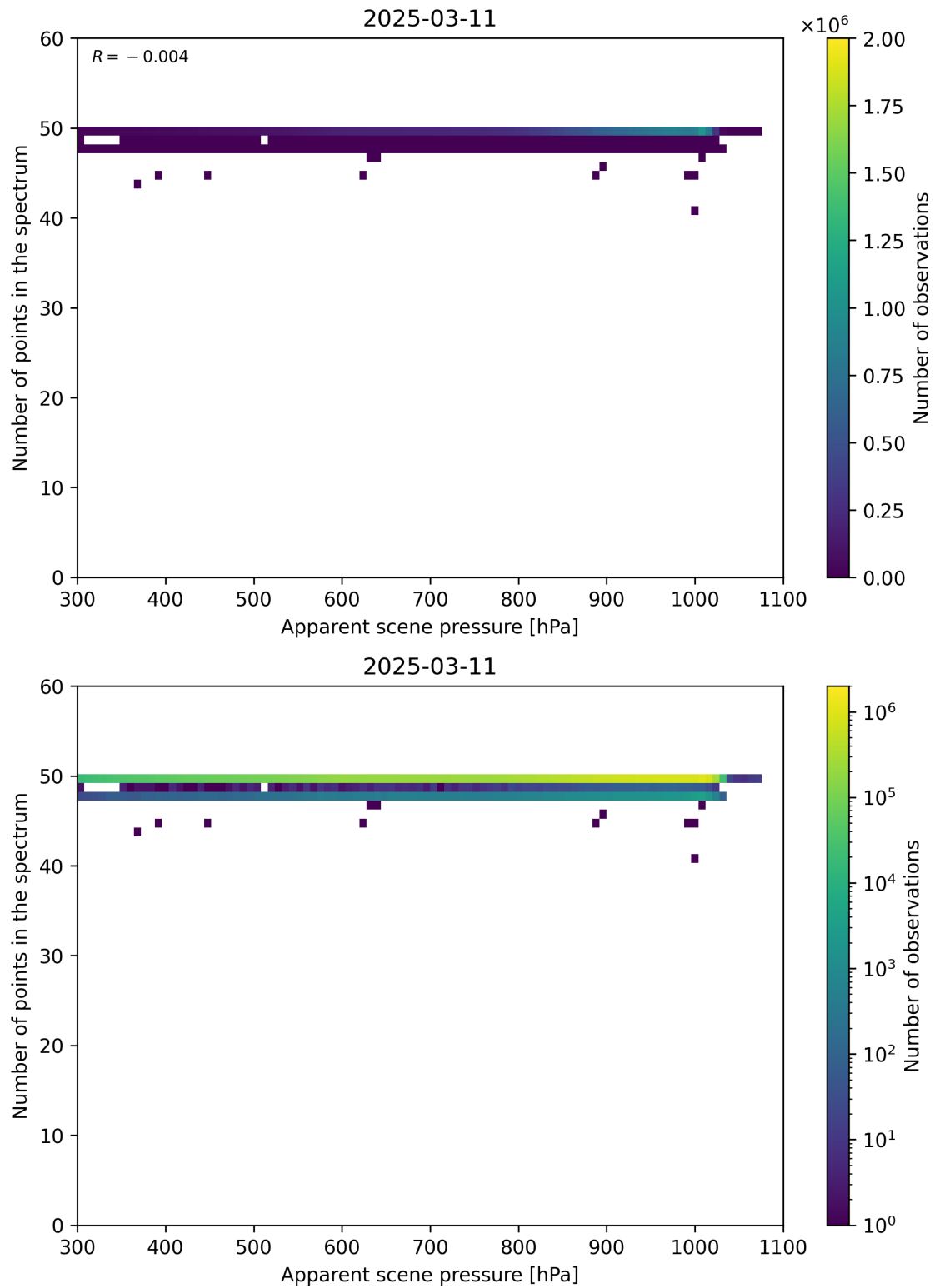
Figure 66: Scatter density plot of “Apparent scene pressure” against “Number of points in the spectrum” for 2025-03-10 to 2025-03-12.
