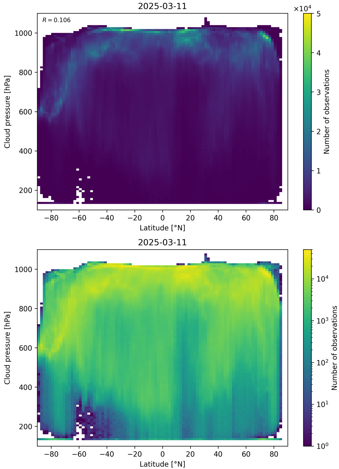
Figure 91: Scatter density plot of “Latitude” against “Cloud pressure” for 2025-03-10 to 2025-03-12.
