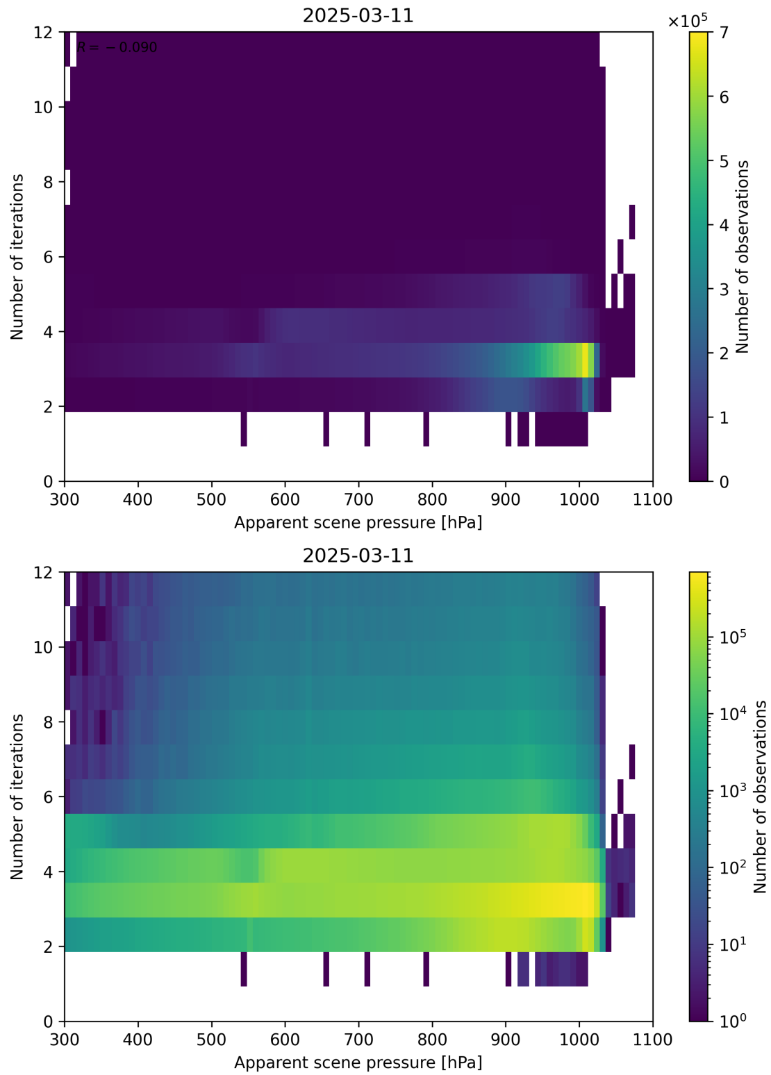
Figure 65: Scatter density plot of “Apparent scene pressure” against “Number of iterations” for 2025-03-10 to 2025-03-12.
