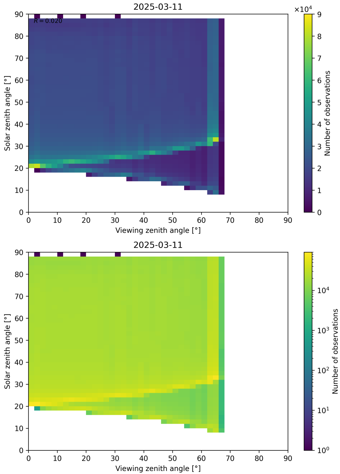
Figure 127: Scatter density plot of “Viewing zenith angle” against “Solar zenith angle” for 2025-03-10 to 2025-03-12.
