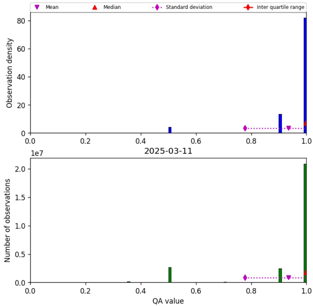
Figure 29: Histogram of “QA value” for 2025-03-10 to 2025-03-12
