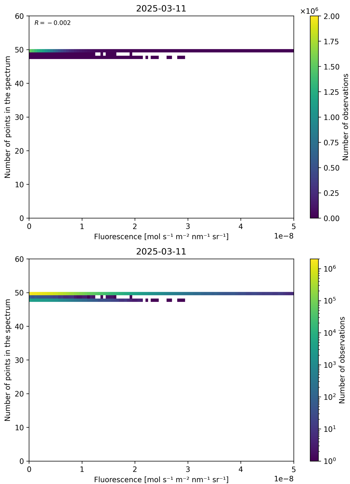
Figure 86: Scatter density plot of “Fluorescence” against “Number of points in the spectrum” for 2025-03-10 to 2025-03-12.
