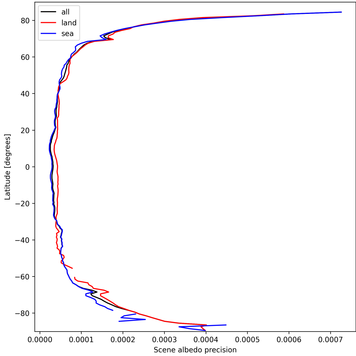
Figure 18: Zonal average of “Scene albedo precision” for 2025-03-10 to 2025-03-12.
