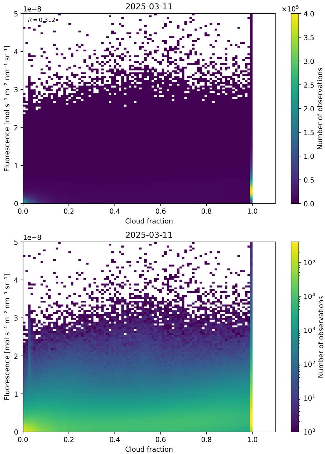
Figure 72: Scatter density plot of “Cloud fraction” against “Fluorescence” for 2025-03-10 to 2025-03-12.
