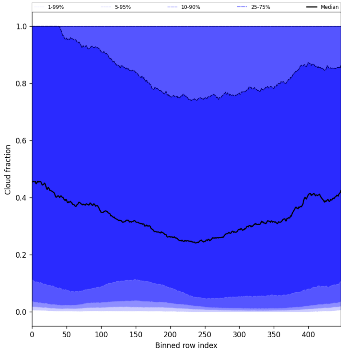
Figure 49: Along track statistics of “Cloud fraction” for 2025-03-10 to 2025-03-12
