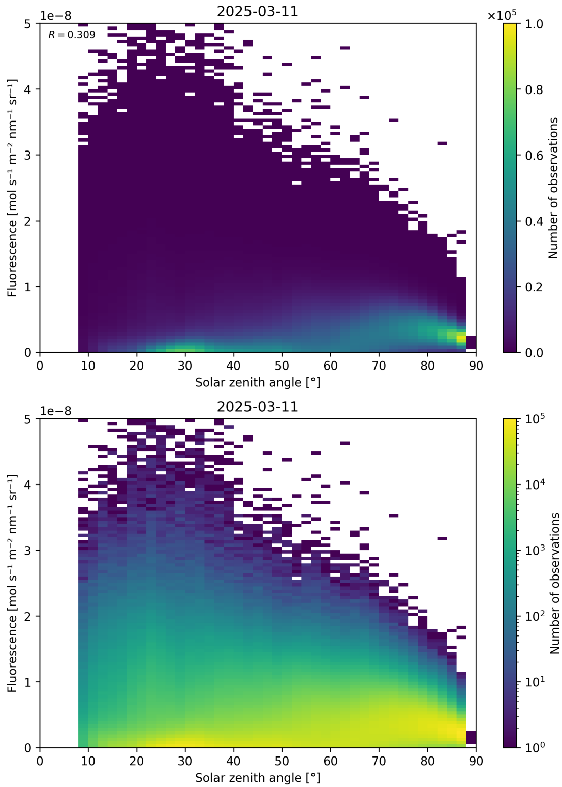
Figure 112: Scatter density plot of “Solar zenith angle” against “Fluorescence” for 2025-03-10 to 2025-03-12.
