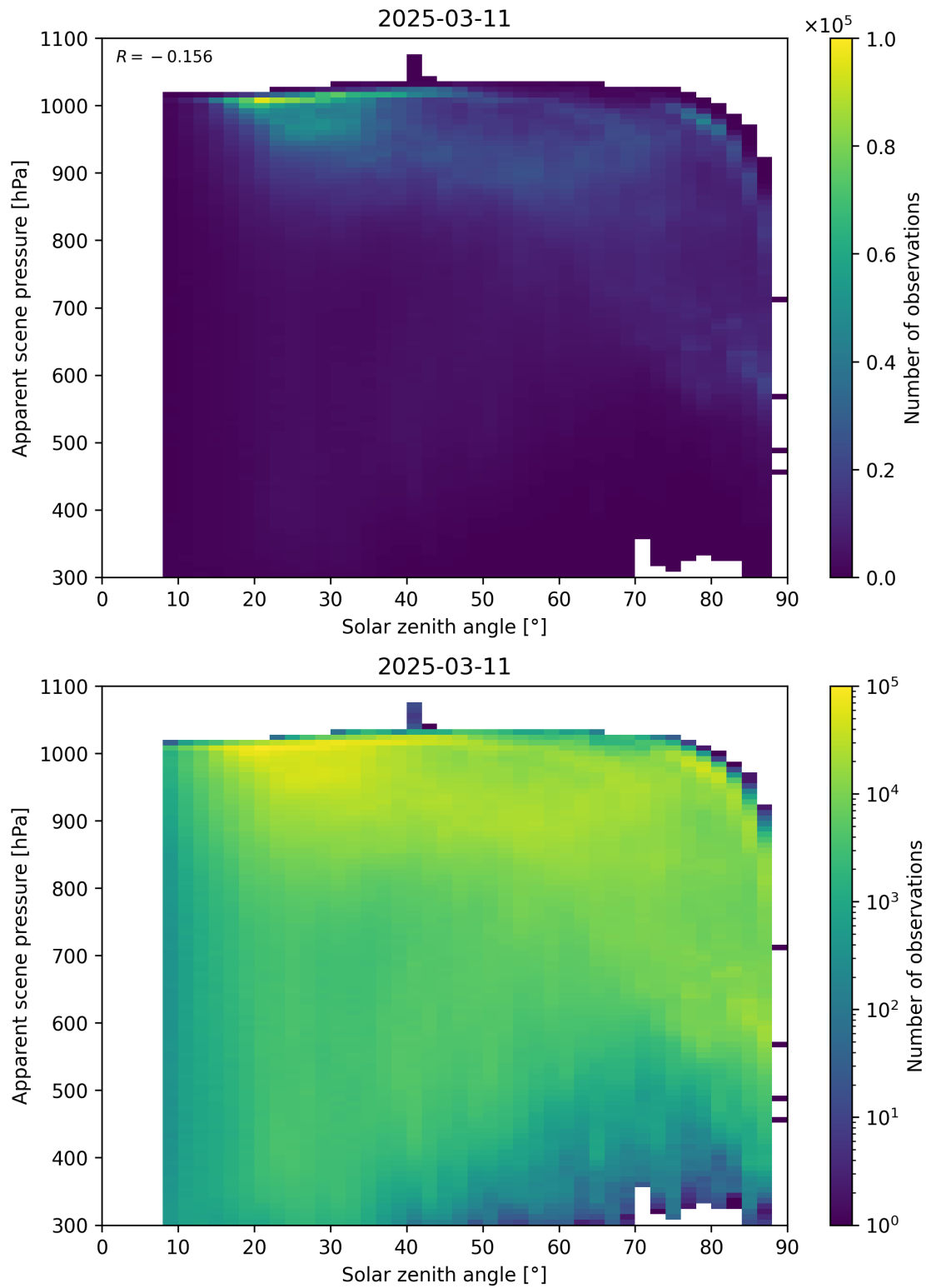
Figure 108: Scatter density plot of “Solar zenith angle” against “Apparent scene pressure” for 2025-03-10 to 2025-03-12.
