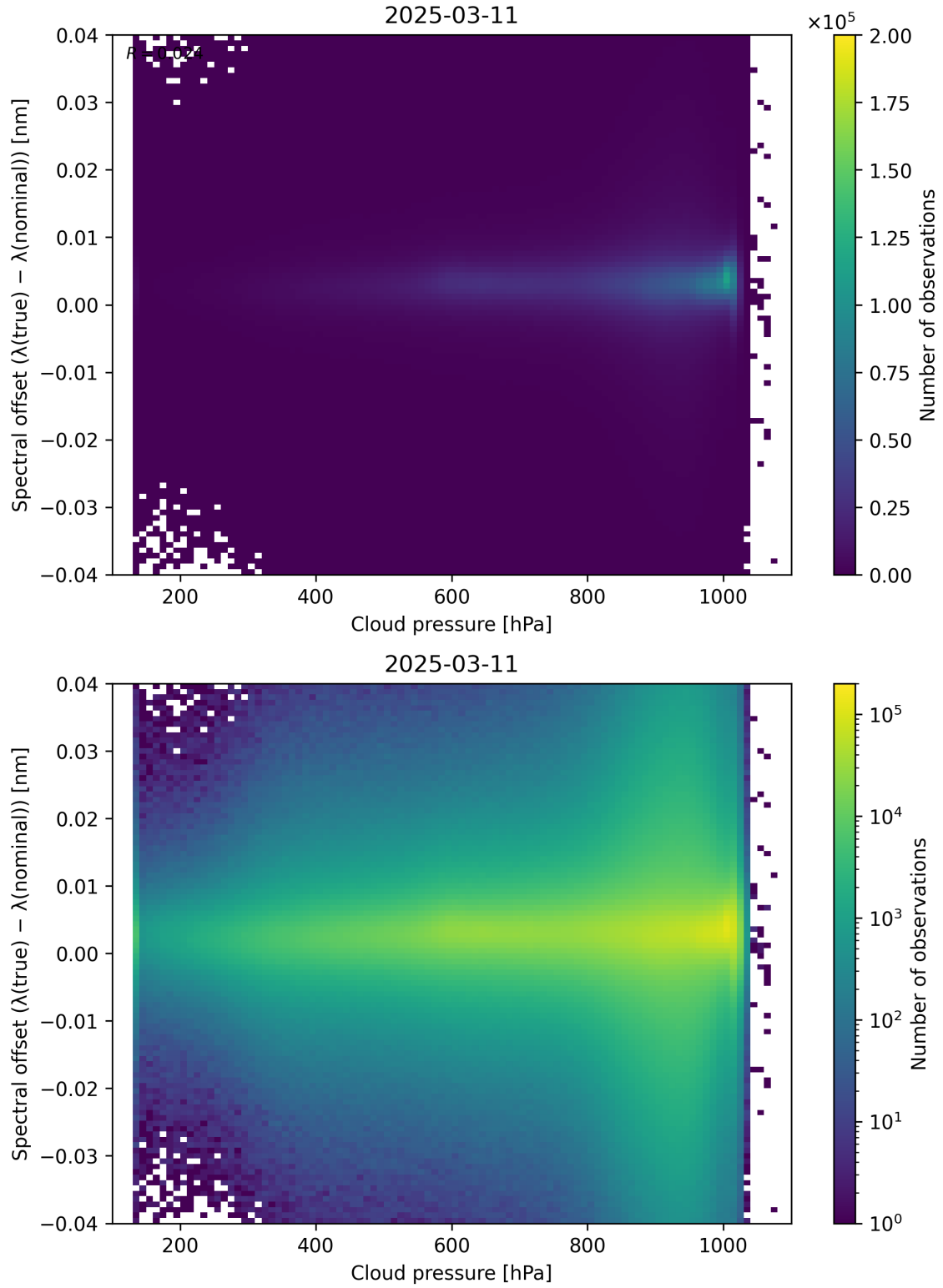
Figure 84: Scatter density plot of “Cloud pressure” against “Spectral offset ( \lambda_{\text{true}} - \lambda_{\text{nominal}} )” for 2025-03-10 to 2025-03-12.
