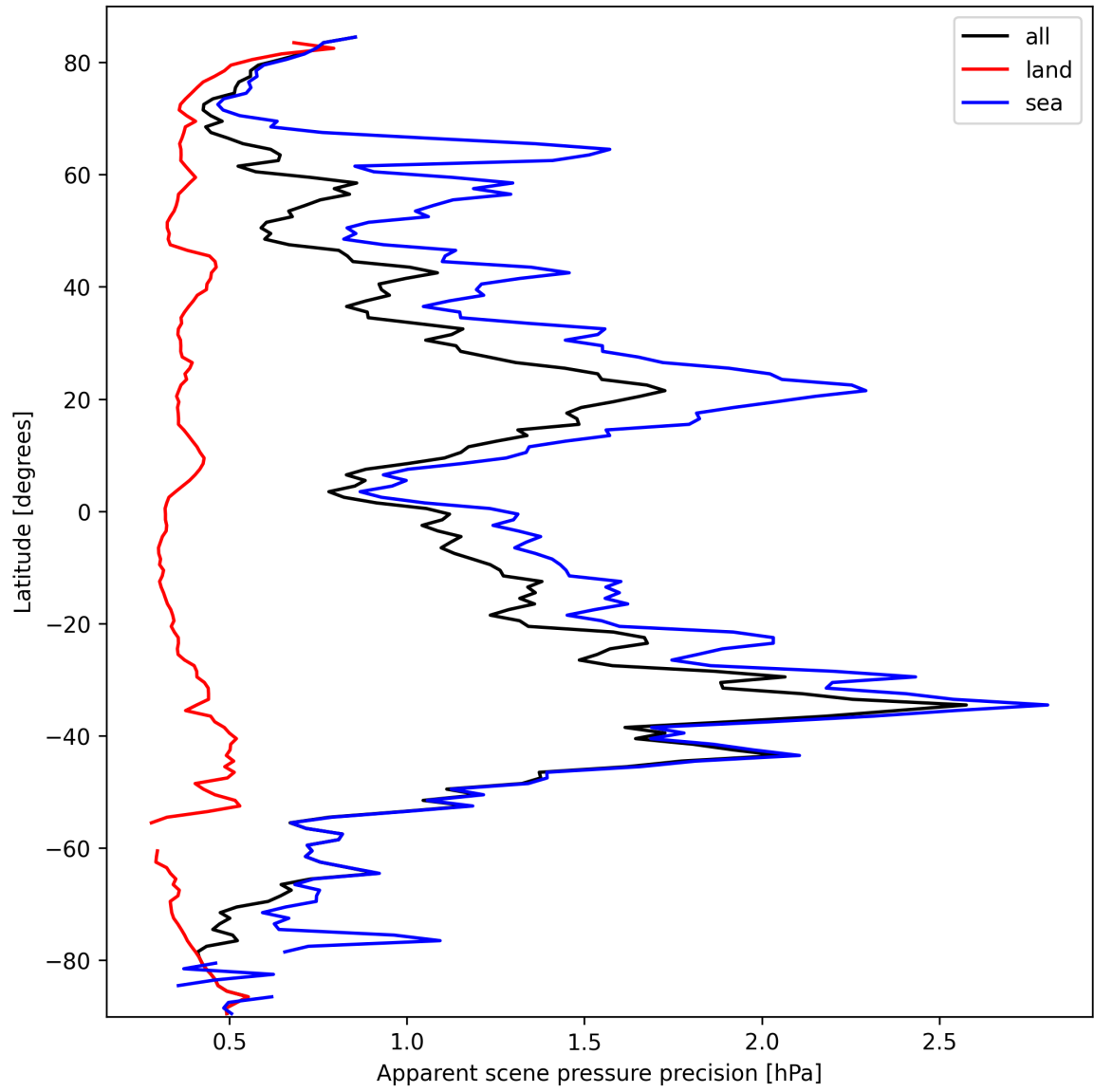
Figure 20: Zonal average of “Apparent scene pressure precision” for 2025-03-10 to 2025-03-12.
