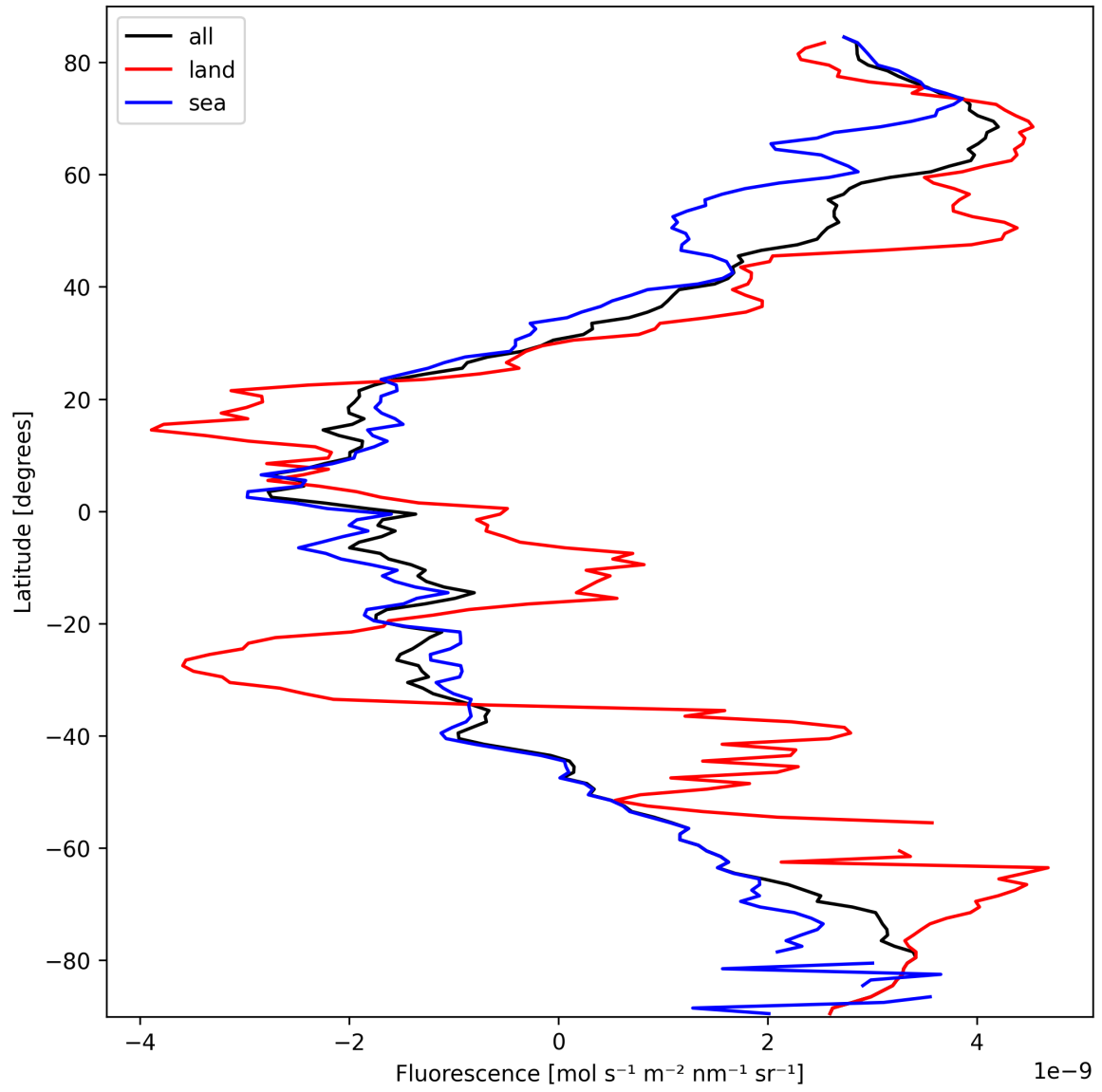
Figure 23: Zonal average of “Fluorescence” for 2025-03-10 to 2025-03-12.
