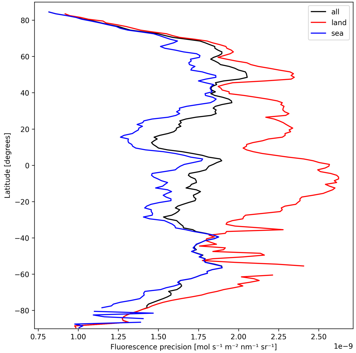
Figure 24: Zonal average of “Fluorescence precision” for 2025-03-10 to 2025-03-12.
