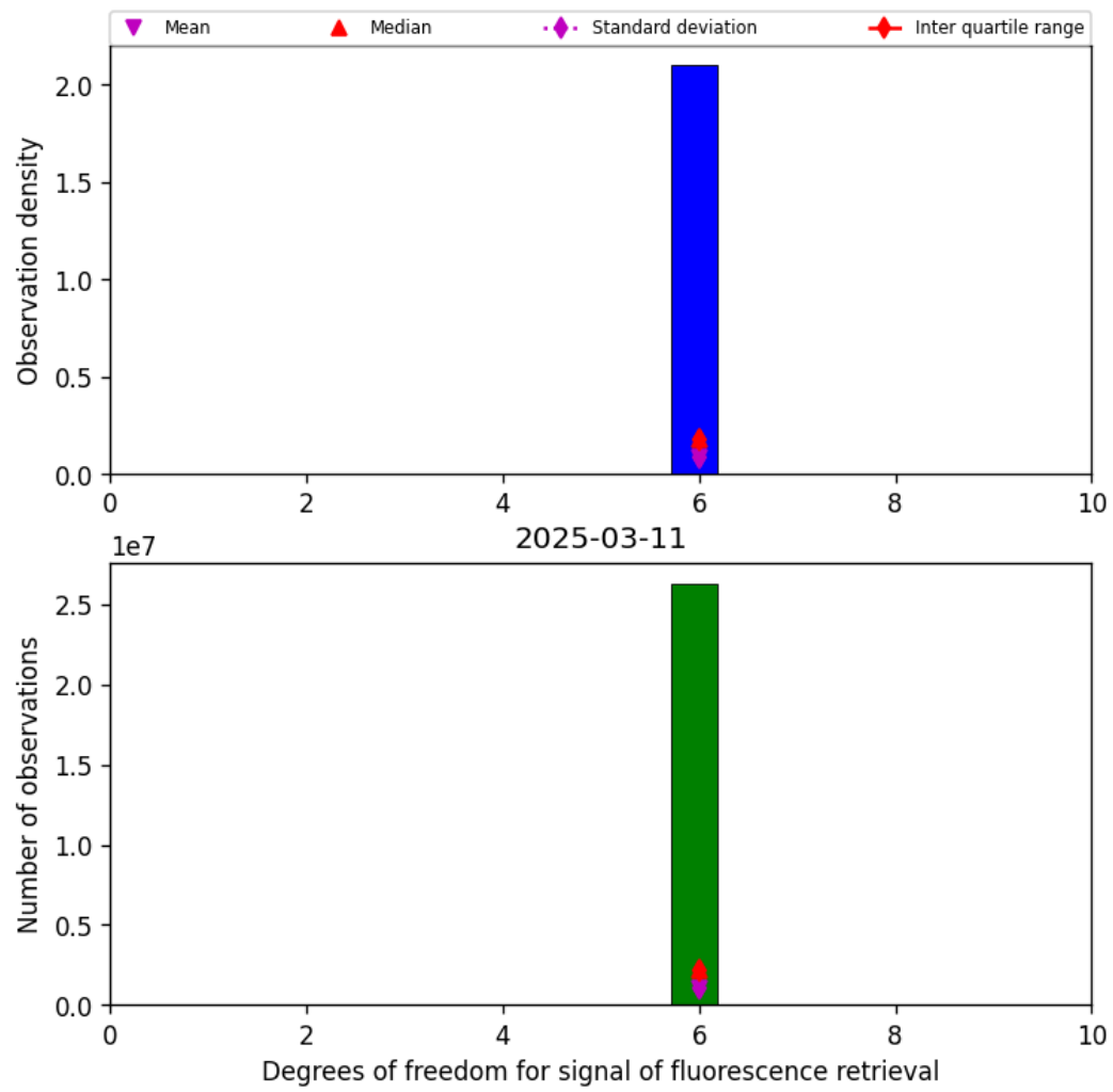
Figure 43: Histogram of “Degrees of freedom for signal of fluorescence retrieval” for 2025-03-10 to 2025-03-12
