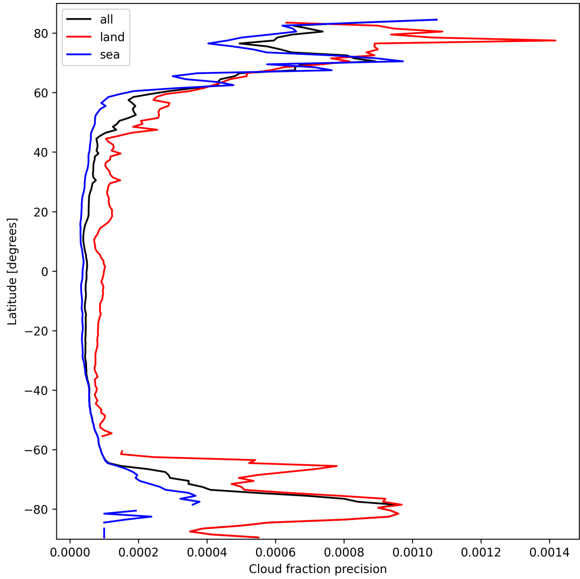
Figure 16: Zonal average of “Cloud fraction precision” for 2025-03-10 to 2025-03-12.
