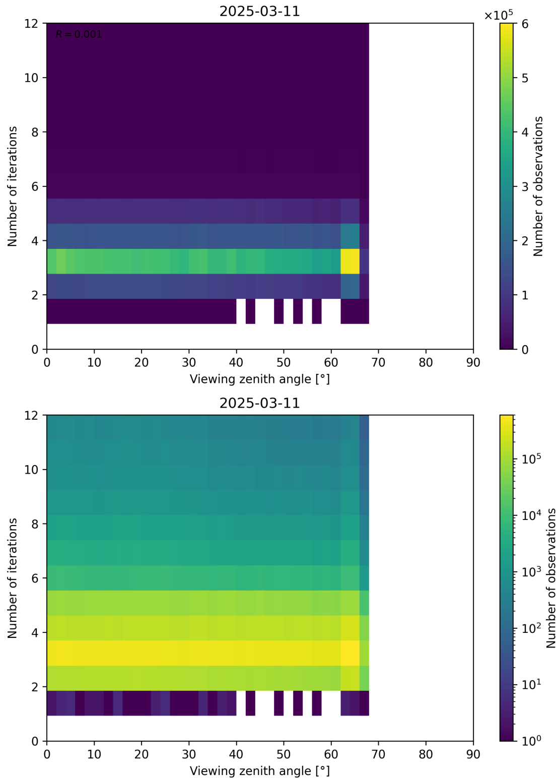
Figure 124: Scatter density plot of “Viewing zenith angle” against “Number of iterations” for 2025-03-10 to 2025-03-12.
