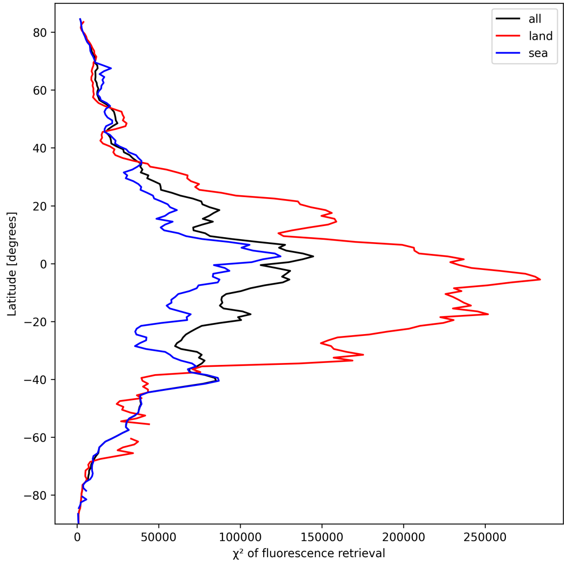
Figure 25: Zonal average of “ \chi^2 of fluorescence retrieval” for 2025-03-10 to 2025-03-12.
