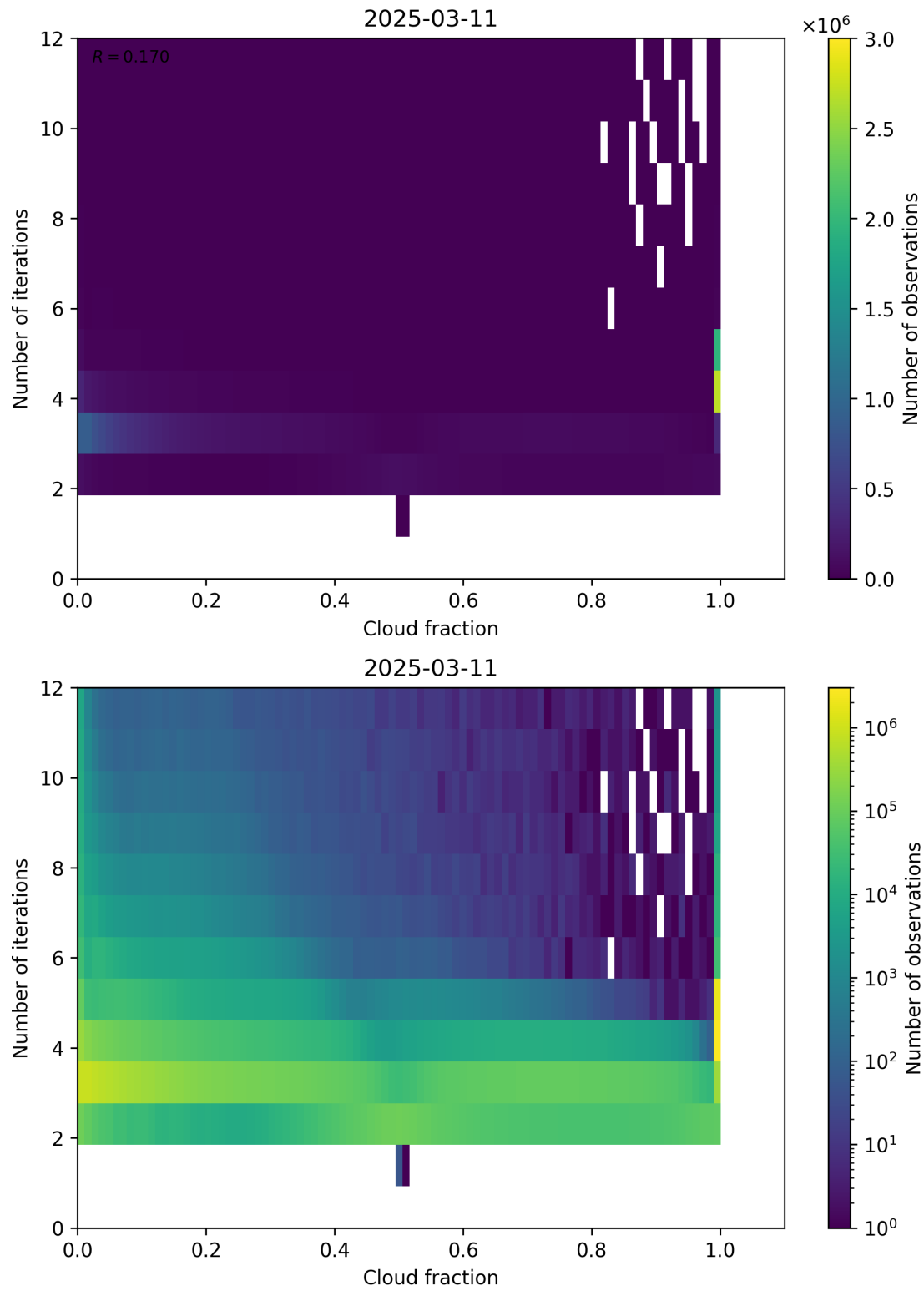
Figure 73: Scatter density plot of “Cloud fraction” against “Number of iterations” for 2025-03-10 to 2025-03-12.
