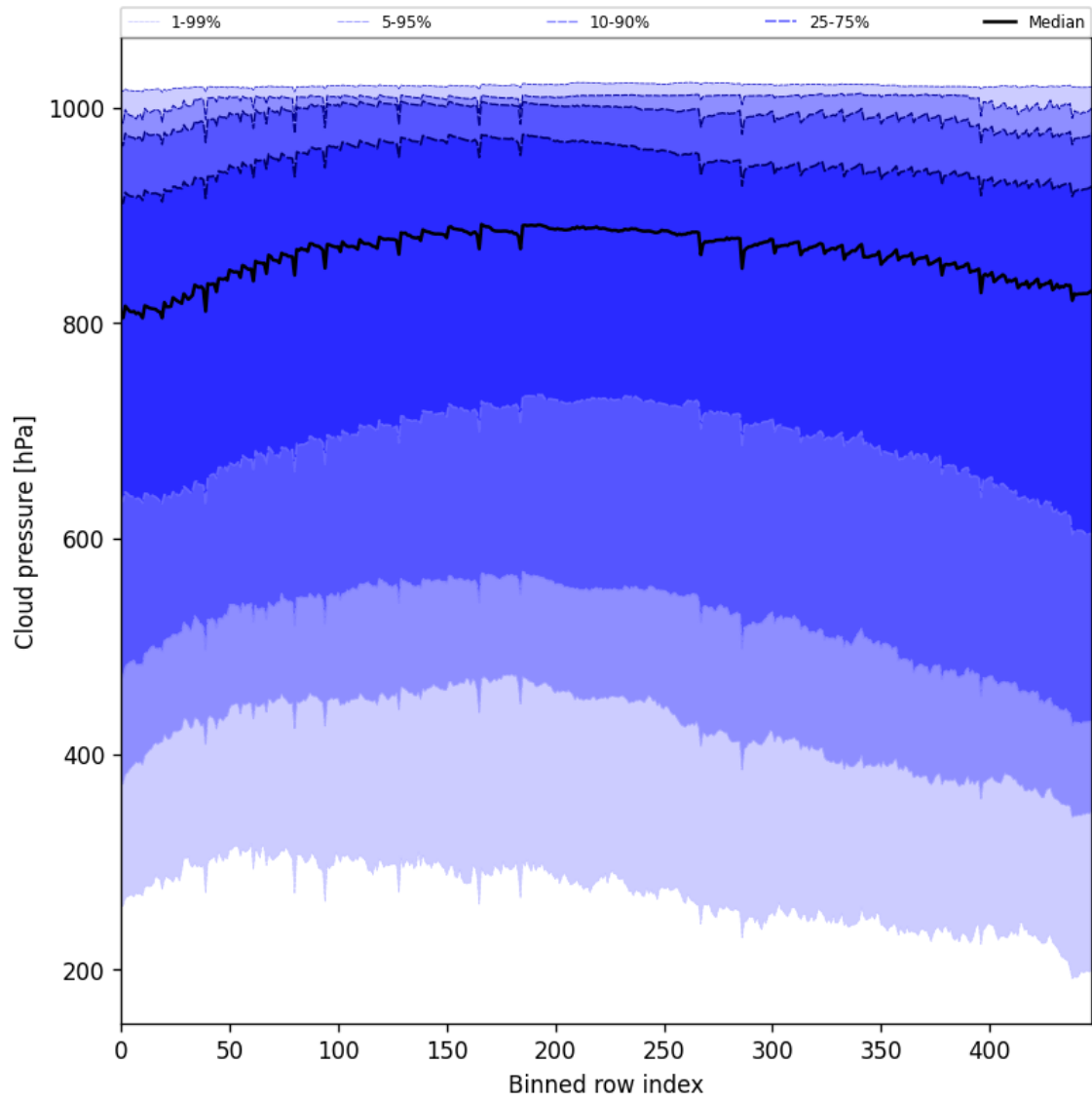
Figure 47: Along track statistics of “Cloud pressure” for 2025-03-10 to 2025-03-12
