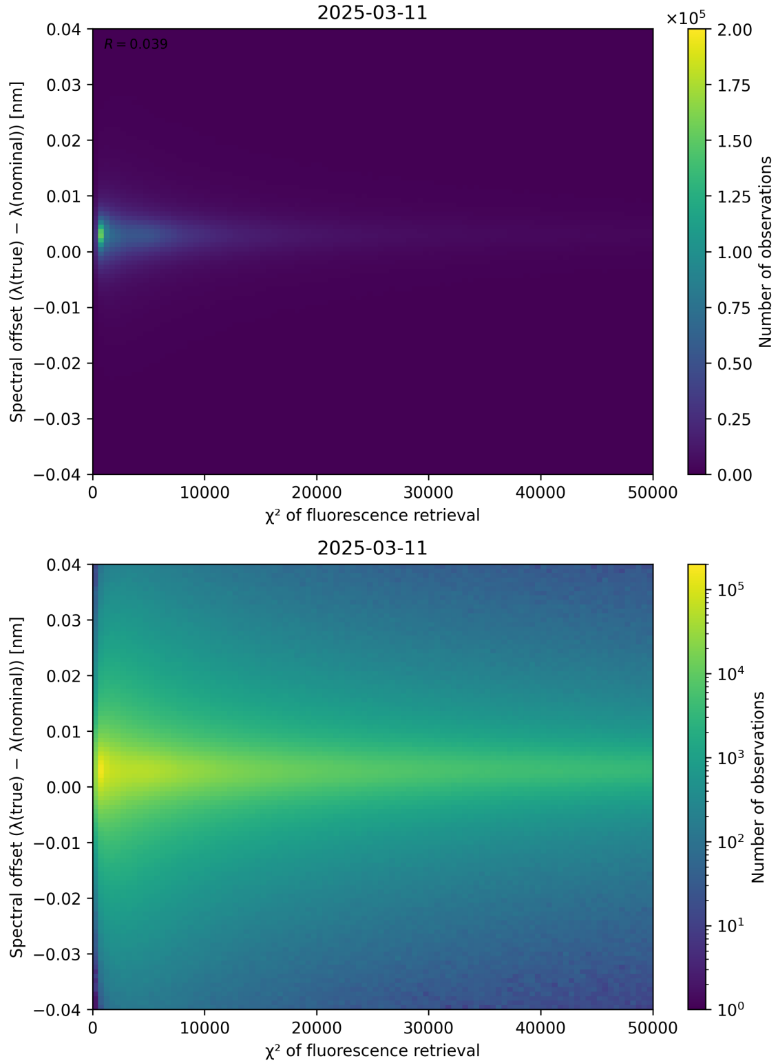
Figure 69: Scatter density plot of “ \chi^2 of fluorescence retrieval” against “Spectral offset ( \lambda_{\text{true}} - \lambda_{\text{nominal}} )” for 2025-03-10 to 2025-03-12.
