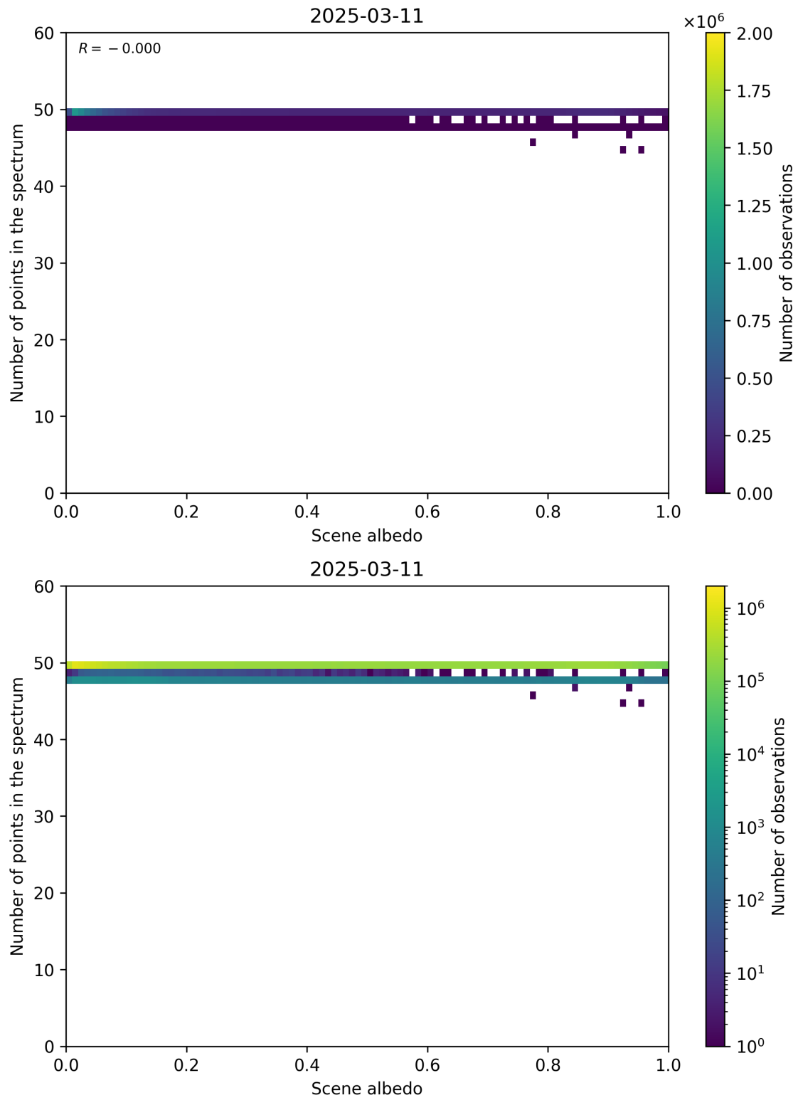
Figure 106: Scatter density plot of “Scene albedo” against “Number of points in the spectrum” for 2025-03-10 to 2025-03-12.
