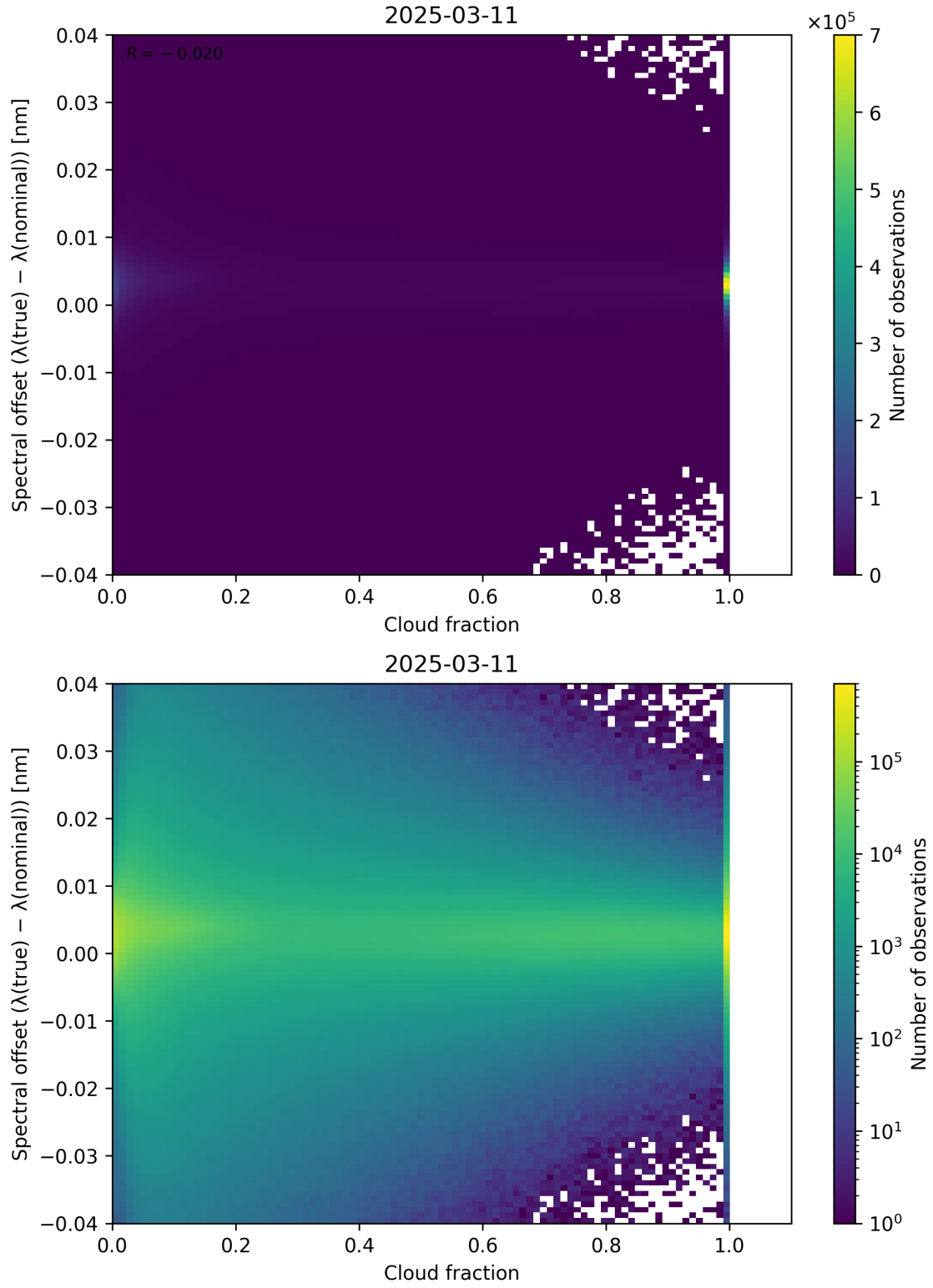
Figure 76: Scatter density plot of “Cloud fraction” against “Spectral offset ( \lambda_{\text{true}} - \lambda_{\text{nominal}} )” for 2025-03-10 to 2025-03-12.
