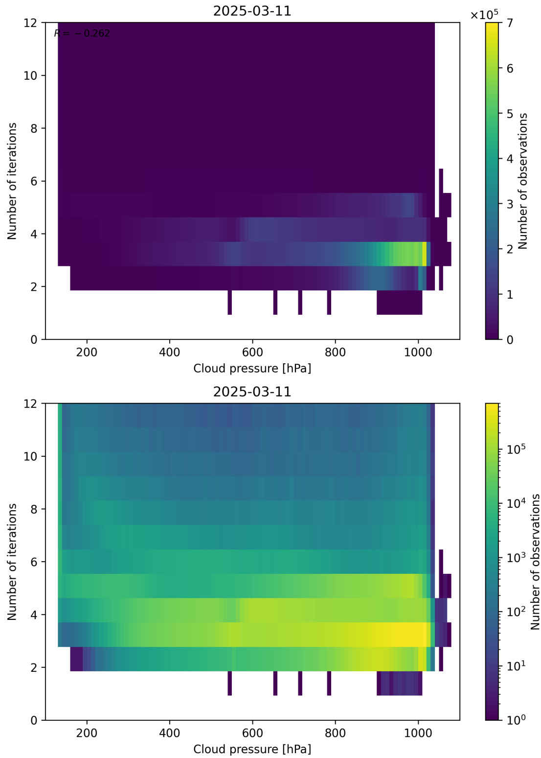
Figure 81: Scatter density plot of “Cloud pressure” against “Number of iterations” for 2025-03-10 to 2025-03-12.
