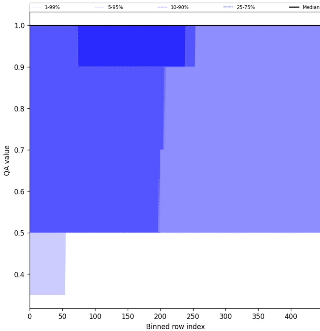
Figure 46: Along track statistics of “QA value” for 2025-03-10 to 2025-03-12
