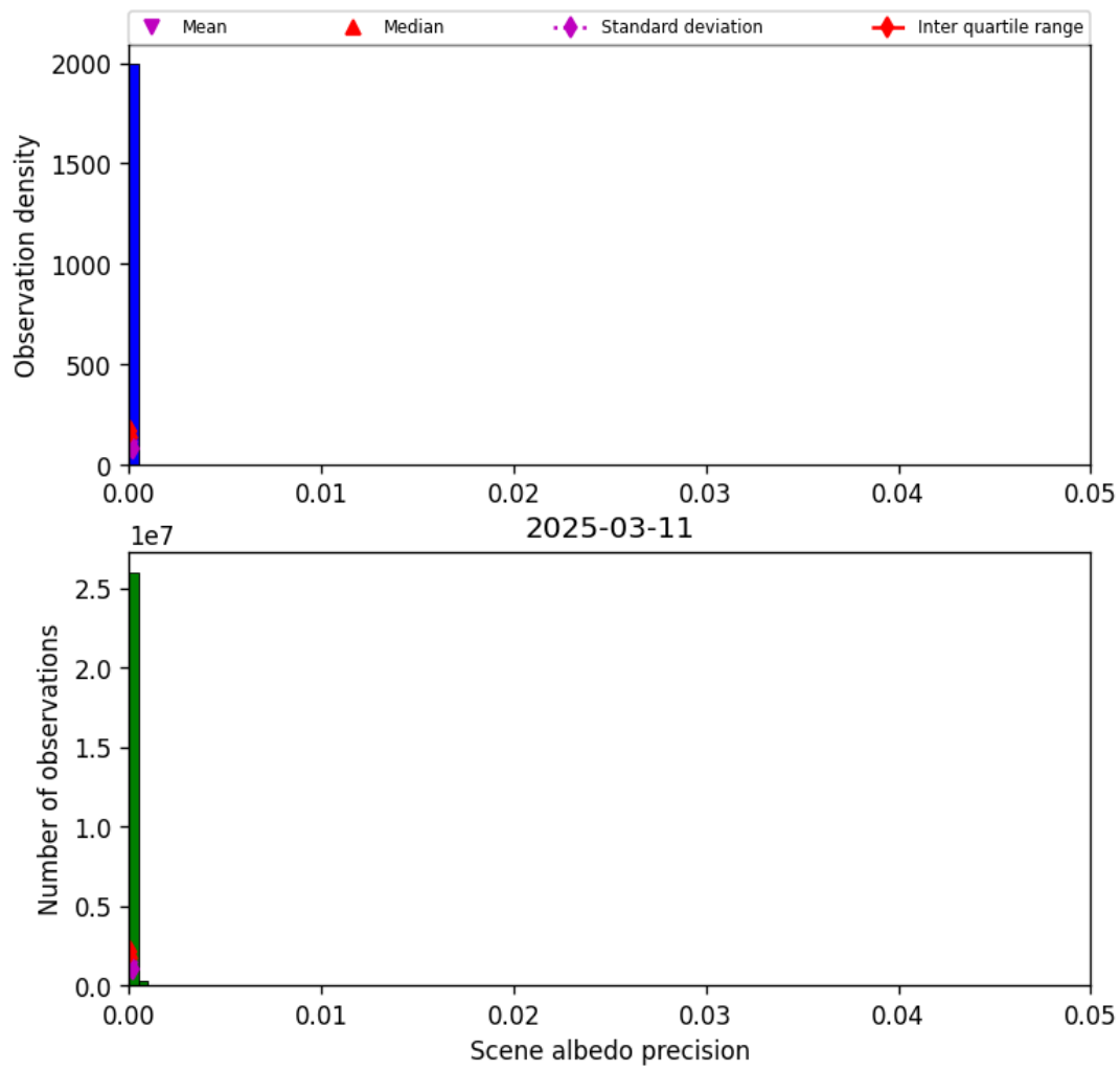
Figure 35: Histogram of “Scene albedo precision” for 2025-03-10 to 2025-03-12
