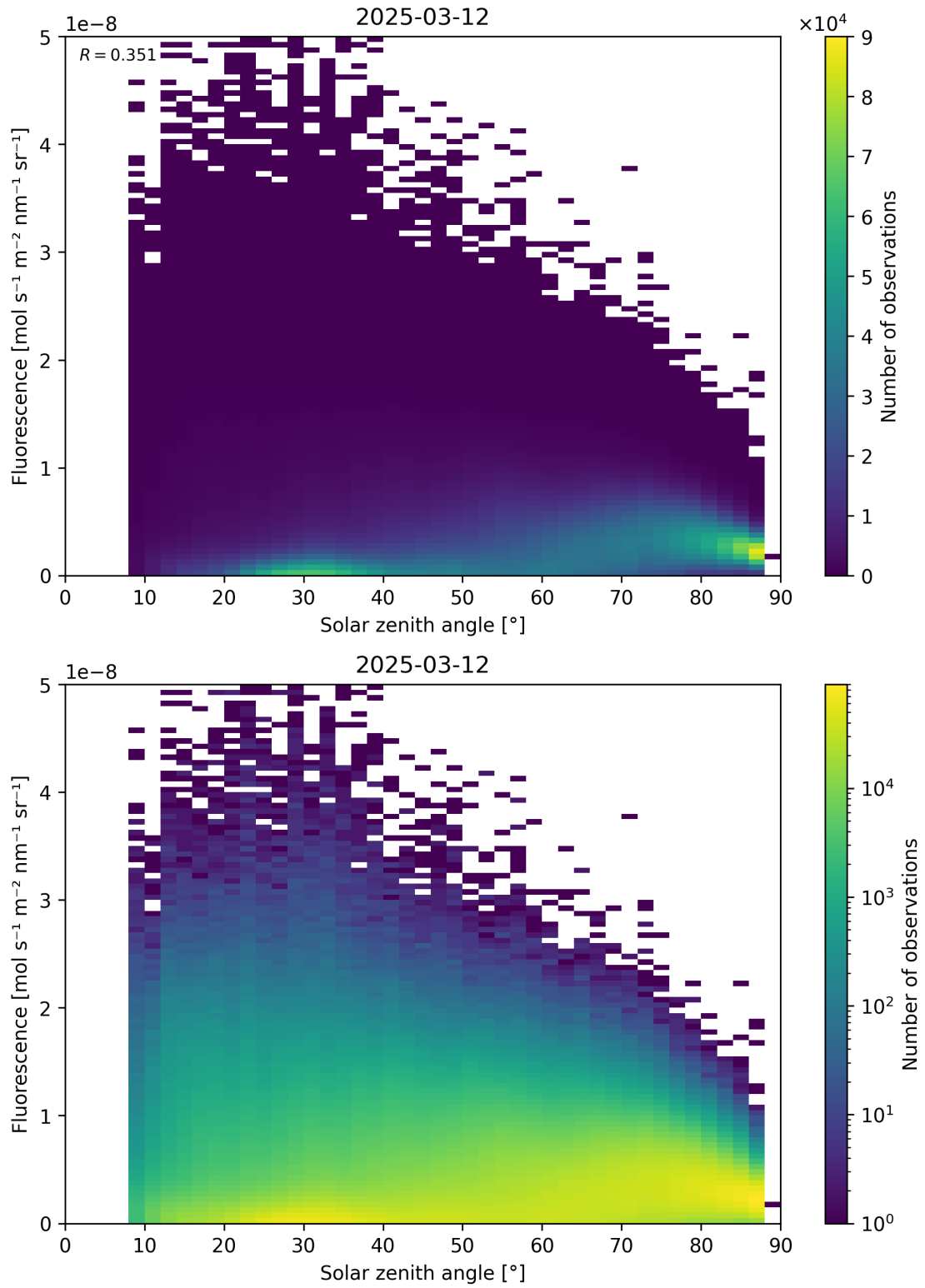
Figure 112: Scatter density plot of “Solar zenith angle” against “Fluorescence” for 2025-03-12 to 2025-03-13.
