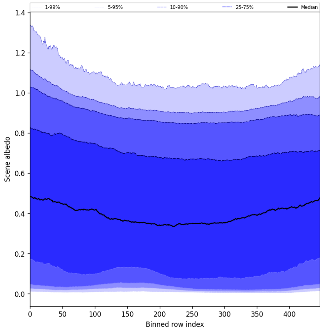
Figure 51: Along track statistics of “Scene albedo” for 2025-03-12 to 2025-03-13
