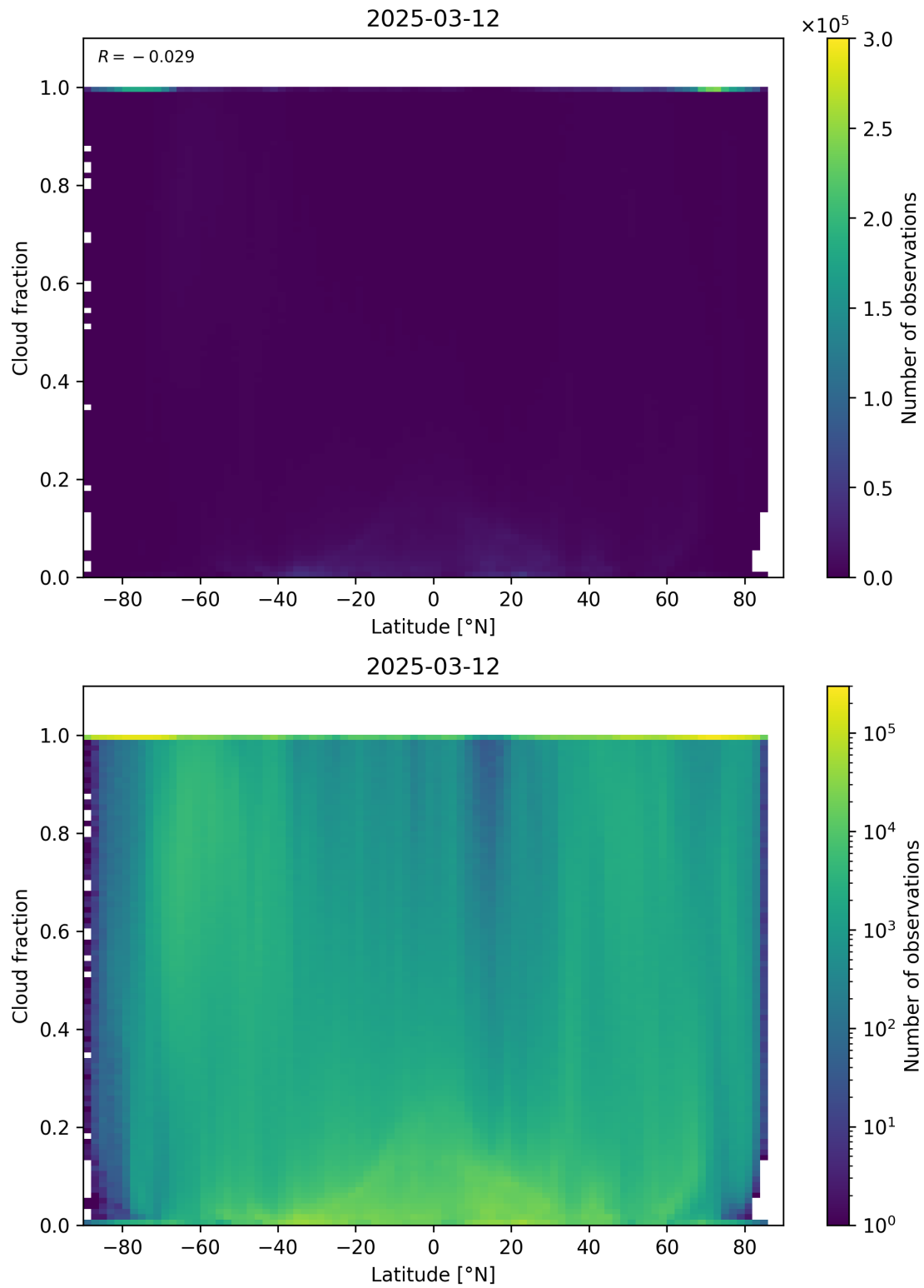
Figure 90: Scatter density plot of “Latitude” against “Cloud fraction” for 2025-03-12 to 2025-03-13.
