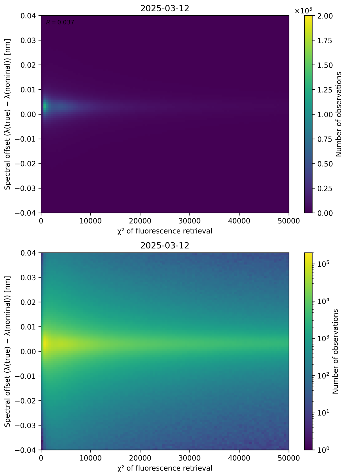
Figure 69: Scatter density plot of “ \chi^2 of fluorescence retrieval” against “Spectral offset ( \lambda_{\text{true}} - \lambda_{\text{nominal}} )” for 2025-03-12 to 2025-03-13.
