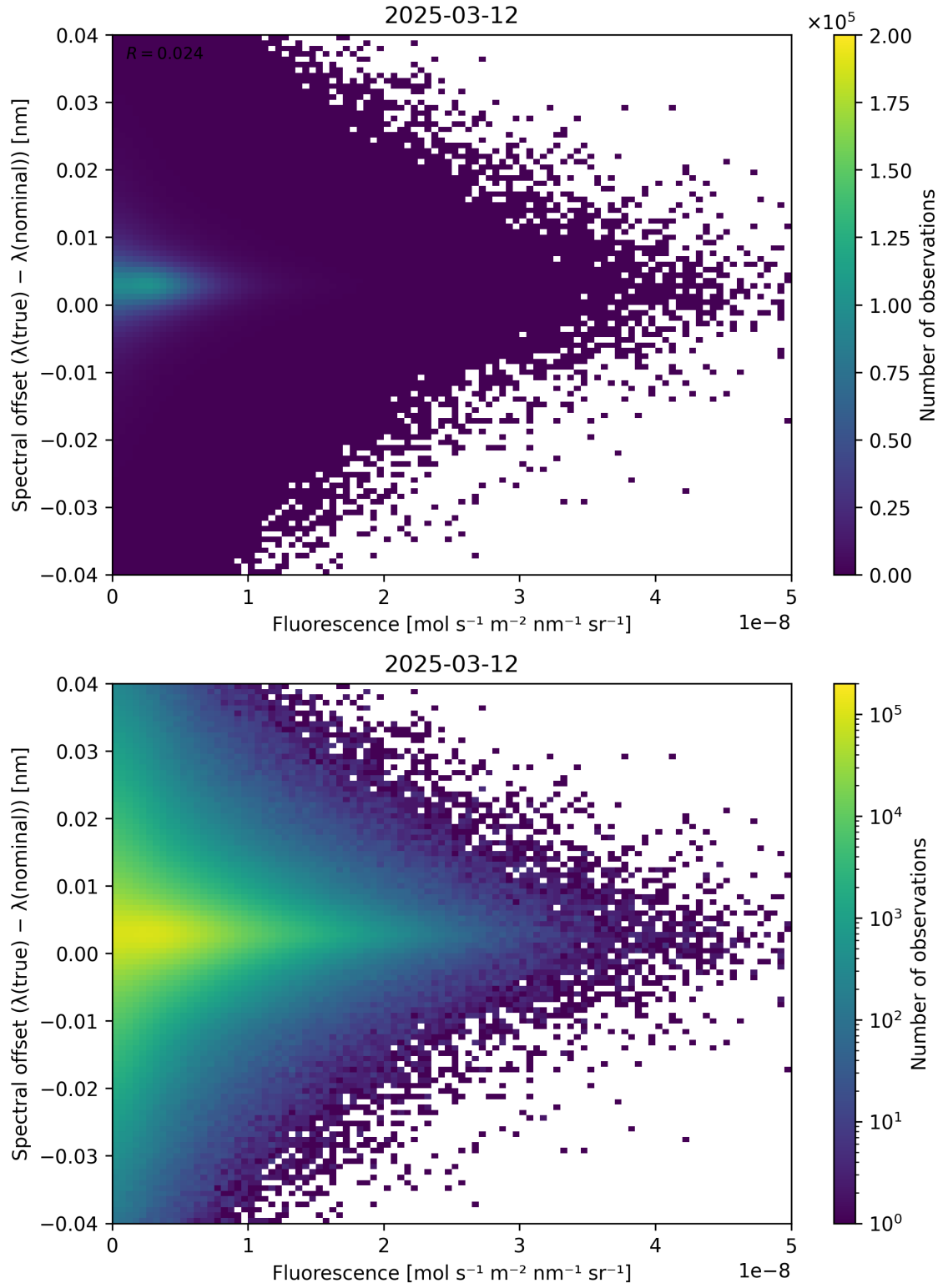
Figure 87: Scatter density plot of “Fluorescence” against “Spectral offset ( \lambda_{\text{true}} - \lambda_{\text{nominal}} )” for 2025-03-12 to 2025-03-13.
