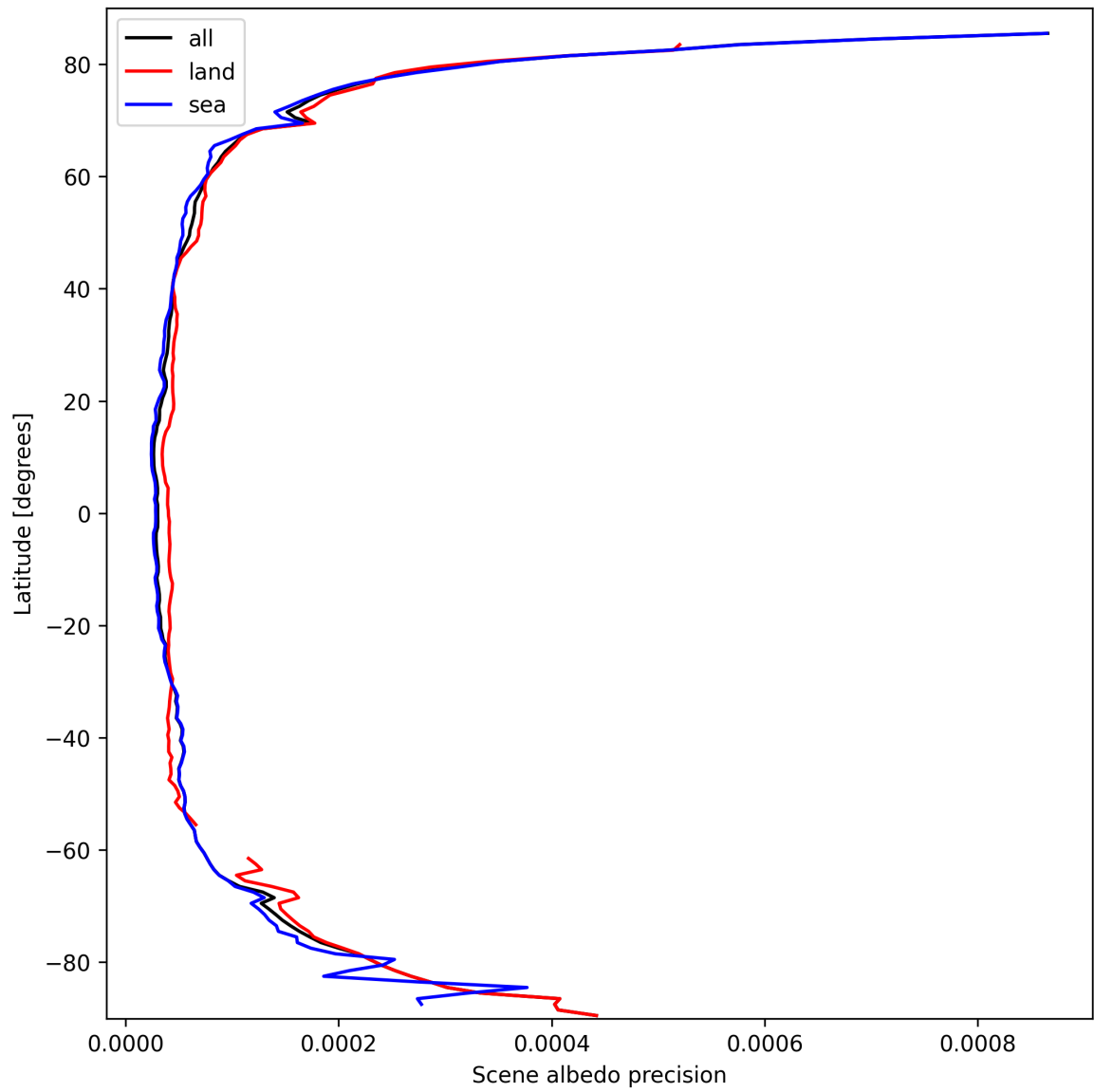
Figure 18: Zonal average of “Scene albedo precision” for 2025-03-12 to 2025-03-13.
