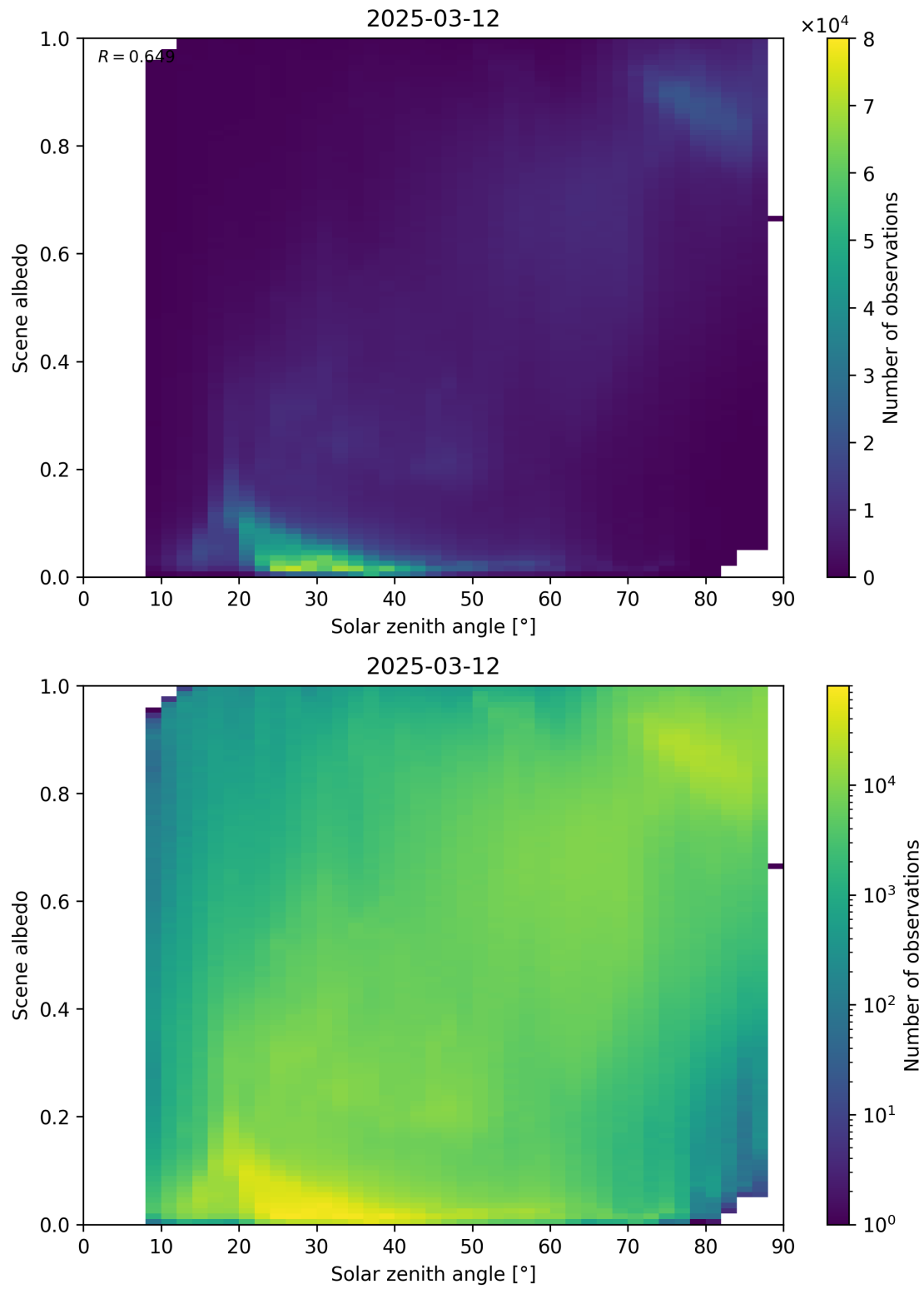
Figure 116: Scatter density plot of “Solar zenith angle” against “Scene albedo” for 2025-03-12 to 2025-03-13.
