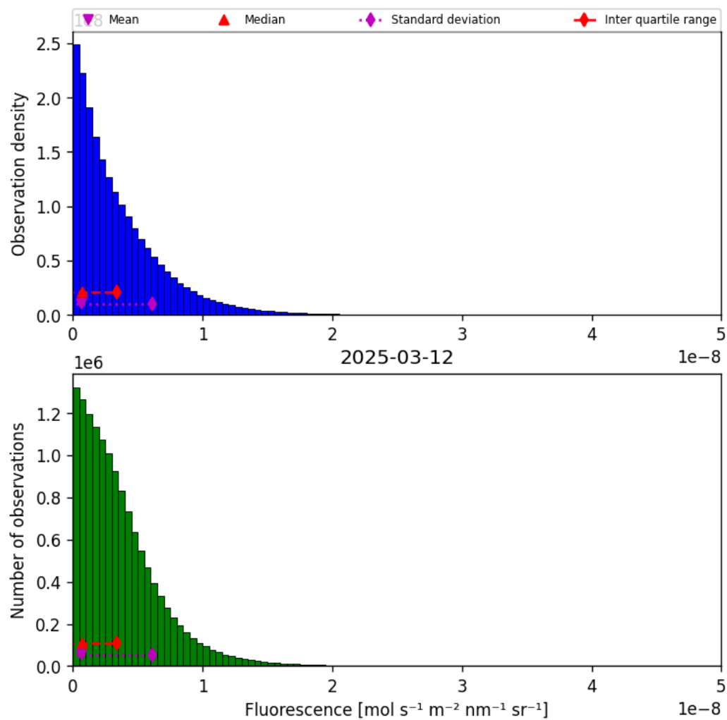
Figure 40: Histogram of “Fluorescence” for 2025-03-12 to 2025-03-13
