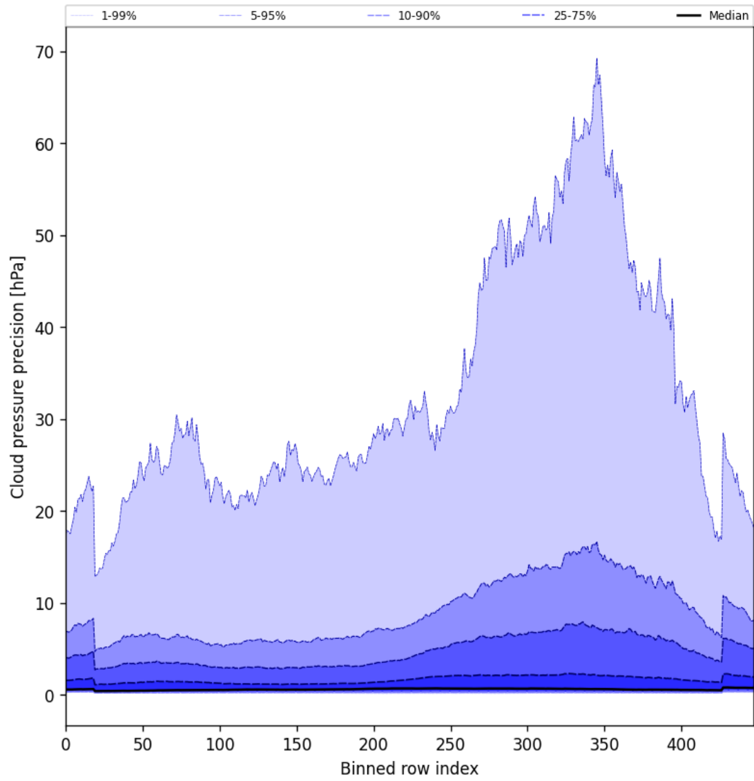
Figure 48: Along track statistics of “Cloud pressure precision” for 2025-03-12 to 2025-03-13
