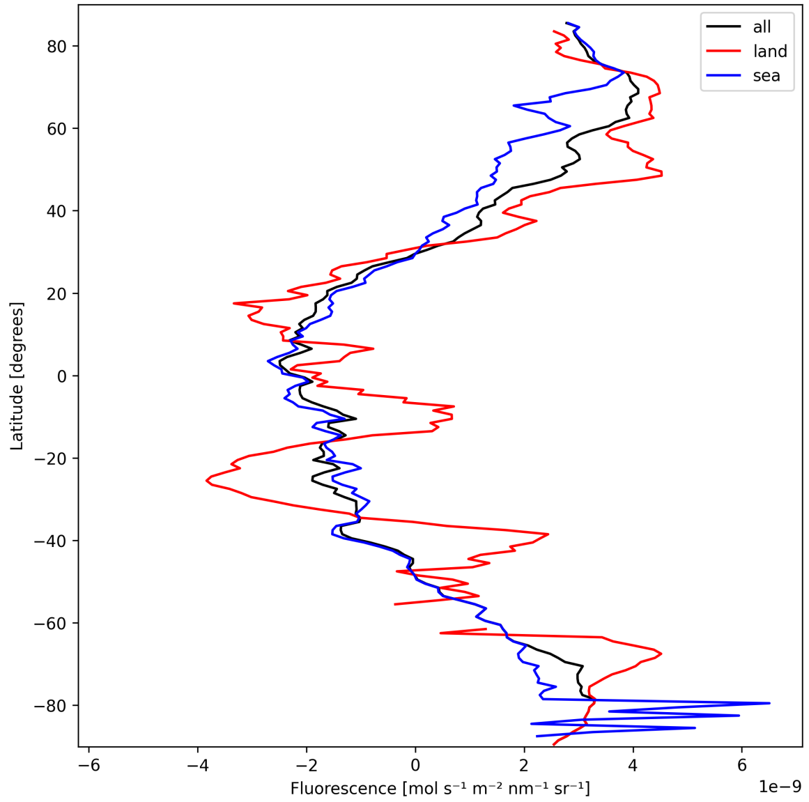
Figure 23: Zonal average of “Fluorescence” for 2025-03-12 to 2025-03-13.
