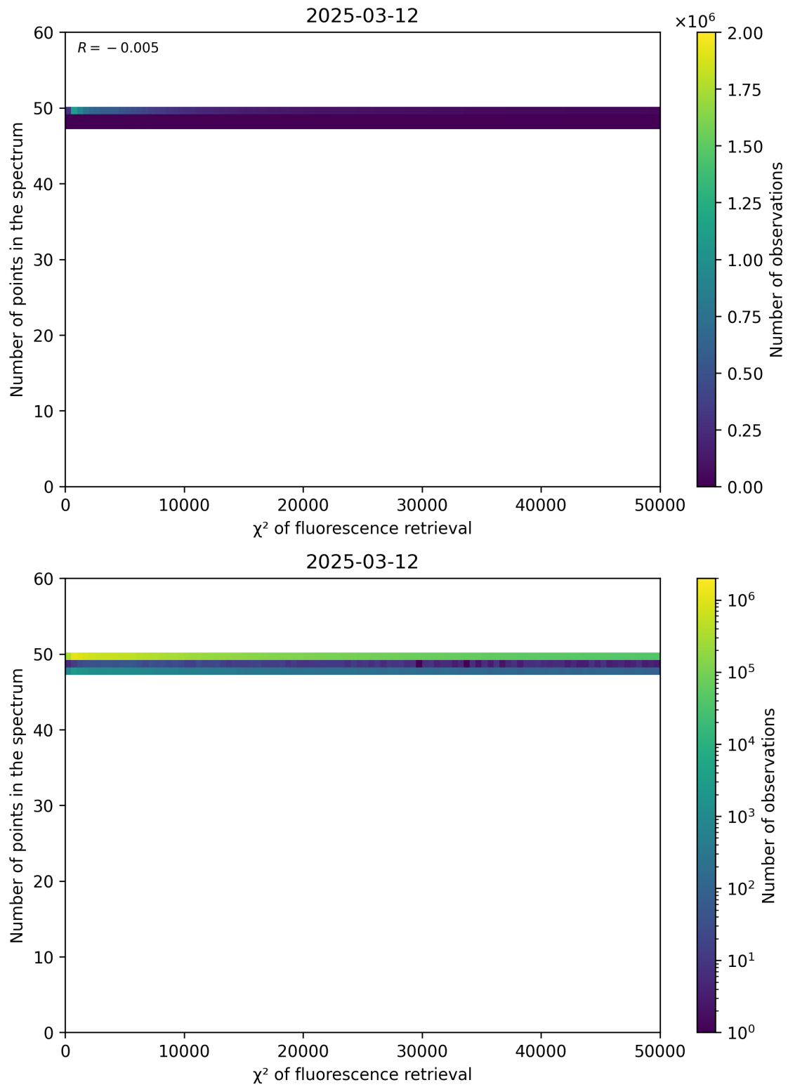
Figure 68: Scatter density plot of " \chi^2 of fluorescence retrieval" against "Number of points in the spectrum" for 2025-03-12 to 2025-03-13.
