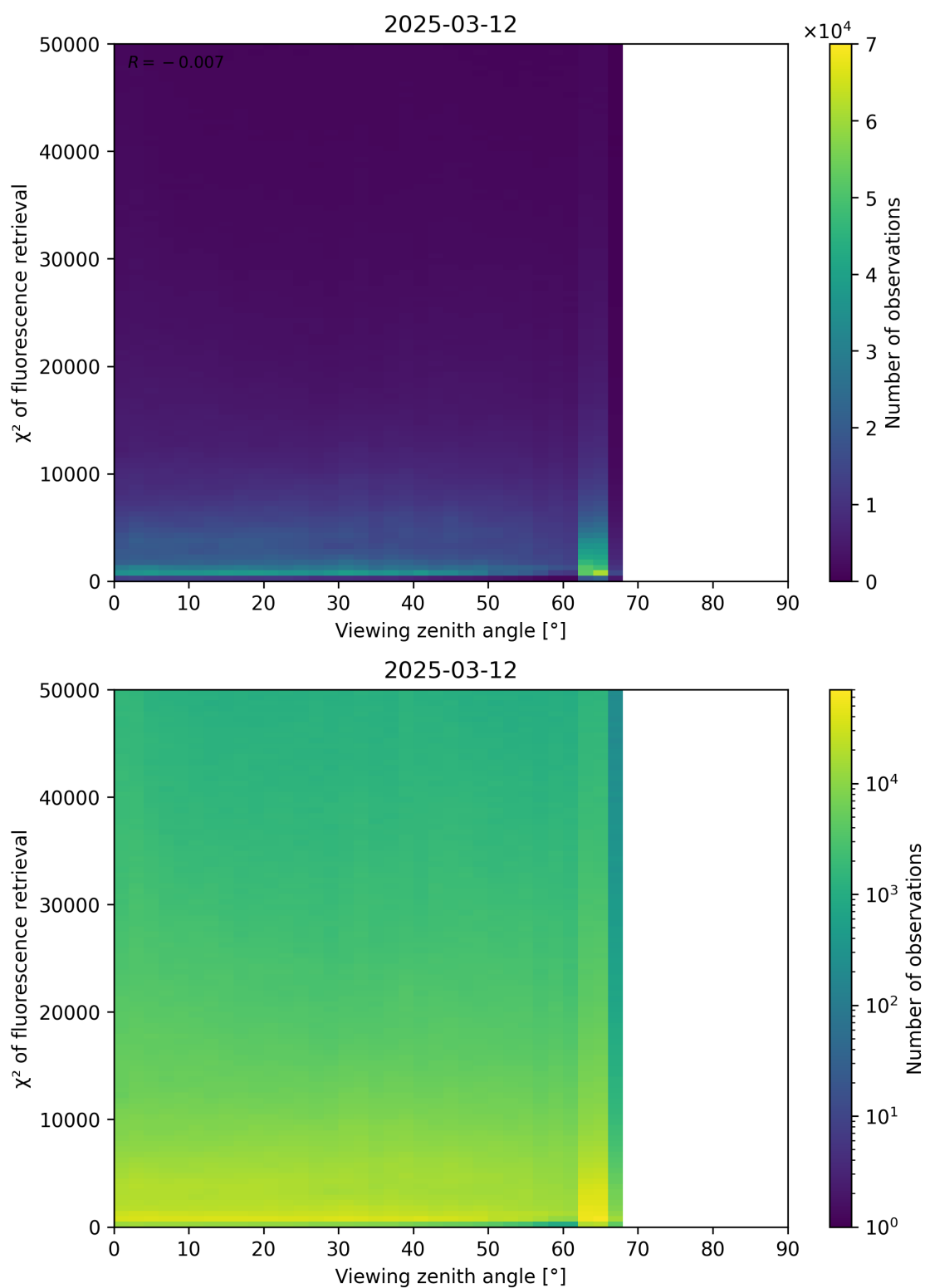
Figure 119: Scatter density plot of “Viewing zenith angle” against “ \chi^2 of fluorescence retrieval” for 2025-03-12 to 2025-03-13.
