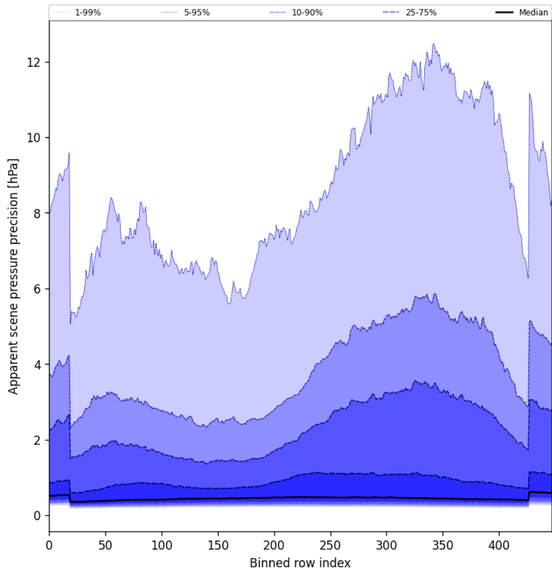
Figure 54: Along track statistics of “Apparent scene pressure precision” for 2025-03-12 to 2025-03-13
