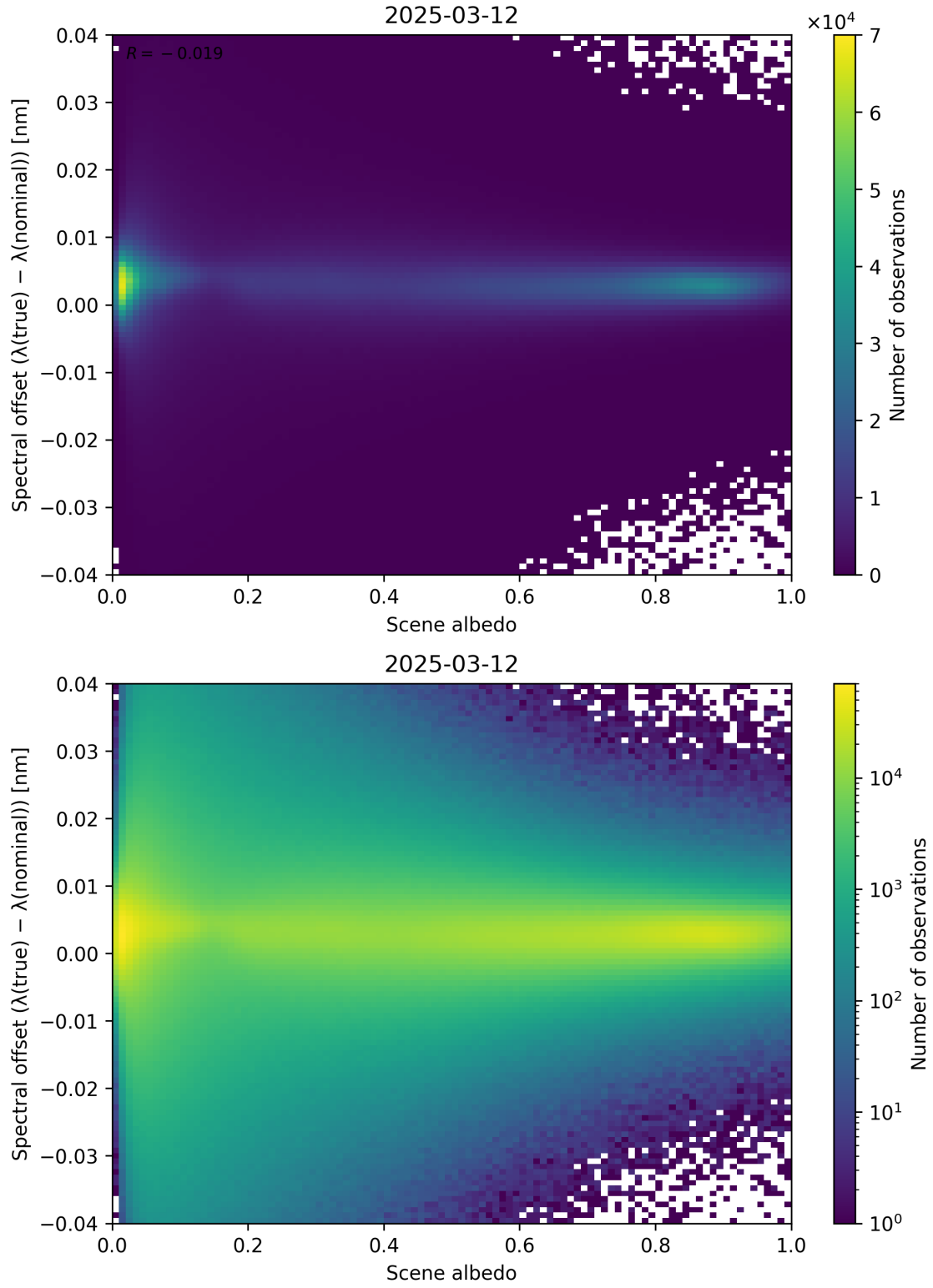
Figure 107: Scatter density plot of “Scene albedo” against “Spectral offset ( \lambda_{\text{true}} - \lambda_{\text{nominal}} )” for 2025-03-12 to 2025-03-13.
