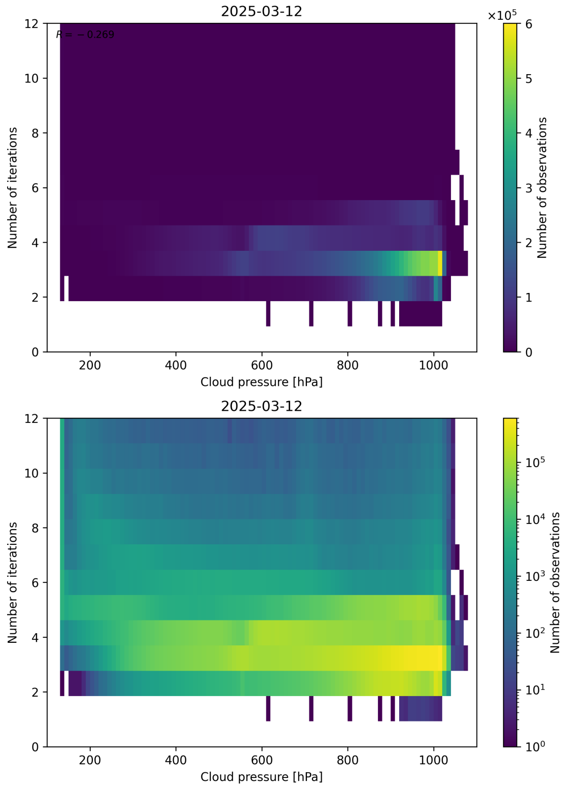
Figure 81: Scatter density plot of “Cloud pressure” against “Number of iterations” for 2025-03-12 to 2025-03-13.
