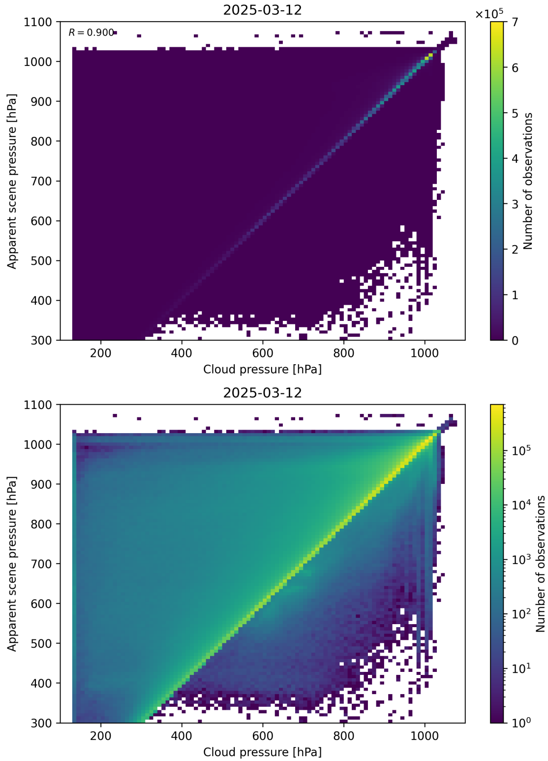
Figure 77: Scatter density plot of “Cloud pressure” against “Apparent scene pressure” for 2025-03-12 to 2025-03-13.
