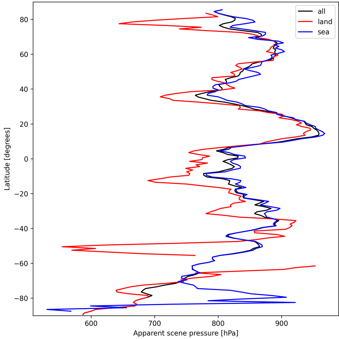
Figure 19: Zonal average of “Apparent scene pressure” for 2025-03-12 to 2025-03-13.
