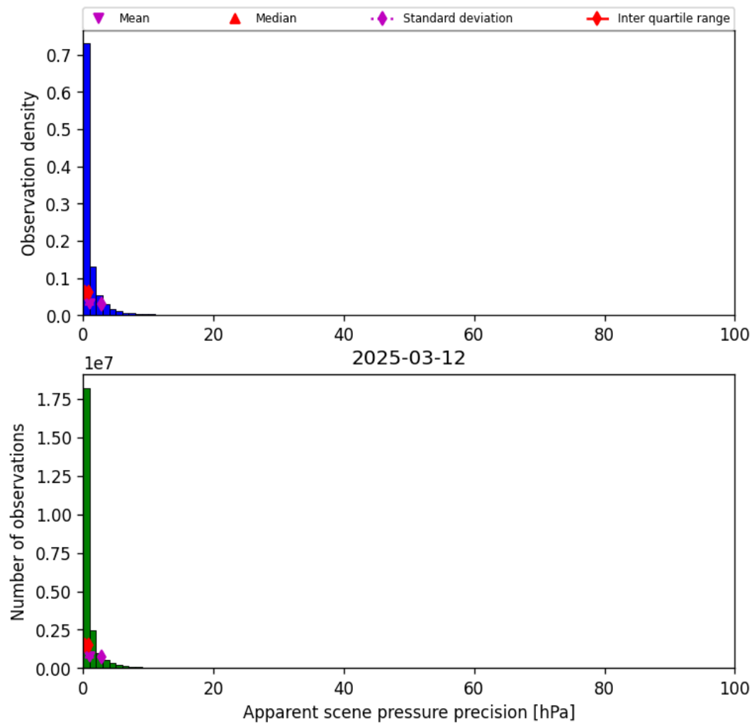
Figure 37: Histogram of “Apparent scene pressure precision” for 2025-03-12 to 2025-03-13
