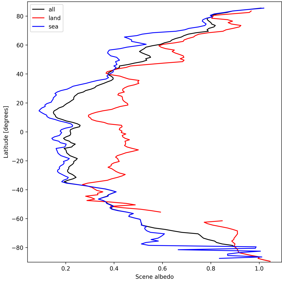
Figure 17: Zonal average of "Scene albedo" for 2025-03-12 to 2025-03-13.
