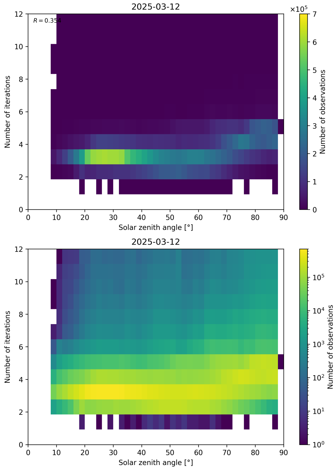
Figure 114: Scatter density plot of “Solar zenith angle” against “Number of iterations” for 2025-03-12 to 2025-03-13.
