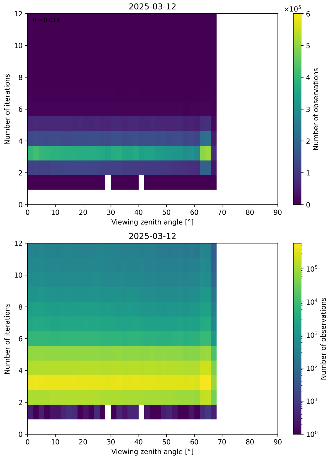
Figure 124: Scatter density plot of “Viewing zenith angle” against “Number of iterations” for 2025-03-12 to 2025-03-13.
