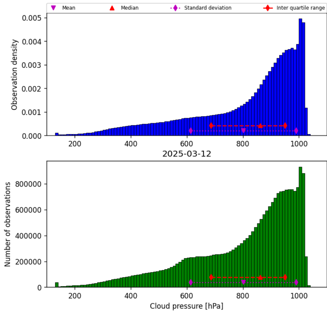
Figure 30: Histogram of “Cloud pressure” for 2025-03-12 to 2025-03-13
