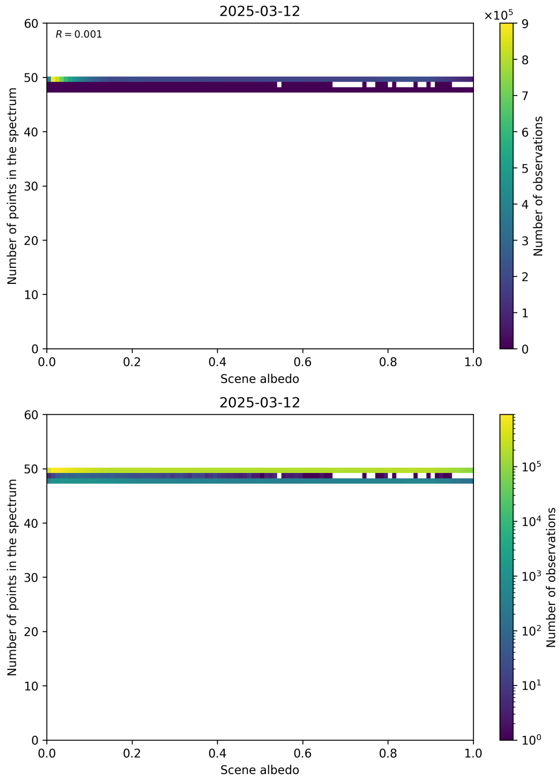
Figure 106: Scatter density plot of “Scene albedo” against “Number of points in the spectrum” for 2025-03-12 to 2025-03-13.
