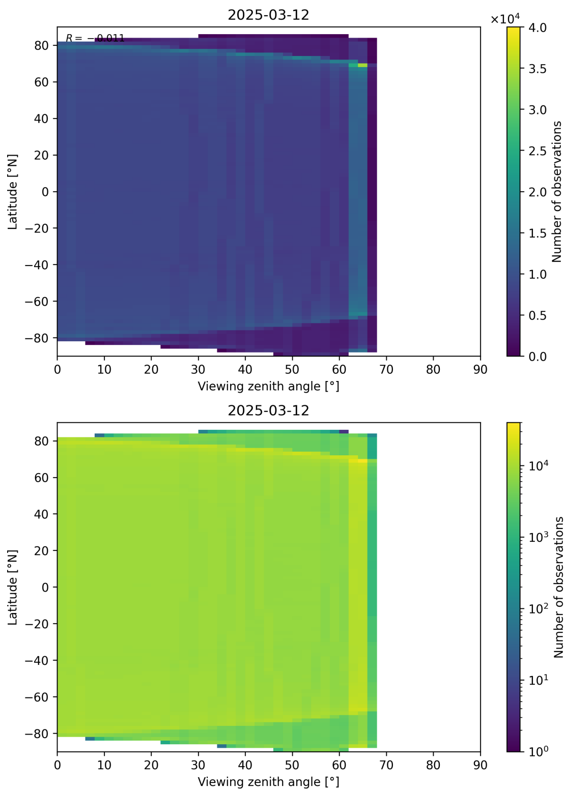
Figure 123: Scatter density plot of “Viewing zenith angle” against “Latitude” for 2025-03-12 to 2025-03-13.
