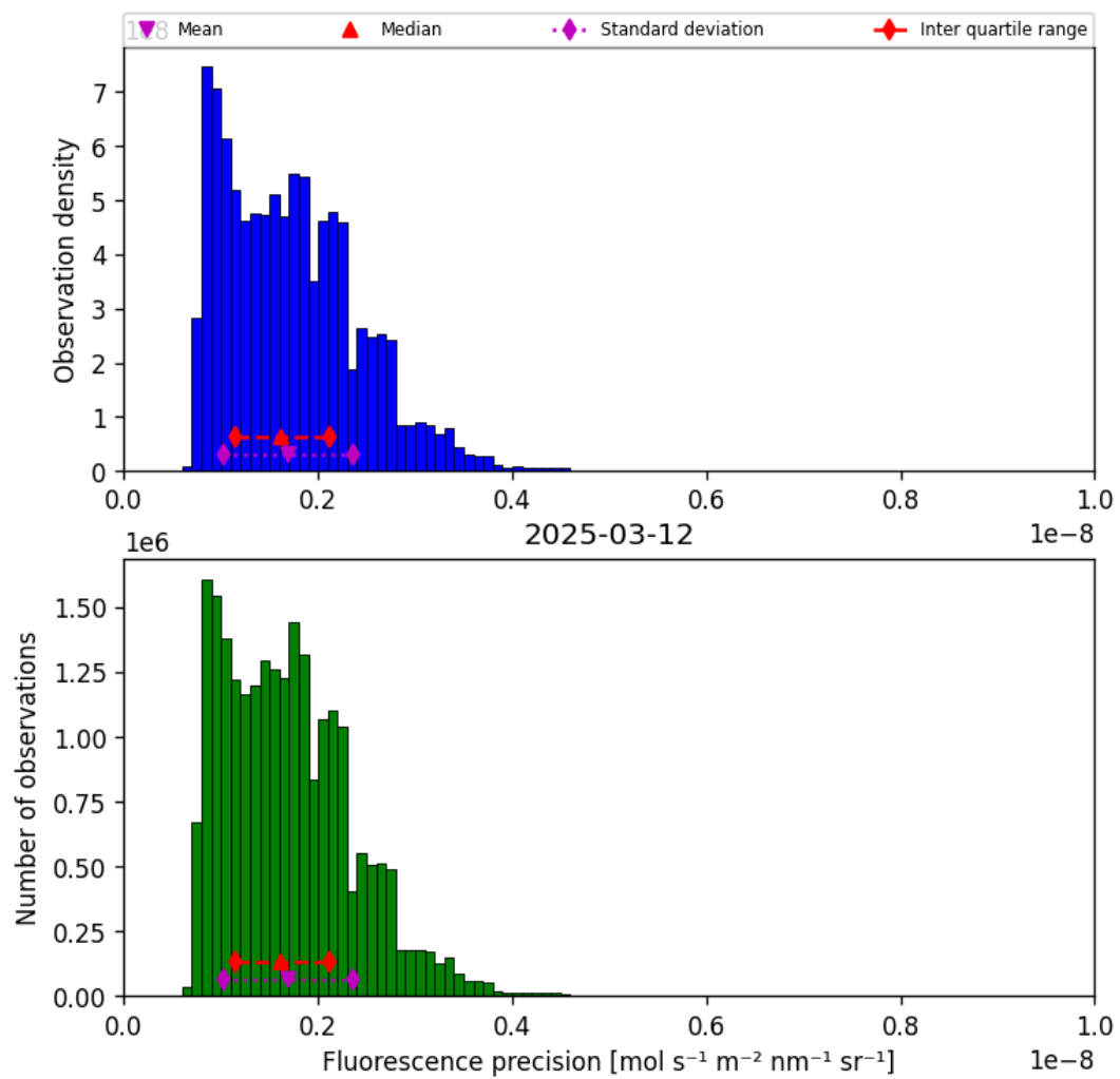
Figure 41: Histogram of “Fluorescence precision” for 2025-03-12 to 2025-03-13
