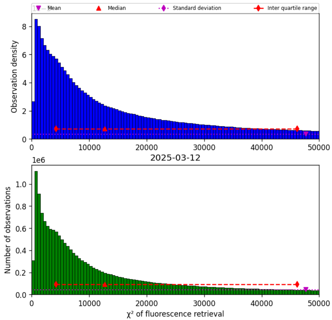
Figure 42: Histogram of “ \chi^2 of fluorescence retrieval” for 2025-03-12 to 2025-03-13
