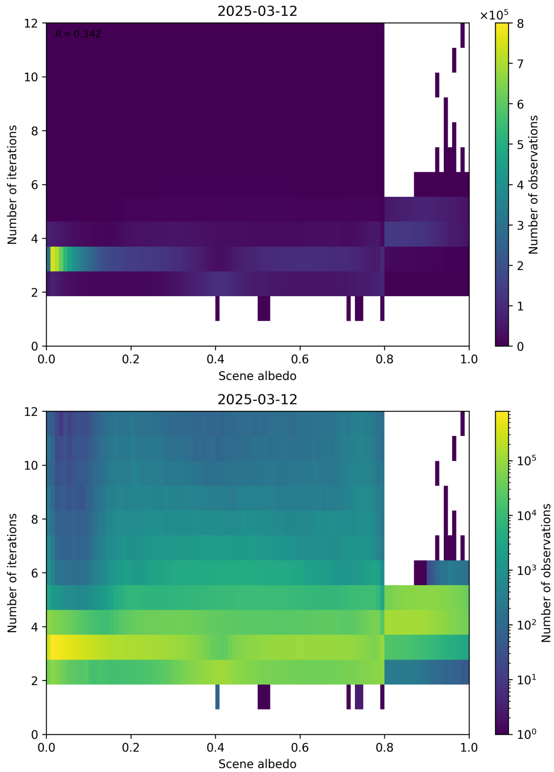
Figure 105: Scatter density plot of “Scene albedo” against “Number of iterations” for 2025-03-12 to 2025-03-13.
