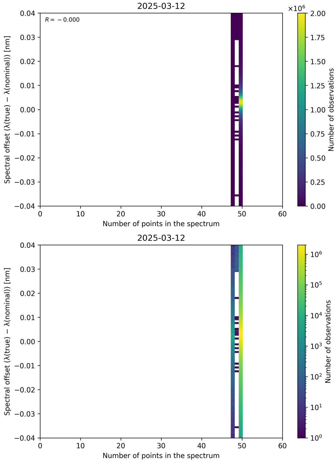
Figure 101: Scatter density plot of “Number of points in the spectrum” against “Spectral offset ( \lambda_{\text{true}} - \lambda_{\text{nominal}} )” for 2025-03-12 to 2025-03-13.
