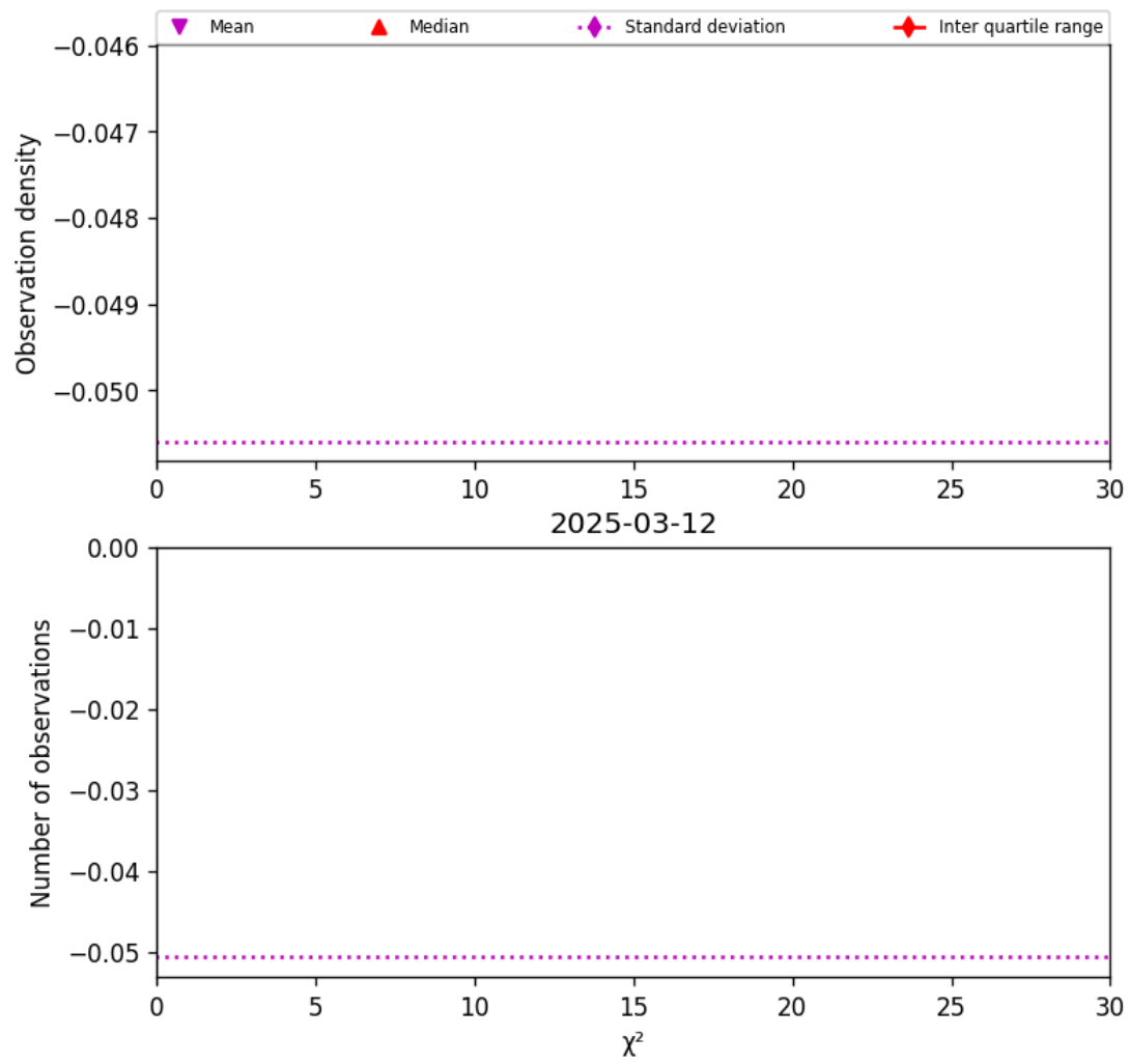
Figure 38: Histogram of “ \chi^2 ” for 2025-03-12 to 2025-03-13
