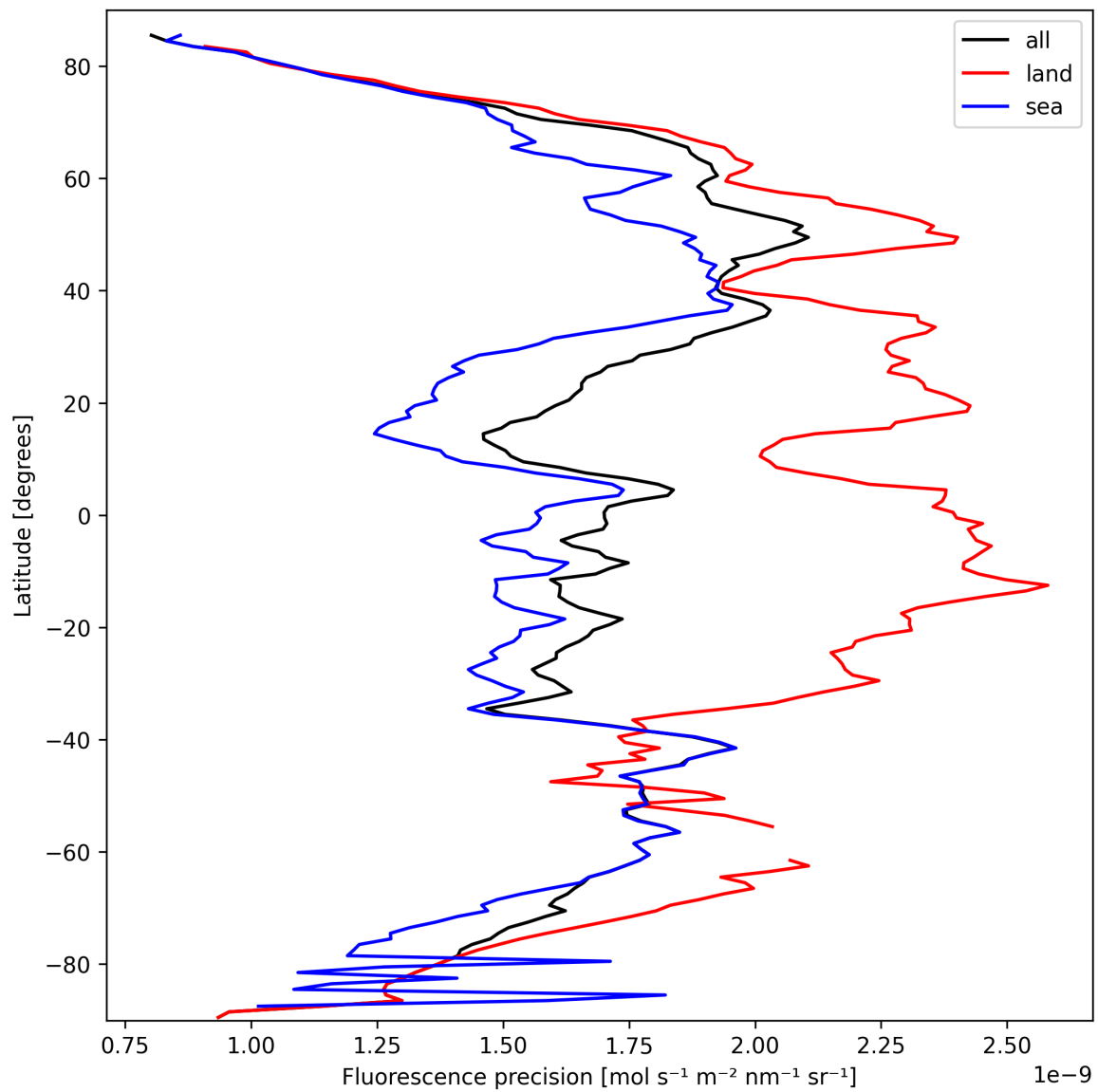
Figure 24: Zonal average of “Fluorescence precision” for 2025-03-12 to 2025-03-13.
