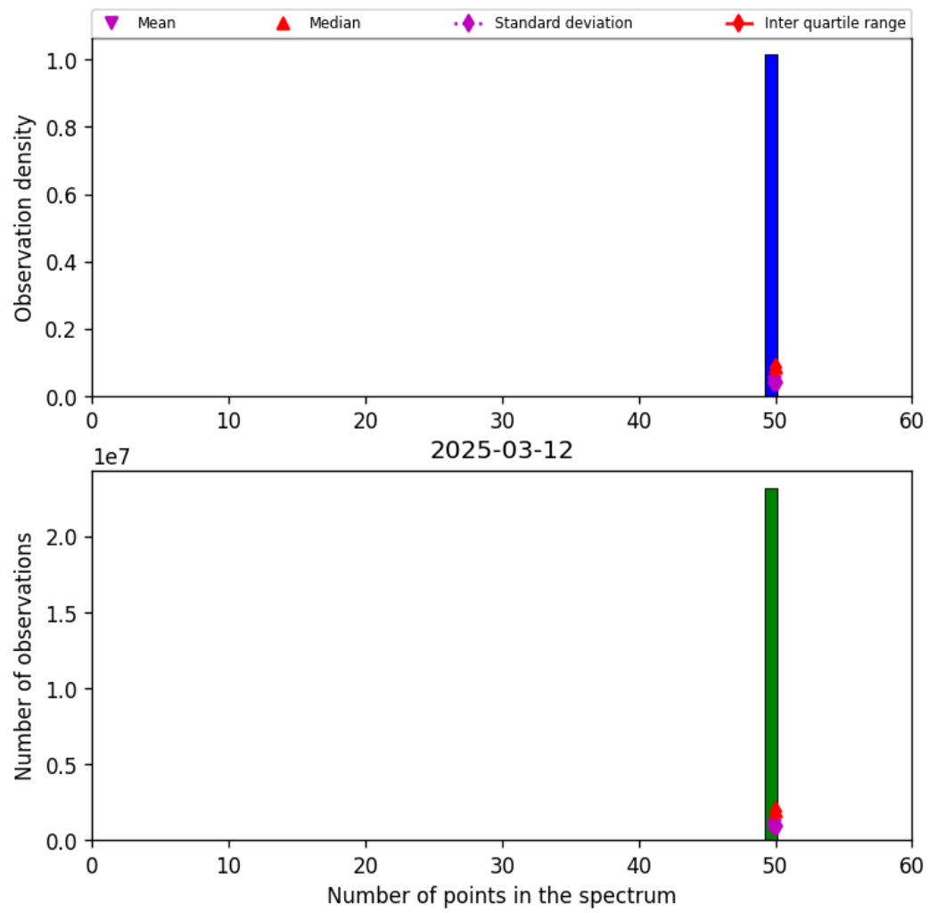
Figure 44: Histogram of “Number of points in the spectrum” for 2025-03-12 to 2025-03-13
