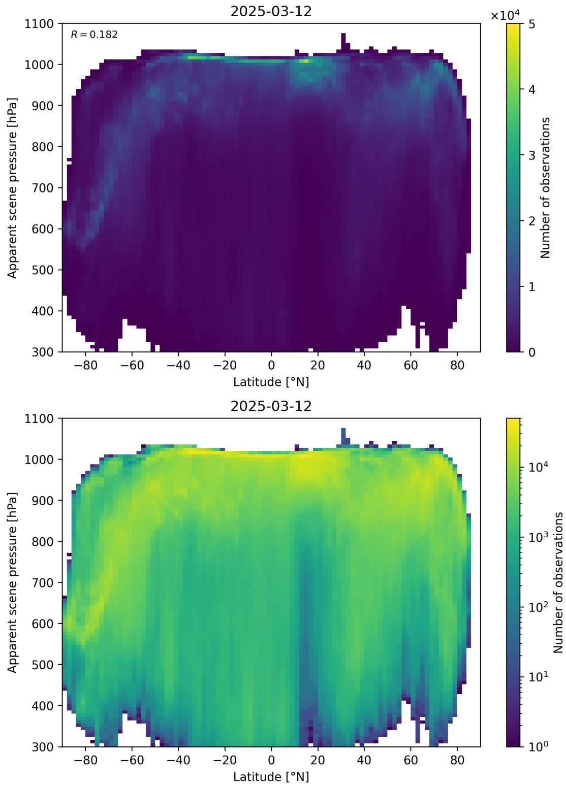
Figure 88: Scatter density plot of “Latitude” against “Apparent scene pressure” for 2025-03-12 to 2025-03-13.
