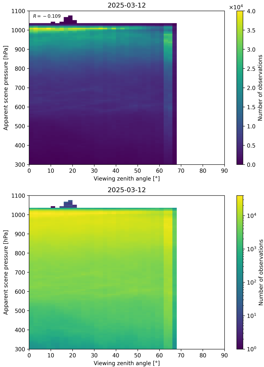
Figure 118: Scatter density plot of “Viewing zenith angle” against “Apparent scene pressure” for 2025-03-12 to 2025-03-13.
