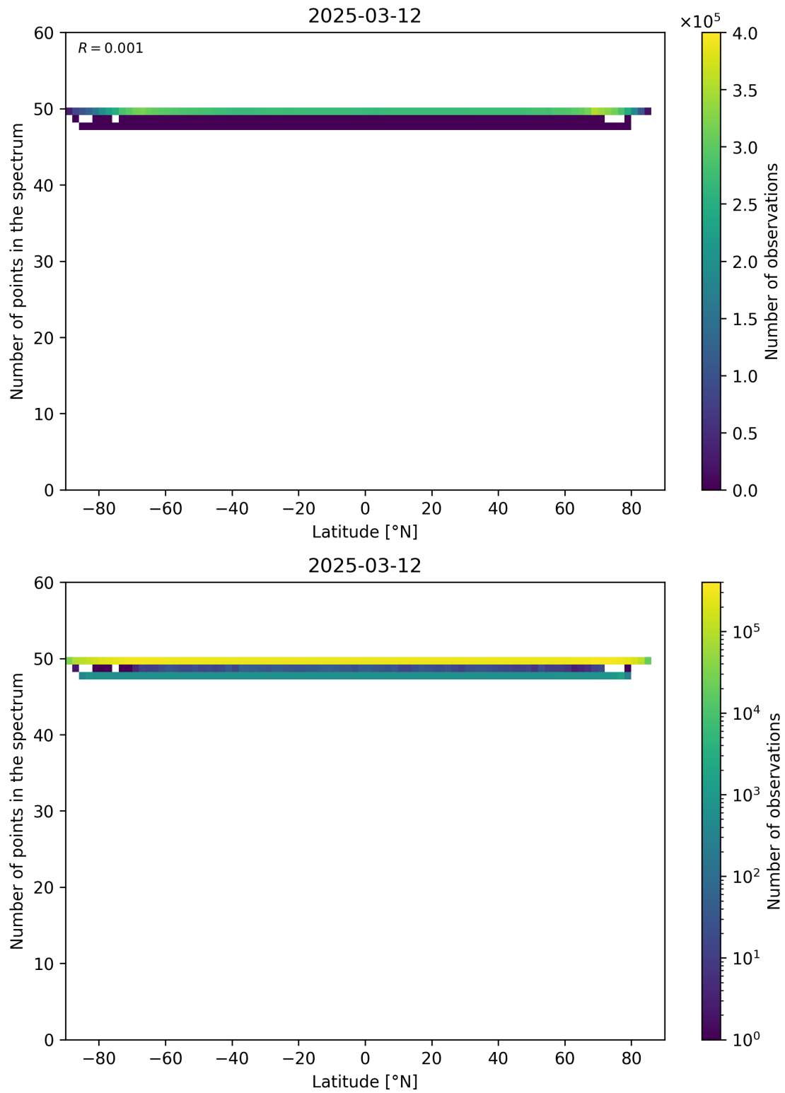
Figure 94: Scatter density plot of “Latitude” against “Number of points in the spectrum” for 2025-03-12 to 2025-03-13.
