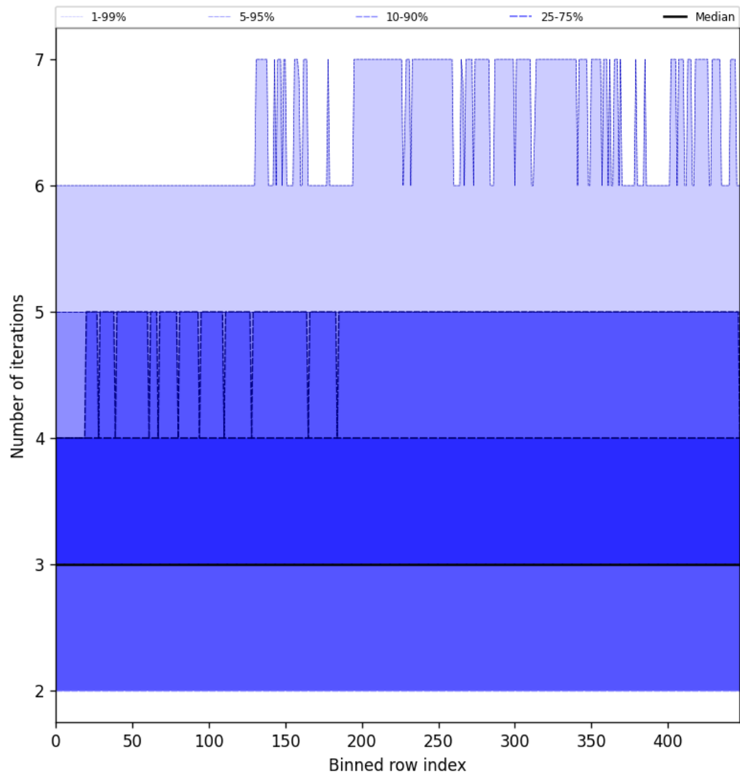
Figure 56: Along track statistics of “Number of iterations” for 2025-03-12 to 2025-03-13
