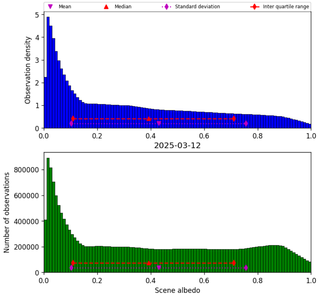
Figure 34: Histogram of “Scene albedo” for 2025-03-12 to 2025-03-13
