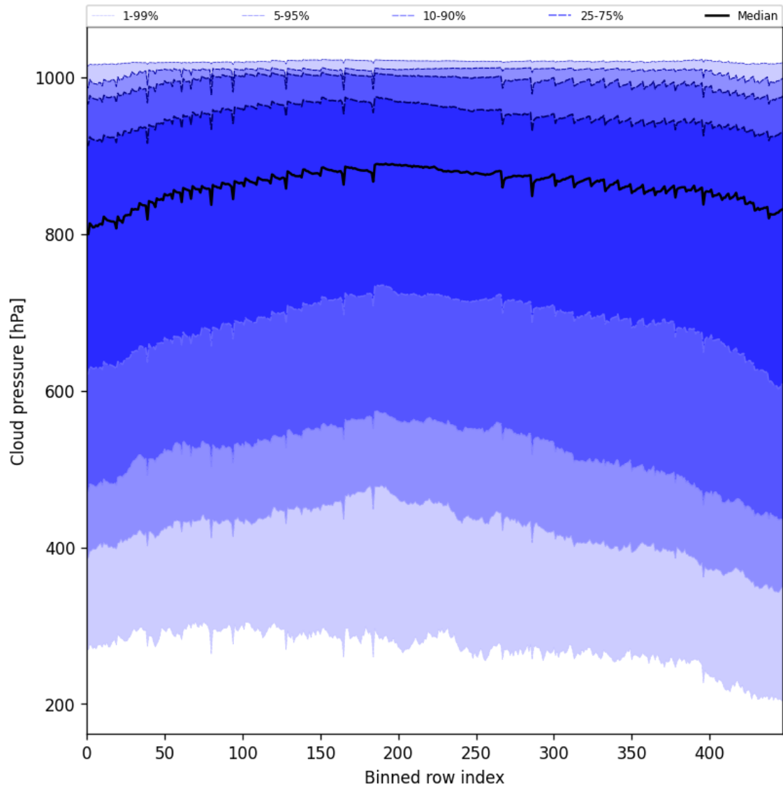
Figure 47: Along track statistics of “Cloud pressure” for 2025-03-12 to 2025-03-13
