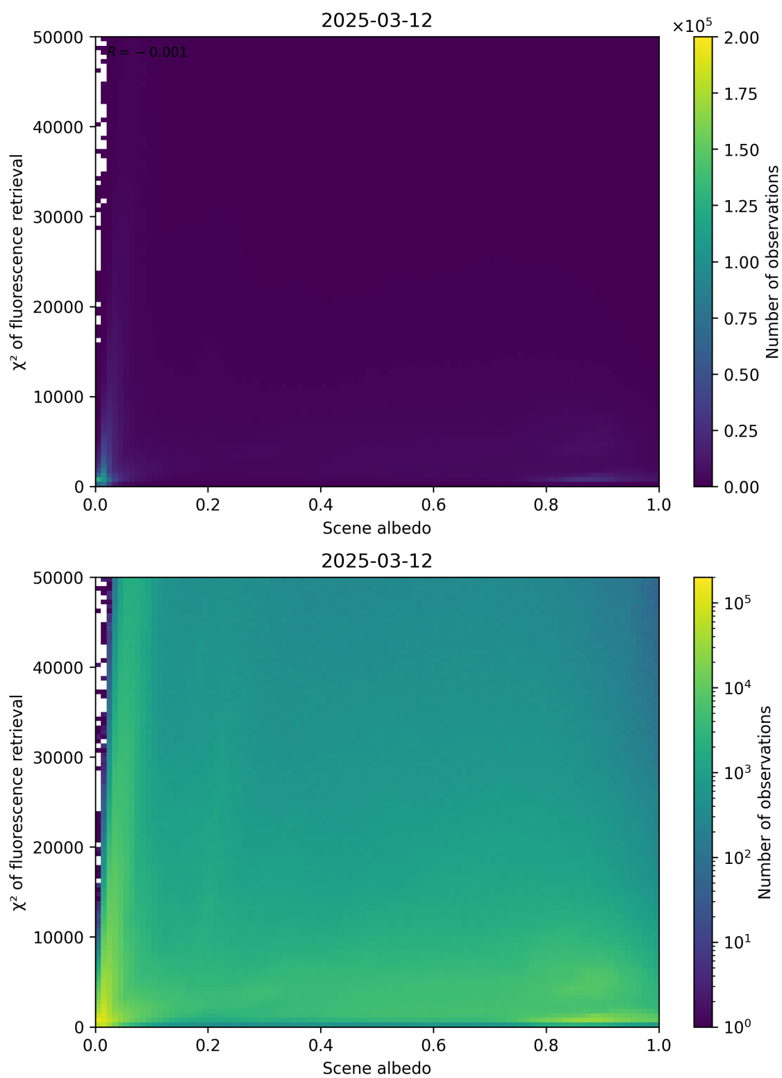
Figure 103: Scatter density plot of “Scene albedo” against “ \chi^2 of fluorescence retrieval” for 2025-03-12 to 2025-03-13.
