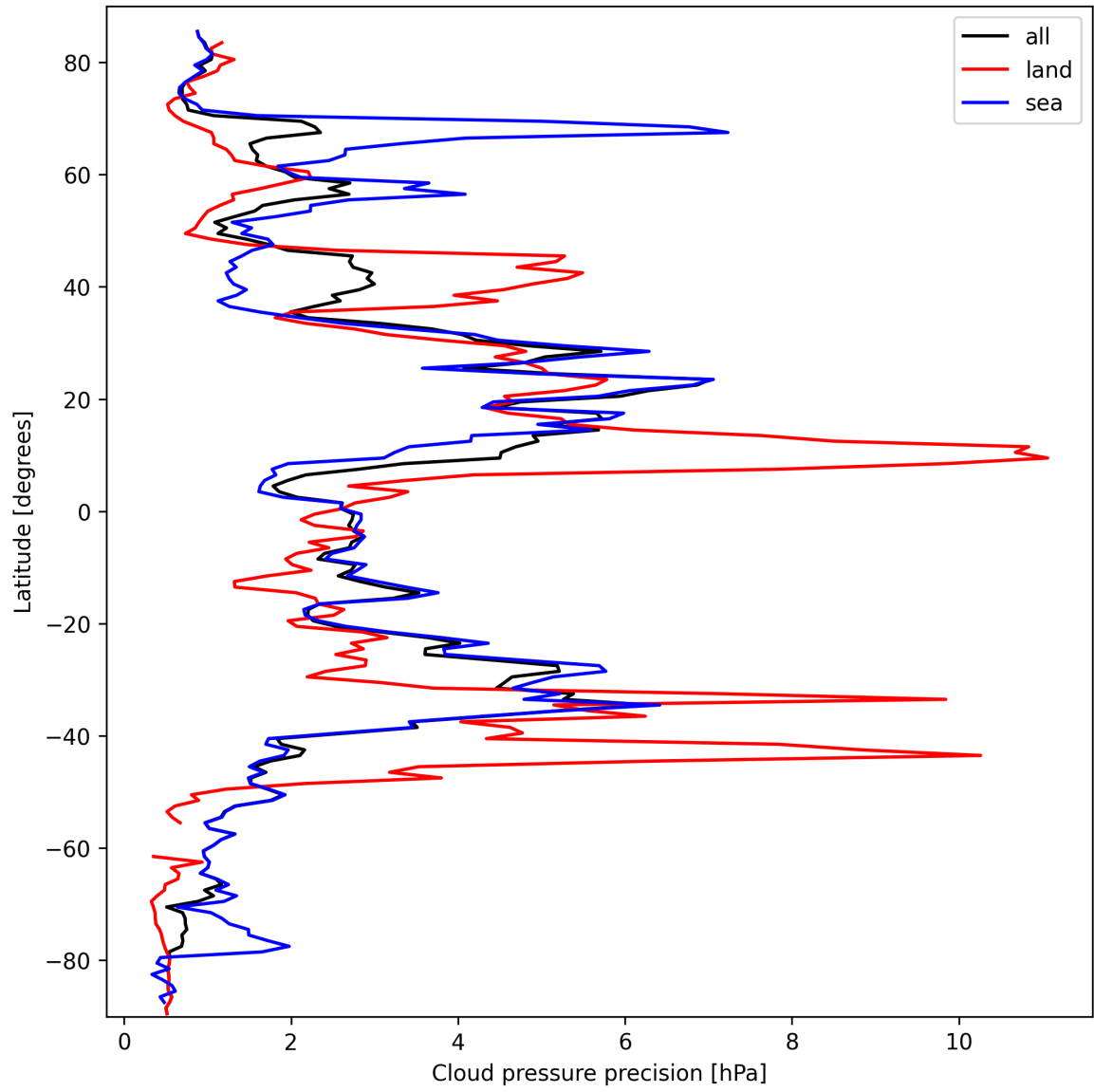
Figure 14: Zonal average of “Cloud pressure precision” for 2025-03-12 to 2025-03-13.
