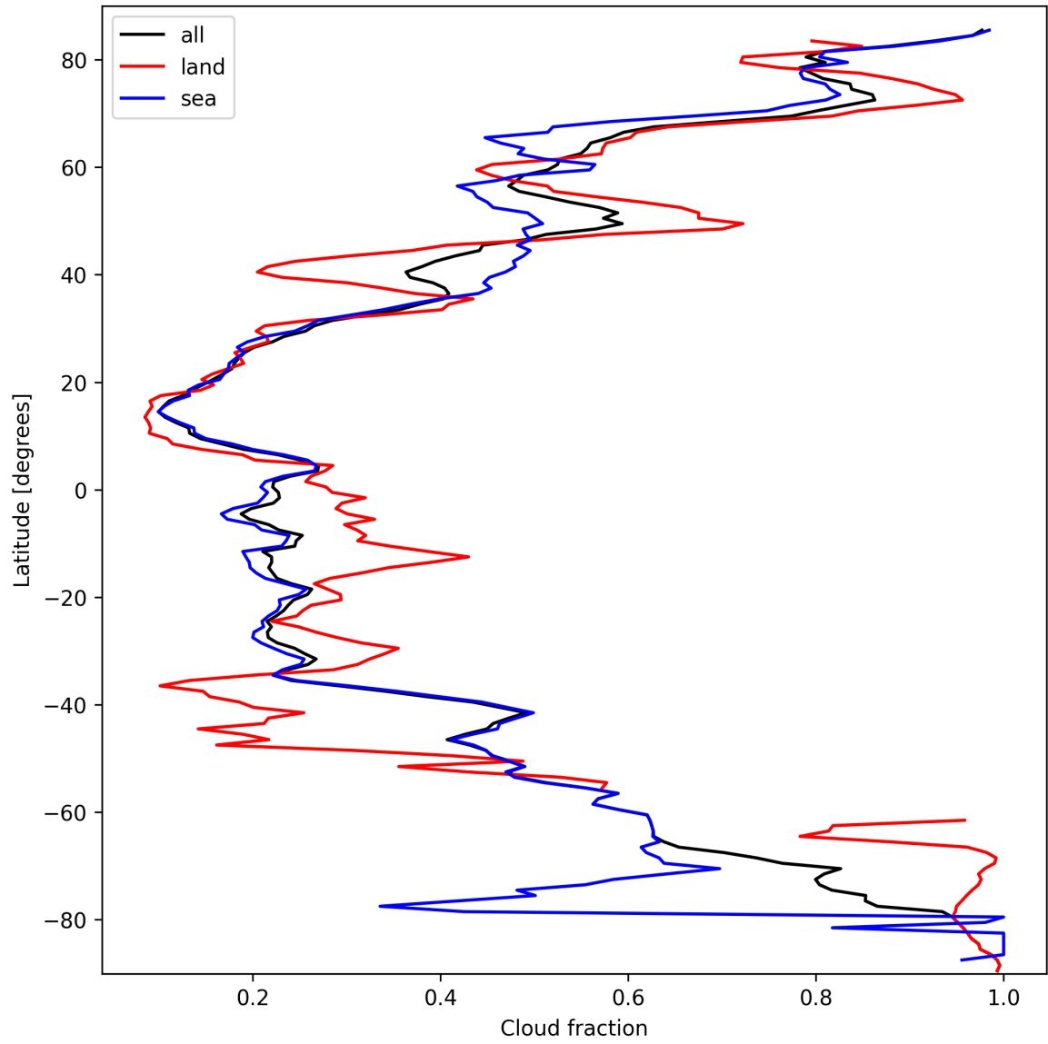
Figure 15: Zonal average of “Cloud fraction” for 2025-03-12 to 2025-03-13.
