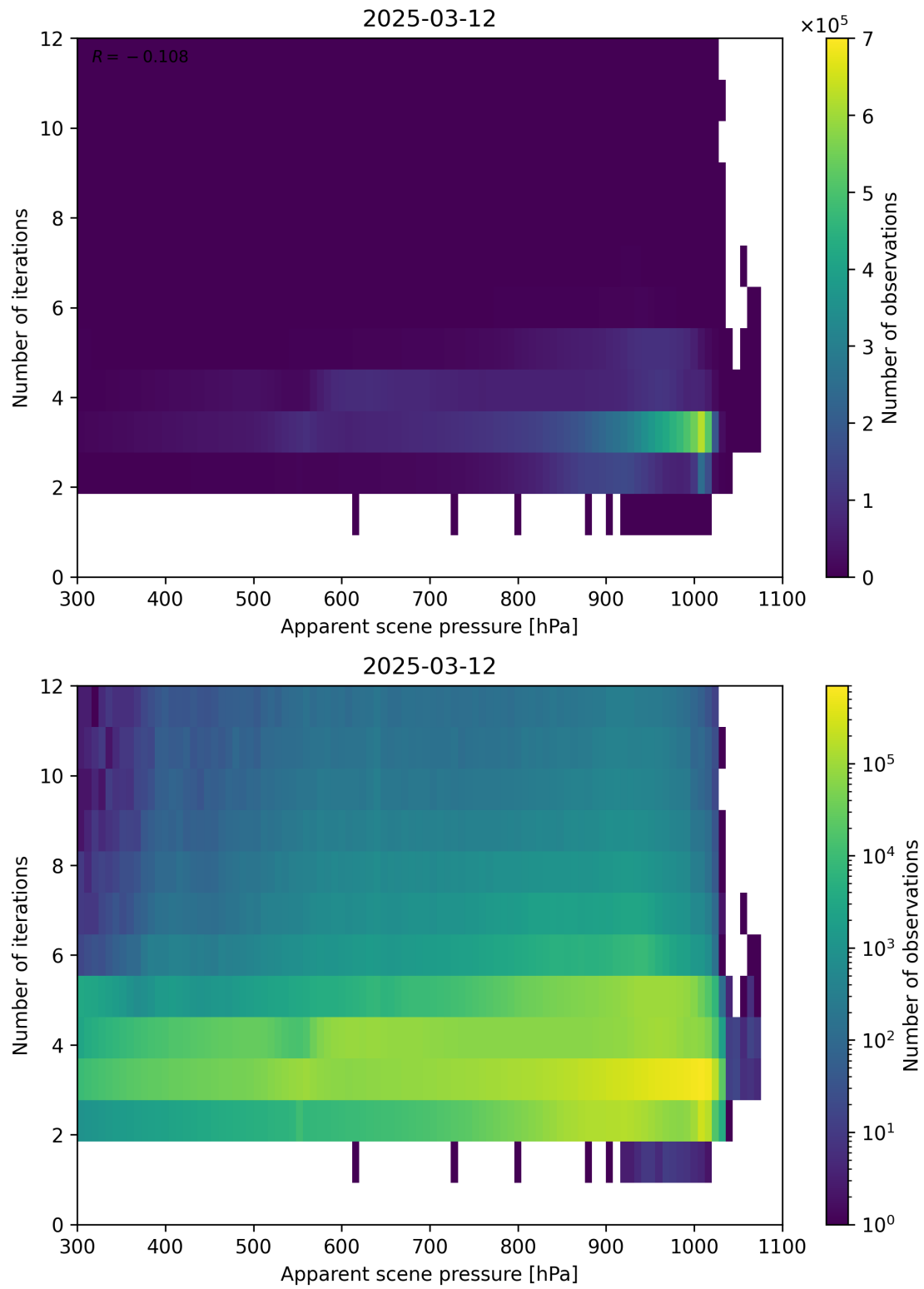
Figure 65: Scatter density plot of “Apparent scene pressure” against “Number of iterations” for 2025-03-12 to 2025-03-13.
