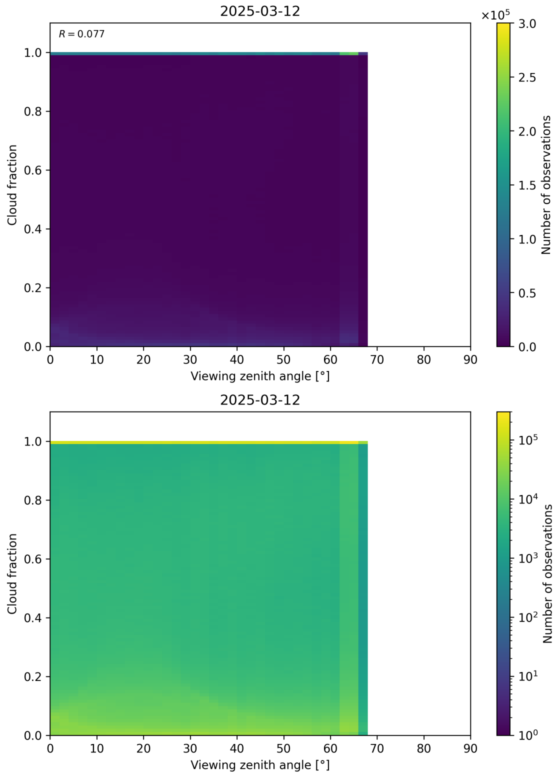
Figure 120: Scatter density plot of “Viewing zenith angle” against “Cloud fraction” for 2025-03-12 to 2025-03-13.
