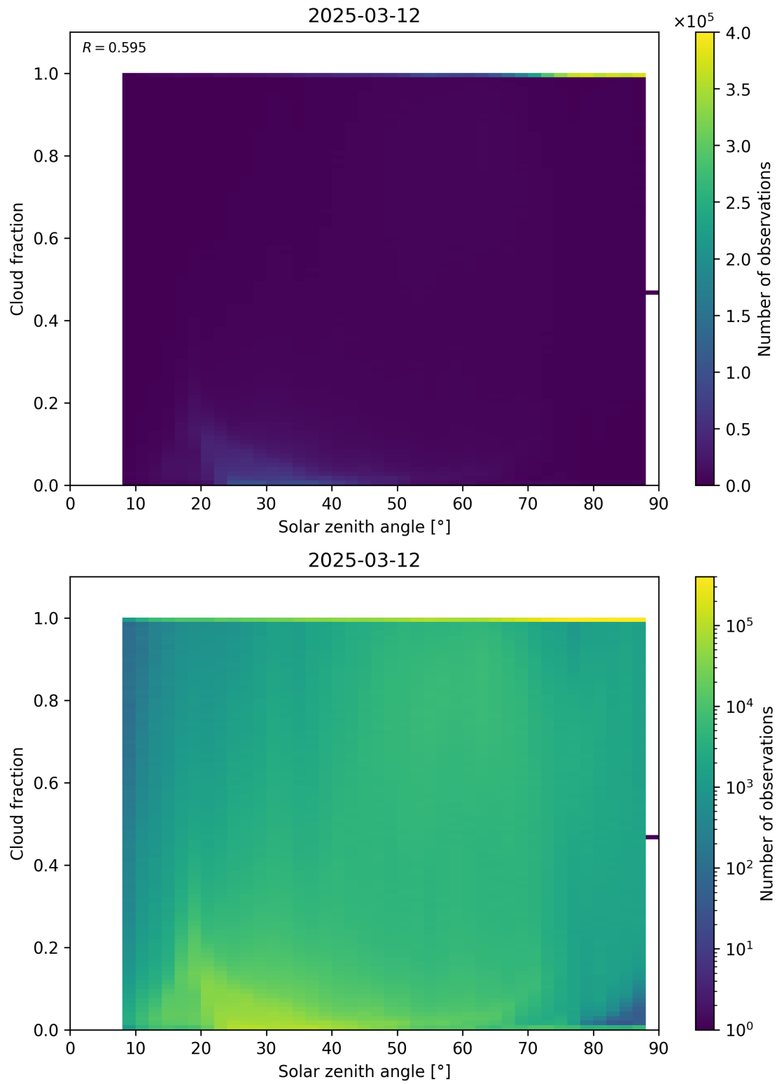
Figure 110: Scatter density plot of “Solar zenith angle” against “Cloud fraction” for 2025-03-12 to 2025-03-13.
