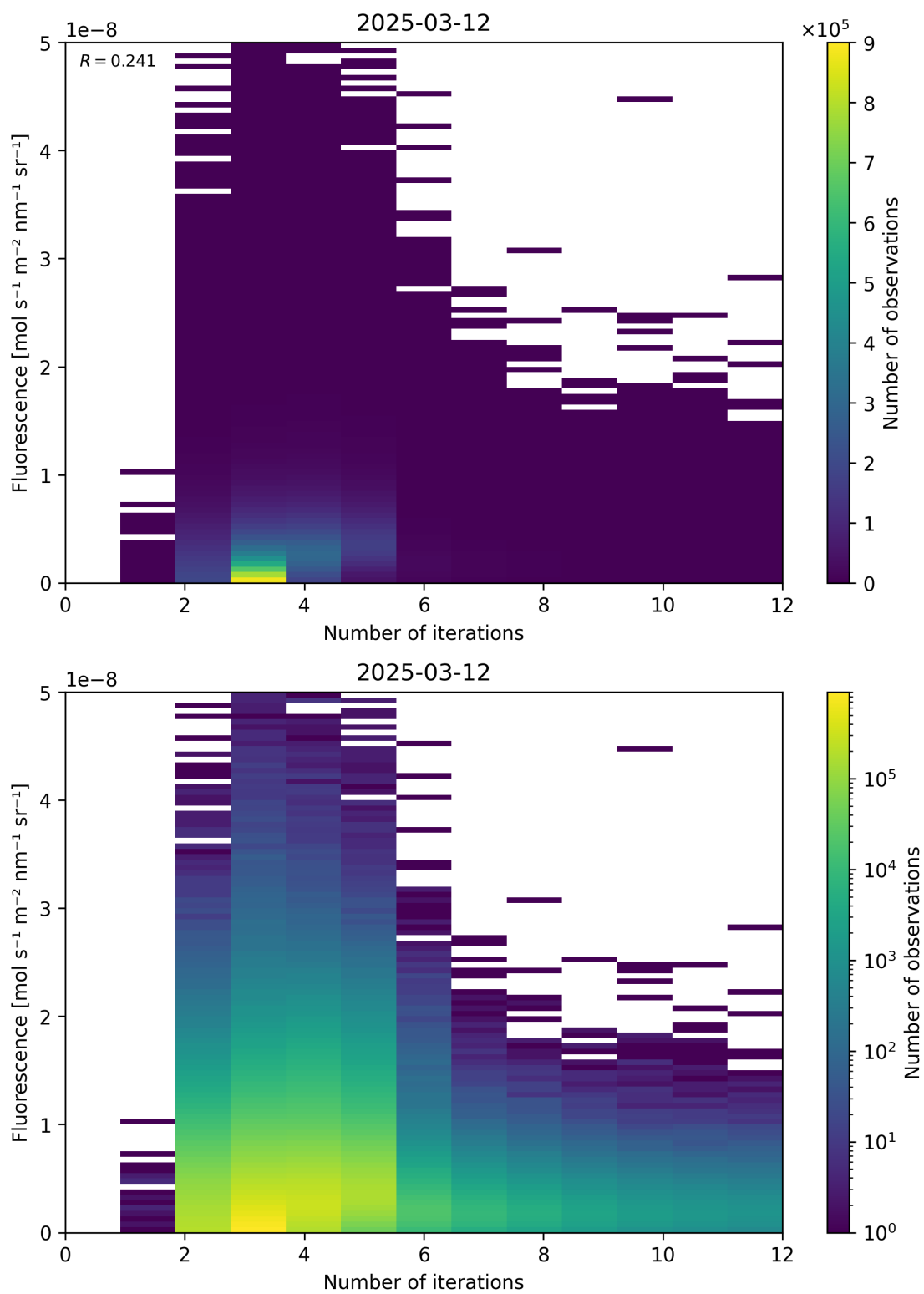
Figure 98: Scatter density plot of “Number of iterations” against “Fluorescence” for 2025-03-12 to 2025-03-13.
