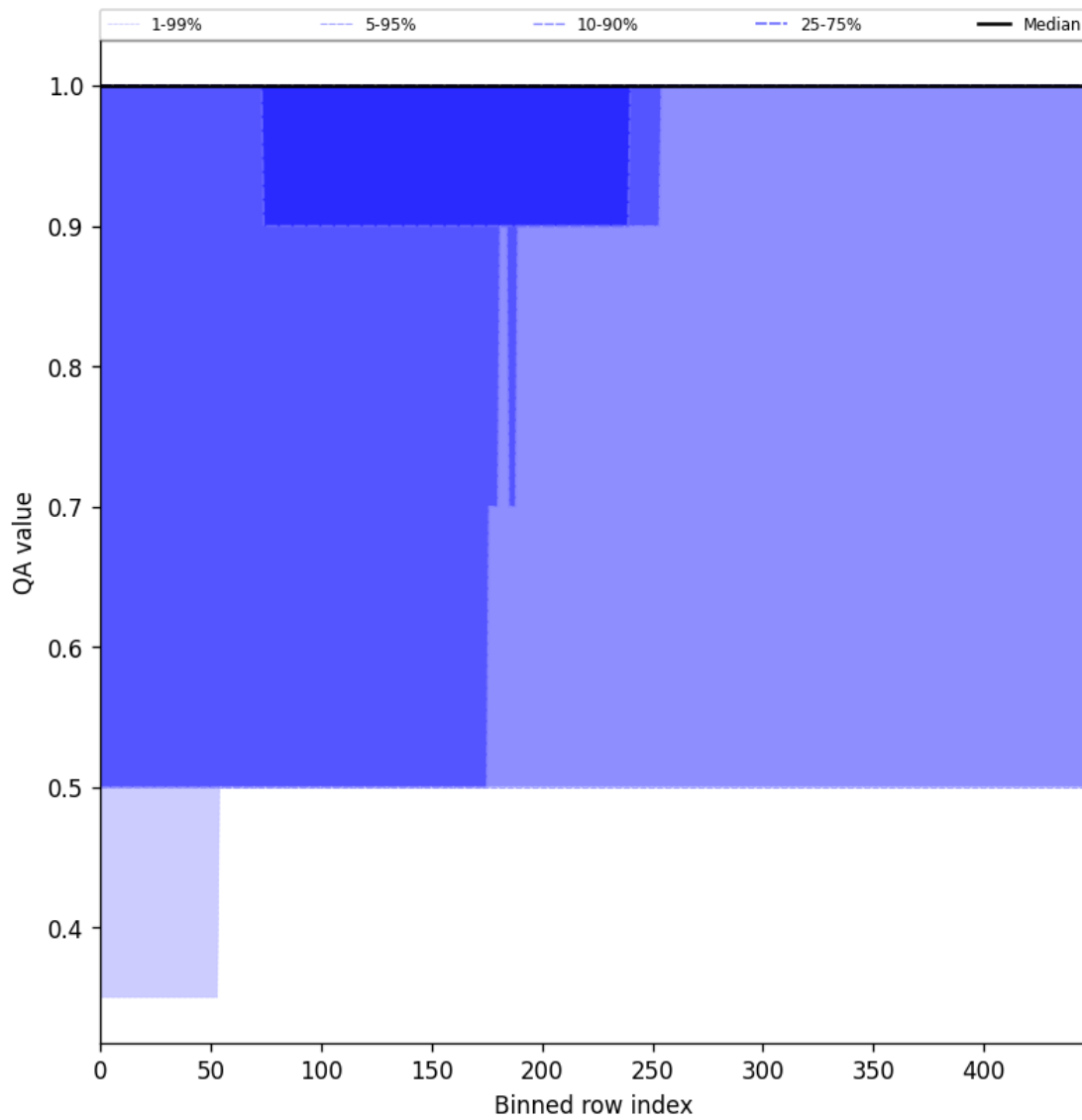
Figure 46: Along track statistics of “QA value” for 2025-03-12 to 2025-03-13
