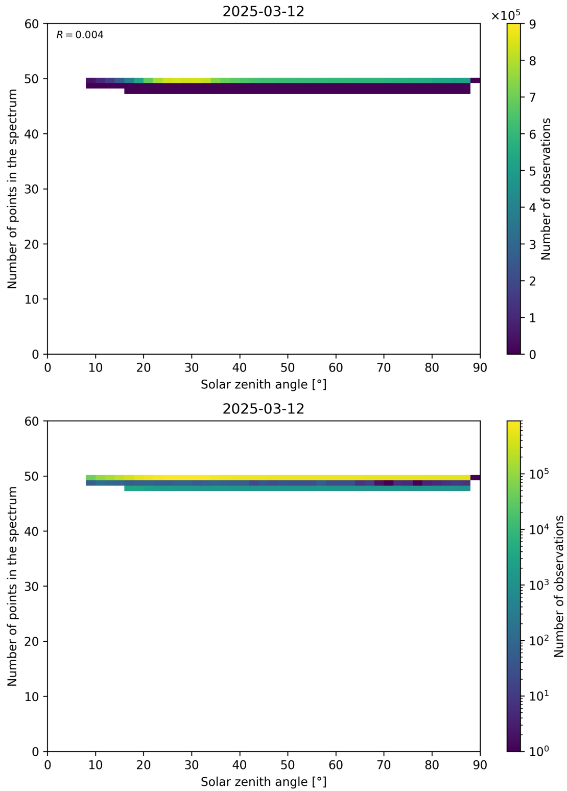
Figure 115: Scatter density plot of “Solar zenith angle” against “Number of points in the spectrum” for 2025-03-12 to 2025-03-13.
