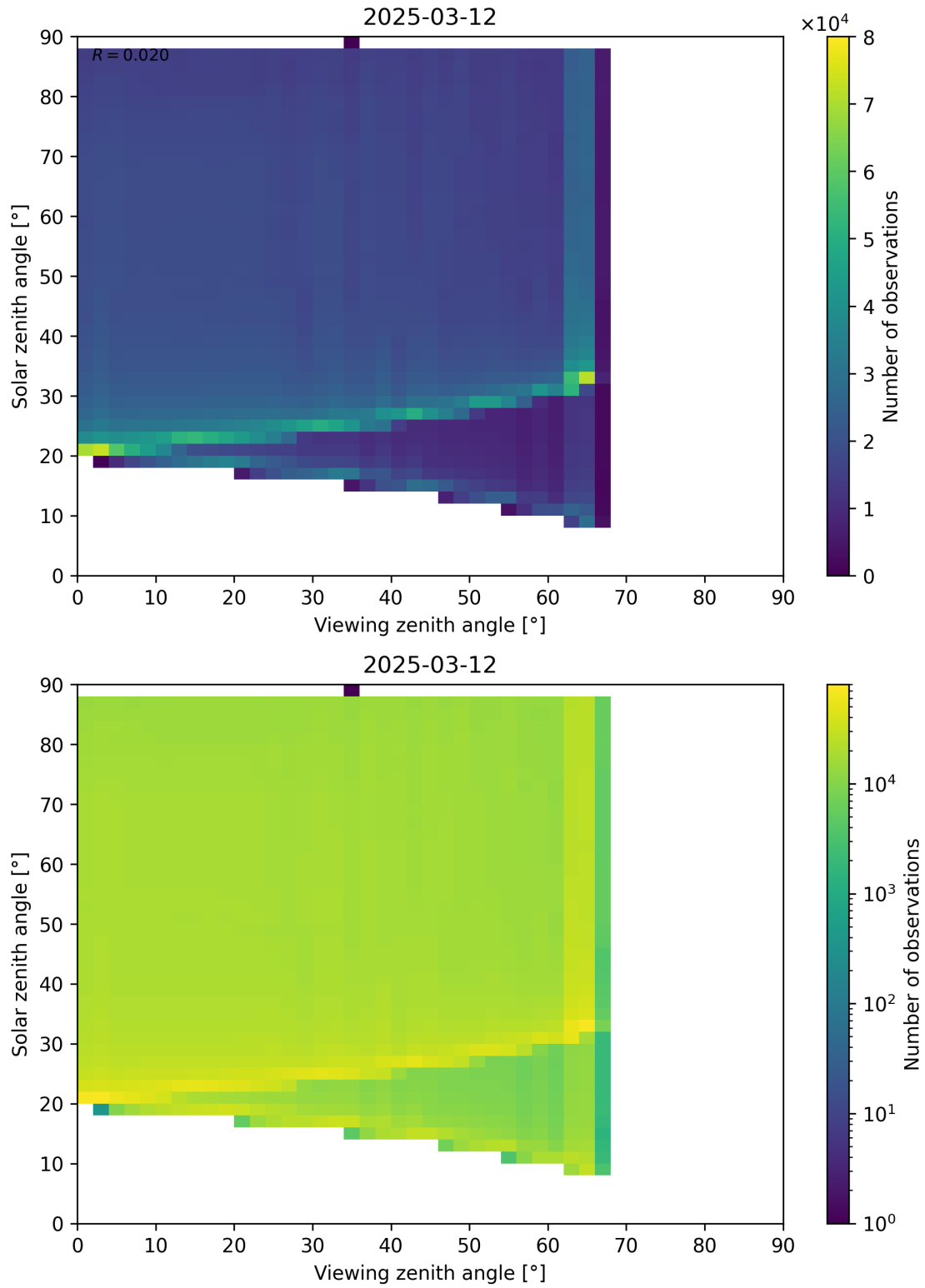
Figure 127: Scatter density plot of “Viewing zenith angle” against “Solar zenith angle” for 2025-03-12 to 2025-03-13.
