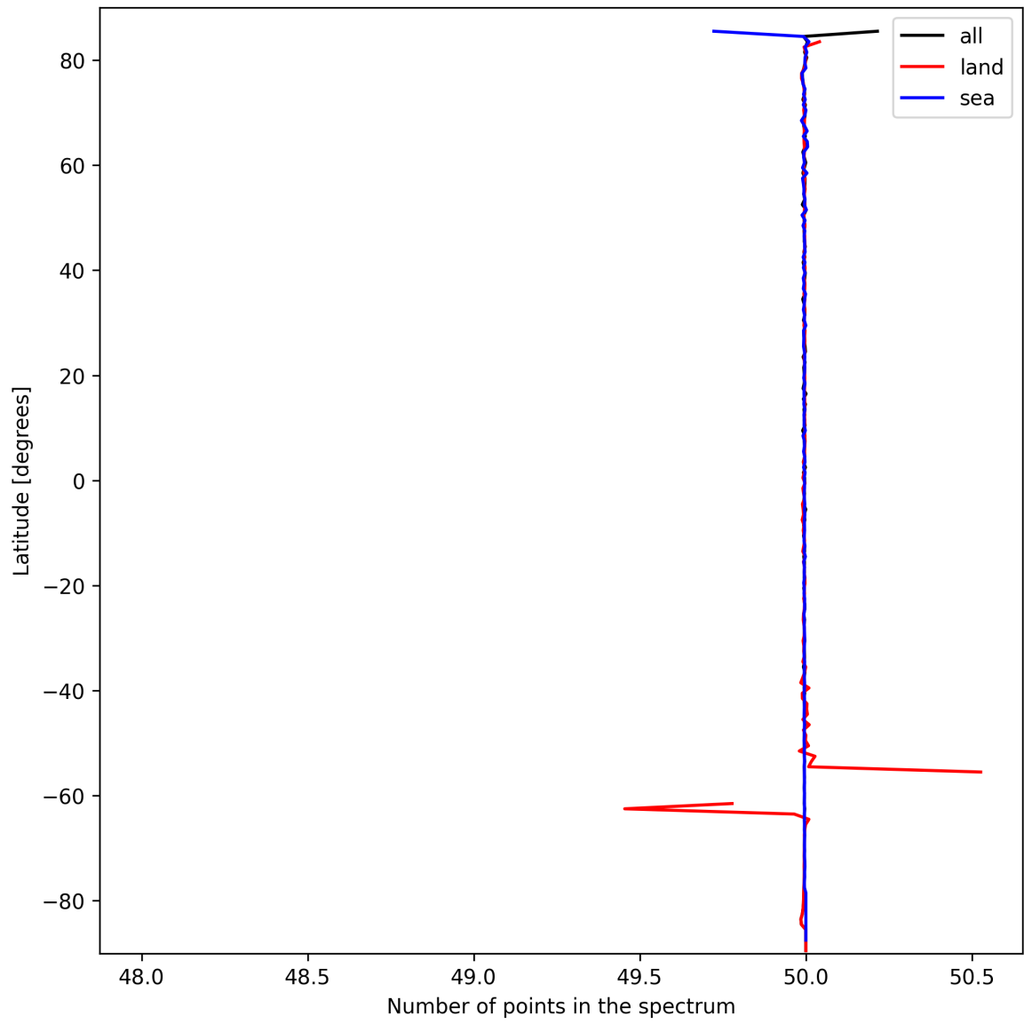
Figure 27: Zonal average of “Number of points in the spectrum” for 2025-03-12 to 2025-03-13.
