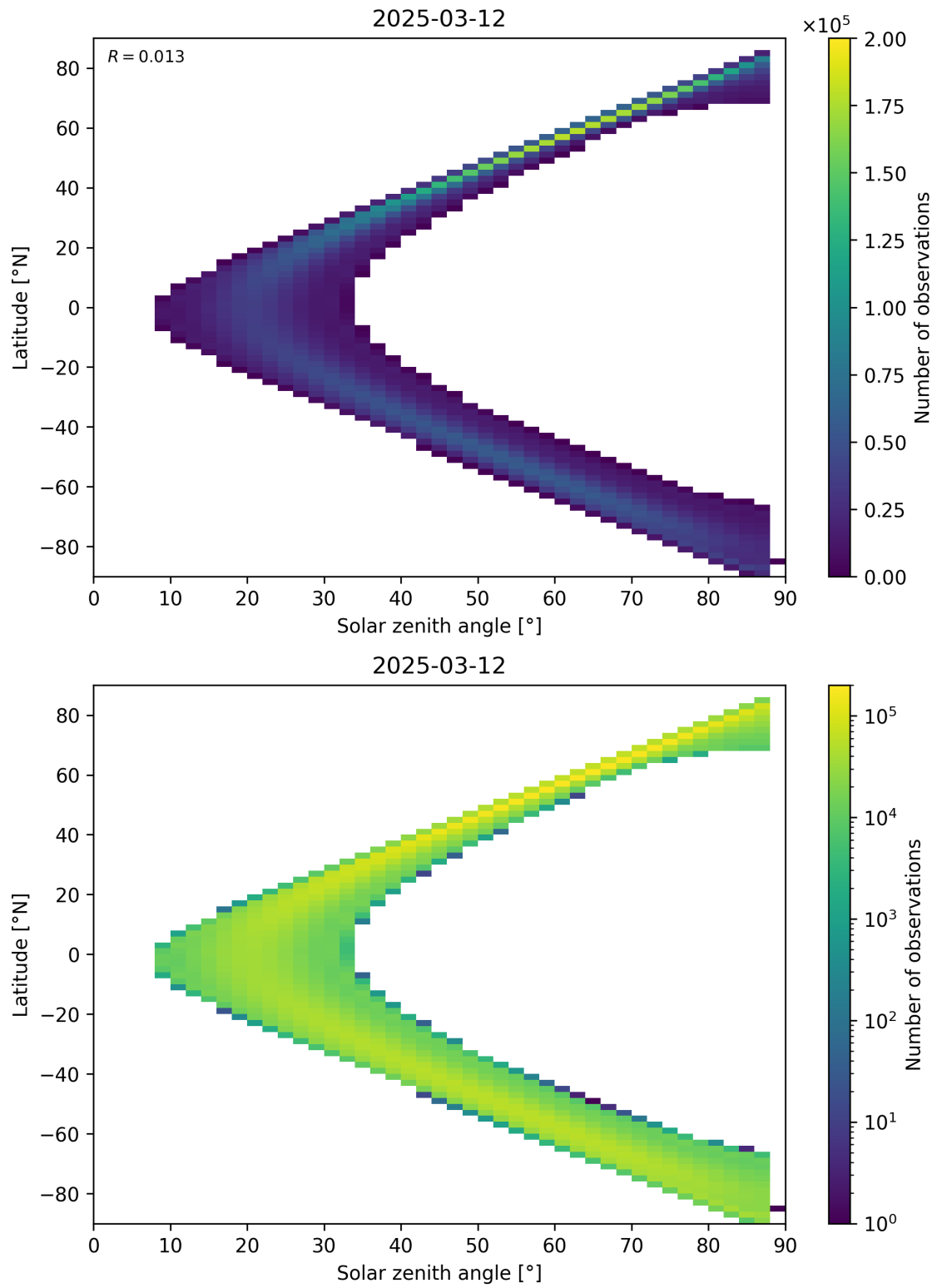
Figure 113: Scatter density plot of “Solar zenith angle” against “Latitude” for 2025-03-12 to 2025-03-13.
