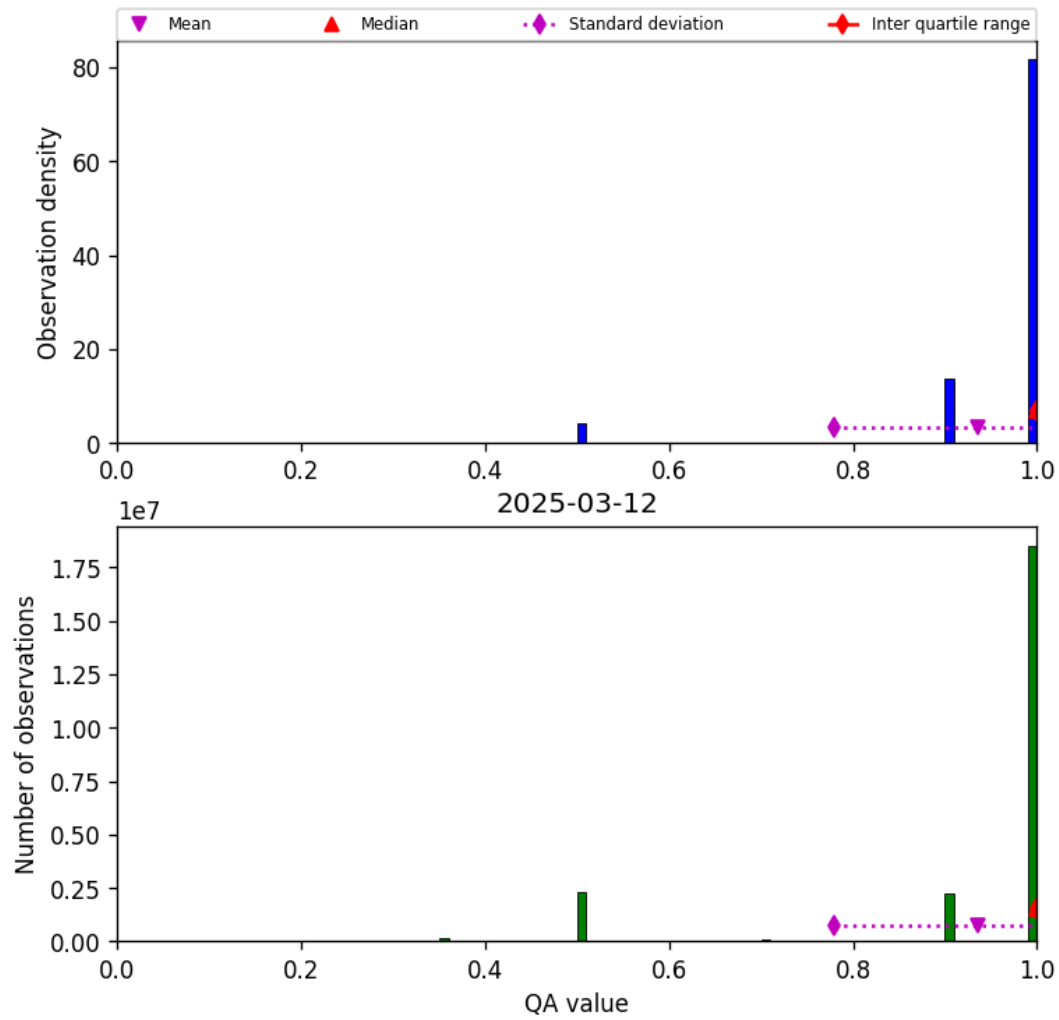
Figure 29: Histogram of “QA value” for 2025-03-12 to 2025-03-13
