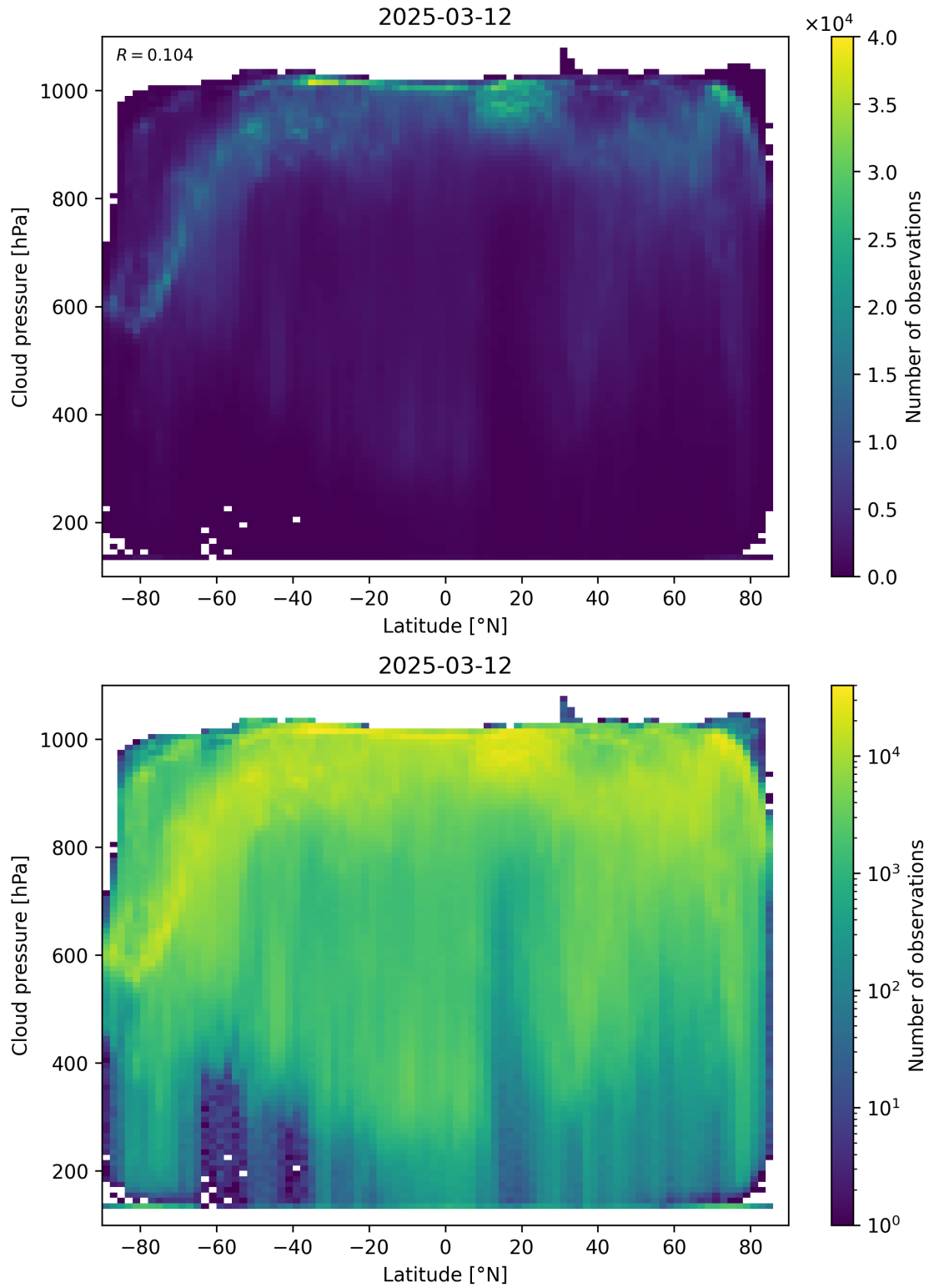
Figure 91: Scatter density plot of “Latitude” against “Cloud pressure” for 2025-03-12 to 2025-03-13.
