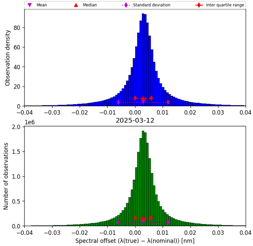
Figure 45: Histogram of “Spectral offset ( \lambda_{\text{true}} - \lambda_{\text{nominal}} )” for 2025-03-12 to 2025-03-13
