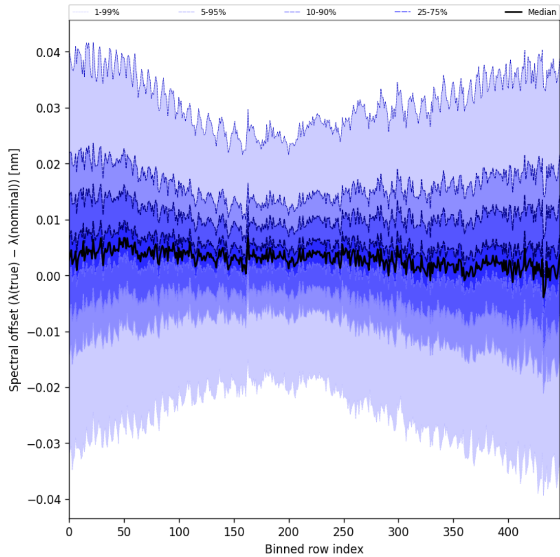
Figure 62: Along track statistics of “Spectral offset ( \lambda_{\text{true}} - \lambda_{\text{nominal}} )” for 2025-03-12 to 2025-03-13
