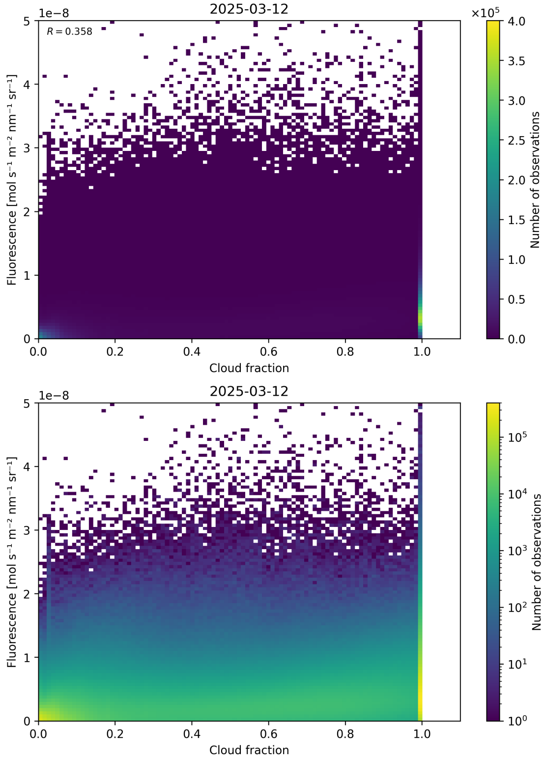
Figure 72: Scatter density plot of “Cloud fraction” against “Fluorescence” for 2025-03-12 to 2025-03-13.
