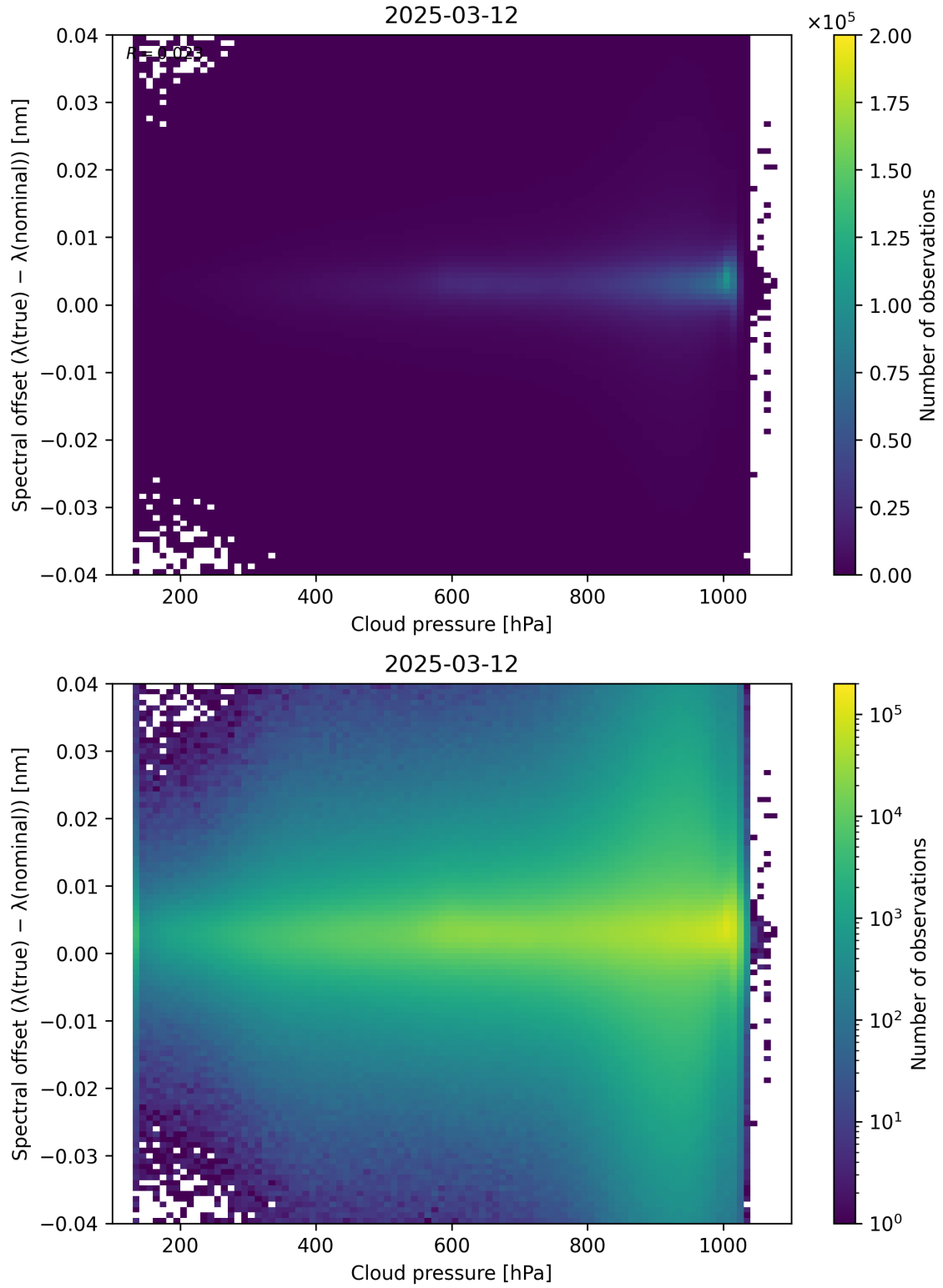
Figure 84: Scatter density plot of “Cloud pressure” against “Spectral offset ( \lambda_{\text{true}} - \lambda_{\text{nominal}} )” for 2025-03-12 to 2025-03-13.
