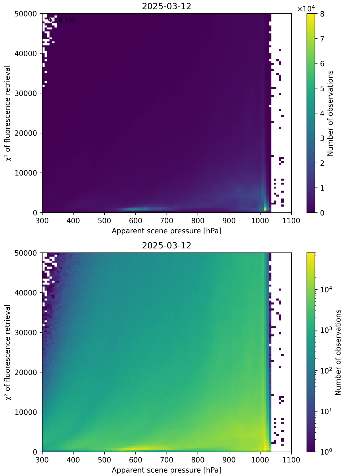
Figure 63: Scatter density plot of “Apparent scene pressure” against “ \chi^2 of fluorescence retrieval” for 2025-03-12 to 2025-03-13.
