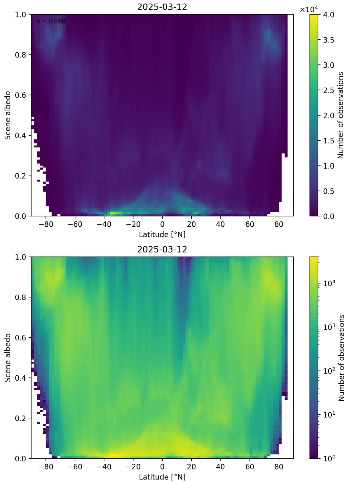
Figure 95: Scatter density plot of “Latitude” against “Scene albedo” for 2025-03-12 to 2025-03-13.
