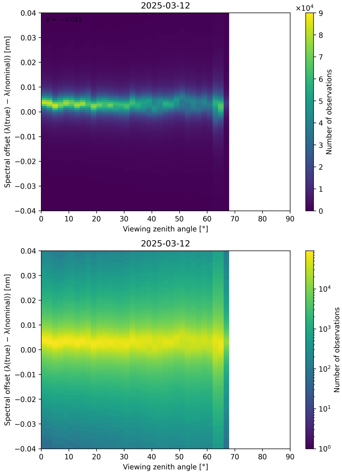
Figure 128: Scatter density plot of “Viewing zenith angle” against “Spectral offset ( \lambda_{\text{true}} - \lambda_{\text{nominal}} )” for 2025-03-12 to 2025-03-13.
