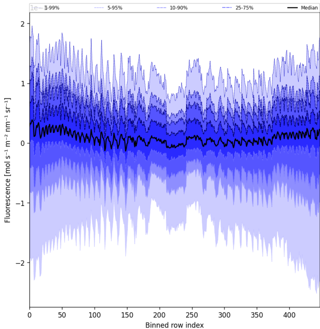
Figure 57: Along track statistics of “Fluorescence” for 2025-03-12 to 2025-03-13
