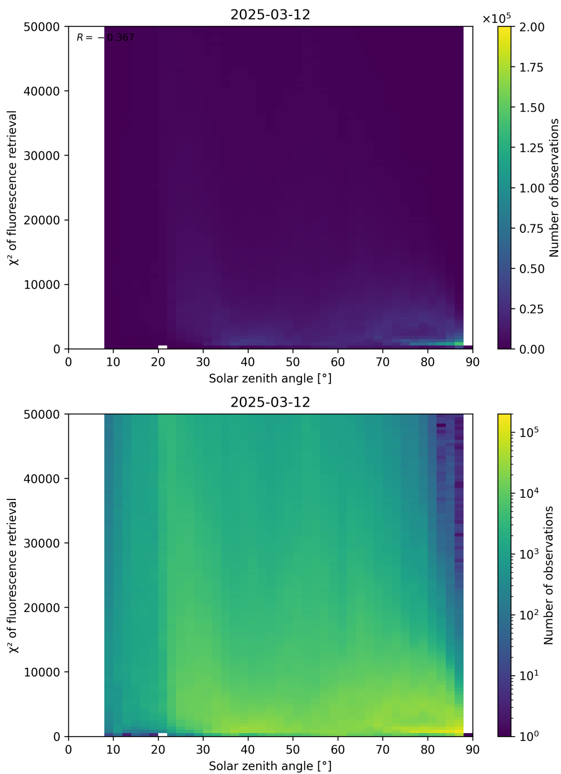
Figure 109: Scatter density plot of “Solar zenith angle” against “ \chi^2 of fluorescence retrieval” for 2025-03-12 to 2025-03-13.
