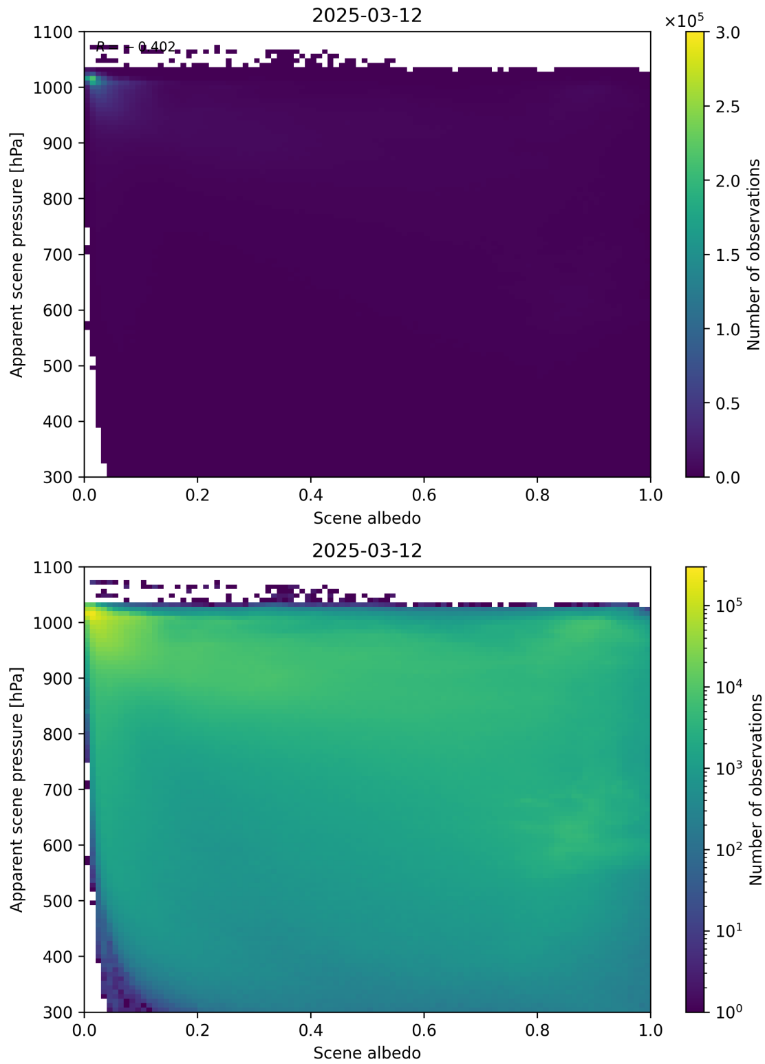
Figure 102: Scatter density plot of “Scene albedo” against “Apparent scene pressure” for 2025-03-12 to 2025-03-13.
