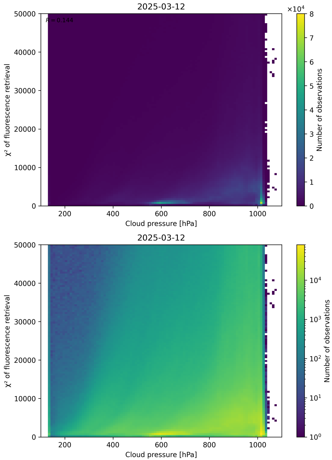
Figure 78: Scatter density plot of “Cloud pressure” against “ \chi^2 of fluorescence retrieval” for 2025-03-12 to 2025-03-13.
