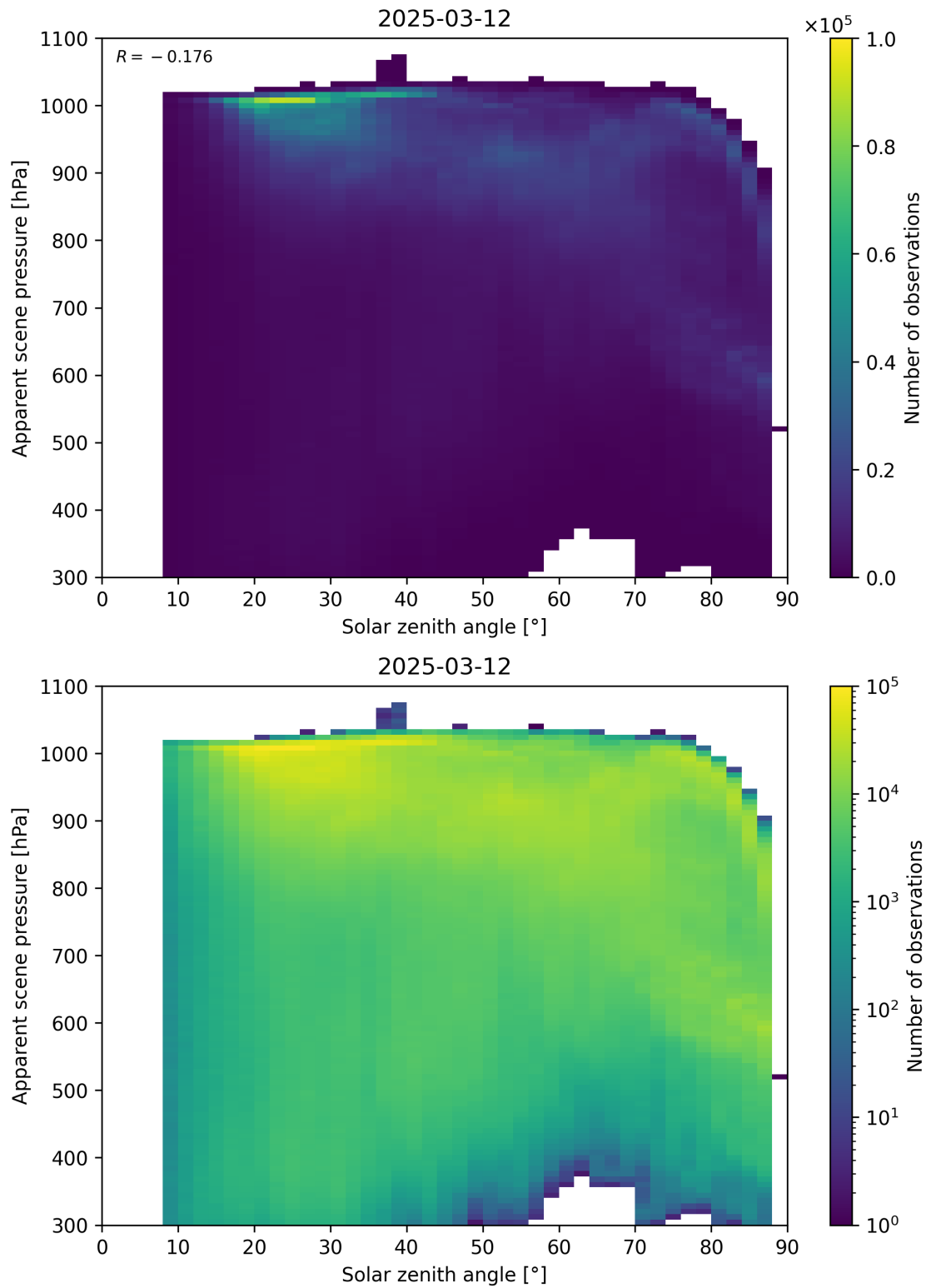
Figure 108: Scatter density plot of “Solar zenith angle” against “Apparent scene pressure” for 2025-03-12 to 2025-03-13.
