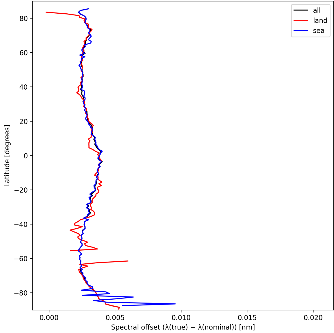
Figure 28: Zonal average of “Spectral offset ( \lambda_{\text{true}} - \lambda_{\text{nominal}} )” for 2025-03-12 to 2025-03-13.
