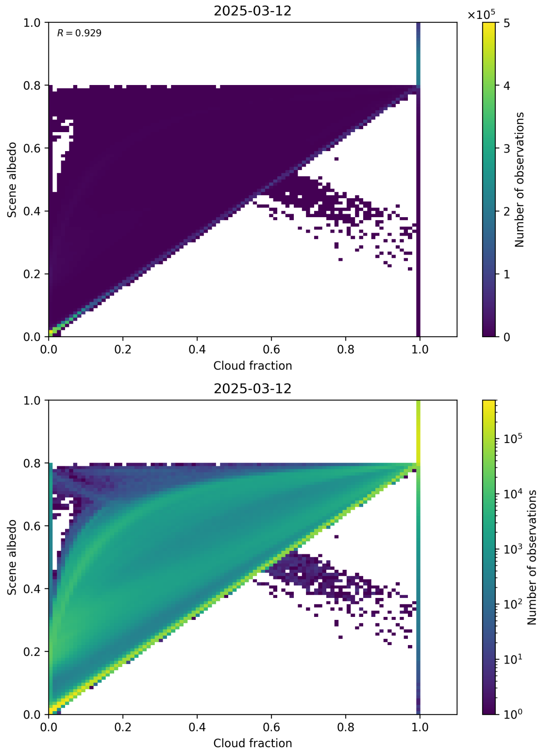
Figure 75: Scatter density plot of “Cloud fraction” against “Scene albedo” for 2025-03-12 to 2025-03-13.
