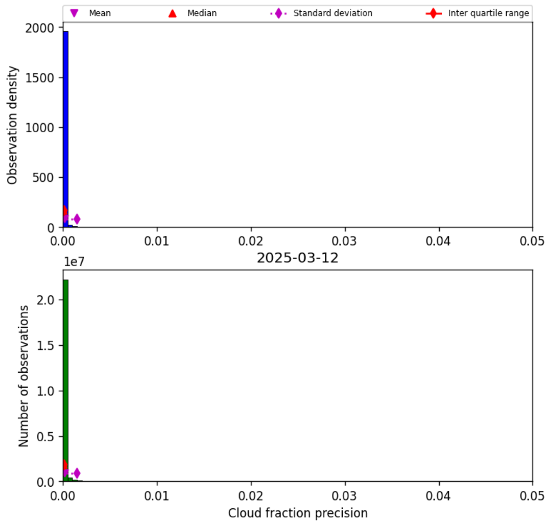
Figure 33: Histogram of “Cloud fraction precision” for 2025-03-12 to 2025-03-13
