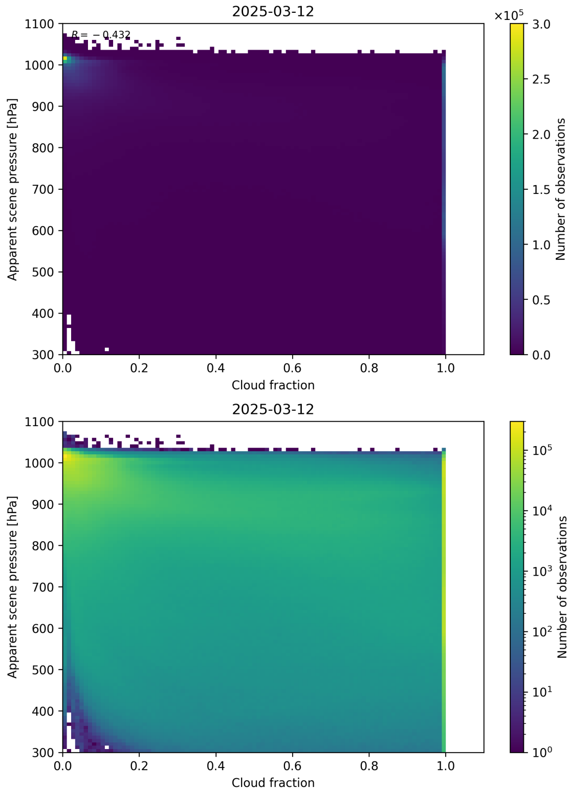
Figure 70: Scatter density plot of “Cloud fraction” against “Apparent scene pressure” for 2025-03-12 to 2025-03-13.
