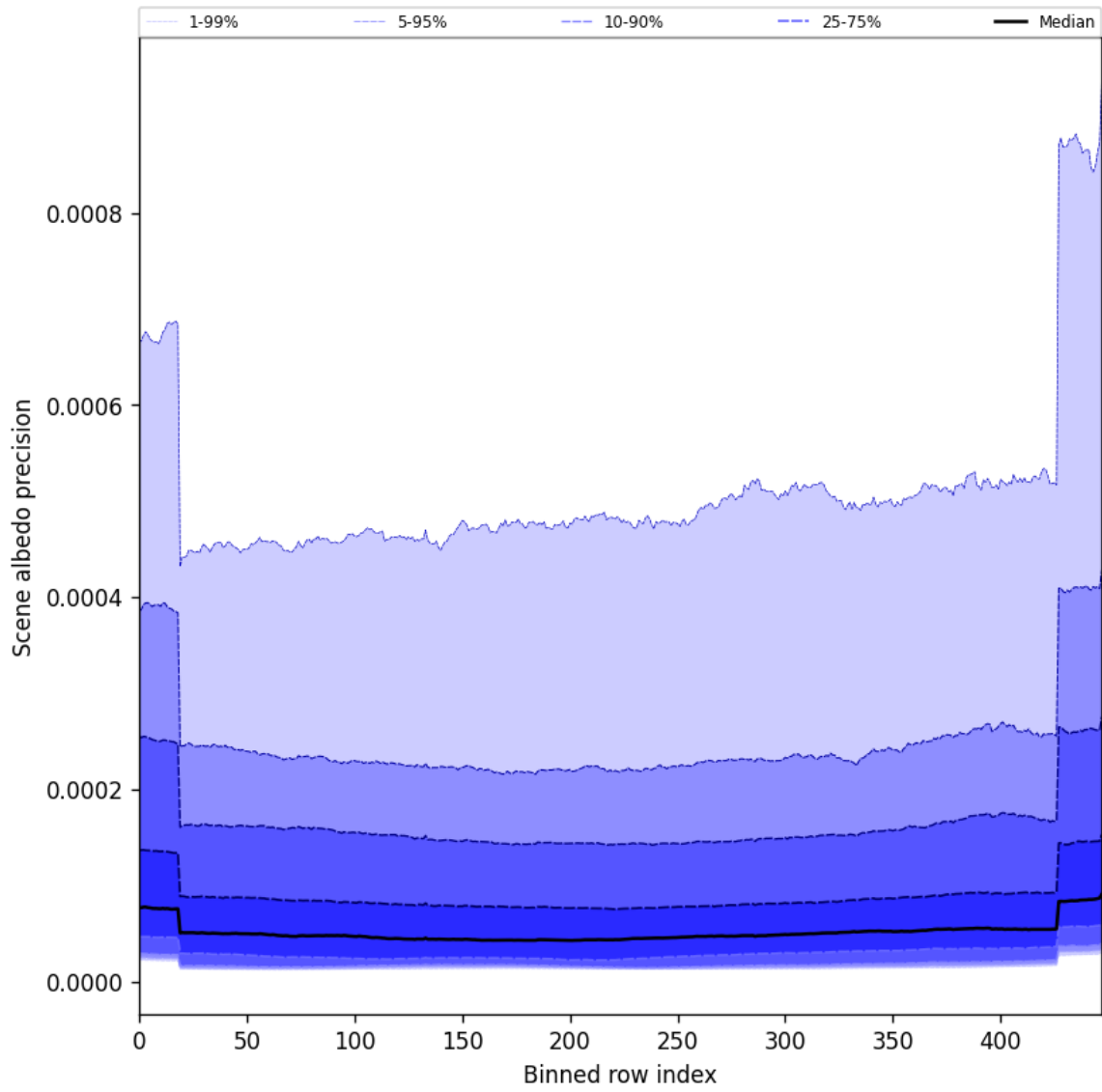
Figure 52: Along track statistics of “Scene albedo precision” for 2025-03-12 to 2025-03-13
