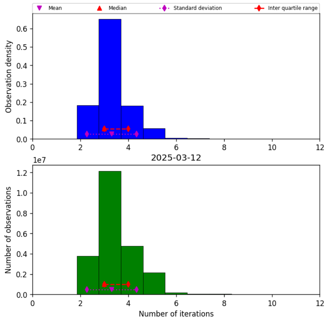
Figure 39: Histogram of “Number of iterations” for 2025-03-12 to 2025-03-13
