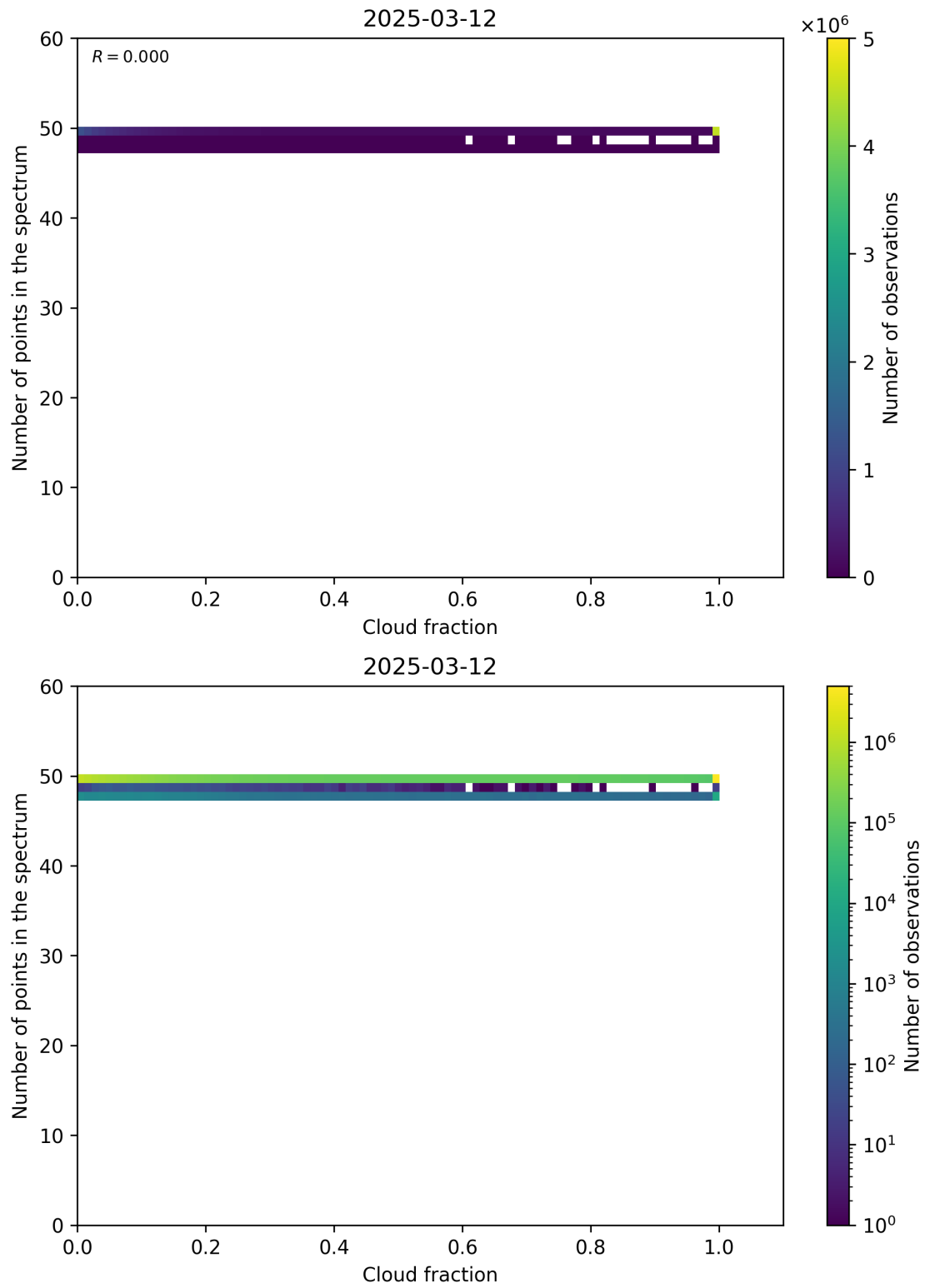
Figure 74: Scatter density plot of “Cloud fraction” against “Number of points in the spectrum” for 2025-03-12 to 2025-03-13.
