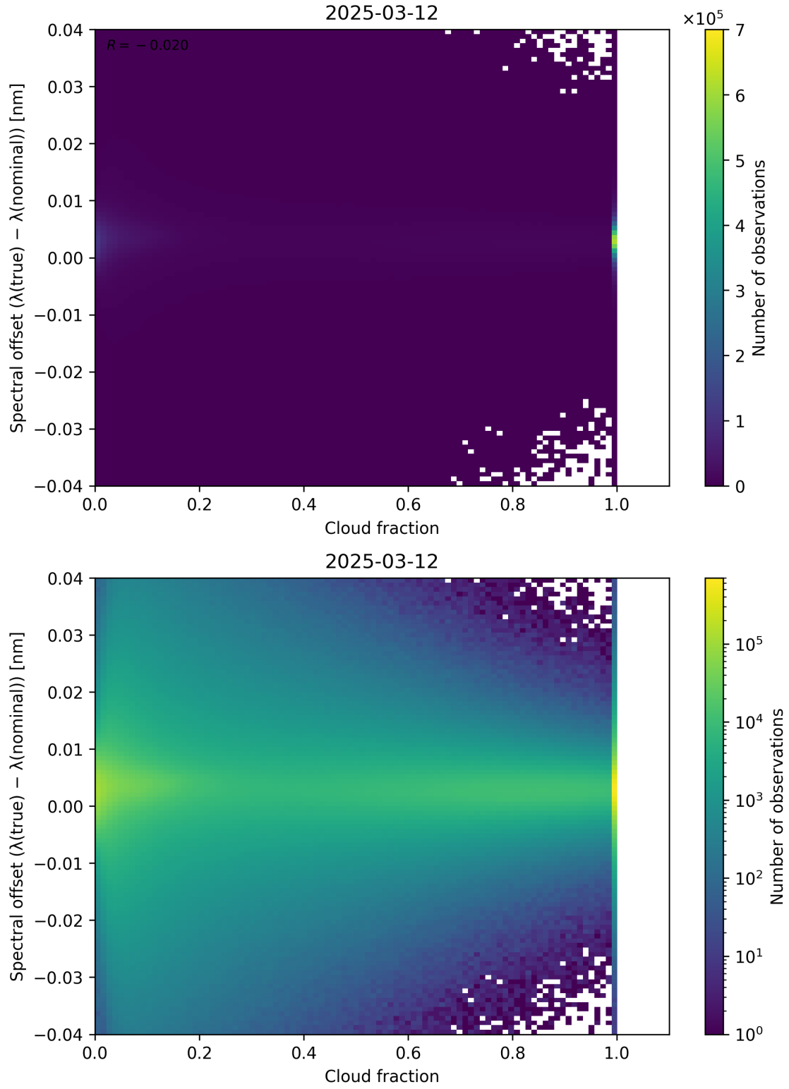
Figure 76: Scatter density plot of “Cloud fraction” against “Spectral offset ( \lambda_{\text{true}} - \lambda_{\text{nominal}} )” for 2025-03-12 to 2025-03-13.
