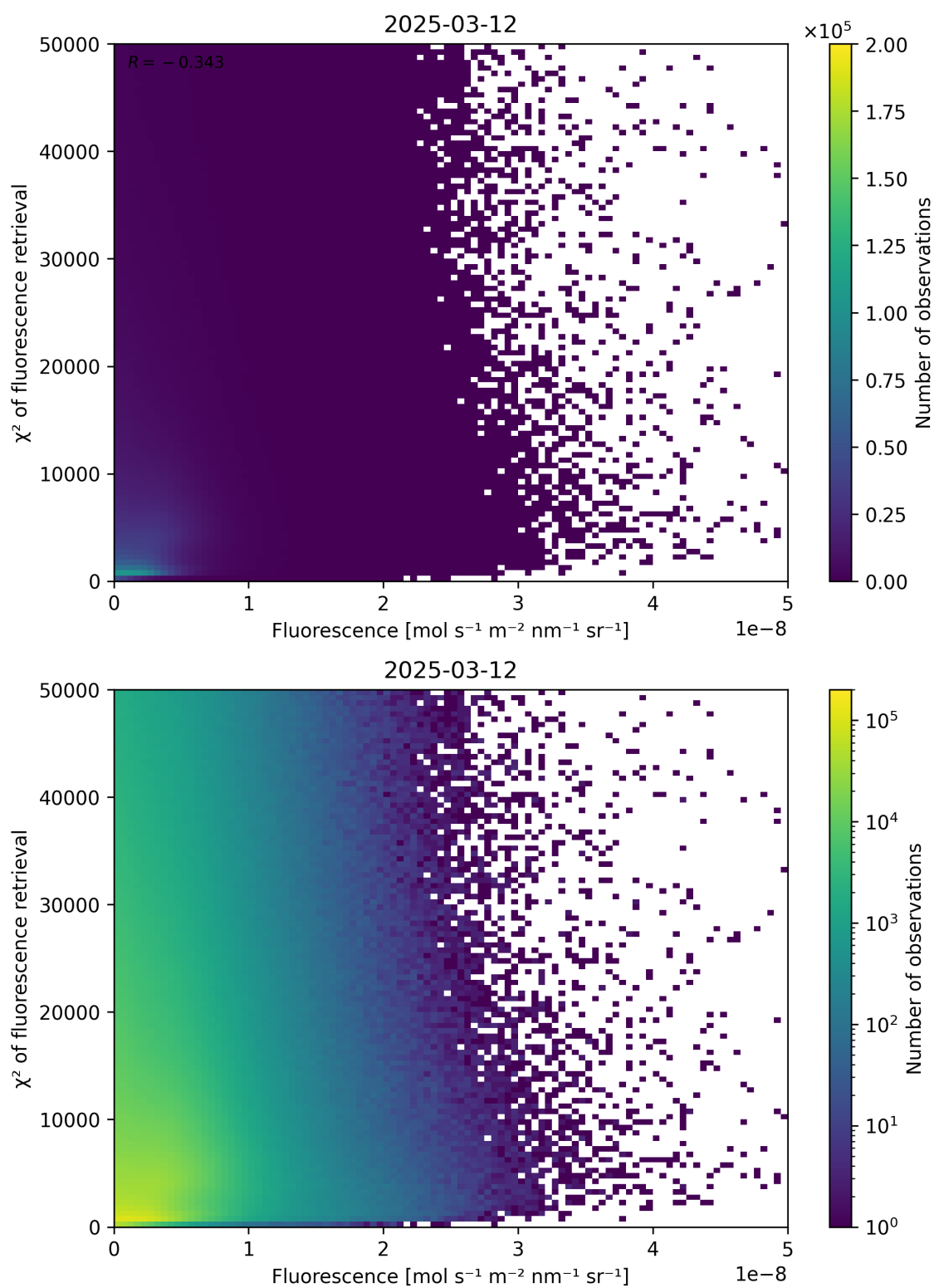
Figure 85: Scatter density plot of “Fluorescence” against “ \chi^2 of fluorescence retrieval” for 2025-03-12 to 2025-03-13.
