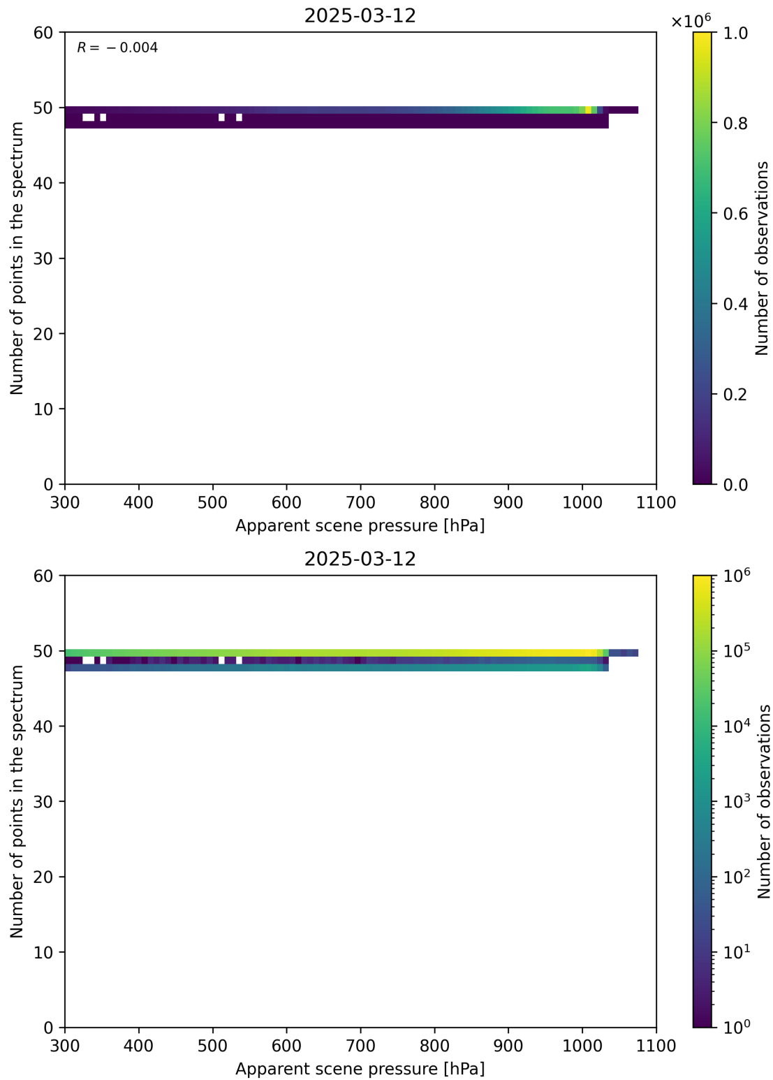
Figure 66: Scatter density plot of “Apparent scene pressure” against “Number of points in the spectrum” for 2025-03-12 to 2025-03-13.
