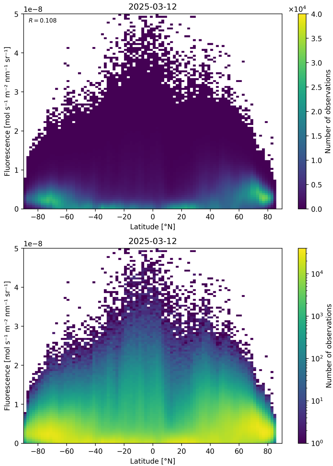
Figure 92: Scatter density plot of “Latitude” against “Fluorescence” for 2025-03-12 to 2025-03-13.
