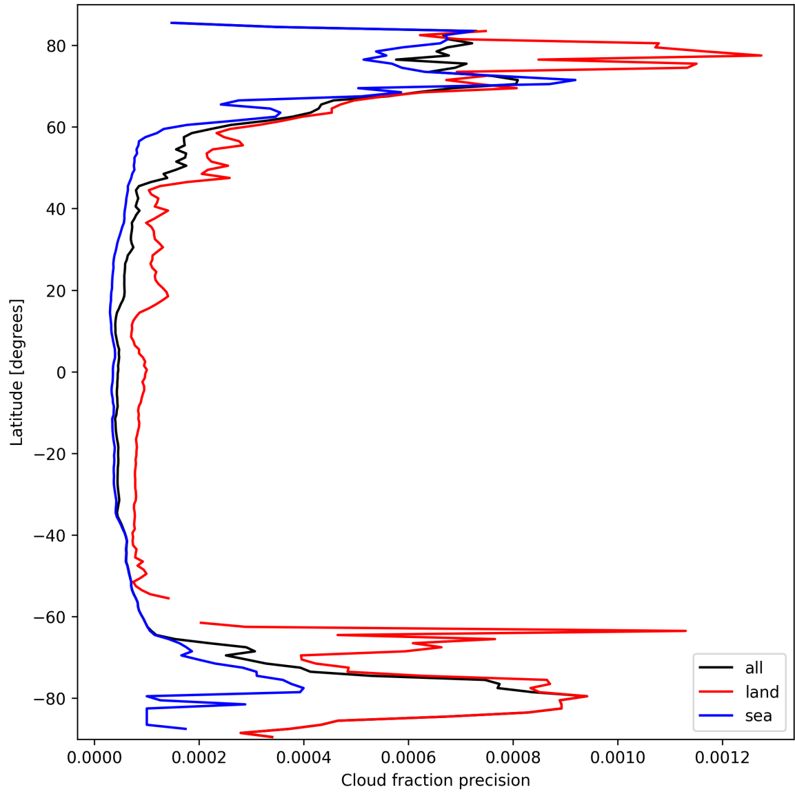
Figure 16: Zonal average of “Cloud fraction precision” for 2025-03-12 to 2025-03-13.
