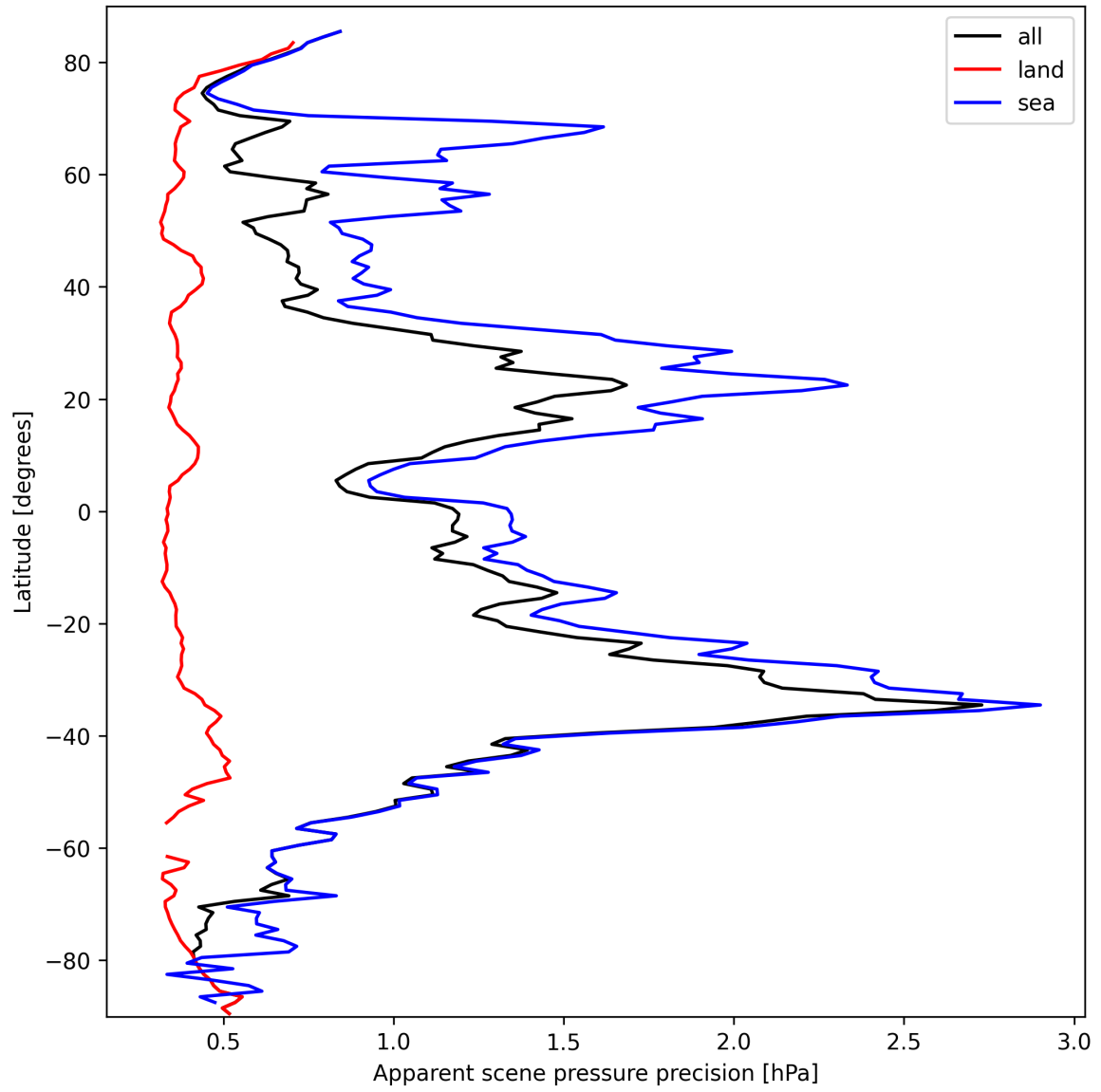
Figure 20: Zonal average of “Apparent scene pressure precision” for 2025-03-12 to 2025-03-13.
