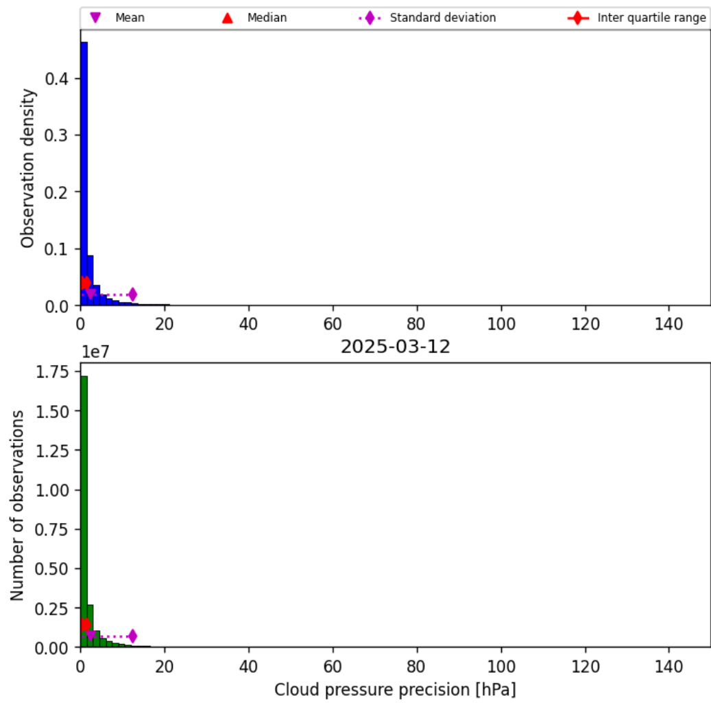
Figure 31: Histogram of "Cloud pressure precision" for 2025-03-12 to 2025-03-13
