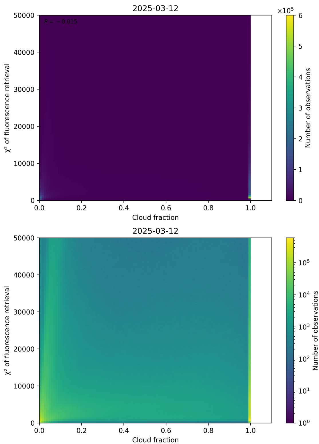
Figure 71: Scatter density plot of “Cloud fraction” against “ \chi^2 of fluorescence retrieval” for 2025-03-12 to 2025-03-13.
