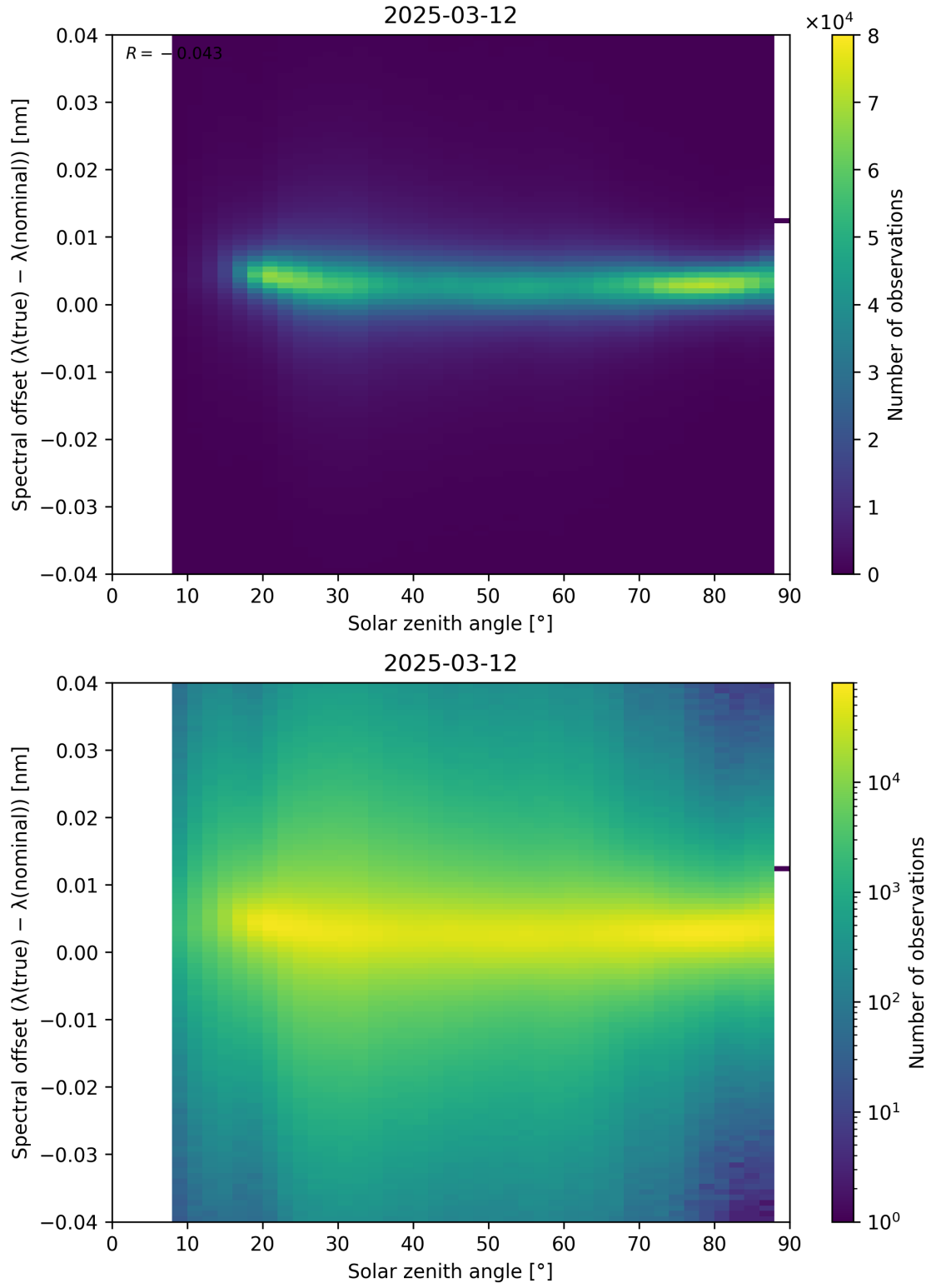
Figure 117: Scatter density plot of “Solar zenith angle” against “Spectral offset ( \lambda_{\text{true}} - \lambda_{\text{nominal}} )” for 2025-03-12 to 2025-03-13.
