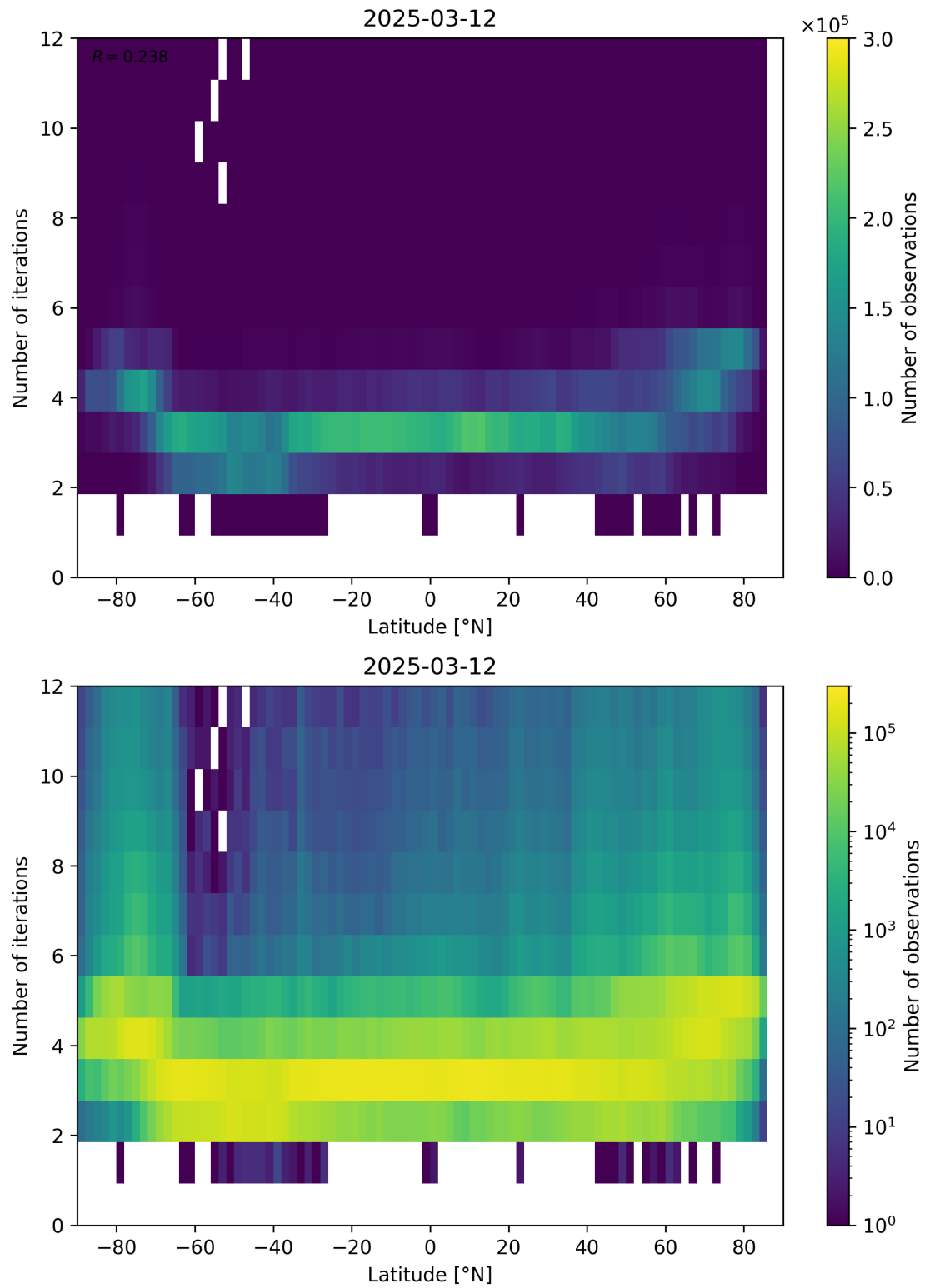
Figure 93: Scatter density plot of “Latitude” against “Number of iterations” for 2025-03-12 to 2025-03-13.
