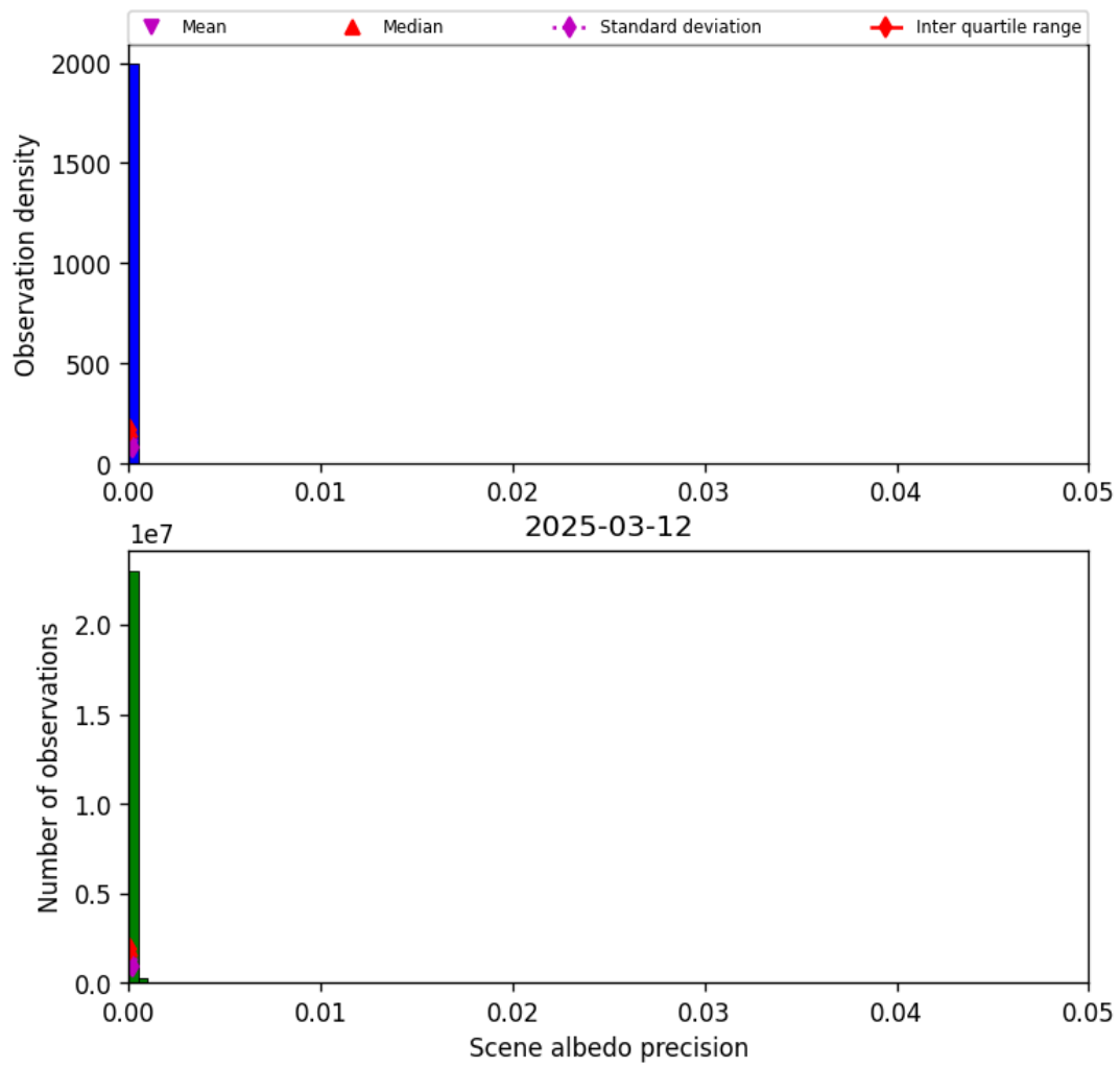
Figure 35: Histogram of “Scene albedo precision” for 2025-03-12 to 2025-03-13
