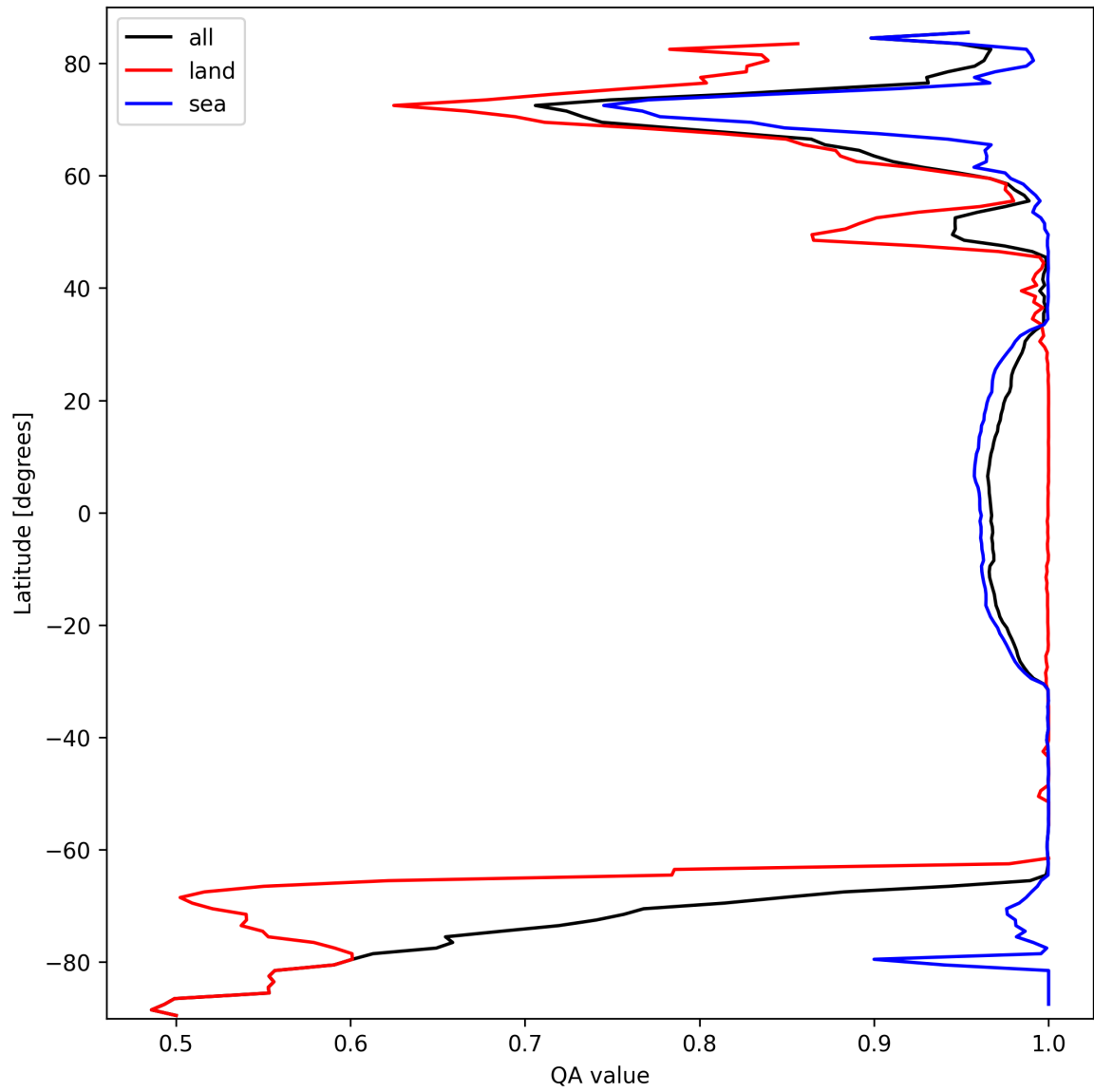
Figure 12: Zonal average of "QA value" for 2025-03-12 to 2025-03-13.
