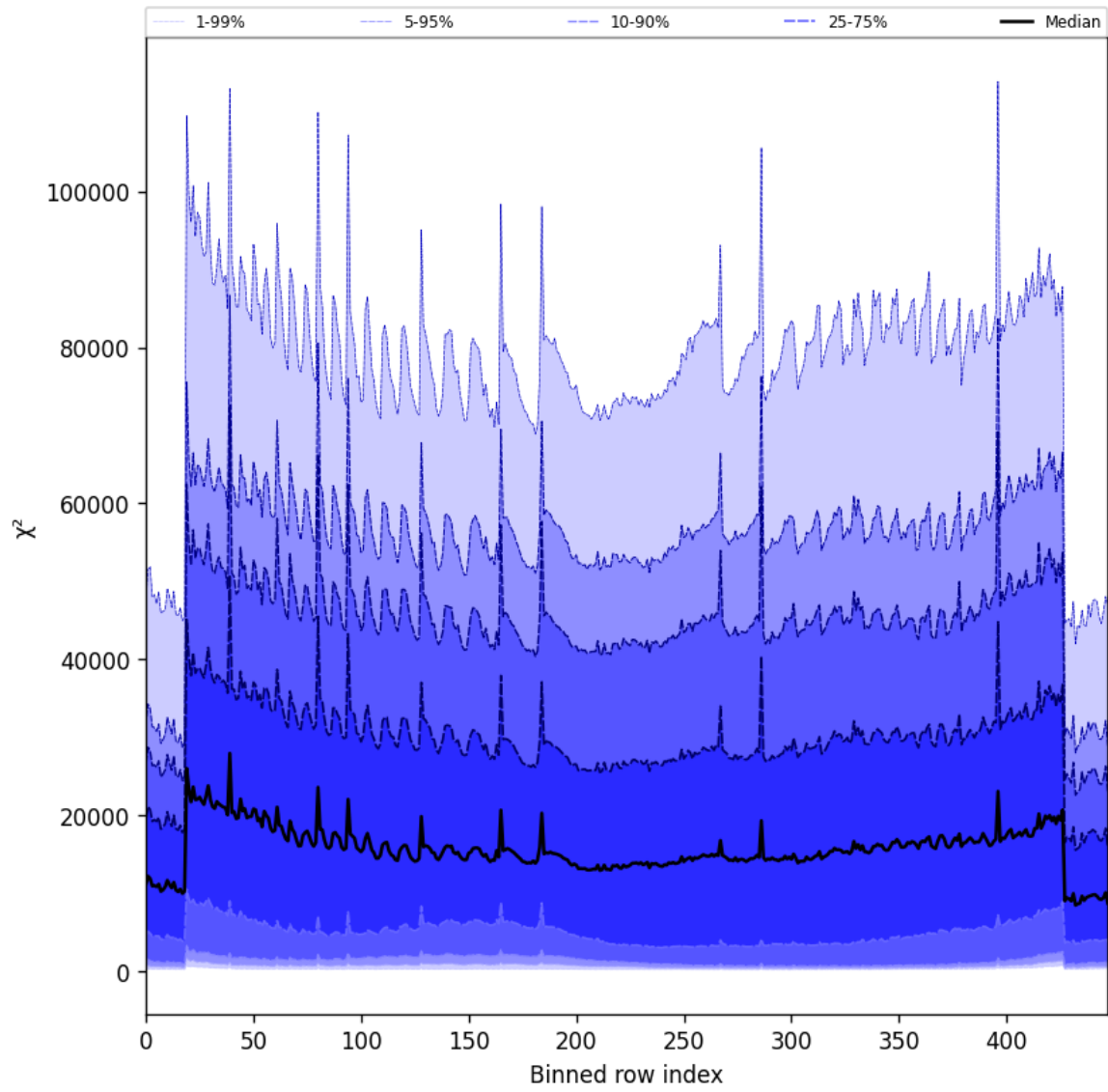
Figure 55: Along track statistics of “ \chi^2 ” for 2025-03-12 to 2025-03-13
