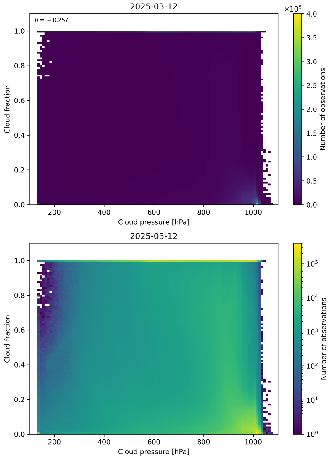
Figure 79: Scatter density plot of “Cloud pressure” against “Cloud fraction” for 2025-03-12 to 2025-03-13.
