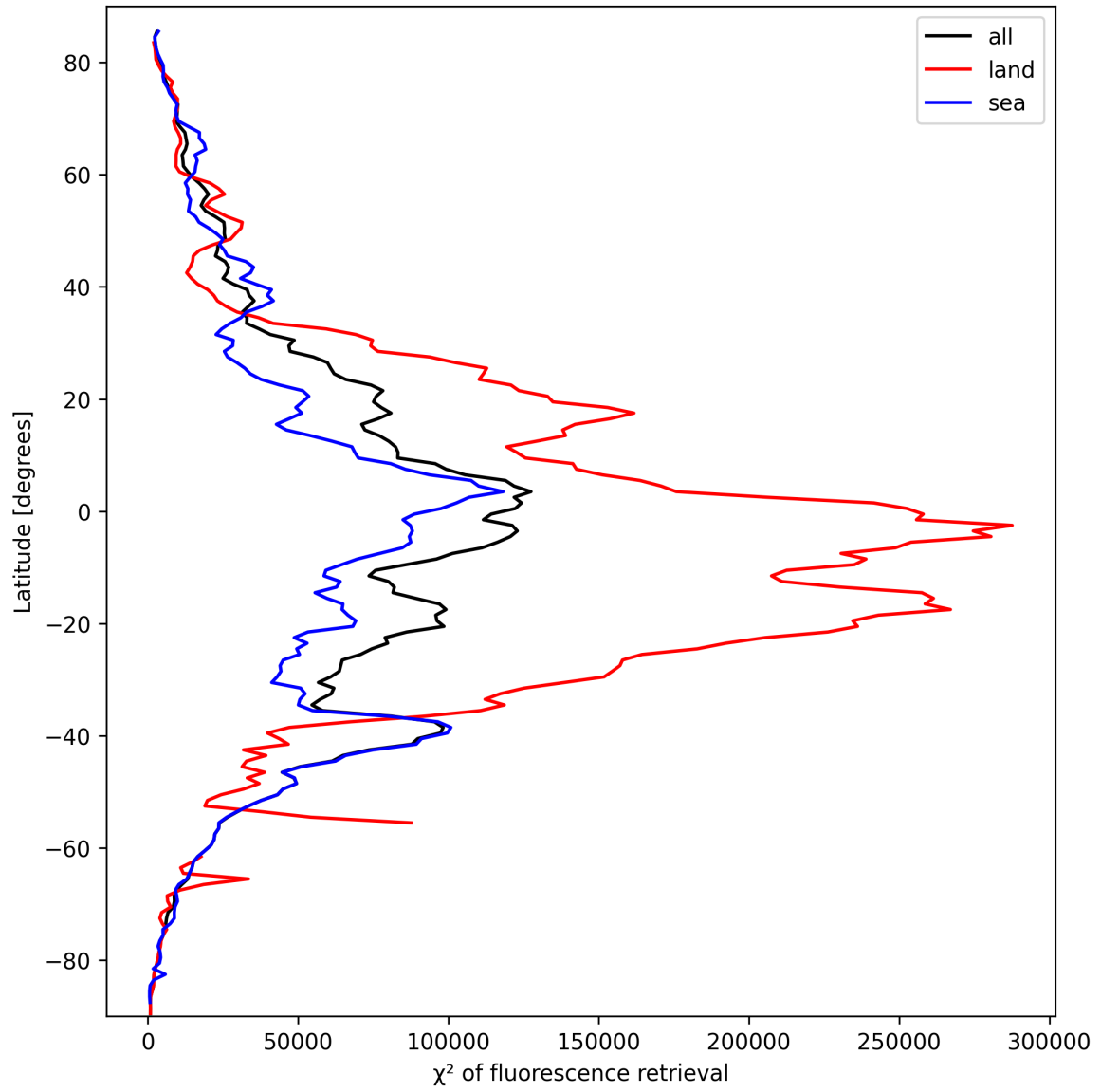
Figure 25: Zonal average of “ \chi^2 of fluorescence retrieval” for 2025-03-12 to 2025-03-13.
