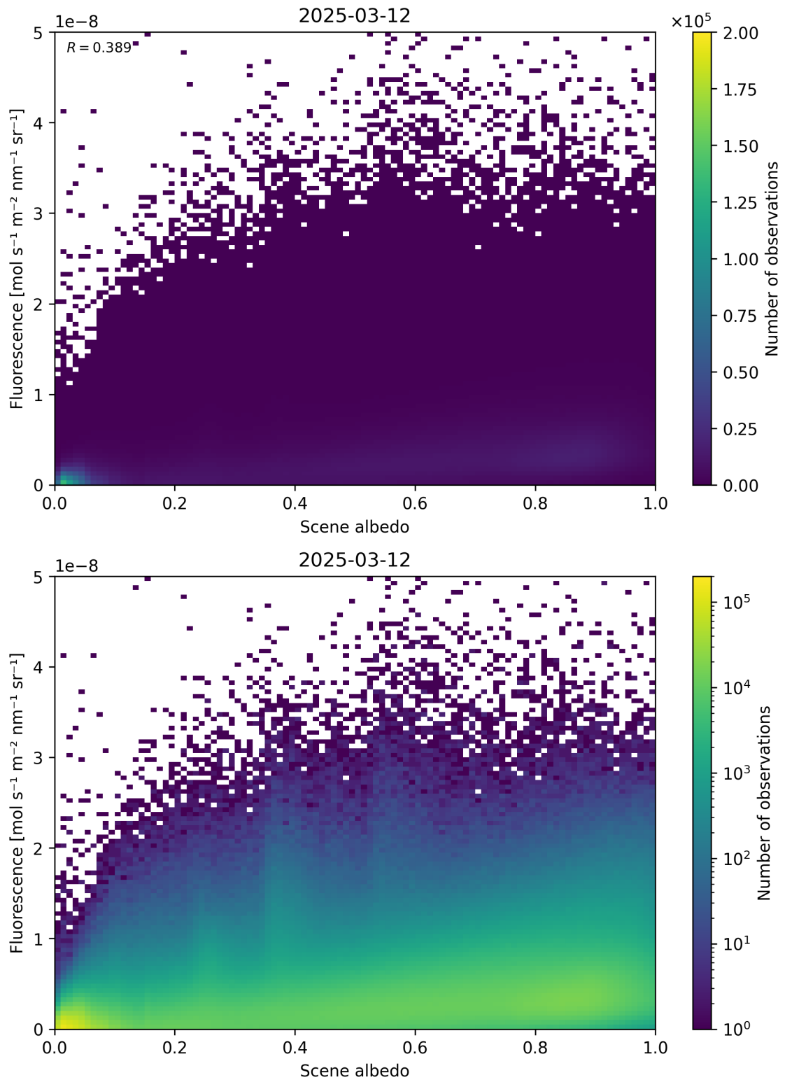
Figure 104: Scatter density plot of “Scene albedo” against “Fluorescence” for 2025-03-12 to 2025-03-13.
