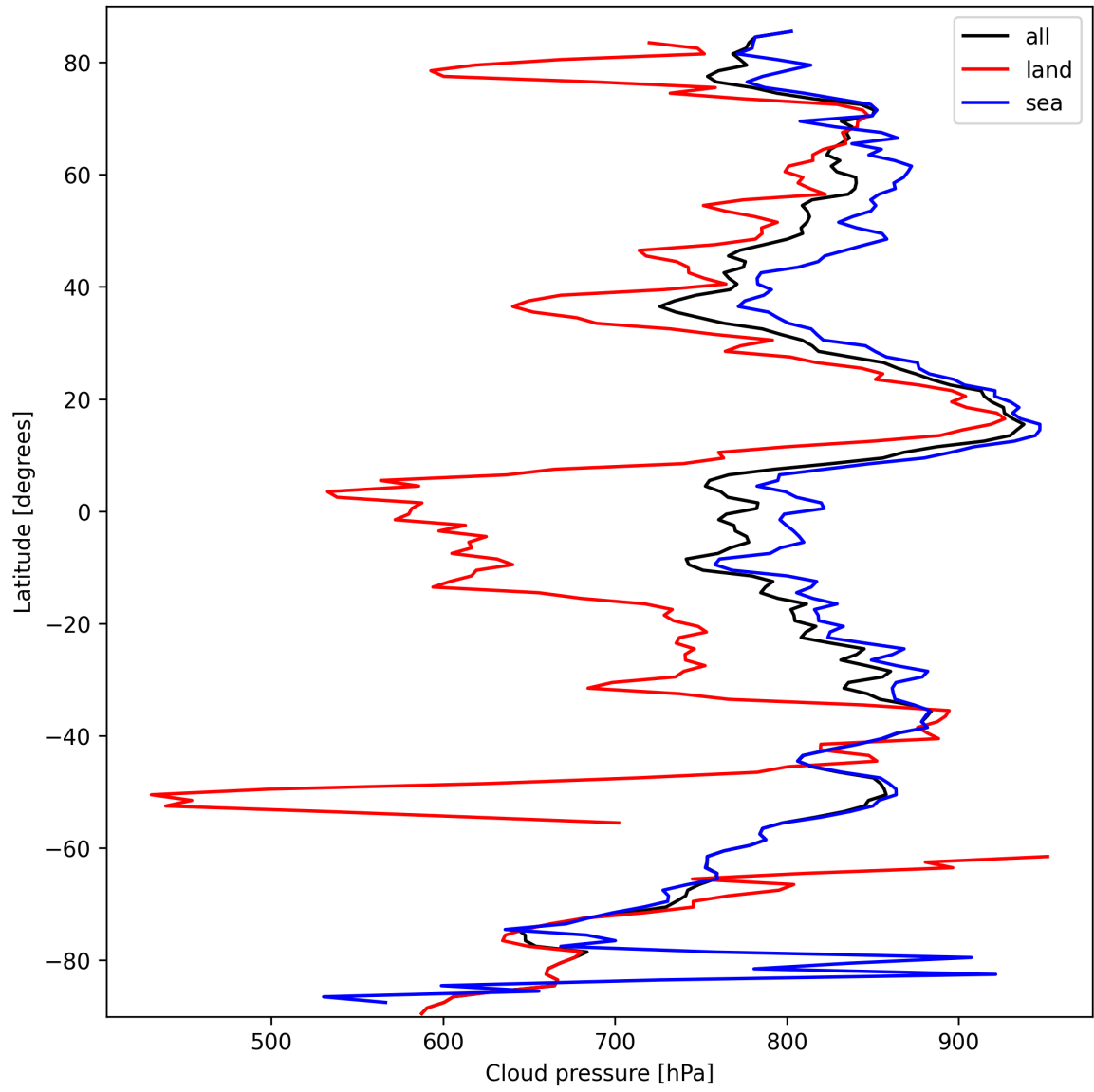
Figure 13: Zonal average of “Cloud pressure” for 2025-03-12 to 2025-03-13.
