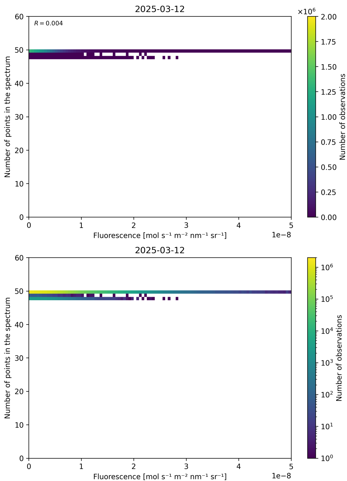
Figure 86: Scatter density plot of “Fluorescence” against “Number of points in the spectrum” for 2025-03-12 to 2025-03-13.
