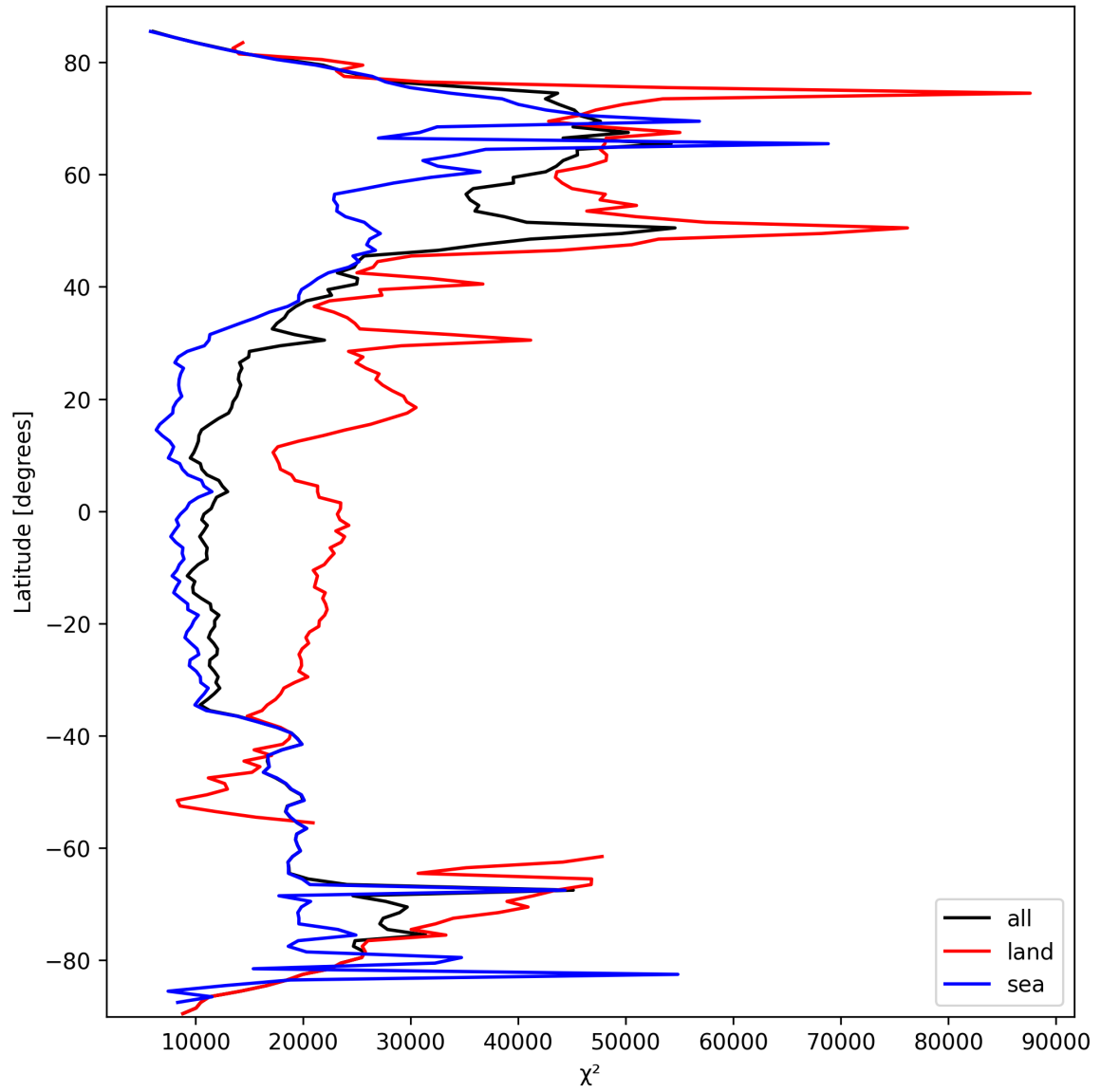
Figure 21: Zonal average of “ \chi^2 ” for 2025-03-12 to 2025-03-13.
