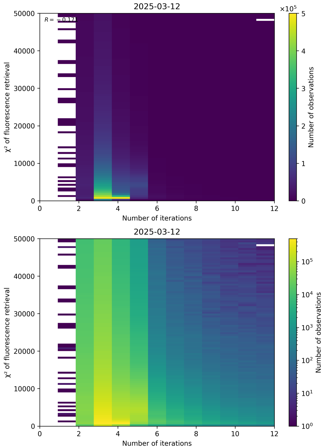
Figure 97: Scatter density plot of “Number of iterations” against “ \chi^2 of fluorescence retrieval” for 2025-03-12 to 2025-03-13.
