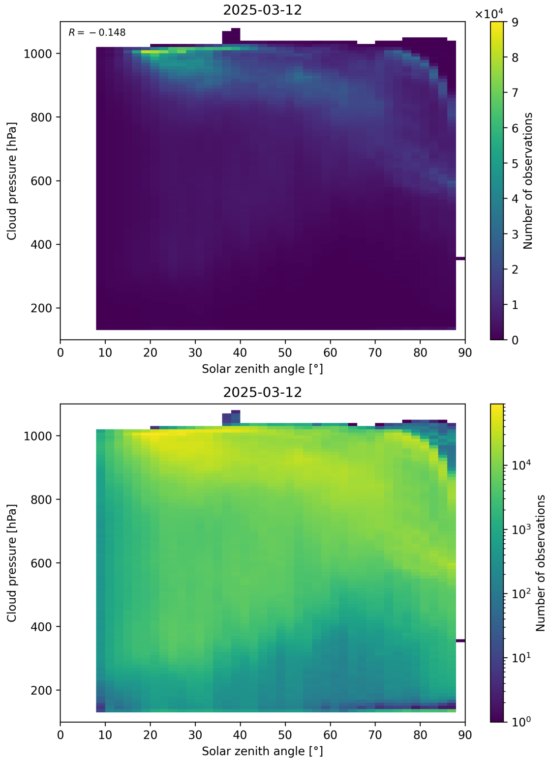
Figure 111: Scatter density plot of “Solar zenith angle” against “Cloud pressure” for 2025-03-12 to 2025-03-13.
