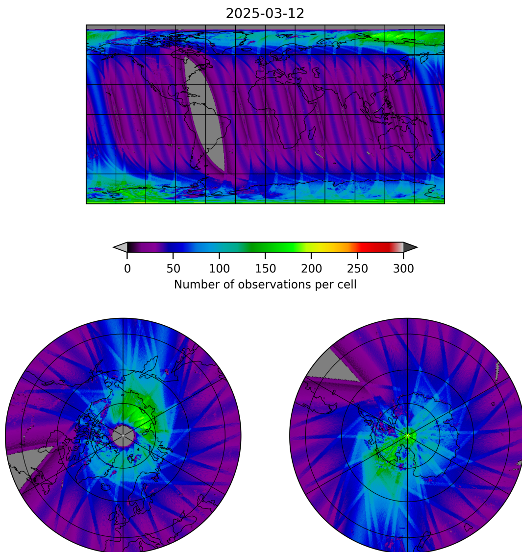
Figure 11: Map of the number of observations for 2025-03-12 to 2025-03-13
