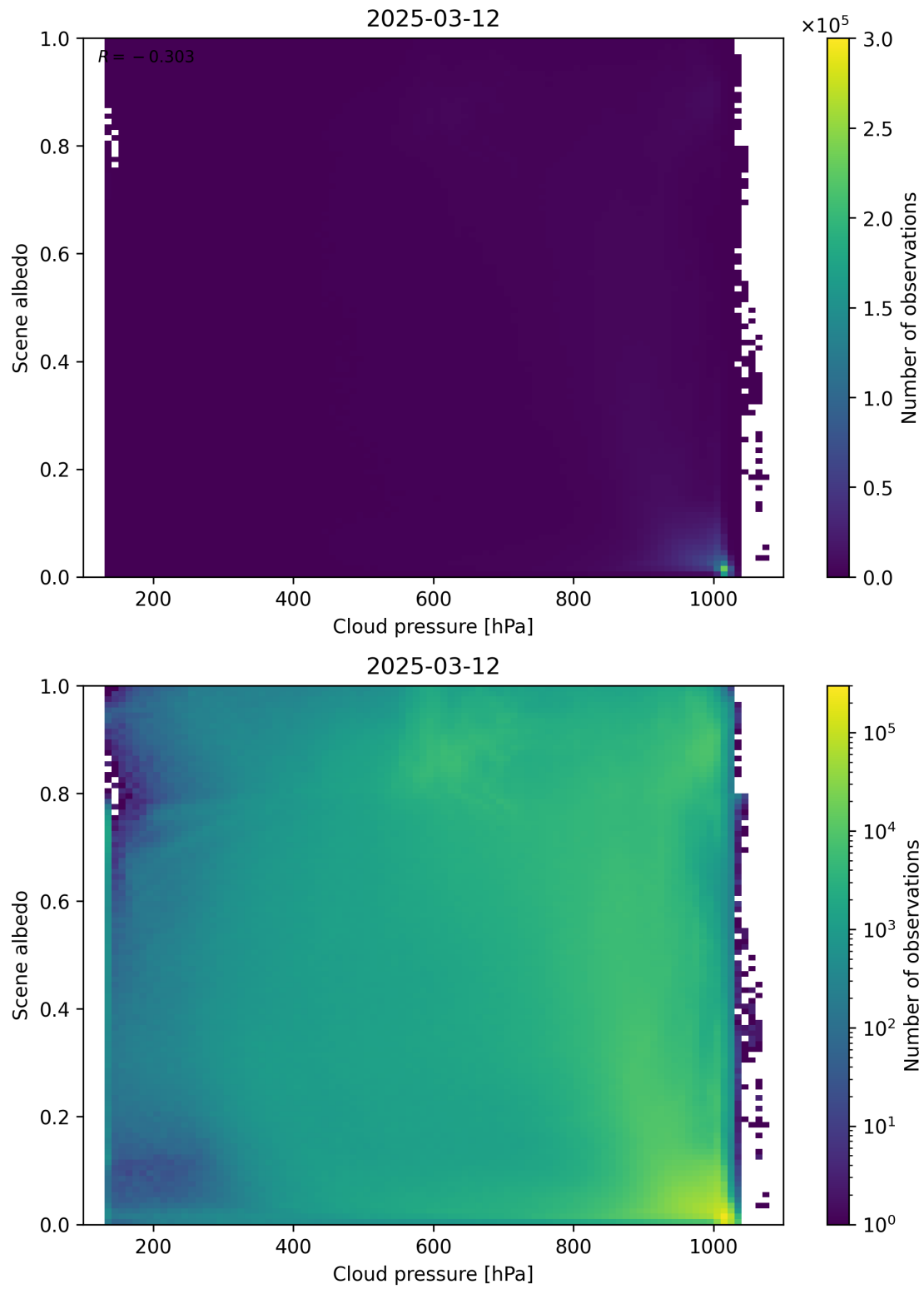
Figure 83: Scatter density plot of “Cloud pressure” against “Scene albedo” for 2025-03-12 to 2025-03-13.
