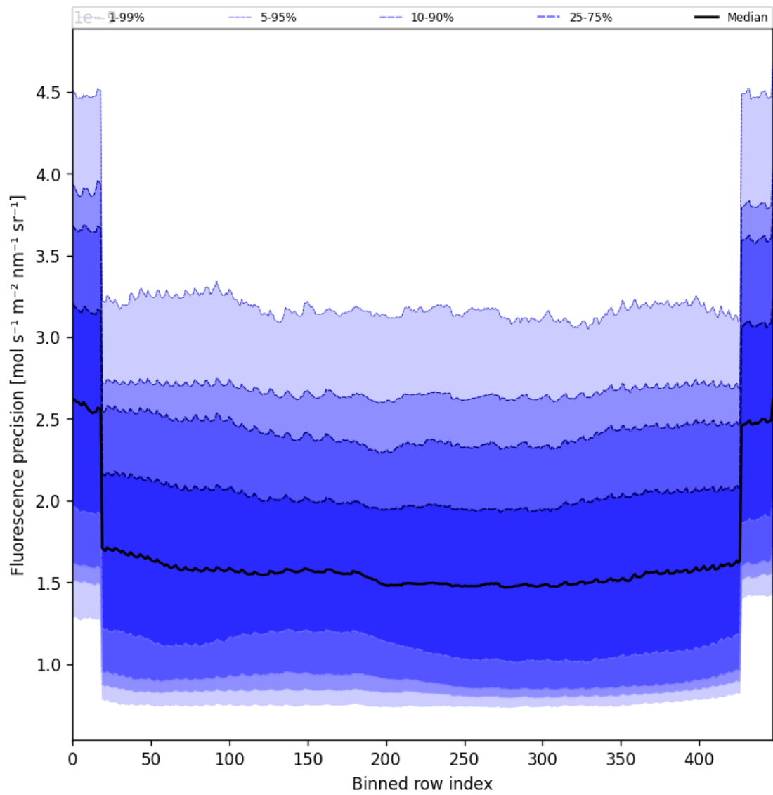
Figure 58: Along track statistics of “Fluorescence precision” for 2025-03-12 to 2025-03-13
