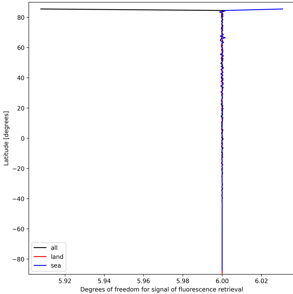
Figure 26: Zonal average of “Degrees of freedom for signal of fluorescence retrieval” for 2025-03-12 to 2025-03-13.
