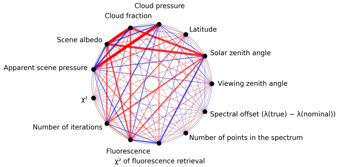
Figure 1: Map of correlation graph for 2025-03-12 to 2025-03-13.
