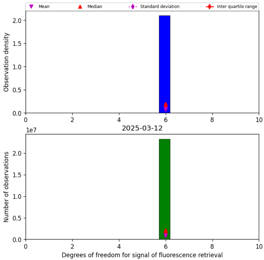
Figure 43: Histogram of “Degrees of freedom for signal of fluorescence retrieval” for 2025-03-12 to 2025-03-13
