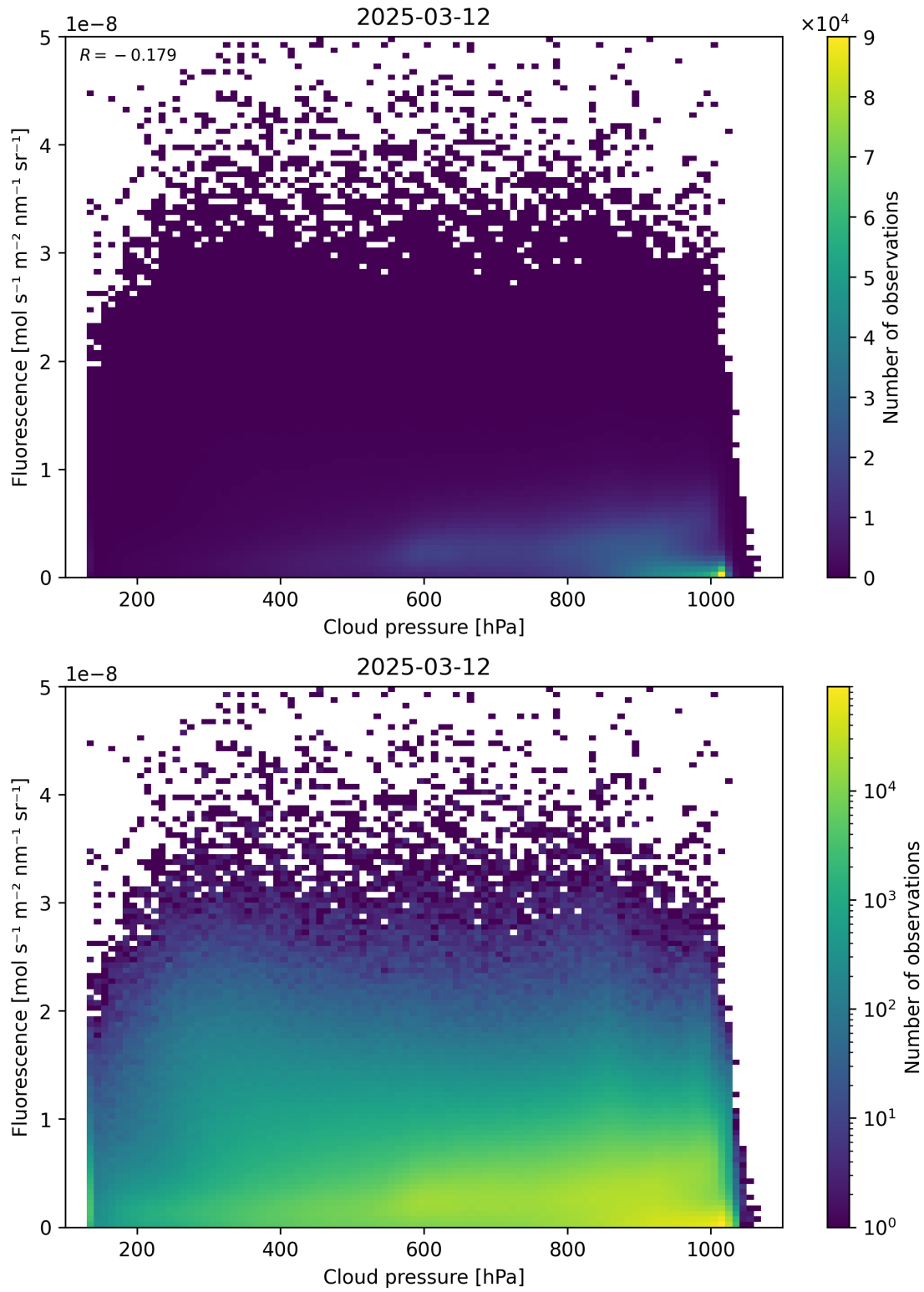
Figure 80: Scatter density plot of “Cloud pressure” against “Fluorescence” for 2025-03-12 to 2025-03-13.
