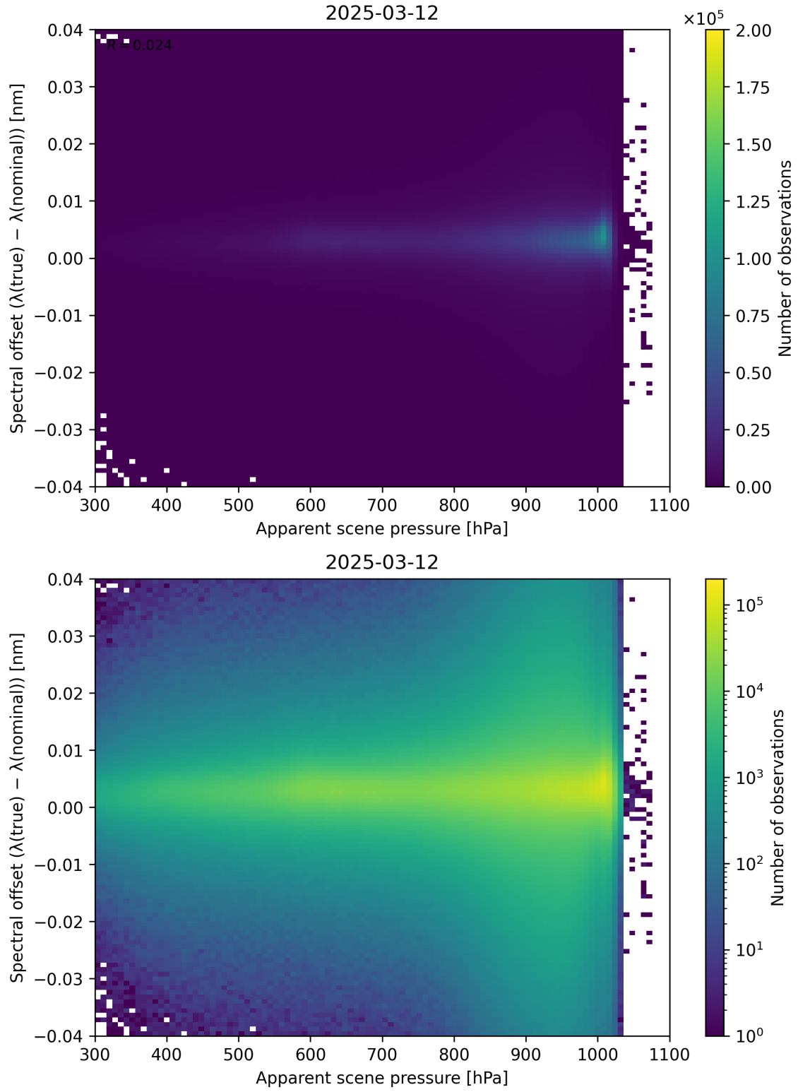
Figure 67: Scatter density plot of “Apparent scene pressure” against “Spectral offset ( \lambda_{\text{true}} - \lambda_{\text{nominal}} )” for 2025-03-12 to 2025-03-13.
