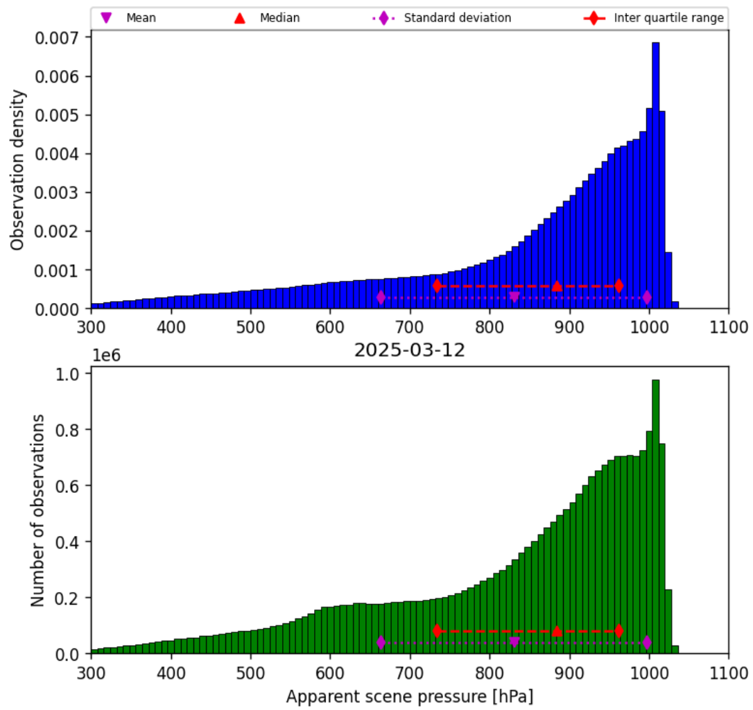
Figure 36: Histogram of “Apparent scene pressure” for 2025-03-12 to 2025-03-13
