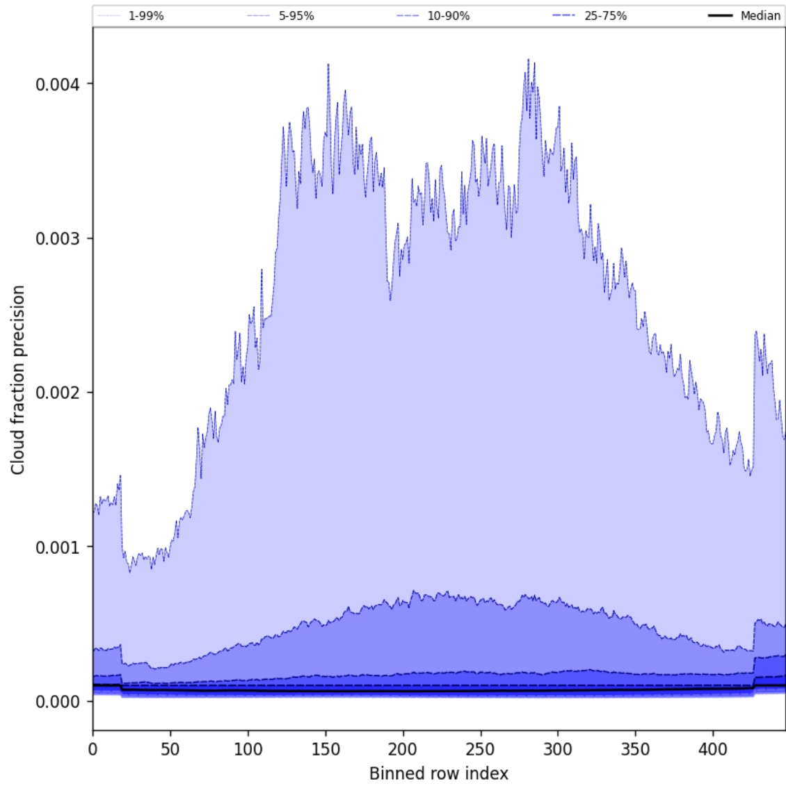
Figure 50: Along track statistics of “Cloud fraction precision” for 2025-03-12 to 2025-03-13
