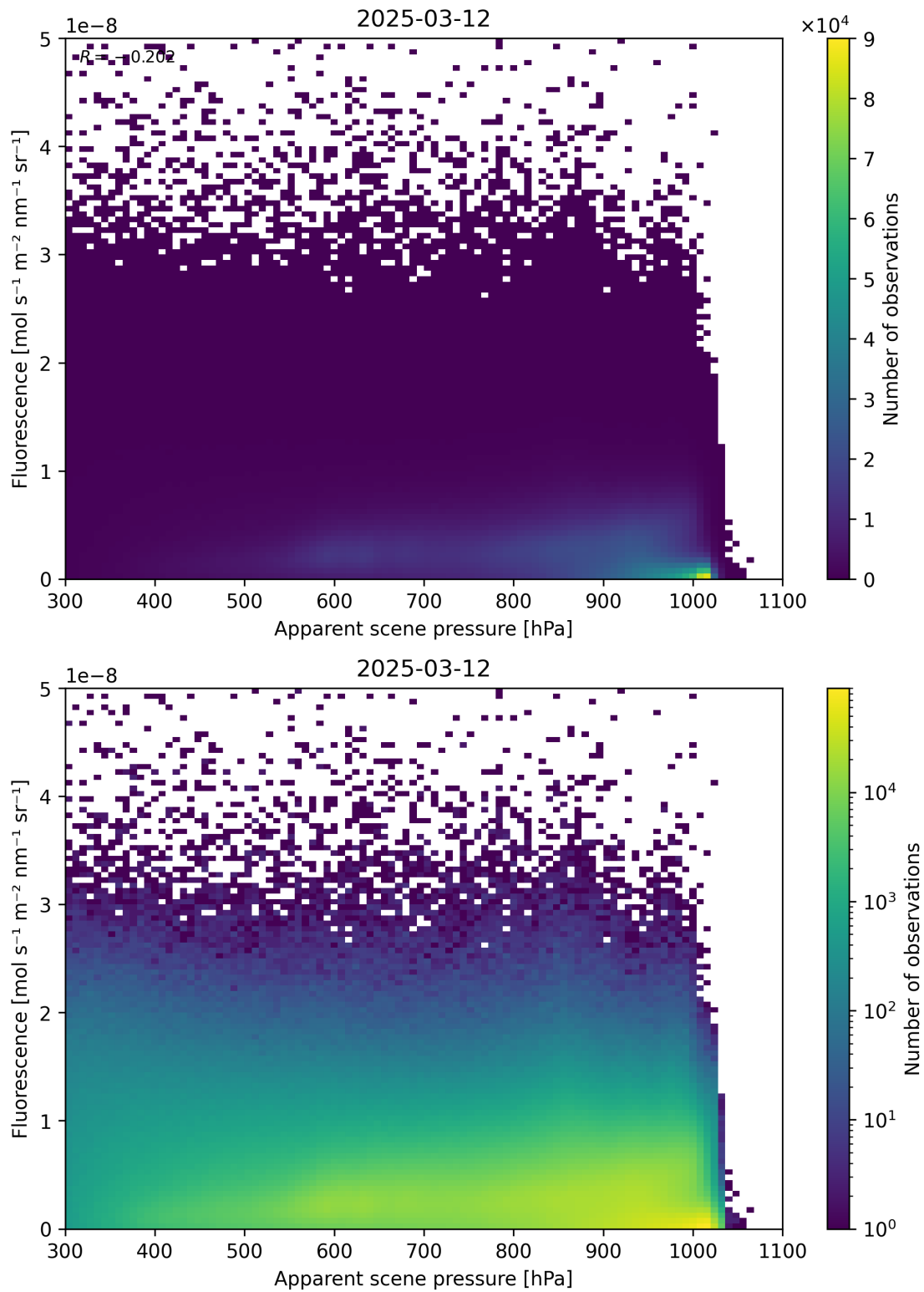
Figure 64: Scatter density plot of “Apparent scene pressure” against “Fluorescence” for 2025-03-12 to 2025-03-13.
