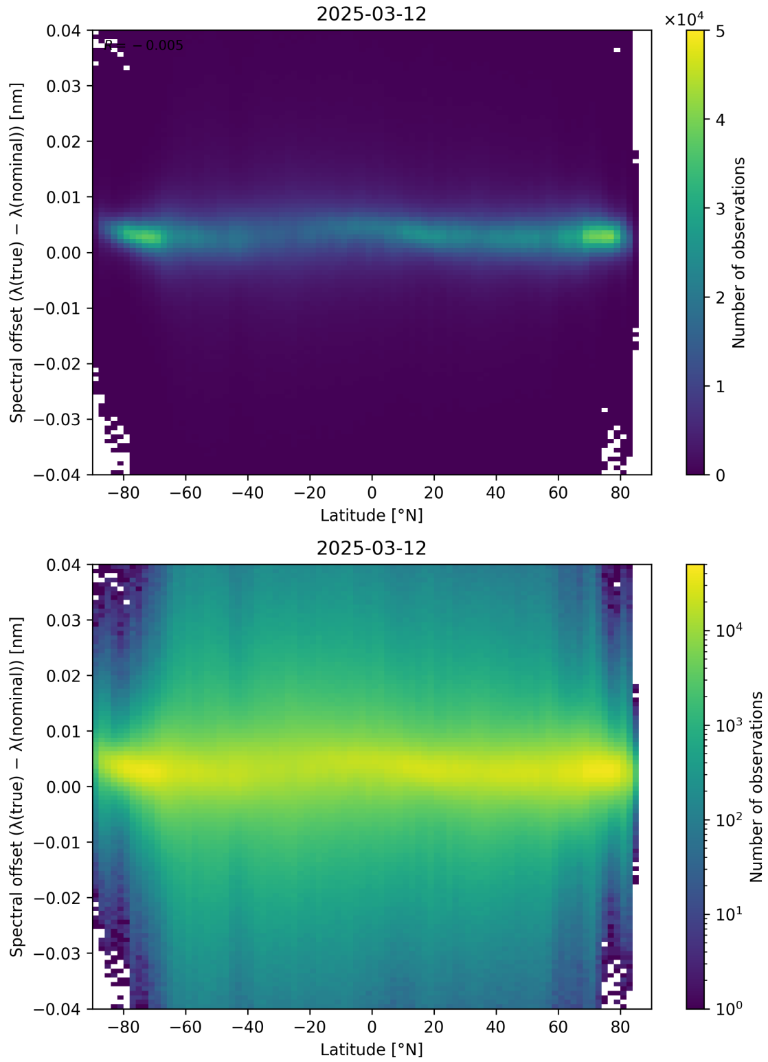
Figure 96: Scatter density plot of “Latitude” against “Spectral offset ( \lambda_{\text{true}} - \lambda_{\text{nominal}} )” for 2025-03-12 to 2025-03-13.
