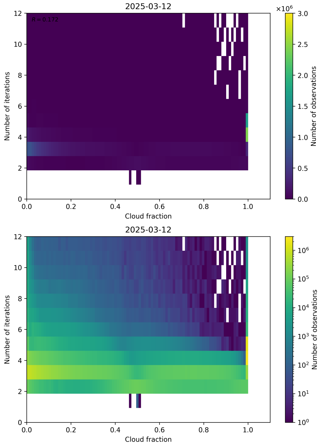
Figure 73: Scatter density plot of “Cloud fraction” against “Number of iterations” for 2025-03-12 to 2025-03-13.
