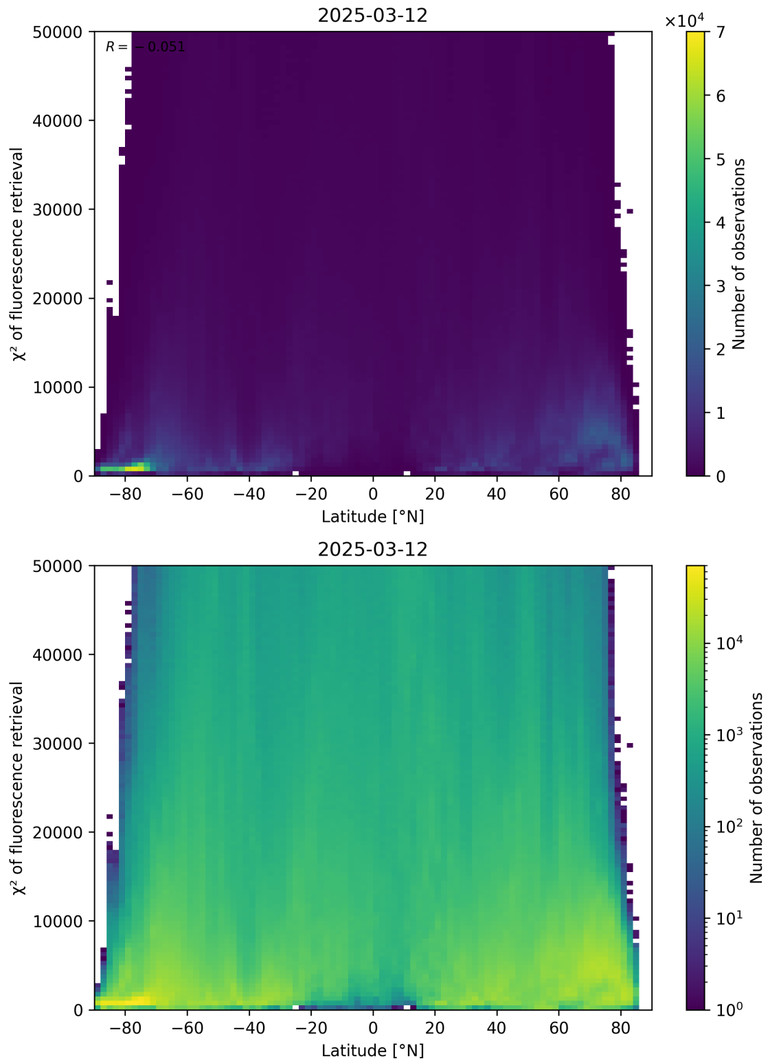
Figure 89: Scatter density plot of “Latitude” against “ \chi^2 of fluorescence retrieval” for 2025-03-12 to 2025-03-13.
