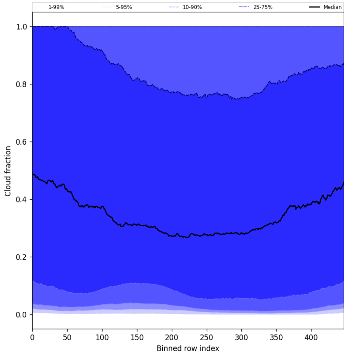
Figure 49: Along track statistics of “Cloud fraction” for 2025-03-12 to 2025-03-13
