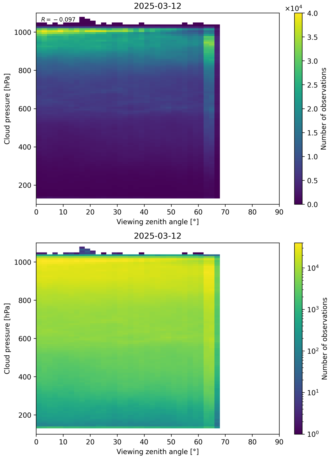
Figure 121: Scatter density plot of “Viewing zenith angle” against “Cloud pressure” for 2025-03-12 to 2025-03-13.
