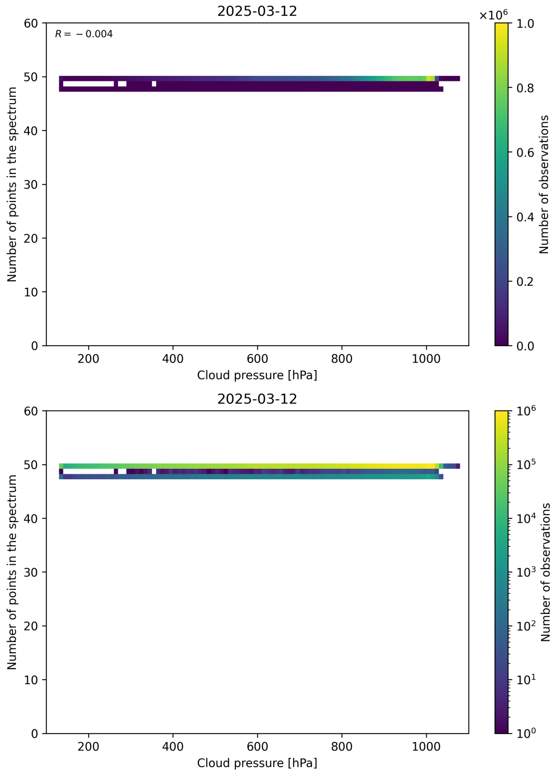
Figure 82: Scatter density plot of “Cloud pressure” against “Number of points in the spectrum” for 2025-03-12 to 2025-03-13.
