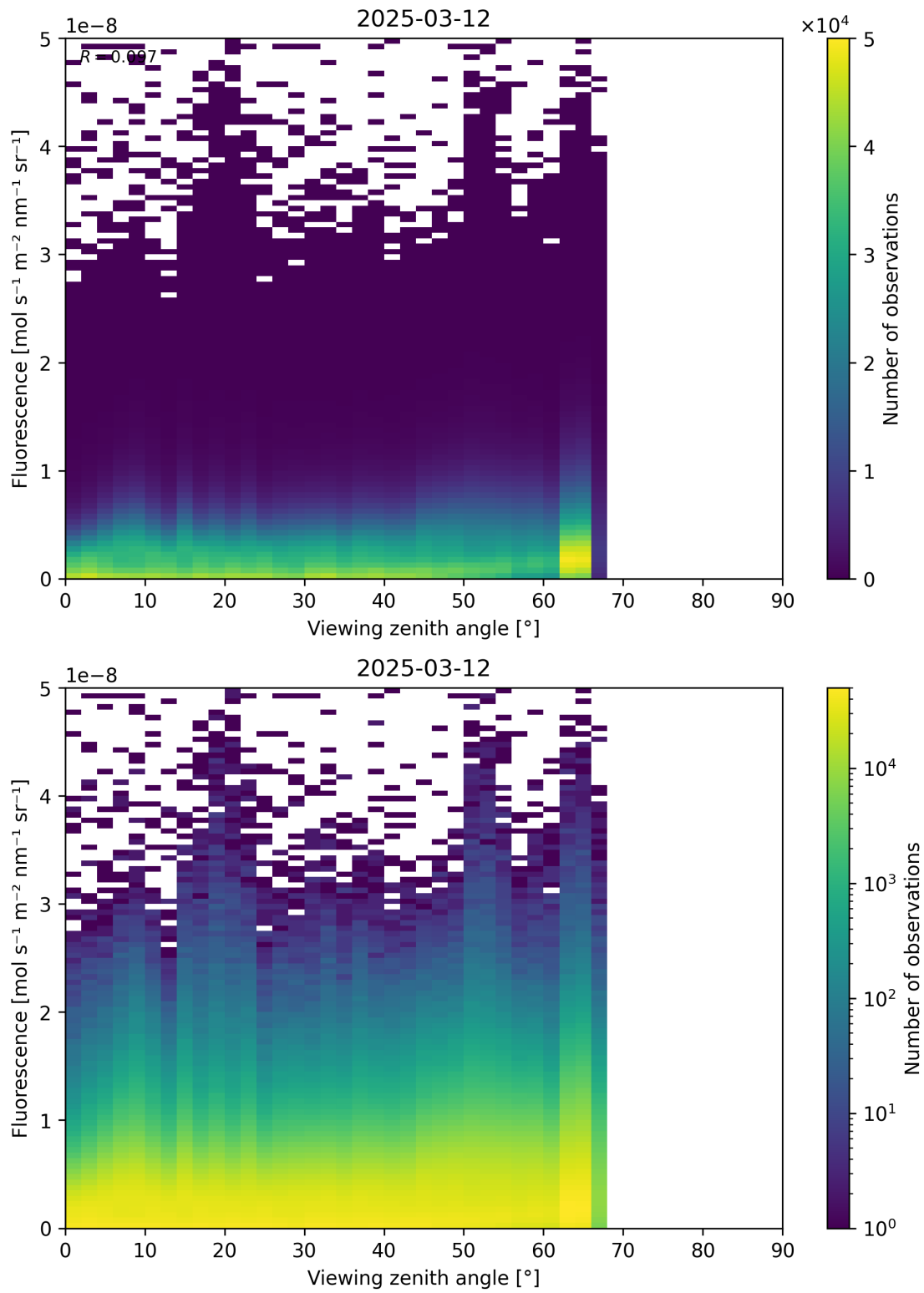
Figure 122: Scatter density plot of "Viewing zenith angle" against "Fluorescence" for 2025-03-12 to 2025-03-13.
