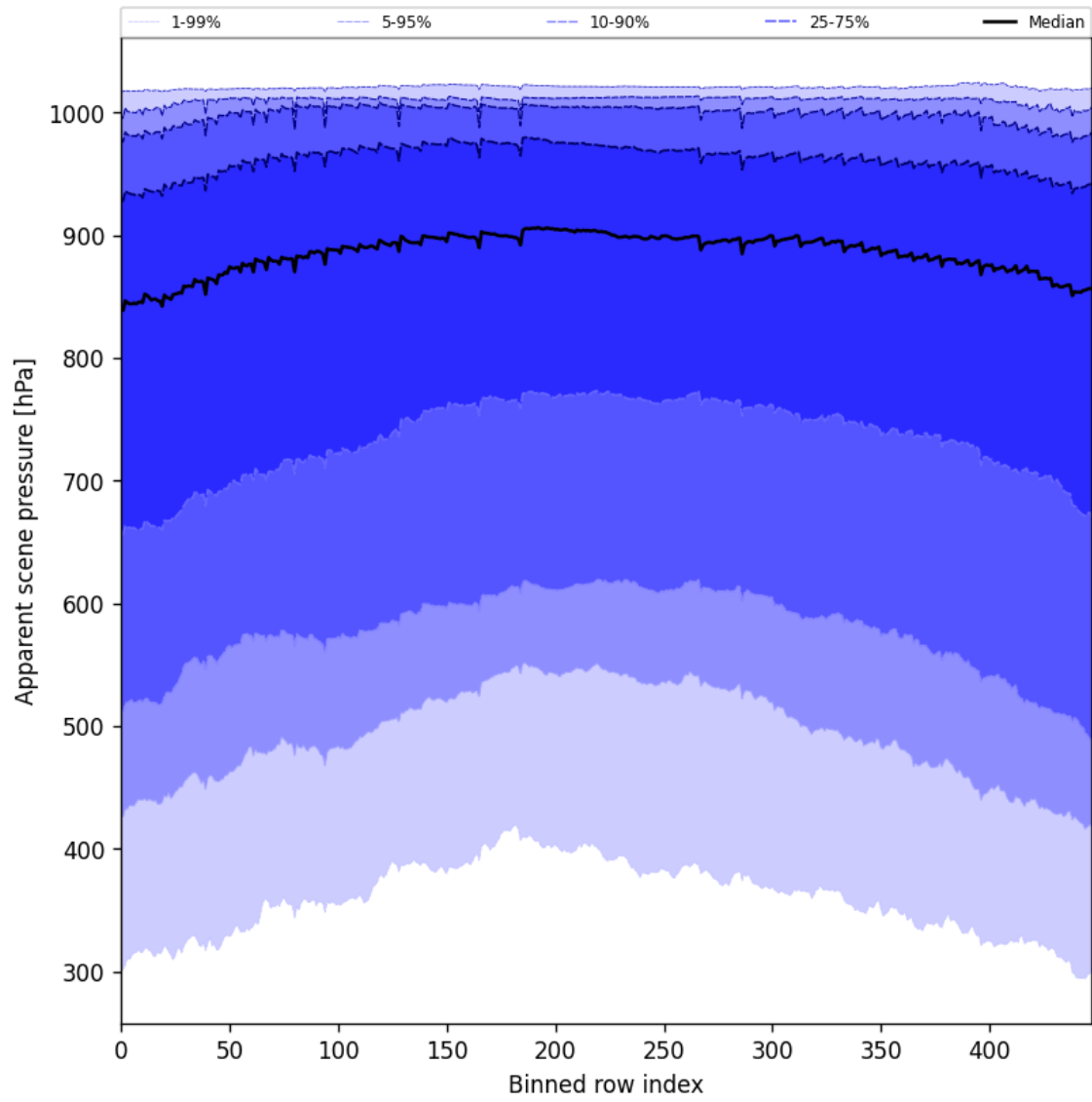
Figure 53: Along track statistics of “Apparent scene pressure” for 2025-03-12 to 2025-03-13
