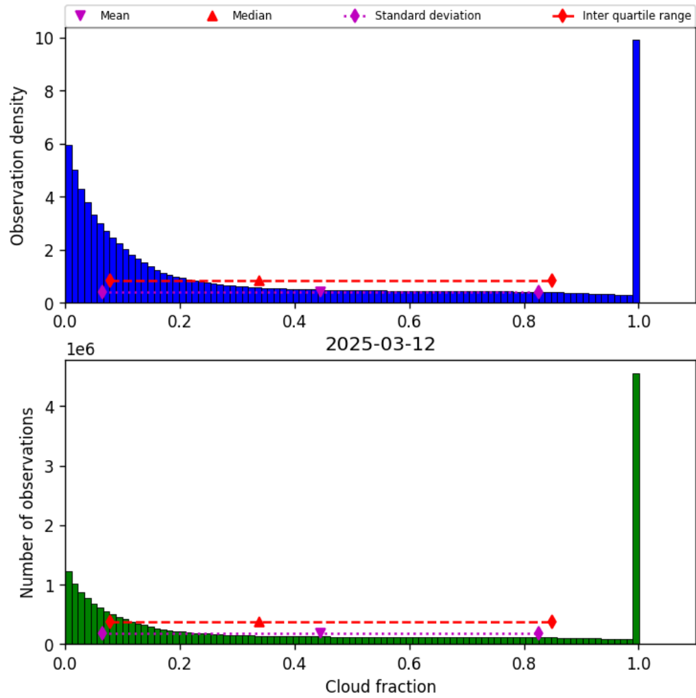
Figure 32: Histogram of “Cloud fraction” for 2025-03-12 to 2025-03-13
