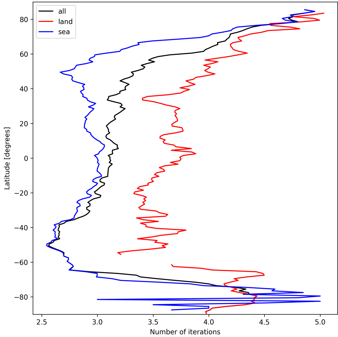
Figure 22: Zonal average of “Number of iterations” for 2025-03-12 to 2025-03-13.
