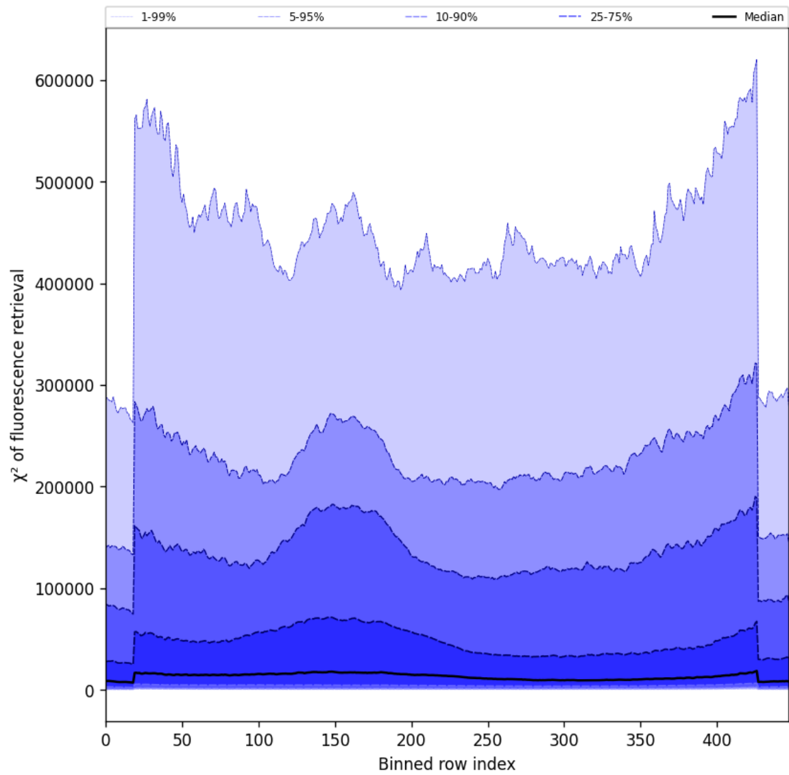
Figure 59: Along track statistics of “ \chi^2 of fluorescence retrieval” for 2025-03-12 to 2025-03-13
