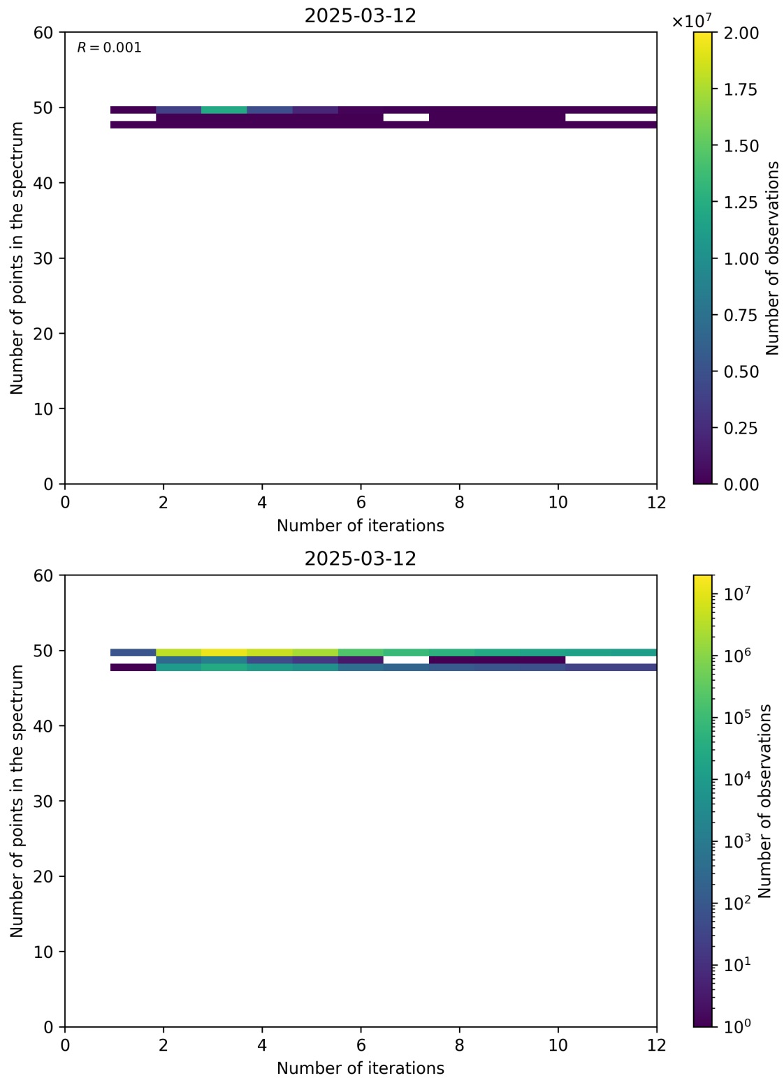
Figure 99: Scatter density plot of “Number of iterations” against “Number of points in the spectrum” for 2025-03-12 to 2025-03-13.
