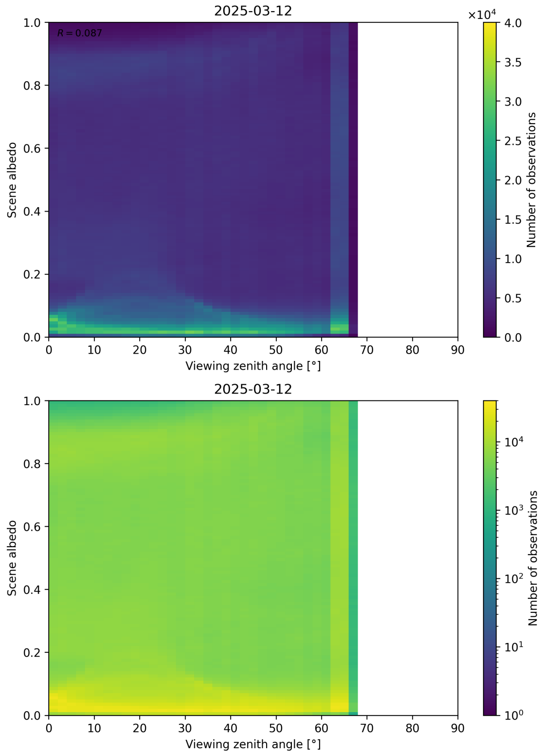
Figure 126: Scatter density plot of “Viewing zenith angle” against “Scene albedo” for 2025-03-12 to 2025-03-13.
