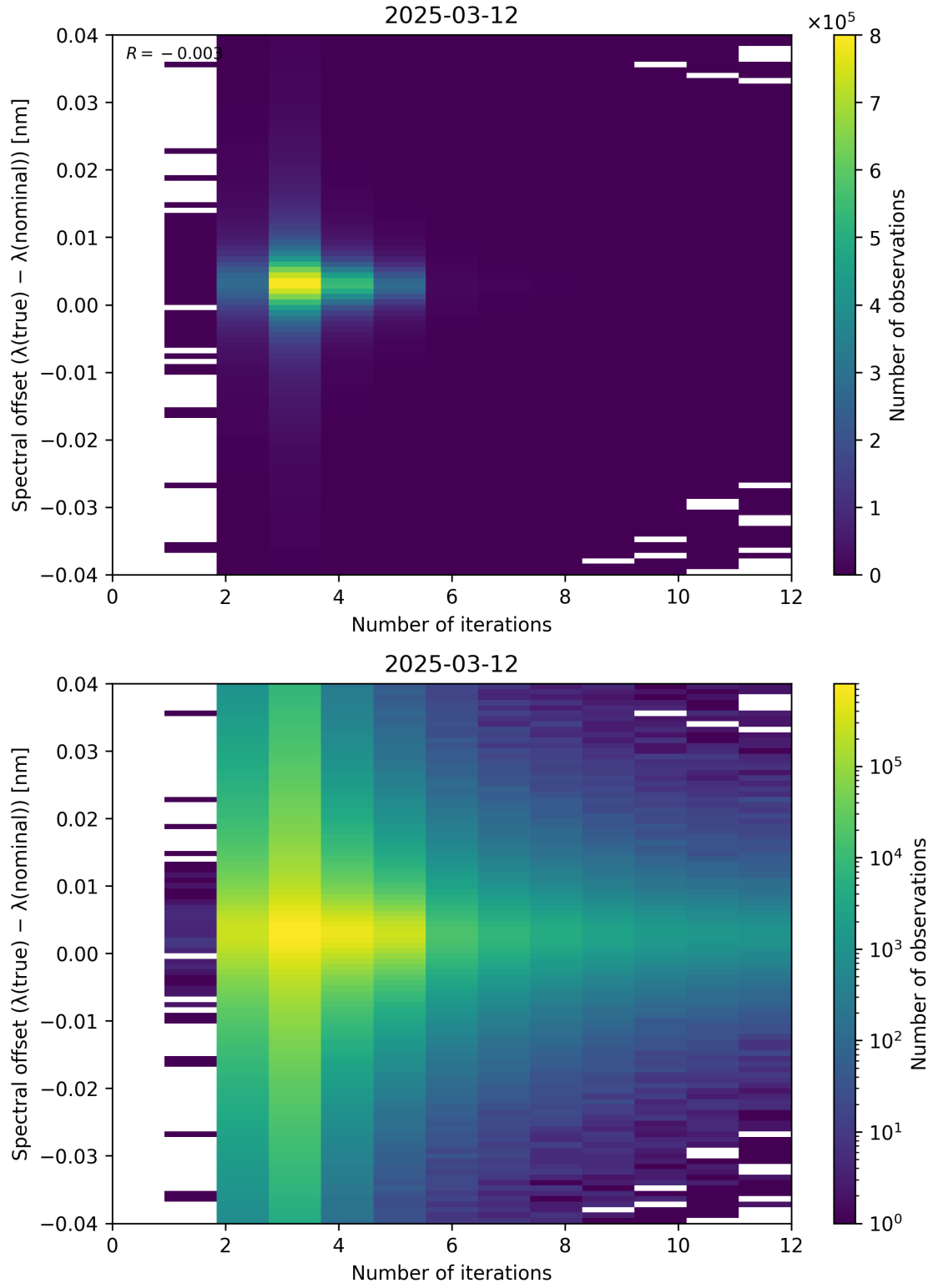
Figure 100: Scatter density plot of “Number of iterations” against “Spectral offset ( \lambda_{\text{true}} - \lambda_{\text{nominal}} )” for 2025-03-12 to 2025-03-13.
