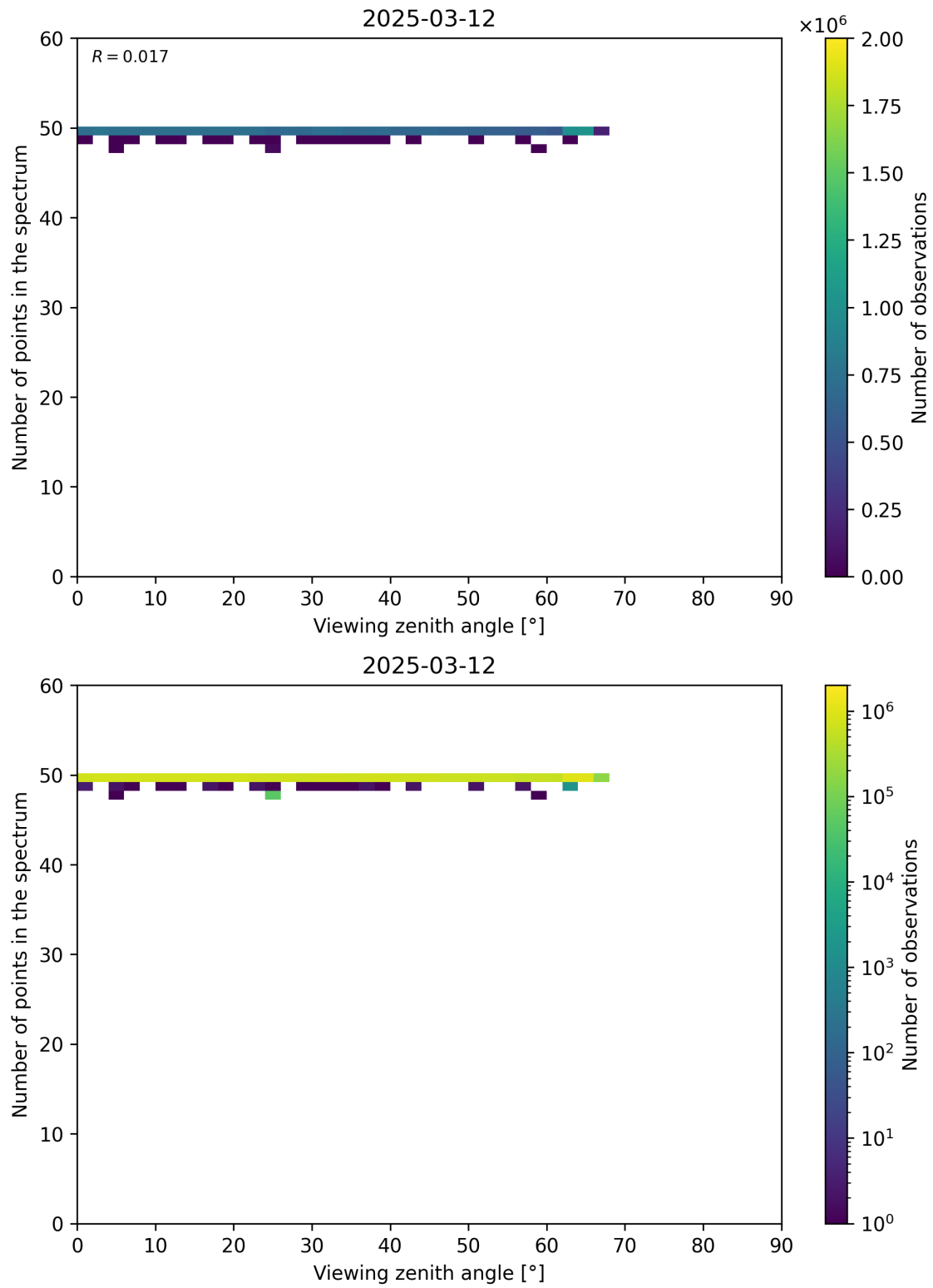
Figure 125: Scatter density plot of “Viewing zenith angle” against “Number of points in the spectrum” for 2025-03-12 to 2025-03-13.
