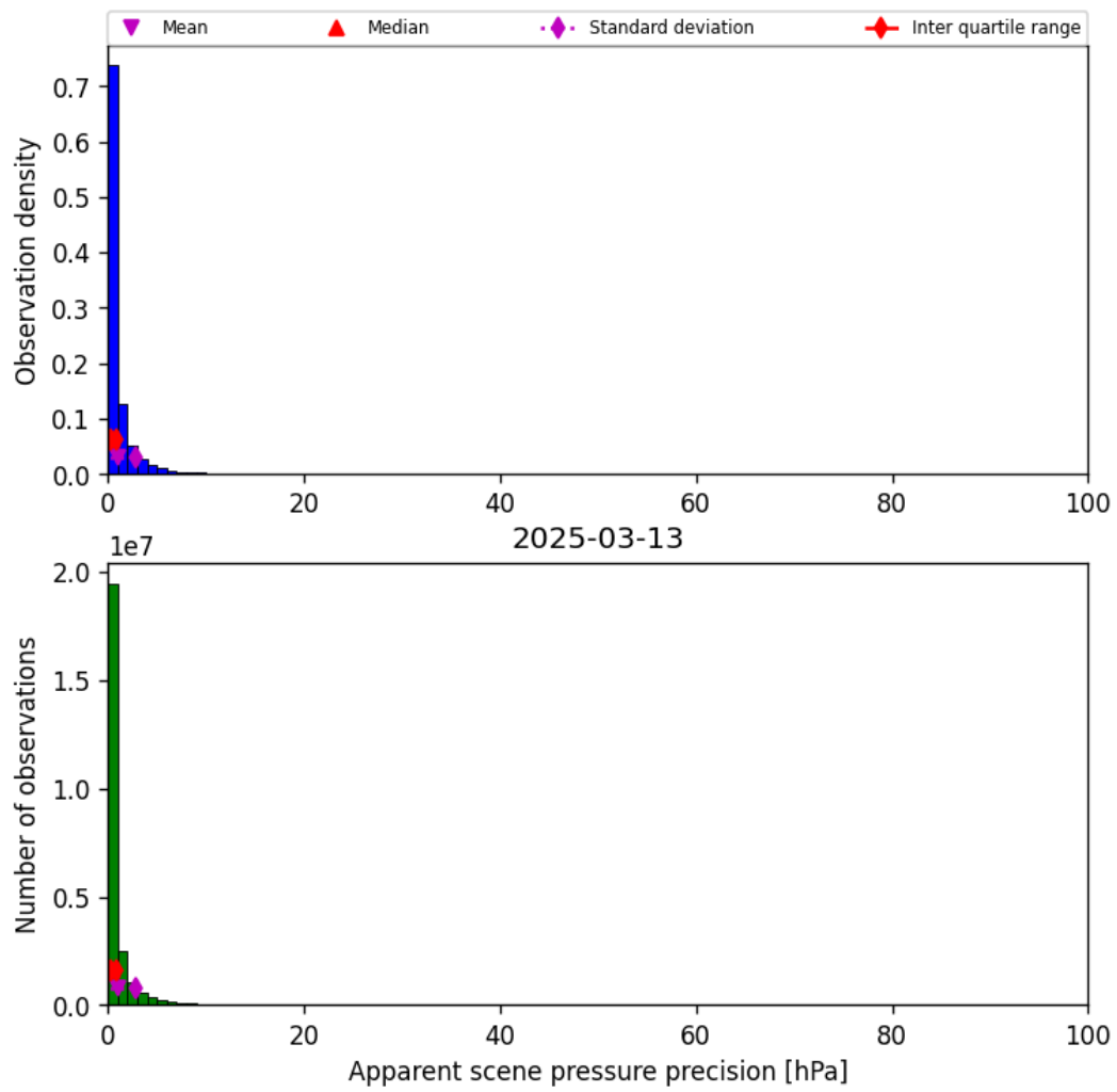
Figure 37: Histogram of “Apparent scene pressure precision” for 2025-03-12 to 2025-03-14
