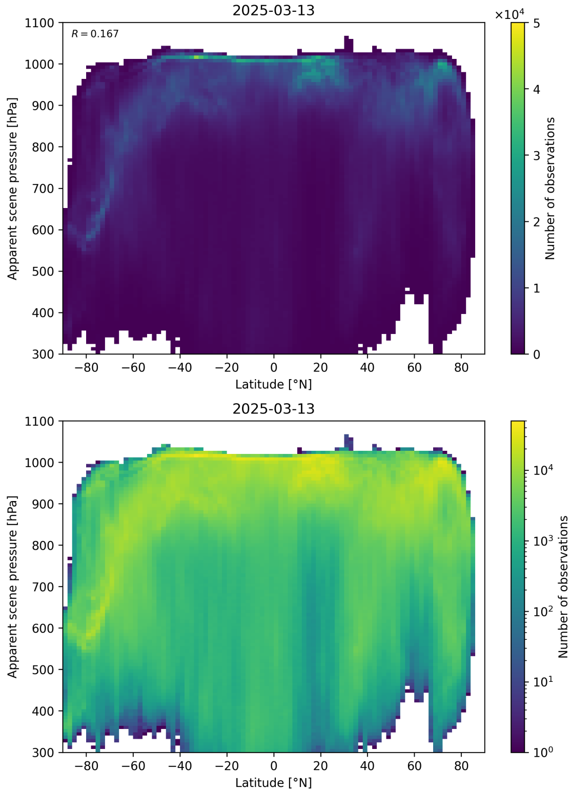
Figure 88: Scatter density plot of “Latitude” against “Apparent scene pressure” for 2025-03-12 to 2025-03-14.
