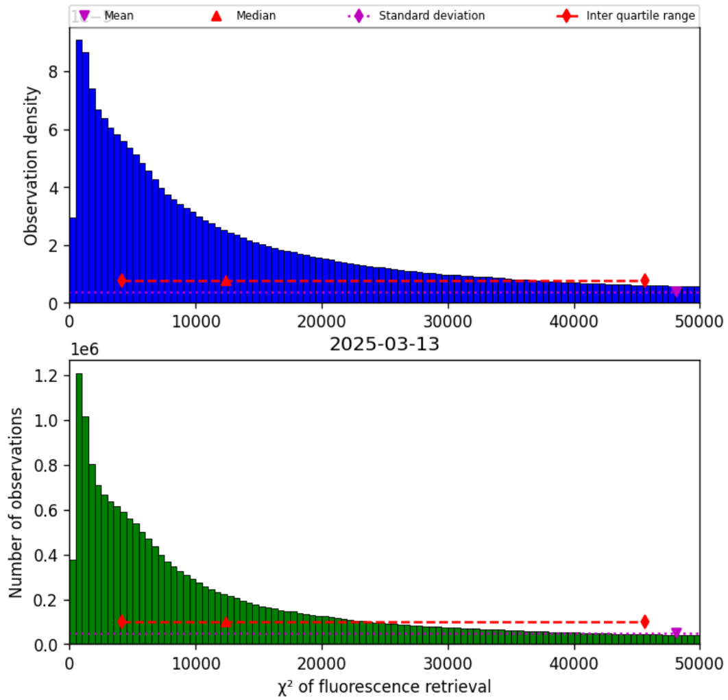
Figure 42: Histogram of “ \chi^2 of fluorescence retrieval” for 2025-03-12 to 2025-03-14
