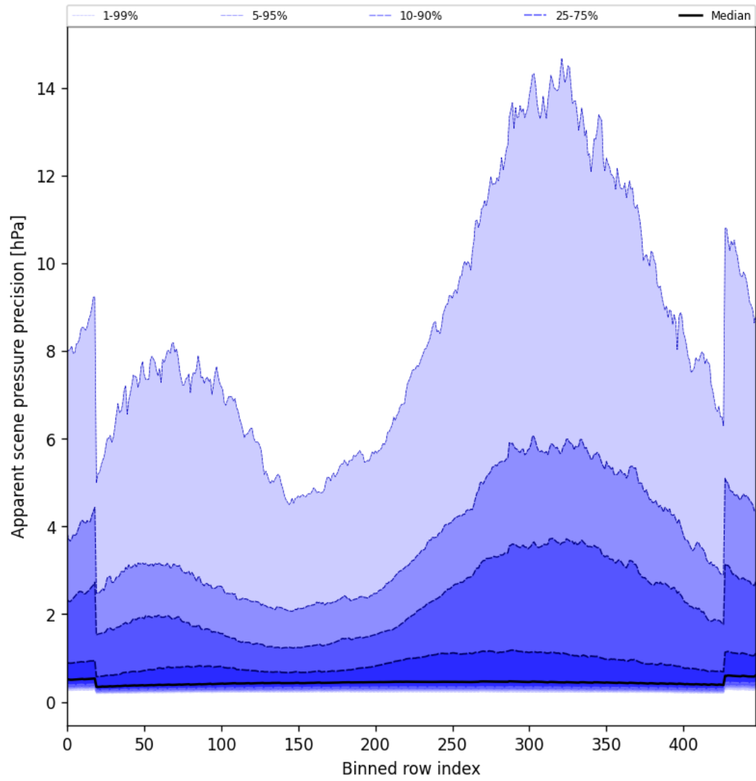
Figure 54: Along track statistics of “Apparent scene pressure precision” for 2025-03-12 to 2025-03-14
