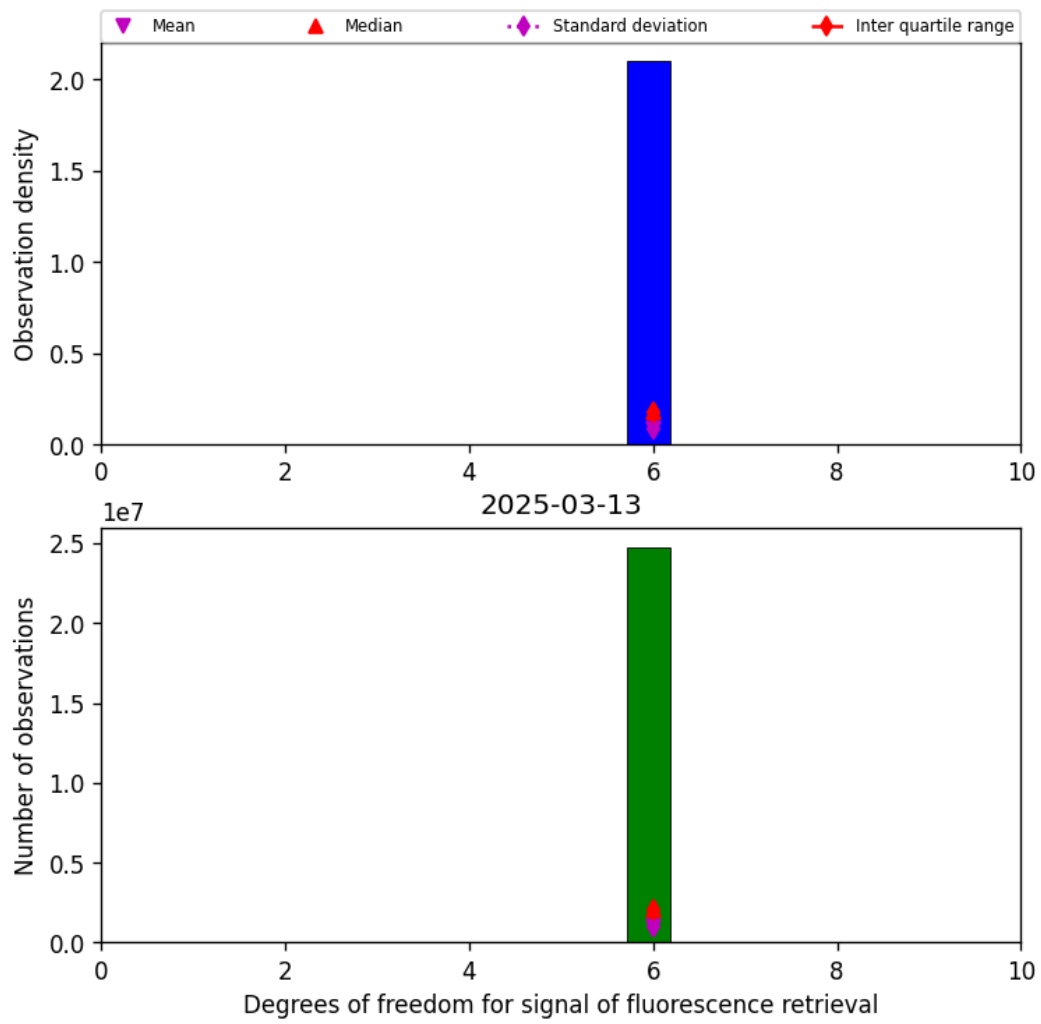
Figure 43: Histogram of “Degrees of freedom for signal of fluorescence retrieval” for 2025-03-12 to 2025-03-14
