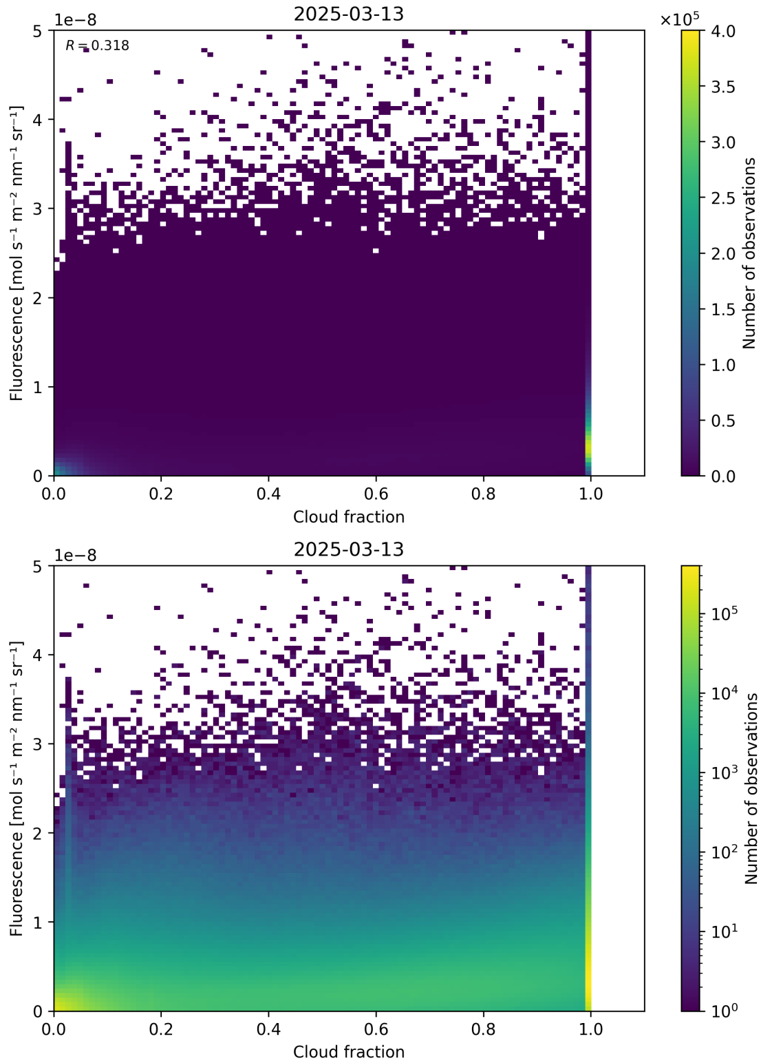
Figure 72: Scatter density plot of “Cloud fraction” against “Fluorescence” for 2025-03-12 to 2025-03-14.
