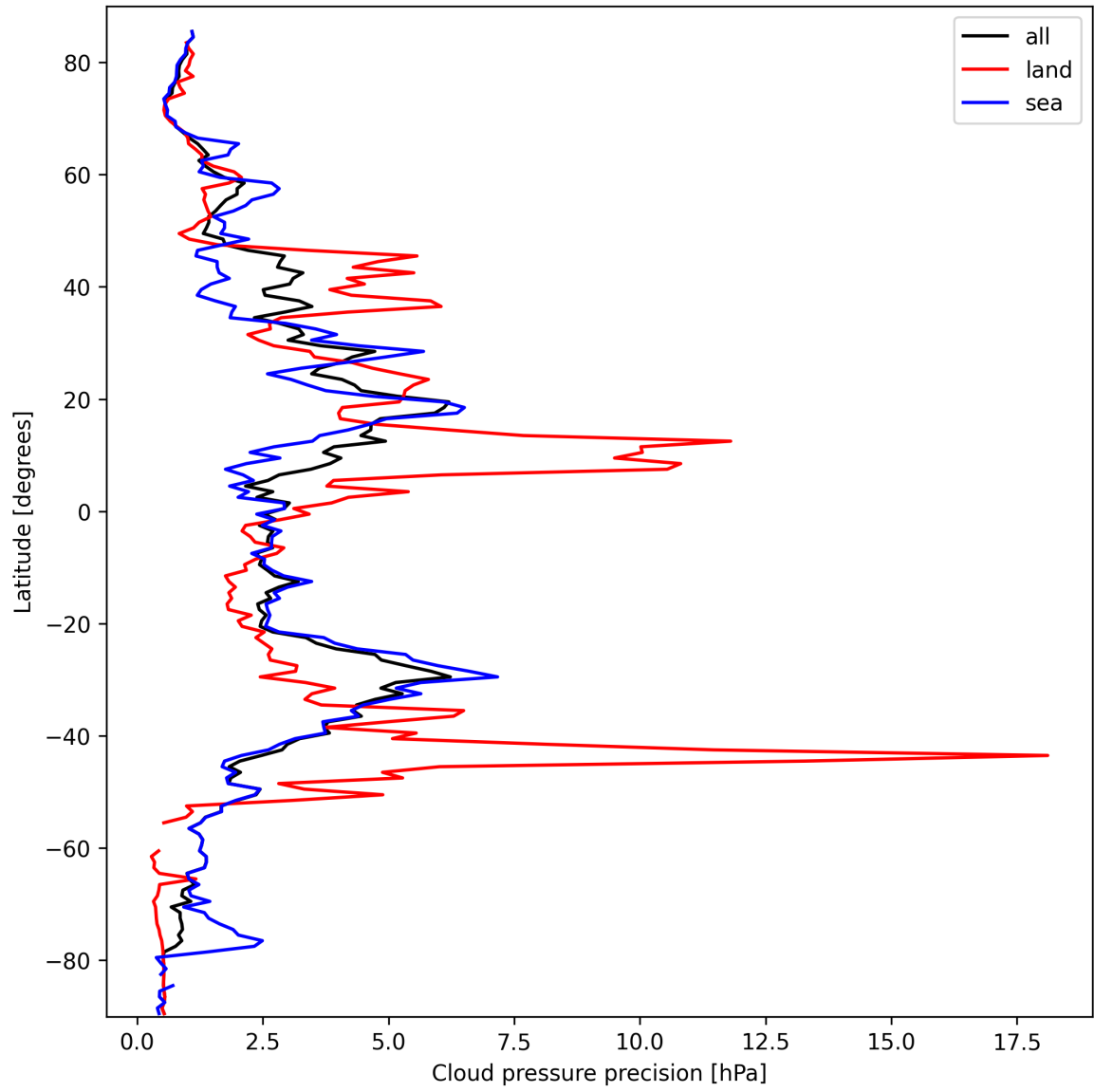
Figure 14: Zonal average of “Cloud pressure precision” for 2025-03-12 to 2025-03-14.
