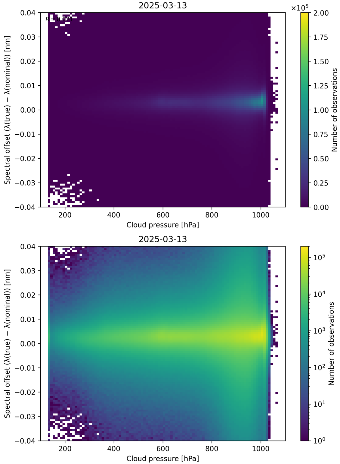
Figure 84: Scatter density plot of “Cloud pressure” against “Spectral offset ( \lambda_{\text{true}} - \lambda_{\text{nominal}} )” for 2025-03-12 to 2025-03-14.
