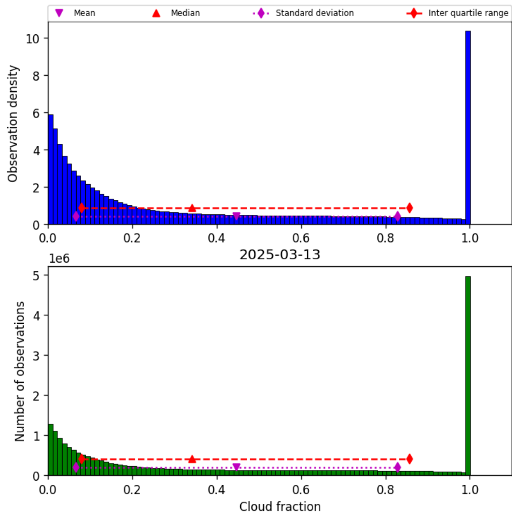
Figure 32: Histogram of “Cloud fraction” for 2025-03-12 to 2025-03-14
