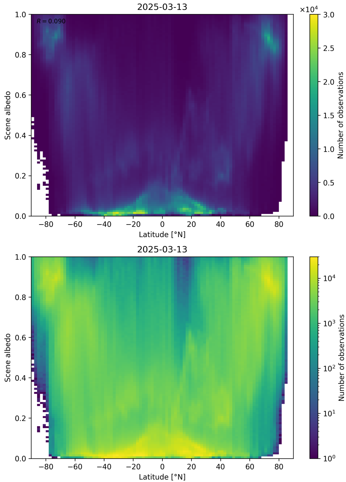
Figure 95: Scatter density plot of “Latitude” against “Scene albedo” for 2025-03-12 to 2025-03-14.
