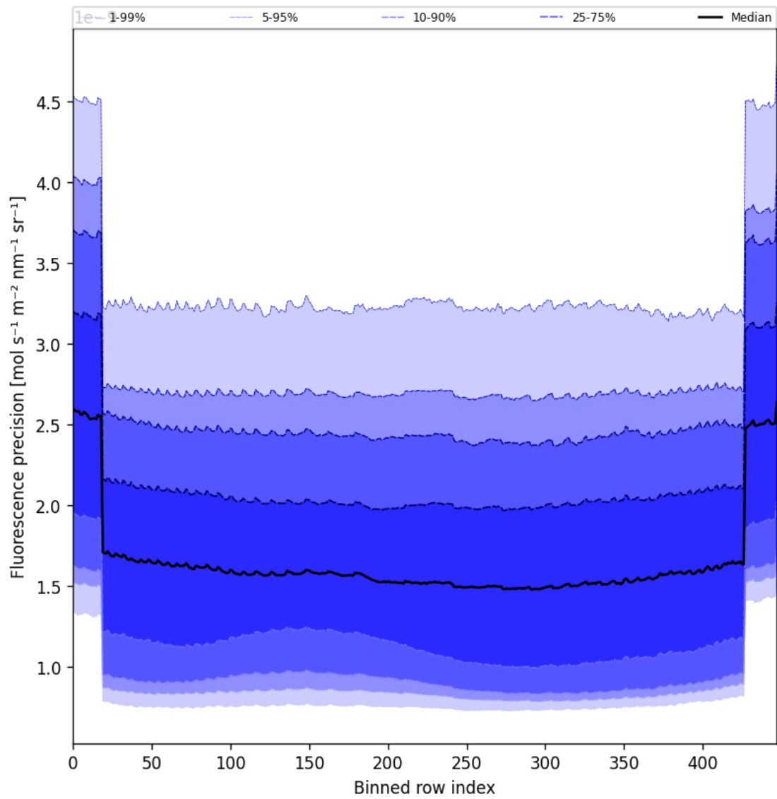
Figure 58: Along track statistics of “Fluorescence precision” for 2025-03-12 to 2025-03-14
