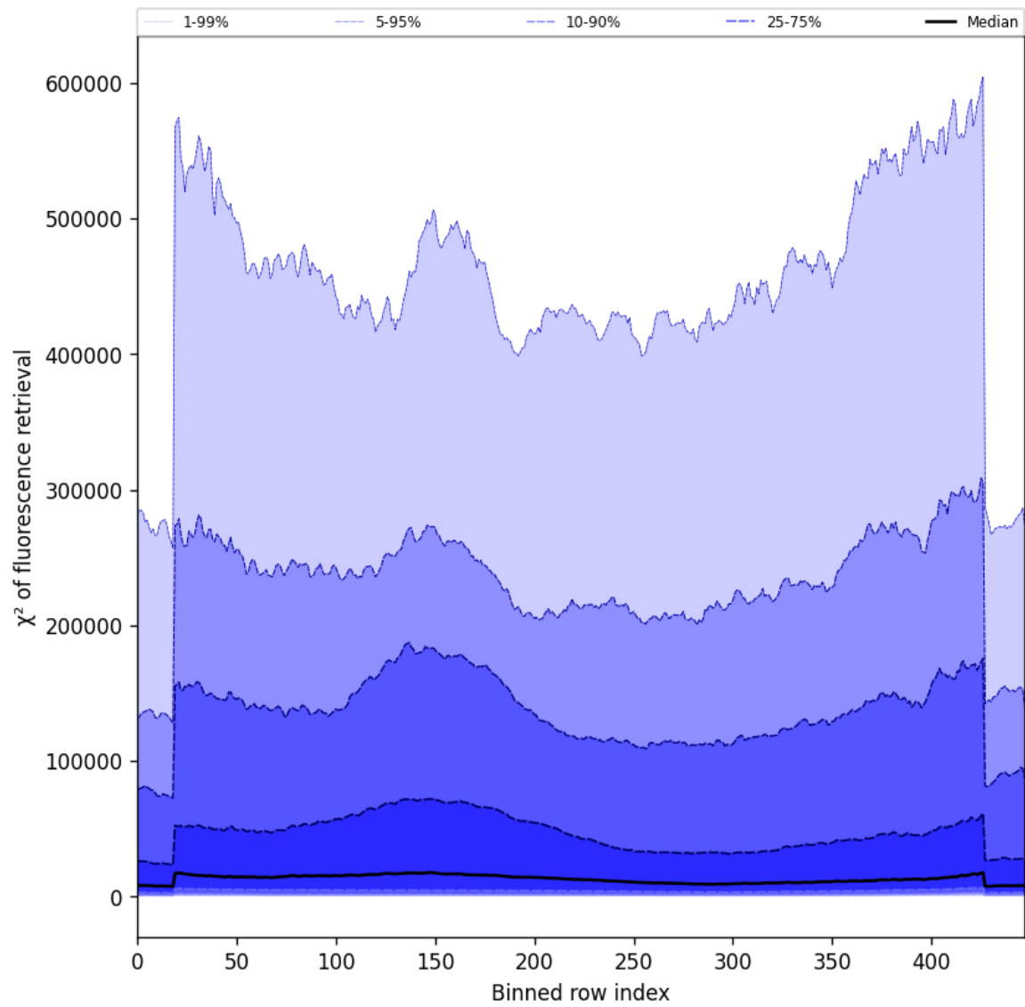
Figure 59: Along track statistics of “ \chi^2 of fluorescence retrieval” for 2025-03-12 to 2025-03-14
