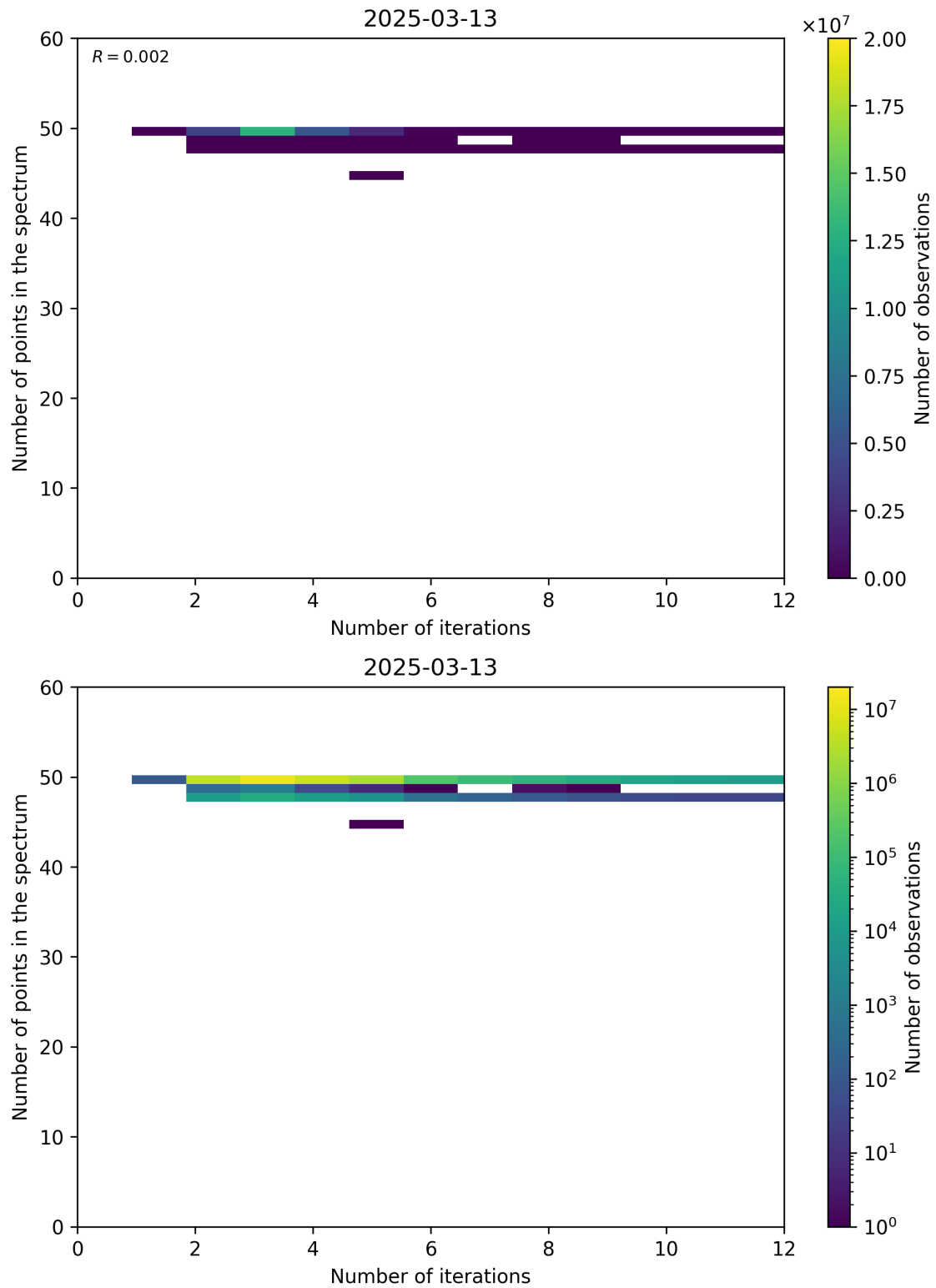
Figure 99: Scatter density plot of “Number of iterations” against “Number of points in the spectrum” for 2025-03-12 to 2025-03-14.
