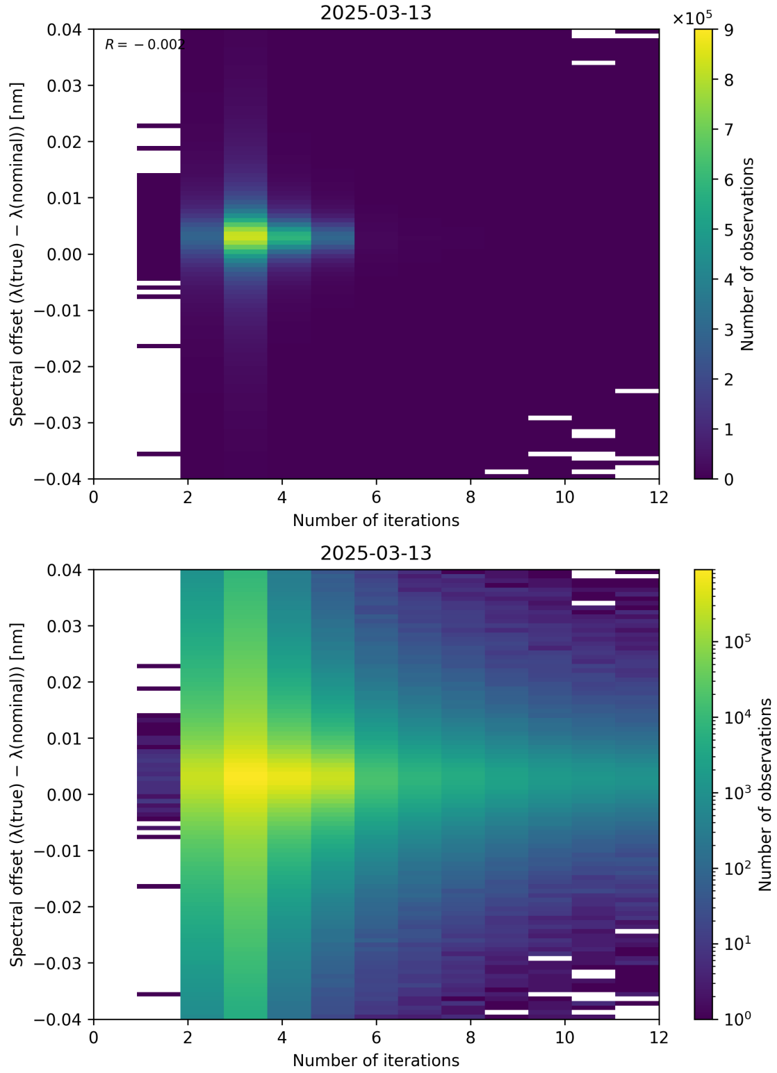
Figure 100: Scatter density plot of “Number of iterations” against “Spectral offset ( \lambda_{\text{true}} - \lambda_{\text{nominal}} )” for 2025-03-12 to 2025-03-14.
