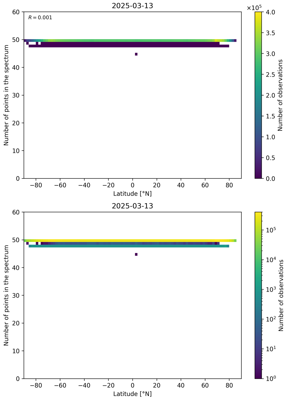
Figure 94: Scatter density plot of “Latitude” against “Number of points in the spectrum” for 2025-03-12 to 2025-03-14.
