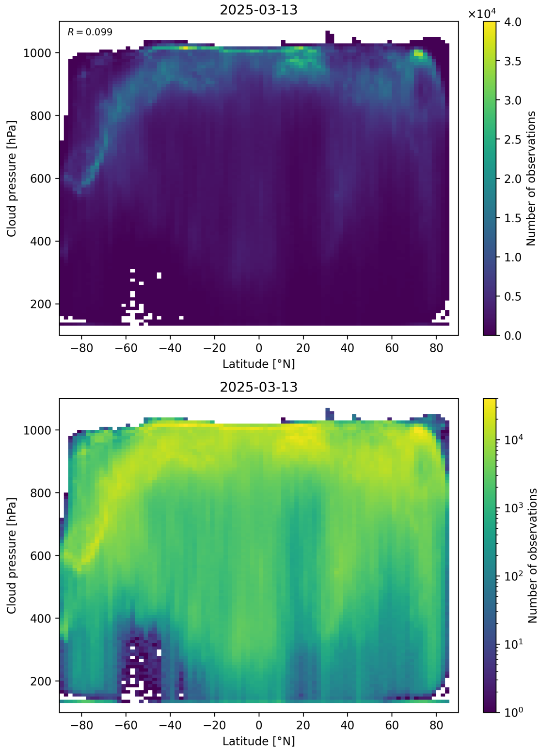
Figure 91: Scatter density plot of “Latitude” against “Cloud pressure” for 2025-03-12 to 2025-03-14.
