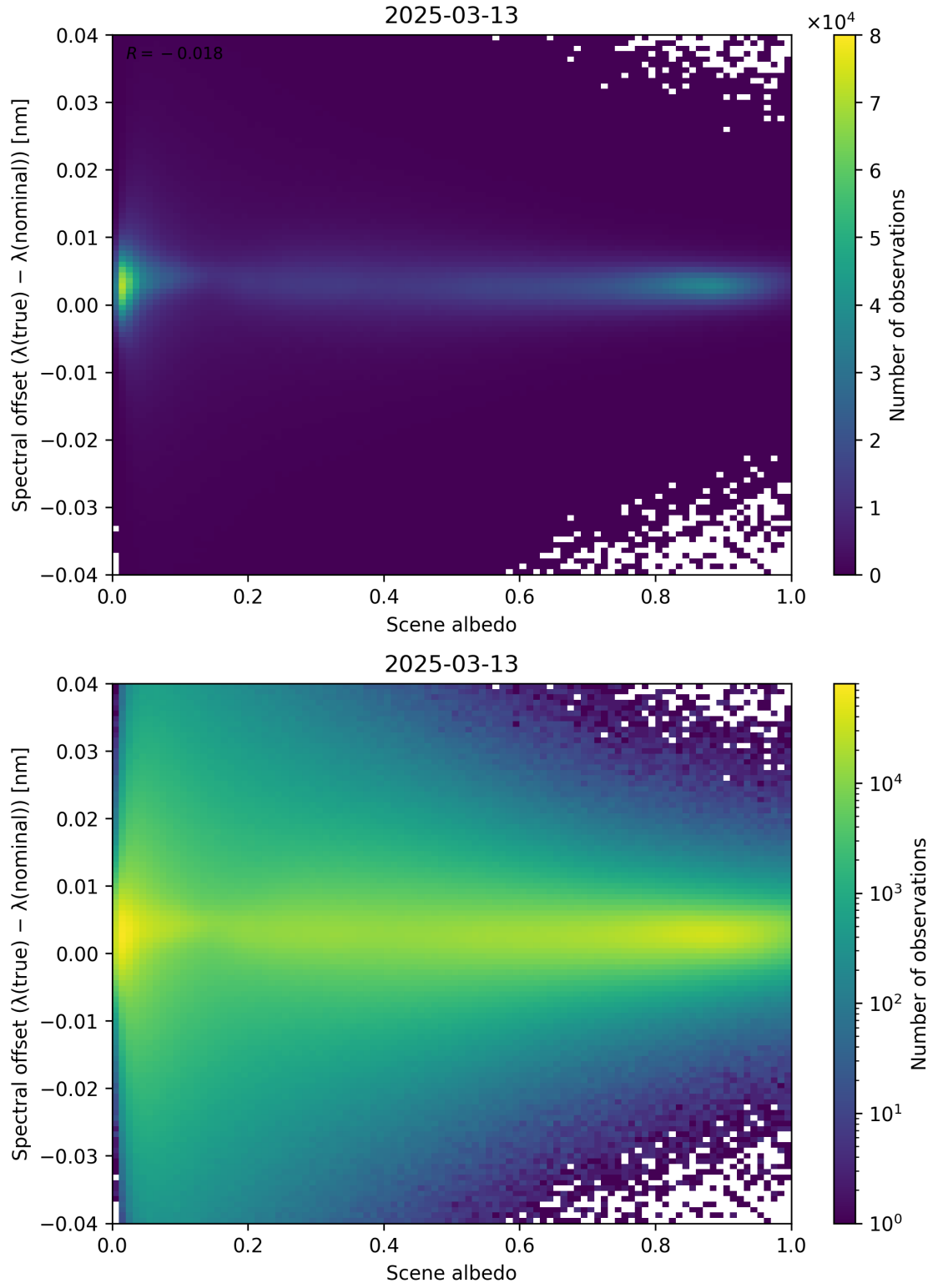
Figure 107: Scatter density plot of “Scene albedo” against “Spectral offset ( \lambda_{\text{true}} - \lambda_{\text{nominal}} )” for 2025-03-12 to 2025-03-14.
