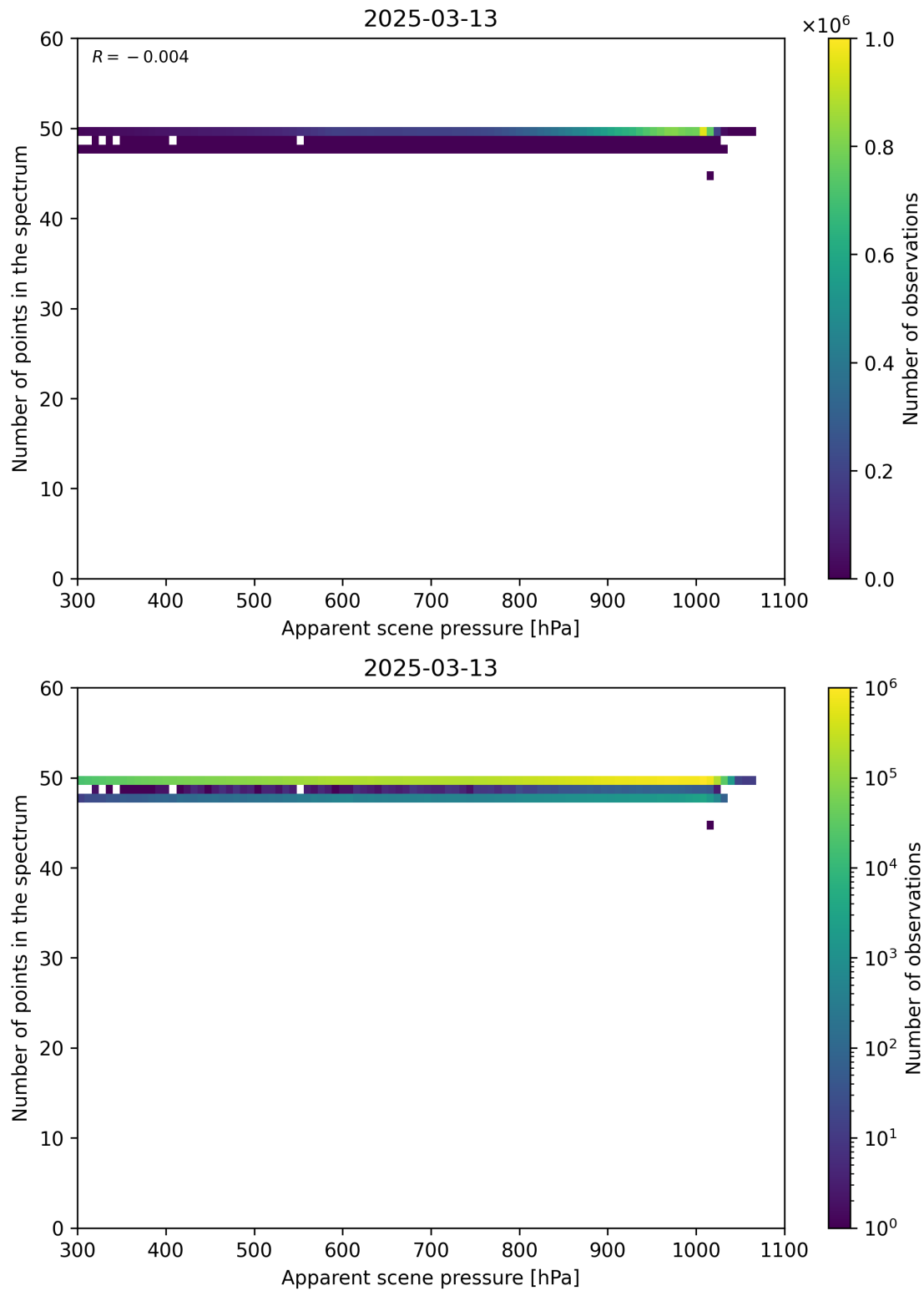
Figure 66: Scatter density plot of “Apparent scene pressure” against “Number of points in the spectrum” for 2025-03-12 to 2025-03-14.
