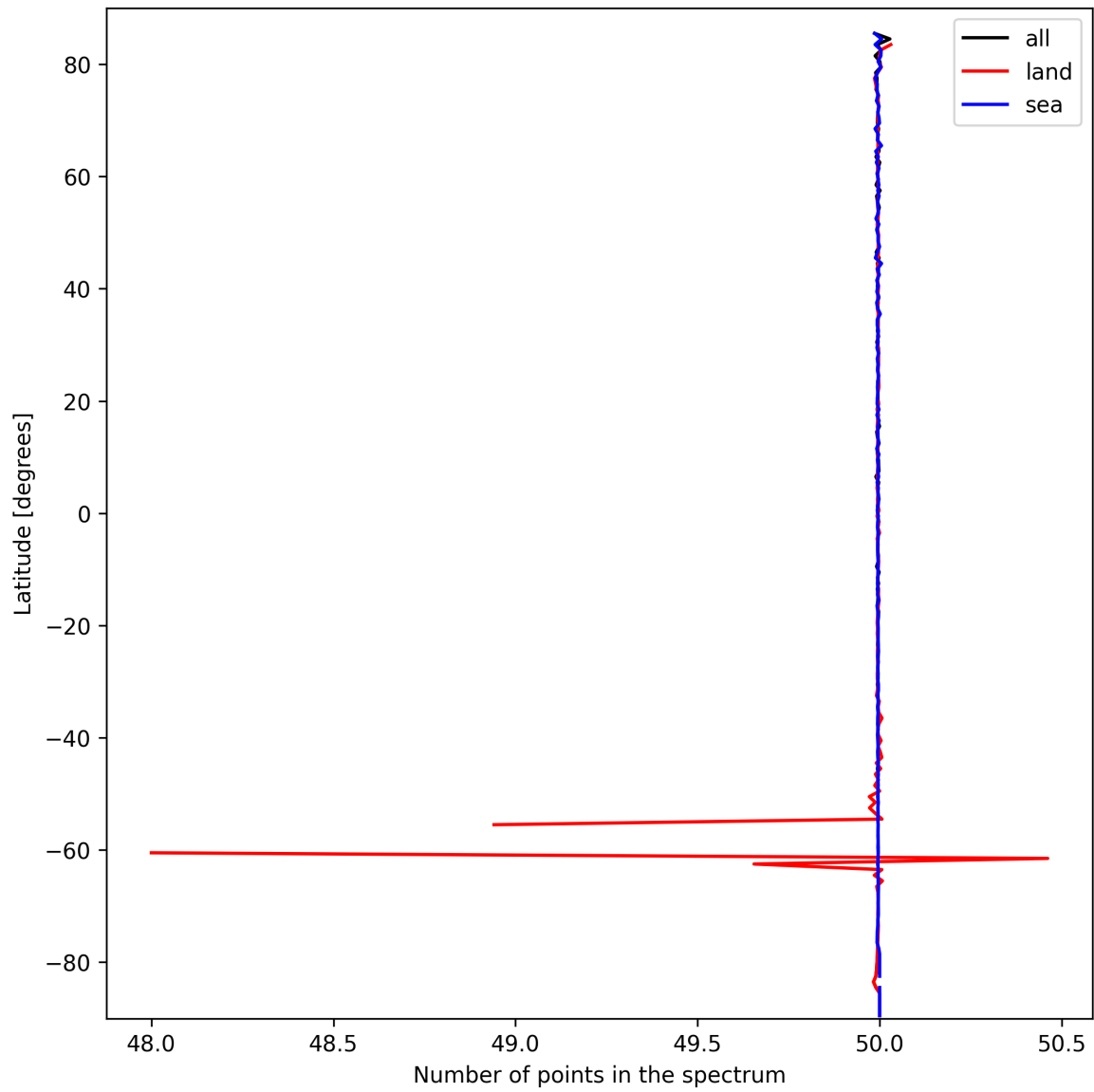
Figure 27: Zonal average of “Number of points in the spectrum” for 2025-03-12 to 2025-03-14.
