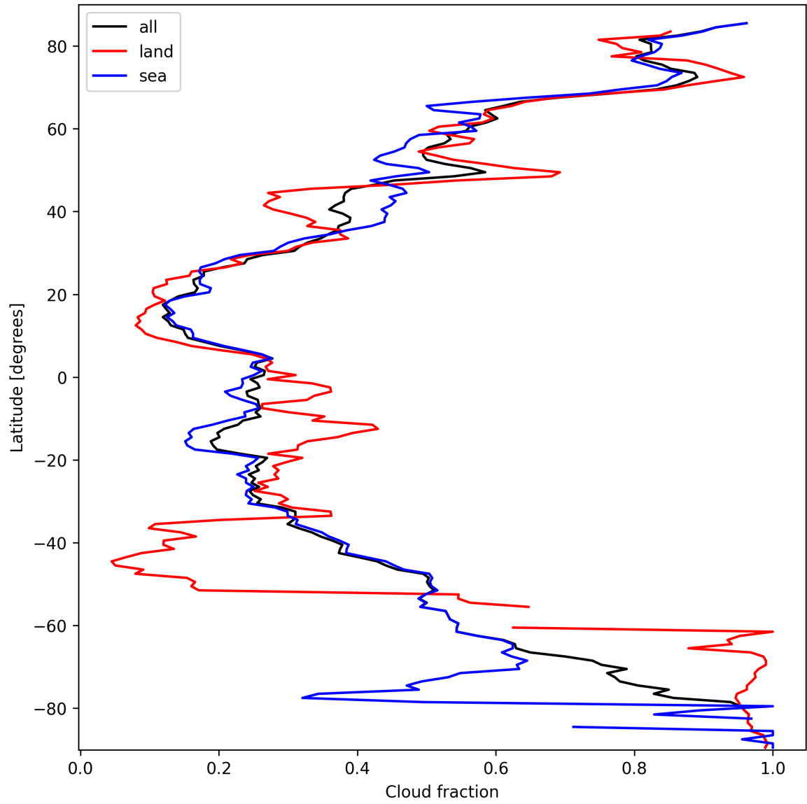
Figure 15: Zonal average of “Cloud fraction” for 2025-03-12 to 2025-03-14.
