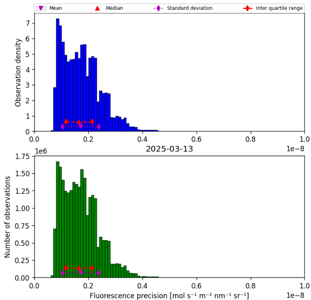
Figure 41: Histogram of “Fluorescence precision” for 2025-03-12 to 2025-03-14
