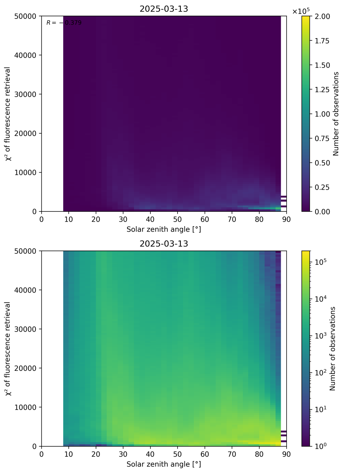
Figure 109: Scatter density plot of “Solar zenith angle” against “ \chi^2 of fluorescence retrieval” for 2025-03-12 to 2025-03-14.
