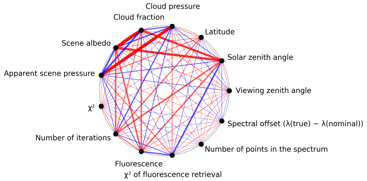
Figure 1: Map of correlation graph for 2025-03-12 to 2025-03-14.
