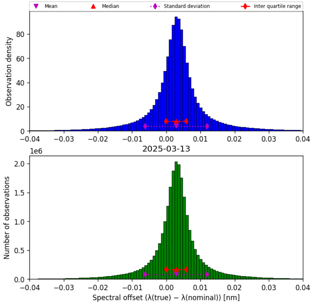
Figure 45: Histogram of “Spectral offset ( \lambda_{\text{true}} - \lambda_{\text{nominal}} )” for 2025-03-12 to 2025-03-14
