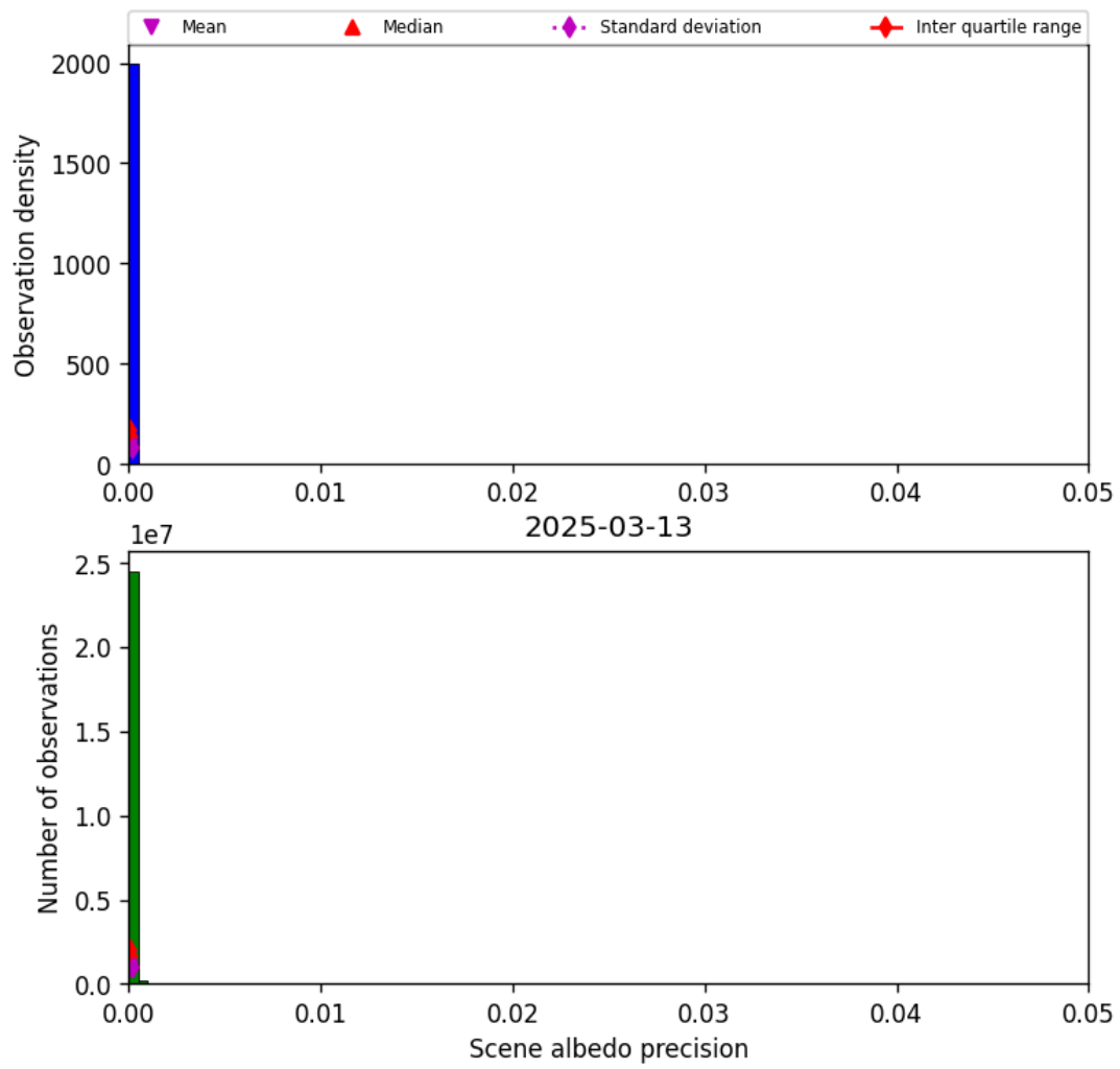
Figure 35: Histogram of “Scene albedo precision” for 2025-03-12 to 2025-03-14
