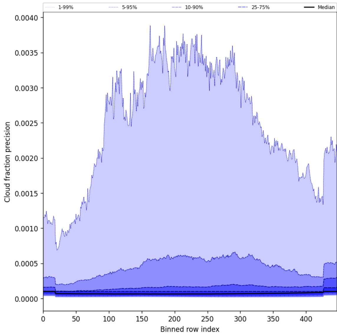
Figure 50: Along track statistics of “Cloud fraction precision” for 2025-03-12 to 2025-03-14
