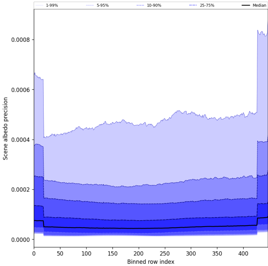
Figure 52: Along track statistics of “Scene albedo precision” for 2025-03-12 to 2025-03-14
