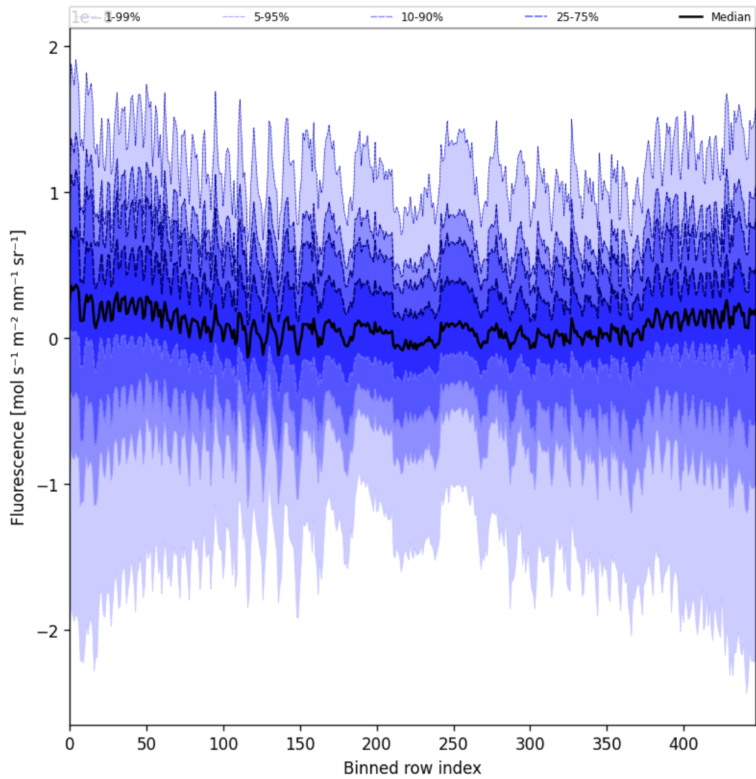
Figure 57: Along track statistics of “Fluorescence” for 2025-03-12 to 2025-03-14
