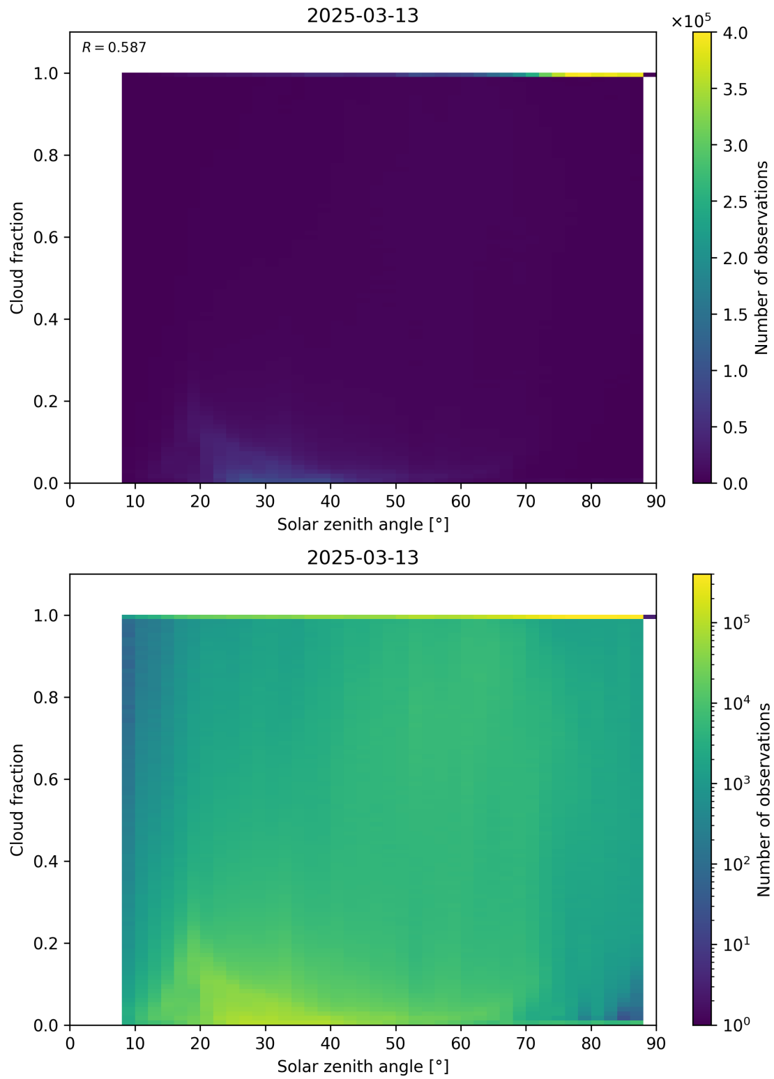
Figure 110: Scatter density plot of “Solar zenith angle” against “Cloud fraction” for 2025-03-12 to 2025-03-14.
