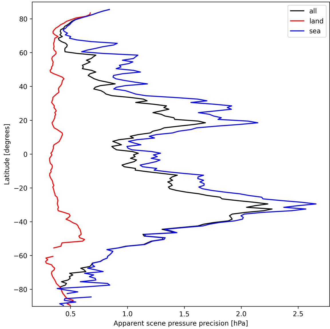
Figure 20: Zonal average of “Apparent scene pressure precision” for 2025-03-12 to 2025-03-14.
