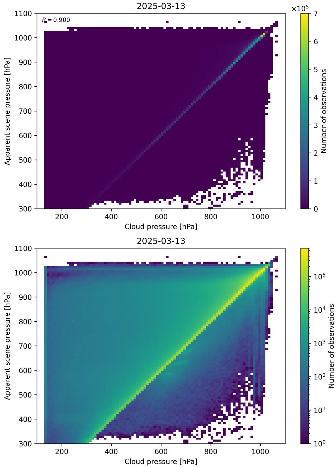
Figure 77: Scatter density plot of “Cloud pressure” against “Apparent scene pressure” for 2025-03-12 to 2025-03-14.
