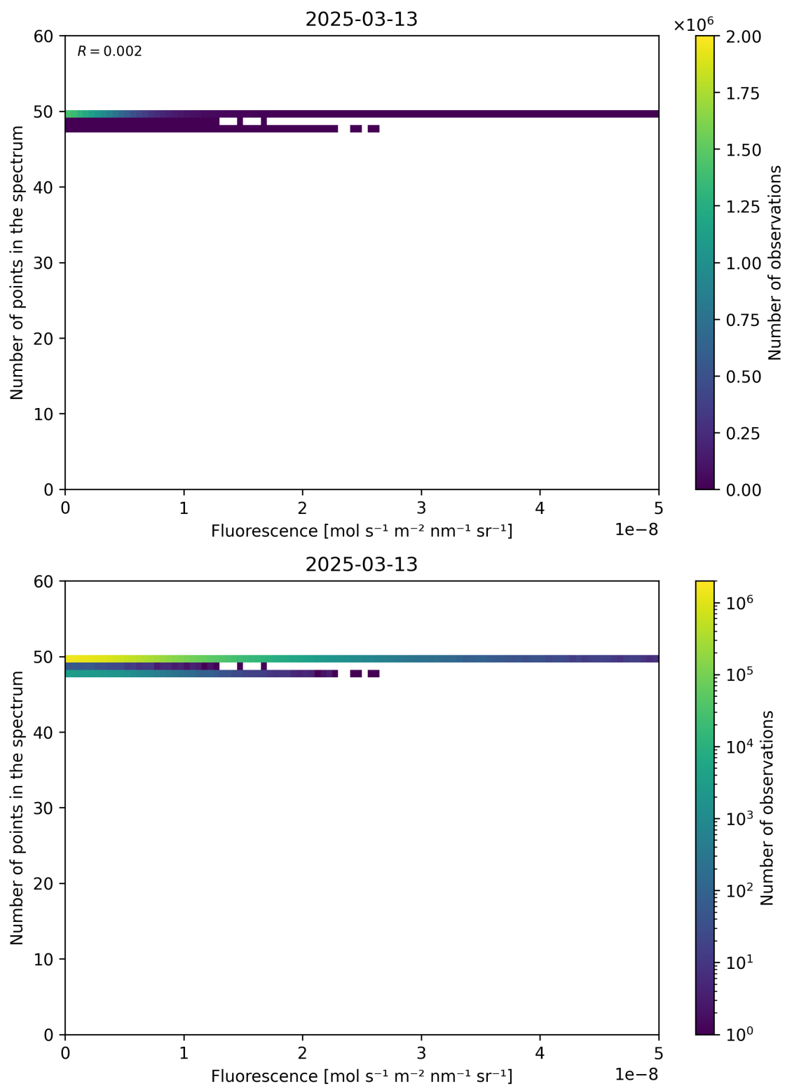
Figure 86: Scatter density plot of “Fluorescence” against “Number of points in the spectrum” for 2025-03-12 to 2025-03-14.
