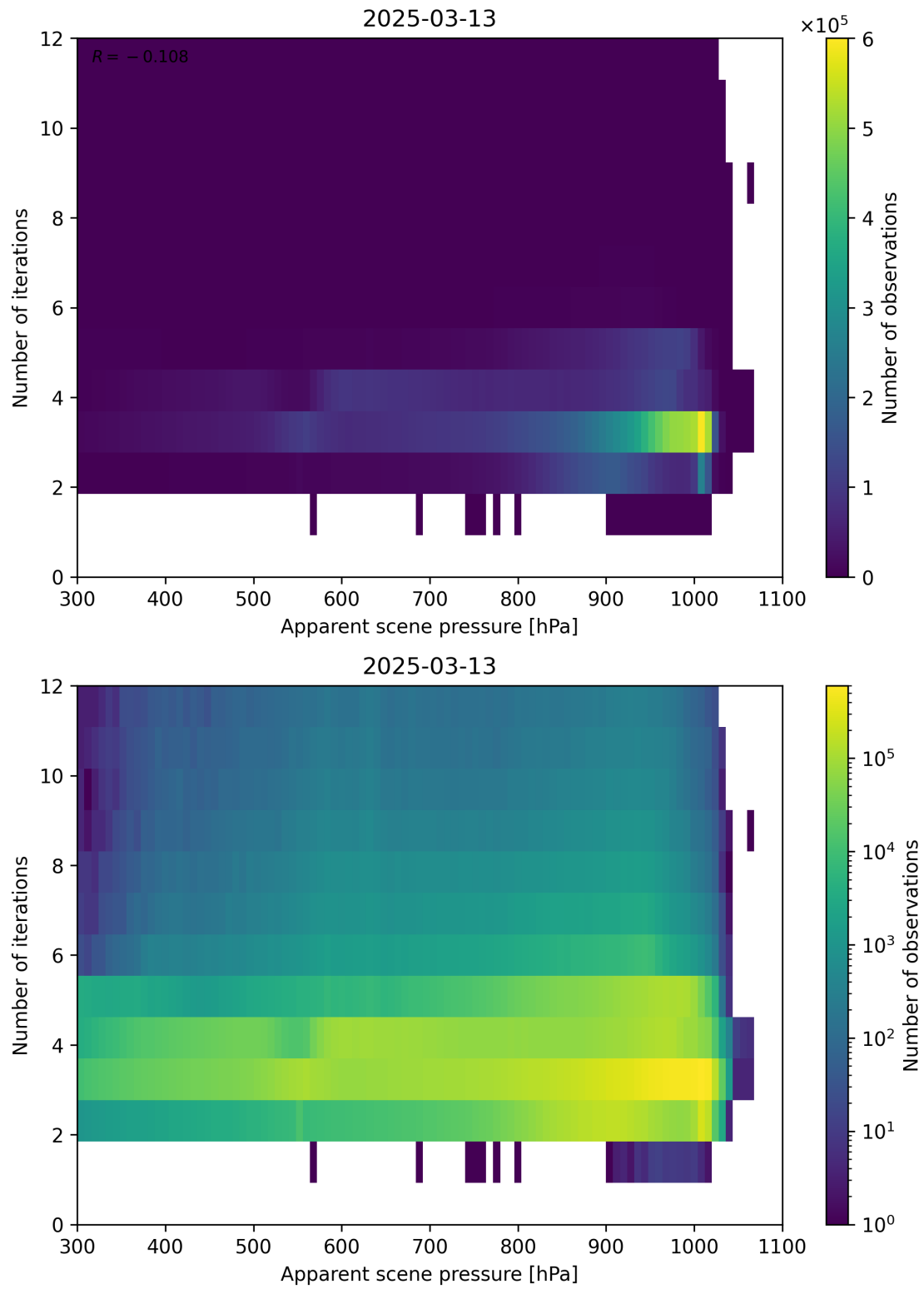
Figure 65: Scatter density plot of “Apparent scene pressure” against “Number of iterations” for 2025-03-12 to 2025-03-14.
