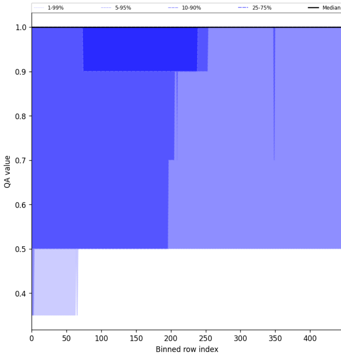
Figure 46: Along track statistics of “QA value” for 2025-03-12 to 2025-03-14
