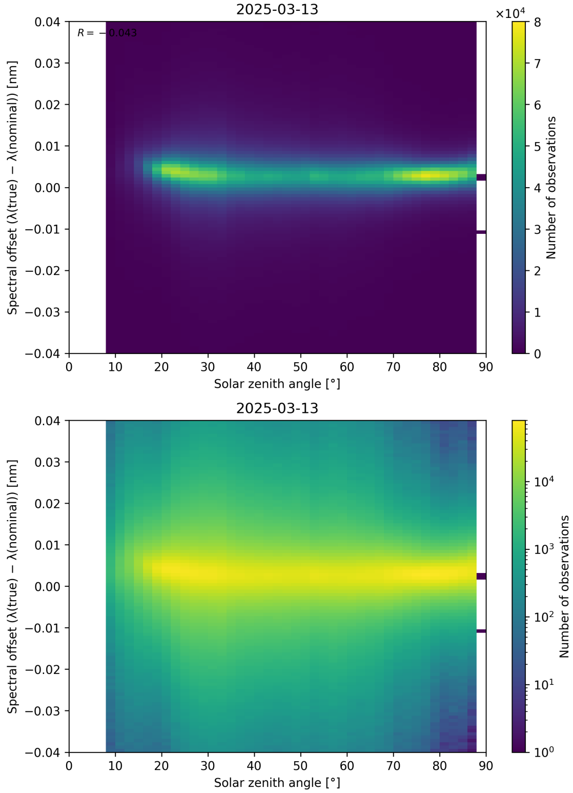
Figure 117: Scatter density plot of “Solar zenith angle” against “Spectral offset ( \lambda_{\text{true}} - \lambda_{\text{nominal}} )” for 2025-03-12 to 2025-03-14.
