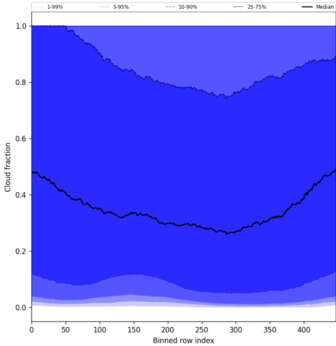
Figure 49: Along track statistics of “Cloud fraction” for 2025-03-12 to 2025-03-14
