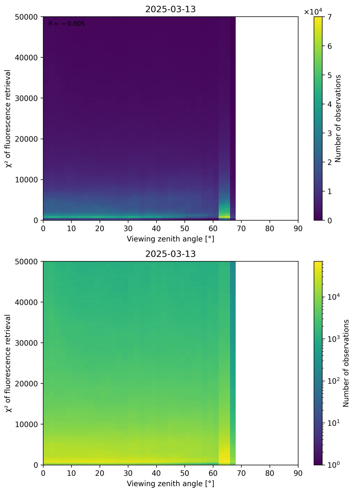
Figure 119: Scatter density plot of “Viewing zenith angle” against “ \chi^2 of fluorescence retrieval” for 2025-03-12 to 2025-03-14.
