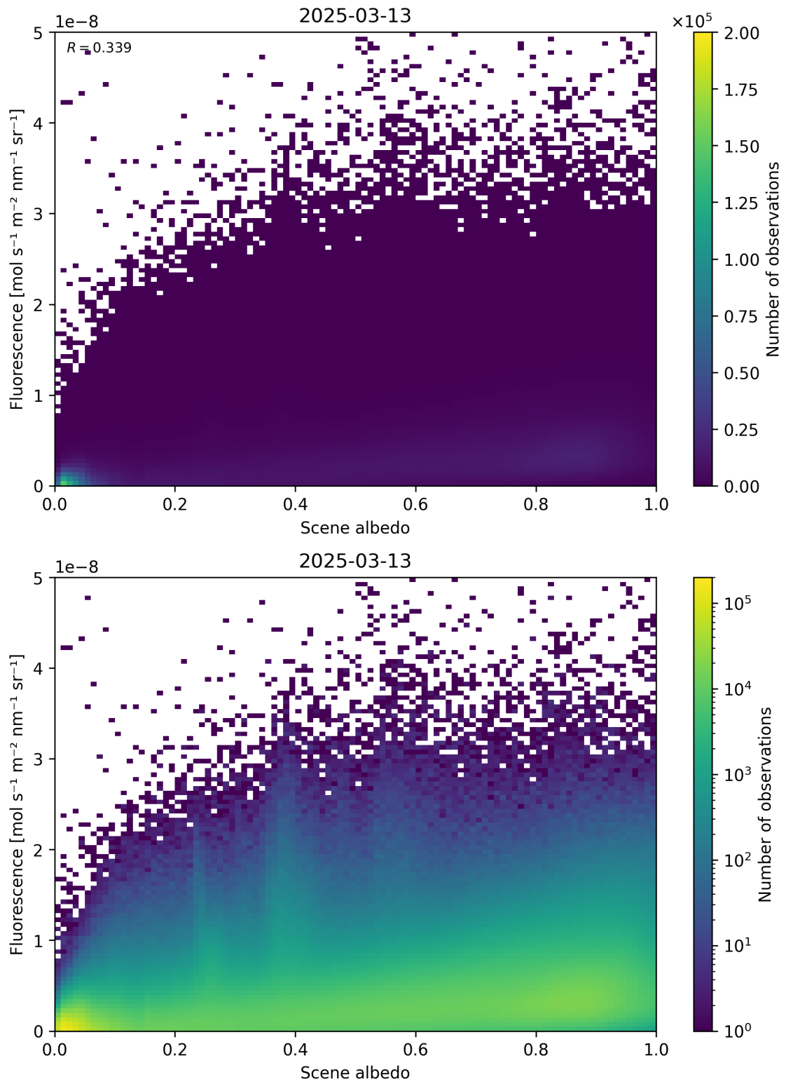
Figure 104: Scatter density plot of “Scene albedo” against “Fluorescence” for 2025-03-12 to 2025-03-14.
