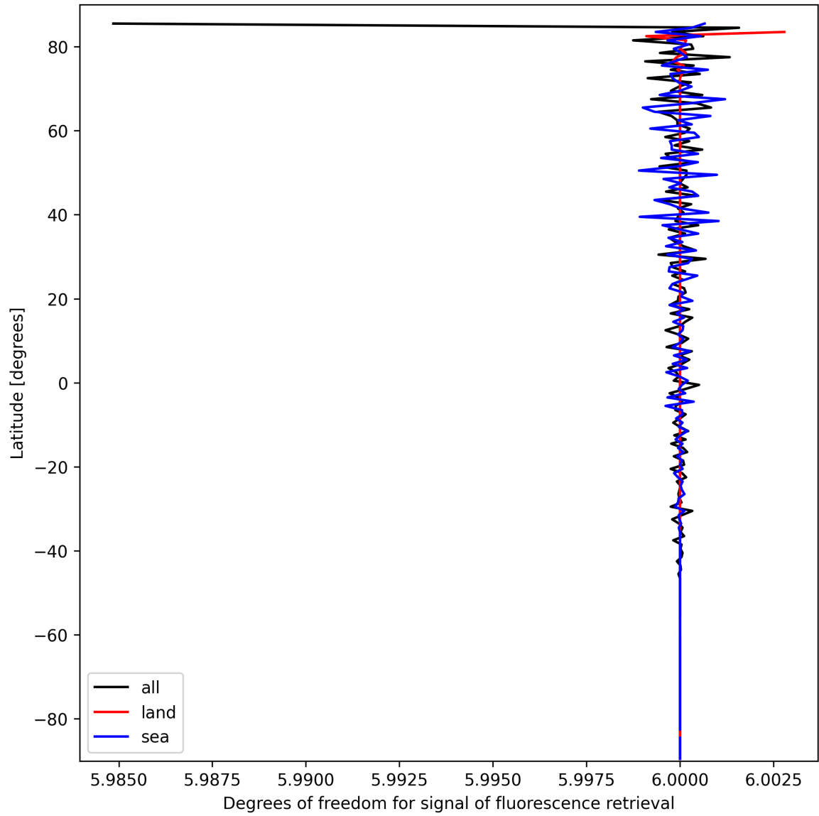
Figure 26: Zonal average of “Degrees of freedom for signal of fluorescence retrieval” for 2025-03-12 to 2025-03-14.
