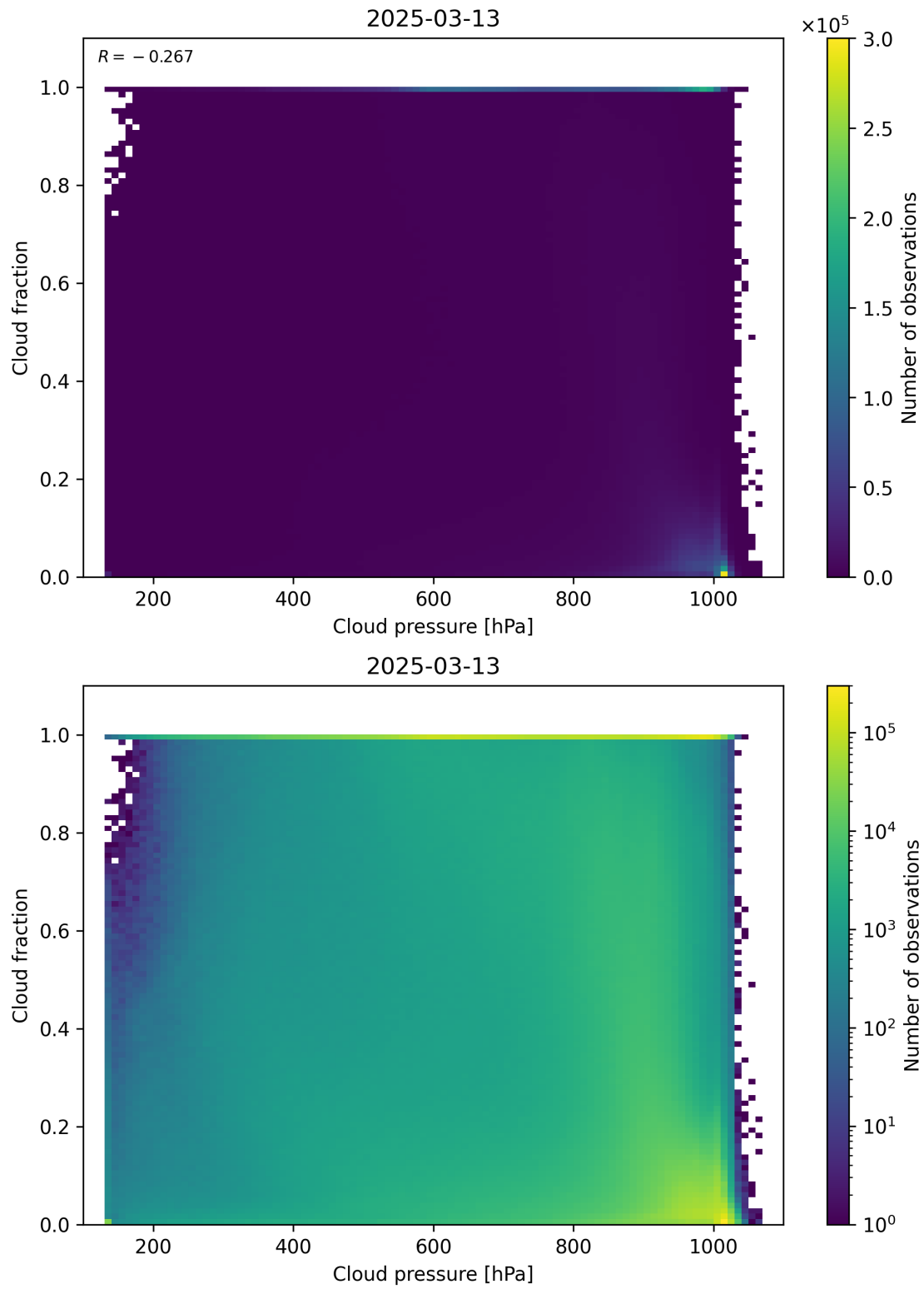
Figure 79: Scatter density plot of “Cloud pressure” against “Cloud fraction” for 2025-03-12 to 2025-03-14.
