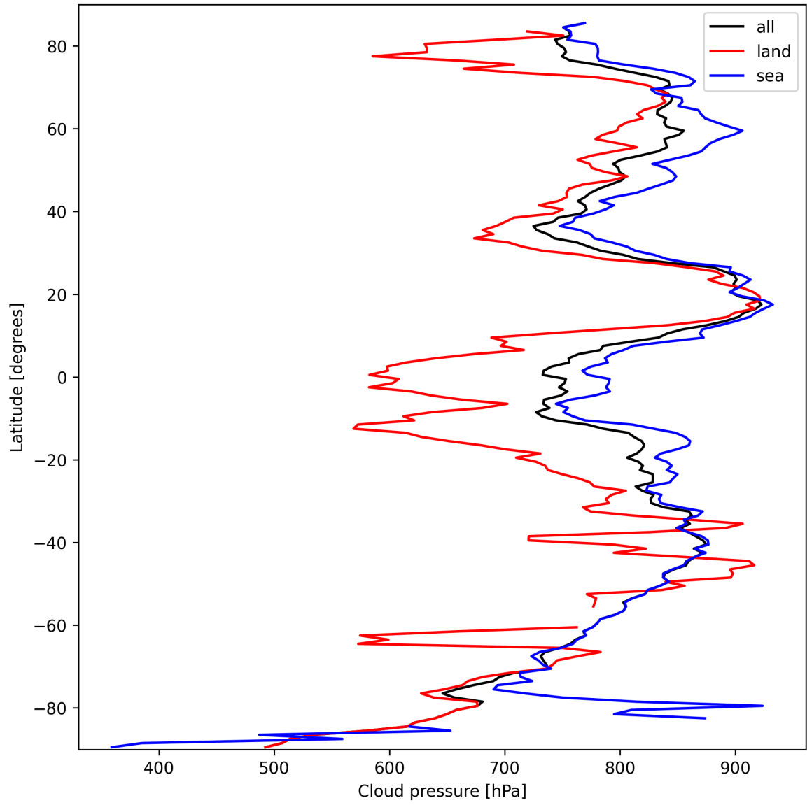
Figure 13: Zonal average of “Cloud pressure” for 2025-03-12 to 2025-03-14.
