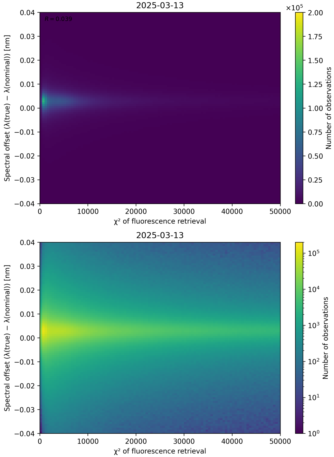
Figure 69: Scatter density plot of “ \chi^2 of fluorescence retrieval” against “Spectral offset ( \lambda_{\text{true}} - \lambda_{\text{nominal}} )” for 2025-03-12 to 2025-03-14.
