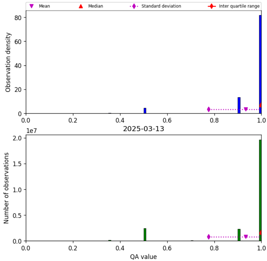
Figure 29: Histogram of “QA value” for 2025-03-12 to 2025-03-14
