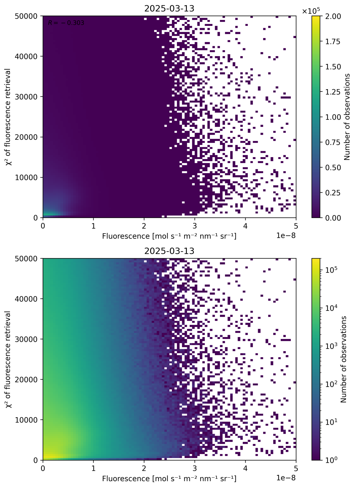
Figure 85: Scatter density plot of “Fluorescence” against “ \chi^2 of fluorescence retrieval” for 2025-03-12 to 2025-03-14.
