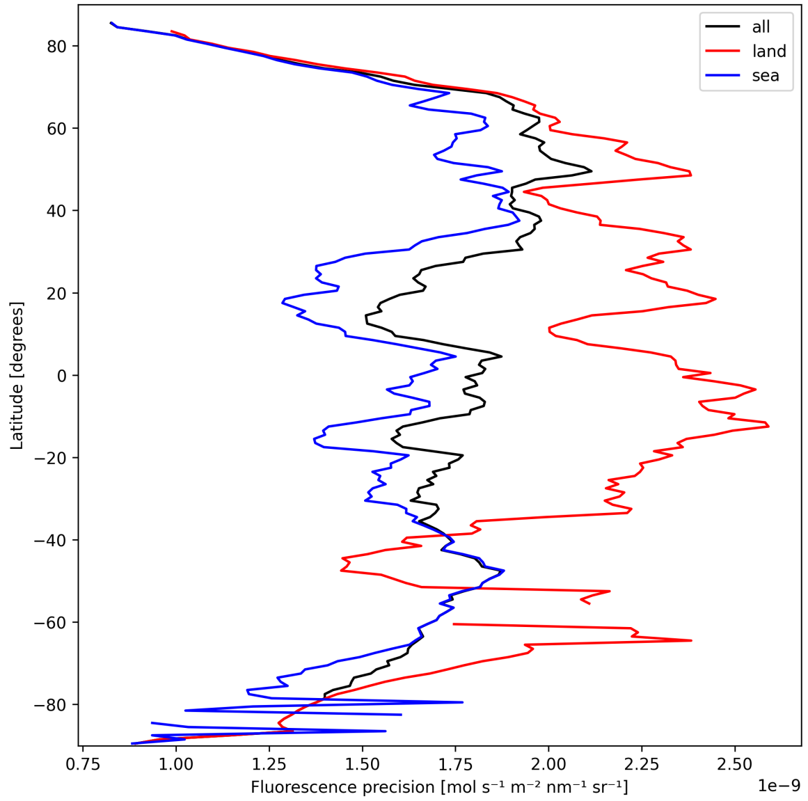
Figure 24: Zonal average of “Fluorescence precision” for 2025-03-12 to 2025-03-14.
