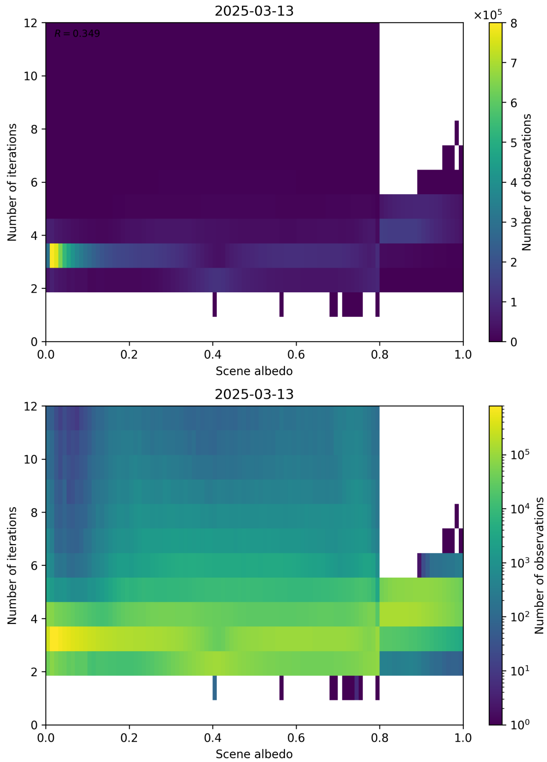
Figure 105: Scatter density plot of “Scene albedo” against “Number of iterations” for 2025-03-12 to 2025-03-14.
