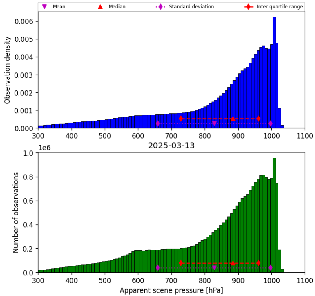
Figure 36: Histogram of “Apparent scene pressure” for 2025-03-12 to 2025-03-14
