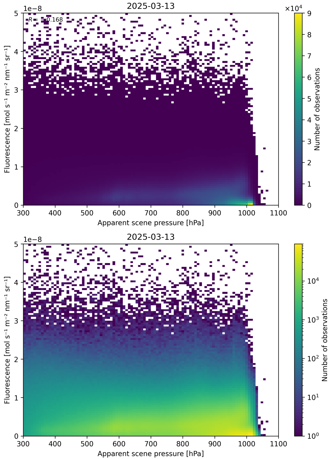
Figure 64: Scatter density plot of “Apparent scene pressure” against “Fluorescence” for 2025-03-12 to 2025-03-14.
