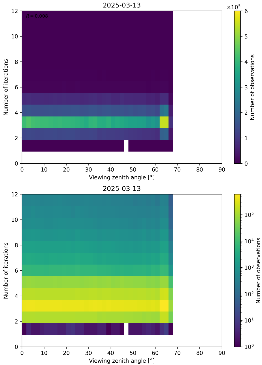
Figure 124: Scatter density plot of “Viewing zenith angle” against “Number of iterations” for 2025-03-12 to 2025-03-14.
