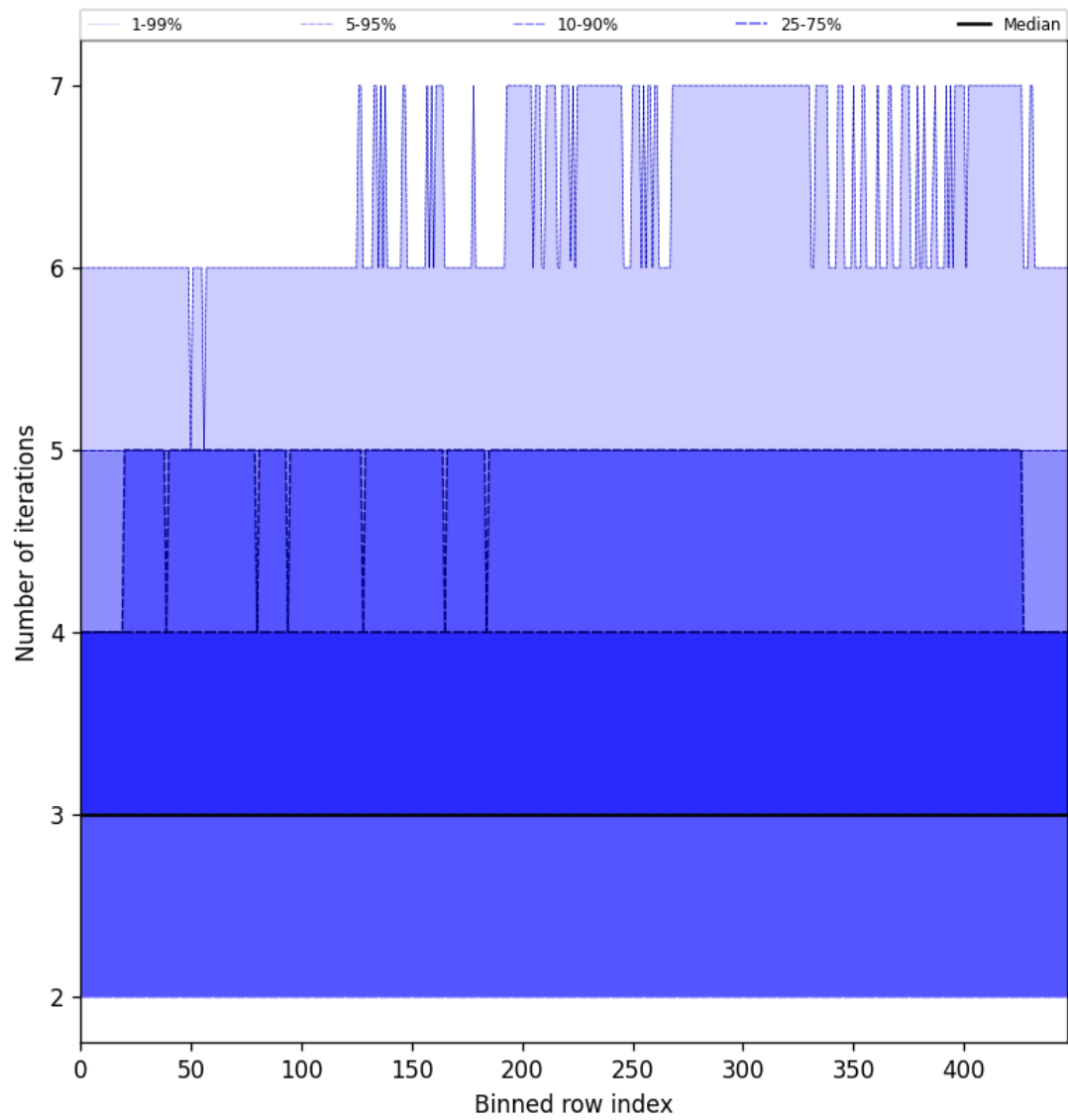
Figure 56: Along track statistics of “Number of iterations” for 2025-03-12 to 2025-03-14
