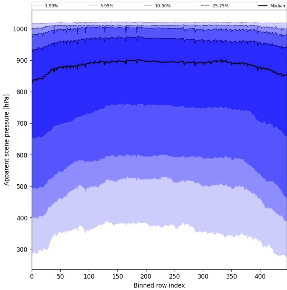
Figure 53: Along track statistics of “Apparent scene pressure” for 2025-03-12 to 2025-03-14
