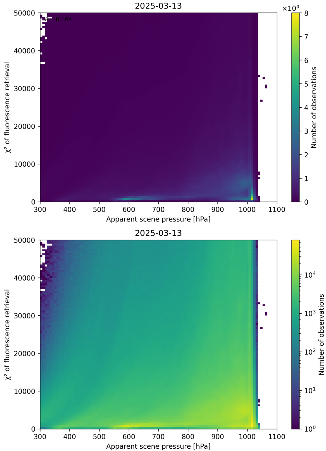
Figure 63: Scatter density plot of “Apparent scene pressure” against “ \chi^2 of fluorescence retrieval” for 2025-03-12 to 2025-03-14.
