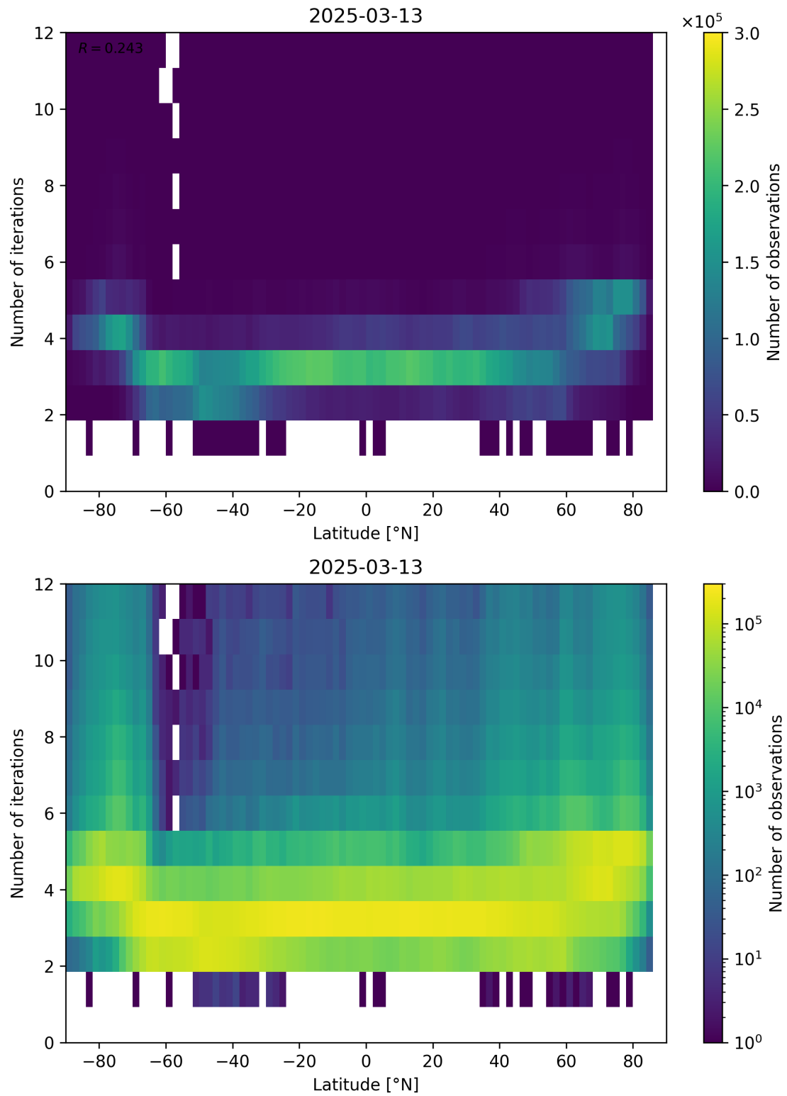
Figure 93: Scatter density plot of “Latitude” against “Number of iterations” for 2025-03-12 to 2025-03-14.
