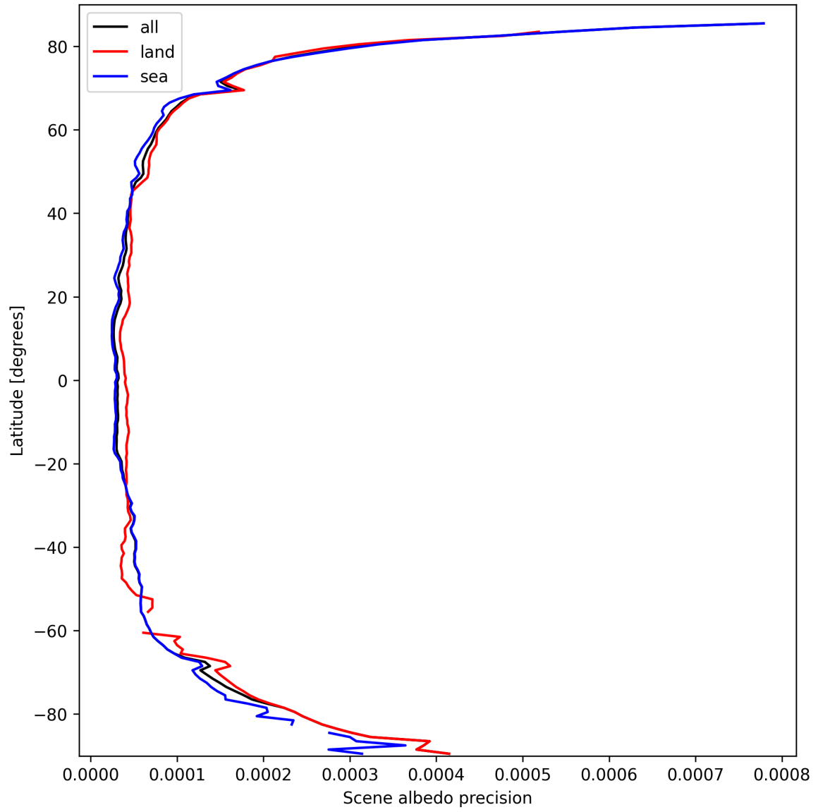
Figure 18: Zonal average of “Scene albedo precision” for 2025-03-12 to 2025-03-14.
