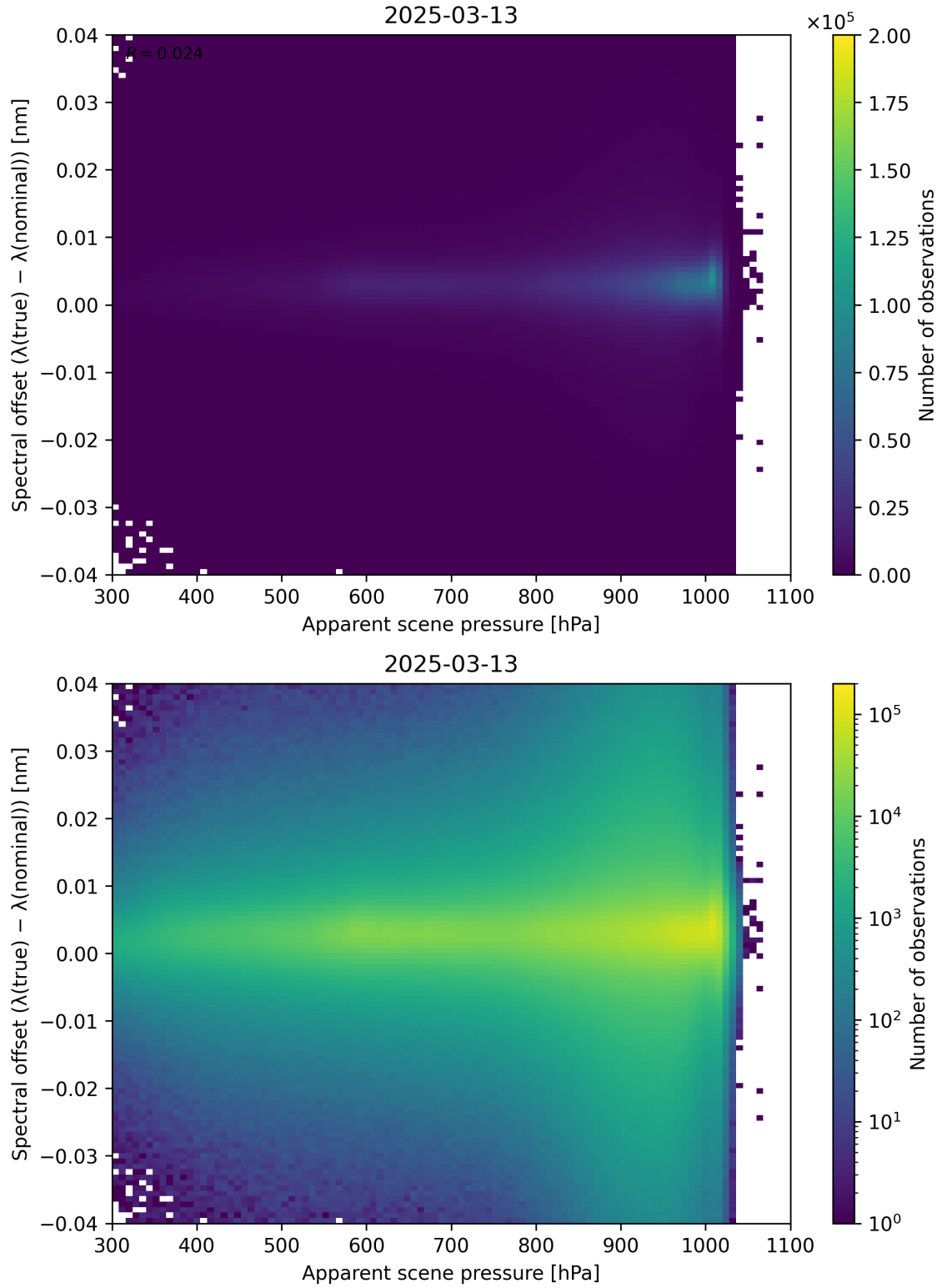
Figure 67: Scatter density plot of “Apparent scene pressure” against “Spectral offset ( \lambda_{\text{true}} - \lambda_{\text{nominal}} )” for 2025-03-12 to 2025-03-14.
