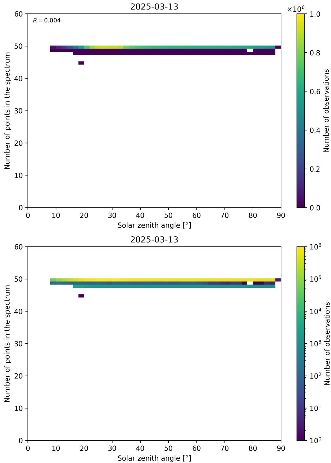
Figure 115: Scatter density plot of “Solar zenith angle” against “Number of points in the spectrum” for 2025-03-12 to 2025-03-14.
