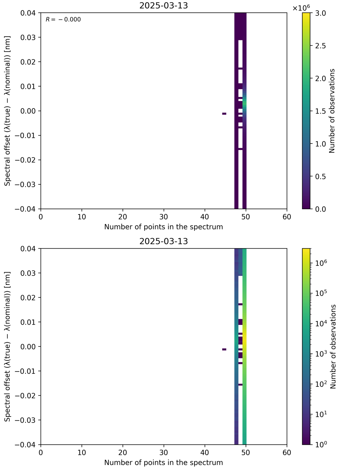
Figure 101: Scatter density plot of “Number of points in the spectrum” against “Spectral offset ( \lambda_{\text{true}} - \lambda_{\text{nominal}} )” for 2025-03-12 to 2025-03-14.
