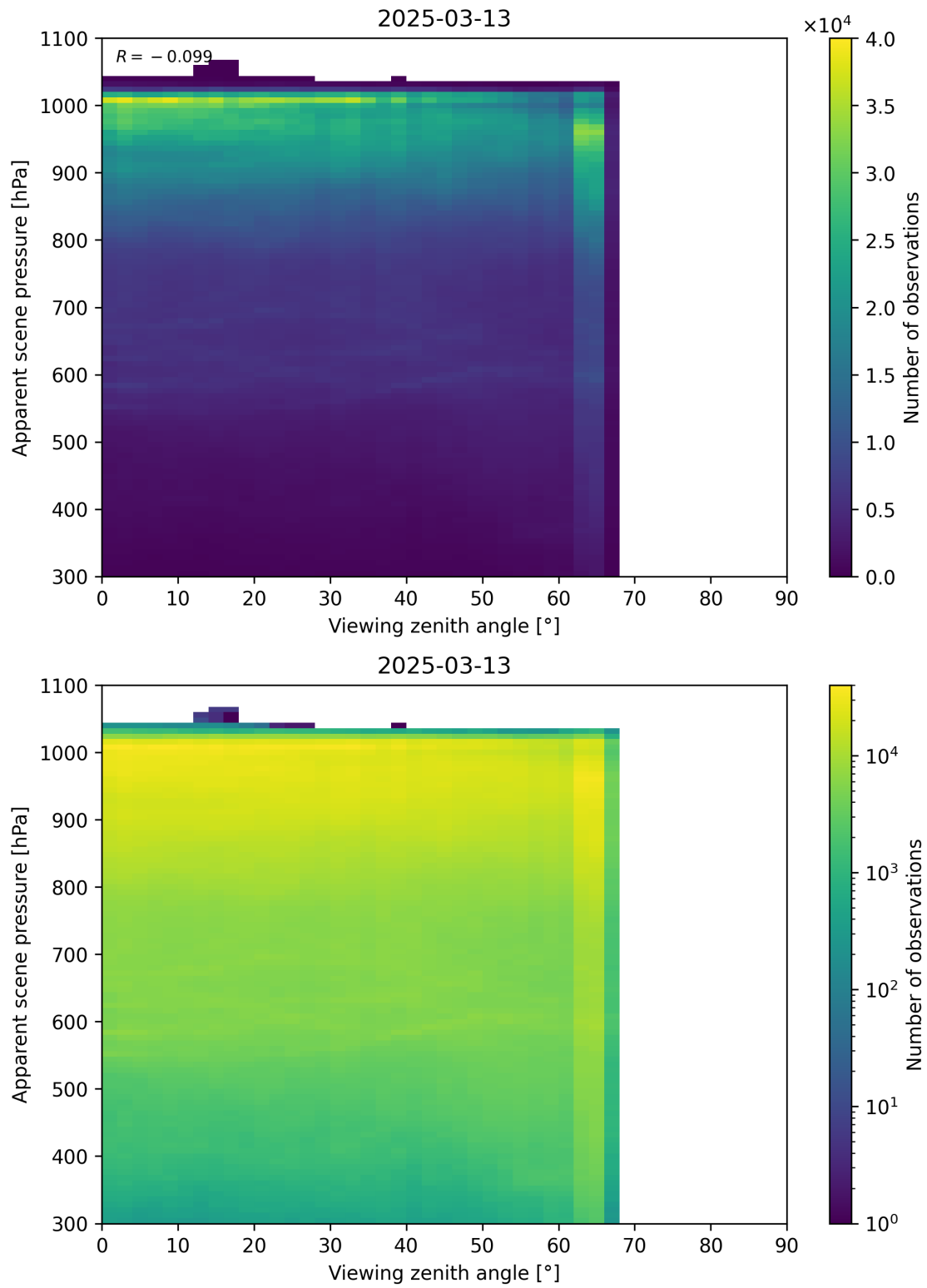
Figure 118: Scatter density plot of “Viewing zenith angle” against “Apparent scene pressure” for 2025-03-12 to 2025-03-14.
