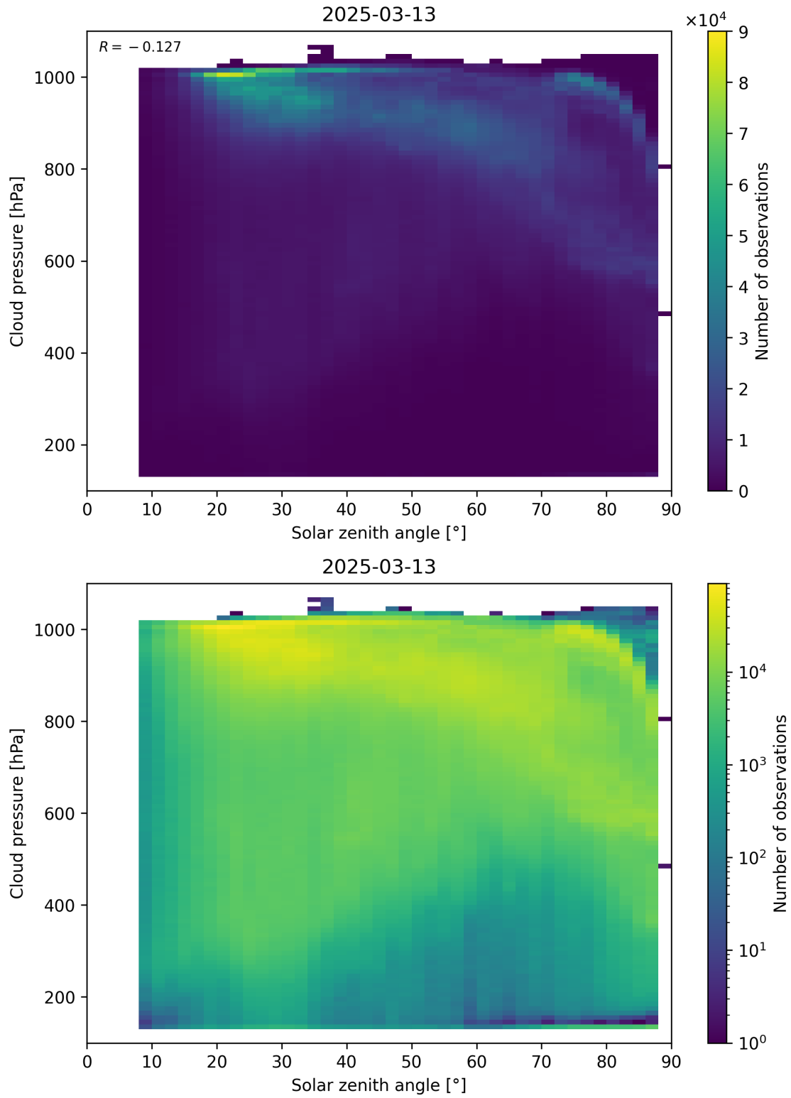
Figure 111: Scatter density plot of “Solar zenith angle” against “Cloud pressure” for 2025-03-12 to 2025-03-14.
