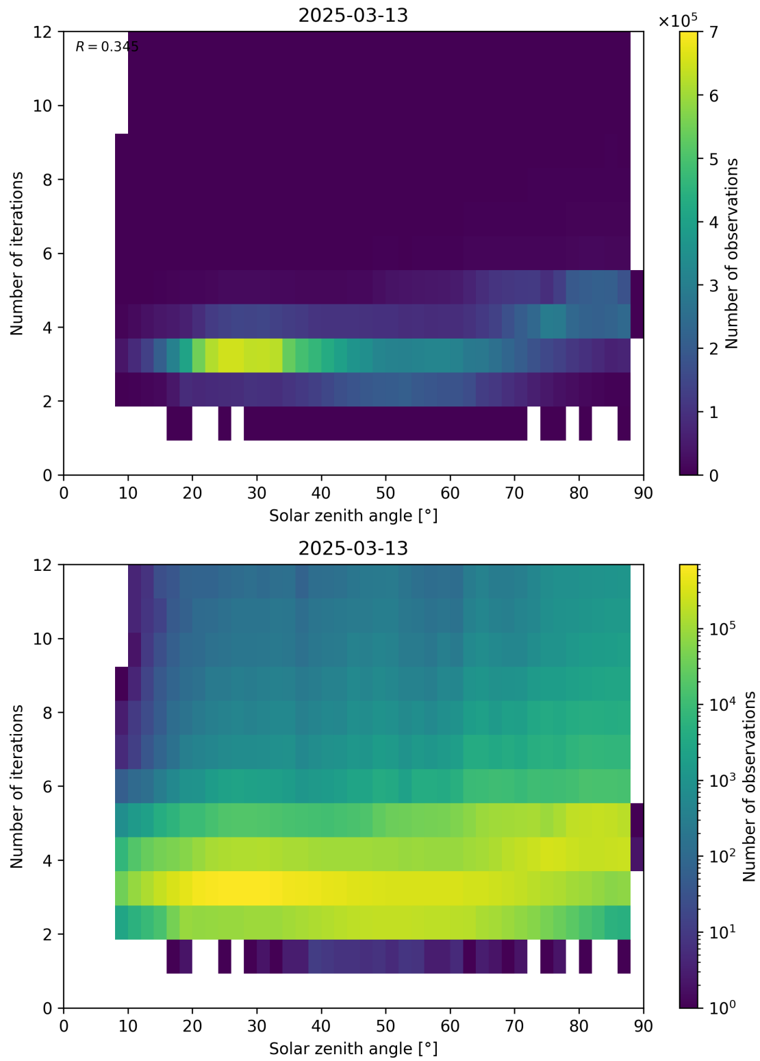
Figure 114: Scatter density plot of “Solar zenith angle” against “Number of iterations” for 2025-03-12 to 2025-03-14.
