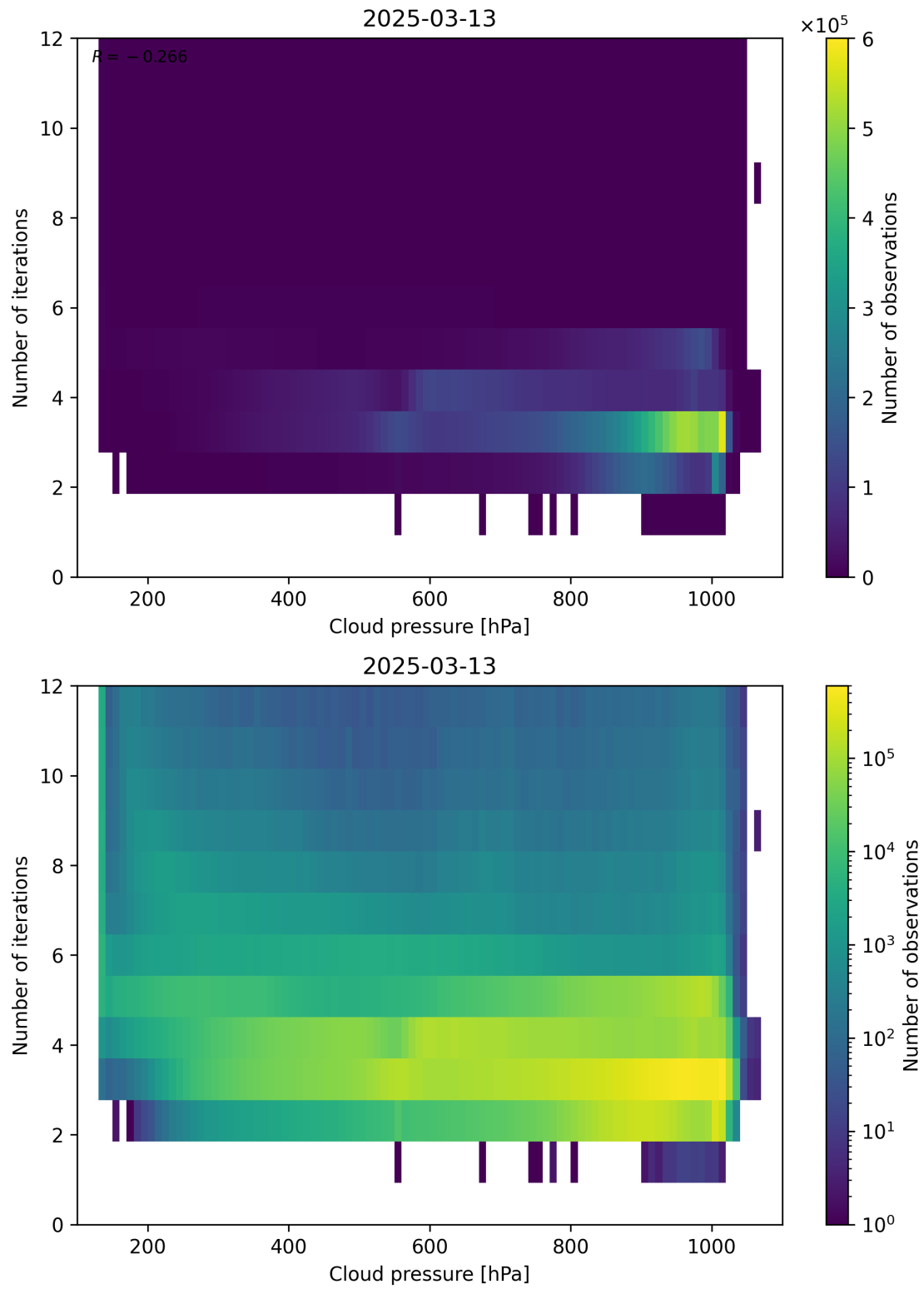
Figure 81: Scatter density plot of “Cloud pressure” against “Number of iterations” for 2025-03-12 to 2025-03-14.
