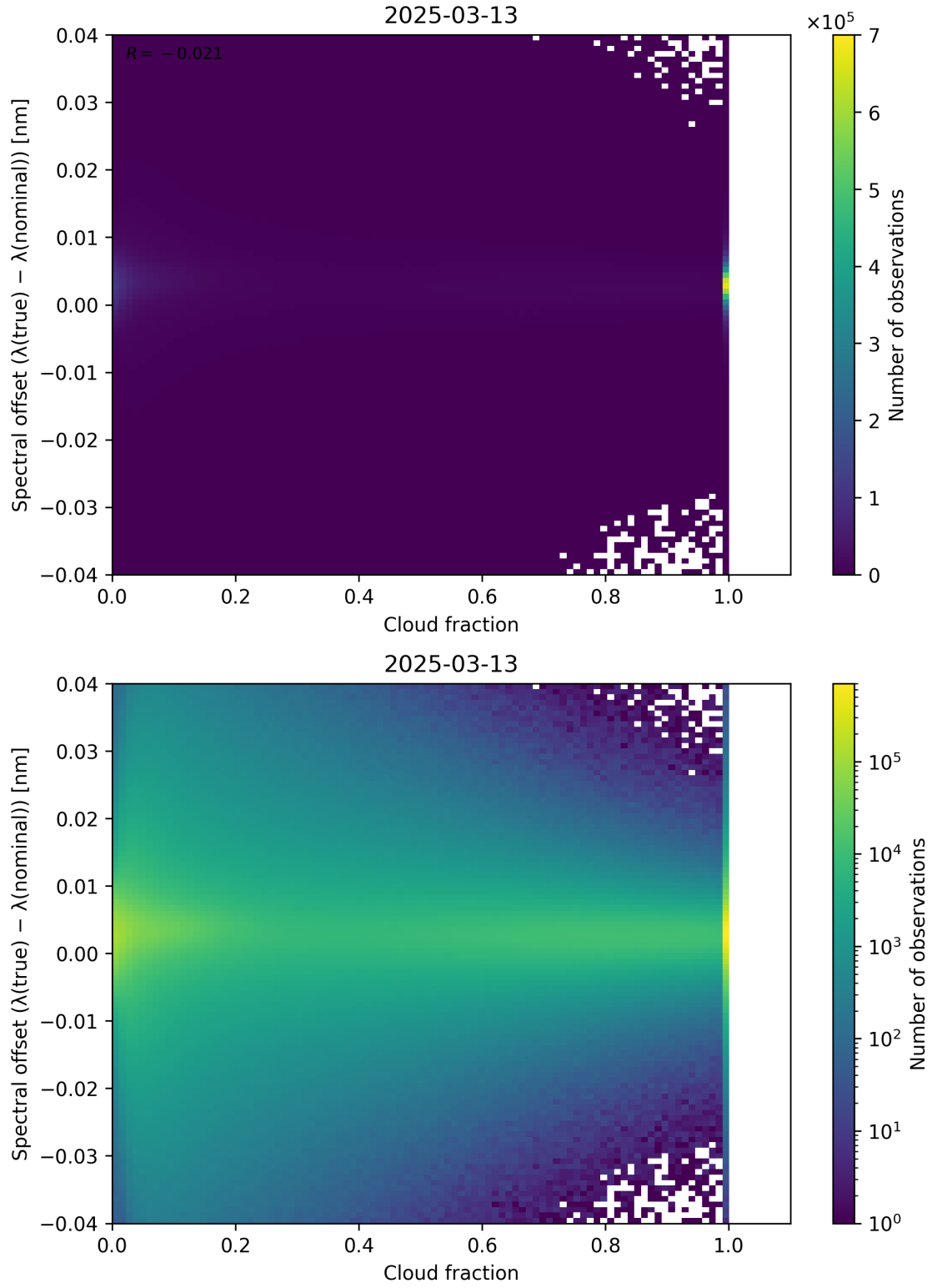
Figure 76: Scatter density plot of “Cloud fraction” against “Spectral offset ( \lambda_{\text{true}} - \lambda_{\text{nominal}} )” for 2025-03-12 to 2025-03-14.
