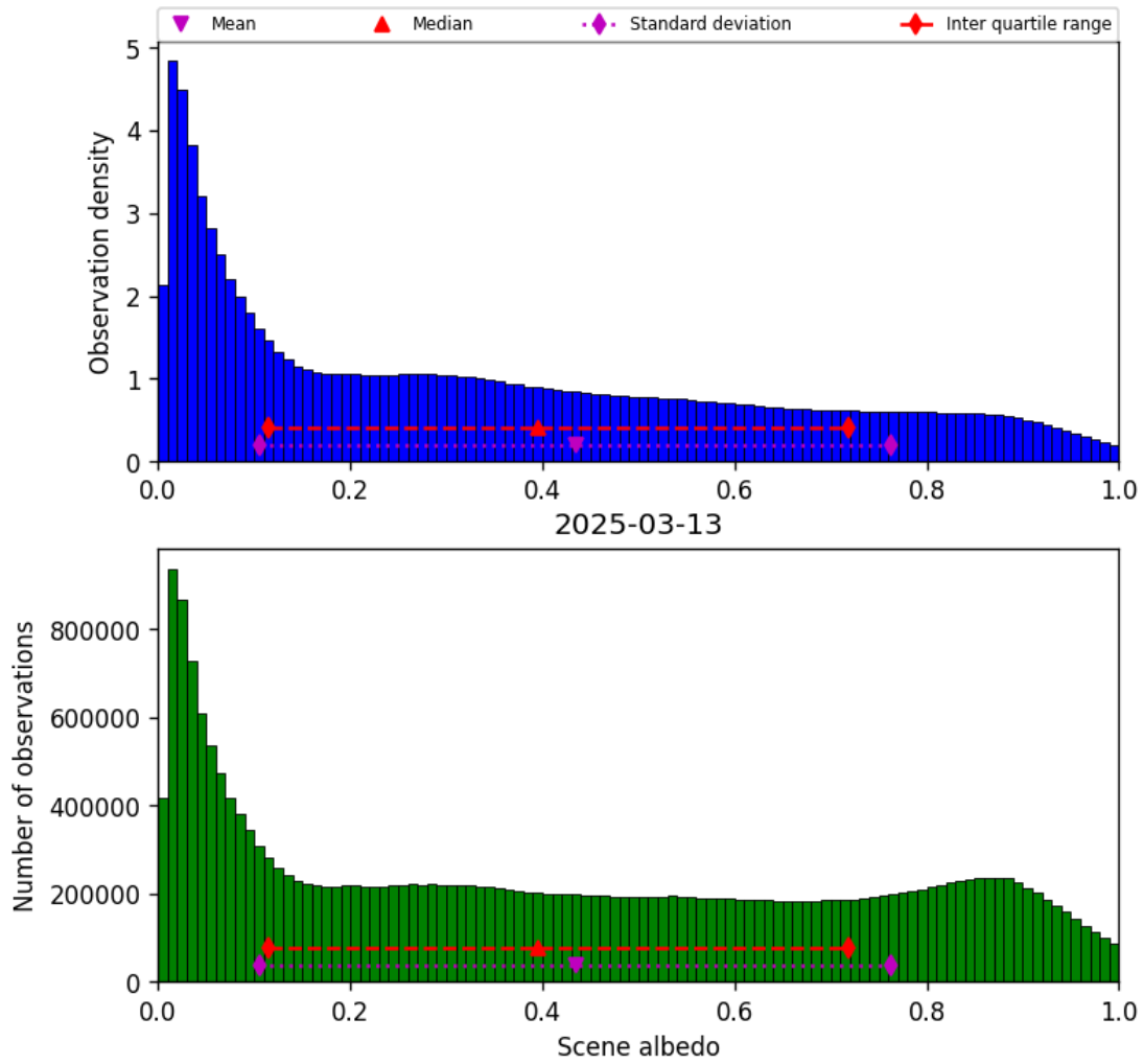
Figure 34: Histogram of “Scene albedo” for 2025-03-12 to 2025-03-14
