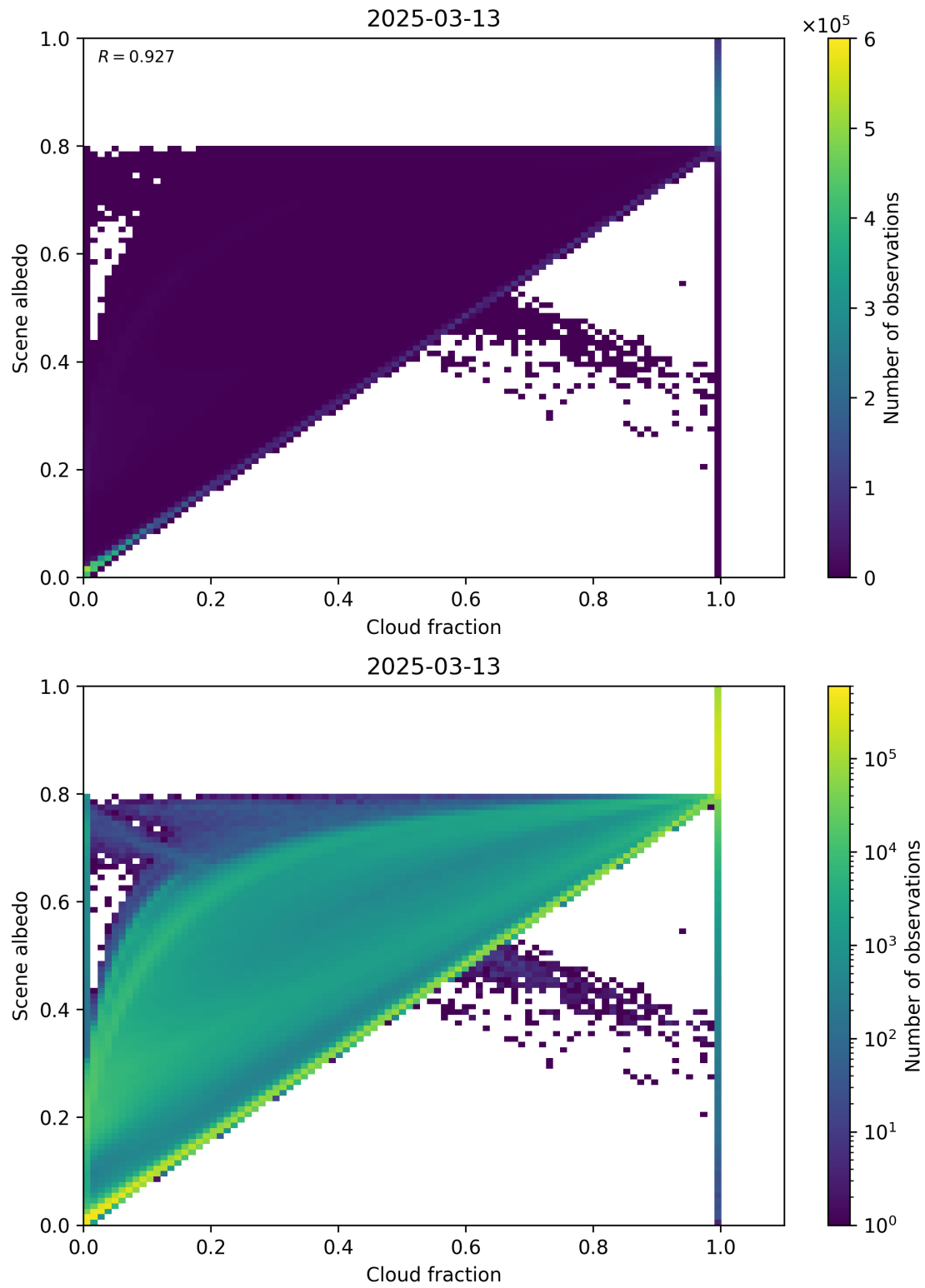
Figure 75: Scatter density plot of “Cloud fraction” against “Scene albedo” for 2025-03-12 to 2025-03-14.
