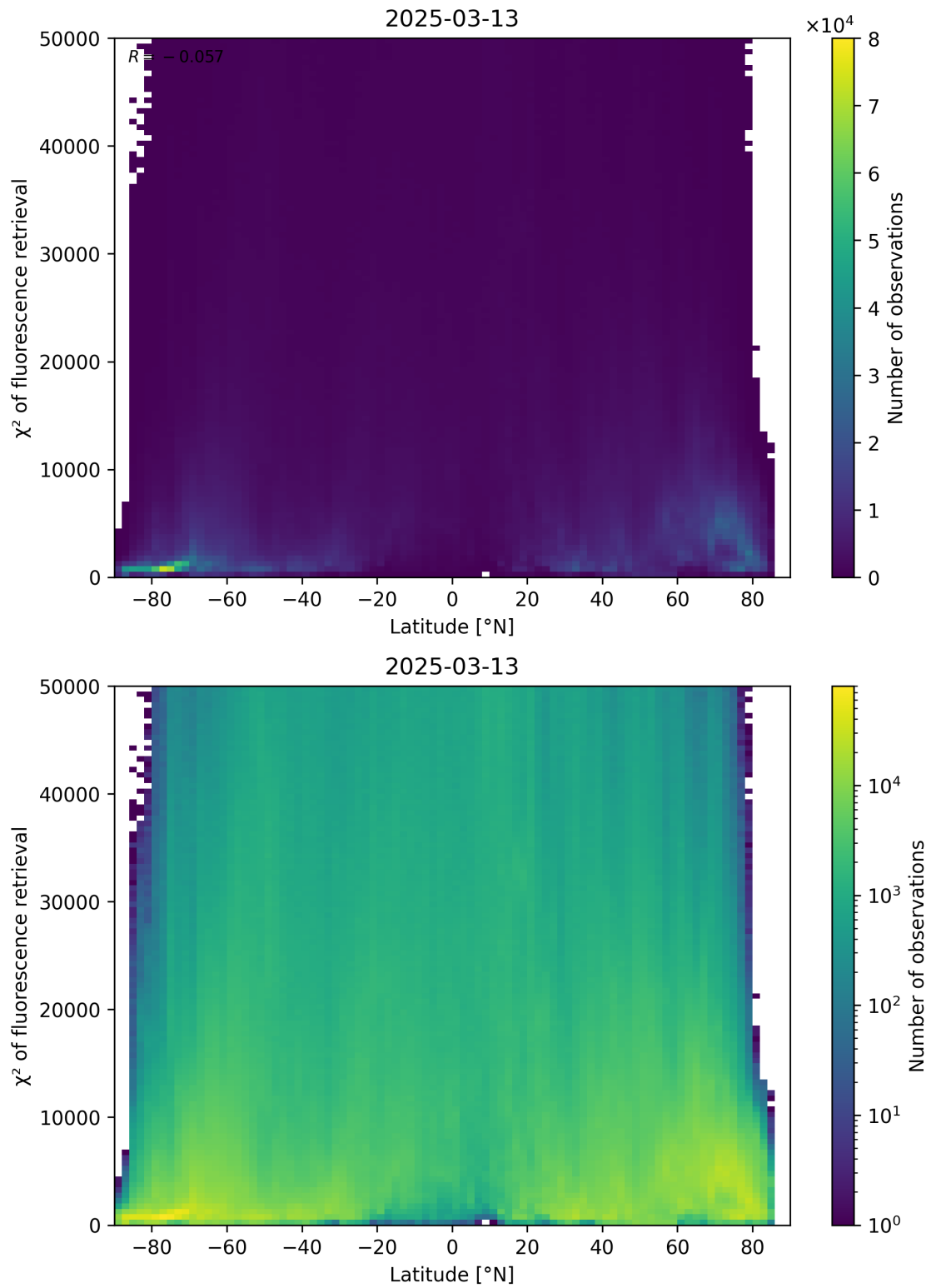
Figure 89: Scatter density plot of “Latitude” against “ \chi^2 of fluorescence retrieval” for 2025-03-12 to 2025-03-14.
