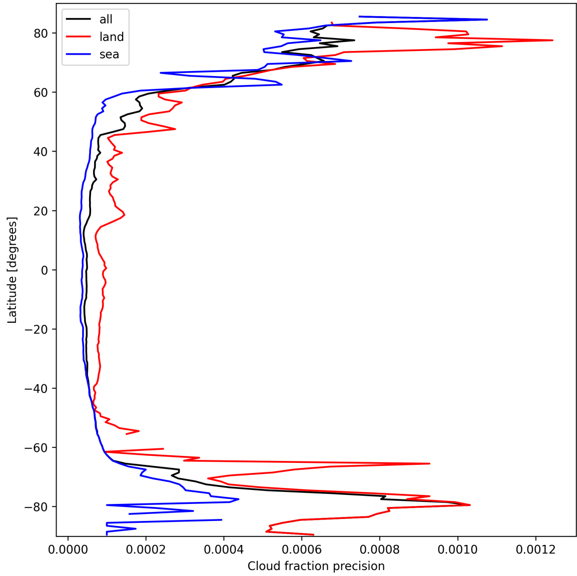
Figure 16: Zonal average of “Cloud fraction precision” for 2025-03-12 to 2025-03-14.
