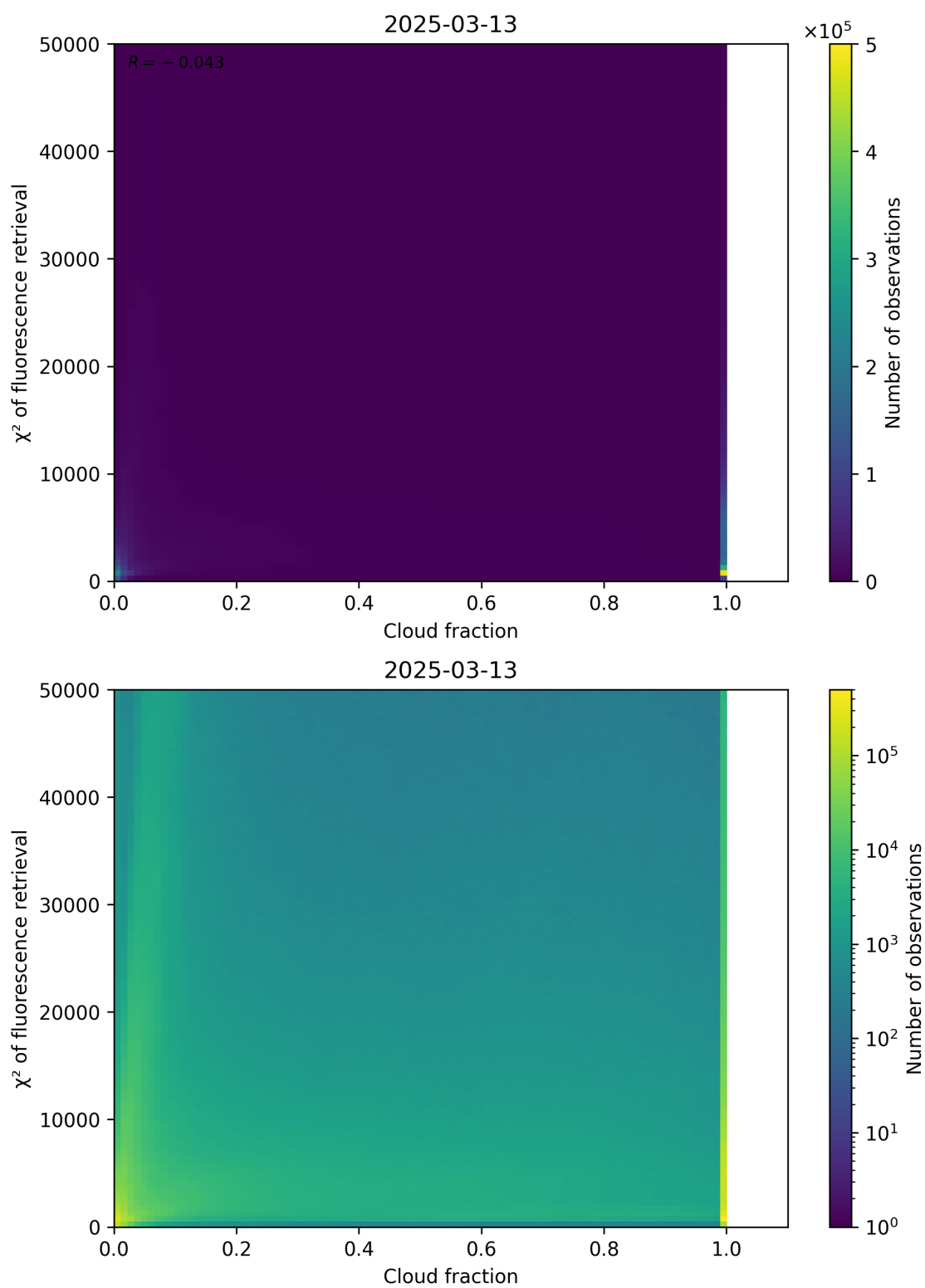
Figure 71: Scatter density plot of “Cloud fraction” against “ \chi^2 of fluorescence retrieval” for 2025-03-12 to 2025-03-14.
