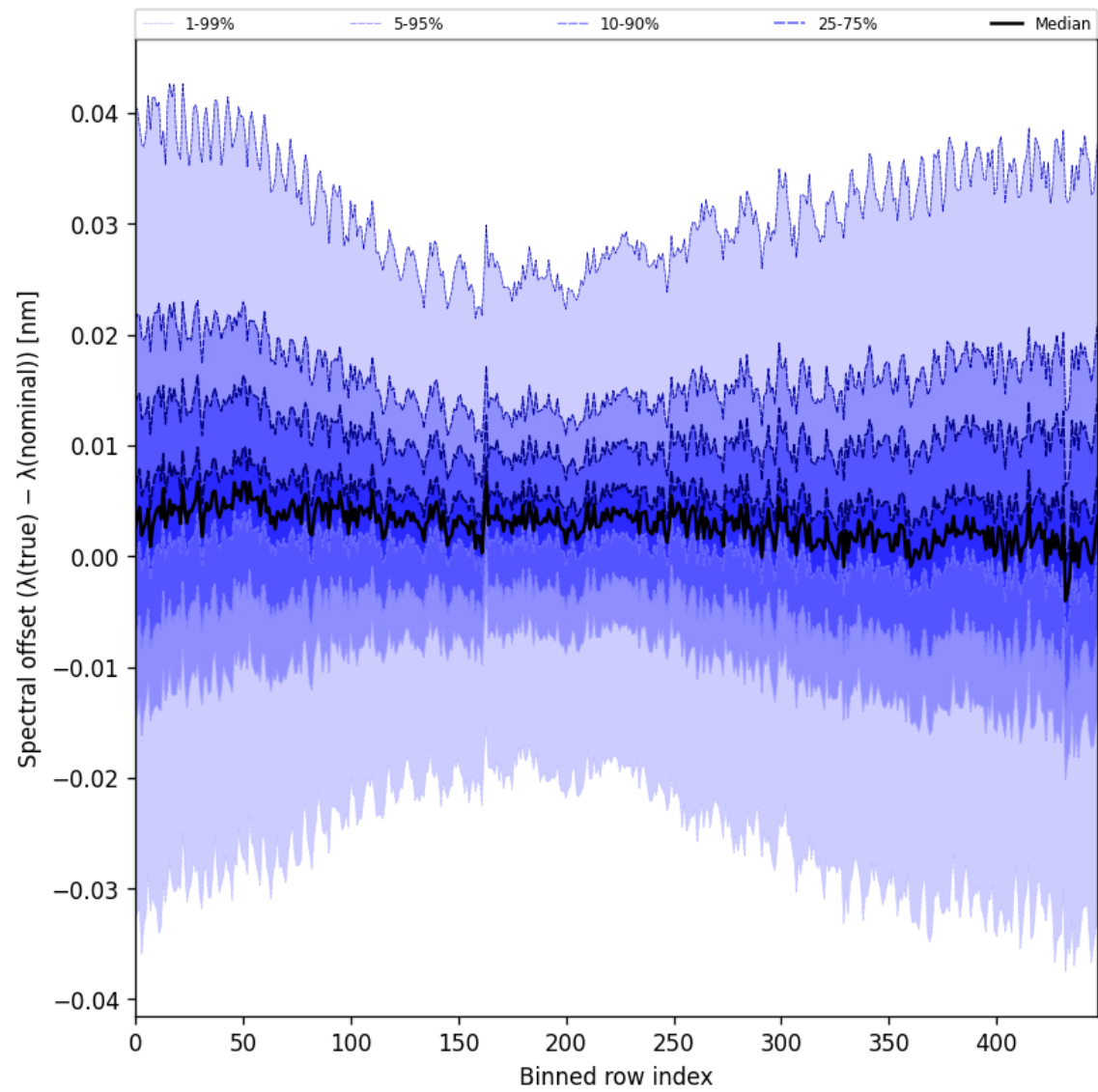
Figure 62: Along track statistics of “Spectral offset ( \lambda_{\text{true}} - \lambda_{\text{nominal}} )” for 2025-03-12 to 2025-03-14
