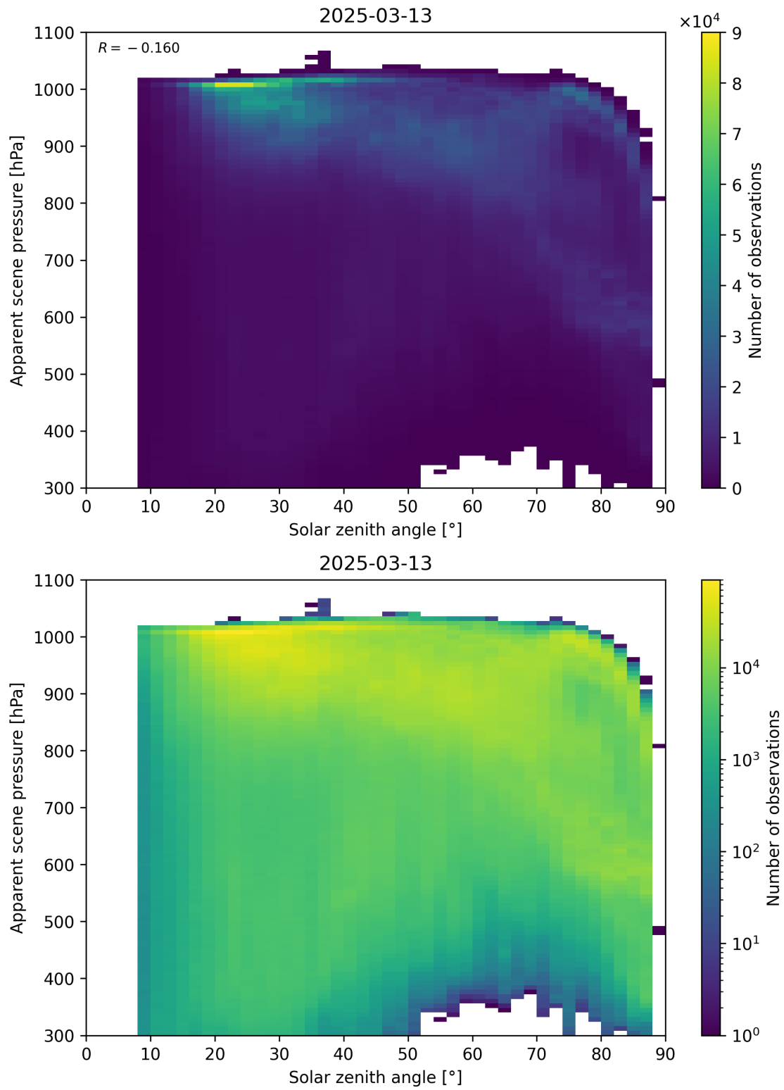
Figure 108: Scatter density plot of “Solar zenith angle” against “Apparent scene pressure” for 2025-03-12 to 2025-03-14.
