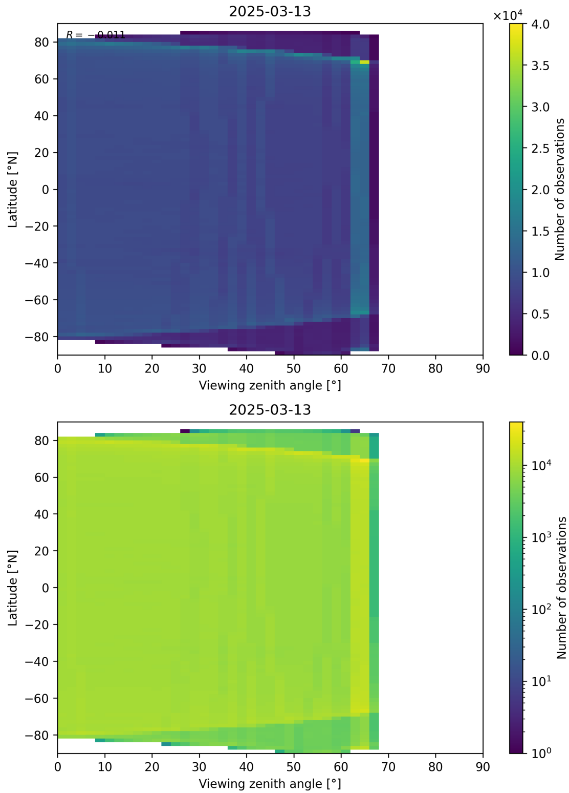
Figure 123: Scatter density plot of “Viewing zenith angle” against “Latitude” for 2025-03-12 to 2025-03-14.
