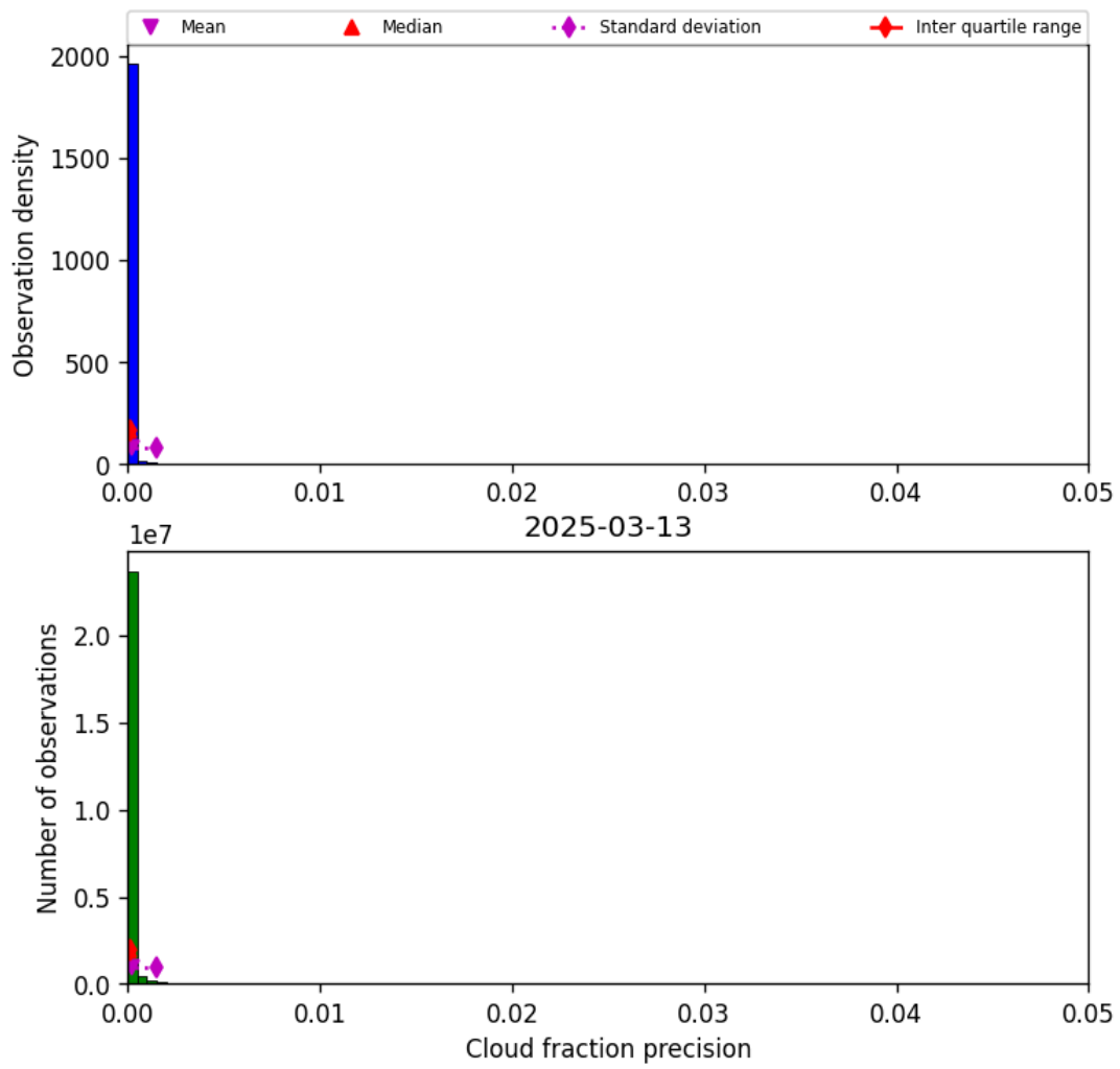
Figure 33: Histogram of “Cloud fraction precision” for 2025-03-12 to 2025-03-14
