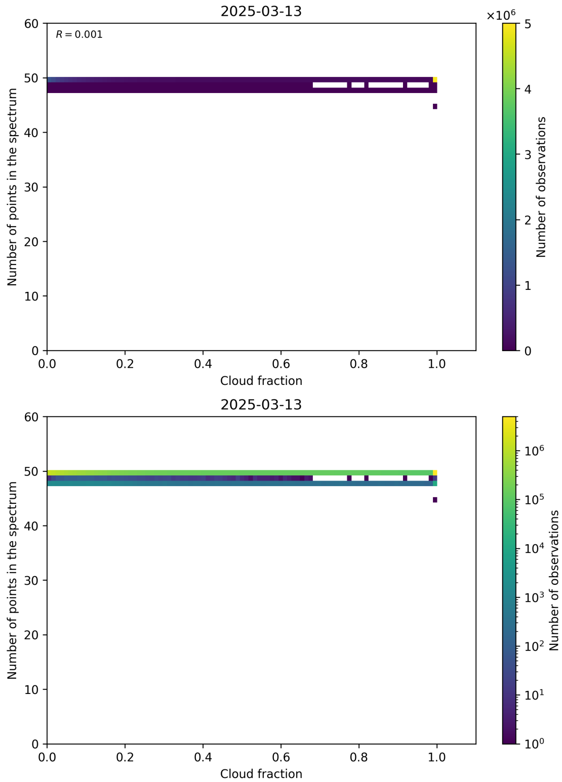
Figure 74: Scatter density plot of “Cloud fraction” against “Number of points in the spectrum” for 2025-03-12 to 2025-03-14.
