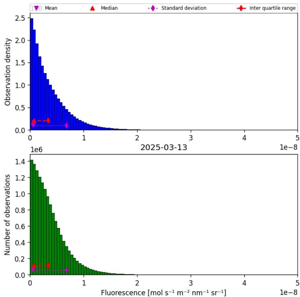
Figure 40: Histogram of “Fluorescence” for 2025-03-12 to 2025-03-14
