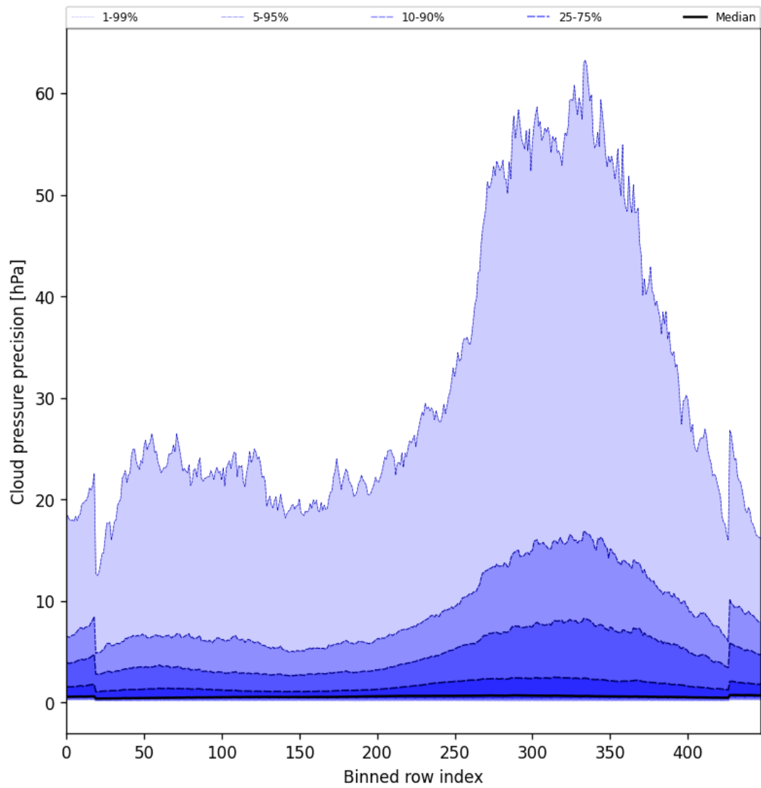
Figure 48: Along track statistics of “Cloud pressure precision” for 2025-03-12 to 2025-03-14
