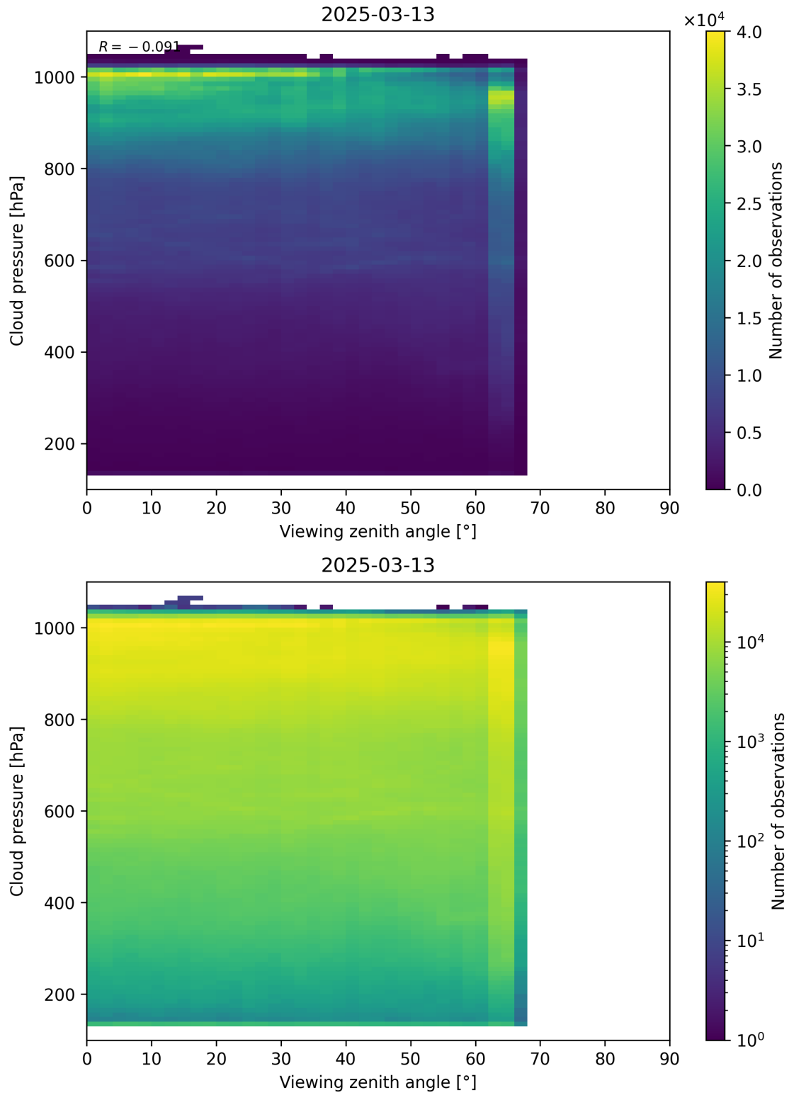
Figure 121: Scatter density plot of “Viewing zenith angle” against “Cloud pressure” for 2025-03-12 to 2025-03-14.
