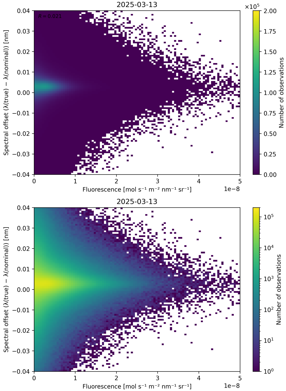
Figure 87: Scatter density plot of “Fluorescence” against “Spectral offset ( \lambda_{\text{true}} - \lambda_{\text{nominal}} )” for 2025-03-12 to 2025-03-14.
