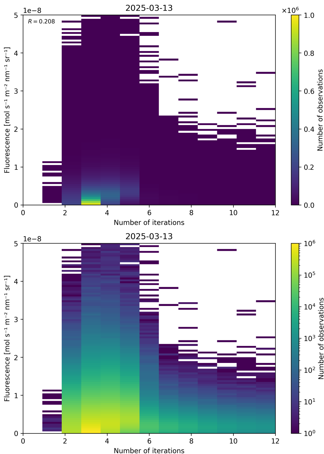
Figure 98: Scatter density plot of “Number of iterations” against “Fluorescence” for 2025-03-12 to 2025-03-14.
