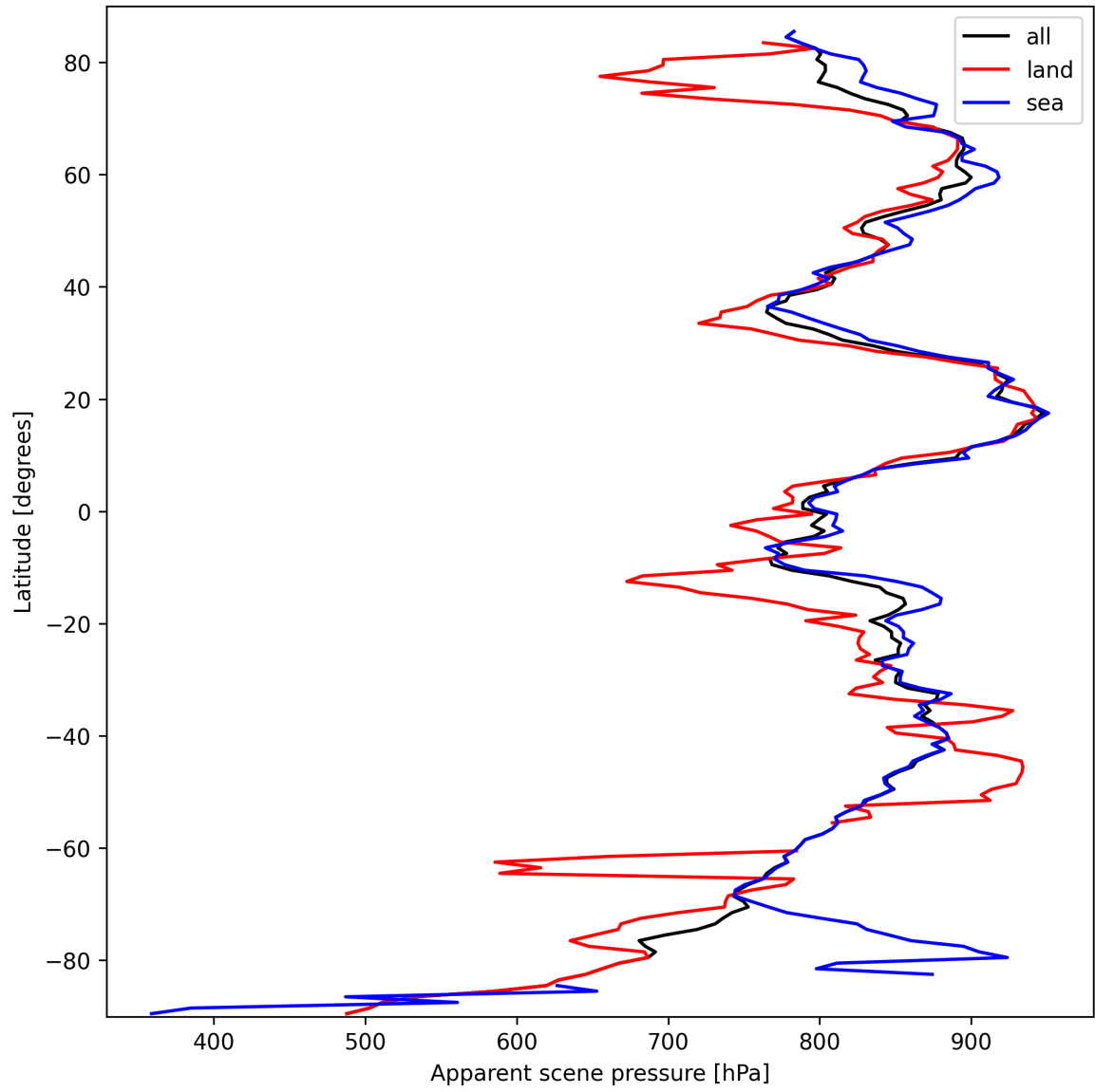
Figure 19: Zonal average of “Apparent scene pressure” for 2025-03-12 to 2025-03-14.
