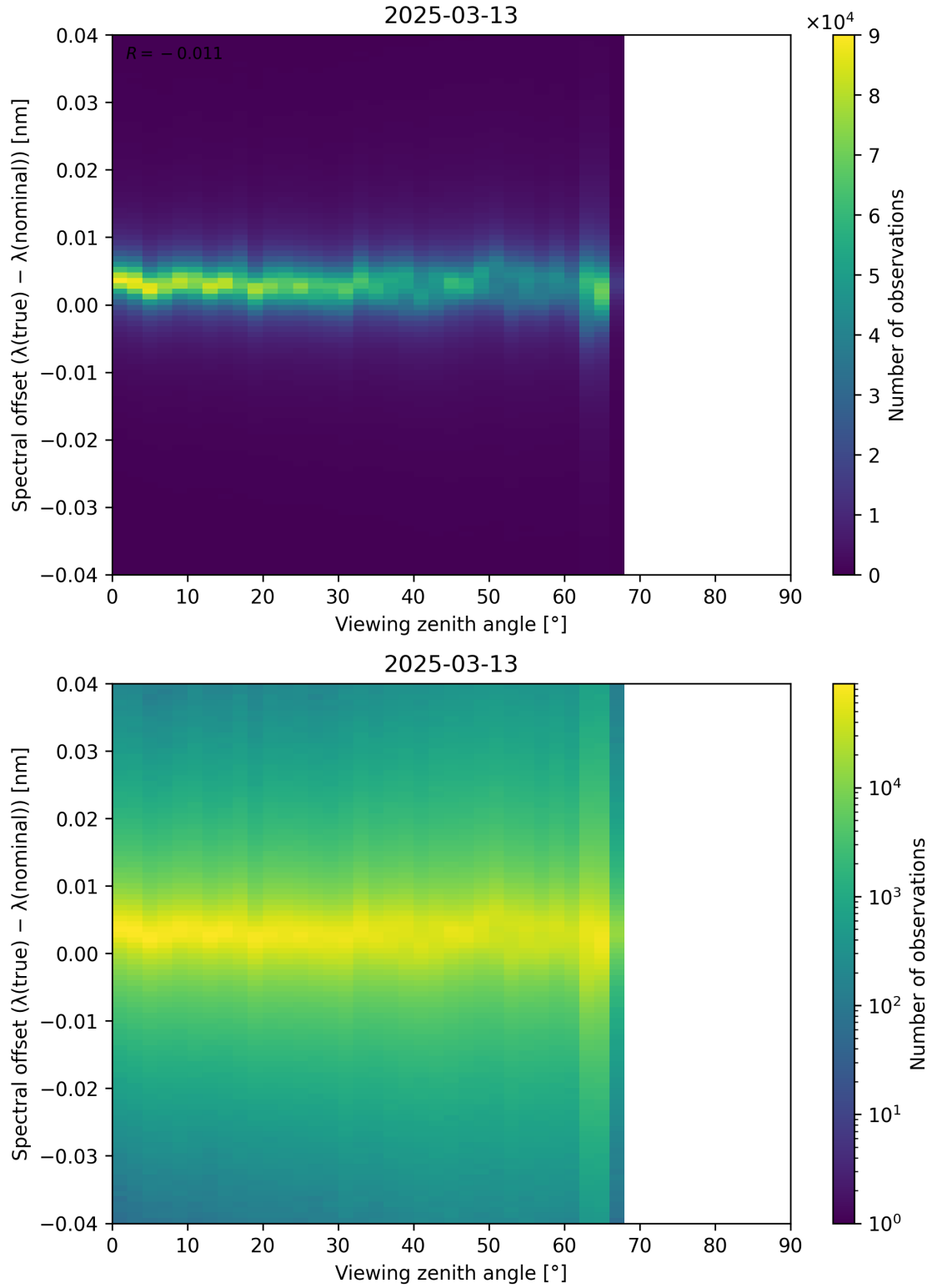
Figure 128: Scatter density plot of “Viewing zenith angle” against “Spectral offset ( \lambda_{\text{true}} - \lambda_{\text{nominal}} )” for 2025-03-12 to 2025-03-14.
