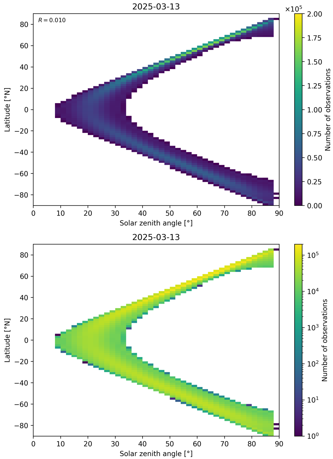
Figure 113: Scatter density plot of “Solar zenith angle” against “Latitude” for 2025-03-12 to 2025-03-14.
