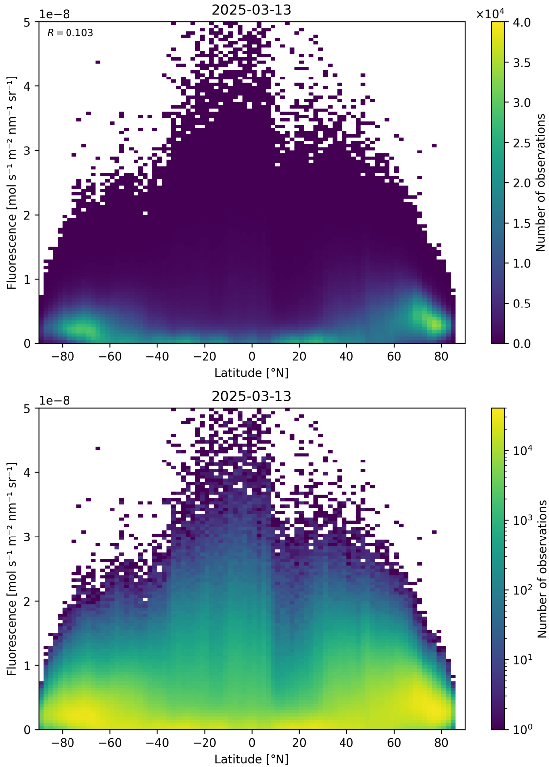
Figure 92: Scatter density plot of “Latitude” against “Fluorescence” for 2025-03-12 to 2025-03-14.
