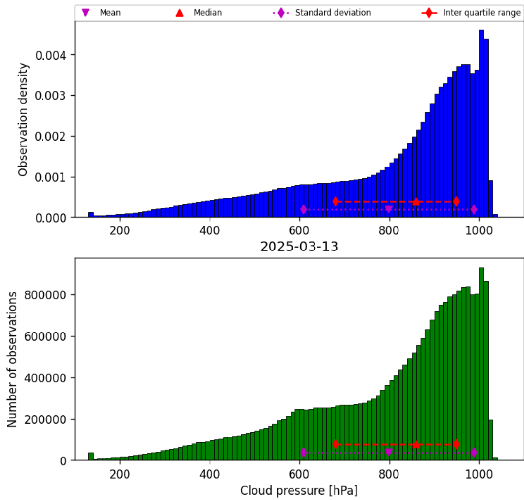
Figure 30: Histogram of “Cloud pressure” for 2025-03-12 to 2025-03-14
