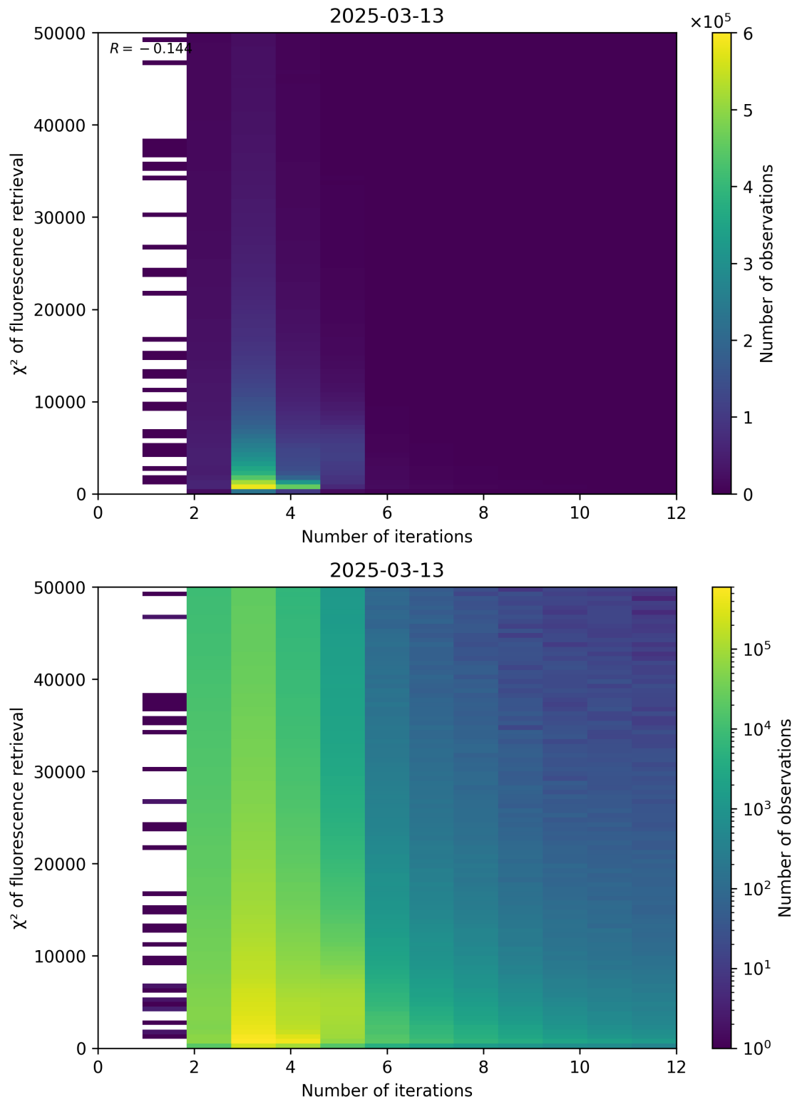
Figure 97: Scatter density plot of “Number of iterations” against “ \chi^2 of fluorescence retrieval” for 2025-03-12 to 2025-03-14.
