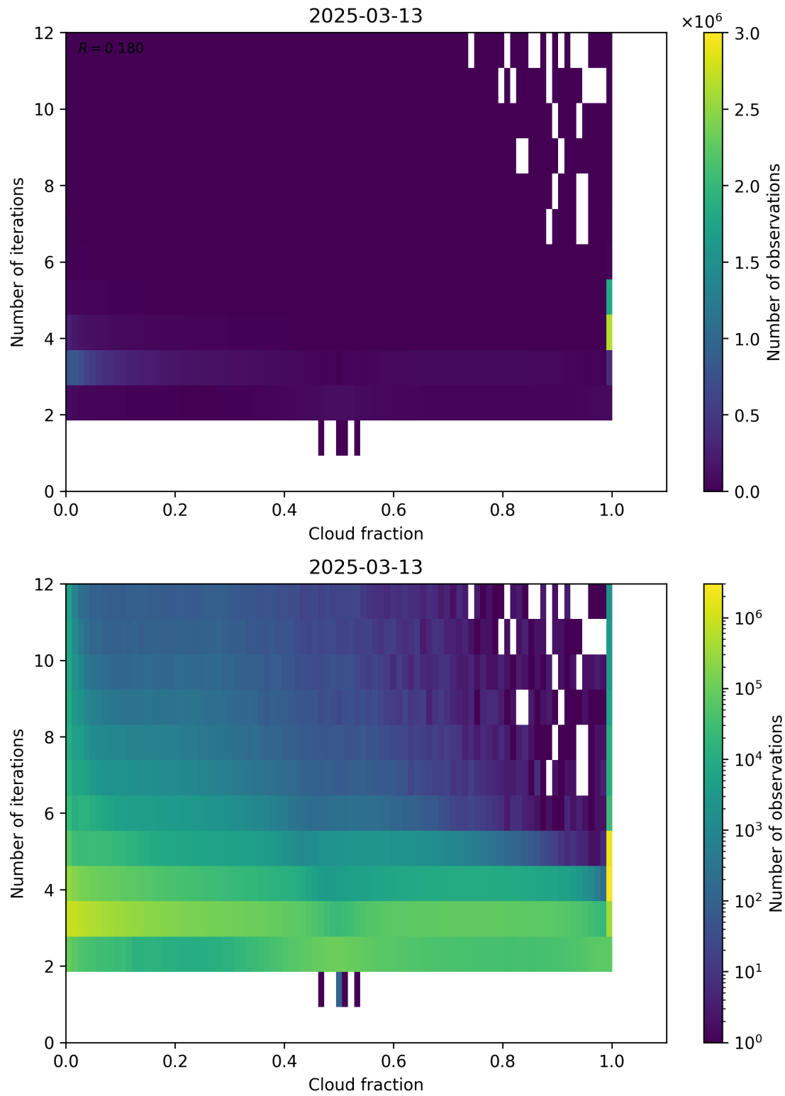
Figure 73: Scatter density plot of “Cloud fraction” against “Number of iterations” for 2025-03-12 to 2025-03-14.
