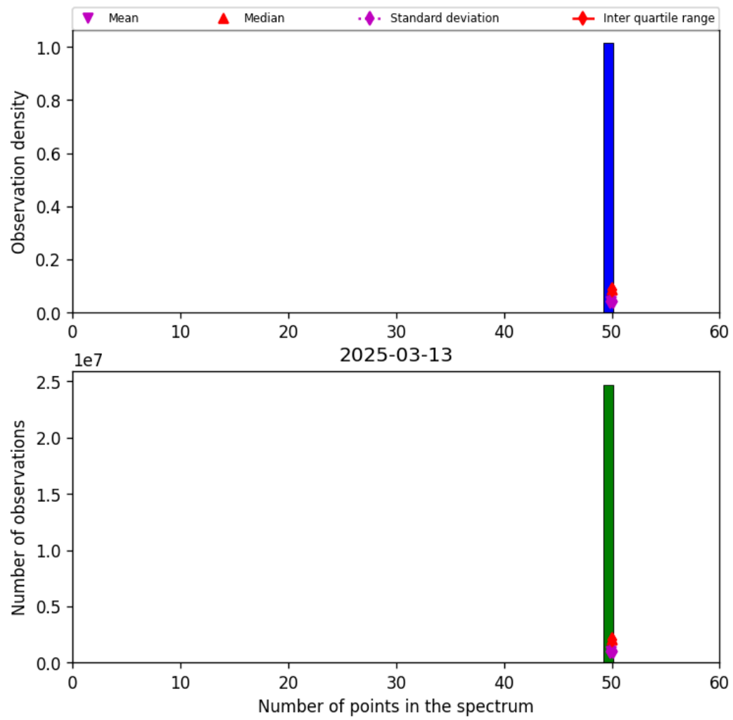
Figure 44: Histogram of “Number of points in the spectrum” for 2025-03-12 to 2025-03-14
