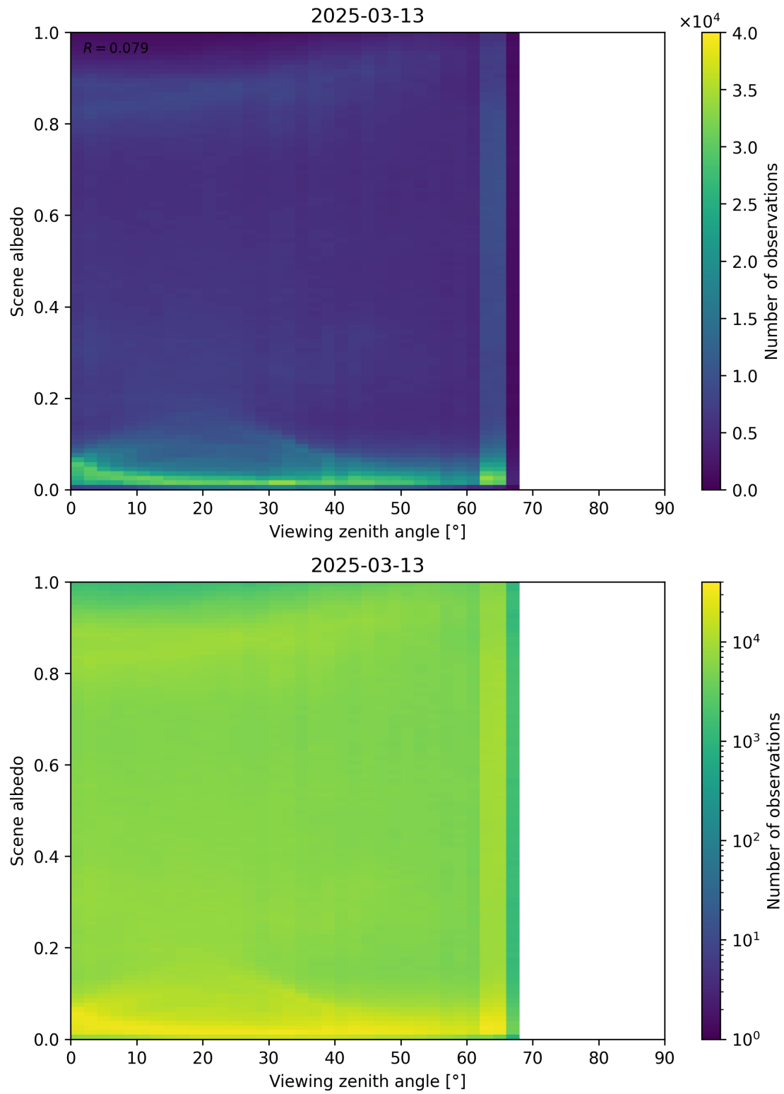
Figure 126: Scatter density plot of “Viewing zenith angle” against “Scene albedo” for 2025-03-12 to 2025-03-14.
