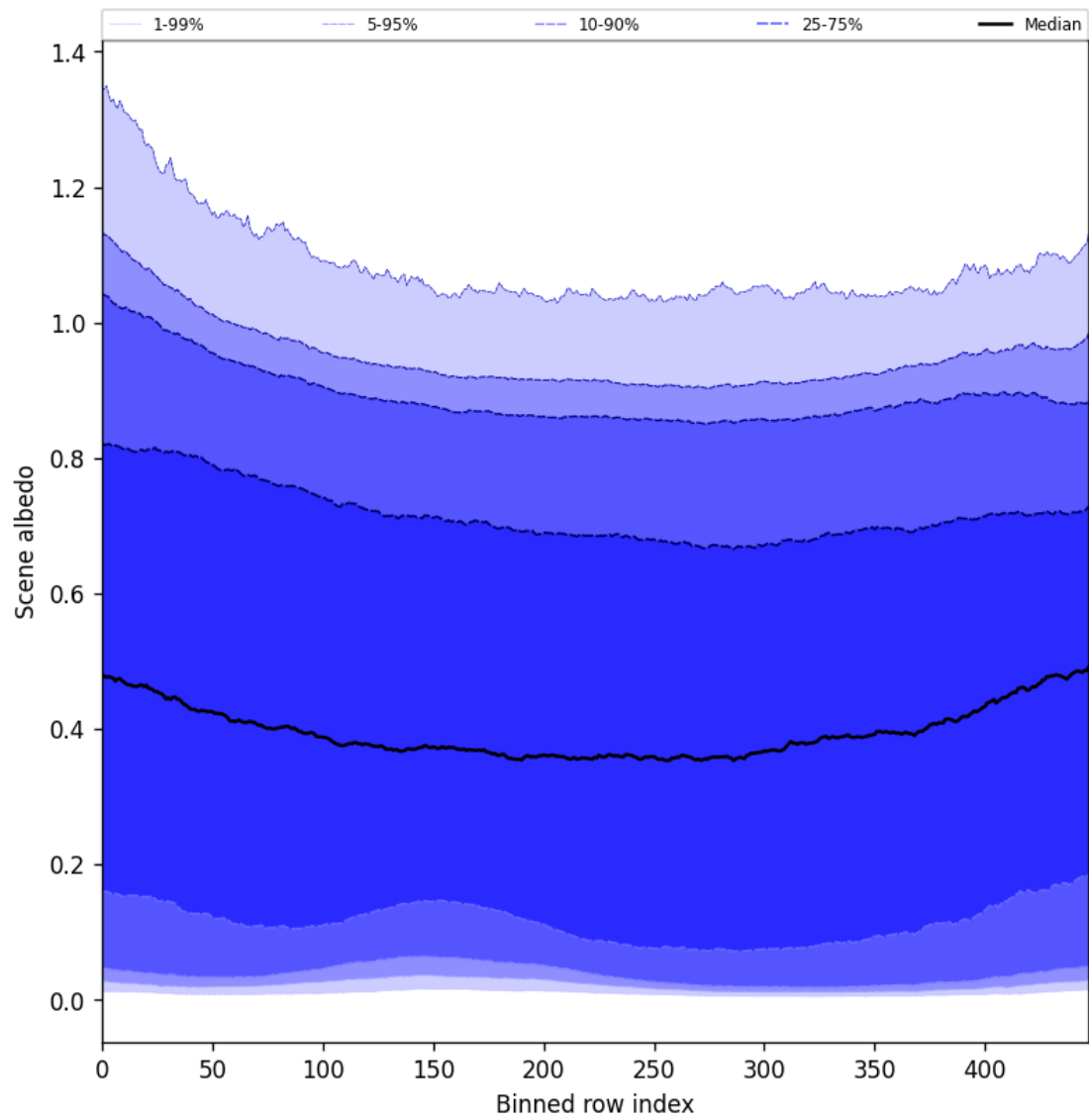
Figure 51: Along track statistics of “Scene albedo” for 2025-03-12 to 2025-03-14
