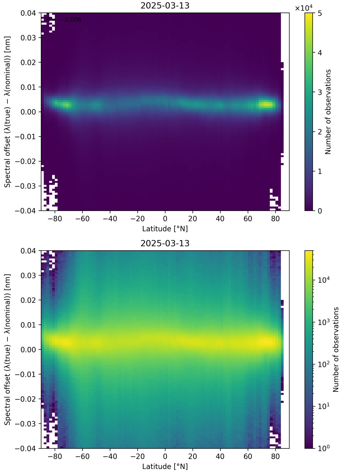
Figure 96: Scatter density plot of “Latitude” against “Spectral offset ( \lambda_{\text{true}} - \lambda_{\text{nominal}} )” for 2025-03-12 to 2025-03-14.
