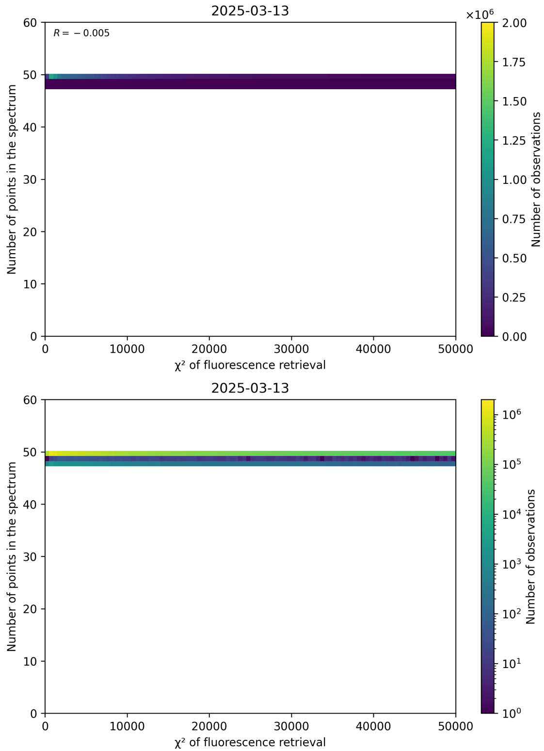
Figure 68: Scatter density plot of " \chi^2 of fluorescence retrieval" against "Number of points in the spectrum" for 2025-03-12 to 2025-03-14.
