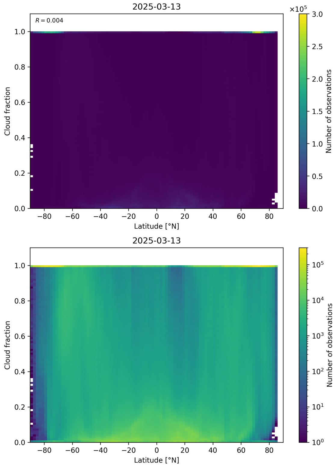
Figure 90: Scatter density plot of “Latitude” against “Cloud fraction” for 2025-03-12 to 2025-03-14.
