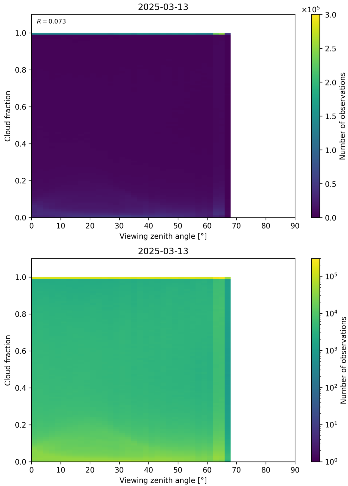
Figure 120: Scatter density plot of “Viewing zenith angle” against “Cloud fraction” for 2025-03-12 to 2025-03-14.
