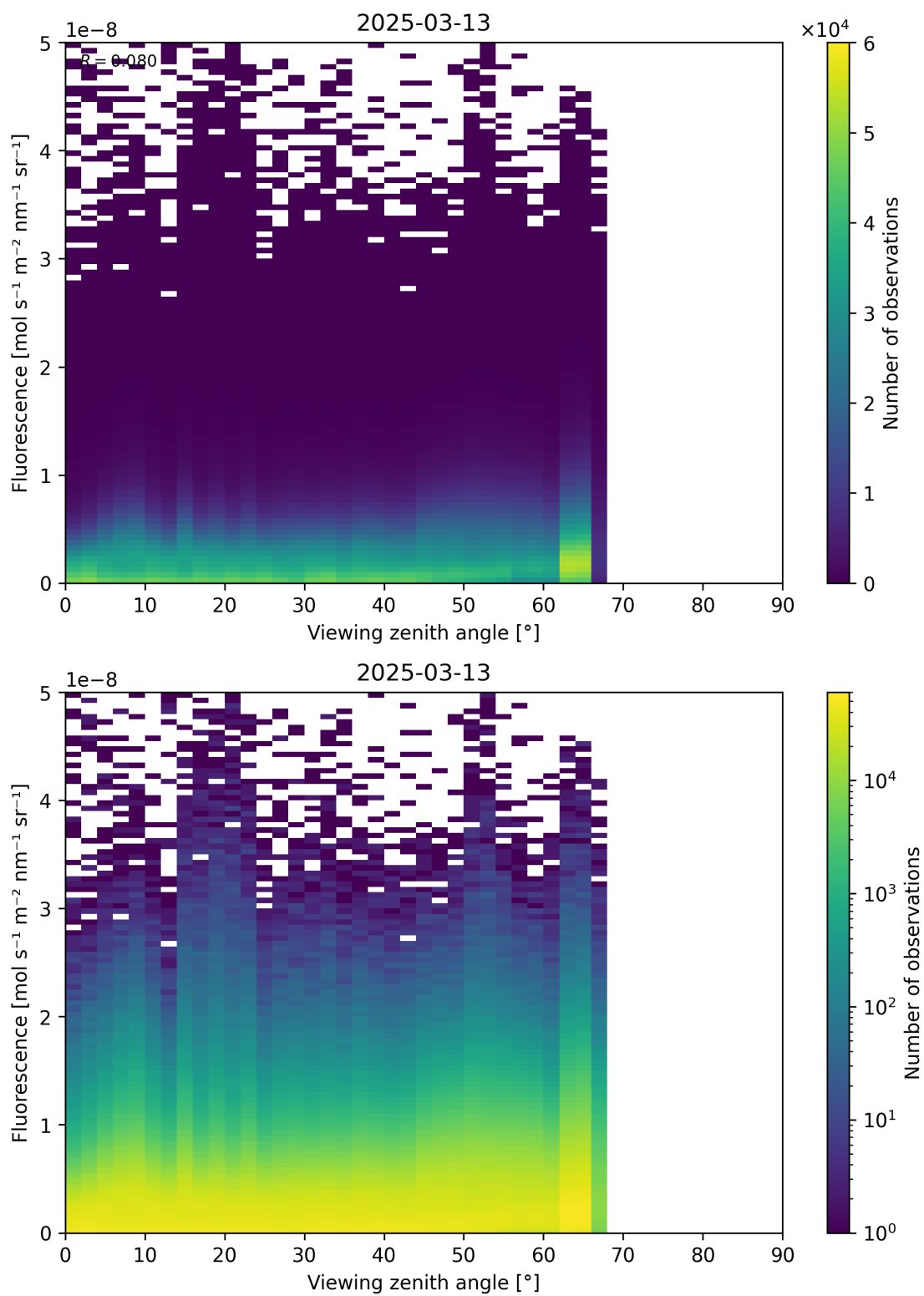
Figure 122: Scatter density plot of “Viewing zenith angle” against “Fluorescence” for 2025-03-12 to 2025-03-14.
