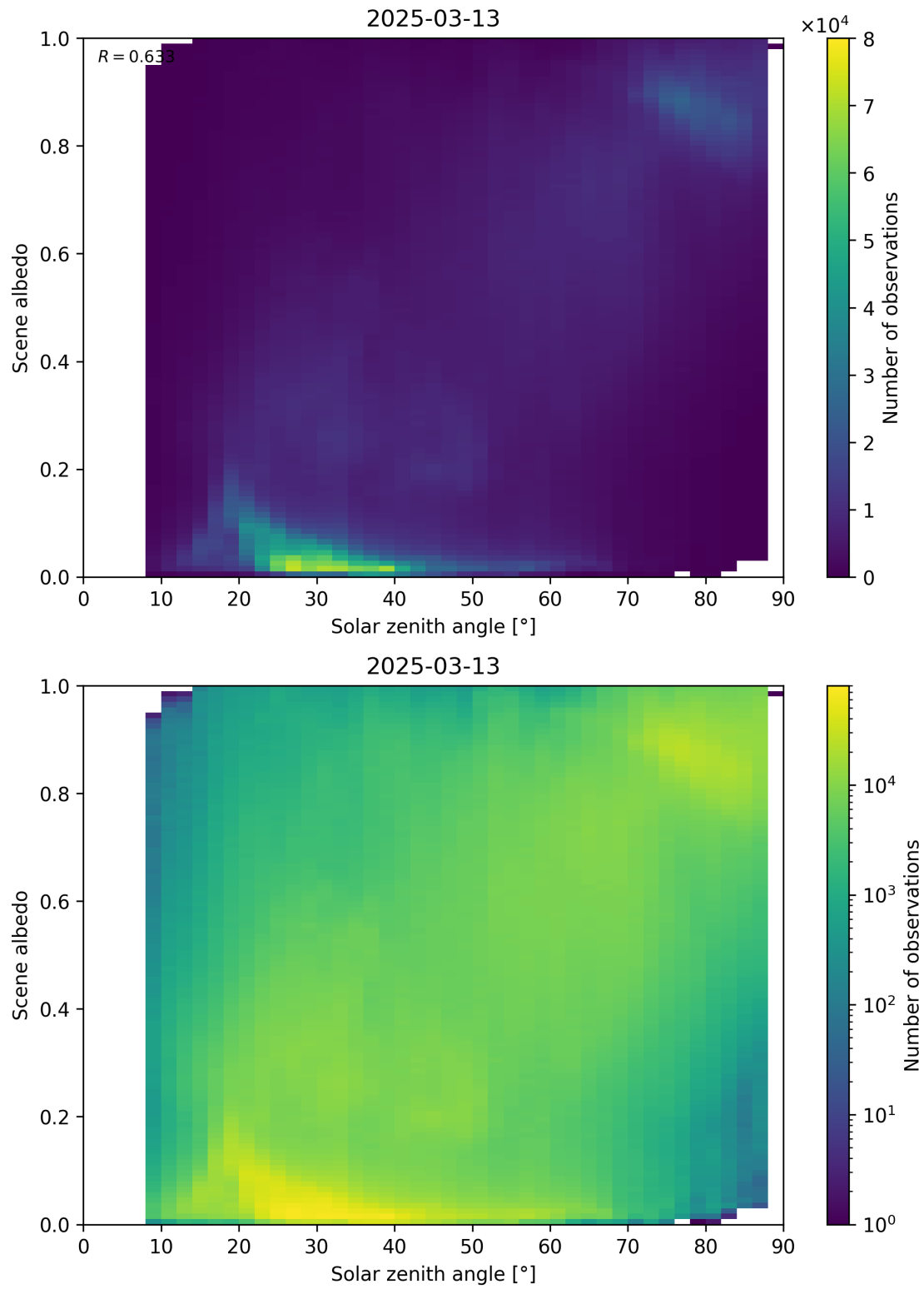
Figure 116: Scatter density plot of “Solar zenith angle” against “Scene albedo” for 2025-03-12 to 2025-03-14.
