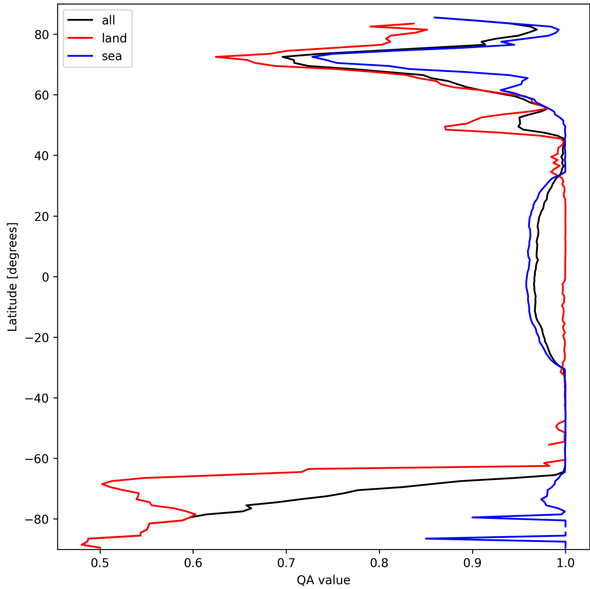
Figure 12: Zonal average of "QA value" for 2025-03-12 to 2025-03-14.
