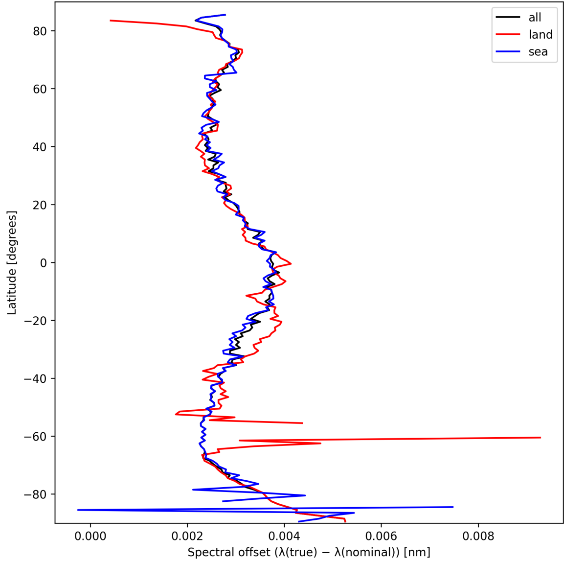
Figure 28: Zonal average of “Spectral offset ( \lambda_{\text{true}} - \lambda_{\text{nominal}} )” for 2025-03-12 to 2025-03-14.
