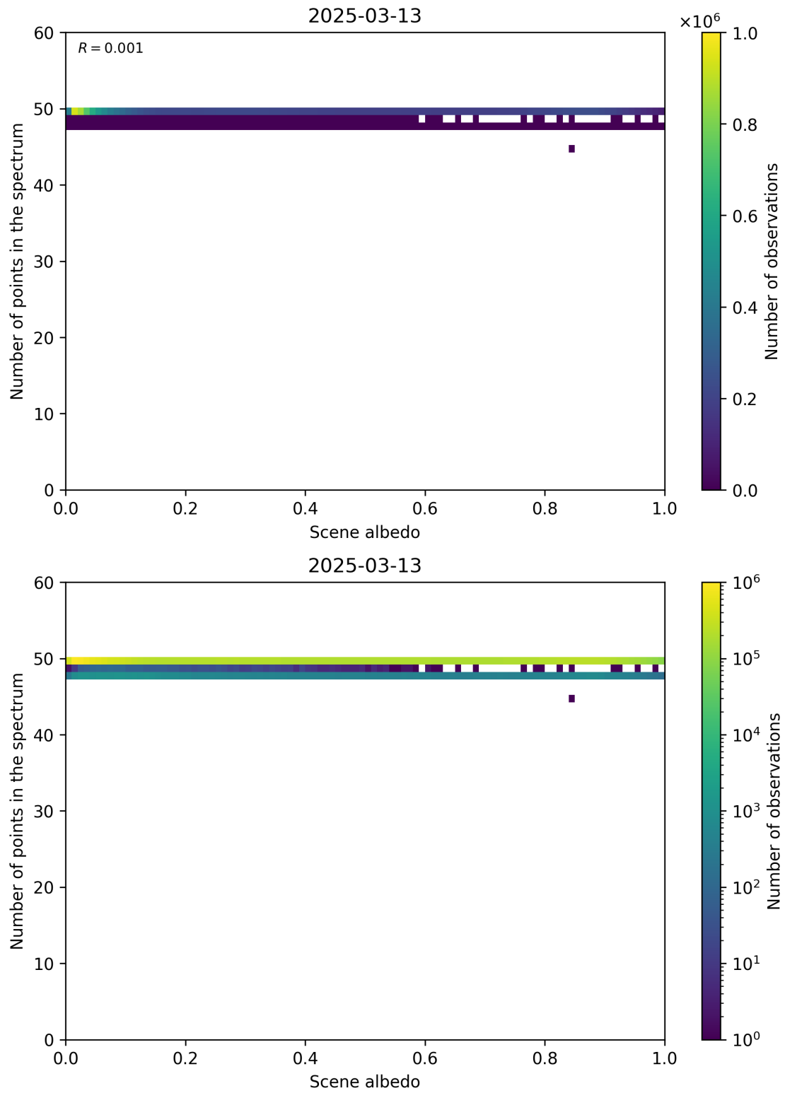
Figure 106: Scatter density plot of “Scene albedo” against “Number of points in the spectrum” for 2025-03-12 to 2025-03-14.
