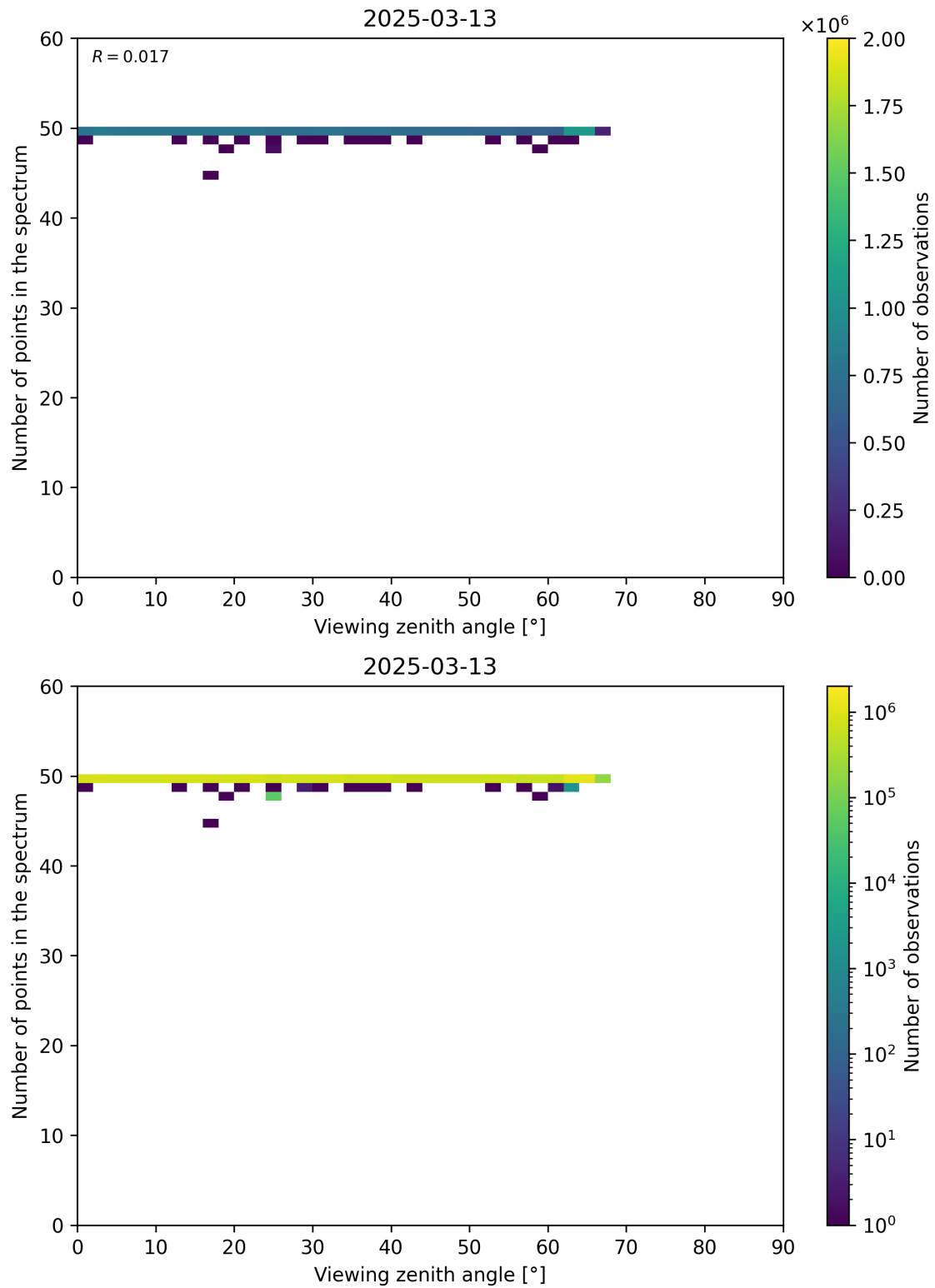
Figure 125: Scatter density plot of “Viewing zenith angle” against “Number of points in the spectrum” for 2025-03-12 to 2025-03-14.
