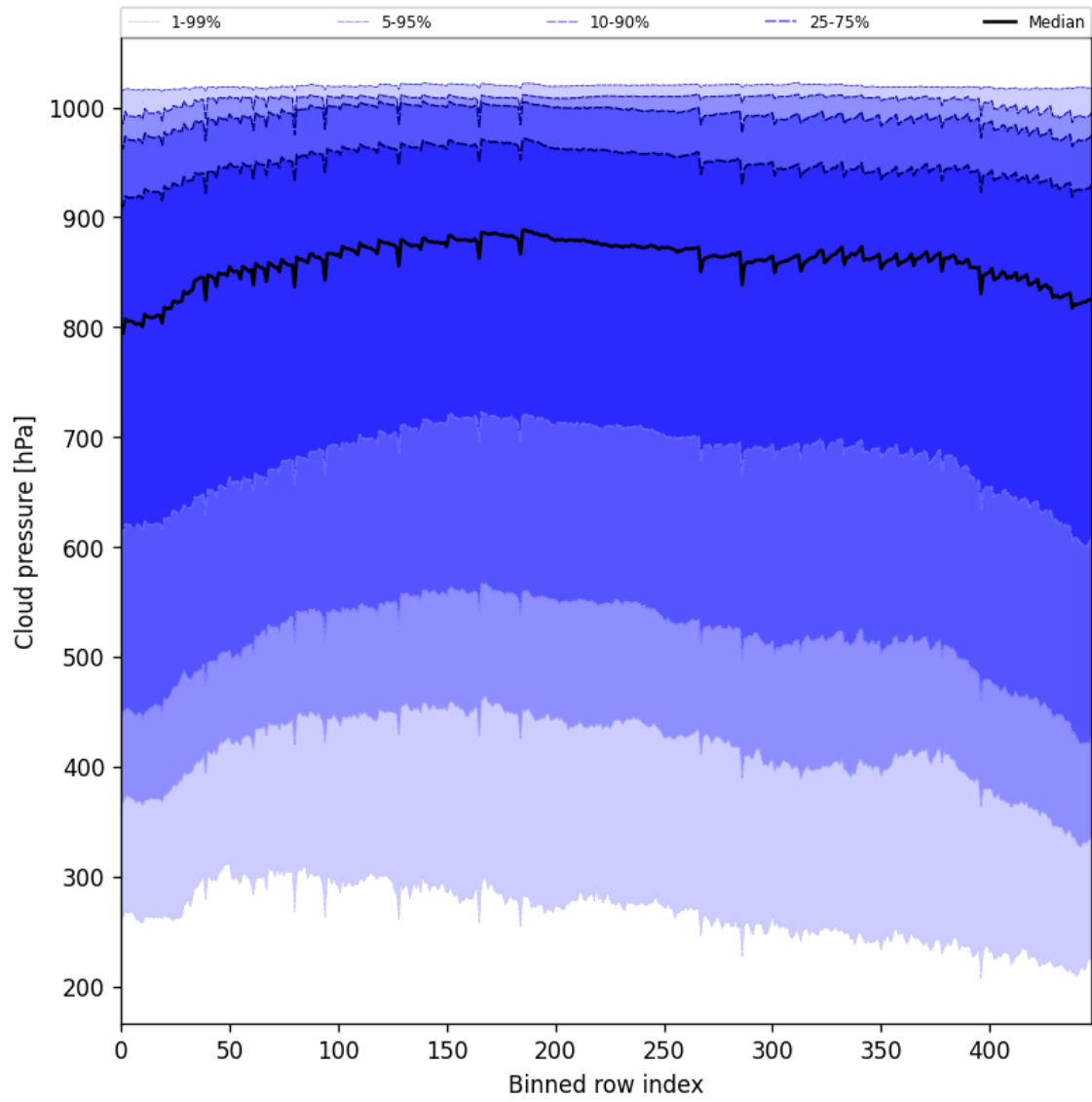
Figure 47: Along track statistics of “Cloud pressure” for 2025-03-12 to 2025-03-14
