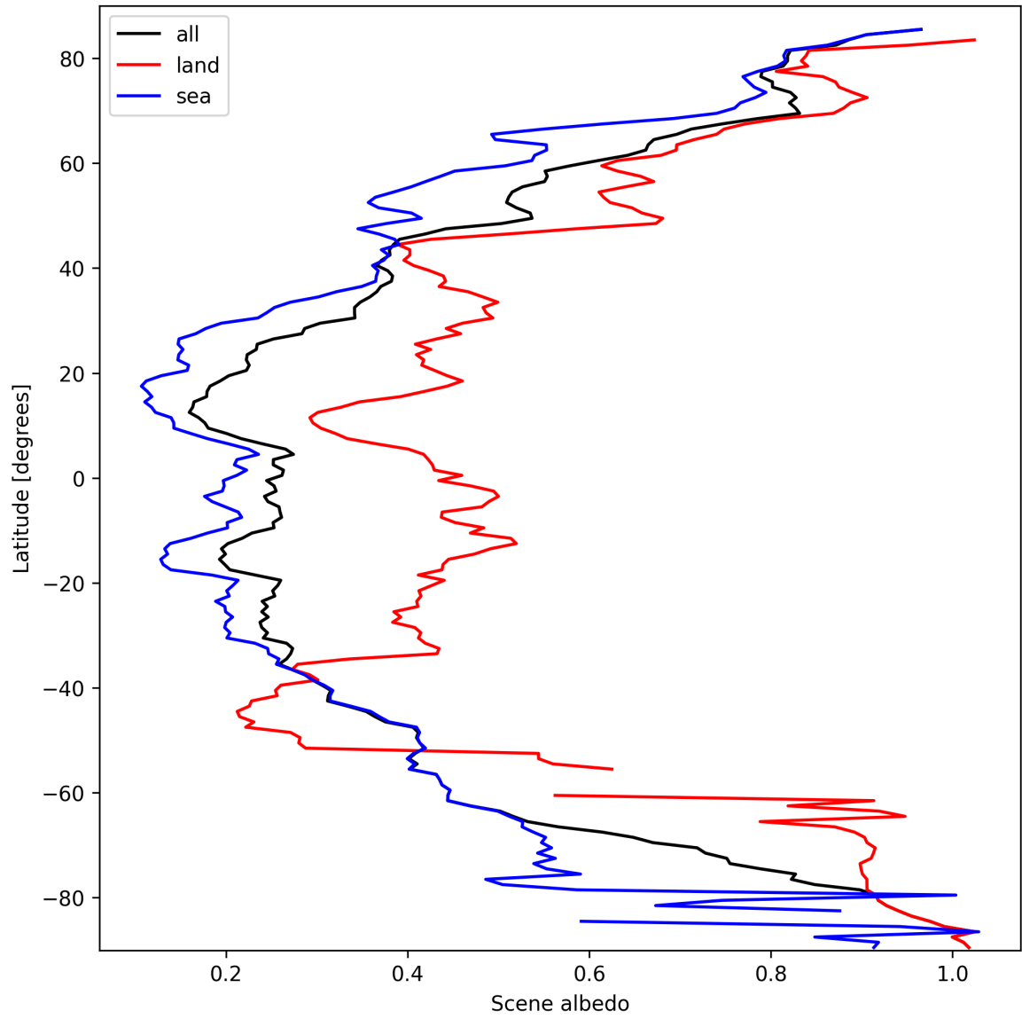
Figure 17: Zonal average of “Scene albedo” for 2025-03-12 to 2025-03-14.
