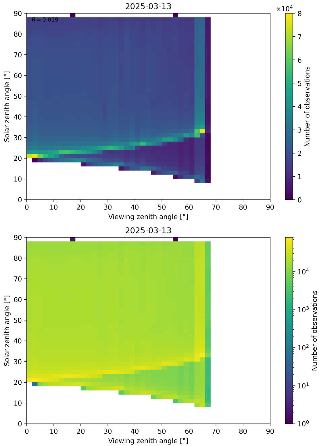
Figure 127: Scatter density plot of “Viewing zenith angle” against “Solar zenith angle” for 2025-03-12 to 2025-03-14.
