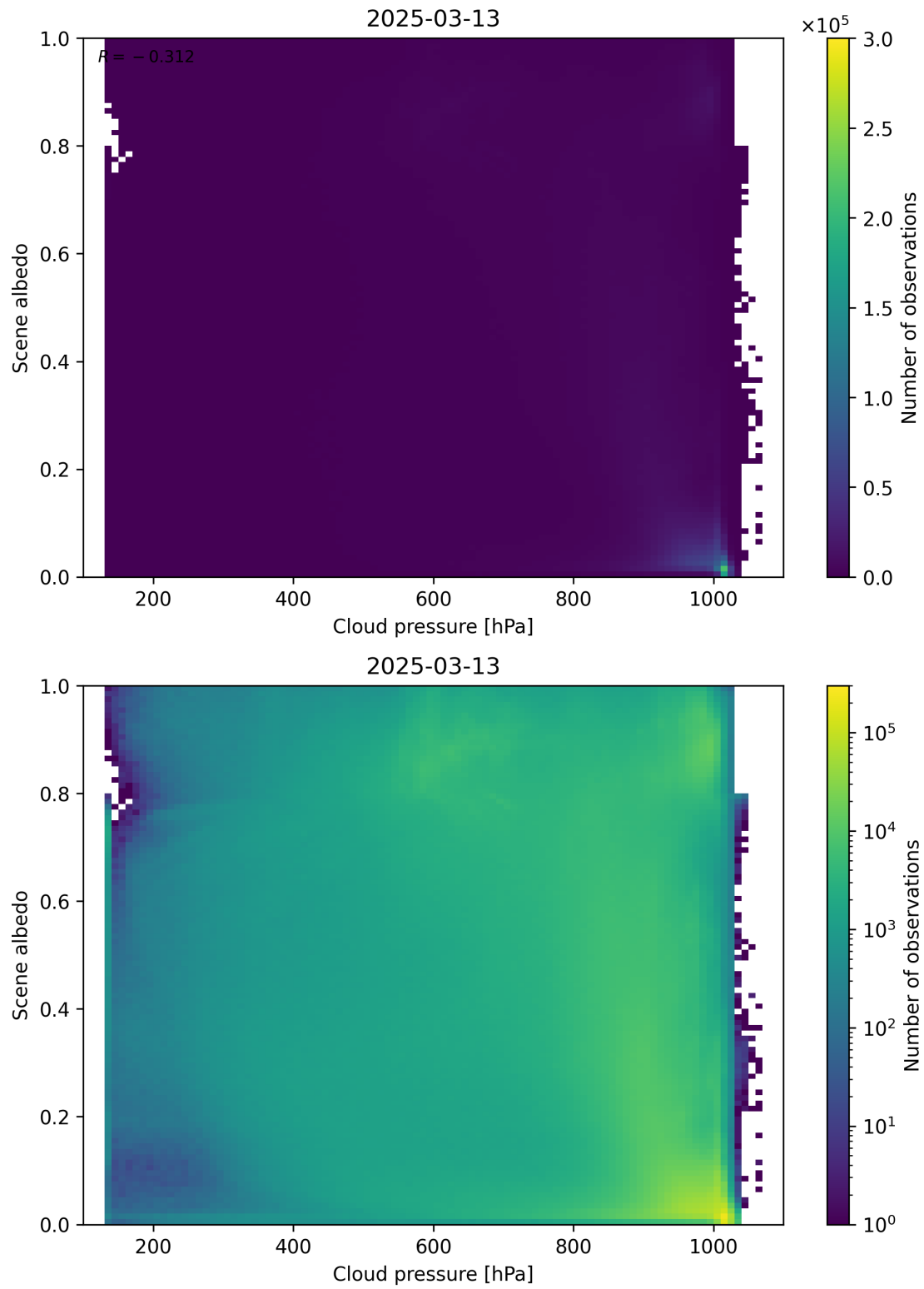
Figure 83: Scatter density plot of “Cloud pressure” against “Scene albedo” for 2025-03-12 to 2025-03-14.
