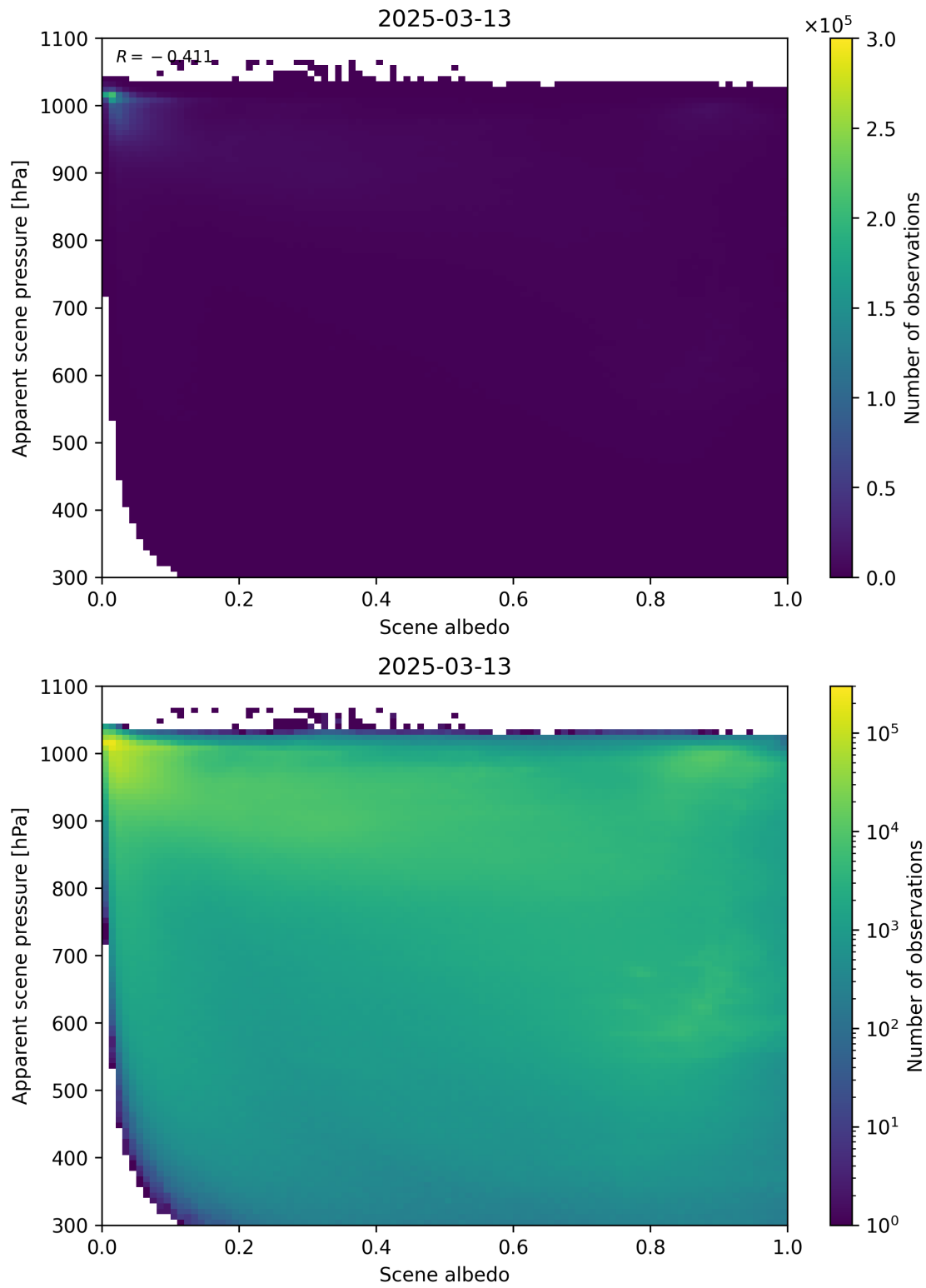
Figure 102: Scatter density plot of “Scene albedo” against “Apparent scene pressure” for 2025-03-12 to 2025-03-14.
