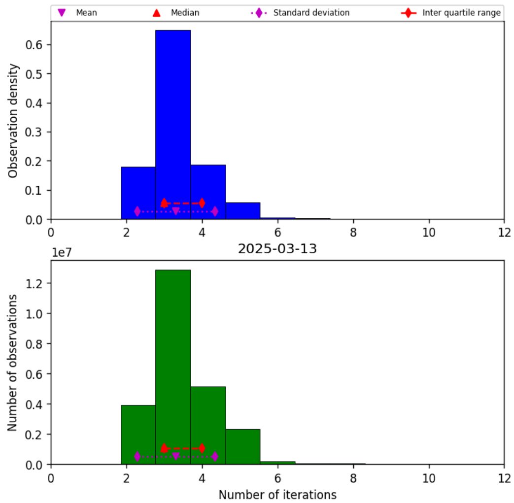
Figure 39: Histogram of “Number of iterations” for 2025-03-12 to 2025-03-14
