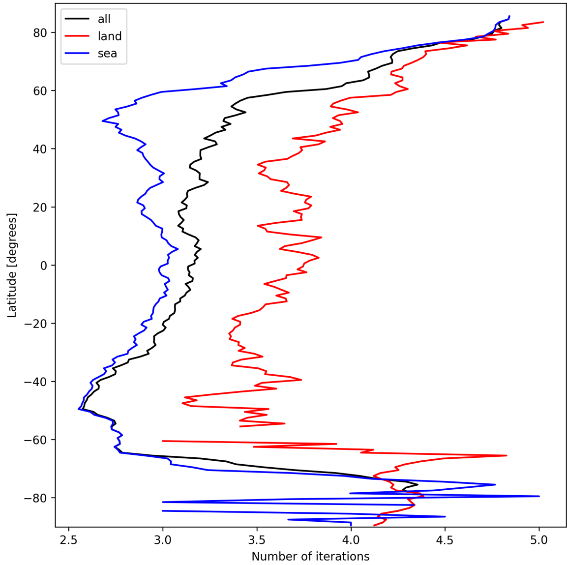
Figure 22: Zonal average of “Number of iterations” for 2025-03-12 to 2025-03-14.
