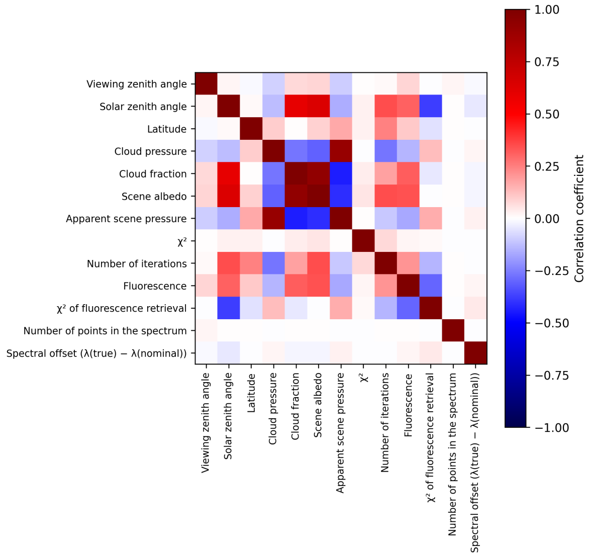
Figure 2: Map of correlation matrix for 2025-03-12 to 2025-03-14.
