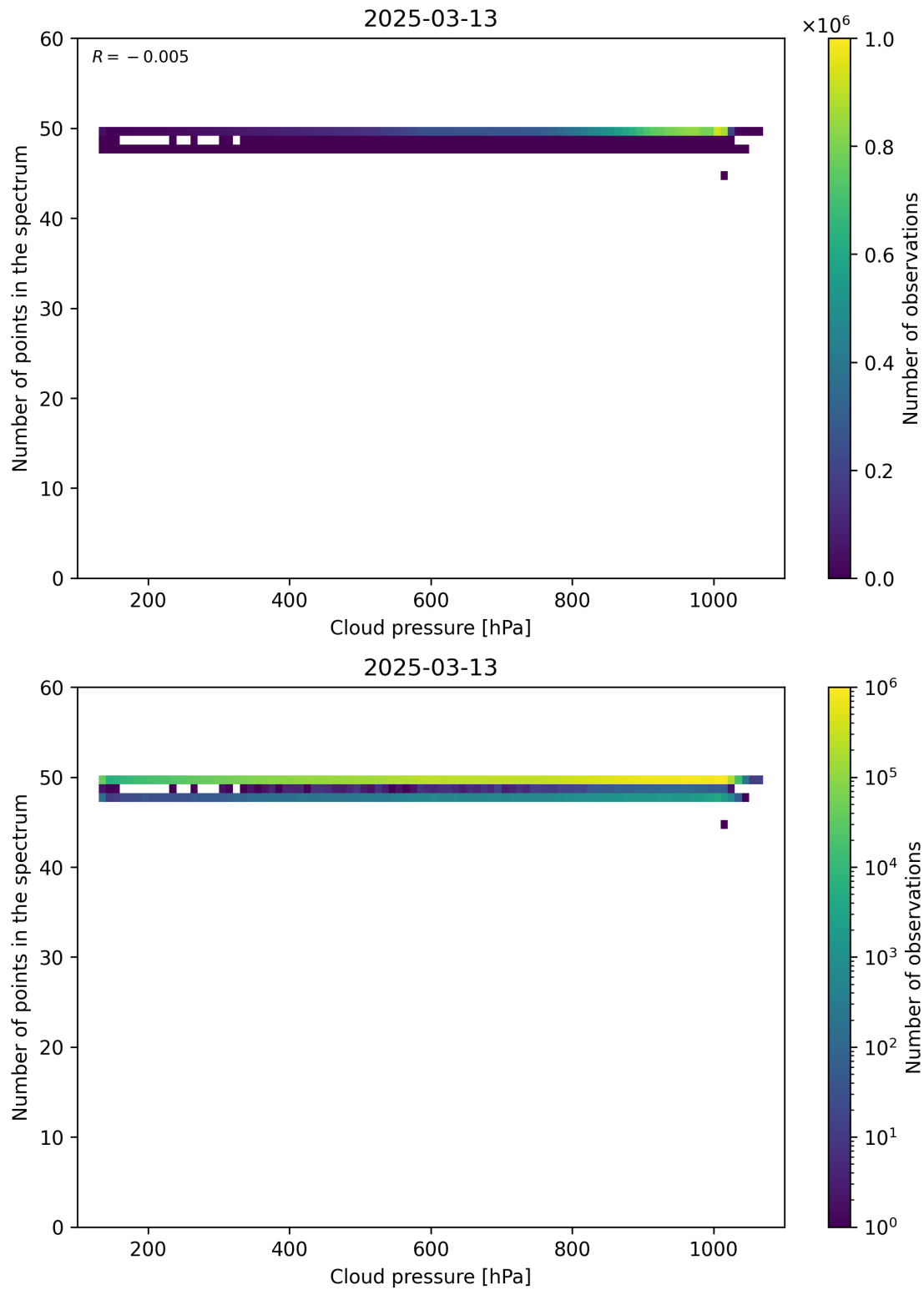
Figure 82: Scatter density plot of “Cloud pressure” against “Number of points in the spectrum” for 2025-03-12 to 2025-03-14.
