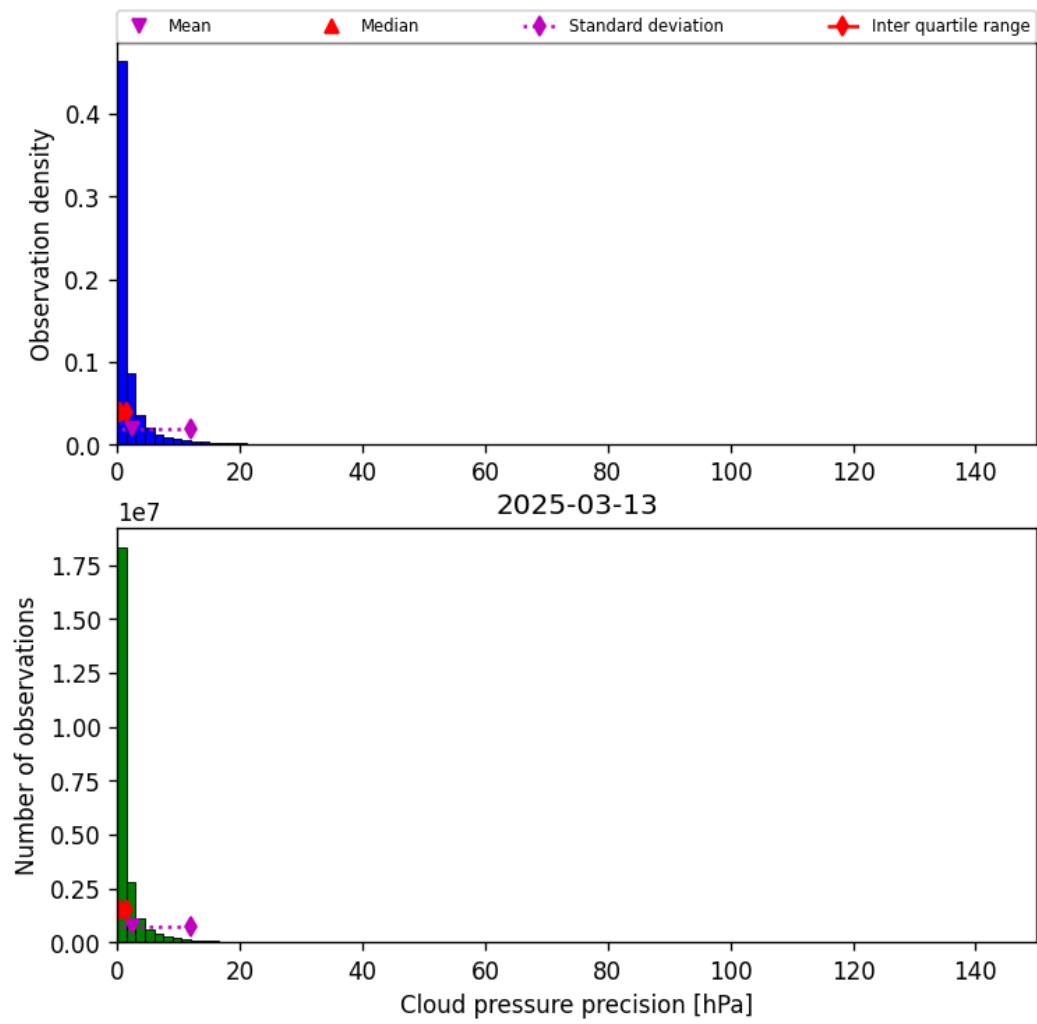
Figure 31: Histogram of “Cloud pressure precision” for 2025-03-12 to 2025-03-14
