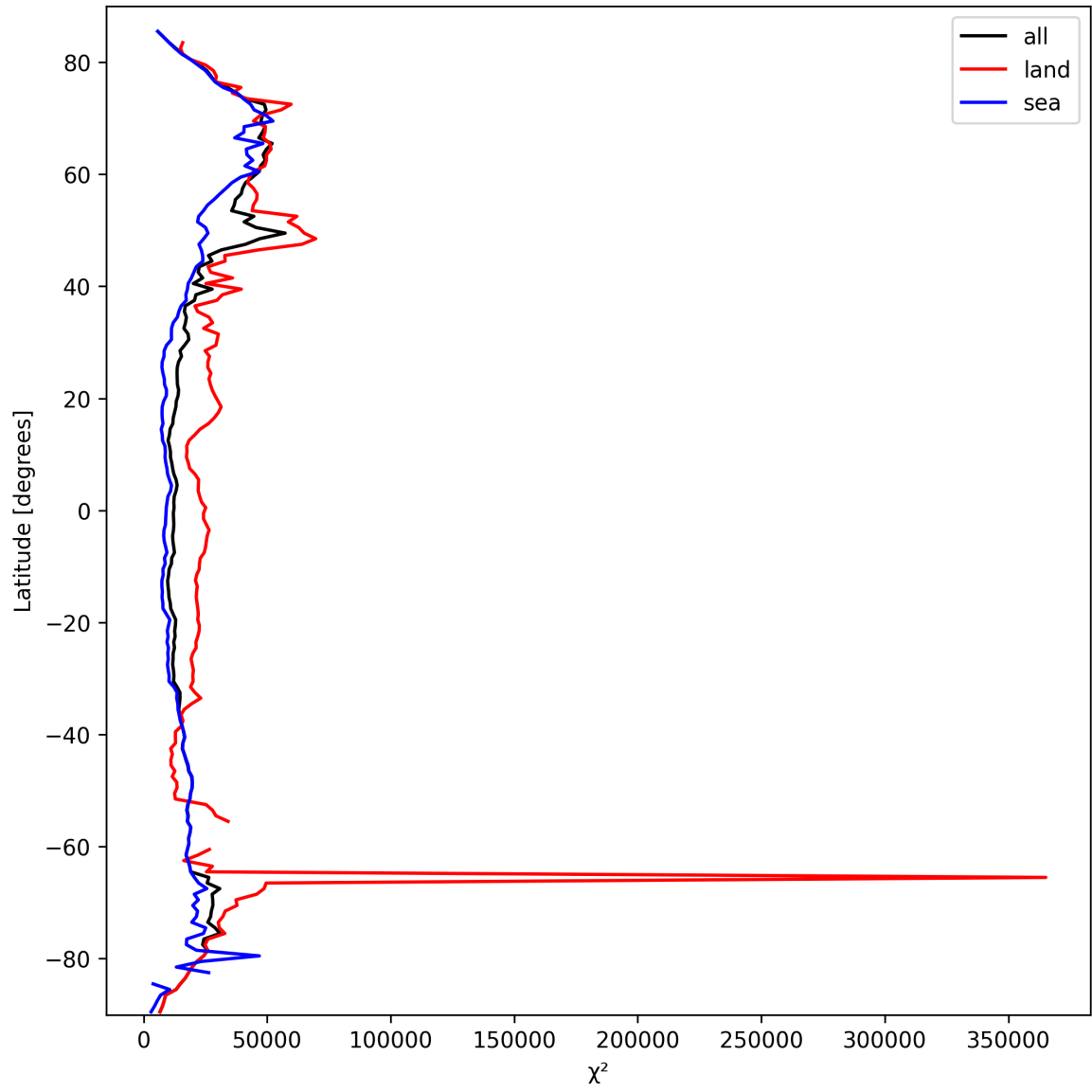
Figure 21: Zonal average of “ \chi^2 ” for 2025-03-12 to 2025-03-14.
