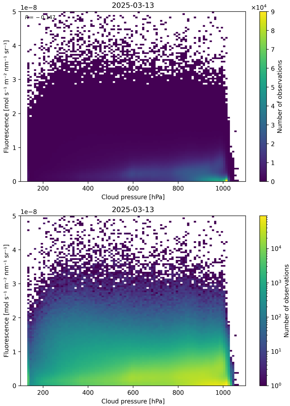
Figure 80: Scatter density plot of “Cloud pressure” against “Fluorescence” for 2025-03-12 to 2025-03-14.
