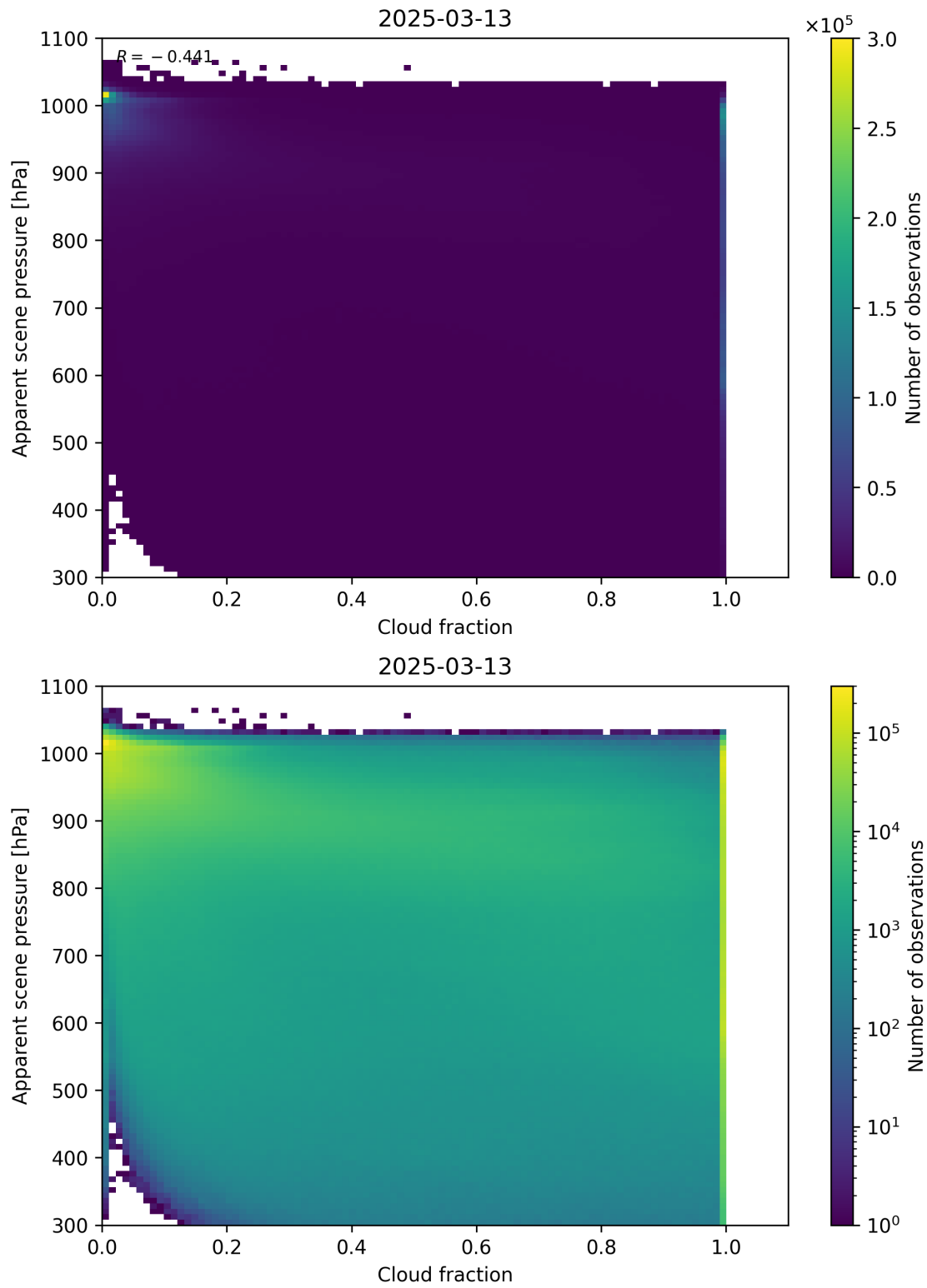
Figure 70: Scatter density plot of “Cloud fraction” against “Apparent scene pressure” for 2025-03-12 to 2025-03-14.
