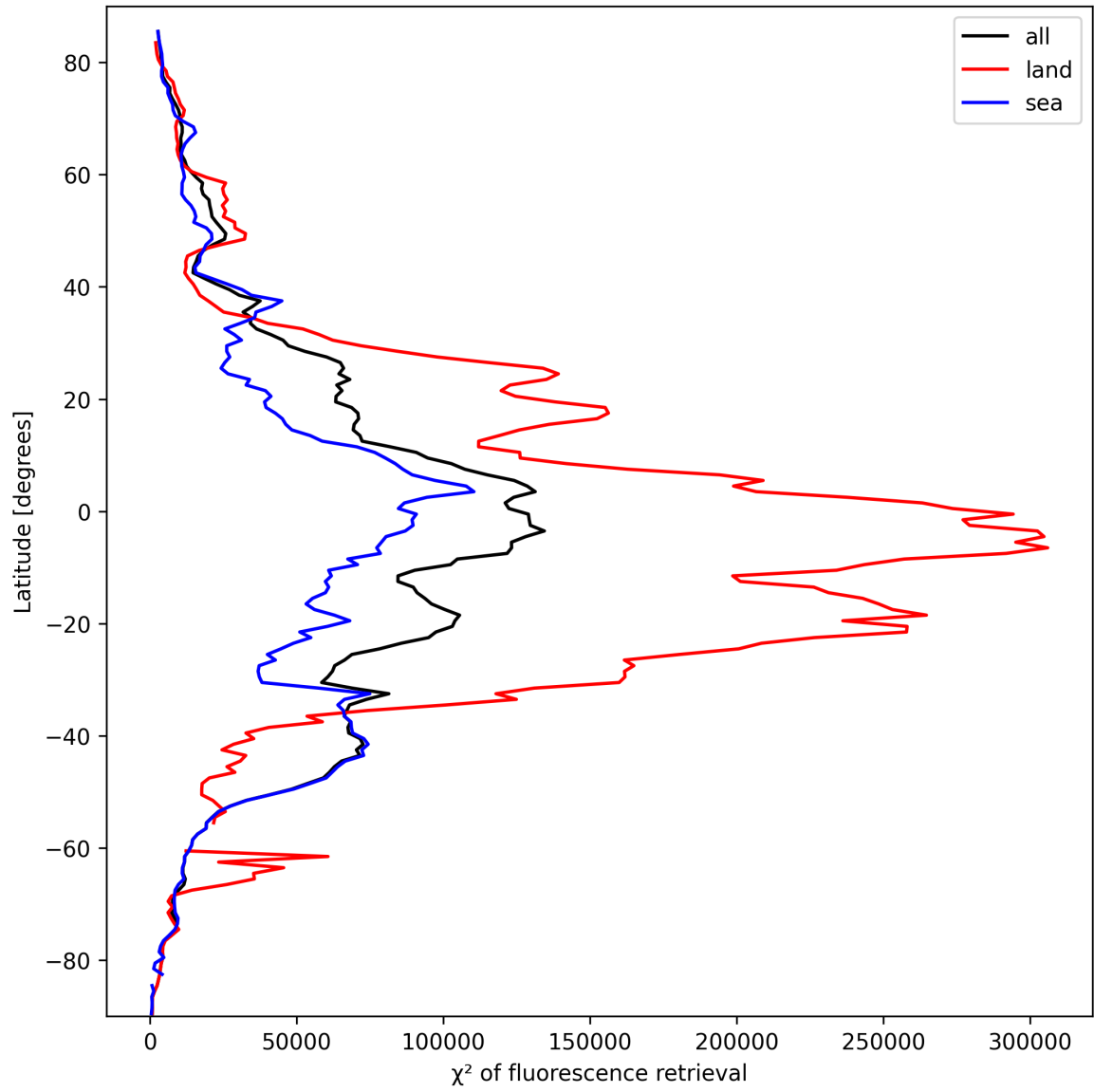
Figure 25: Zonal average of “ \chi^2 of fluorescence retrieval” for 2025-03-12 to 2025-03-14.
