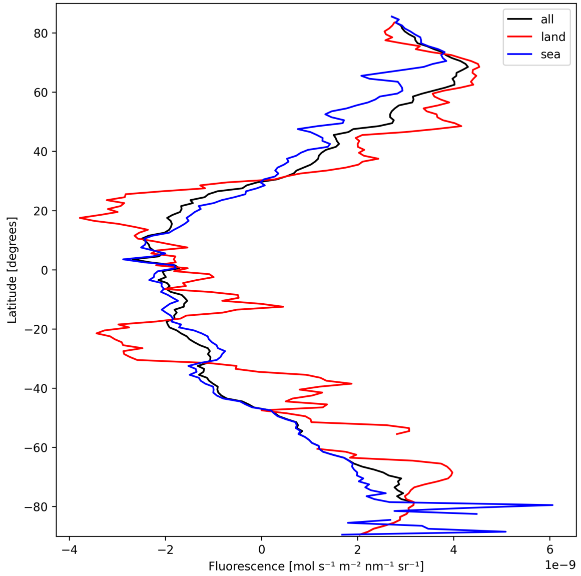
Figure 23: Zonal average of “Fluorescence” for 2025-03-12 to 2025-03-14.
