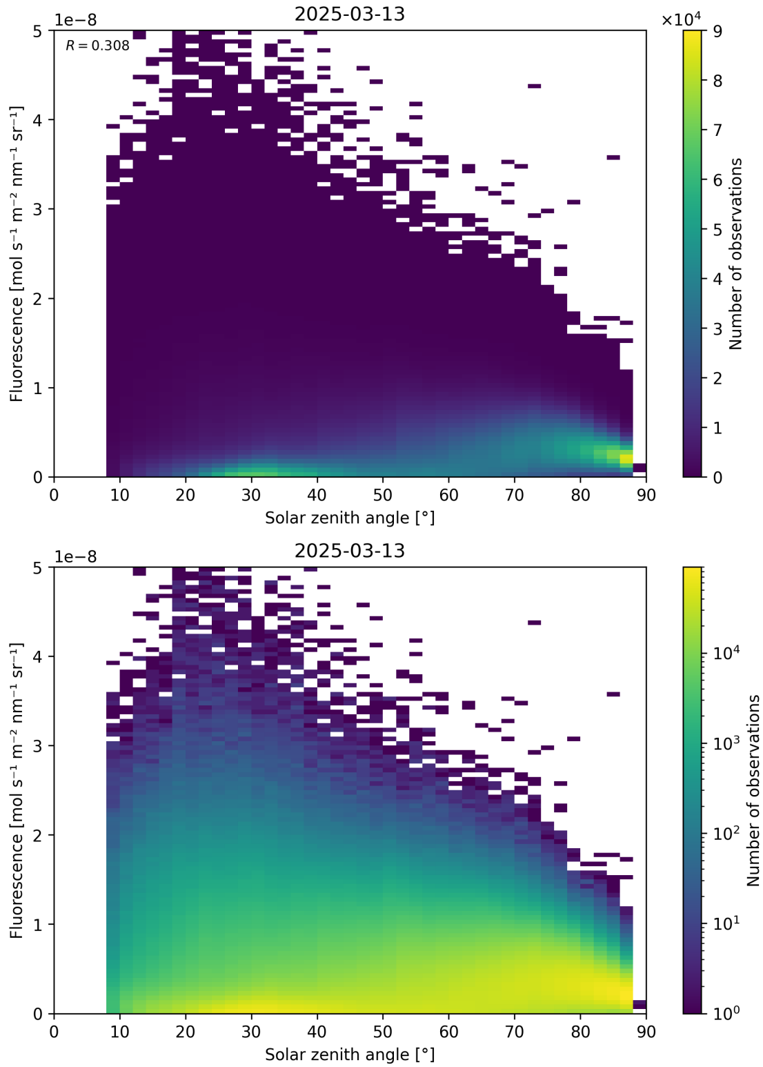
Figure 112: Scatter density plot of “Solar zenith angle” against “Fluorescence” for 2025-03-12 to 2025-03-14.
