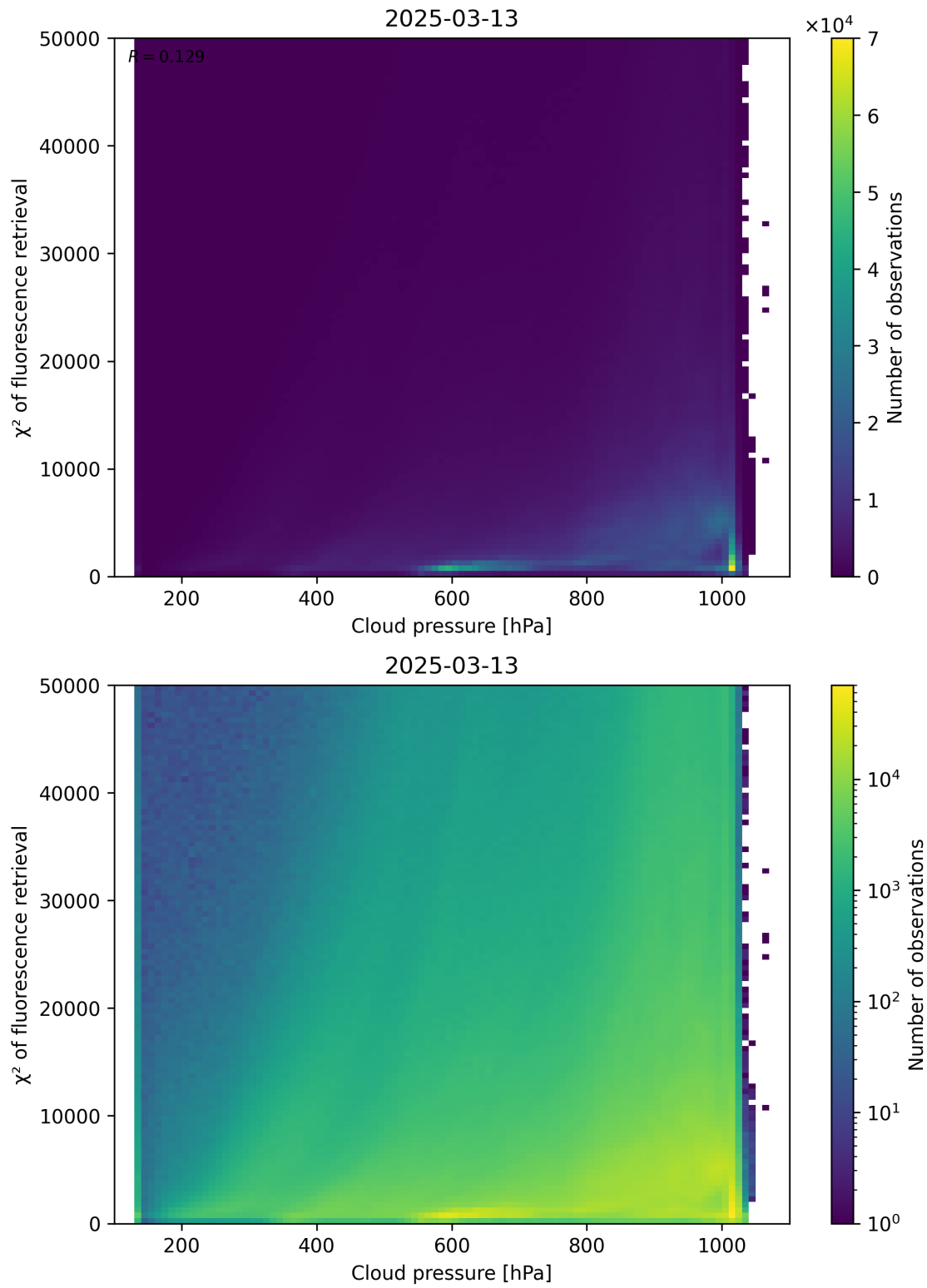
Figure 78: Scatter density plot of “Cloud pressure” against “ \chi^2 of fluorescence retrieval” for 2025-03-12 to 2025-03-14.
