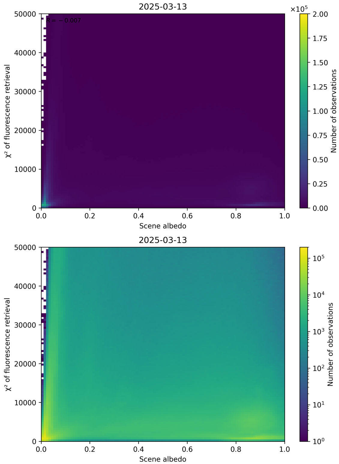
Figure 103: Scatter density plot of “Scene albedo” against “ \chi^2 of fluorescence retrieval” for 2025-03-12 to 2025-03-14.
