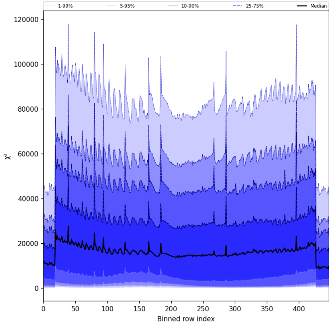
Figure 55: Along track statistics of “ \chi^2 ” for 2025-03-12 to 2025-03-14
