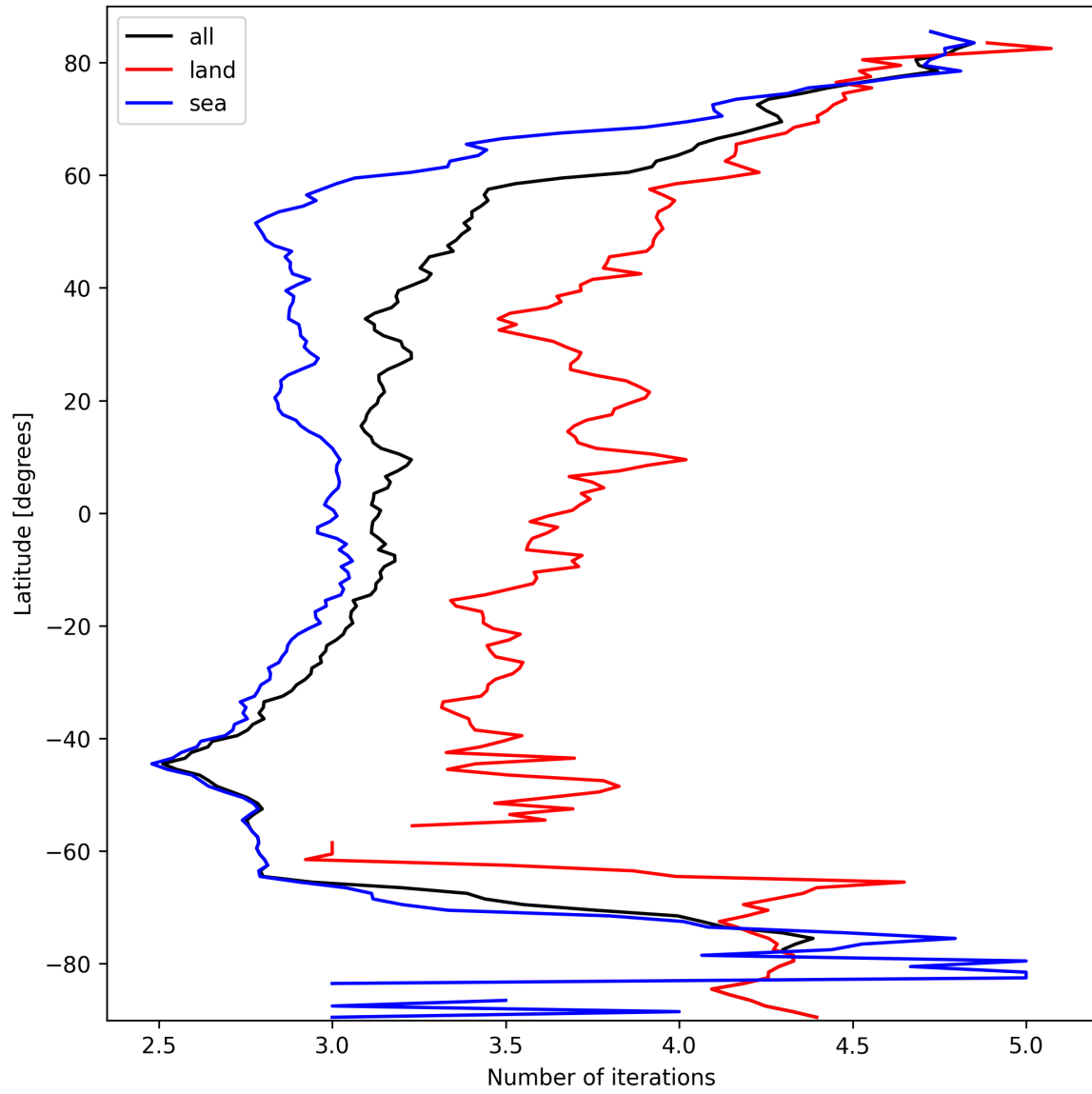
Figure 22: Zonal average of “Number of iterations” for 2025-03-13 to 2025-03-15.
