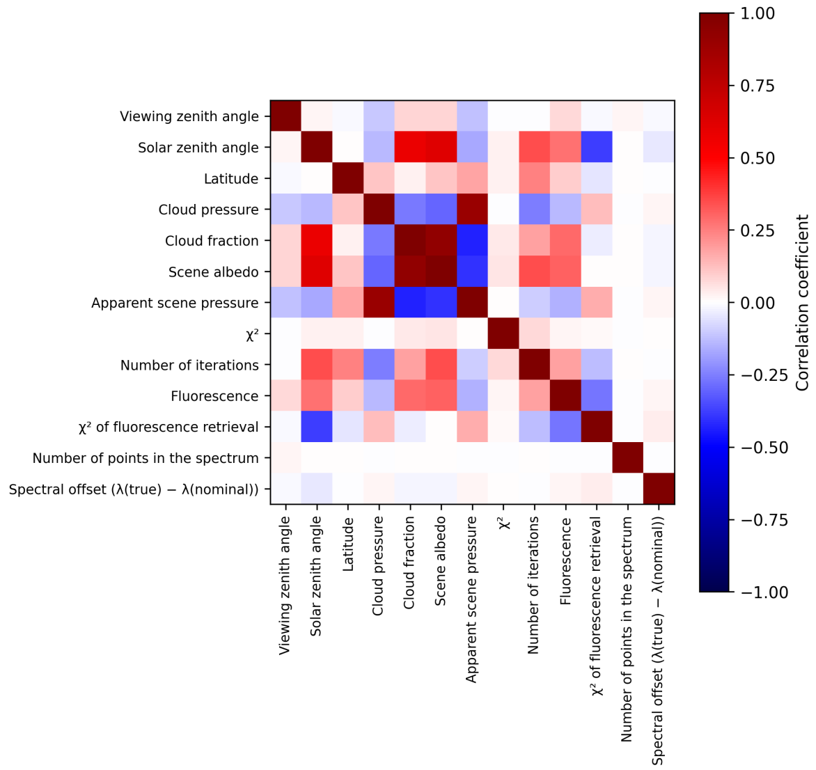
Figure 2: Map of correlation matrix for 2025-03-13 to 2025-03-15.
