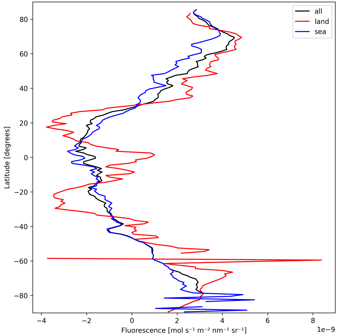
Figure 23: Zonal average of “Fluorescence” for 2025-03-13 to 2025-03-15.
