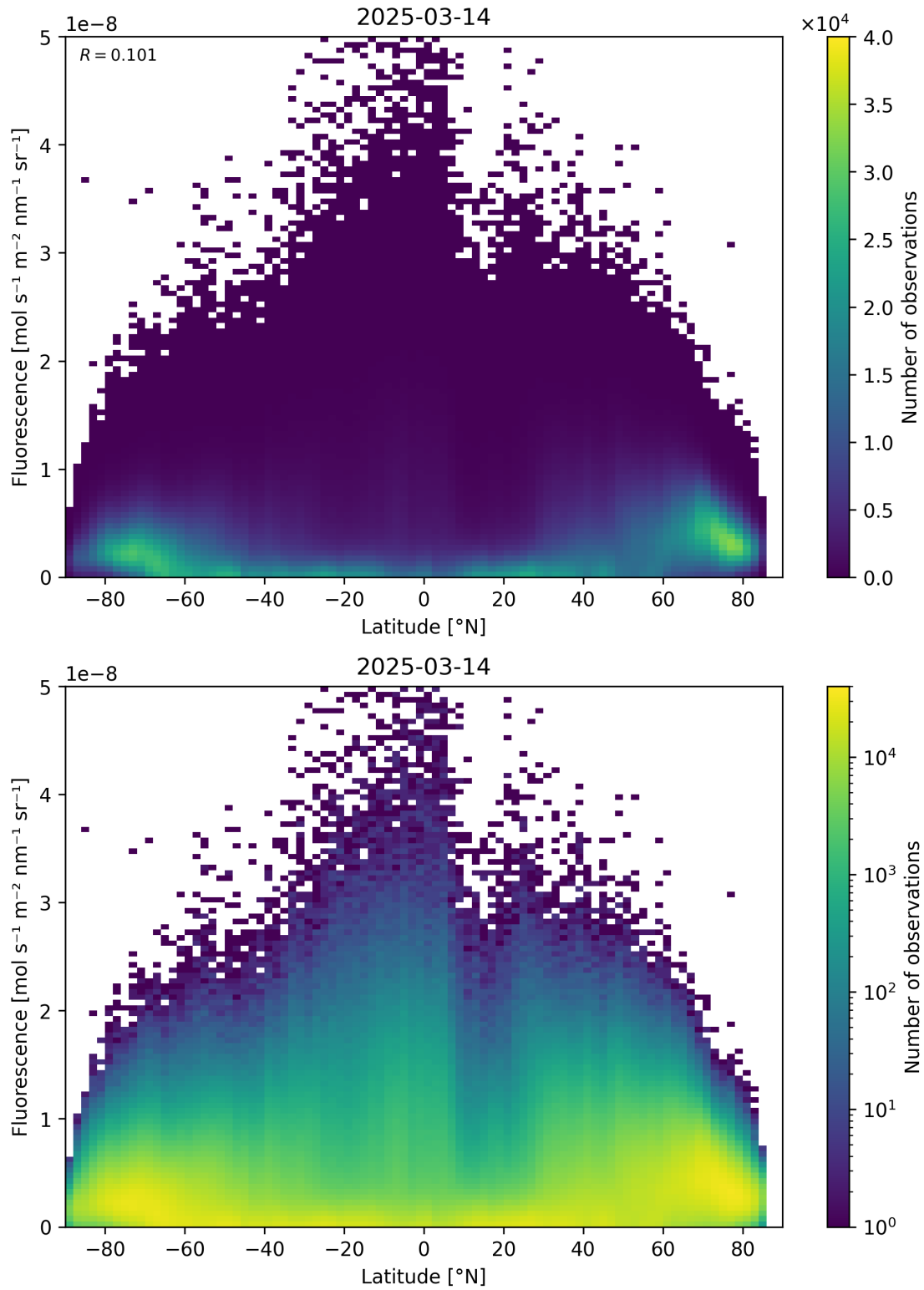
Figure 92: Scatter density plot of “Latitude” against “Fluorescence” for 2025-03-13 to 2025-03-15.
