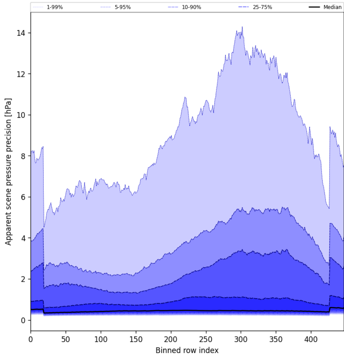
Figure 54: Along track statistics of “Apparent scene pressure precision” for 2025-03-13 to 2025-03-15
