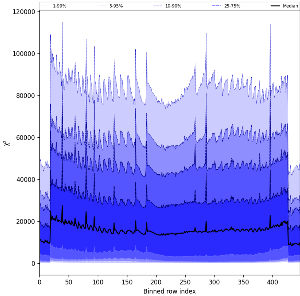
Figure 55: Along track statistics of “ \chi^2 ” for 2025-03-13 to 2025-03-15
