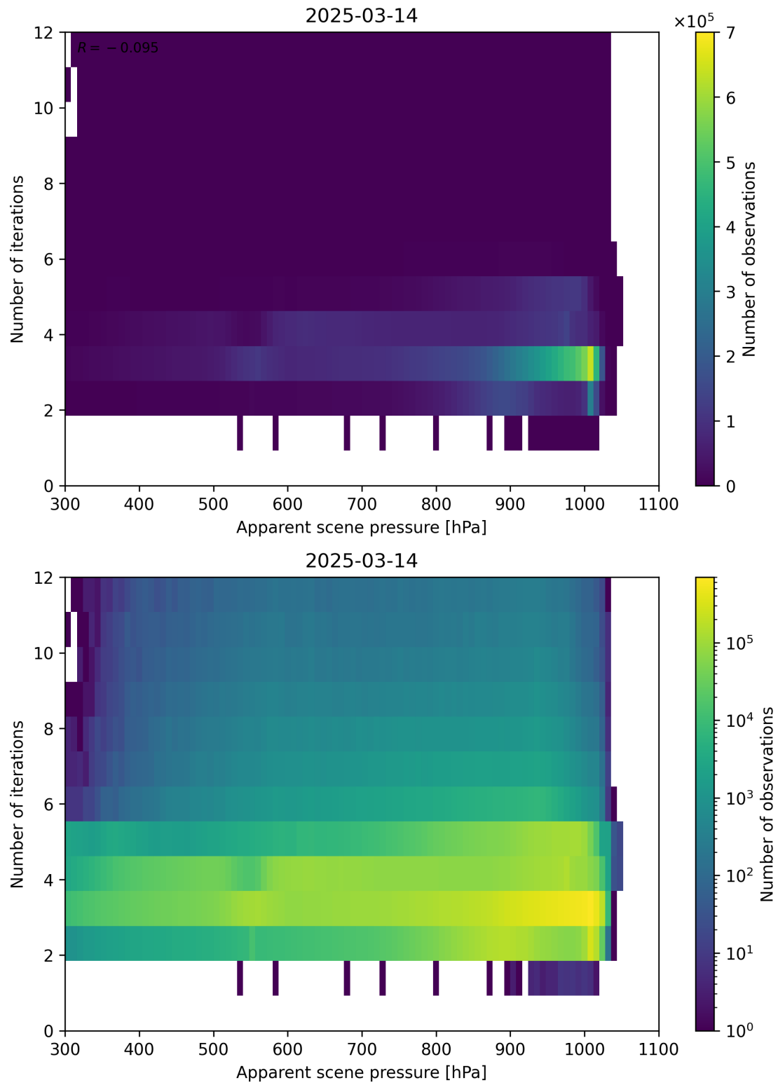
Figure 65: Scatter density plot of “Apparent scene pressure” against “Number of iterations” for 2025-03-13 to 2025-03-15.
