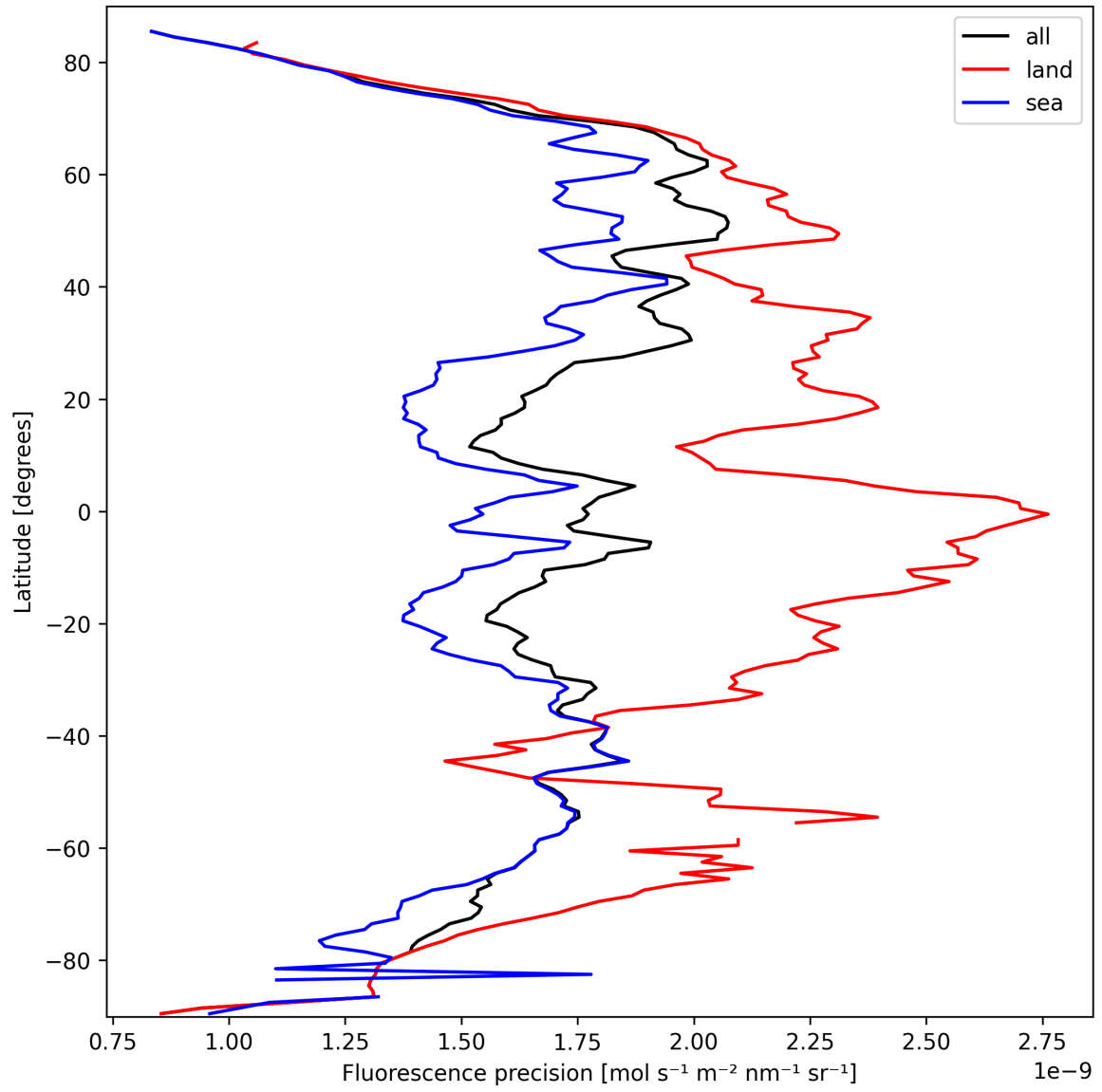
Figure 24: Zonal average of “Fluorescence precision” for 2025-03-13 to 2025-03-15.
