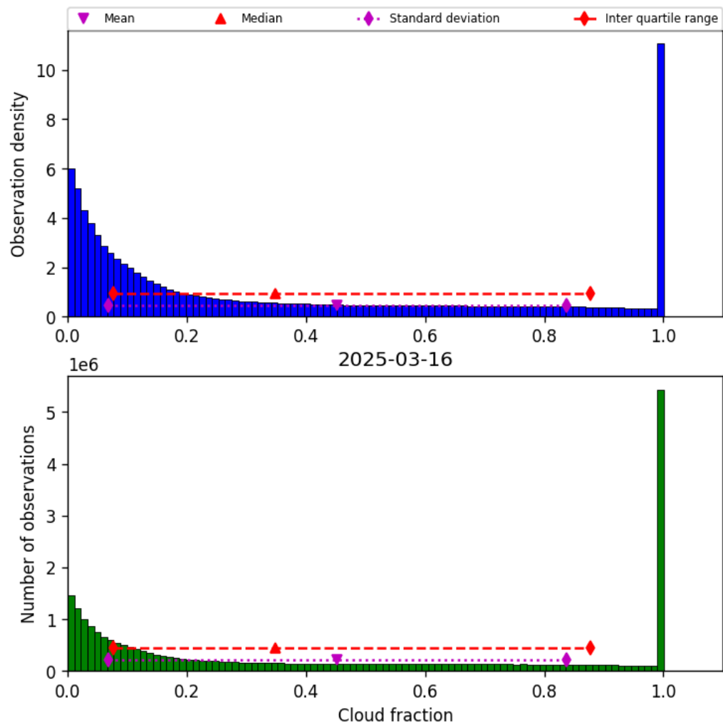
Figure 32: Histogram of “Cloud fraction” for 2025-03-15 to 2025-03-17
