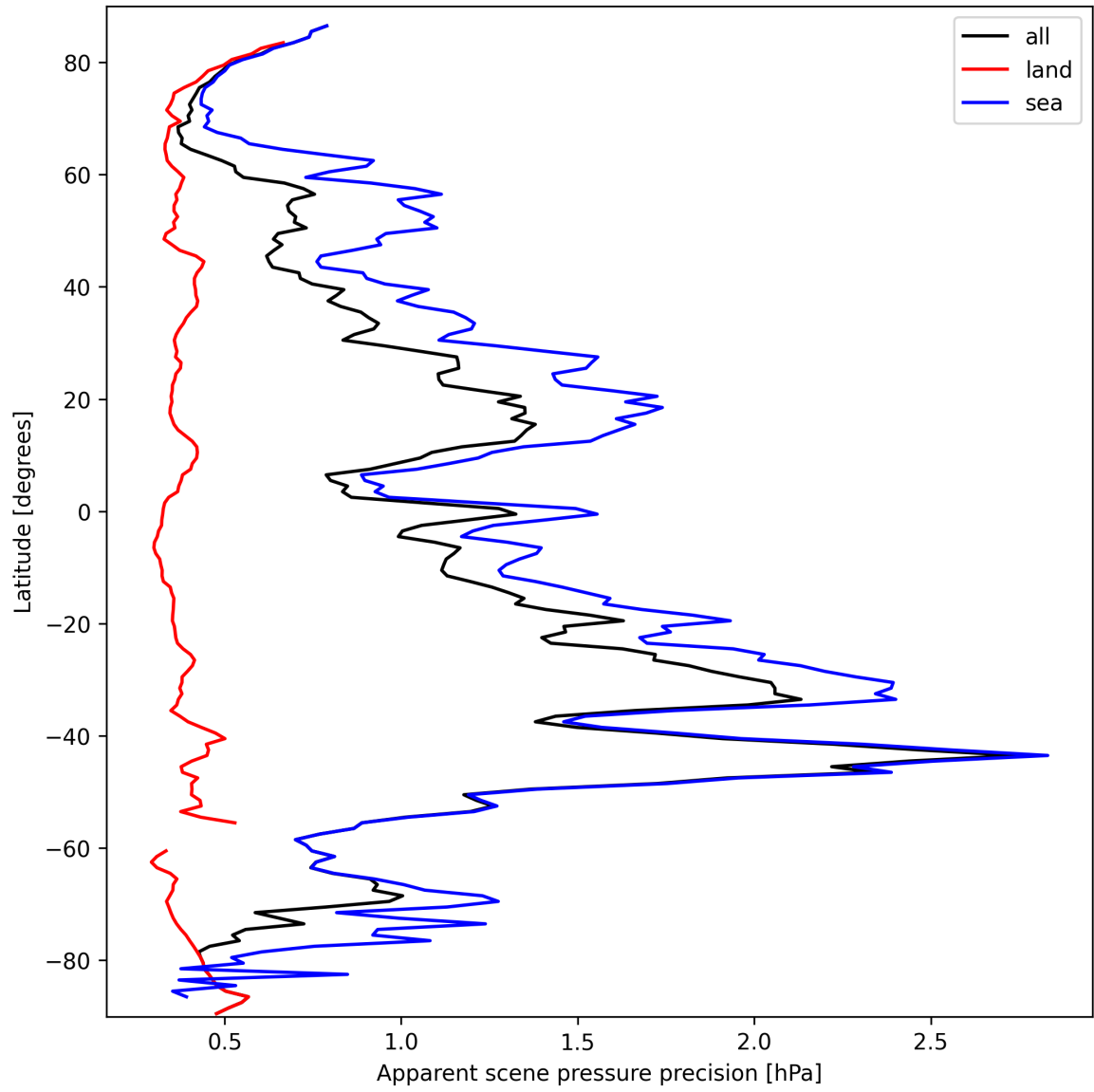
Figure 20: Zonal average of “Apparent scene pressure precision” for 2025-03-15 to 2025-03-17.
