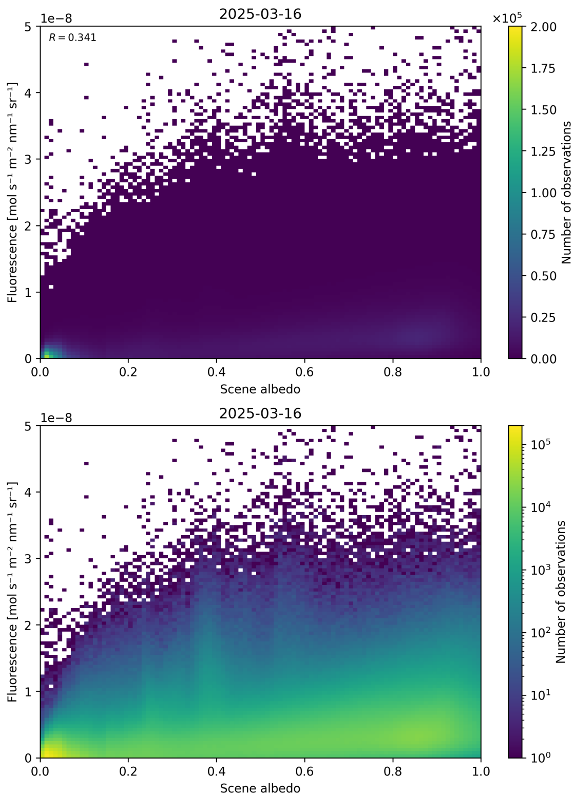
Figure 104: Scatter density plot of “Scene albedo” against “Fluorescence” for 2025-03-15 to 2025-03-17.
