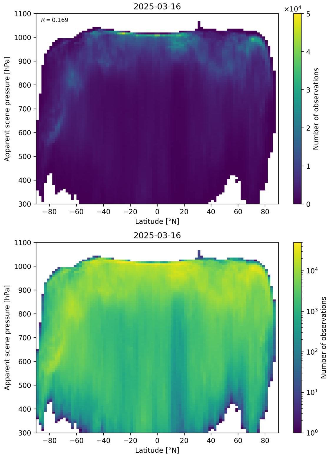
Figure 88: Scatter density plot of “Latitude” against “Apparent scene pressure” for 2025-03-15 to 2025-03-17.
