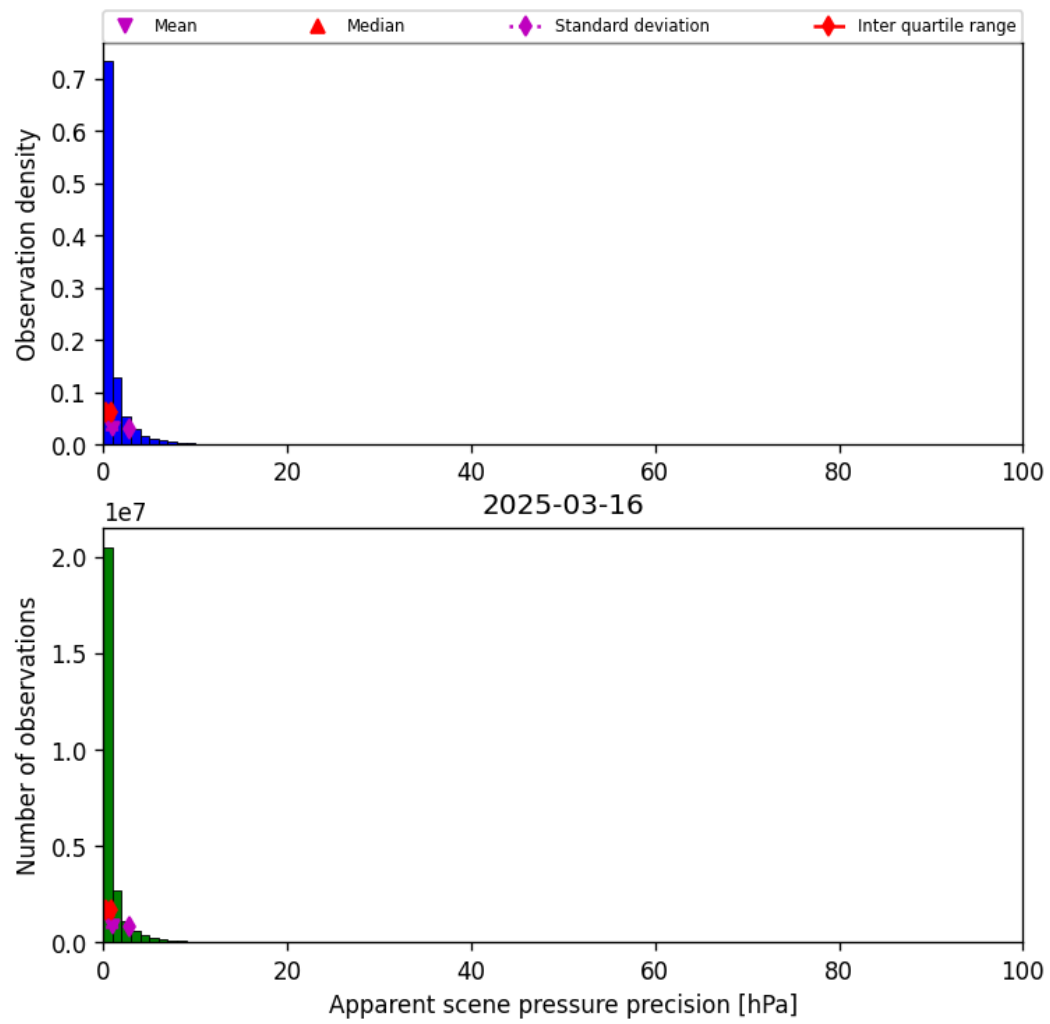
Figure 37: Histogram of “Apparent scene pressure precision” for 2025-03-15 to 2025-03-17
