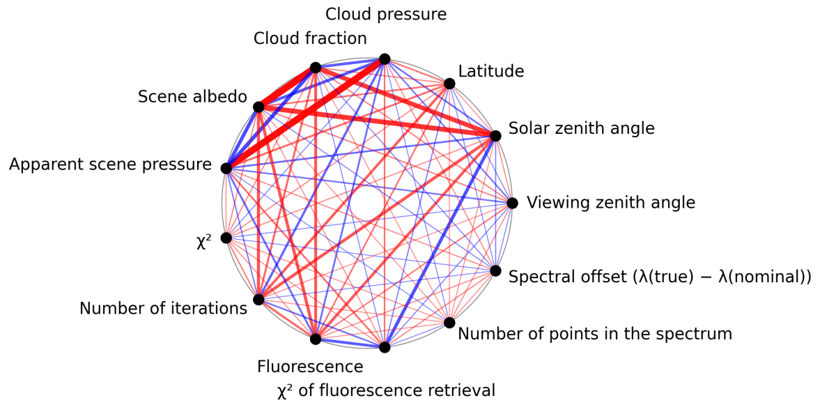
Figure 1: Map of correlation graph for 2025-03-15 to 2025-03-17.
