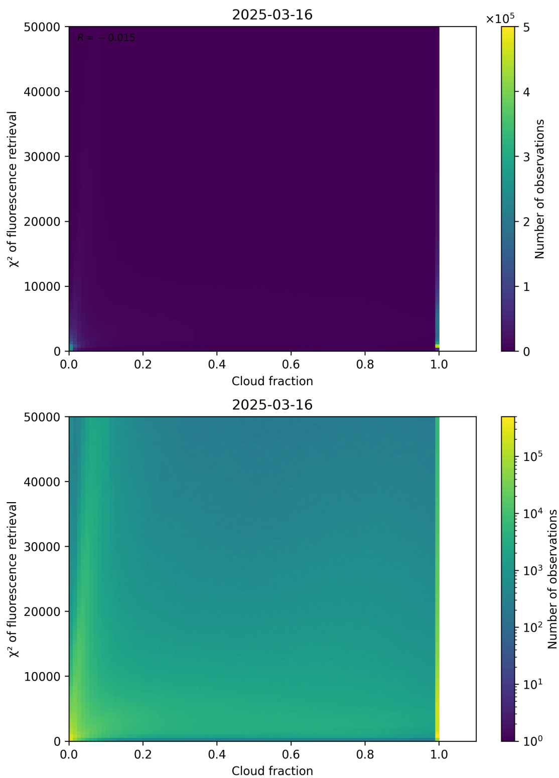
Figure 71: Scatter density plot of “Cloud fraction” against “ \chi^2 of fluorescence retrieval” for 2025-03-15 to 2025-03-17.
