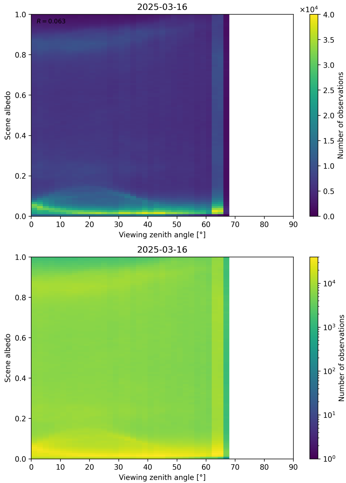
Figure 126: Scatter density plot of “Viewing zenith angle” against “Scene albedo” for 2025-03-15 to 2025-03-17.
