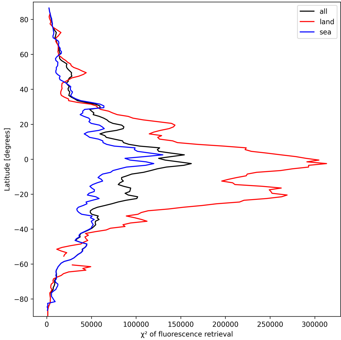
Figure 25: Zonal average of “ \chi^2 of fluorescence retrieval” for 2025-03-15 to 2025-03-17.
