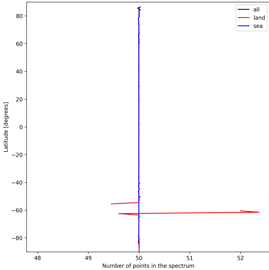
Figure 27: Zonal average of “Number of points in the spectrum” for 2025-03-15 to 2025-03-17.
