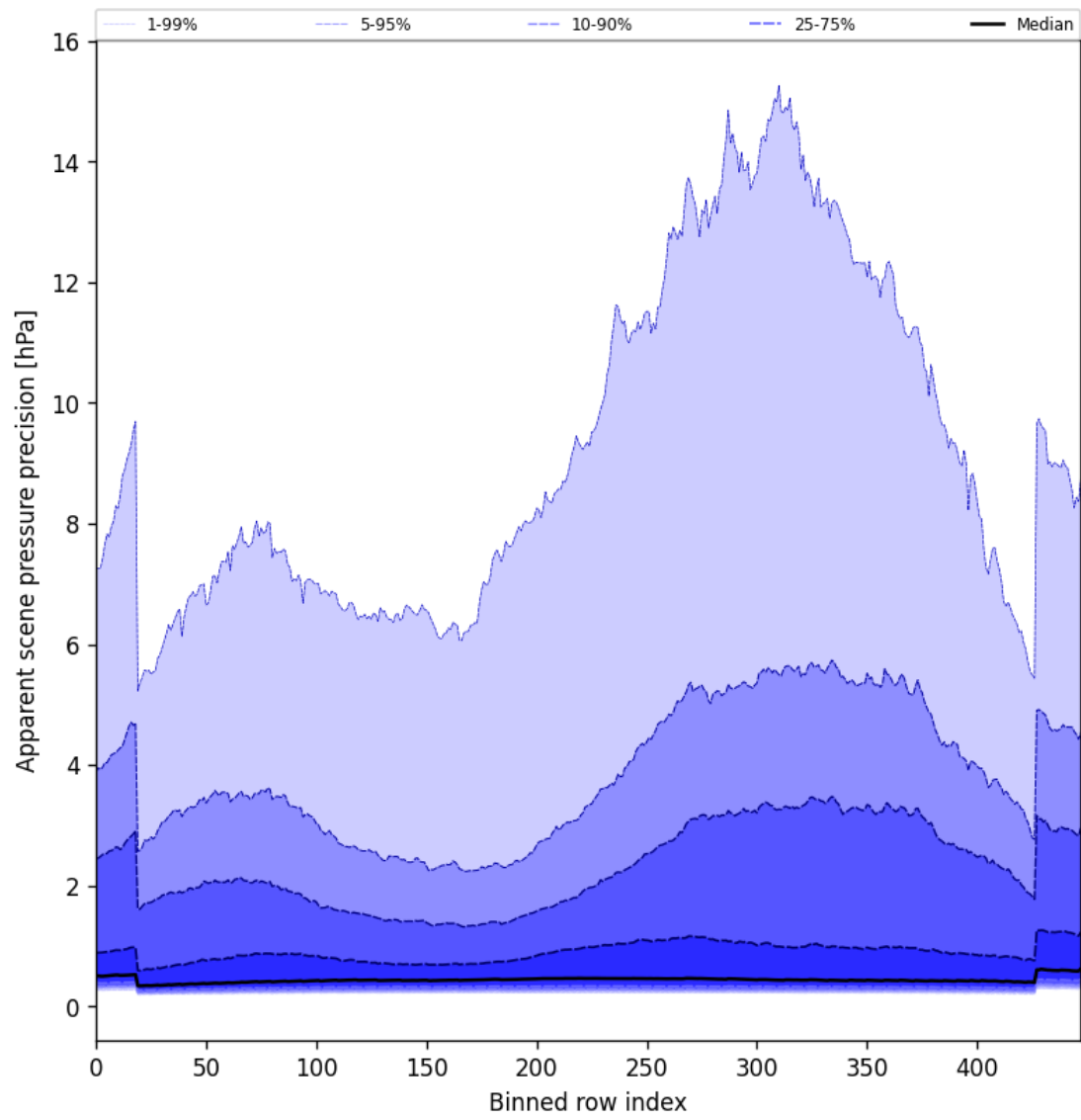
Figure 54: Along track statistics of “Apparent scene pressure precision” for 2025-03-15 to 2025-03-17
