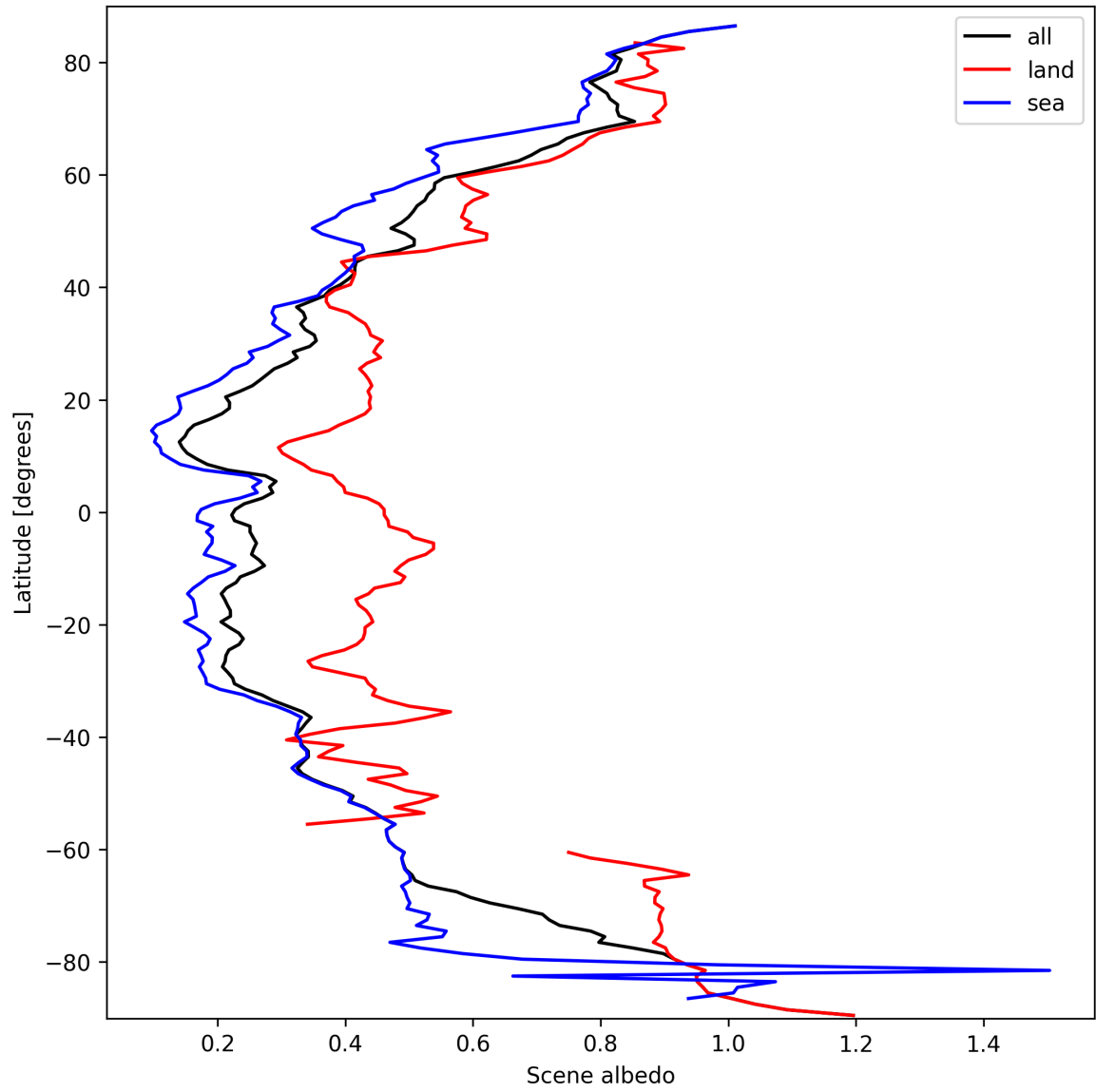
Figure 17: Zonal average of “Scene albedo” for 2025-03-15 to 2025-03-17.
