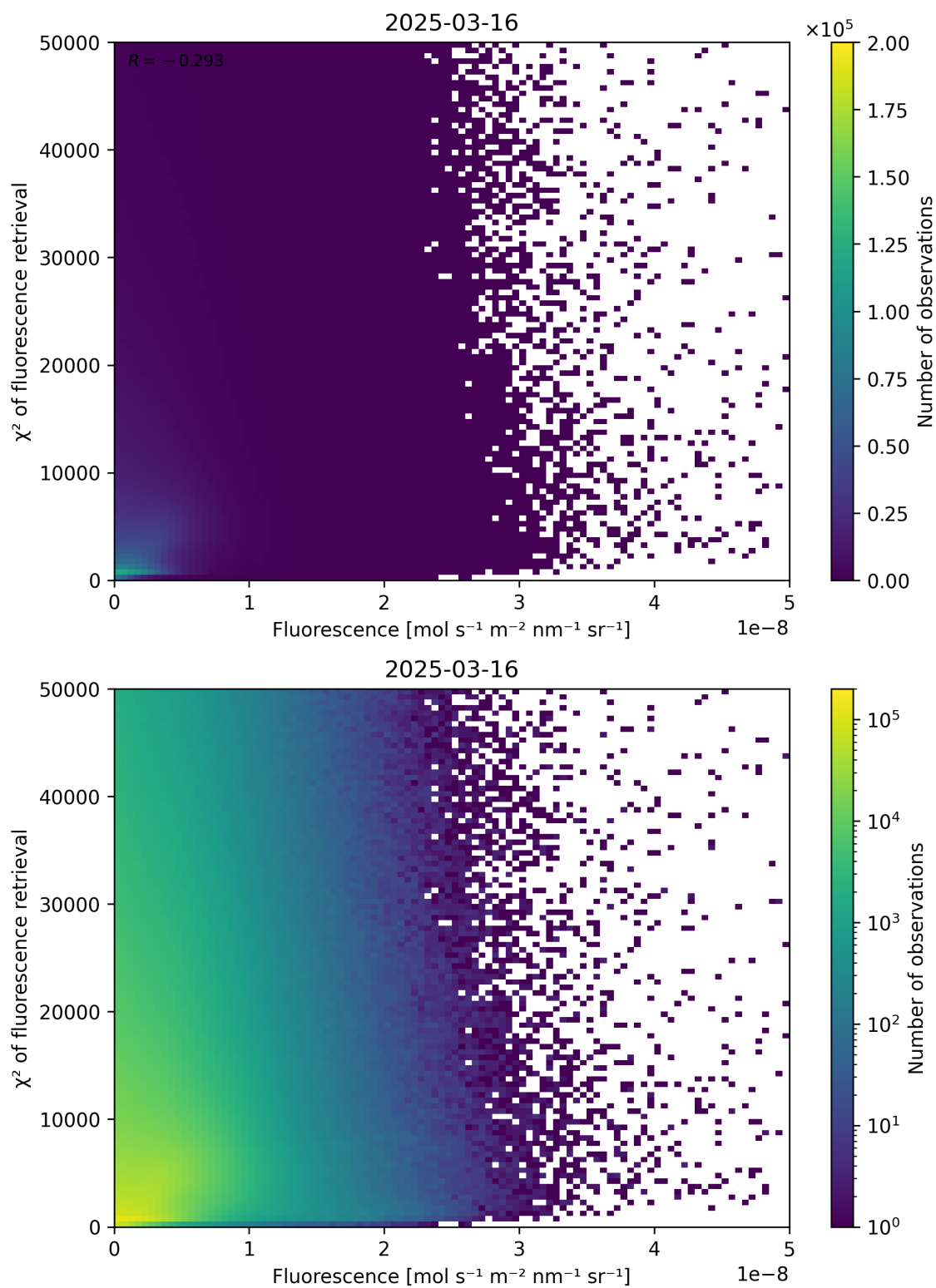
Figure 85: Scatter density plot of “Fluorescence” against “ \chi^2 of fluorescence retrieval” for 2025-03-15 to 2025-03-17.
