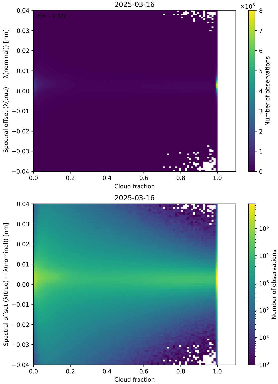
Figure 76: Scatter density plot of “Cloud fraction” against “Spectral offset ( \lambda_{\text{true}} - \lambda_{\text{nominal}} )” for 2025-03-15 to 2025-03-17.
