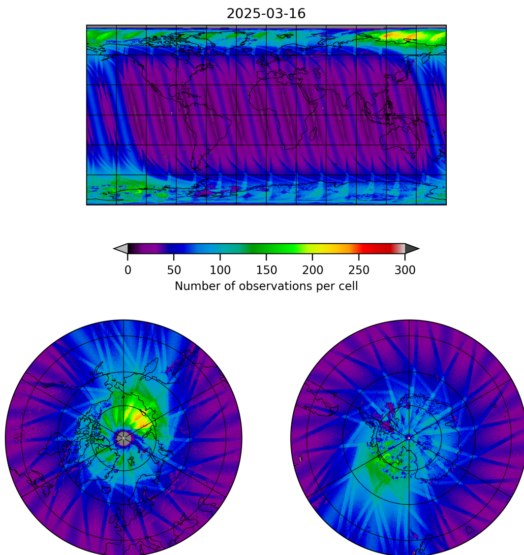
Figure 11: Map of the number of observations for 2025-03-15 to 2025-03-17
