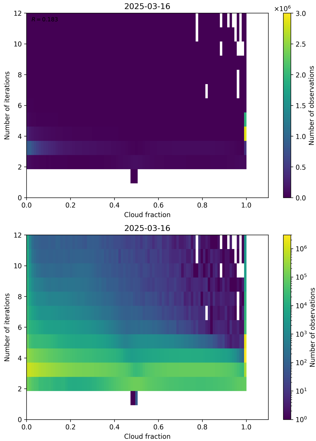
Figure 73: Scatter density plot of “Cloud fraction” against “Number of iterations” for 2025-03-15 to 2025-03-17.
