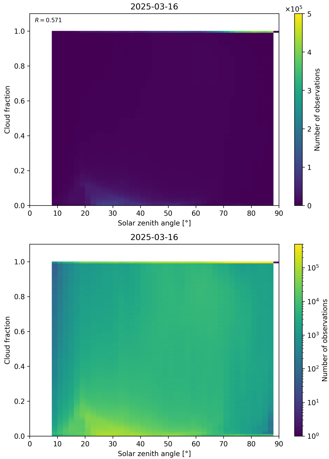
Figure 110: Scatter density plot of “Solar zenith angle” against “Cloud fraction” for 2025-03-15 to 2025-03-17.
