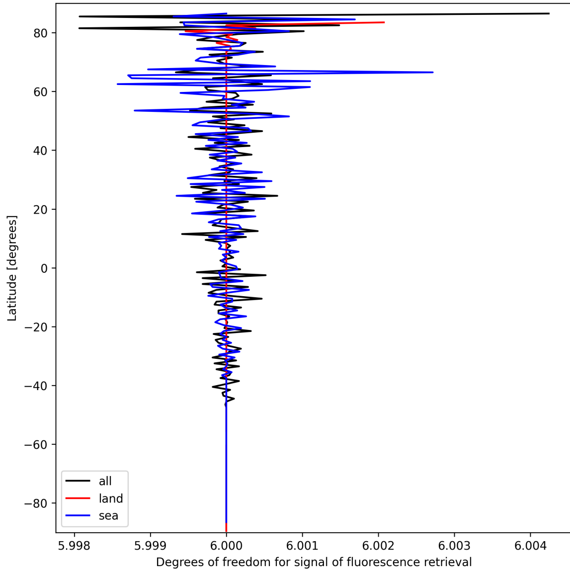
Figure 26: Zonal average of “Degrees of freedom for signal of fluorescence retrieval” for 2025-03-15 to 2025-03-17.
