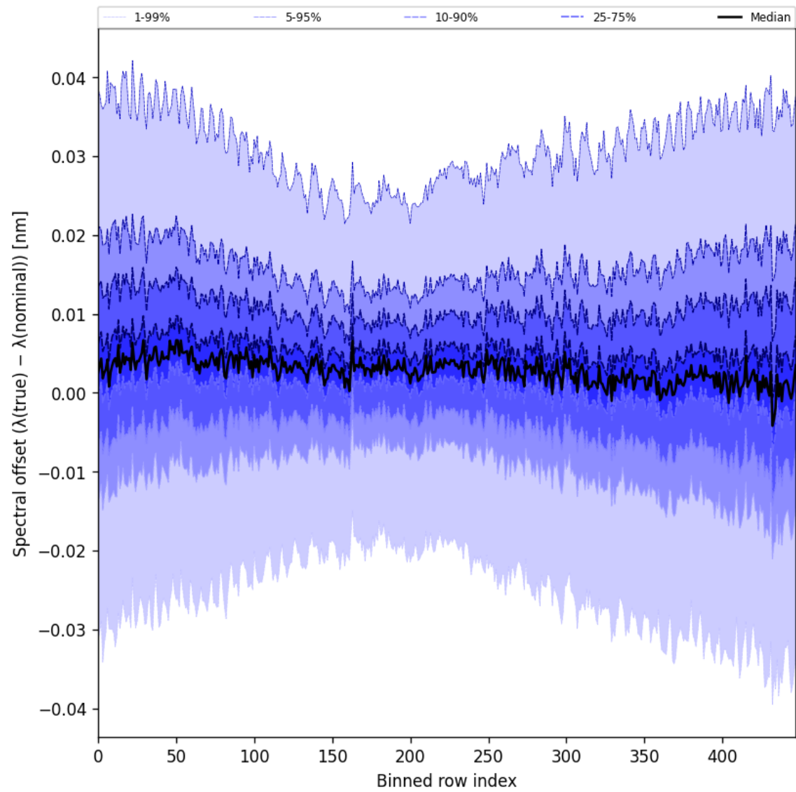
Figure 62: Along track statistics of “Spectral offset ( \lambda_{\text{true}} - \lambda_{\text{nominal}} )” for 2025-03-15 to 2025-03-17
