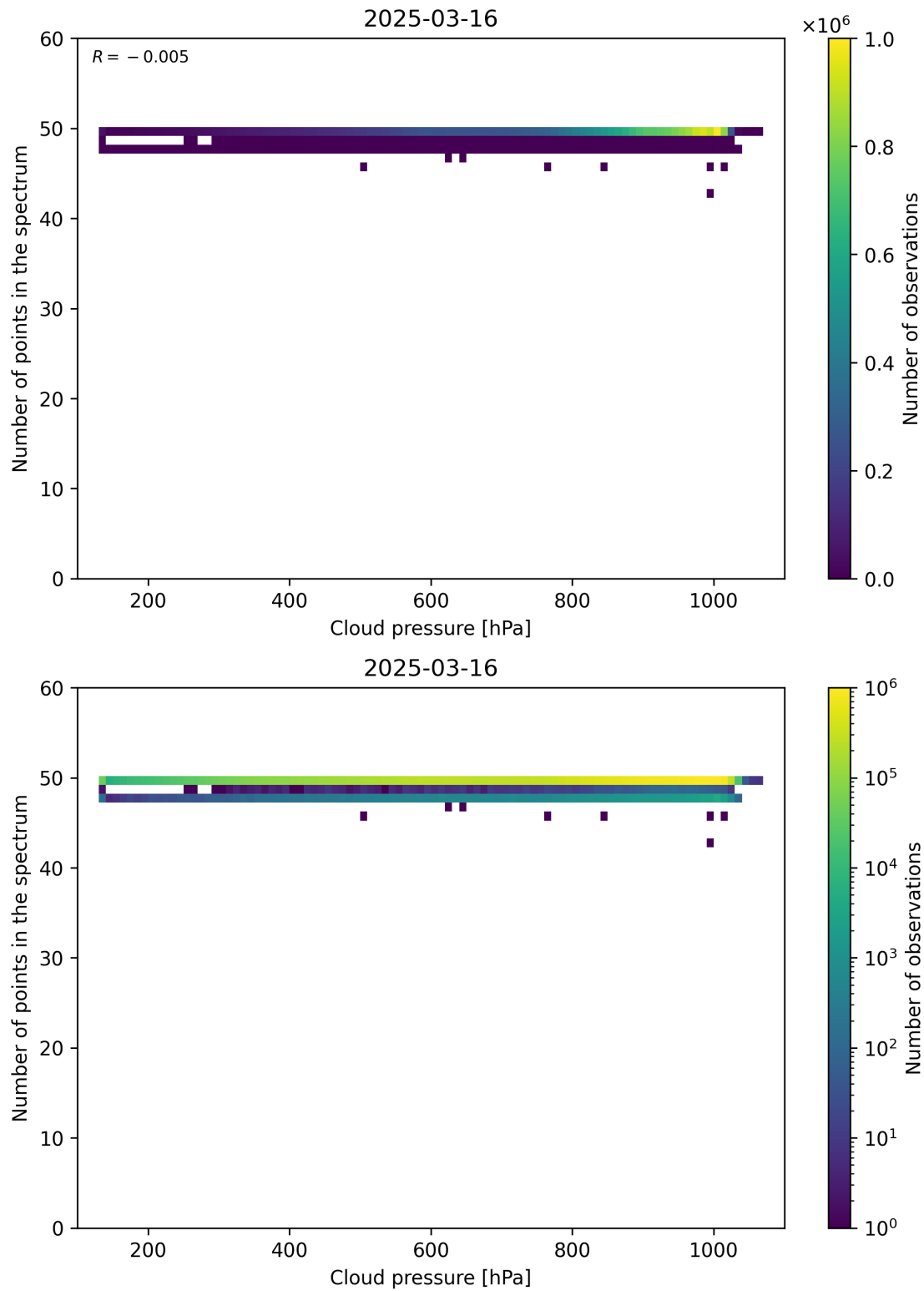
Figure 82: Scatter density plot of “Cloud pressure” against “Number of points in the spectrum” for 2025-03-15 to 2025-03-17.
