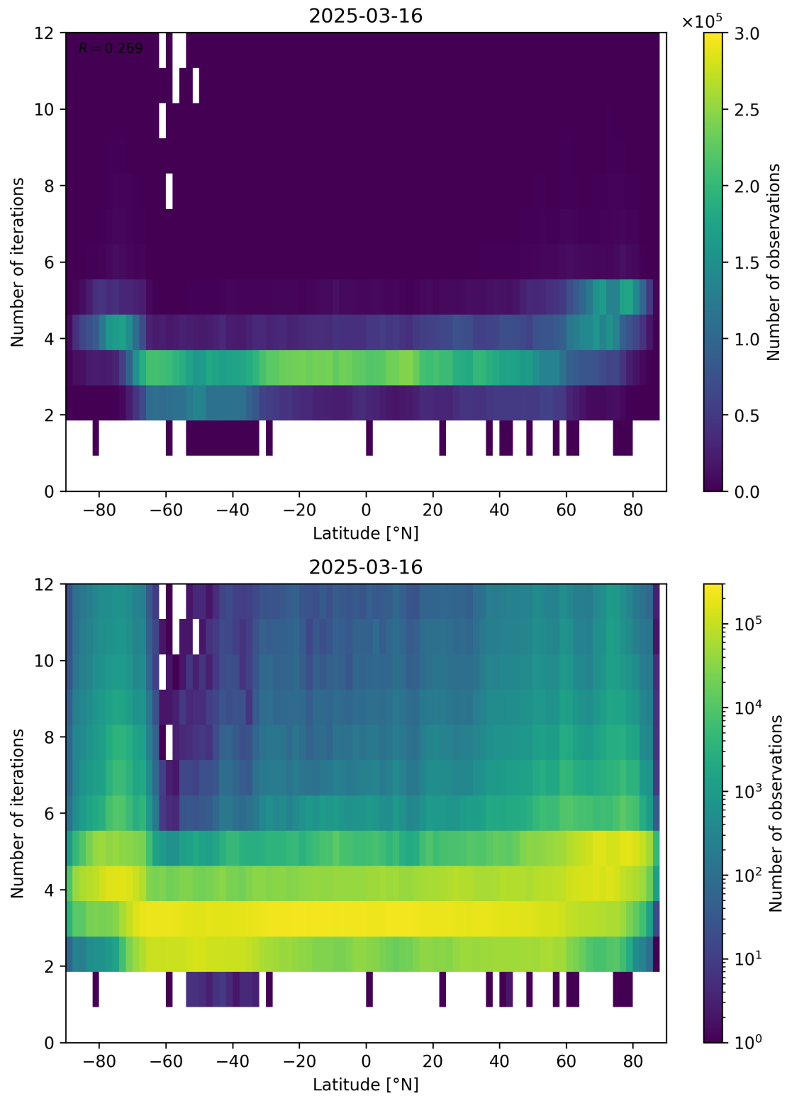
Figure 93: Scatter density plot of “Latitude” against “Number of iterations” for 2025-03-15 to 2025-03-17.
