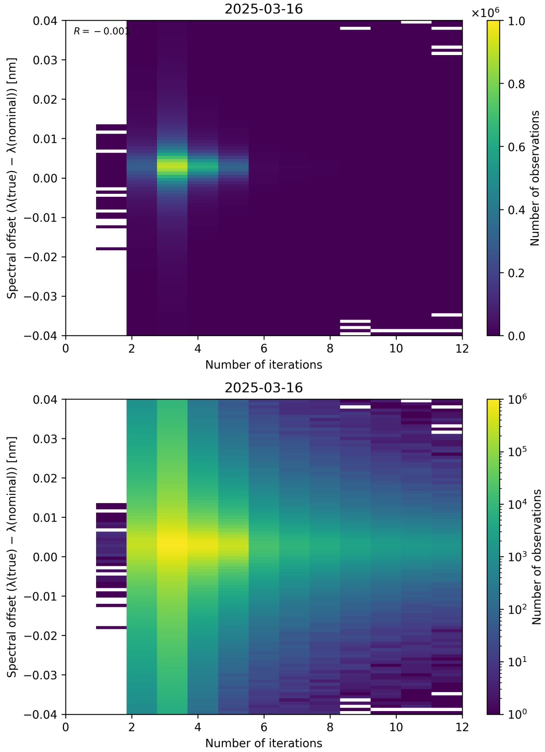
Figure 100: Scatter density plot of “Number of iterations” against “Spectral offset ( \lambda_{\text{true}} - \lambda_{\text{nominal}} )” for 2025-03-15 to 2025-03-17.
