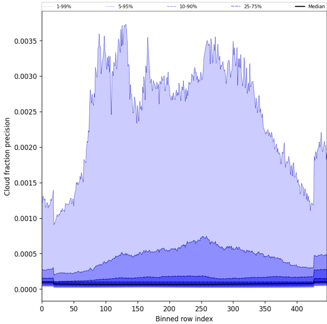
Figure 50: Along track statistics of “Cloud fraction precision” for 2025-03-15 to 2025-03-17
