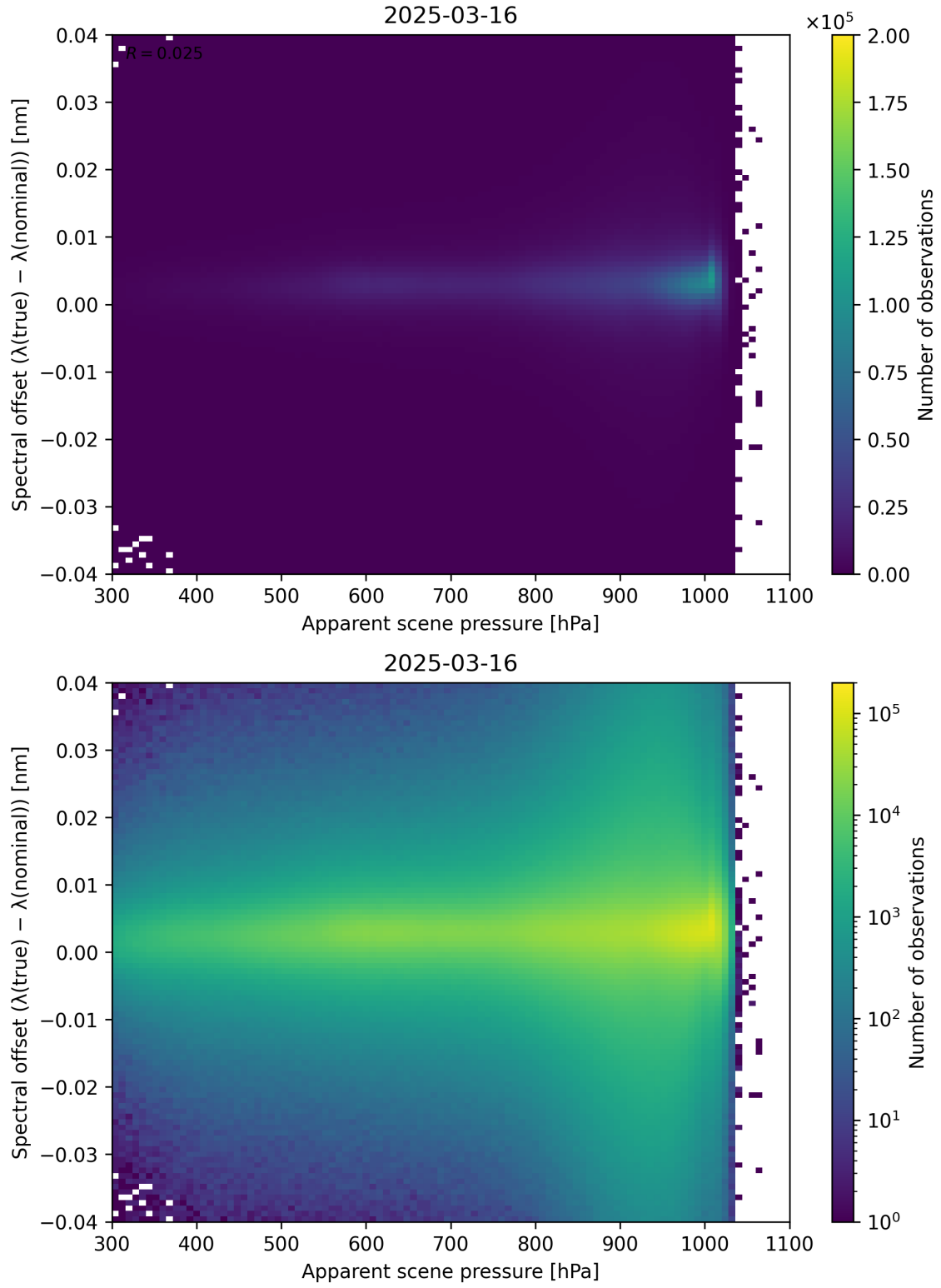
Figure 67: Scatter density plot of “Apparent scene pressure” against “Spectral offset ( \lambda_{\text{true}} - \lambda_{\text{nominal}} )” for 2025-03-15 to 2025-03-17.
