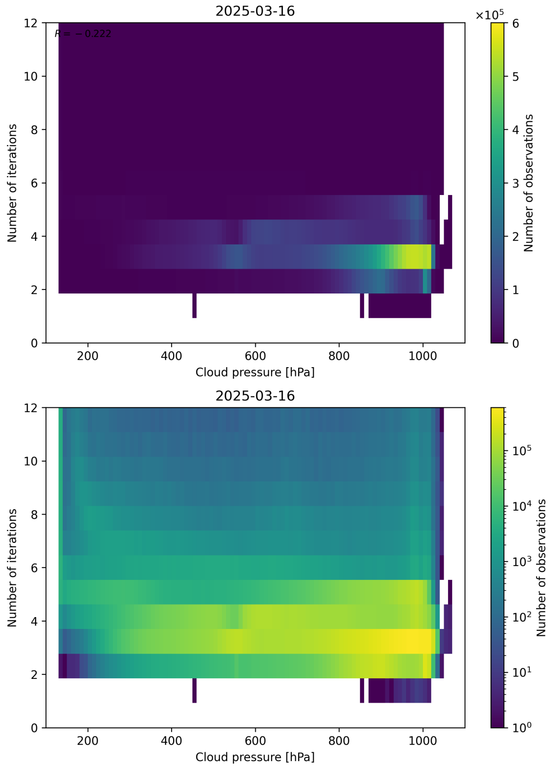
Figure 81: Scatter density plot of “Cloud pressure” against “Number of iterations” for 2025-03-15 to 2025-03-17.
